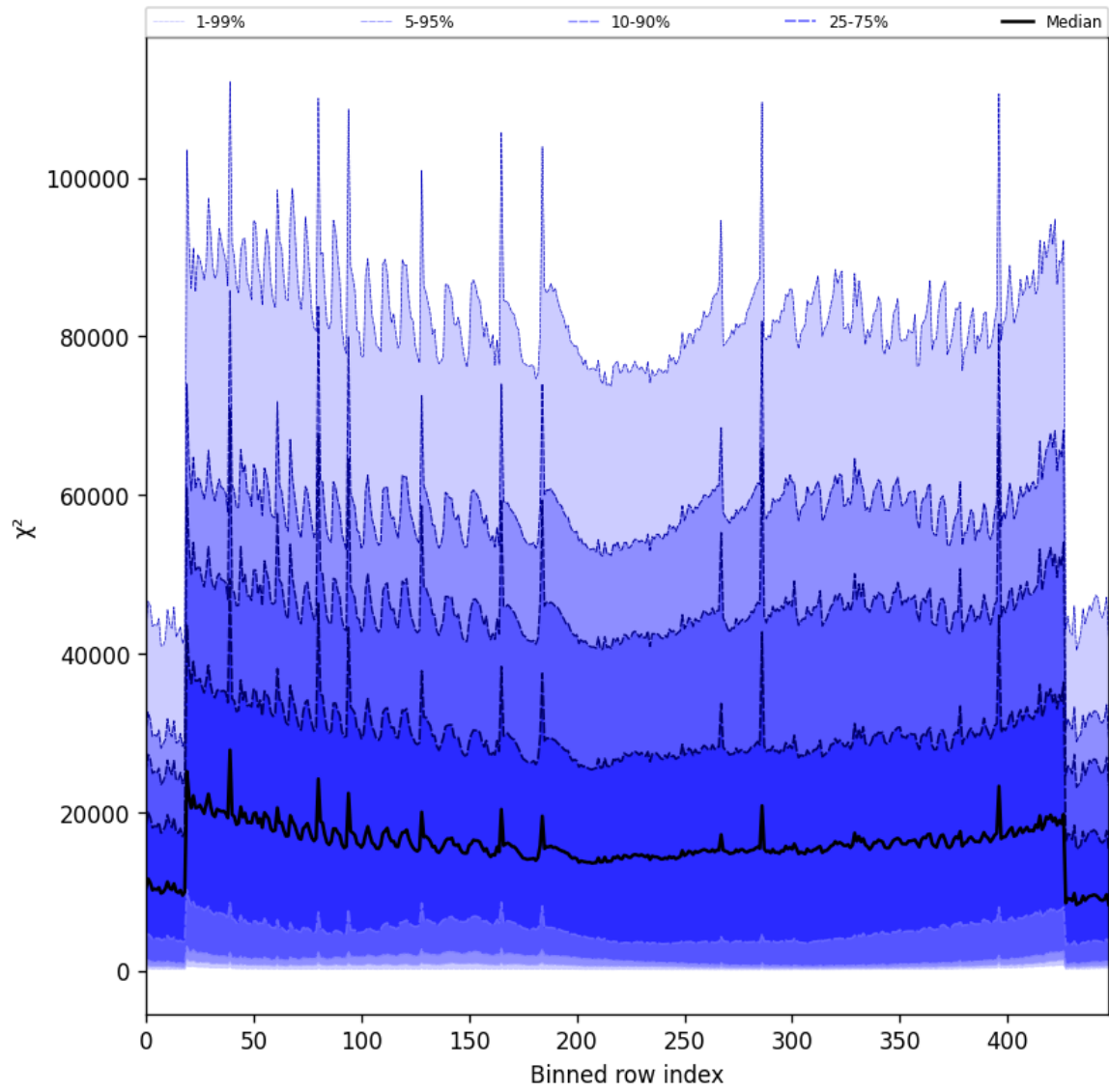
Figure 55: Along track statistics of “ \chi^2 ” for 2025-03-17 to 2025-03-18
