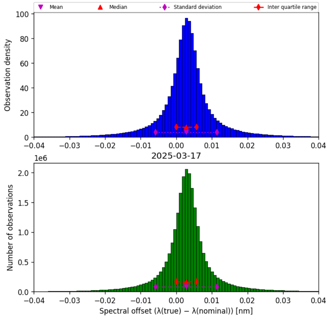
Figure 45: Histogram of “Spectral offset ( \lambda_{\text{true}} - \lambda_{\text{nominal}} )” for 2025-03-17 to 2025-03-18
