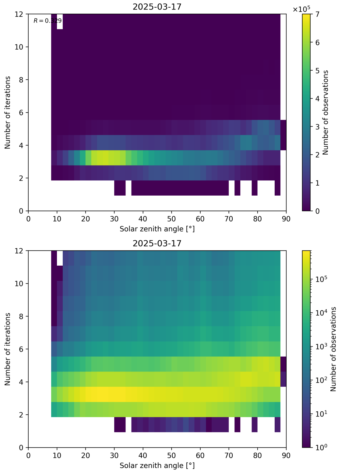
Figure 114: Scatter density plot of “Solar zenith angle” against “Number of iterations” for 2025-03-17 to 2025-03-18.
