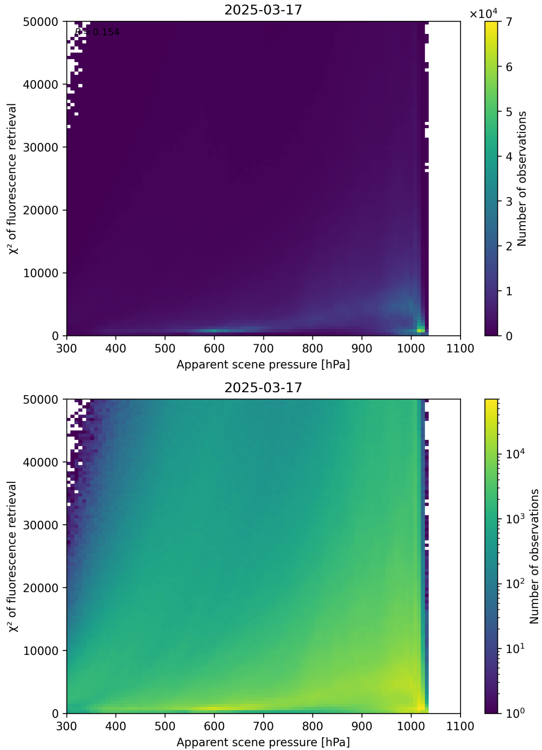
Figure 63: Scatter density plot of “Apparent scene pressure” against “ \chi^2 of fluorescence retrieval” for 2025-03-17 to 2025-03-18.
