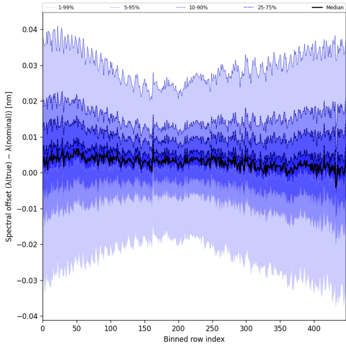
Figure 62: Along track statistics of “Spectral offset ( \lambda_{\text{true}} - \lambda_{\text{nominal}} )” for 2025-03-17 to 2025-03-18
