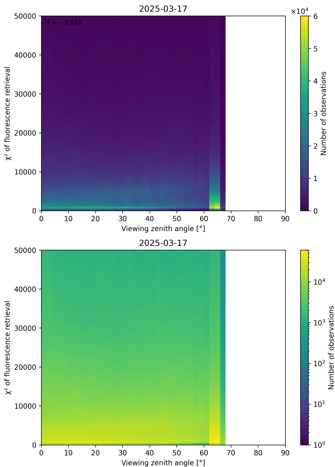
Figure 119: Scatter density plot of “Viewing zenith angle” against “ \chi^2 of fluorescence retrieval” for 2025-03-17 to 2025-03-18.
