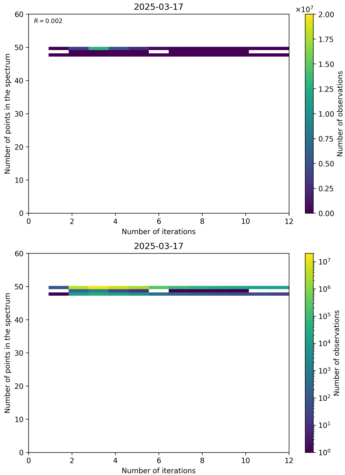
Figure 99: Scatter density plot of “Number of iterations” against “Number of points in the spectrum” for 2025-03-17 to 2025-03-18.
