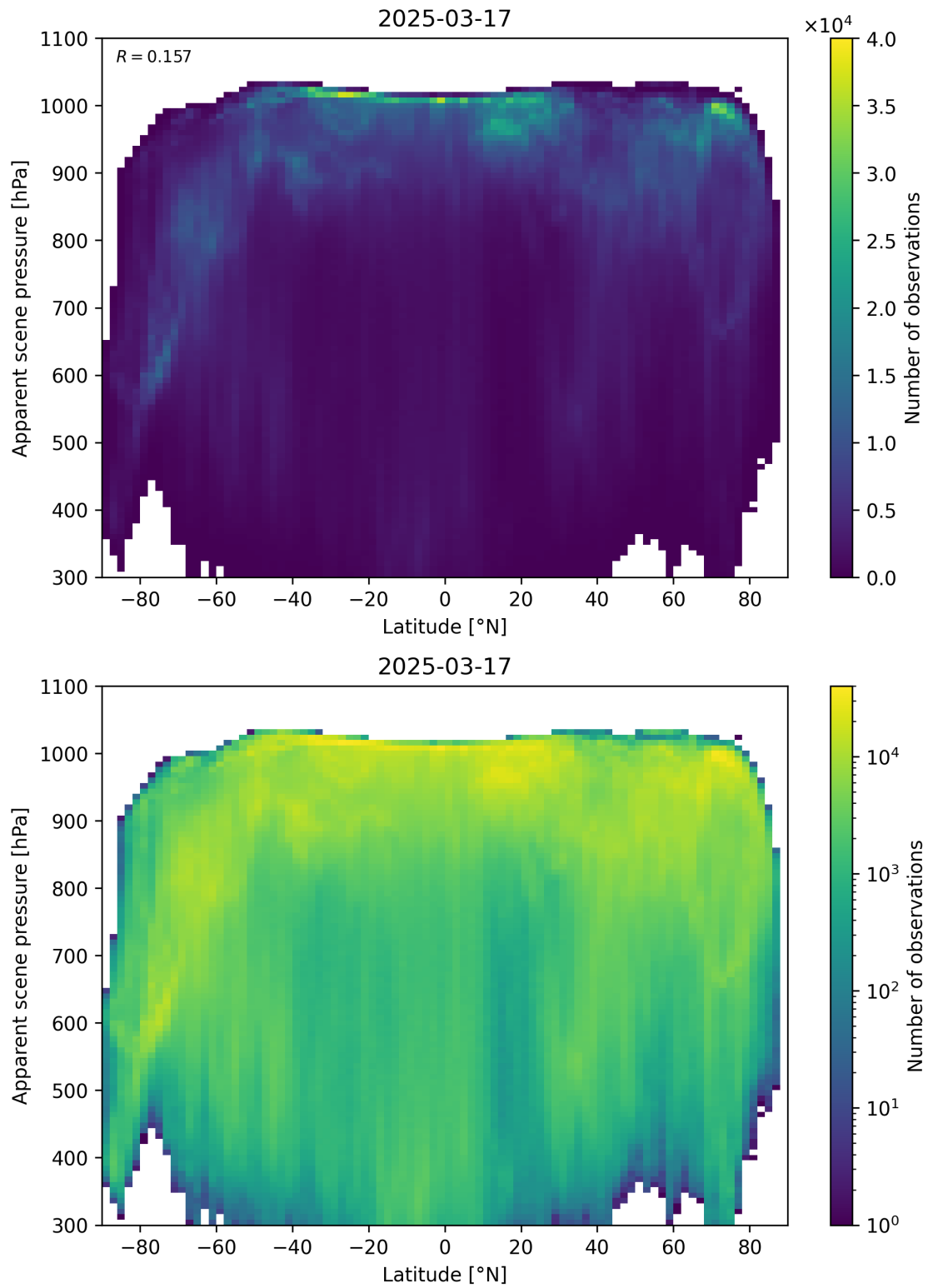
Figure 88: Scatter density plot of “Latitude” against “Apparent scene pressure” for 2025-03-17 to 2025-03-18.
