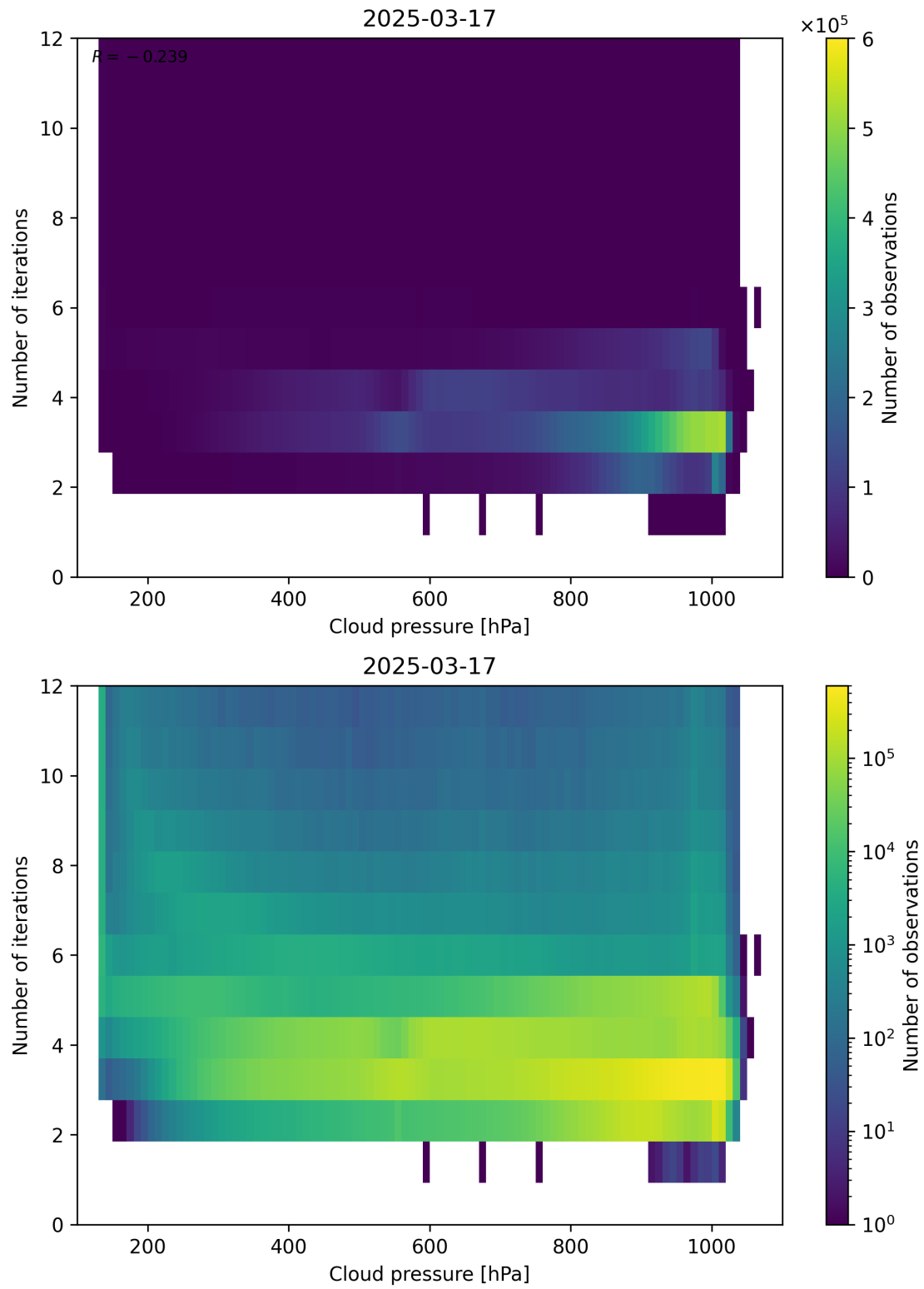
Figure 81: Scatter density plot of “Cloud pressure” against “Number of iterations” for 2025-03-17 to 2025-03-18.
