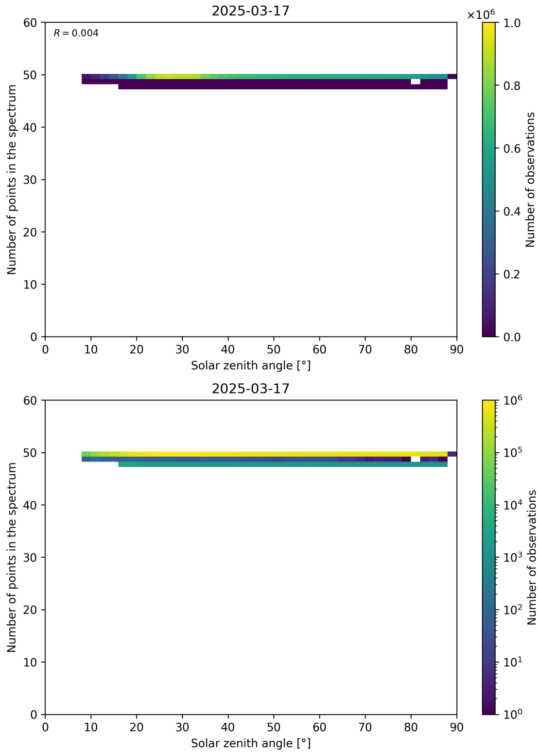
Figure 115: Scatter density plot of “Solar zenith angle” against “Number of points in the spectrum” for 2025-03-17 to 2025-03-18.
