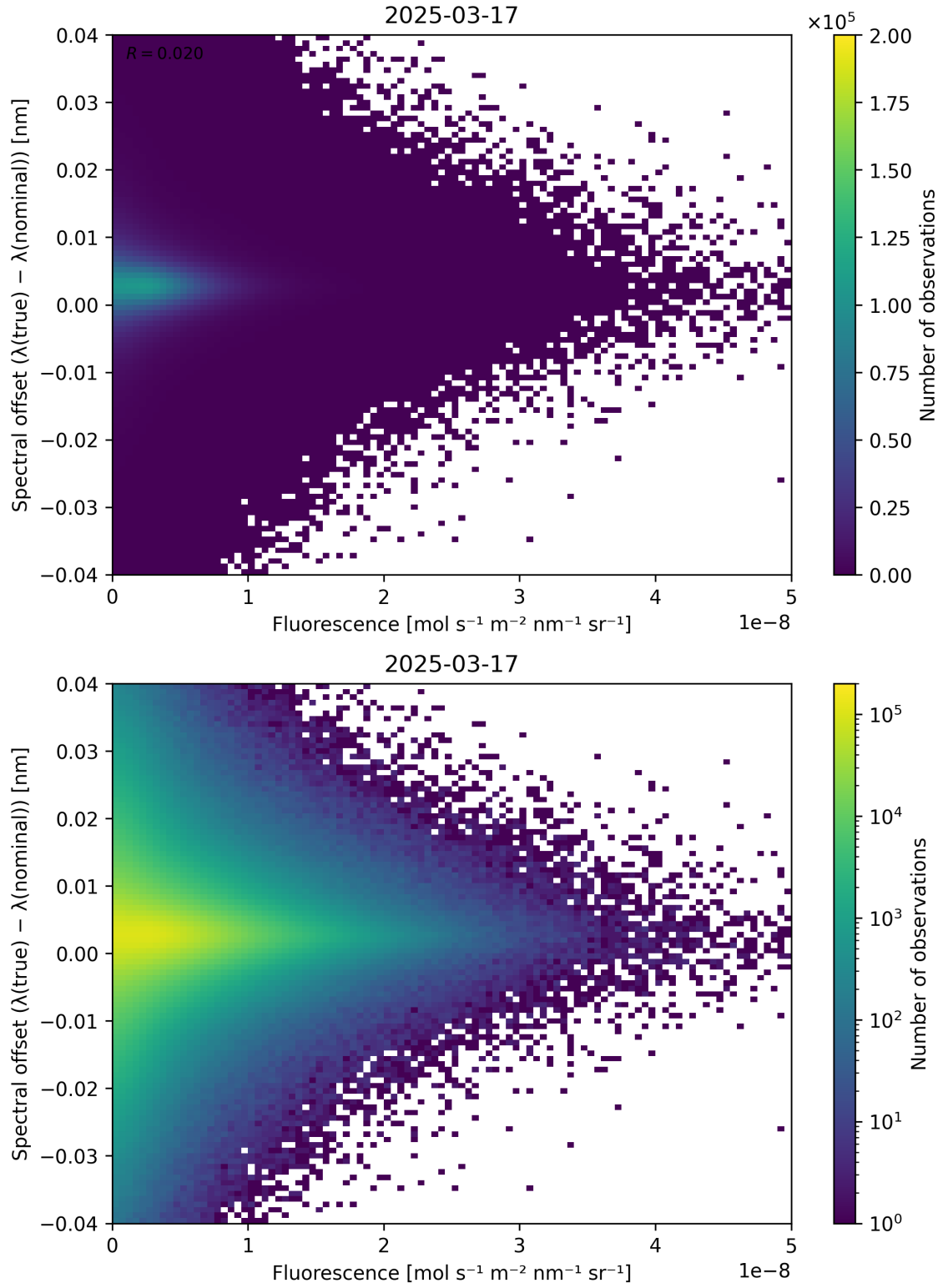
Figure 87: Scatter density plot of “Fluorescence” against “Spectral offset ( \lambda_{\text{true}} - \lambda_{\text{nominal}} )” for 2025-03-17 to 2025-03-18.
