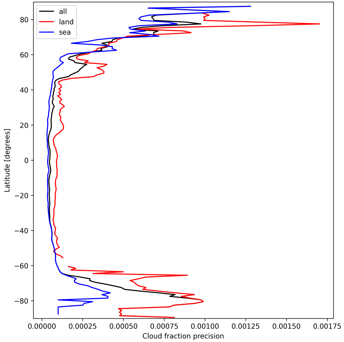
Figure 16: Zonal average of “Cloud fraction precision” for 2025-03-17 to 2025-03-18.
