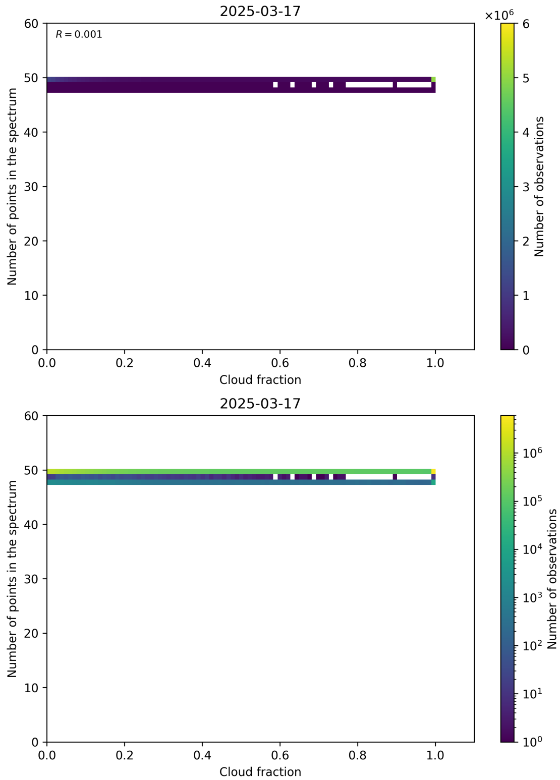
Figure 74: Scatter density plot of “Cloud fraction” against “Number of points in the spectrum” for 2025-03-17 to 2025-03-18.
