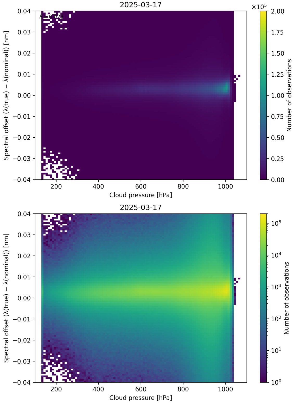
Figure 84: Scatter density plot of “Cloud pressure” against “Spectral offset ( \lambda_{\text{true}} - \lambda_{\text{nominal}} )” for 2025-03-17 to 2025-03-18.
