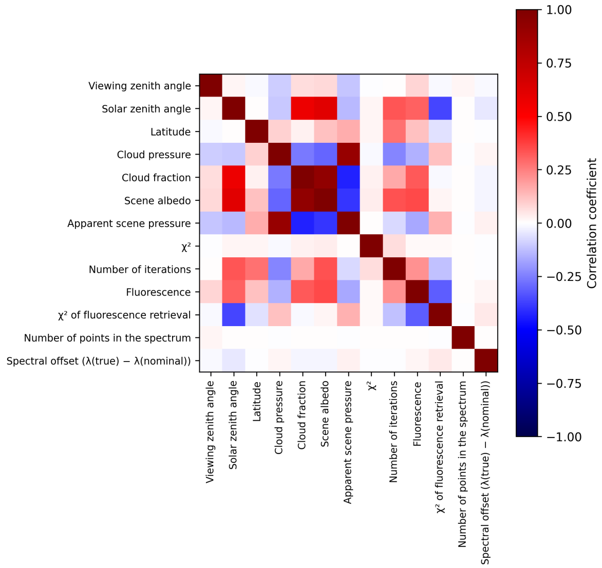
Figure 2: Map of correlation matrix for 2025-03-17 to 2025-03-18.
