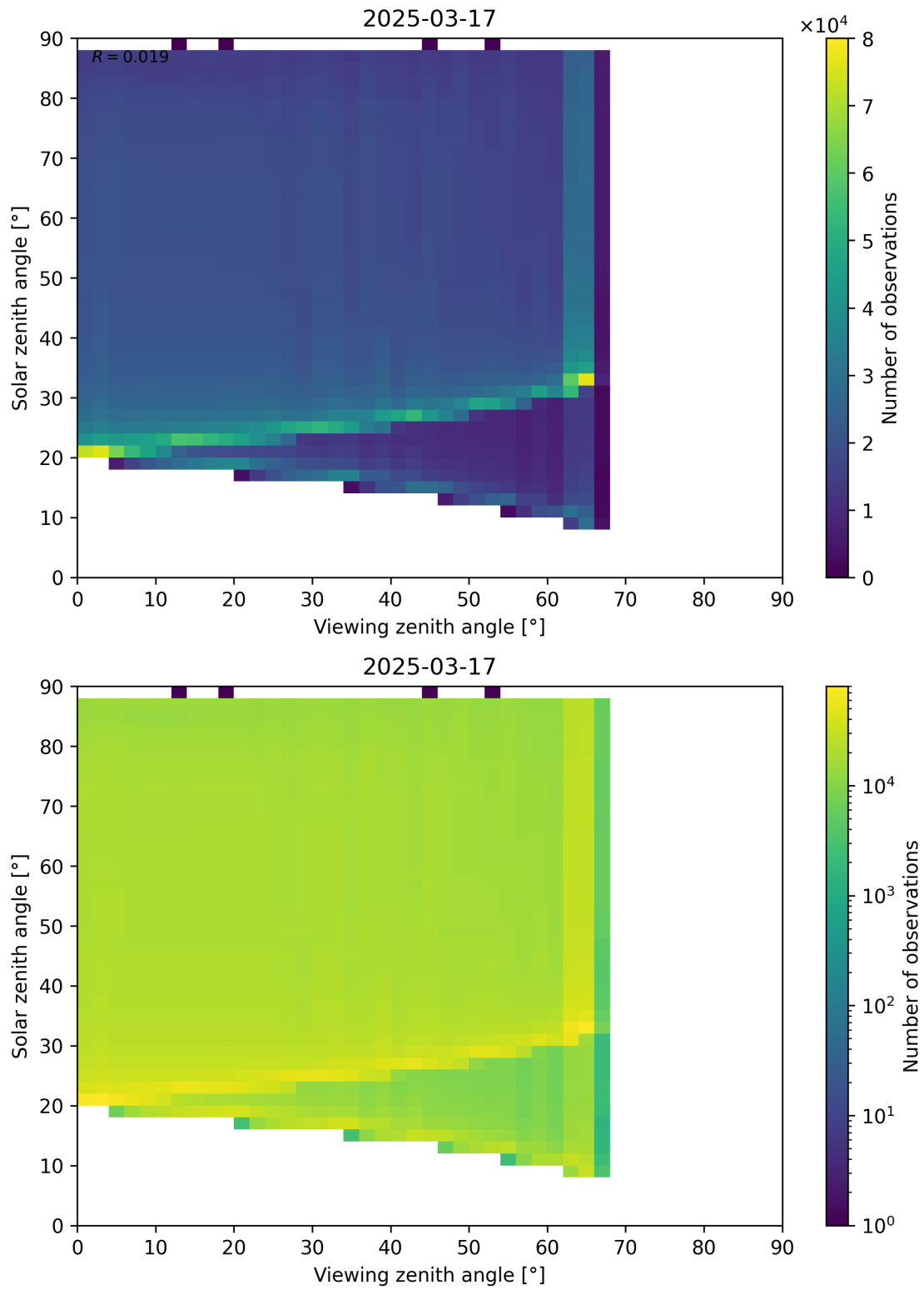
Figure 127: Scatter density plot of “Viewing zenith angle” against “Solar zenith angle” for 2025-03-17 to 2025-03-18.
