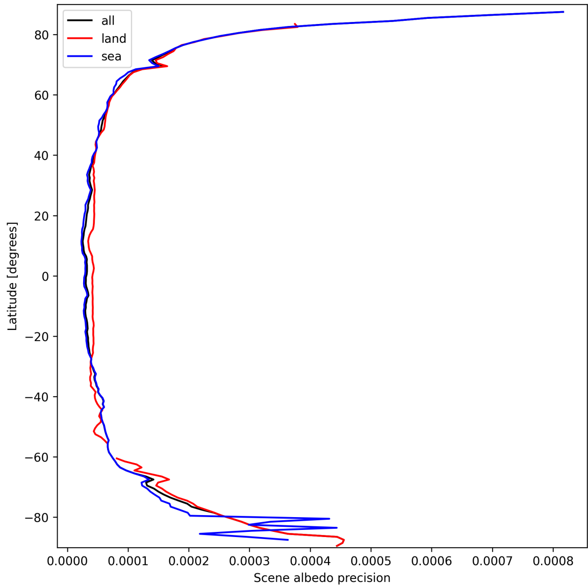
Figure 18: Zonal average of “Scene albedo precision” for 2025-03-17 to 2025-03-18.
