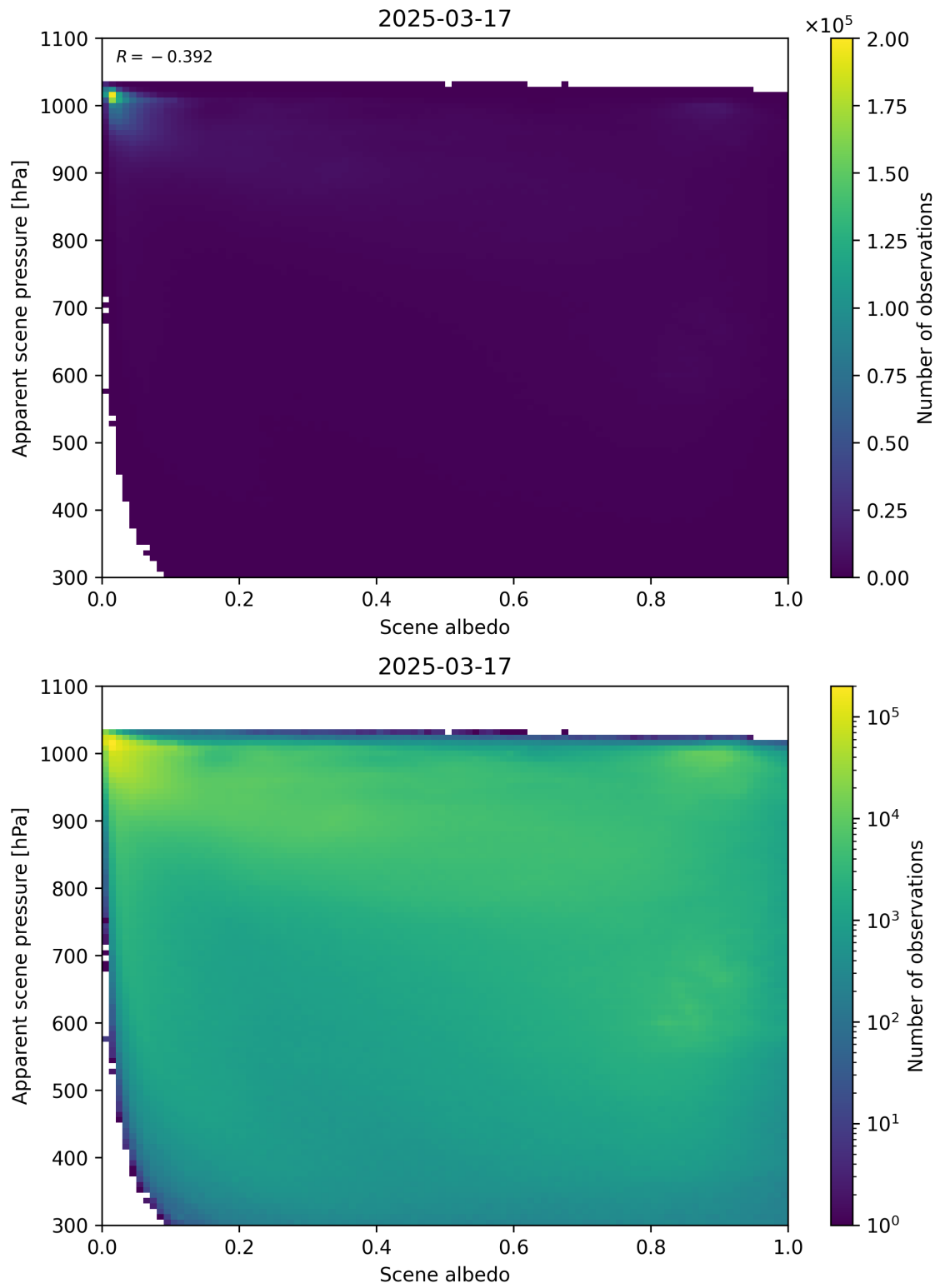
Figure 102: Scatter density plot of “Scene albedo” against “Apparent scene pressure” for 2025-03-17 to 2025-03-18.
