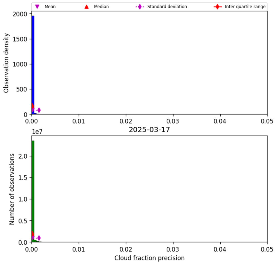
Figure 33: Histogram of “Cloud fraction precision” for 2025-03-17 to 2025-03-18
