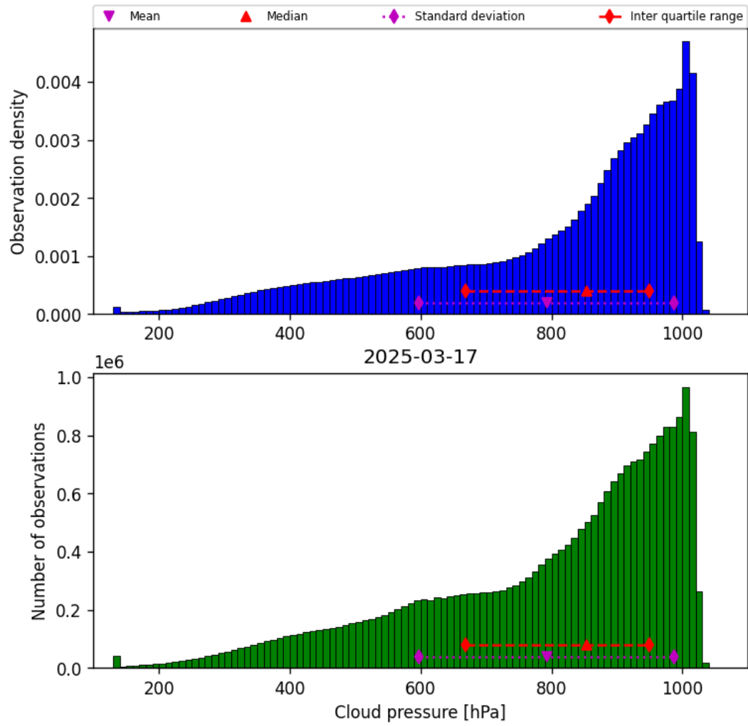
Figure 30: Histogram of “Cloud pressure” for 2025-03-17 to 2025-03-18
