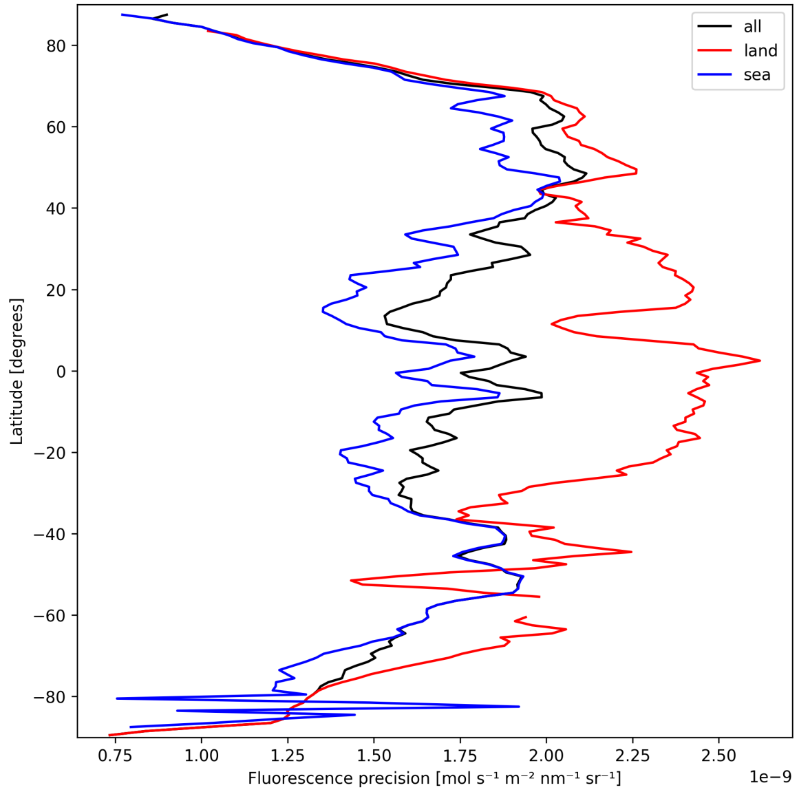
Figure 24: Zonal average of “Fluorescence precision” for 2025-03-17 to 2025-03-18.
