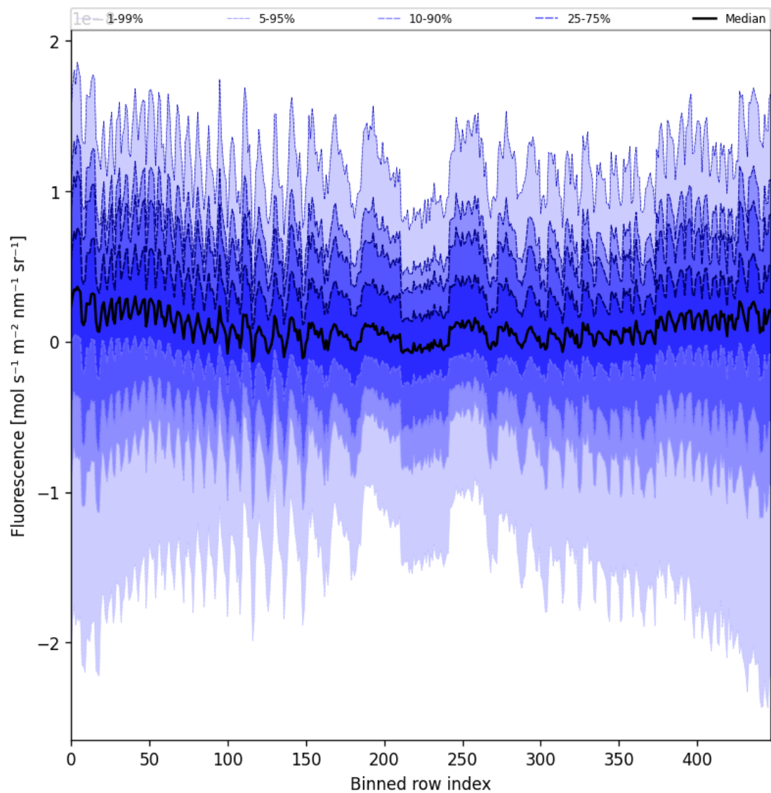
Figure 57: Along track statistics of “Fluorescence” for 2025-03-17 to 2025-03-18
