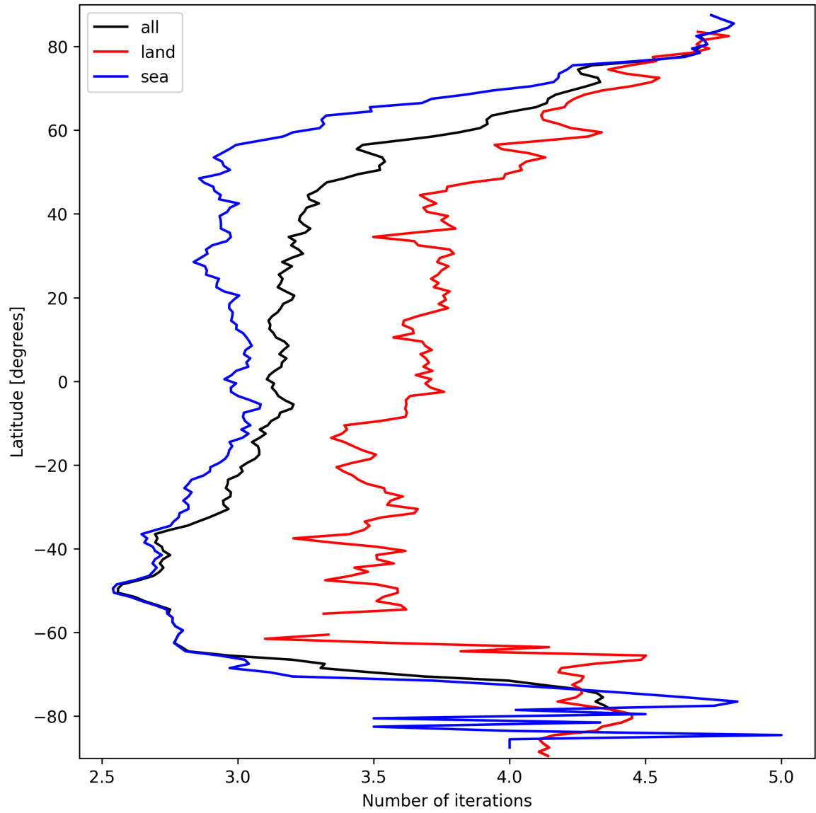
Figure 22: Zonal average of “Number of iterations” for 2025-03-17 to 2025-03-18.
