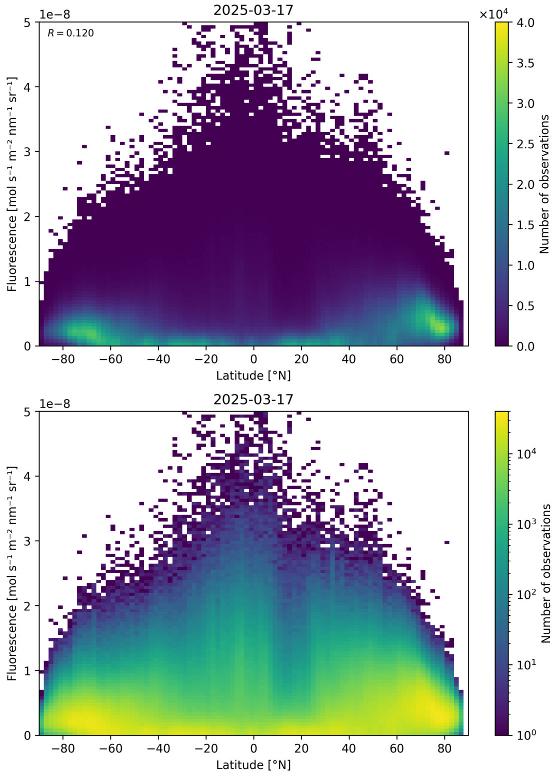
Figure 92: Scatter density plot of “Latitude” against “Fluorescence” for 2025-03-17 to 2025-03-18.
