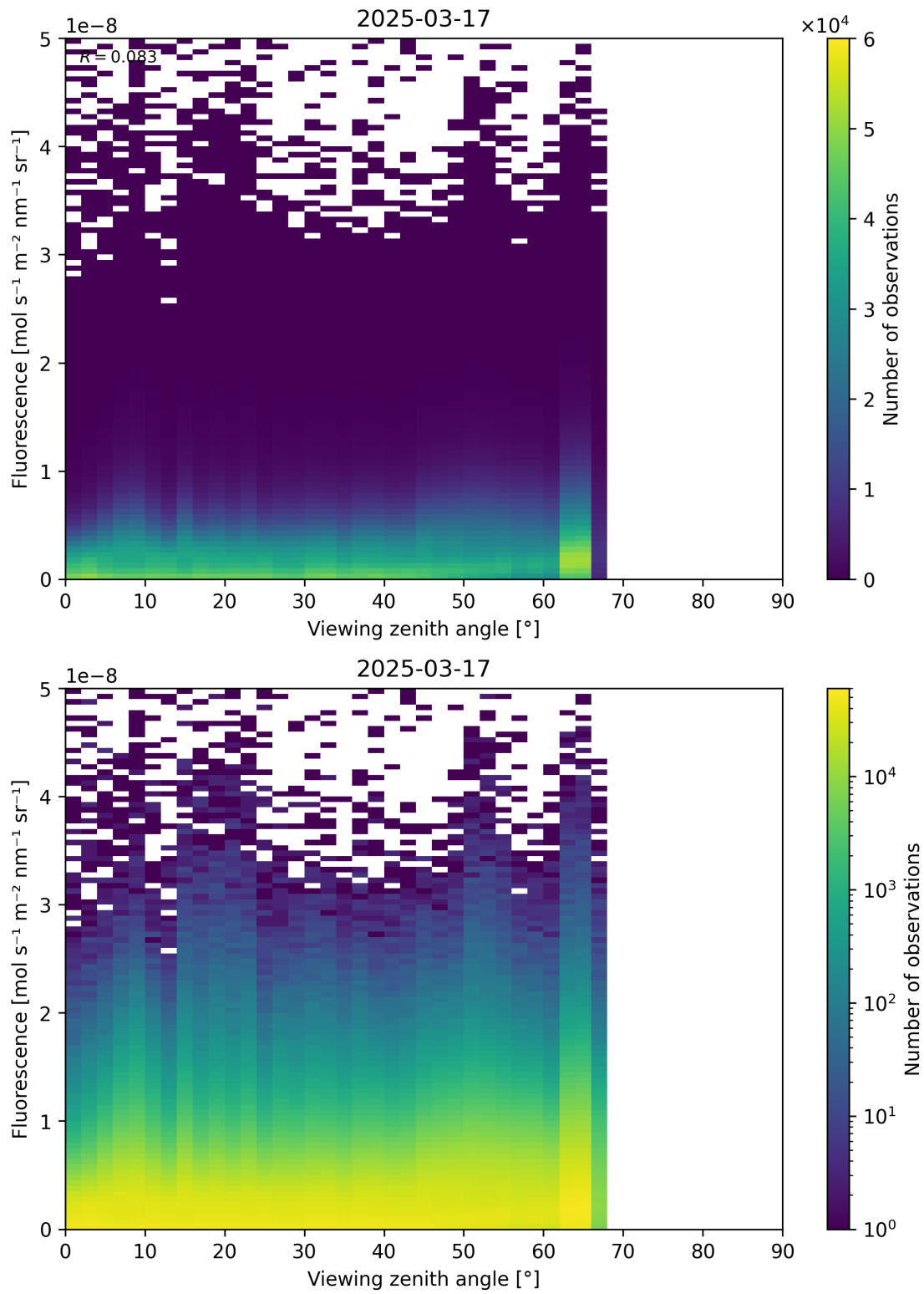
Figure 122: Scatter density plot of “Viewing zenith angle” against “Fluorescence” for 2025-03-17 to 2025-03-18.
