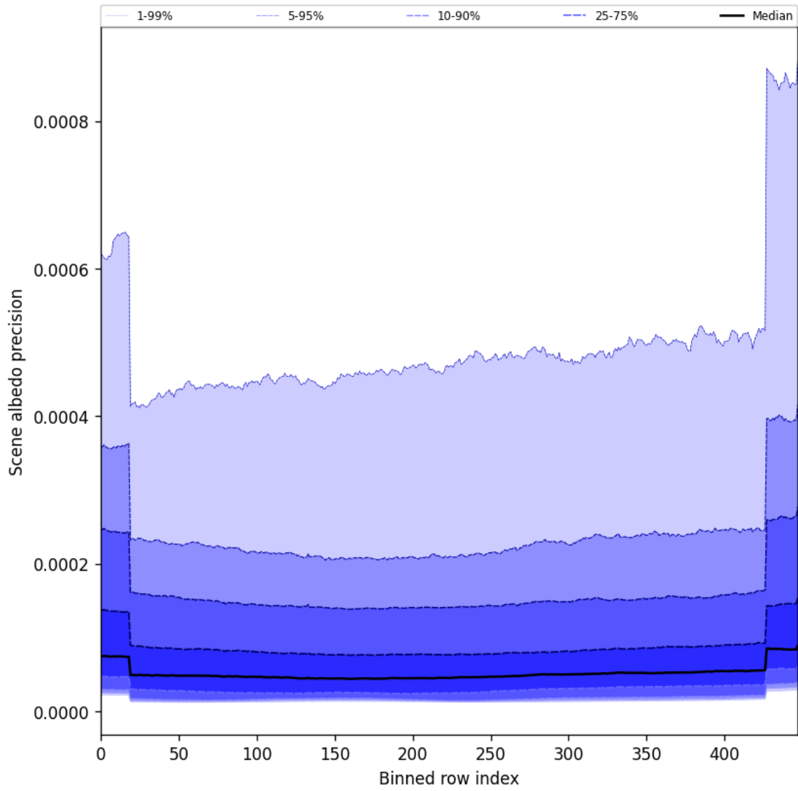
Figure 52: Along track statistics of “Scene albedo precision” for 2025-03-17 to 2025-03-18
