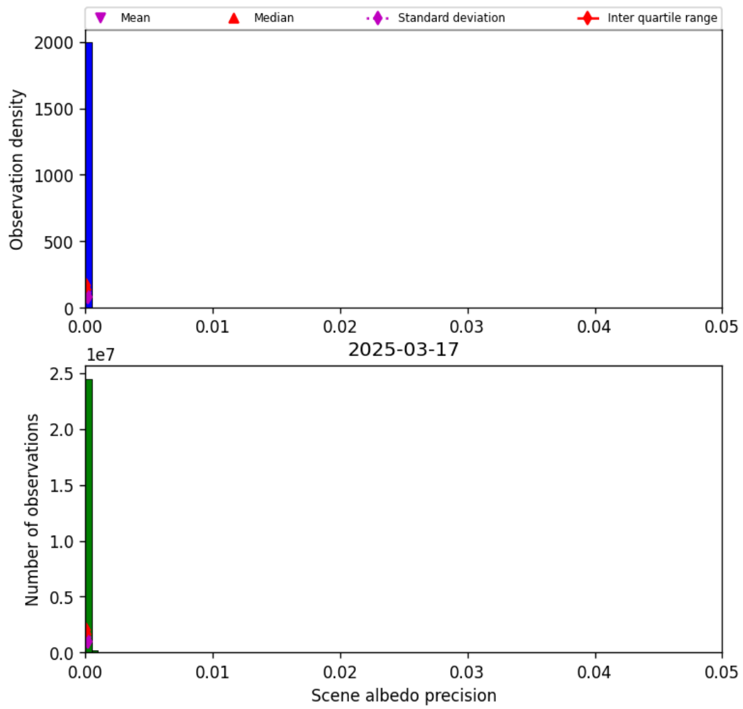
Figure 35: Histogram of “Scene albedo precision” for 2025-03-17 to 2025-03-18
