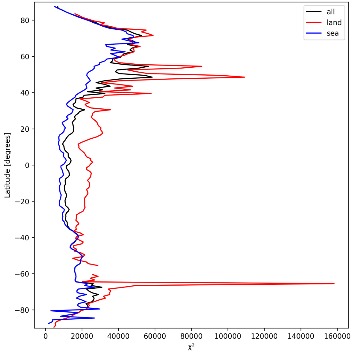
Figure 21: Zonal average of “ \chi^2 ” for 2025-03-17 to 2025-03-18.
