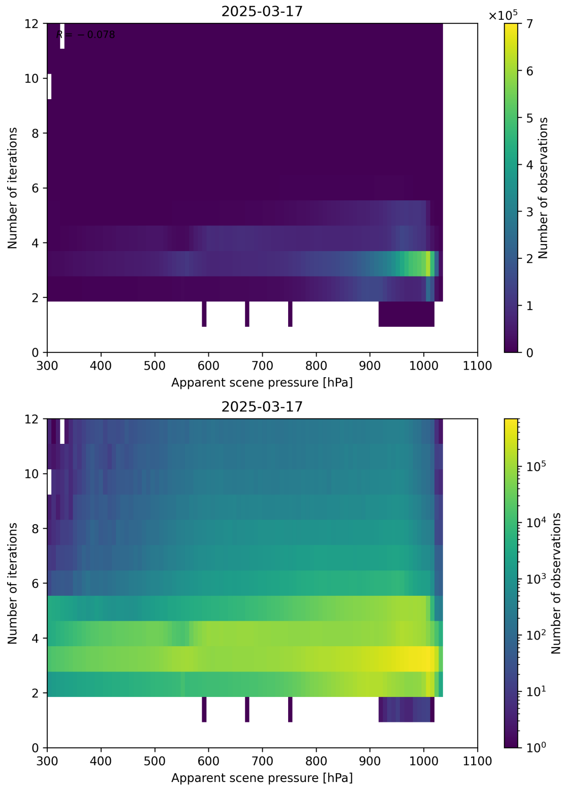
Figure 65: Scatter density plot of “Apparent scene pressure” against “Number of iterations” for 2025-03-17 to 2025-03-18.
