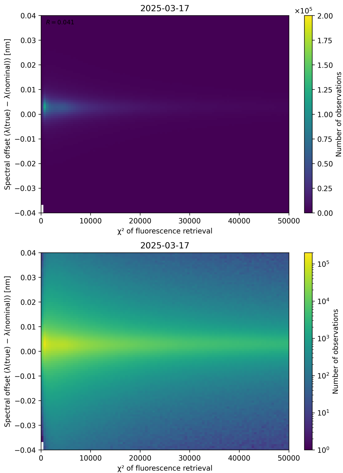
Figure 69: Scatter density plot of “ \chi^2 of fluorescence retrieval” against “Spectral offset ( \lambda_{\text{true}} - \lambda_{\text{nominal}} )” for 2025-03-17 to 2025-03-18.
