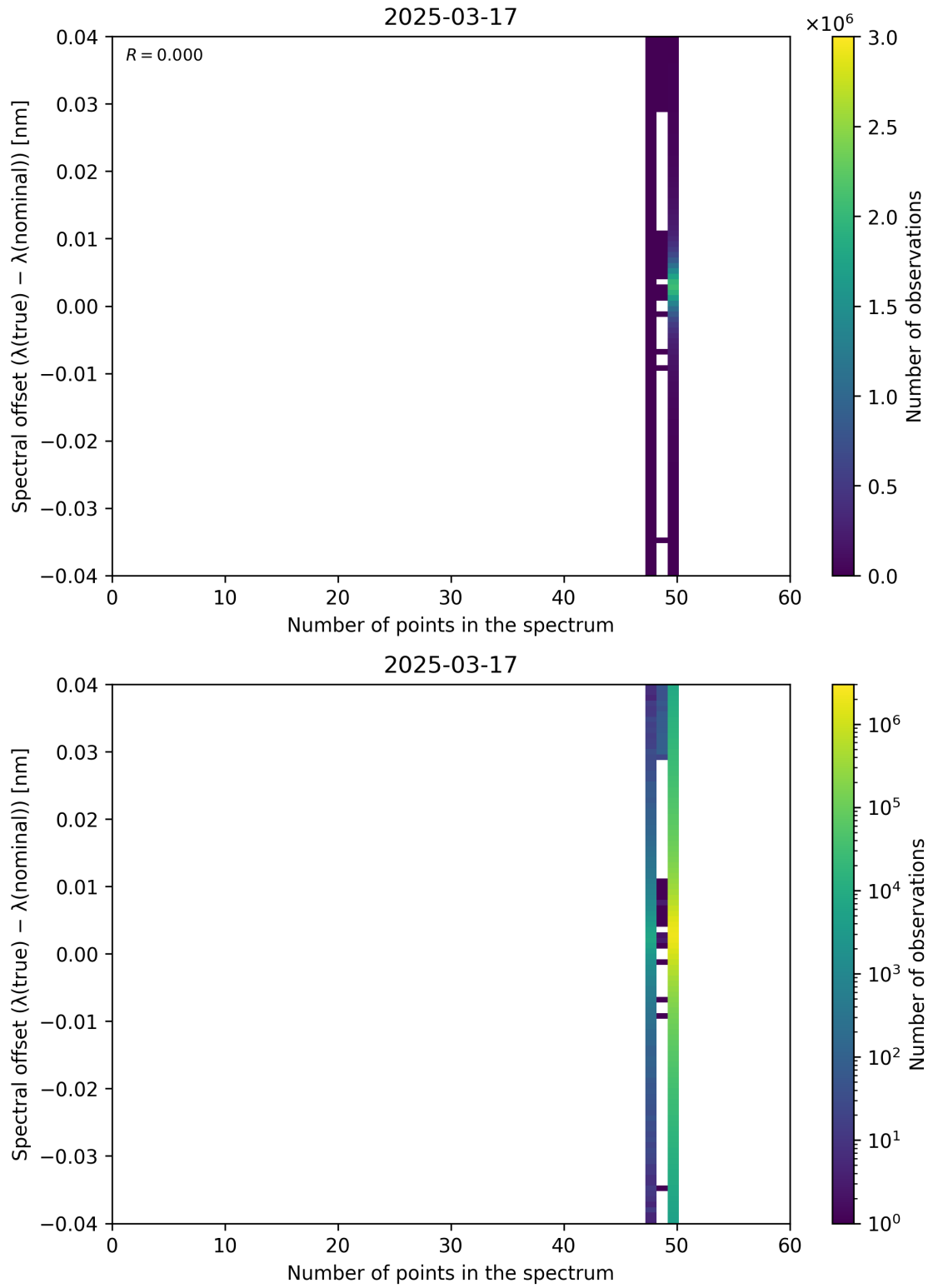
Figure 101: Scatter density plot of “Number of points in the spectrum” against “Spectral offset ( \lambda_{\text{true}} - \lambda_{\text{nominal}} )” for 2025-03-17 to 2025-03-18.
