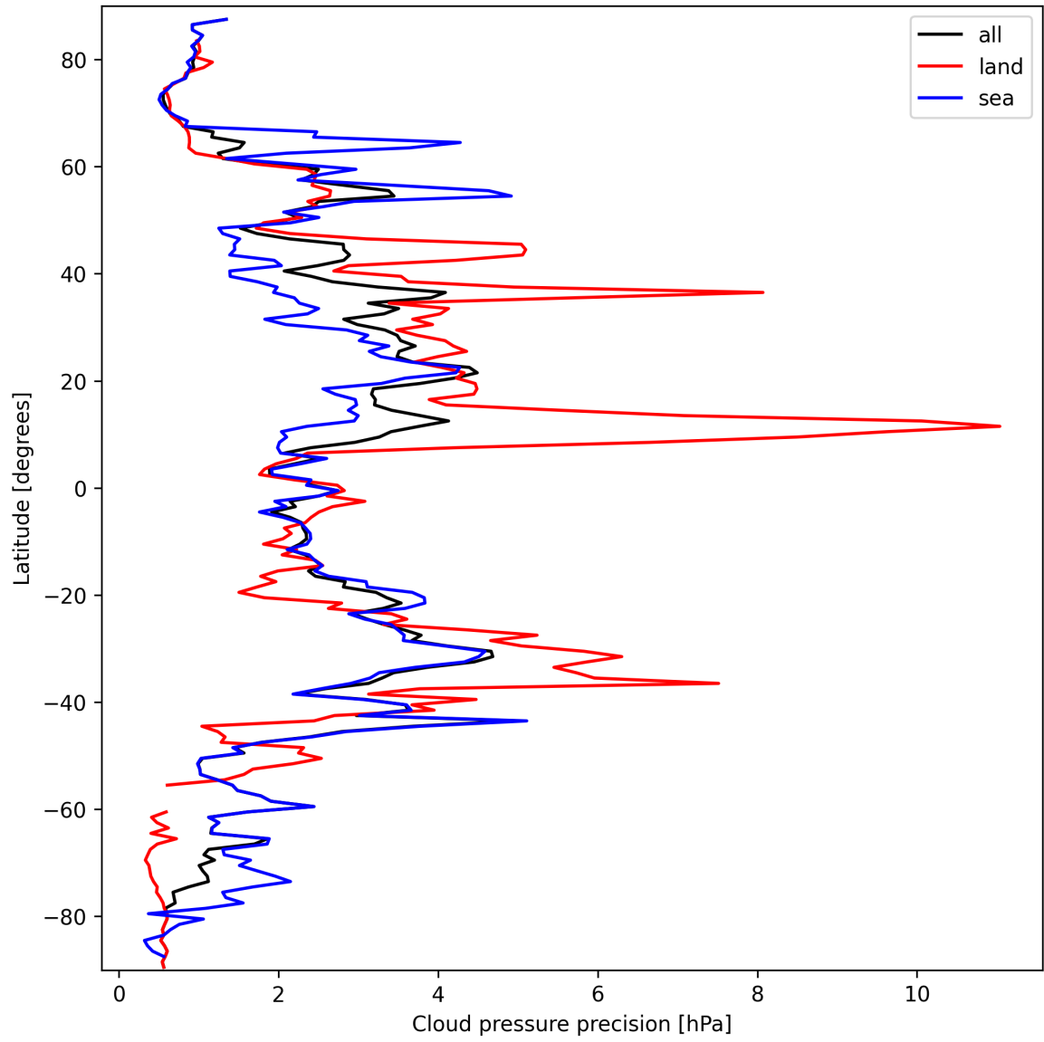
Figure 14: Zonal average of "Cloud pressure precision" for 2025-03-17 to 2025-03-18.
