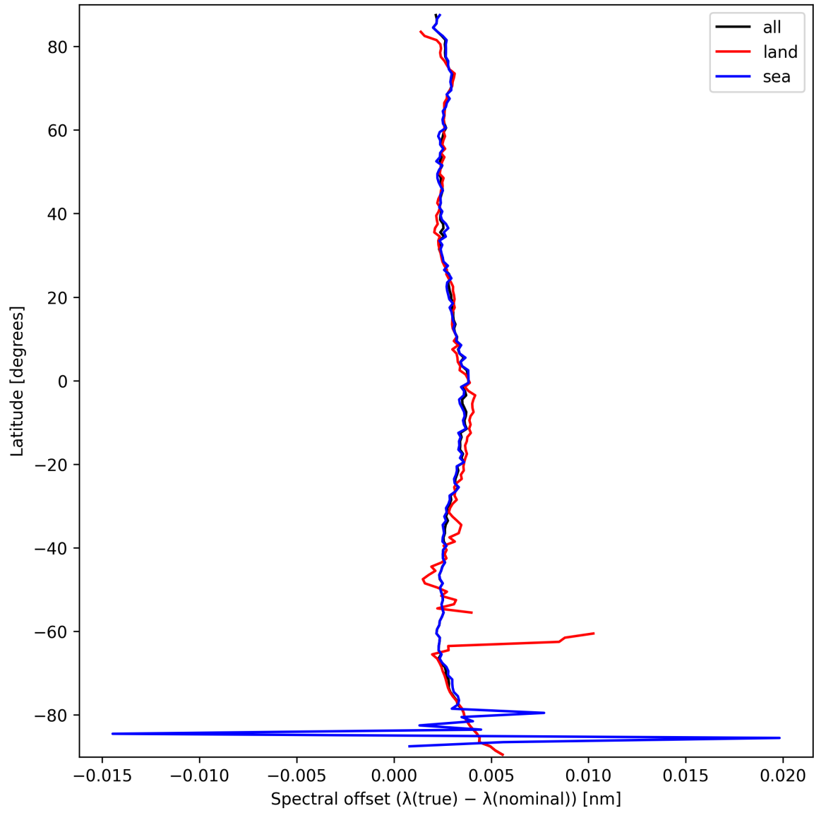
Figure 28: Zonal average of “Spectral offset ( \lambda_{\text{true}} - \lambda_{\text{nominal}} )” for 2025-03-17 to 2025-03-18.
