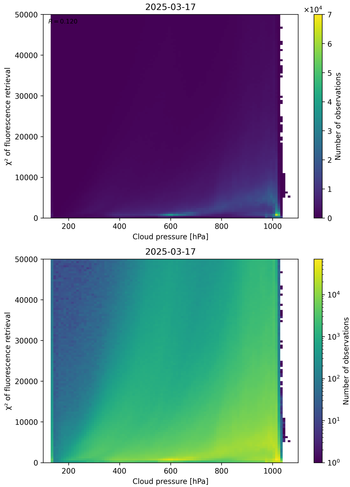
Figure 78: Scatter density plot of “Cloud pressure” against “ \chi^2 of fluorescence retrieval” for 2025-03-17 to 2025-03-18.
