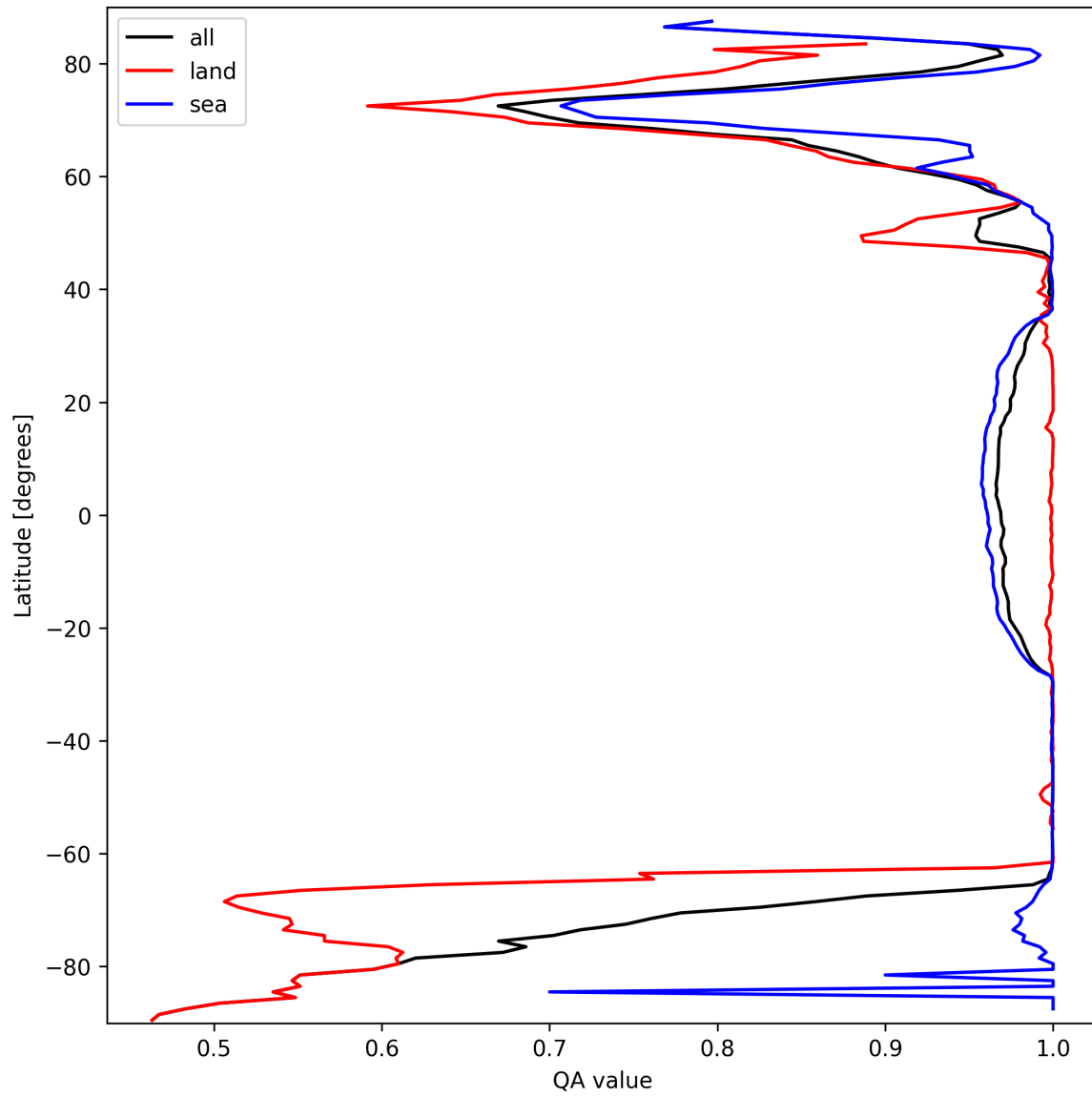
Figure 12: Zonal average of “QA value” for 2025-03-17 to 2025-03-18.
