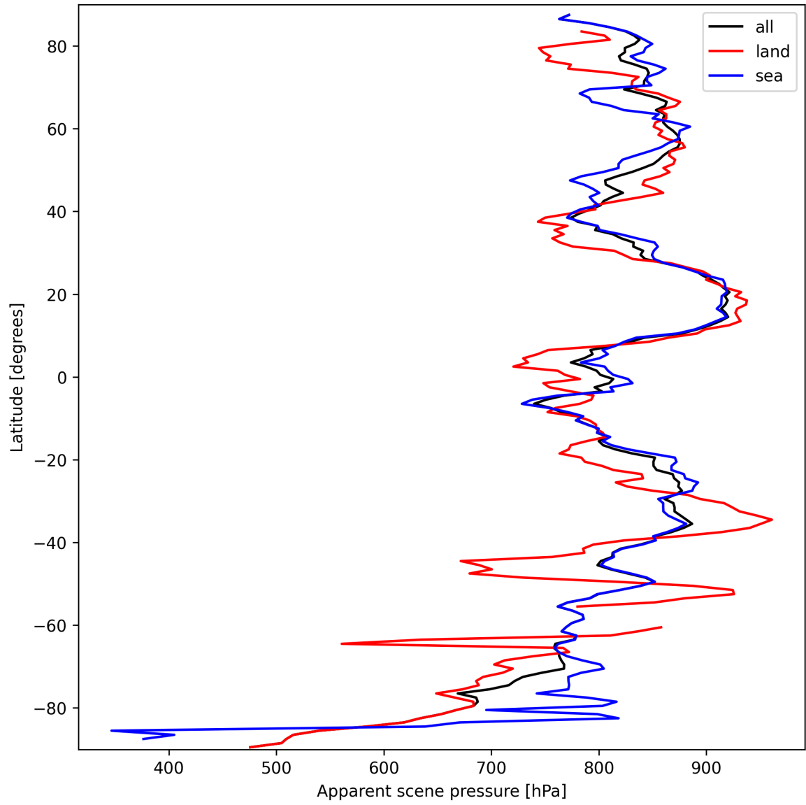
Figure 19: Zonal average of “Apparent scene pressure” for 2025-03-17 to 2025-03-18.
