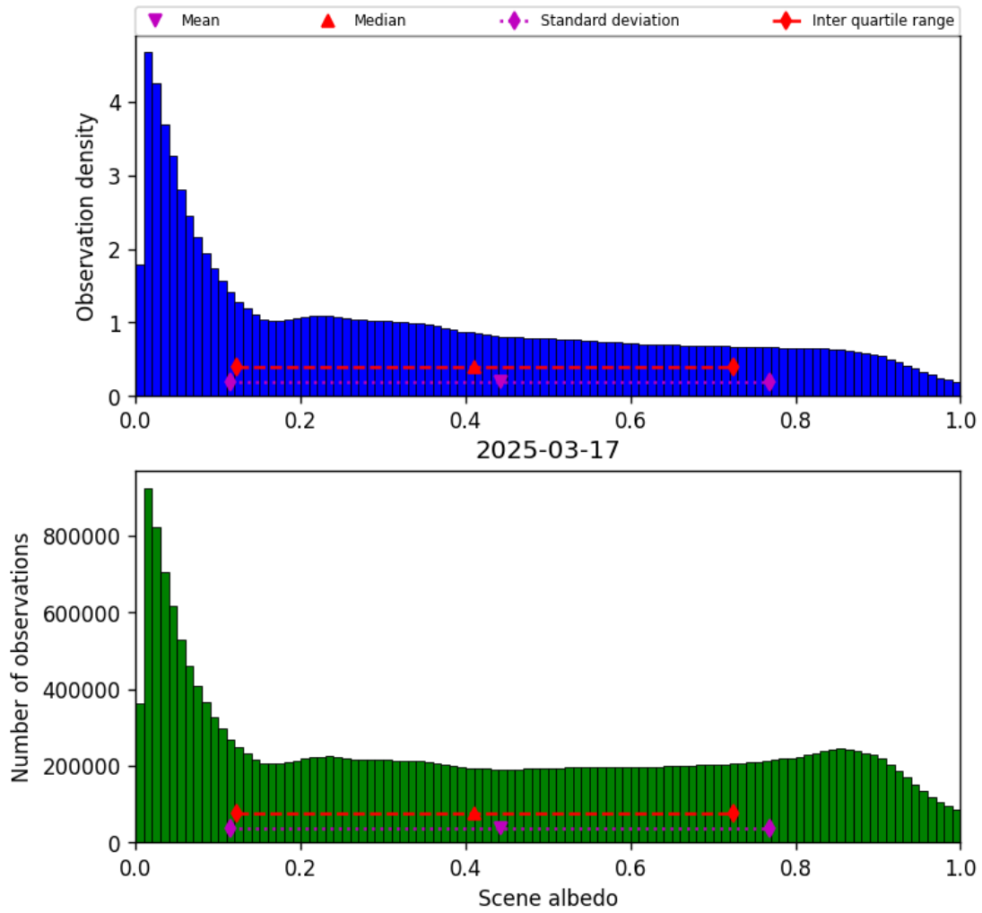
Figure 34: Histogram of “Scene albedo” for 2025-03-17 to 2025-03-18
