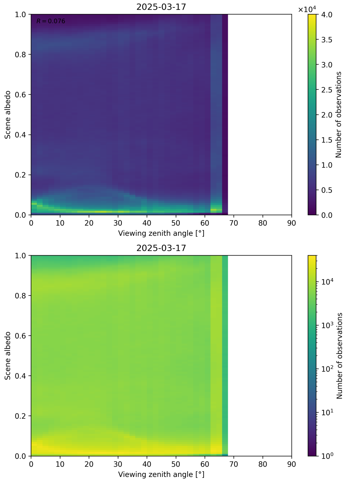
Figure 126: Scatter density plot of “Viewing zenith angle” against “Scene albedo” for 2025-03-17 to 2025-03-18.
