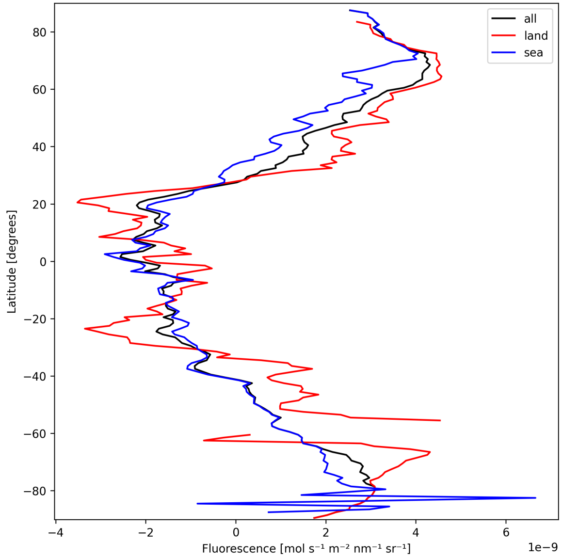
Figure 23: Zonal average of “Fluorescence” for 2025-03-17 to 2025-03-18.
