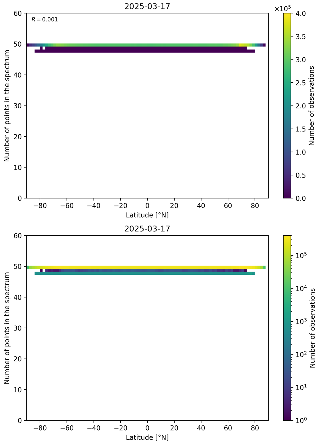
Figure 94: Scatter density plot of “Latitude” against “Number of points in the spectrum” for 2025-03-17 to 2025-03-18.
