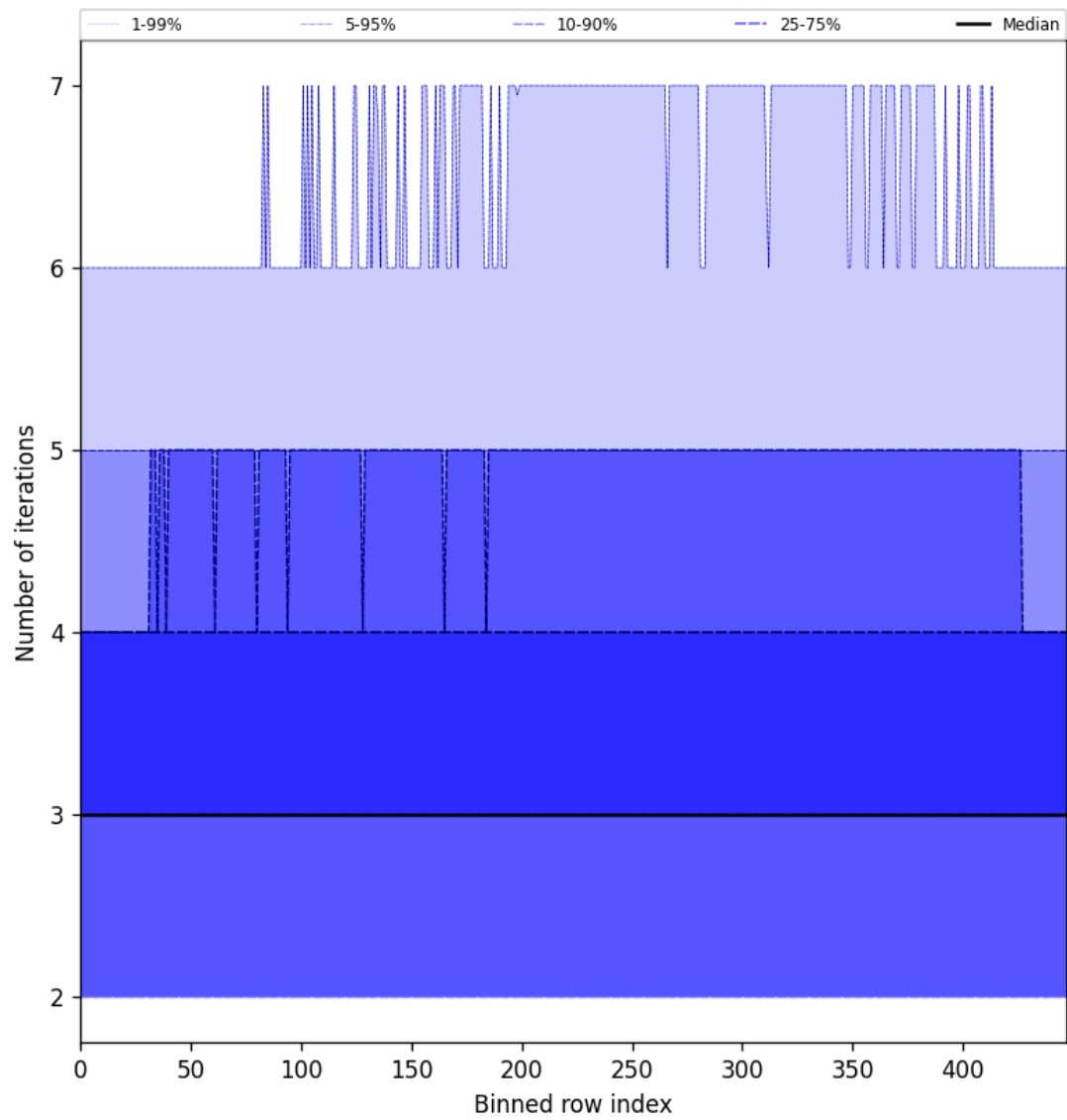
Figure 56: Along track statistics of “Number of iterations” for 2025-03-17 to 2025-03-18
