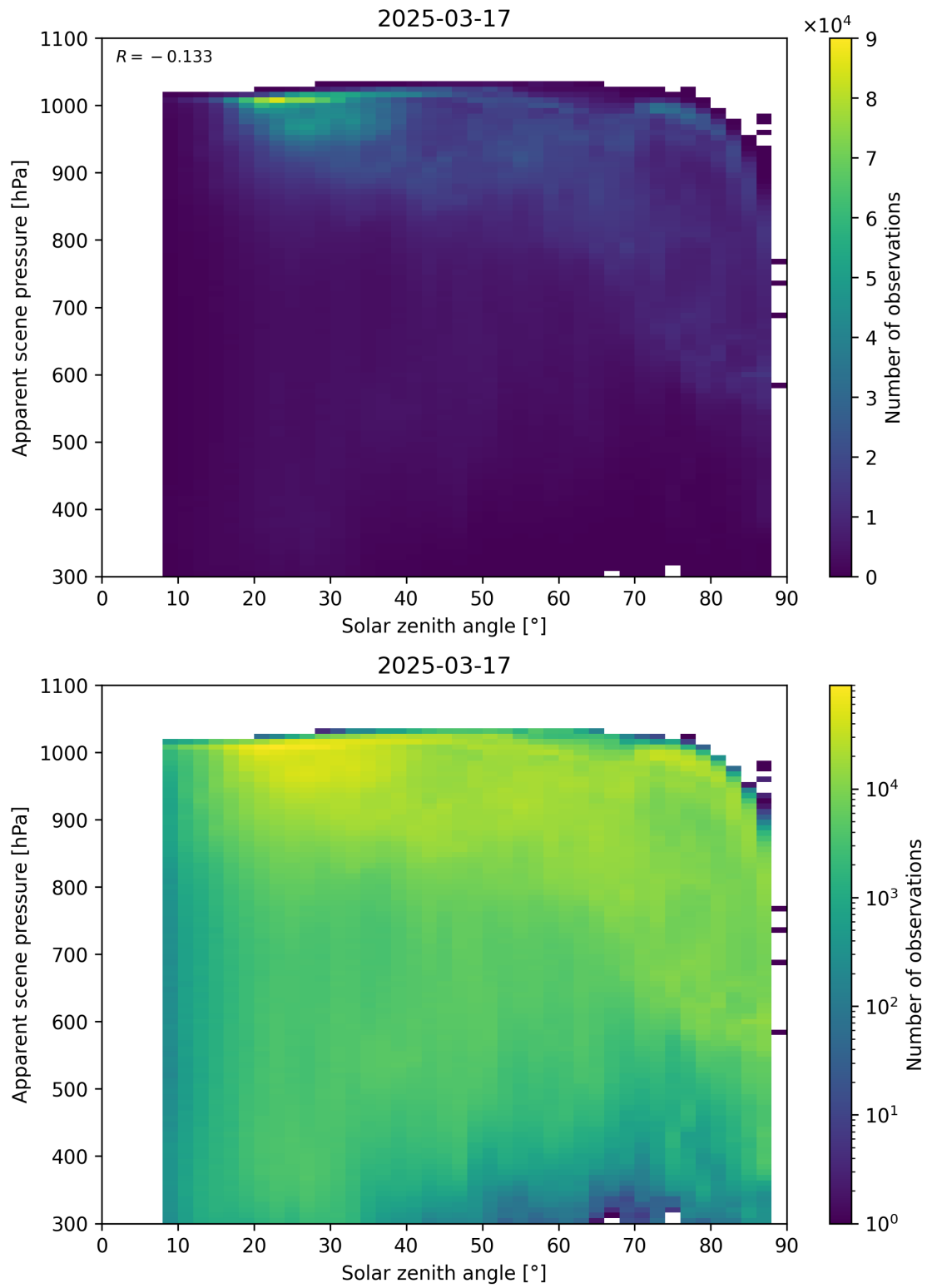
Figure 108: Scatter density plot of “Solar zenith angle” against “Apparent scene pressure” for 2025-03-17 to 2025-03-18.
