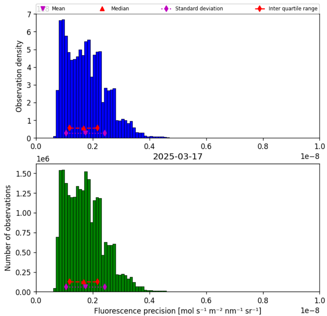
Figure 41: Histogram of “Fluorescence precision” for 2025-03-17 to 2025-03-18
