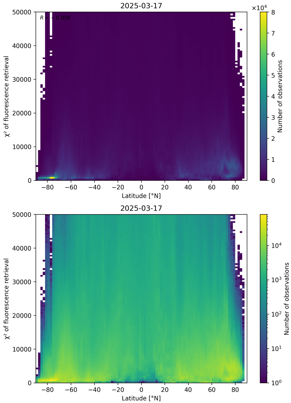
Figure 89: Scatter density plot of “Latitude” against “ \chi^2 of fluorescence retrieval” for 2025-03-17 to 2025-03-18.
