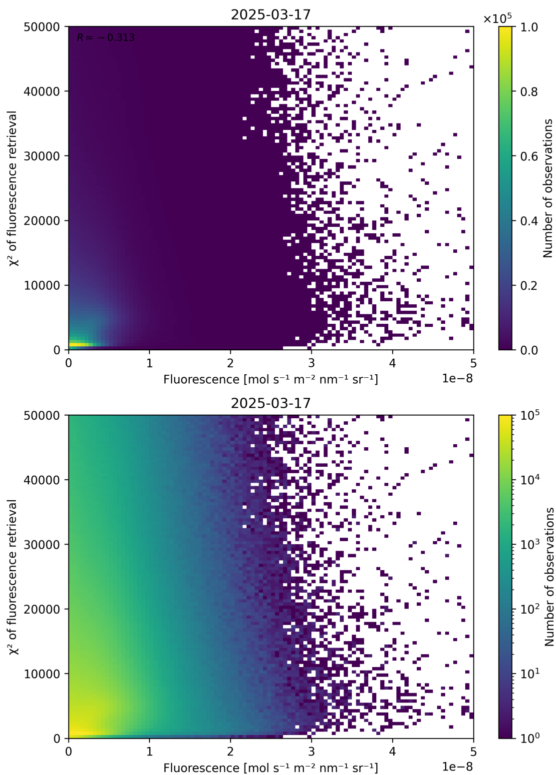
Figure 85: Scatter density plot of “Fluorescence” against “ \chi^2 of fluorescence retrieval” for 2025-03-17 to 2025-03-18.
