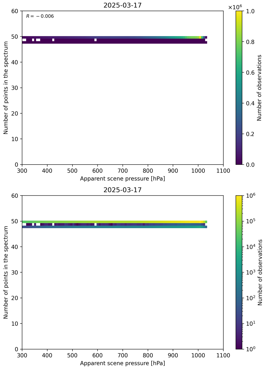
Figure 66: Scatter density plot of “Apparent scene pressure” against “Number of points in the spectrum” for 2025-03-17 to 2025-03-18.
