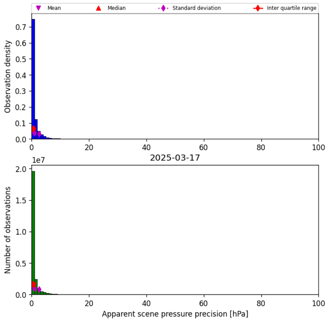
Figure 37: Histogram of “Apparent scene pressure precision” for 2025-03-17 to 2025-03-18
