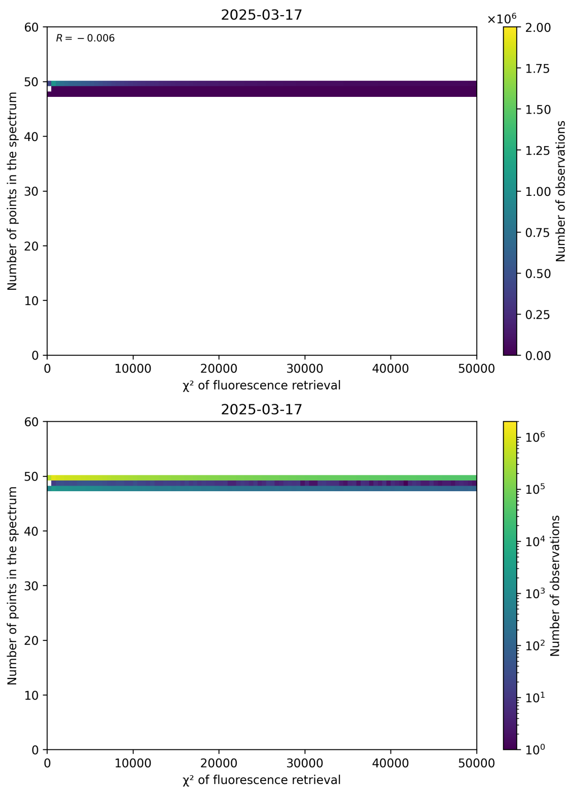
Figure 68: Scatter density plot of " \chi^2 of fluorescence retrieval" against "Number of points in the spectrum" for 2025-03-17 to 2025-03-18.
