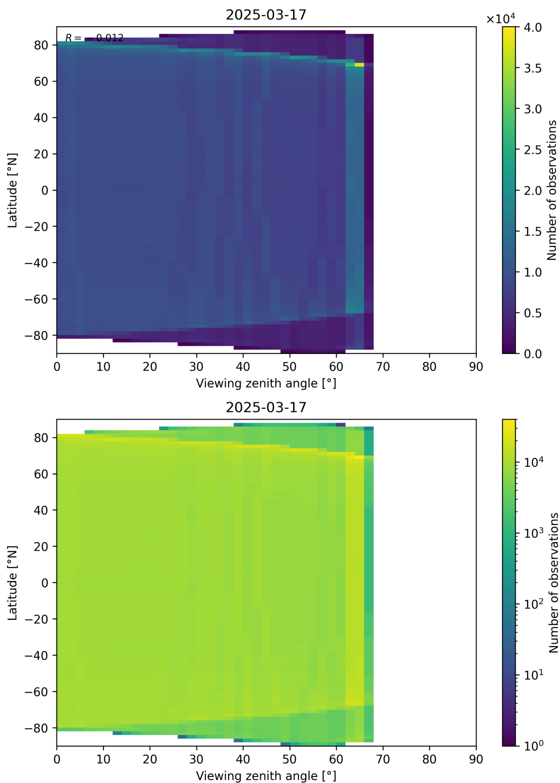
Figure 123: Scatter density plot of “Viewing zenith angle” against “Latitude” for 2025-03-17 to 2025-03-18.
