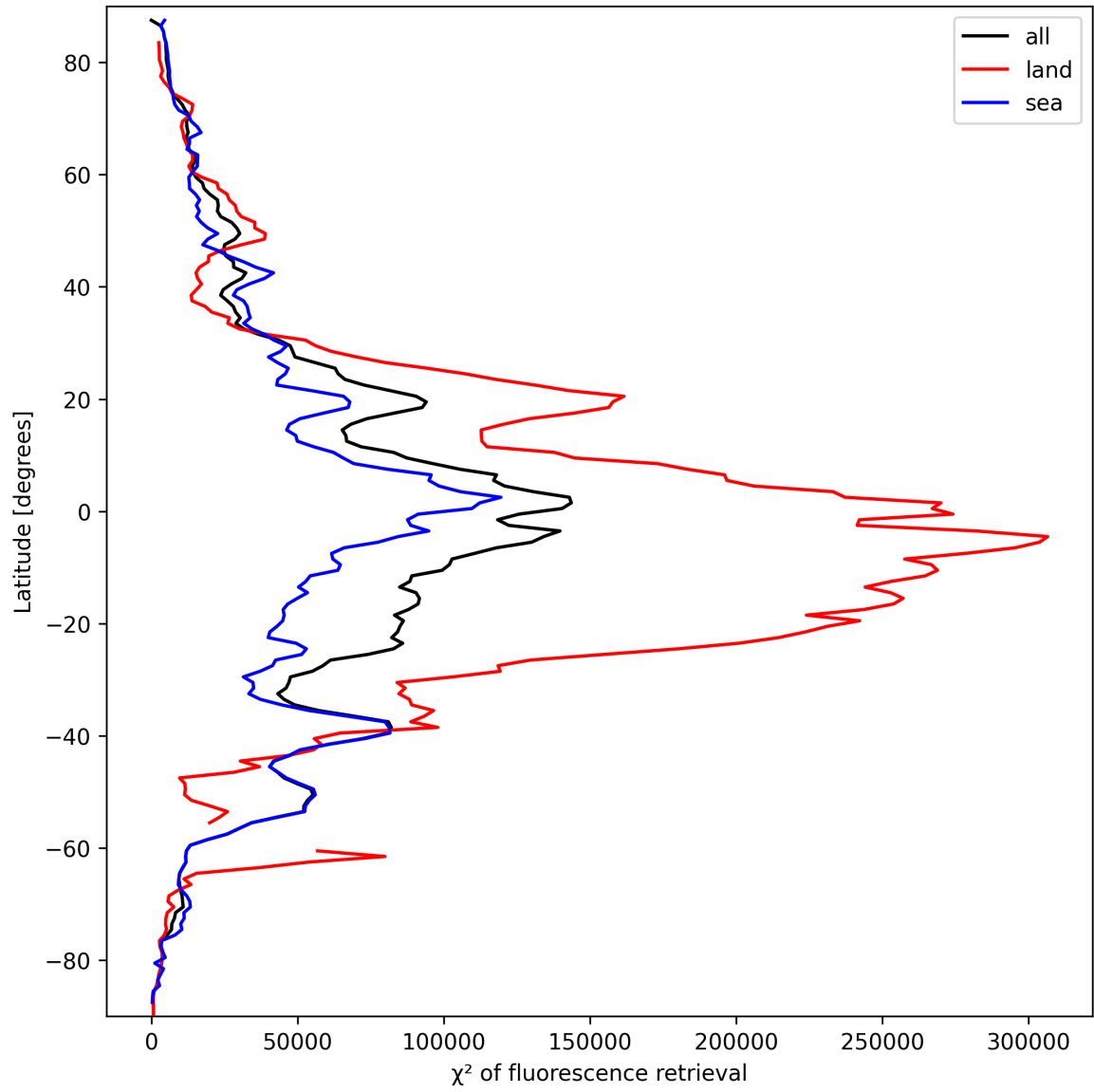
Figure 25: Zonal average of “ \chi^2 of fluorescence retrieval” for 2025-03-17 to 2025-03-18.
