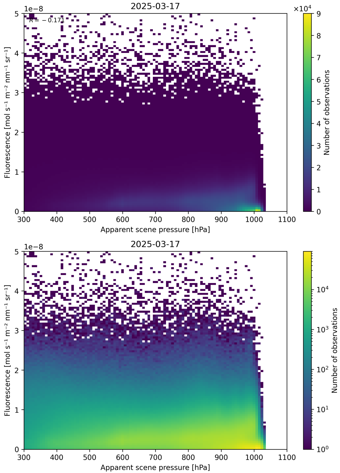
Figure 64: Scatter density plot of “Apparent scene pressure” against “Fluorescence” for 2025-03-17 to 2025-03-18.
