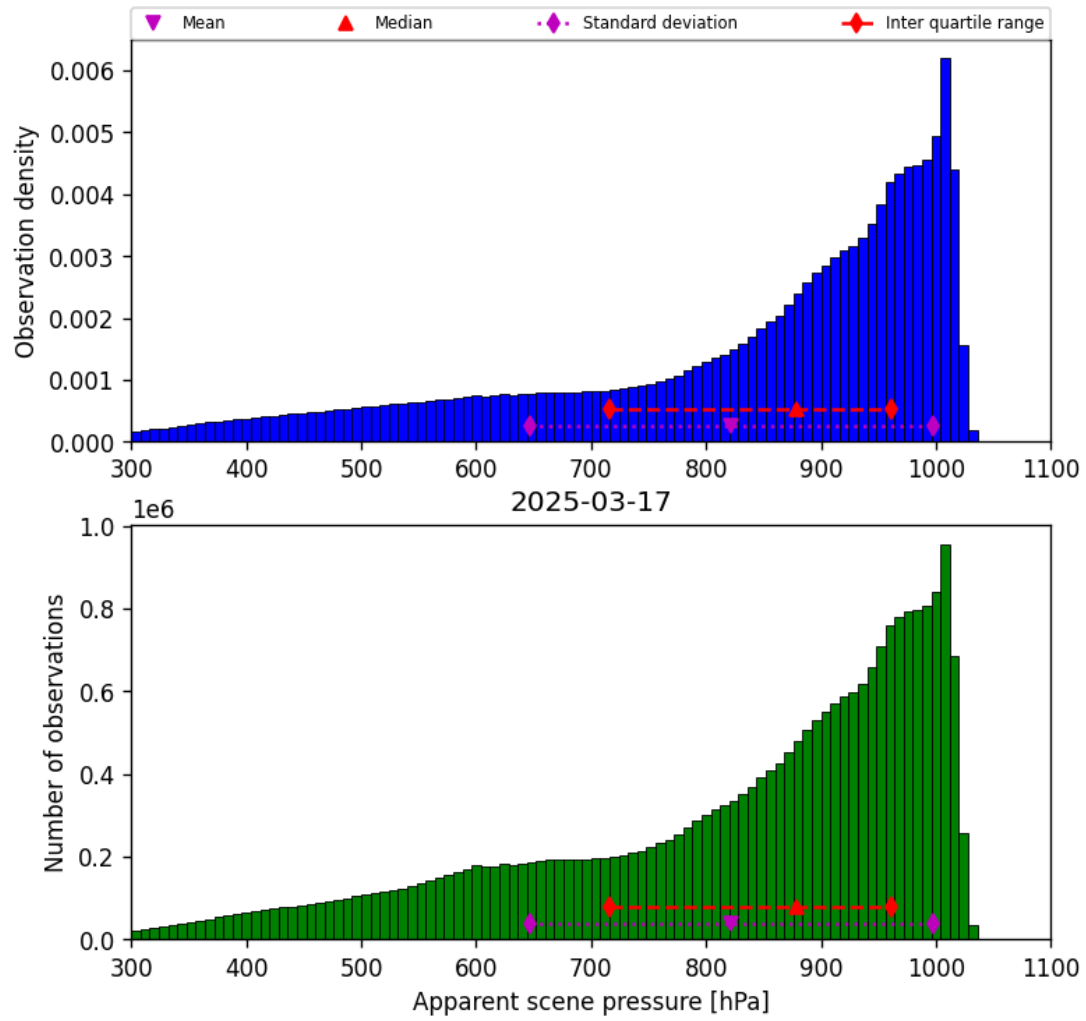
Figure 36: Histogram of “Apparent scene pressure” for 2025-03-17 to 2025-03-18
