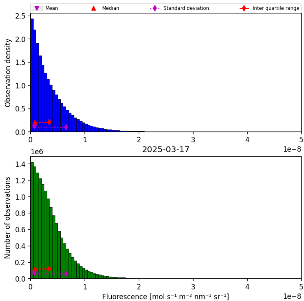
Figure 40: Histogram of “Fluorescence” for 2025-03-17 to 2025-03-18
