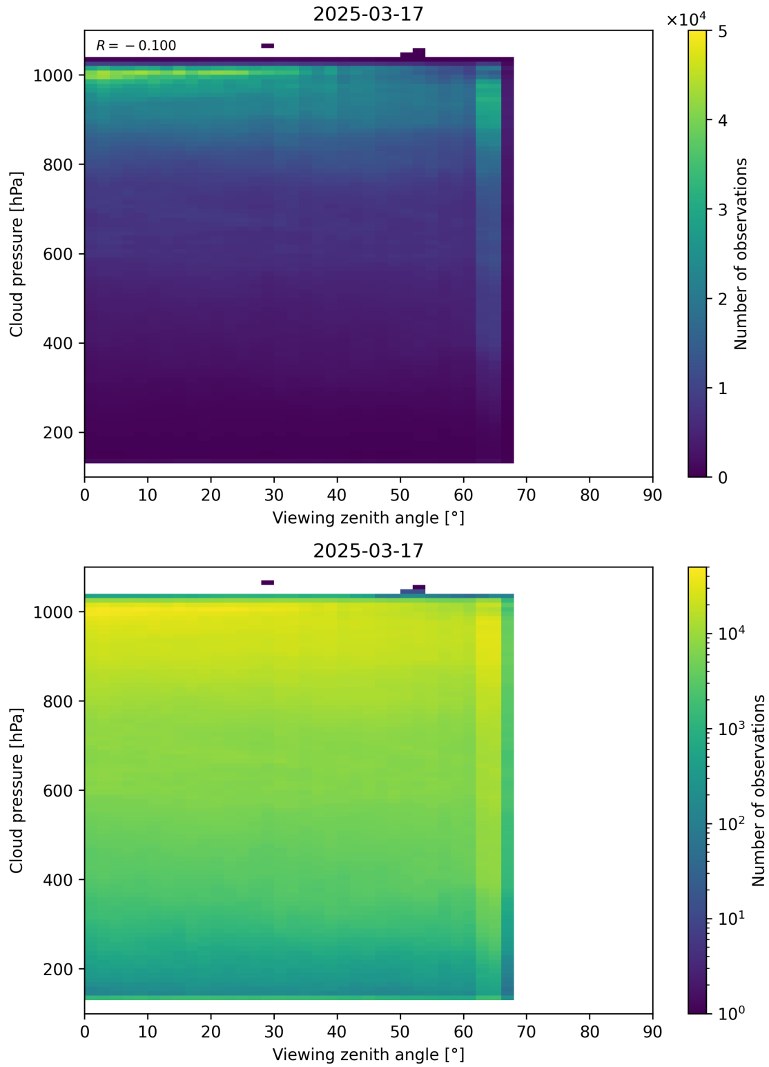
Figure 121: Scatter density plot of “Viewing zenith angle” against “Cloud pressure” for 2025-03-17 to 2025-03-18.
