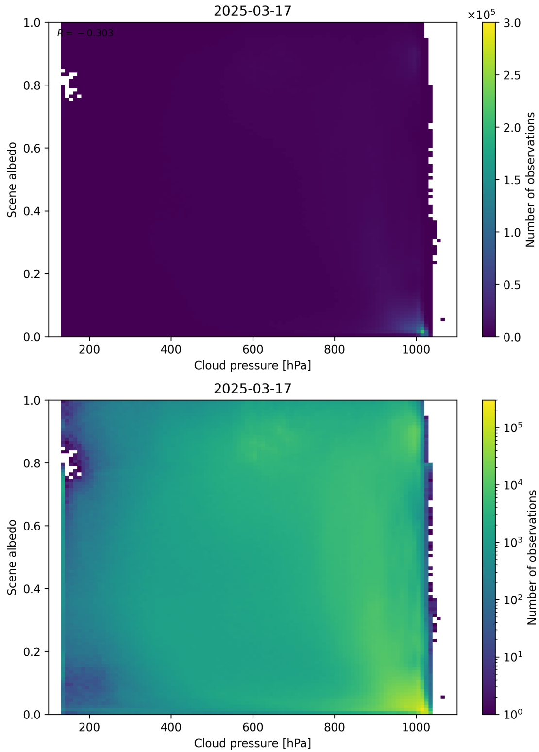
Figure 83: Scatter density plot of “Cloud pressure” against “Scene albedo” for 2025-03-17 to 2025-03-18.
