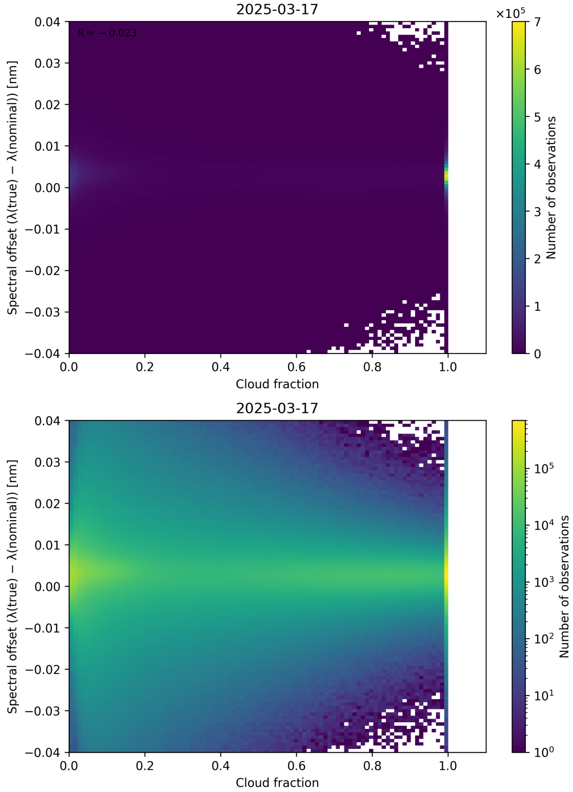
Figure 76: Scatter density plot of “Cloud fraction” against “Spectral offset ( \lambda_{\text{true}} - \lambda_{\text{nominal}} )” for 2025-03-17 to 2025-03-18.
