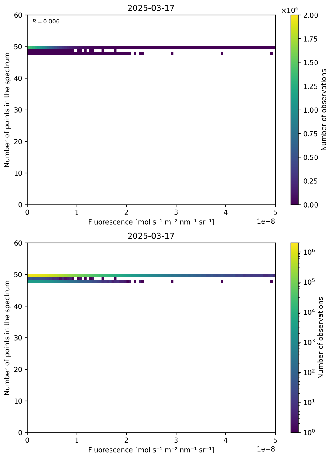
Figure 86: Scatter density plot of “Fluorescence” against “Number of points in the spectrum” for 2025-03-17 to 2025-03-18.
