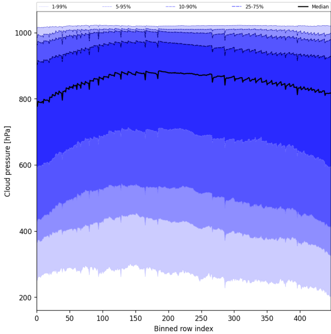
Figure 47: Along track statistics of “Cloud pressure” for 2025-03-17 to 2025-03-18
