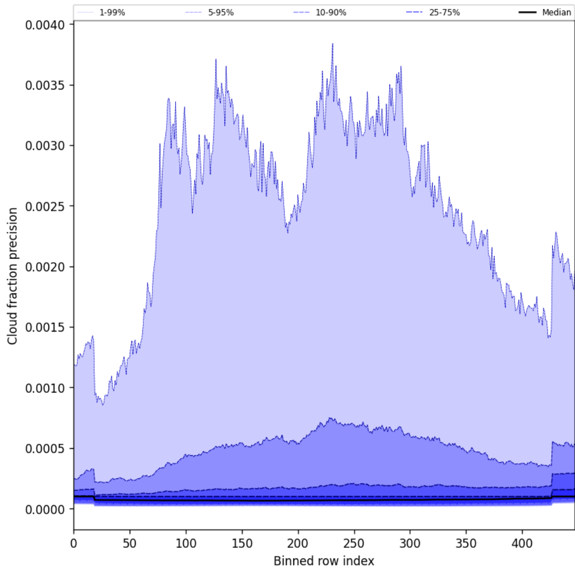
Figure 50: Along track statistics of “Cloud fraction precision” for 2025-03-17 to 2025-03-18
