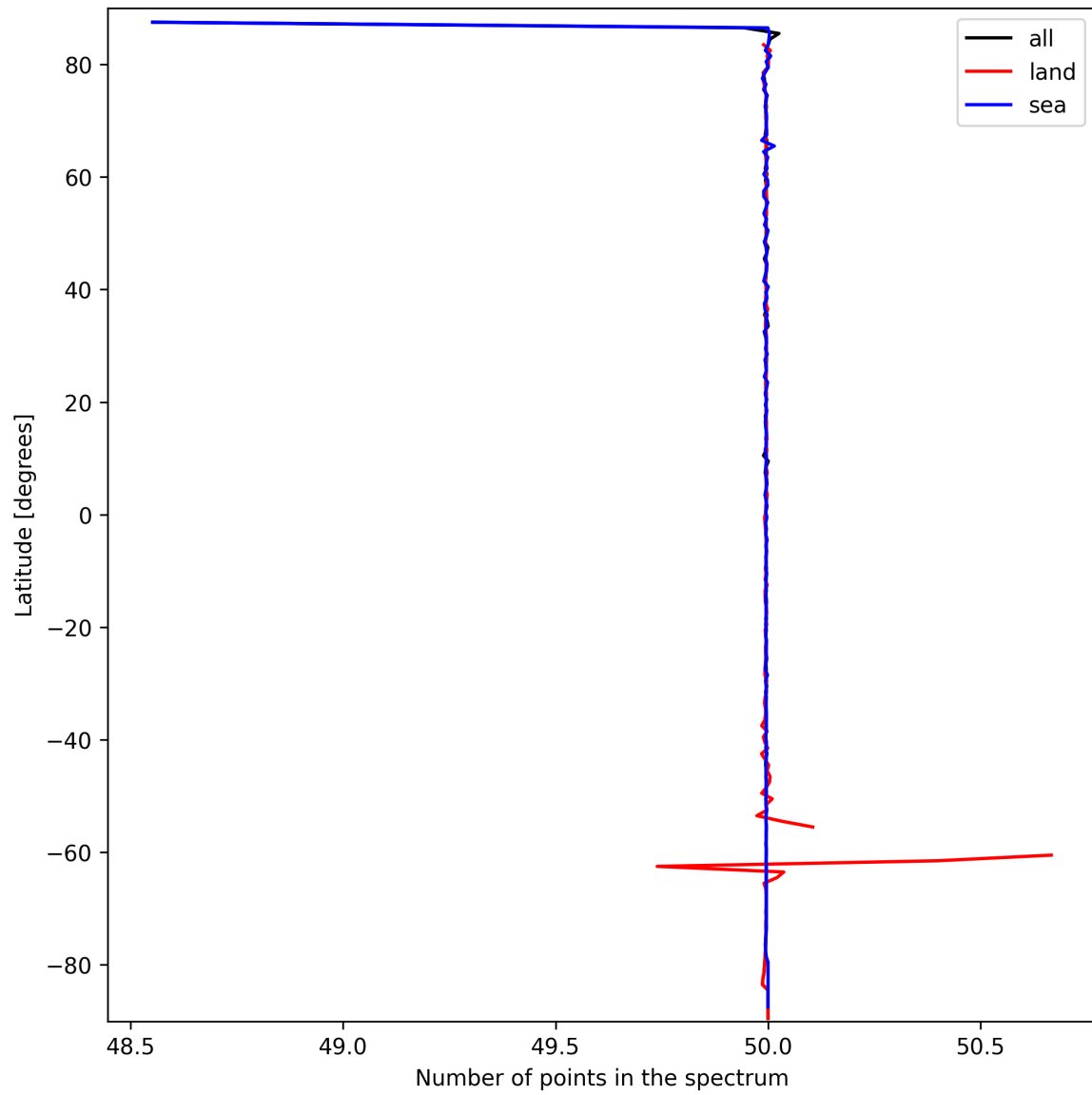
Figure 27: Zonal average of “Number of points in the spectrum” for 2025-03-17 to 2025-03-18.
