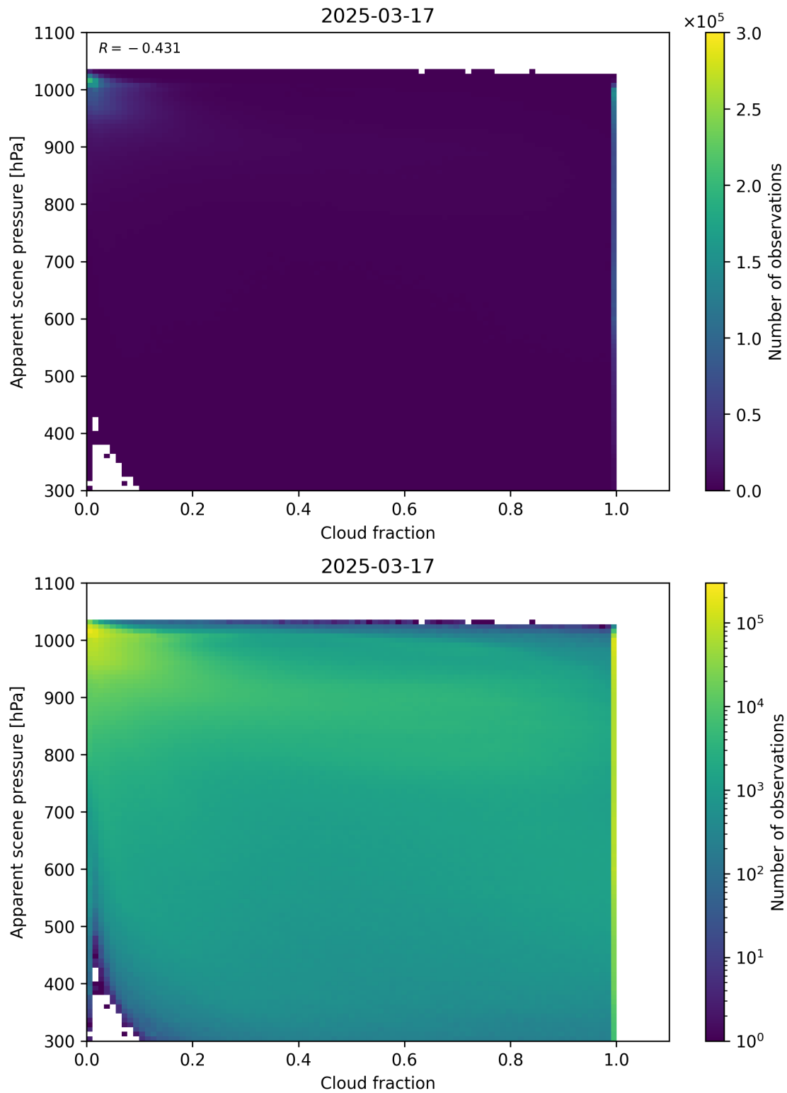
Figure 70: Scatter density plot of “Cloud fraction” against “Apparent scene pressure” for 2025-03-17 to 2025-03-18.
