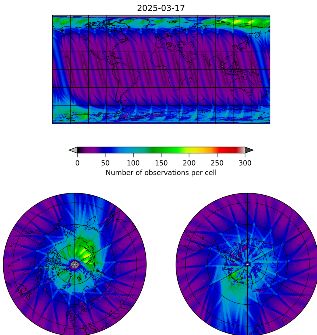
Figure 11: Map of the number of observations for 2025-03-17 to 2025-03-18
