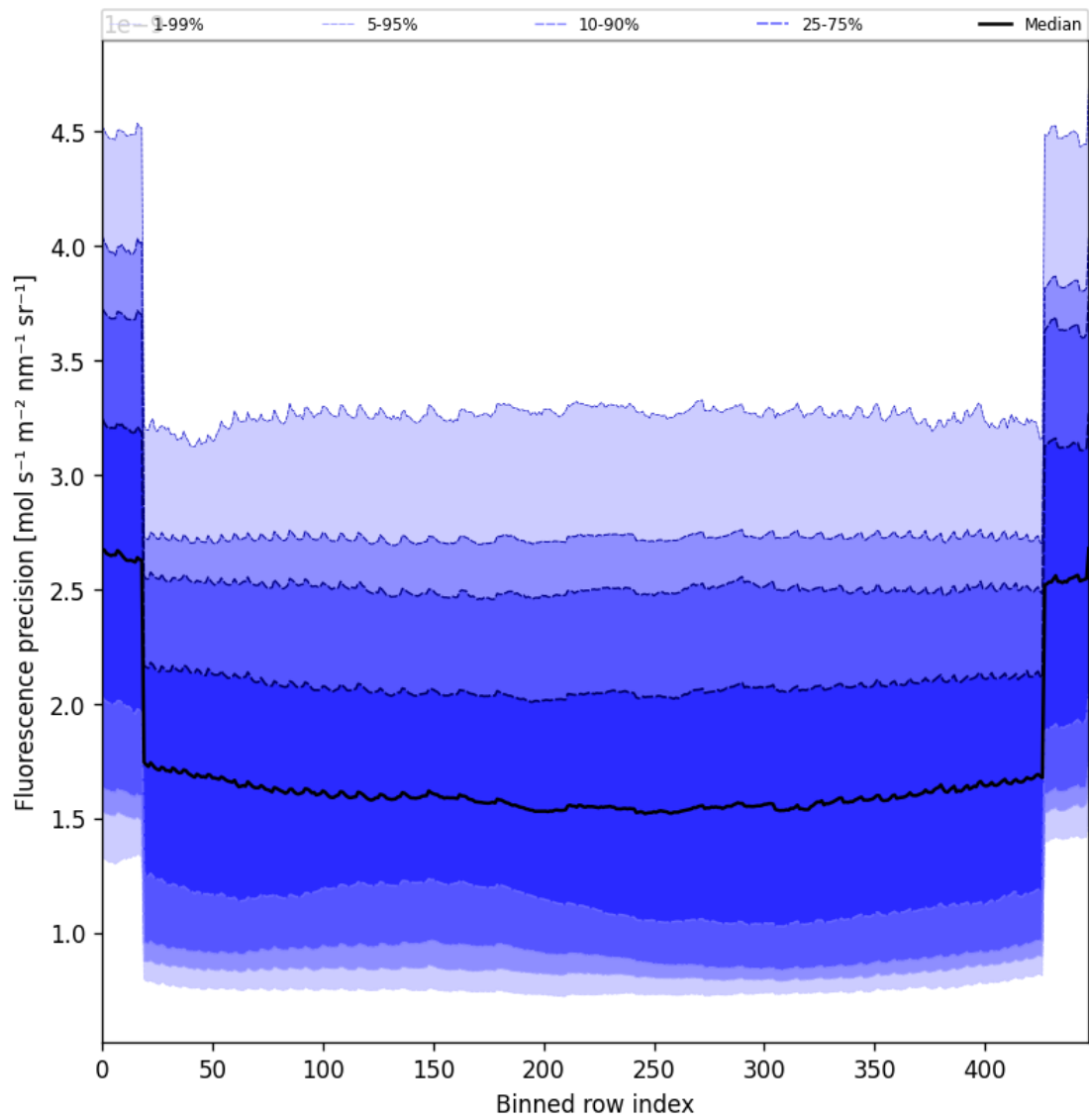
Figure 58: Along track statistics of “Fluorescence precision” for 2025-03-17 to 2025-03-18
