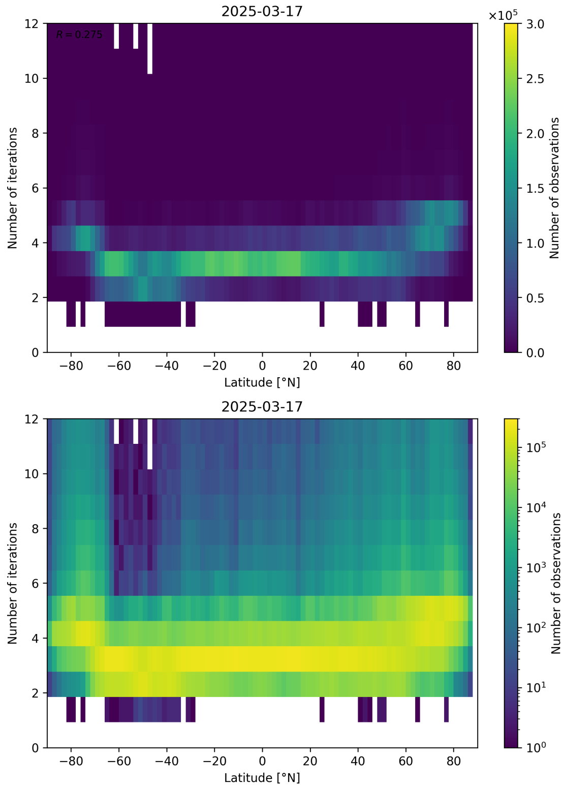
Figure 93: Scatter density plot of “Latitude” against “Number of iterations” for 2025-03-17 to 2025-03-18.
