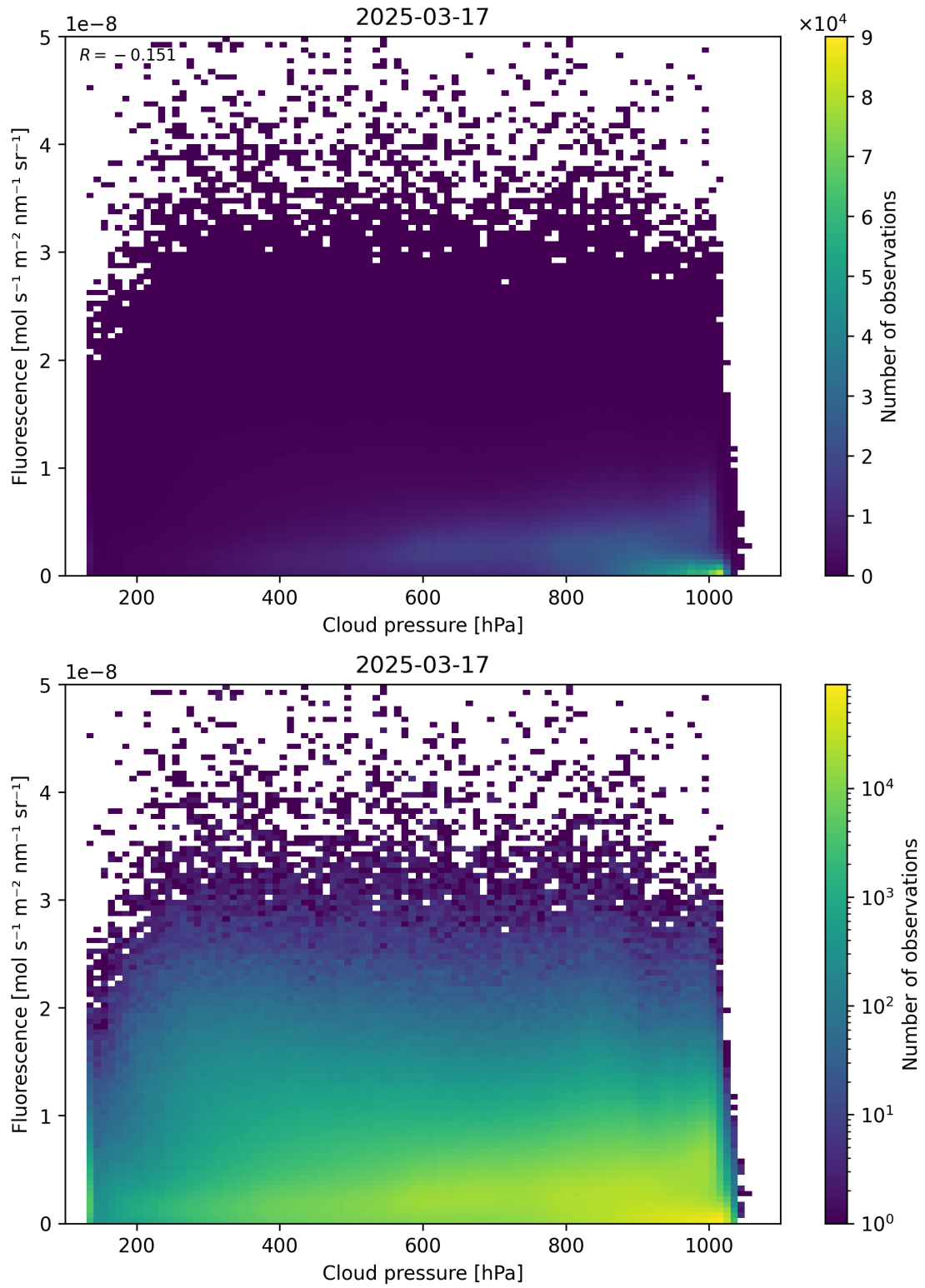
Figure 80: Scatter density plot of “Cloud pressure” against “Fluorescence” for 2025-03-17 to 2025-03-18.
