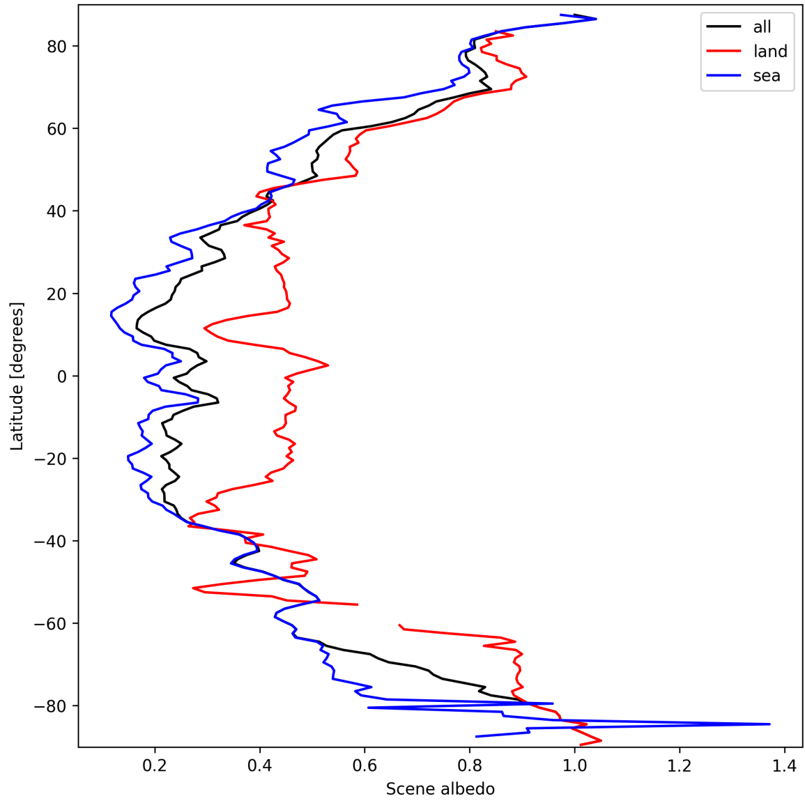
Figure 17: Zonal average of “Scene albedo” for 2025-03-17 to 2025-03-18.
