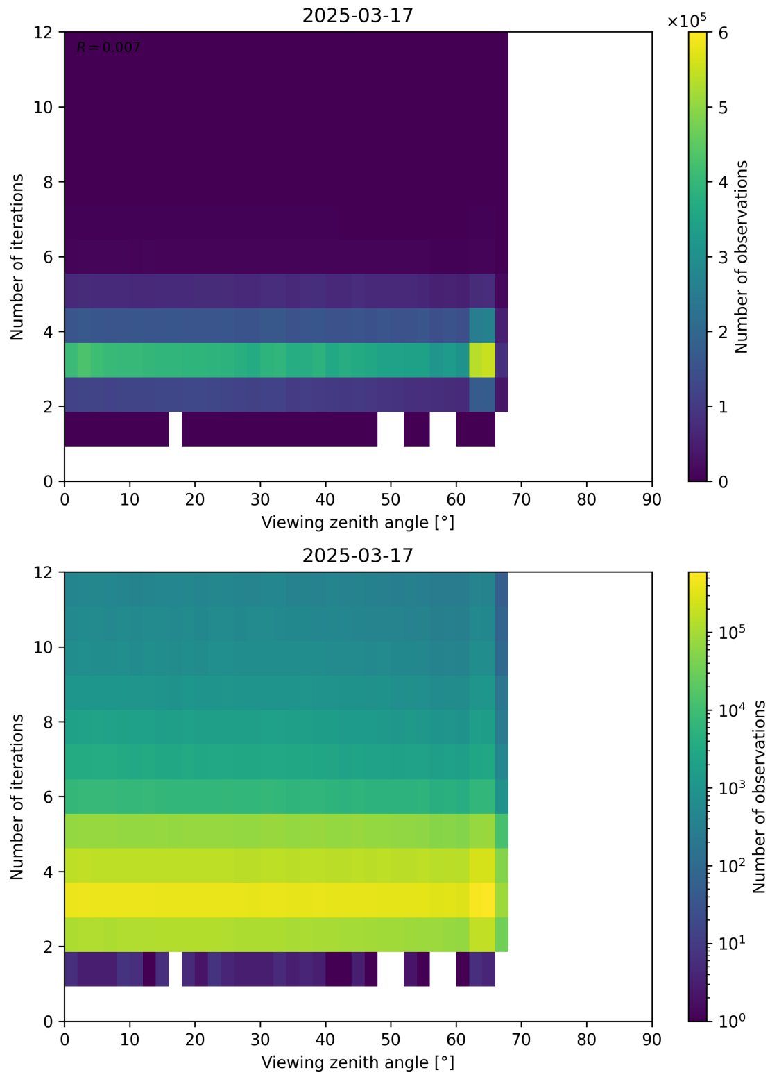
Figure 124: Scatter density plot of “Viewing zenith angle” against “Number of iterations” for 2025-03-17 to 2025-03-18.
