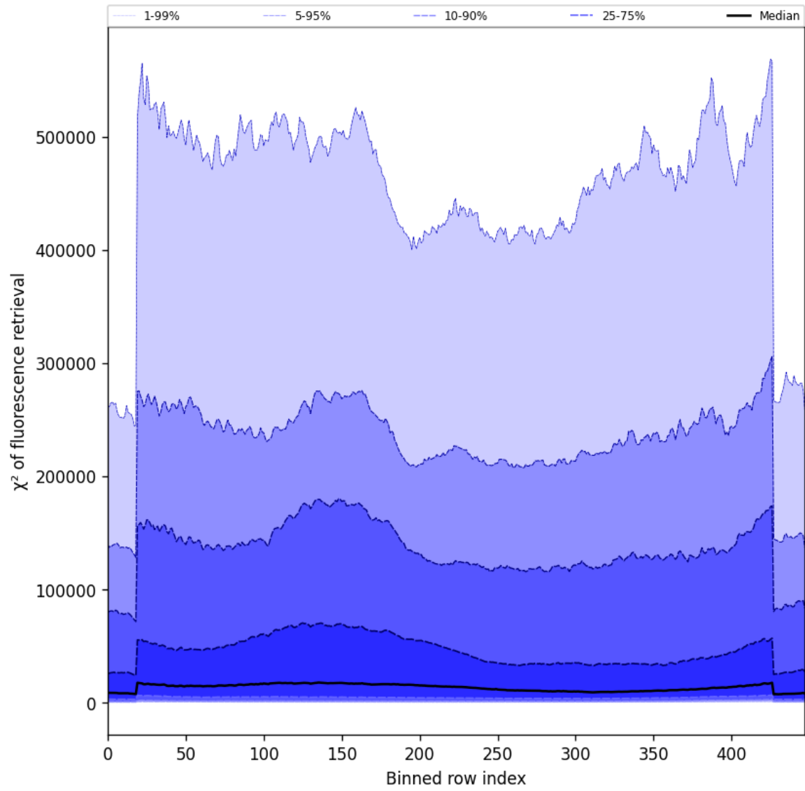
Figure 59: Along track statistics of “ \chi^2 of fluorescence retrieval” for 2025-03-17 to 2025-03-18
