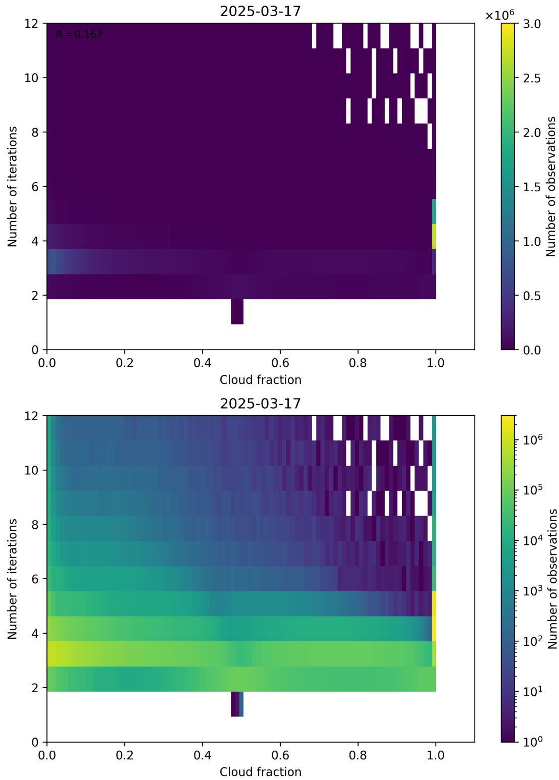
Figure 73: Scatter density plot of “Cloud fraction” against “Number of iterations” for 2025-03-17 to 2025-03-18.
