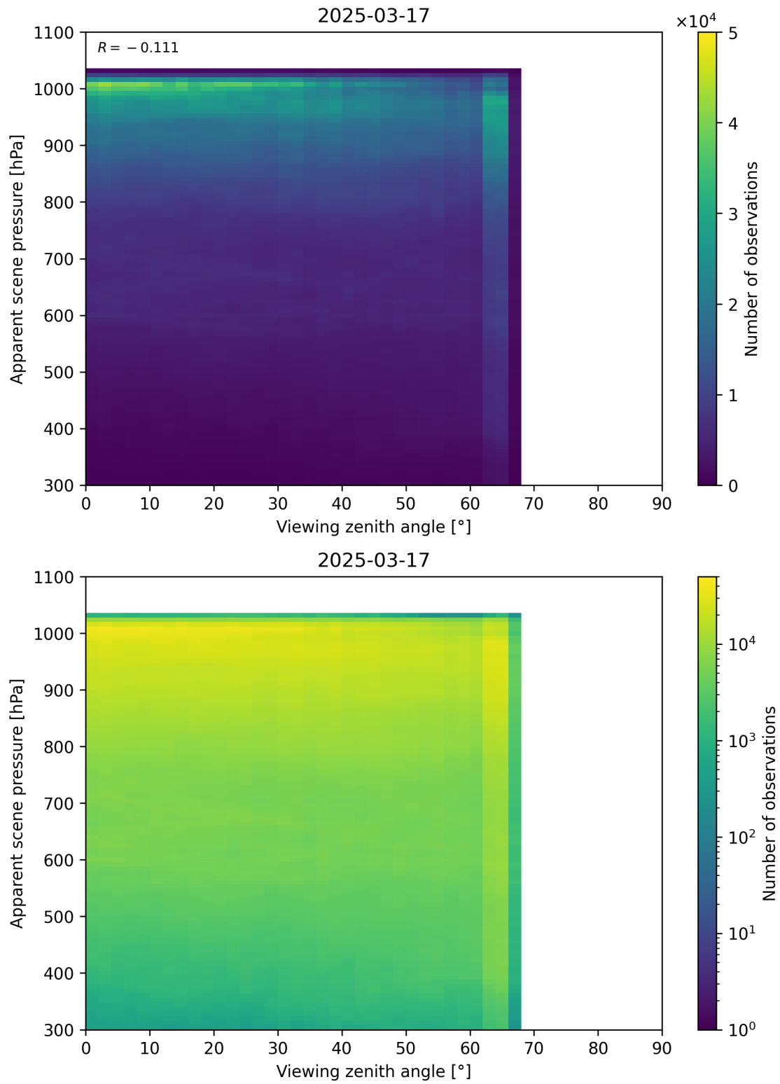
Figure 118: Scatter density plot of “Viewing zenith angle” against “Apparent scene pressure” for 2025-03-17 to 2025-03-18.
