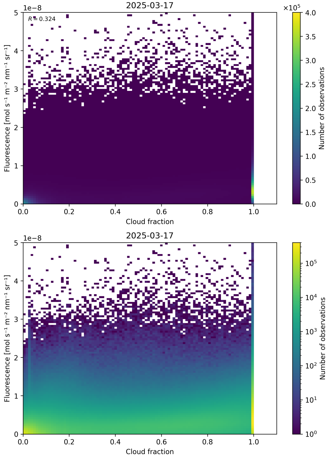
Figure 72: Scatter density plot of “Cloud fraction” against “Fluorescence” for 2025-03-17 to 2025-03-18.
