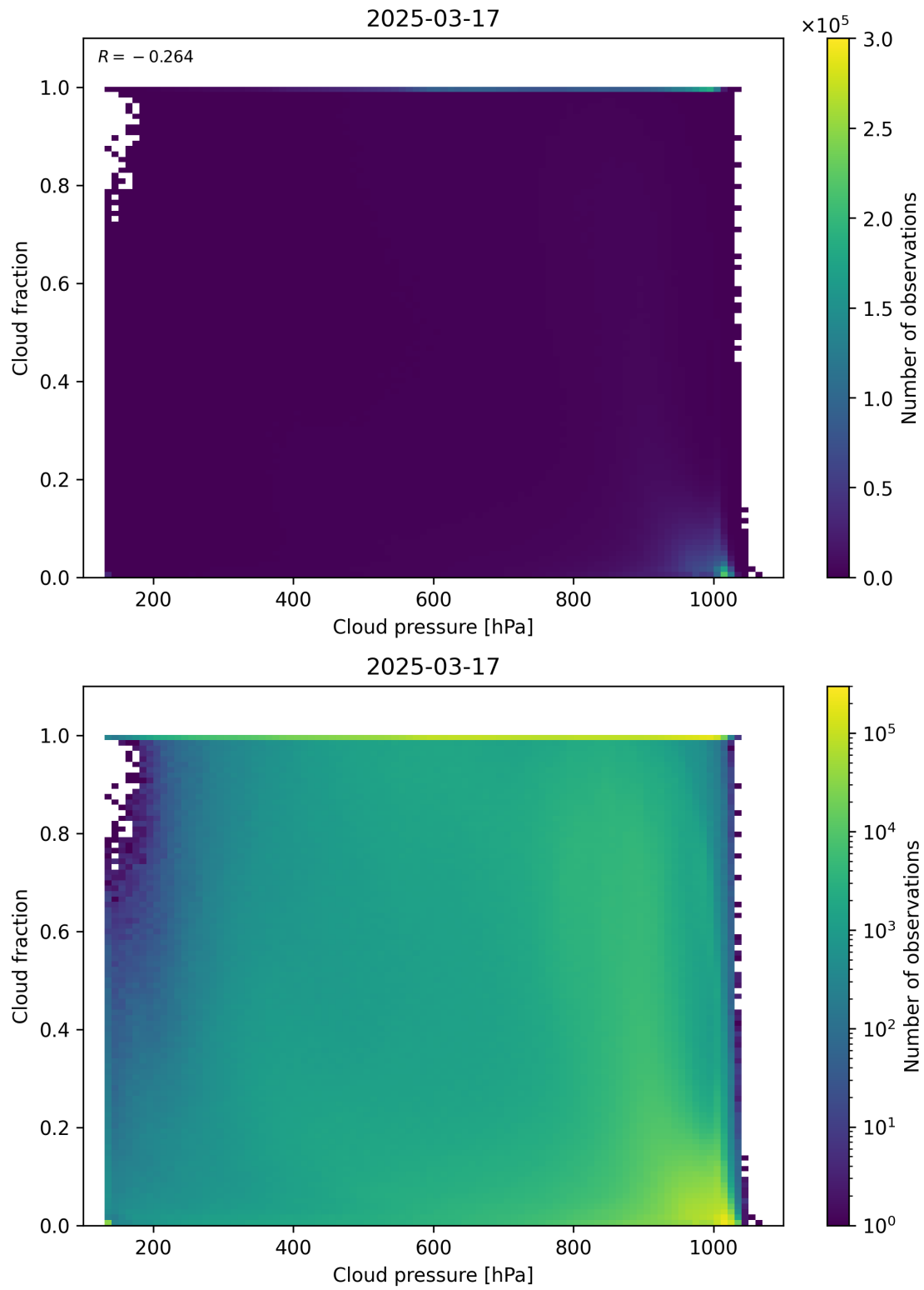
Figure 79: Scatter density plot of “Cloud pressure” against “Cloud fraction” for 2025-03-17 to 2025-03-18.
