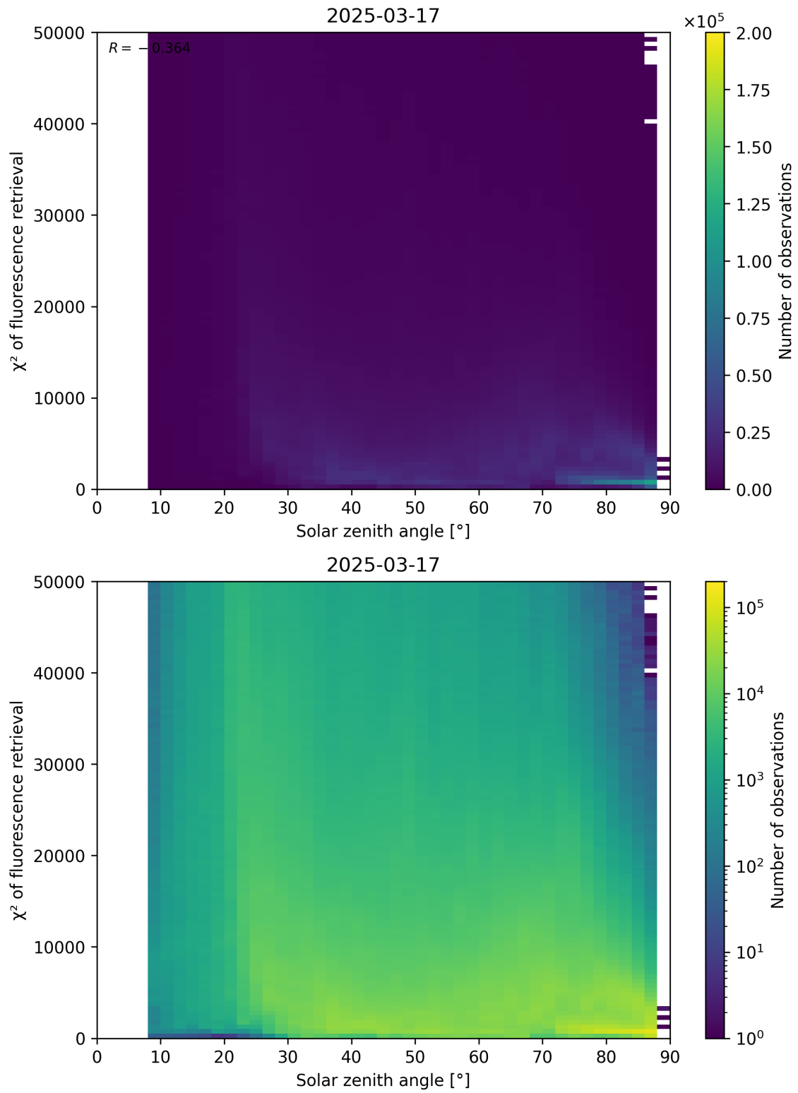
Figure 109: Scatter density plot of “Solar zenith angle” against “ \chi^2 of fluorescence retrieval” for 2025-03-17 to 2025-03-18.
