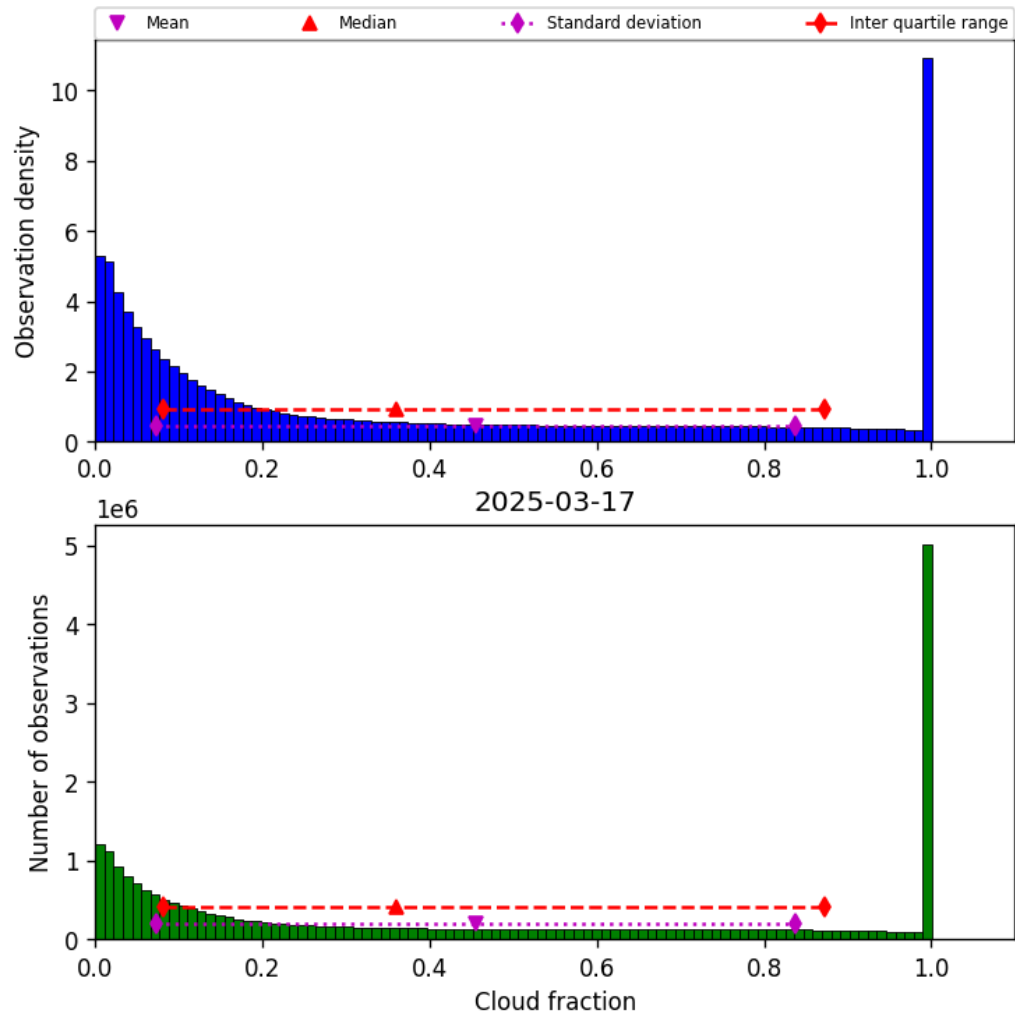
Figure 32: Histogram of “Cloud fraction” for 2025-03-17 to 2025-03-18
