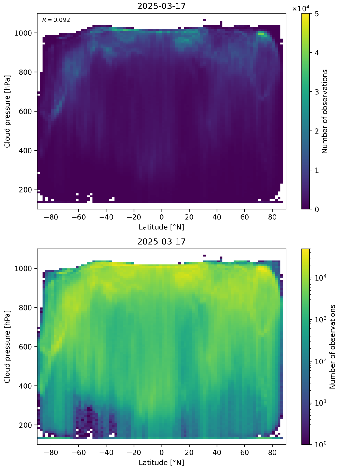
Figure 91: Scatter density plot of “Latitude” against “Cloud pressure” for 2025-03-17 to 2025-03-18.
