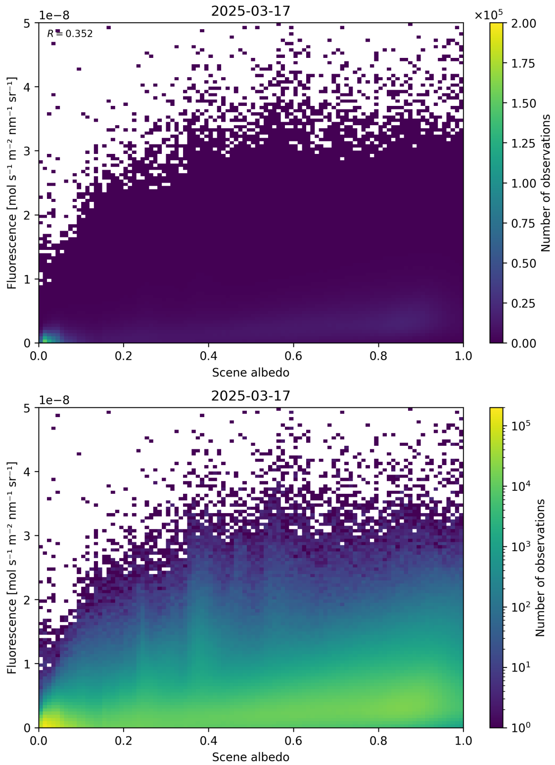
Figure 104: Scatter density plot of “Scene albedo” against “Fluorescence” for 2025-03-17 to 2025-03-18.
