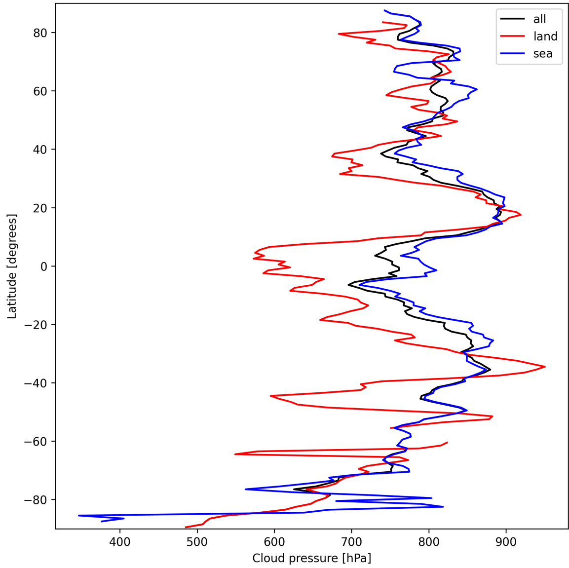
Figure 13: Zonal average of “Cloud pressure” for 2025-03-17 to 2025-03-18.
