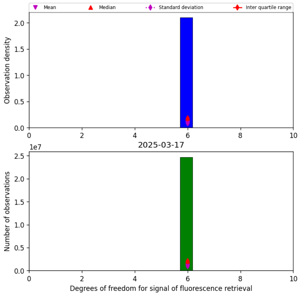
Figure 43: Histogram of “Degrees of freedom for signal of fluorescence retrieval” for 2025-03-17 to 2025-03-18
