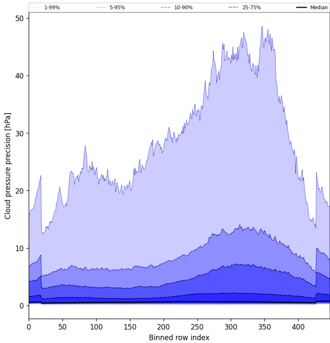
Figure 48: Along track statistics of “Cloud pressure precision” for 2025-03-17 to 2025-03-18
