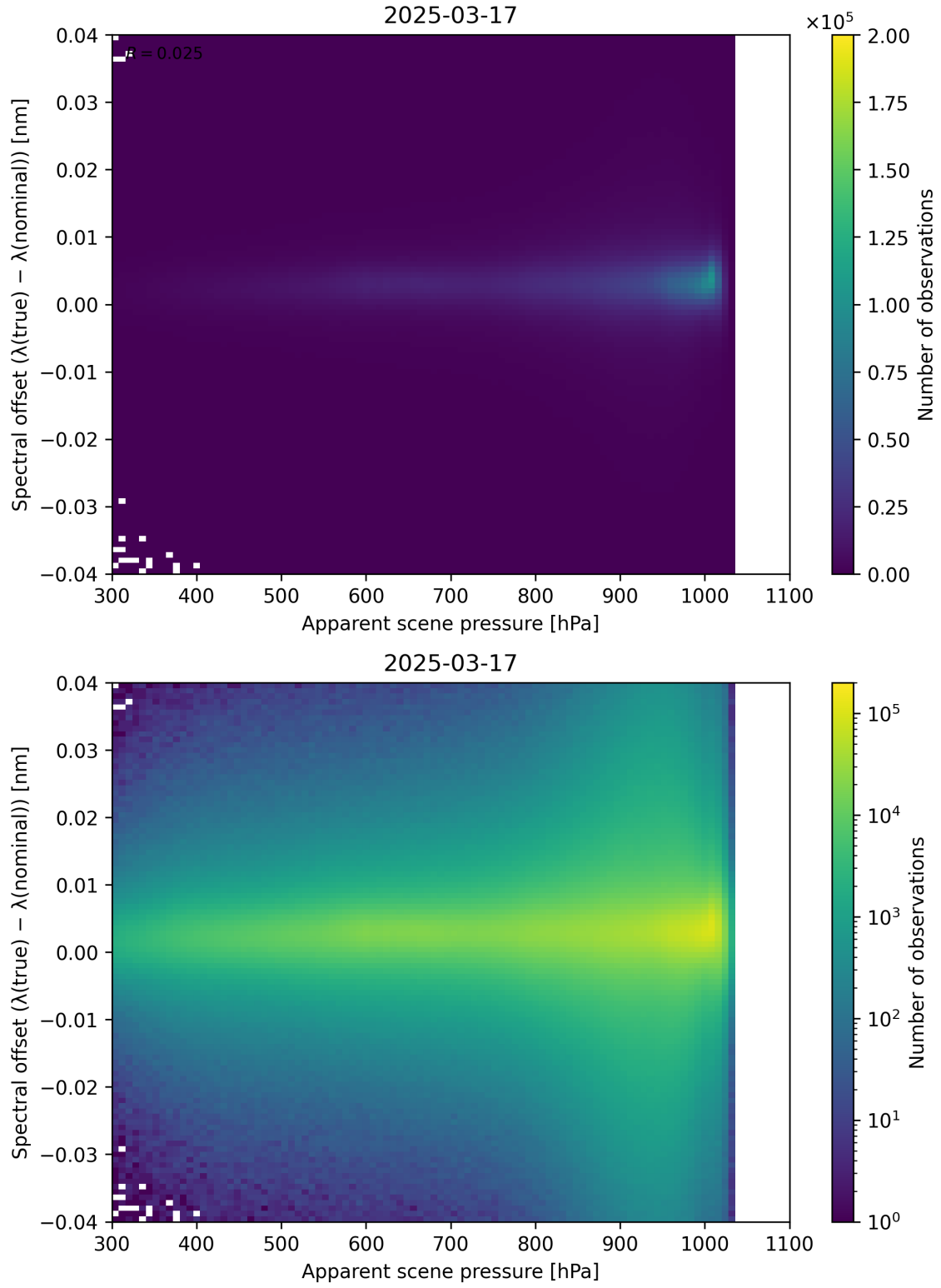
Figure 67: Scatter density plot of “Apparent scene pressure” against “Spectral offset ( \lambda_{\text{true}} - \lambda_{\text{nominal}} )” for 2025-03-17 to 2025-03-18.
