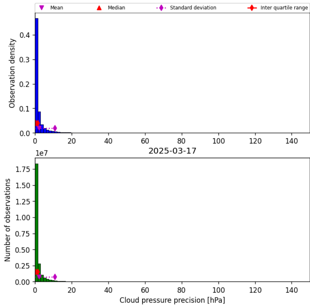
Figure 31: Histogram of “Cloud pressure precision” for 2025-03-17 to 2025-03-18
