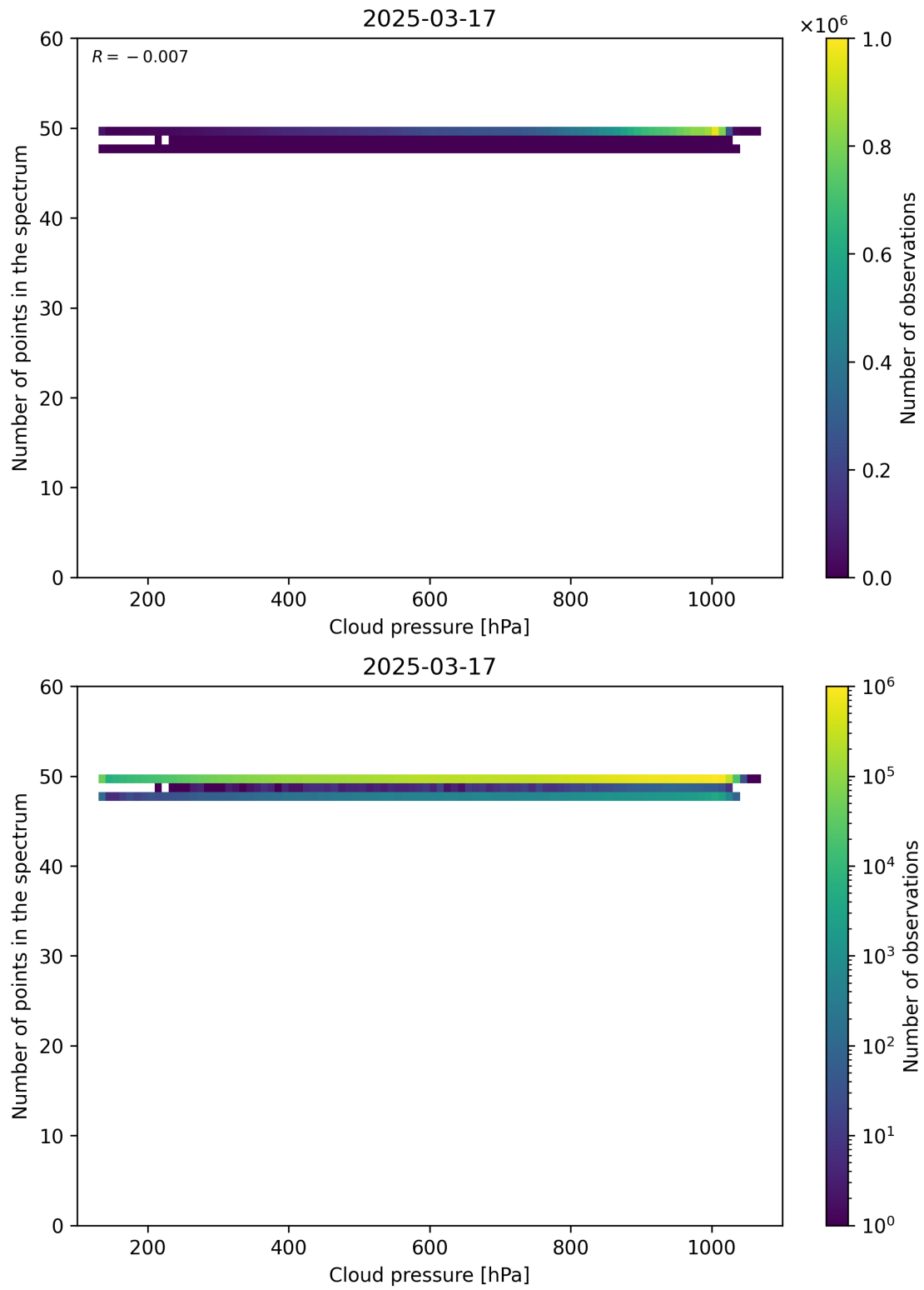
Figure 82: Scatter density plot of “Cloud pressure” against “Number of points in the spectrum” for 2025-03-17 to 2025-03-18.
