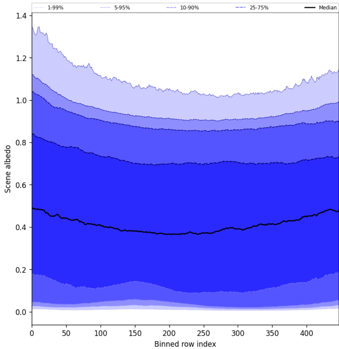
Figure 51: Along track statistics of “Scene albedo” for 2025-03-17 to 2025-03-18
