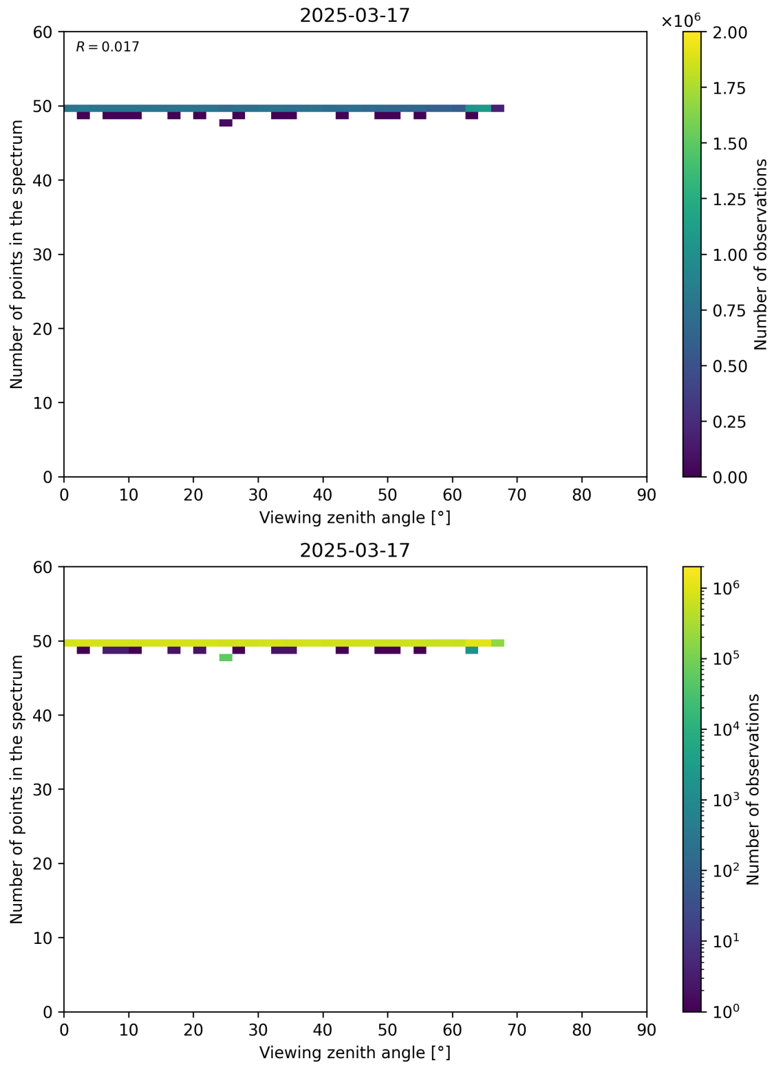
Figure 125: Scatter density plot of “Viewing zenith angle” against “Number of points in the spectrum” for 2025-03-17 to 2025-03-18.
