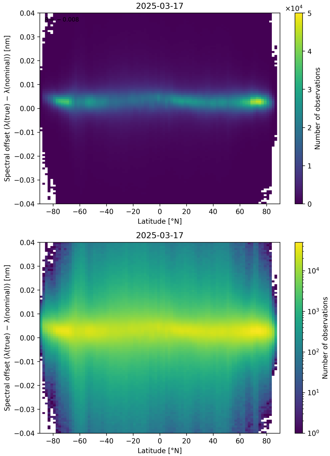
Figure 96: Scatter density plot of “Latitude” against “Spectral offset ( \lambda_{\text{true}} - \lambda_{\text{nominal}} )” for 2025-03-17 to 2025-03-18.
