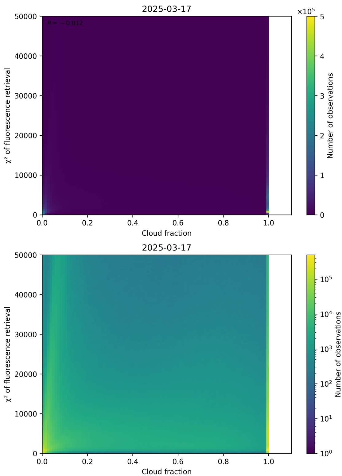
Figure 71: Scatter density plot of “Cloud fraction” against “ \chi^2 of fluorescence retrieval” for 2025-03-17 to 2025-03-18.
