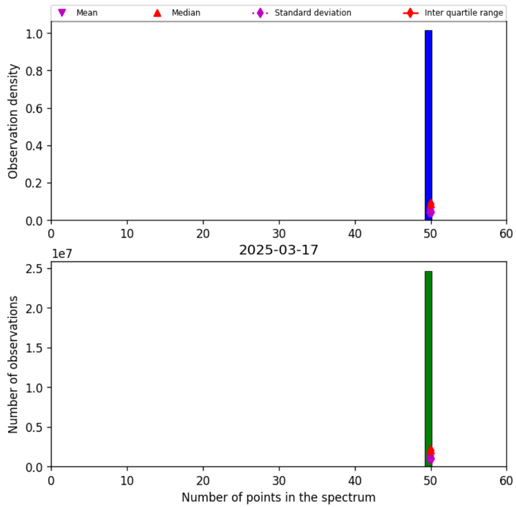
Figure 44: Histogram of “Number of points in the spectrum” for 2025-03-17 to 2025-03-18
