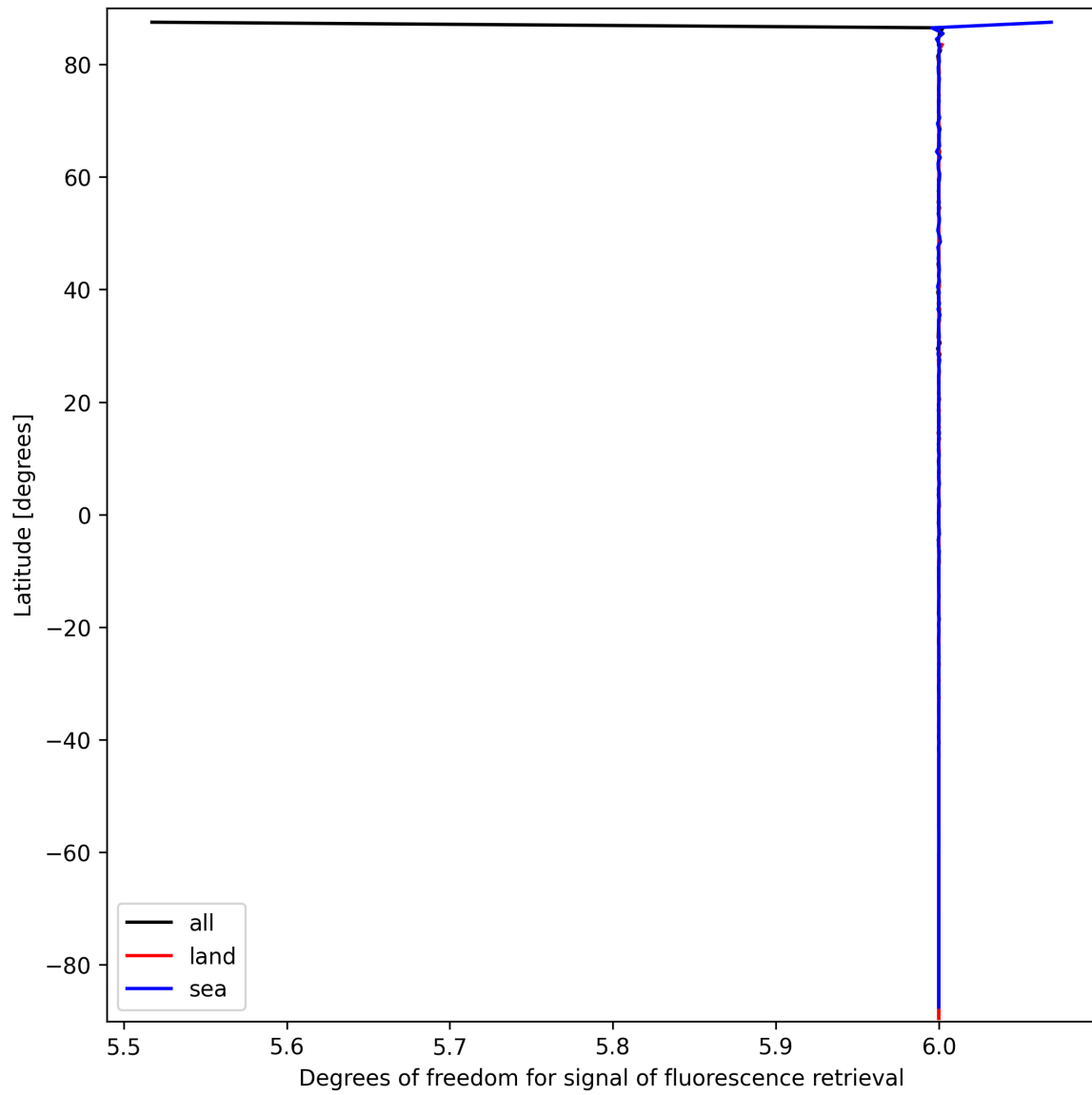
Figure 26: Zonal average of “Degrees of freedom for signal of fluorescence retrieval” for 2025-03-17 to 2025-03-18.
