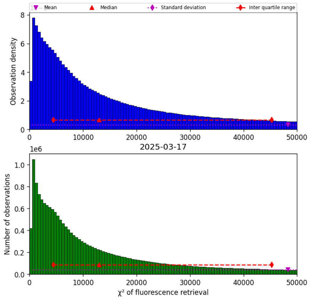
Figure 42: Histogram of “ \chi^2 of fluorescence retrieval” for 2025-03-17 to 2025-03-18
