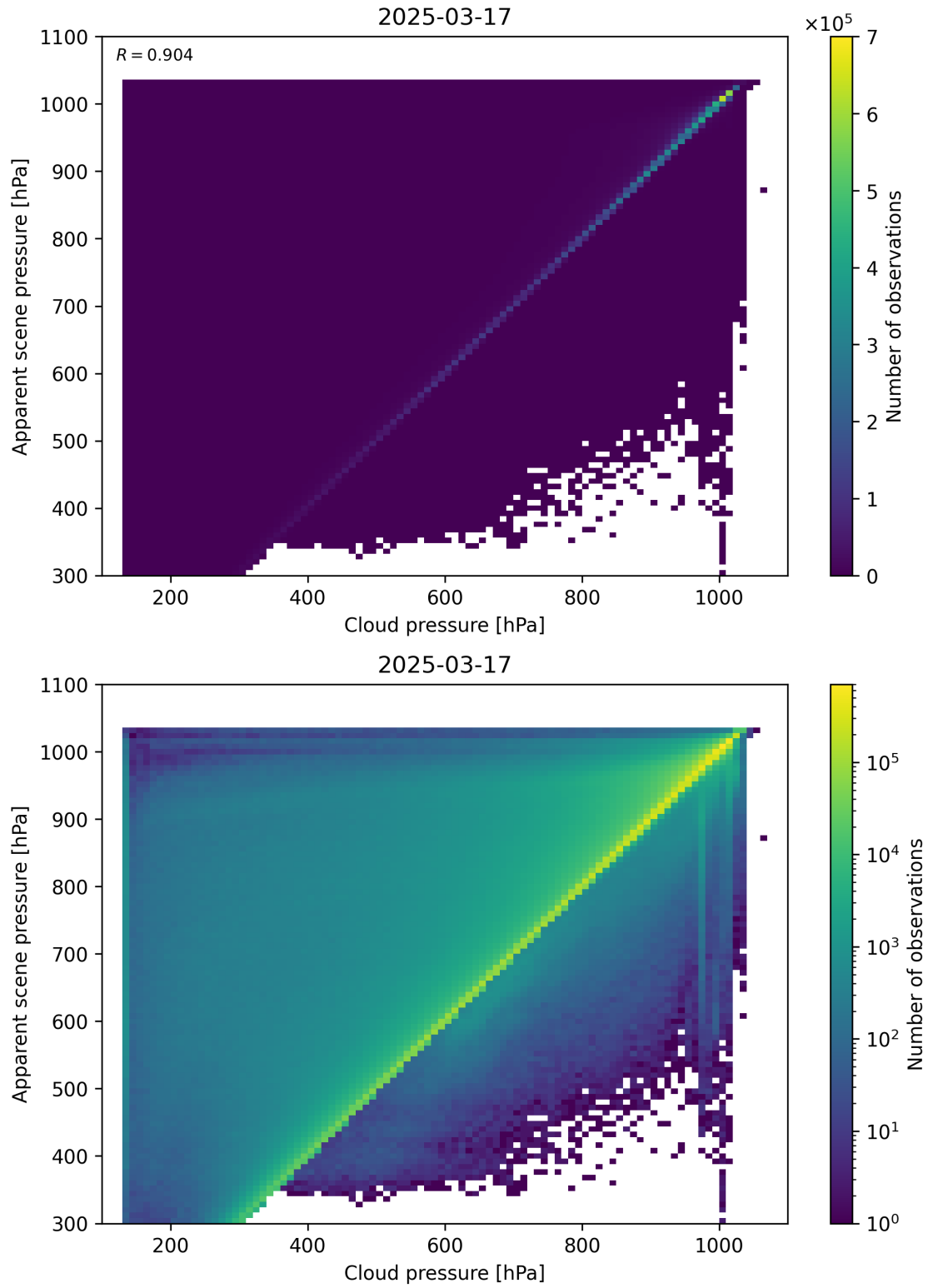
Figure 77: Scatter density plot of “Cloud pressure” against “Apparent scene pressure” for 2025-03-17 to 2025-03-18.
