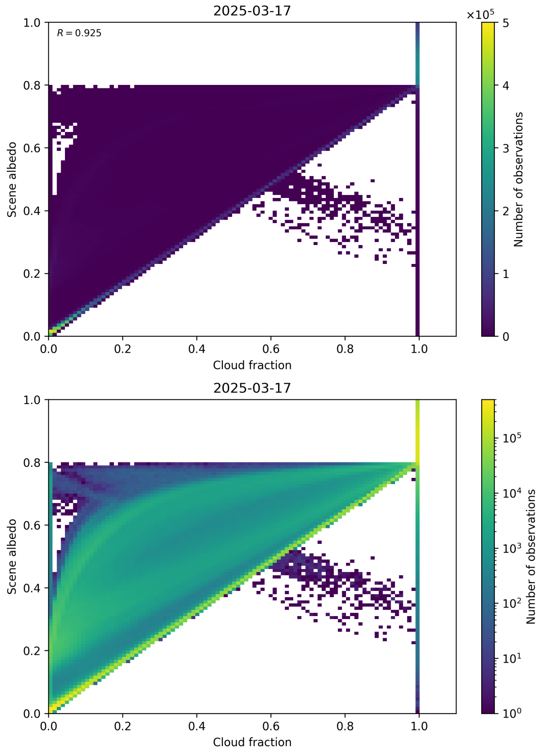
Figure 75: Scatter density plot of “Cloud fraction” against “Scene albedo” for 2025-03-17 to 2025-03-18.
