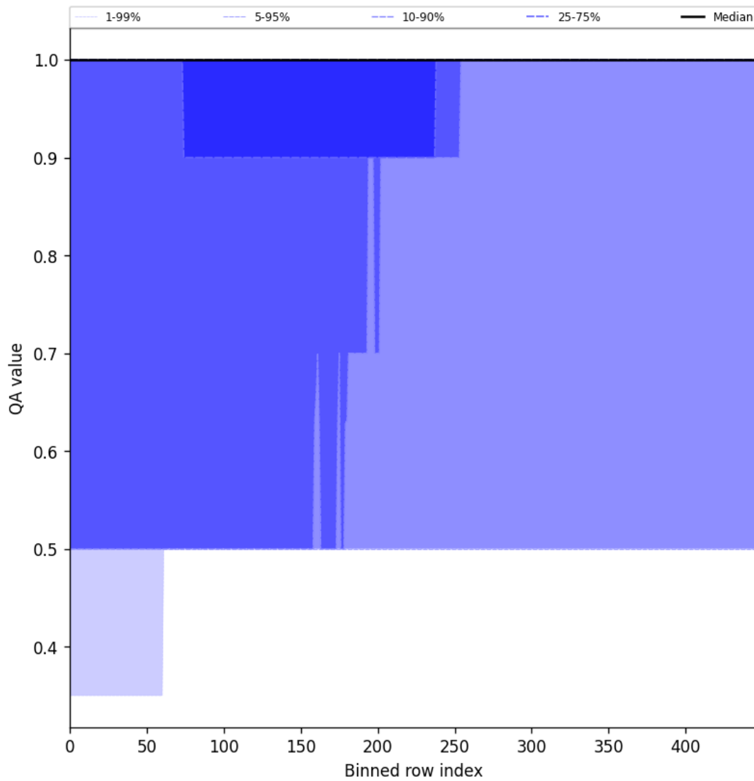
Figure 46: Along track statistics of “QA value” for 2025-03-17 to 2025-03-18
