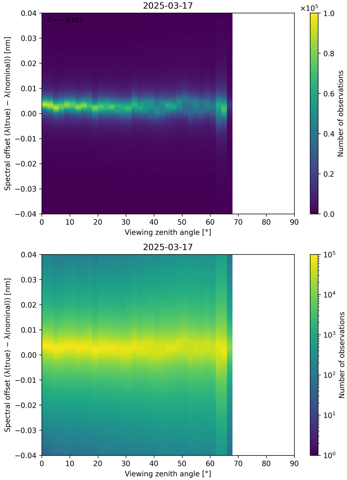
Figure 128: Scatter density plot of “Viewing zenith angle” against “Spectral offset ( \lambda_{\text{true}} - \lambda_{\text{nominal}} )” for 2025-03-17 to 2025-03-18.
