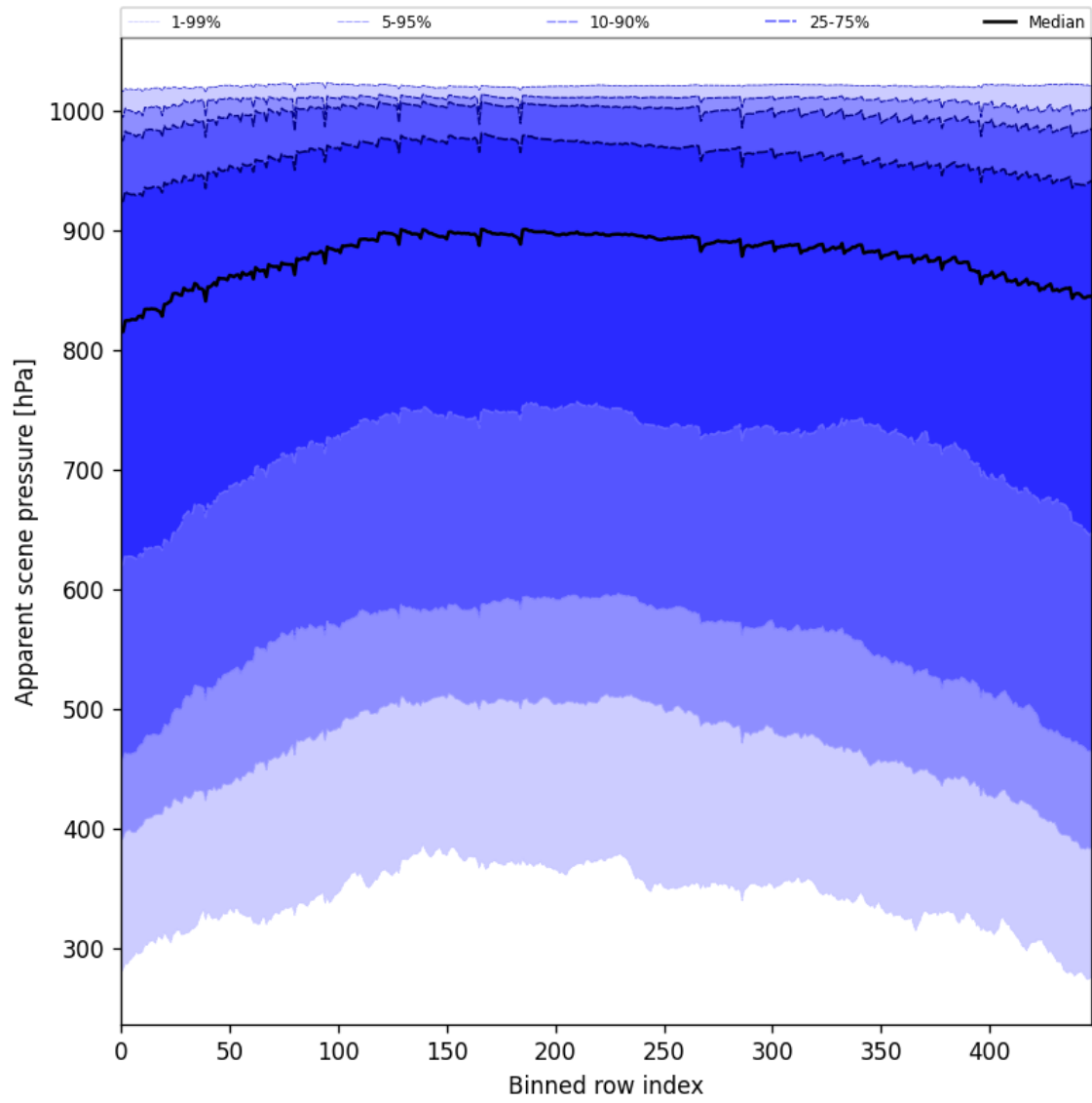
Figure 53: Along track statistics of “Apparent scene pressure” for 2025-03-17 to 2025-03-18
