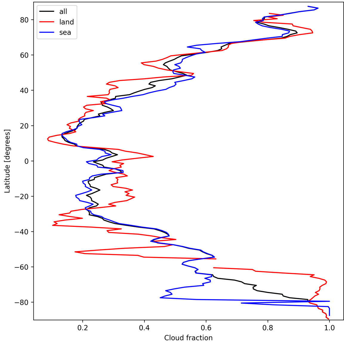
Figure 15: Zonal average of “Cloud fraction” for 2025-03-17 to 2025-03-18.
