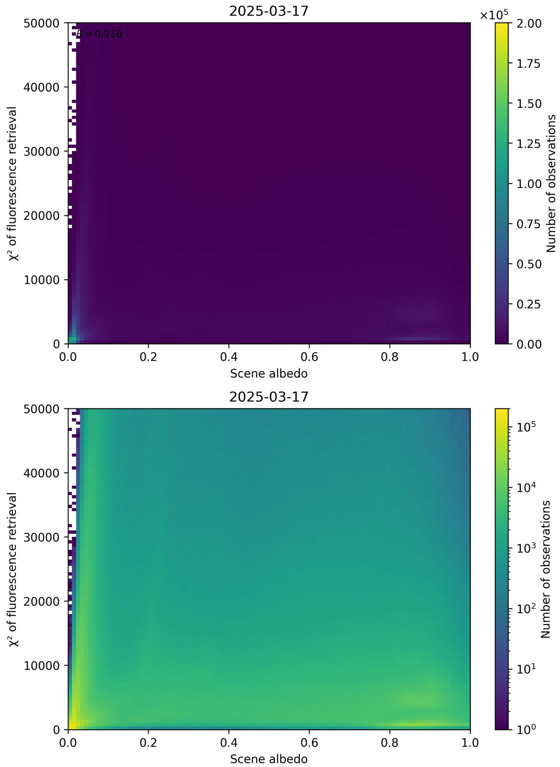
Figure 103: Scatter density plot of “Scene albedo” against “ \chi^2 of fluorescence retrieval” for 2025-03-17 to 2025-03-18.
