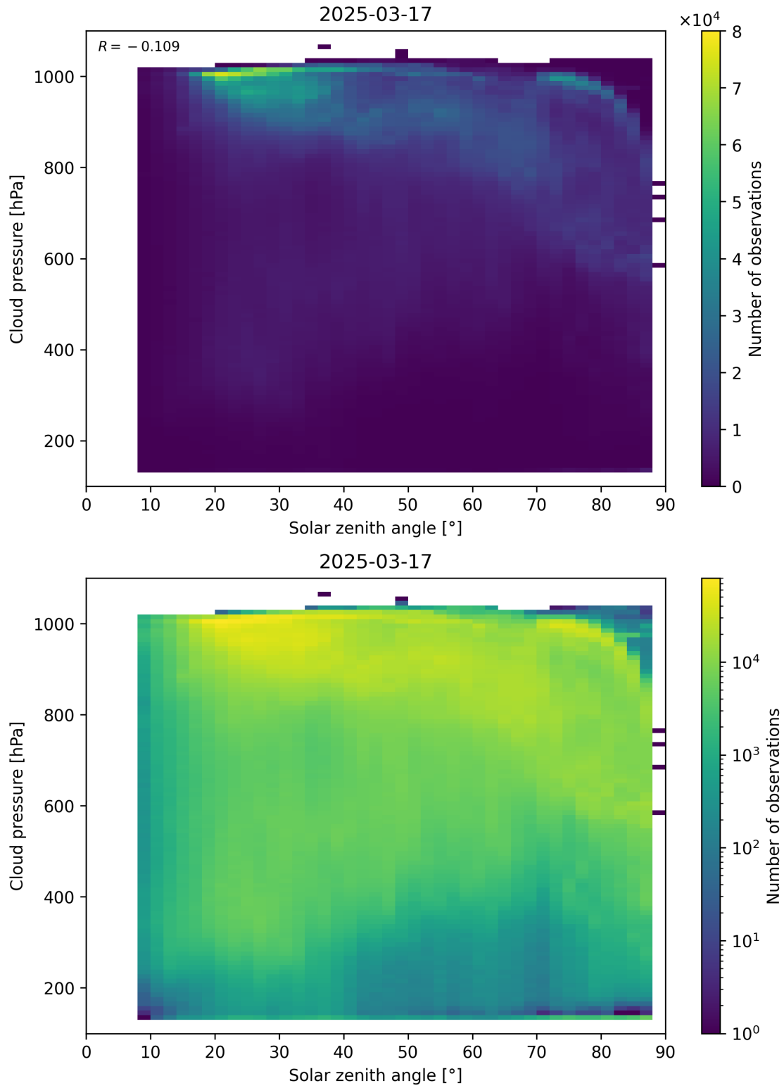
Figure 111: Scatter density plot of “Solar zenith angle” against “Cloud pressure” for 2025-03-17 to 2025-03-18.
