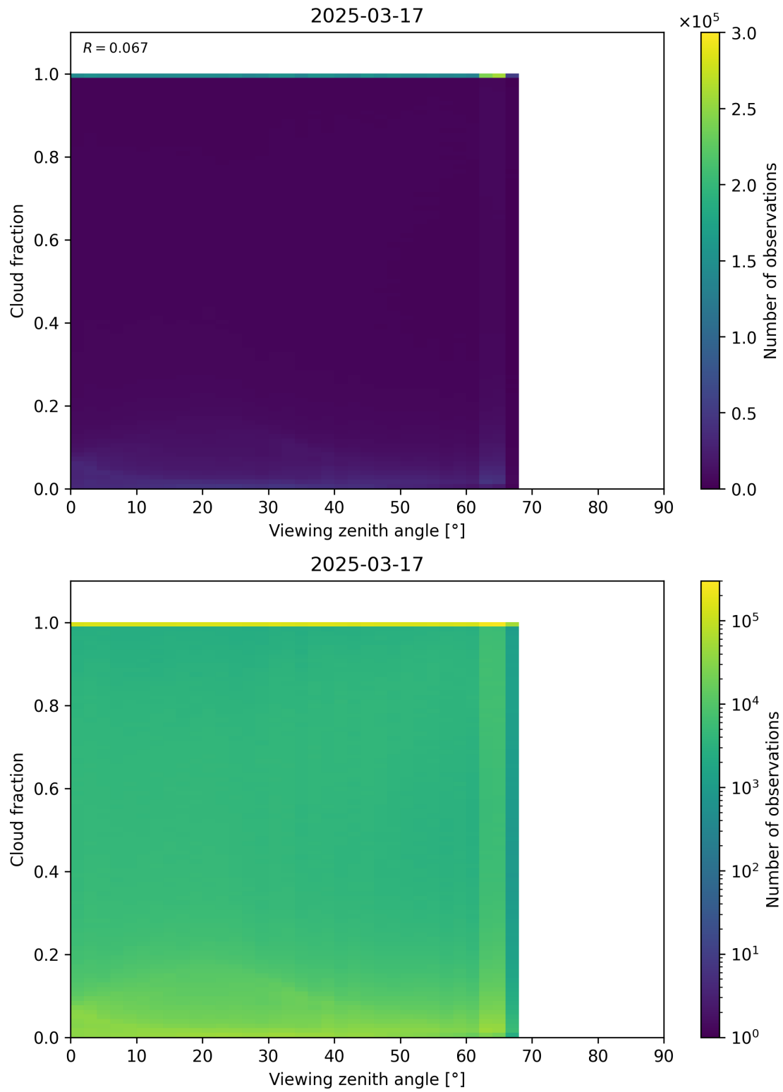
Figure 120: Scatter density plot of “Viewing zenith angle” against “Cloud fraction” for 2025-03-17 to 2025-03-18.
