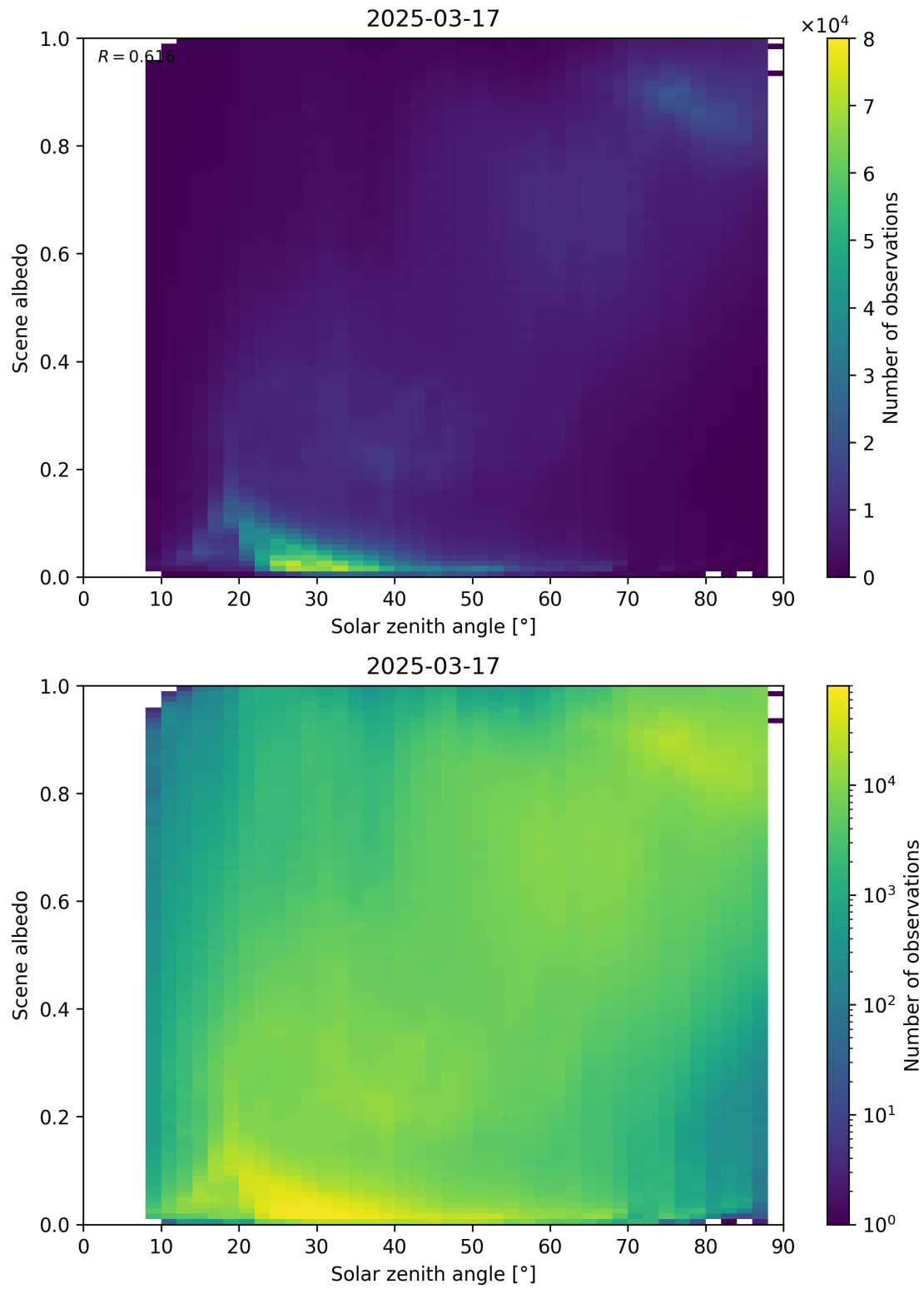
Figure 116: Scatter density plot of “Solar zenith angle” against “Scene albedo” for 2025-03-17 to 2025-03-18.
