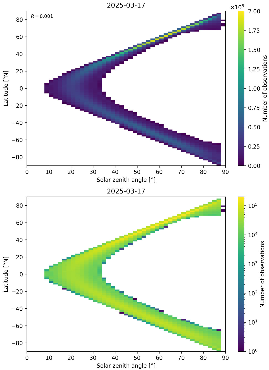
Figure 113: Scatter density plot of “Solar zenith angle” against “Latitude” for 2025-03-17 to 2025-03-18.
