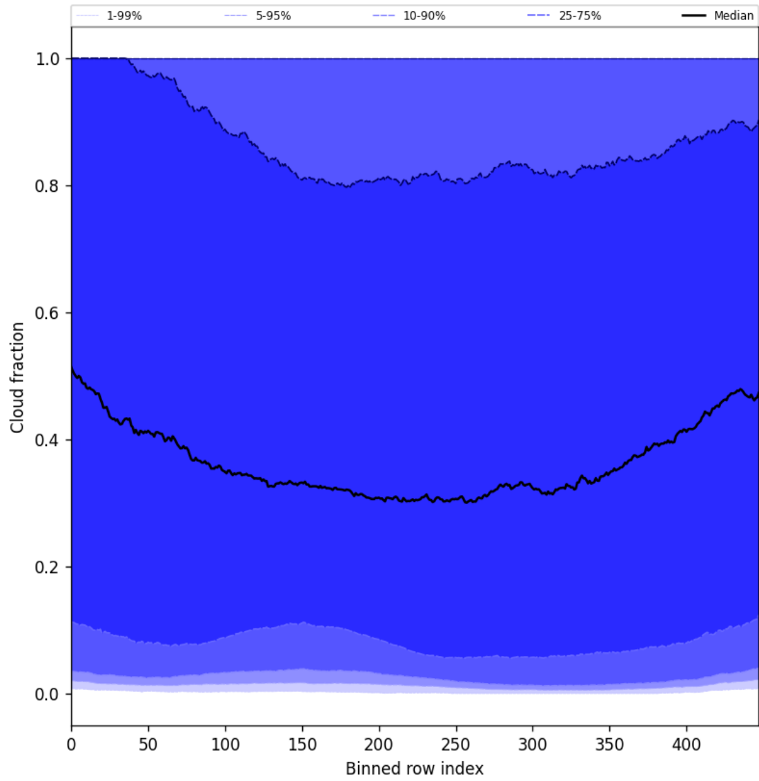
Figure 49: Along track statistics of “Cloud fraction” for 2025-03-17 to 2025-03-18
