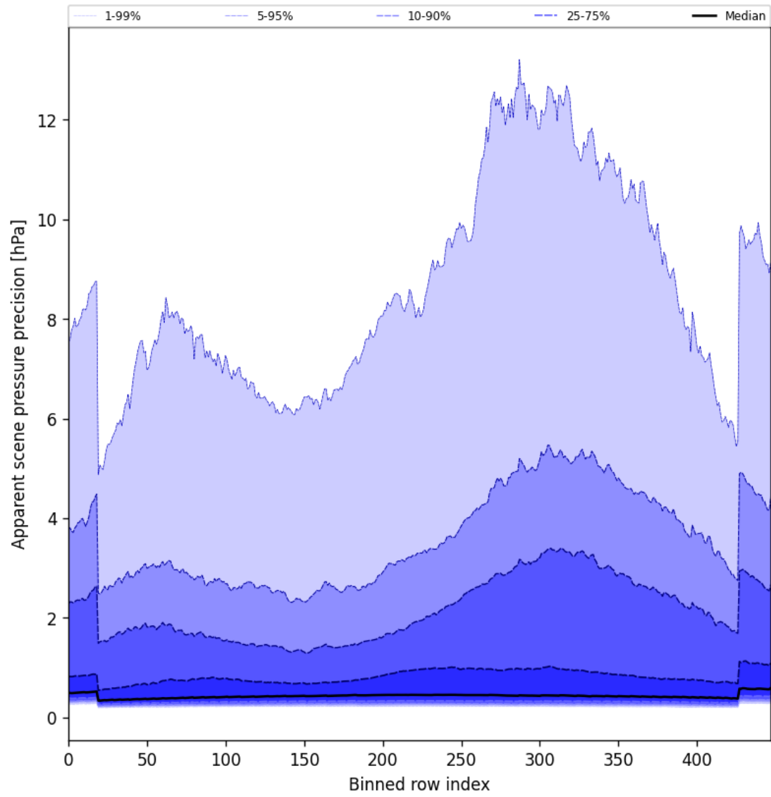
Figure 54: Along track statistics of “Apparent scene pressure precision” for 2025-03-17 to 2025-03-18
