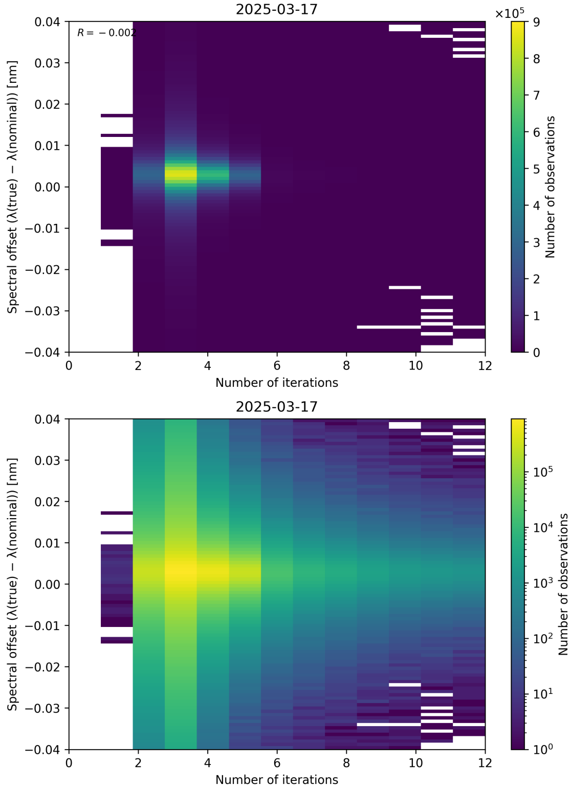
Figure 100: Scatter density plot of “Number of iterations” against “Spectral offset ( \lambda_{\text{true}} - \lambda_{\text{nominal}} )” for 2025-03-17 to 2025-03-18.
