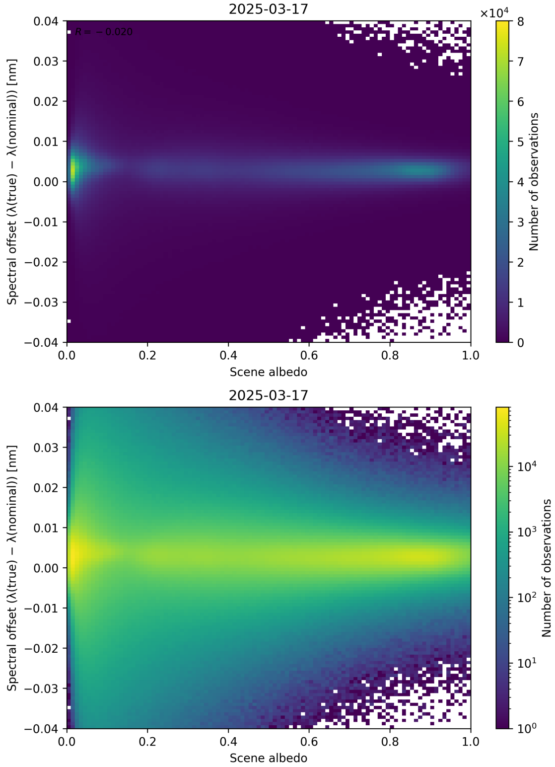
Figure 107: Scatter density plot of “Scene albedo” against “Spectral offset ( \lambda_{\text{true}} - \lambda_{\text{nominal}} )” for 2025-03-17 to 2025-03-18.
