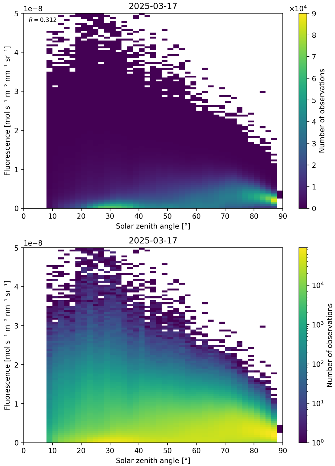
Figure 112: Scatter density plot of “Solar zenith angle” against “Fluorescence” for 2025-03-17 to 2025-03-18.
