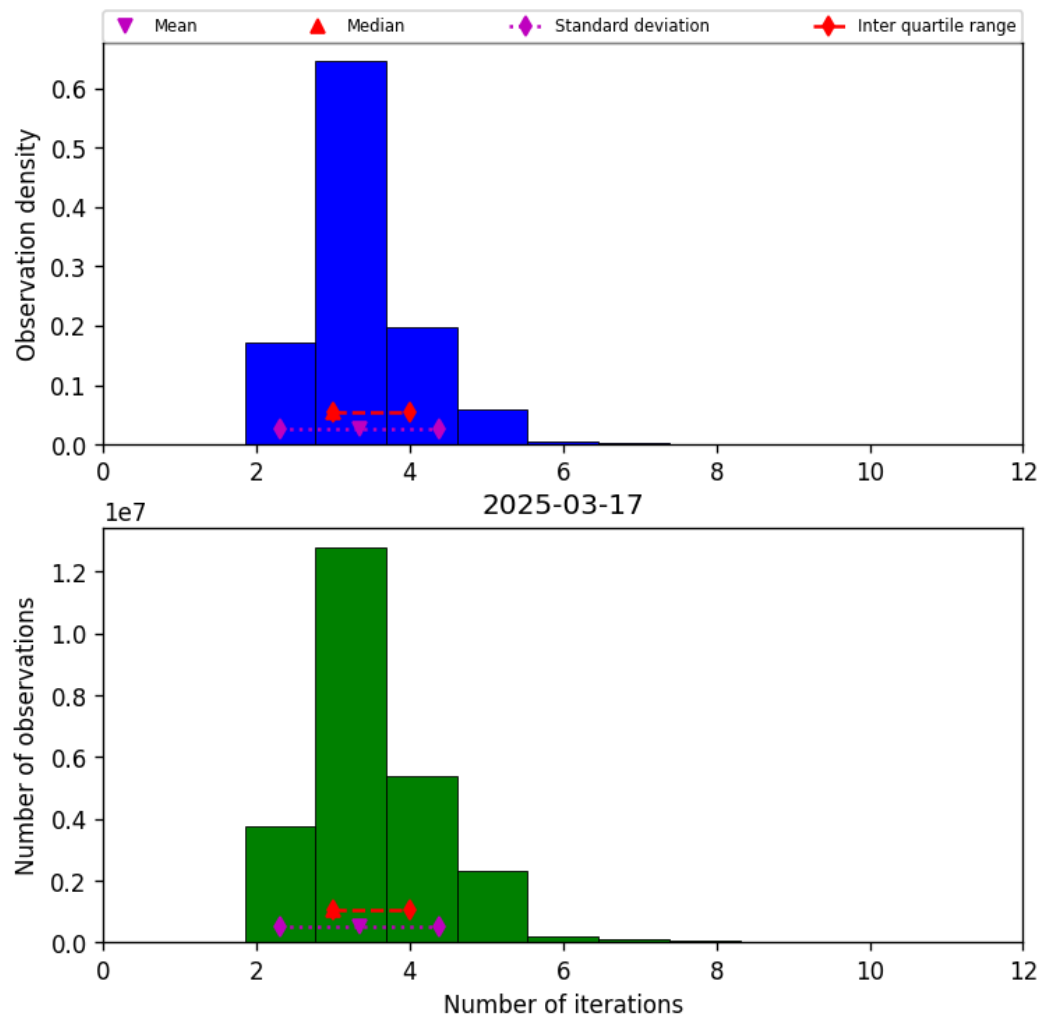
Figure 39: Histogram of “Number of iterations” for 2025-03-17 to 2025-03-18
