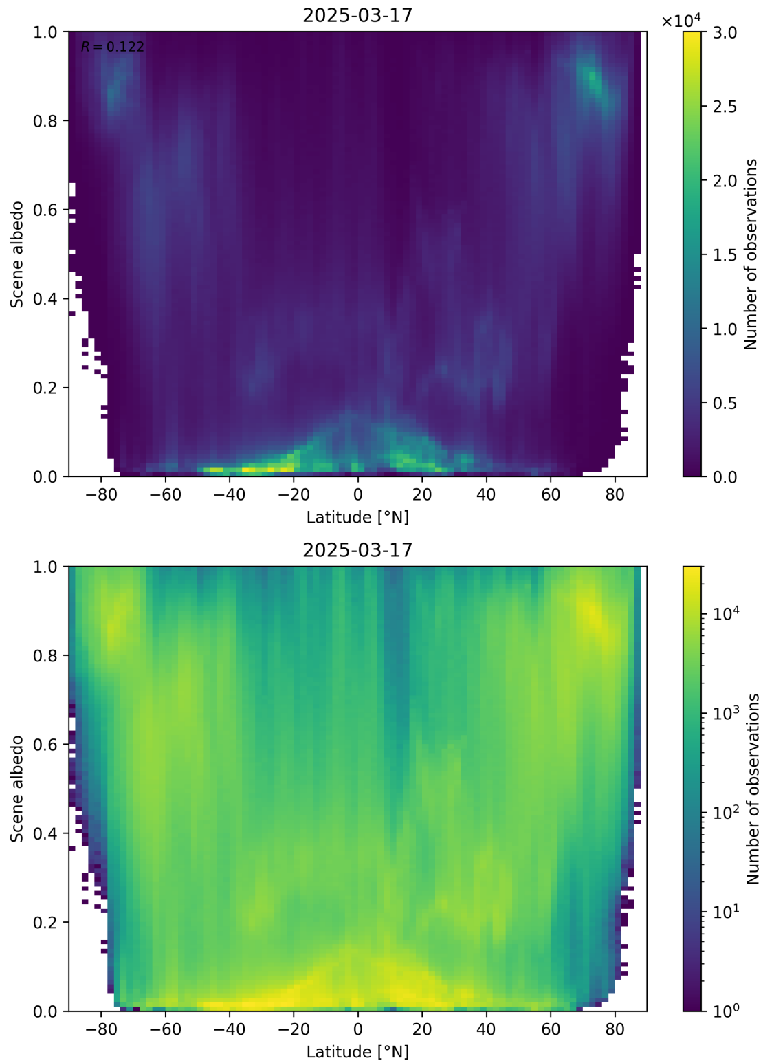
Figure 95: Scatter density plot of “Latitude” against “Scene albedo” for 2025-03-17 to 2025-03-18.
