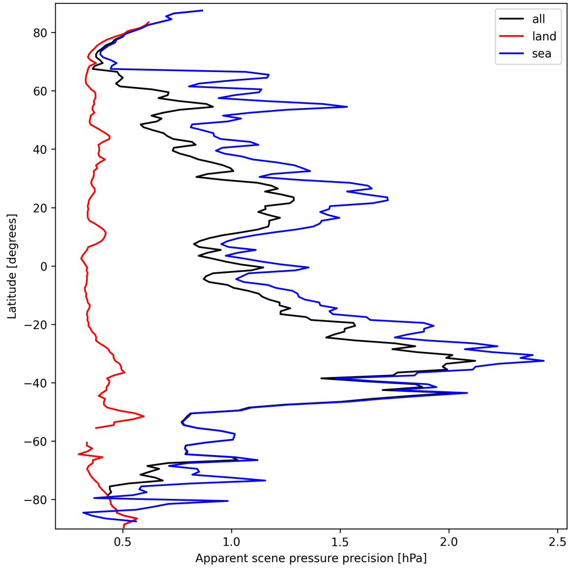
Figure 20: Zonal average of “Apparent scene pressure precision” for 2025-03-17 to 2025-03-18.
