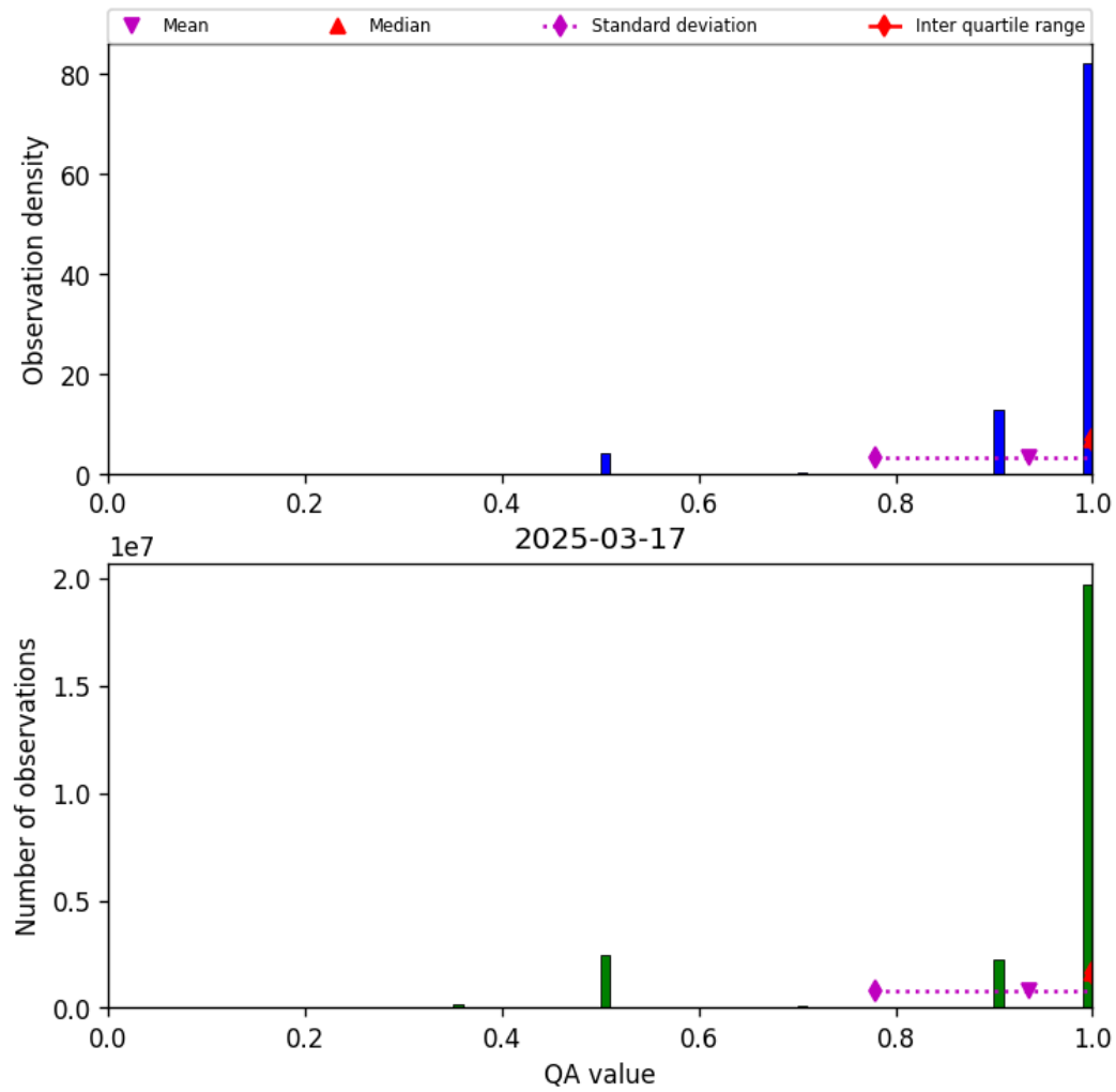
Figure 29: Histogram of “QA value” for 2025-03-17 to 2025-03-18
