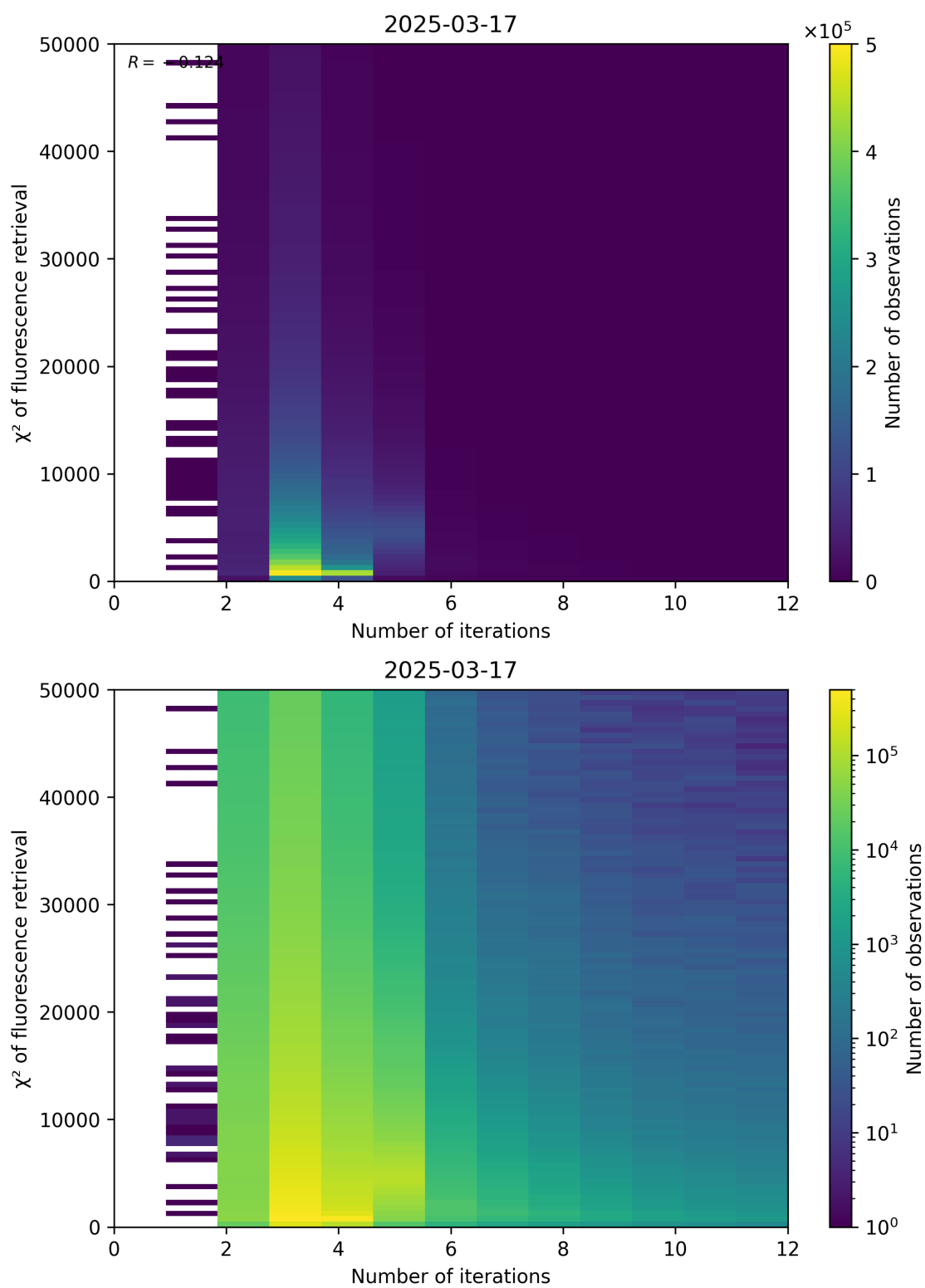
Figure 97: Scatter density plot of “Number of iterations” against “ \chi^2 of fluorescence retrieval” for 2025-03-17 to 2025-03-18.
