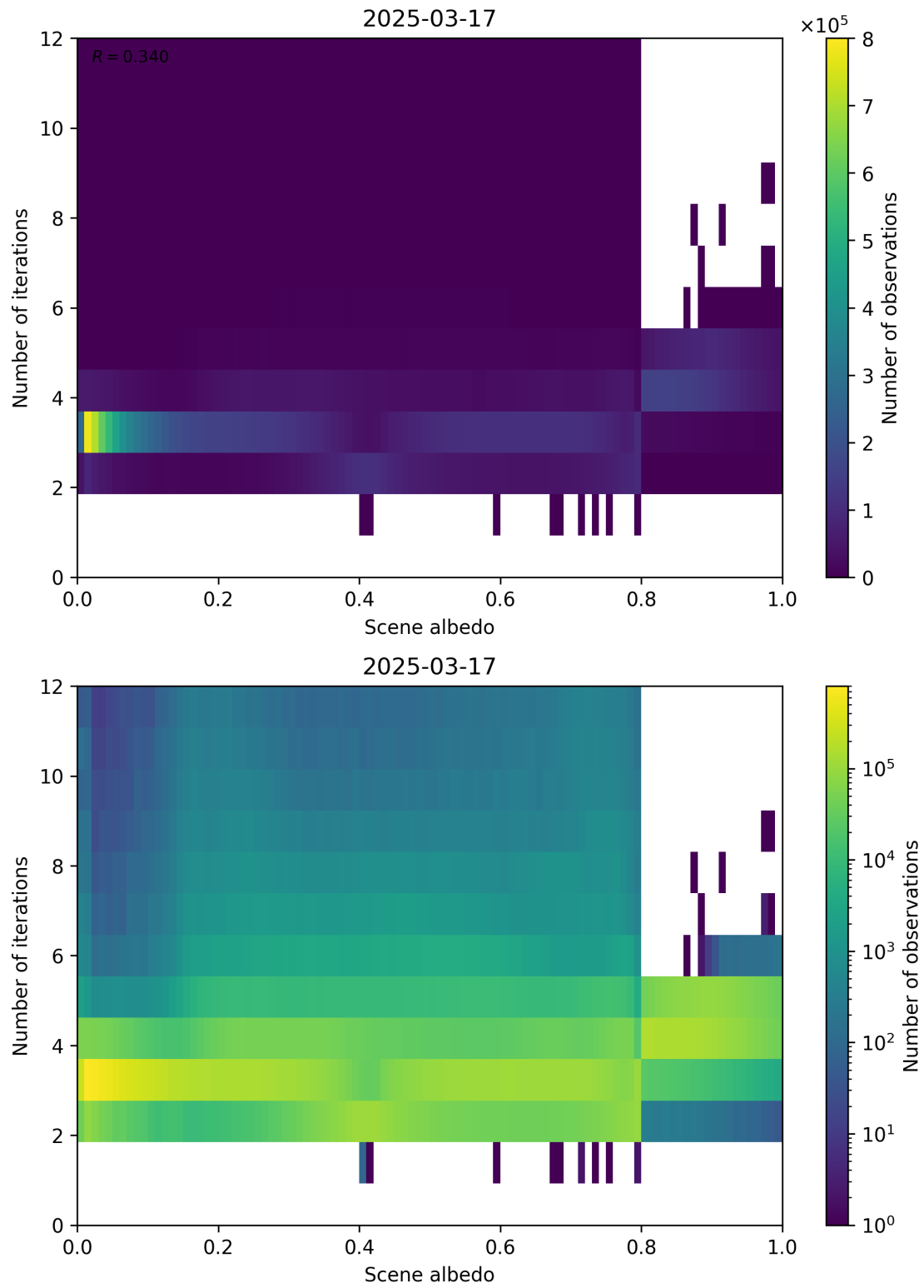
Figure 105: Scatter density plot of “Scene albedo” against “Number of iterations” for 2025-03-17 to 2025-03-18.
