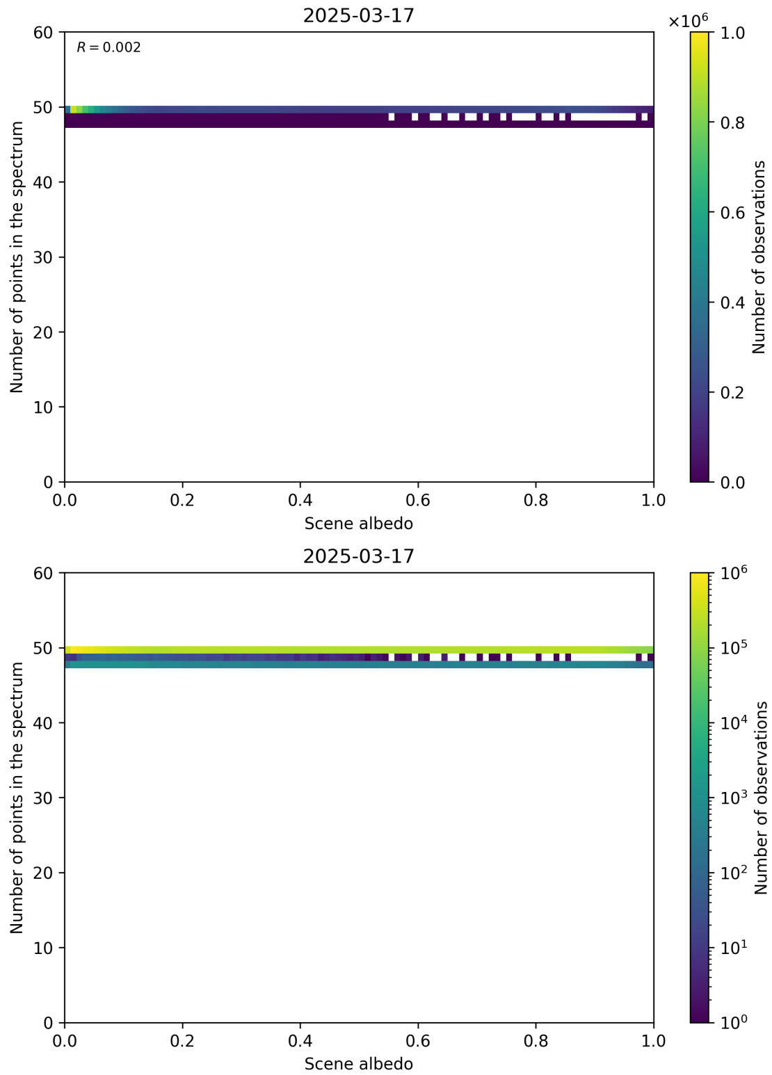
Figure 106: Scatter density plot of “Scene albedo” against “Number of points in the spectrum” for 2025-03-17 to 2025-03-18.
