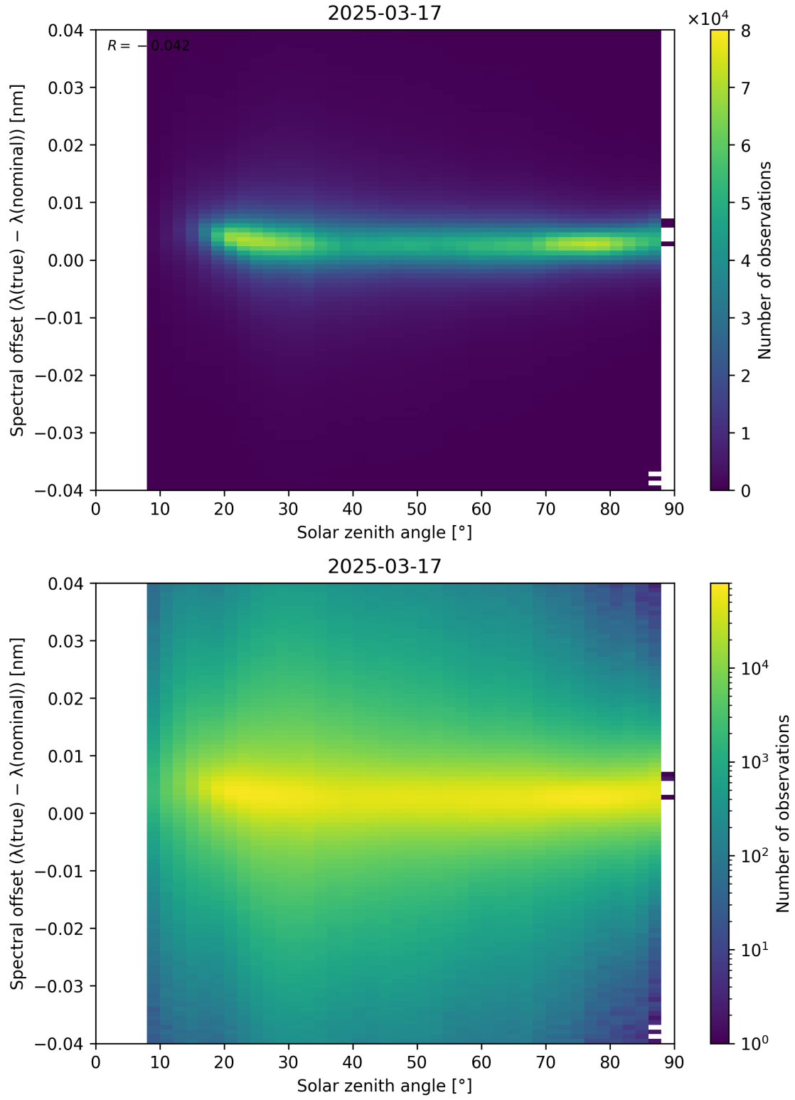
Figure 117: Scatter density plot of “Solar zenith angle” against “Spectral offset ( \lambda_{\text{true}} - \lambda_{\text{nominal}} )” for 2025-03-17 to 2025-03-18.
