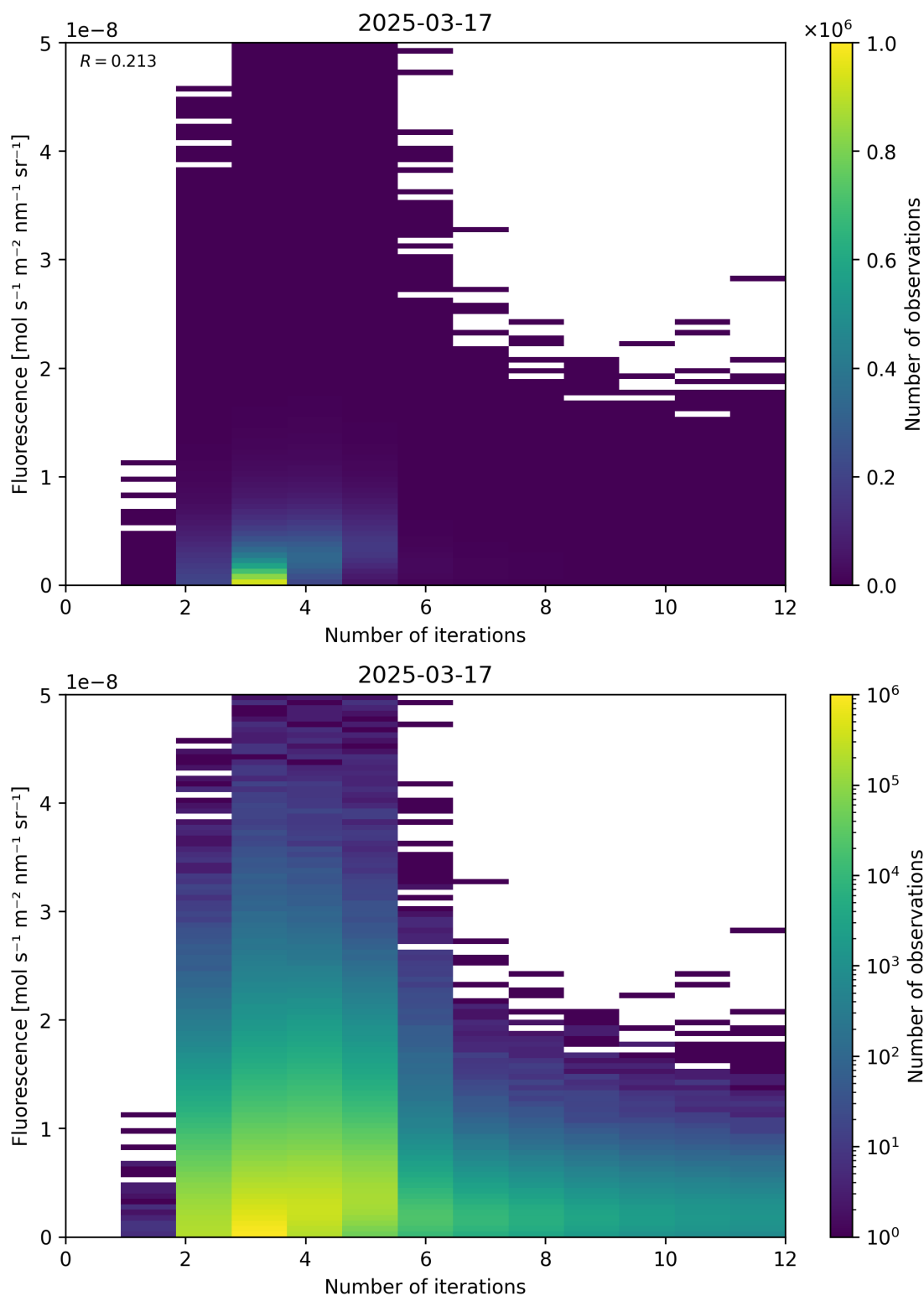
Figure 98: Scatter density plot of “Number of iterations” against “Fluorescence” for 2025-03-17 to 2025-03-18.
