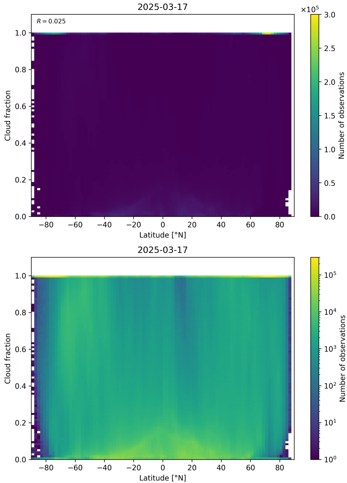
Figure 90: Scatter density plot of “Latitude” against “Cloud fraction” for 2025-03-17 to 2025-03-18.
