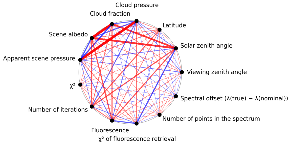
Figure 1: Map of correlation graph for 2025-03-17 to 2025-03-18.
