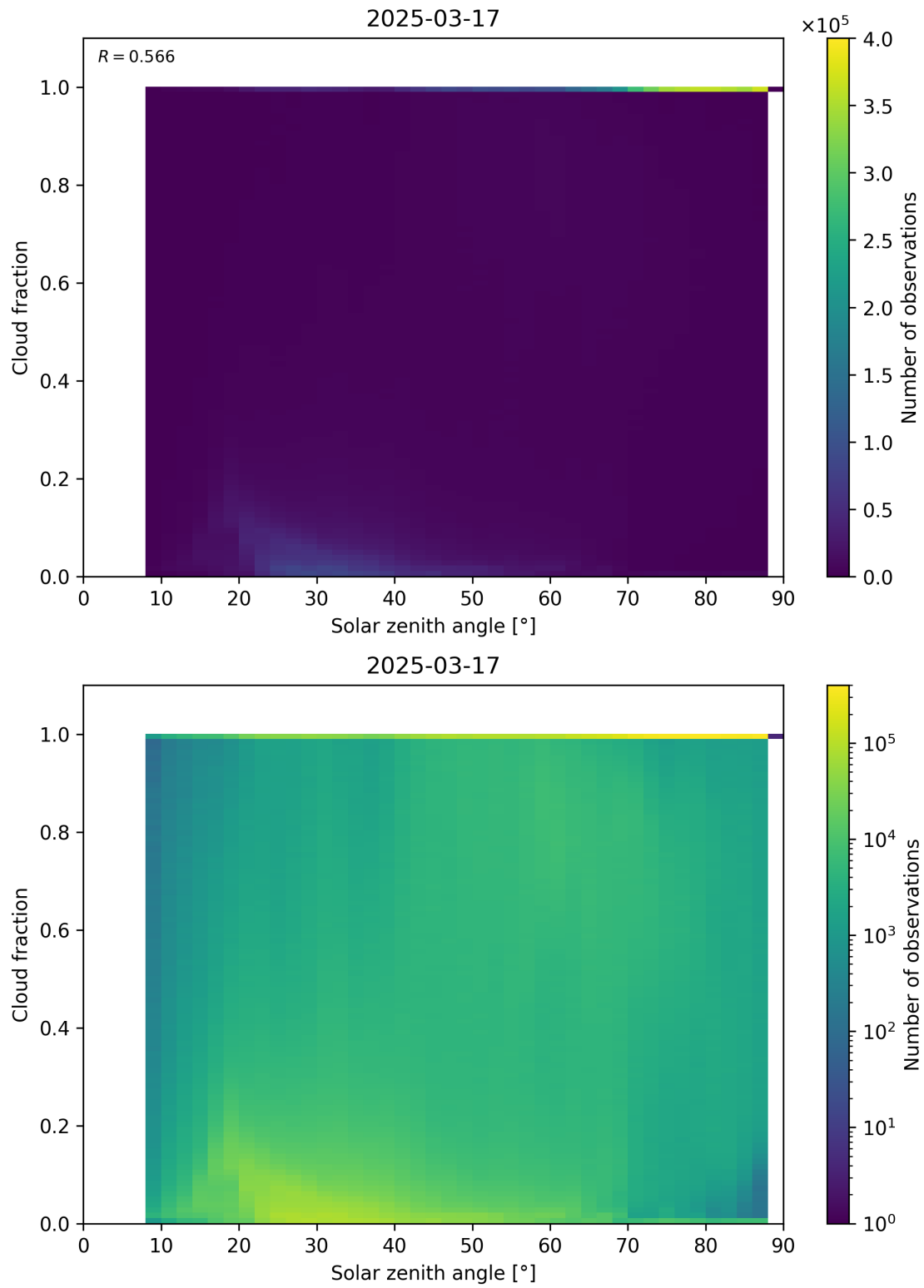
Figure 110: Scatter density plot of “Solar zenith angle” against “Cloud fraction” for 2025-03-17 to 2025-03-18.
