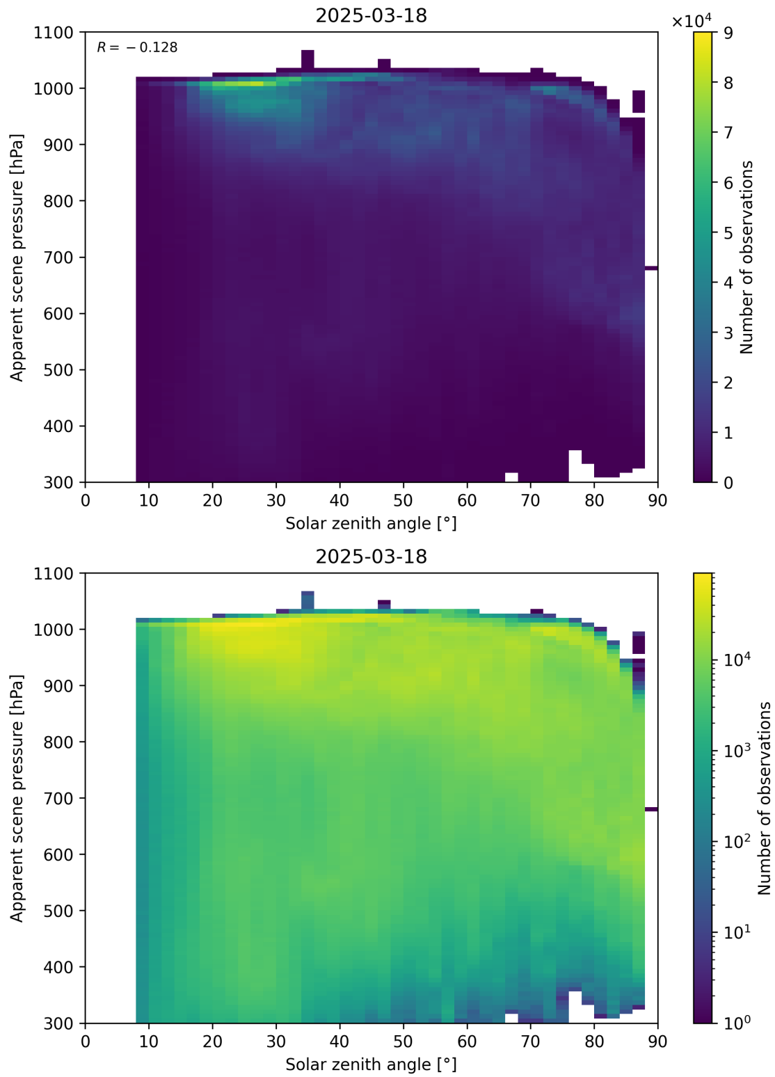
Figure 108: Scatter density plot of “Solar zenith angle” against “Apparent scene pressure” for 2025-03-17 to 2025-03-19.
