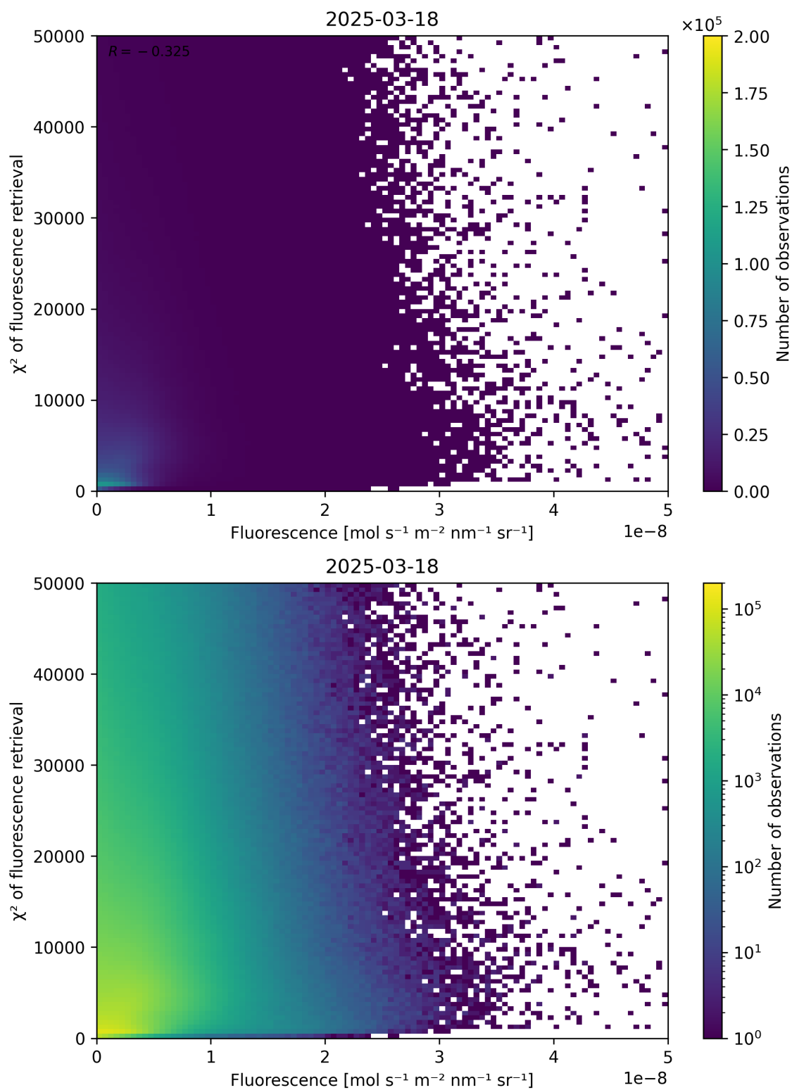
Figure 85: Scatter density plot of “Fluorescence” against “ \chi^2 of fluorescence retrieval” for 2025-03-17 to 2025-03-19.
