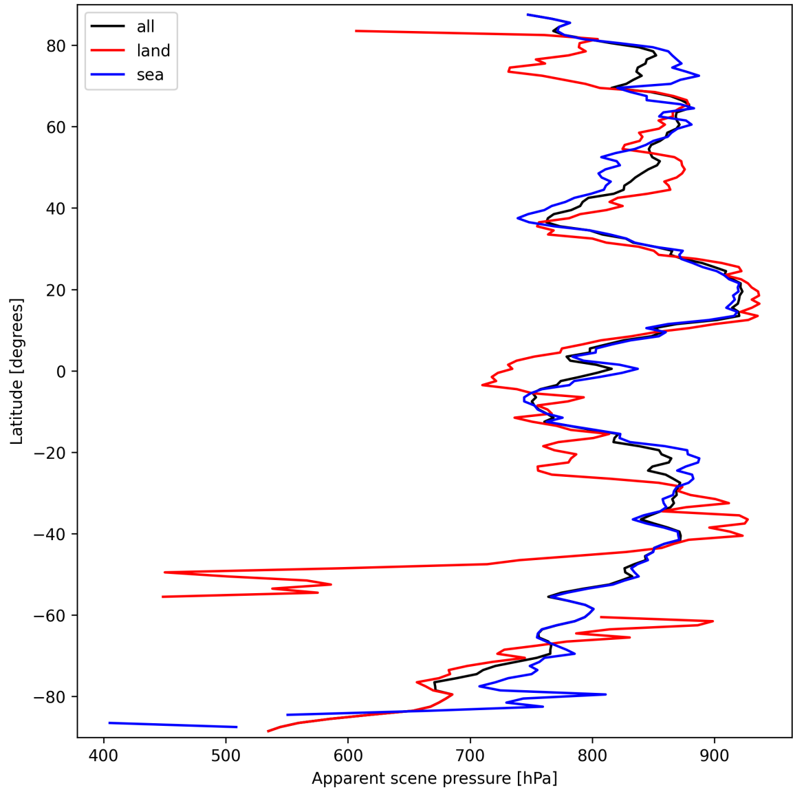
Figure 19: Zonal average of “Apparent scene pressure” for 2025-03-17 to 2025-03-19.
