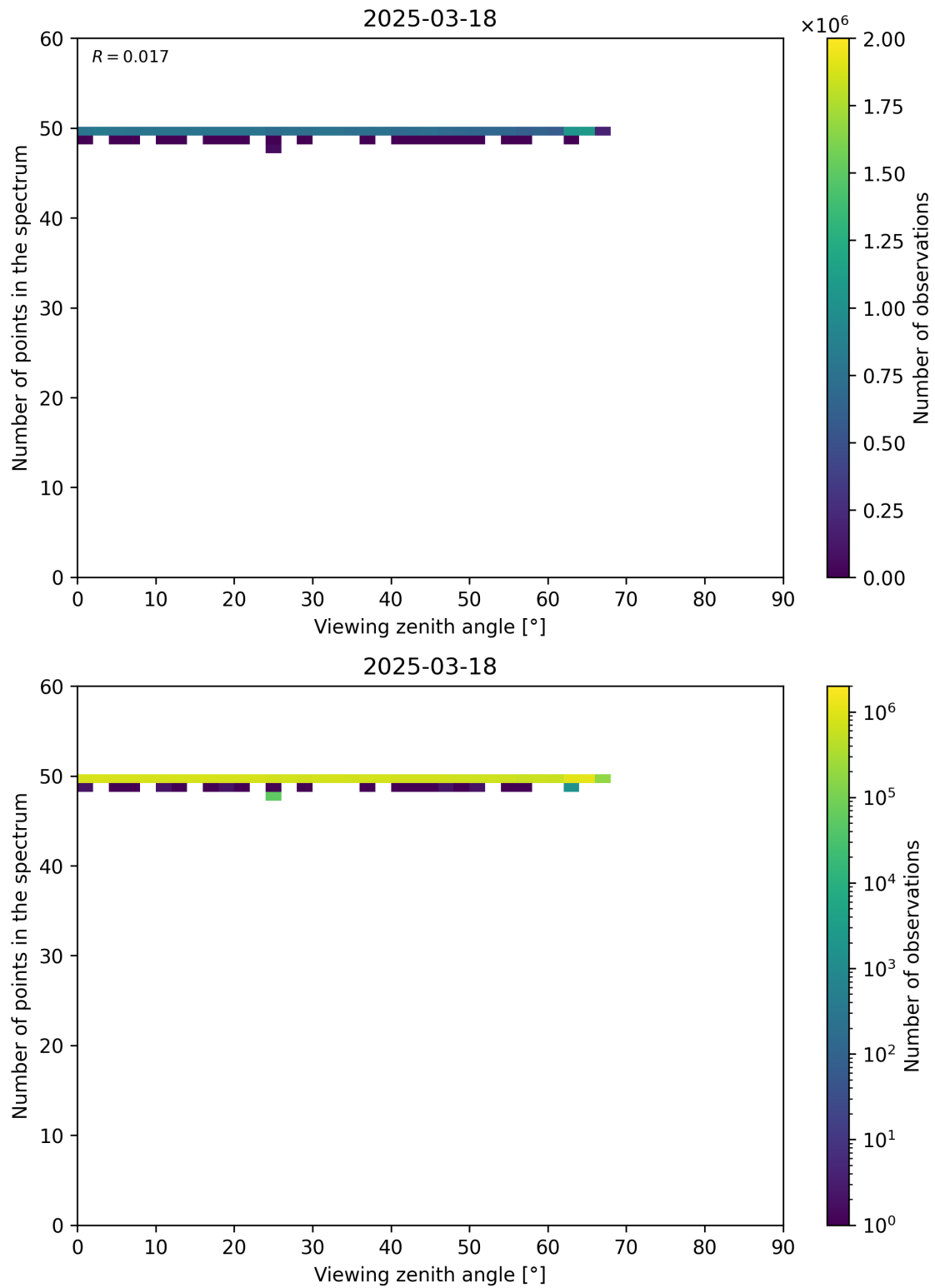
Figure 125: Scatter density plot of “Viewing zenith angle” against “Number of points in the spectrum” for 2025-03-17 to 2025-03-19.
