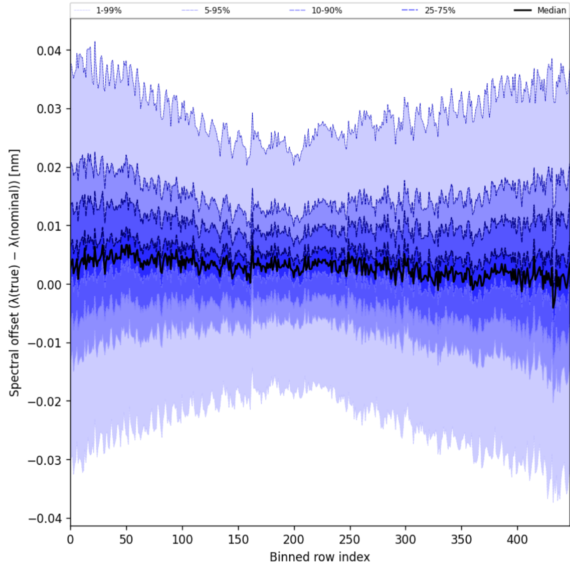
Figure 62: Along track statistics of “Spectral offset ( \lambda_{\text{true}} - \lambda_{\text{nominal}} )” for 2025-03-17 to 2025-03-19
