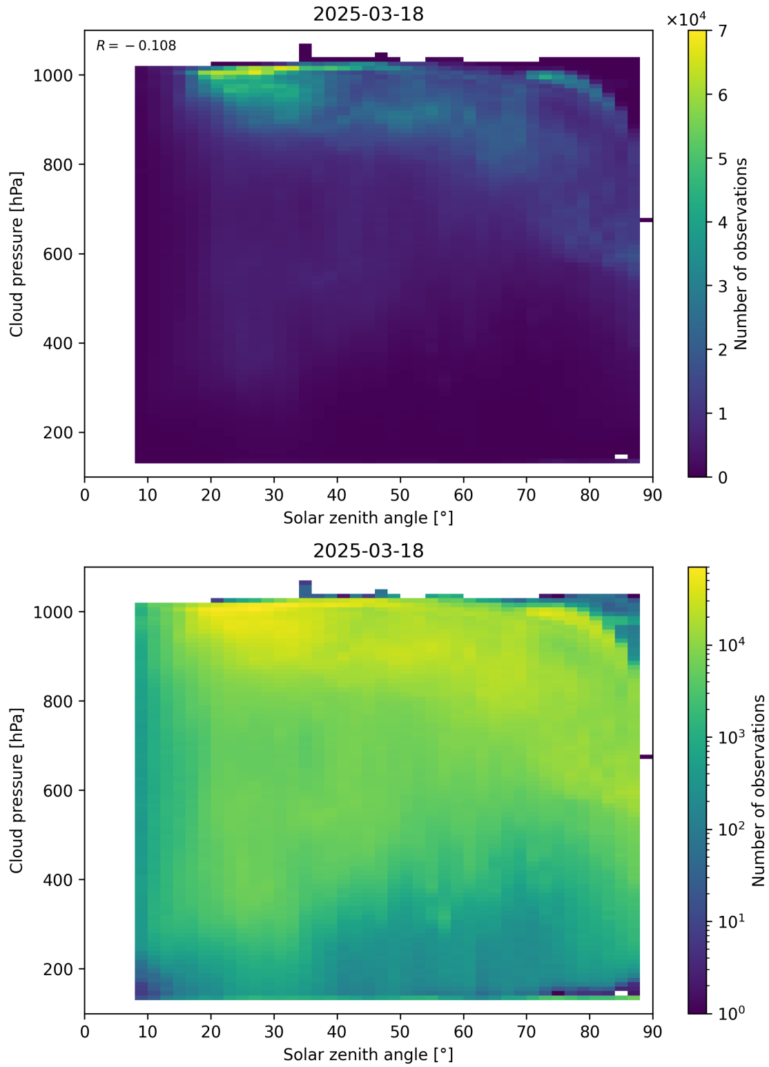
Figure 111: Scatter density plot of “Solar zenith angle” against “Cloud pressure” for 2025-03-17 to 2025-03-19.
