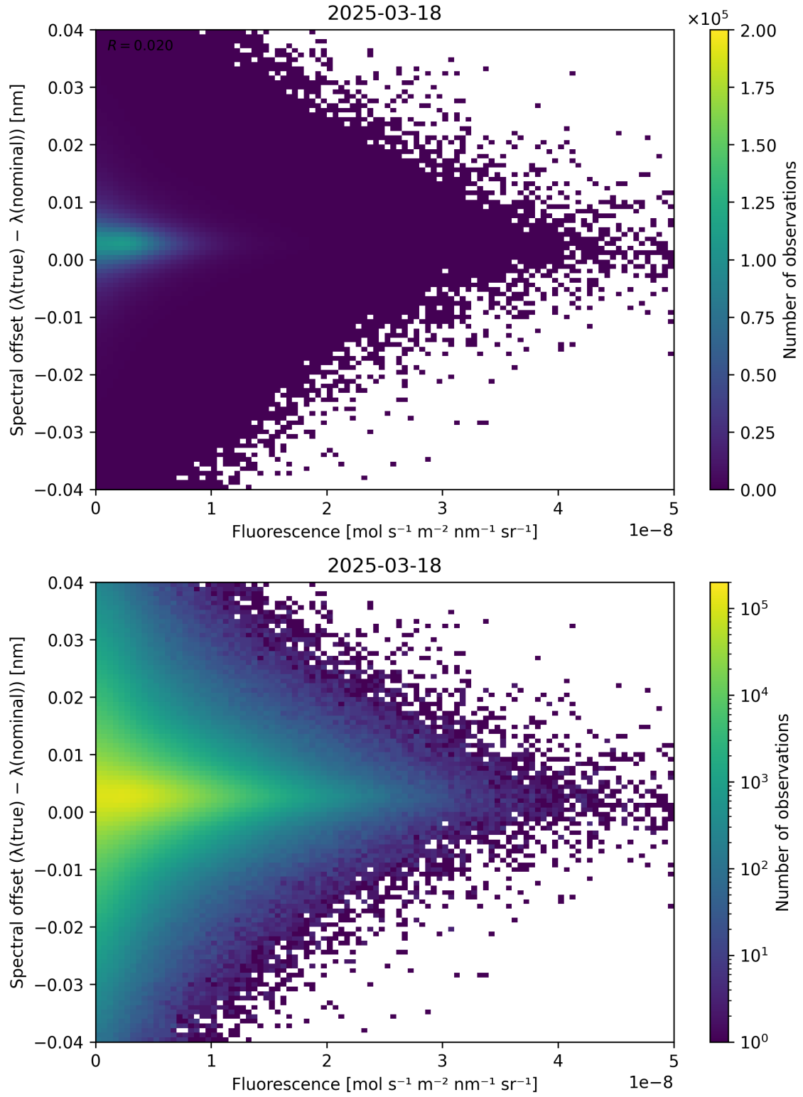
Figure 87: Scatter density plot of “Fluorescence” against “Spectral offset ( \lambda_{\text{true}} - \lambda_{\text{nominal}} )” for 2025-03-17 to 2025-03-19.
