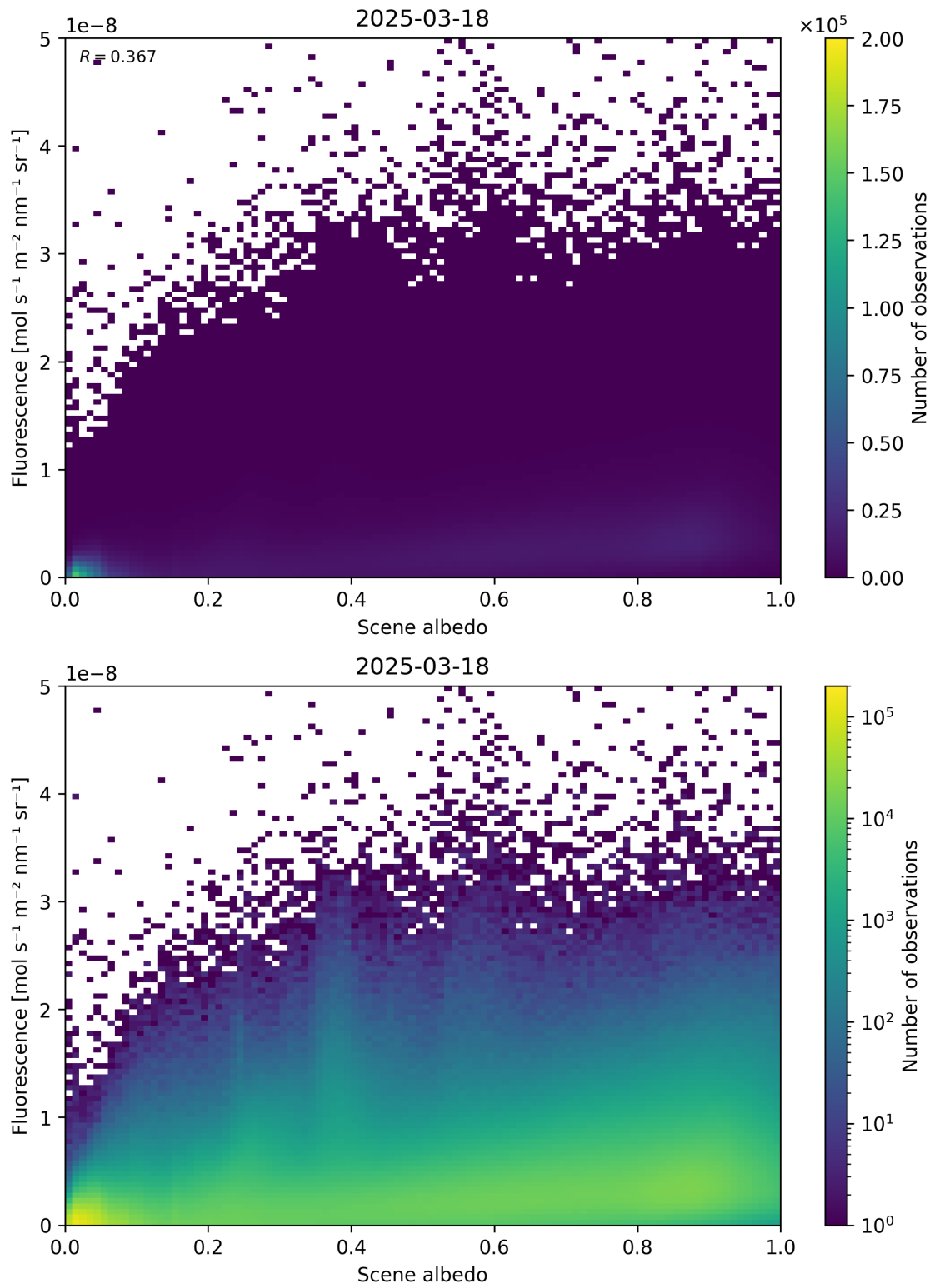
Figure 104: Scatter density plot of “Scene albedo” against “Fluorescence” for 2025-03-17 to 2025-03-19.
