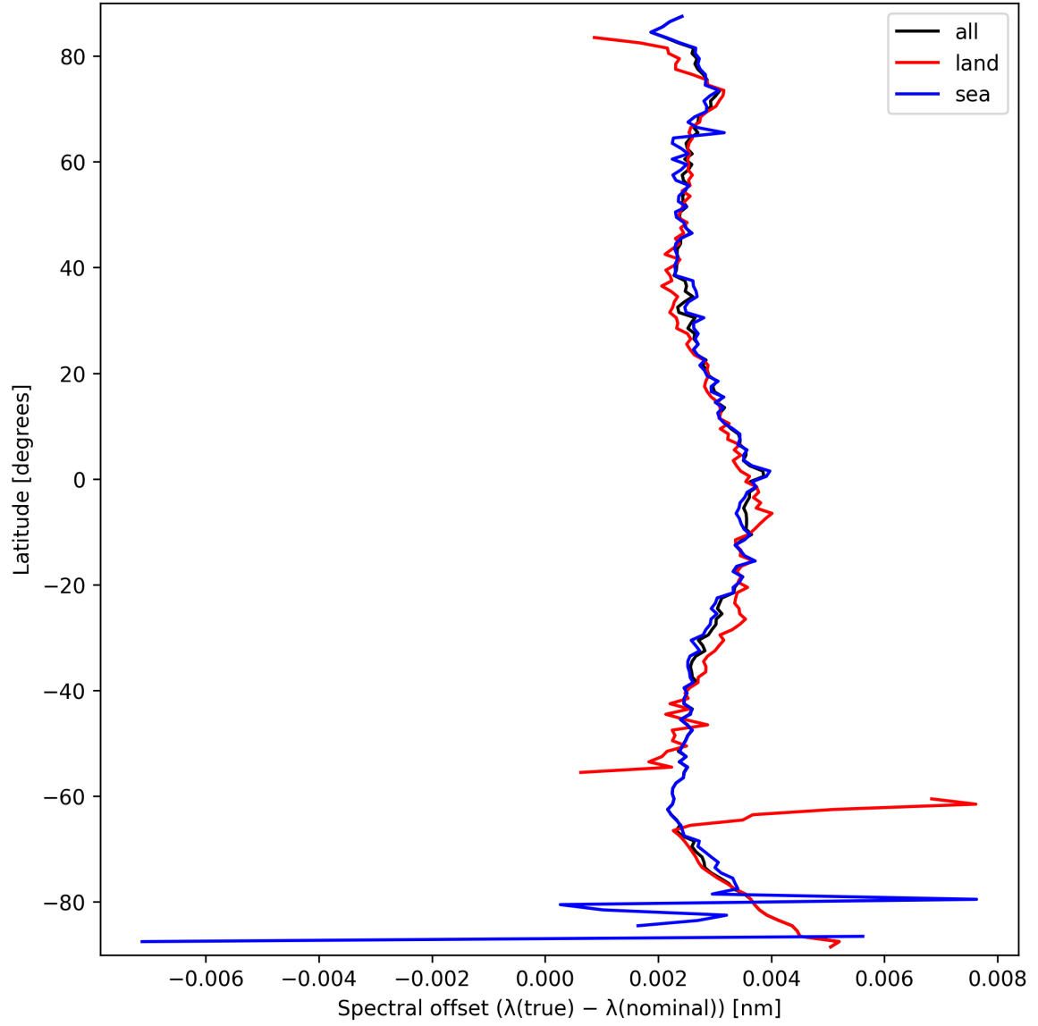
Figure 28: Zonal average of “Spectral offset ( \lambda_{\text{true}} - \lambda_{\text{nominal}} )” for 2025-03-17 to 2025-03-19.
