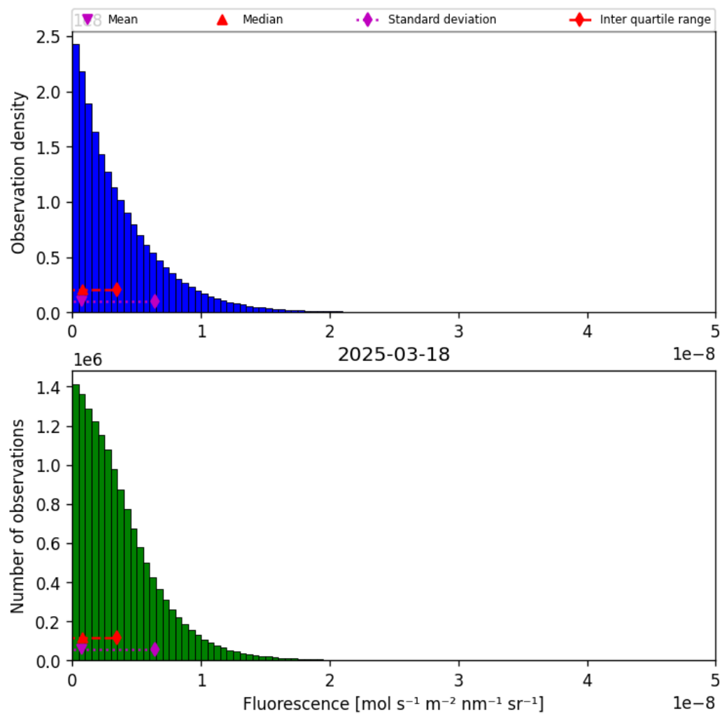
Figure 40: Histogram of “Fluorescence” for 2025-03-17 to 2025-03-19
