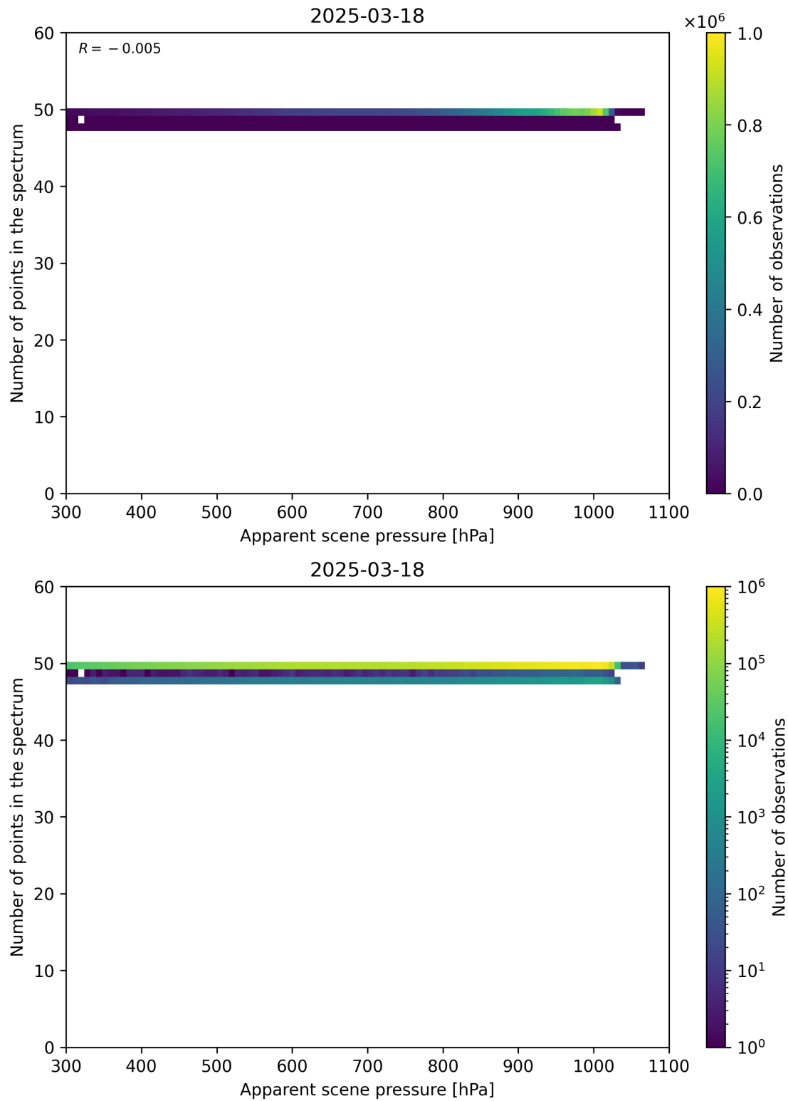
Figure 66: Scatter density plot of “Apparent scene pressure” against “Number of points in the spectrum” for 2025-03-17 to 2025-03-19.
