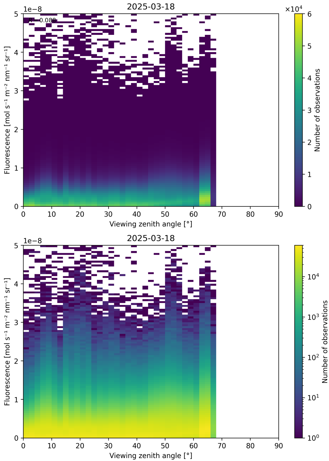
Figure 122: Scatter density plot of "Viewing zenith angle" against "Fluorescence" for 2025-03-17 to 2025-03-19.
