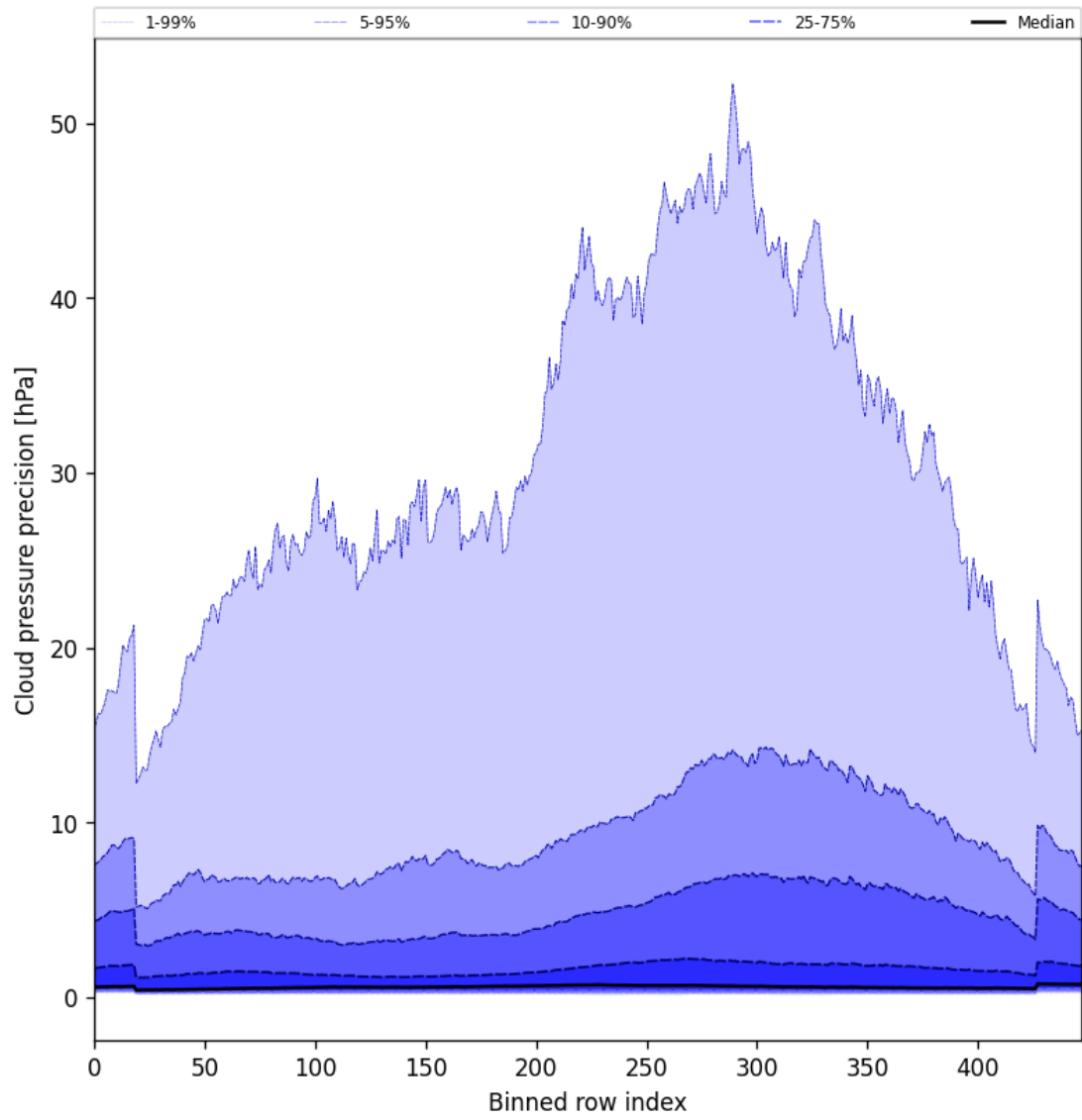
Figure 48: Along track statistics of “Cloud pressure precision” for 2025-03-17 to 2025-03-19
