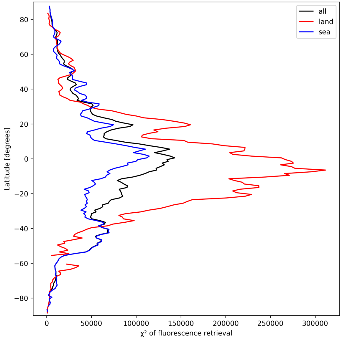
Figure 25: Zonal average of “ \chi^2 of fluorescence retrieval” for 2025-03-17 to 2025-03-19.
