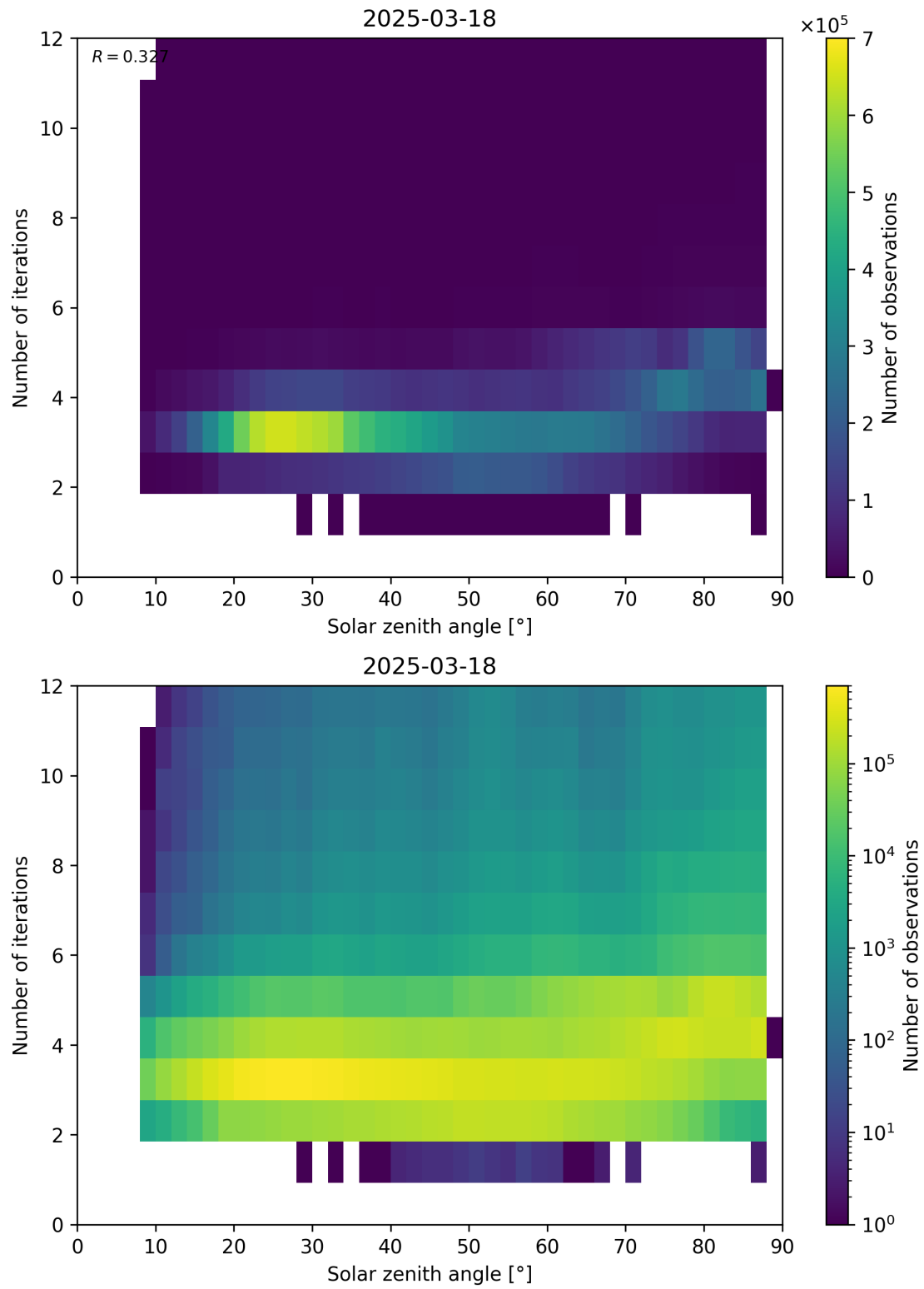
Figure 114: Scatter density plot of “Solar zenith angle” against “Number of iterations” for 2025-03-17 to 2025-03-19.
