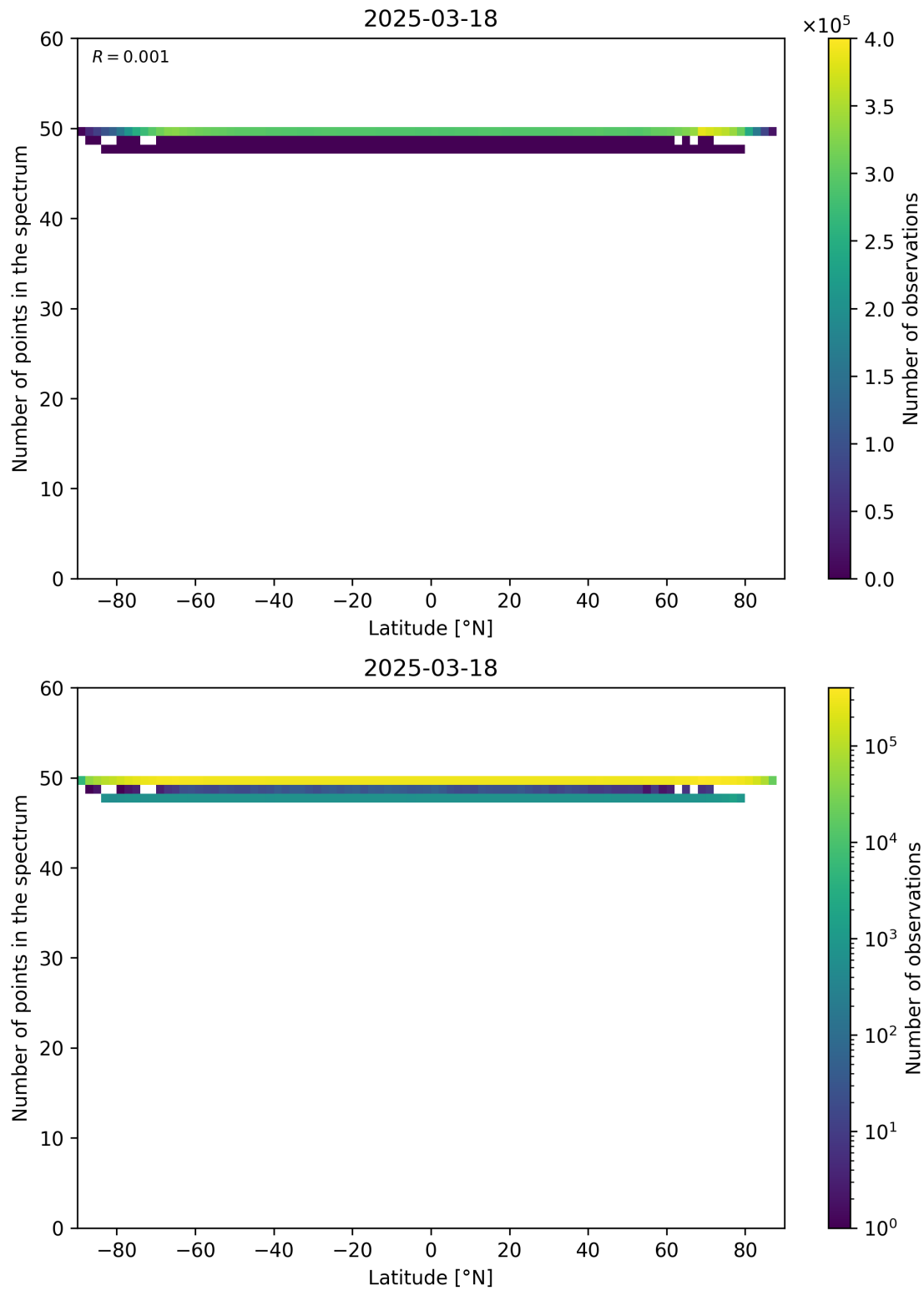
Figure 94: Scatter density plot of “Latitude” against “Number of points in the spectrum” for 2025-03-17 to 2025-03-19.
