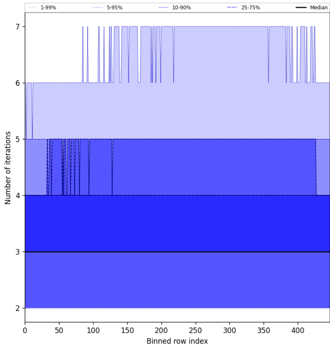
Figure 56: Along track statistics of “Number of iterations” for 2025-03-17 to 2025-03-19
