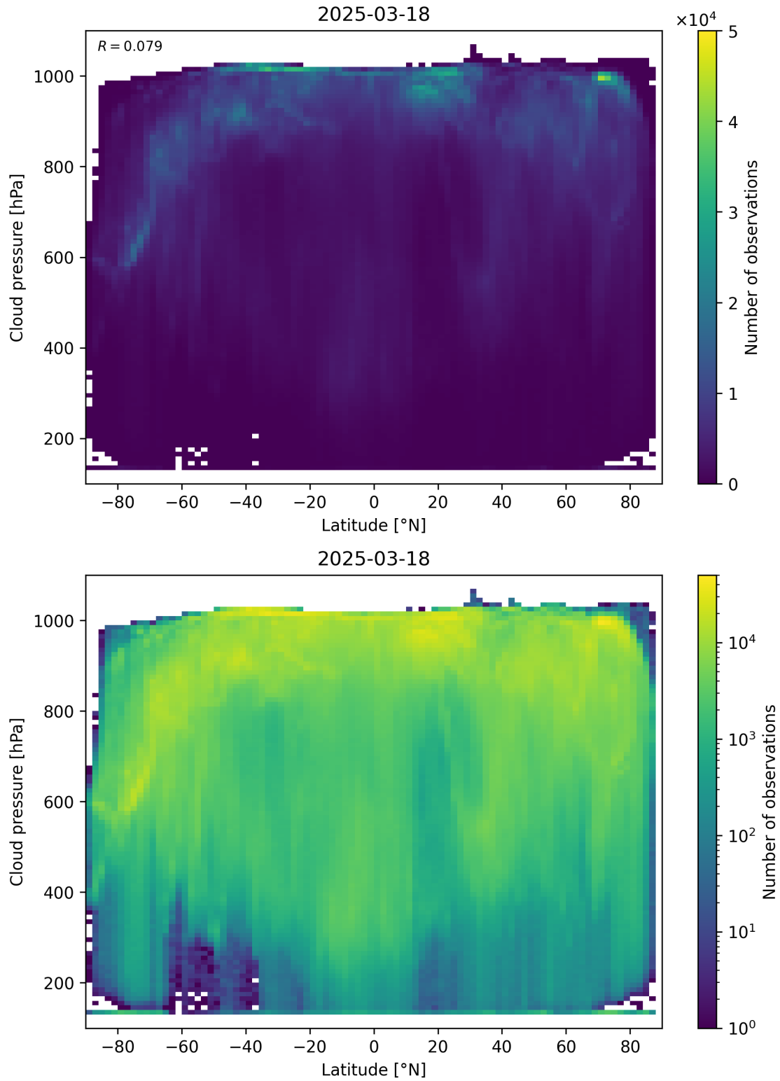
Figure 91: Scatter density plot of “Latitude” against “Cloud pressure” for 2025-03-17 to 2025-03-19.
