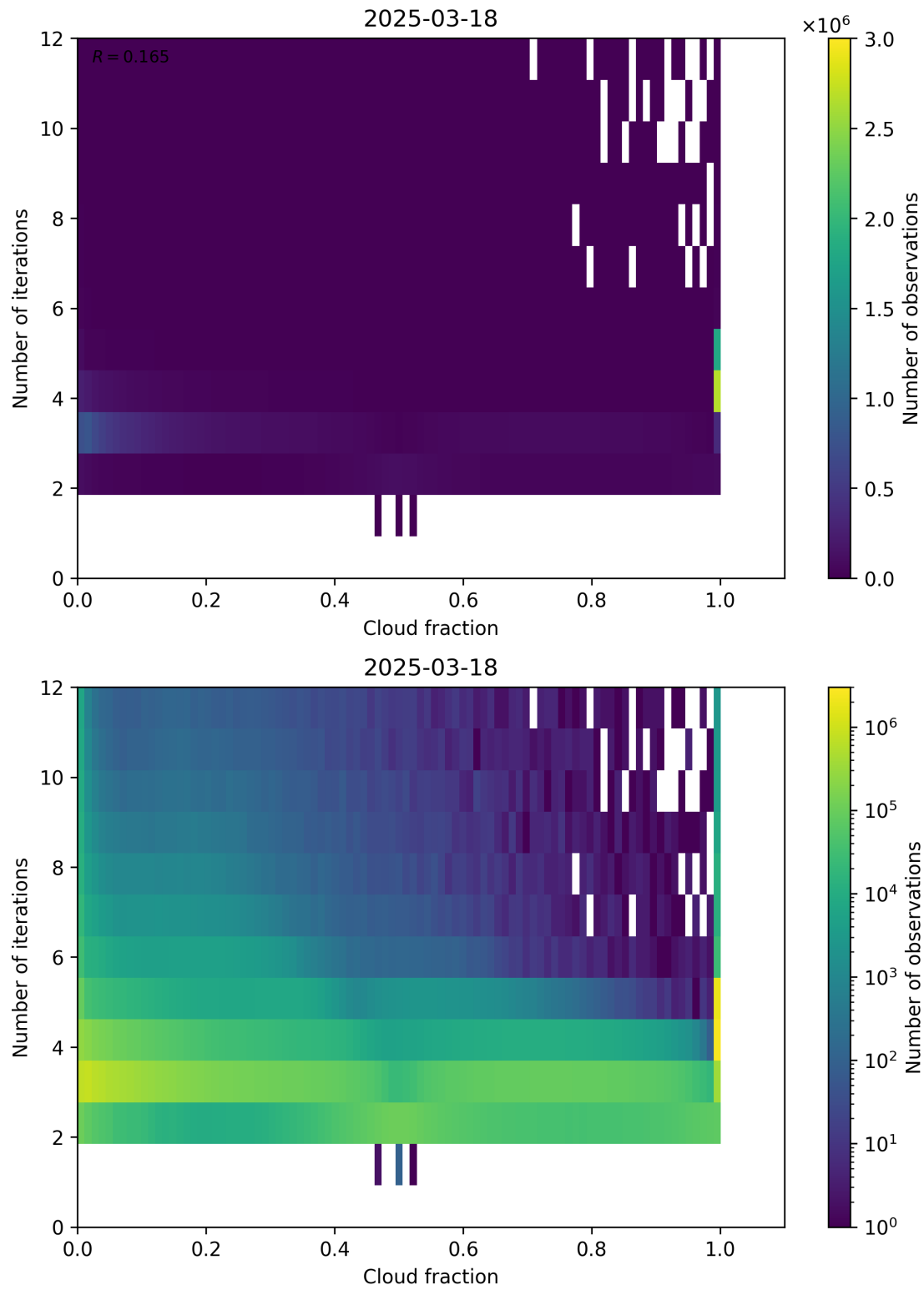
Figure 73: Scatter density plot of “Cloud fraction” against “Number of iterations” for 2025-03-17 to 2025-03-19.
