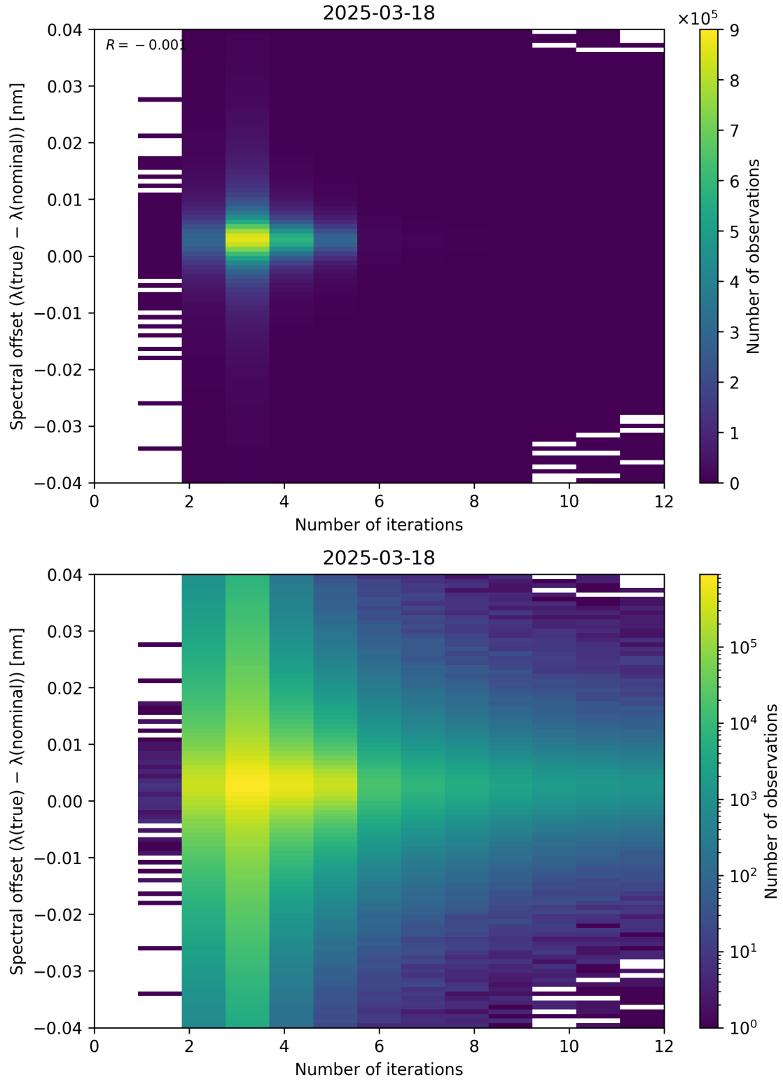
Figure 100: Scatter density plot of “Number of iterations” against “Spectral offset ( \lambda_{\text{true}} - \lambda_{\text{nominal}} )” for 2025-03-17 to 2025-03-19.
