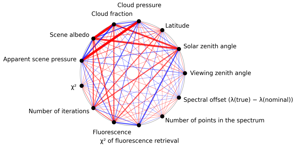
Figure 1: Map of correlation graph for 2025-03-17 to 2025-03-19.
