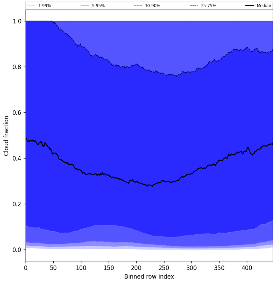
Figure 49: Along track statistics of “Cloud fraction” for 2025-03-17 to 2025-03-19
