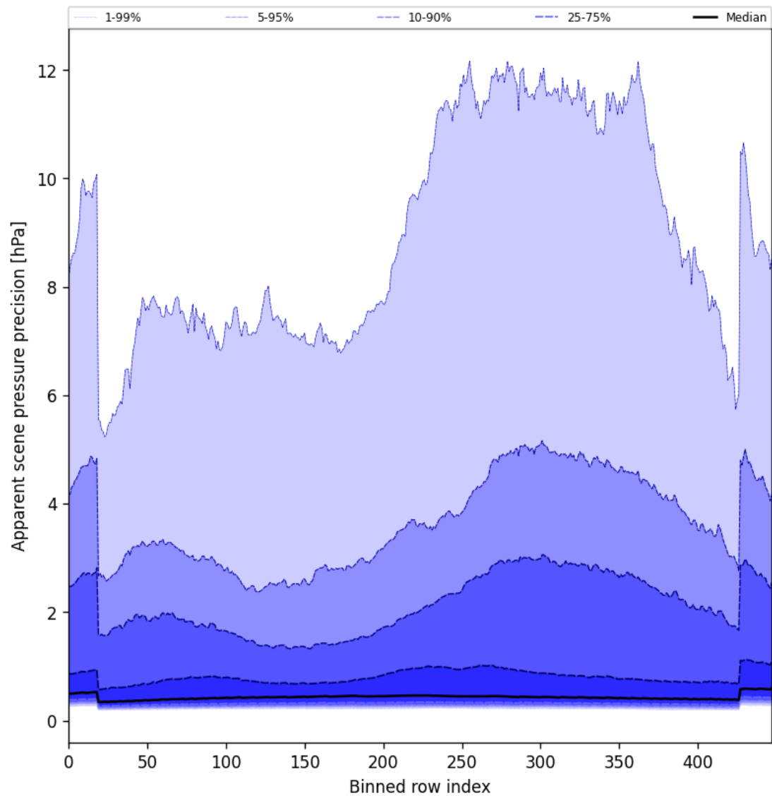
Figure 54: Along track statistics of “Apparent scene pressure precision” for 2025-03-17 to 2025-03-19
