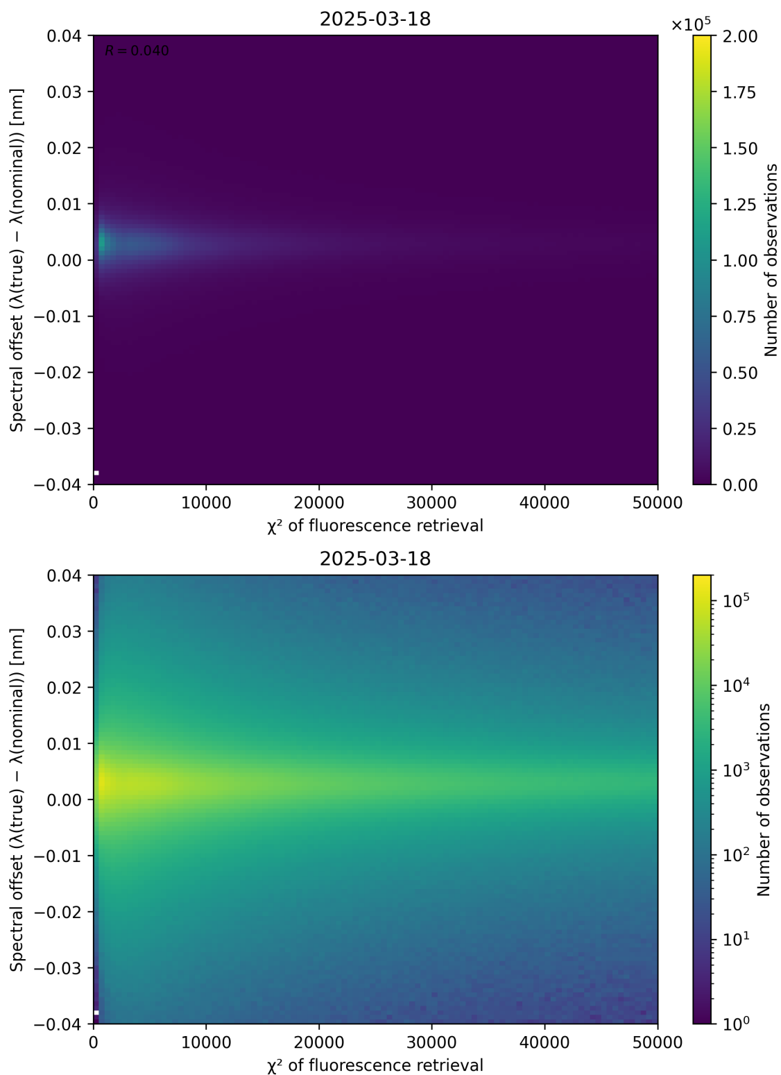
Figure 69: Scatter density plot of “ \chi^2 of fluorescence retrieval” against “Spectral offset ( \lambda_{\text{true}} - \lambda_{\text{nominal}} )” for 2025-03-17 to 2025-03-19.
