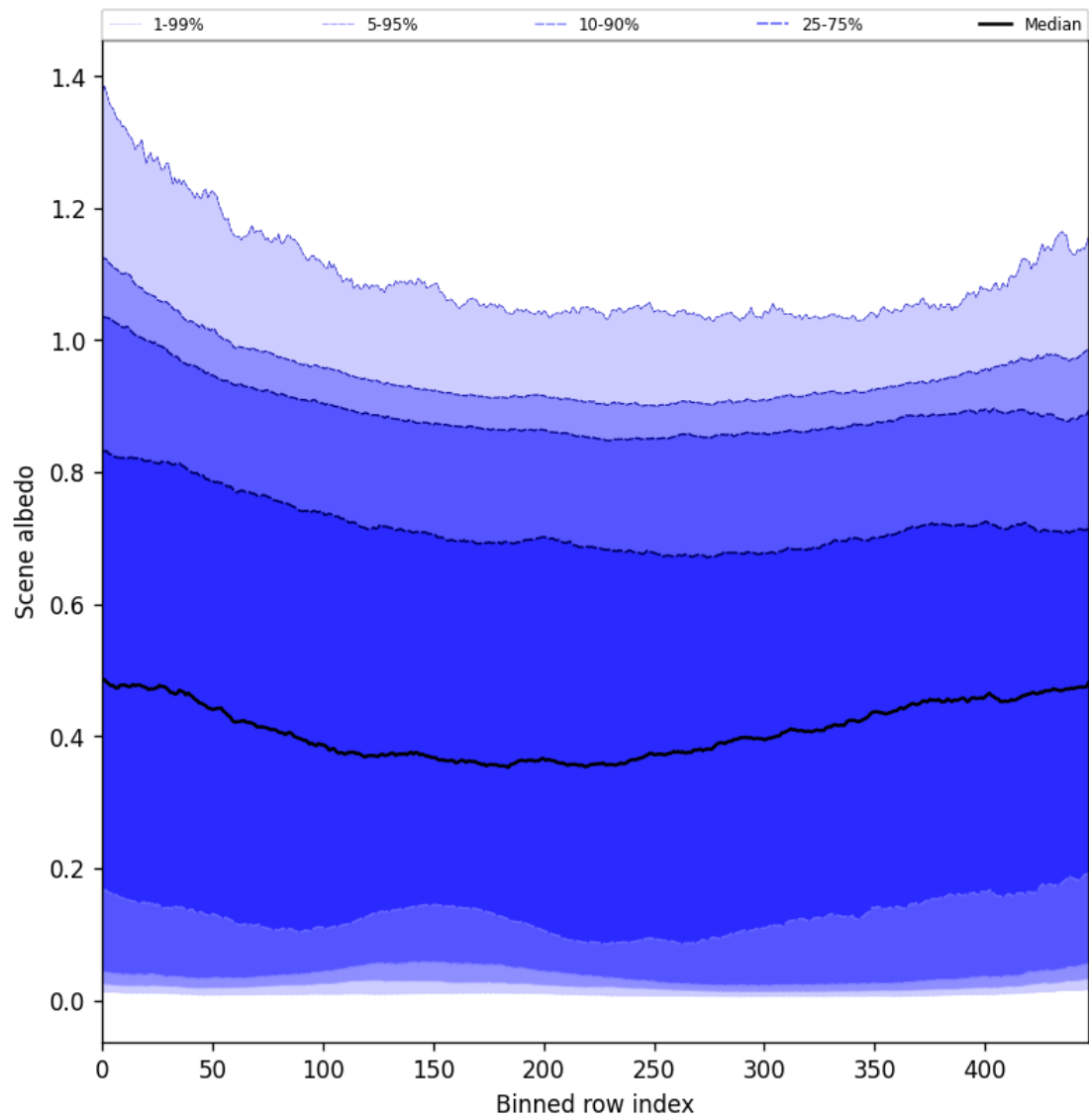
Figure 51: Along track statistics of “Scene albedo” for 2025-03-17 to 2025-03-19
