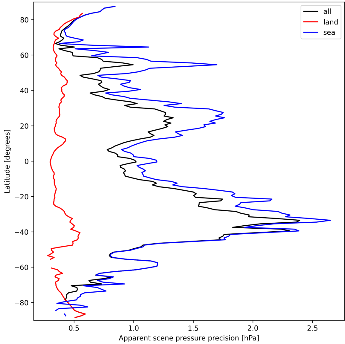
Figure 20: Zonal average of “Apparent scene pressure precision” for 2025-03-17 to 2025-03-19.
