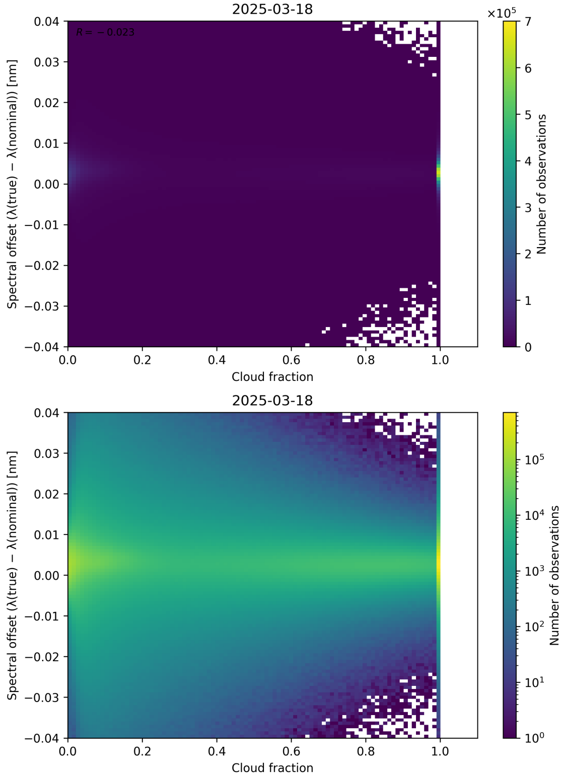
Figure 76: Scatter density plot of “Cloud fraction” against “Spectral offset ( \lambda_{\text{true}} - \lambda_{\text{nominal}} )” for 2025-03-17 to 2025-03-19.
