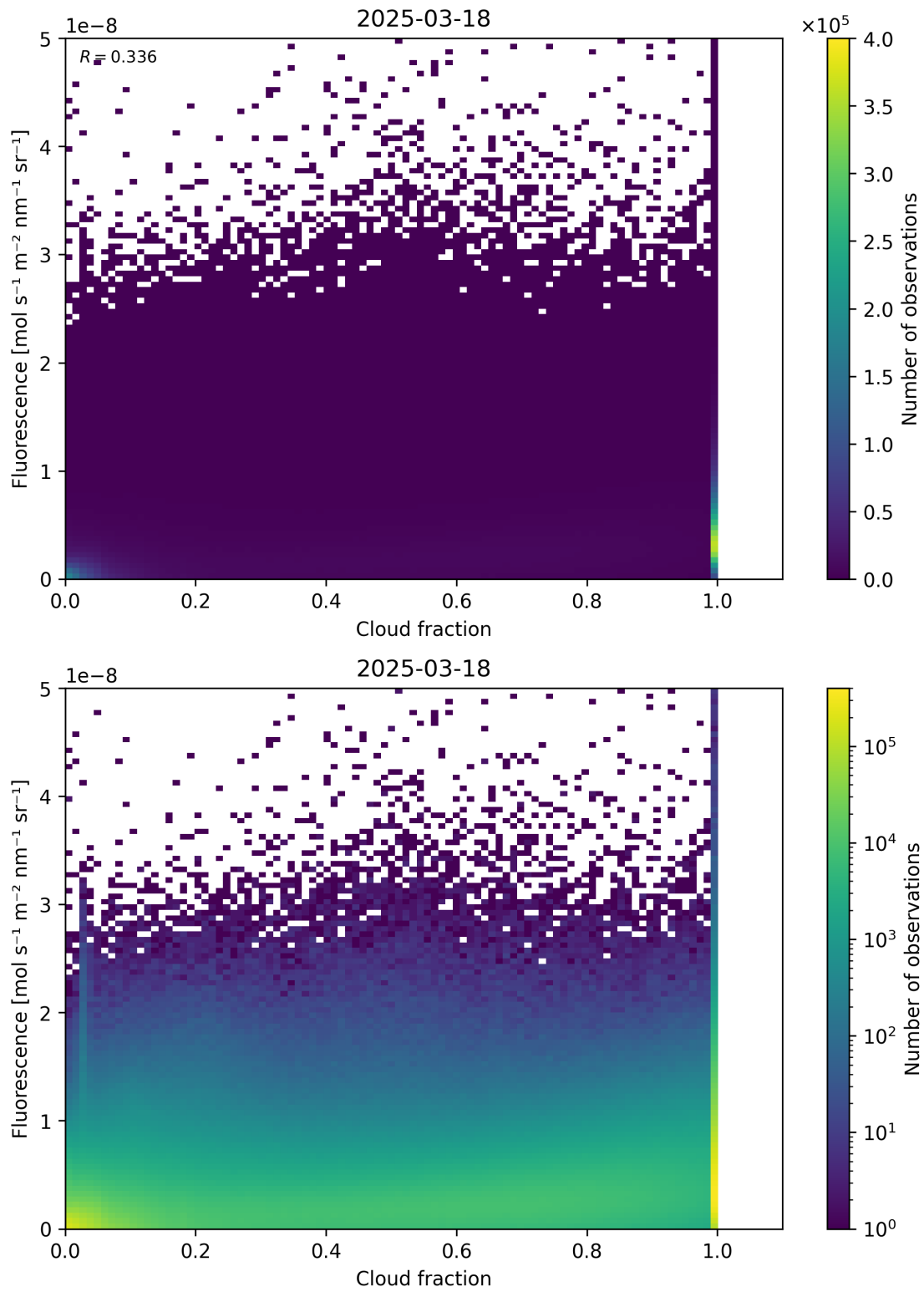
Figure 72: Scatter density plot of “Cloud fraction” against “Fluorescence” for 2025-03-17 to 2025-03-19.
