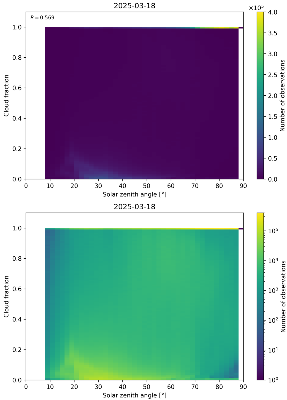
Figure 110: Scatter density plot of “Solar zenith angle” against “Cloud fraction” for 2025-03-17 to 2025-03-19.
