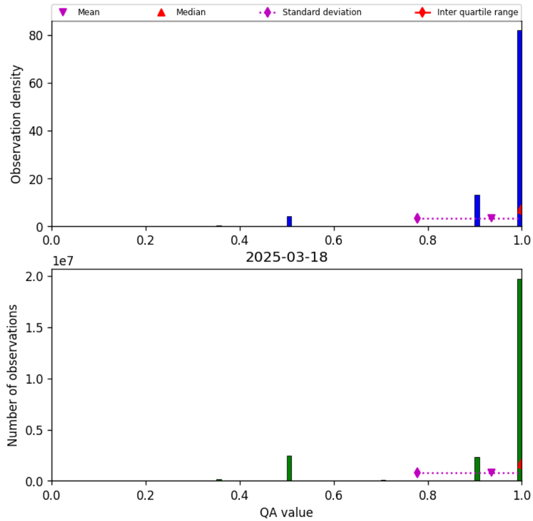
Figure 29: Histogram of “QA value” for 2025-03-17 to 2025-03-19
