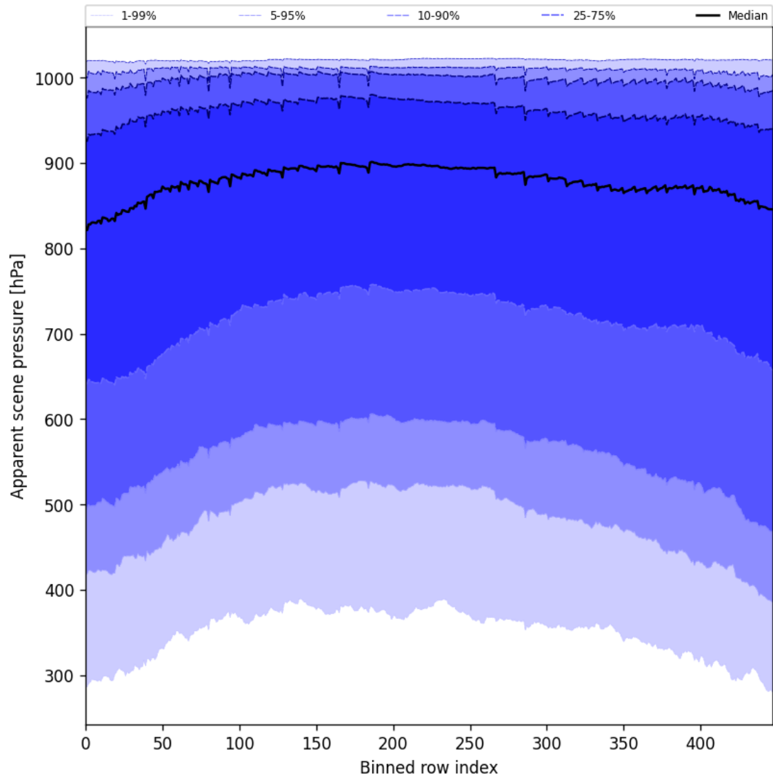
Figure 53: Along track statistics of “Apparent scene pressure” for 2025-03-17 to 2025-03-19
