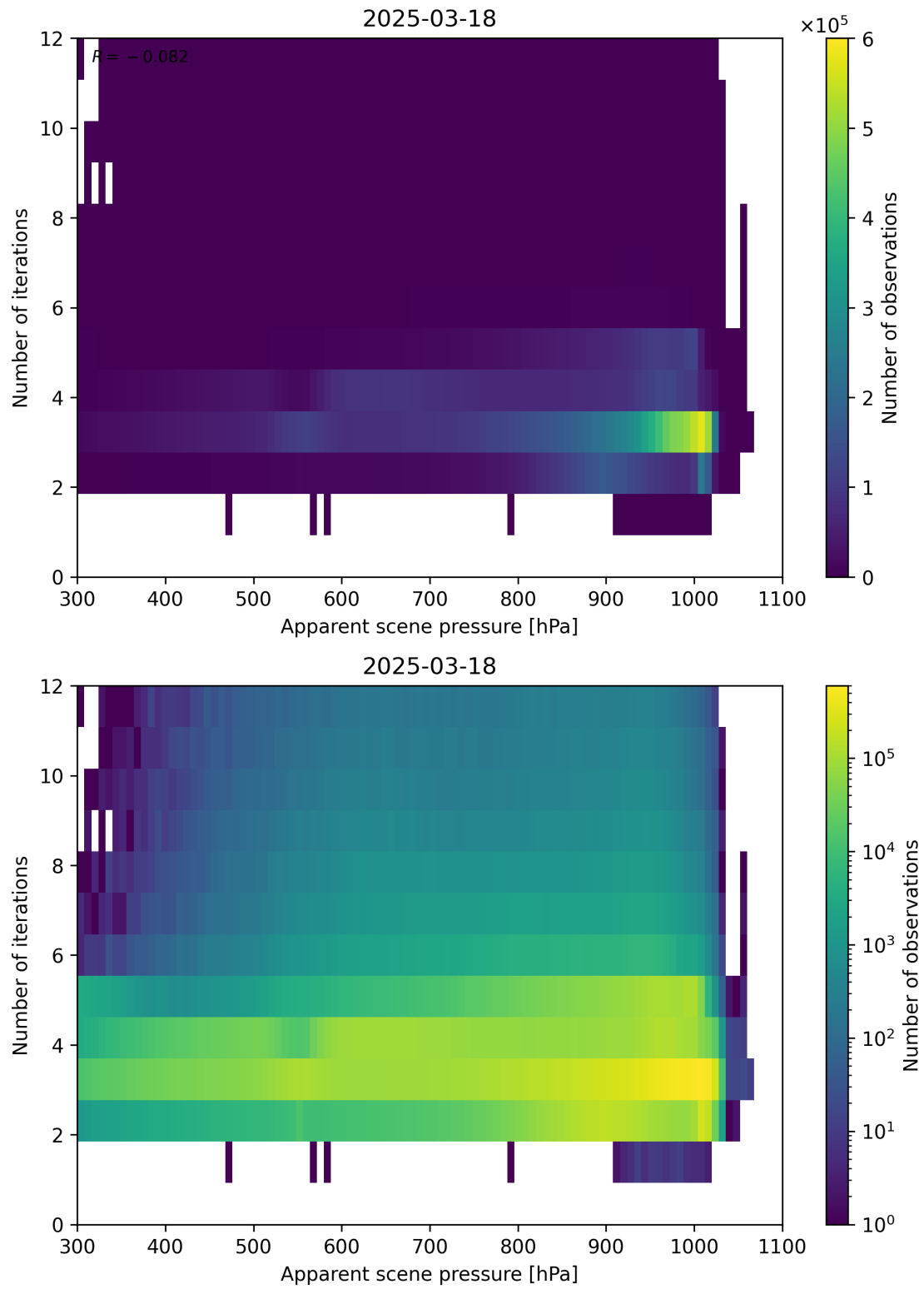
Figure 65: Scatter density plot of “Apparent scene pressure” against “Number of iterations” for 2025-03-17 to 2025-03-19.
