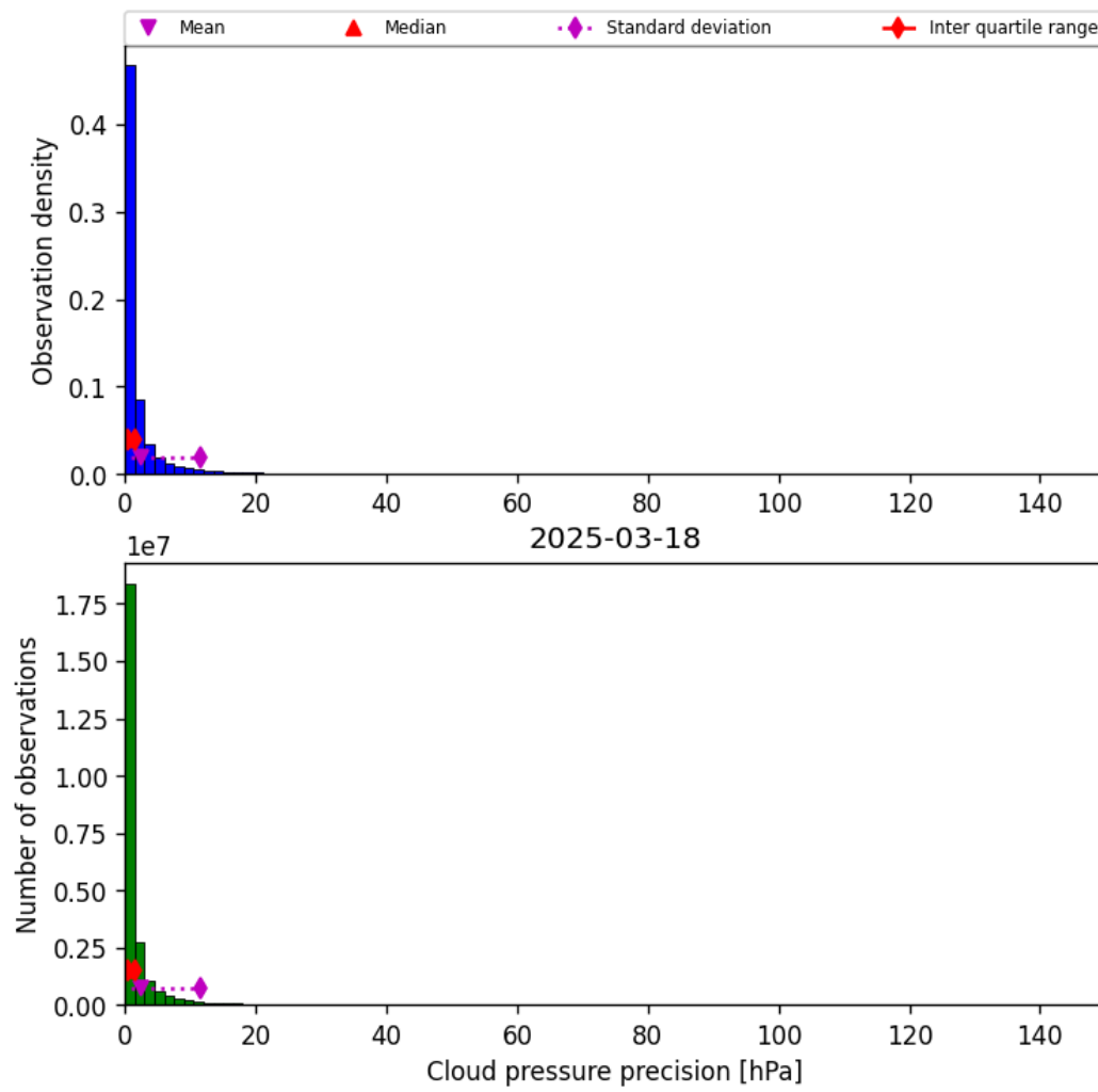
Figure 31: Histogram of “Cloud pressure precision” for 2025-03-17 to 2025-03-19
