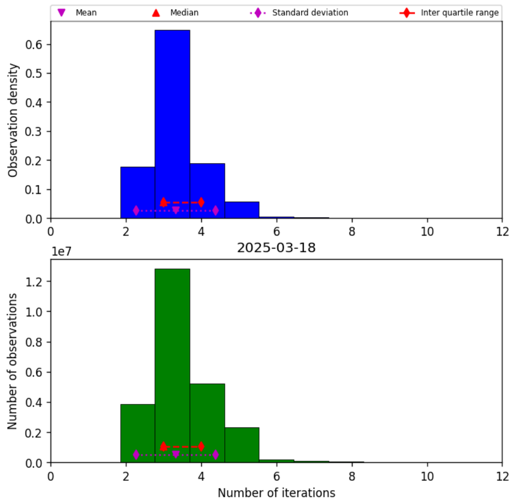
Figure 39: Histogram of “Number of iterations” for 2025-03-17 to 2025-03-19
