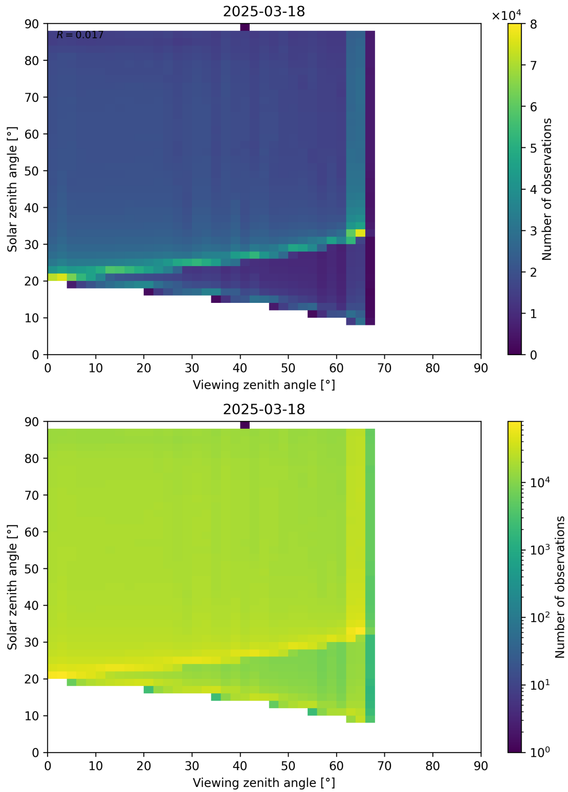
Figure 127: Scatter density plot of “Viewing zenith angle” against “Solar zenith angle” for 2025-03-17 to 2025-03-19.
