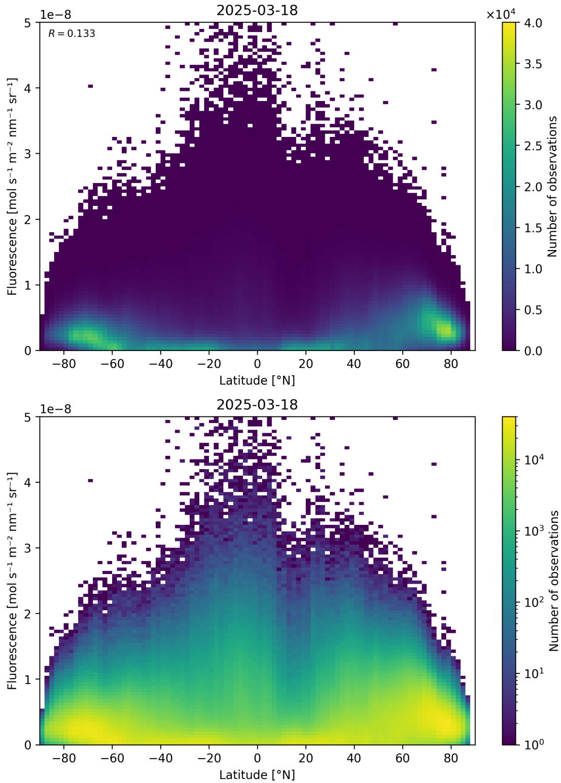
Figure 92: Scatter density plot of “Latitude” against “Fluorescence” for 2025-03-17 to 2025-03-19.
