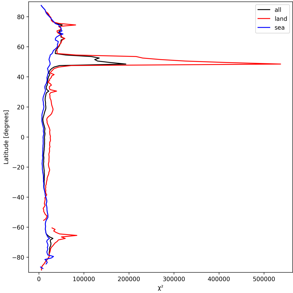
Figure 21: Zonal average of “ \chi^2 ” for 2025-03-17 to 2025-03-19.
