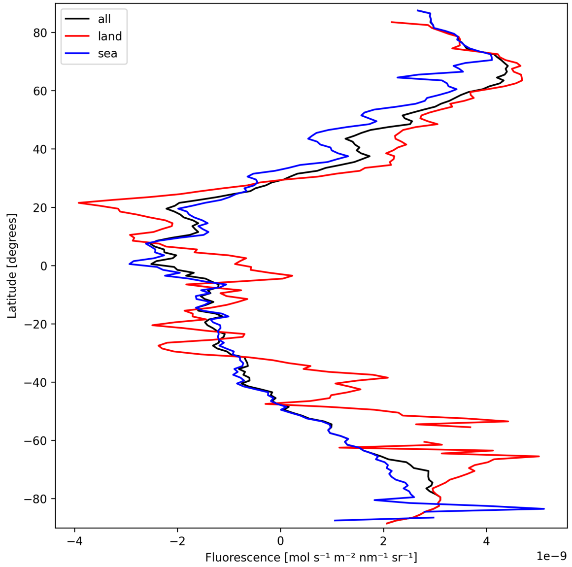
Figure 23: Zonal average of “Fluorescence” for 2025-03-17 to 2025-03-19.
