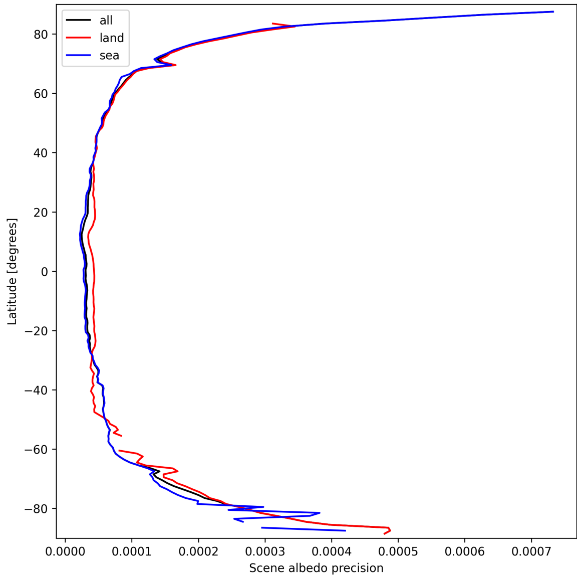
Figure 18: Zonal average of “Scene albedo precision” for 2025-03-17 to 2025-03-19.
