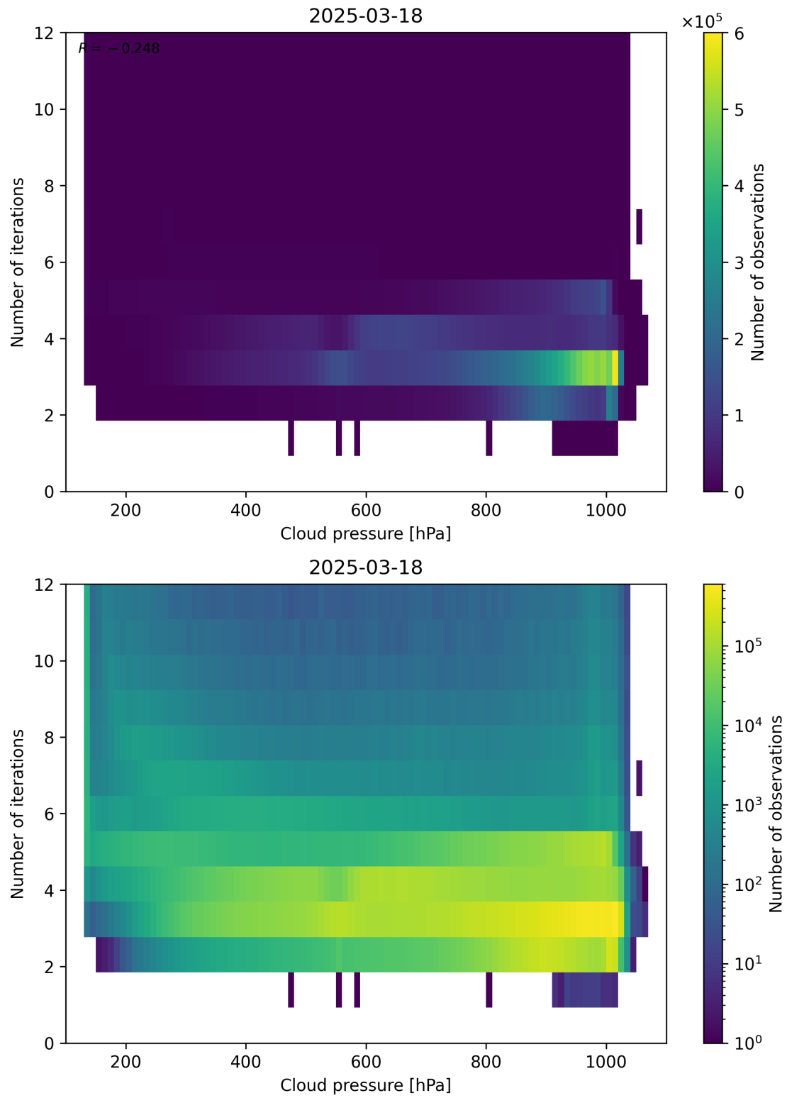
Figure 81: Scatter density plot of “Cloud pressure” against “Number of iterations” for 2025-03-17 to 2025-03-19.
