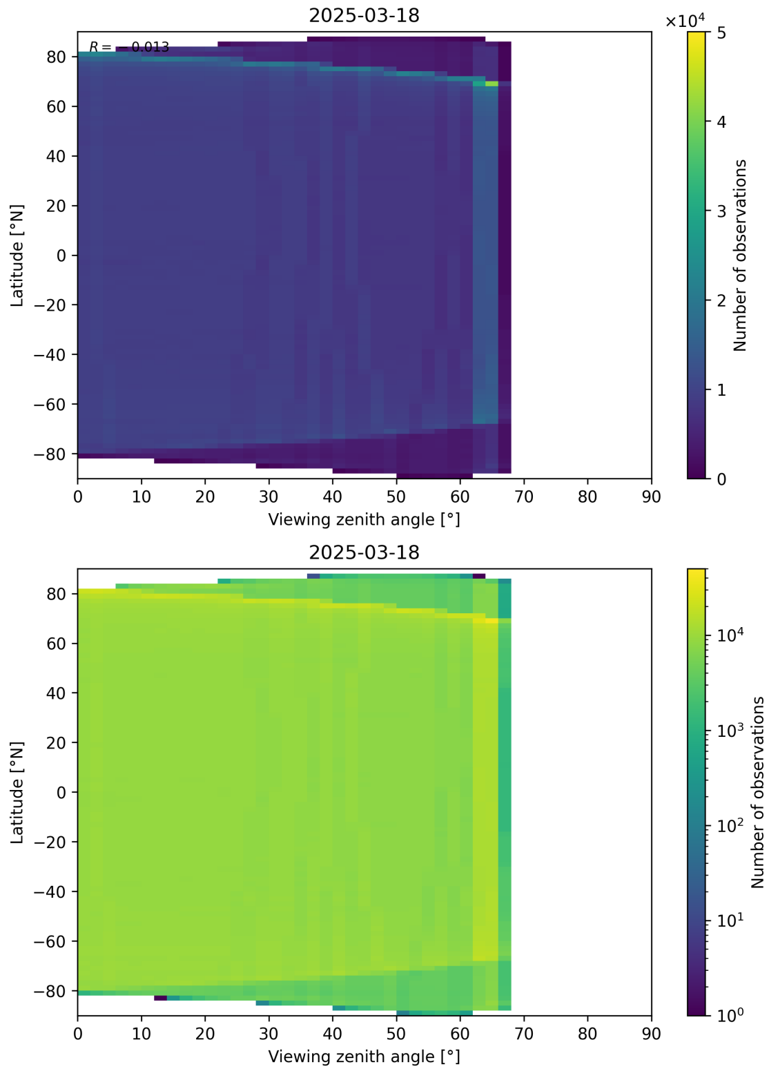
Figure 123: Scatter density plot of “Viewing zenith angle” against “Latitude” for 2025-03-17 to 2025-03-19.
