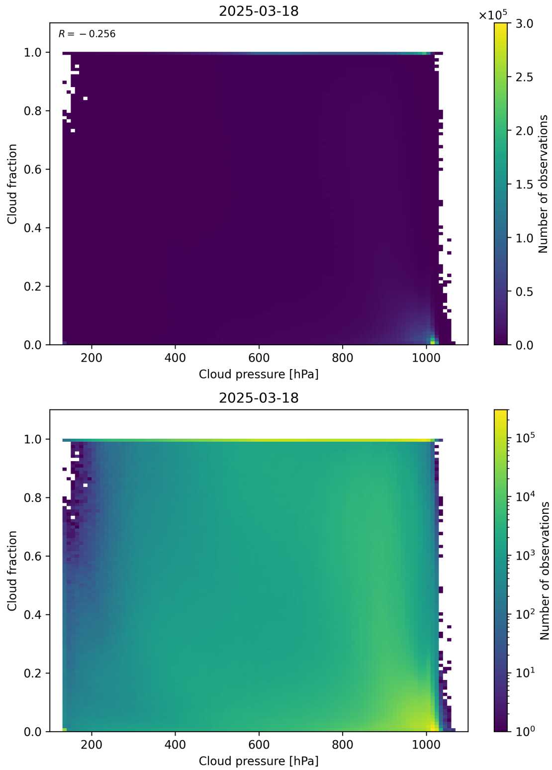
Figure 79: Scatter density plot of “Cloud pressure” against “Cloud fraction” for 2025-03-17 to 2025-03-19.
