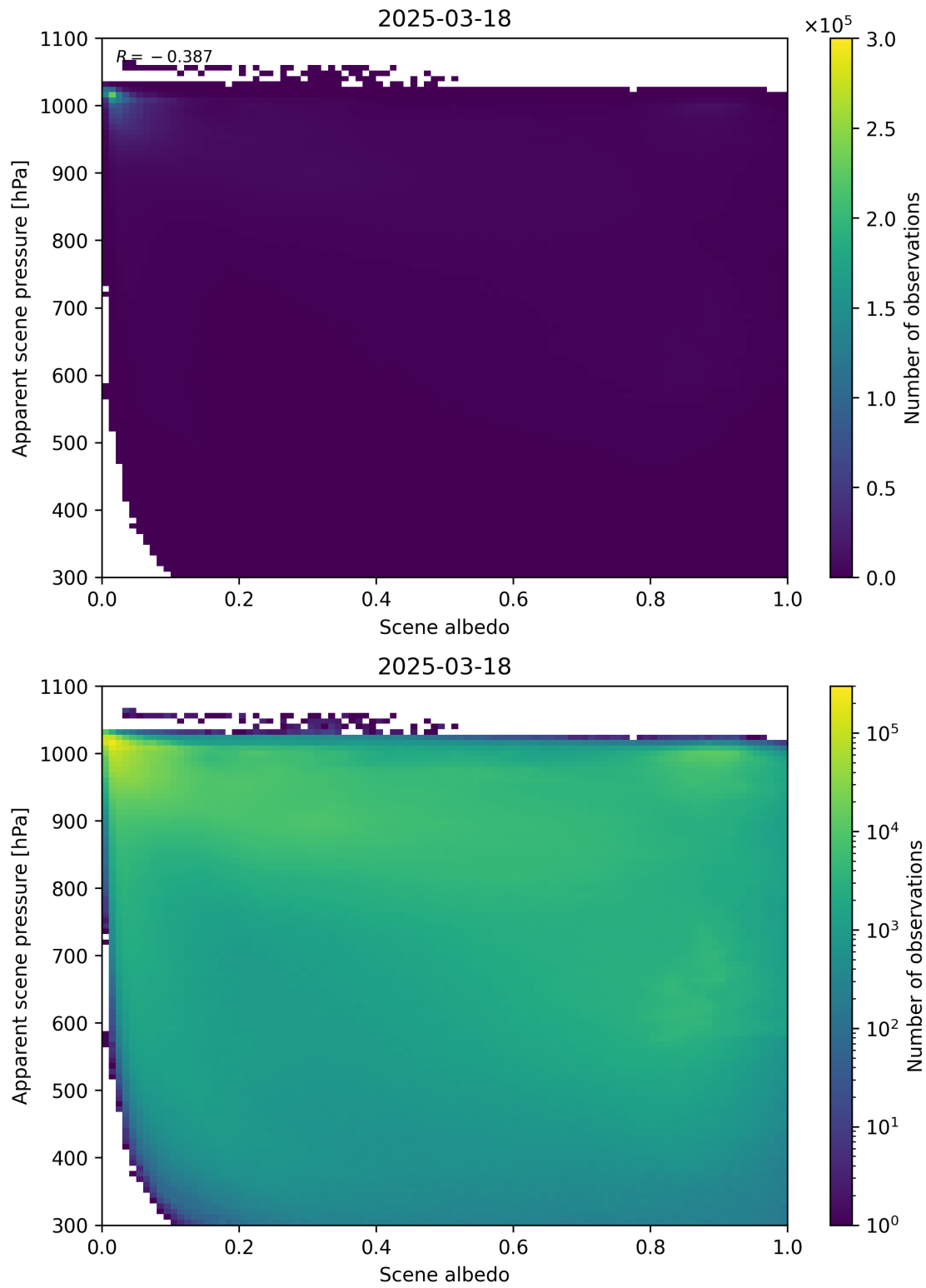
Figure 102: Scatter density plot of “Scene albedo” against “Apparent scene pressure” for 2025-03-17 to 2025-03-19.
