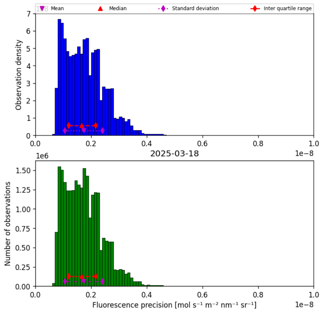
Figure 41: Histogram of “Fluorescence precision” for 2025-03-17 to 2025-03-19
