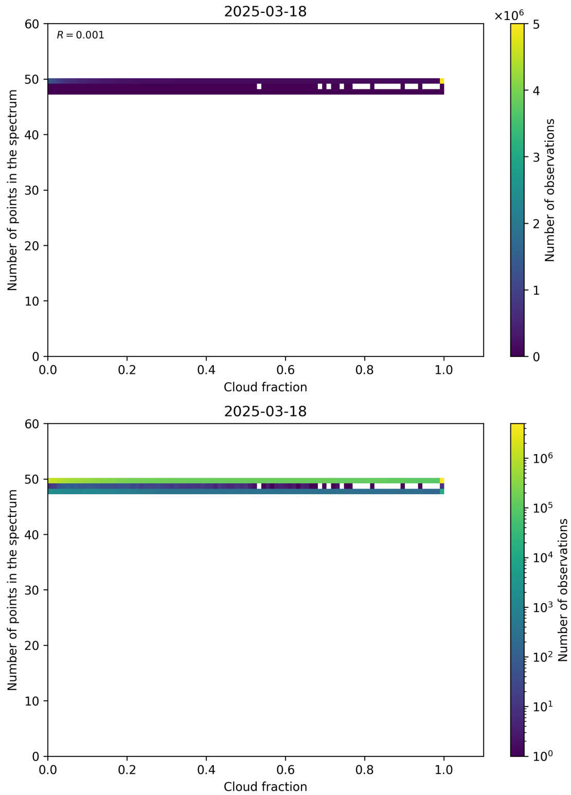
Figure 74: Scatter density plot of “Cloud fraction” against “Number of points in the spectrum” for 2025-03-17 to 2025-03-19.
