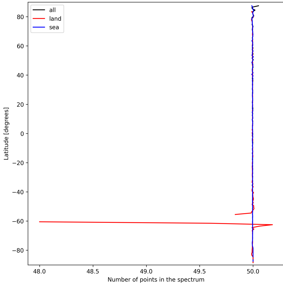
Figure 27: Zonal average of “Number of points in the spectrum” for 2025-03-17 to 2025-03-19.
