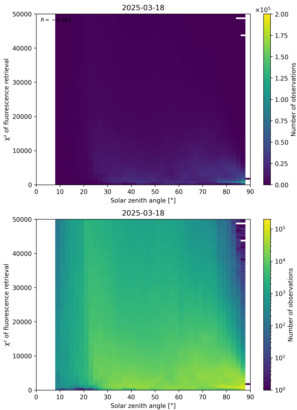
Figure 109: Scatter density plot of “Solar zenith angle” against “ \chi^2 of fluorescence retrieval” for 2025-03-17 to 2025-03-19.
