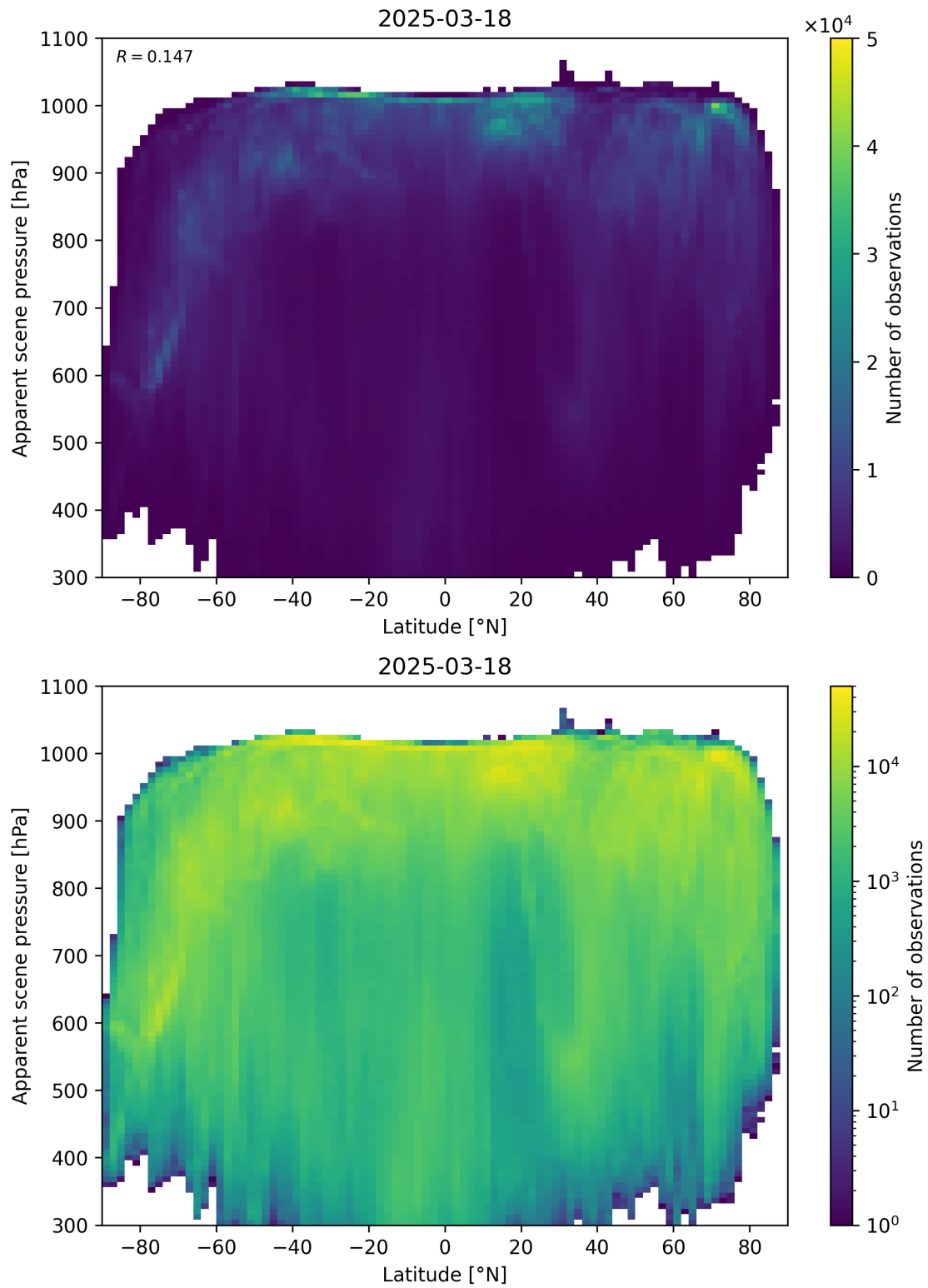
Figure 88: Scatter density plot of “Latitude” against “Apparent scene pressure” for 2025-03-17 to 2025-03-19.
