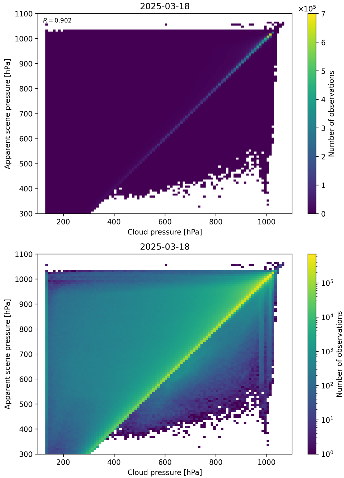
Figure 77: Scatter density plot of “Cloud pressure” against “Apparent scene pressure” for 2025-03-17 to 2025-03-19.
