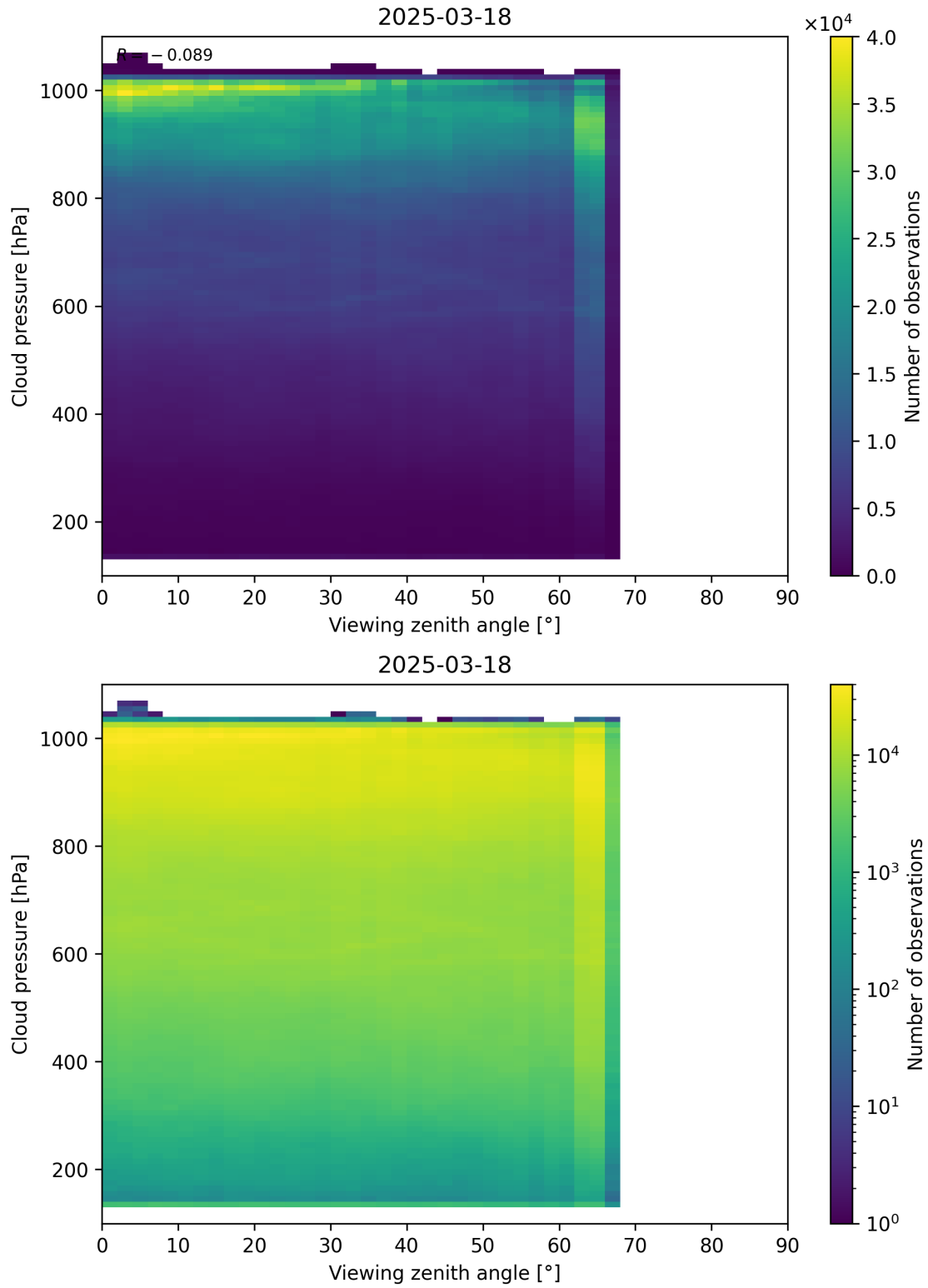
Figure 121: Scatter density plot of “Viewing zenith angle” against “Cloud pressure” for 2025-03-17 to 2025-03-19.
