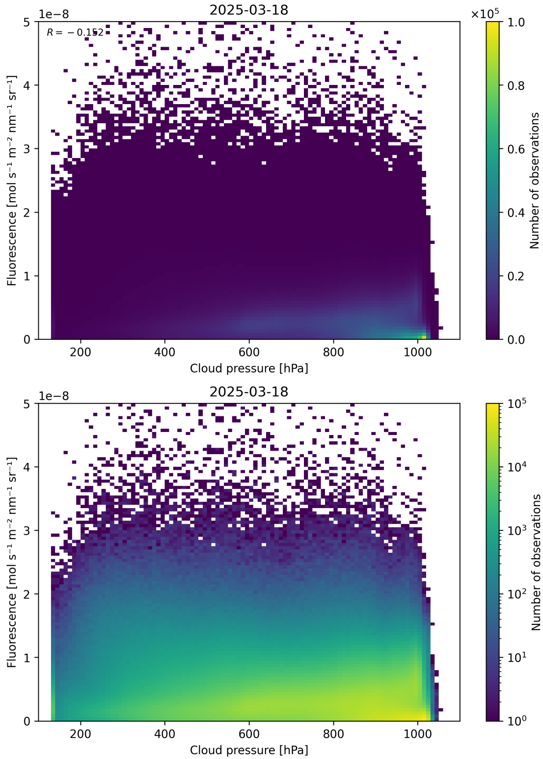
Figure 80: Scatter density plot of “Cloud pressure” against “Fluorescence” for 2025-03-17 to 2025-03-19.
