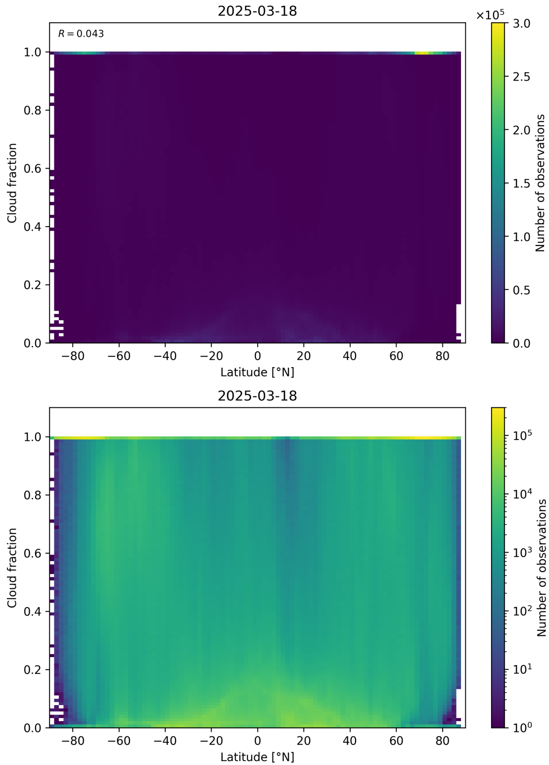
Figure 90: Scatter density plot of “Latitude” against “Cloud fraction” for 2025-03-17 to 2025-03-19.
