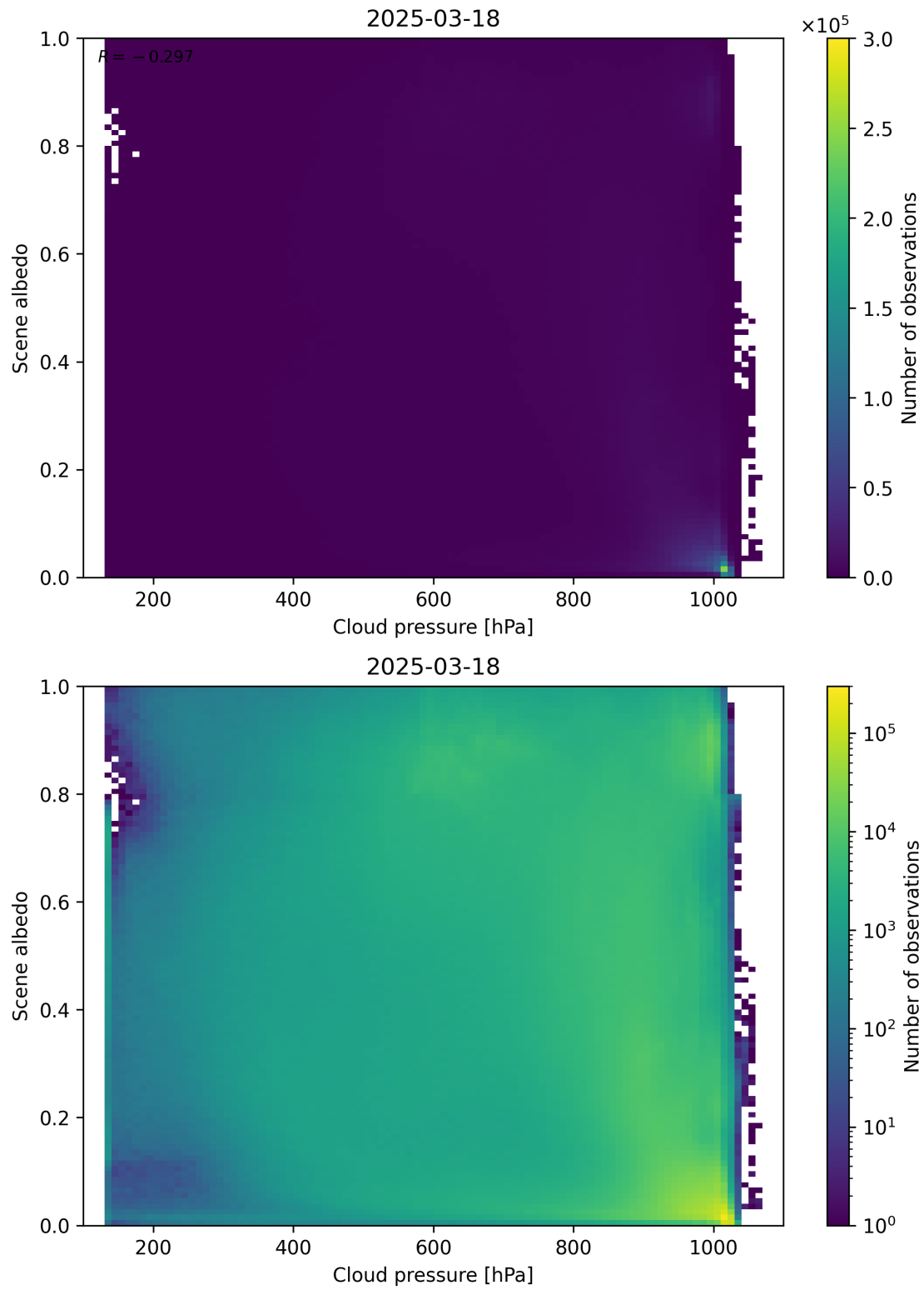
Figure 83: Scatter density plot of “Cloud pressure” against “Scene albedo” for 2025-03-17 to 2025-03-19.
