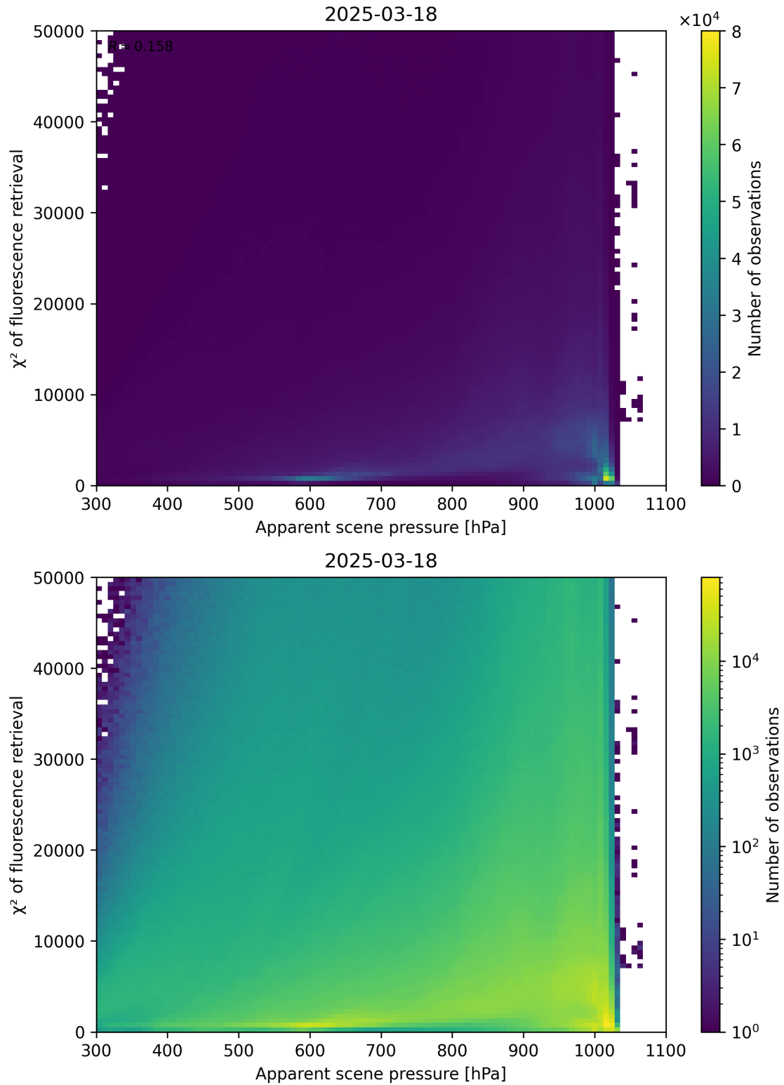
Figure 63: Scatter density plot of “Apparent scene pressure” against “ \chi^2 of fluorescence retrieval” for 2025-03-17 to 2025-03-19.
