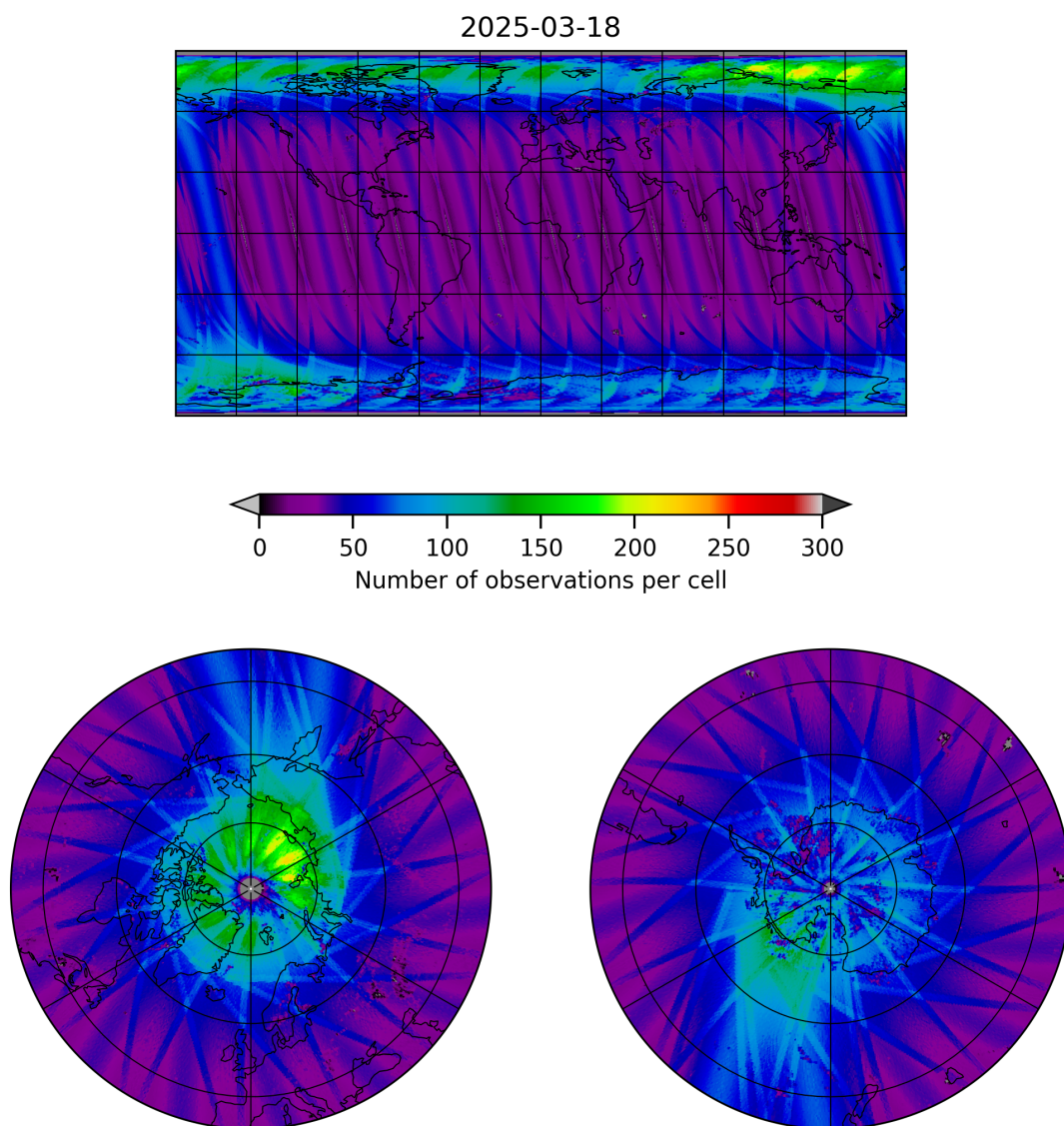
Figure 11: Map of the number of observations for 2025-03-17 to 2025-03-19
