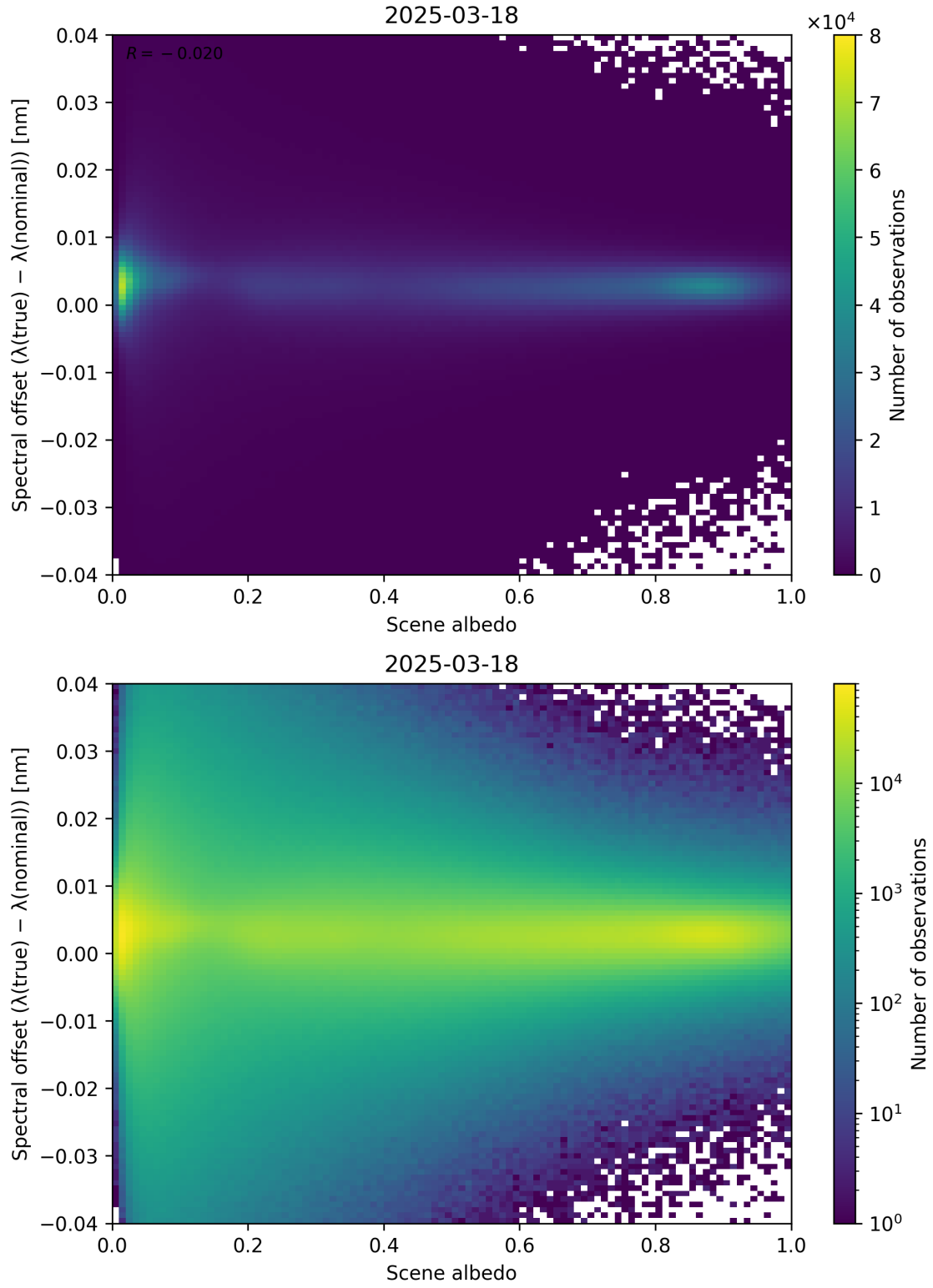
Figure 107: Scatter density plot of “Scene albedo” against “Spectral offset ( \lambda_{\text{true}} - \lambda_{\text{nominal}} )” for 2025-03-17 to 2025-03-19.
