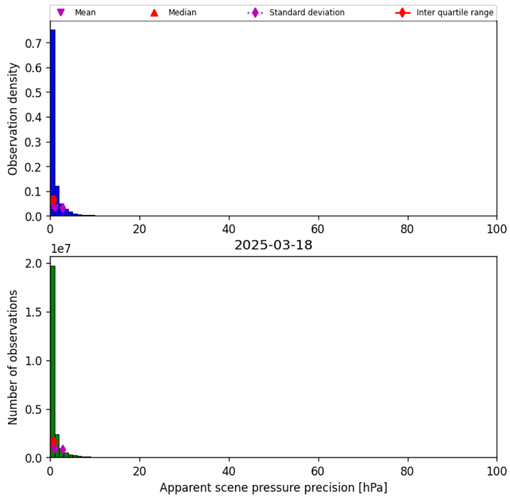
Figure 37: Histogram of “Apparent scene pressure precision” for 2025-03-17 to 2025-03-19
