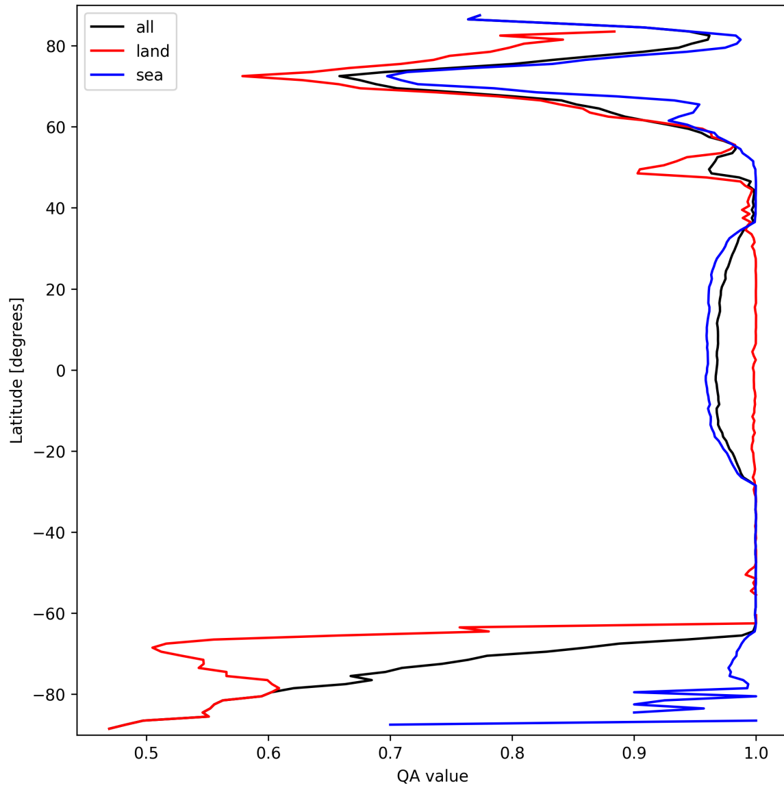
Figure 12: Zonal average of "QA value" for 2025-03-17 to 2025-03-19.
