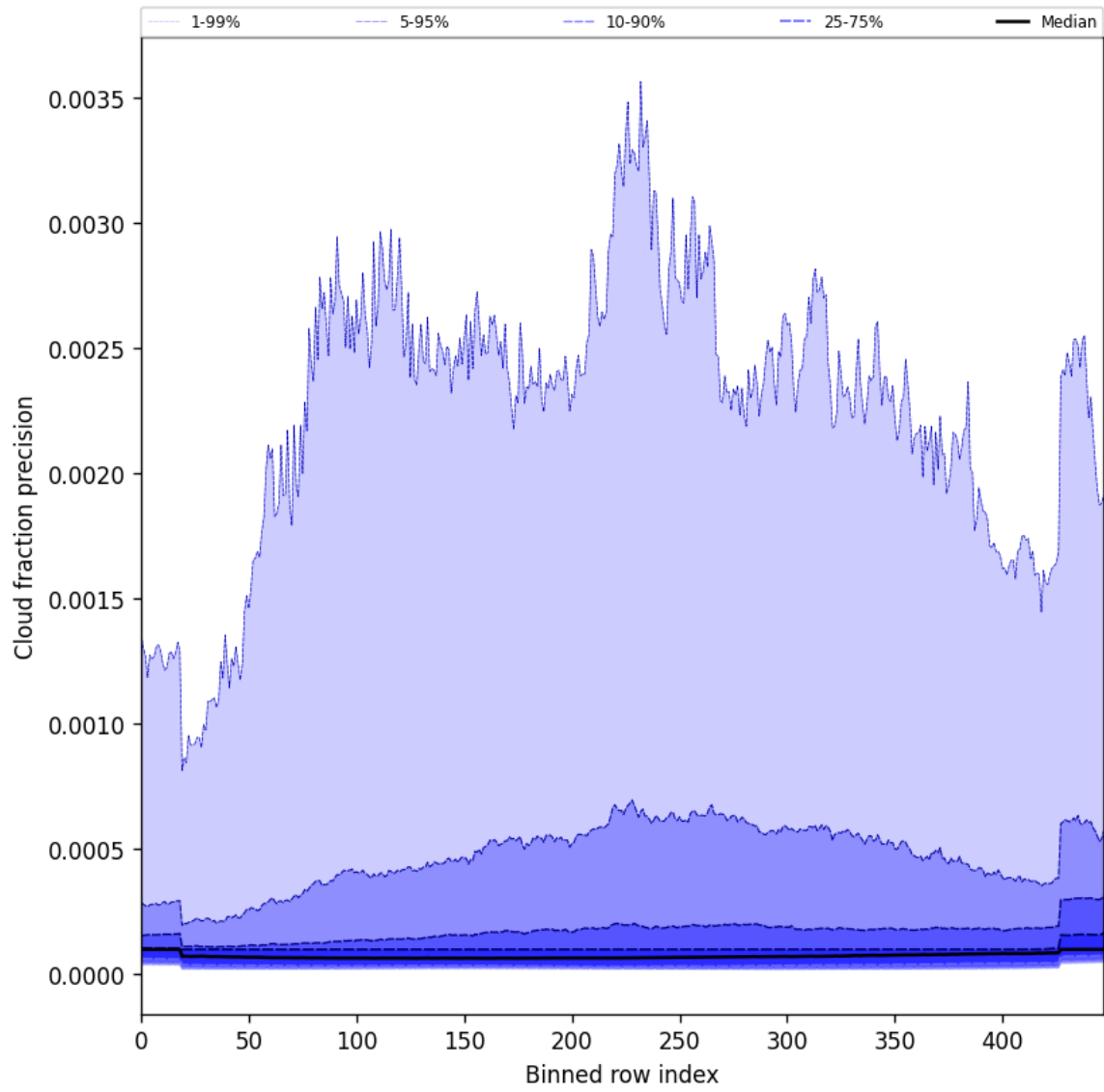
Figure 50: Along track statistics of “Cloud fraction precision” for 2025-03-17 to 2025-03-19
