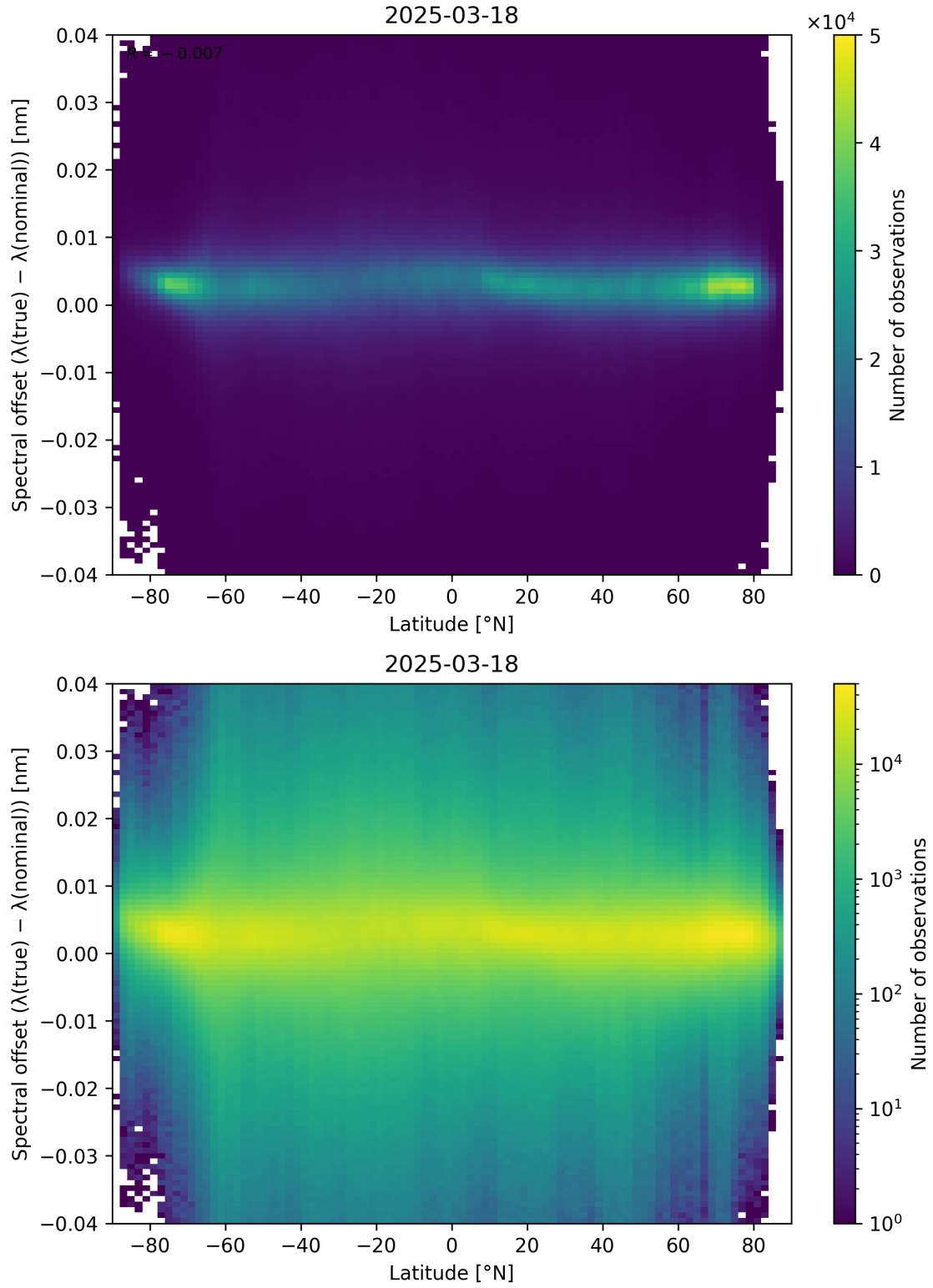
Figure 96: Scatter density plot of “Latitude” against “Spectral offset ( \lambda_{\text{true}} - \lambda_{\text{nominal}} )” for 2025-03-17 to 2025-03-19.
