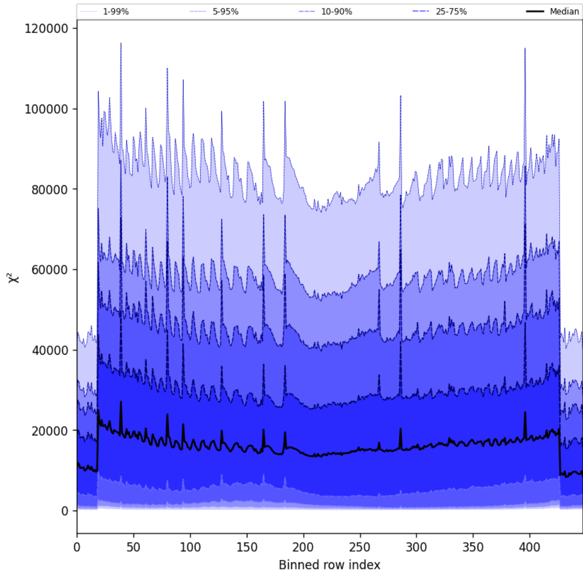
Figure 55: Along track statistics of “ \chi^2 ” for 2025-03-17 to 2025-03-19
