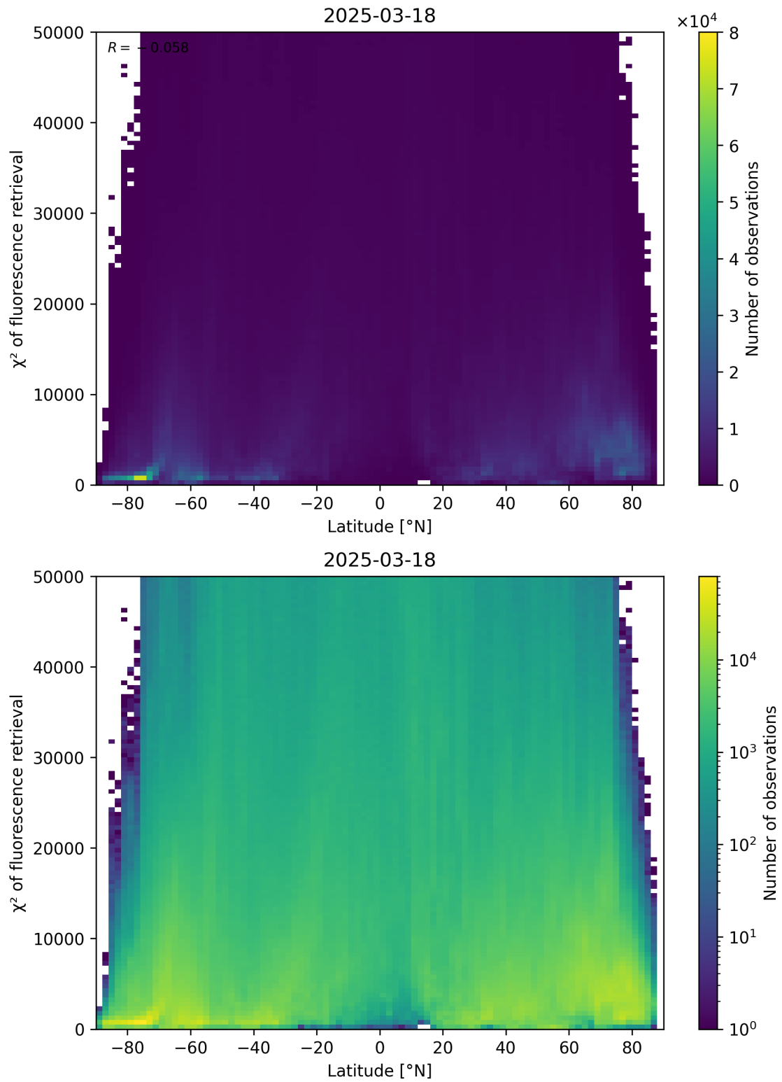
Figure 89: Scatter density plot of “Latitude” against “ \chi^2 of fluorescence retrieval” for 2025-03-17 to 2025-03-19.
