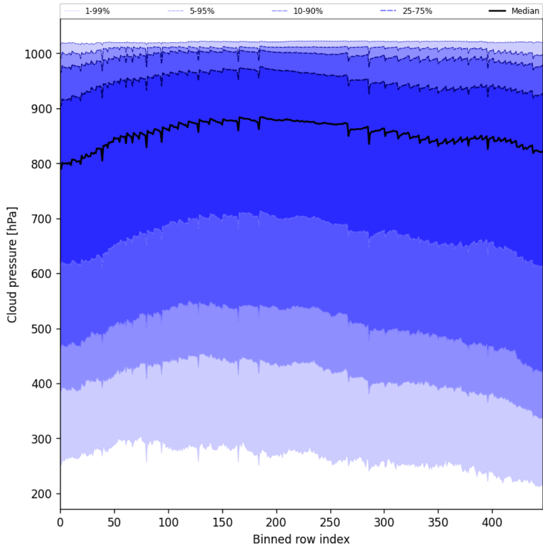
Figure 47: Along track statistics of “Cloud pressure” for 2025-03-17 to 2025-03-19
