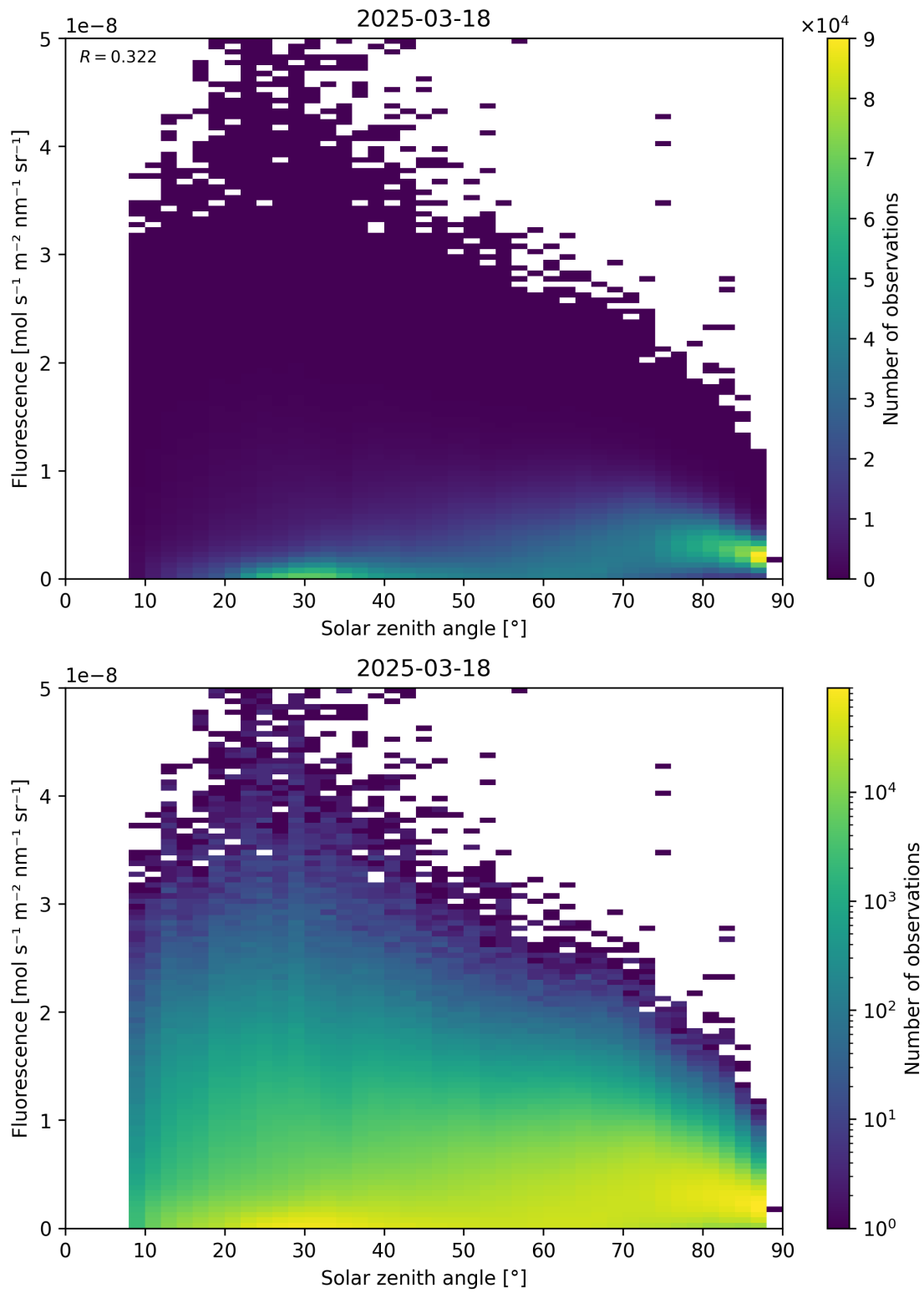
Figure 112: Scatter density plot of “Solar zenith angle” against “Fluorescence” for 2025-03-17 to 2025-03-19.
