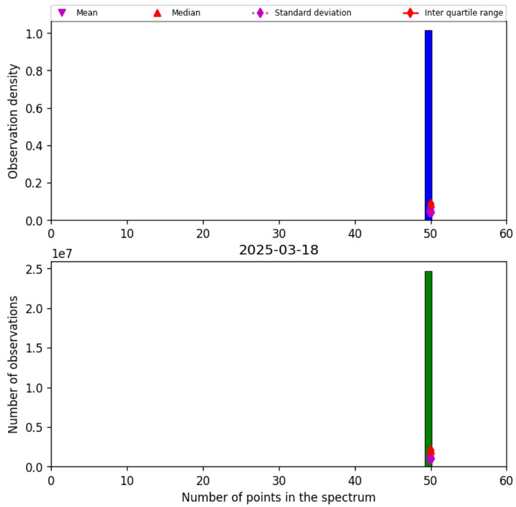
Figure 44: Histogram of “Number of points in the spectrum” for 2025-03-17 to 2025-03-19
