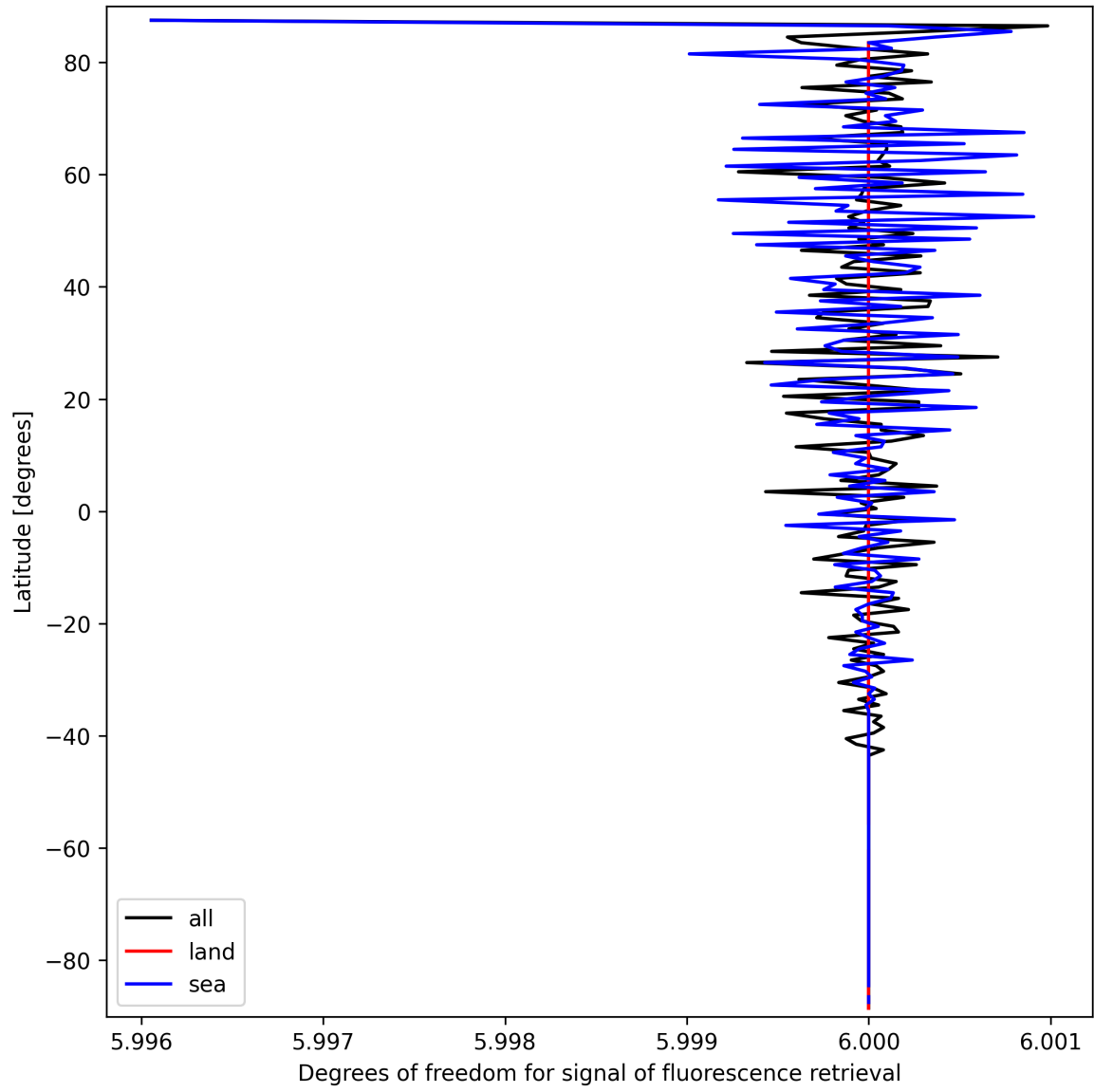
Figure 26: Zonal average of “Degrees of freedom for signal of fluorescence retrieval” for 2025-03-17 to 2025-03-19.
