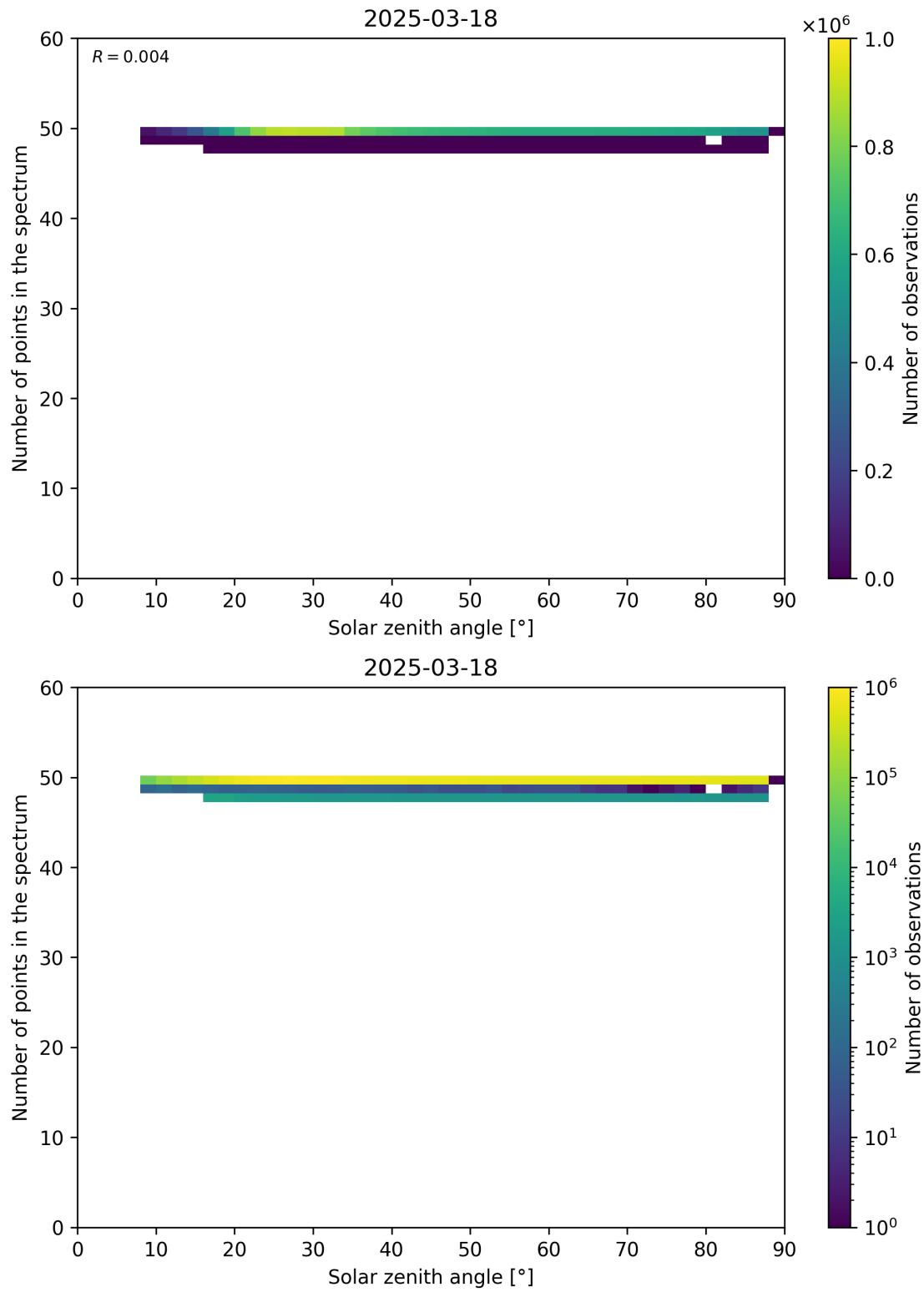
Figure 115: Scatter density plot of “Solar zenith angle” against “Number of points in the spectrum” for 2025-03-17 to 2025-03-19.
