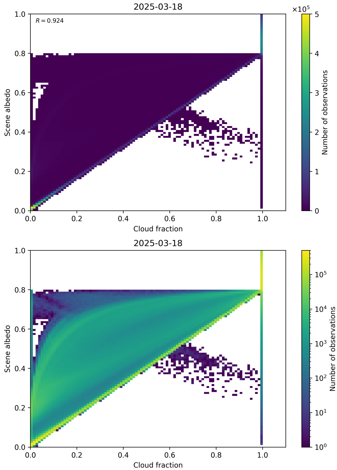
Figure 75: Scatter density plot of “Cloud fraction” against “Scene albedo” for 2025-03-17 to 2025-03-19.
