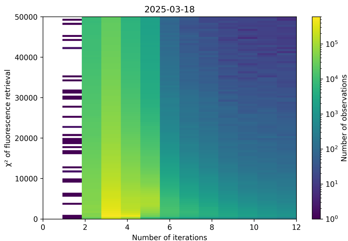
Figure 97: Scatter density plot of “Number of iterations” against “ \chi^2 of fluorescence retrieval” for 2025-03-17 to 2025-03-19.
