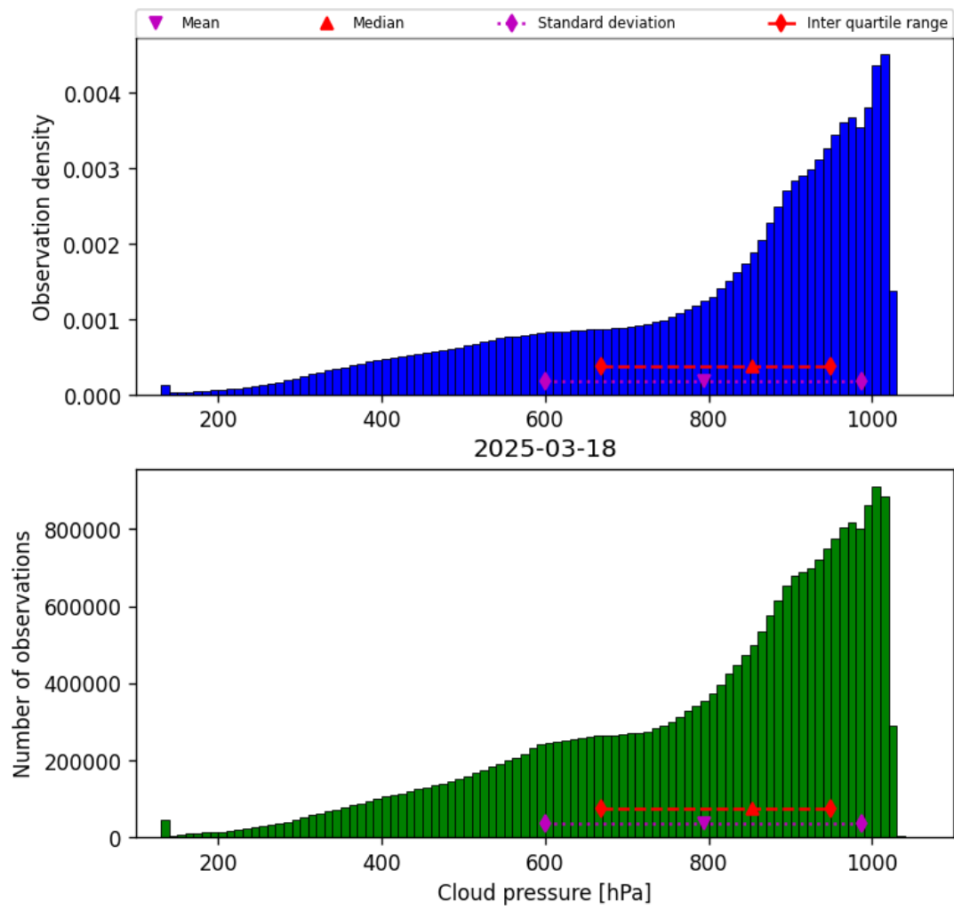
Figure 30: Histogram of “Cloud pressure” for 2025-03-17 to 2025-03-19
