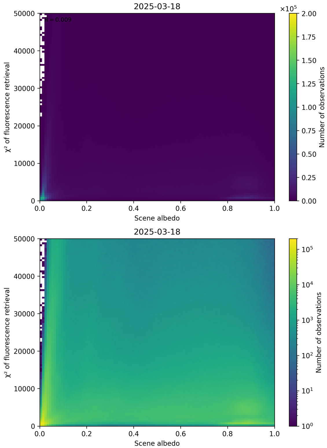
Figure 103: Scatter density plot of “Scene albedo” against “ \chi^2 of fluorescence retrieval” for 2025-03-17 to 2025-03-19.
