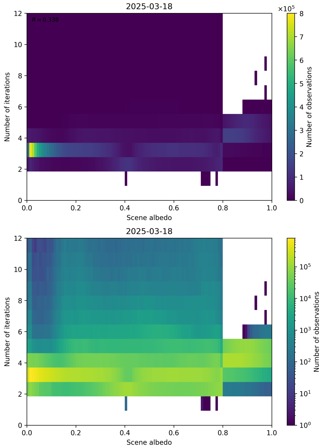
Figure 105: Scatter density plot of “Scene albedo” against “Number of iterations” for 2025-03-17 to 2025-03-19.
