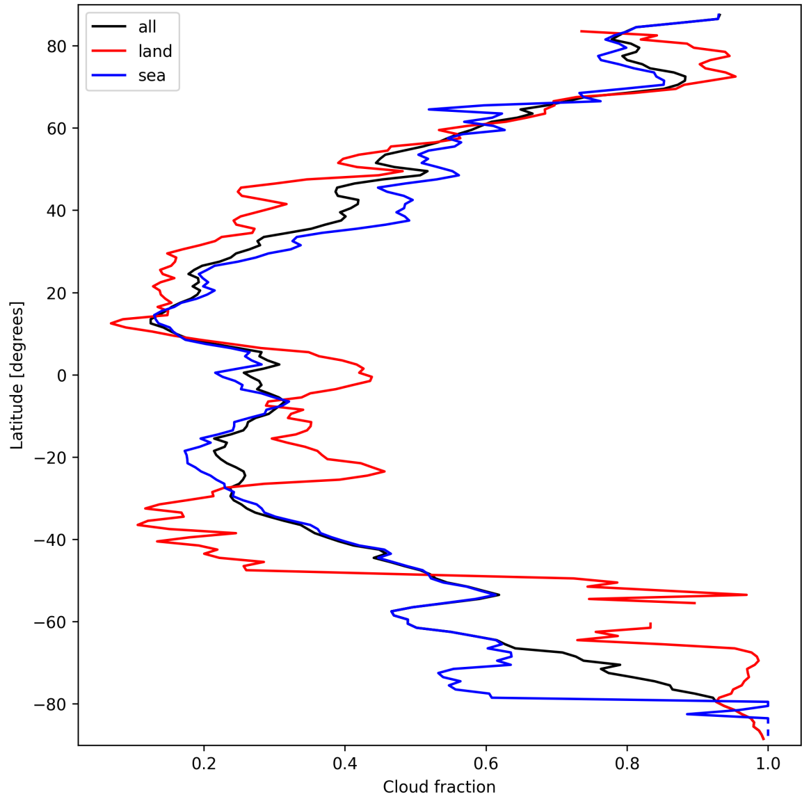
Figure 15: Zonal average of “Cloud fraction” for 2025-03-17 to 2025-03-19.
