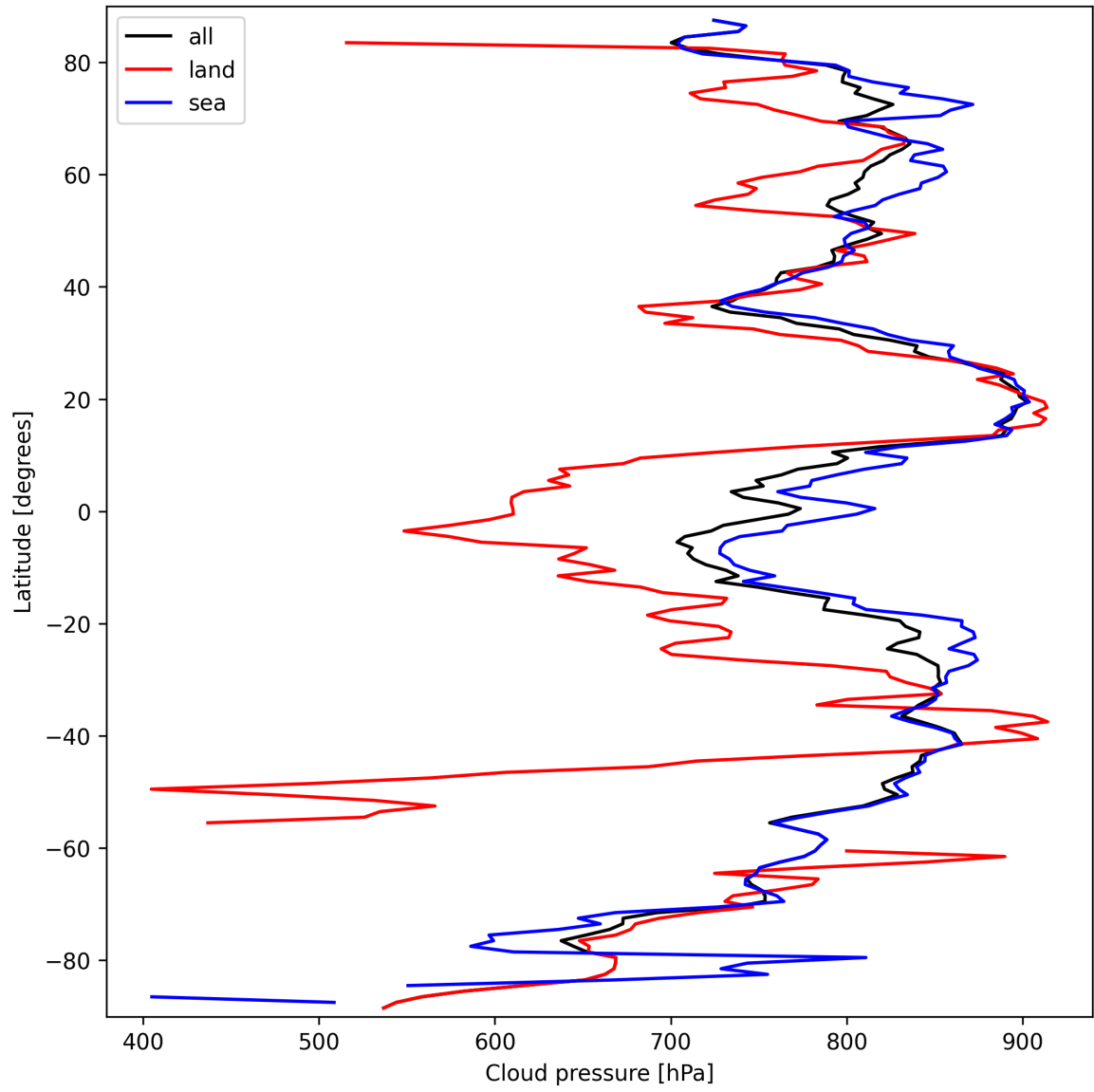
Figure 13: Zonal average of “Cloud pressure” for 2025-03-17 to 2025-03-19.
