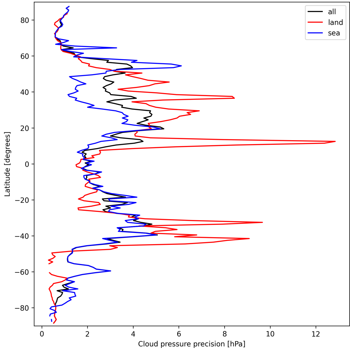
Figure 14: Zonal average of “Cloud pressure precision” for 2025-03-17 to 2025-03-19.
