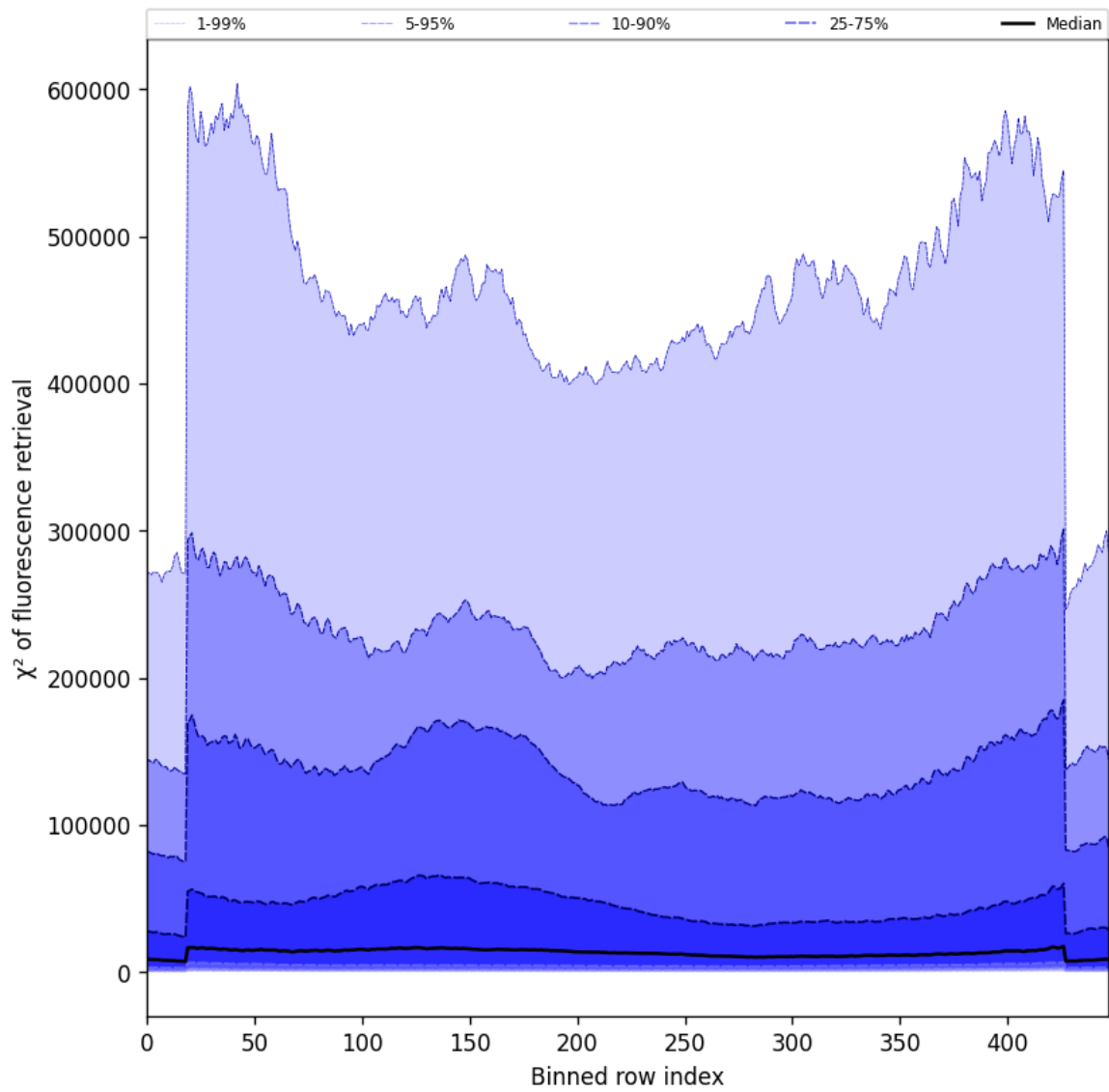
Figure 59: Along track statistics of “ \chi^2 of fluorescence retrieval” for 2025-03-17 to 2025-03-19
