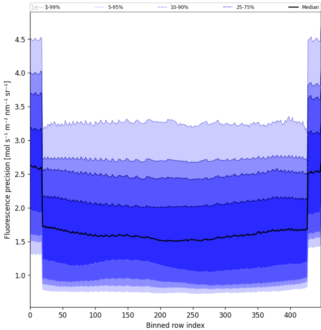
Figure 58: Along track statistics of “Fluorescence precision” for 2025-03-17 to 2025-03-19
