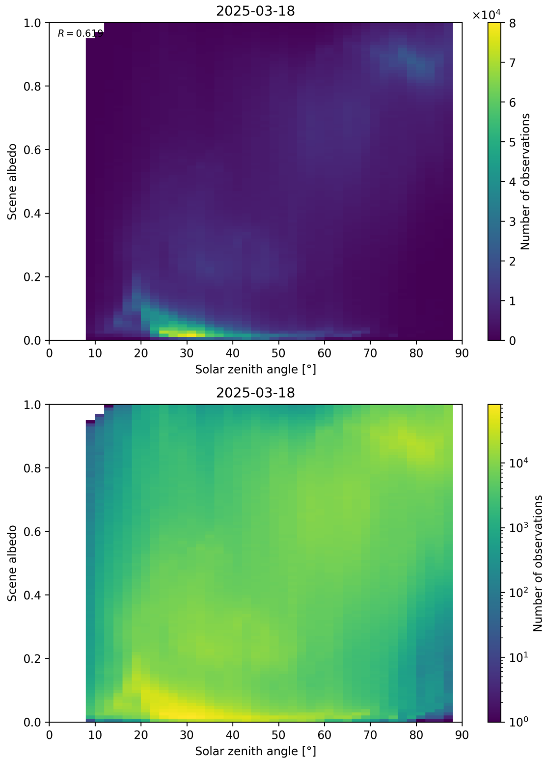
Figure 116: Scatter density plot of “Solar zenith angle” against “Scene albedo” for 2025-03-17 to 2025-03-19.
