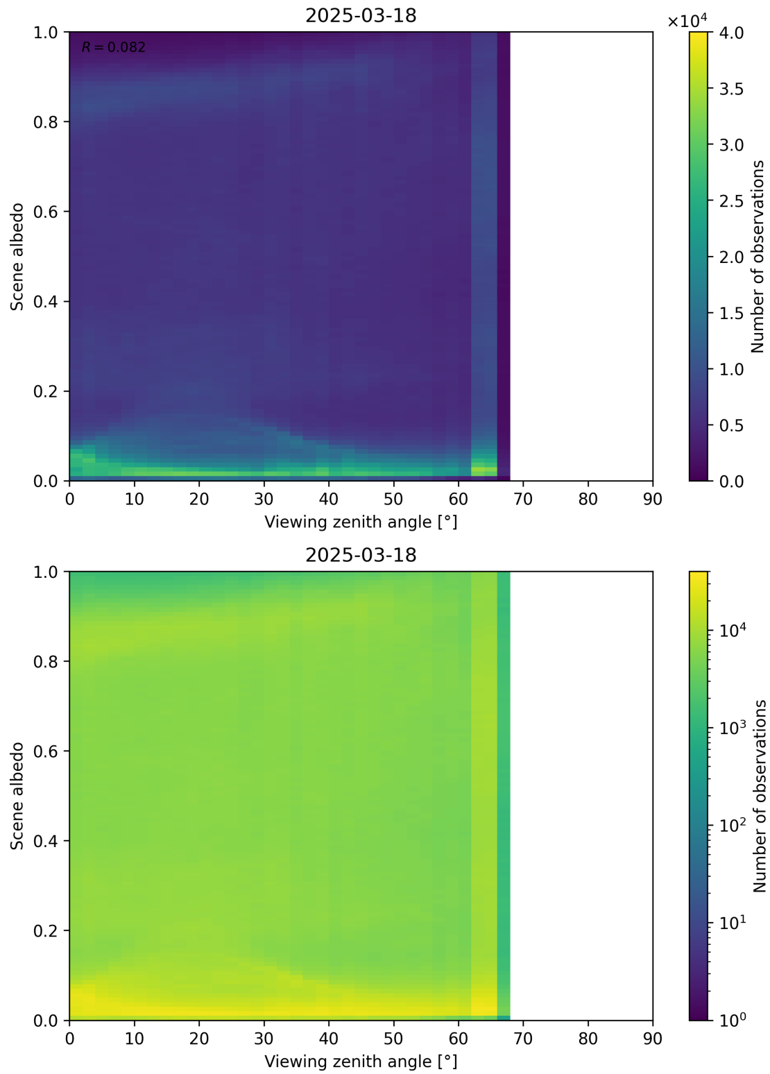
Figure 126: Scatter density plot of “Viewing zenith angle” against “Scene albedo” for 2025-03-17 to 2025-03-19.
