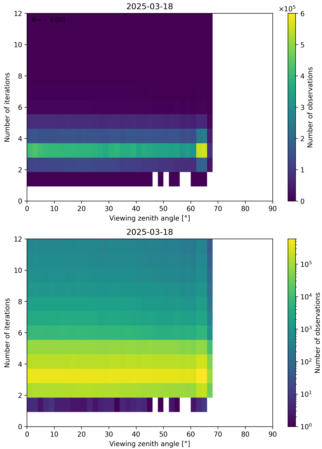
Figure 124: Scatter density plot of “Viewing zenith angle” against “Number of iterations” for 2025-03-17 to 2025-03-19.
