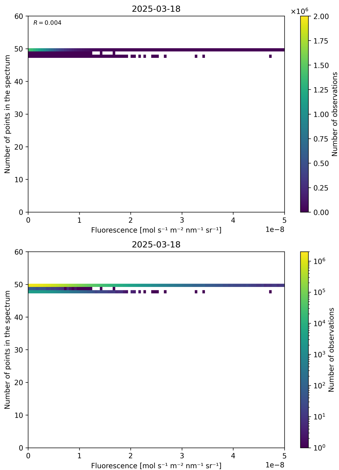
Figure 86: Scatter density plot of “Fluorescence” against “Number of points in the spectrum” for 2025-03-17 to 2025-03-19.
