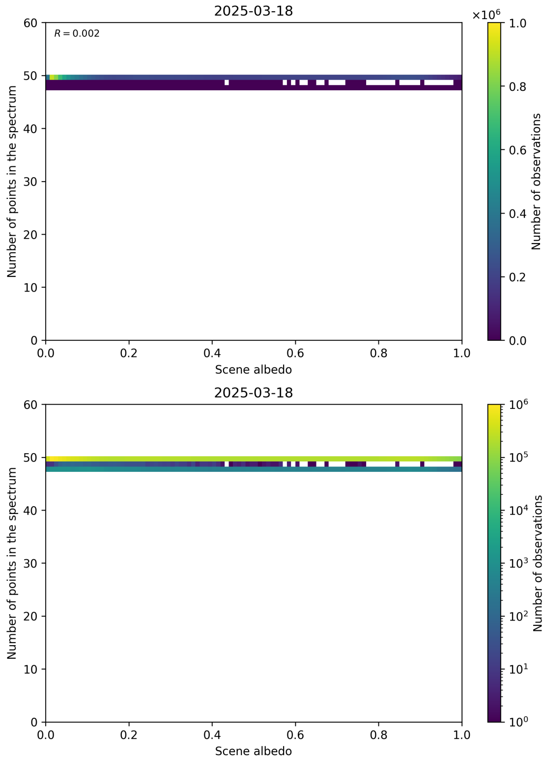
Figure 106: Scatter density plot of “Scene albedo” against “Number of points in the spectrum” for 2025-03-17 to 2025-03-19.
