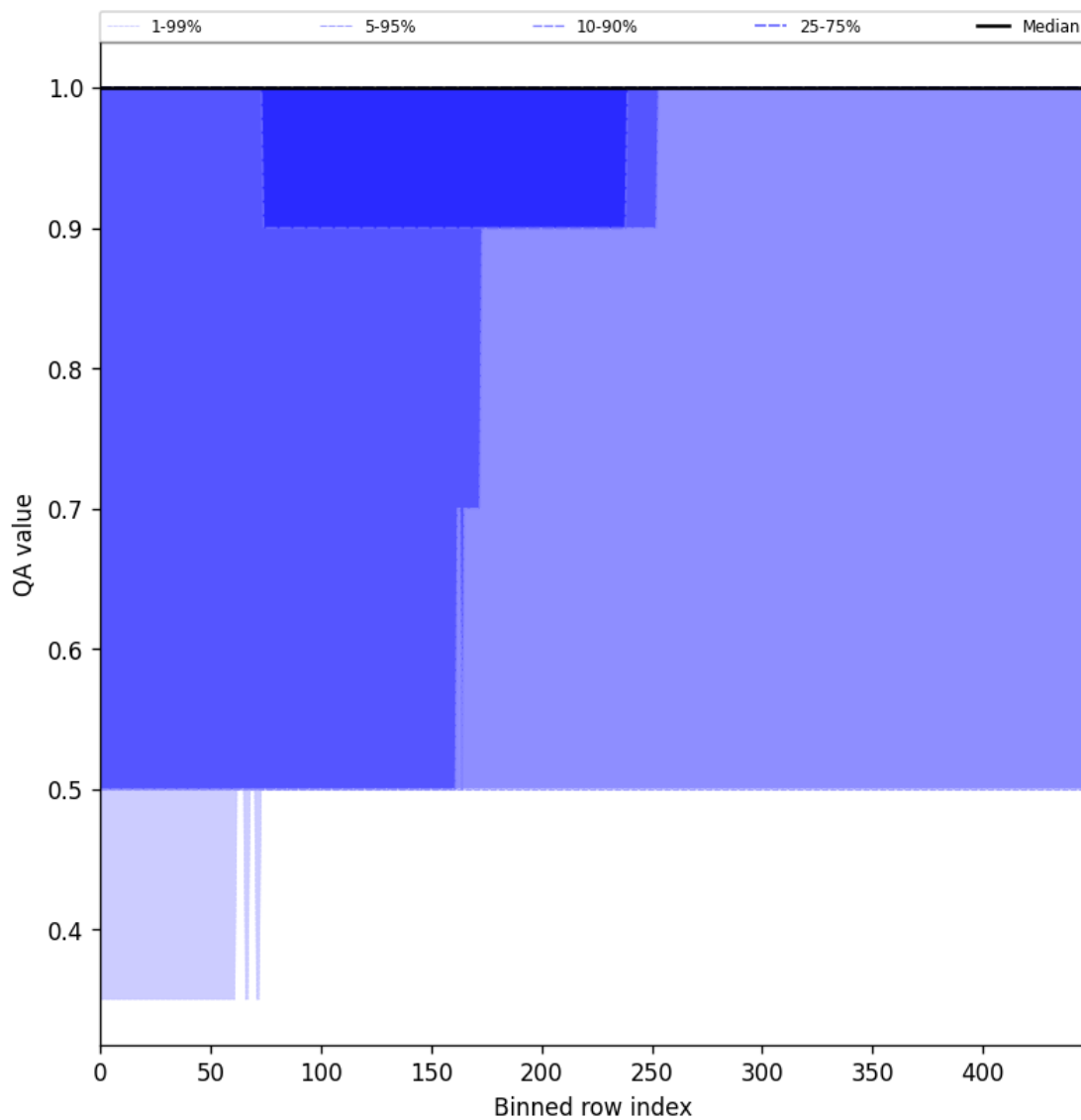
Figure 46: Along track statistics of “QA value” for 2025-03-17 to 2025-03-19
