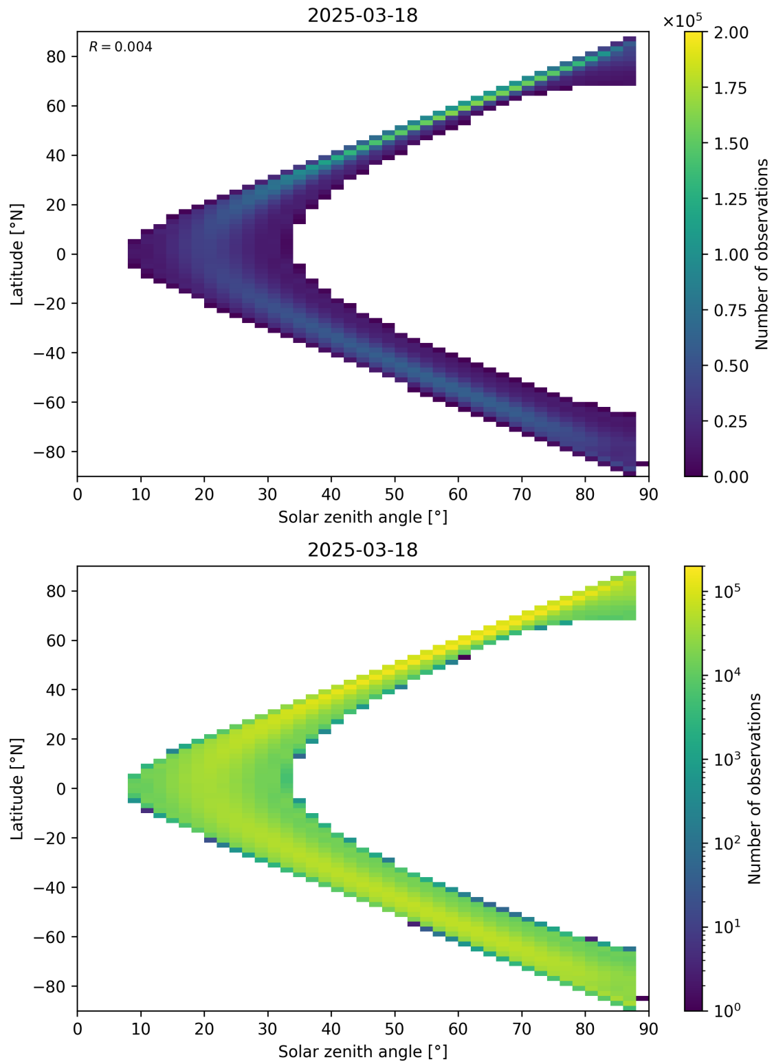
Figure 113: Scatter density plot of “Solar zenith angle” against “Latitude” for 2025-03-17 to 2025-03-19.
