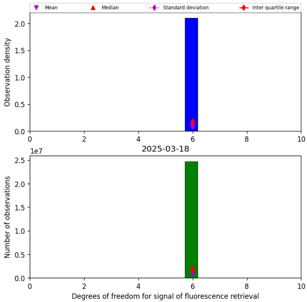
Figure 43: Histogram of “Degrees of freedom for signal of fluorescence retrieval” for 2025-03-17 to 2025-03-19
