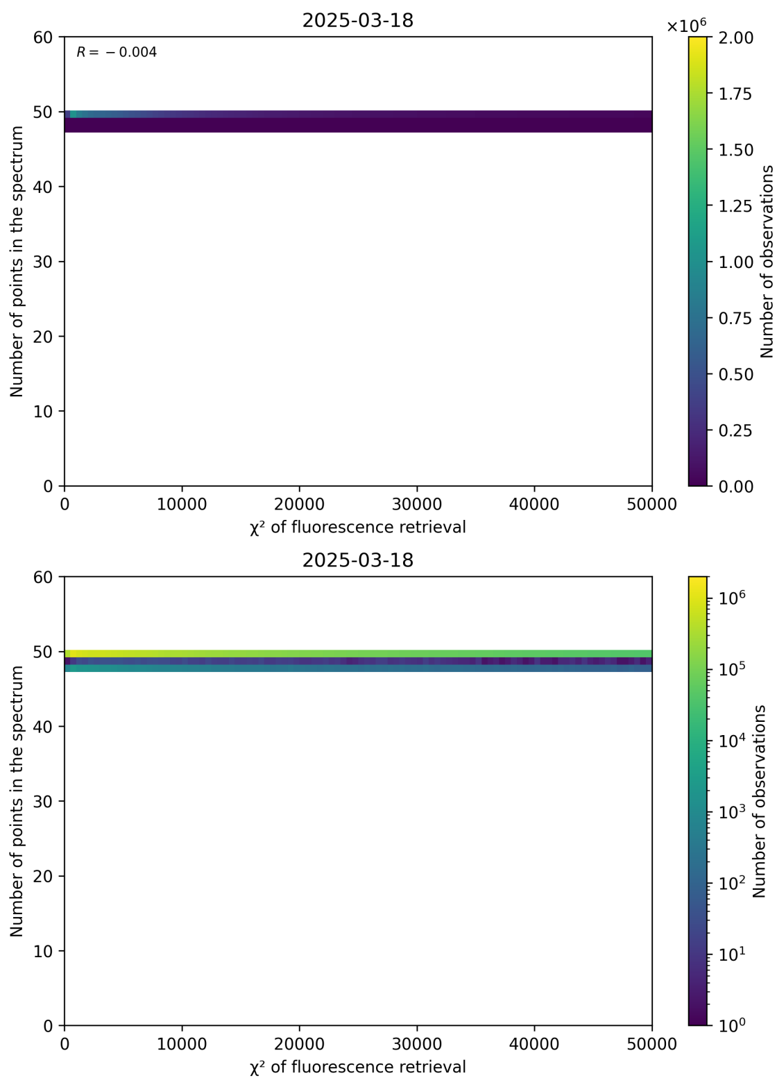
Figure 68: Scatter density plot of “ \chi^2 of fluorescence retrieval” against “Number of points in the spectrum” for 2025-03-17 to 2025-03-19.
