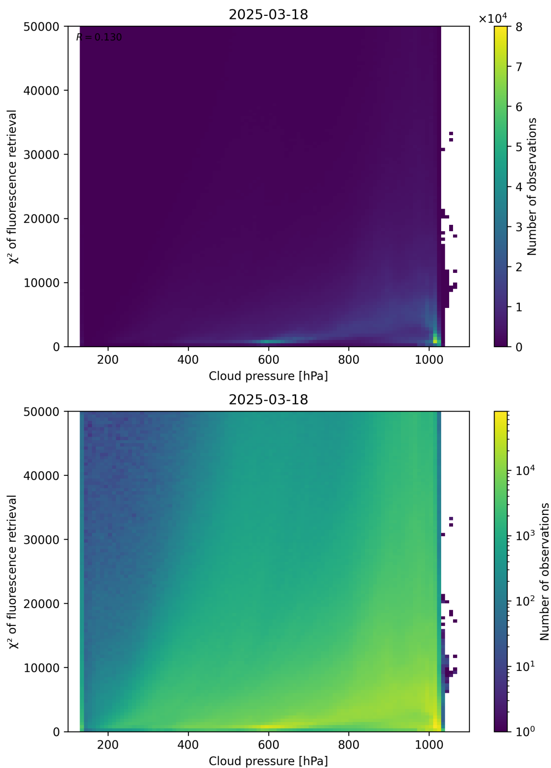
Figure 78: Scatter density plot of “Cloud pressure” against “ \chi^2 of fluorescence retrieval” for 2025-03-17 to 2025-03-19.
