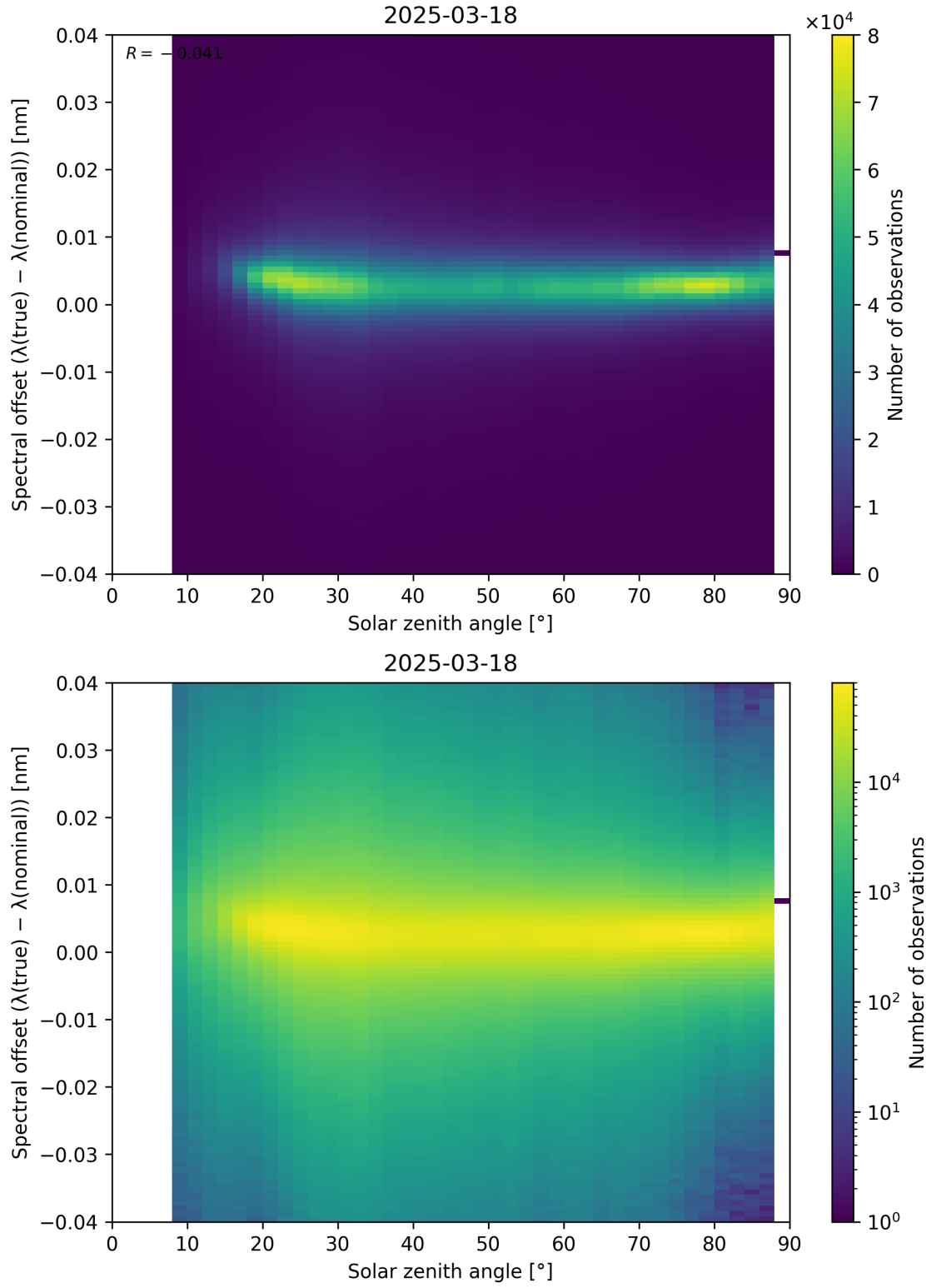
Figure 117: Scatter density plot of “Solar zenith angle” against “Spectral offset ( \lambda_{\text{true}} - \lambda_{\text{nominal}} )” for 2025-03-17 to 2025-03-19.
