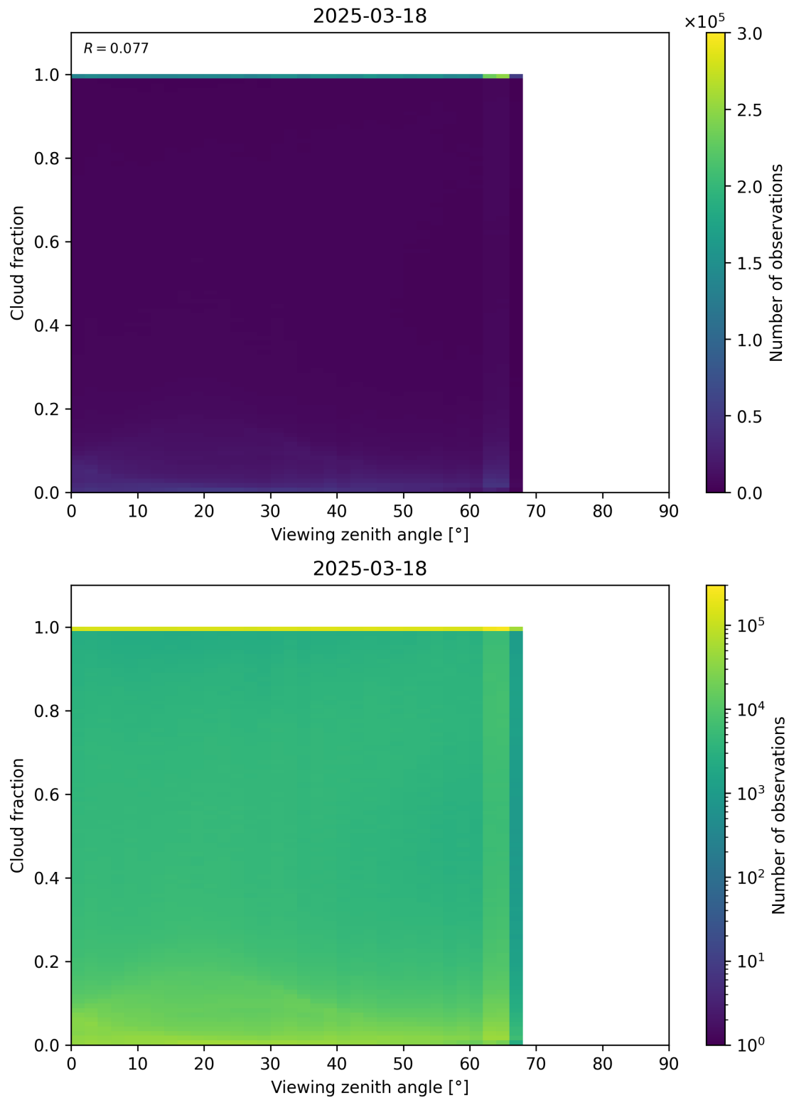
Figure 120: Scatter density plot of “Viewing zenith angle” against “Cloud fraction” for 2025-03-17 to 2025-03-19.
