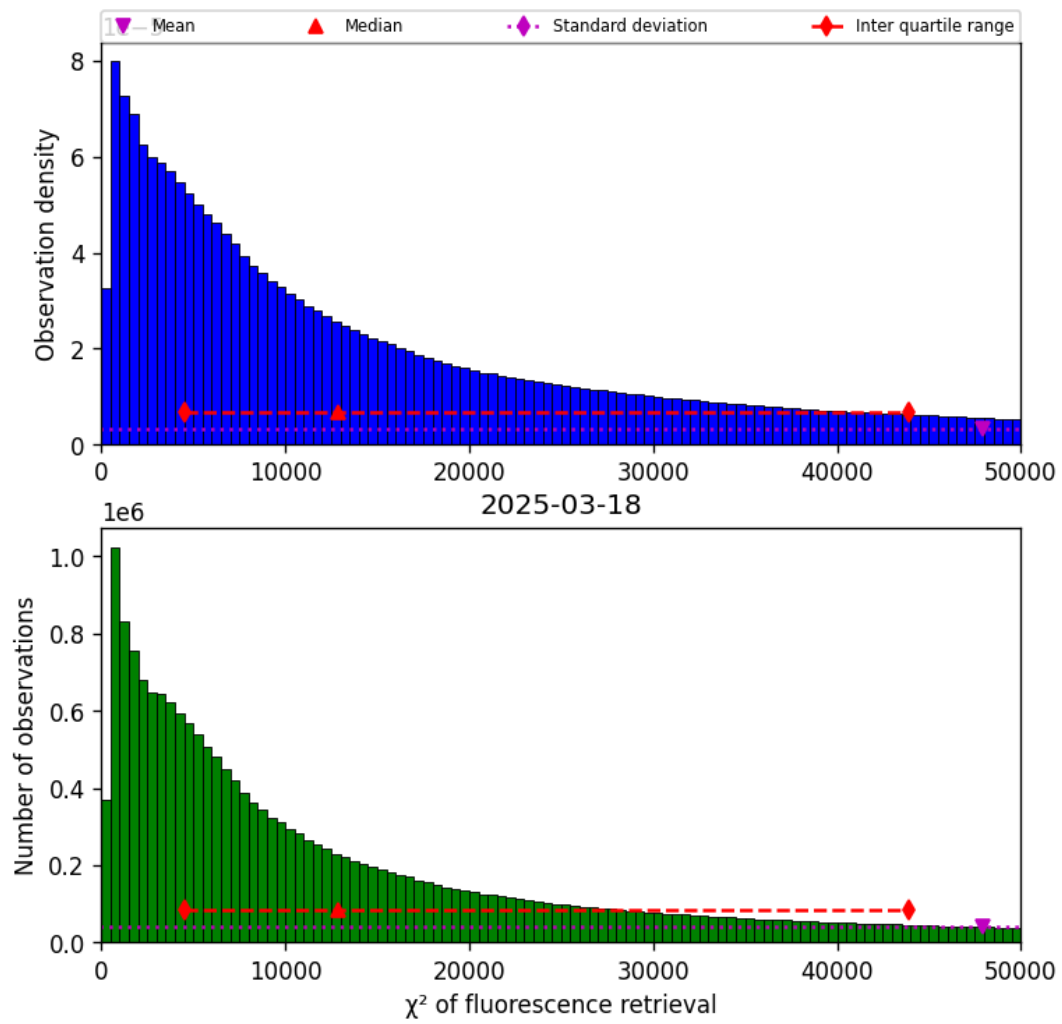
Figure 42: Histogram of “ \chi^2 of fluorescence retrieval” for 2025-03-17 to 2025-03-19
