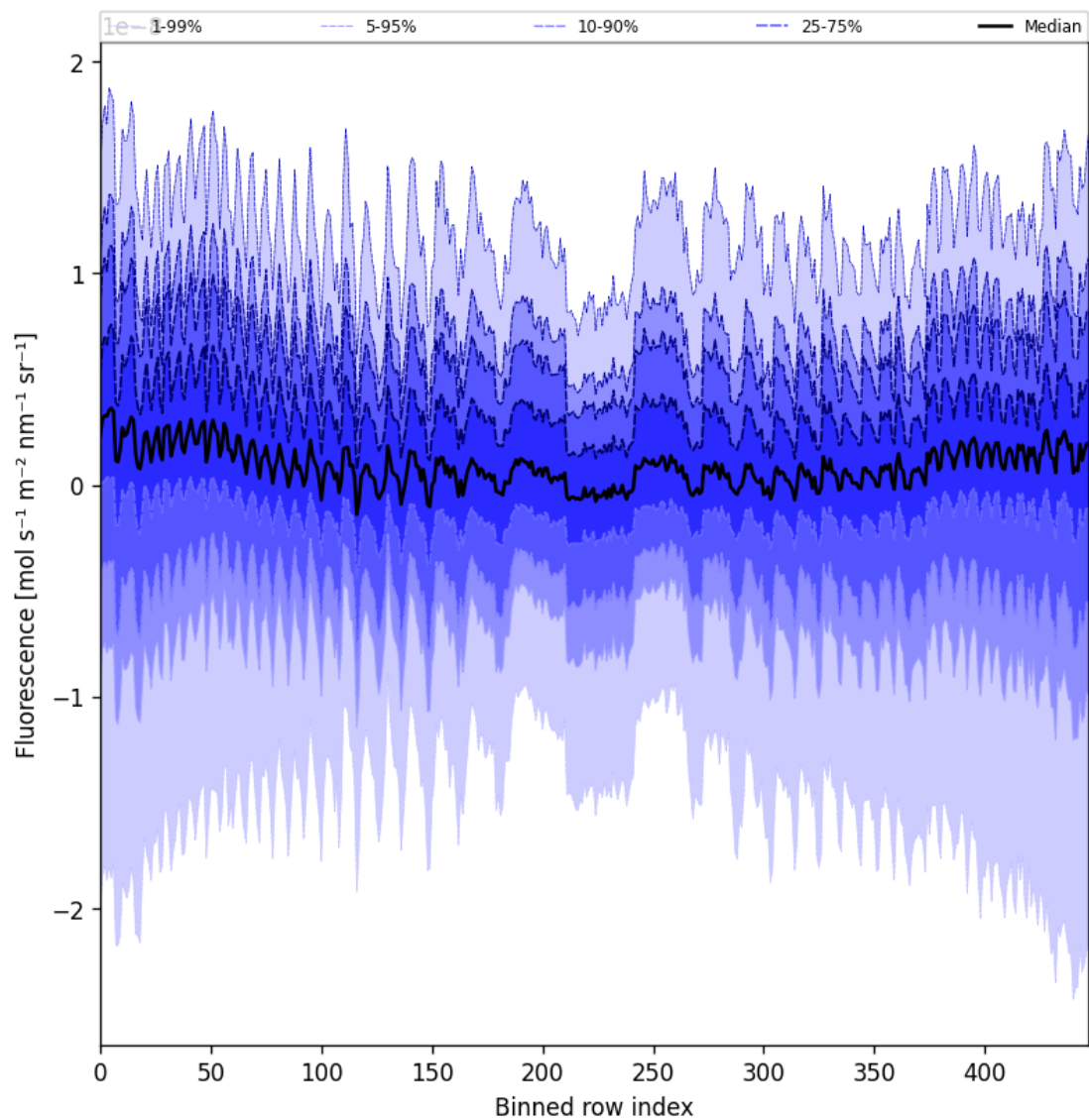
Figure 57: Along track statistics of “Fluorescence” for 2025-03-17 to 2025-03-19
