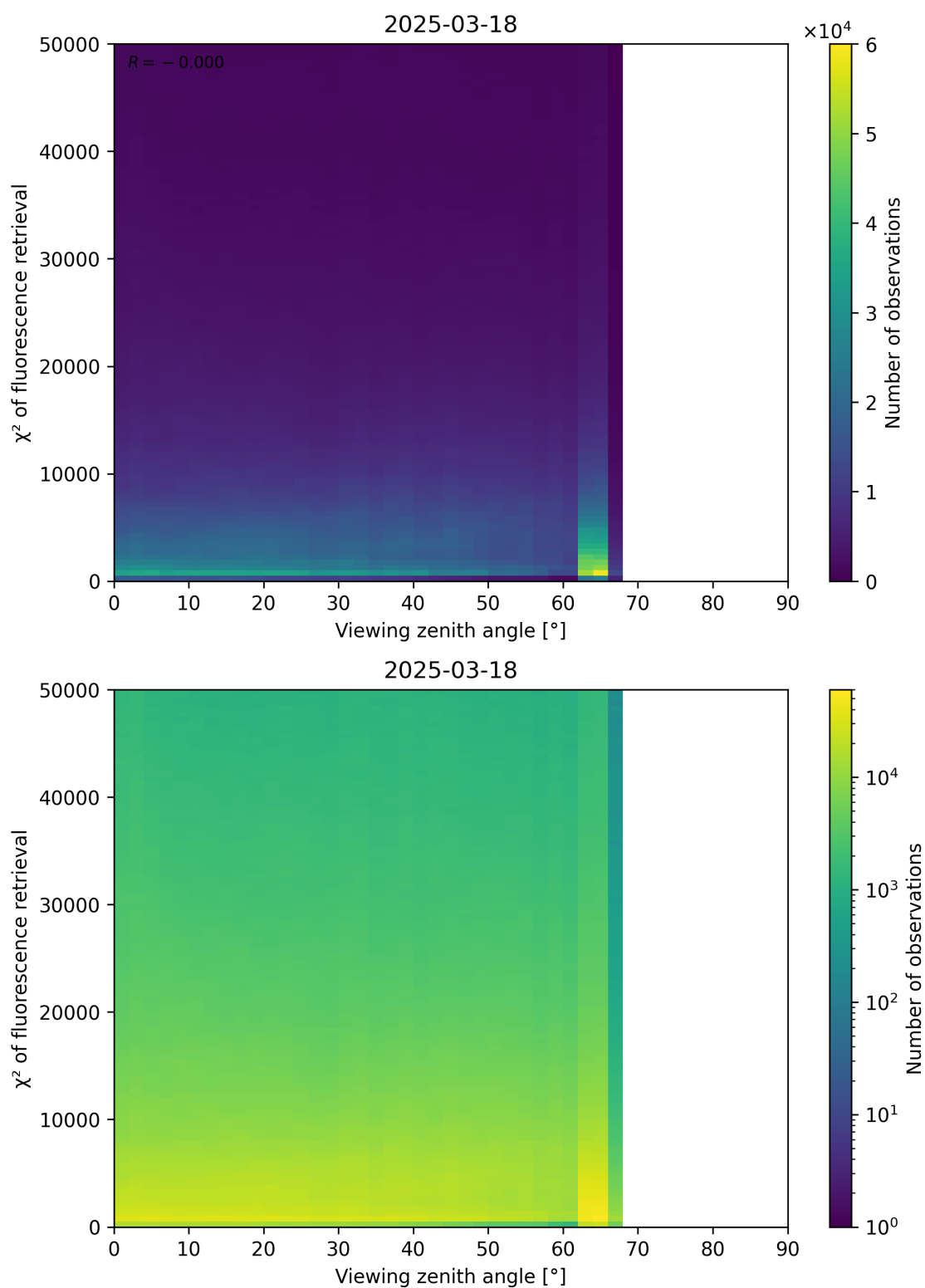
Figure 119: Scatter density plot of “Viewing zenith angle” against “ \chi^2 of fluorescence retrieval” for 2025-03-17 to 2025-03-19.
