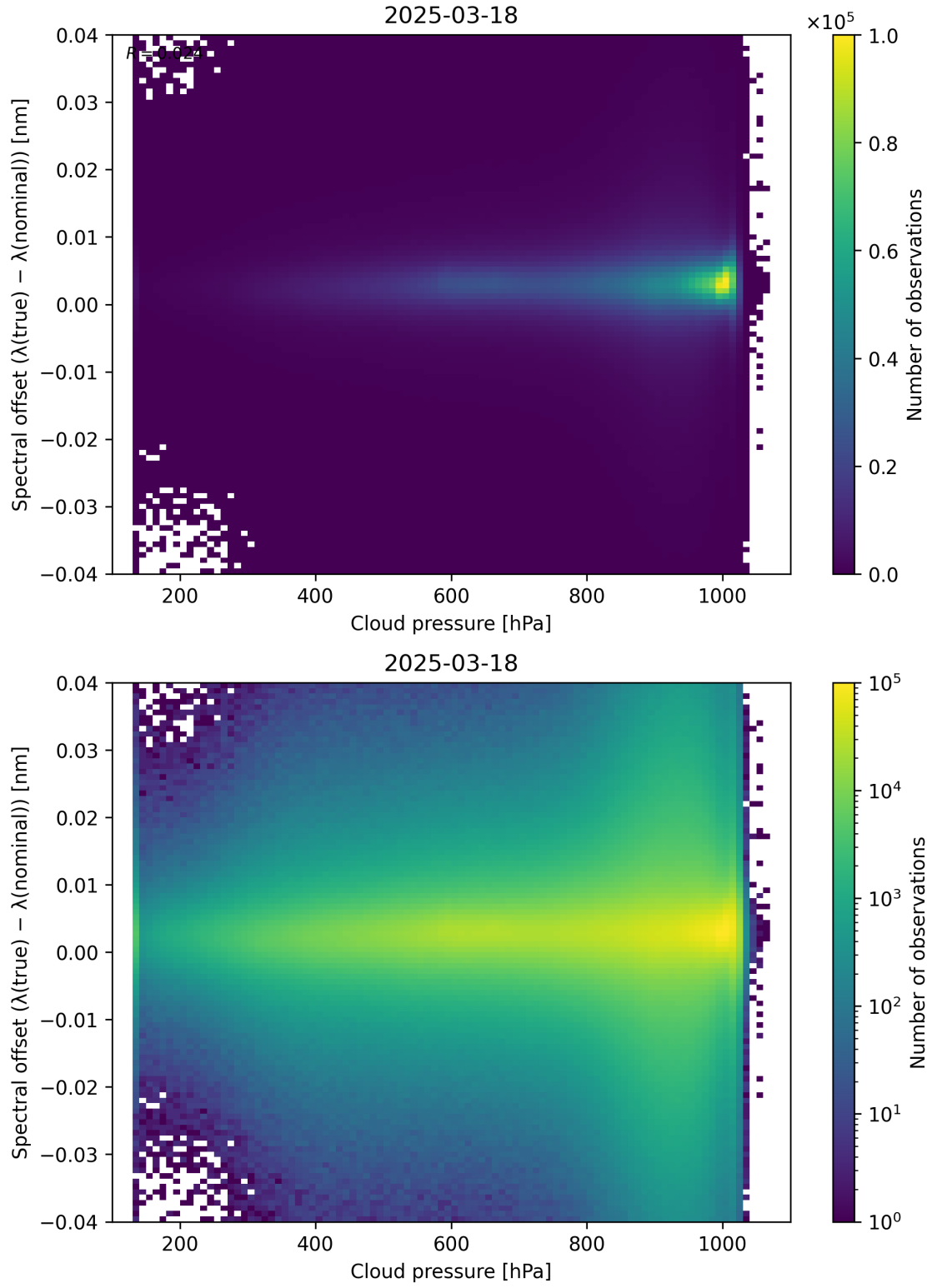
Figure 84: Scatter density plot of “Cloud pressure” against “Spectral offset ( \lambda_{\text{true}} - \lambda_{\text{nominal}} )” for 2025-03-17 to 2025-03-19.
