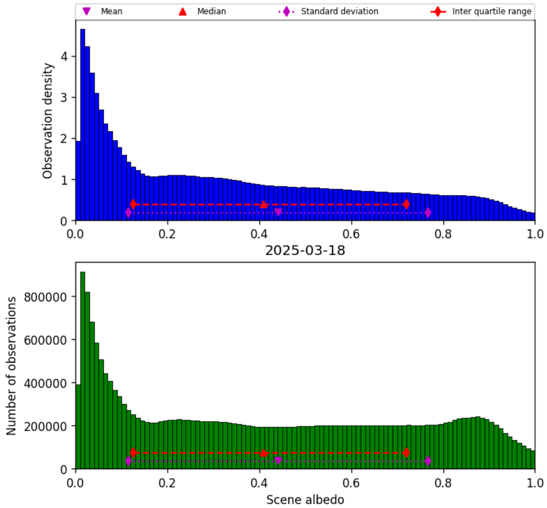
Figure 34: Histogram of “Scene albedo” for 2025-03-17 to 2025-03-19
