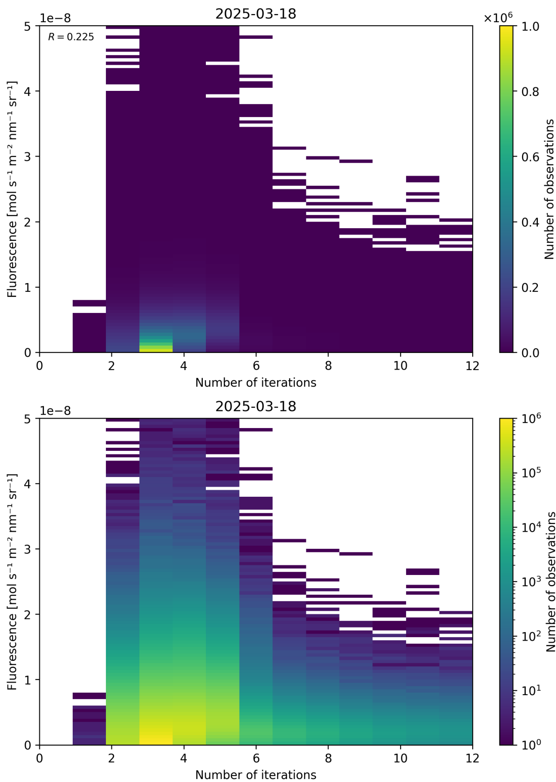
Figure 98: Scatter density plot of “Number of iterations” against “Fluorescence” for 2025-03-17 to 2025-03-19.
