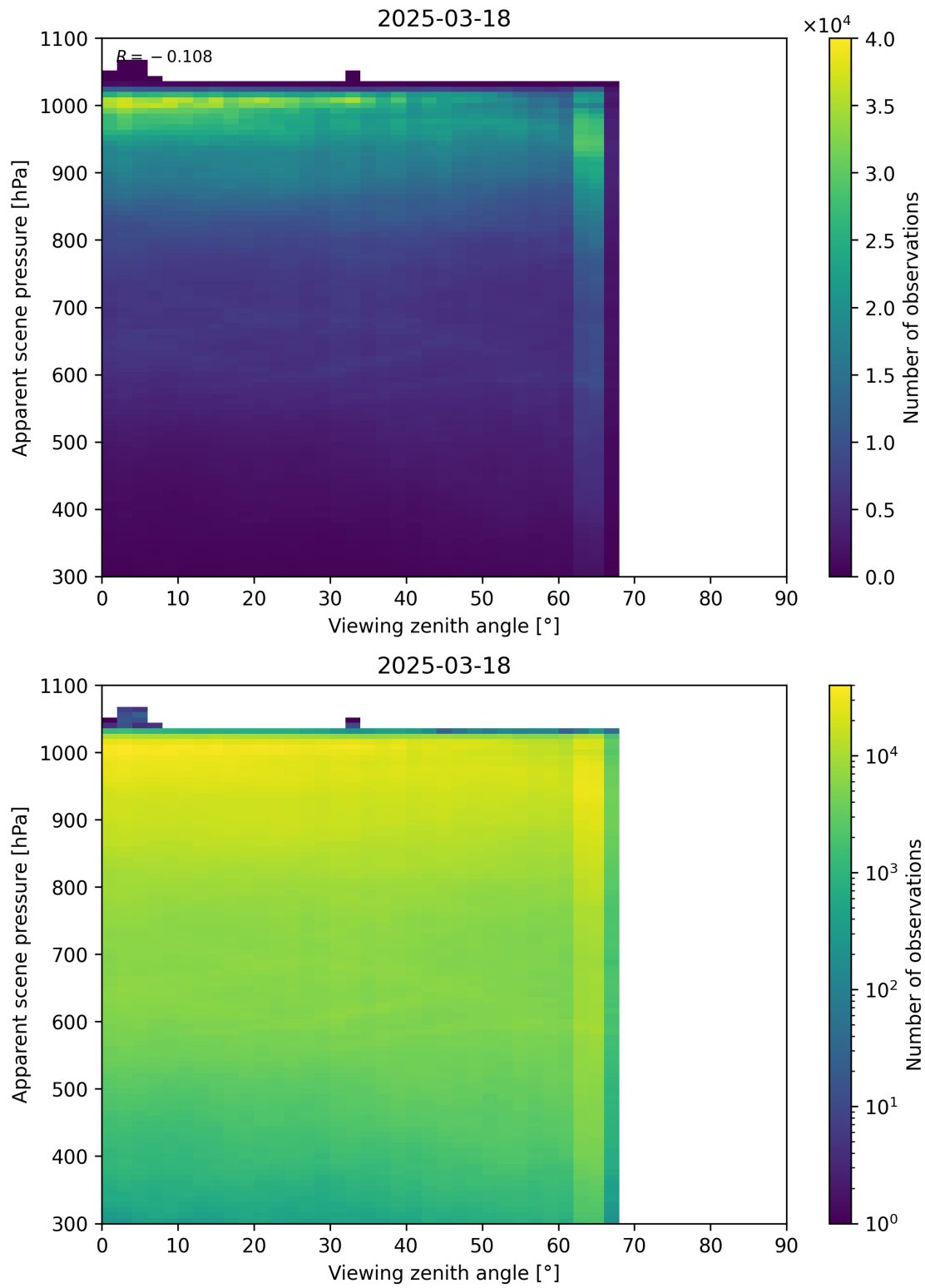
Figure 118: Scatter density plot of “Viewing zenith angle” against “Apparent scene pressure” for 2025-03-17 to 2025-03-19.
