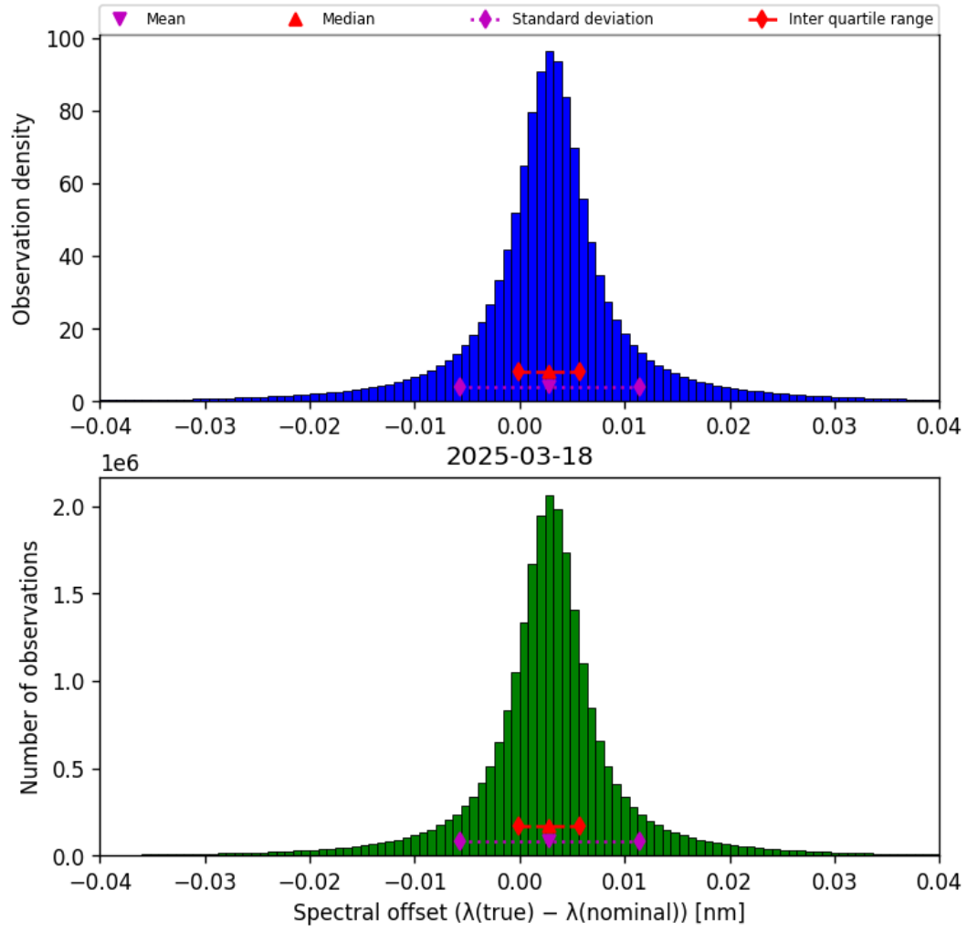
Figure 45: Histogram of “Spectral offset ( \lambda_{\text{true}} - \lambda_{\text{nominal}} )” for 2025-03-17 to 2025-03-19
