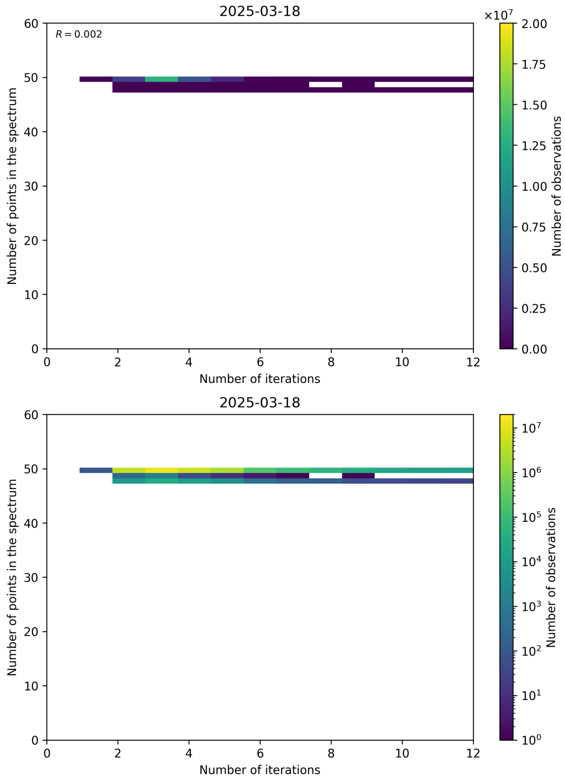
Figure 99: Scatter density plot of “Number of iterations” against “Number of points in the spectrum” for 2025-03-17 to 2025-03-19.
