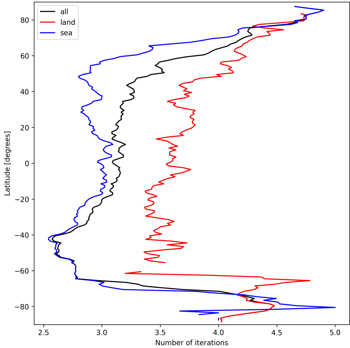
Figure 22: Zonal average of “Number of iterations” for 2025-03-17 to 2025-03-19.
