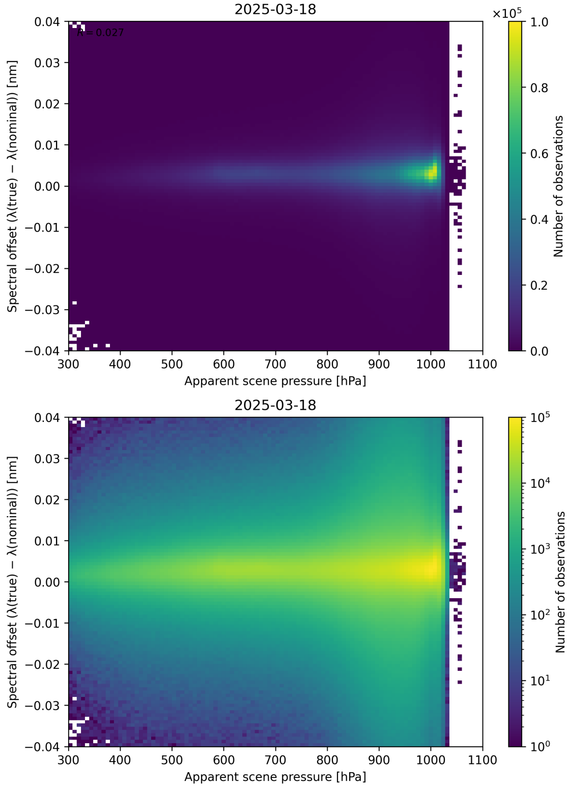
Figure 67: Scatter density plot of “Apparent scene pressure” against “Spectral offset ( \lambda_{\text{true}} - \lambda_{\text{nominal}} )” for 2025-03-17 to 2025-03-19.
