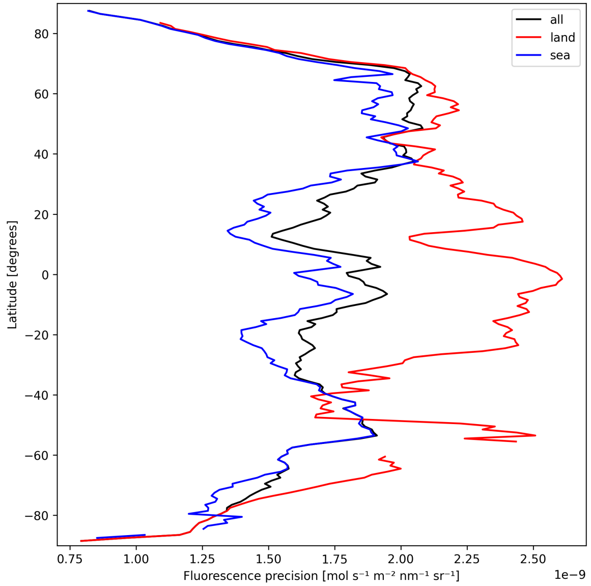
Figure 24: Zonal average of “Fluorescence precision” for 2025-03-17 to 2025-03-19.
