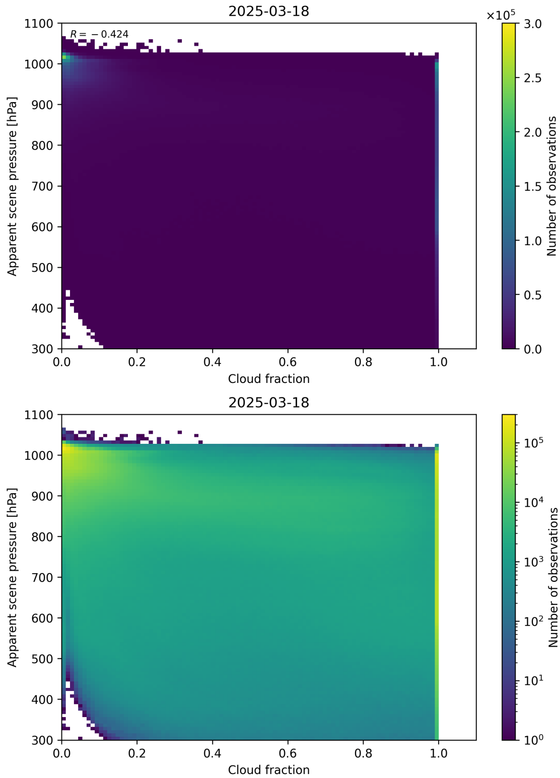
Figure 70: Scatter density plot of “Cloud fraction” against “Apparent scene pressure” for 2025-03-17 to 2025-03-19.
