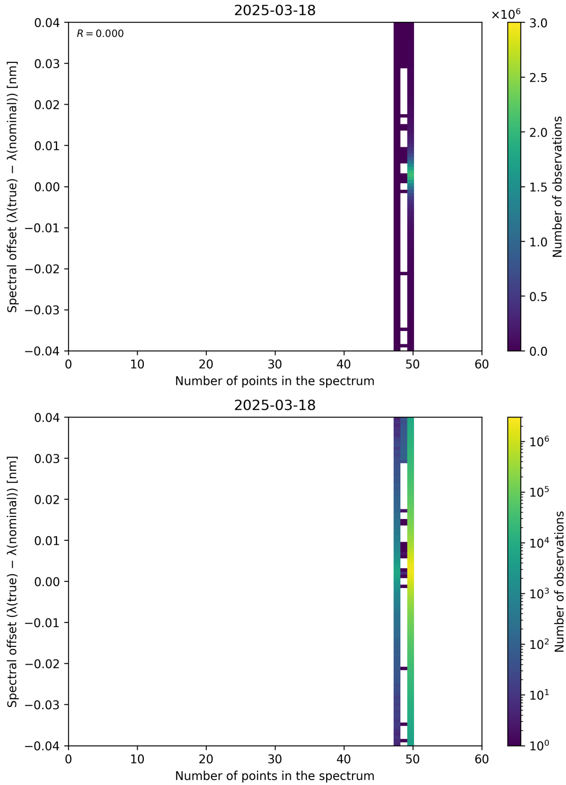
Figure 101: Scatter density plot of “Number of points in the spectrum” against “Spectral offset ( \lambda_{\text{true}} - \lambda_{\text{nominal}} )” for 2025-03-17 to 2025-03-19.
