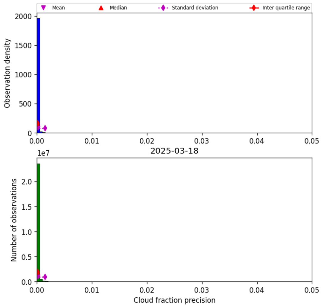
Figure 33: Histogram of “Cloud fraction precision” for 2025-03-17 to 2025-03-19
