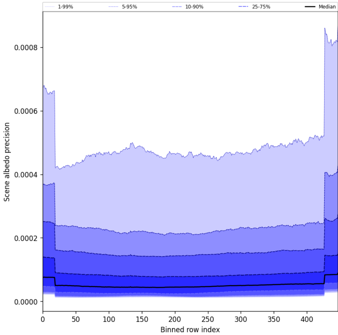
Figure 52: Along track statistics of “Scene albedo precision” for 2025-03-17 to 2025-03-19
