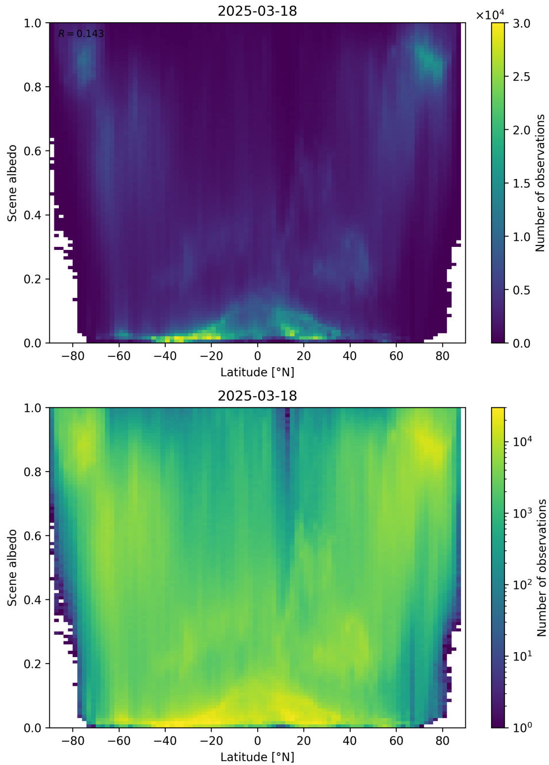
Figure 95: Scatter density plot of “Latitude” against “Scene albedo” for 2025-03-17 to 2025-03-19.
