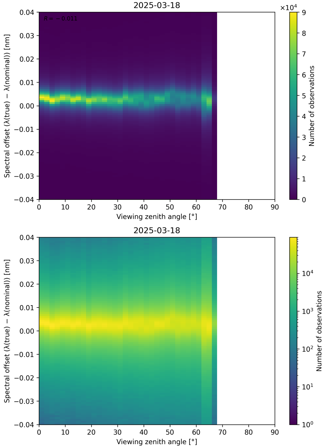
Figure 128: Scatter density plot of “Viewing zenith angle” against “Spectral offset ( \lambda_{\text{true}} - \lambda_{\text{nominal}} )” for 2025-03-17 to 2025-03-19.
