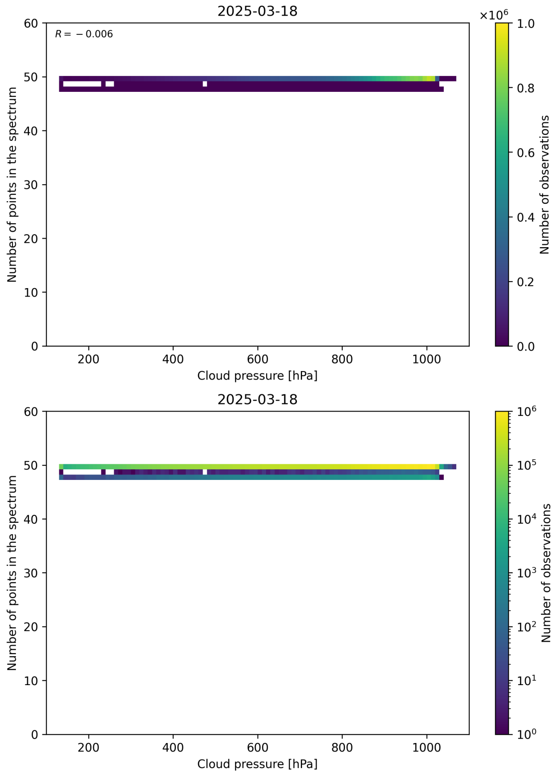
Figure 82: Scatter density plot of “Cloud pressure” against “Number of points in the spectrum” for 2025-03-17 to 2025-03-19.
