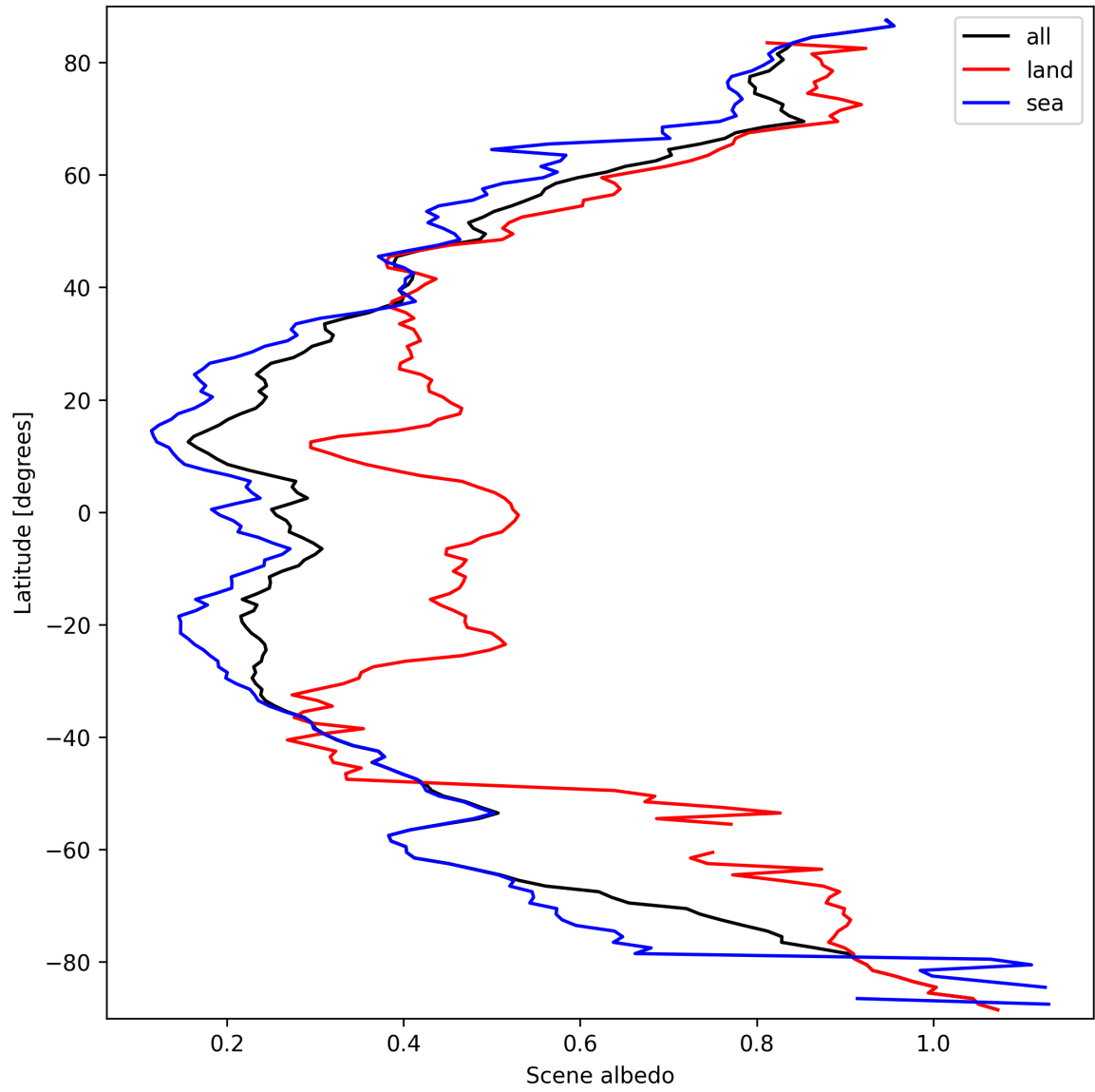
Figure 17: Zonal average of “Scene albedo” for 2025-03-17 to 2025-03-19.
