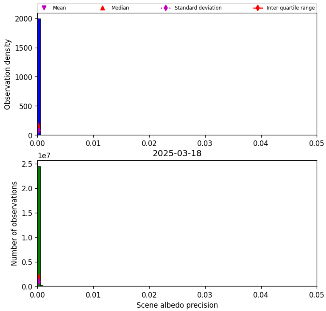
Figure 35: Histogram of “Scene albedo precision” for 2025-03-17 to 2025-03-19
