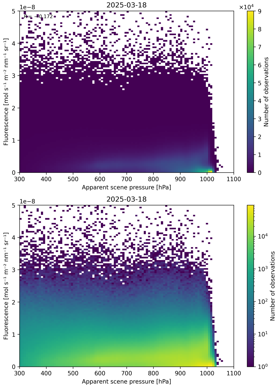
Figure 64: Scatter density plot of “Apparent scene pressure” against “Fluorescence” for 2025-03-17 to 2025-03-19.
