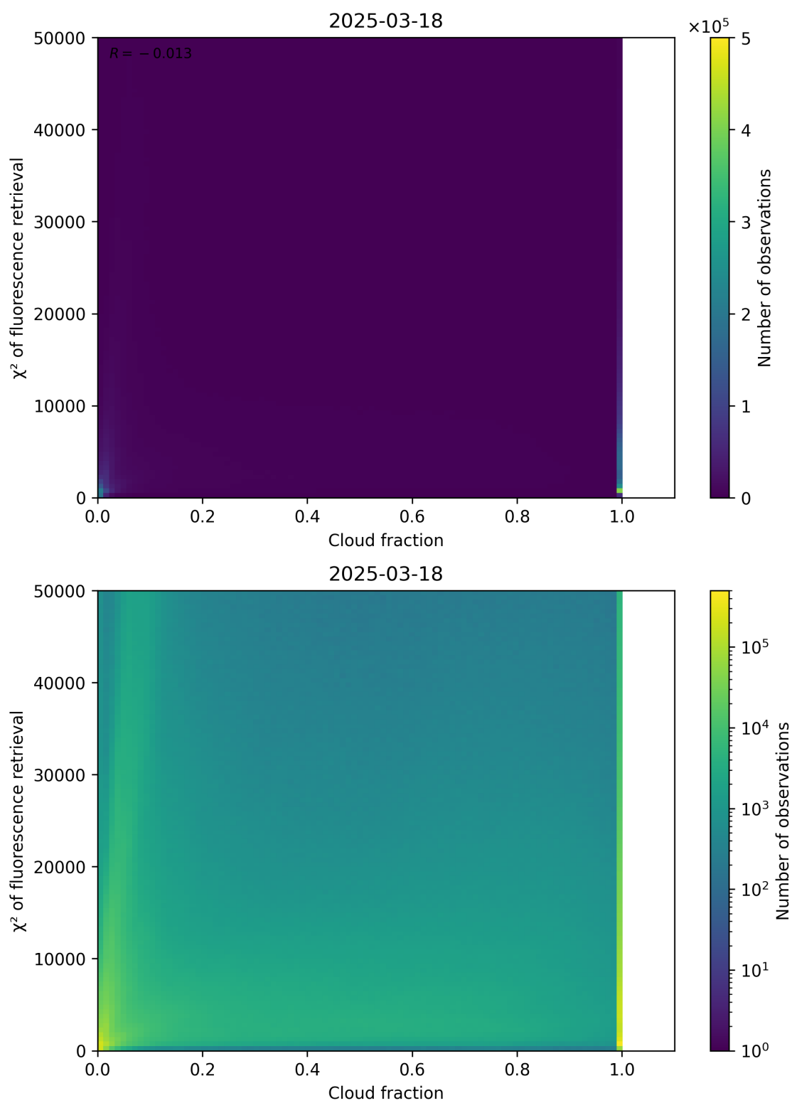
Figure 71: Scatter density plot of “Cloud fraction” against “ \chi^2 of fluorescence retrieval” for 2025-03-17 to 2025-03-19.
