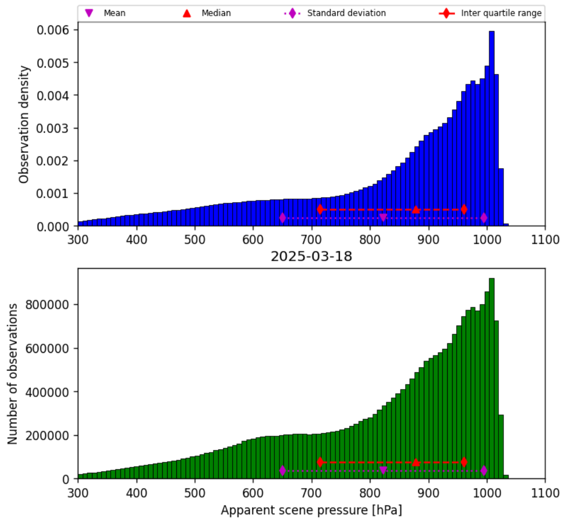
Figure 36: Histogram of “Apparent scene pressure” for 2025-03-17 to 2025-03-19
