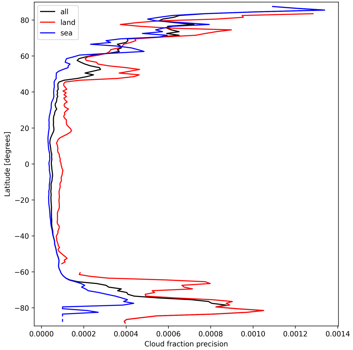
Figure 16: Zonal average of “Cloud fraction precision” for 2025-03-17 to 2025-03-19.
