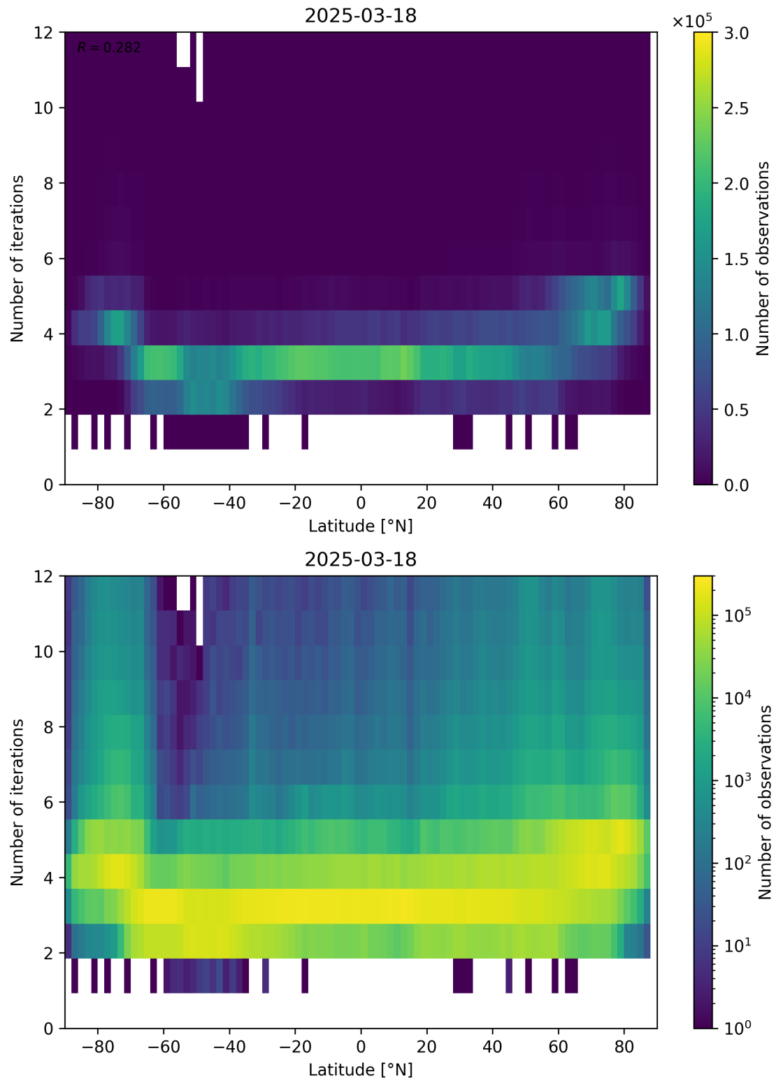
Figure 93: Scatter density plot of “Latitude” against “Number of iterations” for 2025-03-17 to 2025-03-19.
