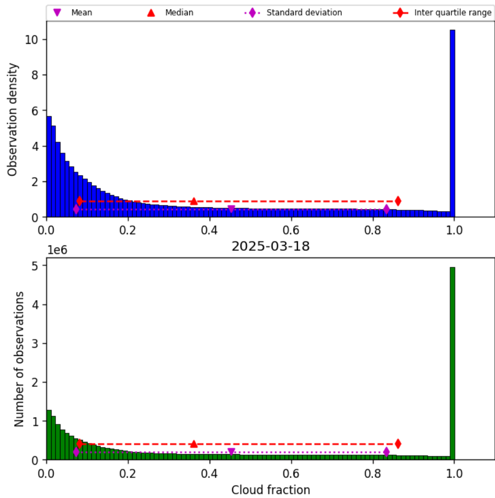
Figure 32: Histogram of “Cloud fraction” for 2025-03-17 to 2025-03-19
