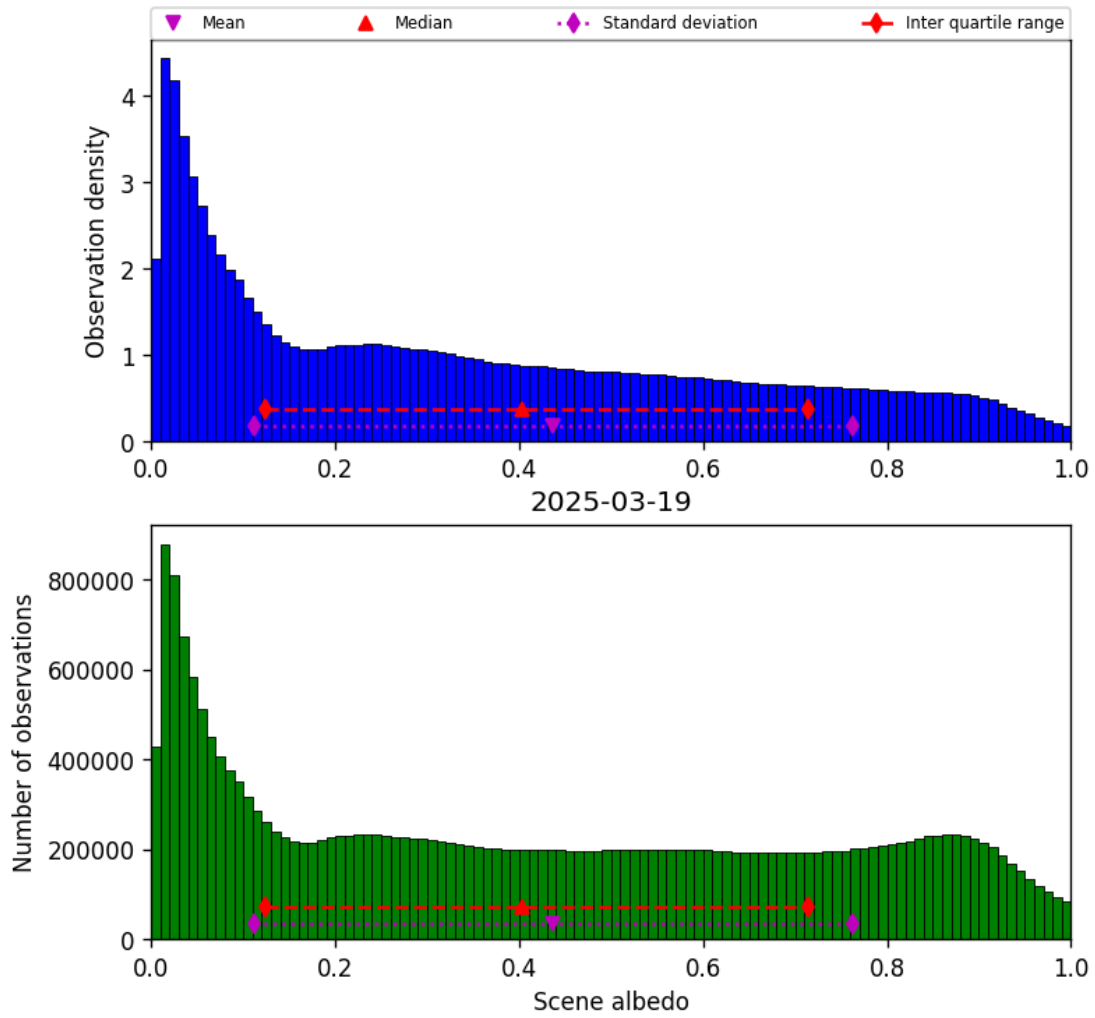
Figure 34: Histogram of “Scene albedo” for 2025-03-18 to 2025-03-20
