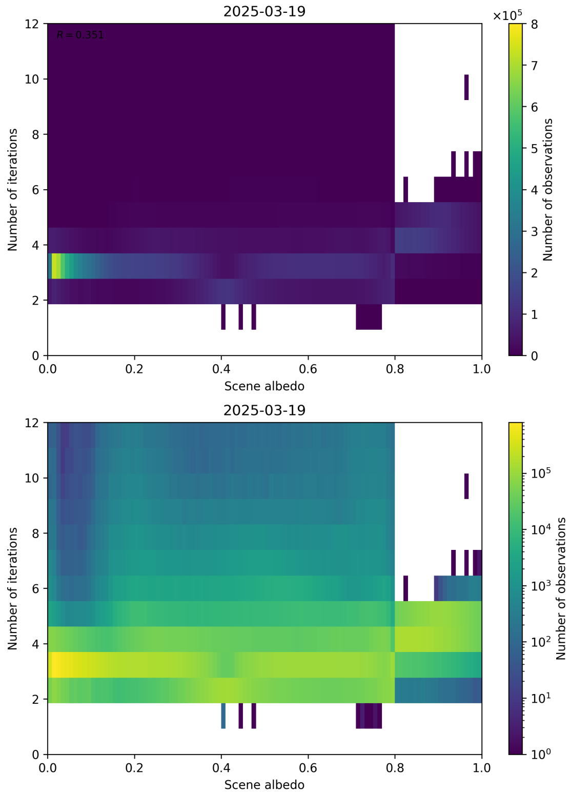
Figure 105: Scatter density plot of “Scene albedo” against “Number of iterations” for 2025-03-18 to 2025-03-20.
