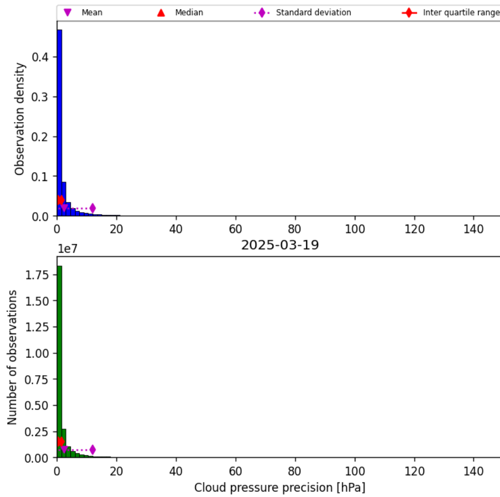
Figure 31: Histogram of “Cloud pressure precision” for 2025-03-18 to 2025-03-20
