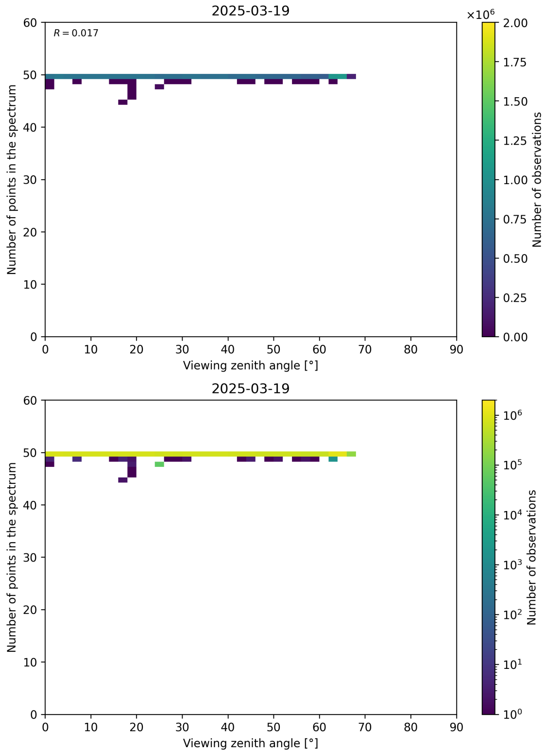
Figure 125: Scatter density plot of “Viewing zenith angle” against “Number of points in the spectrum” for 2025-03-18 to 2025-03-20.
