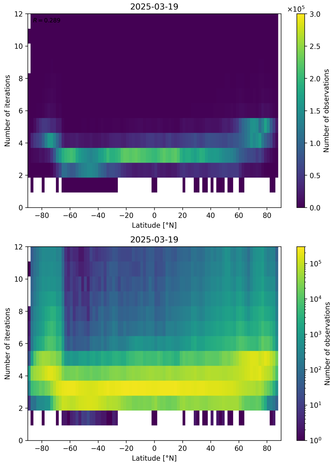
Figure 93: Scatter density plot of “Latitude” against “Number of iterations” for 2025-03-18 to 2025-03-20.
