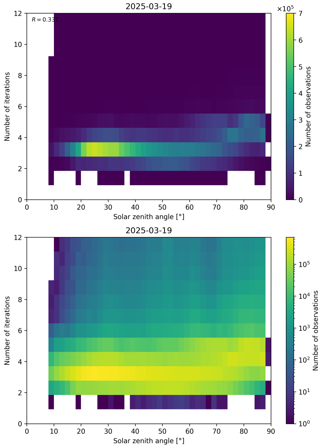
Figure 114: Scatter density plot of “Solar zenith angle” against “Number of iterations” for 2025-03-18 to 2025-03-20.
