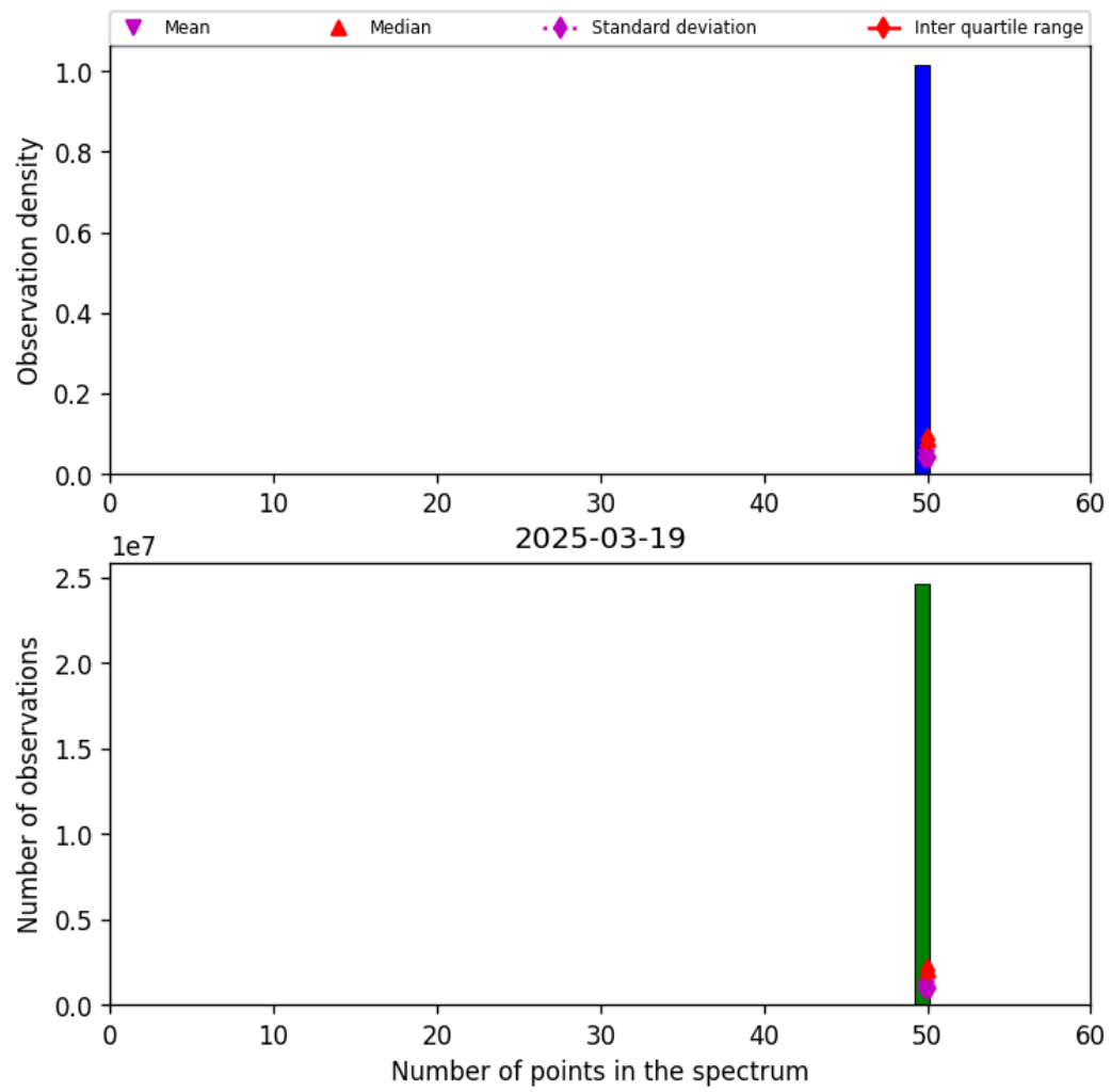
Figure 44: Histogram of “Number of points in the spectrum” for 2025-03-18 to 2025-03-20
