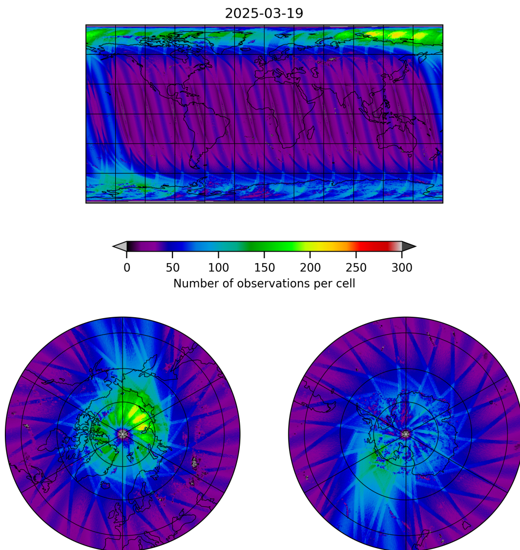
Figure 11: Map of the number of observations for 2025-03-18 to 2025-03-20
