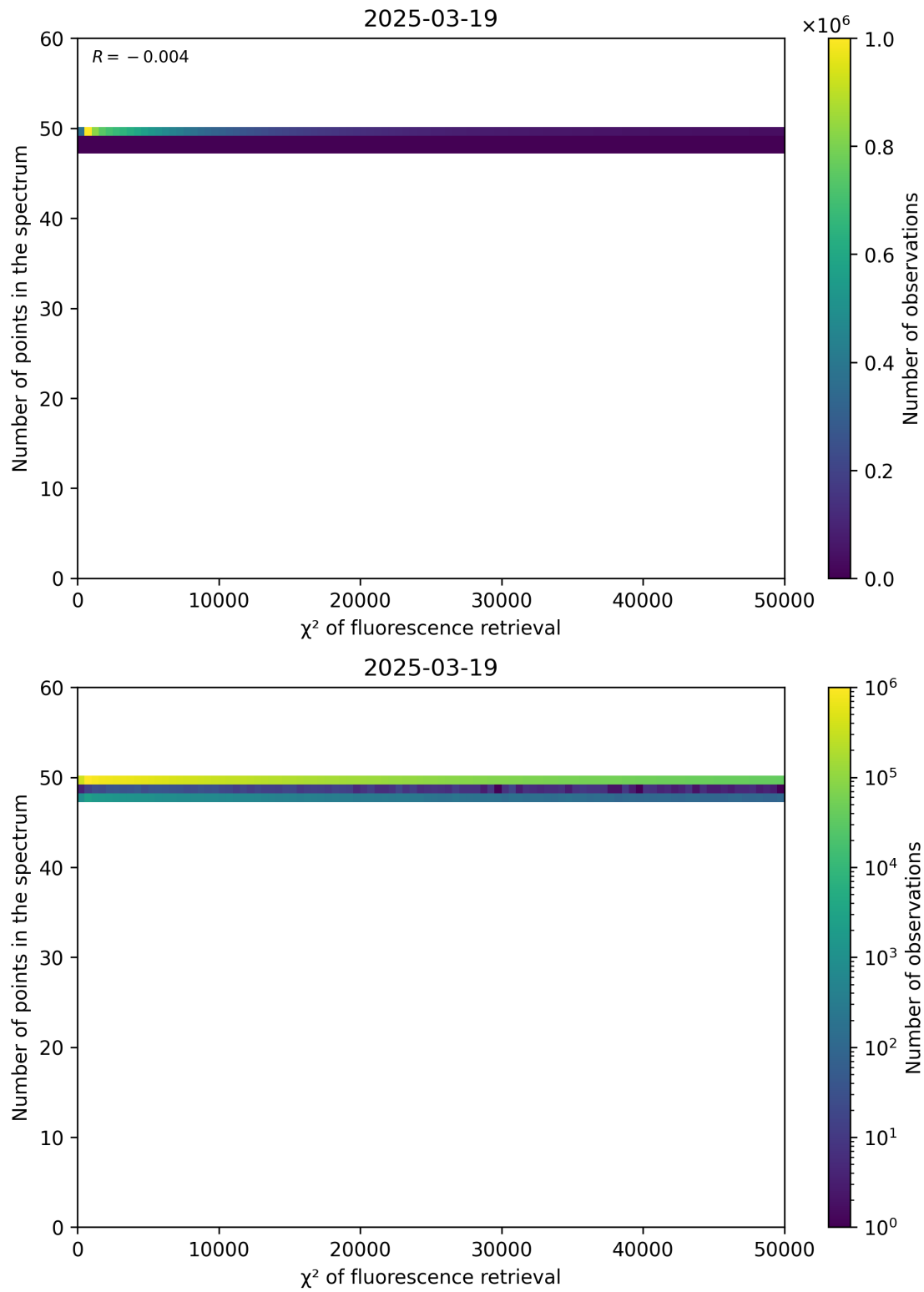
Figure 68: Scatter density plot of " \chi^2 of fluorescence retrieval" against "Number of points in the spectrum" for 2025-03-18 to 2025-03-20.
