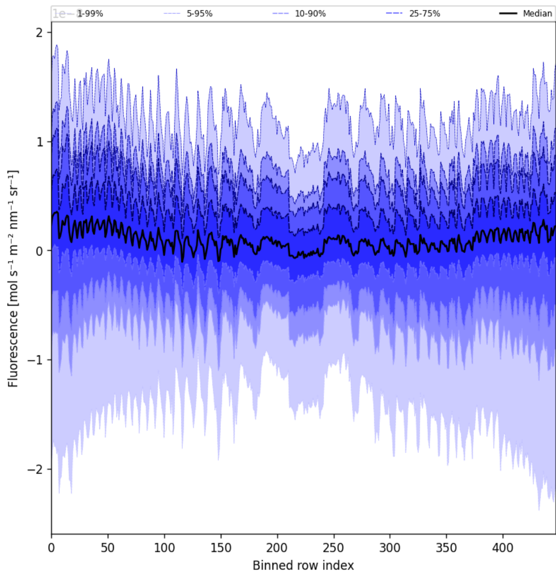
Figure 57: Along track statistics of “Fluorescence” for 2025-03-18 to 2025-03-20
