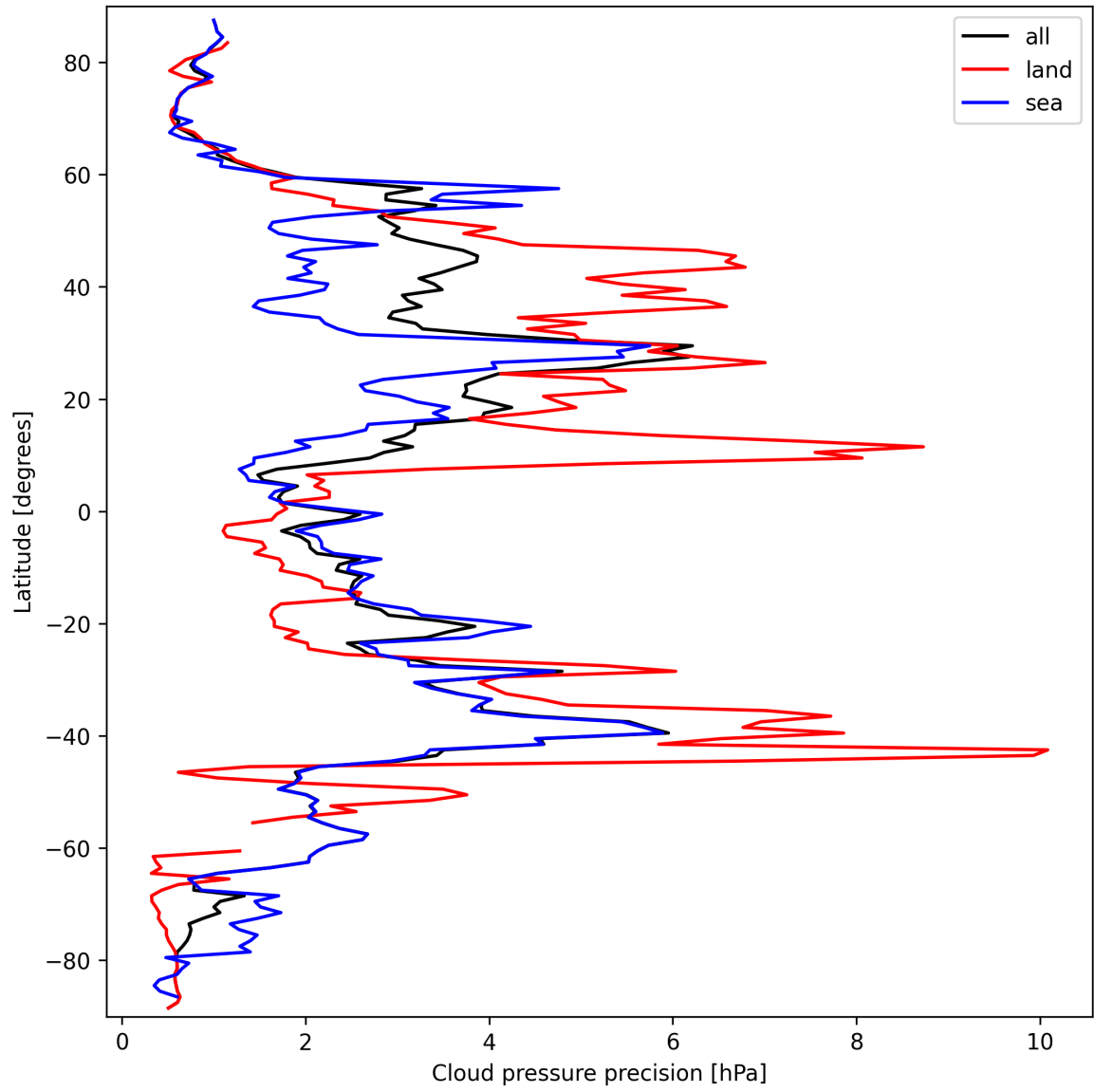
Figure 14: Zonal average of “Cloud pressure precision” for 2025-03-18 to 2025-03-20.
