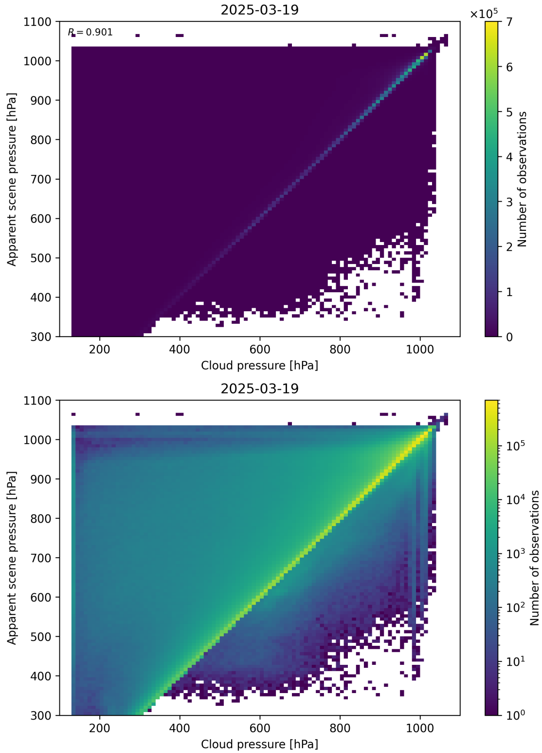
Figure 77: Scatter density plot of “Cloud pressure” against “Apparent scene pressure” for 2025-03-18 to 2025-03-20.
