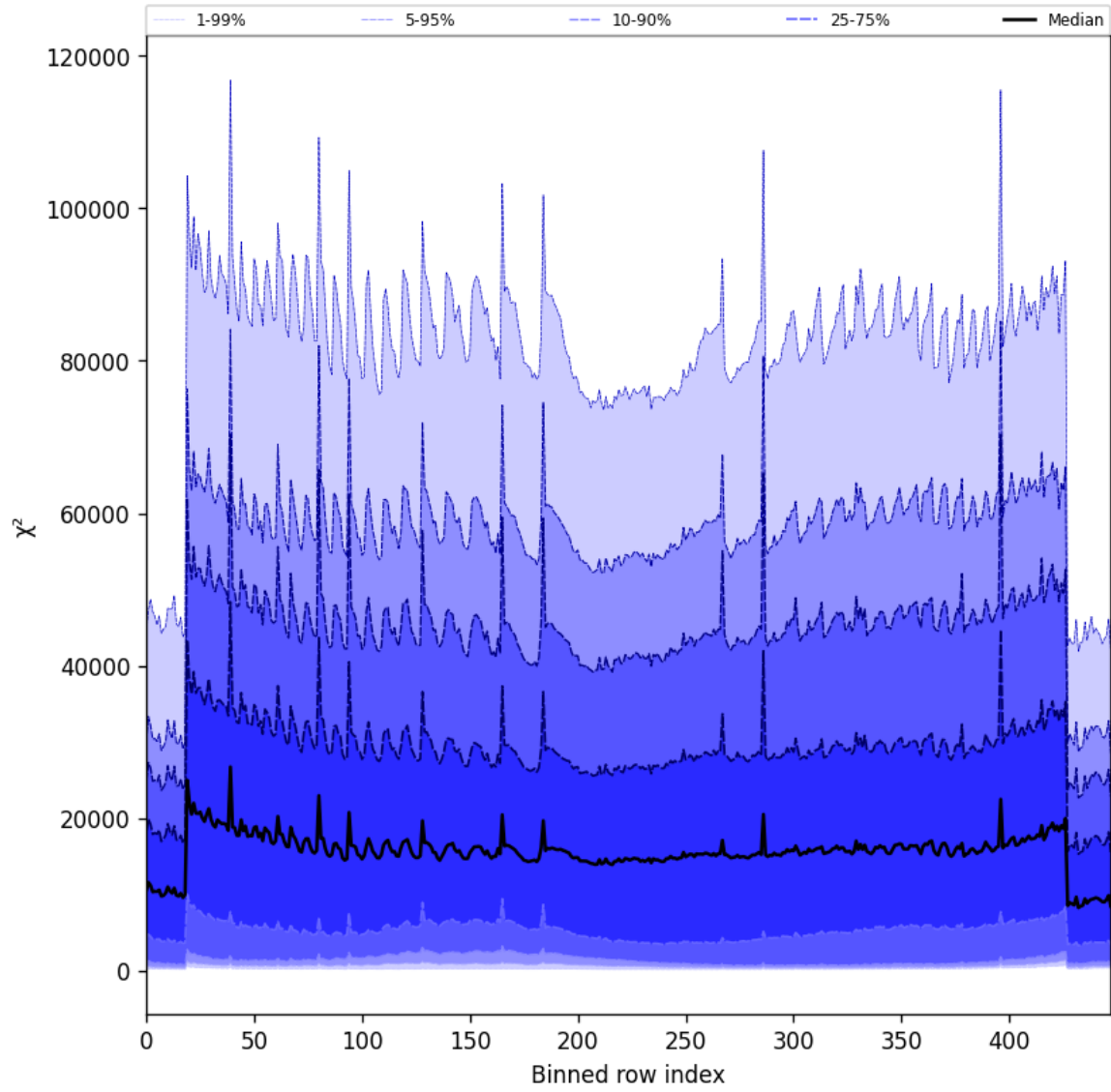
Figure 55: Along track statistics of “ \chi^2 ” for 2025-03-18 to 2025-03-20
