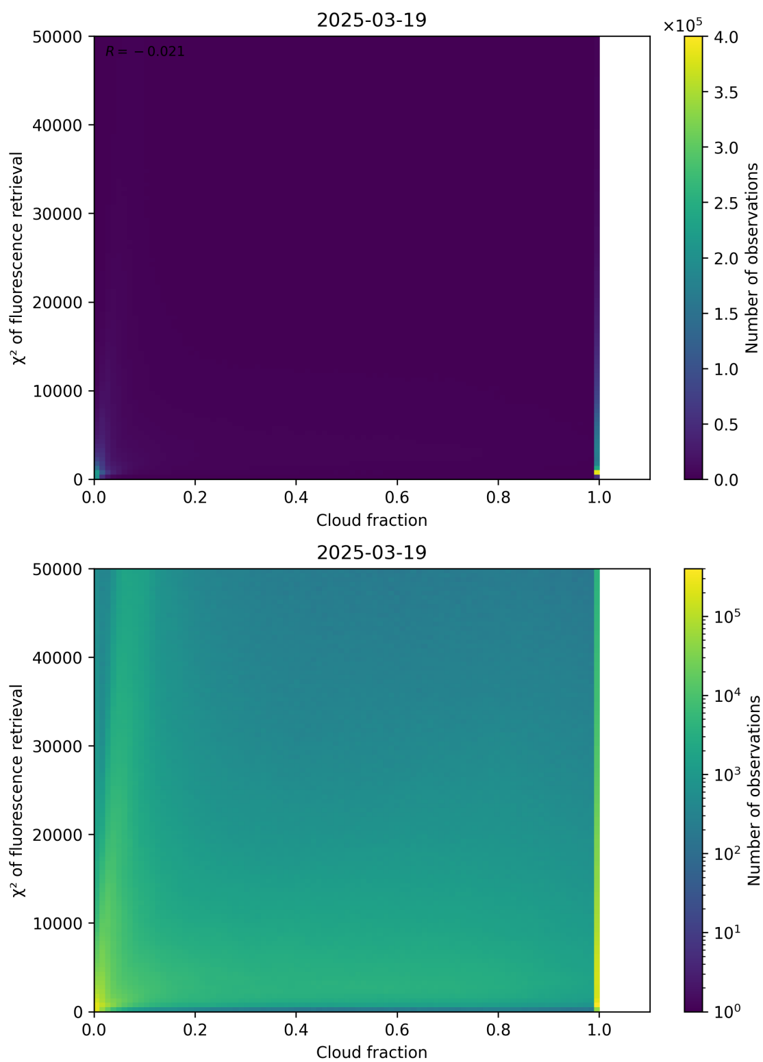
Figure 71: Scatter density plot of “Cloud fraction” against “ \chi^2 of fluorescence retrieval” for 2025-03-18 to 2025-03-20.
