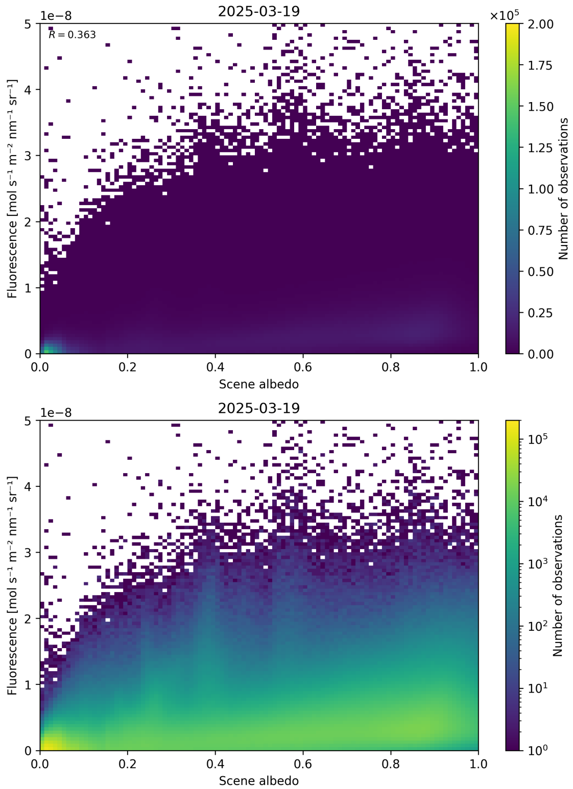
Figure 104: Scatter density plot of “Scene albedo” against “Fluorescence” for 2025-03-18 to 2025-03-20.
