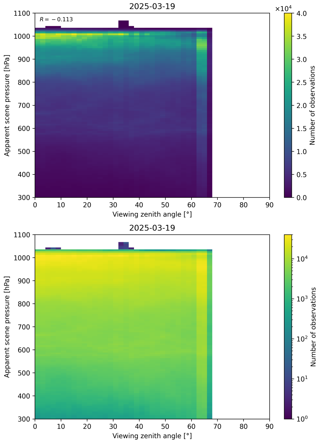
Figure 118: Scatter density plot of “Viewing zenith angle” against “Apparent scene pressure” for 2025-03-18 to 2025-03-20.
