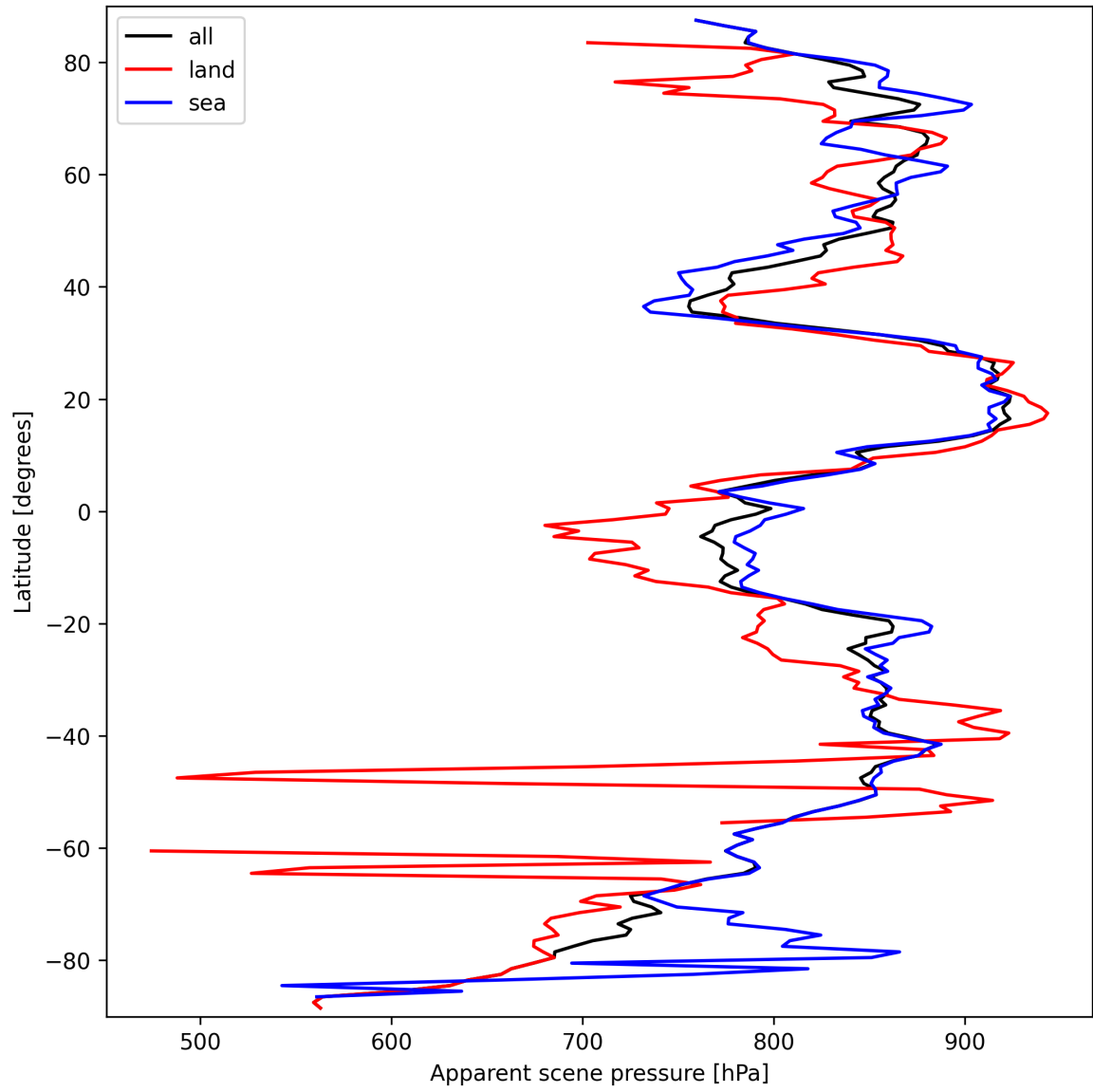
Figure 19: Zonal average of “Apparent scene pressure” for 2025-03-18 to 2025-03-20.
