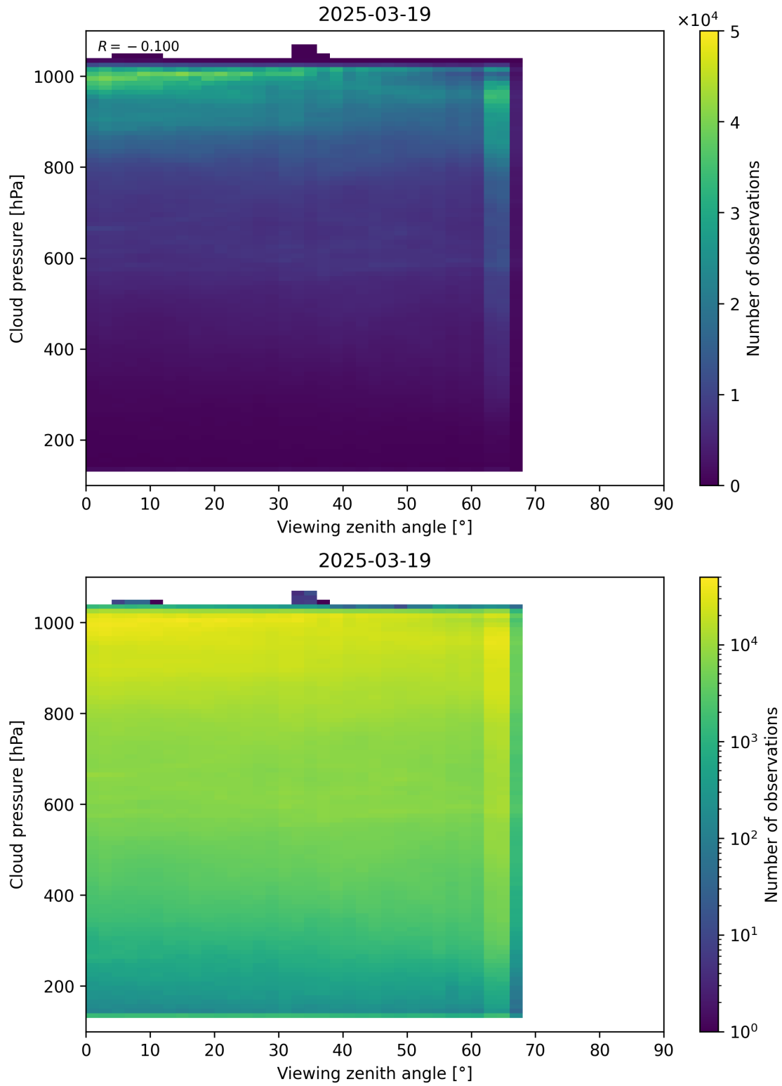
Figure 121: Scatter density plot of “Viewing zenith angle” against “Cloud pressure” for 2025-03-18 to 2025-03-20.
