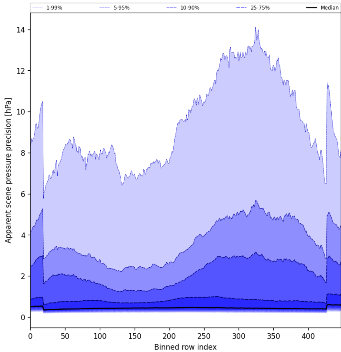
Figure 54: Along track statistics of “Apparent scene pressure precision” for 2025-03-18 to 2025-03-20
