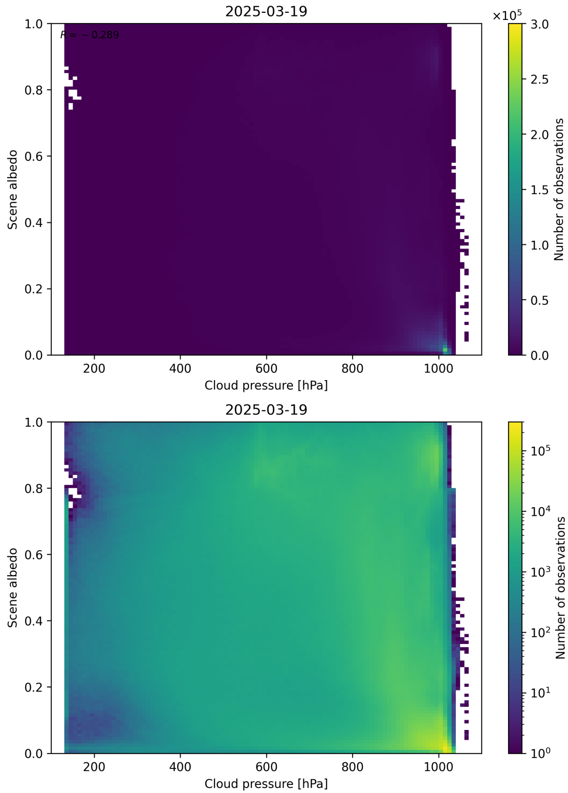
Figure 83: Scatter density plot of “Cloud pressure” against “Scene albedo” for 2025-03-18 to 2025-03-20.
