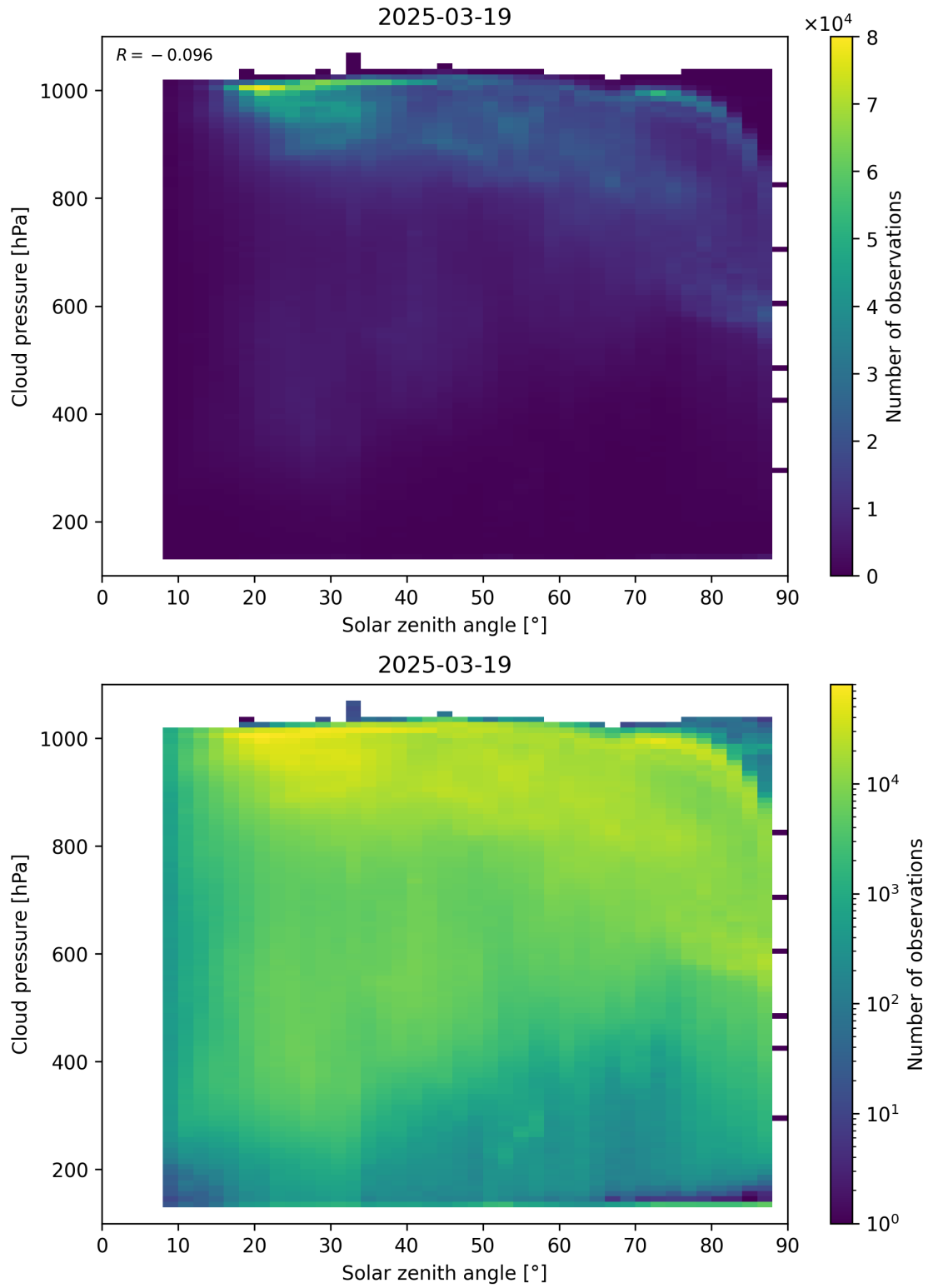
Figure 111: Scatter density plot of “Solar zenith angle” against “Cloud pressure” for 2025-03-18 to 2025-03-20.
