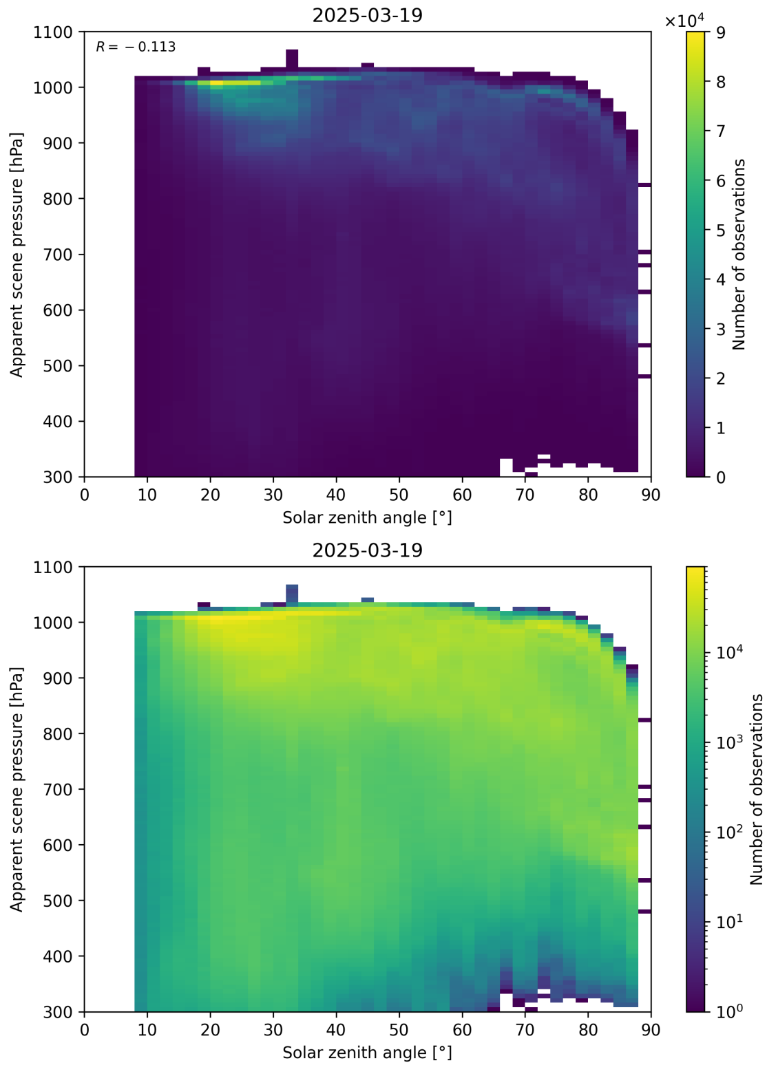
Figure 108: Scatter density plot of “Solar zenith angle” against “Apparent scene pressure” for 2025-03-18 to 2025-03-20.
