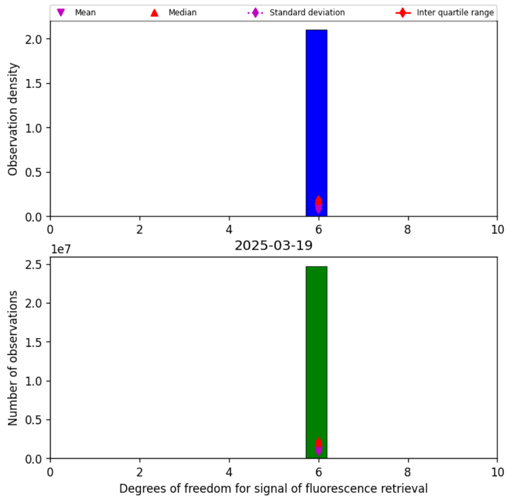
Figure 43: Histogram of “Degrees of freedom for signal of fluorescence retrieval” for 2025-03-18 to 2025-03-20
