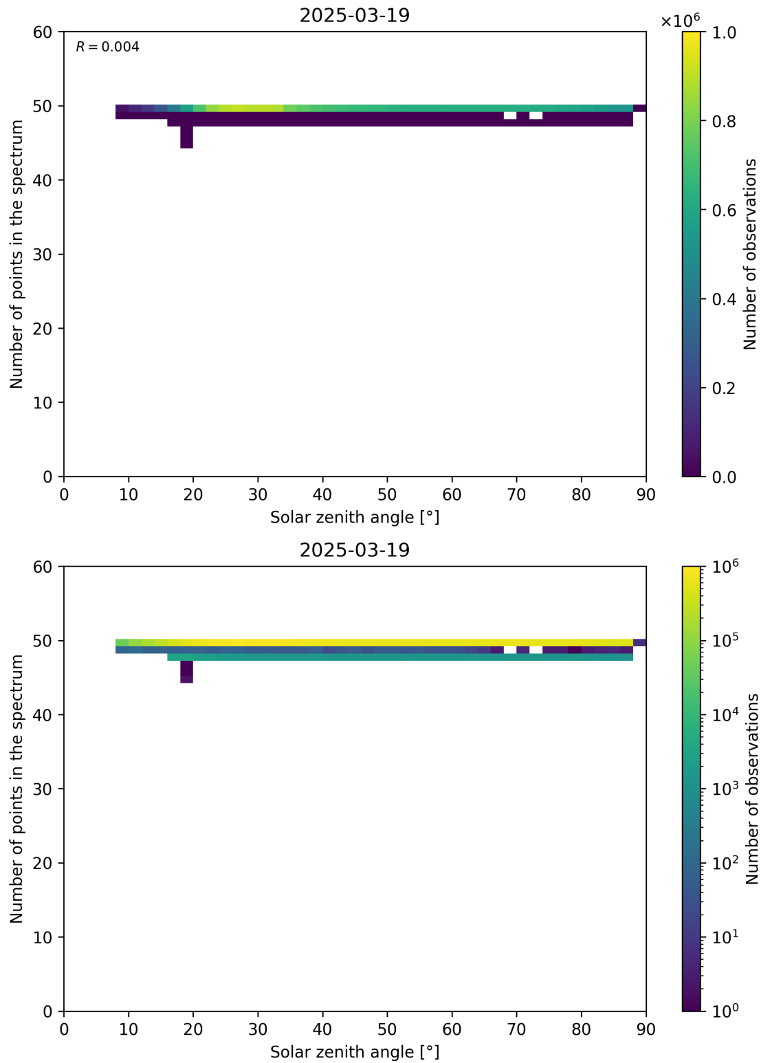
Figure 115: Scatter density plot of “Solar zenith angle” against “Number of points in the spectrum” for 2025-03-18 to 2025-03-20.
