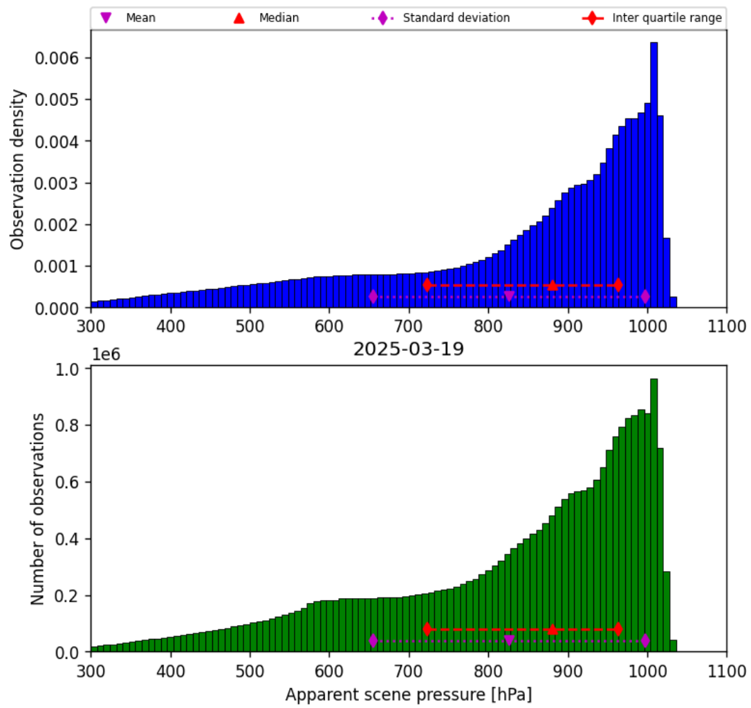
Figure 36: Histogram of “Apparent scene pressure” for 2025-03-18 to 2025-03-20
