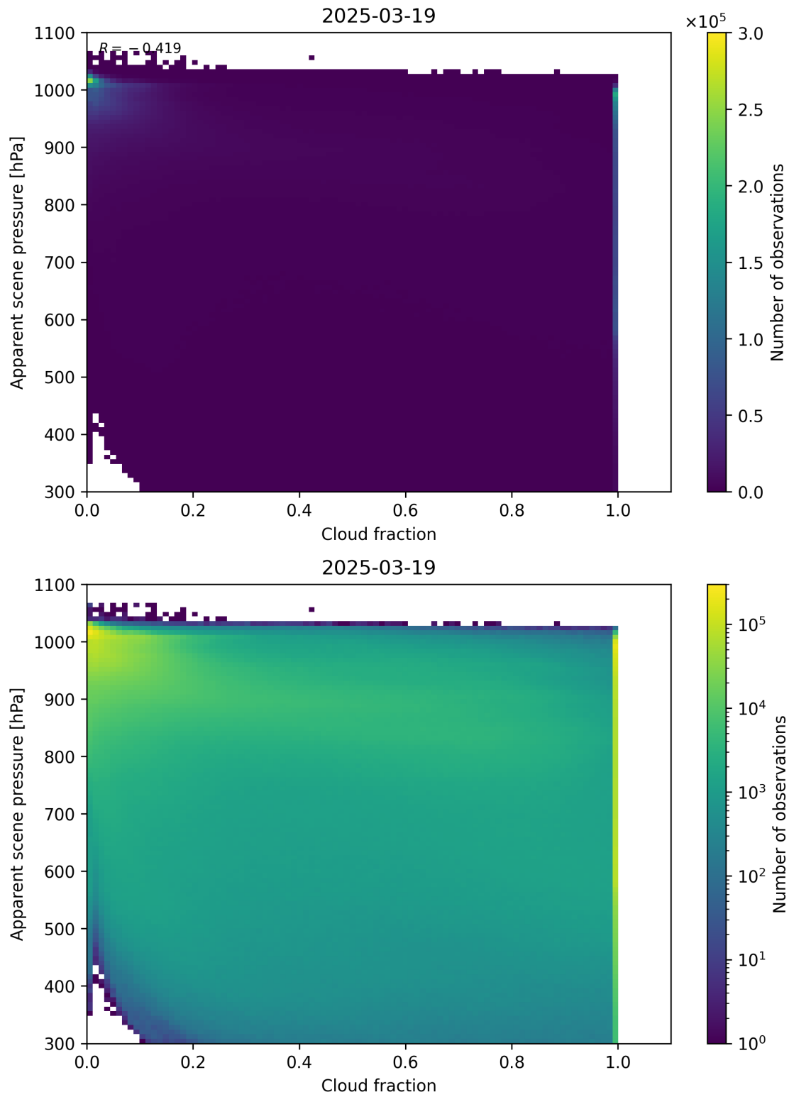
Figure 70: Scatter density plot of “Cloud fraction” against “Apparent scene pressure” for 2025-03-18 to 2025-03-20.
