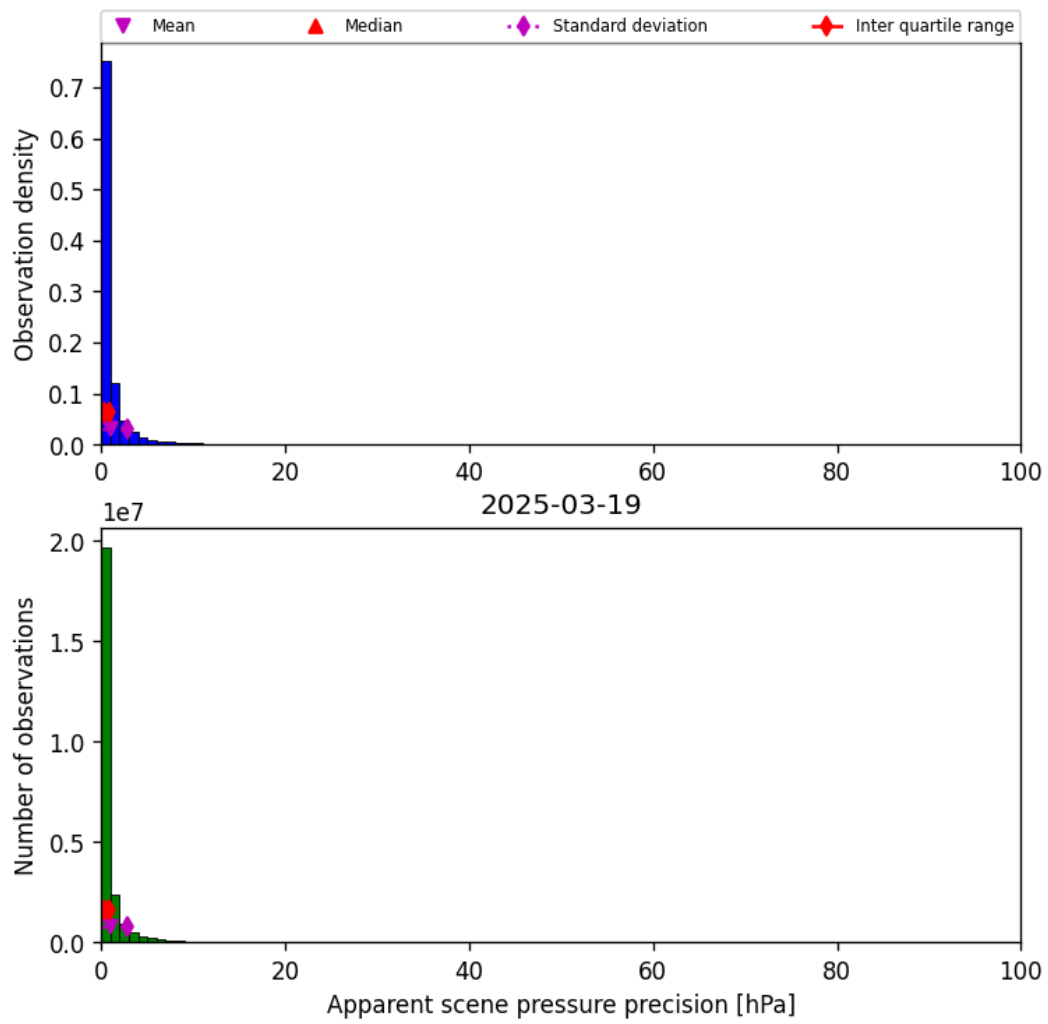
Figure 37: Histogram of “Apparent scene pressure precision” for 2025-03-18 to 2025-03-20
