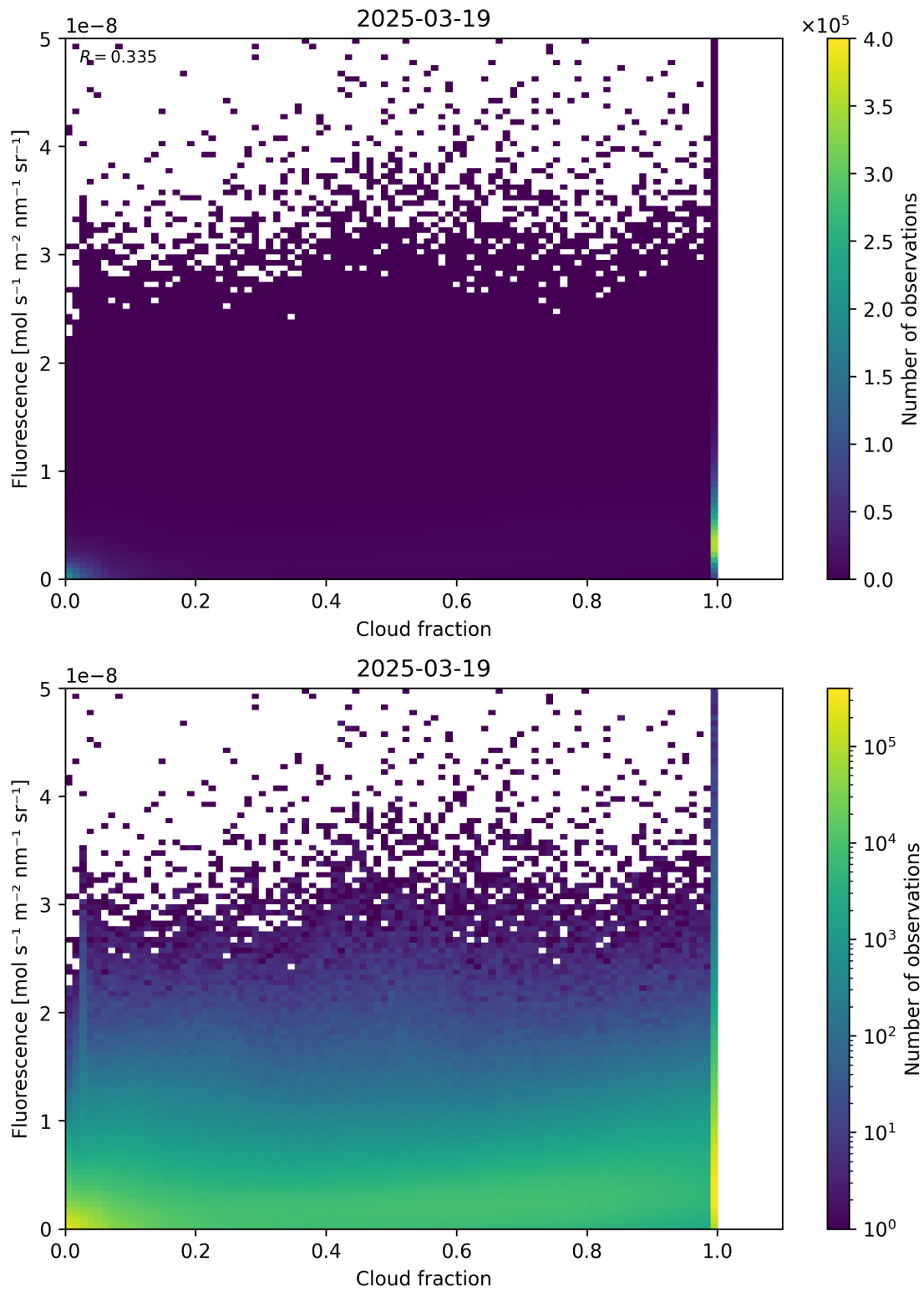
Figure 72: Scatter density plot of “Cloud fraction” against “Fluorescence” for 2025-03-18 to 2025-03-20.
