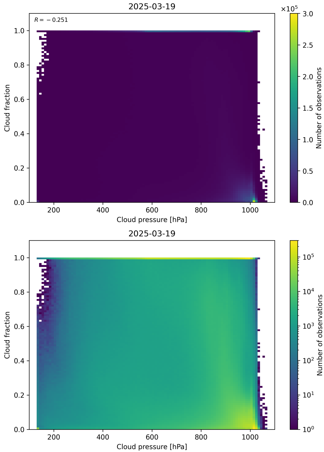
Figure 79: Scatter density plot of “Cloud pressure” against “Cloud fraction” for 2025-03-18 to 2025-03-20.
