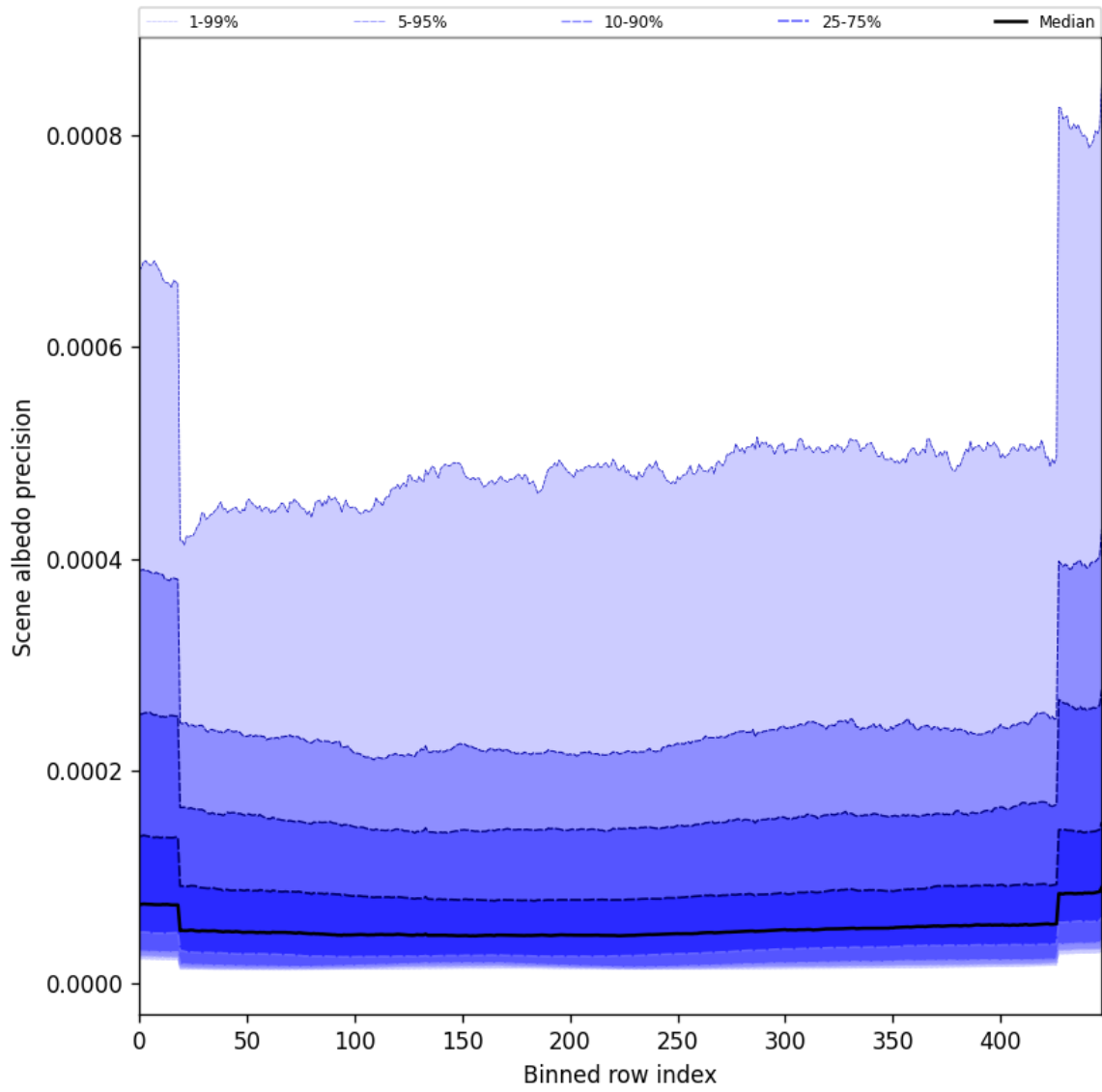
Figure 52: Along track statistics of “Scene albedo precision” for 2025-03-18 to 2025-03-20
