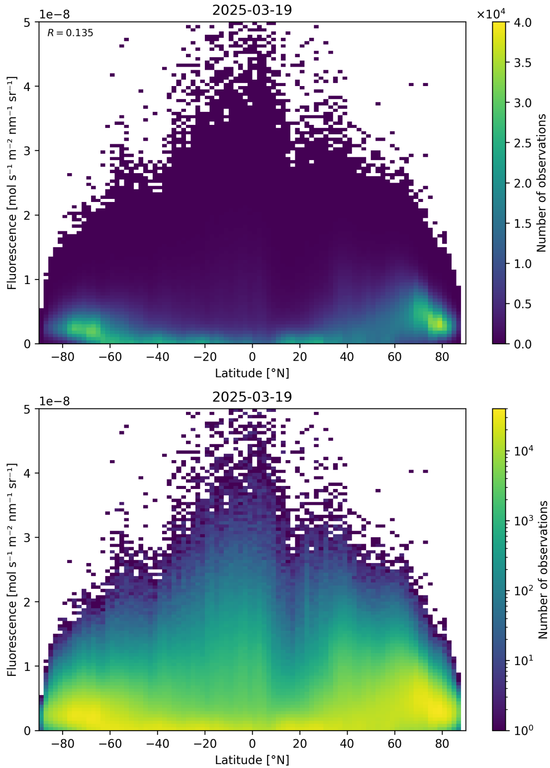
Figure 92: Scatter density plot of “Latitude” against “Fluorescence” for 2025-03-18 to 2025-03-20.
