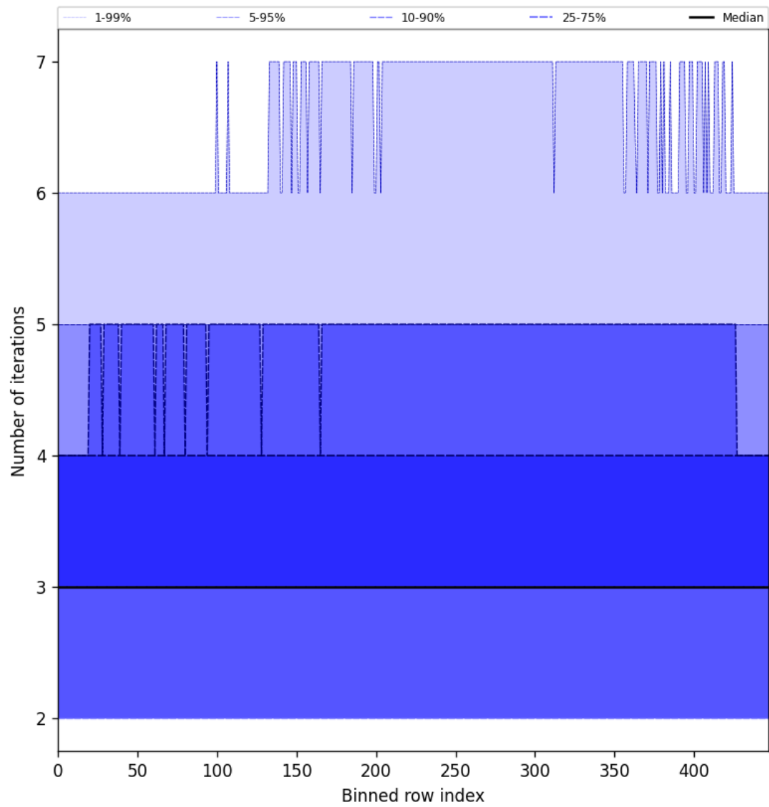
Figure 56: Along track statistics of “Number of iterations” for 2025-03-18 to 2025-03-20
