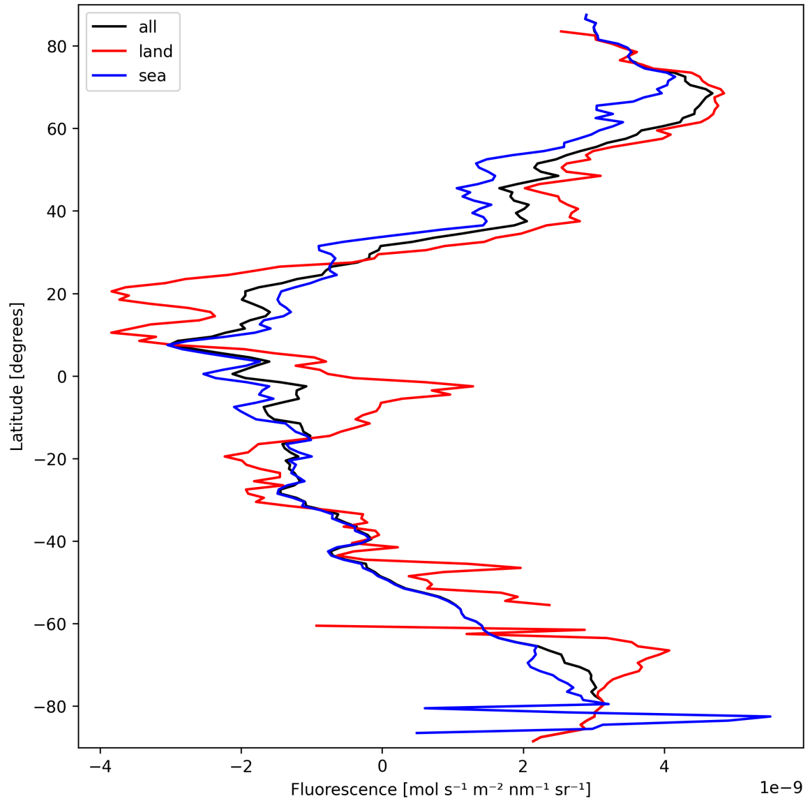
Figure 23: Zonal average of “Fluorescence” for 2025-03-18 to 2025-03-20.
