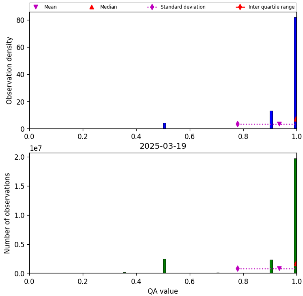
Figure 29: Histogram of “QA value” for 2025-03-18 to 2025-03-20
