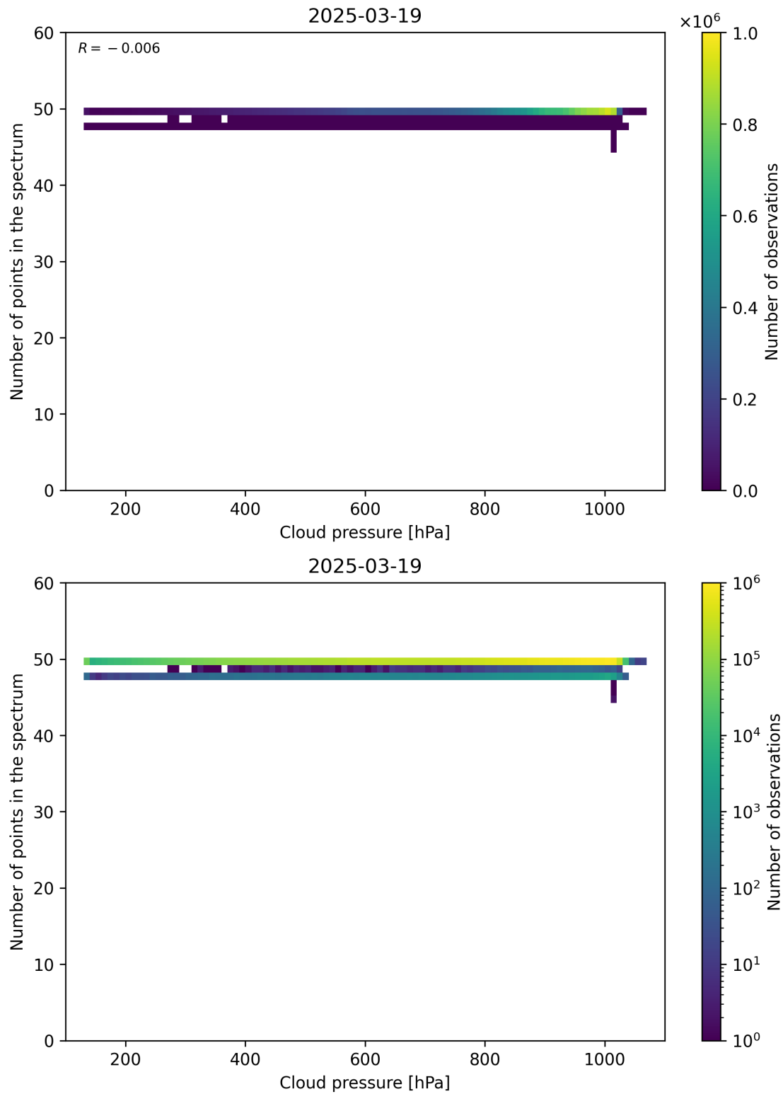
Figure 82: Scatter density plot of “Cloud pressure” against “Number of points in the spectrum” for 2025-03-18 to 2025-03-20.
