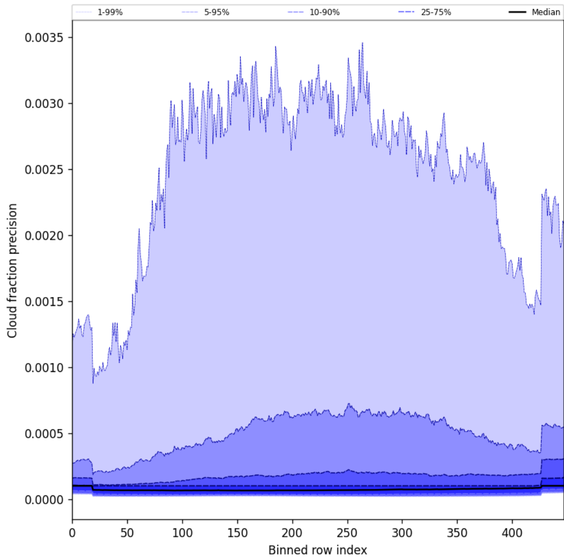
Figure 50: Along track statistics of “Cloud fraction precision” for 2025-03-18 to 2025-03-20
