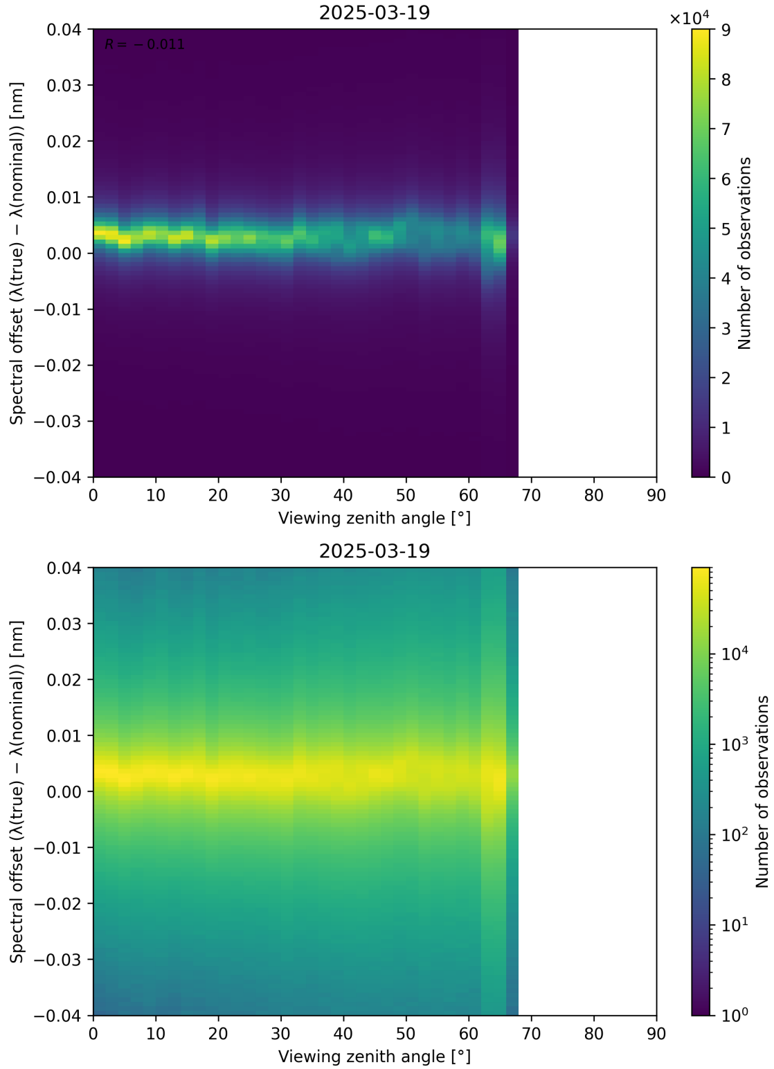
Figure 128: Scatter density plot of “Viewing zenith angle” against “Spectral offset ( \lambda_{\text{true}} - \lambda_{\text{nominal}} )” for 2025-03-18 to 2025-03-20.
