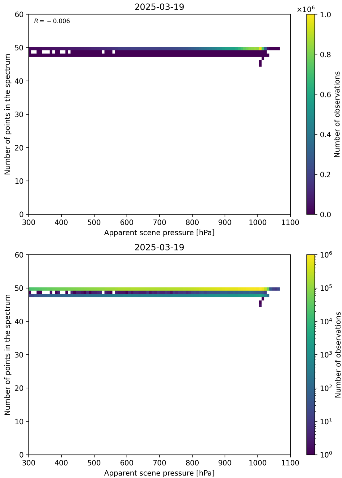
Figure 66: Scatter density plot of “Apparent scene pressure” against “Number of points in the spectrum” for 2025-03-18 to 2025-03-20.
