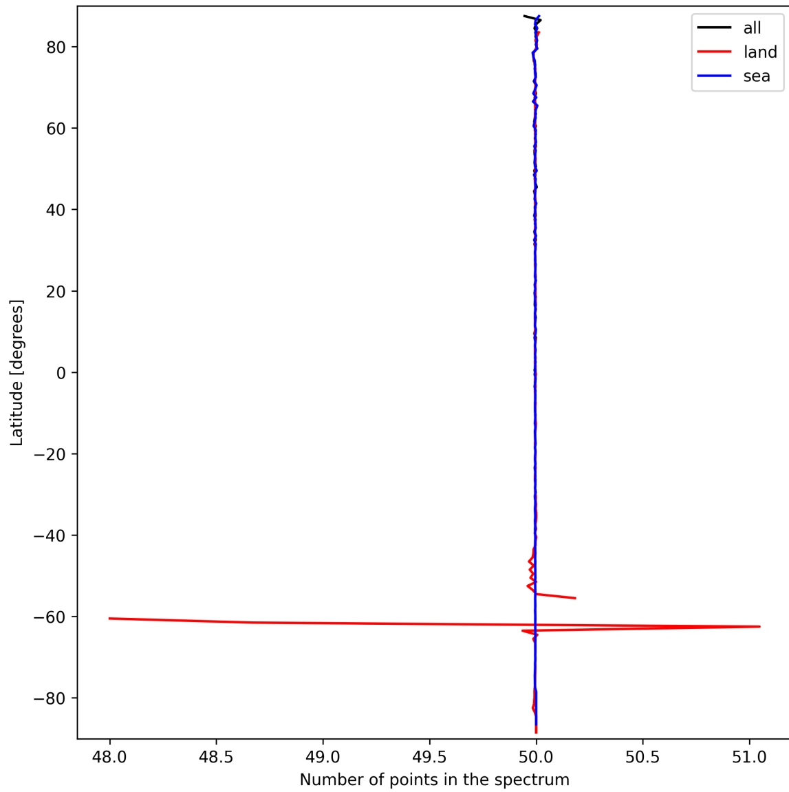
Figure 27: Zonal average of “Number of points in the spectrum” for 2025-03-18 to 2025-03-20.
