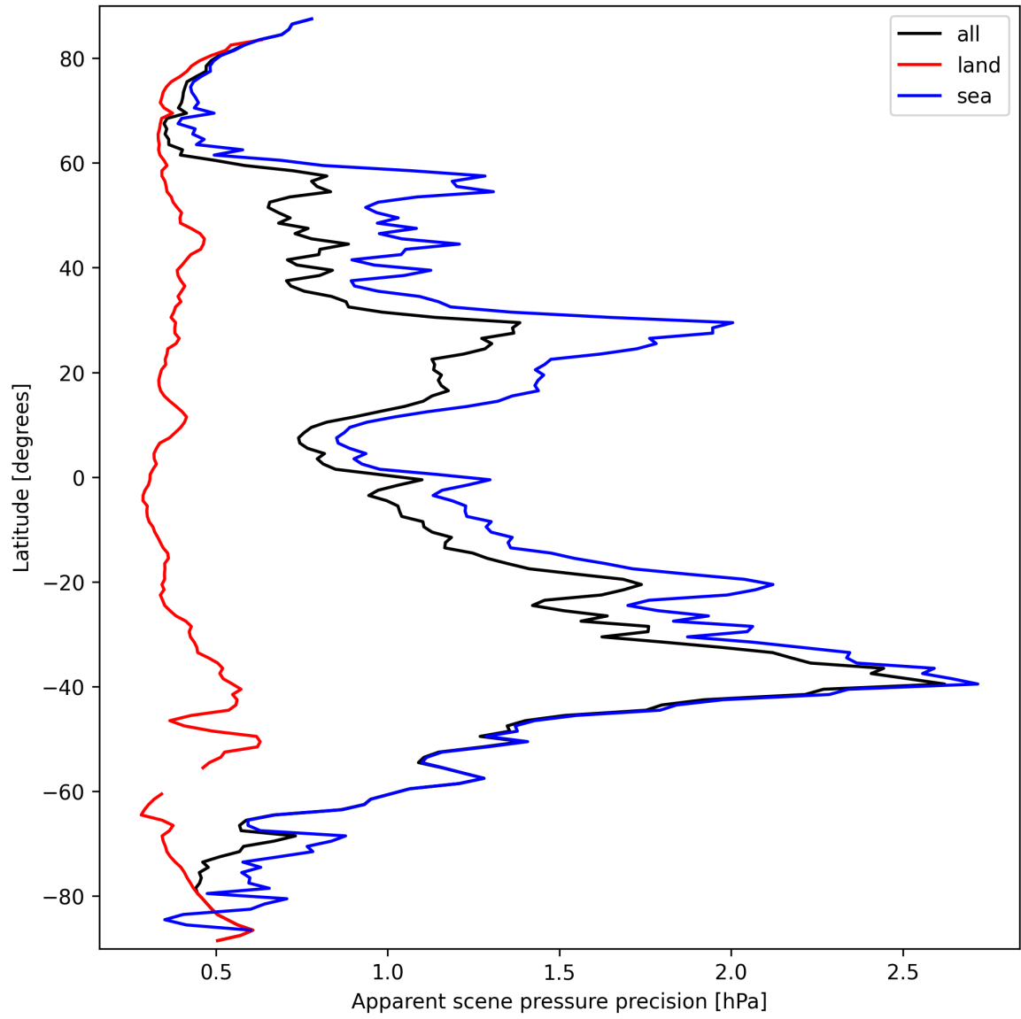
Figure 20: Zonal average of “Apparent scene pressure precision” for 2025-03-18 to 2025-03-20.
