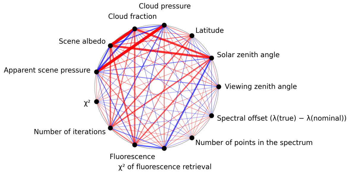
Figure 1: Map of correlation graph for 2025-03-18 to 2025-03-20.
