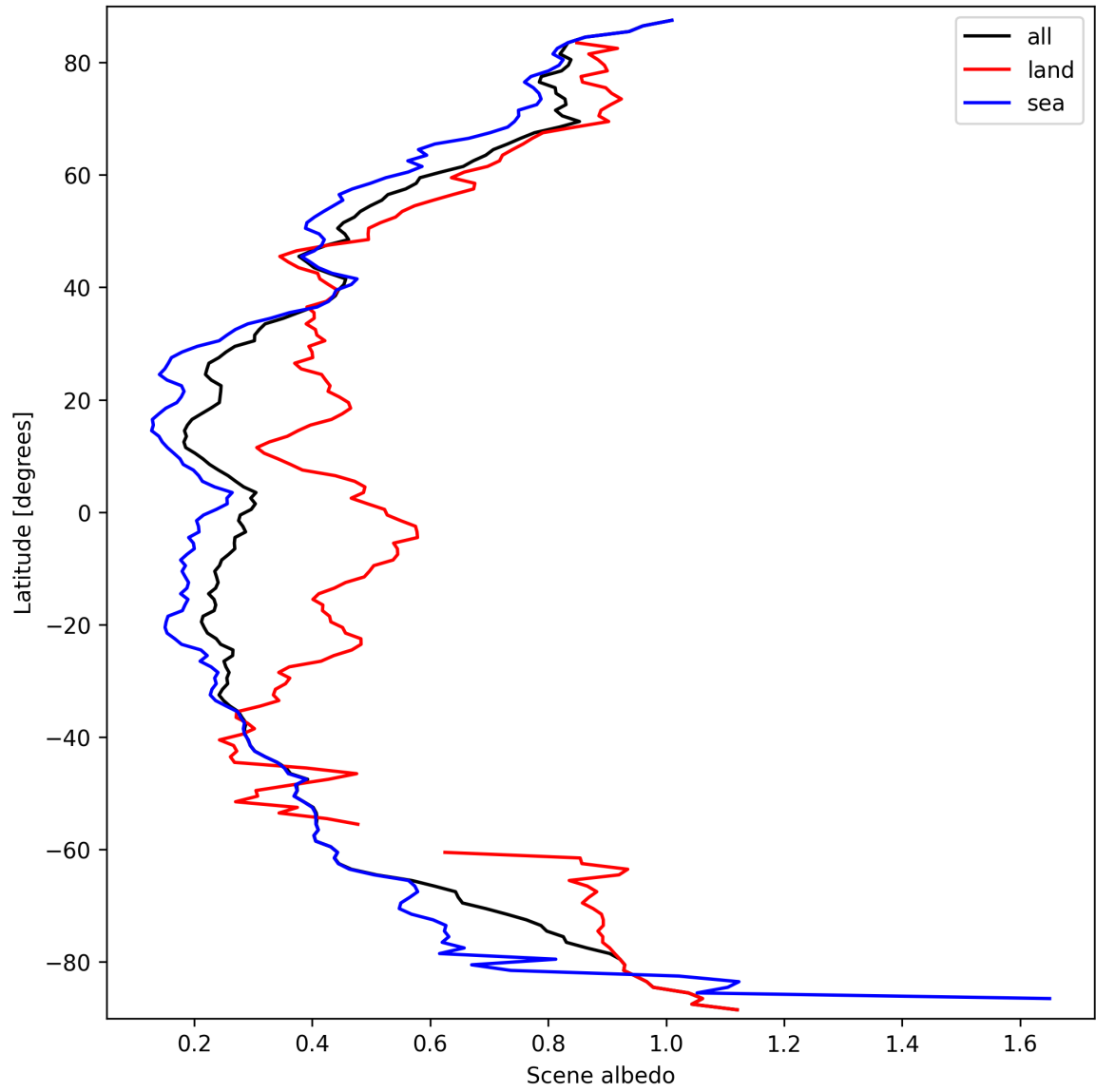
Figure 17: Zonal average of “Scene albedo” for 2025-03-18 to 2025-03-20.
