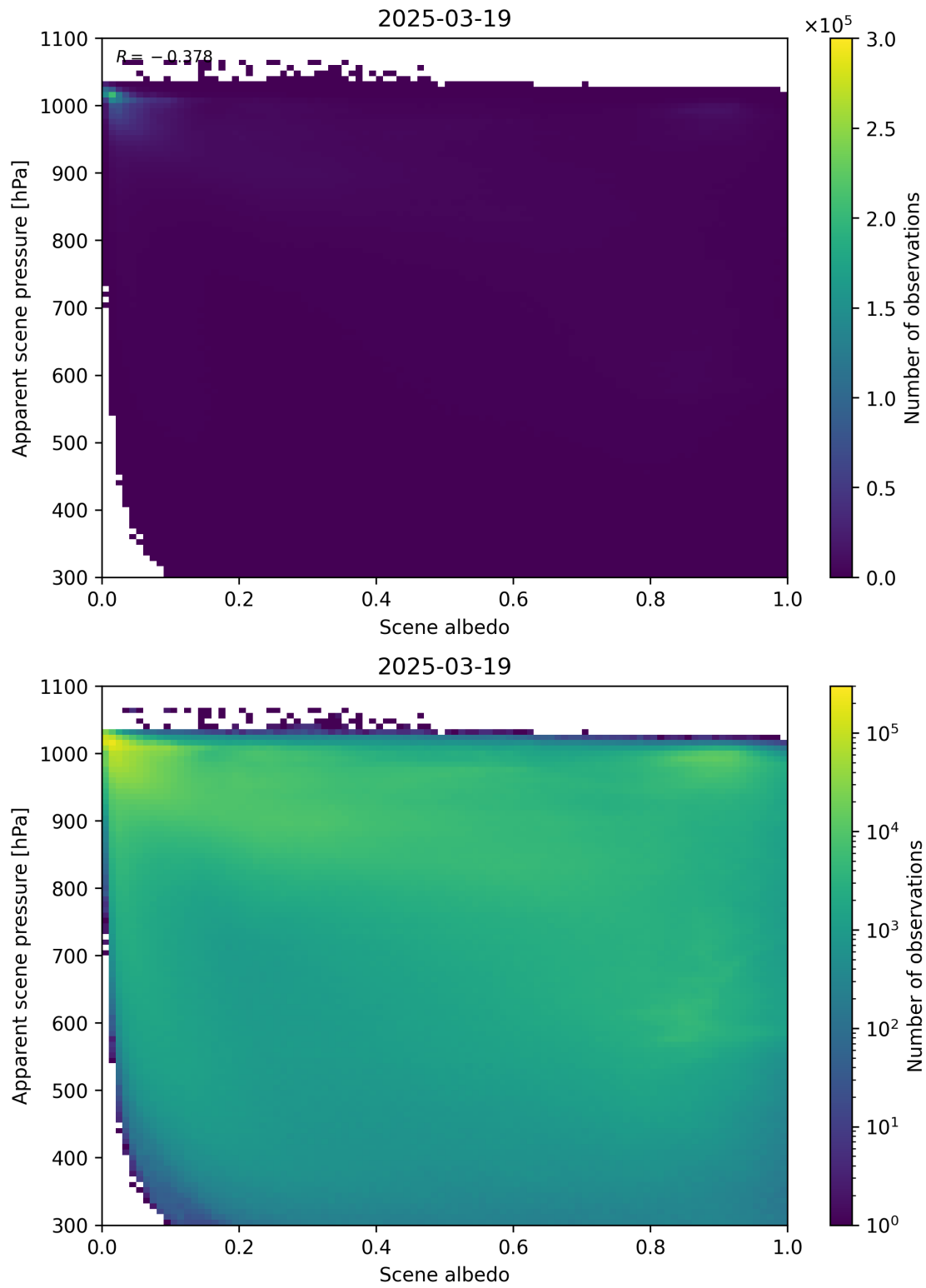
Figure 102: Scatter density plot of “Scene albedo” against “Apparent scene pressure” for 2025-03-18 to 2025-03-20.
