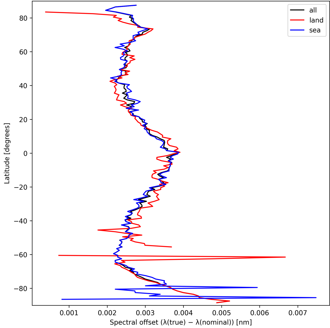
Figure 28: Zonal average of “Spectral offset ( \lambda_{\text{true}} - \lambda_{\text{nominal}} )” for 2025-03-18 to 2025-03-20.
