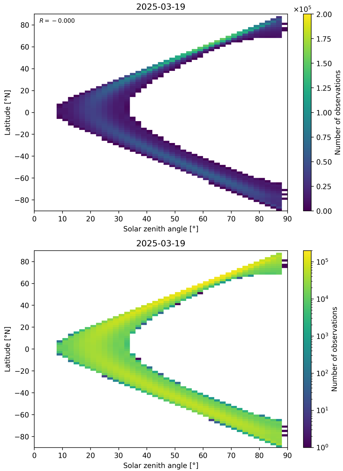
Figure 113: Scatter density plot of “Solar zenith angle” against “Latitude” for 2025-03-18 to 2025-03-20.
