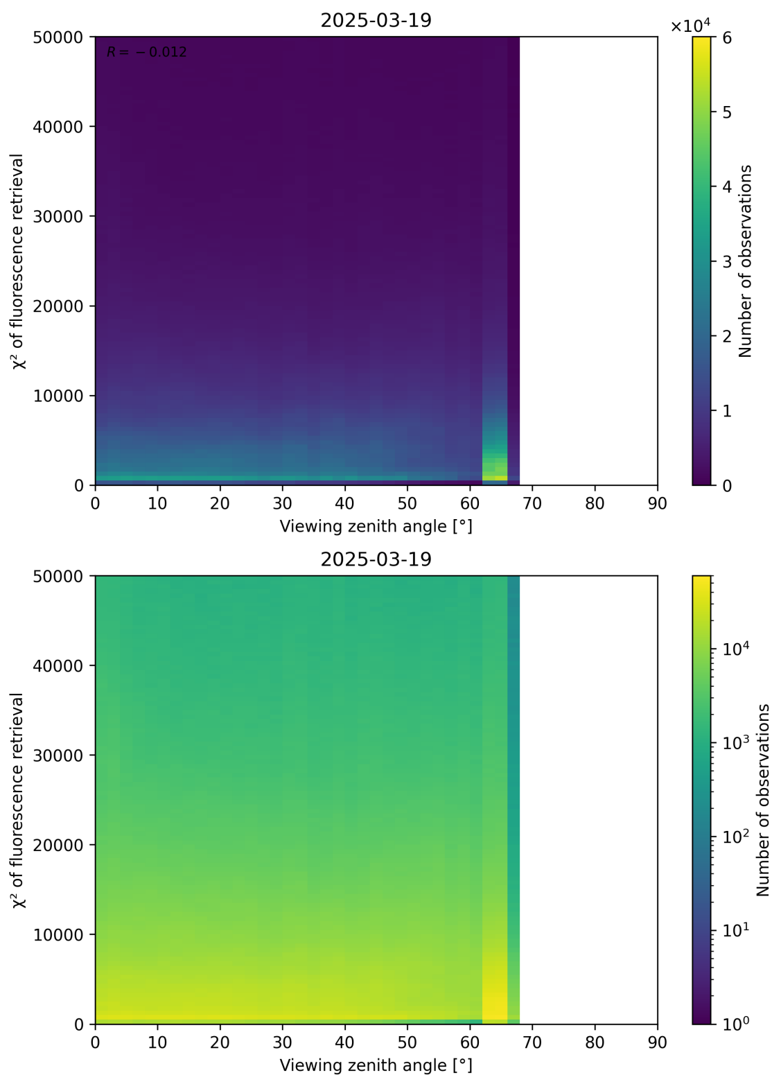
Figure 119: Scatter density plot of “Viewing zenith angle” against “ \chi^2 of fluorescence retrieval” for 2025-03-18 to 2025-03-20.
