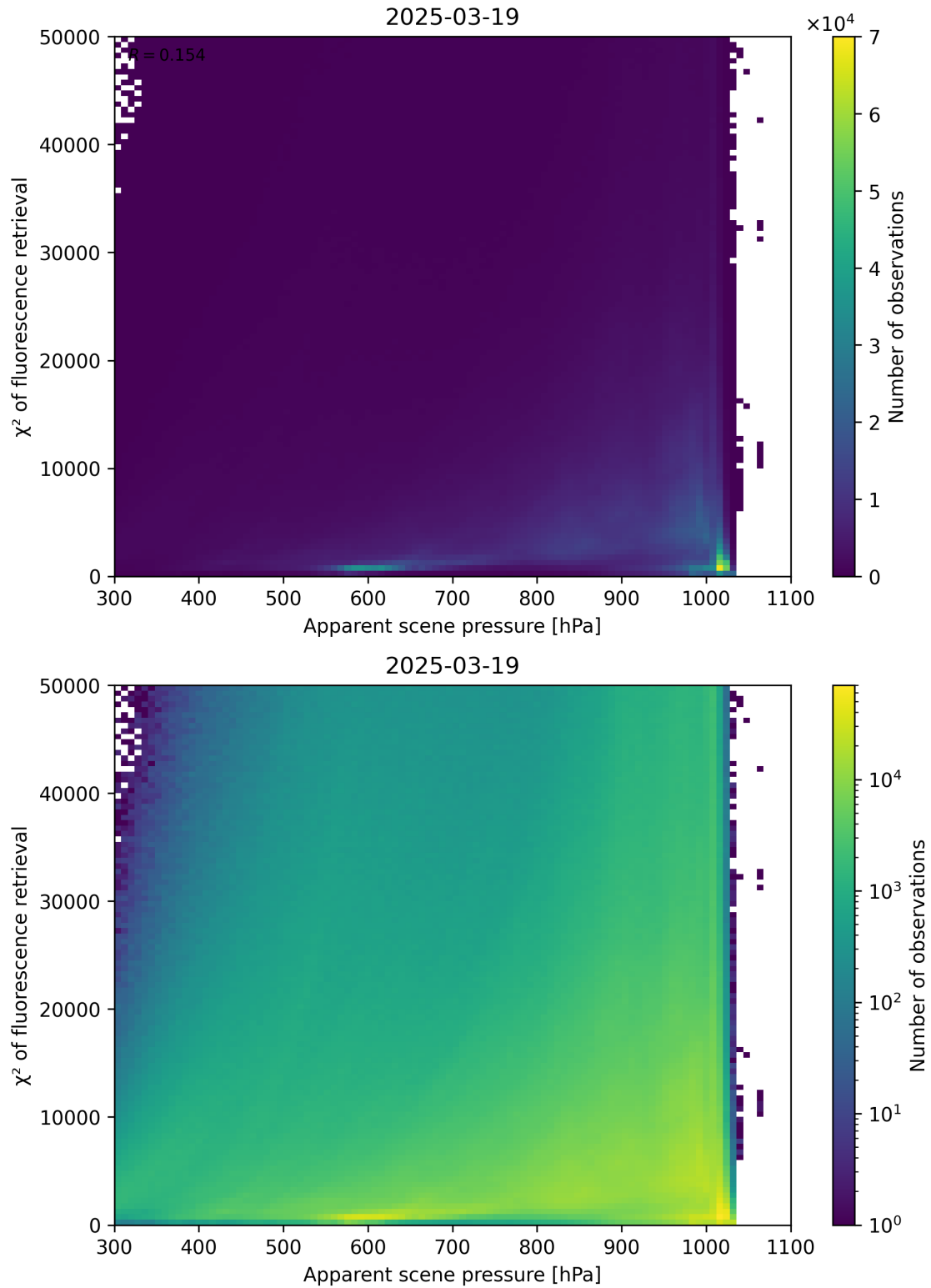
Figure 63: Scatter density plot of “Apparent scene pressure” against “ \chi^2 of fluorescence retrieval” for 2025-03-18 to 2025-03-20.
