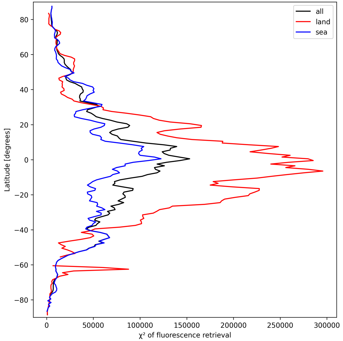
Figure 25: Zonal average of “ \chi^2 of fluorescence retrieval” for 2025-03-18 to 2025-03-20.
