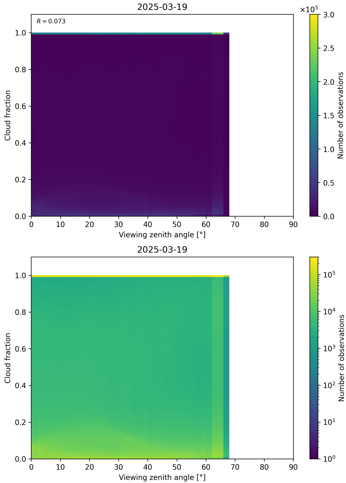
Figure 120: Scatter density plot of “Viewing zenith angle” against “Cloud fraction” for 2025-03-18 to 2025-03-20.
