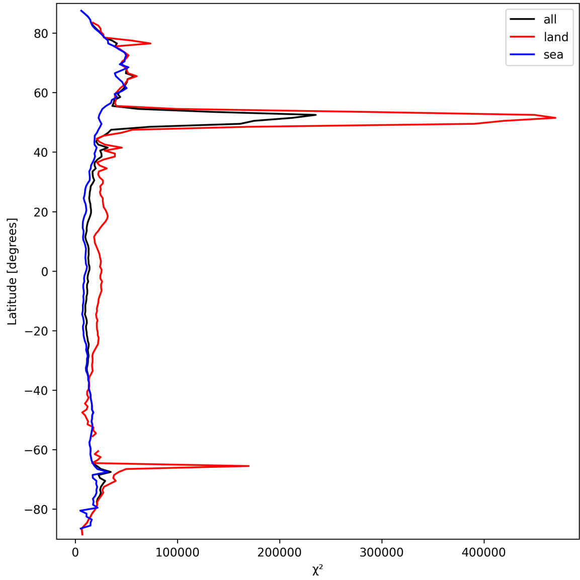
Figure 21: Zonal average of “ \chi^2 ” for 2025-03-18 to 2025-03-20.
