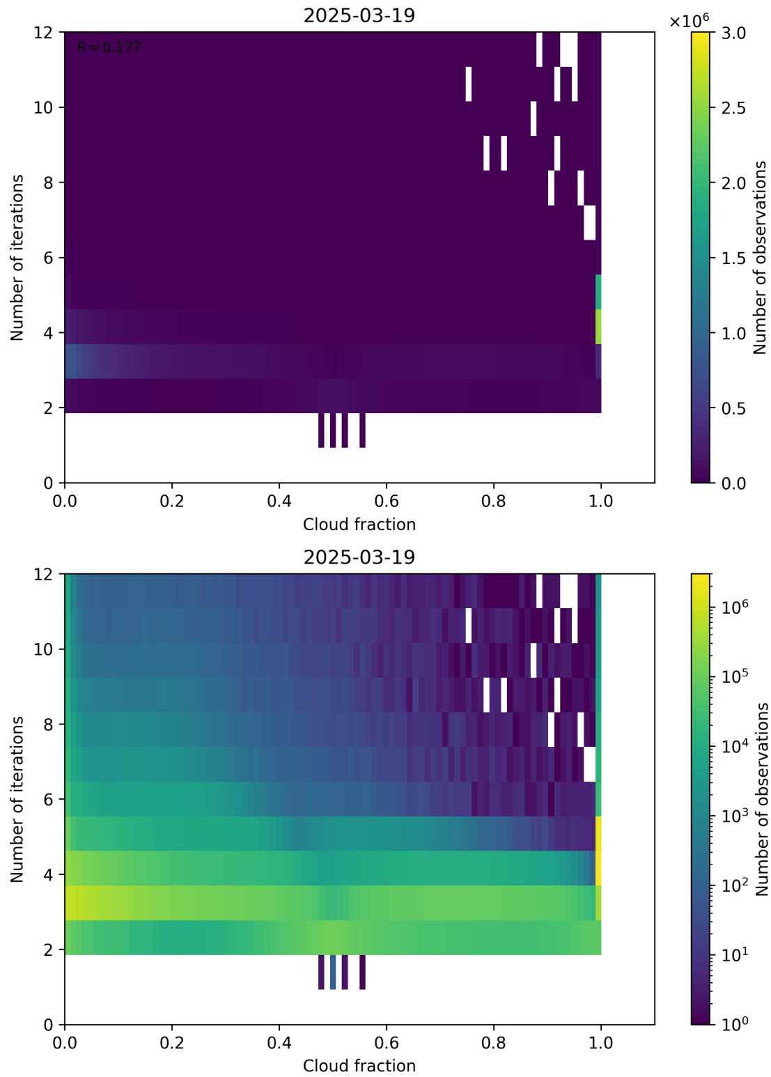
Figure 73: Scatter density plot of “Cloud fraction” against “Number of iterations” for 2025-03-18 to 2025-03-20.
