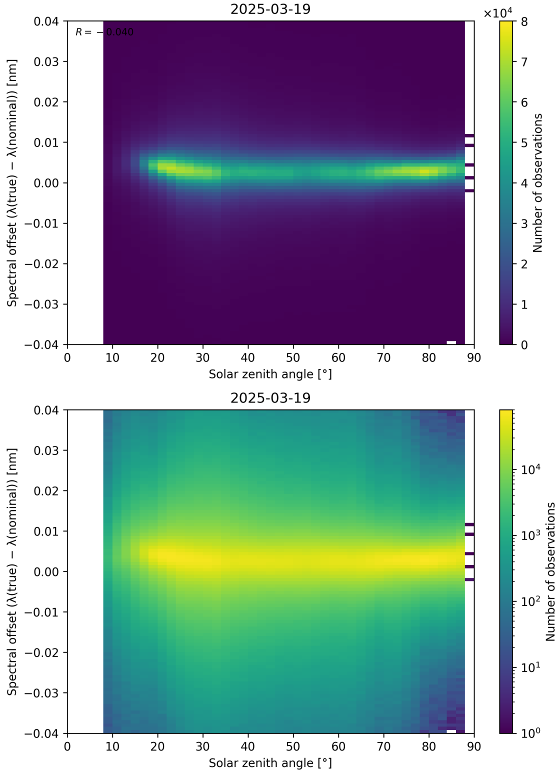
Figure 117: Scatter density plot of “Solar zenith angle” against “Spectral offset ( \lambda_{\text{true}} - \lambda_{\text{nominal}} )” for 2025-03-18 to 2025-03-20.
