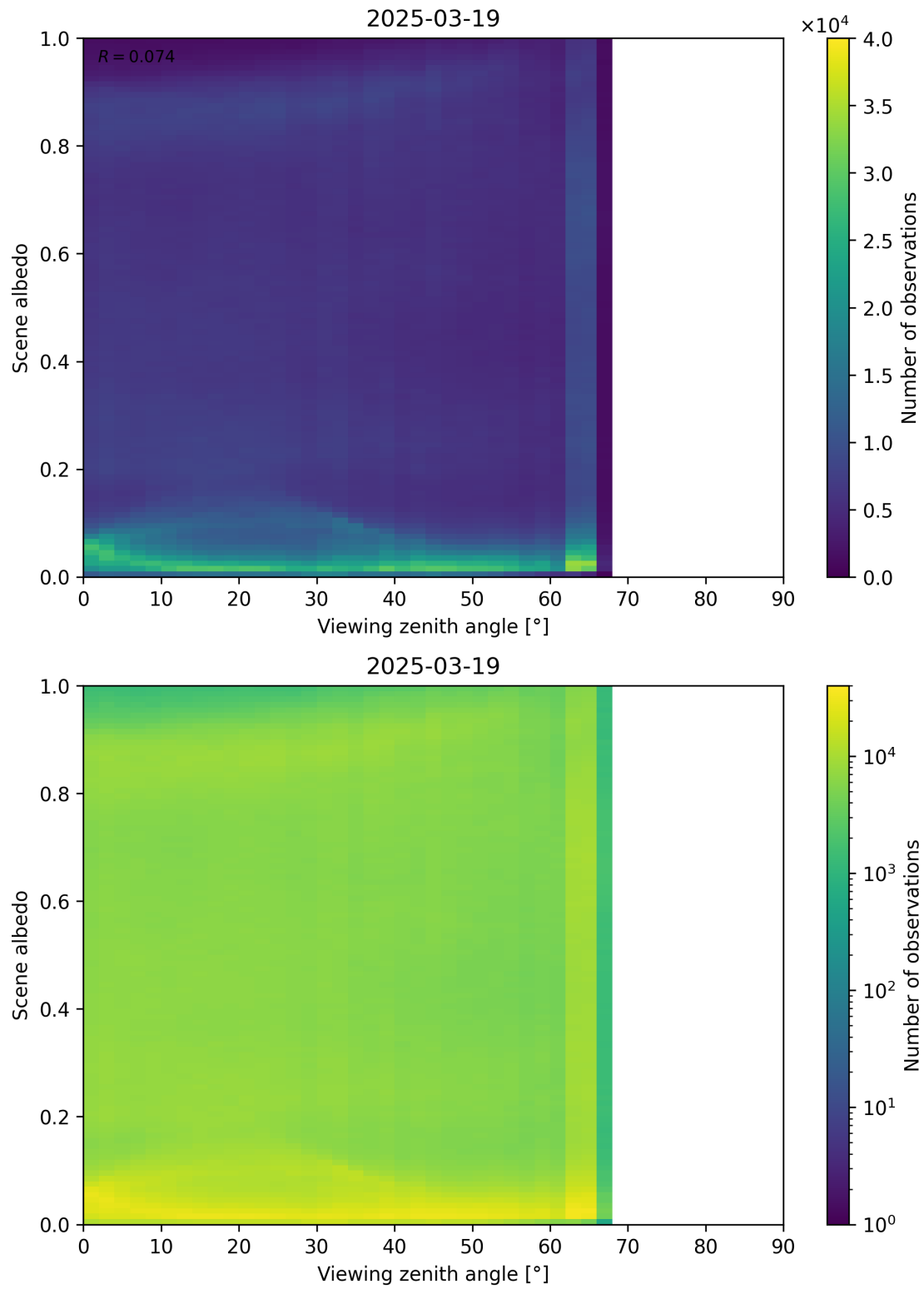
Figure 126: Scatter density plot of “Viewing zenith angle” against “Scene albedo” for 2025-03-18 to 2025-03-20.
