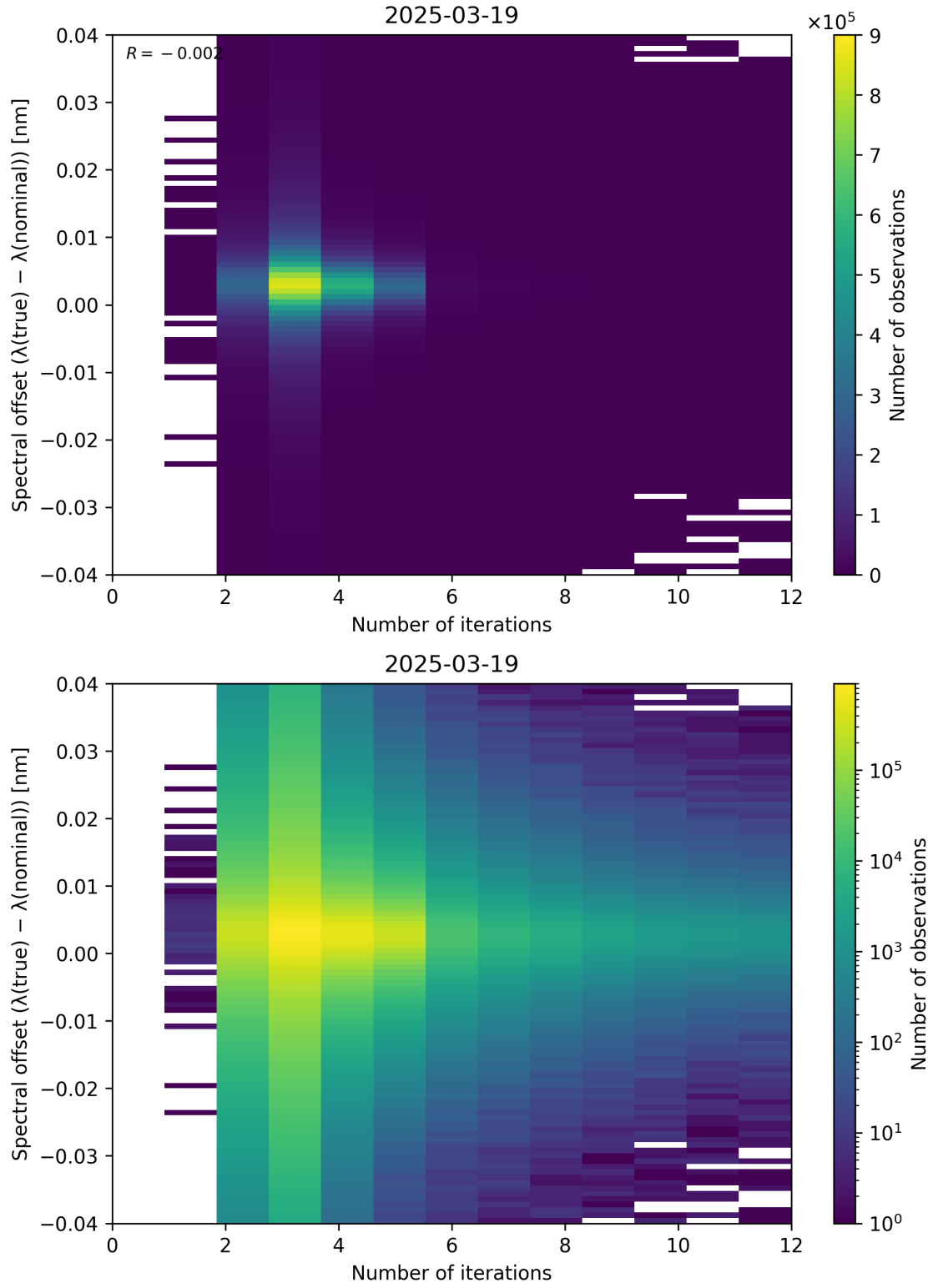
Figure 100: Scatter density plot of “Number of iterations” against “Spectral offset ( \lambda_{\text{true}} - \lambda_{\text{nominal}} )” for 2025-03-18 to 2025-03-20.
