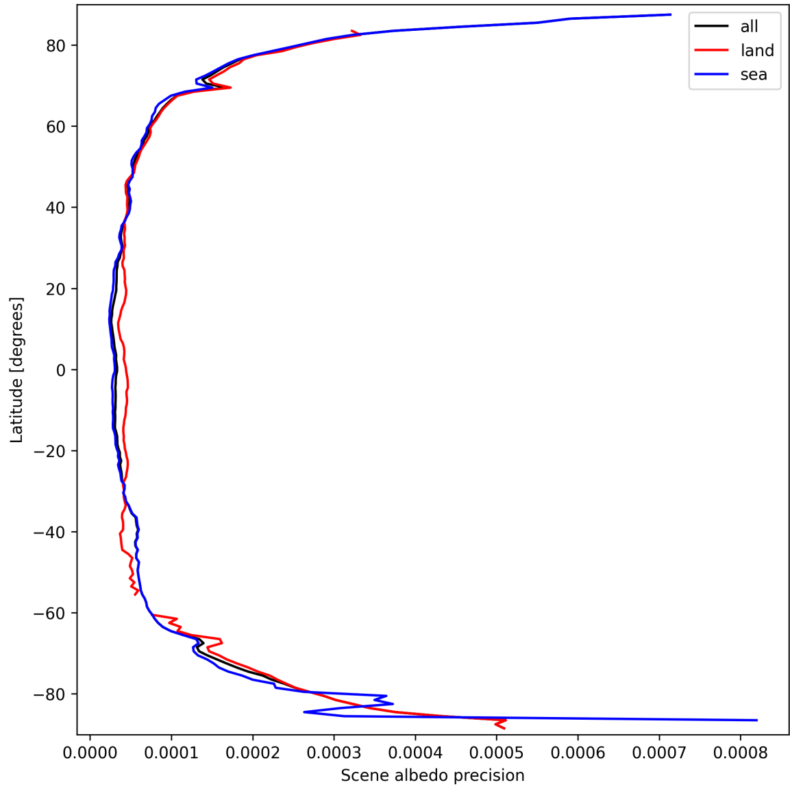
Figure 18: Zonal average of “Scene albedo precision” for 2025-03-18 to 2025-03-20.
