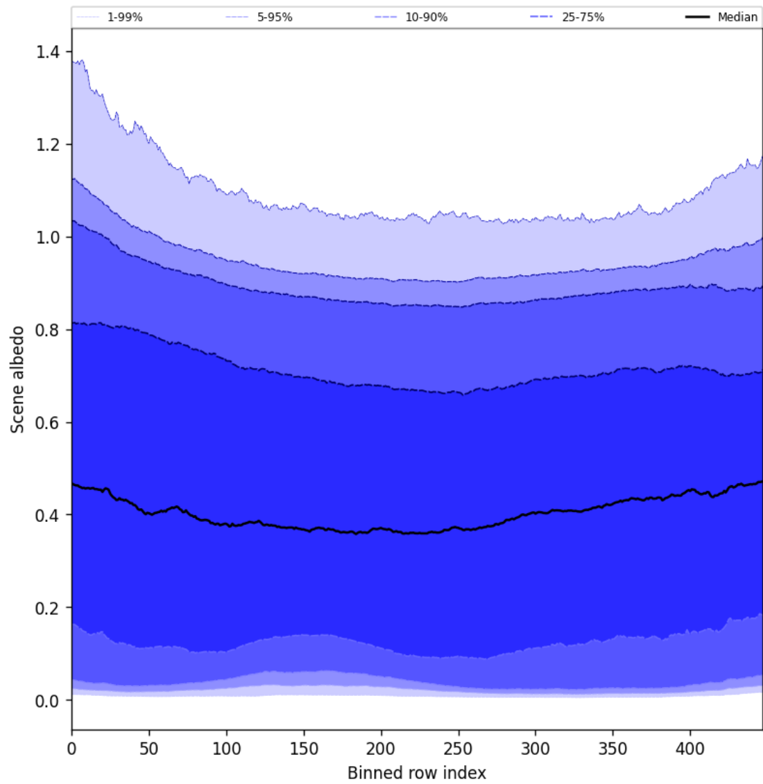
Figure 51: Along track statistics of “Scene albedo” for 2025-03-18 to 2025-03-20
