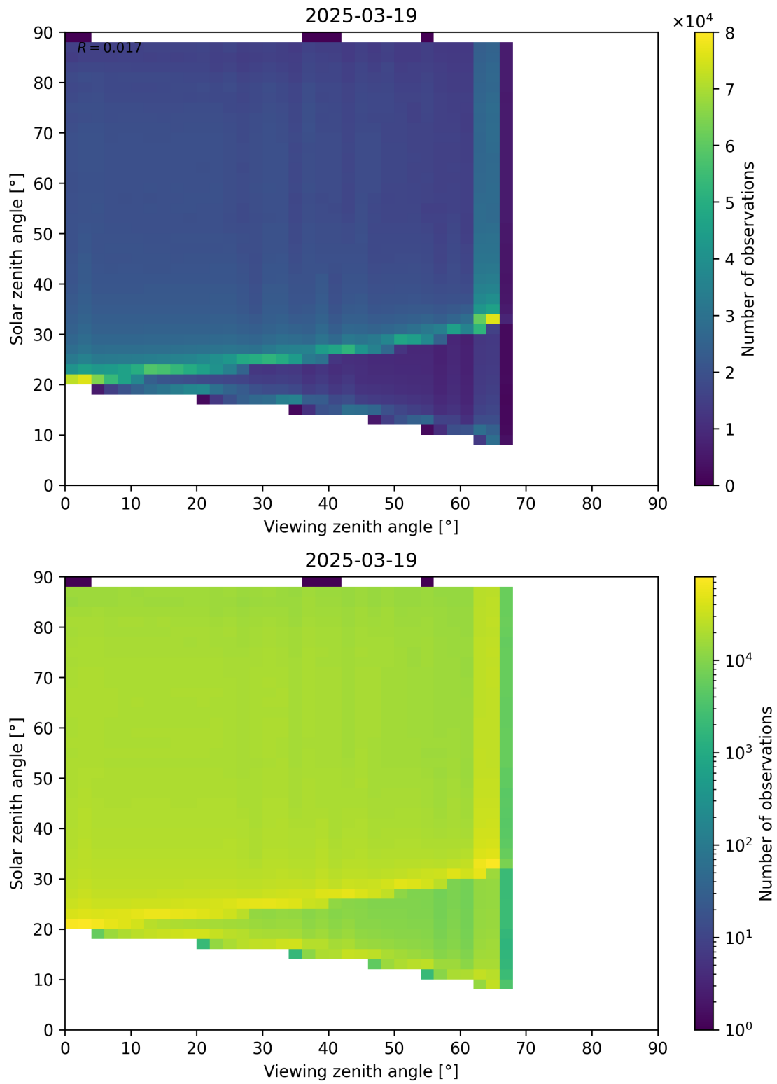
Figure 127: Scatter density plot of “Viewing zenith angle” against “Solar zenith angle” for 2025-03-18 to 2025-03-20.
