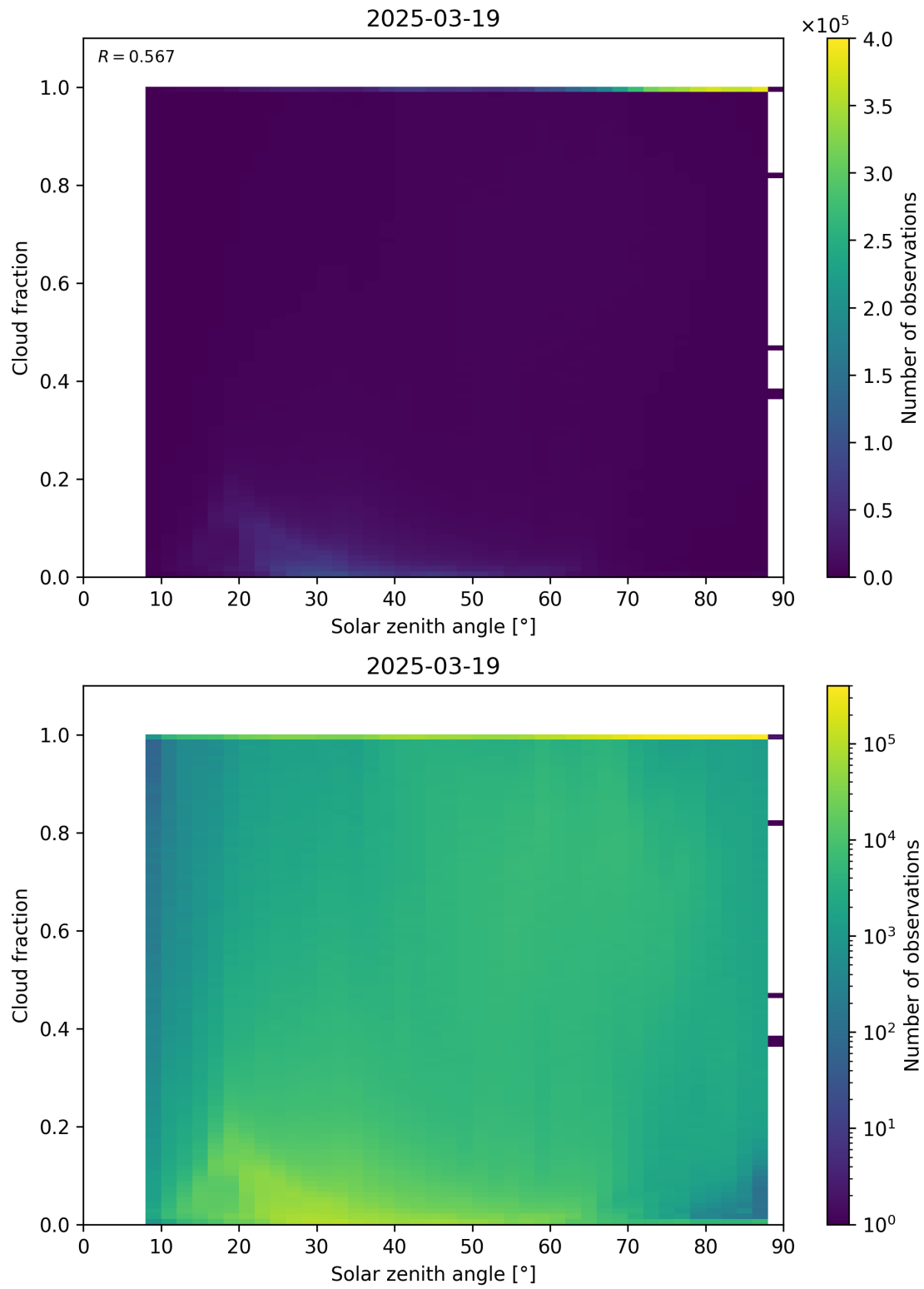
Figure 110: Scatter density plot of “Solar zenith angle” against “Cloud fraction” for 2025-03-18 to 2025-03-20.
