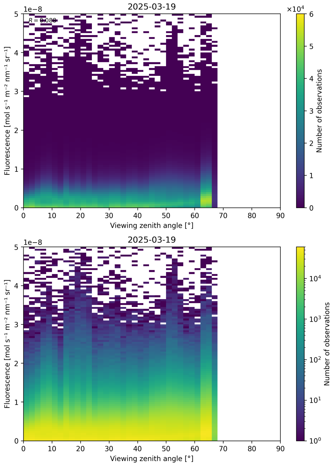
Figure 122: Scatter density plot of “Viewing zenith angle” against “Fluorescence” for 2025-03-18 to 2025-03-20.
