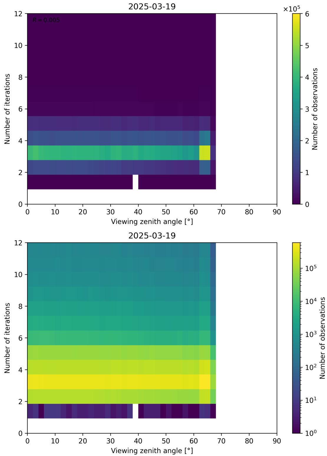
Figure 124: Scatter density plot of “Viewing zenith angle” against “Number of iterations” for 2025-03-18 to 2025-03-20.
