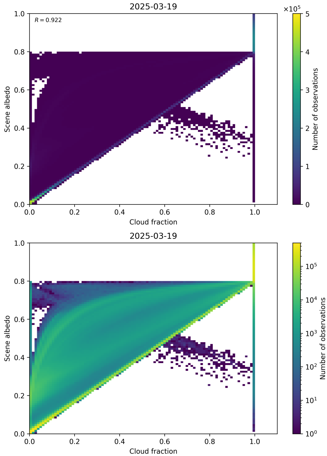
Figure 75: Scatter density plot of “Cloud fraction” against “Scene albedo” for 2025-03-18 to 2025-03-20.
