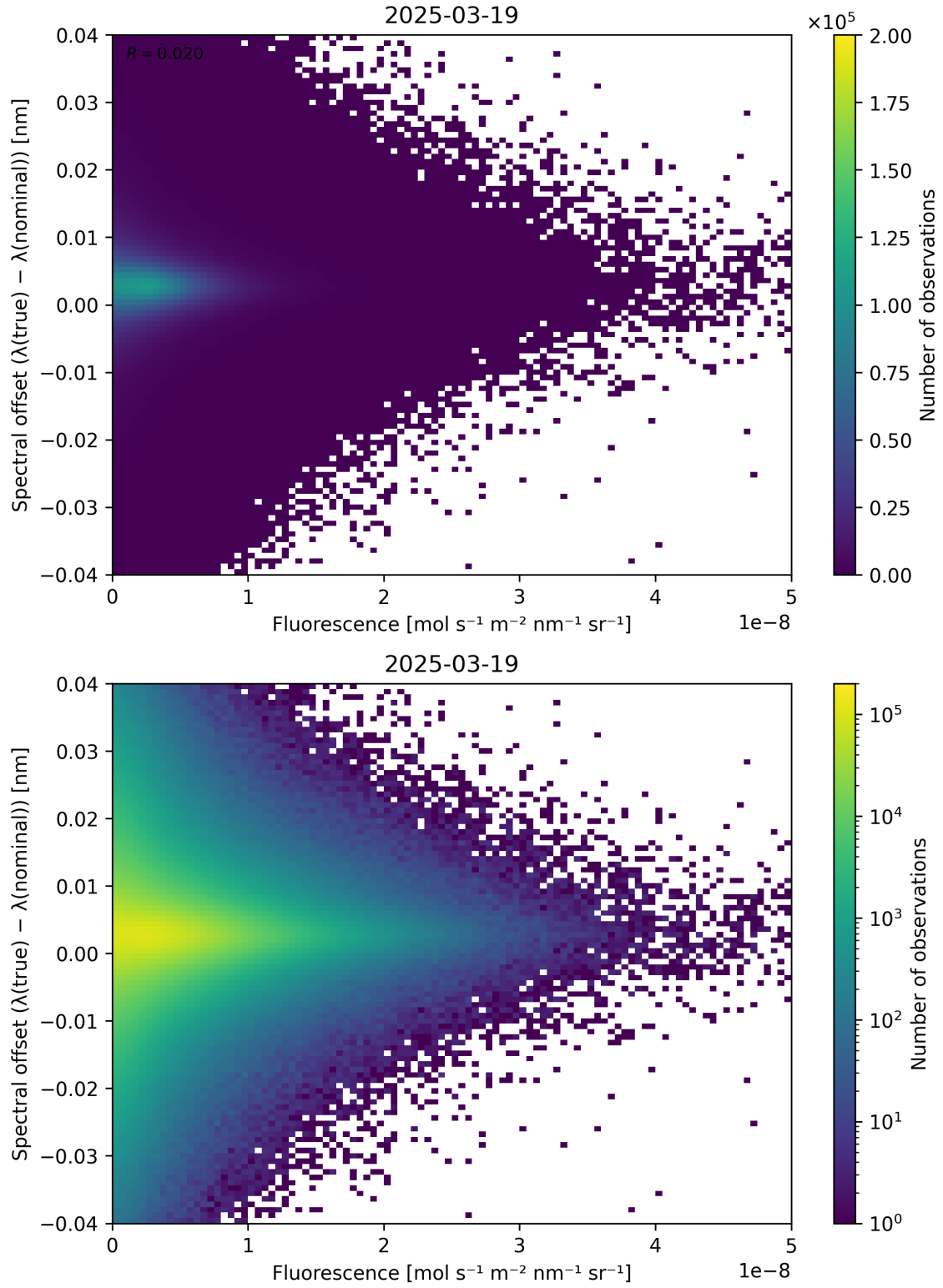
Figure 87: Scatter density plot of “Fluorescence” against “Spectral offset ( \lambda_{\text{true}} - \lambda_{\text{nominal}} )” for 2025-03-18 to 2025-03-20.
