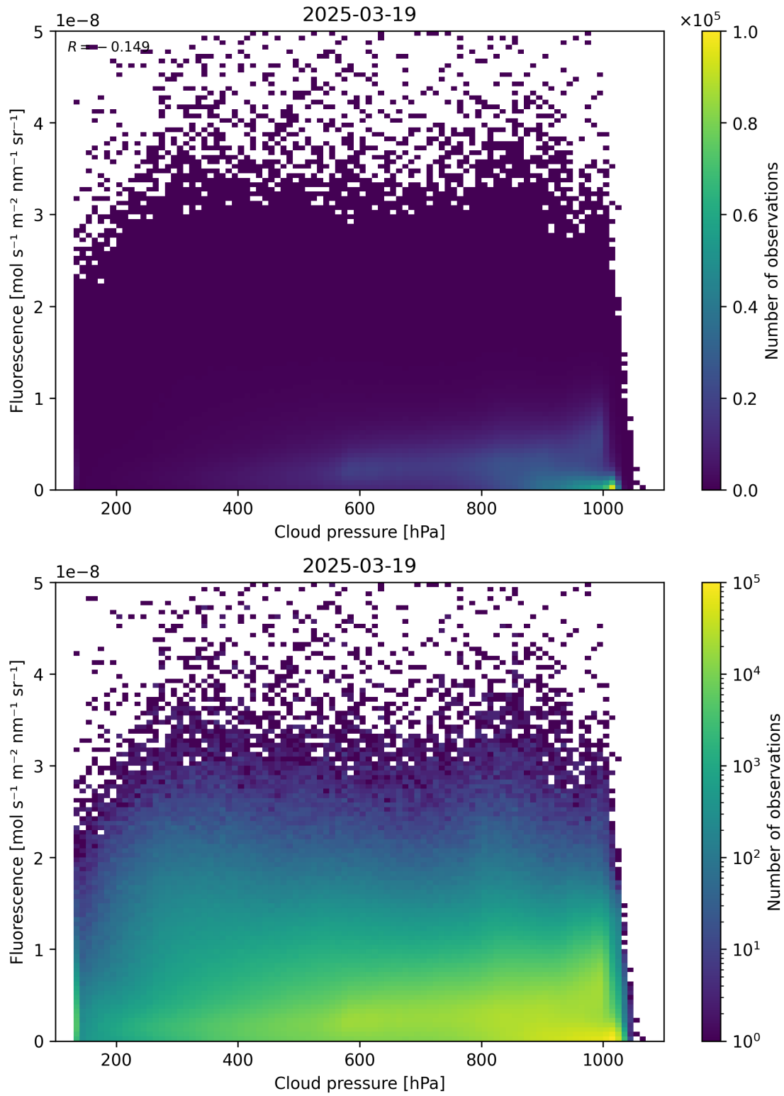
Figure 80: Scatter density plot of “Cloud pressure” against “Fluorescence” for 2025-03-18 to 2025-03-20.
