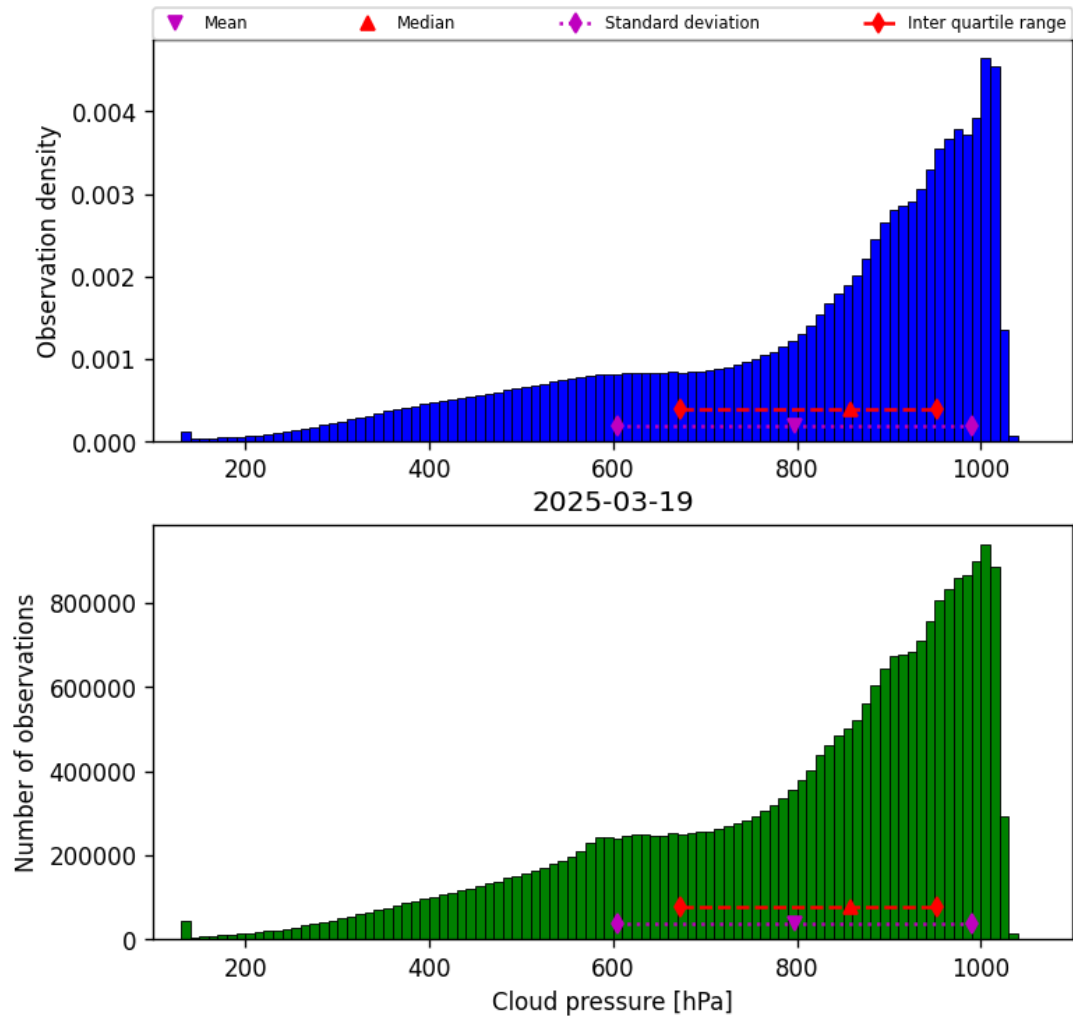
Figure 30: Histogram of “Cloud pressure” for 2025-03-18 to 2025-03-20
