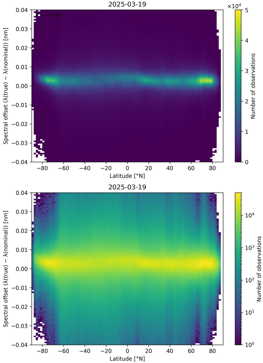
Figure 96: Scatter density plot of “Latitude” against “Spectral offset ( \lambda_{\text{true}} - \lambda_{\text{nominal}} )” for 2025-03-18 to 2025-03-20.
