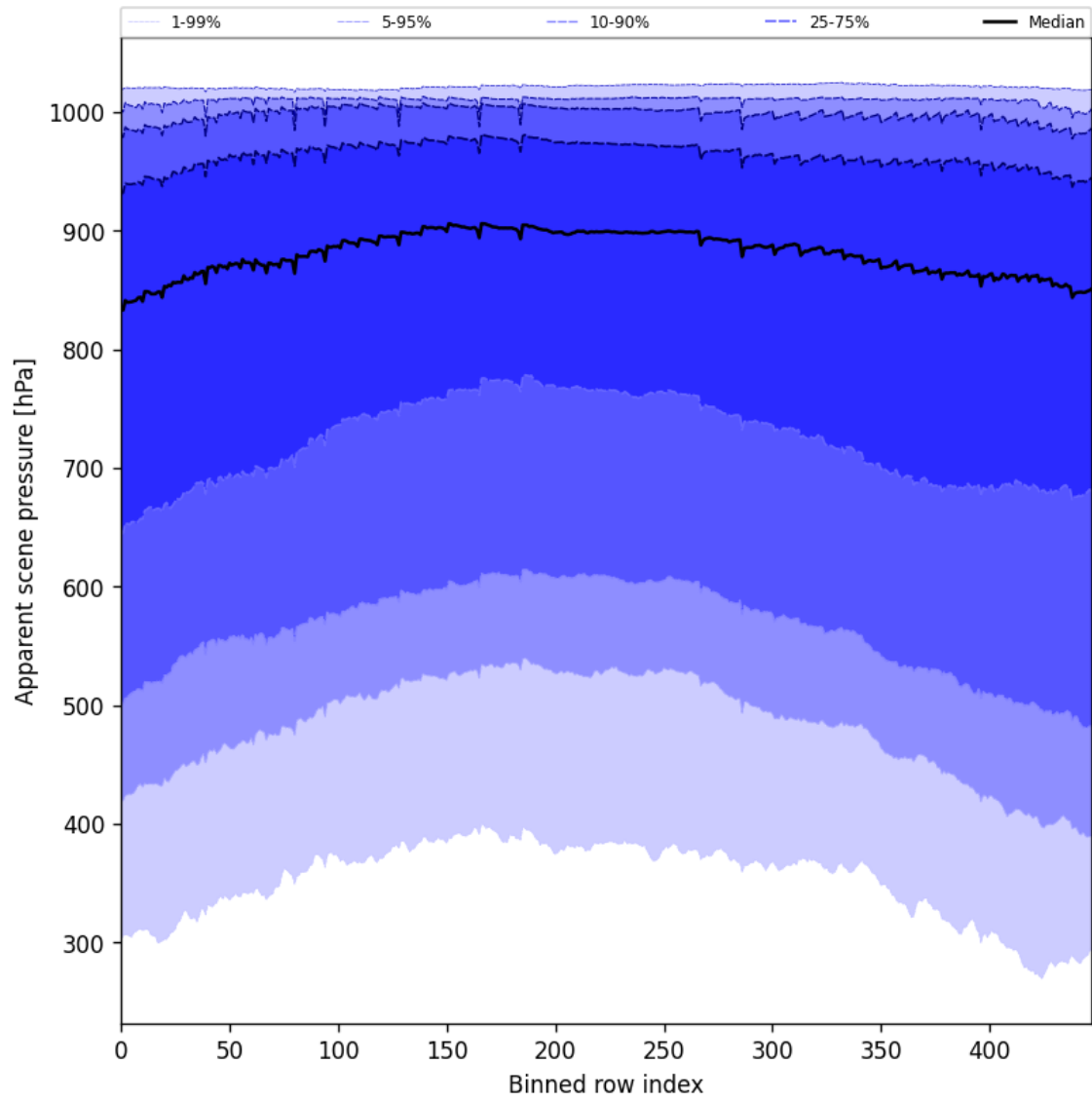
Figure 53: Along track statistics of “Apparent scene pressure” for 2025-03-18 to 2025-03-20
