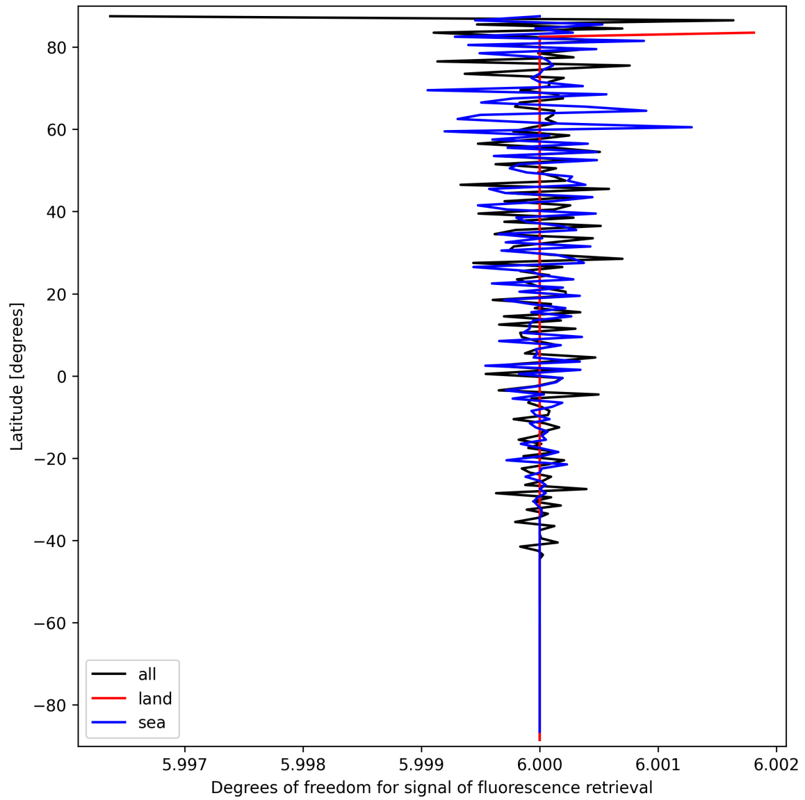
Figure 26: Zonal average of “Degrees of freedom for signal of fluorescence retrieval” for 2025-03-18 to 2025-03-20.
