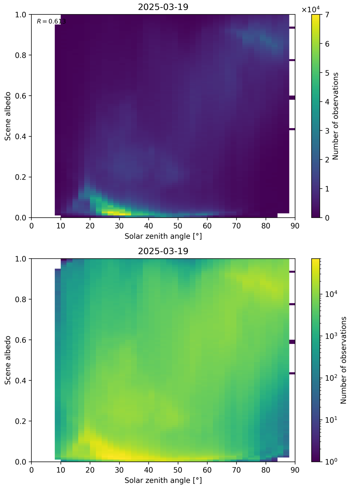
Figure 116: Scatter density plot of “Solar zenith angle” against “Scene albedo” for 2025-03-18 to 2025-03-20.
