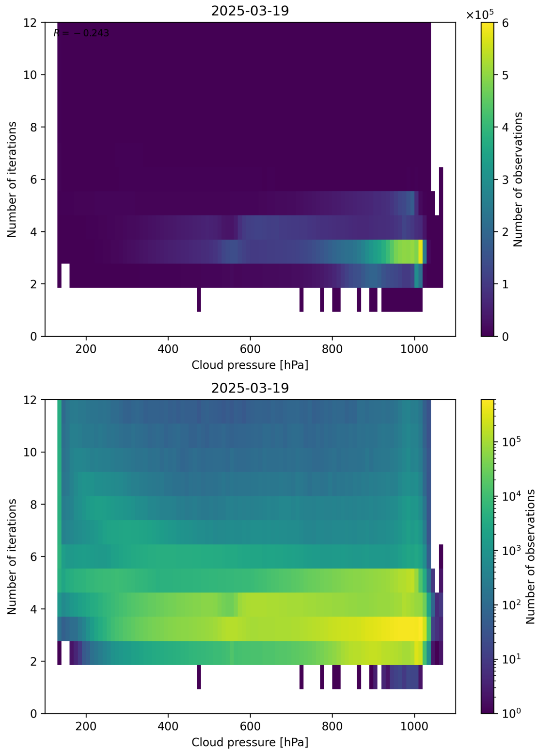
Figure 81: Scatter density plot of “Cloud pressure” against “Number of iterations” for 2025-03-18 to 2025-03-20.
