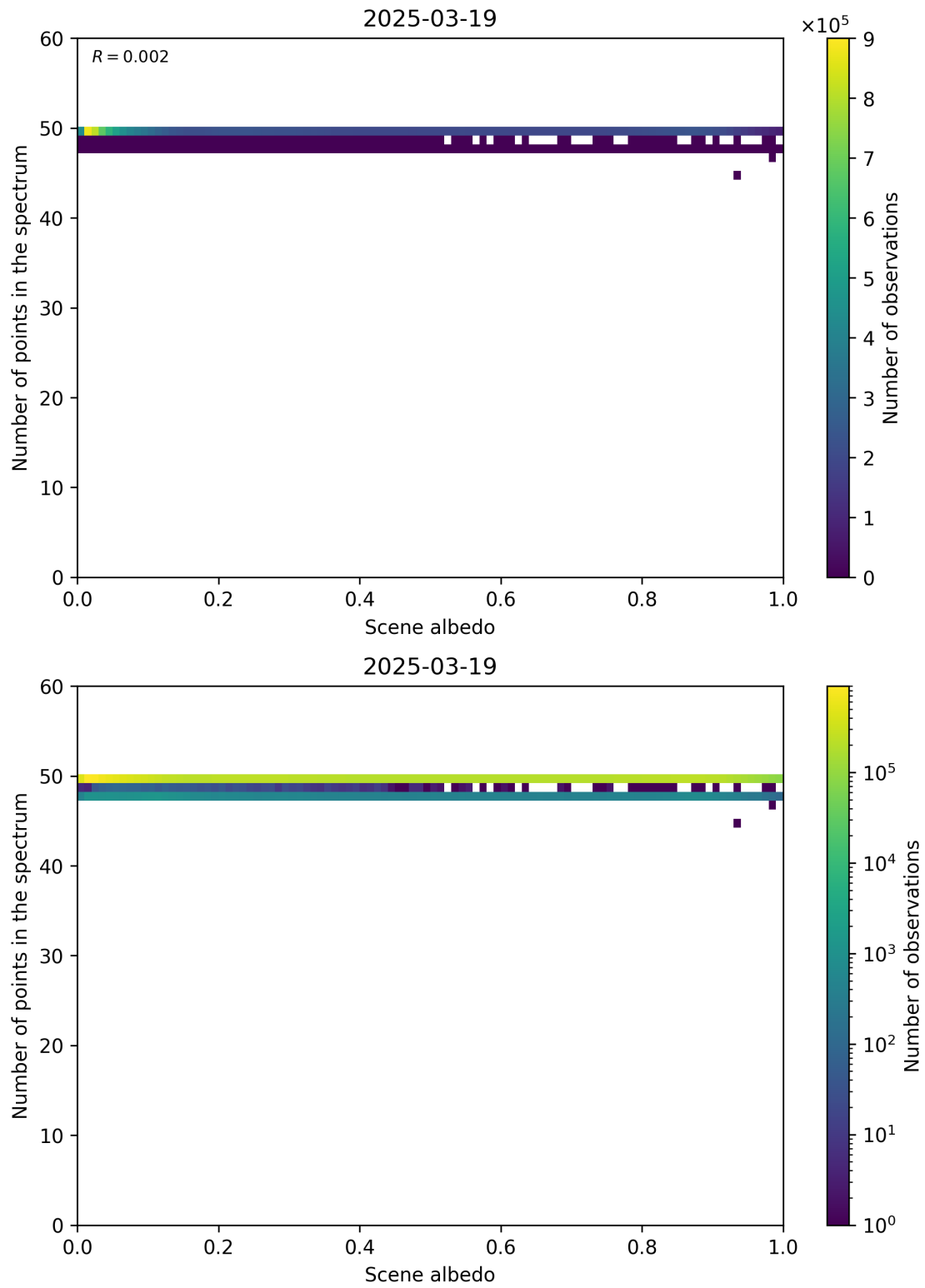
Figure 106: Scatter density plot of “Scene albedo” against “Number of points in the spectrum” for 2025-03-18 to 2025-03-20.
