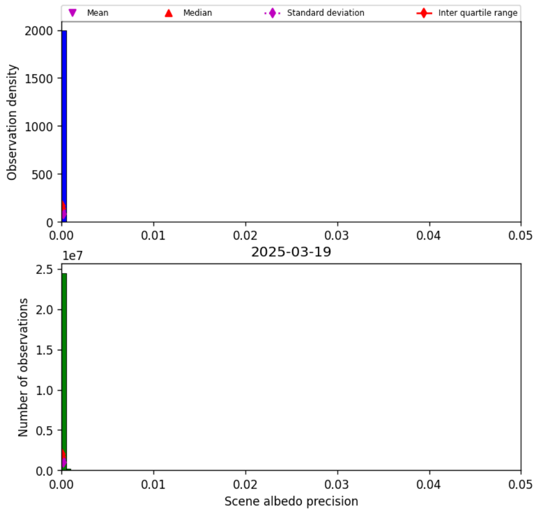
Figure 35: Histogram of “Scene albedo precision” for 2025-03-18 to 2025-03-20
