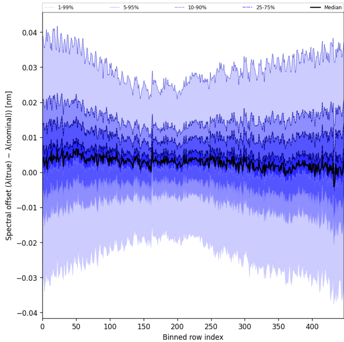
Figure 62: Along track statistics of “Spectral offset ( \lambda_{\text{true}} - \lambda_{\text{nominal}} )” for 2025-03-18 to 2025-03-20
