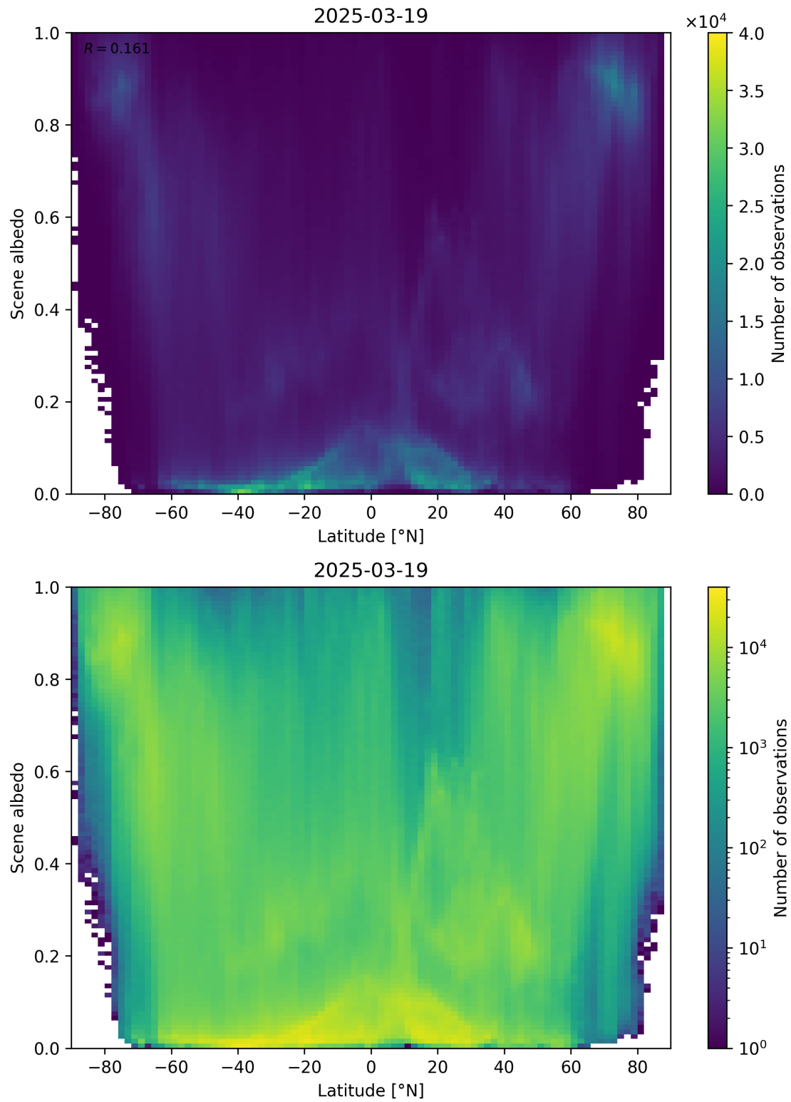
Figure 95: Scatter density plot of “Latitude” against “Scene albedo” for 2025-03-18 to 2025-03-20.
