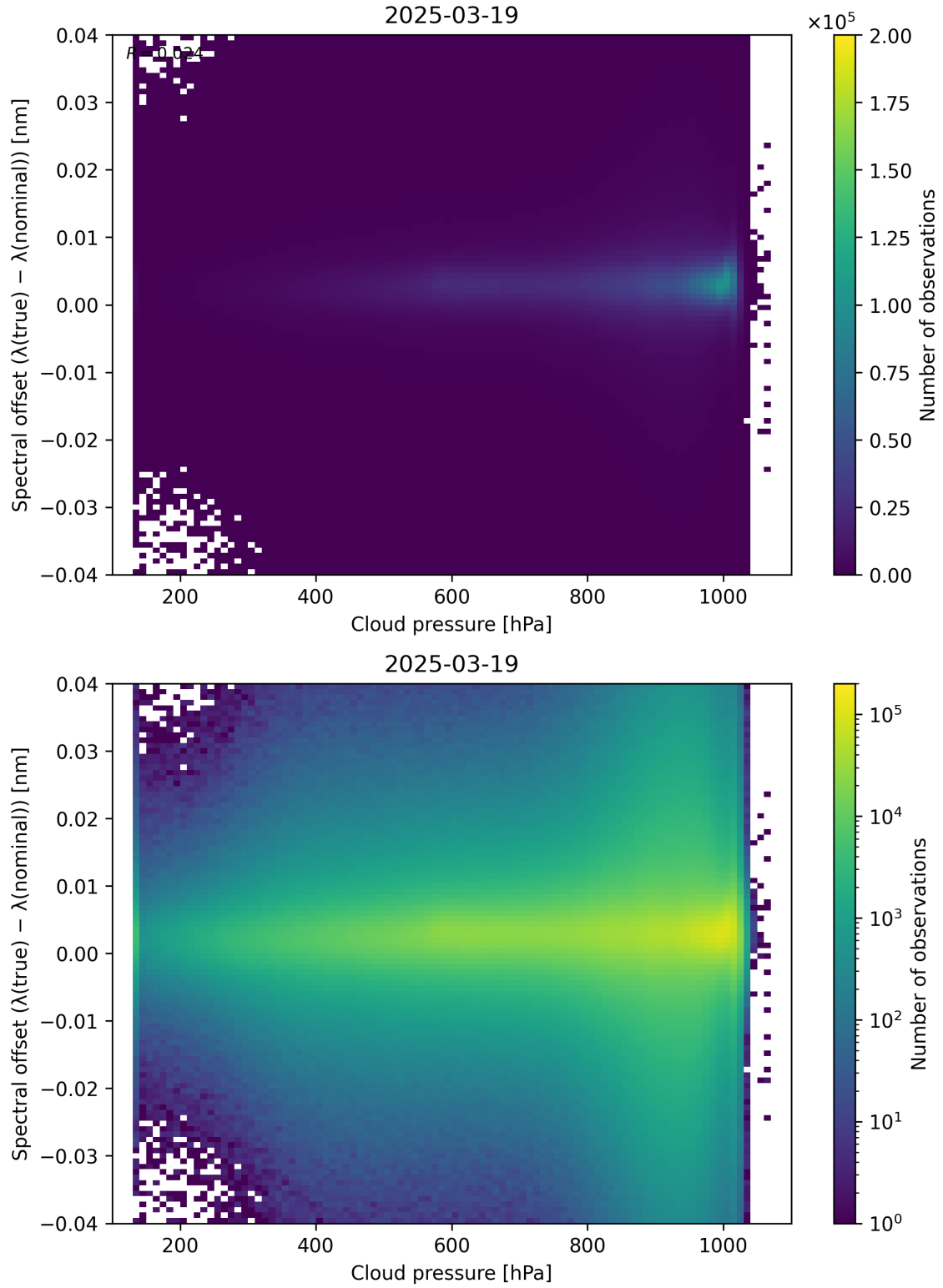
Figure 84: Scatter density plot of “Cloud pressure” against “Spectral offset ( \lambda_{\text{true}} - \lambda_{\text{nominal}} )” for 2025-03-18 to 2025-03-20.
