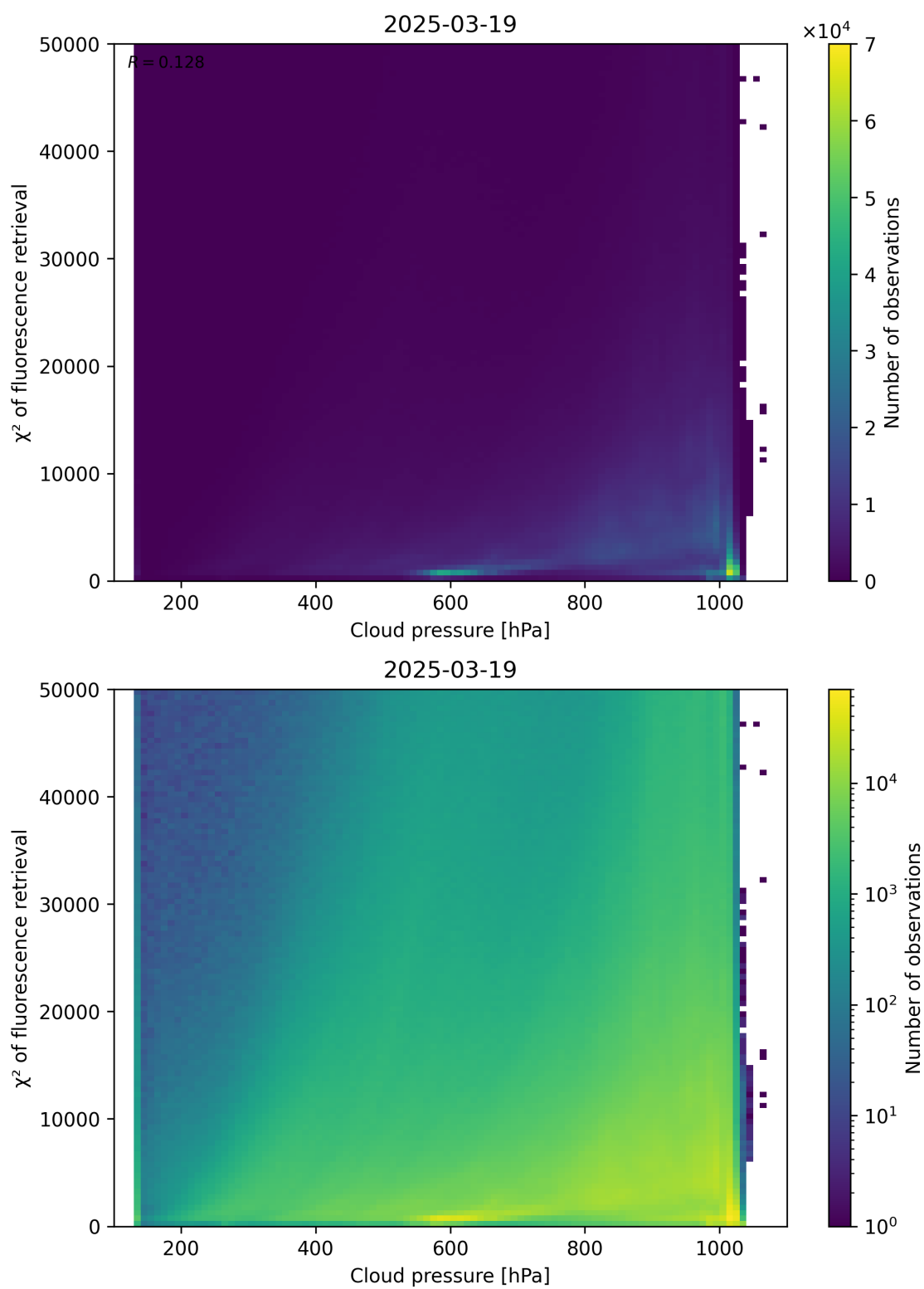
Figure 78: Scatter density plot of “Cloud pressure” against “ \chi^2 of fluorescence retrieval” for 2025-03-18 to 2025-03-20.
