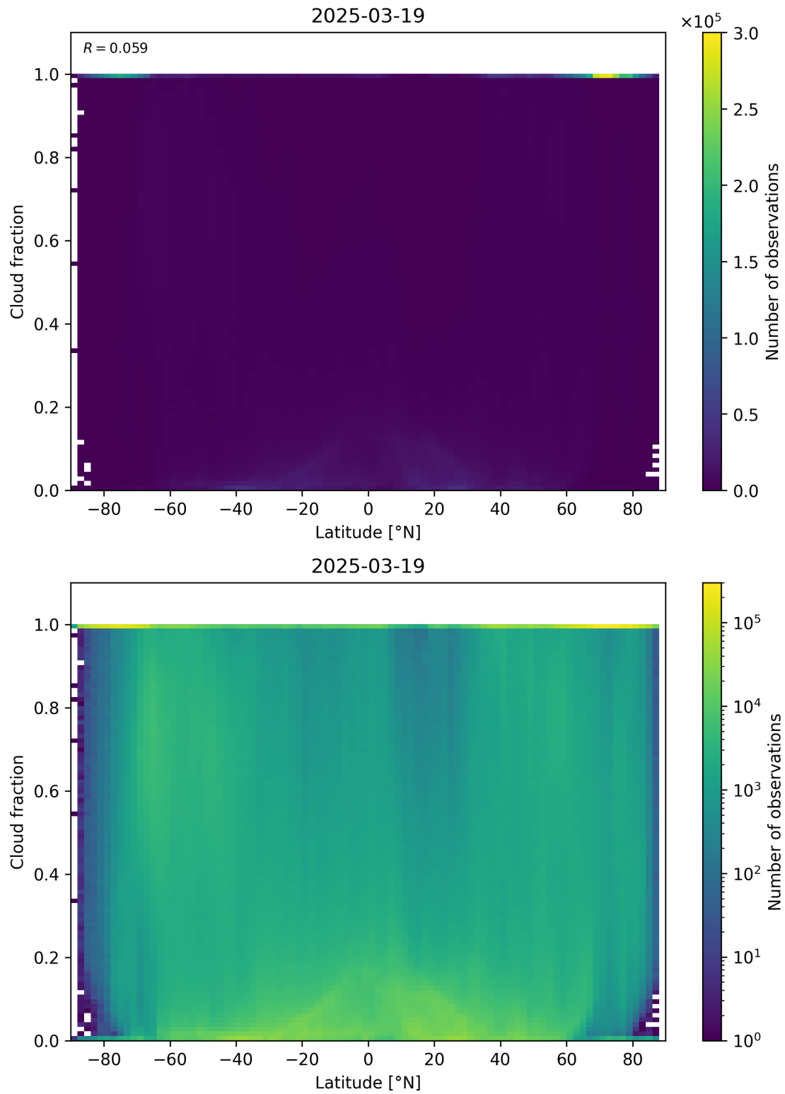
Figure 90: Scatter density plot of “Latitude” against “Cloud fraction” for 2025-03-18 to 2025-03-20.
