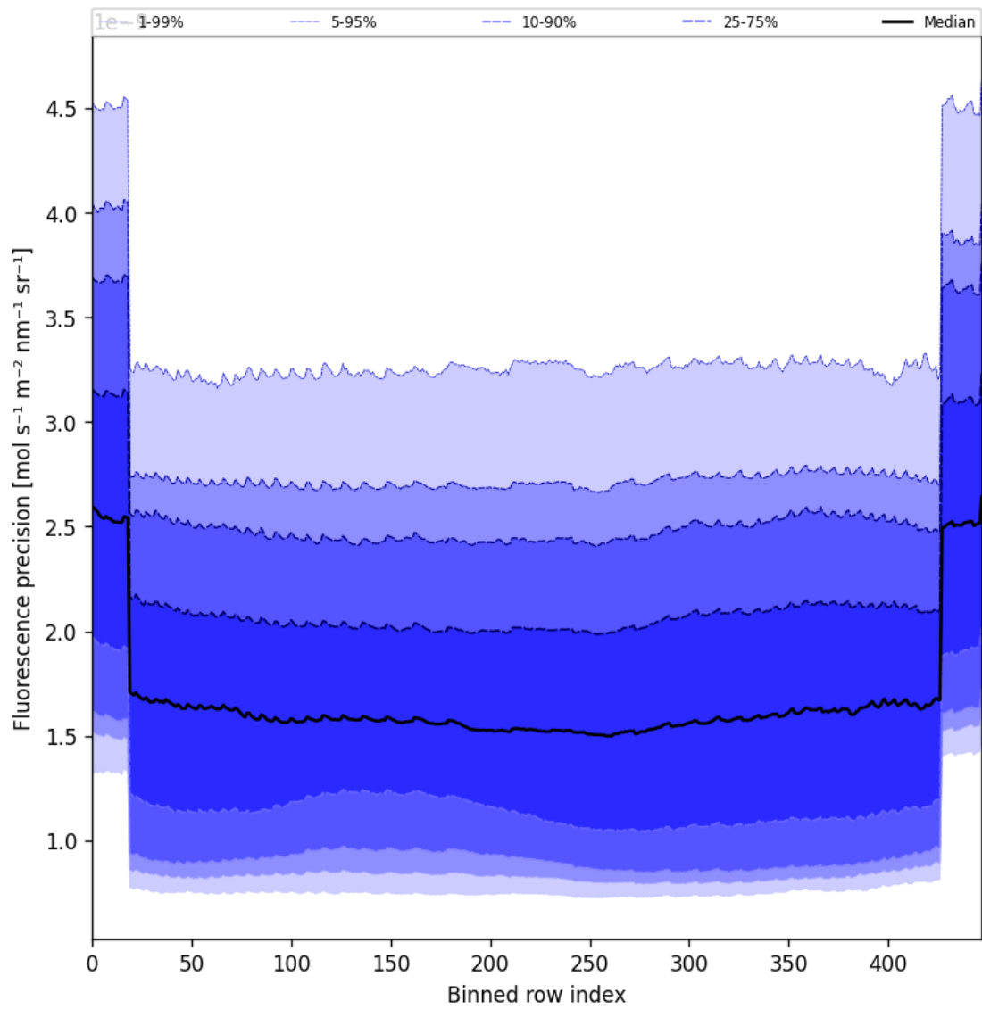
Figure 58: Along track statistics of “Fluorescence precision” for 2025-03-18 to 2025-03-20
