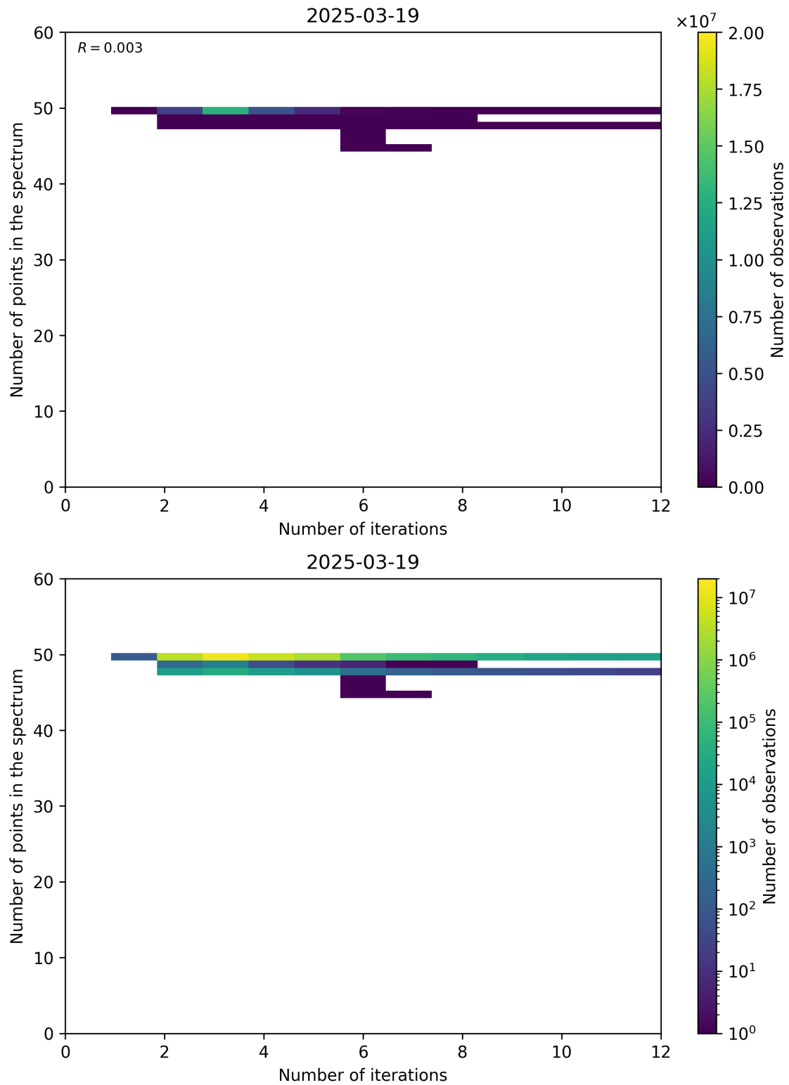
Figure 99: Scatter density plot of “Number of iterations” against “Number of points in the spectrum” for 2025-03-18 to 2025-03-20.
