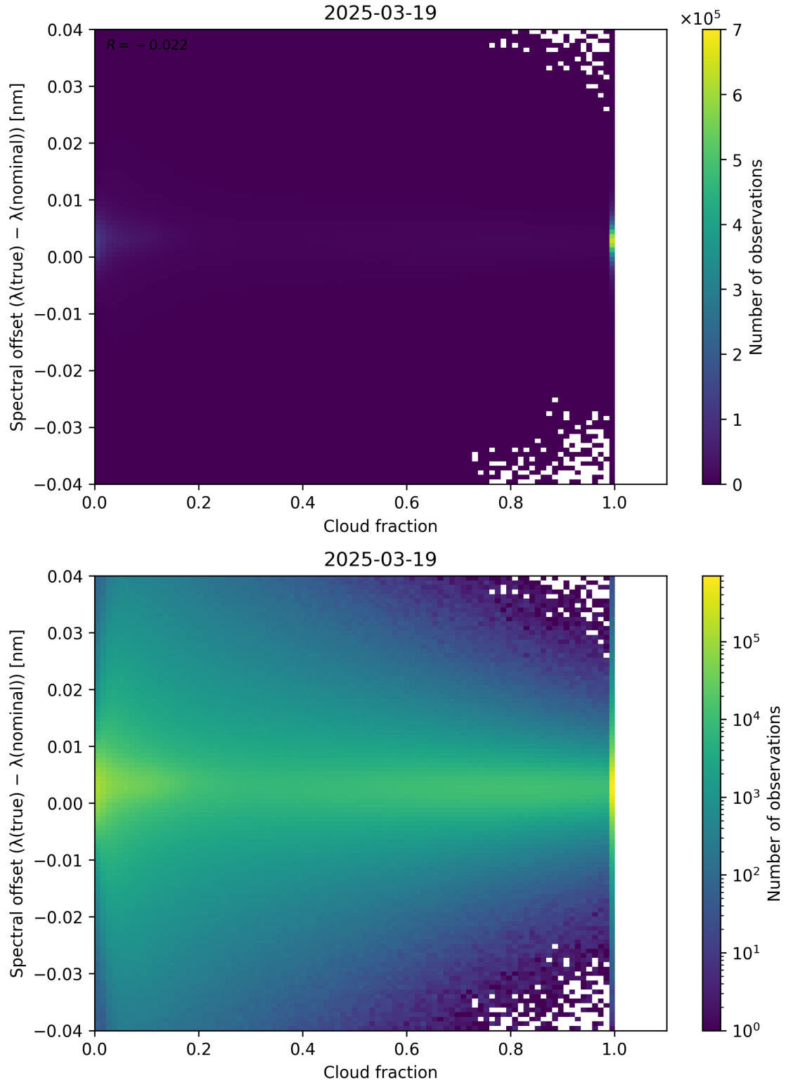
Figure 76: Scatter density plot of “Cloud fraction” against “Spectral offset ( \lambda_{\text{true}} - \lambda_{\text{nominal}} )” for 2025-03-18 to 2025-03-20.
