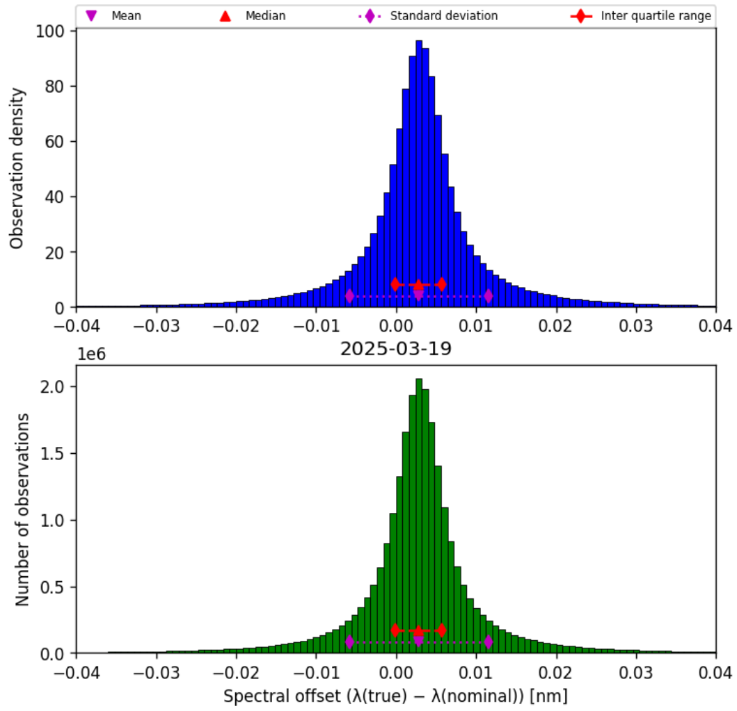
Figure 45: Histogram of “Spectral offset ( \lambda_{\text{true}} - \lambda_{\text{nominal}} )” for 2025-03-18 to 2025-03-20
