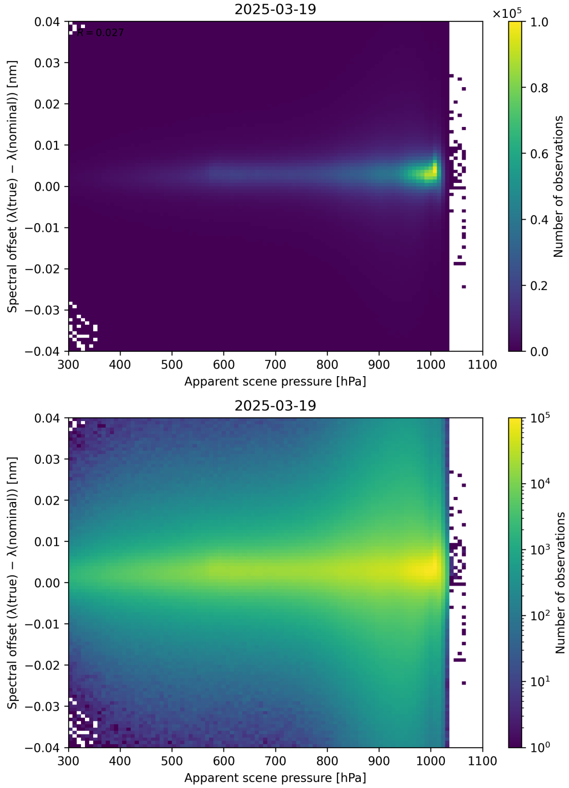
Figure 67: Scatter density plot of “Apparent scene pressure” against “Spectral offset ( \lambda_{\text{true}} - \lambda_{\text{nominal}} )” for 2025-03-18 to 2025-03-20.
