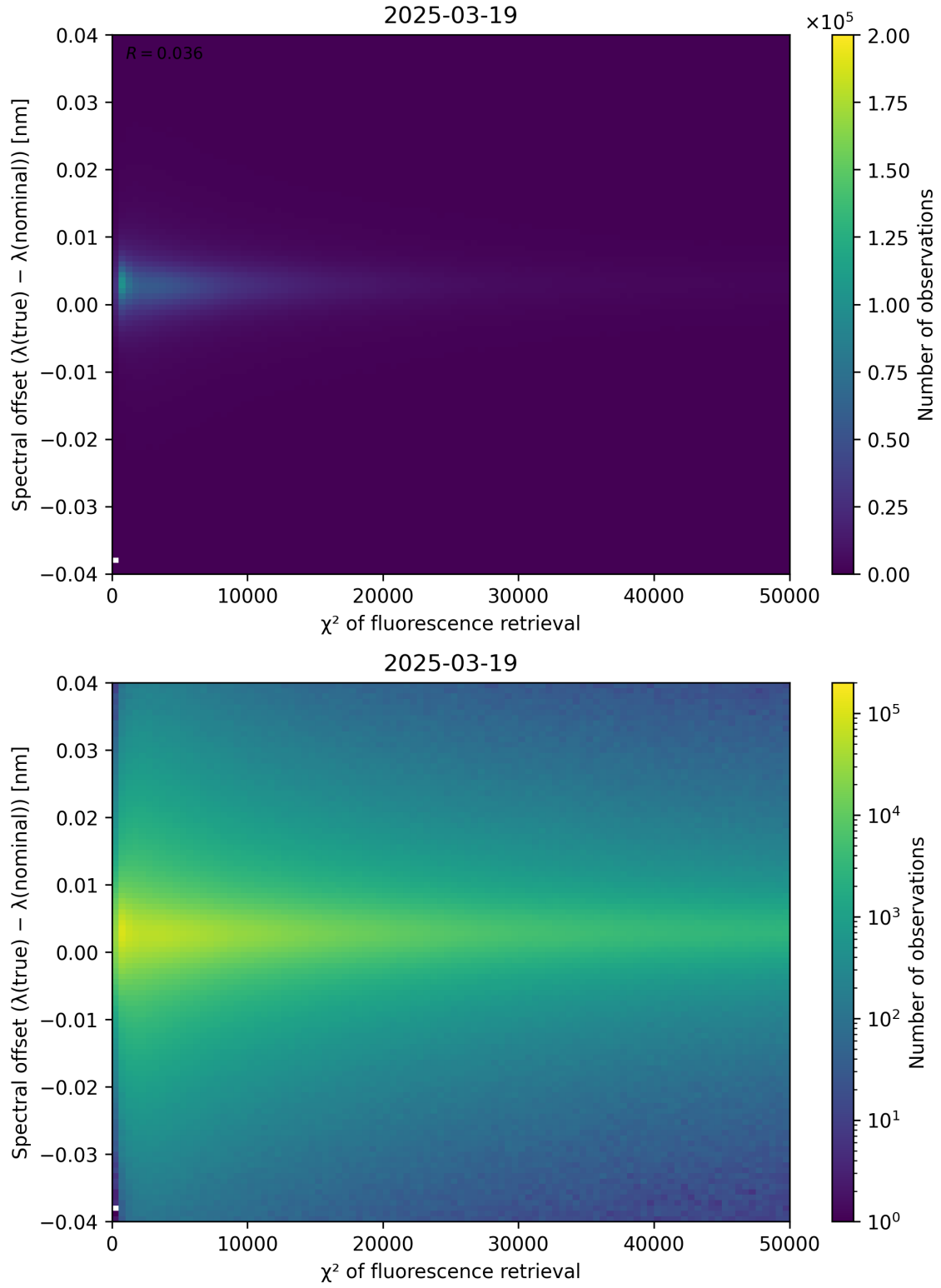
Figure 69: Scatter density plot of “ \chi^2 of fluorescence retrieval” against “Spectral offset ( \lambda_{\text{true}} - \lambda_{\text{nominal}} )” for 2025-03-18 to 2025-03-20.
