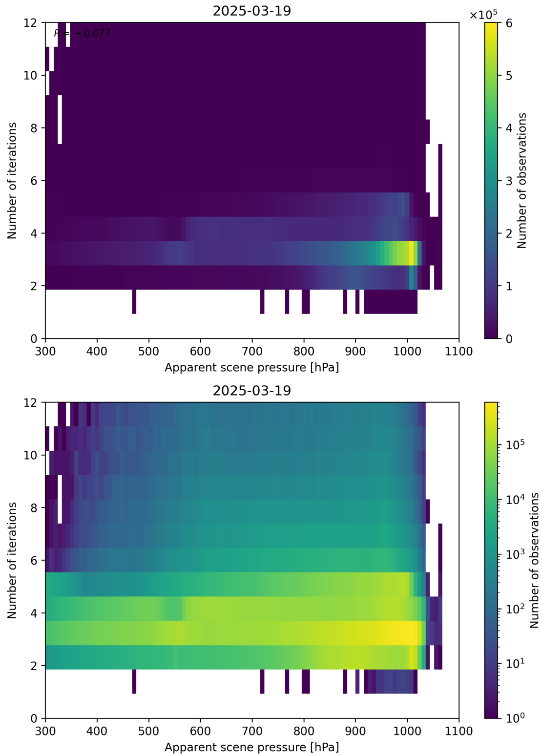
Figure 65: Scatter density plot of “Apparent scene pressure” against “Number of iterations” for 2025-03-18 to 2025-03-20.
