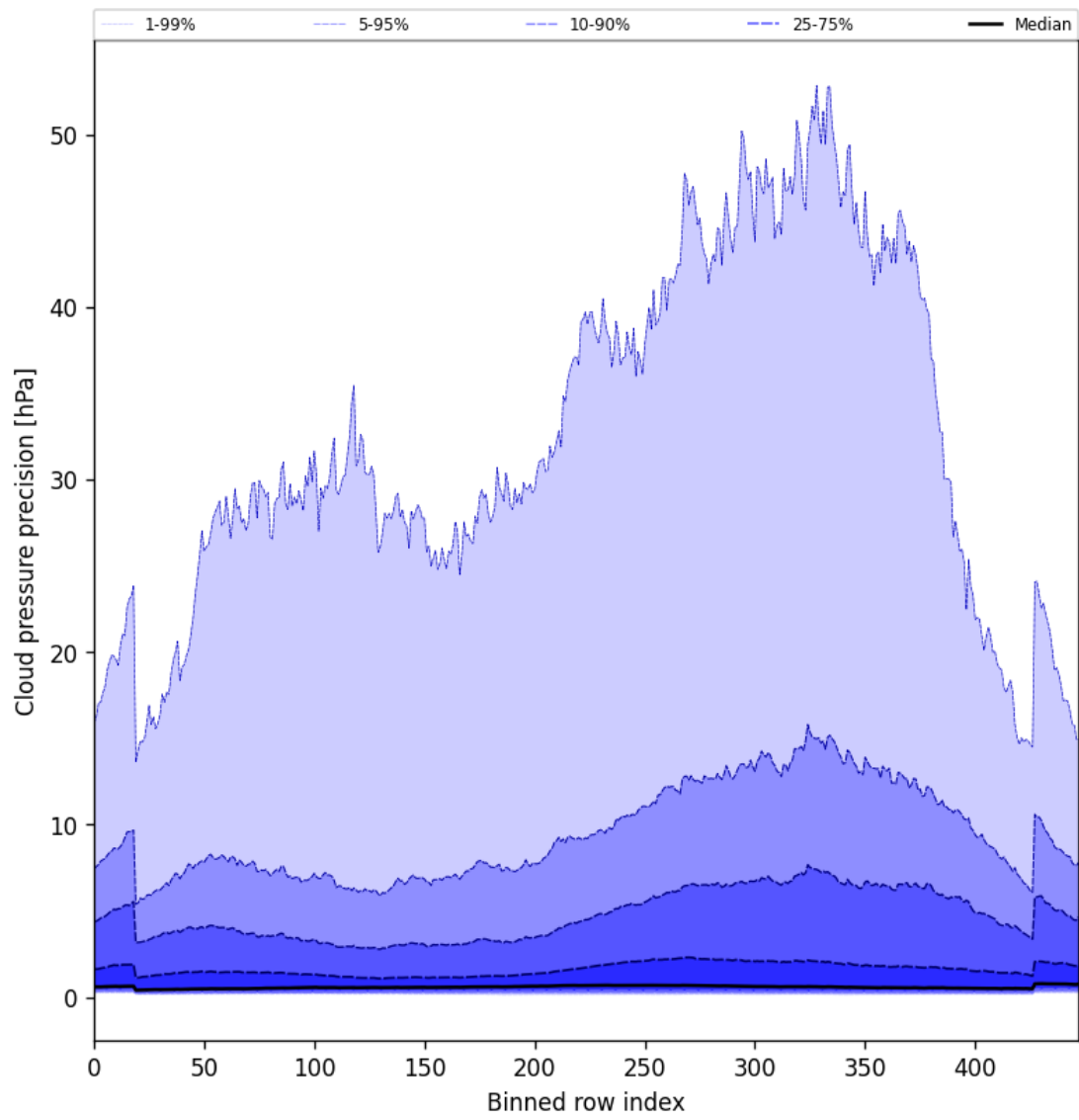
Figure 48: Along track statistics of “Cloud pressure precision” for 2025-03-18 to 2025-03-20
