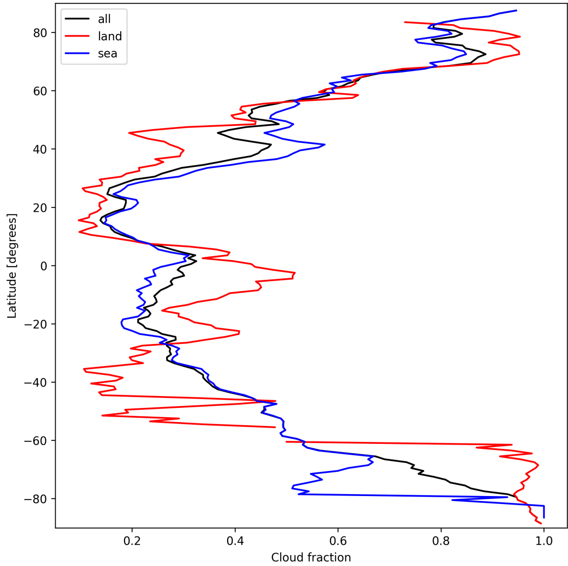
Figure 15: Zonal average of “Cloud fraction” for 2025-03-18 to 2025-03-20.
