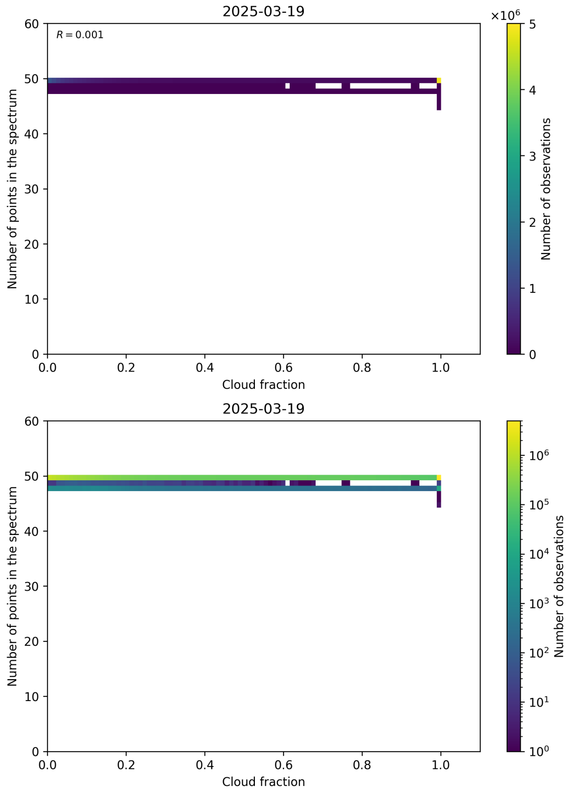
Figure 74: Scatter density plot of “Cloud fraction” against “Number of points in the spectrum” for 2025-03-18 to 2025-03-20.
