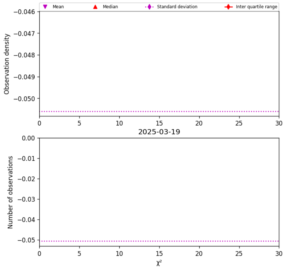
Figure 38: Histogram of “ \chi^2 ” for 2025-03-18 to 2025-03-20
