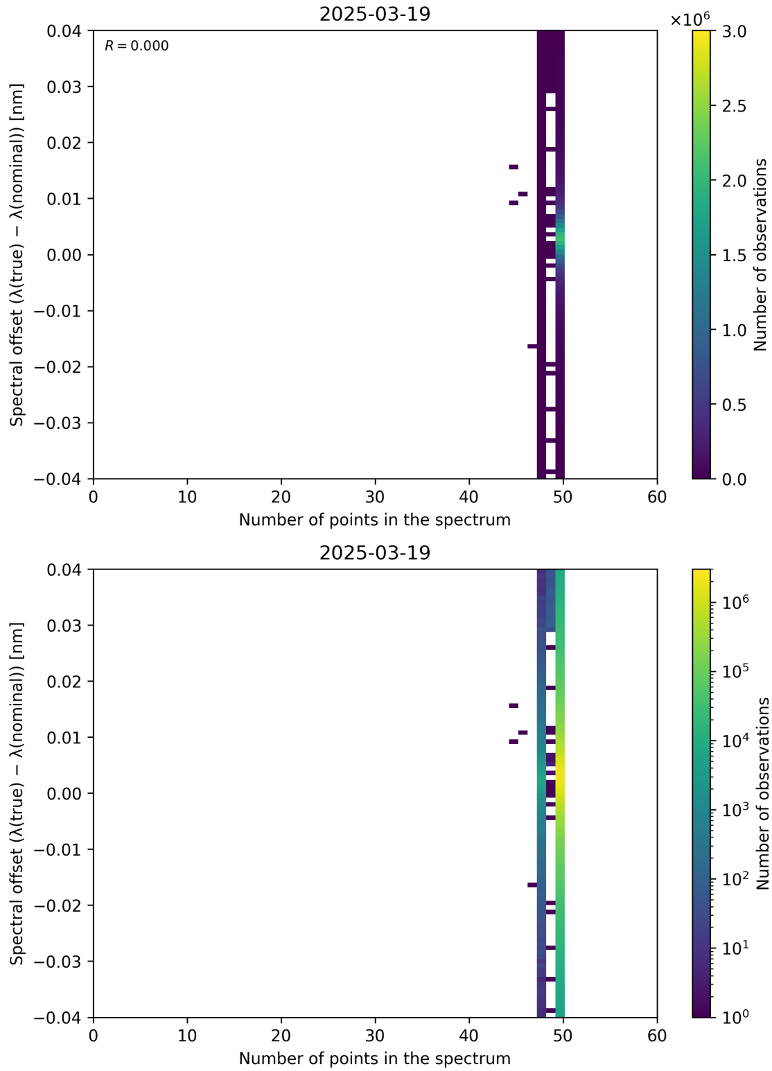
Figure 101: Scatter density plot of “Number of points in the spectrum” against “Spectral offset ( \lambda_{\text{true}} - \lambda_{\text{nominal}} )” for 2025-03-18 to 2025-03-20.
