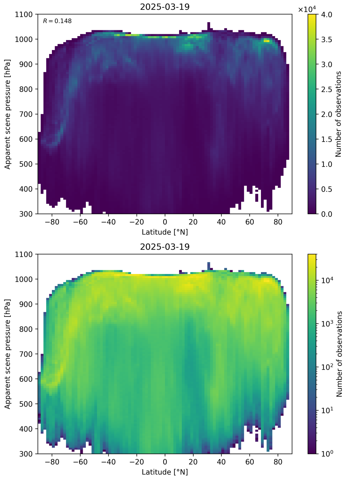
Figure 88: Scatter density plot of “Latitude” against “Apparent scene pressure” for 2025-03-18 to 2025-03-20.
