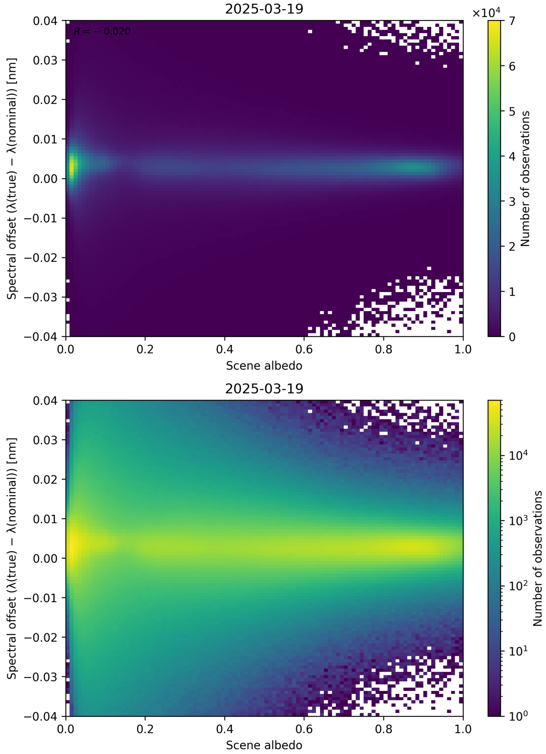
Figure 107: Scatter density plot of “Scene albedo” against “Spectral offset ( \lambda_{\text{true}} - \lambda_{\text{nominal}} )” for 2025-03-18 to 2025-03-20.
