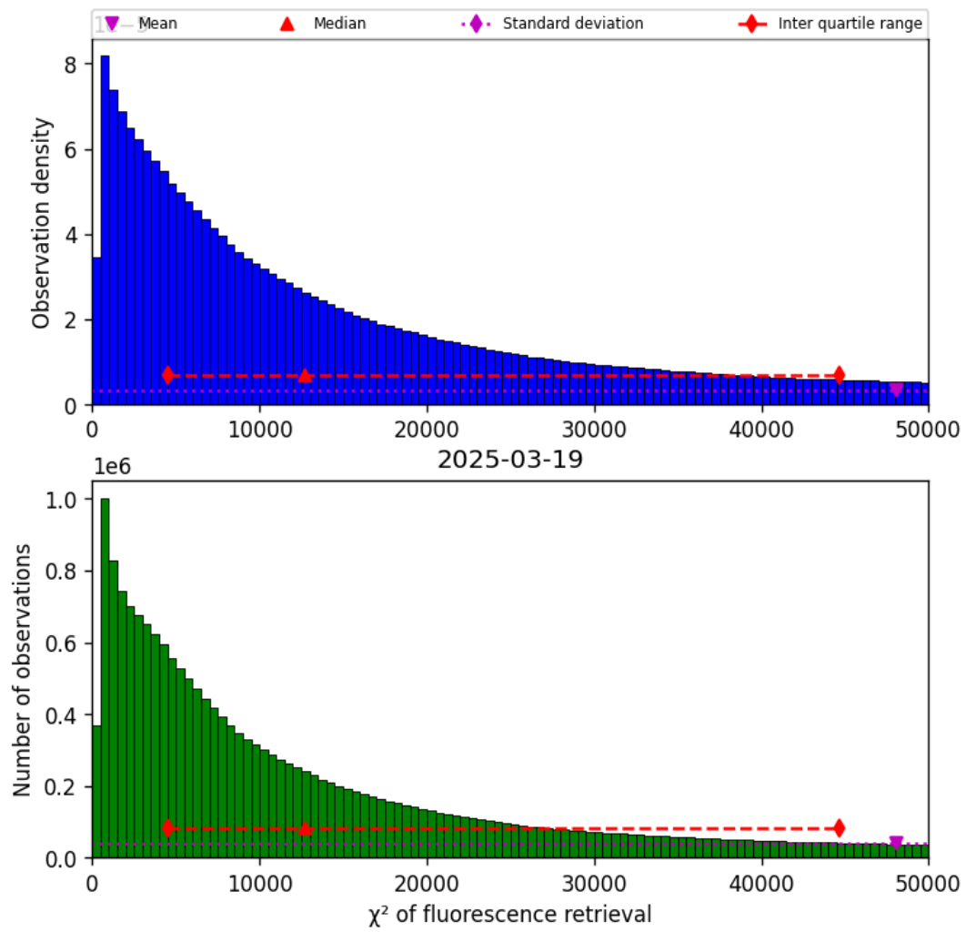
Figure 42: Histogram of “ \chi^2 of fluorescence retrieval” for 2025-03-18 to 2025-03-20
