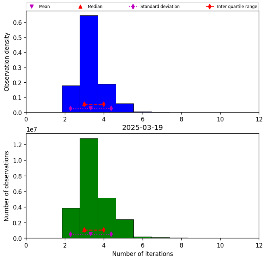
Figure 39: Histogram of “Number of iterations” for 2025-03-18 to 2025-03-20
