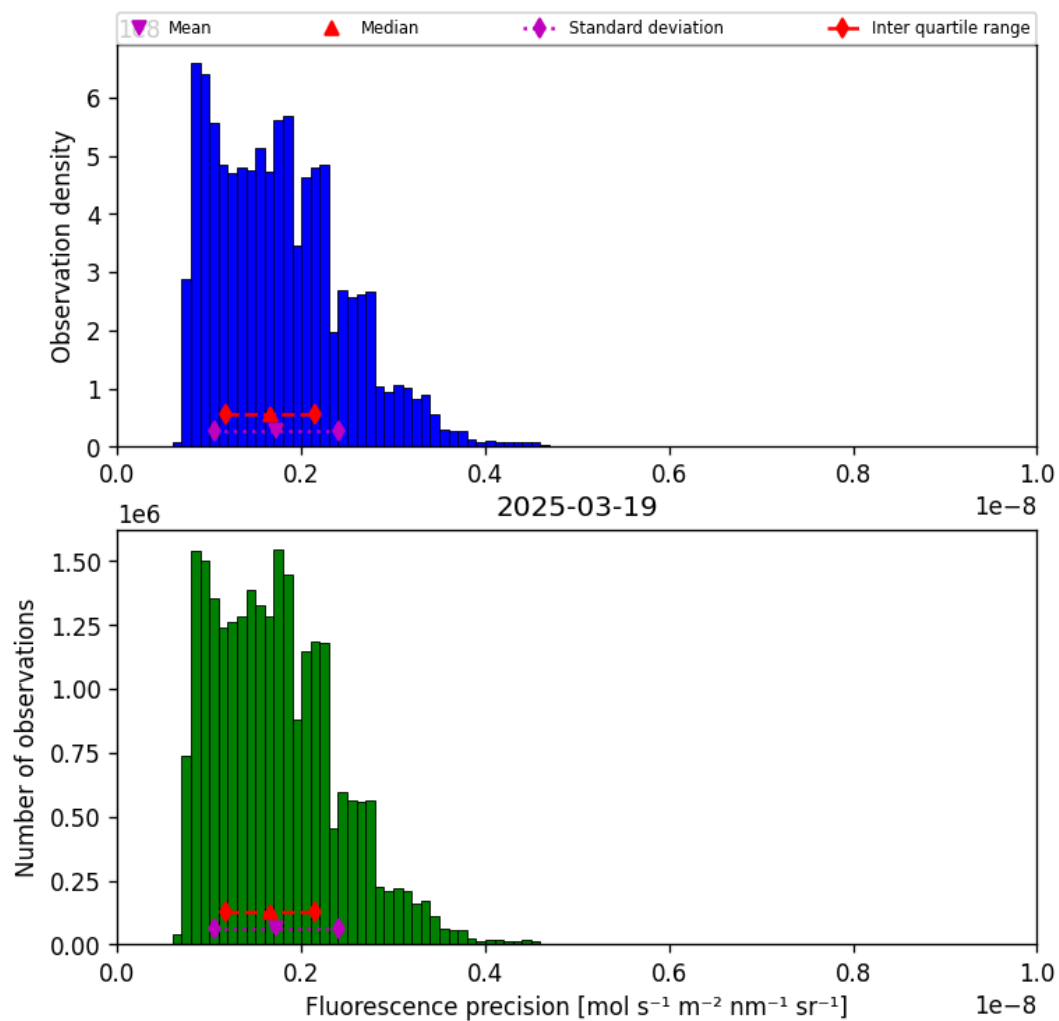
Figure 41: Histogram of “Fluorescence precision” for 2025-03-18 to 2025-03-20
