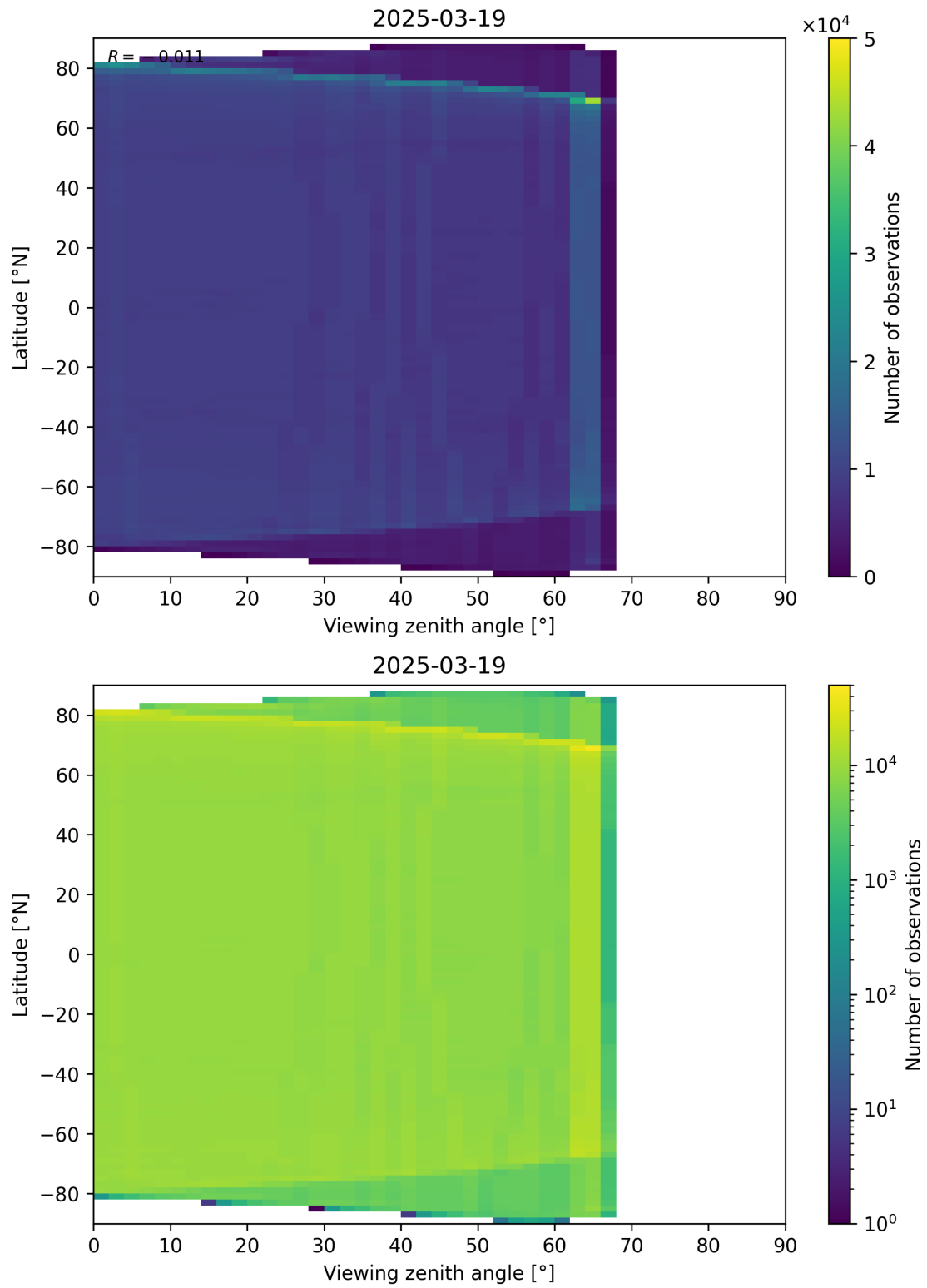
Figure 123: Scatter density plot of “Viewing zenith angle” against “Latitude” for 2025-03-18 to 2025-03-20.
