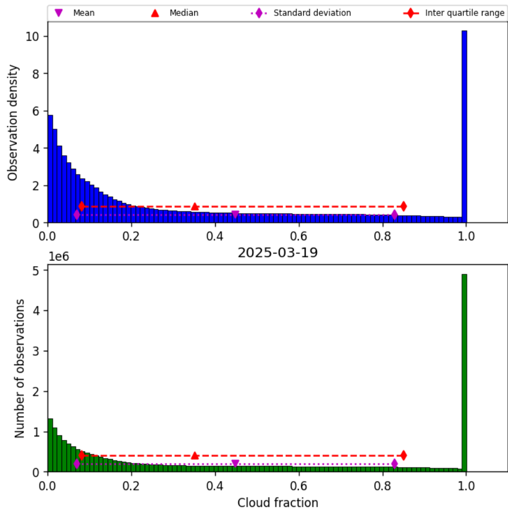
Figure 32: Histogram of “Cloud fraction” for 2025-03-18 to 2025-03-20
