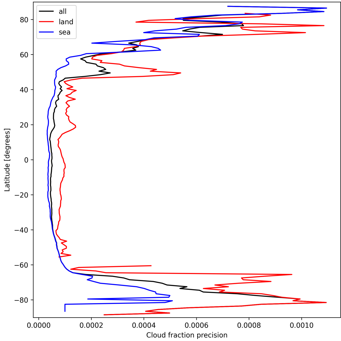
Figure 16: Zonal average of “Cloud fraction precision” for 2025-03-18 to 2025-03-20.
