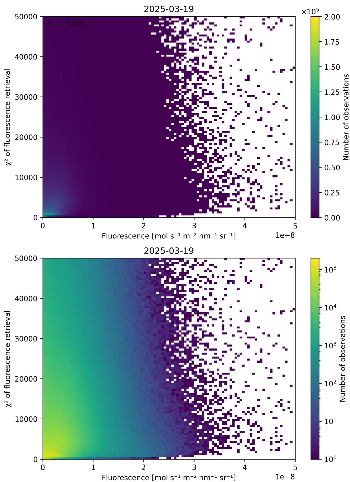
Figure 85: Scatter density plot of “Fluorescence” against “ \chi^2 of fluorescence retrieval” for 2025-03-18 to 2025-03-20.
