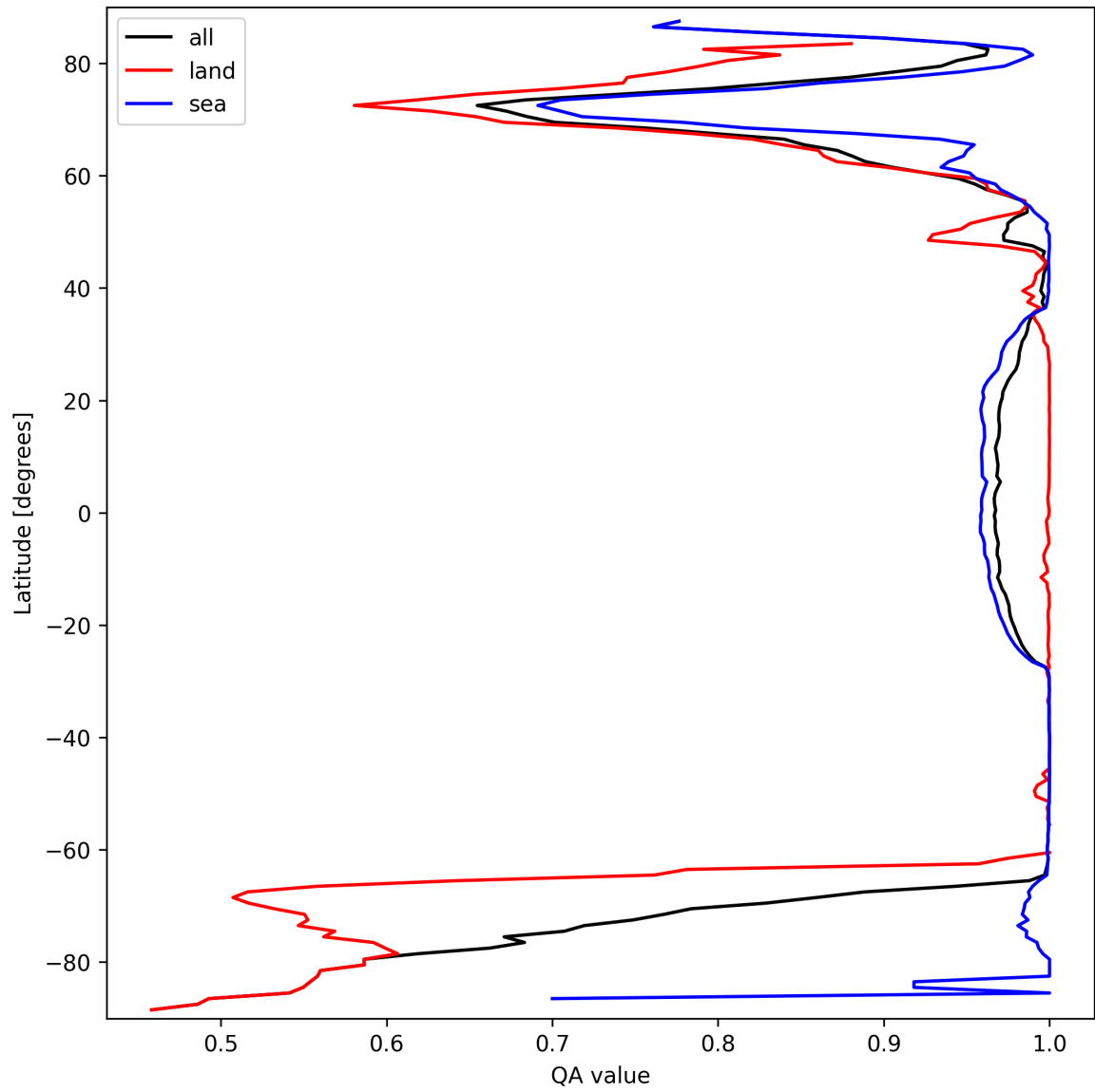
Figure 12: Zonal average of "QA value" for 2025-03-18 to 2025-03-20.
