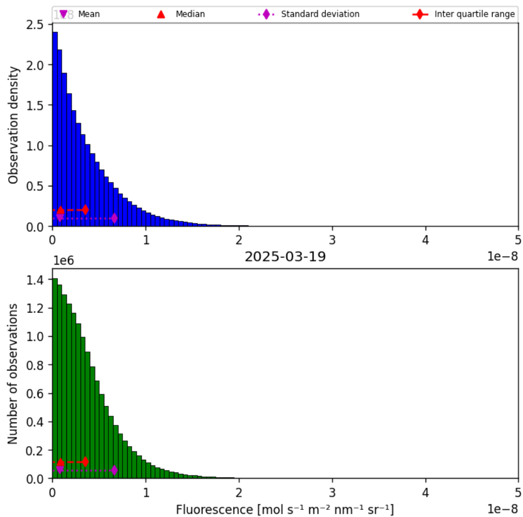
Figure 40: Histogram of “Fluorescence” for 2025-03-18 to 2025-03-20
