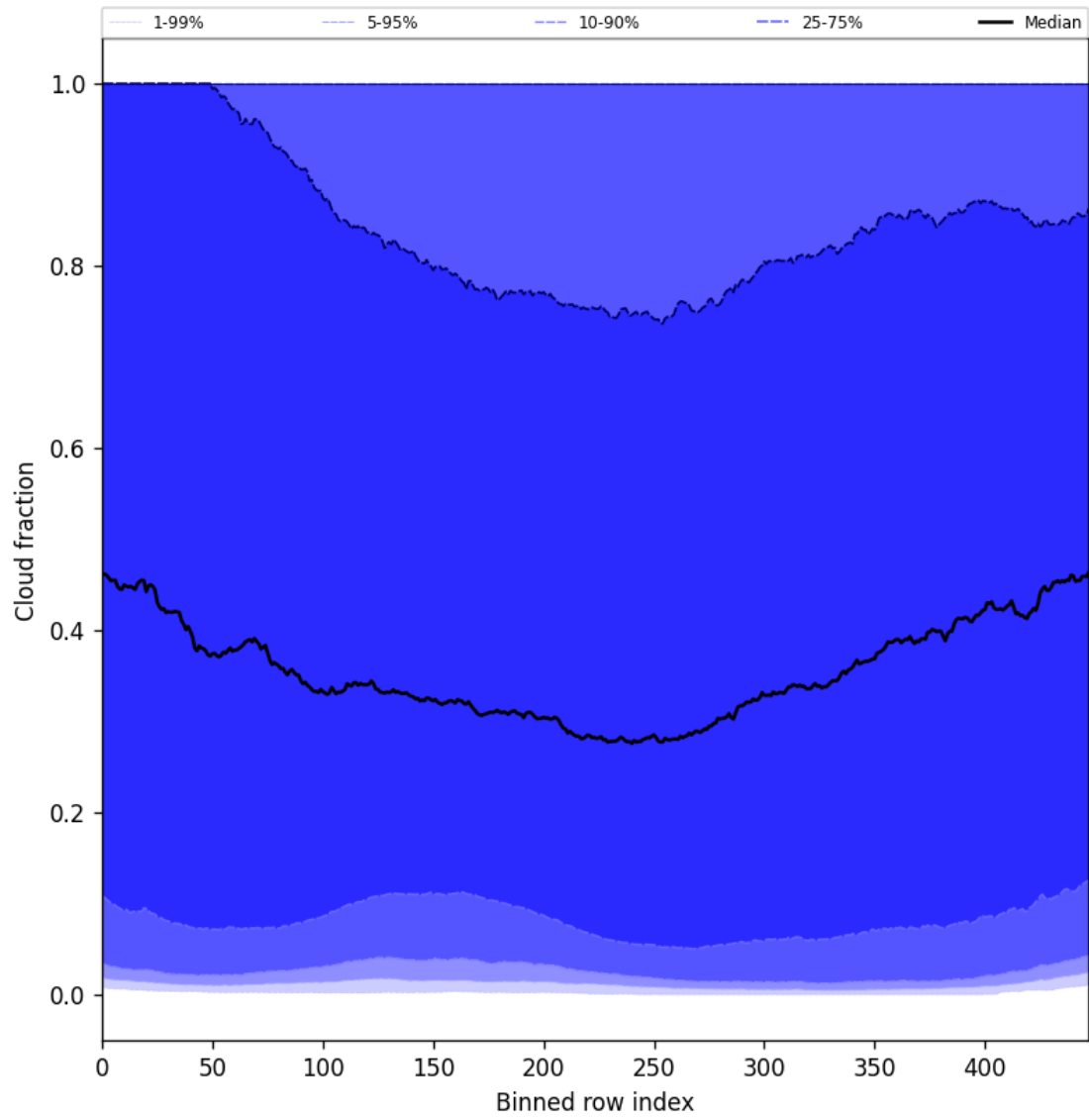
Figure 49: Along track statistics of “Cloud fraction” for 2025-03-18 to 2025-03-20
