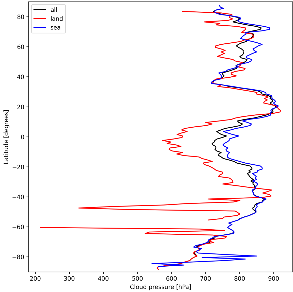
Figure 13: Zonal average of “Cloud pressure” for 2025-03-18 to 2025-03-20.
