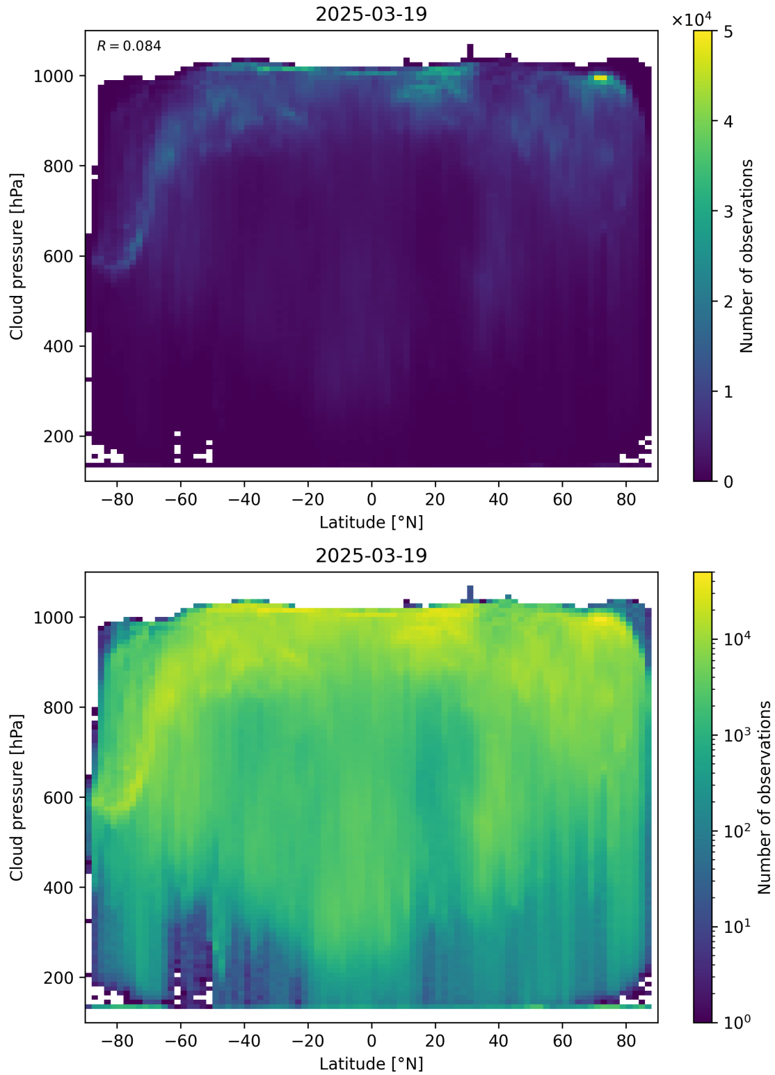
Figure 91: Scatter density plot of “Latitude” against “Cloud pressure” for 2025-03-18 to 2025-03-20.
