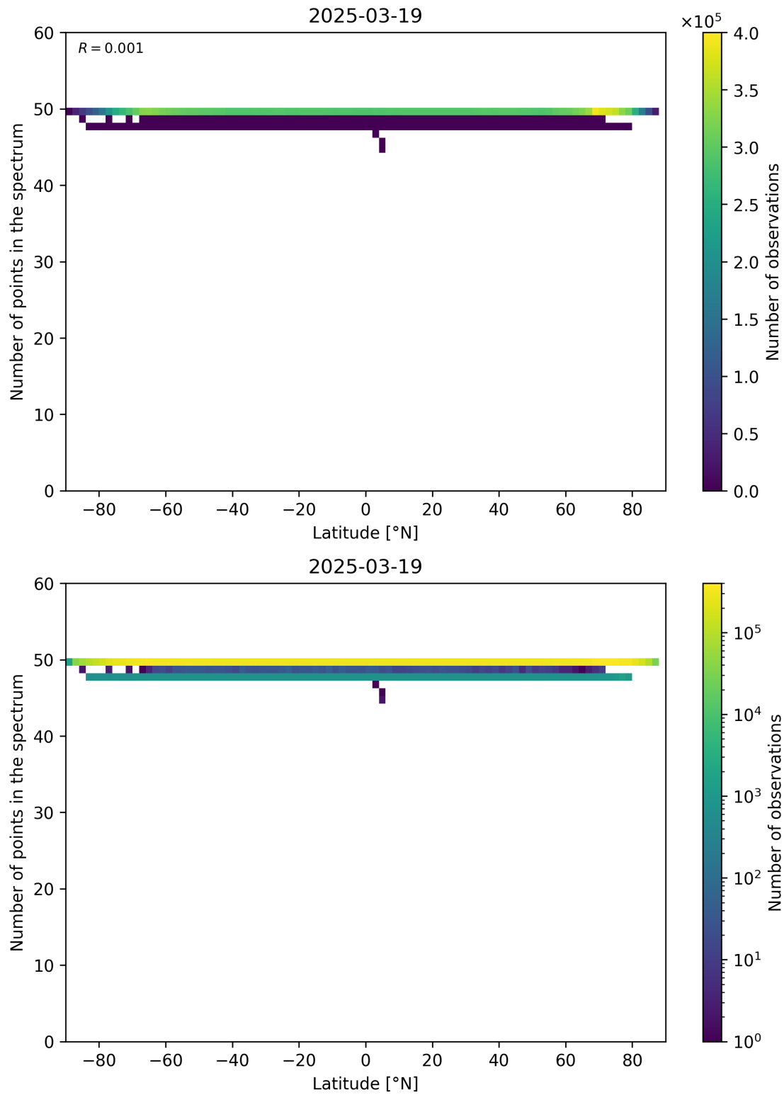
Figure 94: Scatter density plot of “Latitude” against “Number of points in the spectrum” for 2025-03-18 to 2025-03-20.
