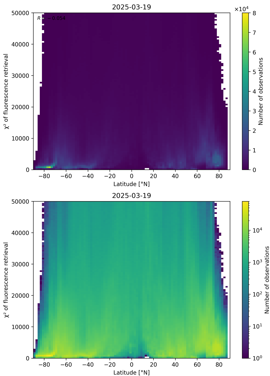
Figure 89: Scatter density plot of “Latitude” against “ \chi^2 of fluorescence retrieval” for 2025-03-18 to 2025-03-20.
