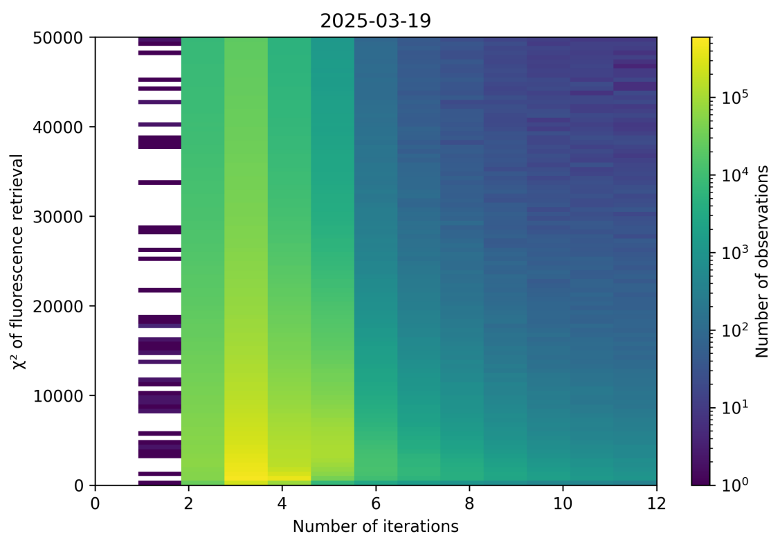
Figure 97: Scatter density plot of “Number of iterations” against “ \chi^2 of fluorescence retrieval” for 2025-03-18 to 2025-03-20.
