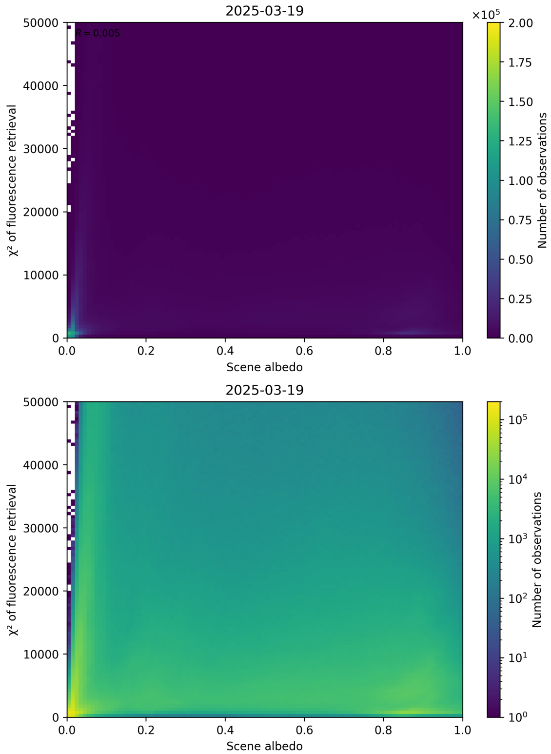
Figure 103: Scatter density plot of “Scene albedo” against “ \chi^2 of fluorescence retrieval” for 2025-03-18 to 2025-03-20.
