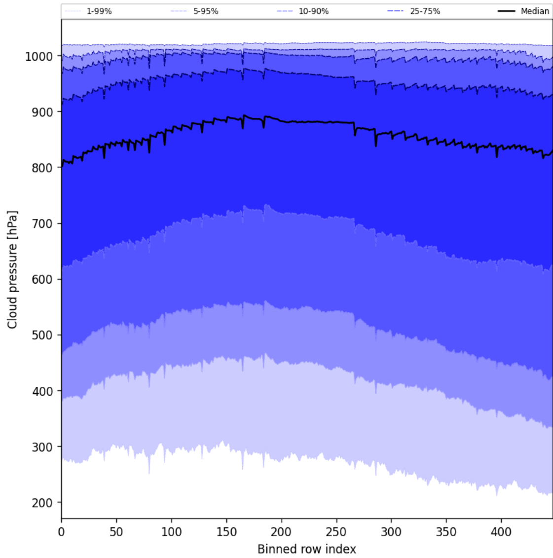
Figure 47: Along track statistics of “Cloud pressure” for 2025-03-18 to 2025-03-20
