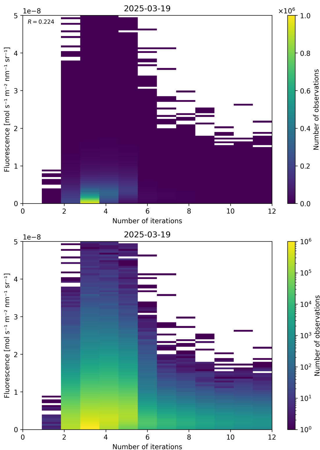
Figure 98: Scatter density plot of “Number of iterations” against “Fluorescence” for 2025-03-18 to 2025-03-20.
