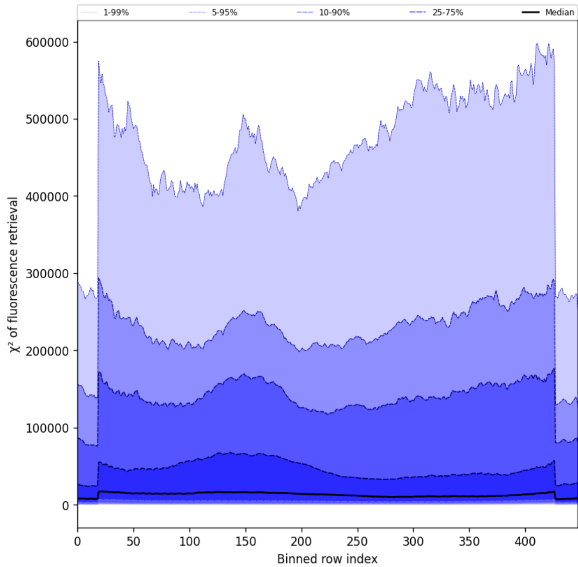
Figure 59: Along track statistics of “ \chi^2 of fluorescence retrieval” for 2025-03-18 to 2025-03-20
