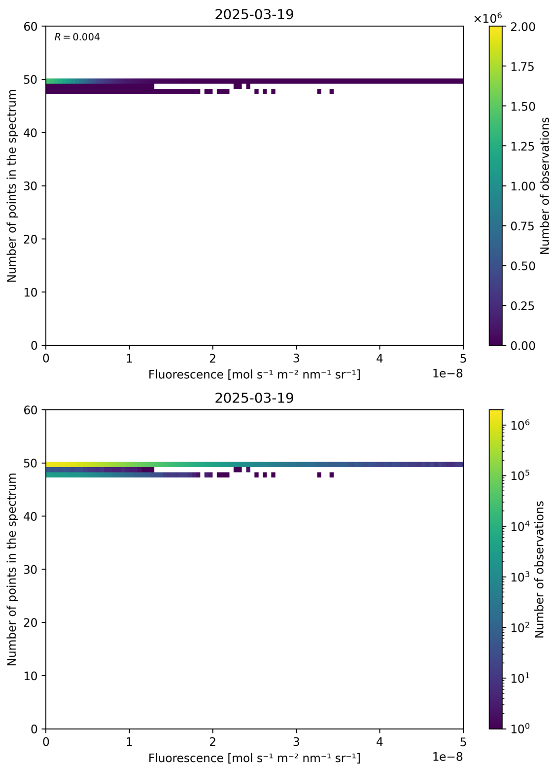
Figure 86: Scatter density plot of “Fluorescence” against “Number of points in the spectrum” for 2025-03-18 to 2025-03-20.
