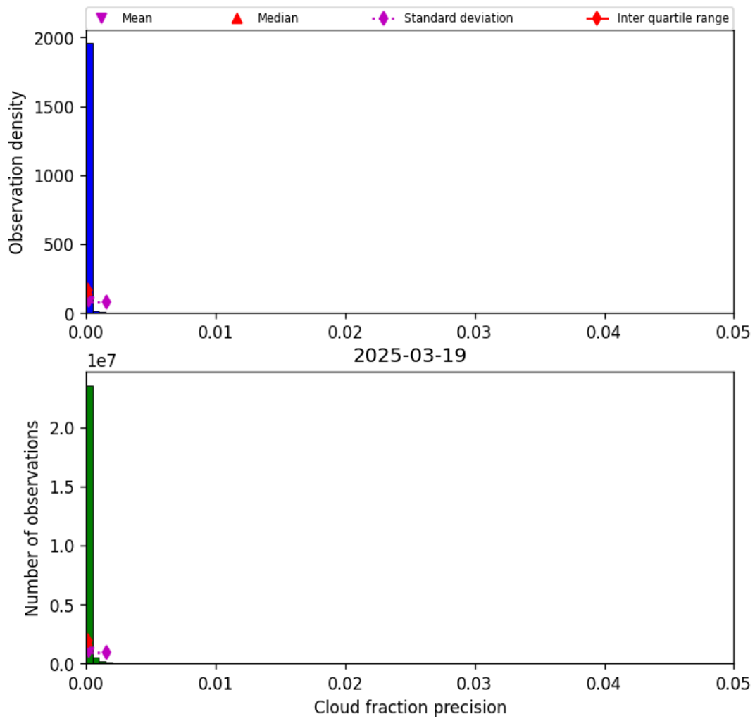
Figure 33: Histogram of “Cloud fraction precision” for 2025-03-18 to 2025-03-20
