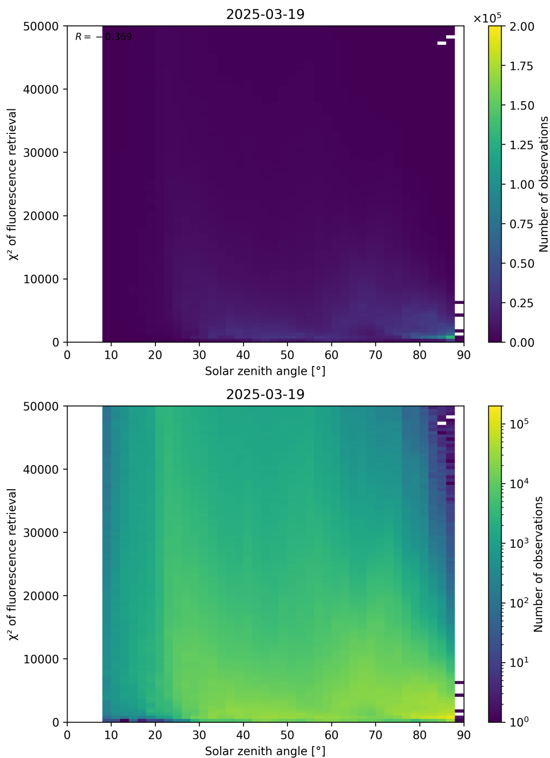
Figure 109: Scatter density plot of “Solar zenith angle” against “ \chi^2 of fluorescence retrieval” for 2025-03-18 to 2025-03-20.
