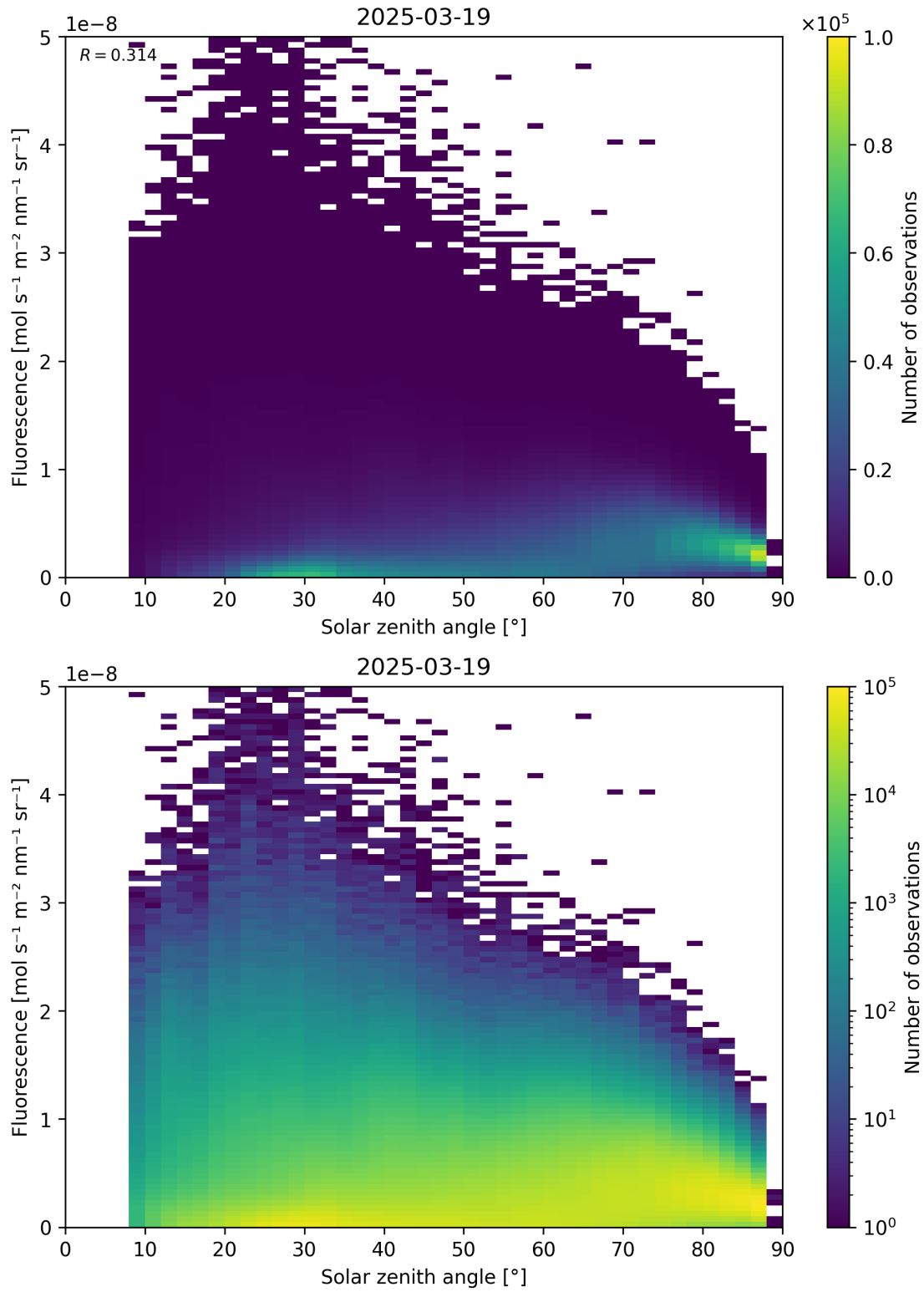
Figure 112: Scatter density plot of “Solar zenith angle” against “Fluorescence” for 2025-03-18 to 2025-03-20.
