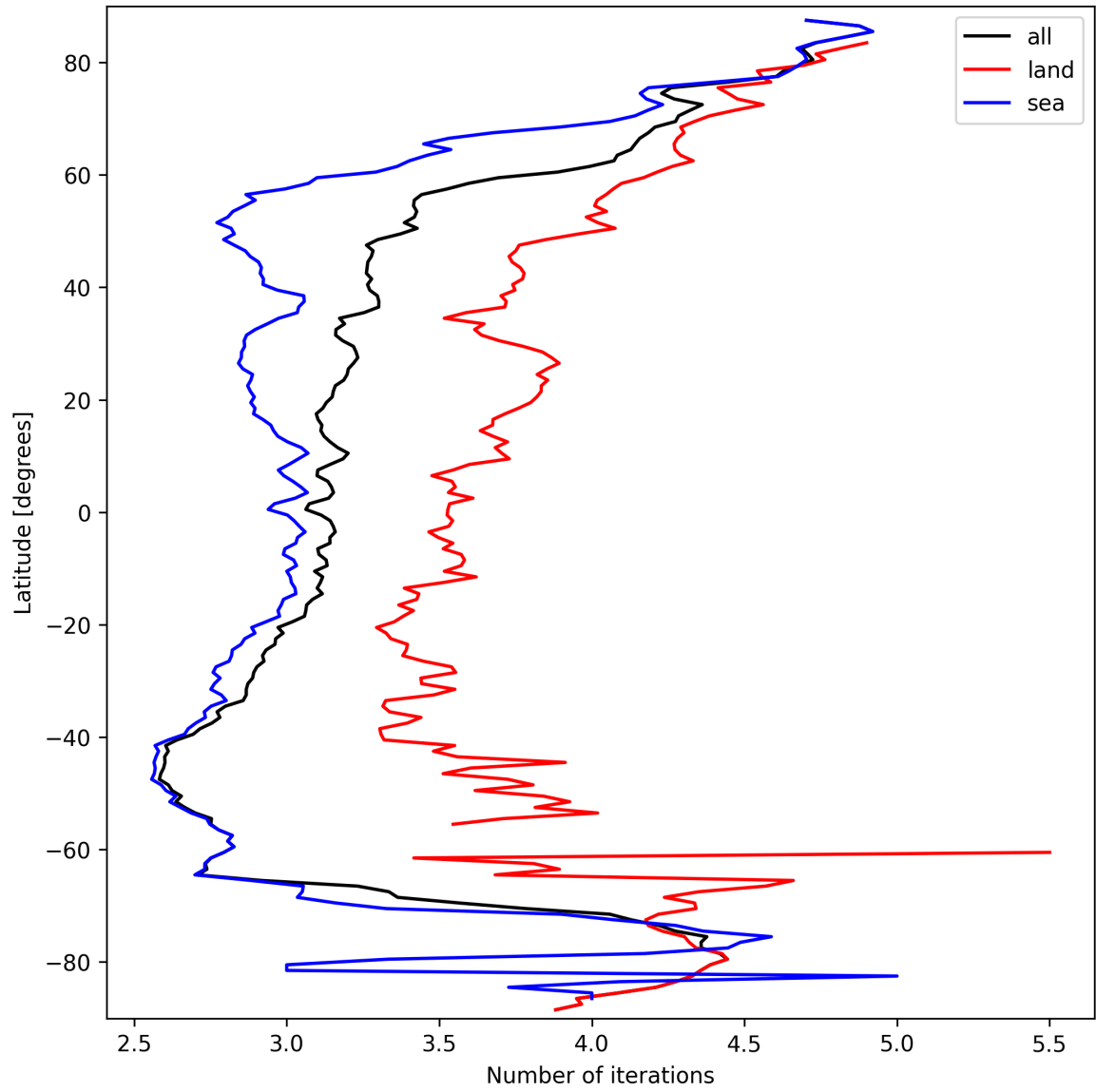
Figure 22: Zonal average of “Number of iterations” for 2025-03-18 to 2025-03-20.
