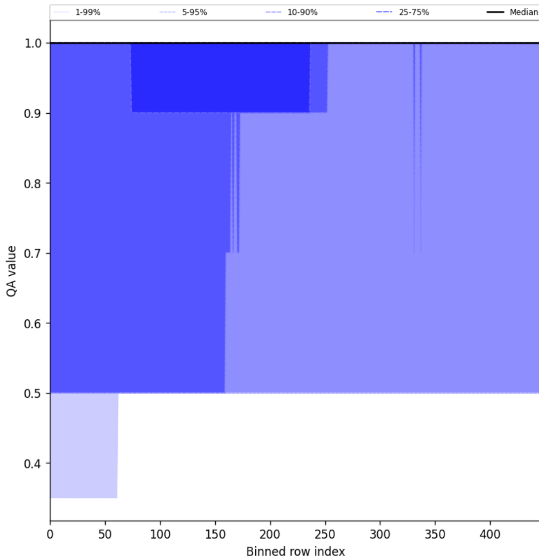
Figure 46: Along track statistics of “QA value” for 2025-03-18 to 2025-03-20
