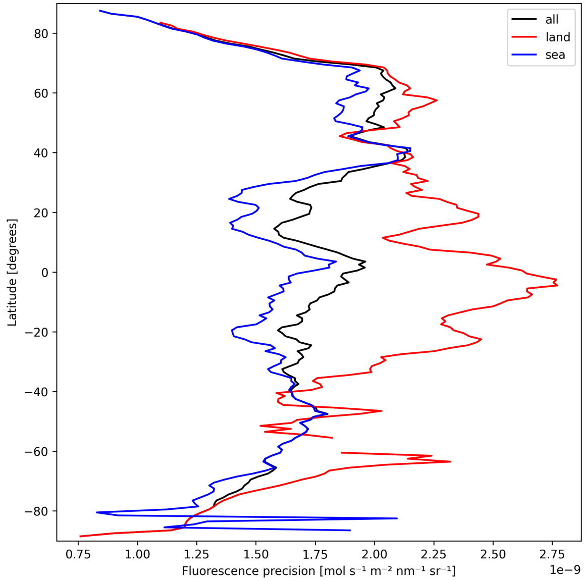
Figure 24: Zonal average of “Fluorescence precision” for 2025-03-18 to 2025-03-20.
