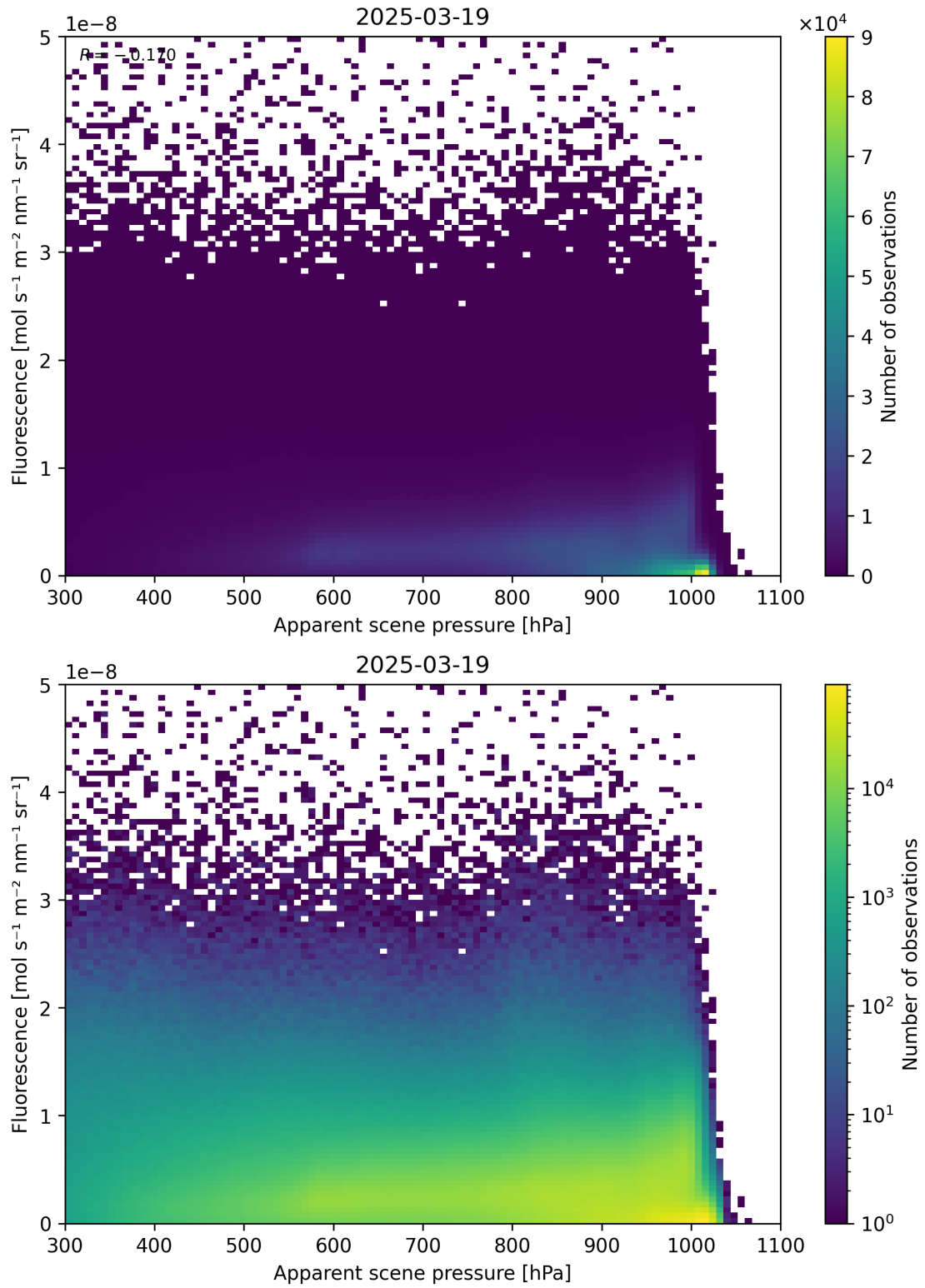
Figure 64: Scatter density plot of “Apparent scene pressure” against “Fluorescence” for 2025-03-18 to 2025-03-20.
