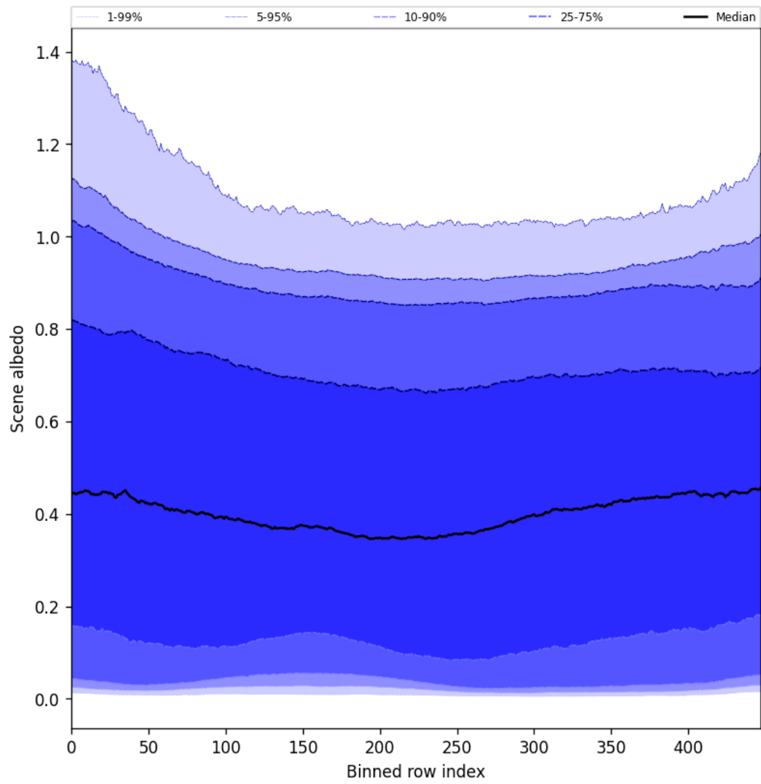
Figure 51: Along track statistics of “Scene albedo” for 2025-03-19 to 2025-03-21
