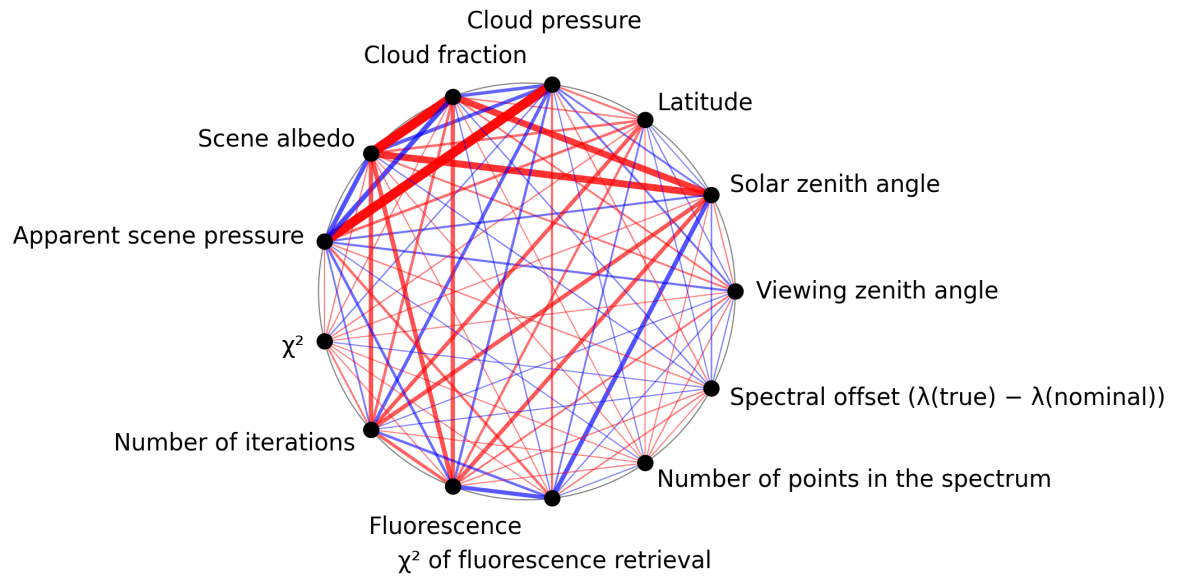
Figure 1: Map of correlation graph for 2025-03-19 to 2025-03-21.
