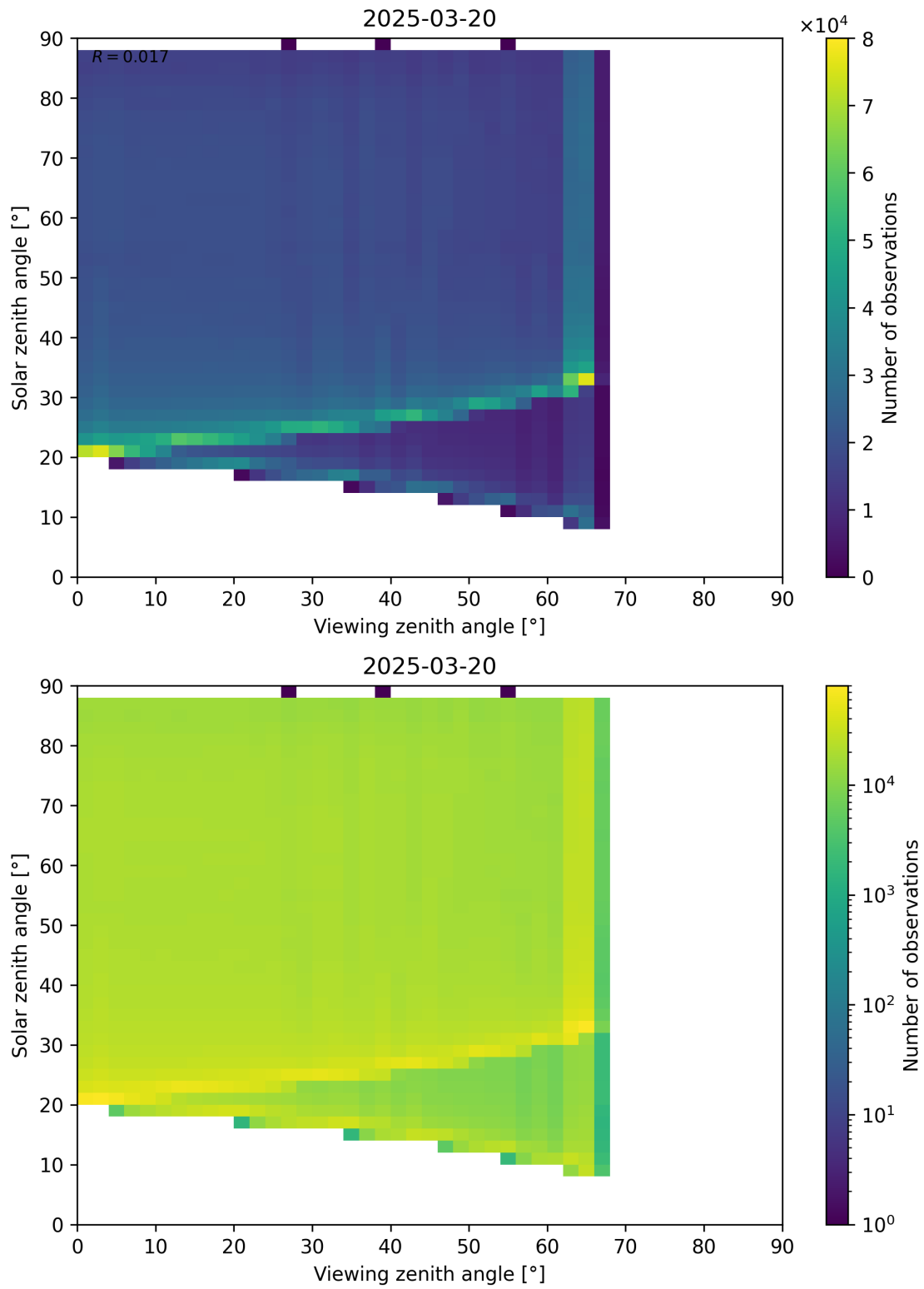
Figure 127: Scatter density plot of “Viewing zenith angle” against “Solar zenith angle” for 2025-03-19 to 2025-03-21.
