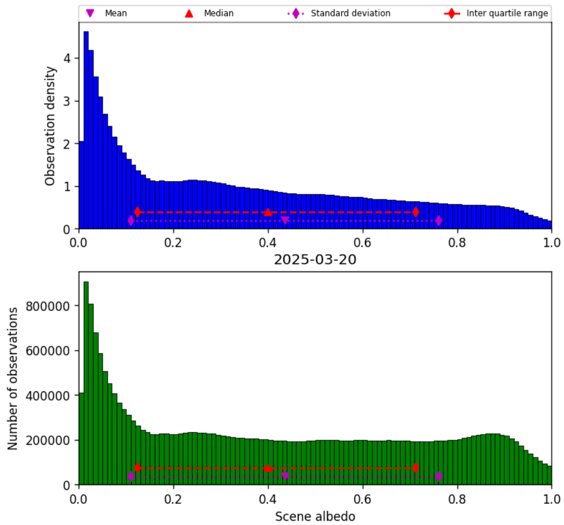
Figure 34: Histogram of “Scene albedo” for 2025-03-19 to 2025-03-21
