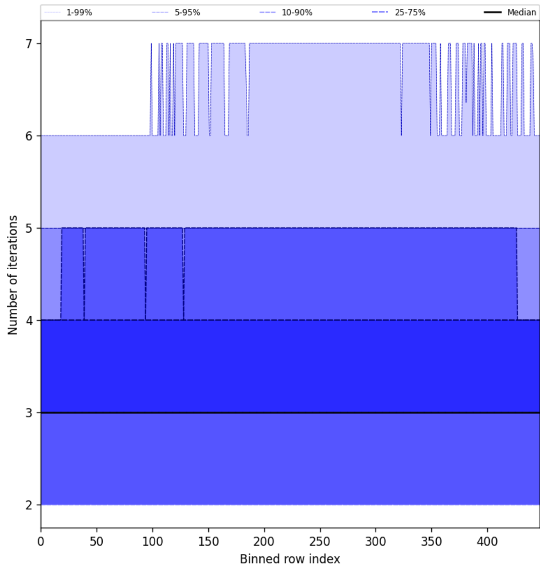
Figure 56: Along track statistics of “Number of iterations” for 2025-03-19 to 2025-03-21
