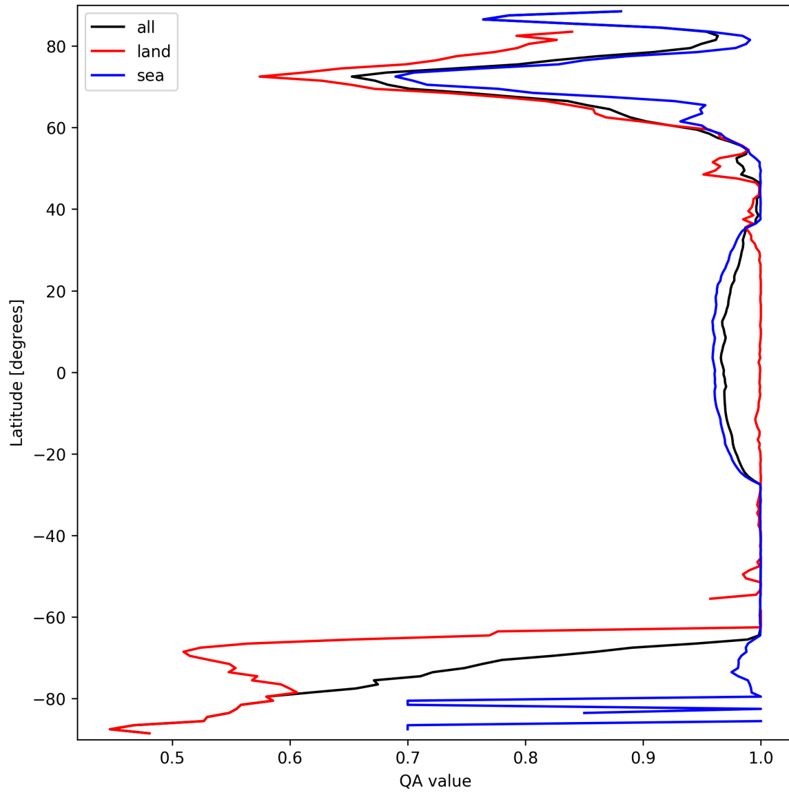
Figure 12: Zonal average of “QA value” for 2025-03-19 to 2025-03-21.
