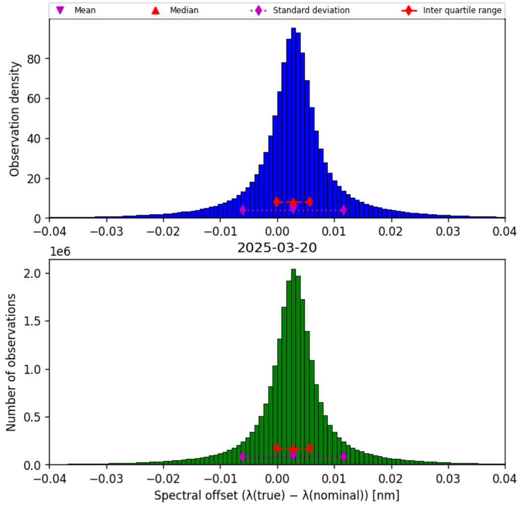
Figure 45: Histogram of “Spectral offset ( \lambda_{\text{true}} - \lambda_{\text{nominal}} )” for 2025-03-19 to 2025-03-21
