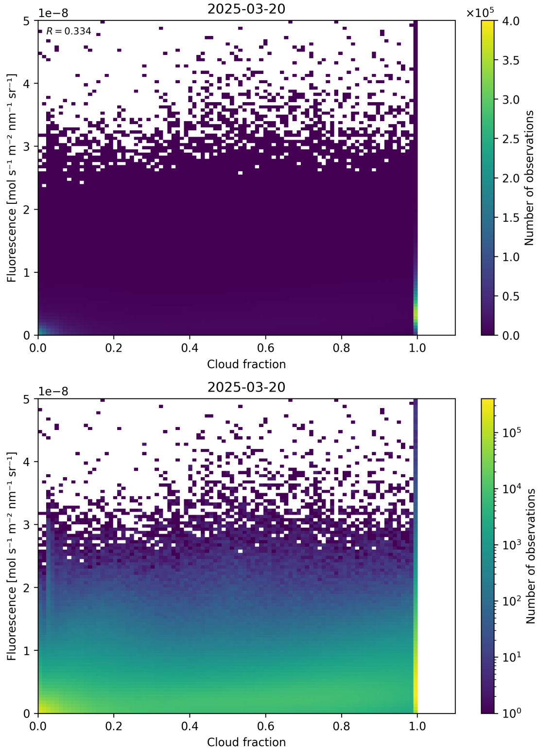
Figure 72: Scatter density plot of “Cloud fraction” against “Fluorescence” for 2025-03-19 to 2025-03-21.
