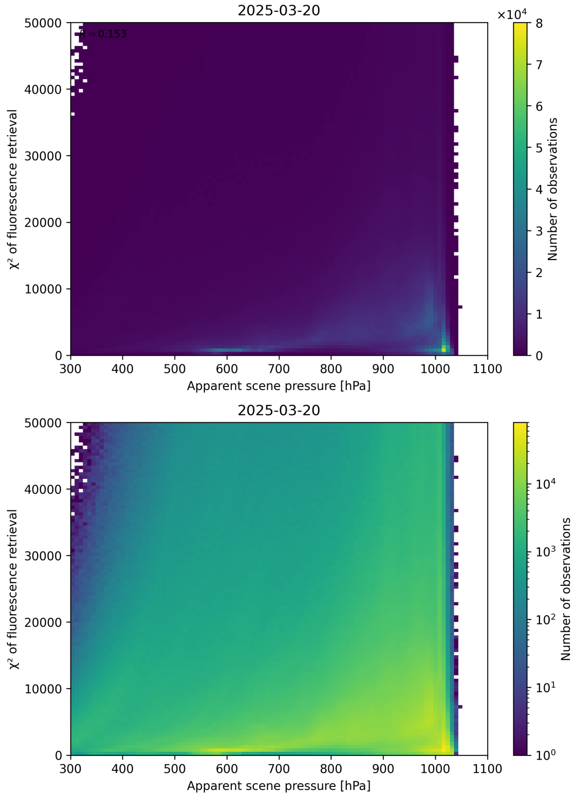
Figure 63: Scatter density plot of “Apparent scene pressure” against “ \chi^2 of fluorescence retrieval” for 2025-03-19 to 2025-03-21.
