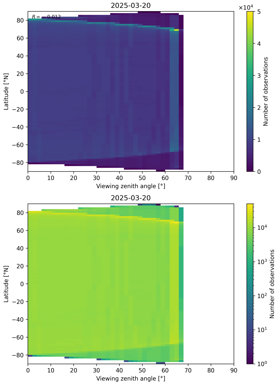
Figure 123: Scatter density plot of “Viewing zenith angle” against “Latitude” for 2025-03-19 to 2025-03-21.
