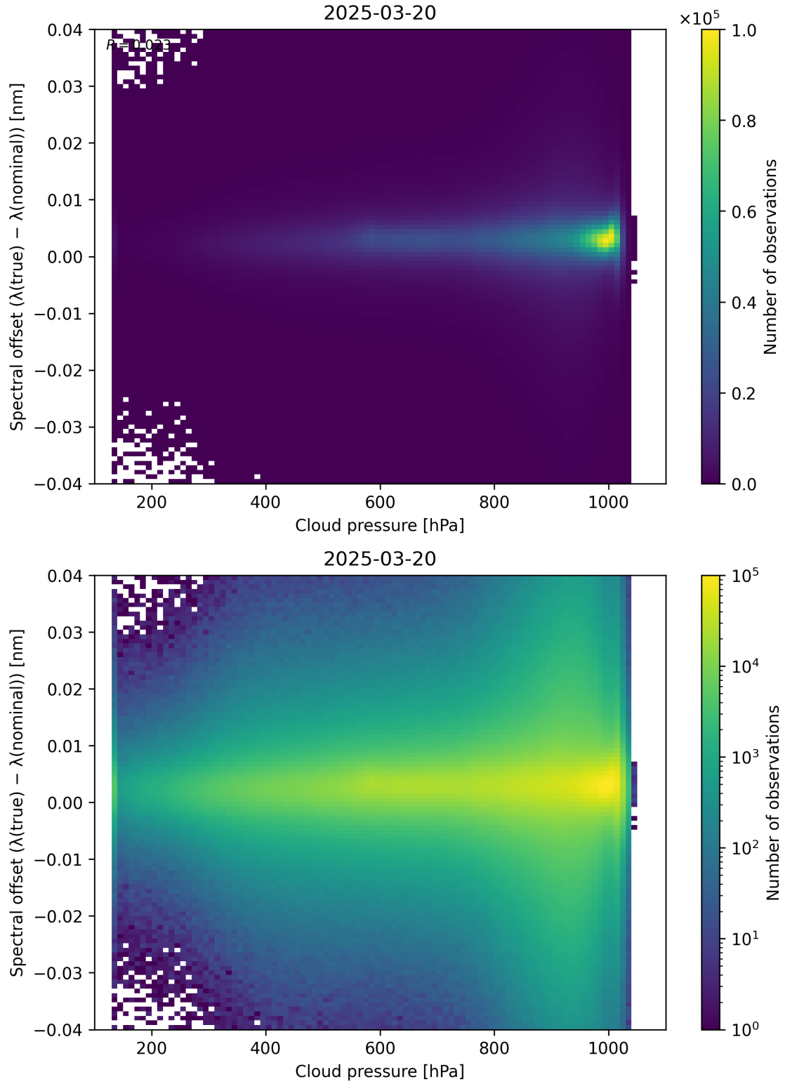
Figure 84: Scatter density plot of “Cloud pressure” against “Spectral offset ( \lambda_{\text{true}} - \lambda_{\text{nominal}} )” for 2025-03-19 to 2025-03-21.
