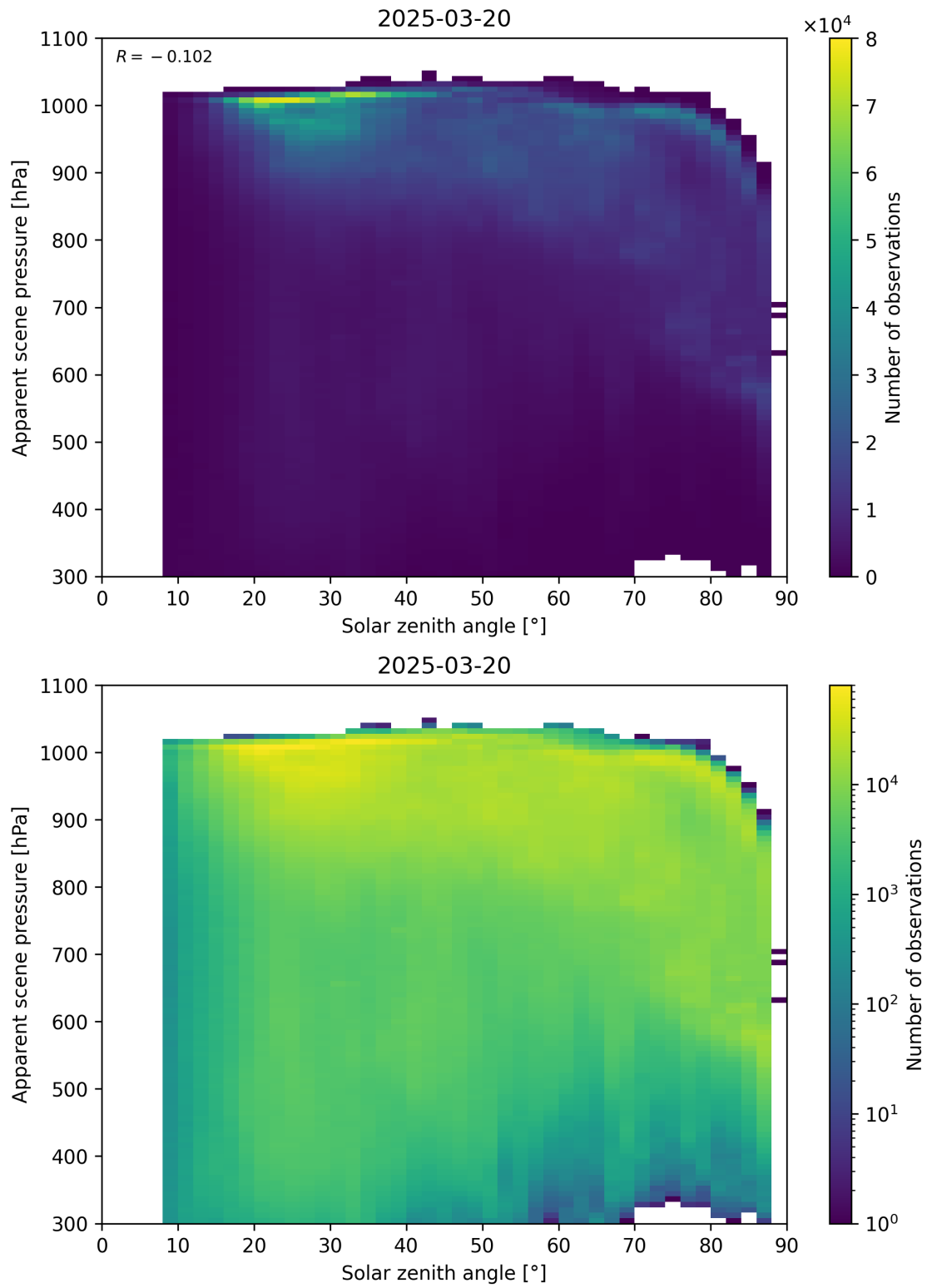
Figure 108: Scatter density plot of “Solar zenith angle” against “Apparent scene pressure” for 2025-03-19 to 2025-03-21.
