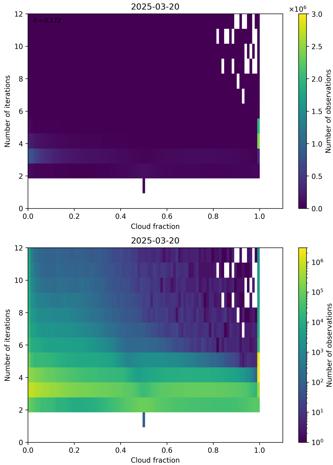
Figure 73: Scatter density plot of “Cloud fraction” against “Number of iterations” for 2025-03-19 to 2025-03-21.
