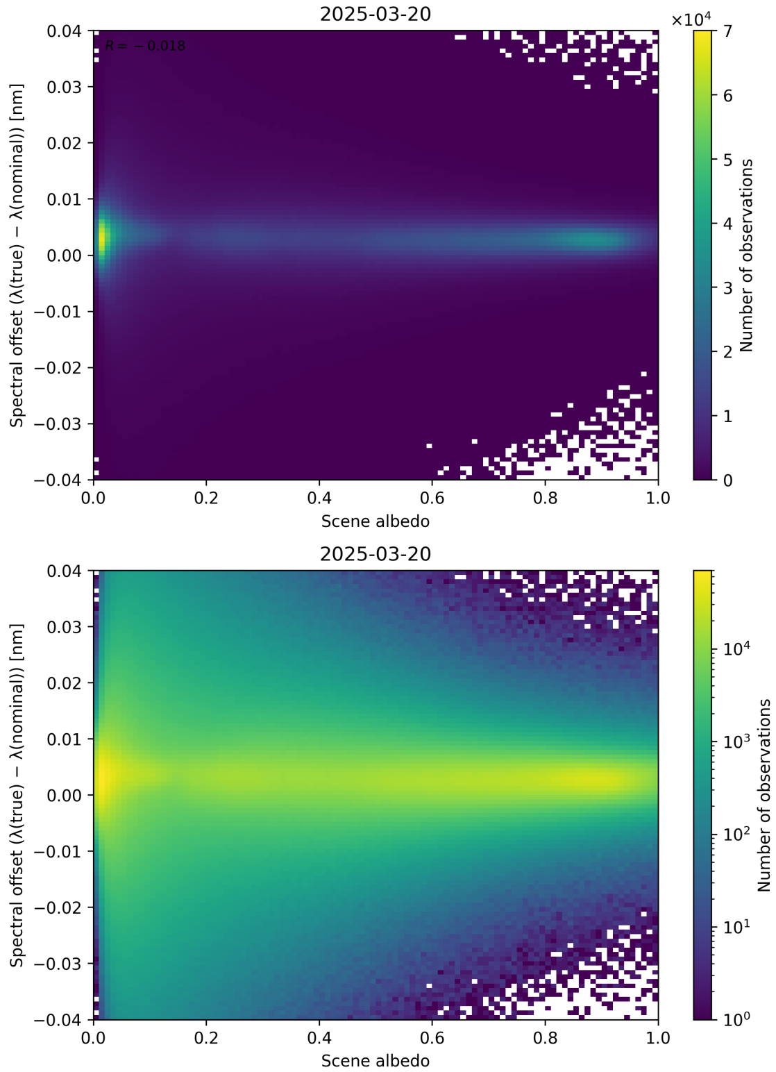
Figure 107: Scatter density plot of “Scene albedo” against “Spectral offset ( \lambda_{\text{true}} - \lambda_{\text{nominal}} )” for 2025-03-19 to 2025-03-21.
