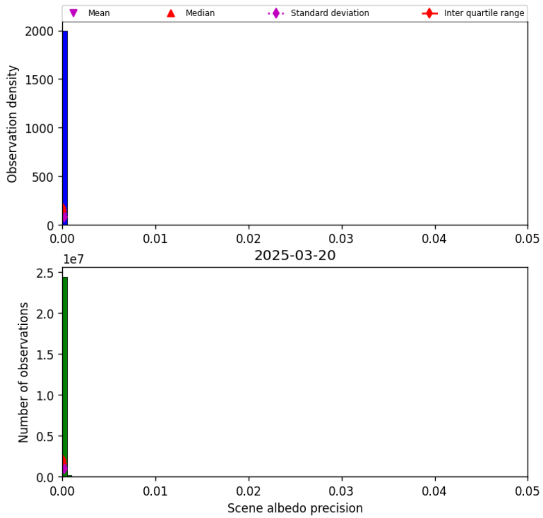
Figure 35: Histogram of “Scene albedo precision” for 2025-03-19 to 2025-03-21
