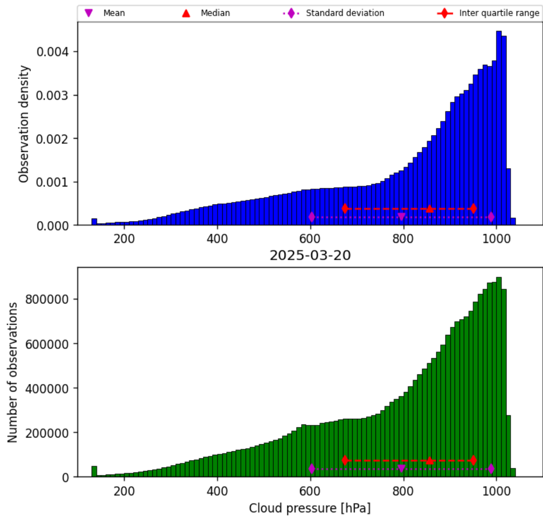
Figure 30: Histogram of “Cloud pressure” for 2025-03-19 to 2025-03-21
