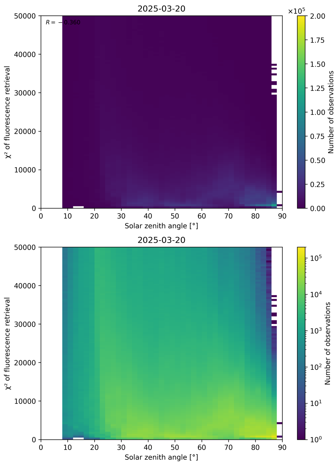
Figure 109: Scatter density plot of “Solar zenith angle” against “ \chi^2 of fluorescence retrieval” for 2025-03-19 to 2025-03-21.
