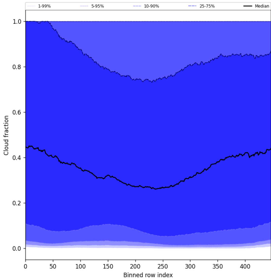
Figure 49: Along track statistics of “Cloud fraction” for 2025-03-19 to 2025-03-21
