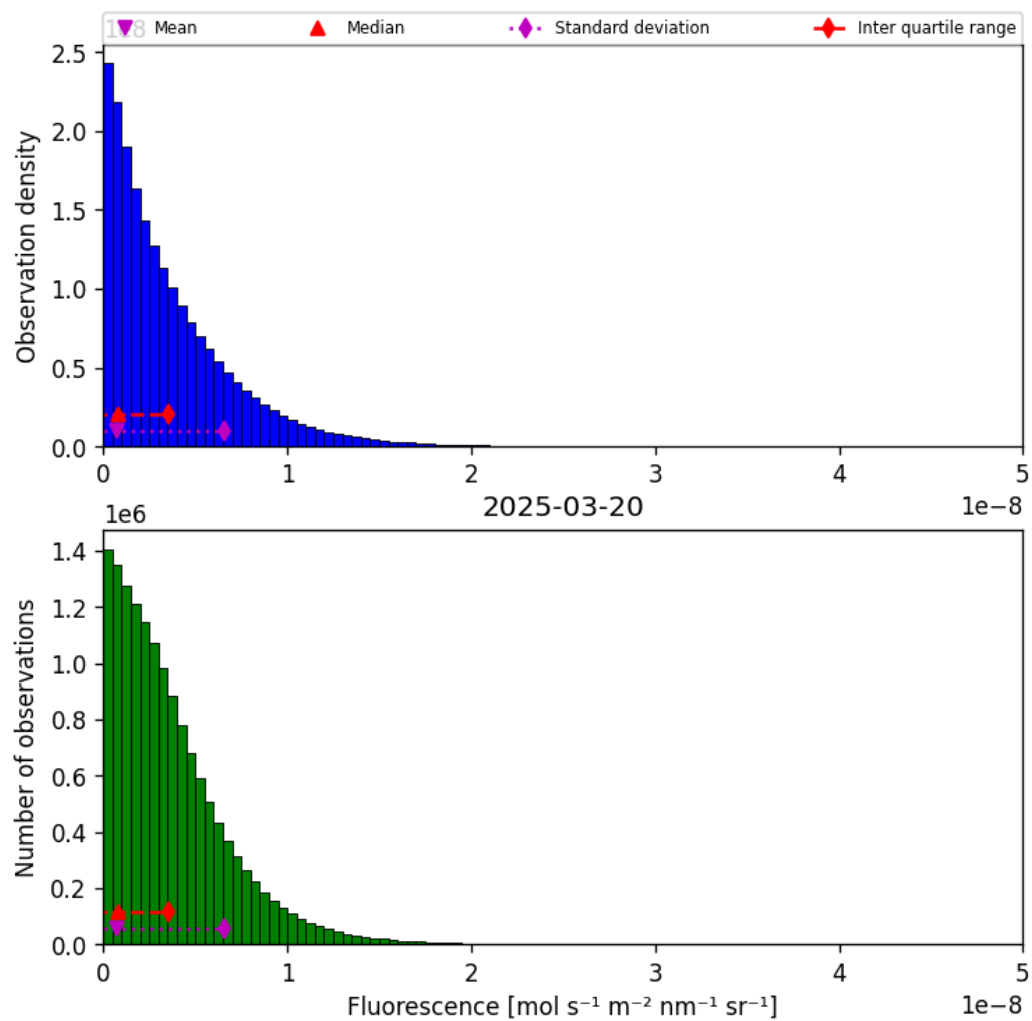
Figure 40: Histogram of “Fluorescence” for 2025-03-19 to 2025-03-21
