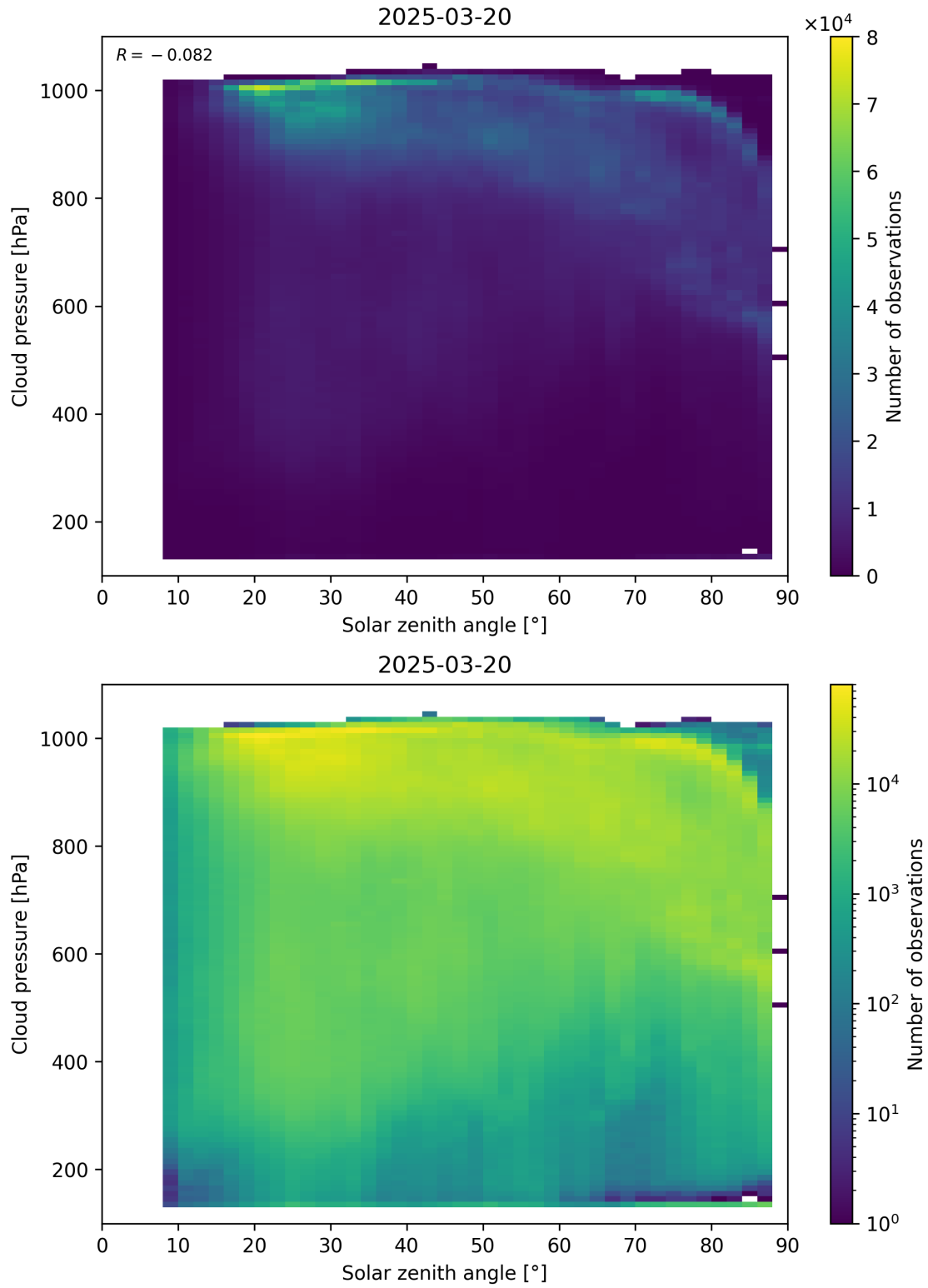
Figure 111: Scatter density plot of “Solar zenith angle” against “Cloud pressure” for 2025-03-19 to 2025-03-21.
