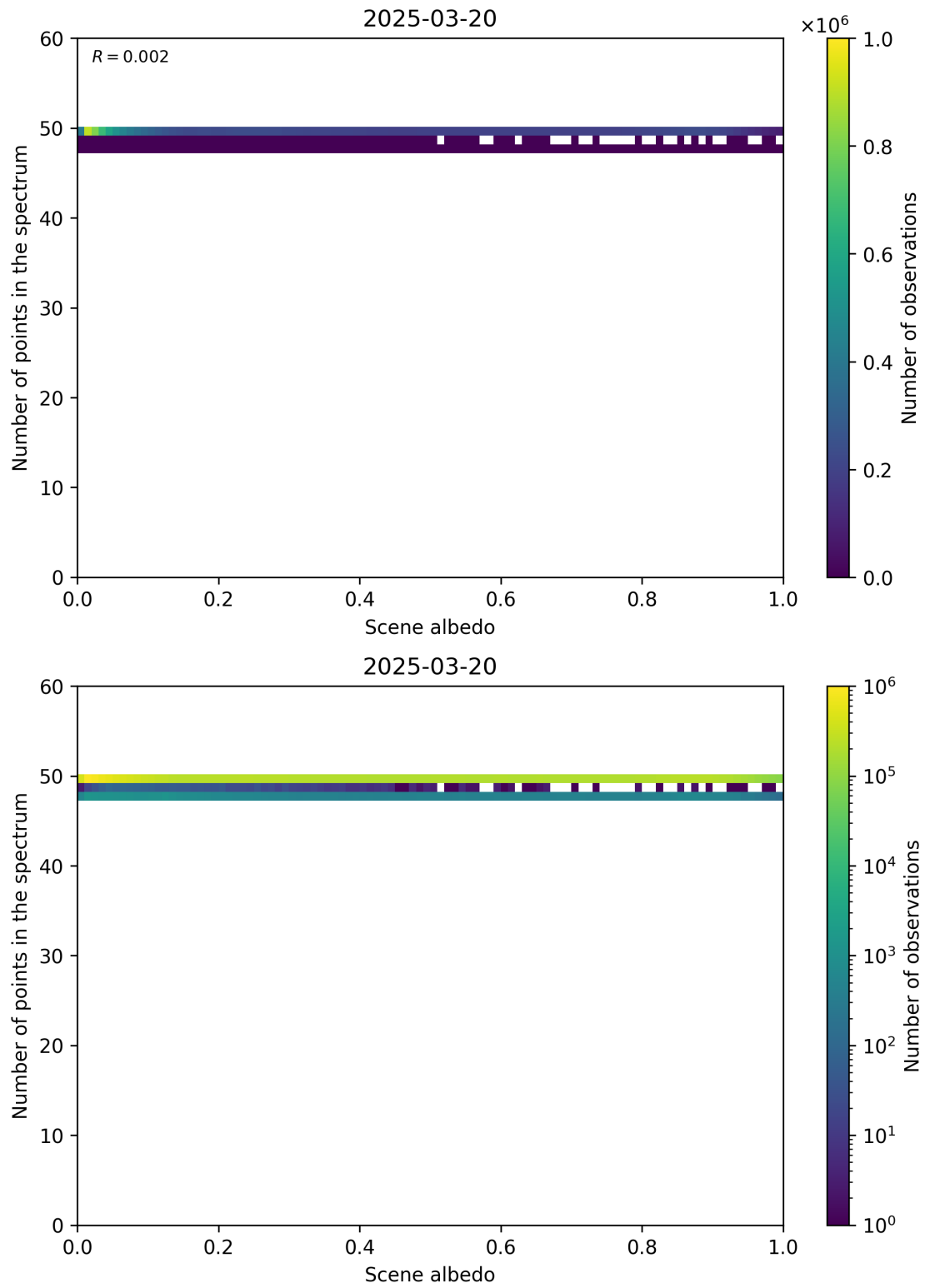
Figure 106: Scatter density plot of “Scene albedo” against “Number of points in the spectrum” for 2025-03-19 to 2025-03-21.
