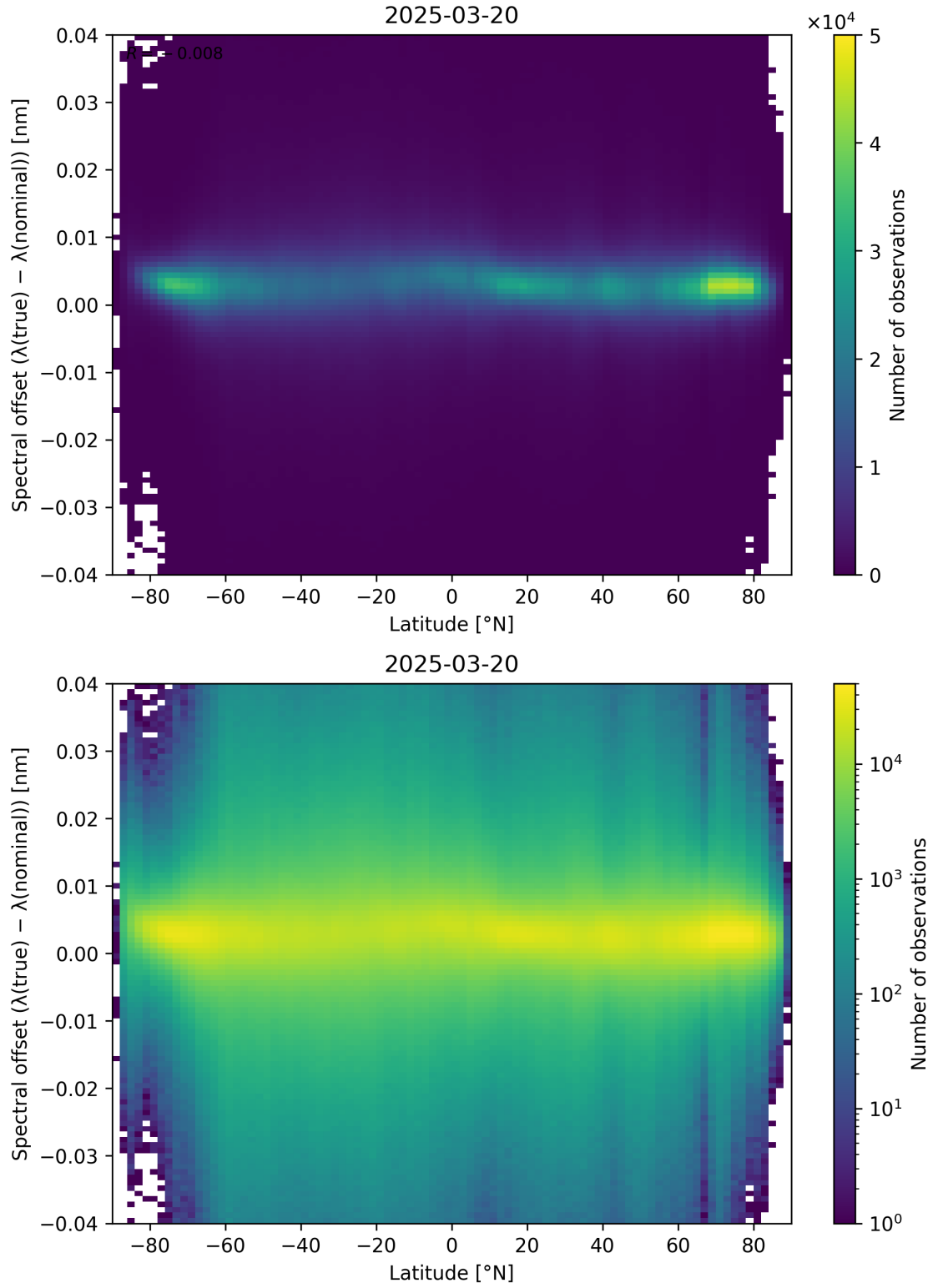
Figure 96: Scatter density plot of “Latitude” against “Spectral offset ( \lambda_{\text{true}} - \lambda_{\text{nominal}} )” for 2025-03-19 to 2025-03-21.
