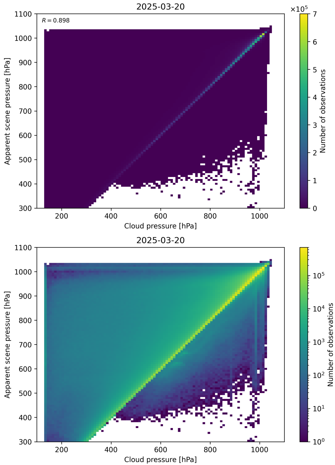
Figure 77: Scatter density plot of “Cloud pressure” against “Apparent scene pressure” for 2025-03-19 to 2025-03-21.
