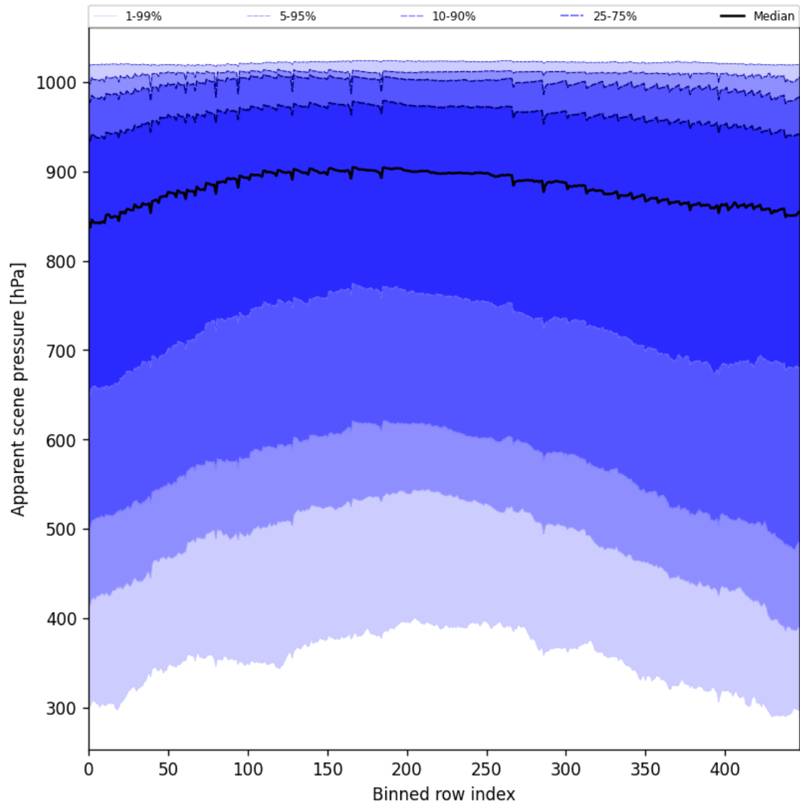
Figure 53: Along track statistics of “Apparent scene pressure” for 2025-03-19 to 2025-03-21
