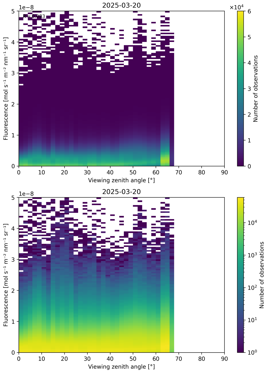
Figure 122: Scatter density plot of “Viewing zenith angle” against “Fluorescence” for 2025-03-19 to 2025-03-21.
