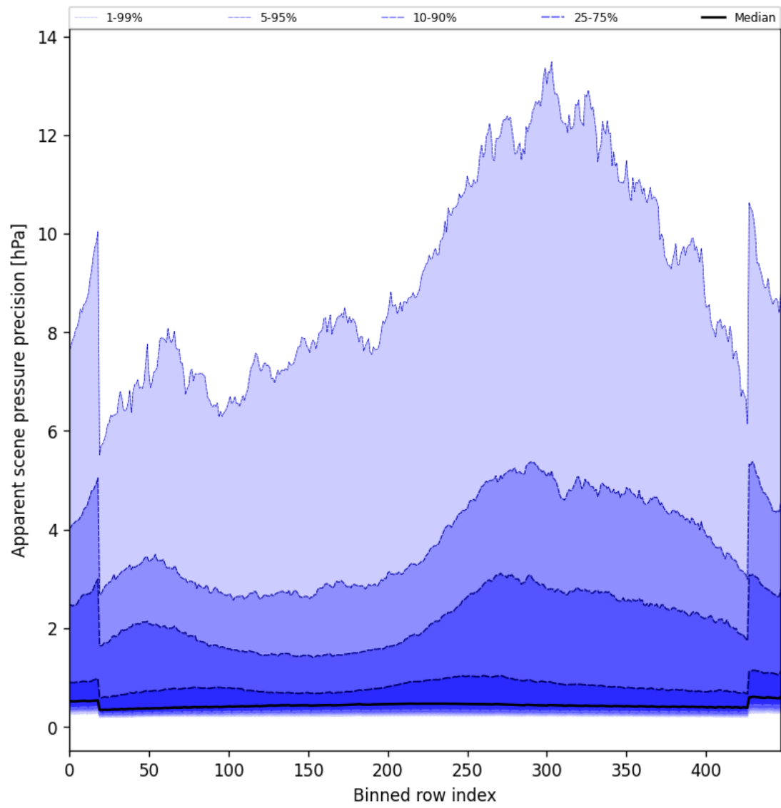
Figure 54: Along track statistics of “Apparent scene pressure precision” for 2025-03-19 to 2025-03-21
