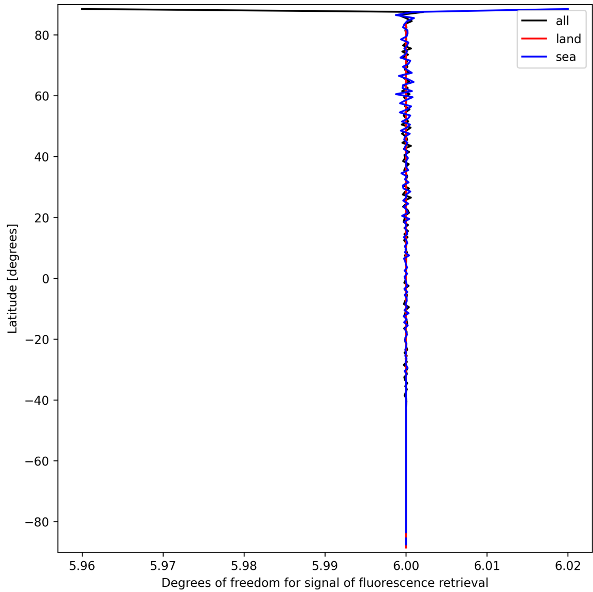
Figure 26: Zonal average of “Degrees of freedom for signal of fluorescence retrieval” for 2025-03-19 to 2025-03-21.
