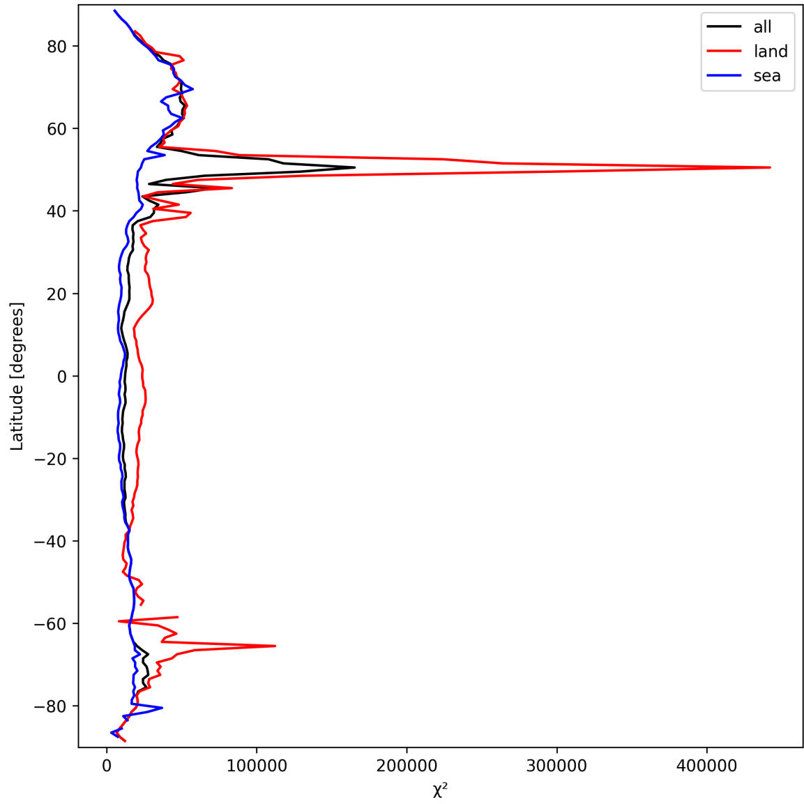
Figure 21: Zonal average of “ \chi^2 ” for 2025-03-19 to 2025-03-21.
