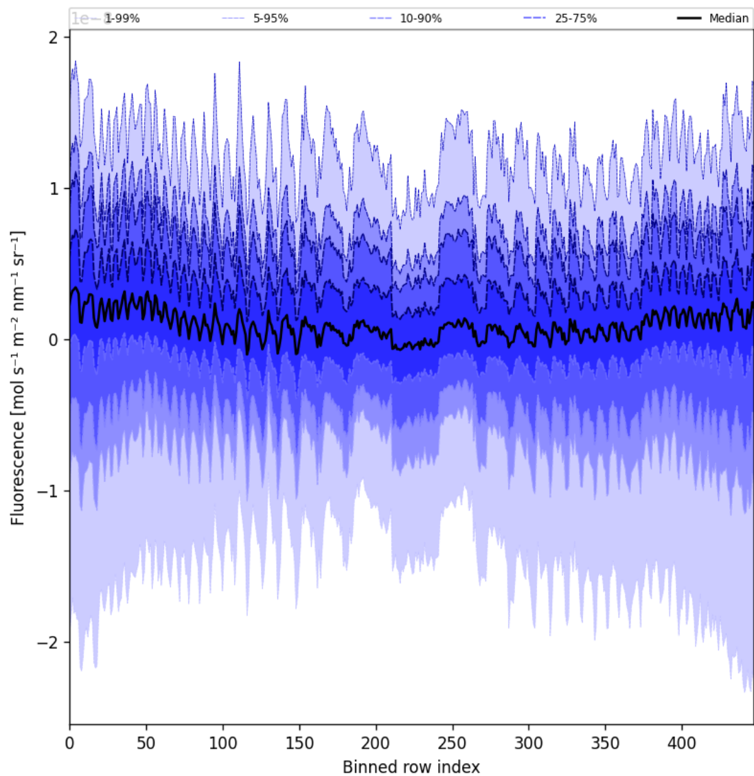
Figure 57: Along track statistics of “Fluorescence” for 2025-03-19 to 2025-03-21
