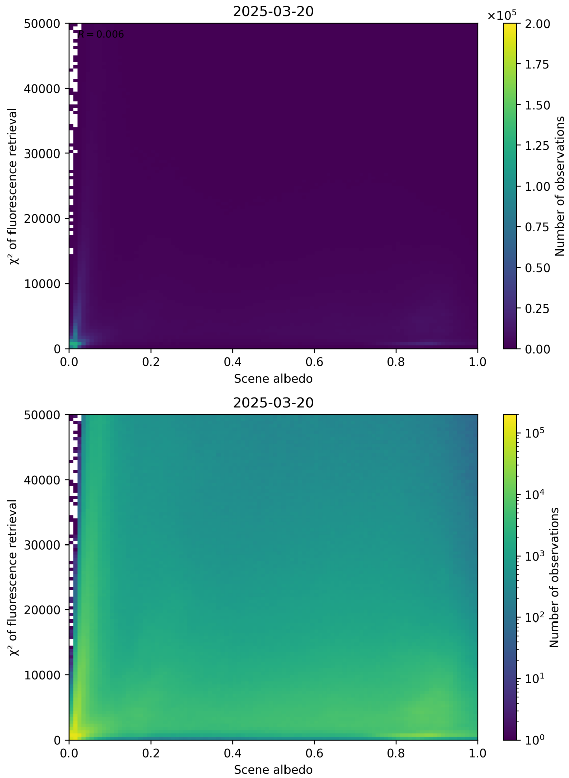
Figure 103: Scatter density plot of “Scene albedo” against “ \chi^2 of fluorescence retrieval” for 2025-03-19 to 2025-03-21.
