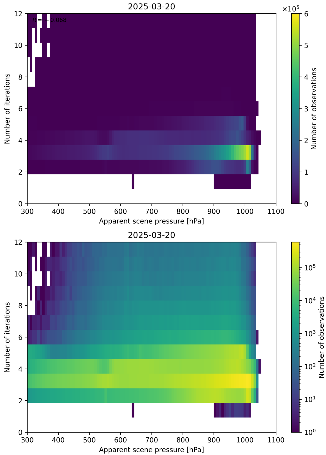
Figure 65: Scatter density plot of “Apparent scene pressure” against “Number of iterations” for 2025-03-19 to 2025-03-21.
