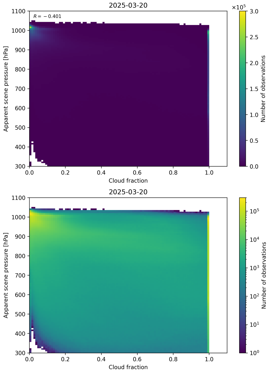
Figure 70: Scatter density plot of “Cloud fraction” against “Apparent scene pressure” for 2025-03-19 to 2025-03-21.
