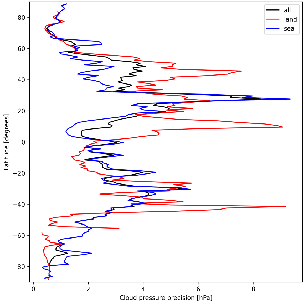
Figure 14: Zonal average of “Cloud pressure precision” for 2025-03-19 to 2025-03-21.
