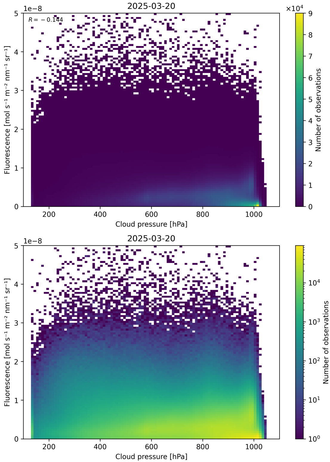
Figure 80: Scatter density plot of “Cloud pressure” against “Fluorescence” for 2025-03-19 to 2025-03-21.
