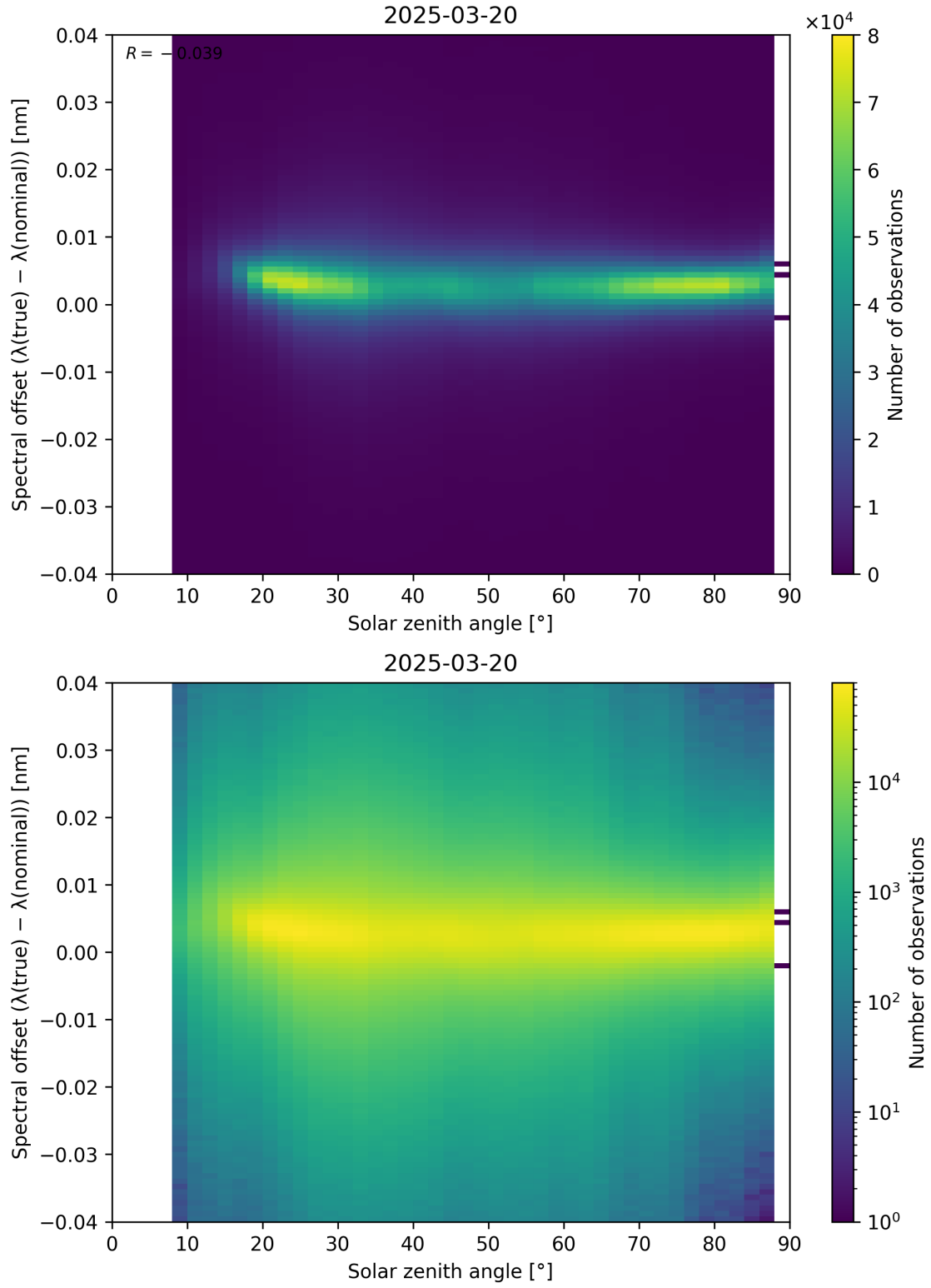
Figure 117: Scatter density plot of “Solar zenith angle” against “Spectral offset ( \lambda_{\text{true}} - \lambda_{\text{nominal}} )” for 2025-03-19 to 2025-03-21.
