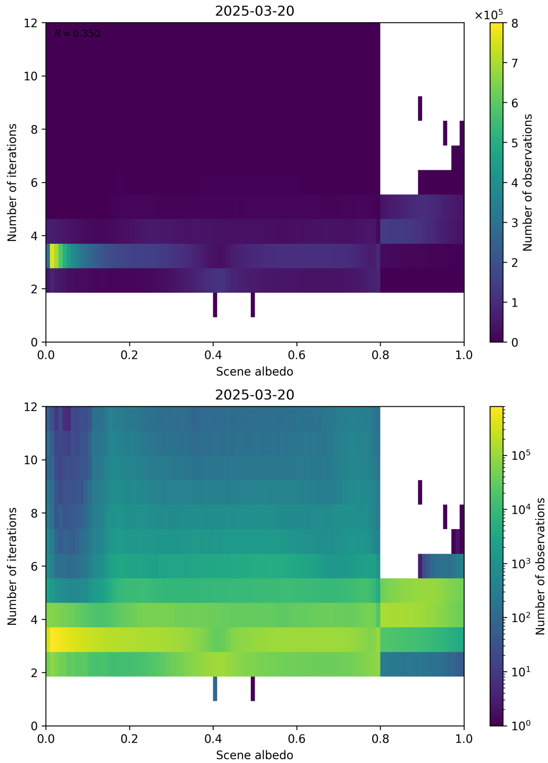
Figure 105: Scatter density plot of “Scene albedo” against “Number of iterations” for 2025-03-19 to 2025-03-21.
