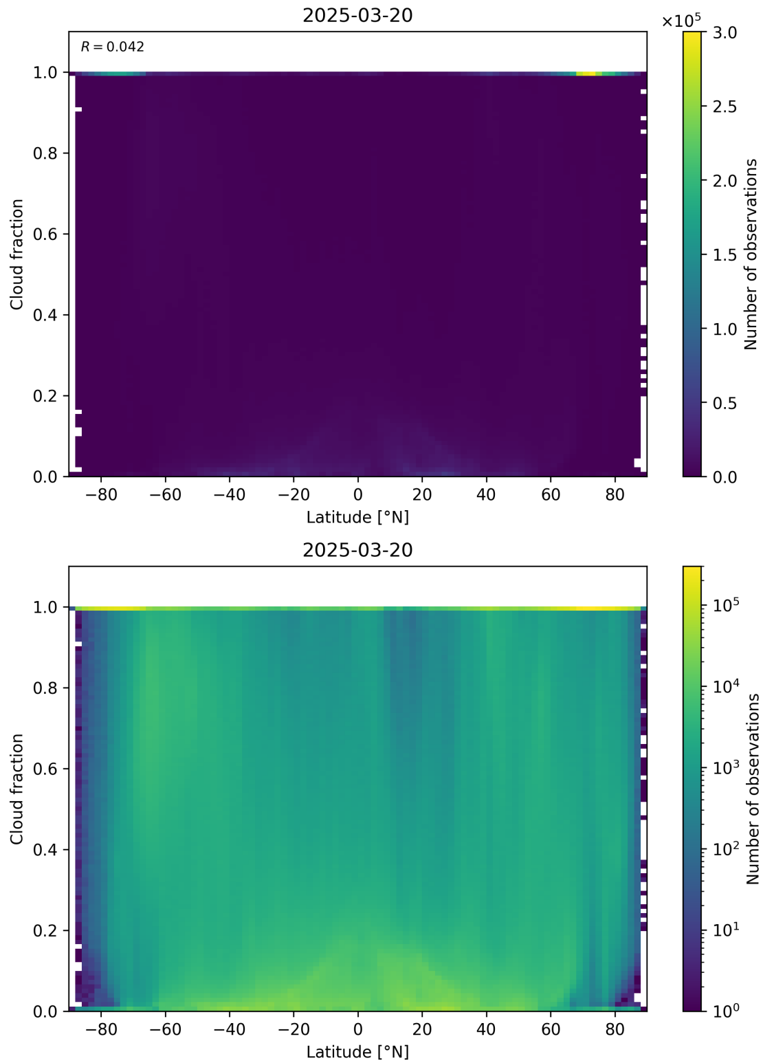
Figure 90: Scatter density plot of “Latitude” against “Cloud fraction” for 2025-03-19 to 2025-03-21.
