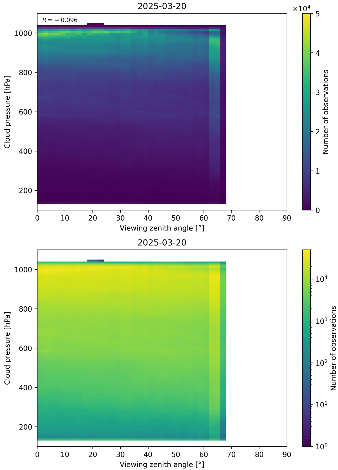
Figure 121: Scatter density plot of “Viewing zenith angle” against “Cloud pressure” for 2025-03-19 to 2025-03-21.
