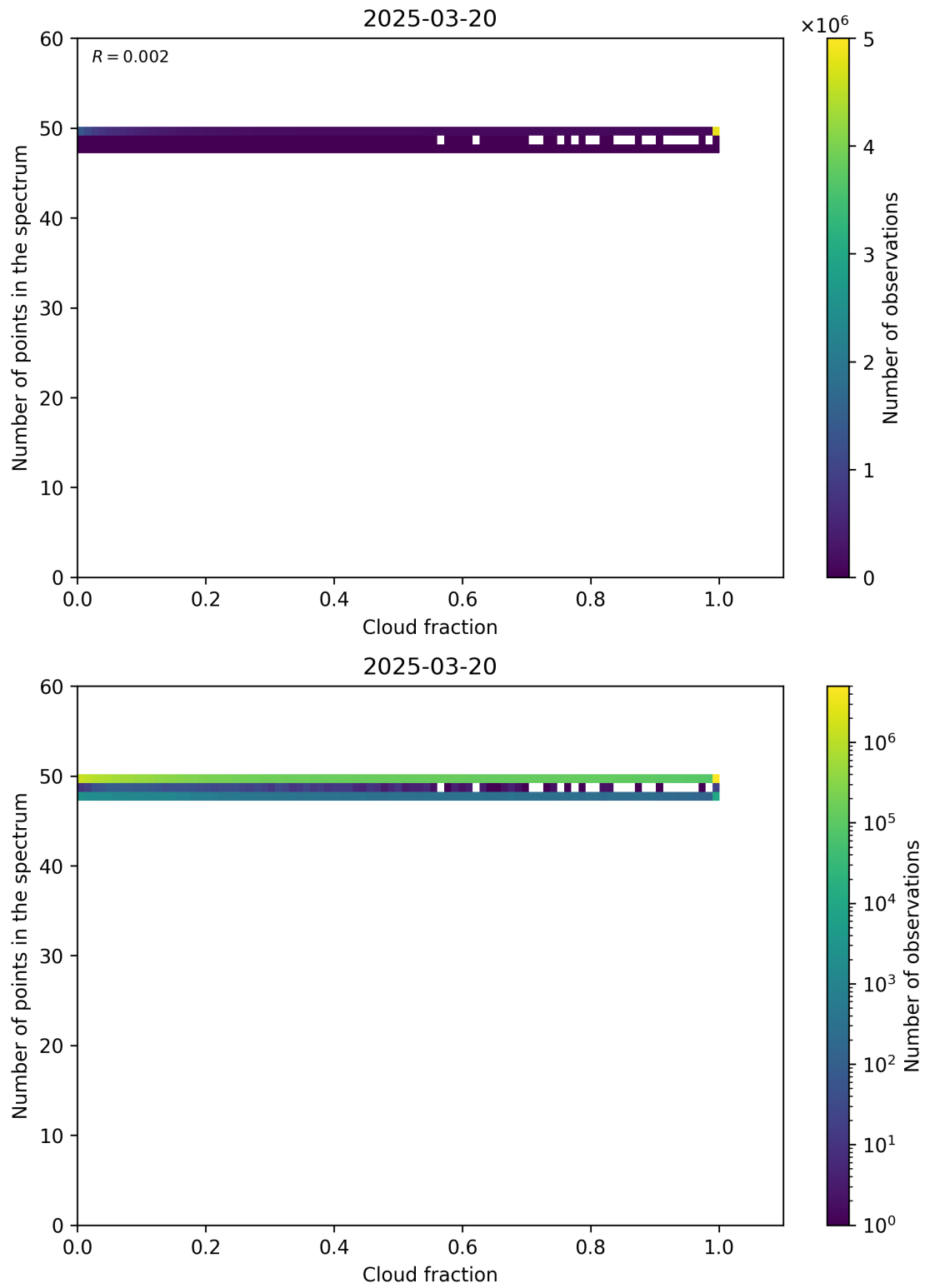
Figure 74: Scatter density plot of “Cloud fraction” against “Number of points in the spectrum” for 2025-03-19 to 2025-03-21.
