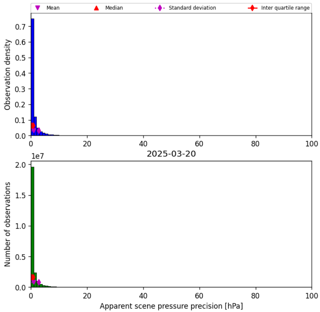
Figure 37: Histogram of “Apparent scene pressure precision” for 2025-03-19 to 2025-03-21
