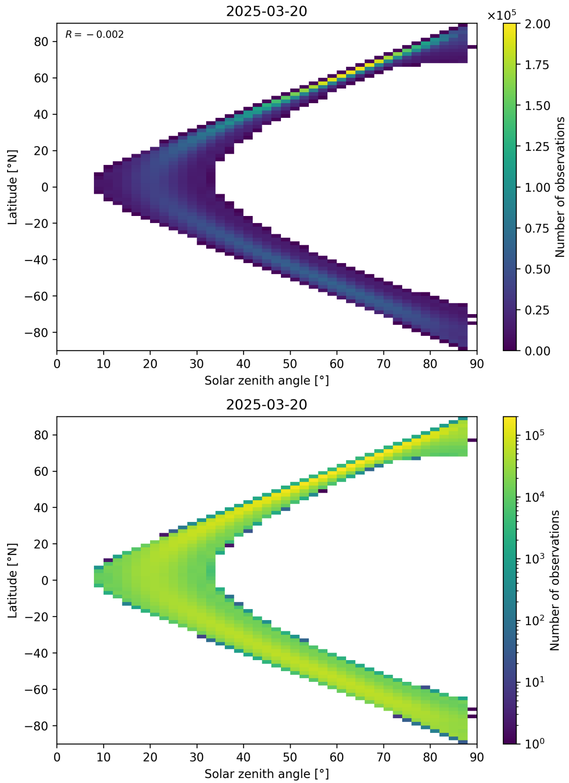
Figure 113: Scatter density plot of “Solar zenith angle” against “Latitude” for 2025-03-19 to 2025-03-21.
