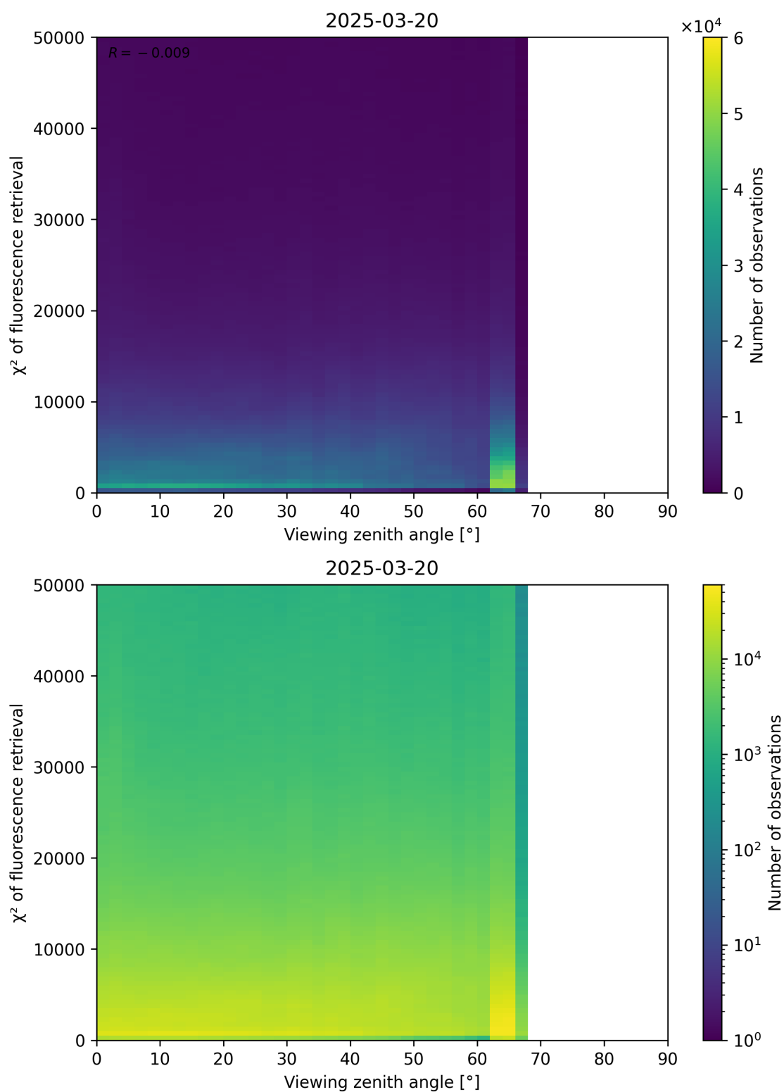
Figure 119: Scatter density plot of “Viewing zenith angle” against “ \chi^2 of fluorescence retrieval” for 2025-03-19 to 2025-03-21.
