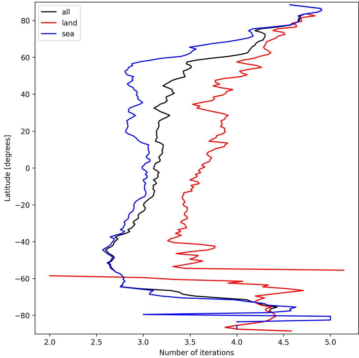
Figure 22: Zonal average of “Number of iterations” for 2025-03-19 to 2025-03-21.
