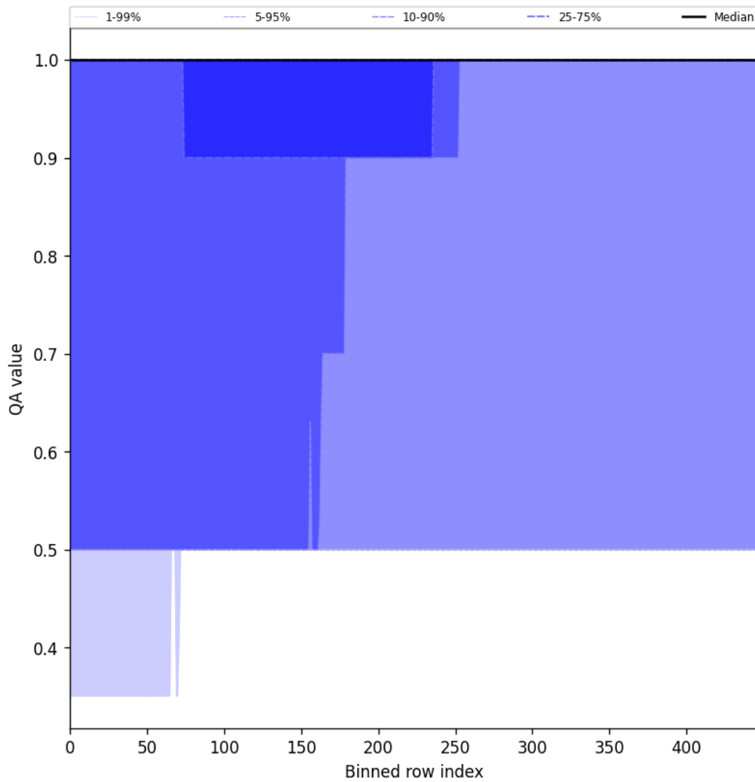
Figure 46: Along track statistics of “QA value” for 2025-03-19 to 2025-03-21
