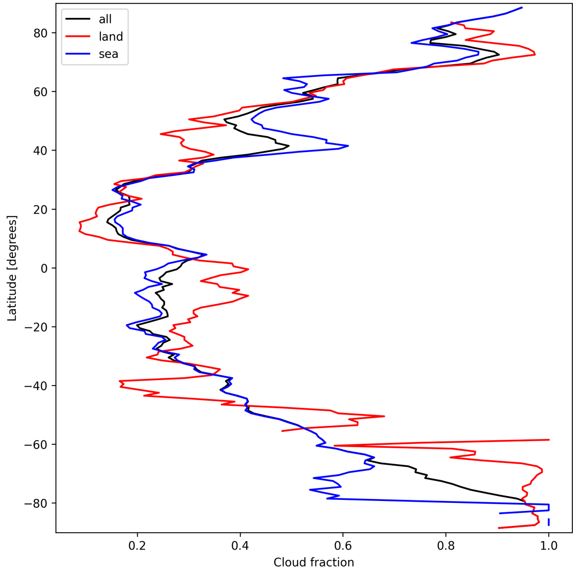
Figure 15: Zonal average of “Cloud fraction” for 2025-03-19 to 2025-03-21.
