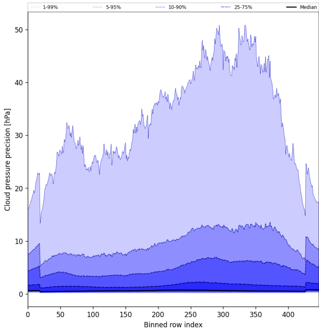
Figure 48: Along track statistics of “Cloud pressure precision” for 2025-03-19 to 2025-03-21
