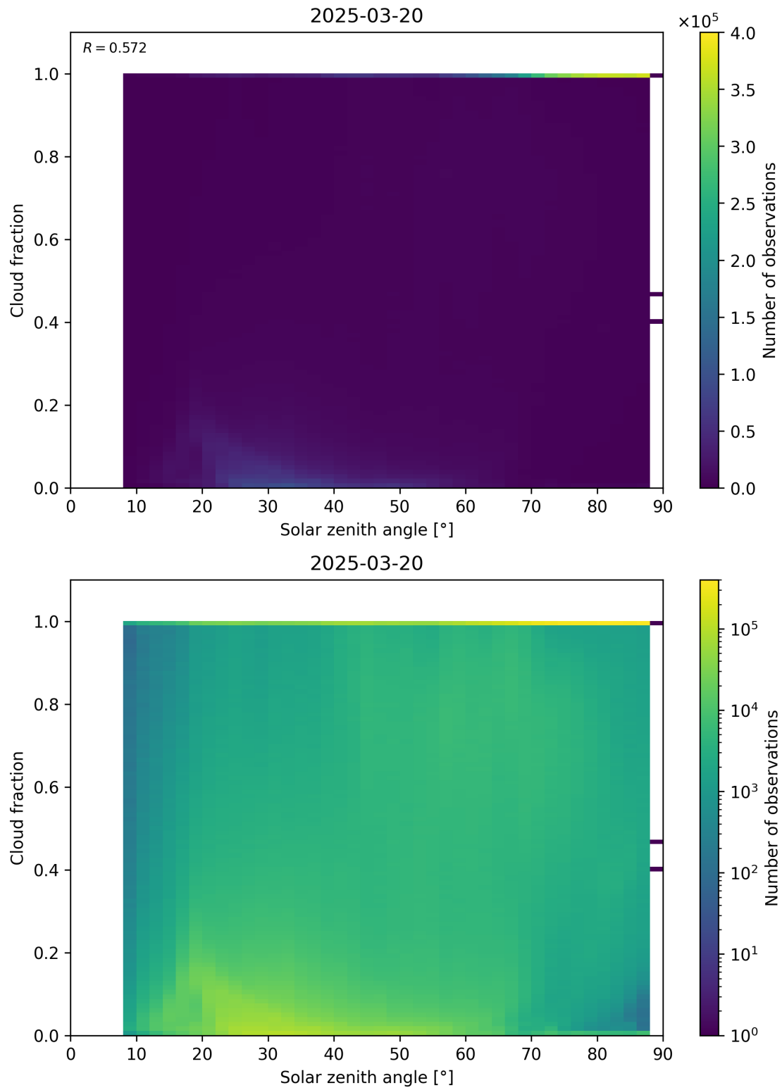
Figure 110: Scatter density plot of “Solar zenith angle” against “Cloud fraction” for 2025-03-19 to 2025-03-21.
