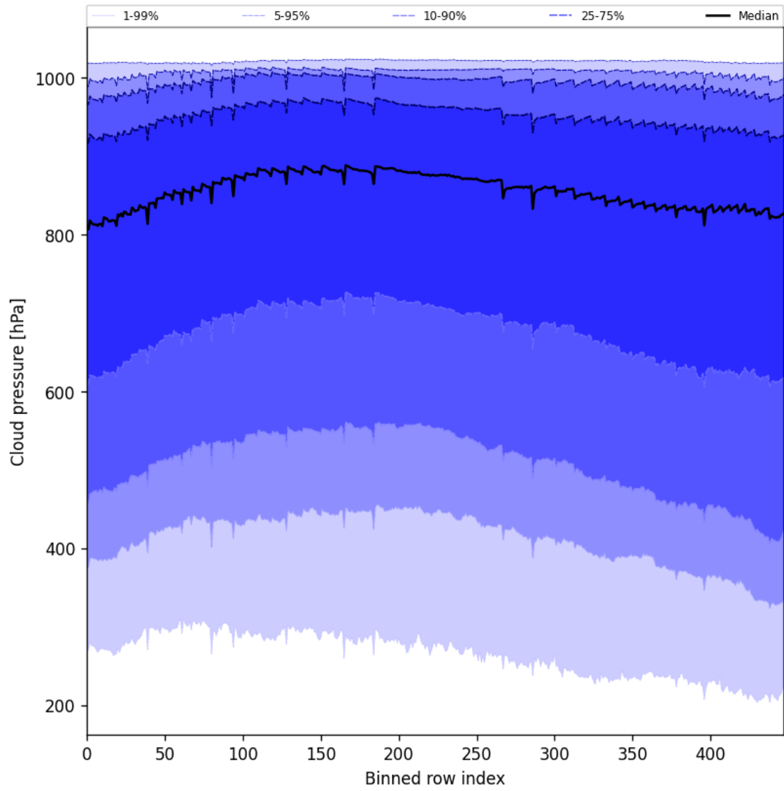
Figure 47: Along track statistics of “Cloud pressure” for 2025-03-19 to 2025-03-21
