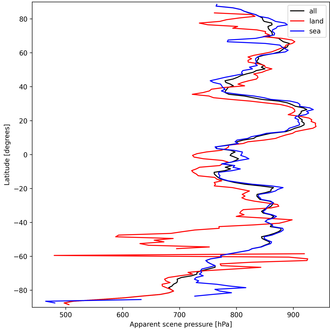
Figure 19: Zonal average of “Apparent scene pressure” for 2025-03-19 to 2025-03-21.
