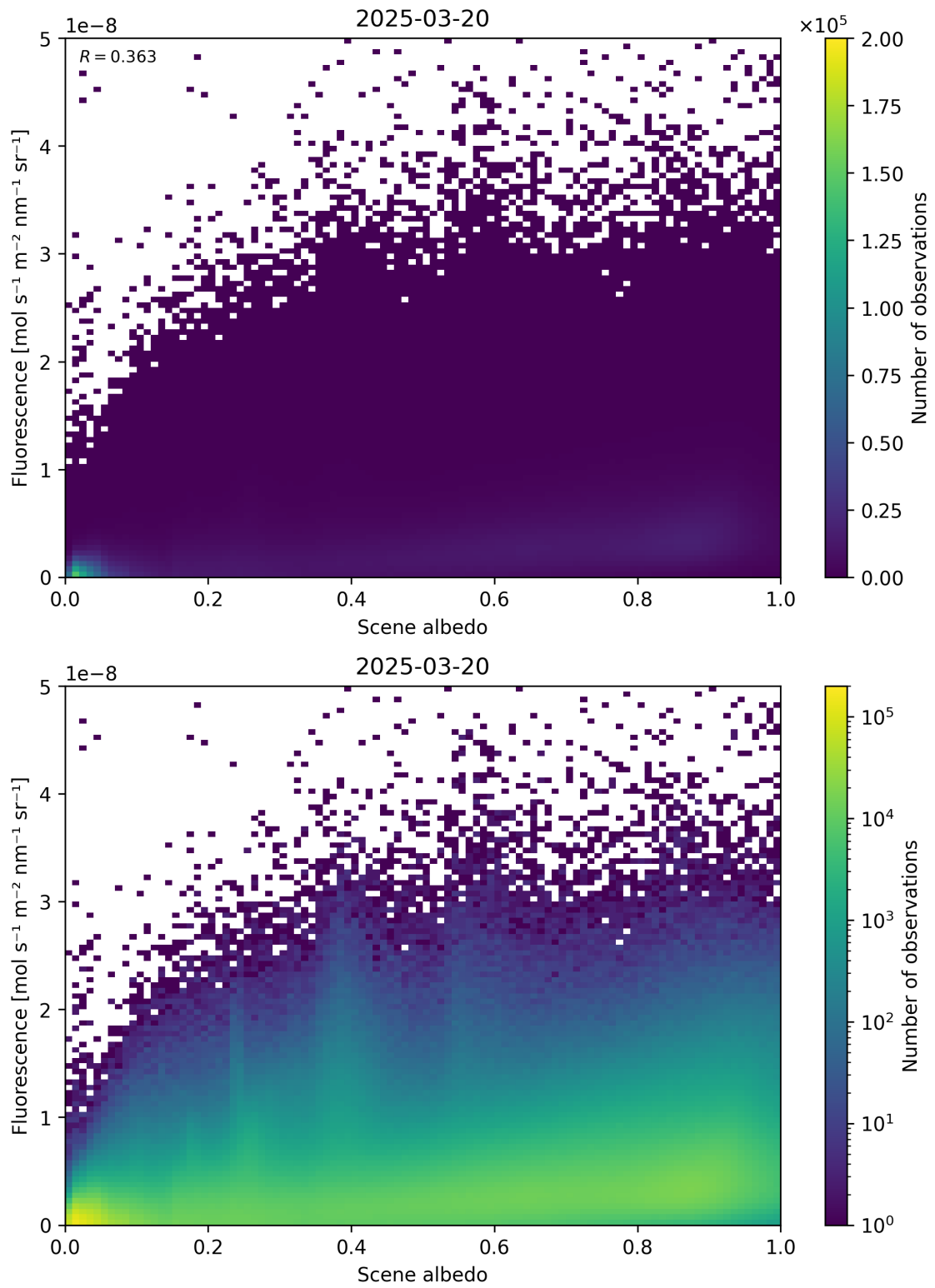
Figure 104: Scatter density plot of “Scene albedo” against “Fluorescence” for 2025-03-19 to 2025-03-21.
