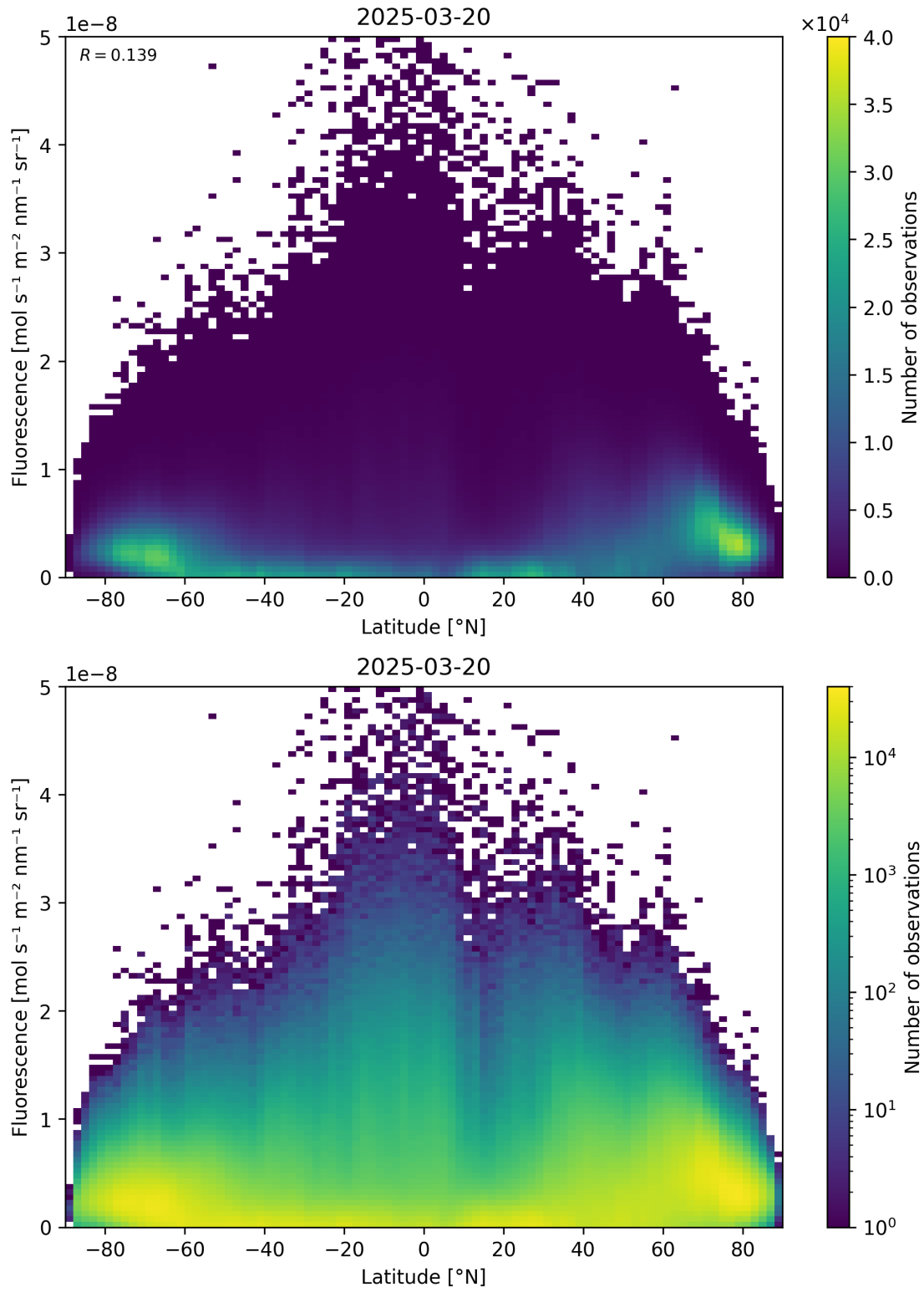
Figure 92: Scatter density plot of “Latitude” against “Fluorescence” for 2025-03-19 to 2025-03-21.
