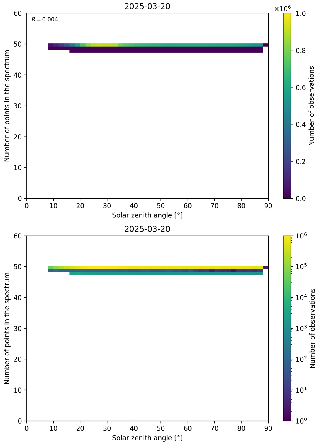
Figure 115: Scatter density plot of “Solar zenith angle” against “Number of points in the spectrum” for 2025-03-19 to 2025-03-21.
