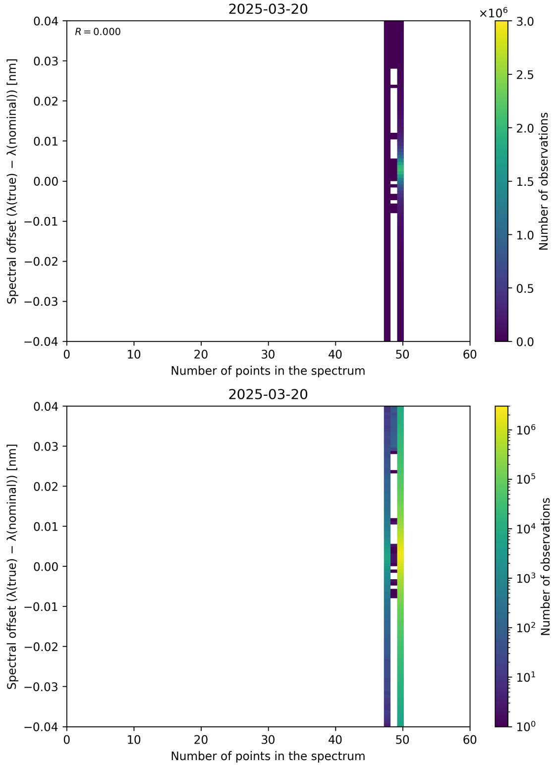
Figure 101: Scatter density plot of “Number of points in the spectrum” against “Spectral offset ( \lambda_{\text{true}} - \lambda_{\text{nominal}} )” for 2025-03-19 to 2025-03-21.
