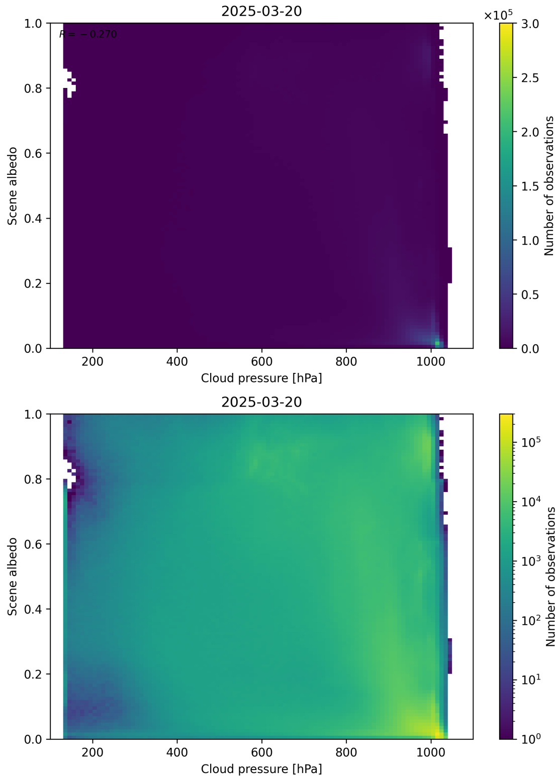
Figure 83: Scatter density plot of “Cloud pressure” against “Scene albedo” for 2025-03-19 to 2025-03-21.
