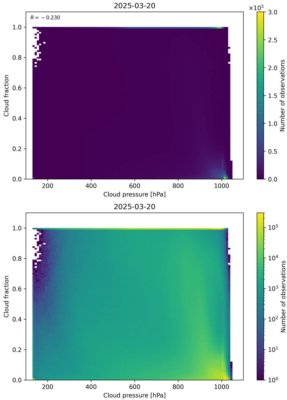
Figure 79: Scatter density plot of “Cloud pressure” against “Cloud fraction” for 2025-03-19 to 2025-03-21.
