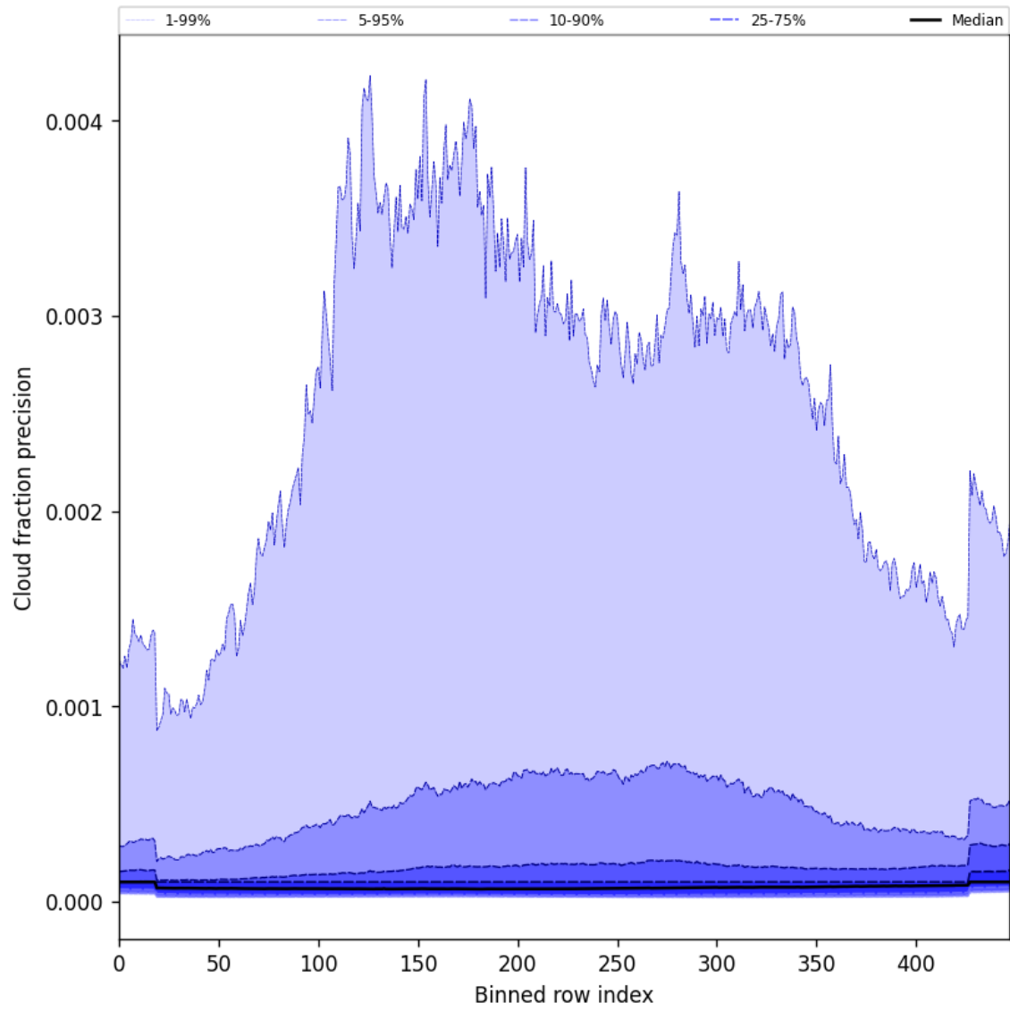
Figure 50: Along track statistics of “Cloud fraction precision” for 2025-03-19 to 2025-03-21
