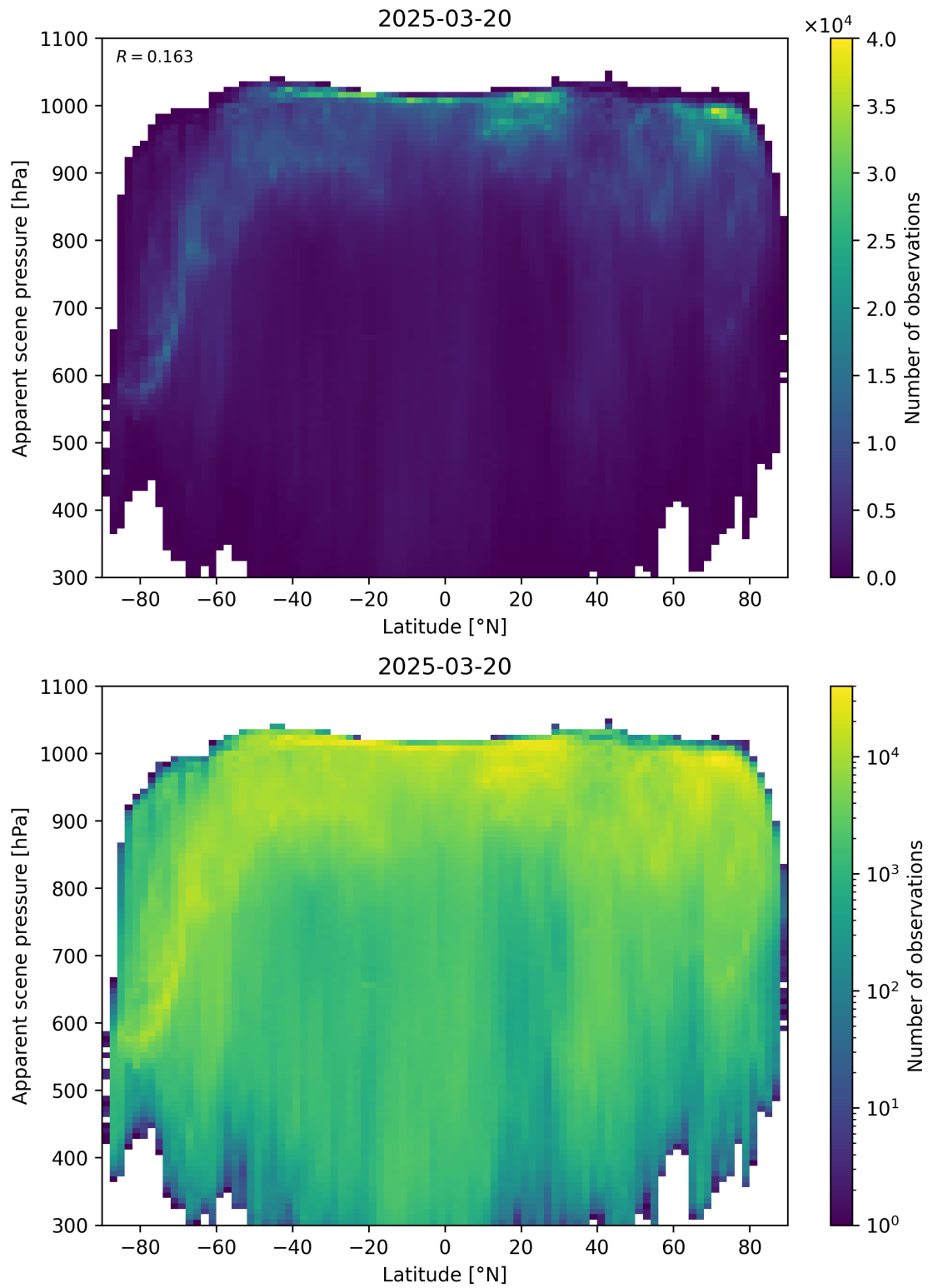
Figure 88: Scatter density plot of “Latitude” against “Apparent scene pressure” for 2025-03-19 to 2025-03-21.
