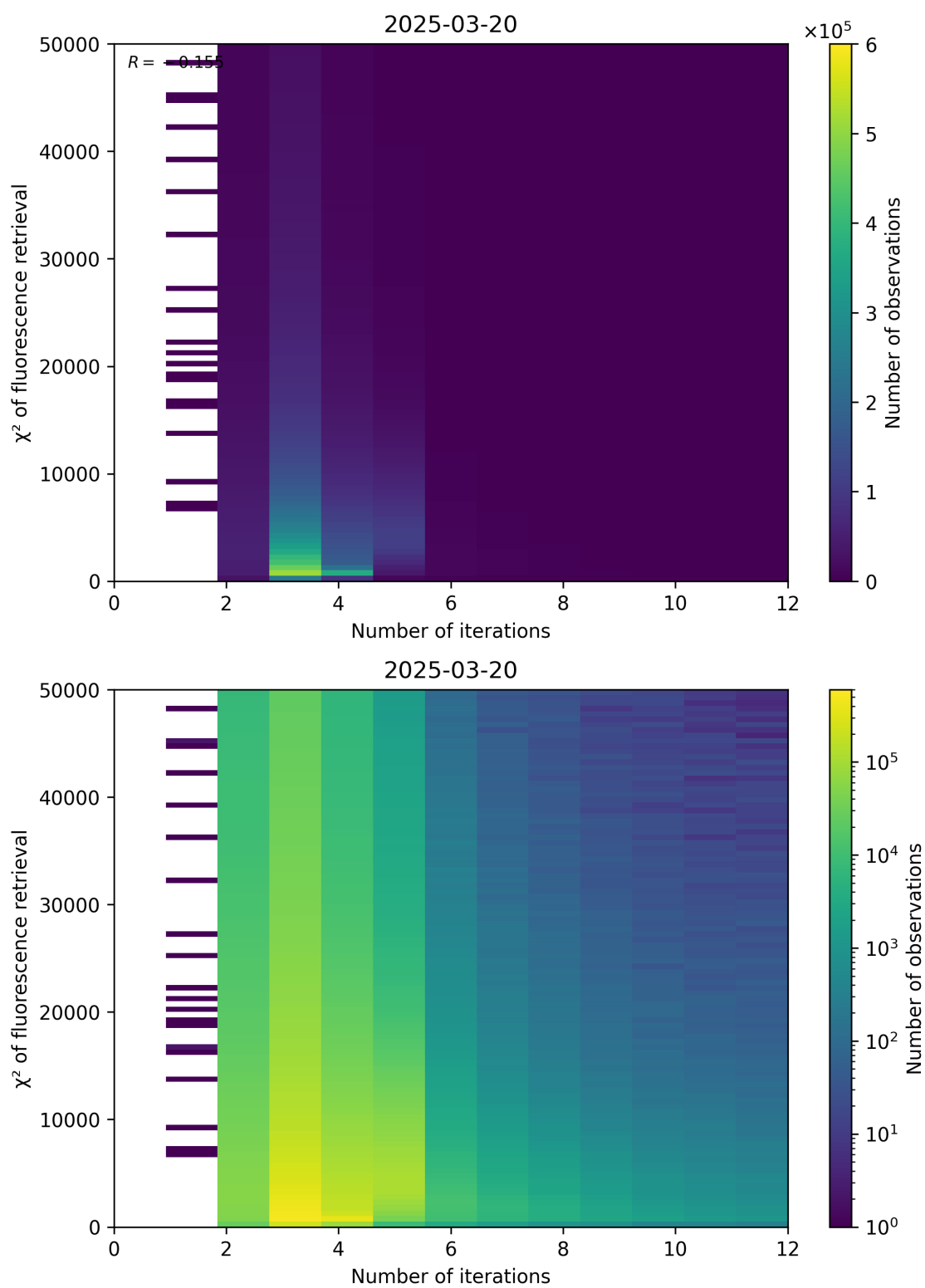
Figure 97: Scatter density plot of “Number of iterations” against “ \chi^2 of fluorescence retrieval” for 2025-03-19 to 2025-03-21.
