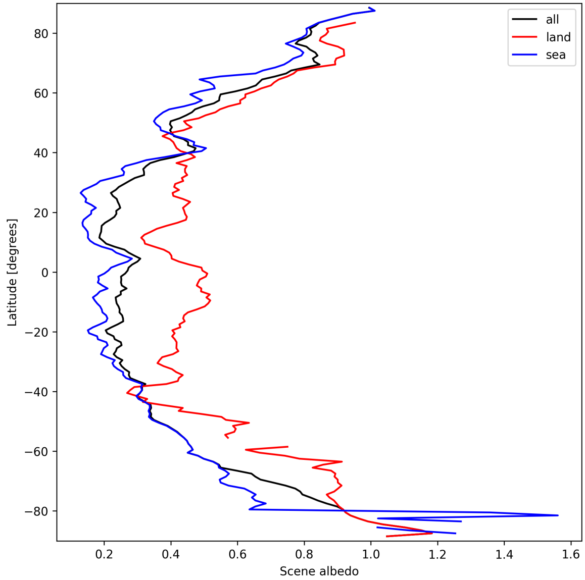
Figure 17: Zonal average of “Scene albedo” for 2025-03-19 to 2025-03-21.
