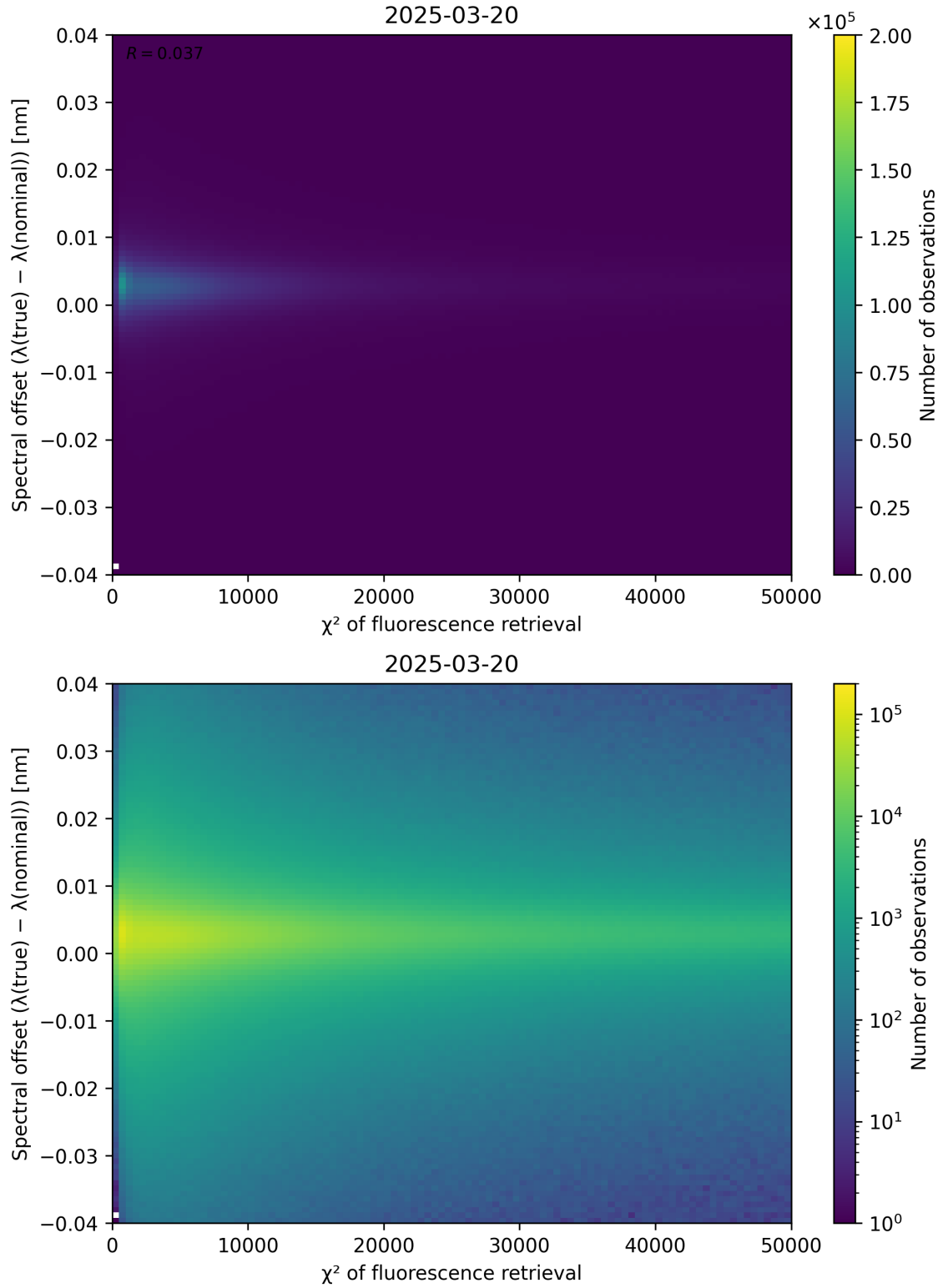
Figure 69: Scatter density plot of “ \chi^2 of fluorescence retrieval” against “Spectral offset ( \lambda_{\text{true}} - \lambda_{\text{nominal}} )” for 2025-03-19 to 2025-03-21.
