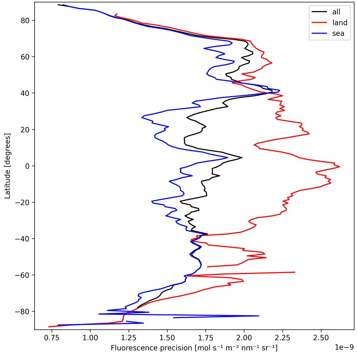
Figure 24: Zonal average of “Fluorescence precision” for 2025-03-19 to 2025-03-21.
