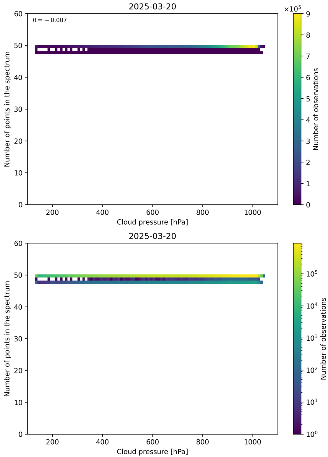
Figure 82: Scatter density plot of “Cloud pressure” against “Number of points in the spectrum” for 2025-03-19 to 2025-03-21.
