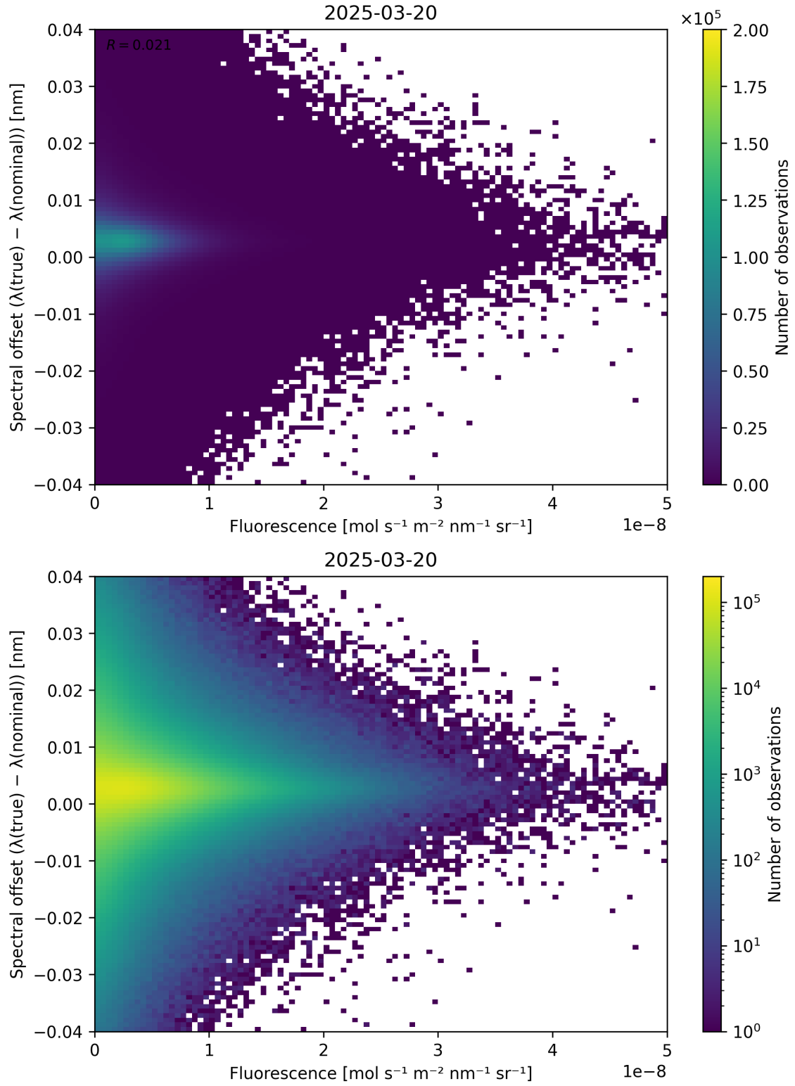
Figure 87: Scatter density plot of “Fluorescence” against “Spectral offset ( \lambda_{\text{true}} - \lambda_{\text{nominal}} )” for 2025-03-19 to 2025-03-21.
