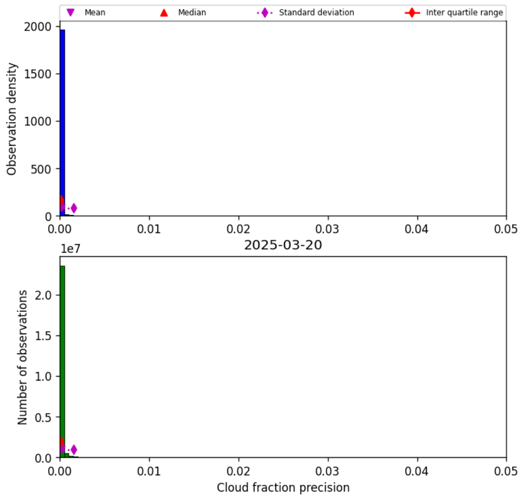
Figure 33: Histogram of “Cloud fraction precision” for 2025-03-19 to 2025-03-21
