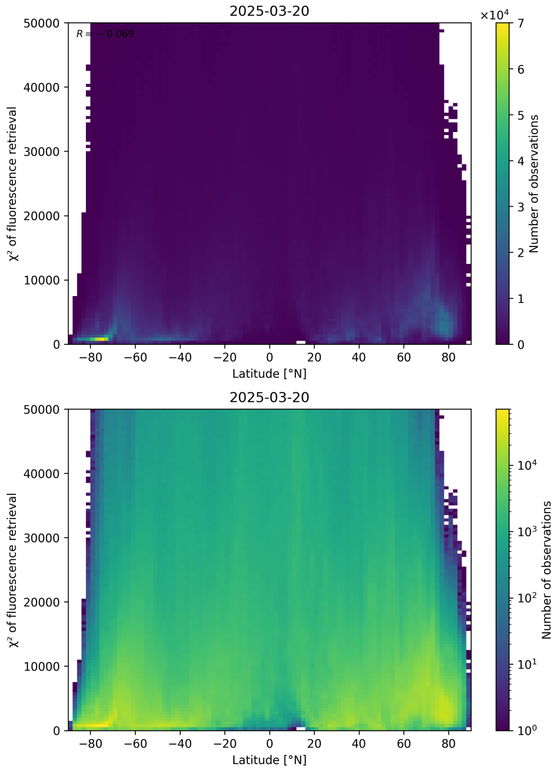
Figure 89: Scatter density plot of “Latitude” against “ \chi^2 of fluorescence retrieval” for 2025-03-19 to 2025-03-21.
