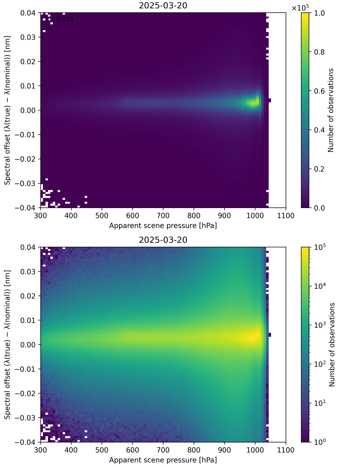
Figure 67: Scatter density plot of “Apparent scene pressure” against “Spectral offset ( \lambda_{\text{true}} - \lambda_{\text{nominal}} )” for 2025-03-19 to 2025-03-21.
