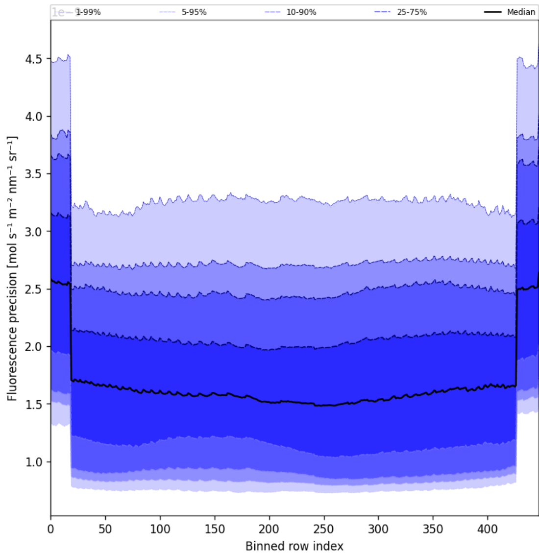
Figure 58: Along track statistics of “Fluorescence precision” for 2025-03-19 to 2025-03-21
