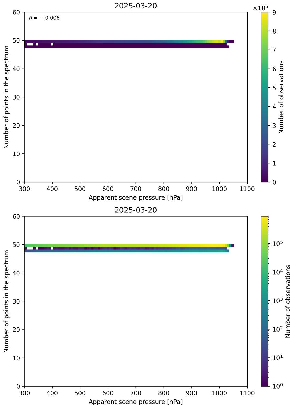
Figure 66: Scatter density plot of “Apparent scene pressure” against “Number of points in the spectrum” for 2025-03-19 to 2025-03-21.
