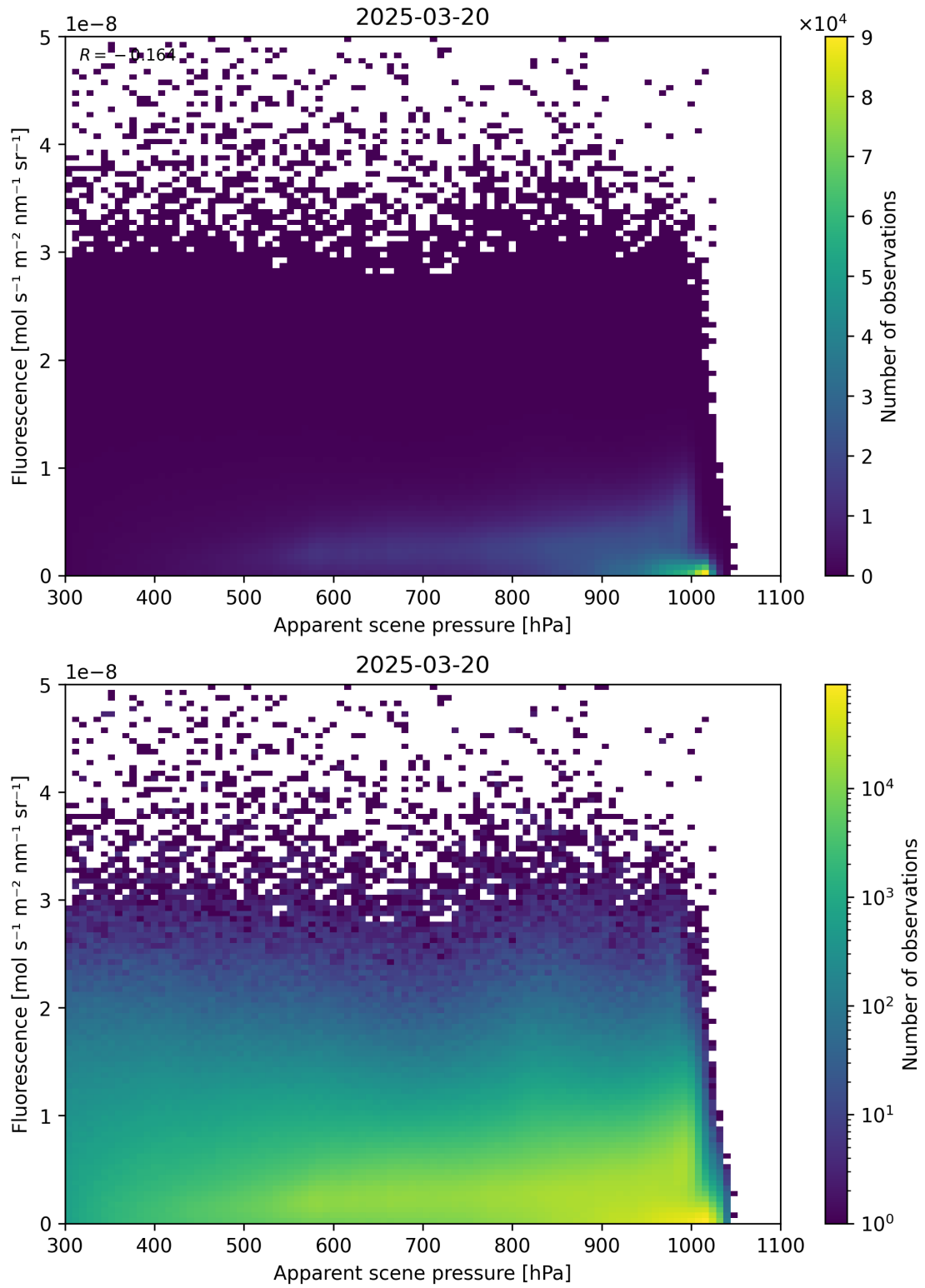
Figure 64: Scatter density plot of “Apparent scene pressure” against “Fluorescence” for 2025-03-19 to 2025-03-21.
