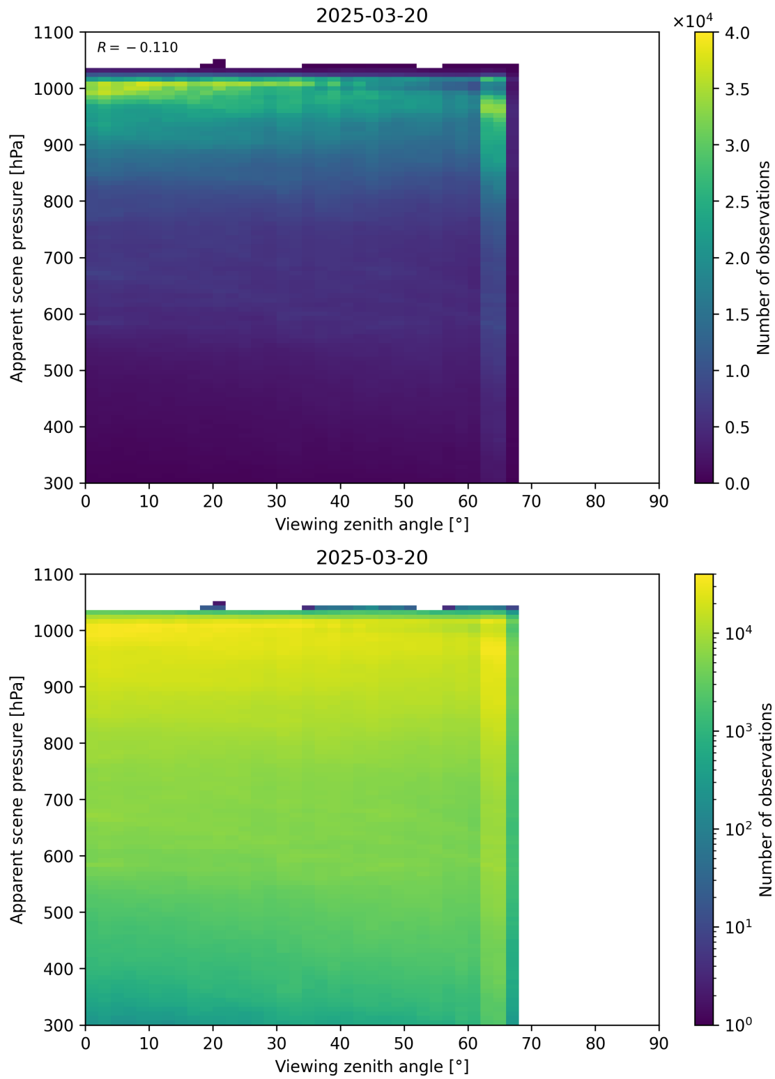
Figure 118: Scatter density plot of “Viewing zenith angle” against “Apparent scene pressure” for 2025-03-19 to 2025-03-21.
