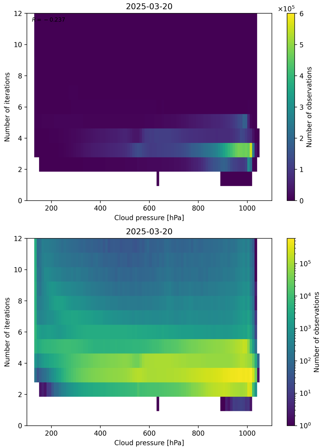
Figure 81: Scatter density plot of “Cloud pressure” against “Number of iterations” for 2025-03-19 to 2025-03-21.
