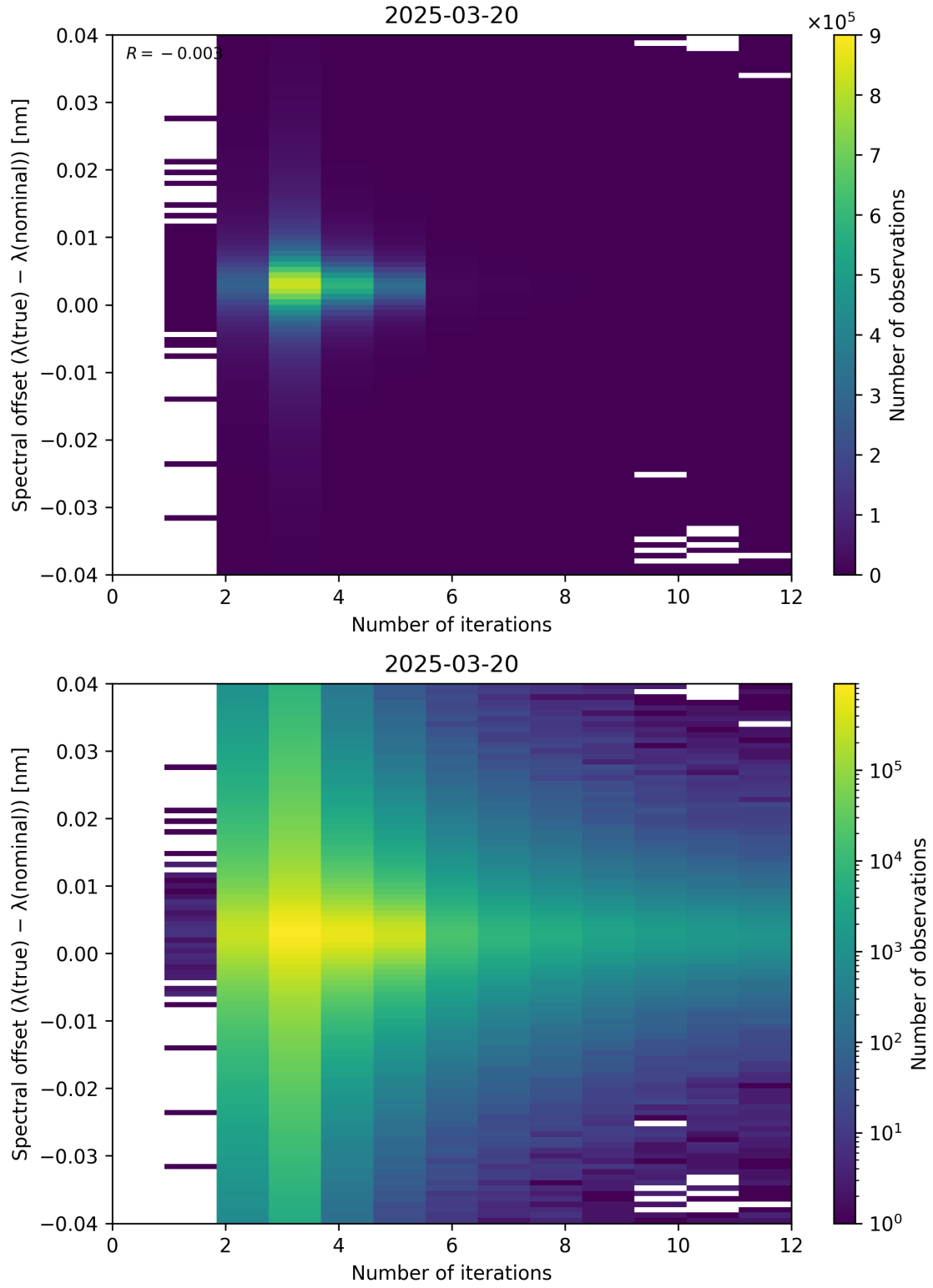
Figure 100: Scatter density plot of “Number of iterations” against “Spectral offset ( \lambda_{\text{true}} - \lambda_{\text{nominal}} )” for 2025-03-19 to 2025-03-21.
