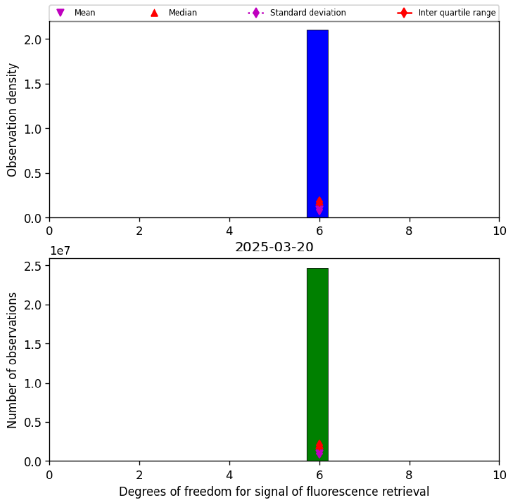
Figure 43: Histogram of “Degrees of freedom for signal of fluorescence retrieval” for 2025-03-19 to 2025-03-21
