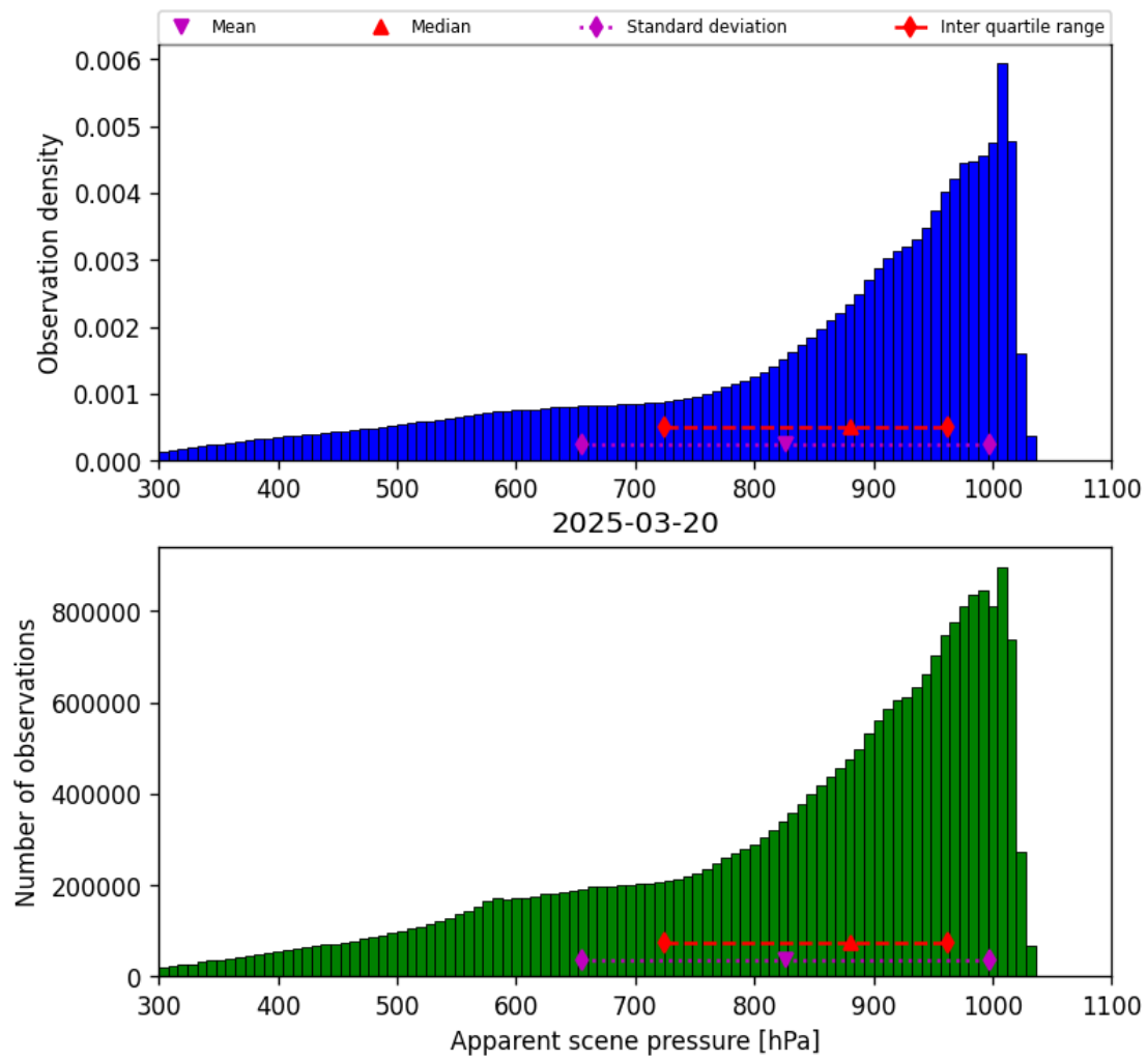
Figure 36: Histogram of “Apparent scene pressure” for 2025-03-19 to 2025-03-21
