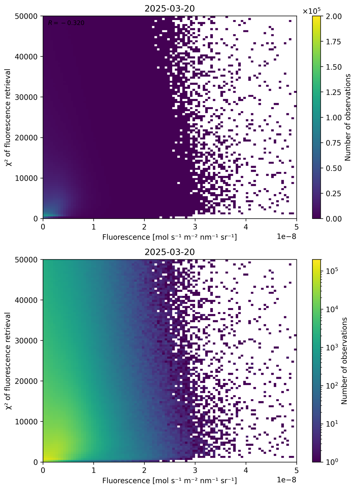
Figure 85: Scatter density plot of “Fluorescence” against “ \chi^2 of fluorescence retrieval” for 2025-03-19 to 2025-03-21.
