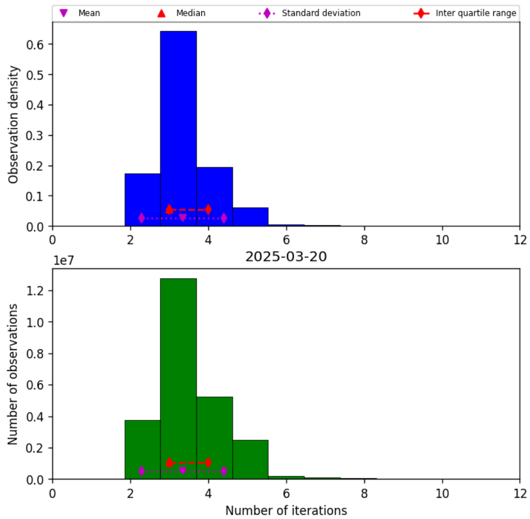
Figure 39: Histogram of “Number of iterations” for 2025-03-19 to 2025-03-21
