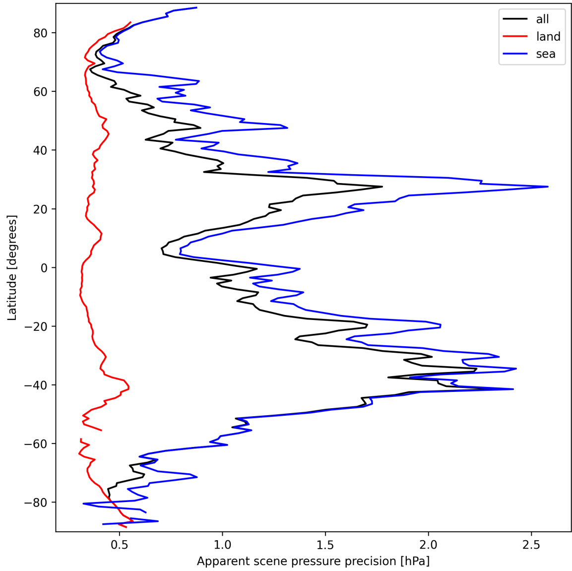
Figure 20: Zonal average of “Apparent scene pressure precision” for 2025-03-19 to 2025-03-21.
