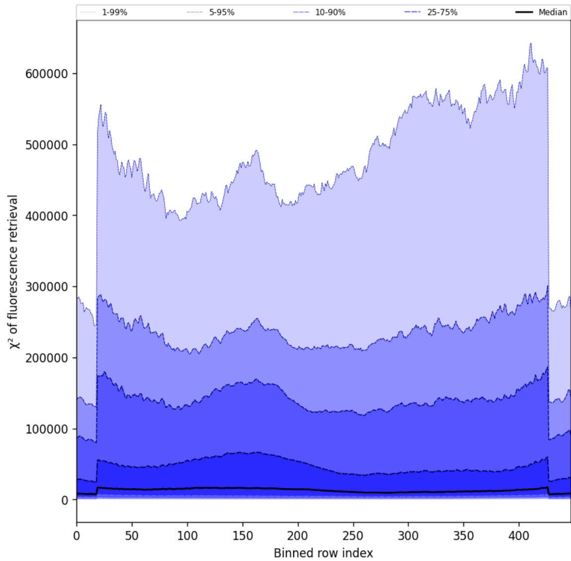
Figure 59: Along track statistics of “ \chi^2 of fluorescence retrieval” for 2025-03-19 to 2025-03-21
