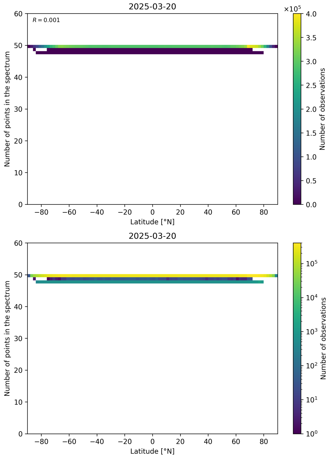
Figure 94: Scatter density plot of “Latitude” against “Number of points in the spectrum” for 2025-03-19 to 2025-03-21.
