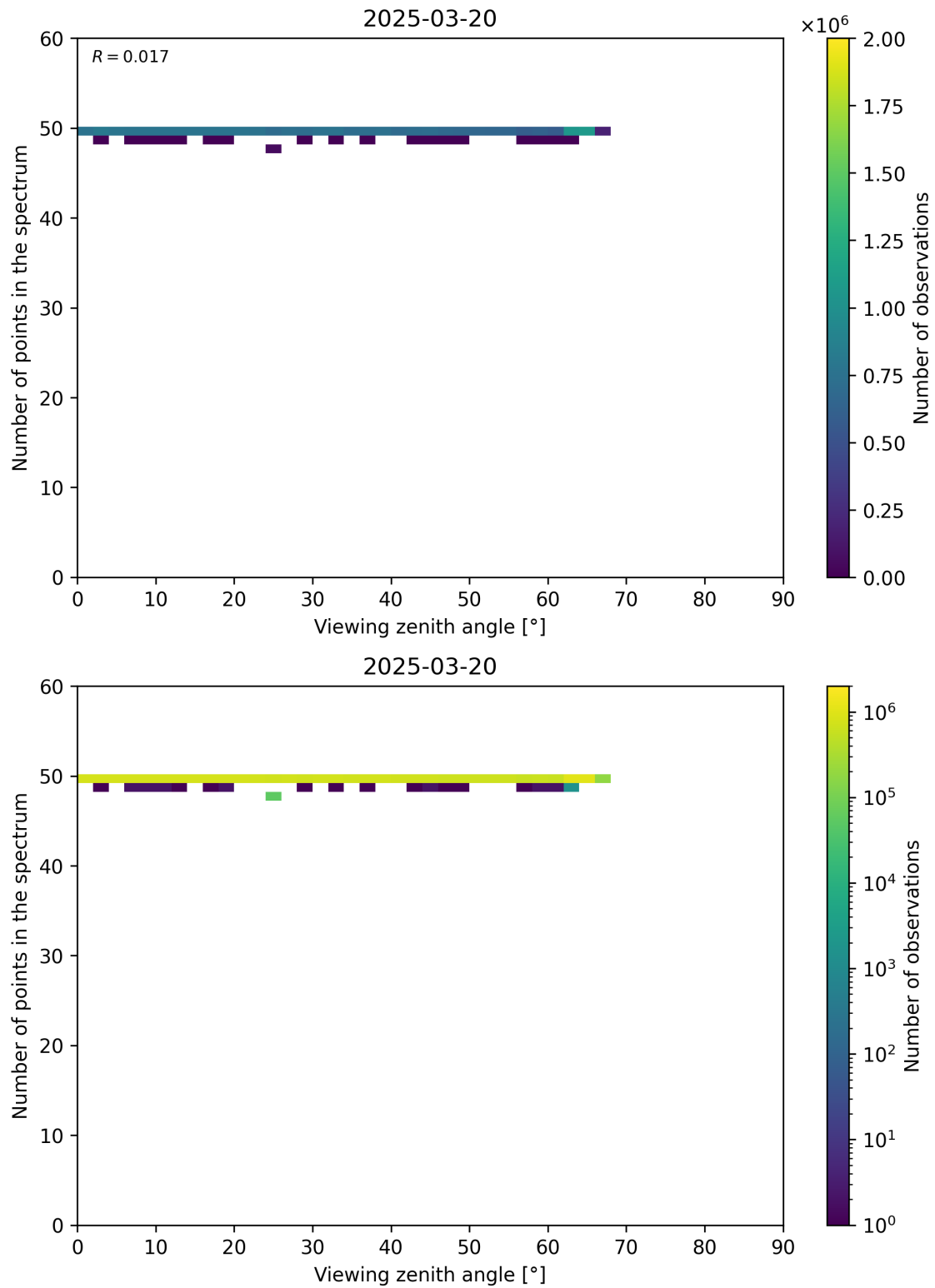
Figure 125: Scatter density plot of “Viewing zenith angle” against “Number of points in the spectrum” for 2025-03-19 to 2025-03-21.
