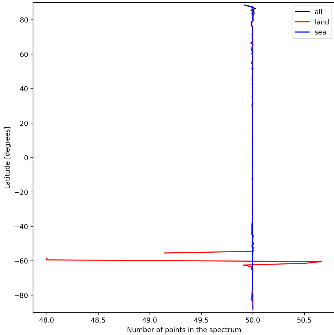
Figure 27: Zonal average of “Number of points in the spectrum” for 2025-03-19 to 2025-03-21.
