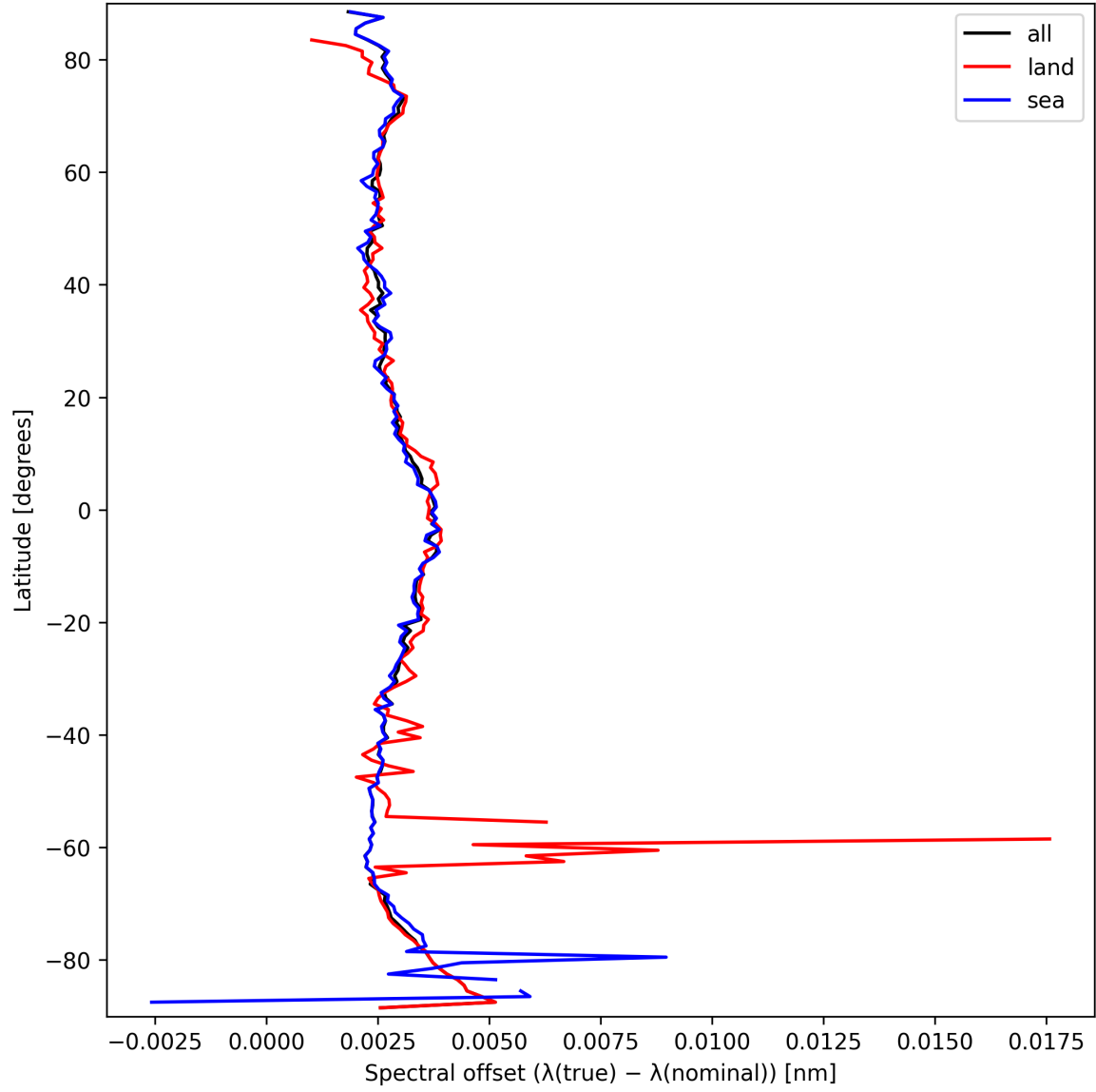
Figure 28: Zonal average of “Spectral offset ( \lambda_{\text{true}} - \lambda_{\text{nominal}} )” for 2025-03-19 to 2025-03-21.
