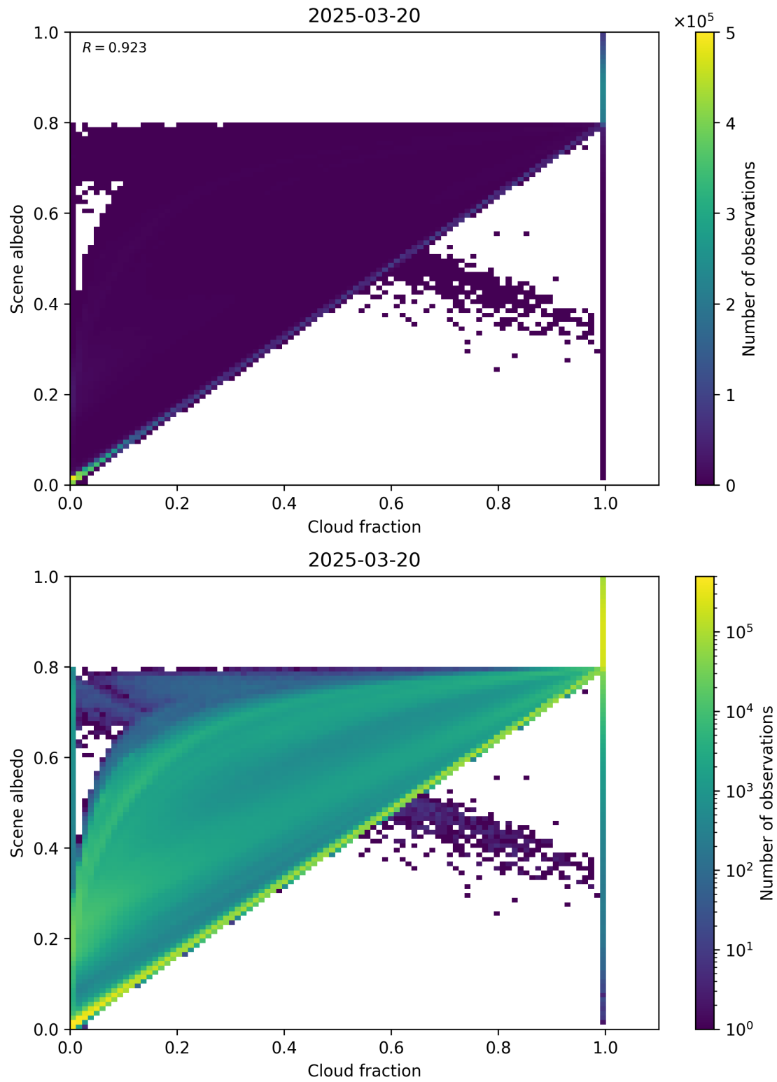
Figure 75: Scatter density plot of “Cloud fraction” against “Scene albedo” for 2025-03-19 to 2025-03-21.
