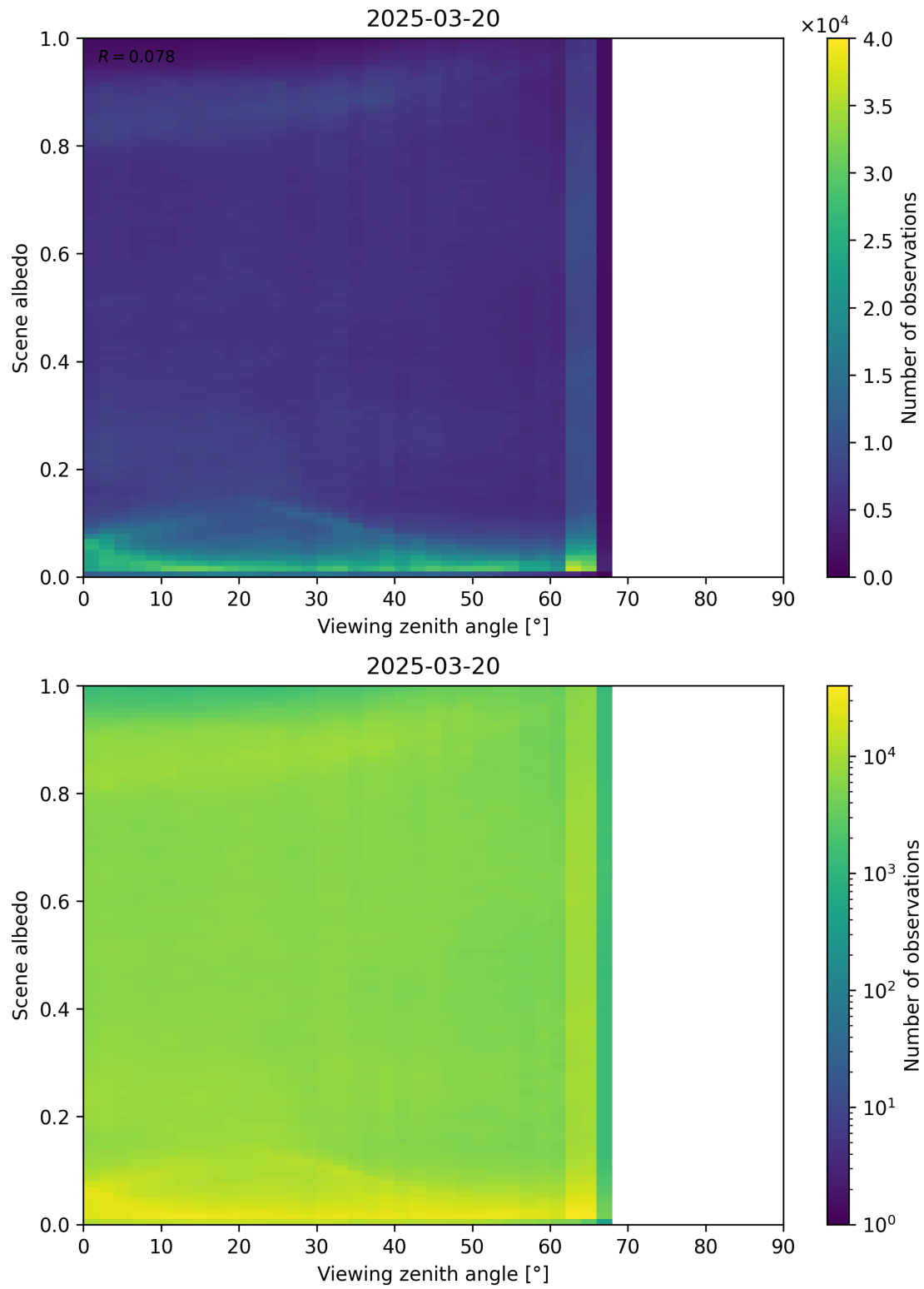
Figure 126: Scatter density plot of “Viewing zenith angle” against “Scene albedo” for 2025-03-19 to 2025-03-21.
