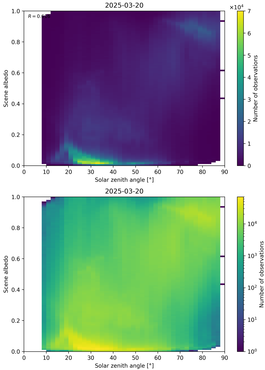
Figure 116: Scatter density plot of “Solar zenith angle” against “Scene albedo” for 2025-03-19 to 2025-03-21.
