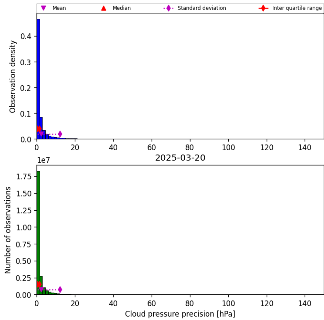
Figure 31: Histogram of “Cloud pressure precision” for 2025-03-19 to 2025-03-21
