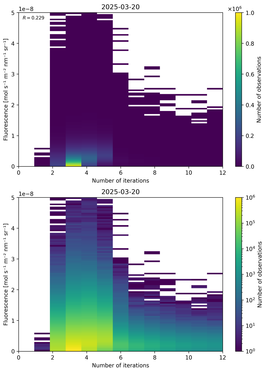
Figure 98: Scatter density plot of “Number of iterations” against “Fluorescence” for 2025-03-19 to 2025-03-21.
