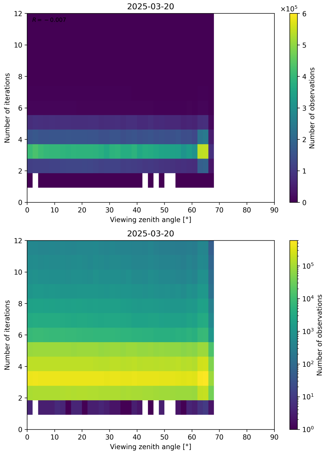
Figure 124: Scatter density plot of “Viewing zenith angle” against “Number of iterations” for 2025-03-19 to 2025-03-21.
