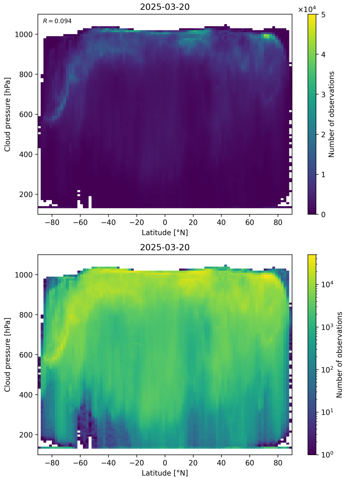
Figure 91: Scatter density plot of “Latitude” against “Cloud pressure” for 2025-03-19 to 2025-03-21.
