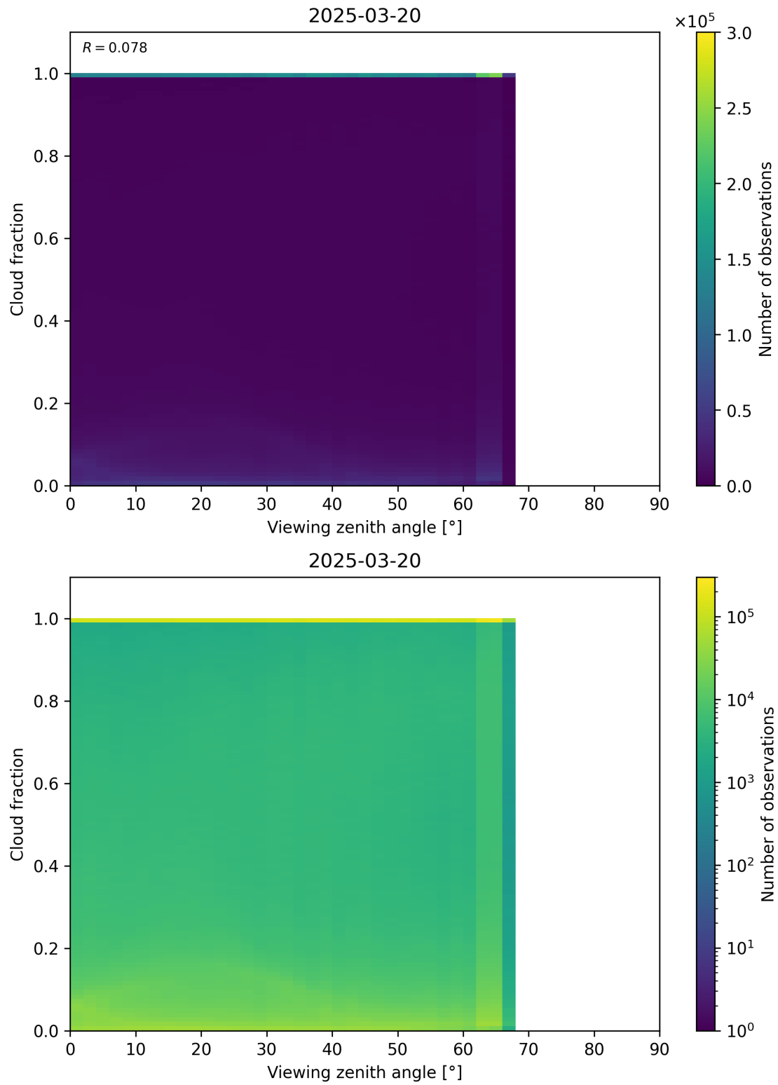
Figure 120: Scatter density plot of “Viewing zenith angle” against “Cloud fraction” for 2025-03-19 to 2025-03-21.
