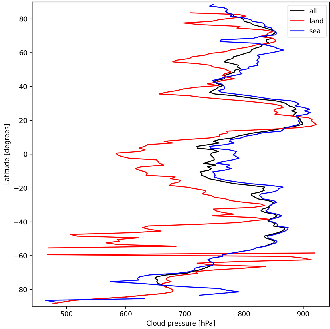
Figure 13: Zonal average of “Cloud pressure” for 2025-03-19 to 2025-03-21.
