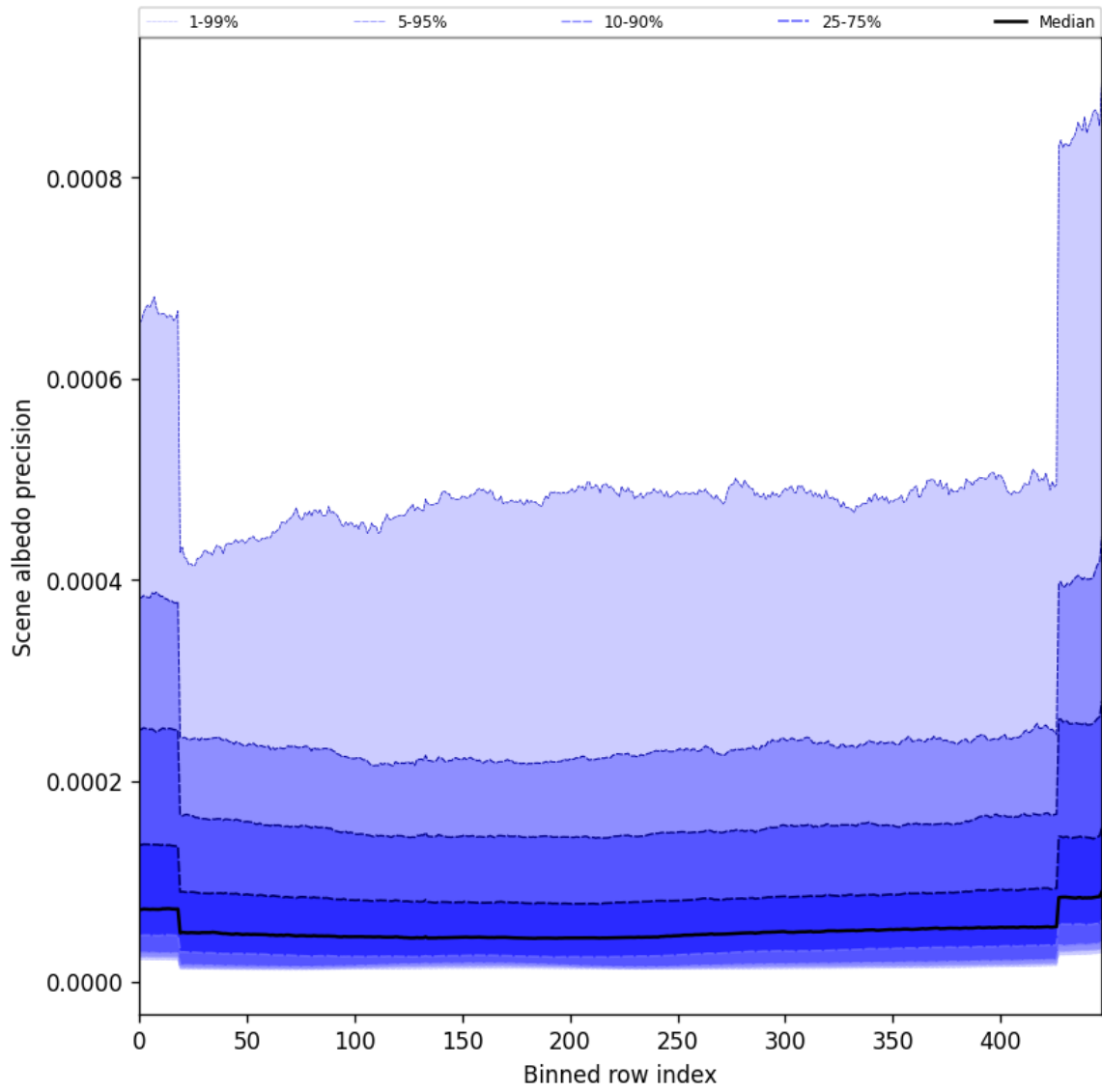
Figure 52: Along track statistics of “Scene albedo precision” for 2025-03-19 to 2025-03-21
