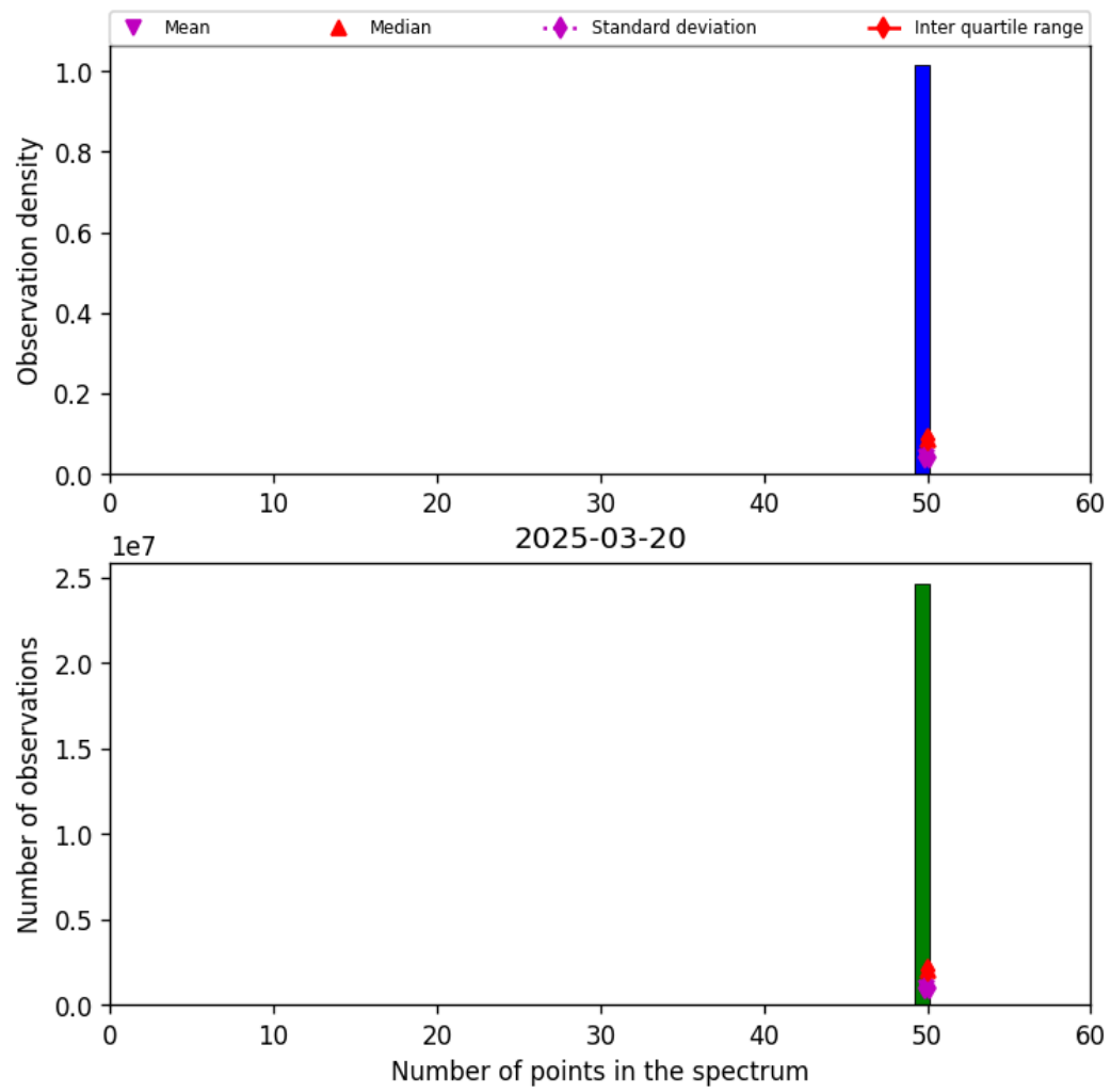
Figure 44: Histogram of "Number of points in the spectrum" for 2025-03-19 to 2025-03-21
