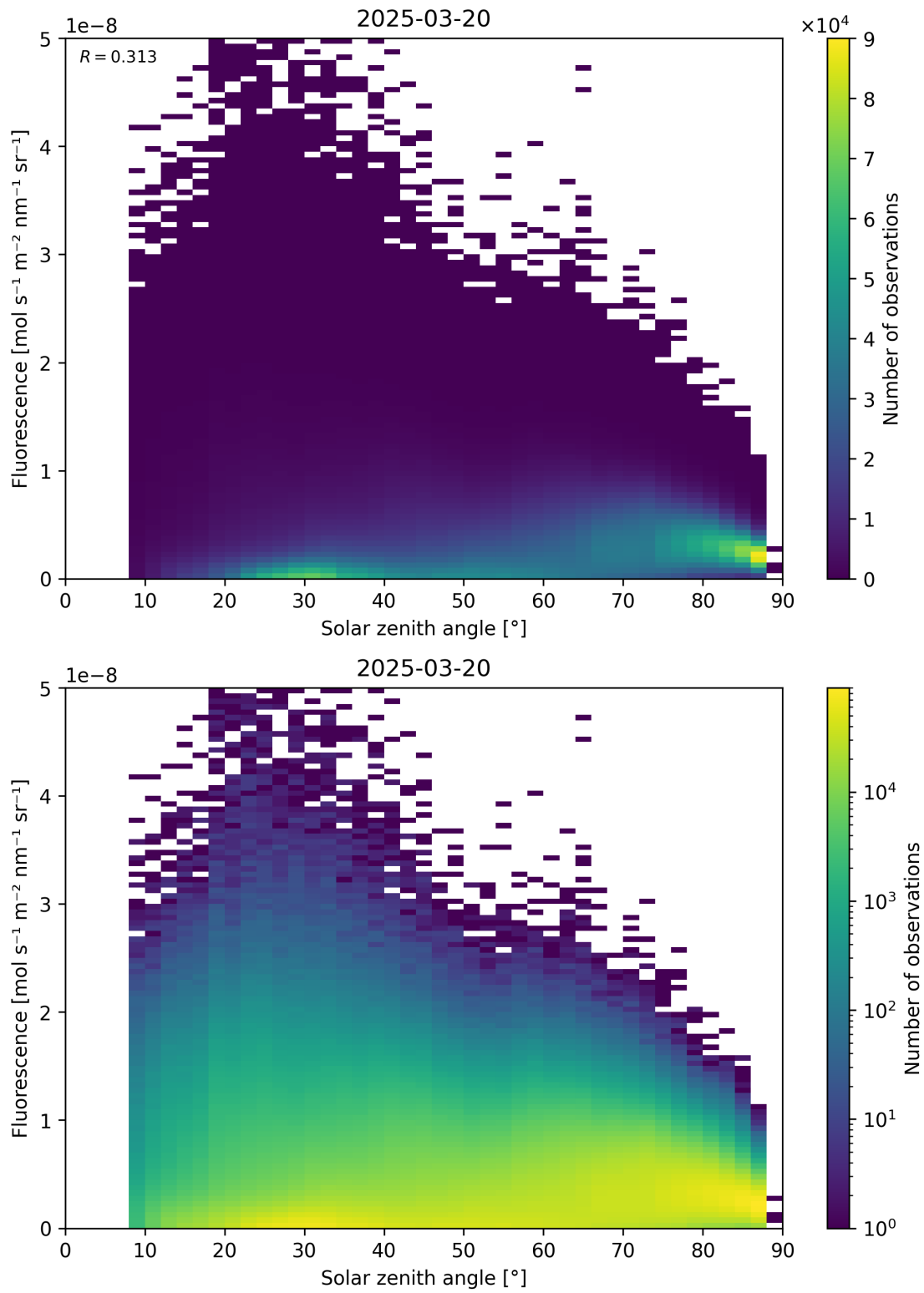
Figure 112: Scatter density plot of “Solar zenith angle” against “Fluorescence” for 2025-03-19 to 2025-03-21.
