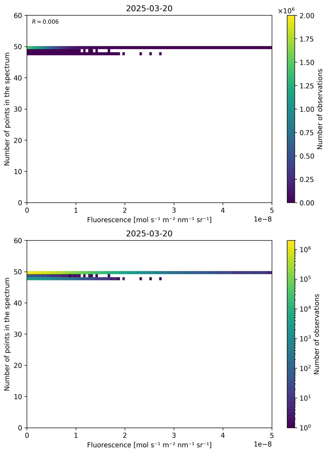
Figure 86: Scatter density plot of “Fluorescence” against “Number of points in the spectrum” for 2025-03-19 to 2025-03-21.
