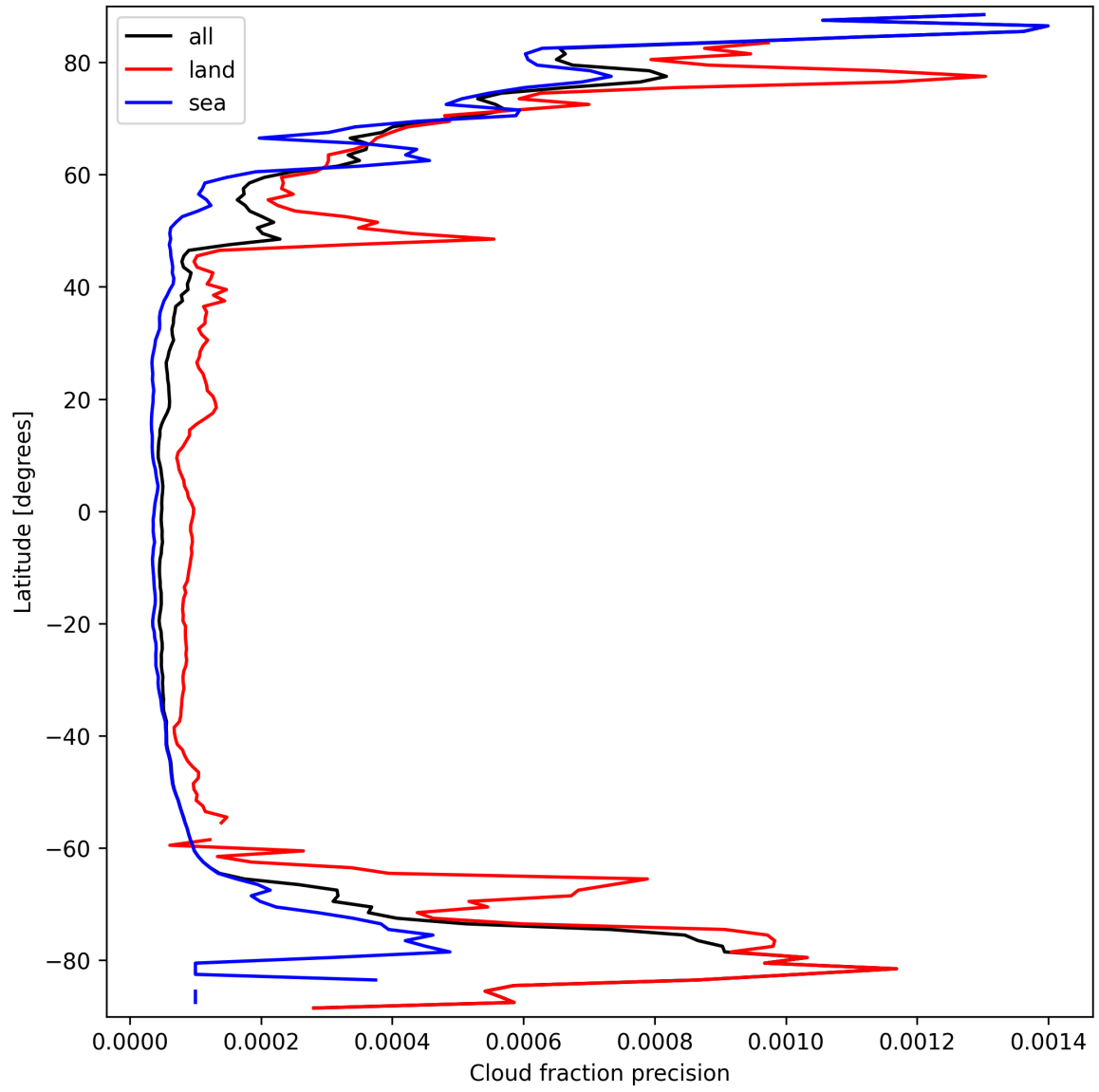
Figure 16: Zonal average of “Cloud fraction precision” for 2025-03-19 to 2025-03-21.
