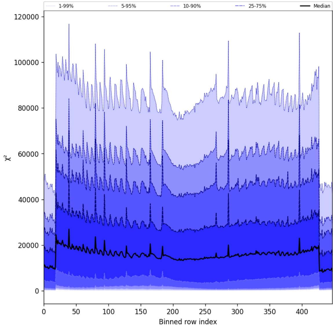
Figure 55: Along track statistics of “ \chi^2 ” for 2025-03-19 to 2025-03-21
