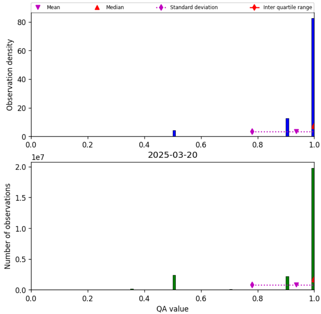
Figure 29: Histogram of “QA value” for 2025-03-19 to 2025-03-21
