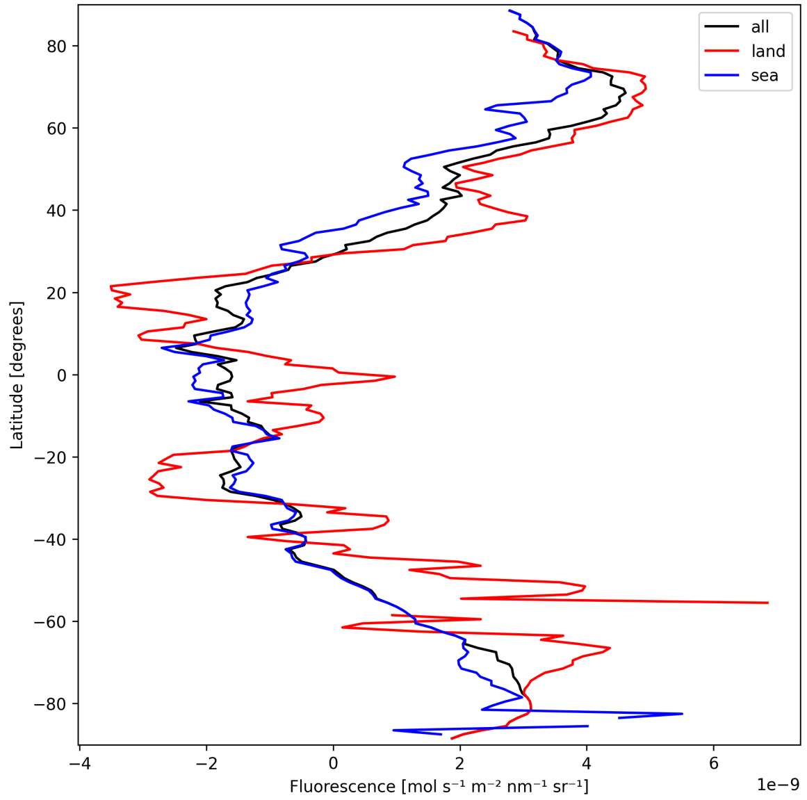
Figure 23: Zonal average of “Fluorescence” for 2025-03-19 to 2025-03-21.
