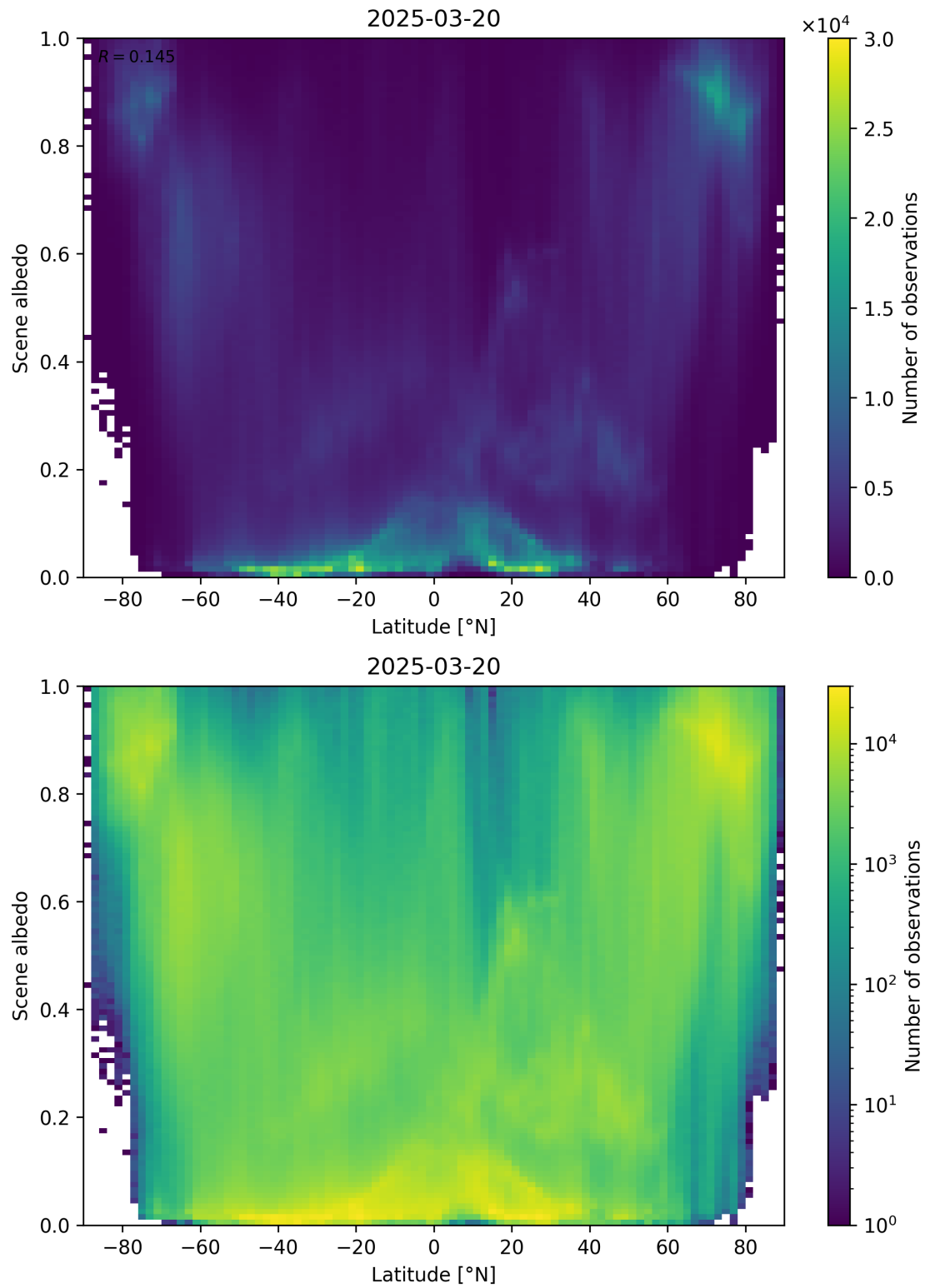
Figure 95: Scatter density plot of “Latitude” against “Scene albedo” for 2025-03-19 to 2025-03-21.
