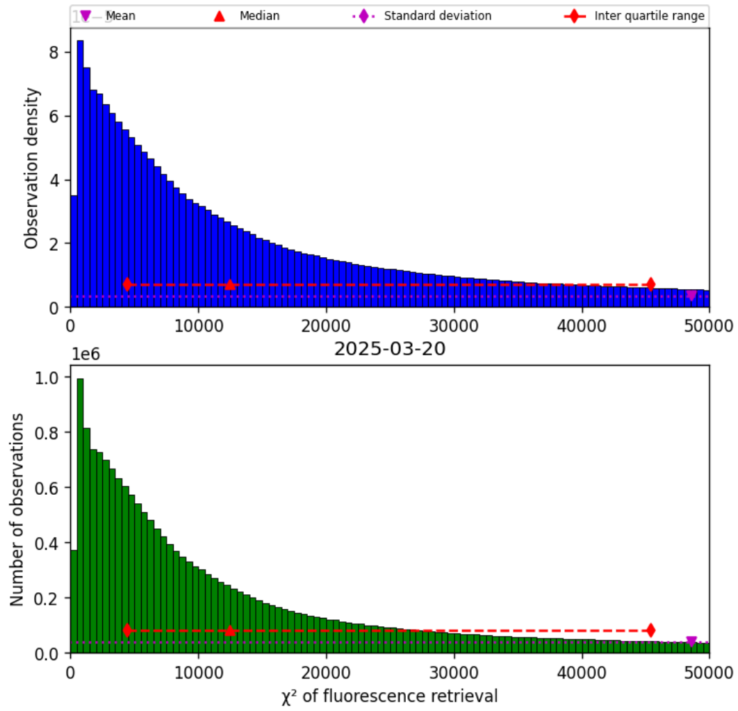
Figure 42: Histogram of “ \chi^2 of fluorescence retrieval” for 2025-03-19 to 2025-03-21
