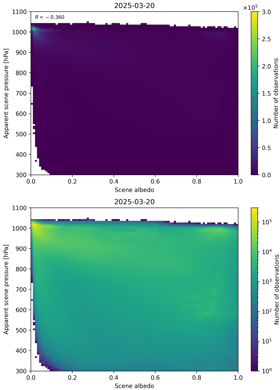
Figure 102: Scatter density plot of “Scene albedo” against “Apparent scene pressure” for 2025-03-19 to 2025-03-21.
