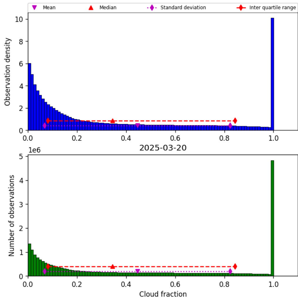
Figure 32: Histogram of “Cloud fraction” for 2025-03-19 to 2025-03-21
