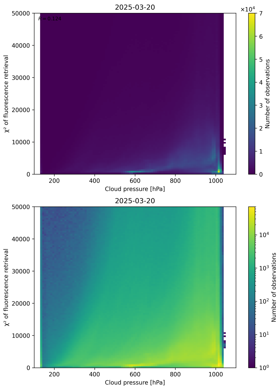
Figure 78: Scatter density plot of “Cloud pressure” against “ \chi^2 of fluorescence retrieval” for 2025-03-19 to 2025-03-21.
