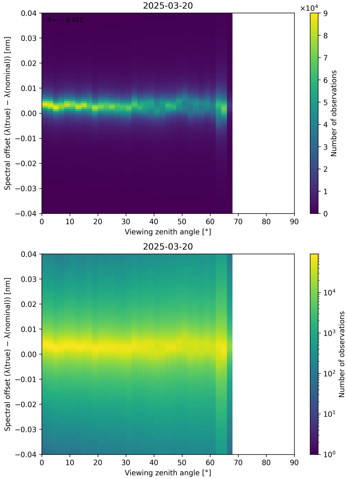
Figure 128: Scatter density plot of “Viewing zenith angle” against “Spectral offset ( \lambda_{\text{true}} - \lambda_{\text{nominal}} )” for 2025-03-19 to 2025-03-21.
