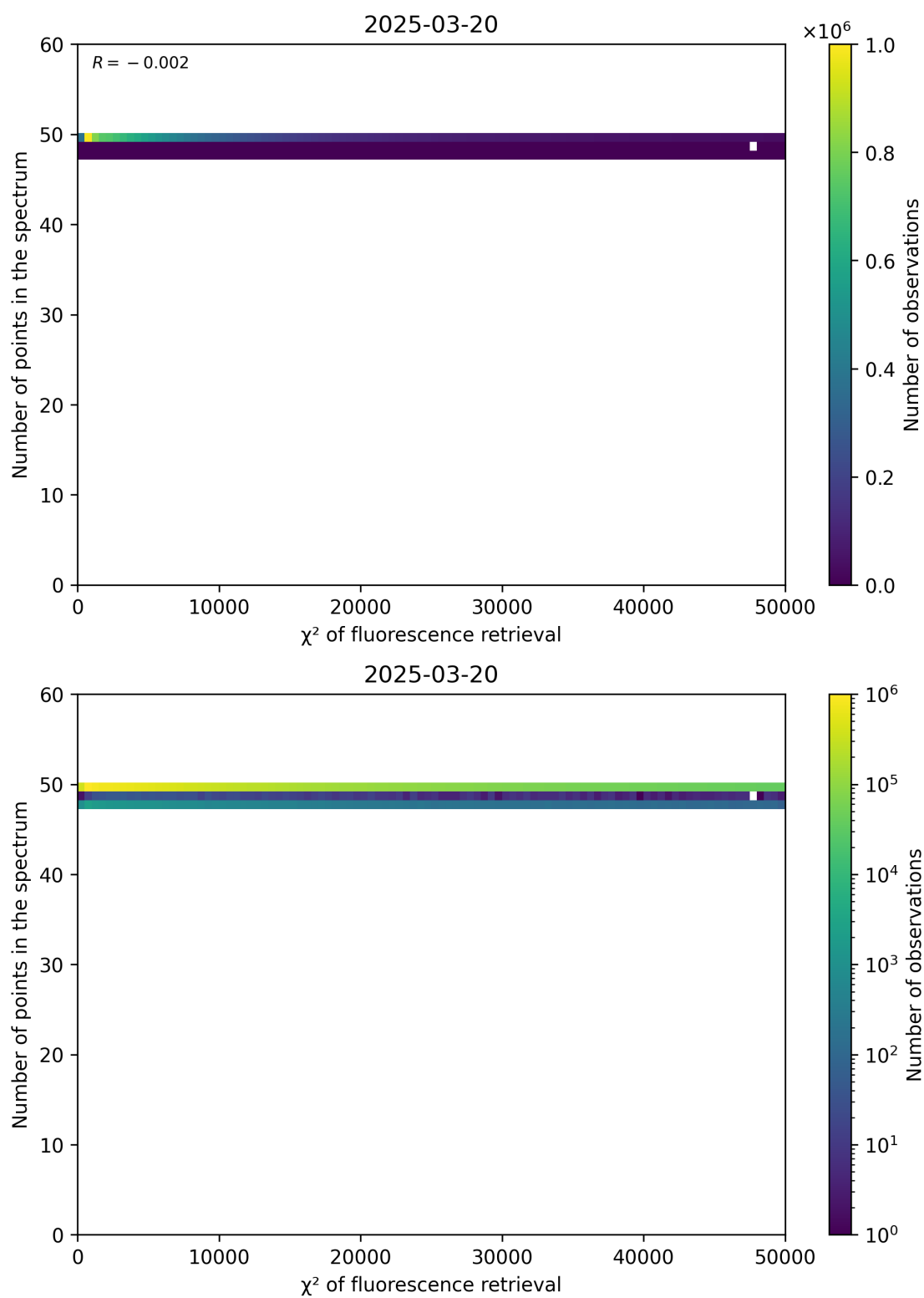
Figure 68: Scatter density plot of " \chi^2 of fluorescence retrieval" against "Number of points in the spectrum" for 2025-03-19 to 2025-03-21.
