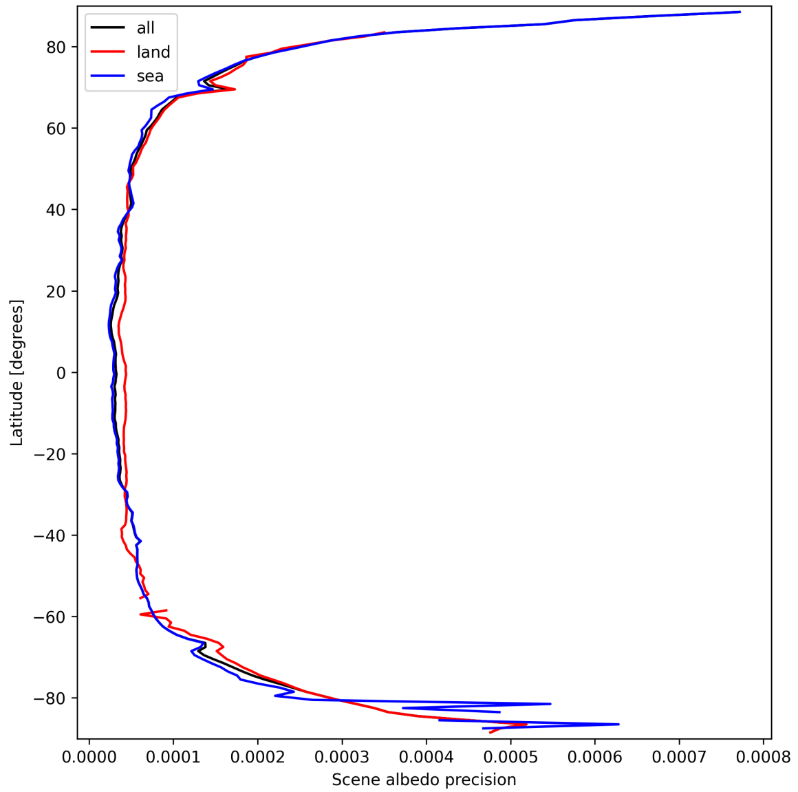
Figure 18: Zonal average of “Scene albedo precision” for 2025-03-19 to 2025-03-21.
