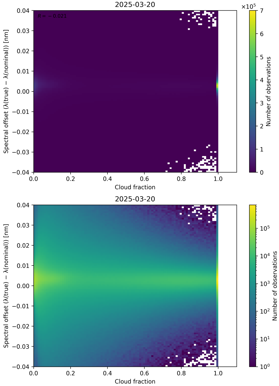
Figure 76: Scatter density plot of “Cloud fraction” against “Spectral offset ( \lambda_{\text{true}} - \lambda_{\text{nominal}} )” for 2025-03-19 to 2025-03-21.
