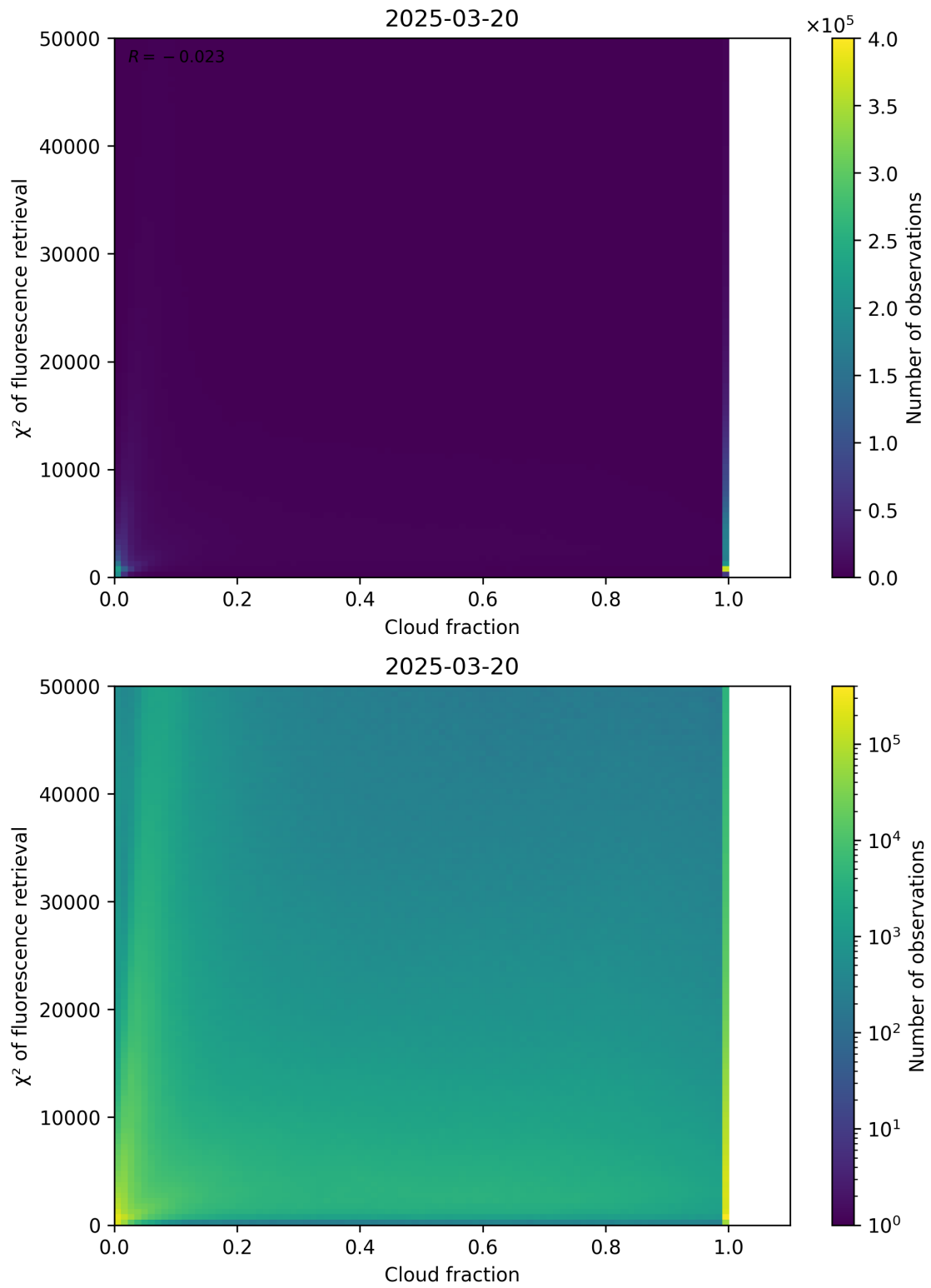
Figure 71: Scatter density plot of “Cloud fraction” against “ \chi^2 of fluorescence retrieval” for 2025-03-19 to 2025-03-21.
