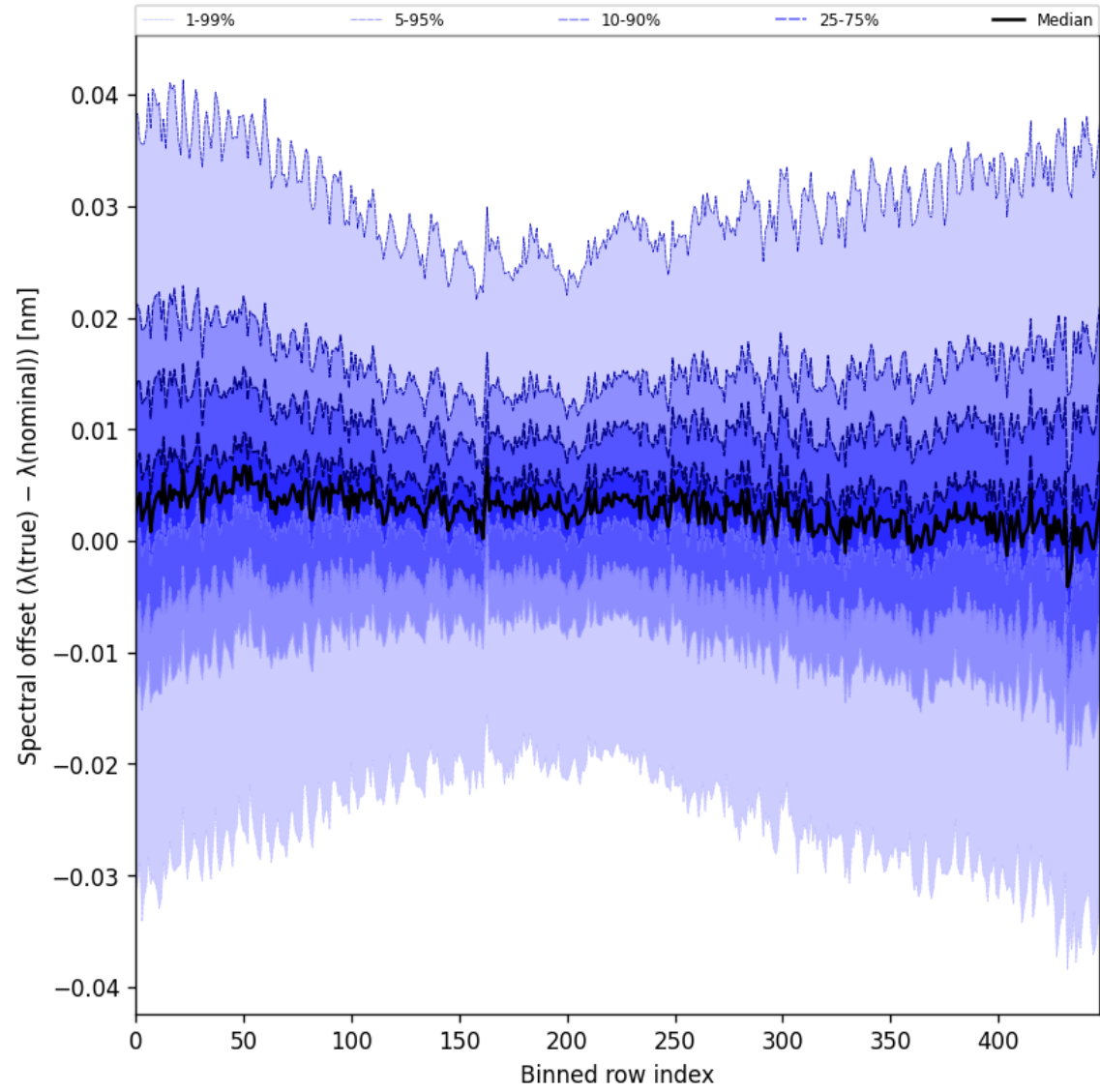
Figure 62: Along track statistics of “Spectral offset ( \lambda_{\text{true}} - \lambda_{\text{nominal}} )” for 2025-03-19 to 2025-03-21
