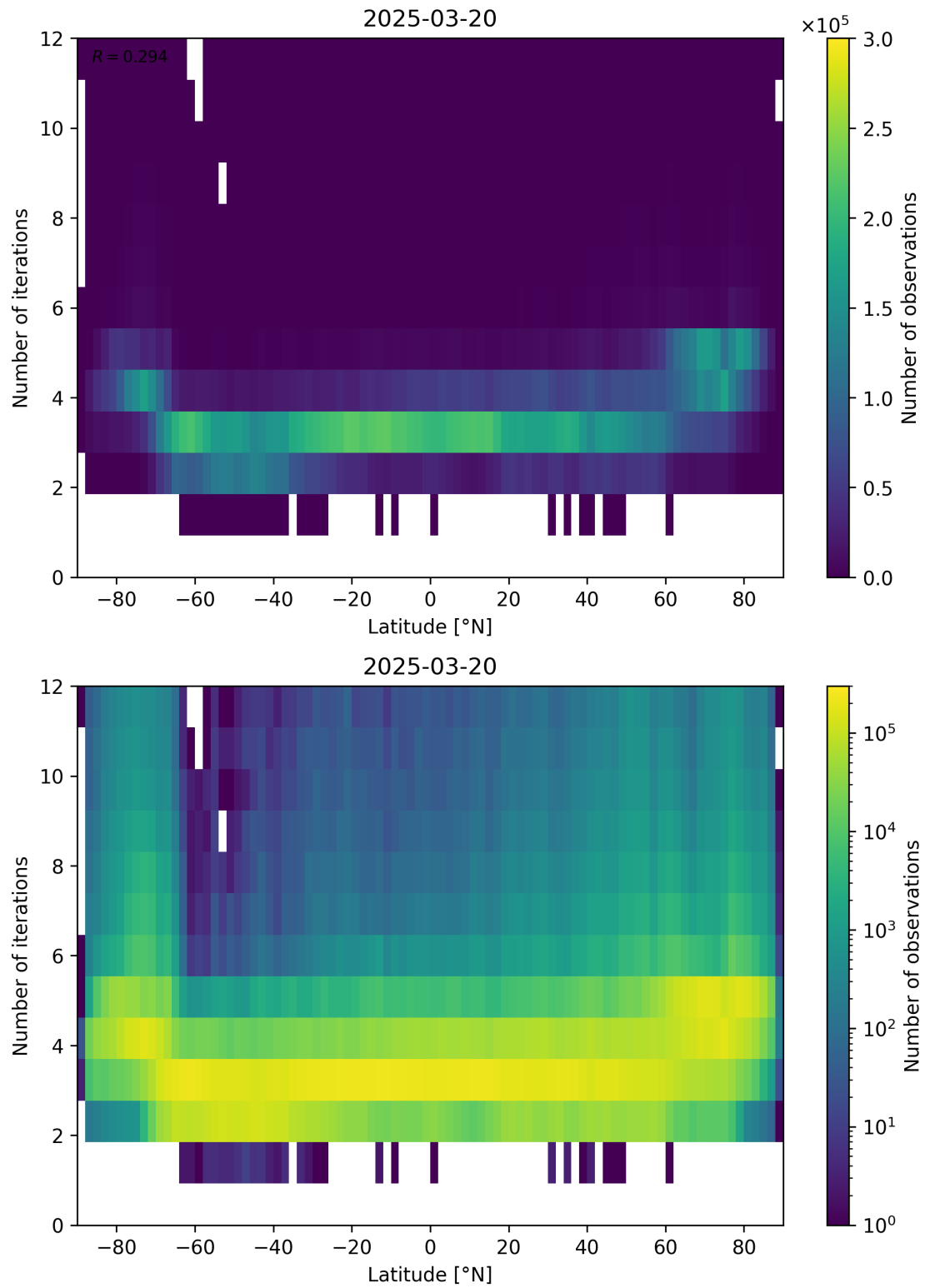
Figure 93: Scatter density plot of “Latitude” against “Number of iterations” for 2025-03-19 to 2025-03-21.
