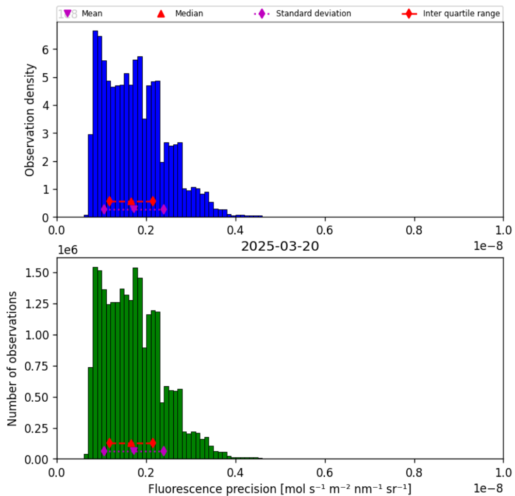
Figure 41: Histogram of “Fluorescence precision” for 2025-03-19 to 2025-03-21
