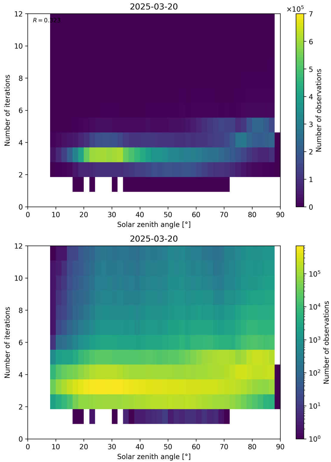
Figure 114: Scatter density plot of “Solar zenith angle” against “Number of iterations” for 2025-03-19 to 2025-03-21.
