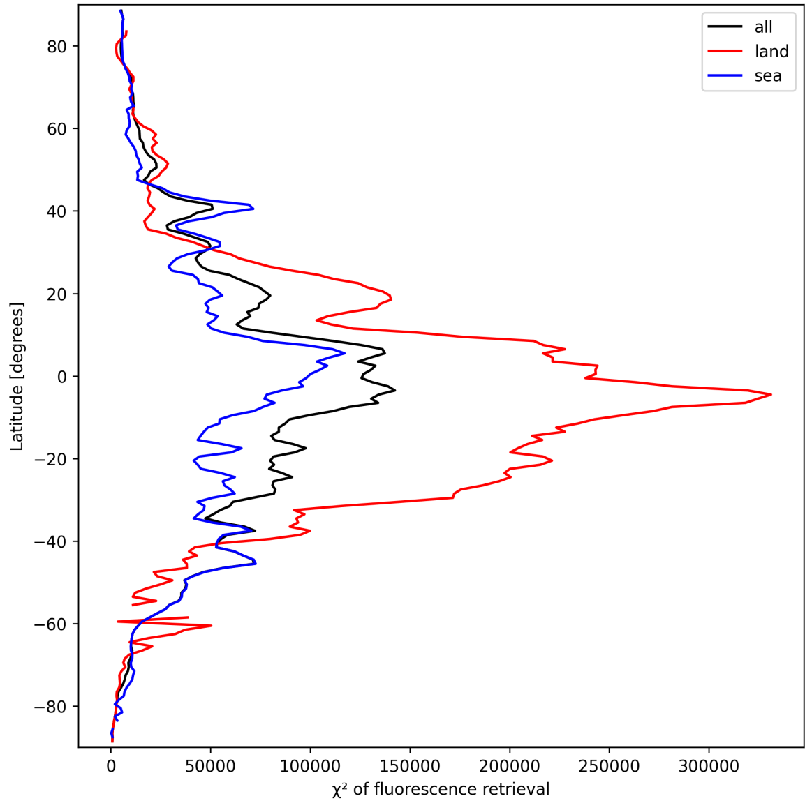
Figure 25: Zonal average of “ \chi^2 of fluorescence retrieval” for 2025-03-19 to 2025-03-21.
