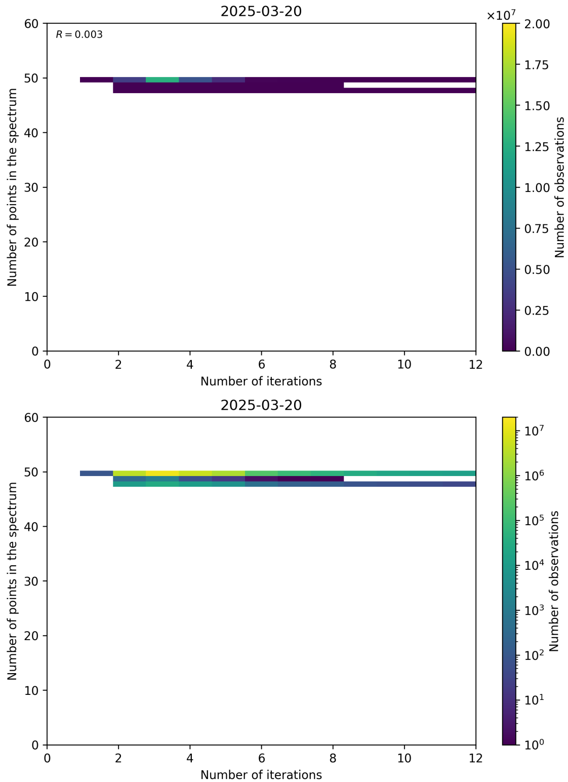
Figure 99: Scatter density plot of “Number of iterations” against “Number of points in the spectrum” for 2025-03-19 to 2025-03-21.
