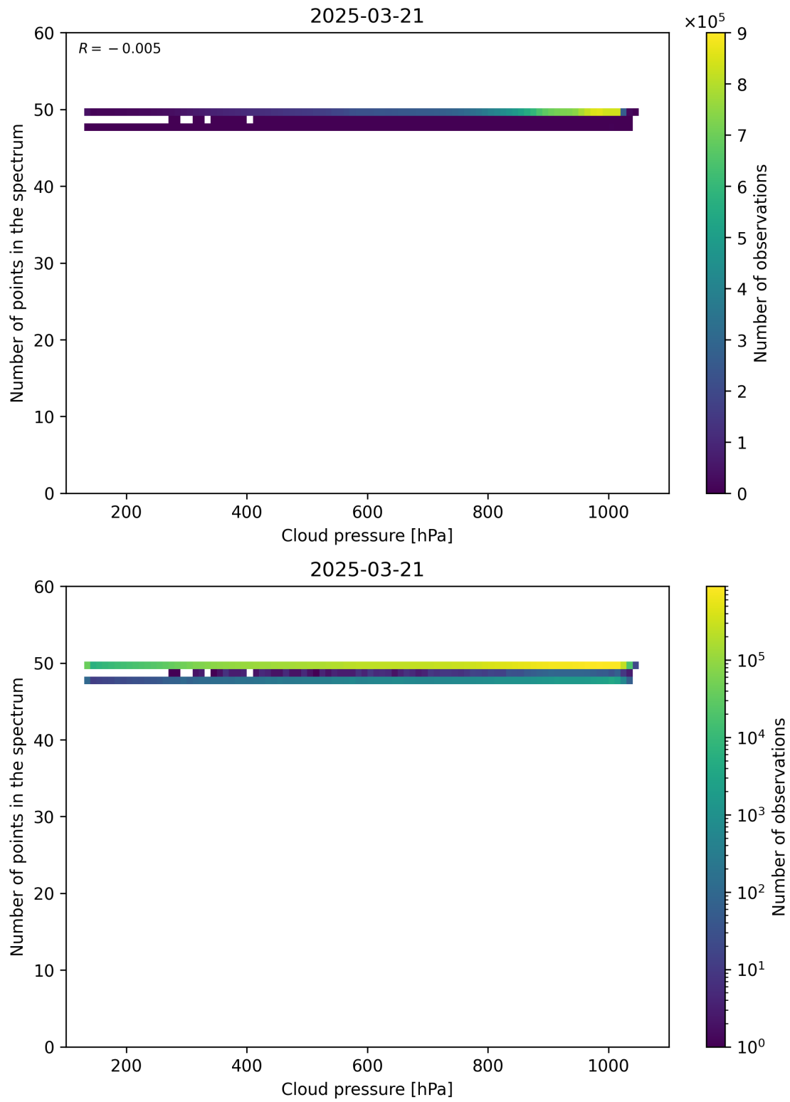
Figure 82: Scatter density plot of “Cloud pressure” against “Number of points in the spectrum” for 2025-03-20 to 2025-03-22.
