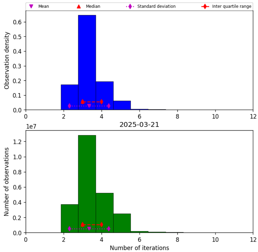
Figure 39: Histogram of “Number of iterations” for 2025-03-20 to 2025-03-22
