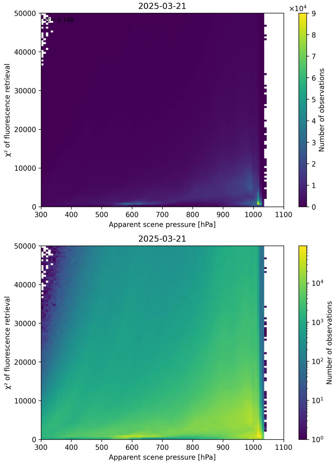
Figure 63: Scatter density plot of “Apparent scene pressure” against “ \chi^2 of fluorescence retrieval” for 2025-03-20 to 2025-03-22.
