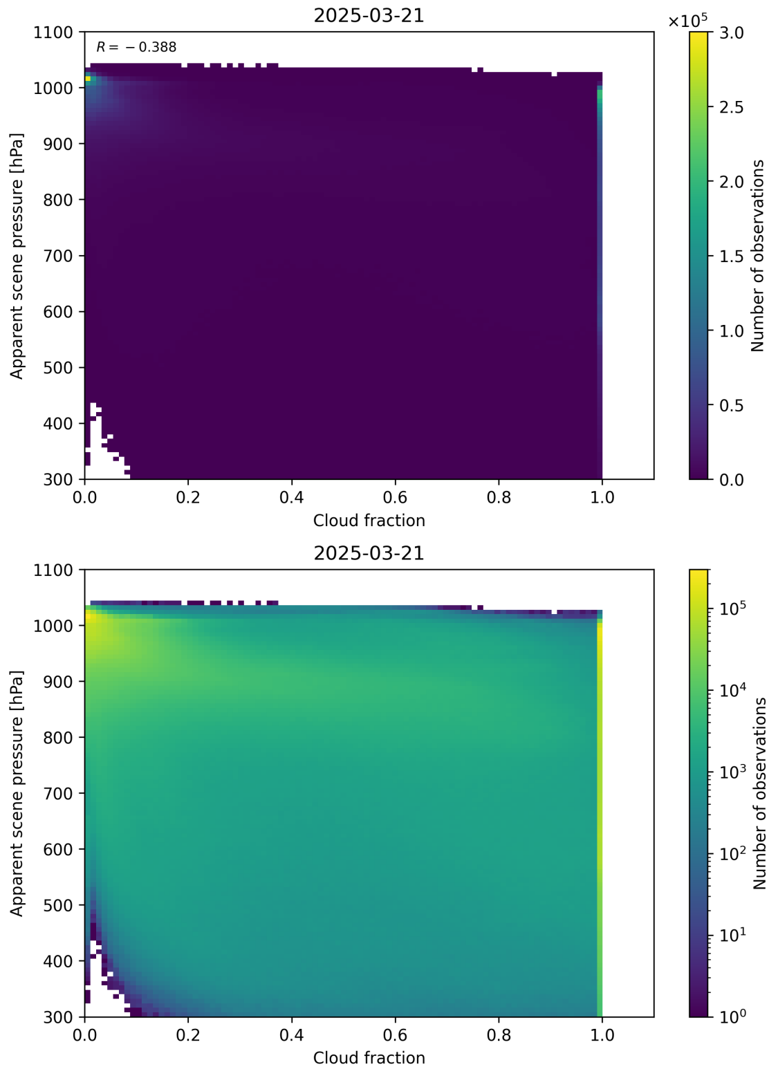
Figure 70: Scatter density plot of “Cloud fraction” against “Apparent scene pressure” for 2025-03-20 to 2025-03-22.
