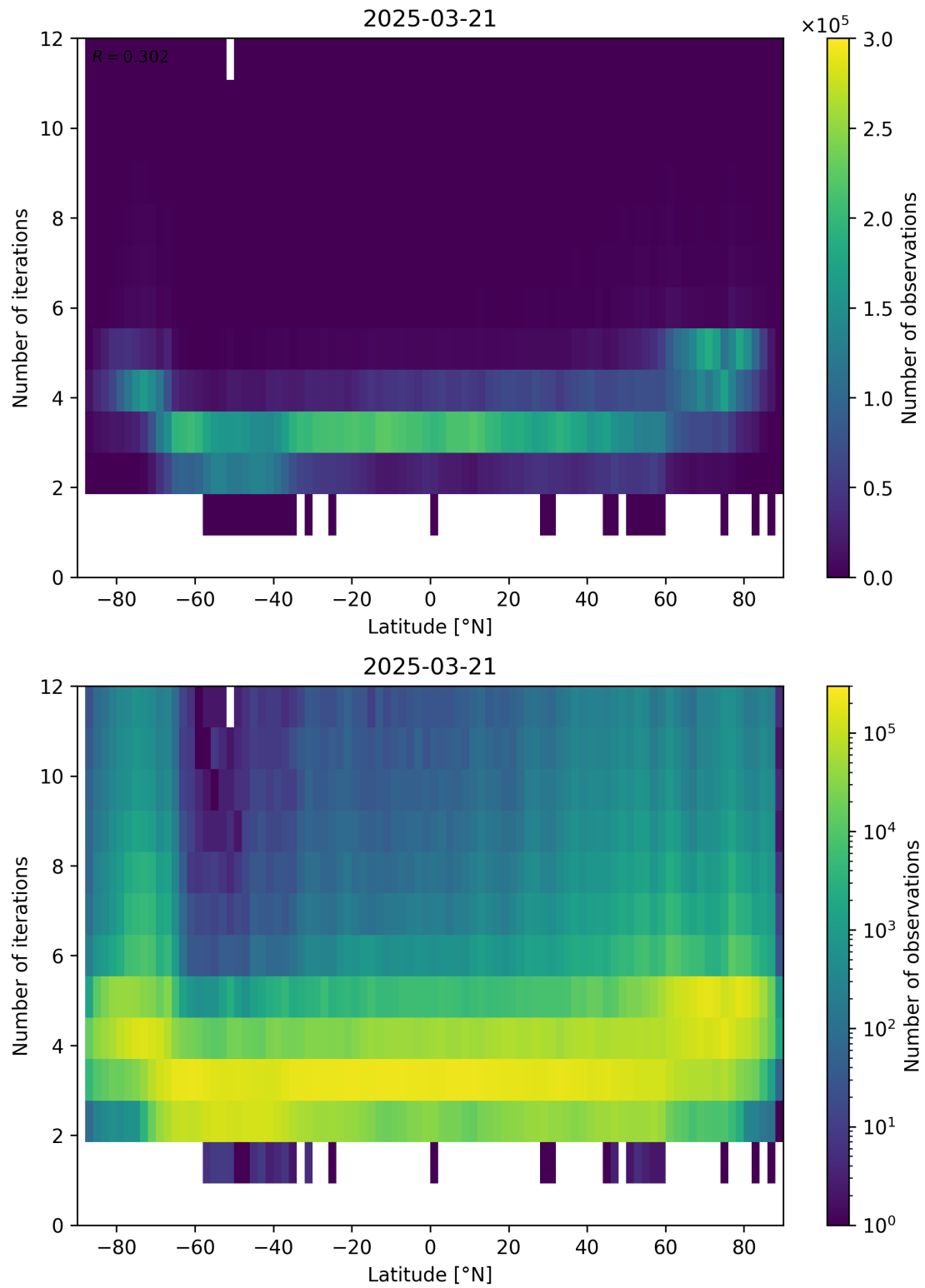
Figure 93: Scatter density plot of “Latitude” against “Number of iterations” for 2025-03-20 to 2025-03-22.
