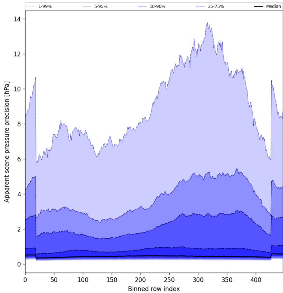
Figure 54: Along track statistics of “Apparent scene pressure precision” for 2025-03-20 to 2025-03-22
