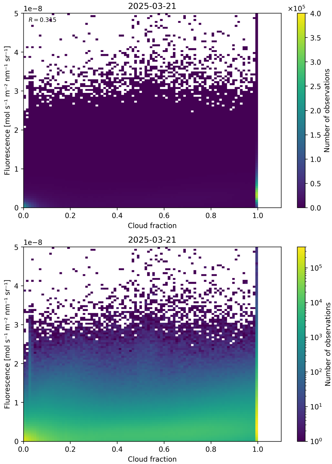
Figure 72: Scatter density plot of “Cloud fraction” against “Fluorescence” for 2025-03-20 to 2025-03-22.
