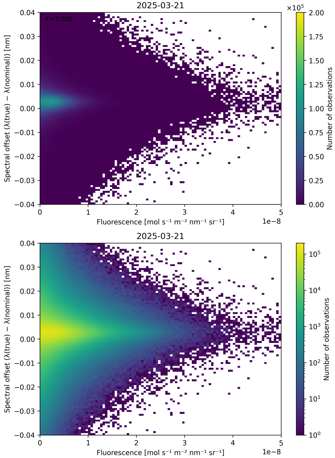
Figure 87: Scatter density plot of “Fluorescence” against “Spectral offset ( \lambda_{\text{true}} - \lambda_{\text{nominal}} )” for 2025-03-20 to 2025-03-22.
