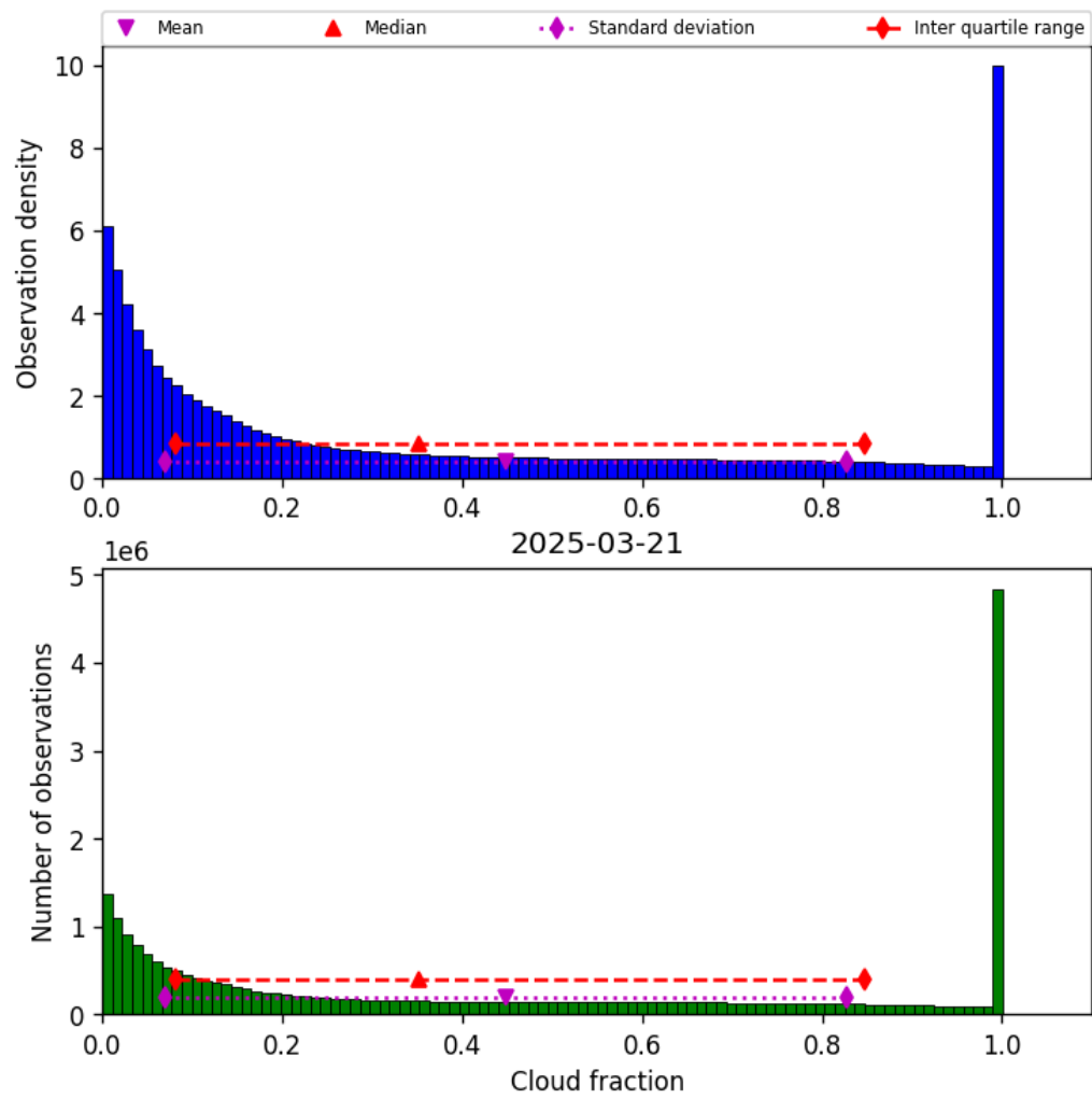
Figure 32: Histogram of “Cloud fraction” for 2025-03-20 to 2025-03-22
