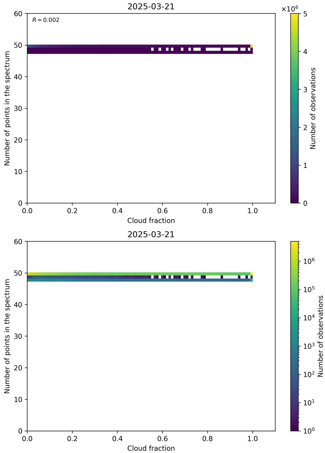
Figure 74: Scatter density plot of “Cloud fraction” against “Number of points in the spectrum” for 2025-03-20 to 2025-03-22.
