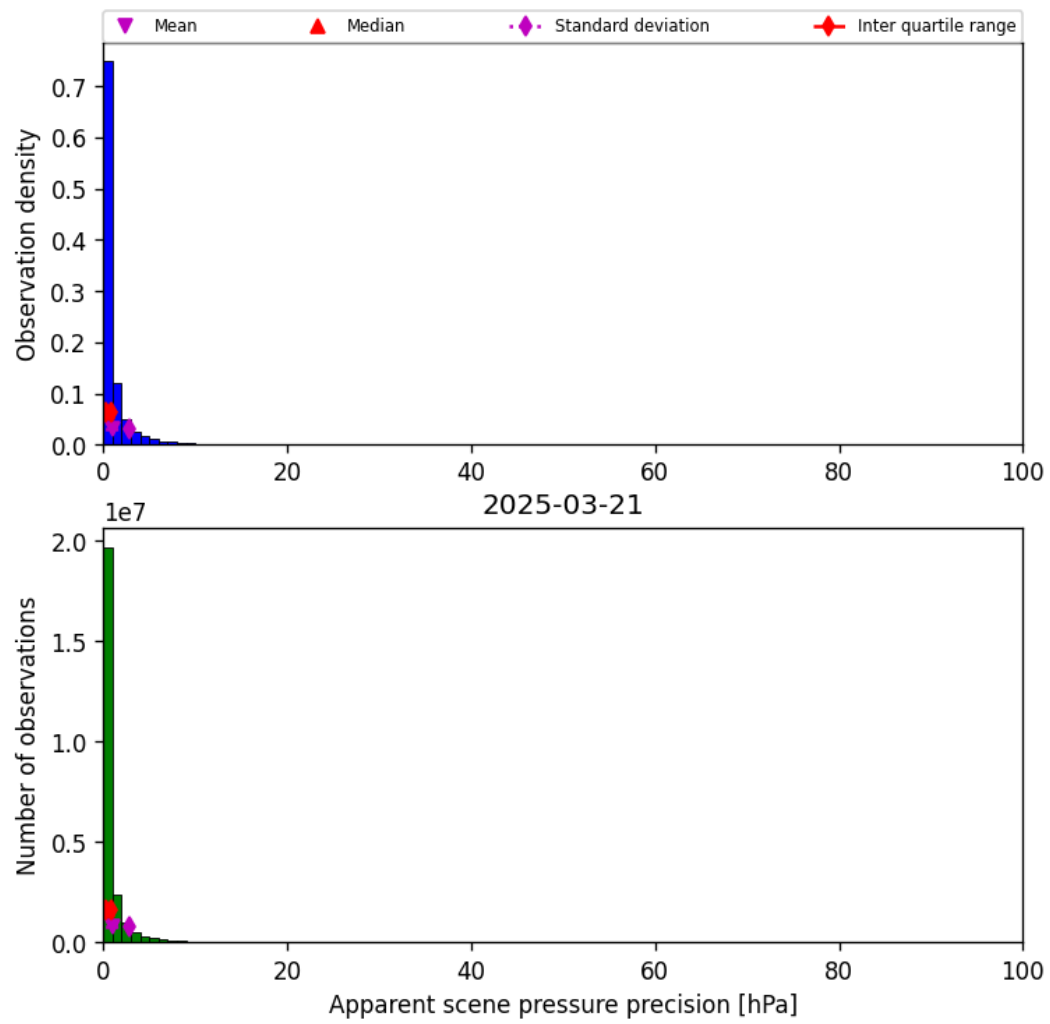
Figure 37: Histogram of “Apparent scene pressure precision” for 2025-03-20 to 2025-03-22
