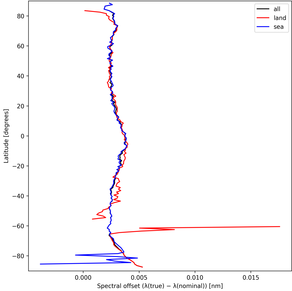
Figure 28: Zonal average of “Spectral offset ( \lambda_{\text{true}} - \lambda_{\text{nominal}} )” for 2025-03-20 to 2025-03-22.
