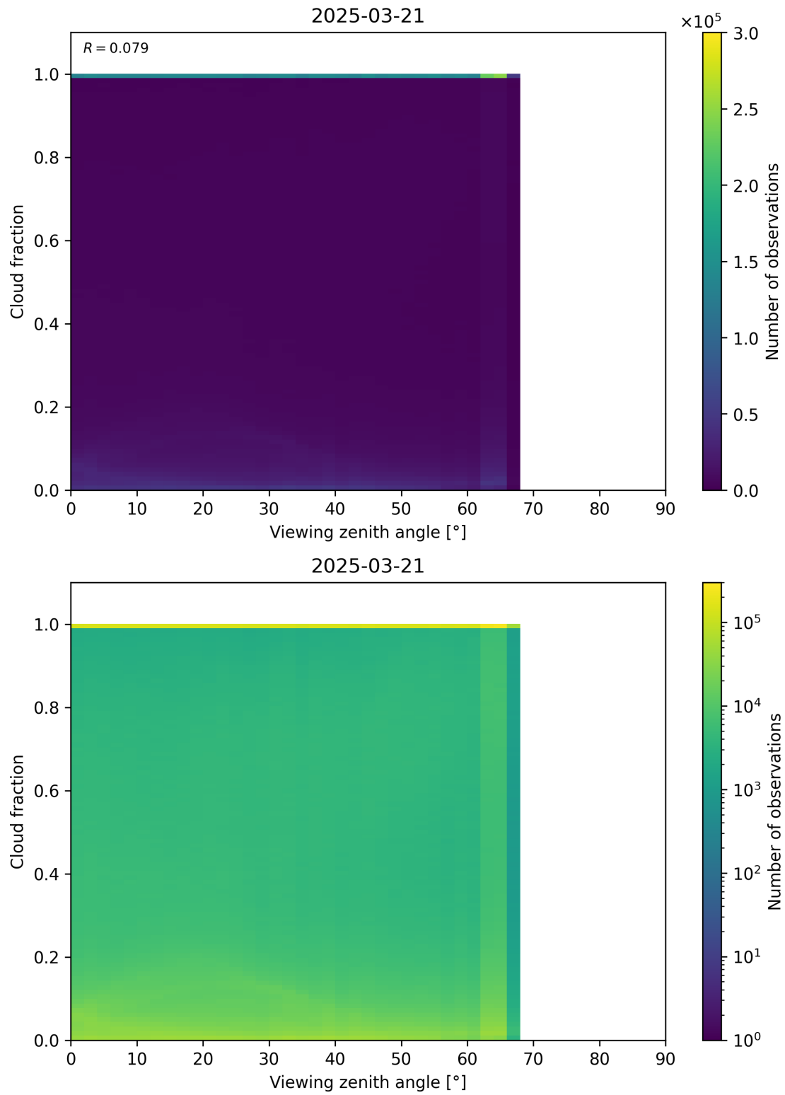
Figure 120: Scatter density plot of “Viewing zenith angle” against “Cloud fraction” for 2025-03-20 to 2025-03-22.
