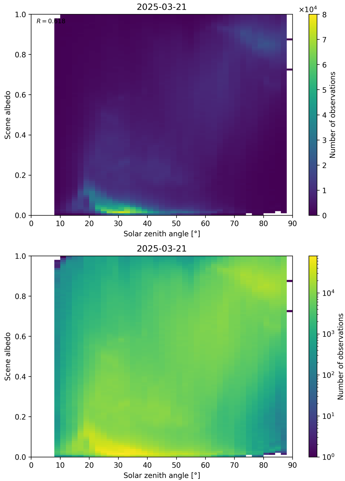
Figure 116: Scatter density plot of “Solar zenith angle” against “Scene albedo” for 2025-03-20 to 2025-03-22.
