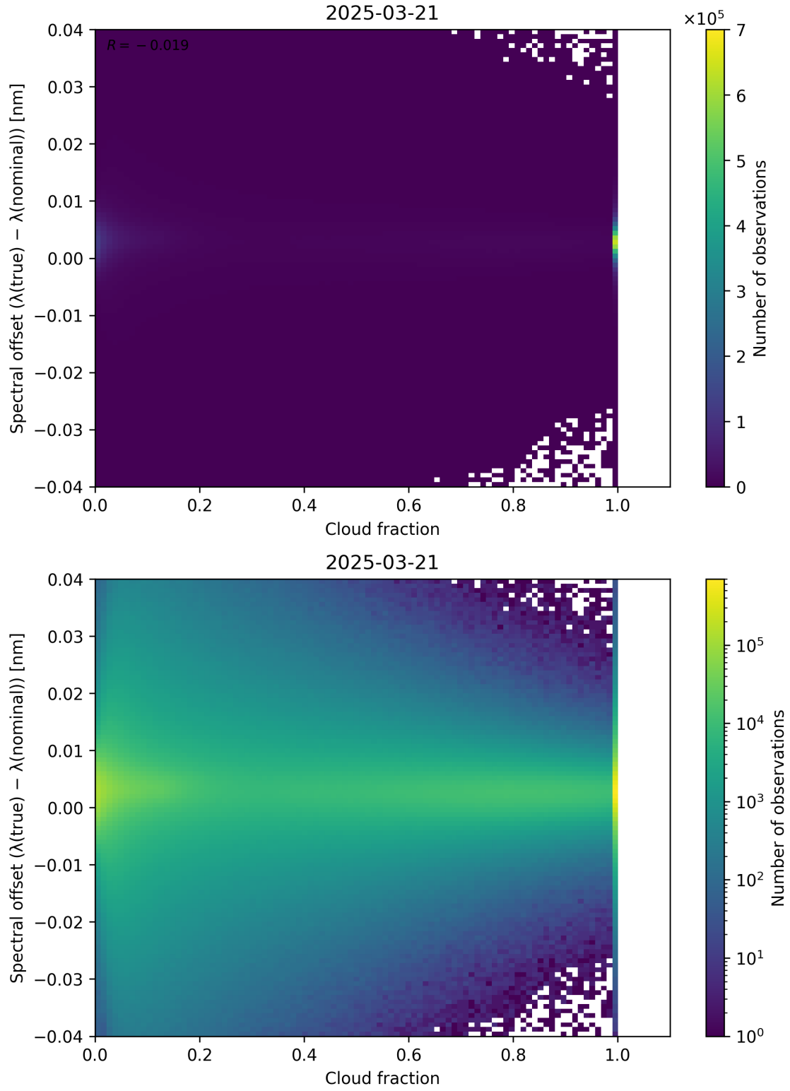
Figure 76: Scatter density plot of “Cloud fraction” against “Spectral offset ( \lambda_{\text{true}} - \lambda_{\text{nominal}} )” for 2025-03-20 to 2025-03-22.
