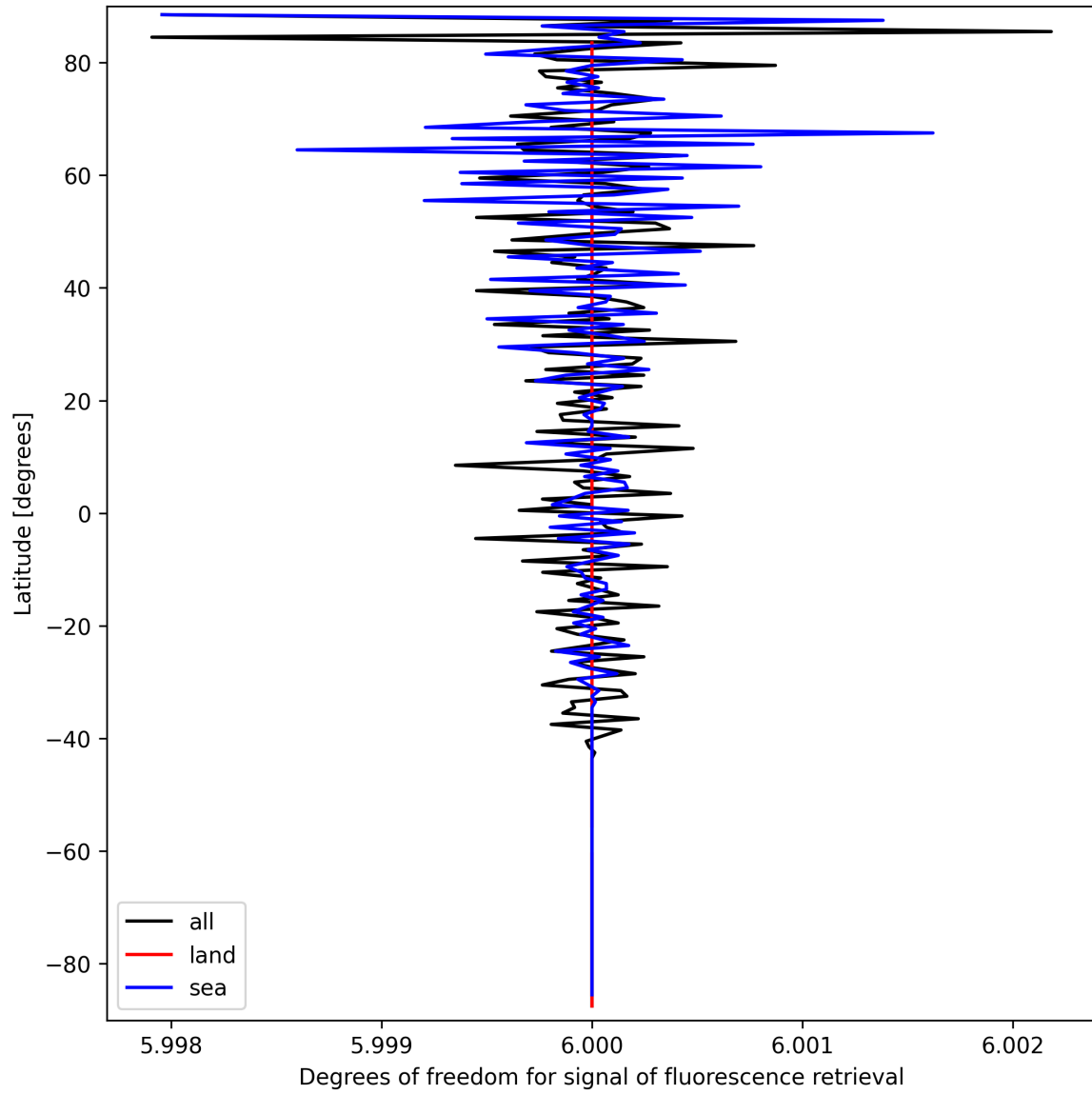
Figure 26: Zonal average of “Degrees of freedom for signal of fluorescence retrieval” for 2025-03-20 to 2025-03-22.
