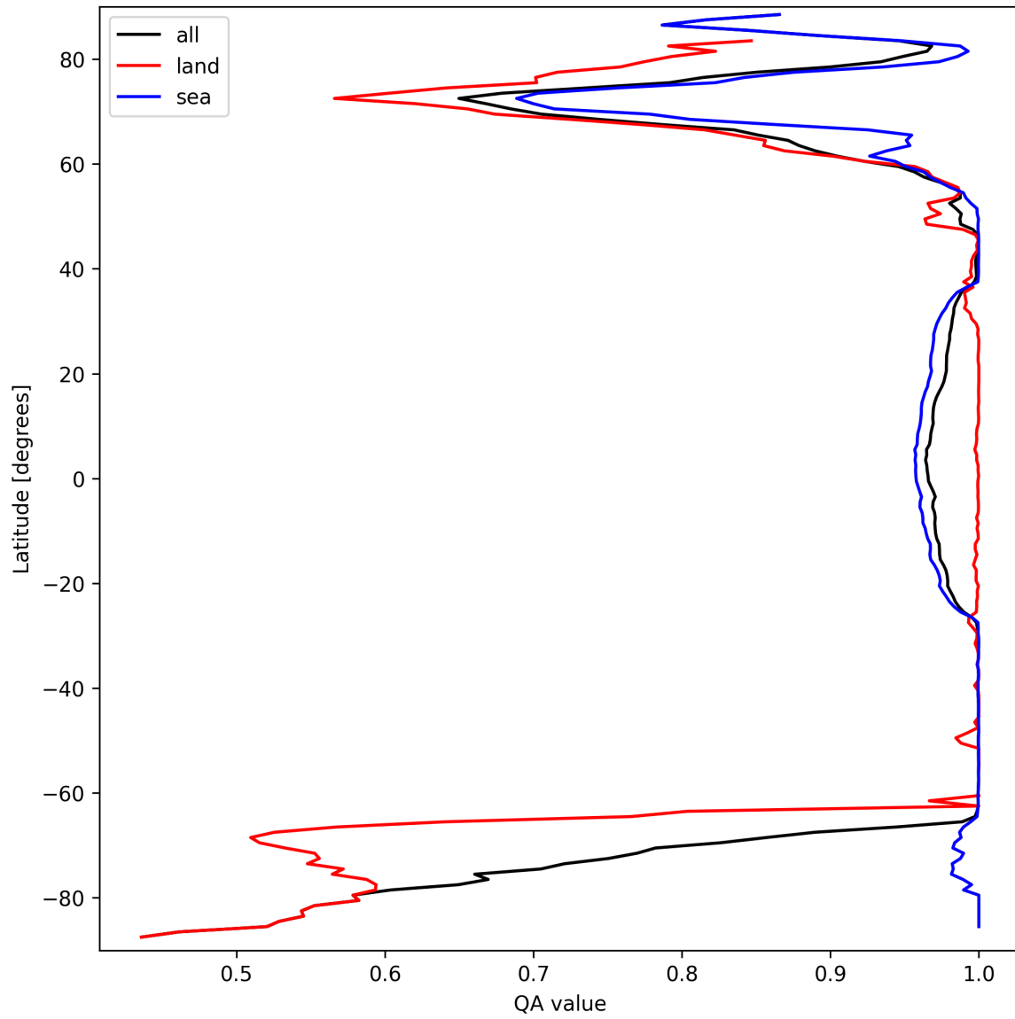
Figure 12: Zonal average of “QA value” for 2025-03-20 to 2025-03-22.
