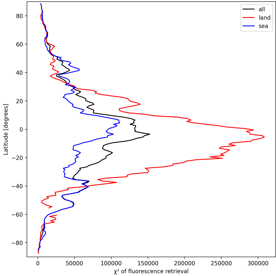
Figure 25: Zonal average of “ \chi^2 of fluorescence retrieval” for 2025-03-20 to 2025-03-22.
