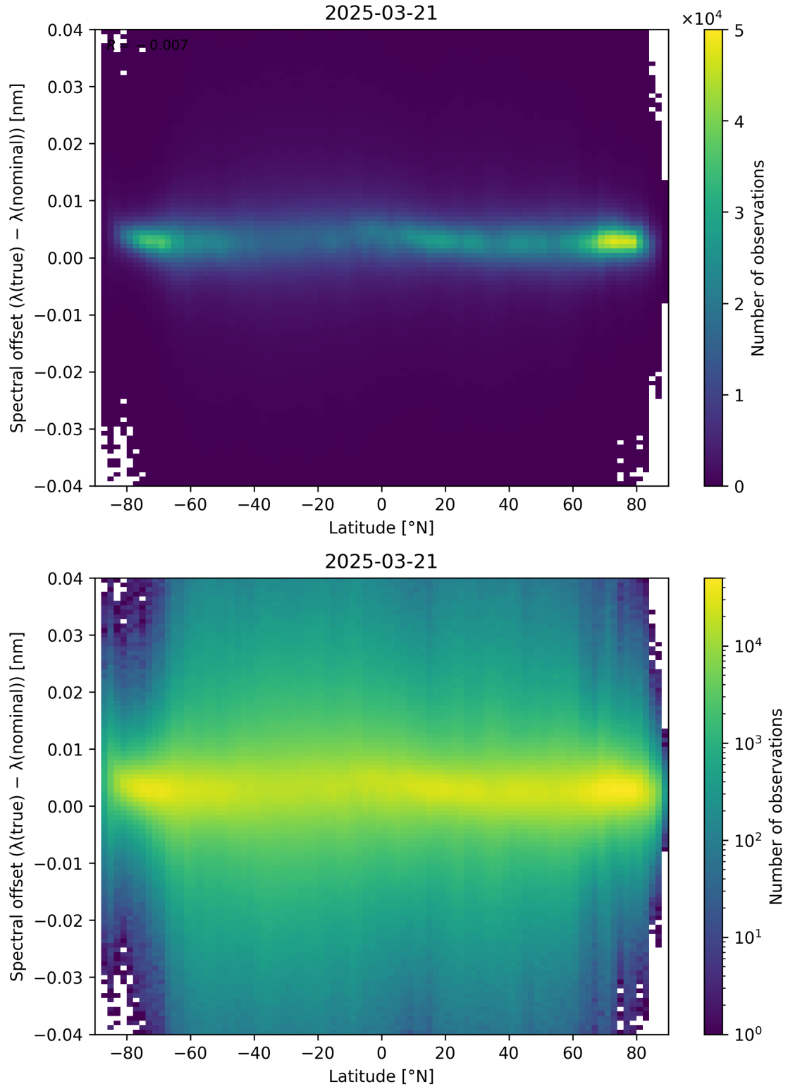
Figure 96: Scatter density plot of “Latitude” against “Spectral offset ( \lambda_{\text{true}} - \lambda_{\text{nominal}} )” for 2025-03-20 to 2025-03-22.
