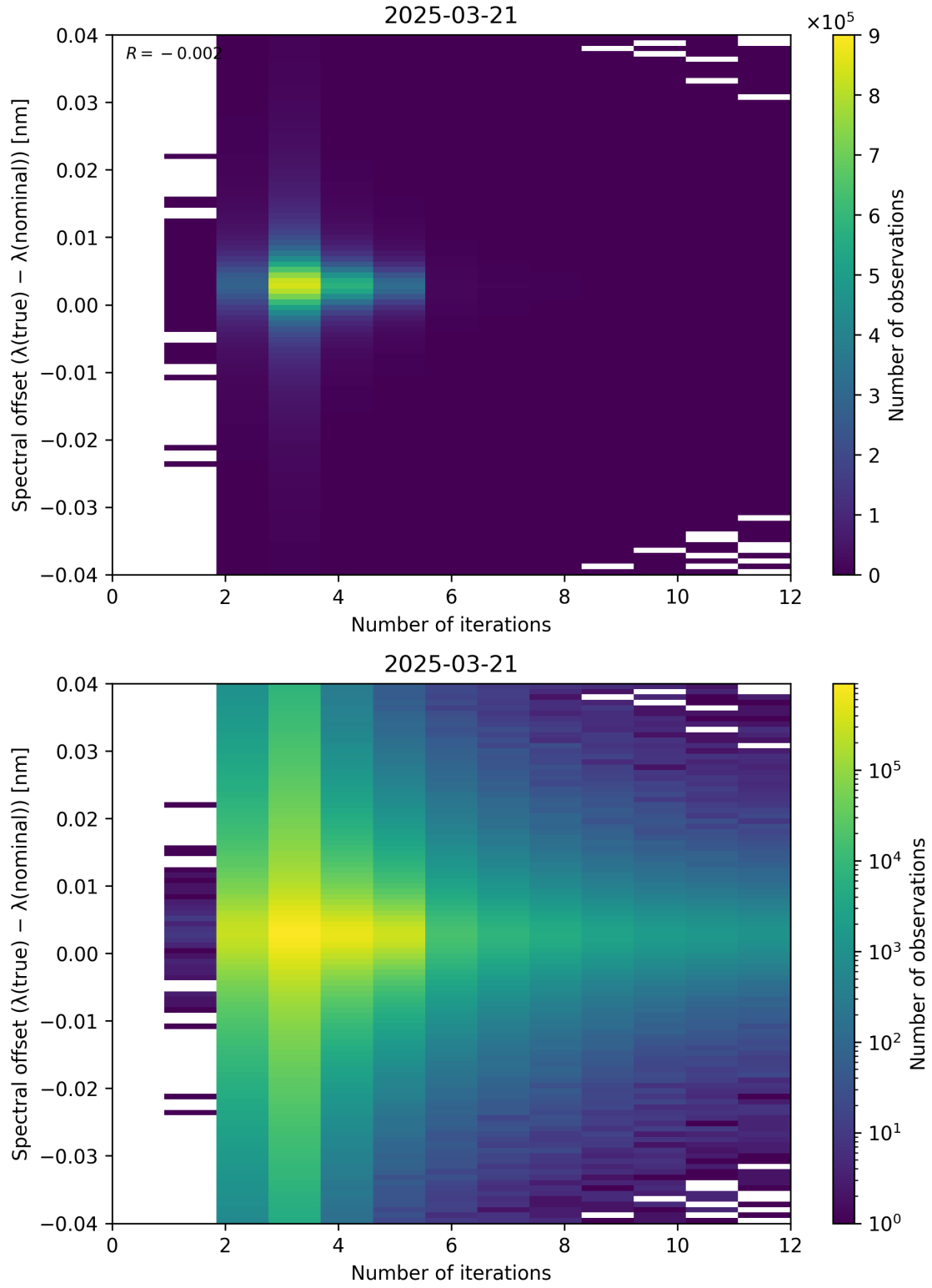
Figure 100: Scatter density plot of “Number of iterations” against “Spectral offset ( \lambda_{\text{true}} - \lambda_{\text{nominal}} )” for 2025-03-20 to 2025-03-22.
