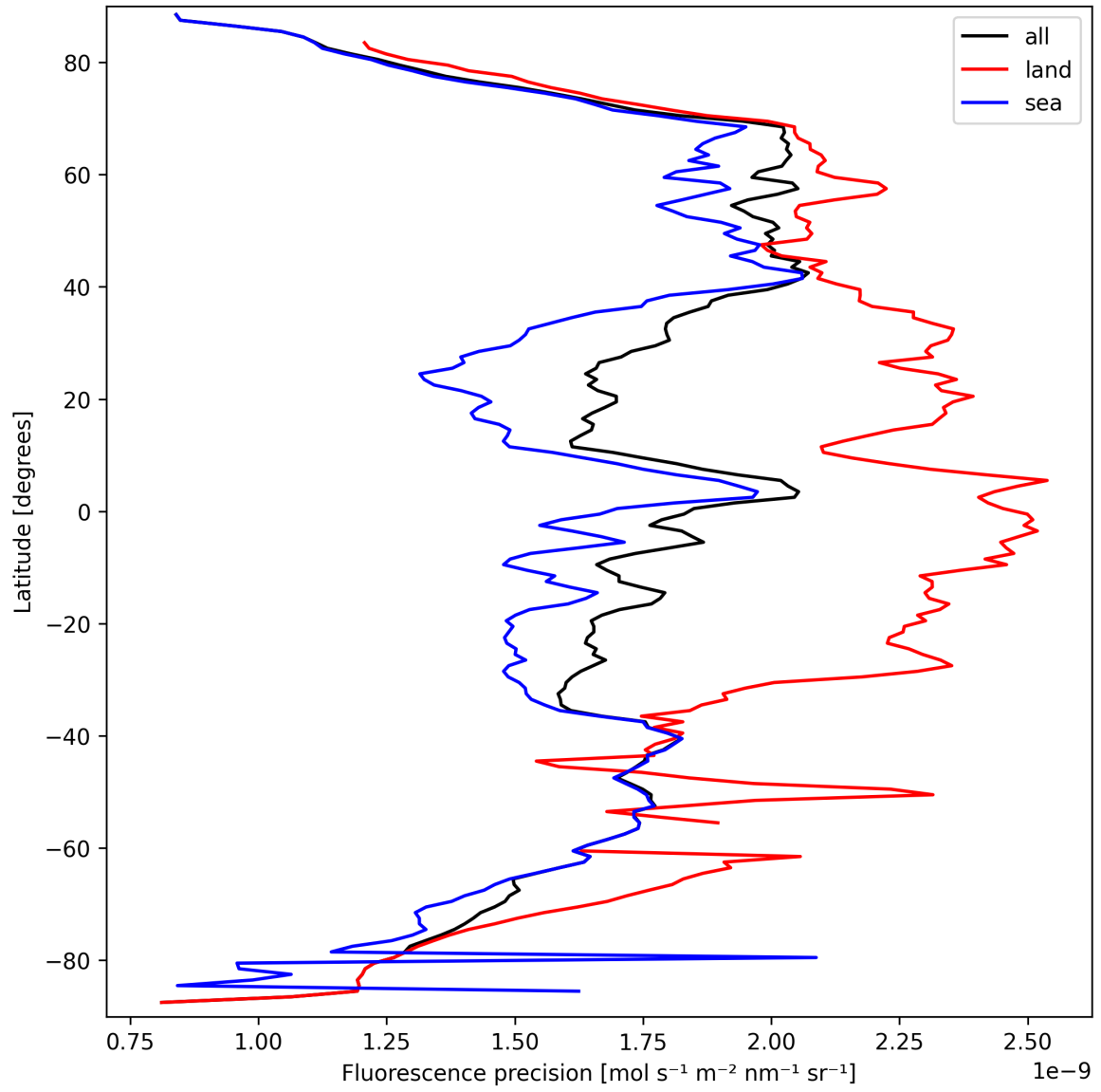
Figure 24: Zonal average of “Fluorescence precision” for 2025-03-20 to 2025-03-22.
