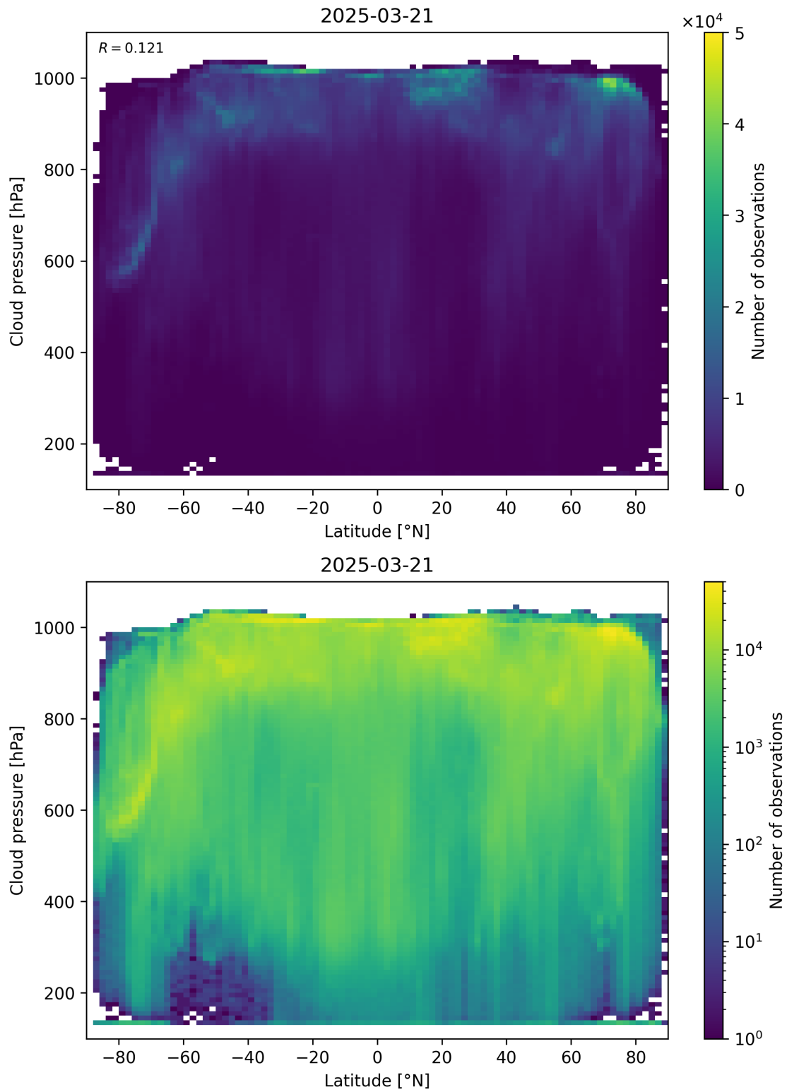
Figure 91: Scatter density plot of “Latitude” against “Cloud pressure” for 2025-03-20 to 2025-03-22.
