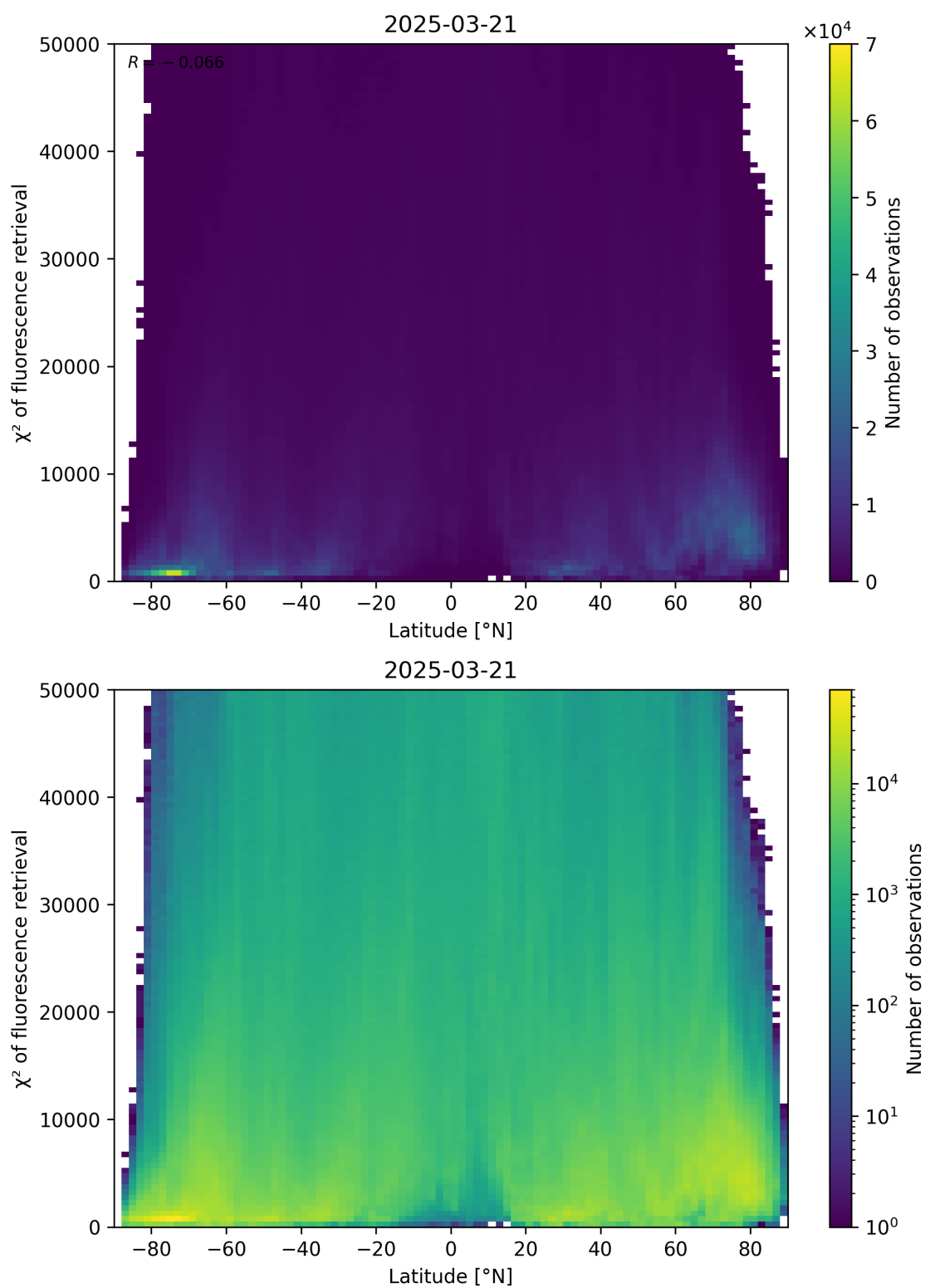
Figure 89: Scatter density plot of “Latitude” against “ \chi^2 of fluorescence retrieval” for 2025-03-20 to 2025-03-22.
