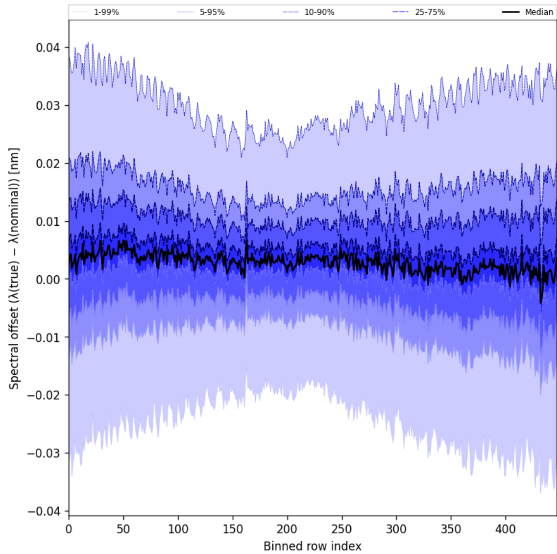
Figure 62: Along track statistics of “Spectral offset ( \lambda_{\text{true}} - \lambda_{\text{nominal}} )” for 2025-03-20 to 2025-03-22
