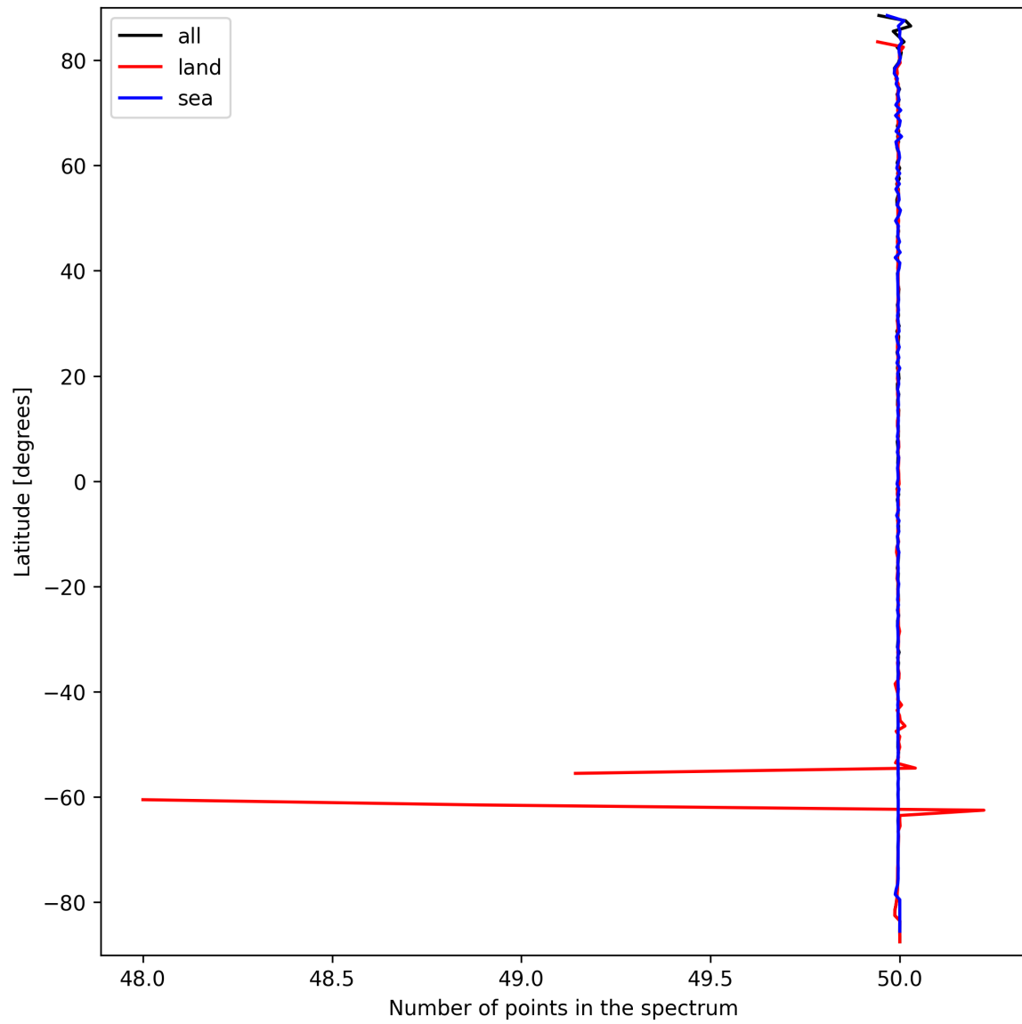
Figure 27: Zonal average of “Number of points in the spectrum” for 2025-03-20 to 2025-03-22.
