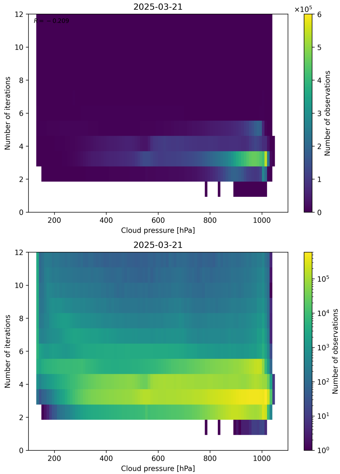
Figure 81: Scatter density plot of “Cloud pressure” against “Number of iterations” for 2025-03-20 to 2025-03-22.
