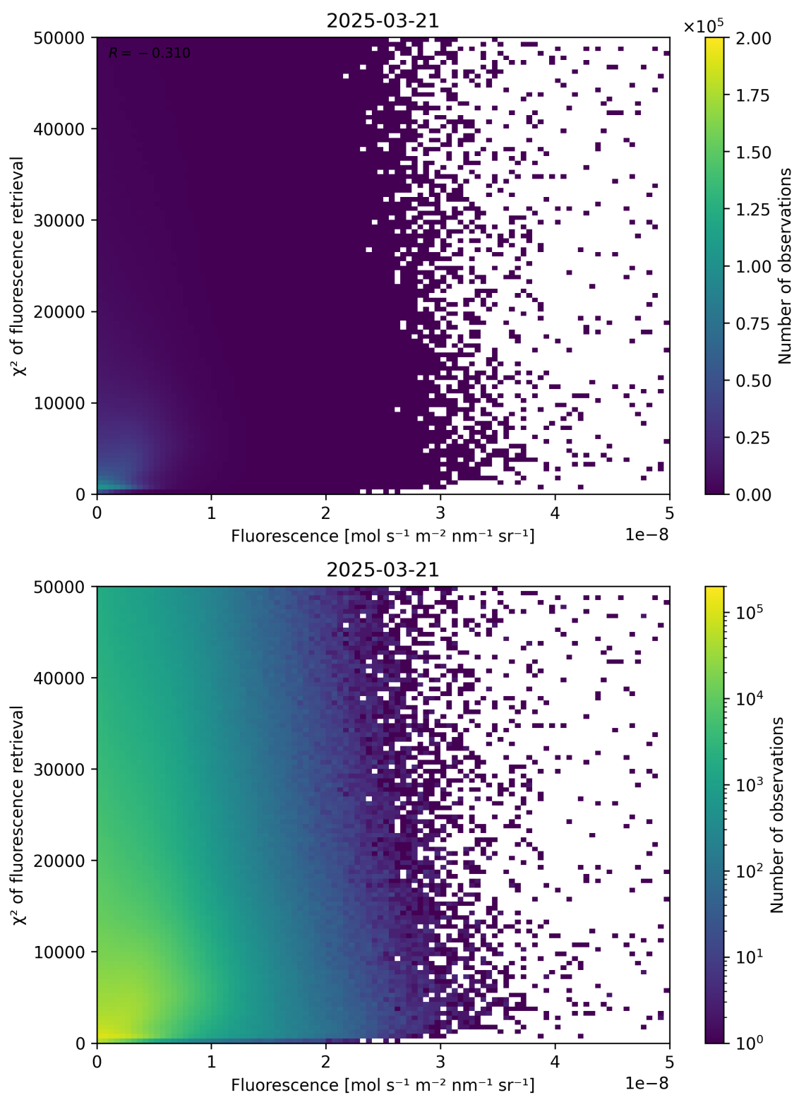
Figure 85: Scatter density plot of “Fluorescence” against “ \chi^2 of fluorescence retrieval” for 2025-03-20 to 2025-03-22.
