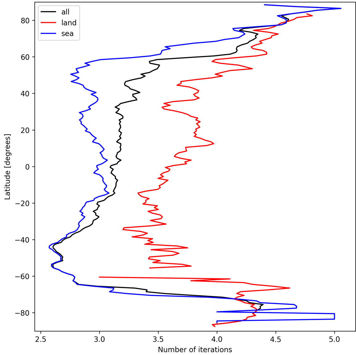
Figure 22: Zonal average of “Number of iterations” for 2025-03-20 to 2025-03-22.
