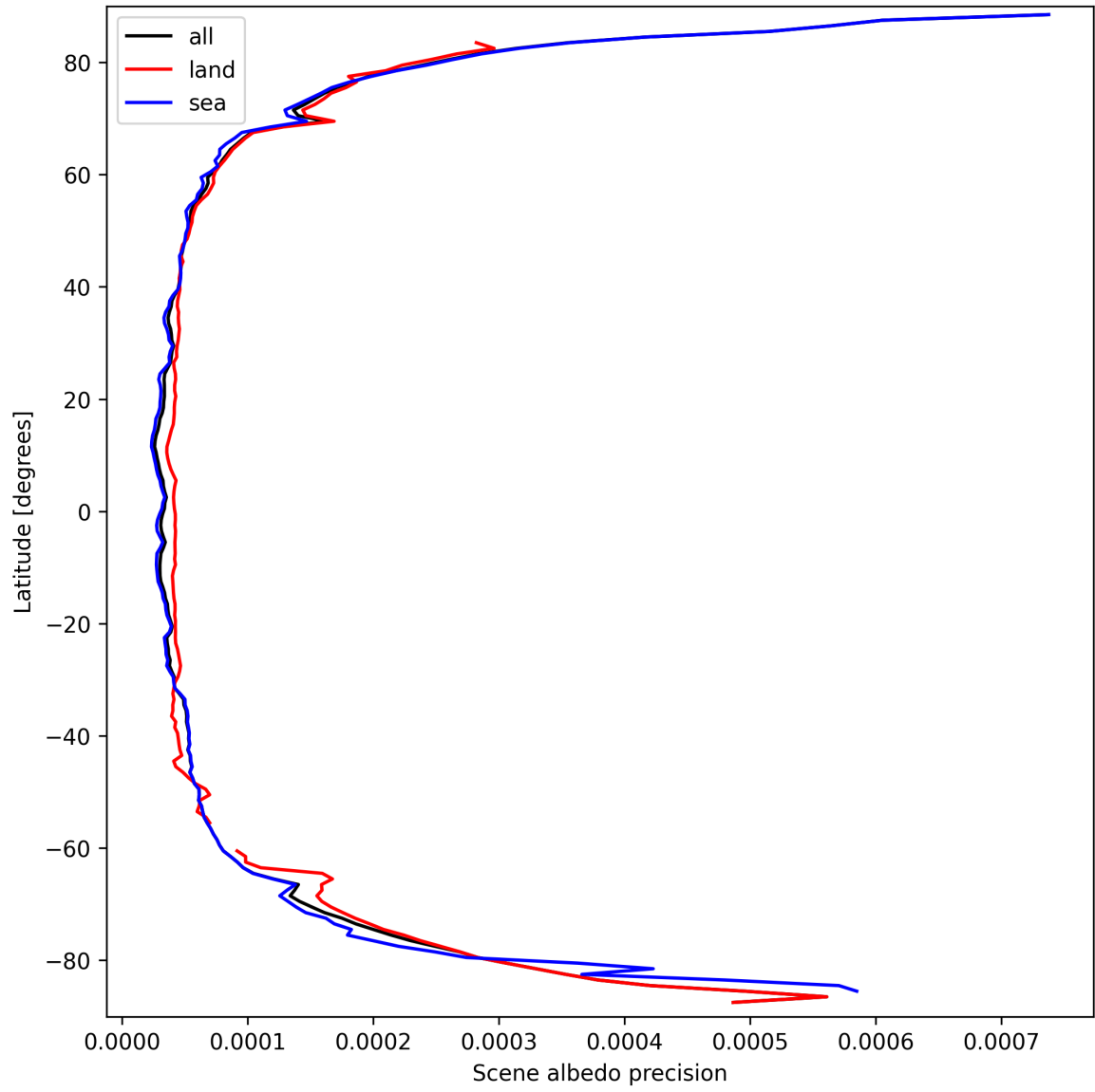
Figure 18: Zonal average of “Scene albedo precision” for 2025-03-20 to 2025-03-22.
