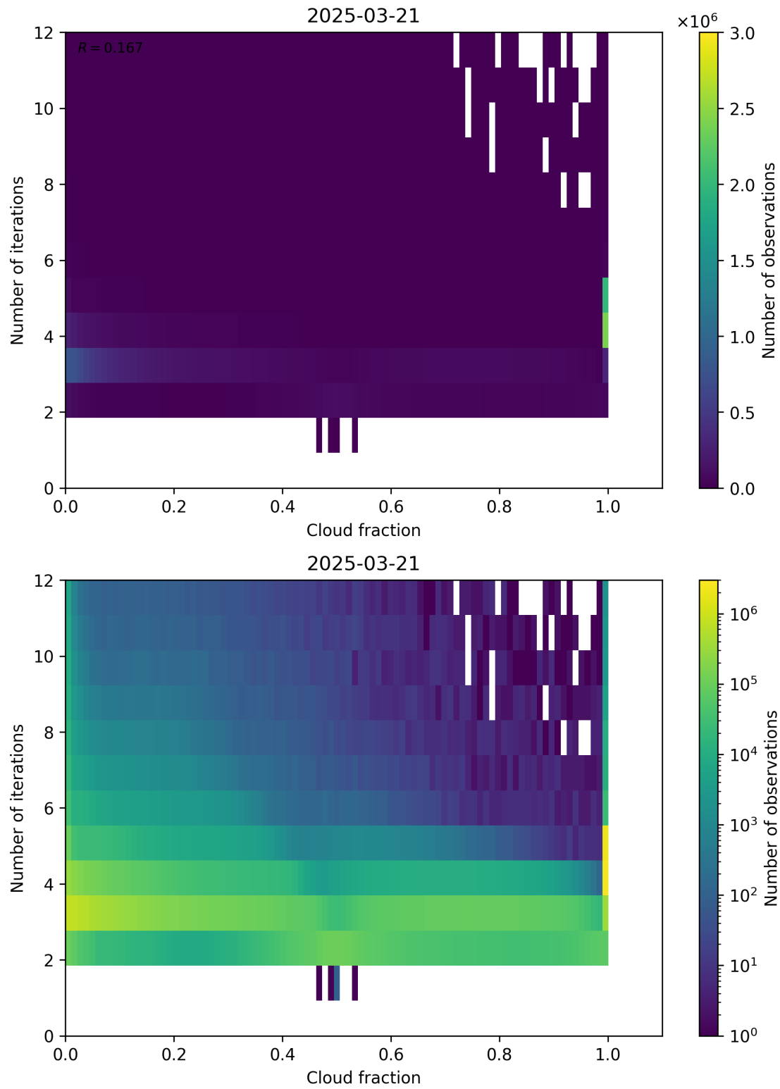
Figure 73: Scatter density plot of “Cloud fraction” against “Number of iterations” for 2025-03-20 to 2025-03-22.
