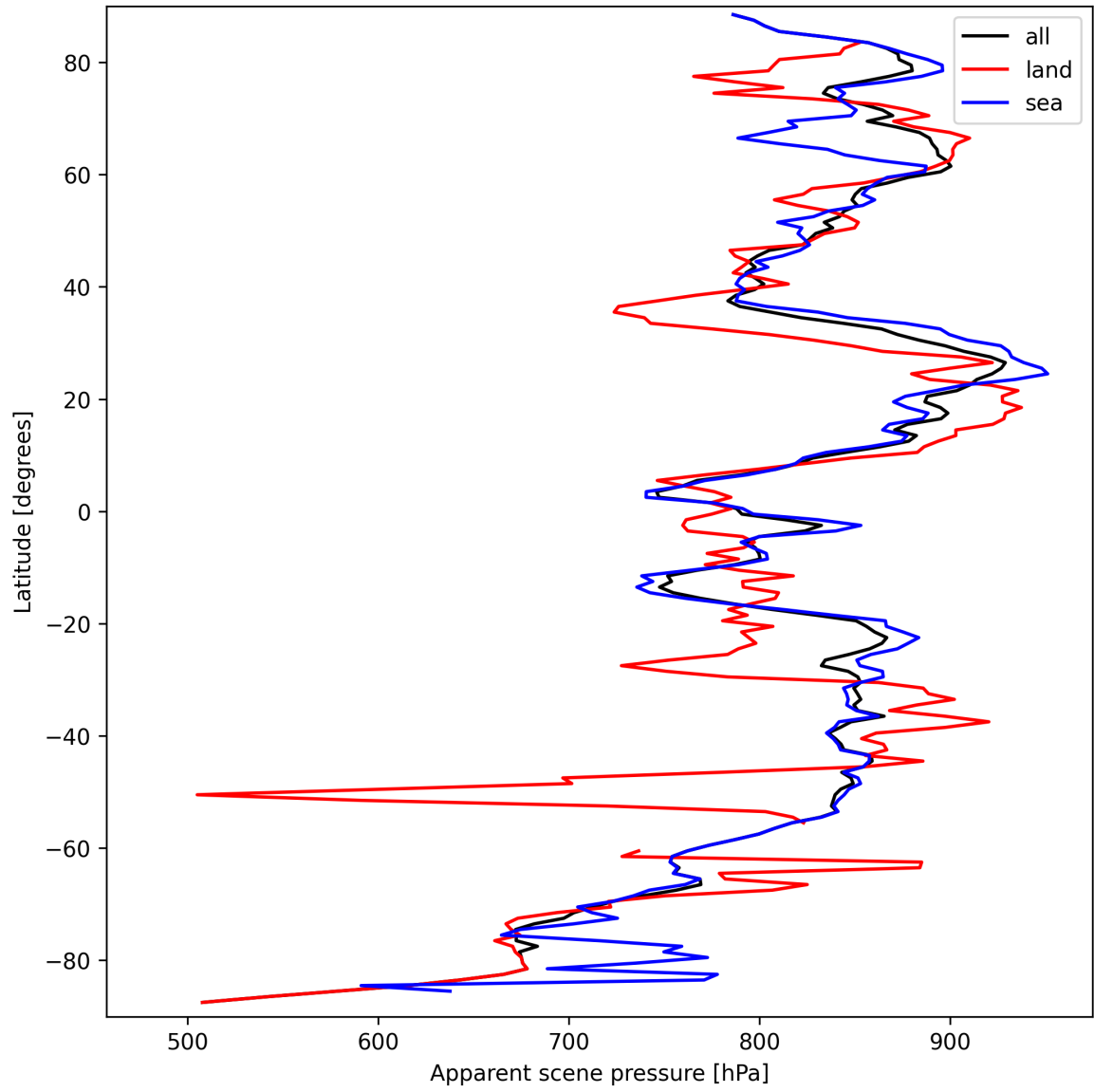
Figure 19: Zonal average of “Apparent scene pressure” for 2025-03-20 to 2025-03-22.
