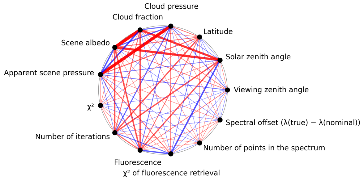
Figure 1: Map of correlation graph for 2025-03-20 to 2025-03-22.
