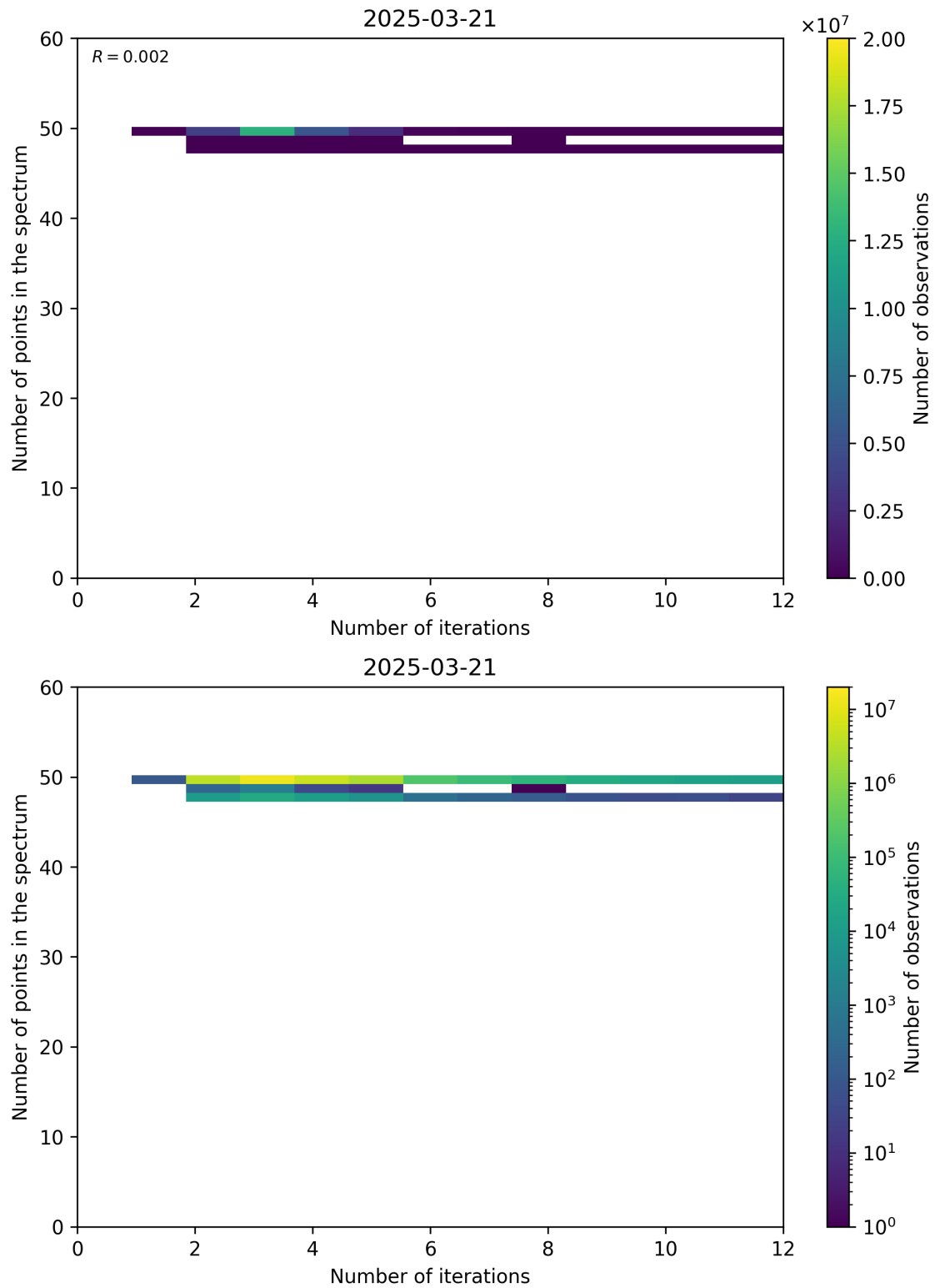
Figure 99: Scatter density plot of “Number of iterations” against “Number of points in the spectrum” for 2025-03-20 to 2025-03-22.
