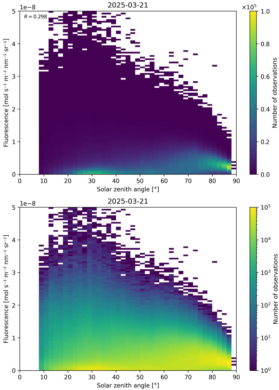
Figure 112: Scatter density plot of “Solar zenith angle” against “Fluorescence” for 2025-03-20 to 2025-03-22.
