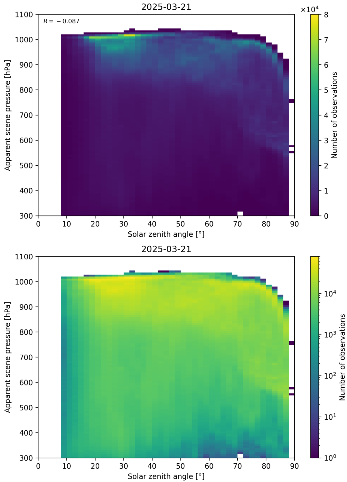
Figure 108: Scatter density plot of “Solar zenith angle” against “Apparent scene pressure” for 2025-03-20 to 2025-03-22.
