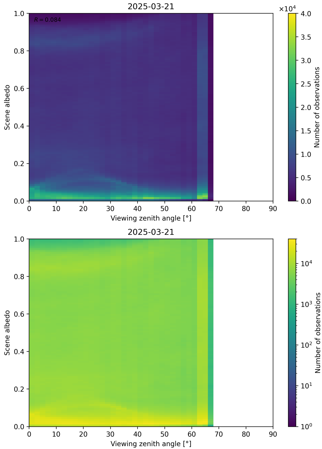
Figure 126: Scatter density plot of “Viewing zenith angle” against “Scene albedo” for 2025-03-20 to 2025-03-22.
