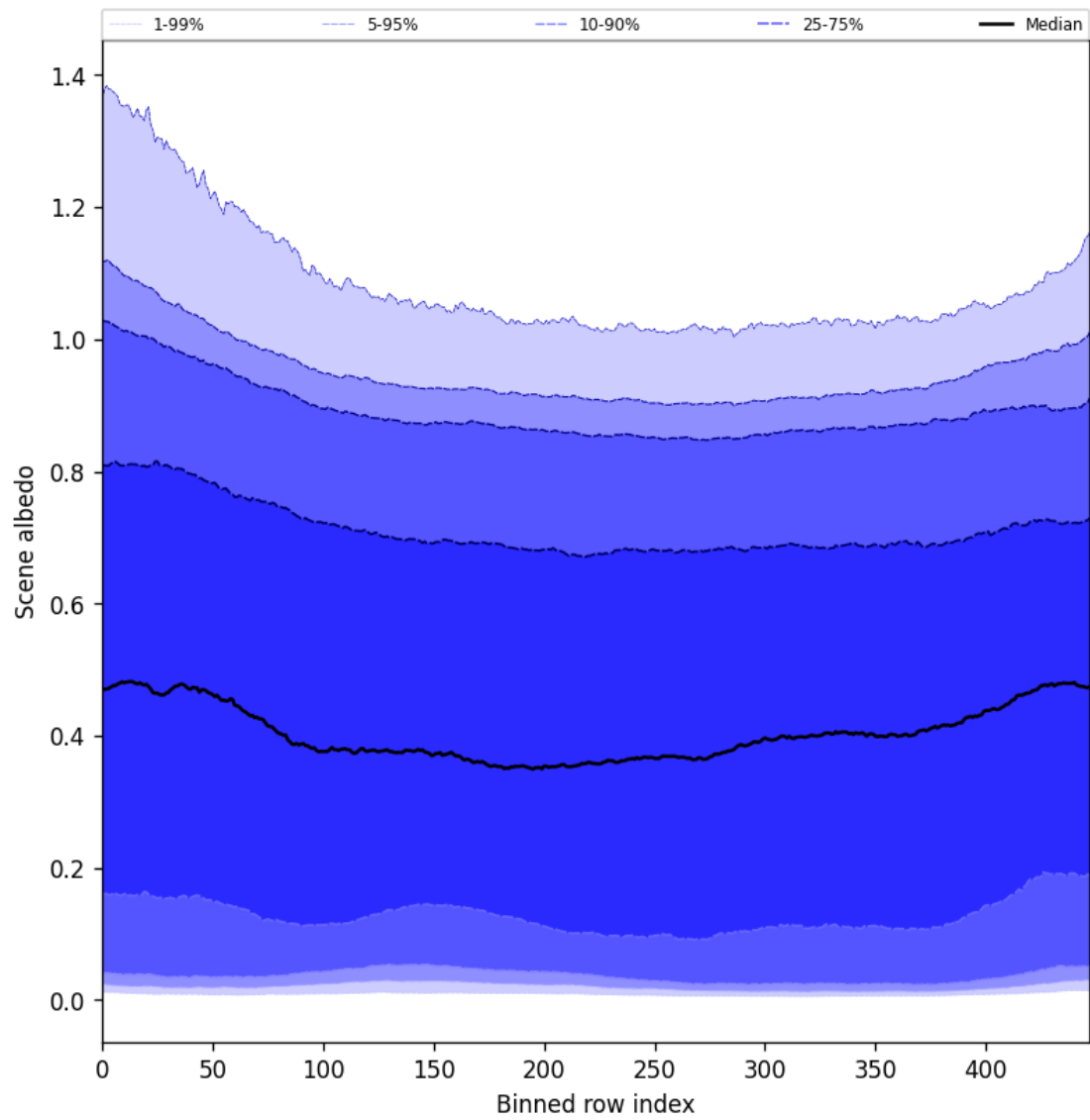
Figure 51: Along track statistics of “Scene albedo” for 2025-03-20 to 2025-03-22
