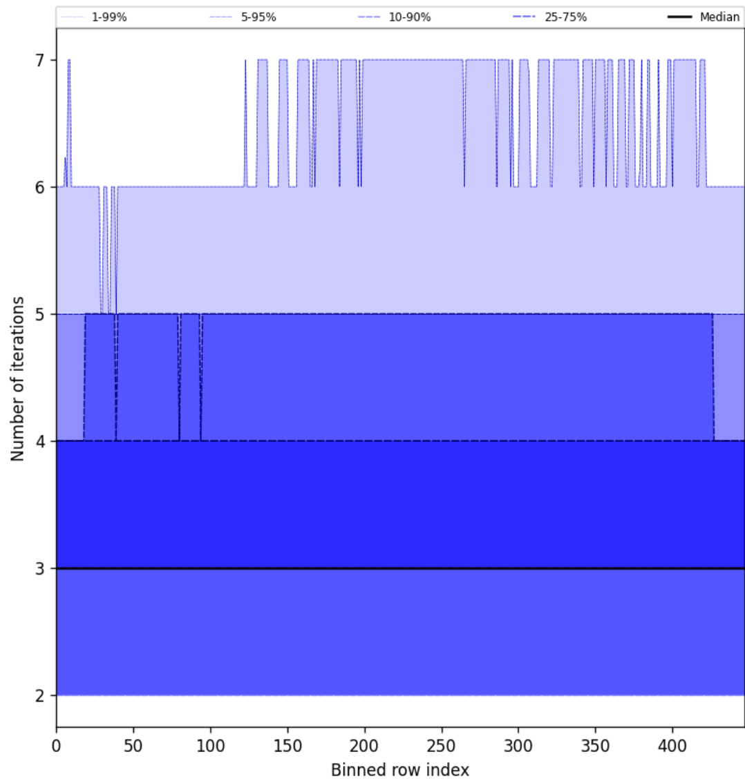
Figure 56: Along track statistics of “Number of iterations” for 2025-03-20 to 2025-03-22
