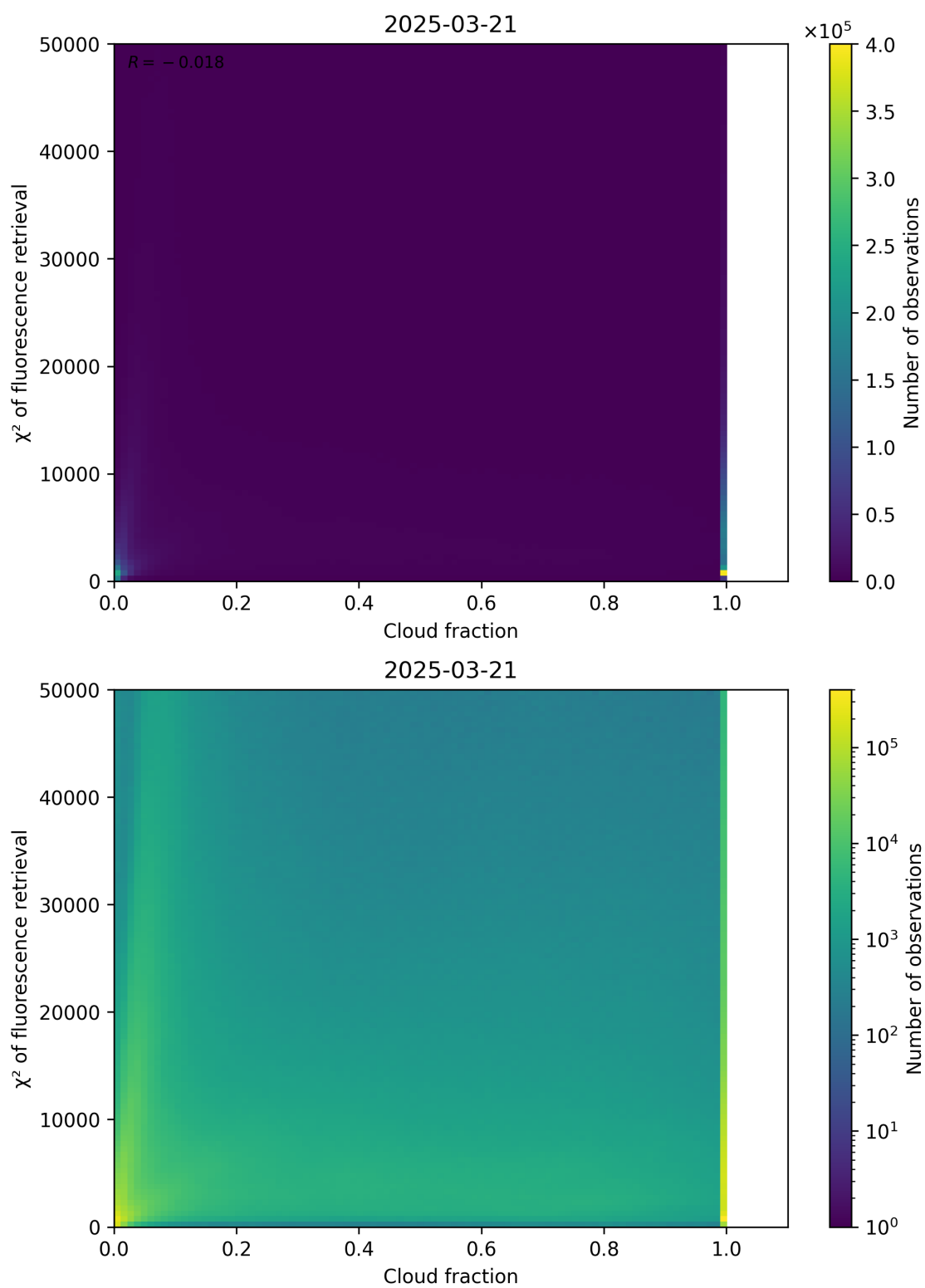
Figure 71: Scatter density plot of “Cloud fraction” against “ \chi^2 of fluorescence retrieval” for 2025-03-20 to 2025-03-22.
