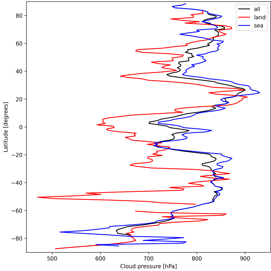
Figure 13: Zonal average of “Cloud pressure” for 2025-03-20 to 2025-03-22.
