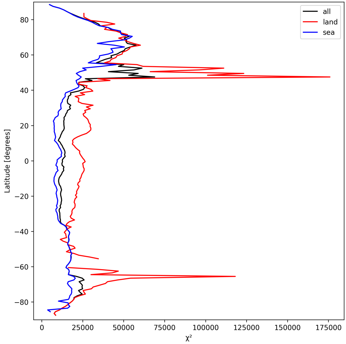
Figure 21: Zonal average of “ \chi^2 ” for 2025-03-20 to 2025-03-22.
