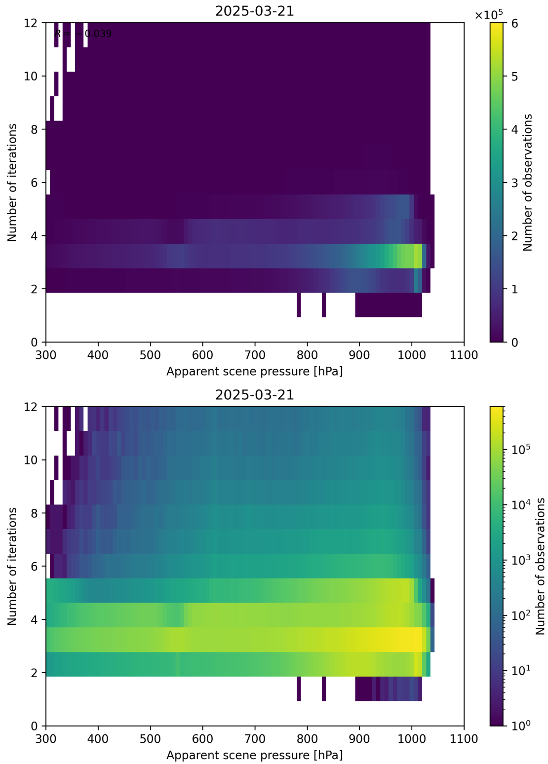
Figure 65: Scatter density plot of “Apparent scene pressure” against “Number of iterations” for 2025-03-20 to 2025-03-22.
