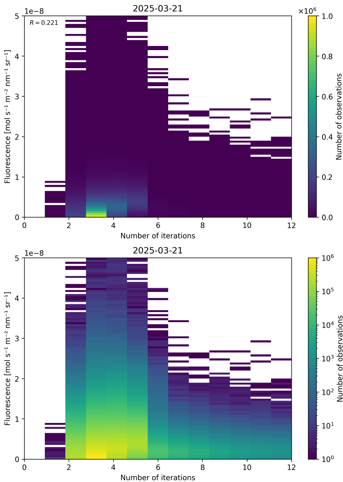
Figure 98: Scatter density plot of “Number of iterations” against “Fluorescence” for 2025-03-20 to 2025-03-22.
