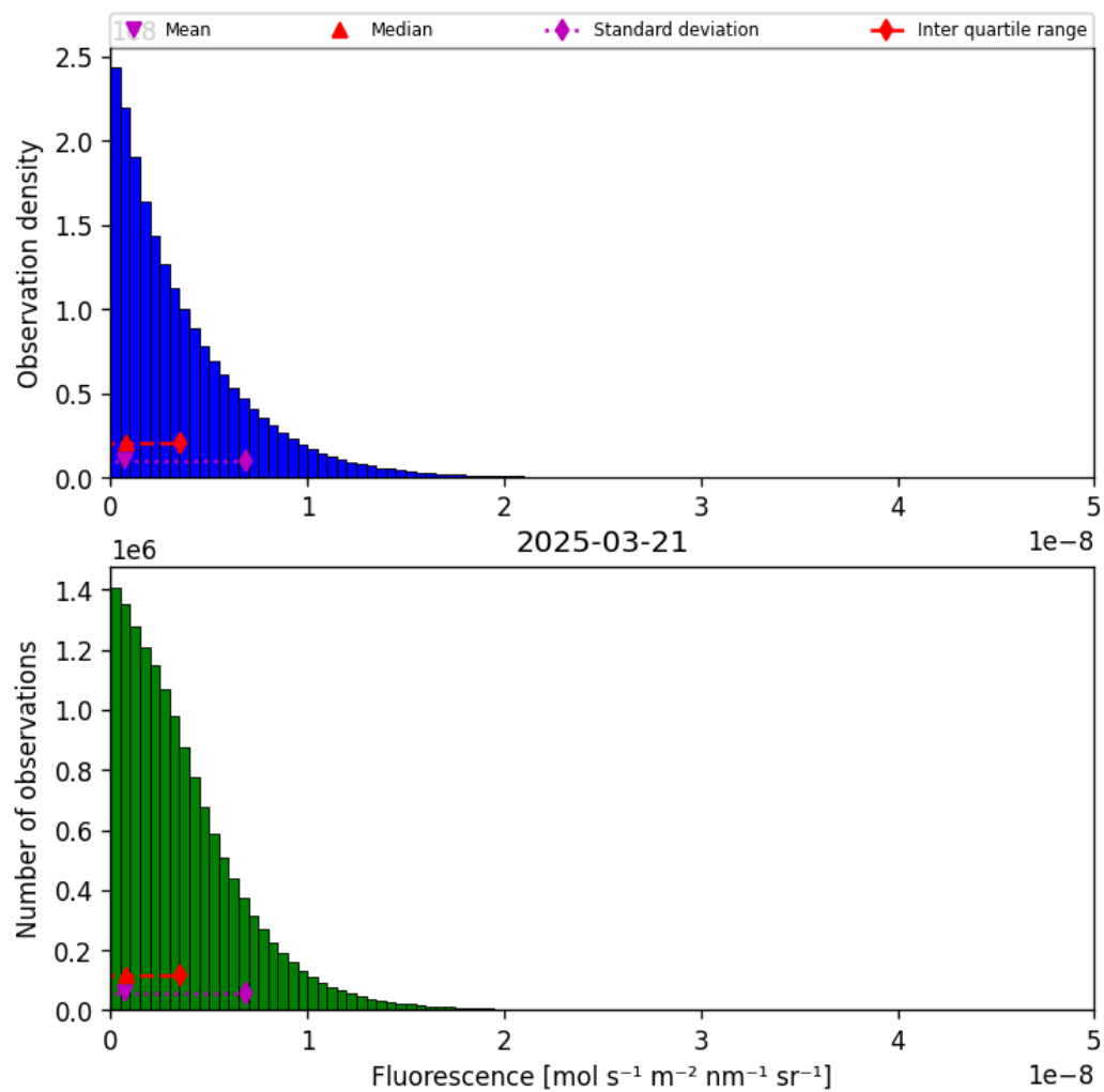
Figure 40: Histogram of “Fluorescence” for 2025-03-20 to 2025-03-22
