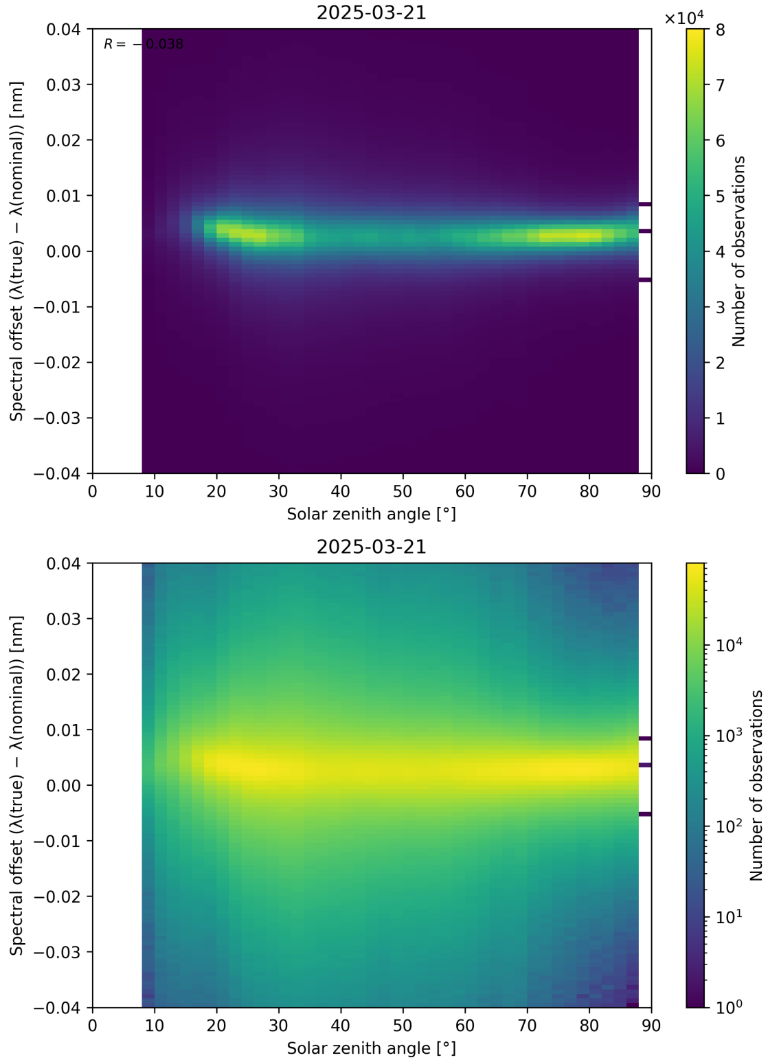
Figure 117: Scatter density plot of “Solar zenith angle” against “Spectral offset ( \lambda_{\text{true}} - \lambda_{\text{nominal}} )” for 2025-03-20 to 2025-03-22.
