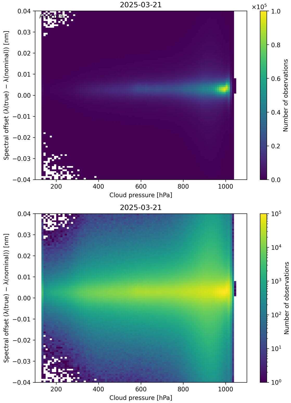
Figure 84: Scatter density plot of “Cloud pressure” against “Spectral offset ( \lambda_{\text{true}} - \lambda_{\text{nominal}} )” for 2025-03-20 to 2025-03-22.
