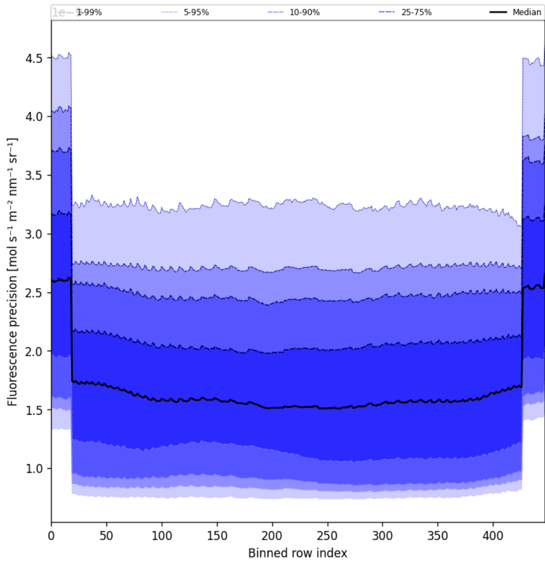
Figure 58: Along track statistics of “Fluorescence precision” for 2025-03-20 to 2025-03-22
