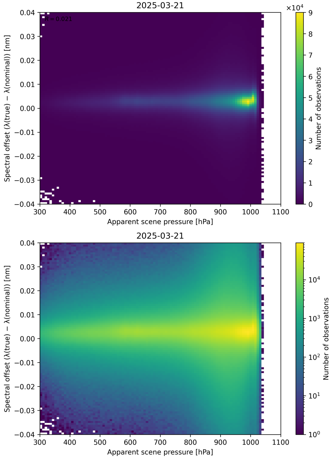
Figure 67: Scatter density plot of “Apparent scene pressure” against “Spectral offset ( \lambda_{\text{true}} - \lambda_{\text{nominal}} )” for 2025-03-20 to 2025-03-22.
