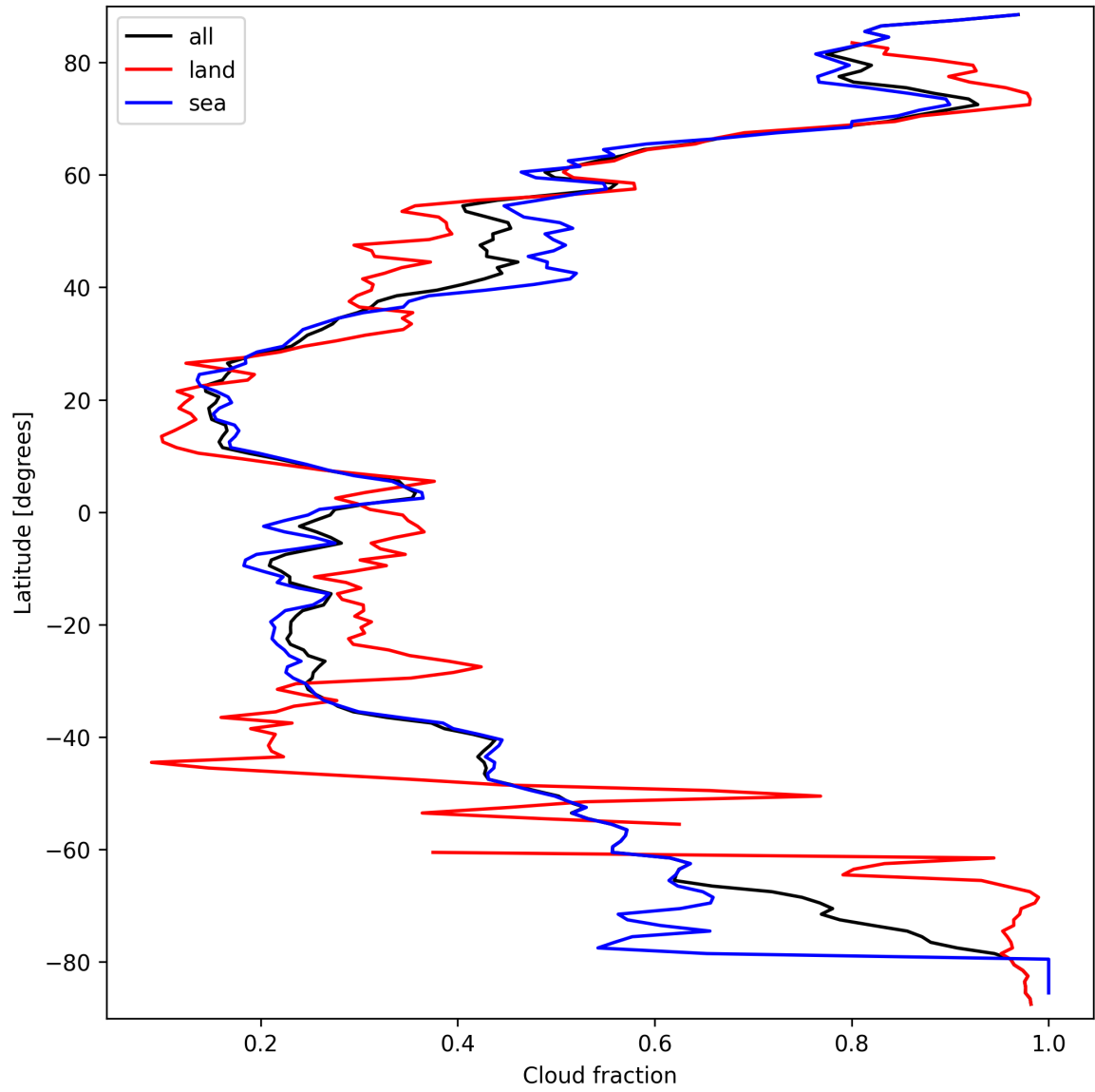
Figure 15: Zonal average of “Cloud fraction” for 2025-03-20 to 2025-03-22.
