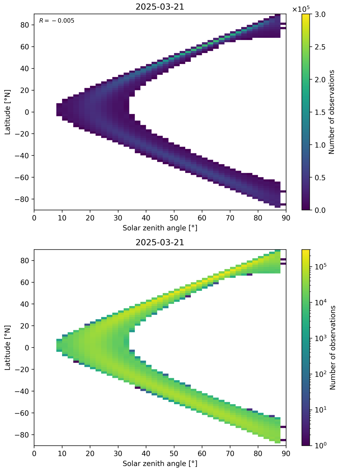
Figure 113: Scatter density plot of “Solar zenith angle” against “Latitude” for 2025-03-20 to 2025-03-22.
