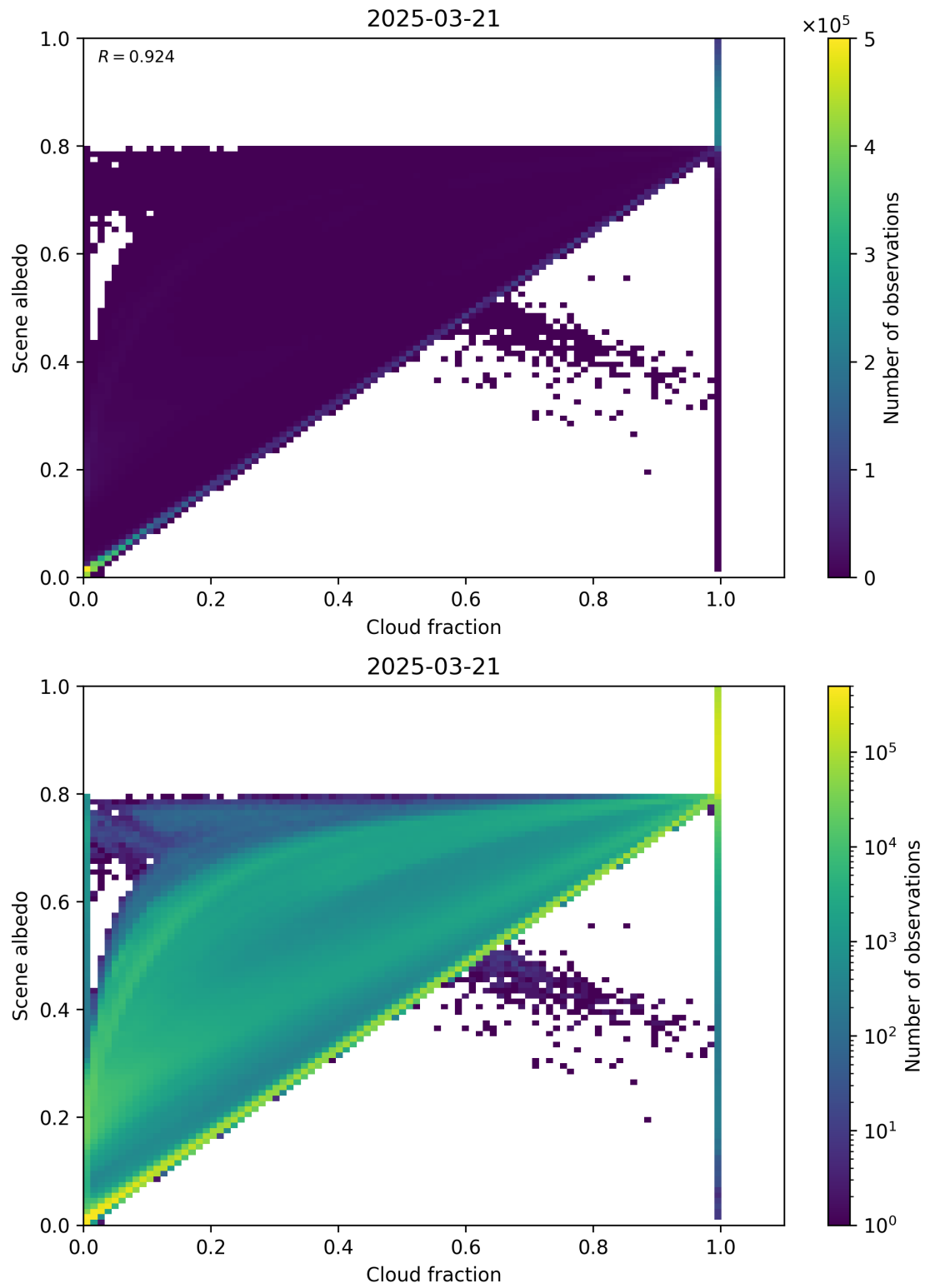
Figure 75: Scatter density plot of “Cloud fraction” against “Scene albedo” for 2025-03-20 to 2025-03-22.
