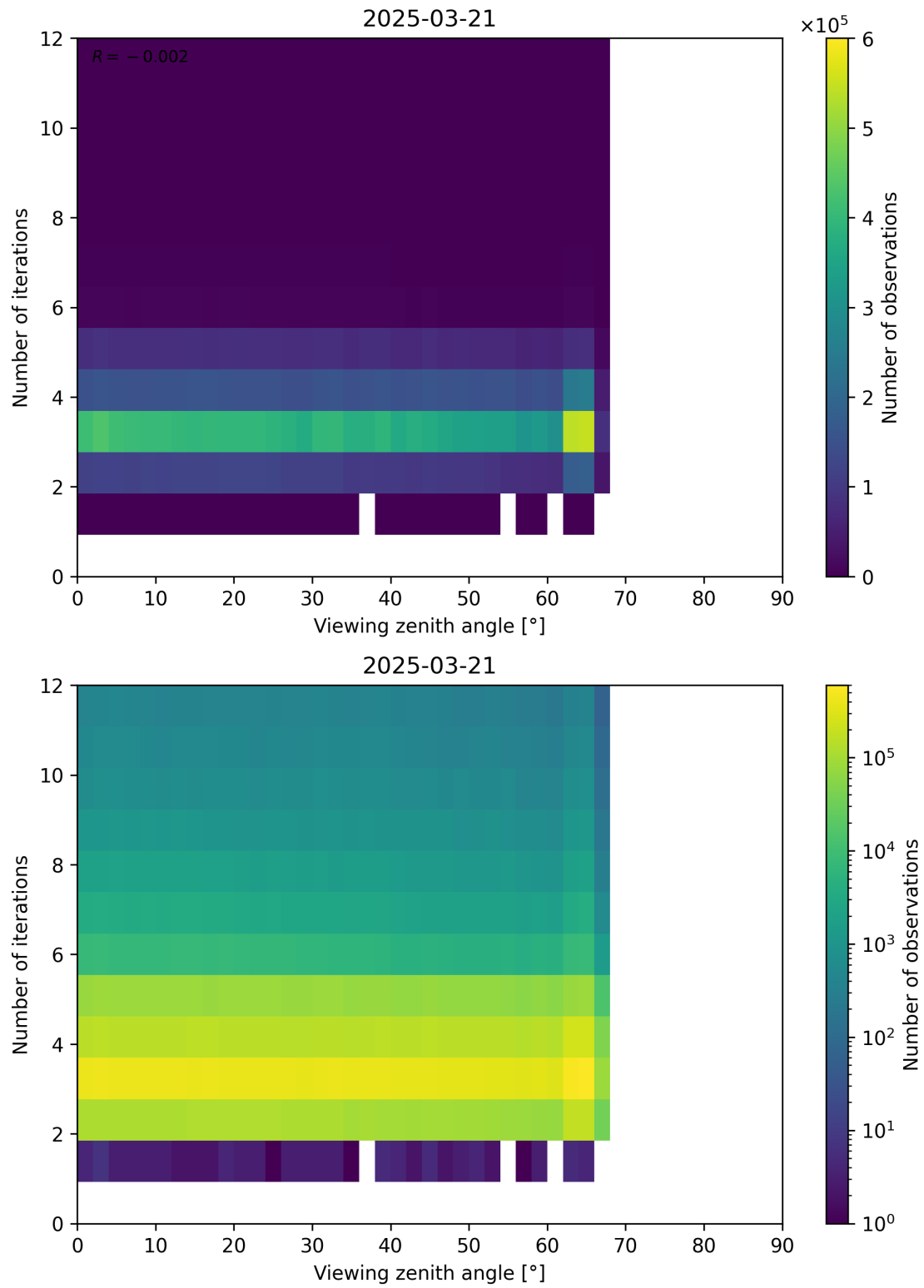
Figure 124: Scatter density plot of “Viewing zenith angle” against “Number of iterations” for 2025-03-20 to 2025-03-22.
