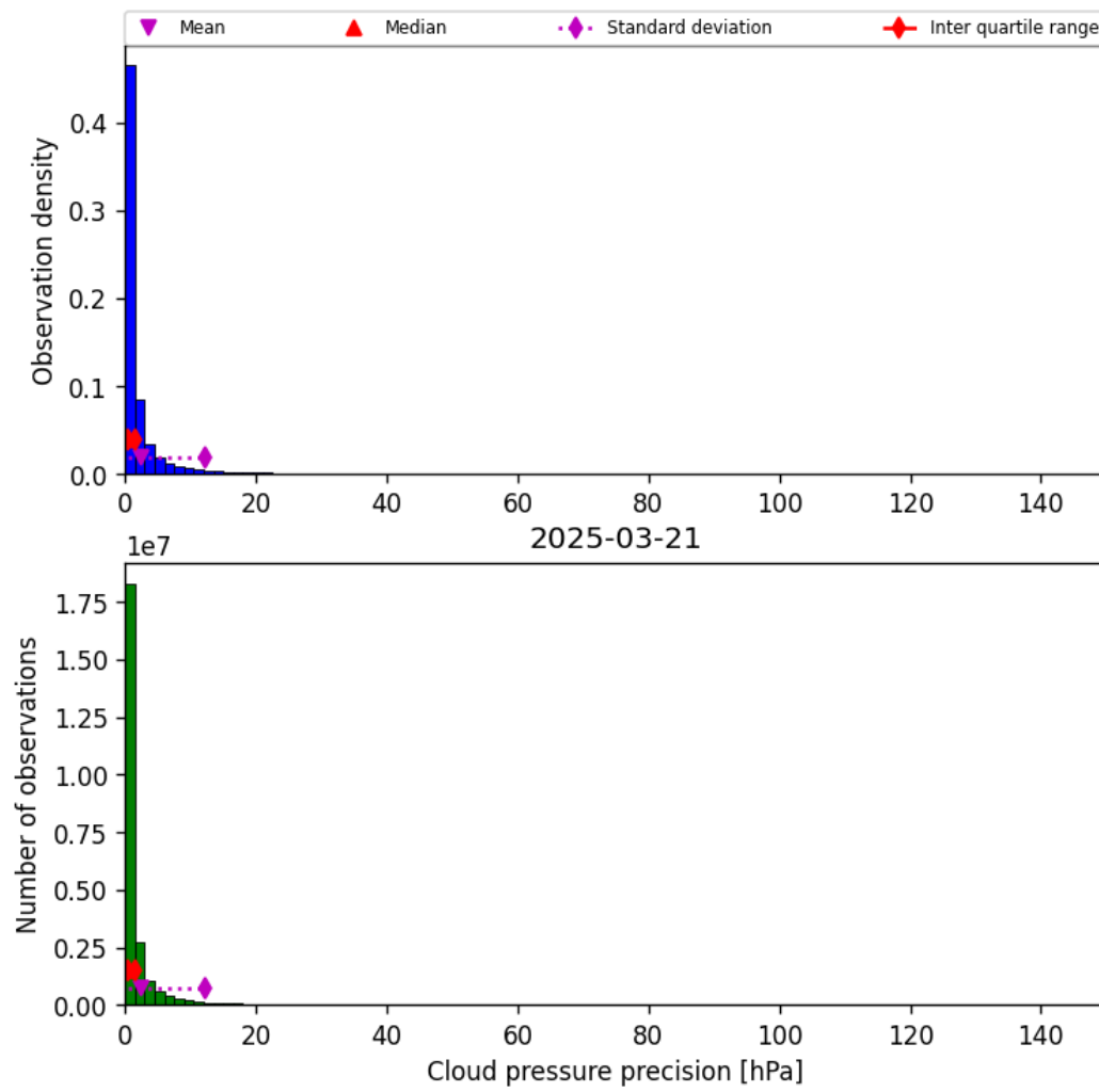
Figure 31: Histogram of “Cloud pressure precision” for 2025-03-20 to 2025-03-22
