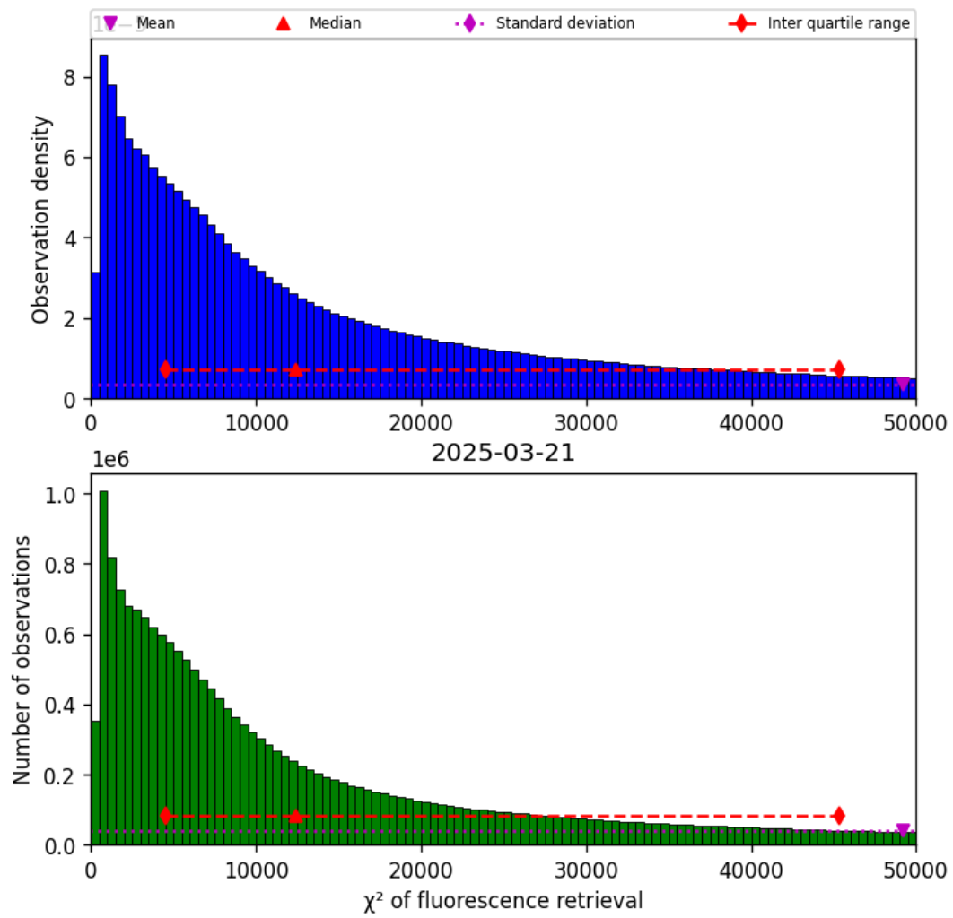
Figure 42: Histogram of “ \chi^2 of fluorescence retrieval” for 2025-03-20 to 2025-03-22
