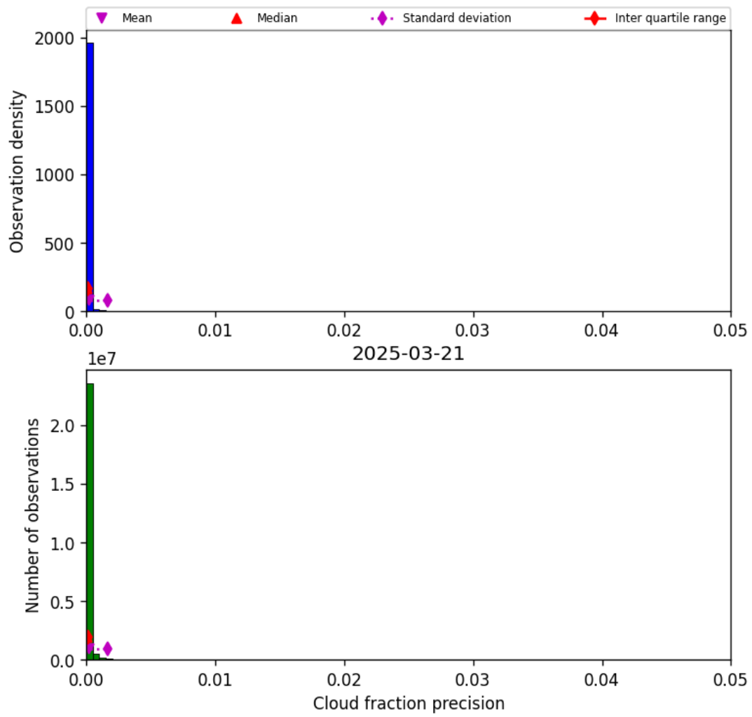
Figure 33: Histogram of “Cloud fraction precision” for 2025-03-20 to 2025-03-22
