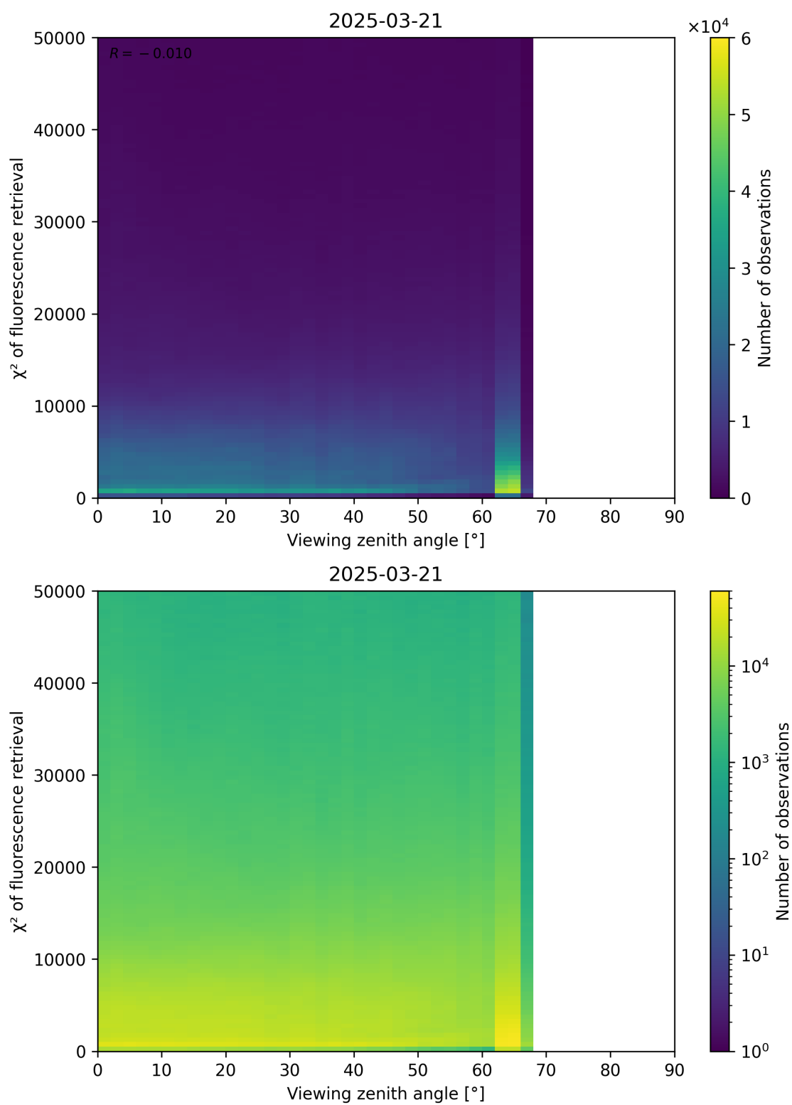
Figure 119: Scatter density plot of “Viewing zenith angle” against “ \chi^2 of fluorescence retrieval” for 2025-03-20 to 2025-03-22.
