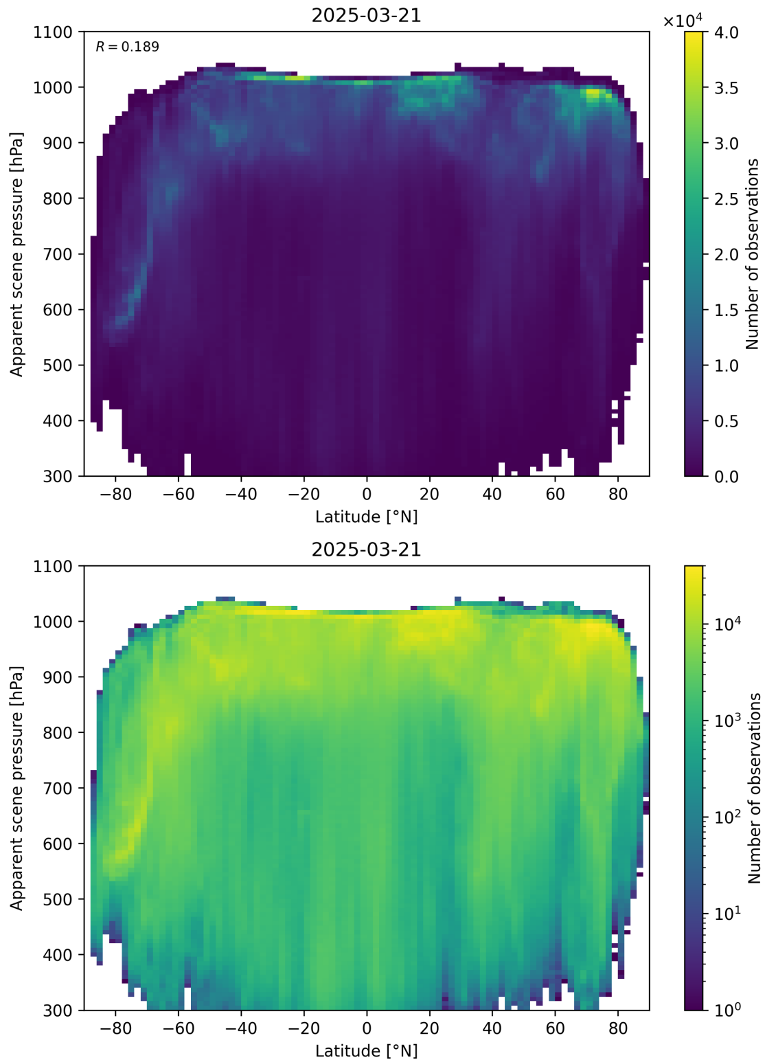
Figure 88: Scatter density plot of “Latitude” against “Apparent scene pressure” for 2025-03-20 to 2025-03-22.
