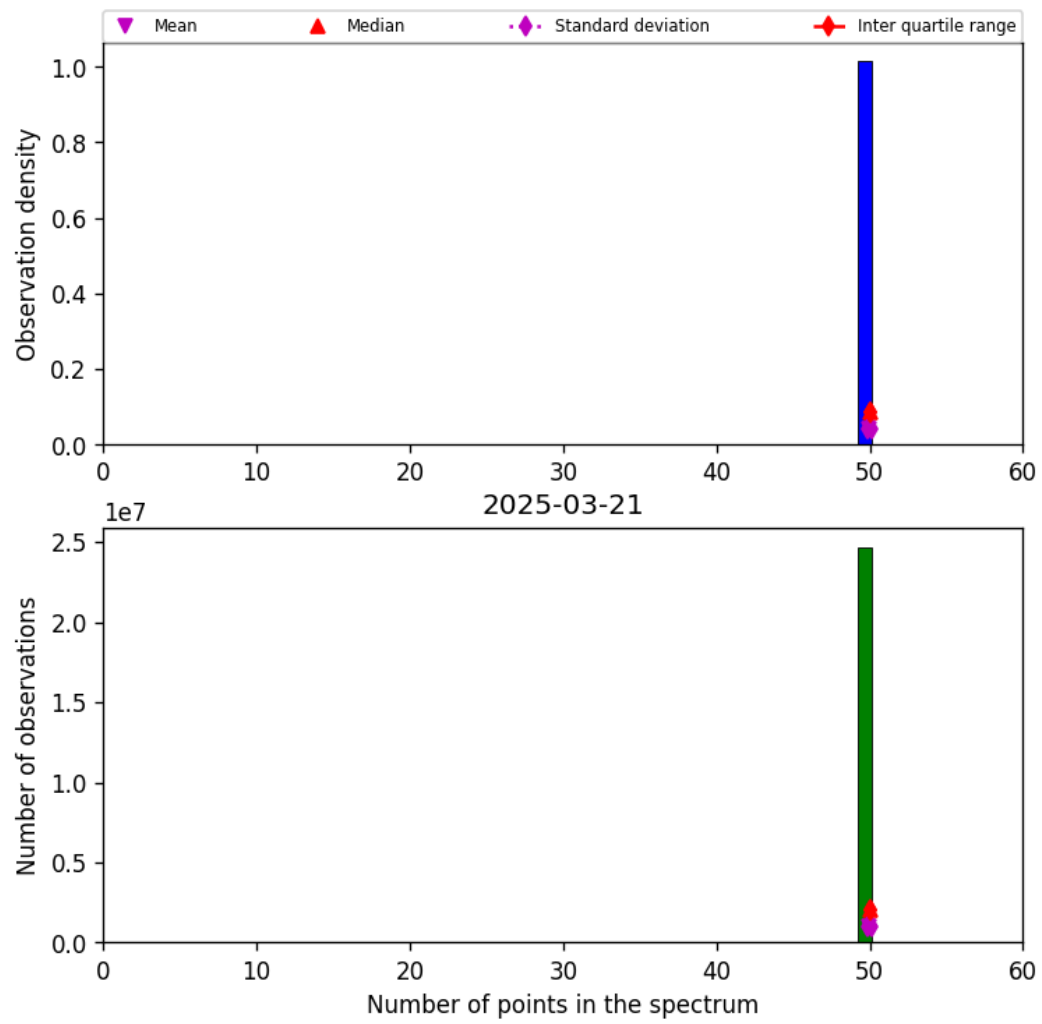
Figure 44: Histogram of “Number of points in the spectrum” for 2025-03-20 to 2025-03-22
