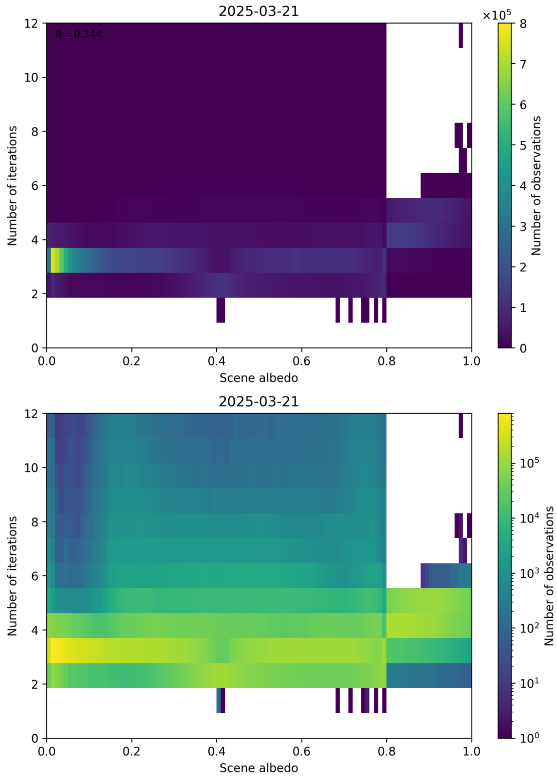
Figure 105: Scatter density plot of “Scene albedo” against “Number of iterations” for 2025-03-20 to 2025-03-22.
