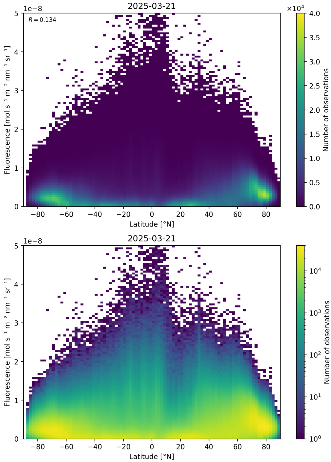
Figure 92: Scatter density plot of “Latitude” against “Fluorescence” for 2025-03-20 to 2025-03-22.
