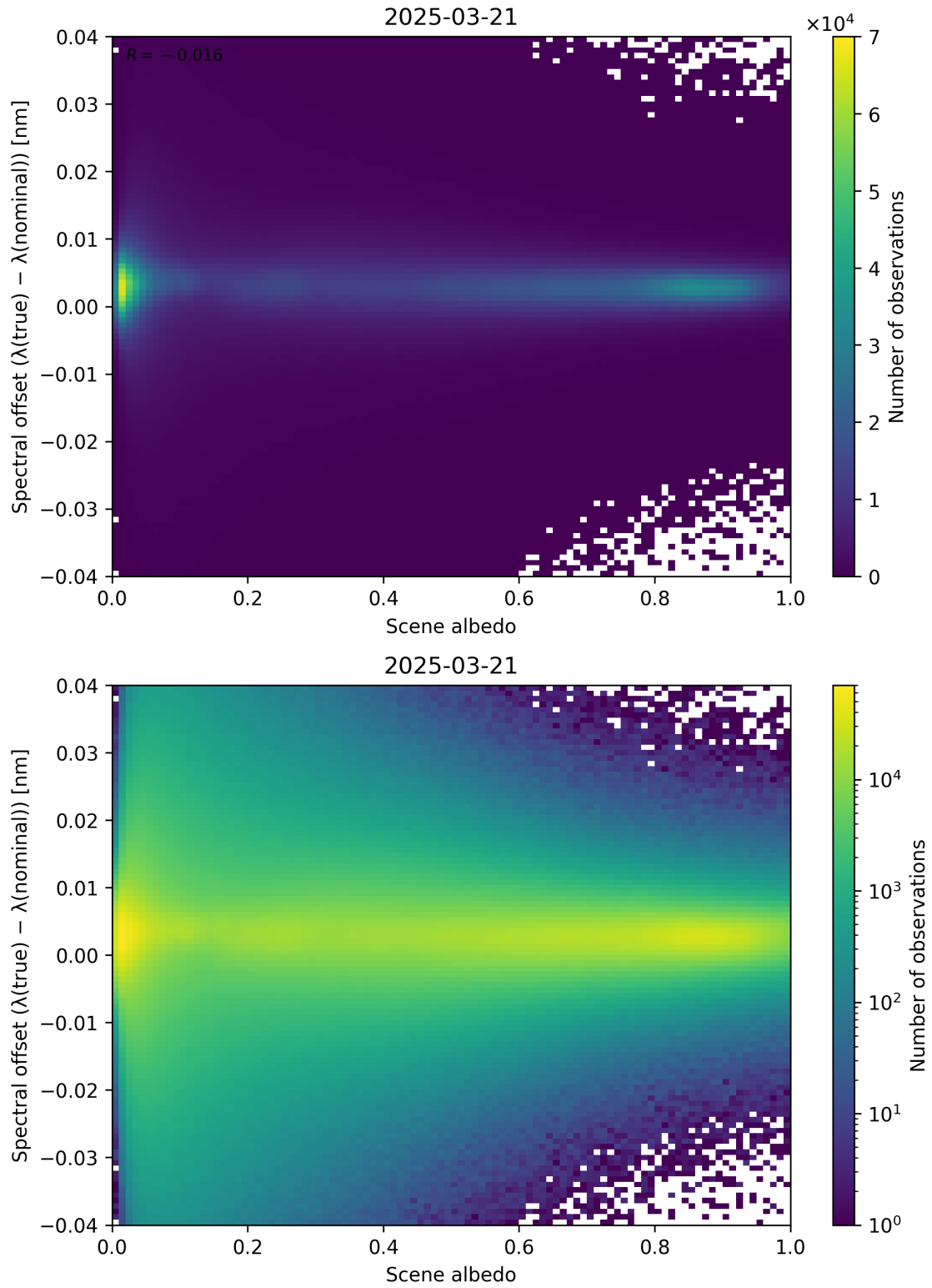
Figure 107: Scatter density plot of “Scene albedo” against “Spectral offset ( \lambda_{\text{true}} - \lambda_{\text{nominal}} )” for 2025-03-20 to 2025-03-22.
