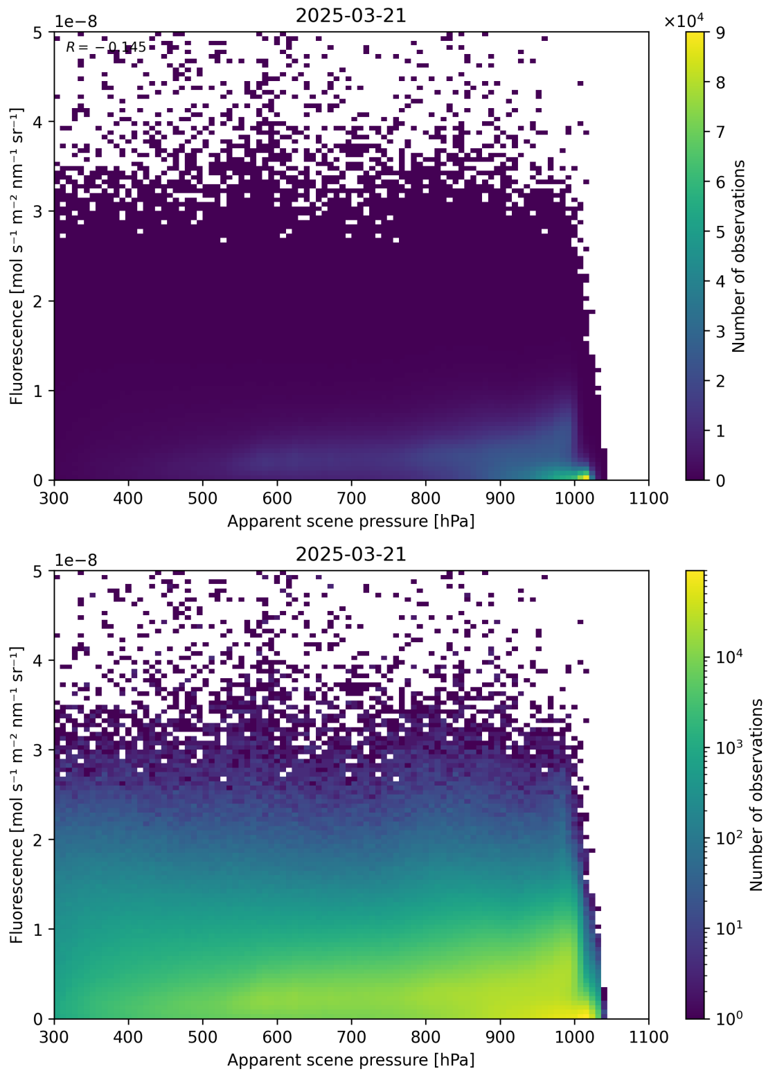
Figure 64: Scatter density plot of “Apparent scene pressure” against “Fluorescence” for 2025-03-20 to 2025-03-22.
