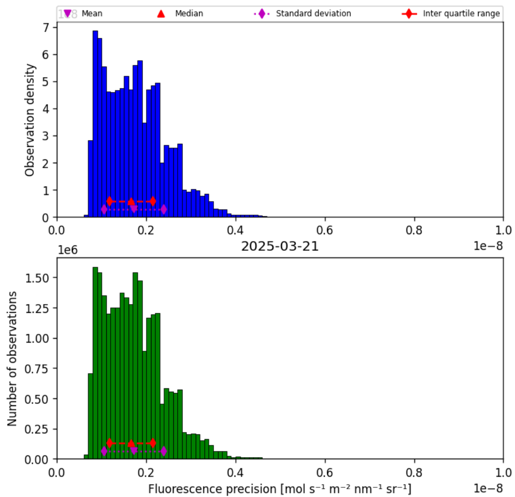
Figure 41: Histogram of “Fluorescence precision” for 2025-03-20 to 2025-03-22
