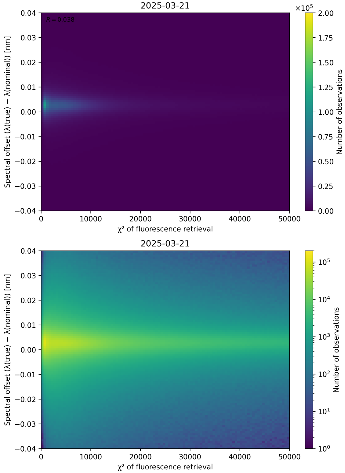
Figure 69: Scatter density plot of “ \chi^2 of fluorescence retrieval” against “Spectral offset ( \lambda_{\text{true}} - \lambda_{\text{nominal}} )” for 2025-03-20 to 2025-03-22.
