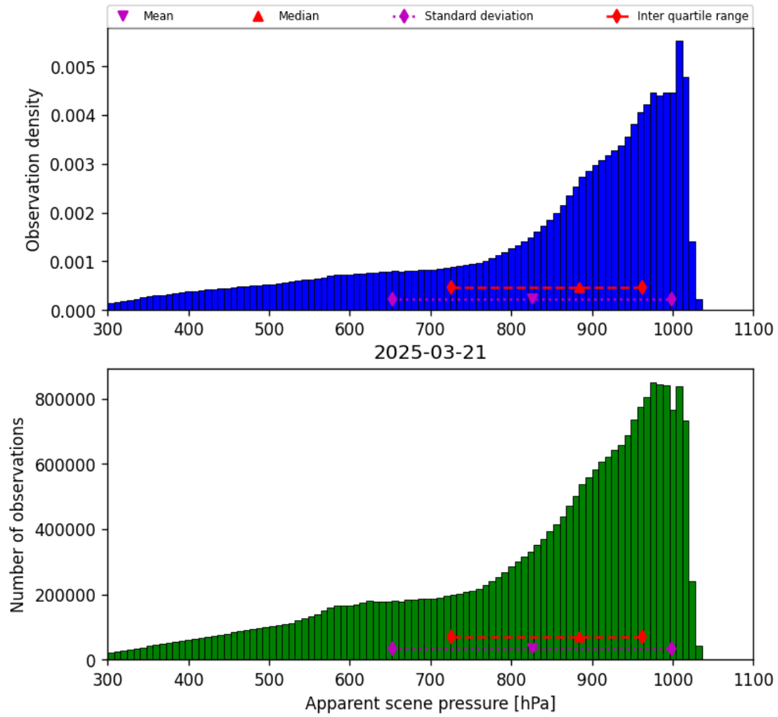
Figure 36: Histogram of “Apparent scene pressure” for 2025-03-20 to 2025-03-22
