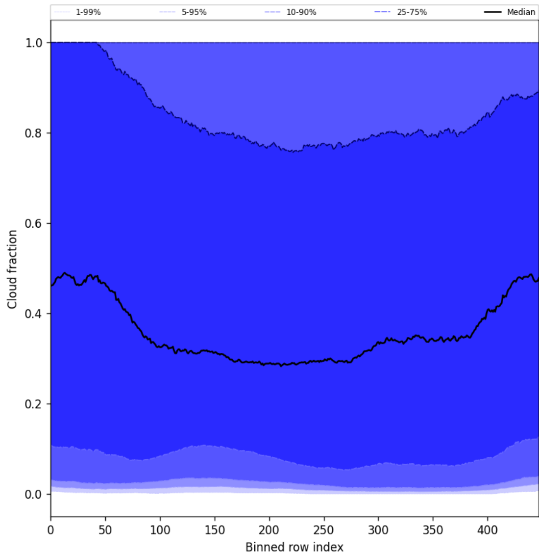
Figure 49: Along track statistics of “Cloud fraction” for 2025-03-20 to 2025-03-22
