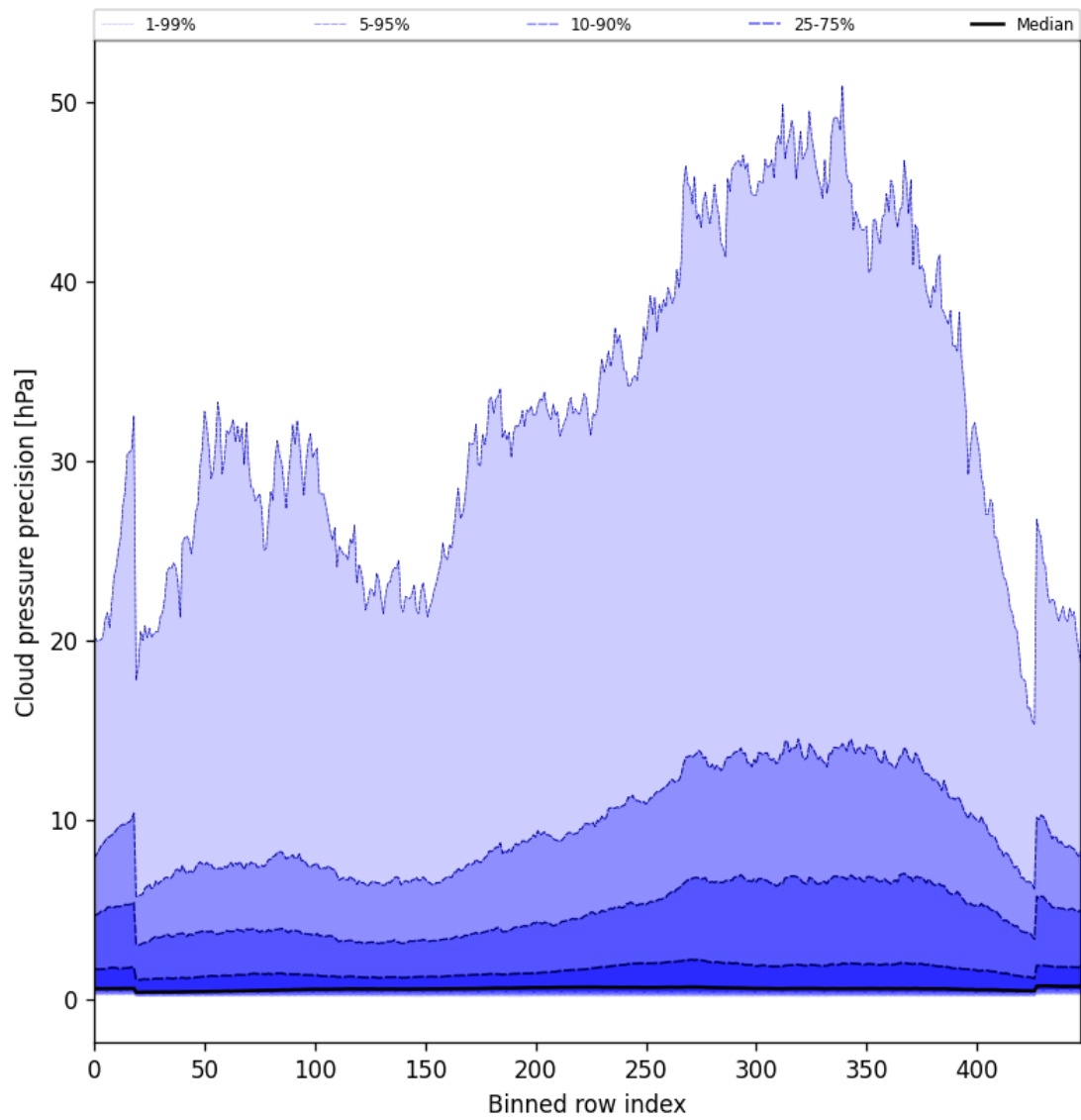
Figure 48: Along track statistics of “Cloud pressure precision” for 2025-03-20 to 2025-03-22
