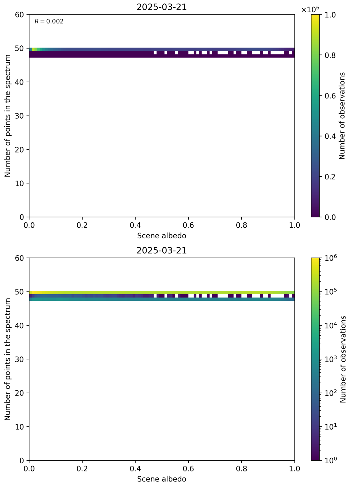
Figure 106: Scatter density plot of “Scene albedo” against “Number of points in the spectrum” for 2025-03-20 to 2025-03-22.
