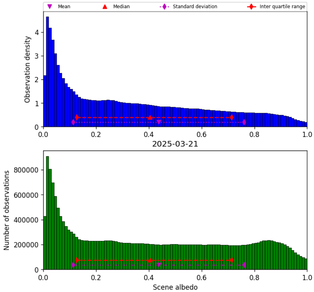
Figure 34: Histogram of “Scene albedo” for 2025-03-20 to 2025-03-22
