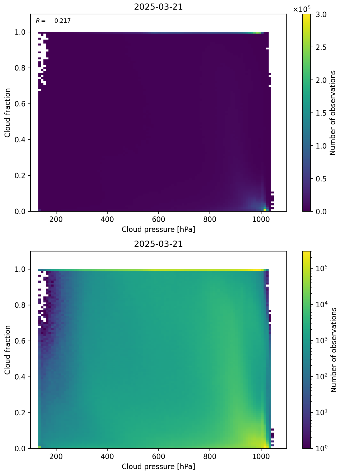
Figure 79: Scatter density plot of “Cloud pressure” against “Cloud fraction” for 2025-03-20 to 2025-03-22.
