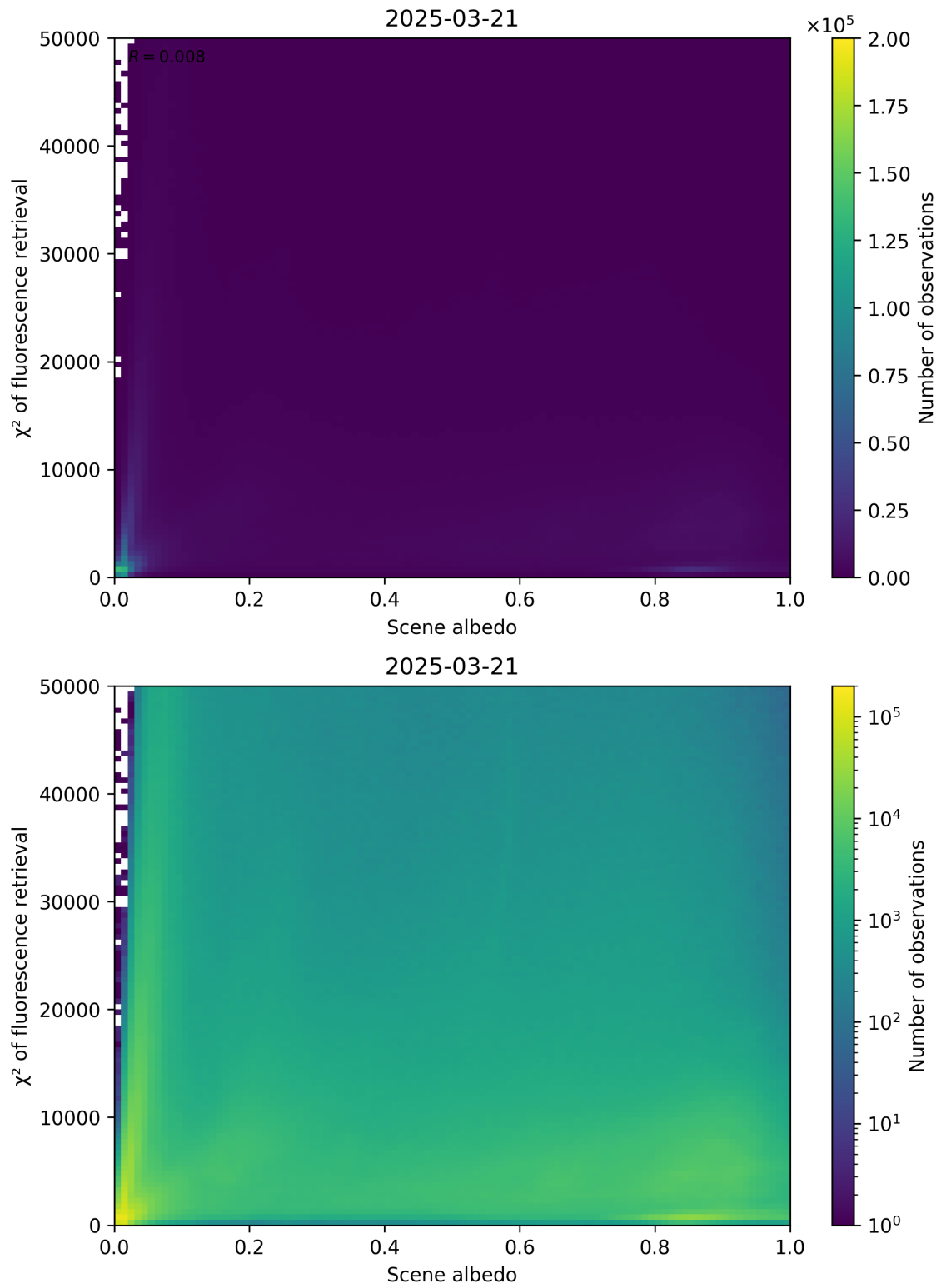
Figure 103: Scatter density plot of “Scene albedo” against “ \chi^2 of fluorescence retrieval” for 2025-03-20 to 2025-03-22.
