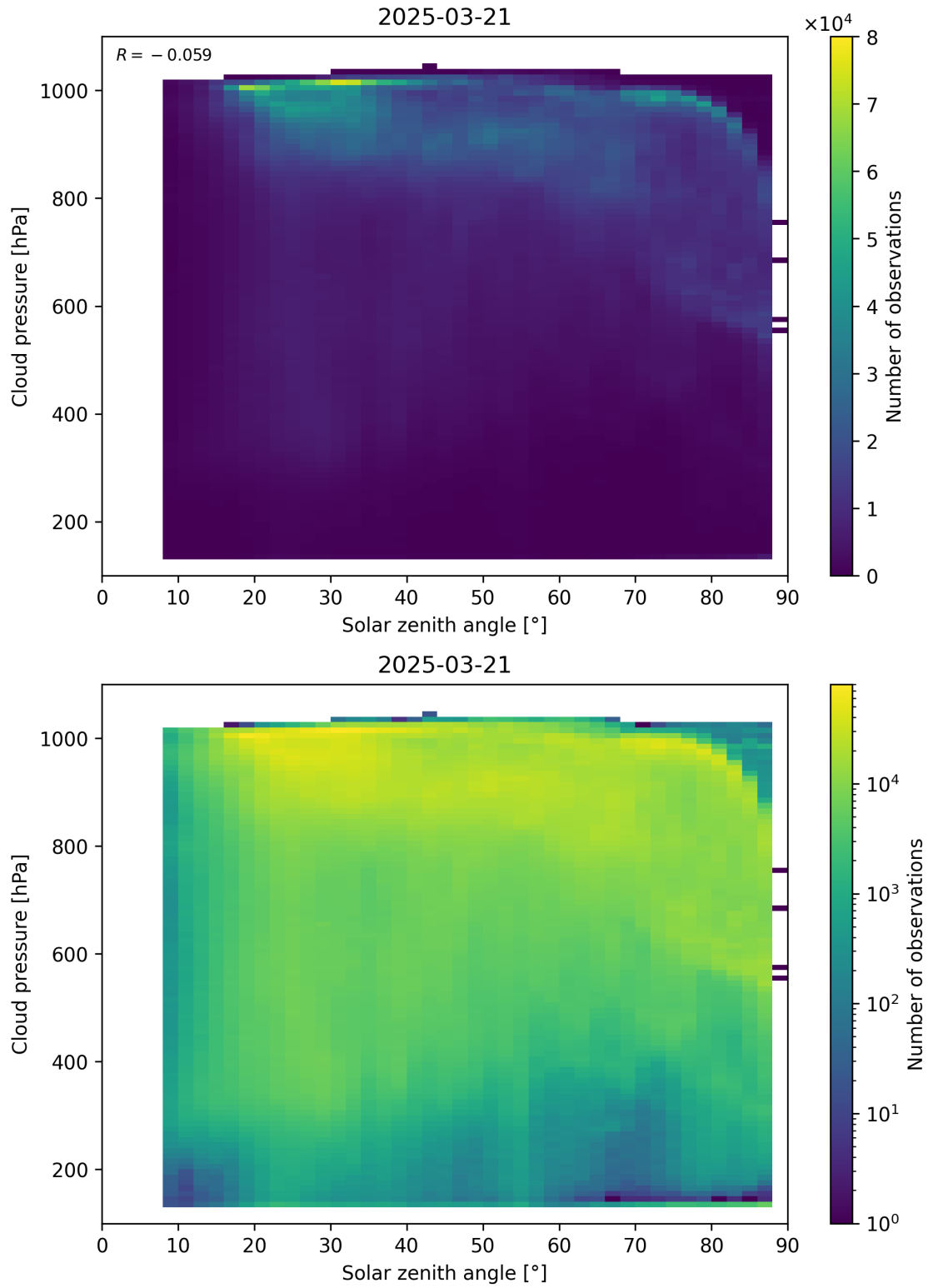
Figure 111: Scatter density plot of “Solar zenith angle” against “Cloud pressure” for 2025-03-20 to 2025-03-22.
