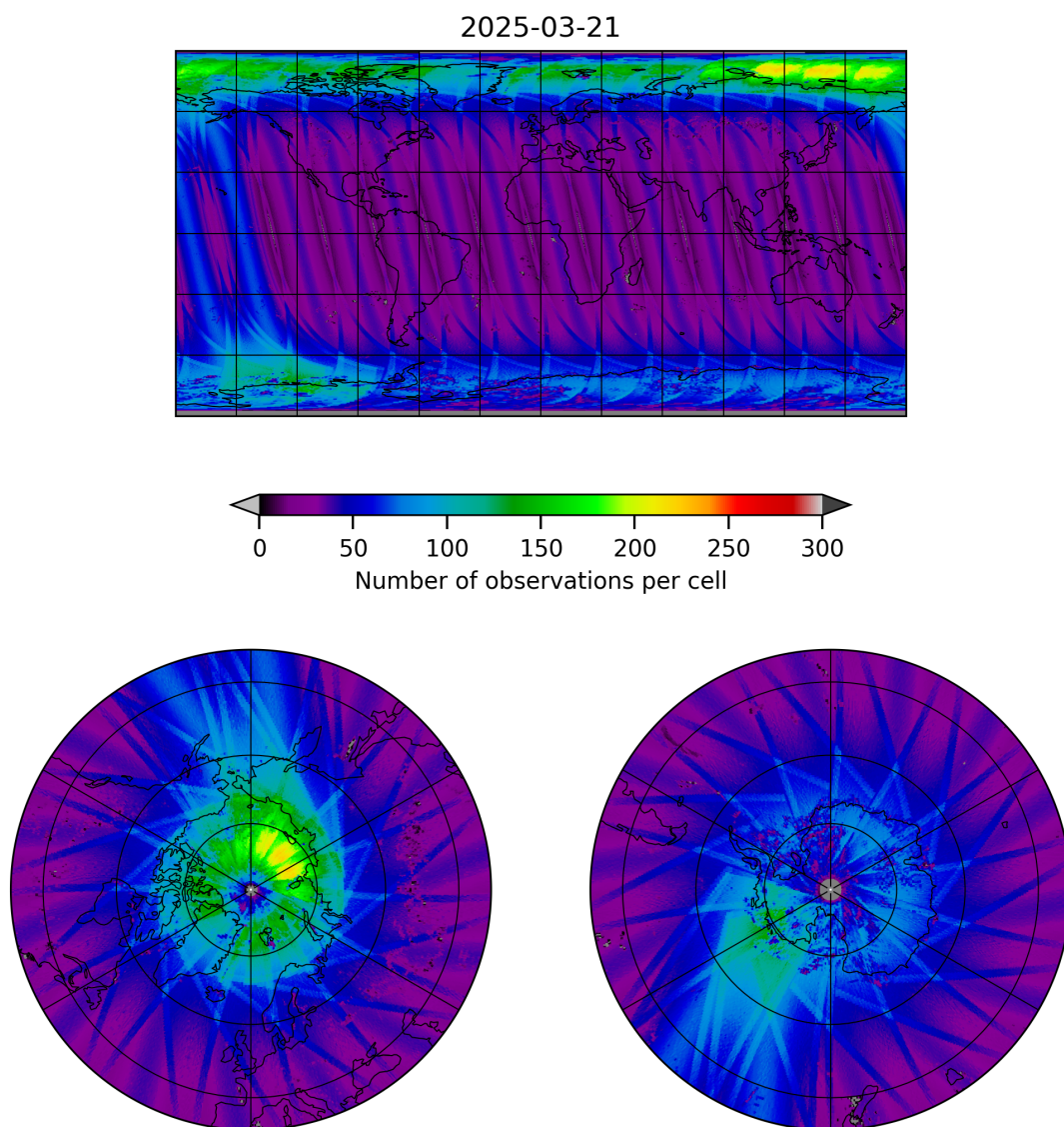
Figure 11: Map of the number of observations for 2025-03-20 to 2025-03-22
