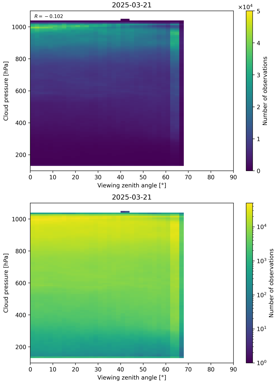
Figure 121: Scatter density plot of “Viewing zenith angle” against “Cloud pressure” for 2025-03-20 to 2025-03-22.
