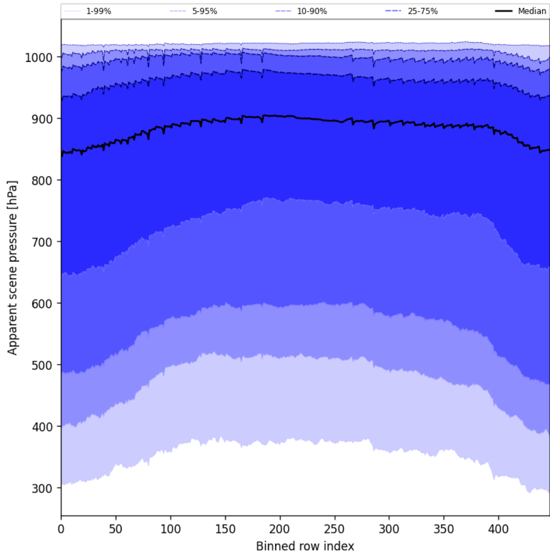
Figure 53: Along track statistics of “Apparent scene pressure” for 2025-03-20 to 2025-03-22
