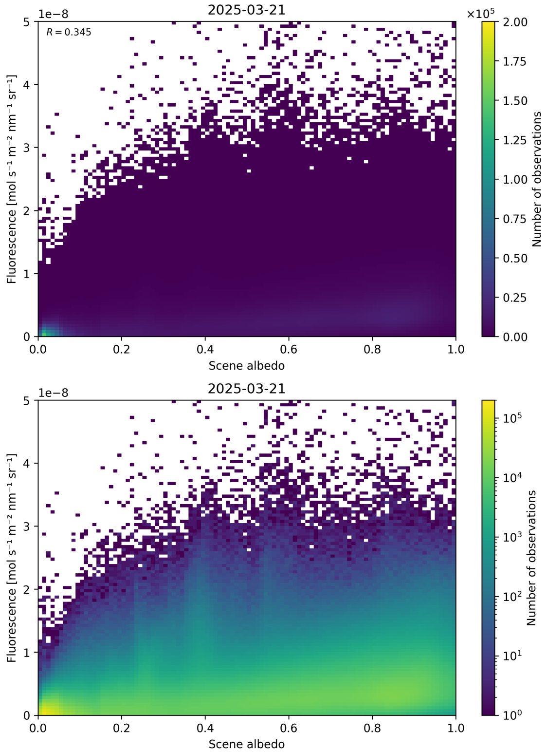
Figure 104: Scatter density plot of “Scene albedo” against “Fluorescence” for 2025-03-20 to 2025-03-22.
