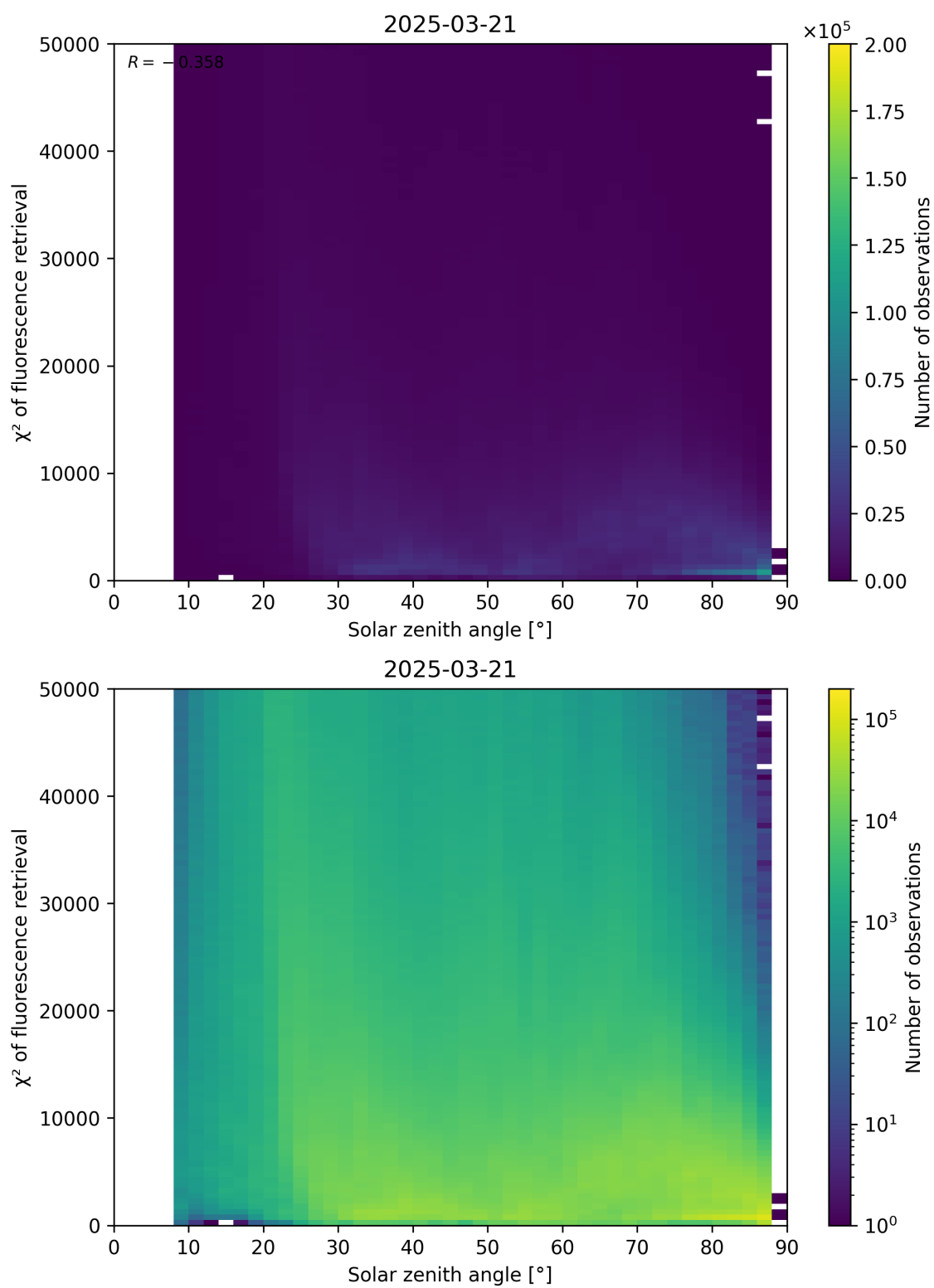
Figure 109: Scatter density plot of “Solar zenith angle” against “ \chi^2 of fluorescence retrieval” for 2025-03-20 to 2025-03-22.
