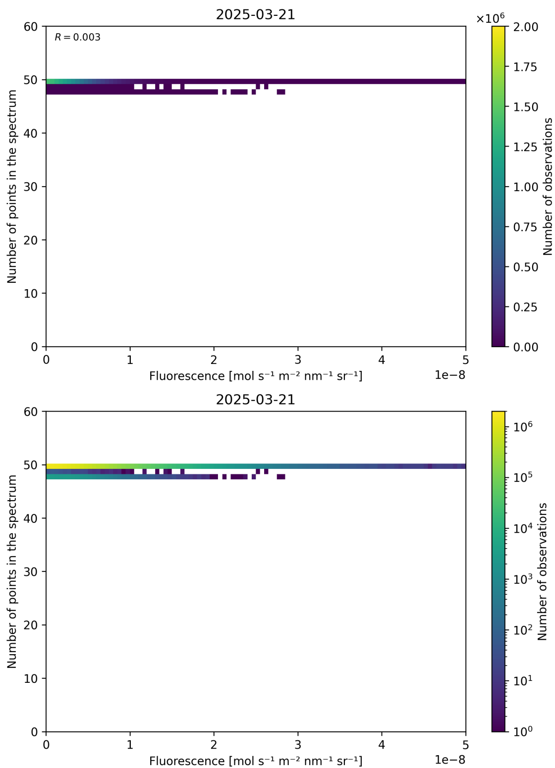
Figure 86: Scatter density plot of “Fluorescence” against “Number of points in the spectrum” for 2025-03-20 to 2025-03-22.
