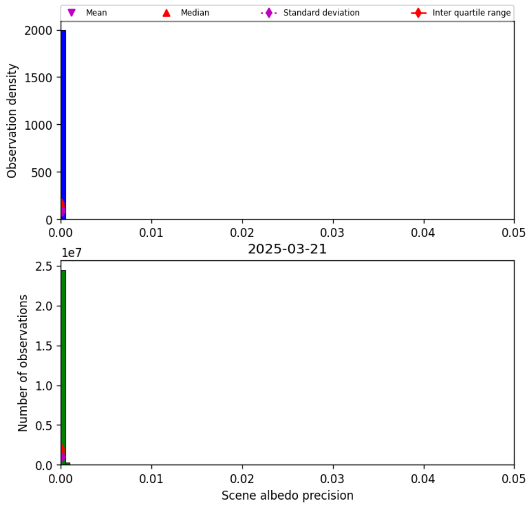
Figure 35: Histogram of “Scene albedo precision” for 2025-03-20 to 2025-03-22
