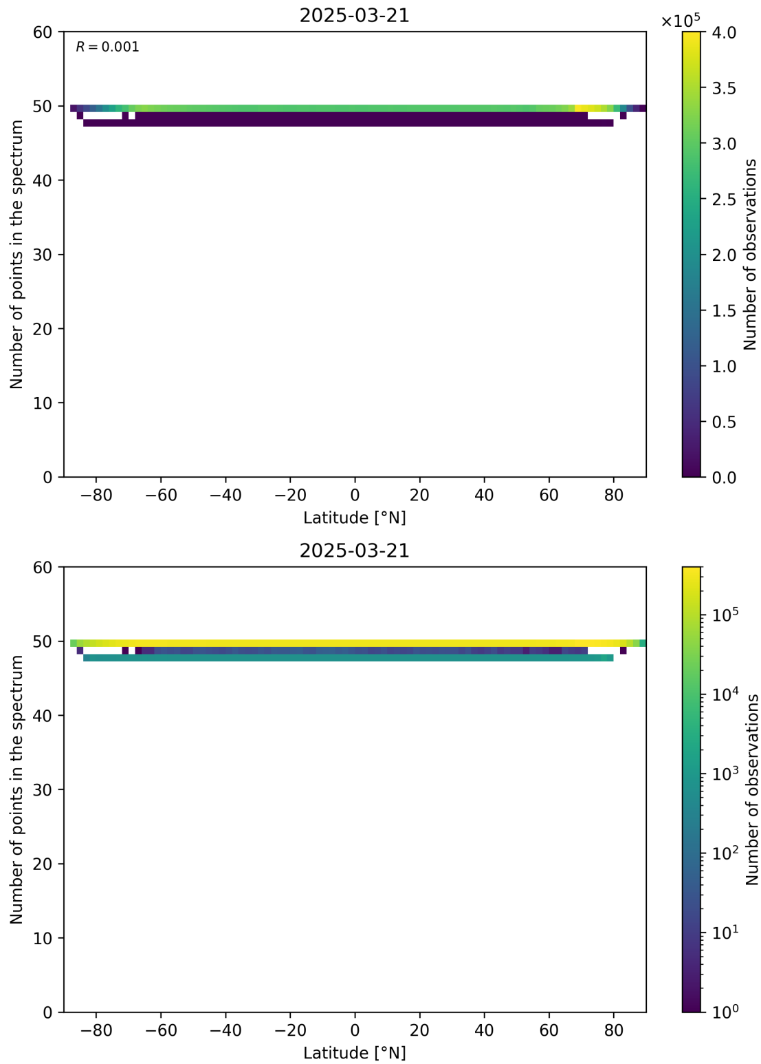
Figure 94: Scatter density plot of “Latitude” against “Number of points in the spectrum” for 2025-03-20 to 2025-03-22.
