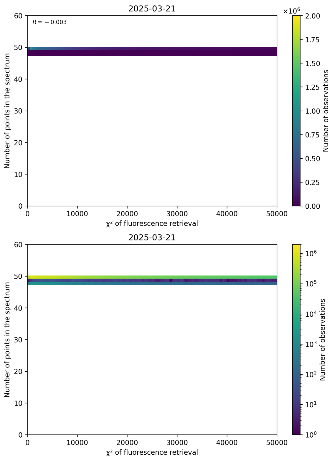
Figure 68: Scatter density plot of “ \chi^2 of fluorescence retrieval” against “Number of points in the spectrum” for 2025-03-20 to 2025-03-22.
