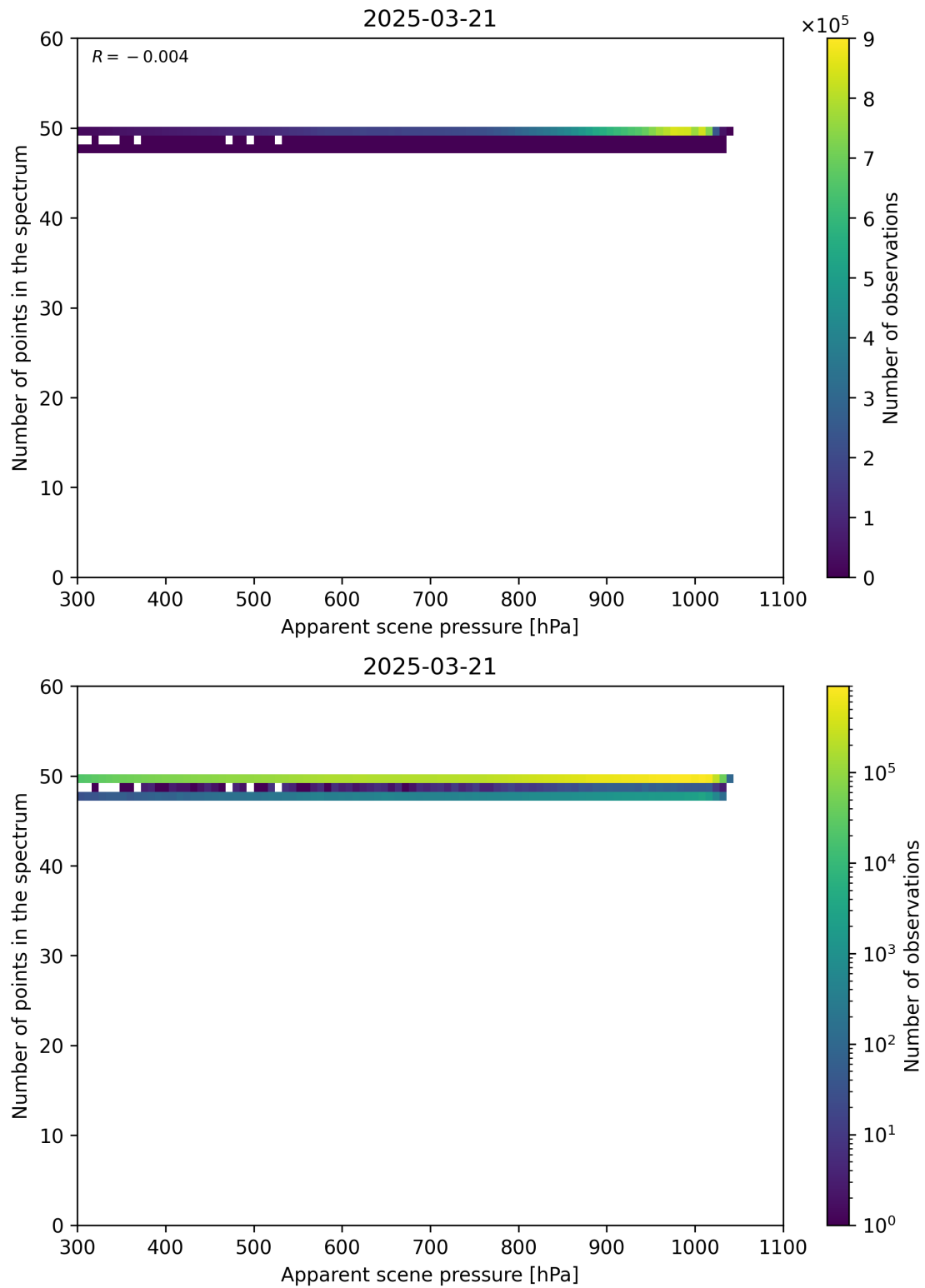
Figure 66: Scatter density plot of “Apparent scene pressure” against “Number of points in the spectrum” for 2025-03-20 to 2025-03-22.
