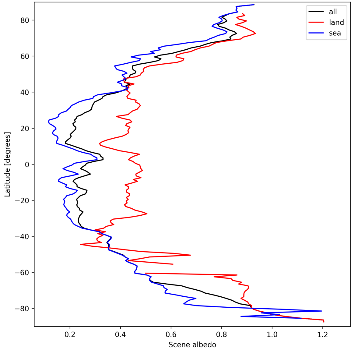
Figure 17: Zonal average of “Scene albedo” for 2025-03-20 to 2025-03-22.
