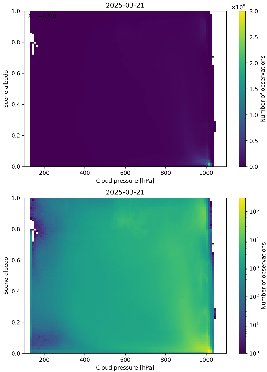
Figure 83: Scatter density plot of “Cloud pressure” against “Scene albedo” for 2025-03-20 to 2025-03-22.
