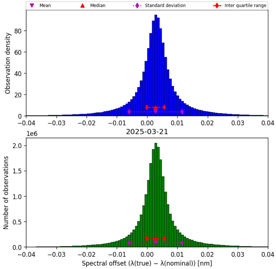
Figure 45: Histogram of “Spectral offset ( \lambda_{\text{true}} - \lambda_{\text{nominal}} )” for 2025-03-20 to 2025-03-22
