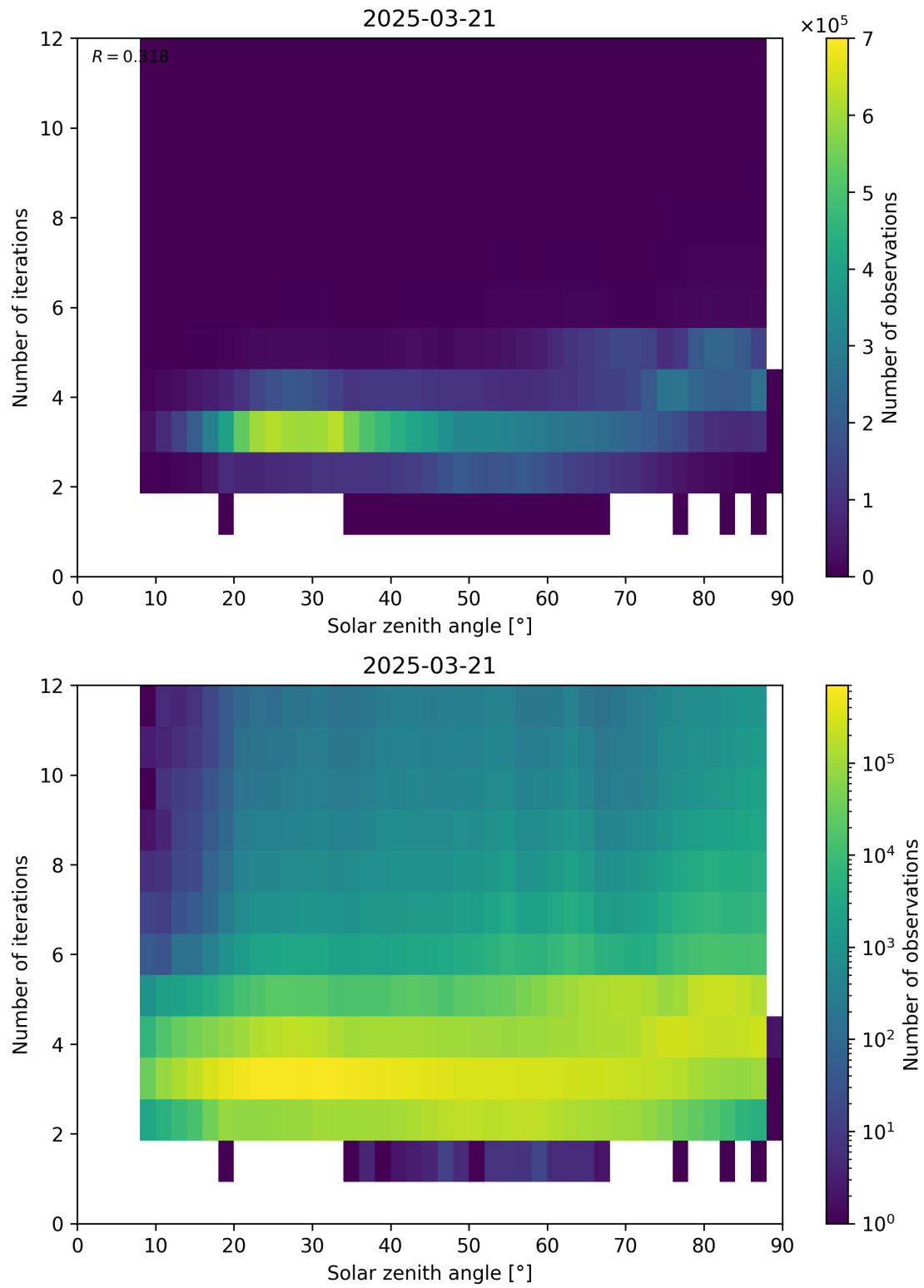
Figure 114: Scatter density plot of “Solar zenith angle” against “Number of iterations” for 2025-03-20 to 2025-03-22.
