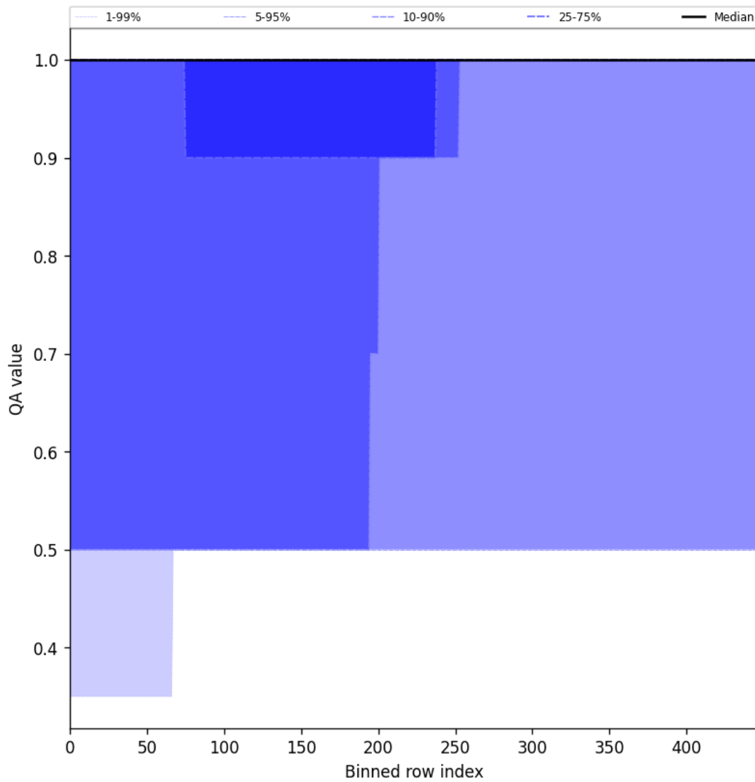
Figure 46: Along track statistics of “QA value” for 2025-03-20 to 2025-03-22
