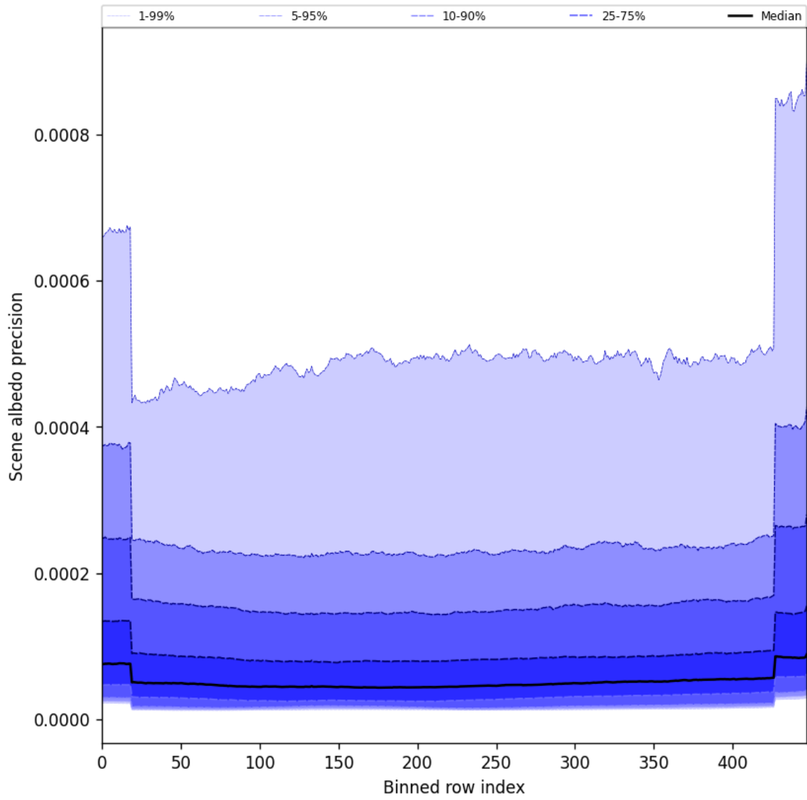
Figure 52: Along track statistics of “Scene albedo precision” for 2025-03-20 to 2025-03-22
