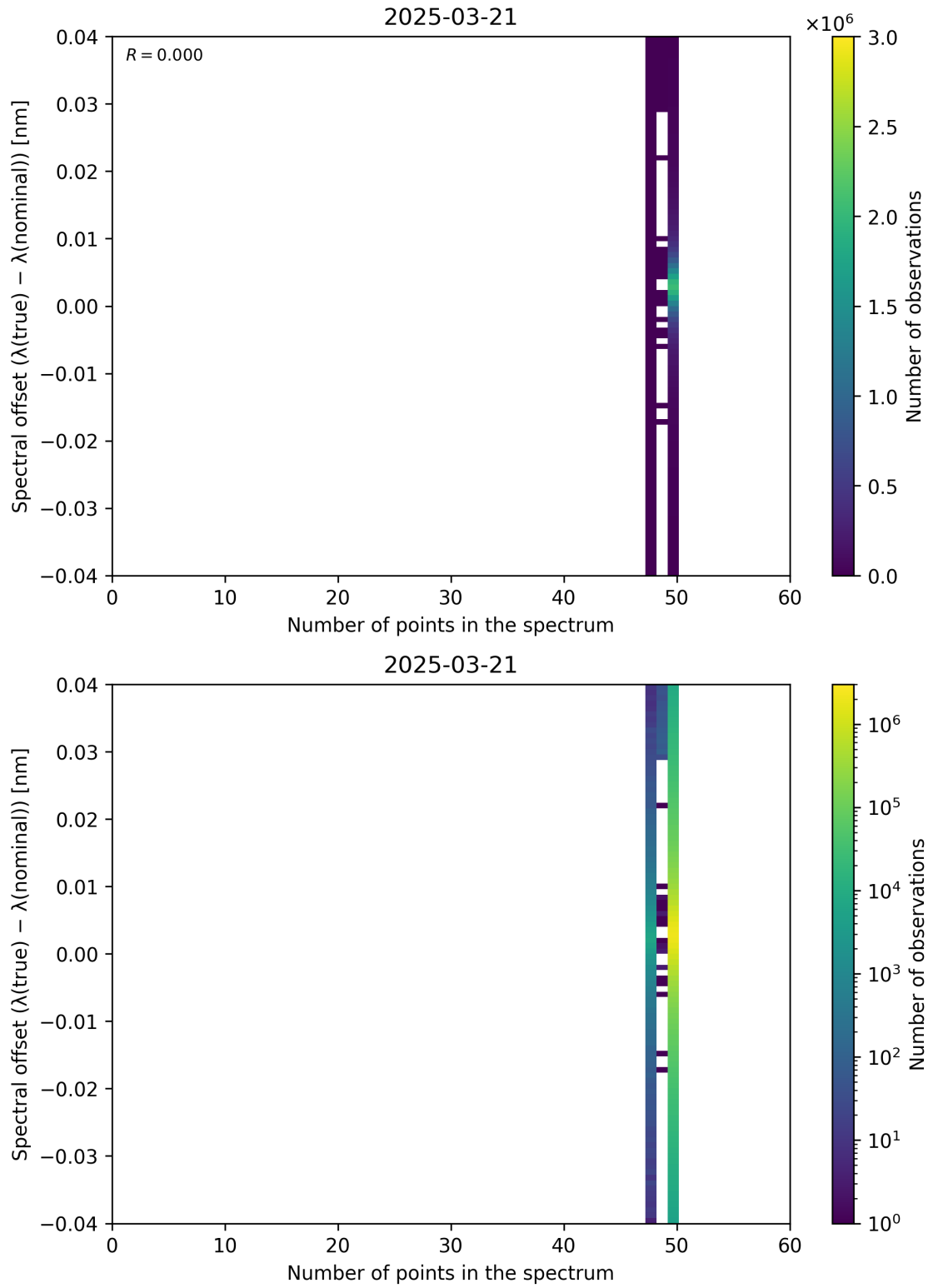
Figure 101: Scatter density plot of “Number of points in the spectrum” against “Spectral offset ( \lambda_{\text{true}} - \lambda_{\text{nominal}} )” for 2025-03-20 to 2025-03-22.
