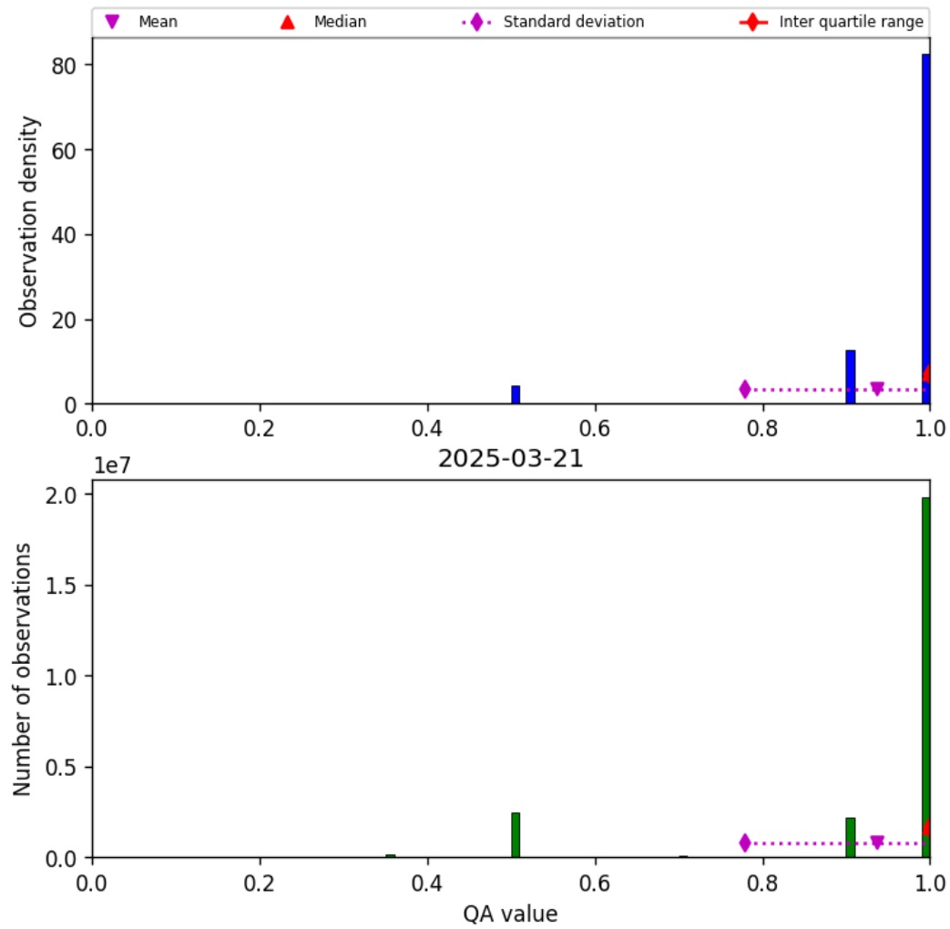
Figure 29: Histogram of “QA value” for 2025-03-20 to 2025-03-22
