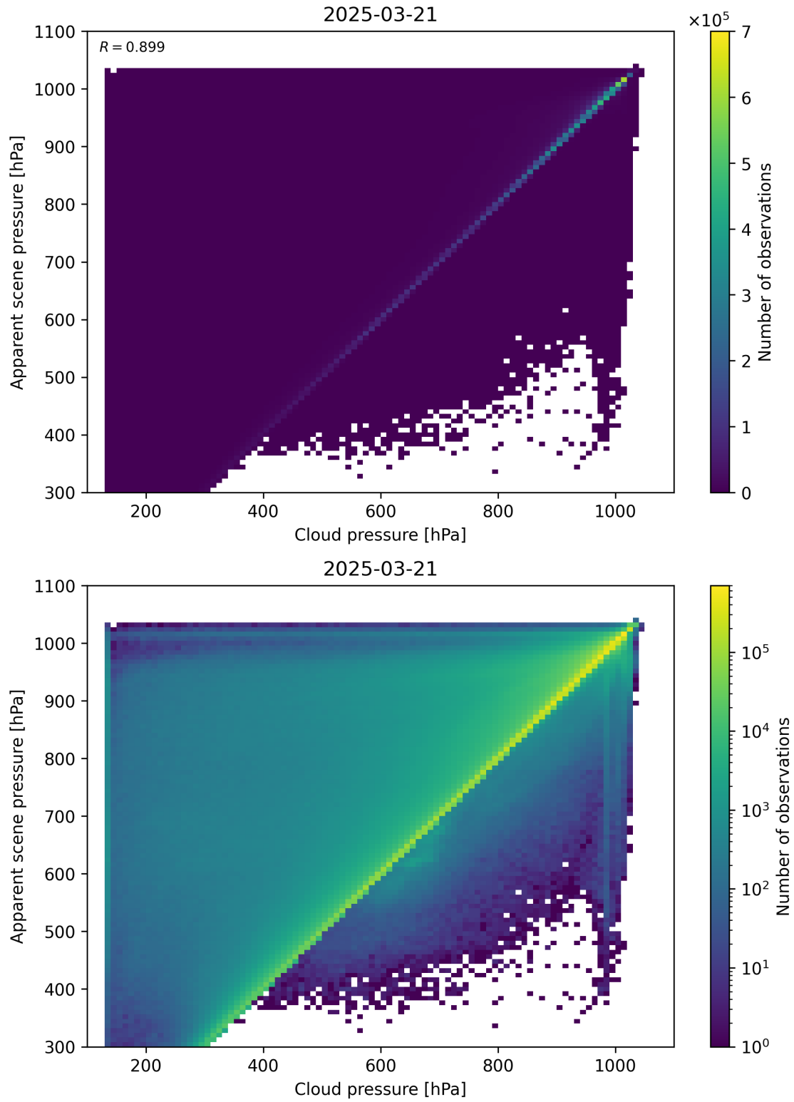
Figure 77: Scatter density plot of “Cloud pressure” against “Apparent scene pressure” for 2025-03-20 to 2025-03-22.
