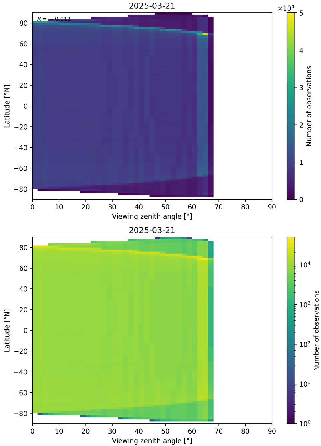
Figure 123: Scatter density plot of “Viewing zenith angle” against “Latitude” for 2025-03-20 to 2025-03-22.
