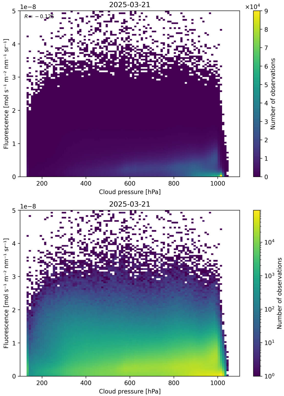
Figure 80: Scatter density plot of “Cloud pressure” against “Fluorescence” for 2025-03-20 to 2025-03-22.
