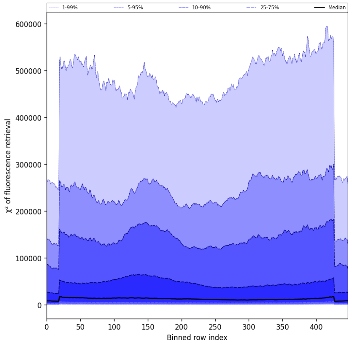
Figure 59: Along track statistics of “ \chi^2 of fluorescence retrieval” for 2025-03-20 to 2025-03-22
