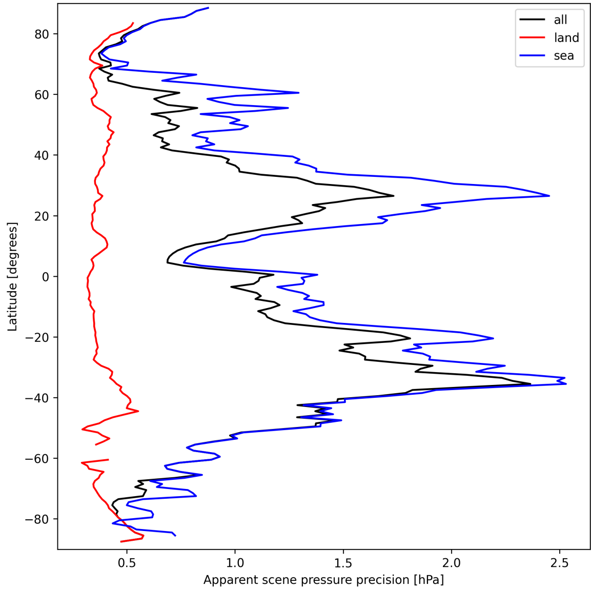
Figure 20: Zonal average of “Apparent scene pressure precision” for 2025-03-20 to 2025-03-22.
