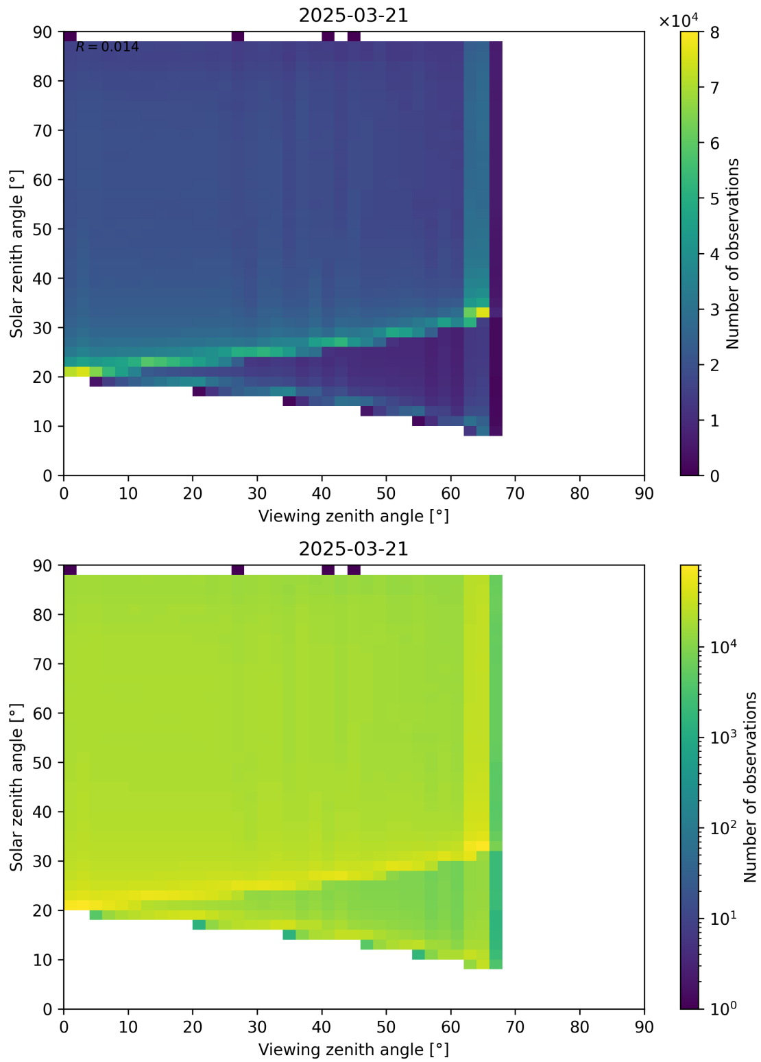
Figure 127: Scatter density plot of “Viewing zenith angle” against “Solar zenith angle” for 2025-03-20 to 2025-03-22.
