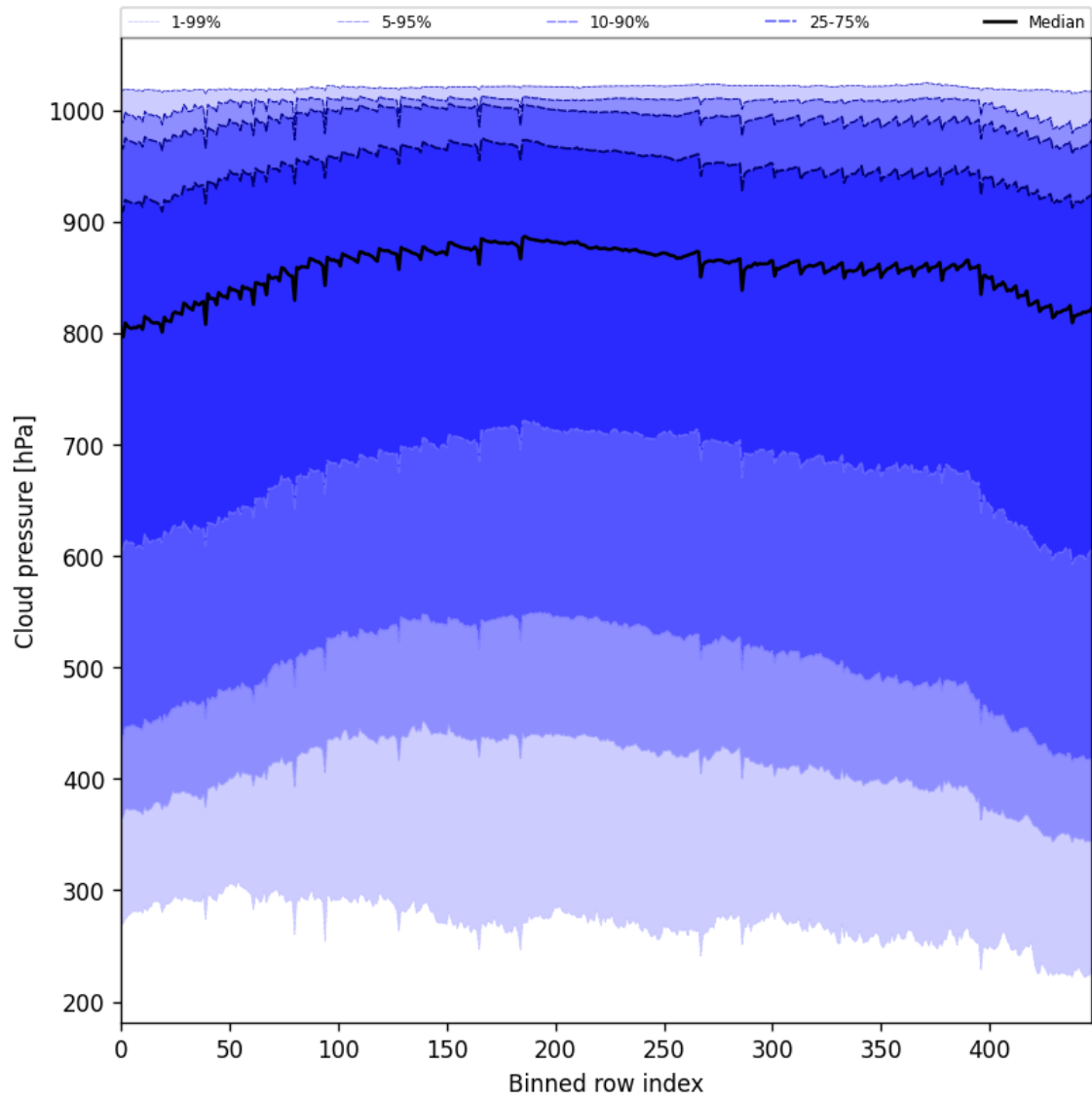
Figure 47: Along track statistics of “Cloud pressure” for 2025-03-20 to 2025-03-22
