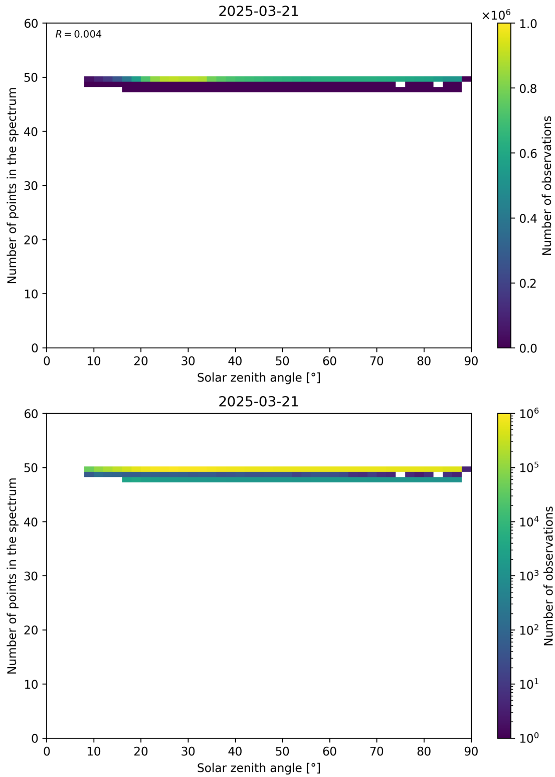
Figure 115: Scatter density plot of “Solar zenith angle” against “Number of points in the spectrum” for 2025-03-20 to 2025-03-22.
