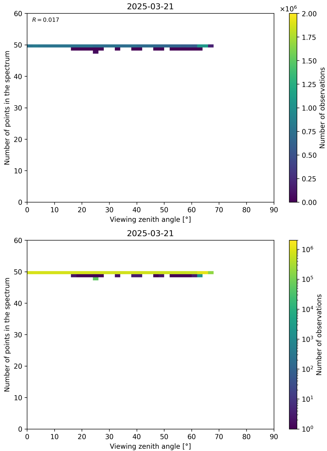
Figure 125: Scatter density plot of “Viewing zenith angle” against “Number of points in the spectrum” for 2025-03-20 to 2025-03-22.
