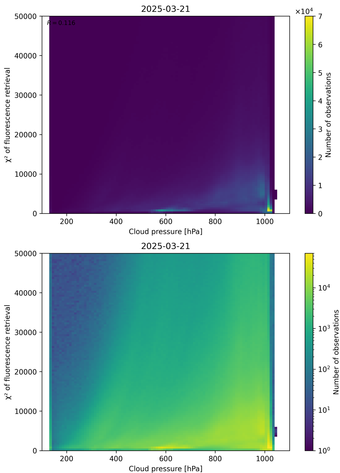
Figure 78: Scatter density plot of “Cloud pressure” against “ \chi^2 of fluorescence retrieval” for 2025-03-20 to 2025-03-22.
