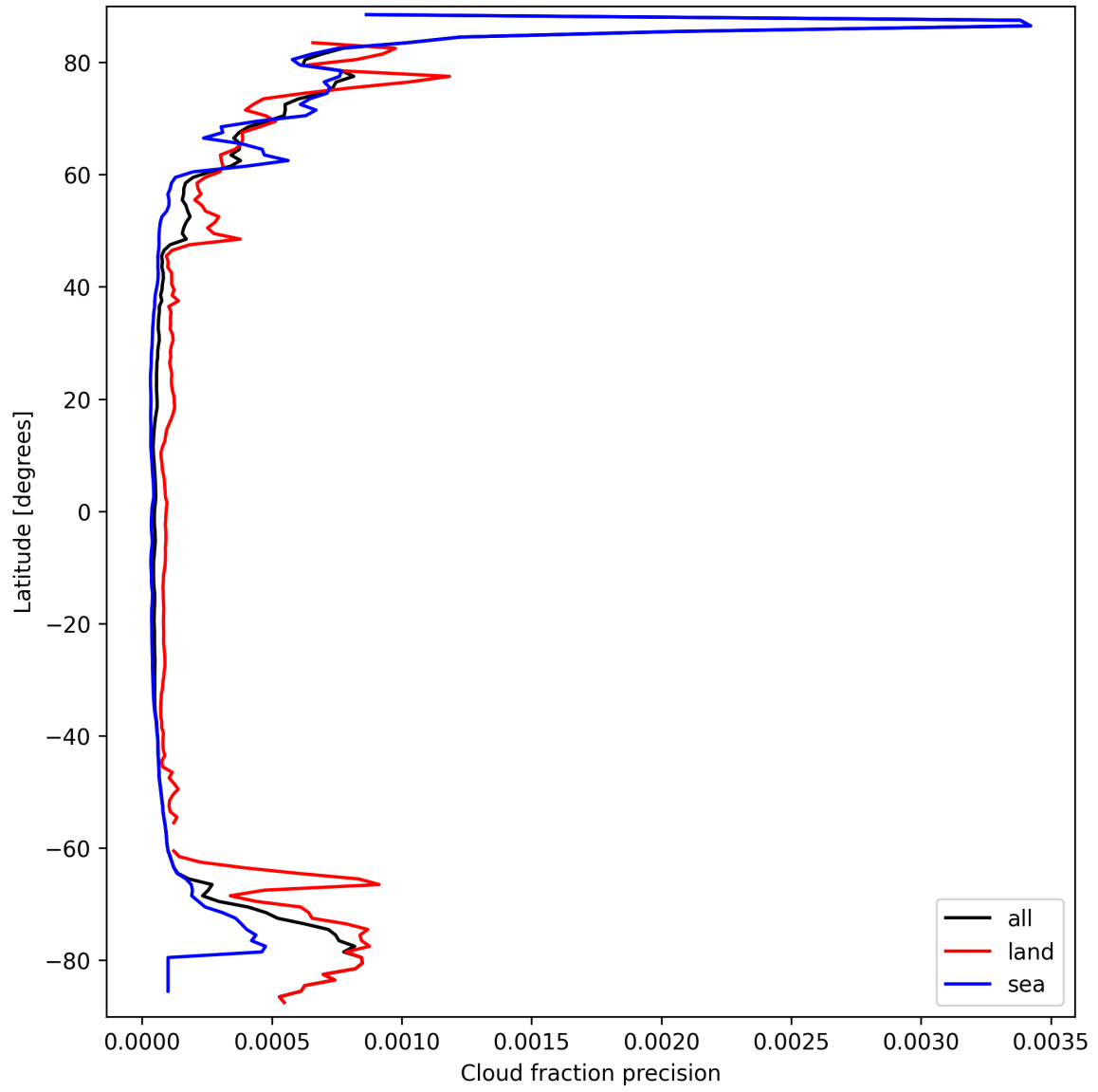
Figure 16: Zonal average of “Cloud fraction precision” for 2025-03-20 to 2025-03-22.
