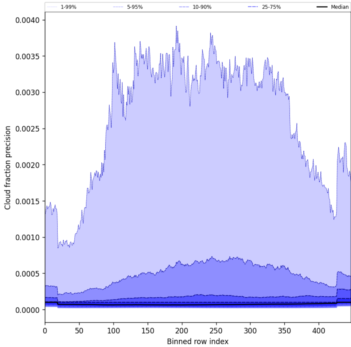
Figure 50: Along track statistics of “Cloud fraction precision” for 2025-03-20 to 2025-03-22
