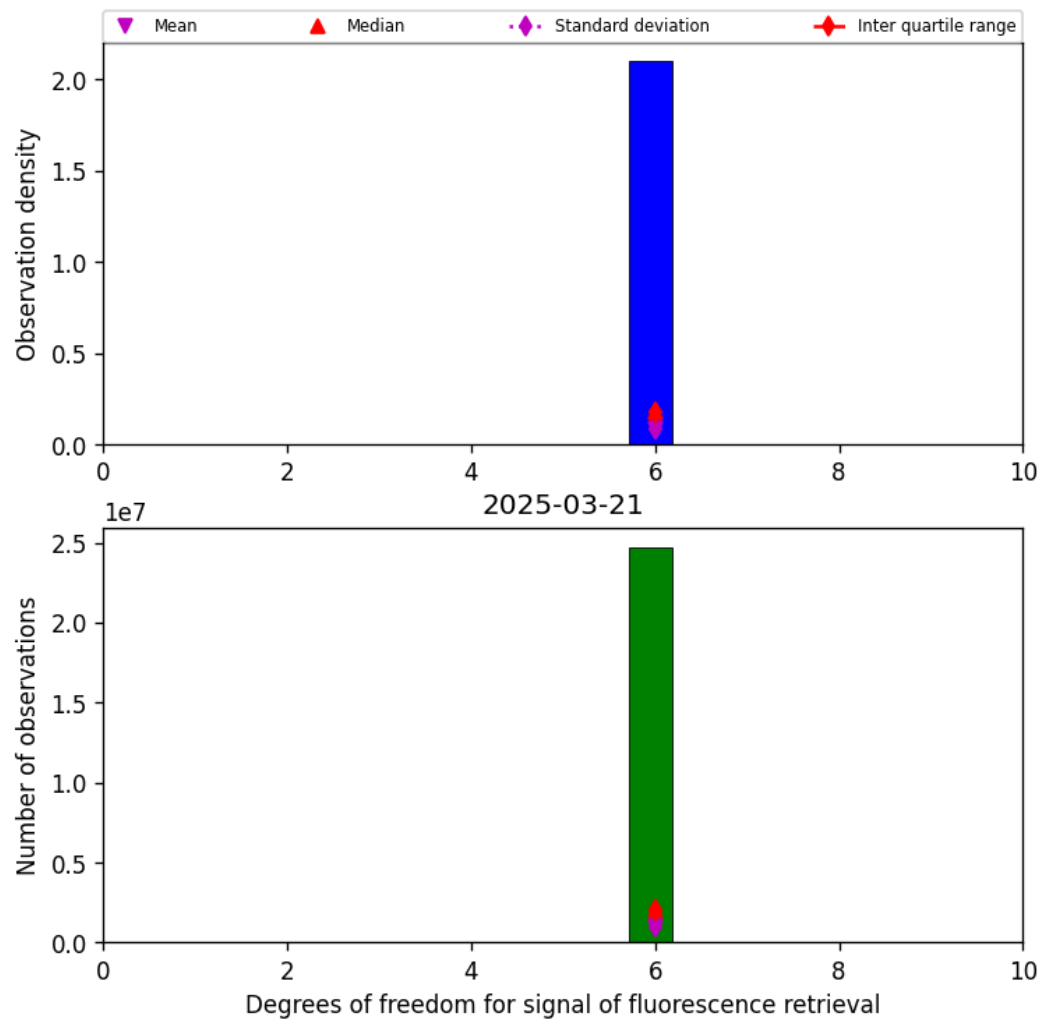
Figure 43: Histogram of “Degrees of freedom for signal of fluorescence retrieval” for 2025-03-20 to 2025-03-22
