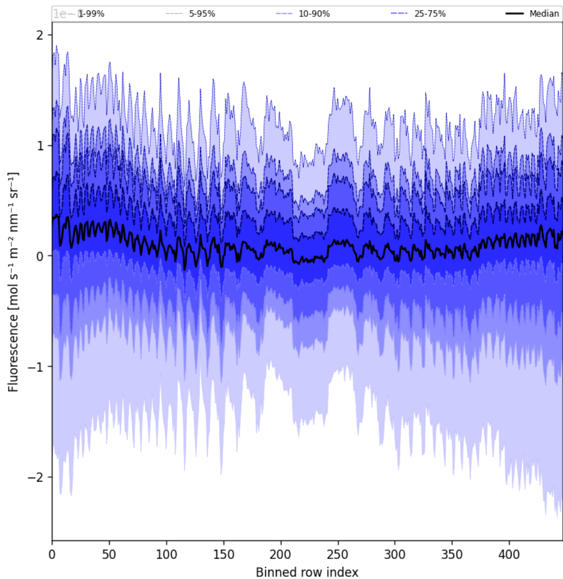
Figure 57: Along track statistics of “Fluorescence” for 2025-03-20 to 2025-03-22
