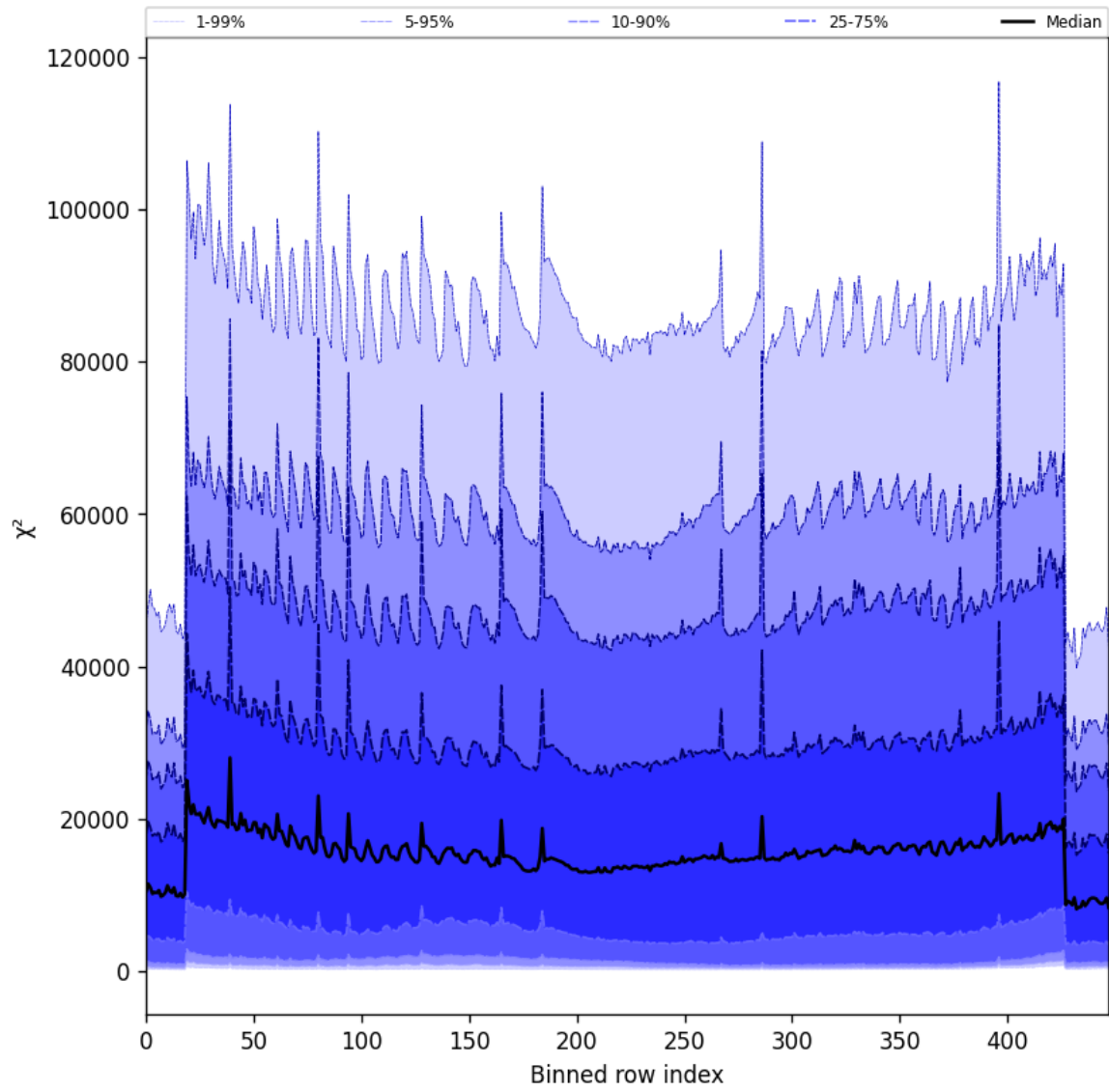
Figure 55: Along track statistics of “ \chi^2 ” for 2025-03-20 to 2025-03-22
