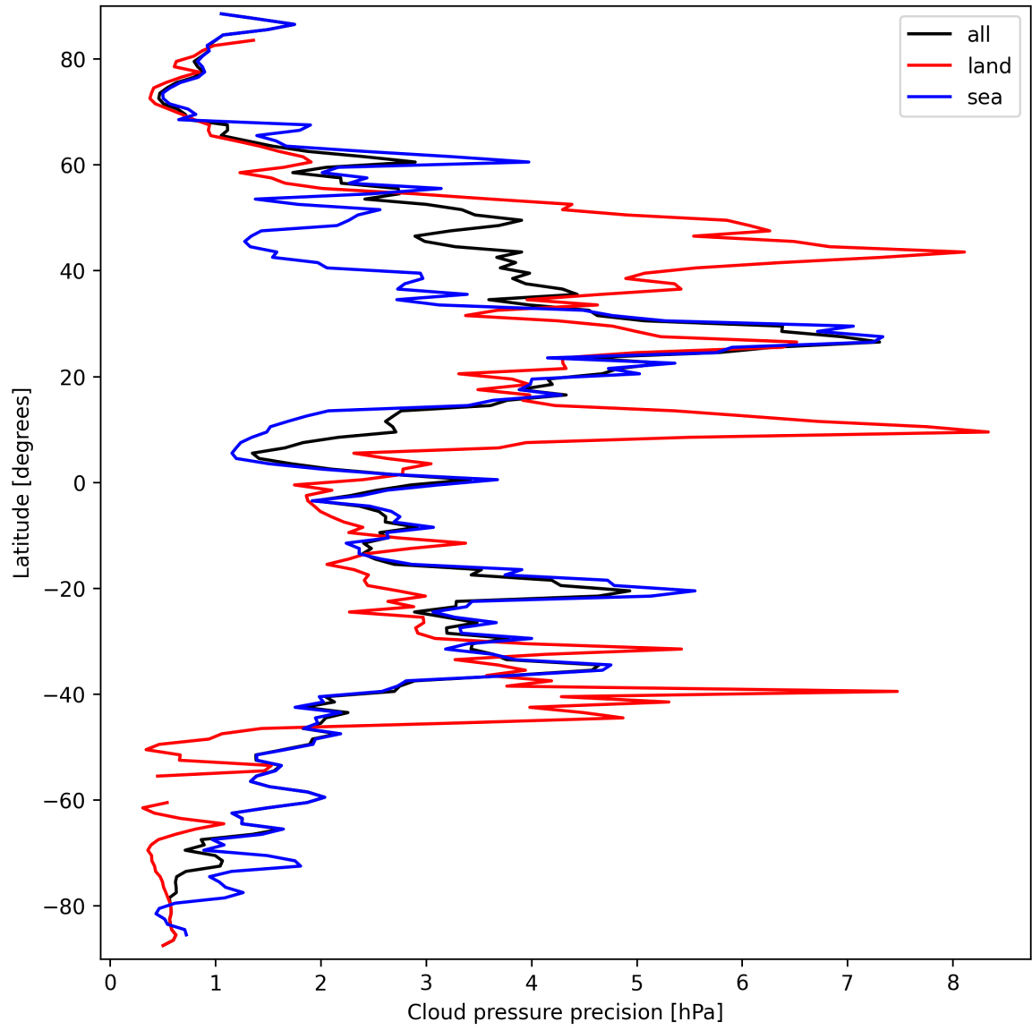
Figure 14: Zonal average of “Cloud pressure precision” for 2025-03-20 to 2025-03-22.
