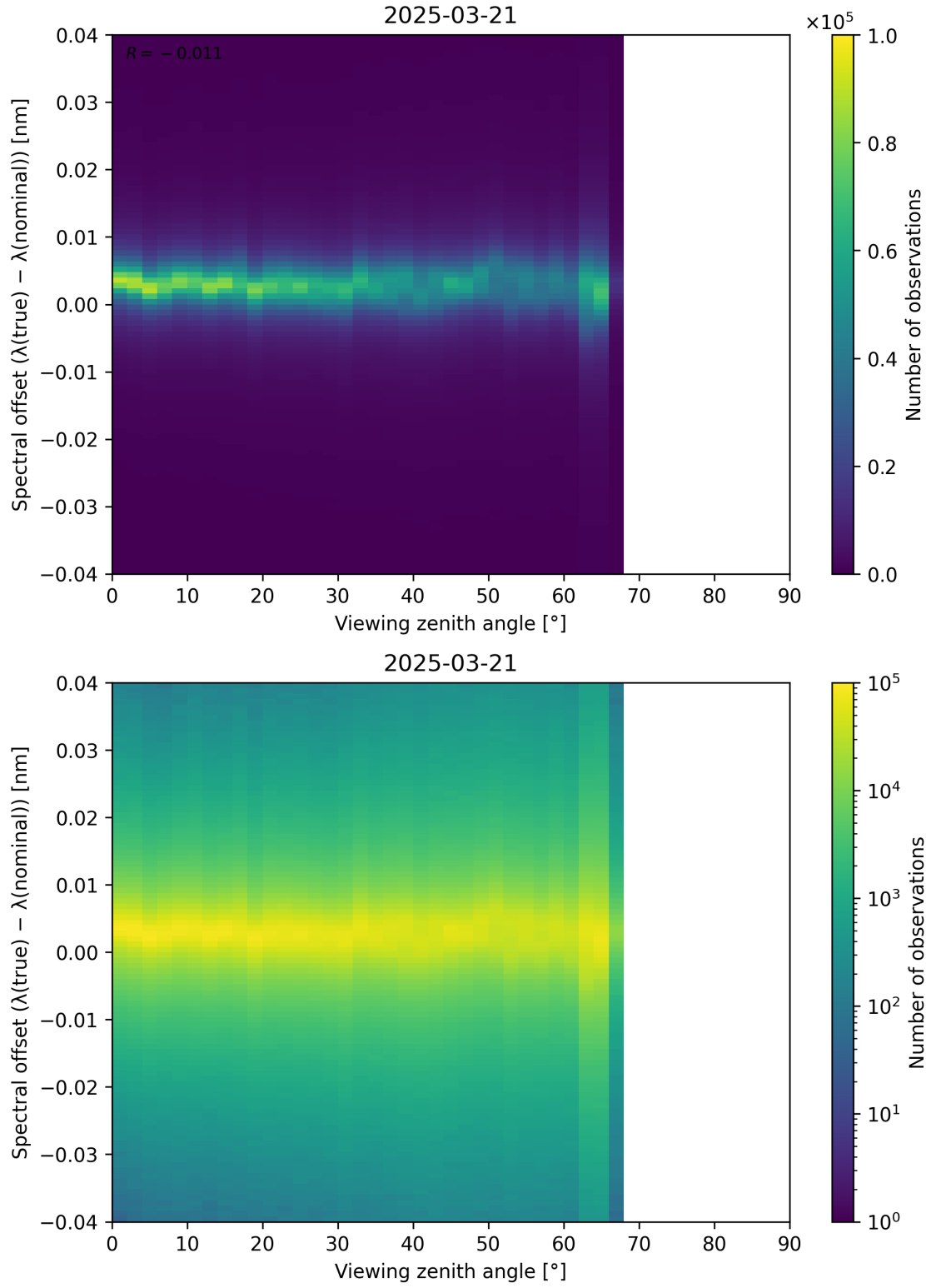
Figure 128: Scatter density plot of “Viewing zenith angle” against “Spectral offset ( \lambda_{\text{true}} - \lambda_{\text{nominal}} )” for 2025-03-20 to 2025-03-22.
