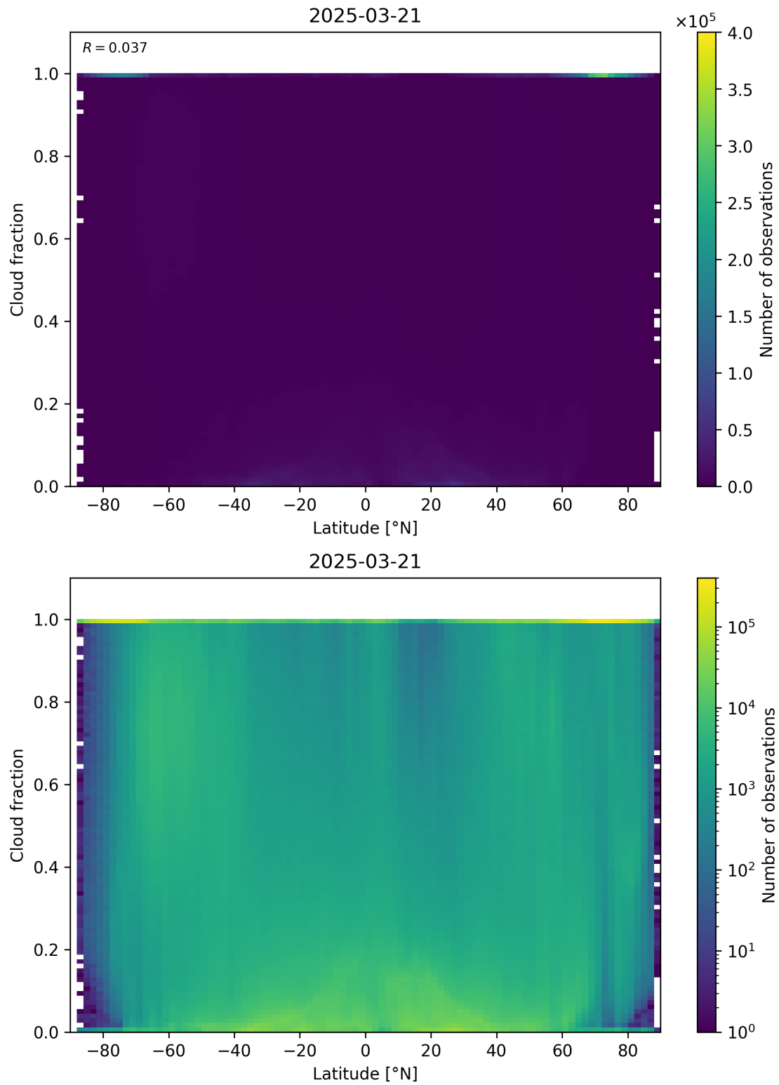
Figure 90: Scatter density plot of “Latitude” against “Cloud fraction” for 2025-03-20 to 2025-03-22.
