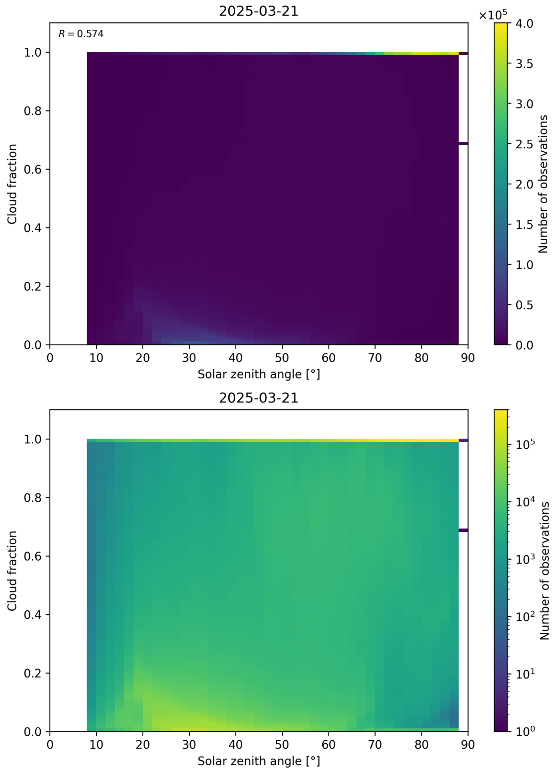
Figure 110: Scatter density plot of “Solar zenith angle” against “Cloud fraction” for 2025-03-20 to 2025-03-22.
