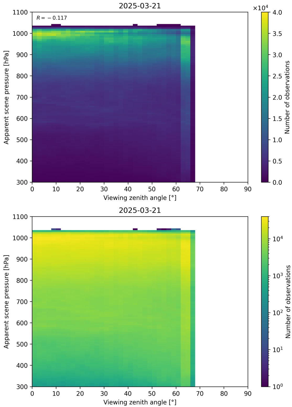
Figure 118: Scatter density plot of “Viewing zenith angle” against “Apparent scene pressure” for 2025-03-20 to 2025-03-22.
