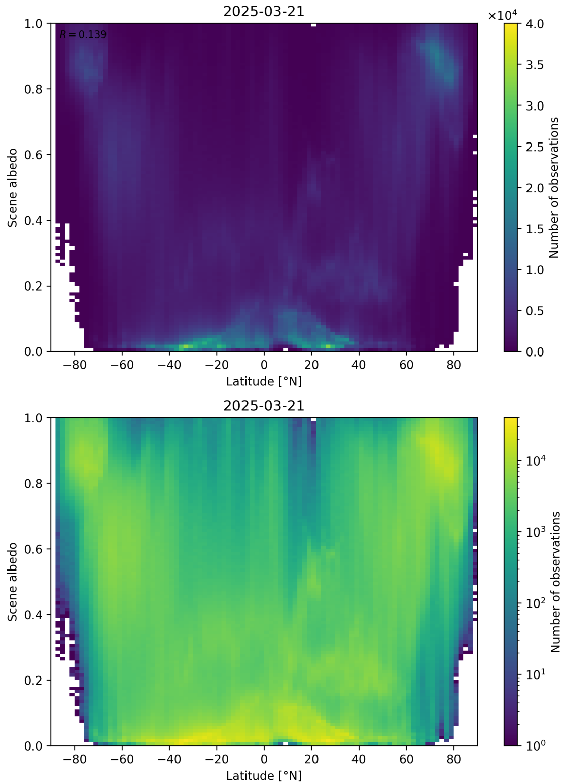
Figure 95: Scatter density plot of “Latitude” against “Scene albedo” for 2025-03-20 to 2025-03-22.
