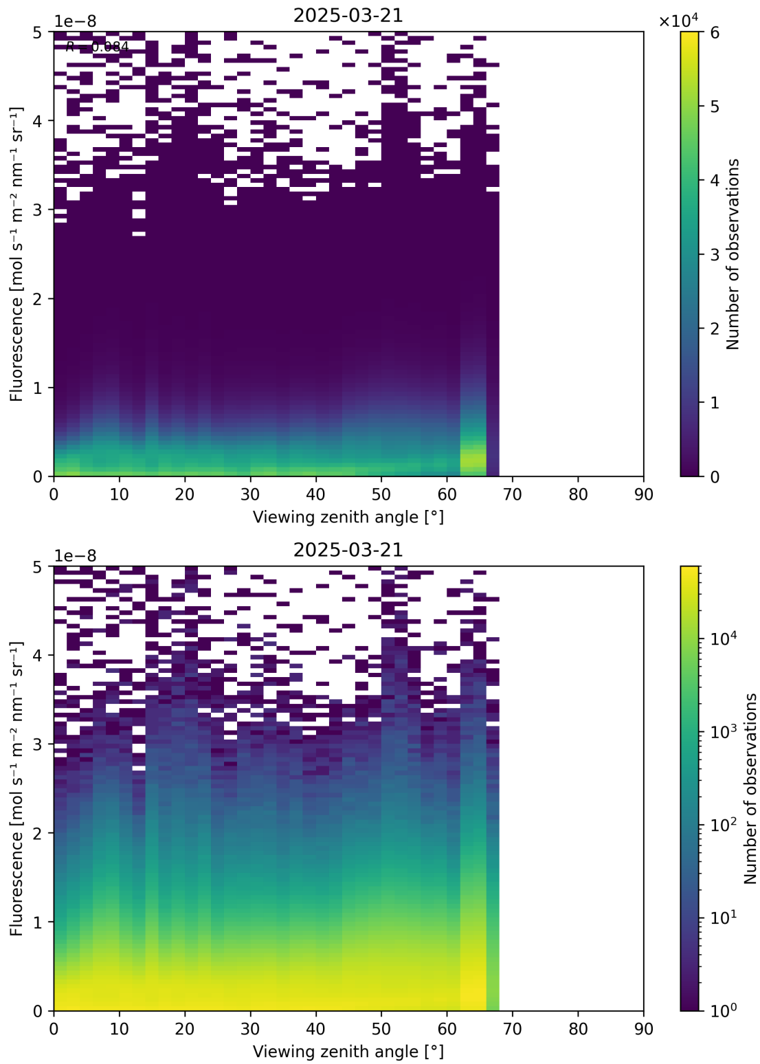
Figure 122: Scatter density plot of “Viewing zenith angle” against “Fluorescence” for 2025-03-20 to 2025-03-22.
