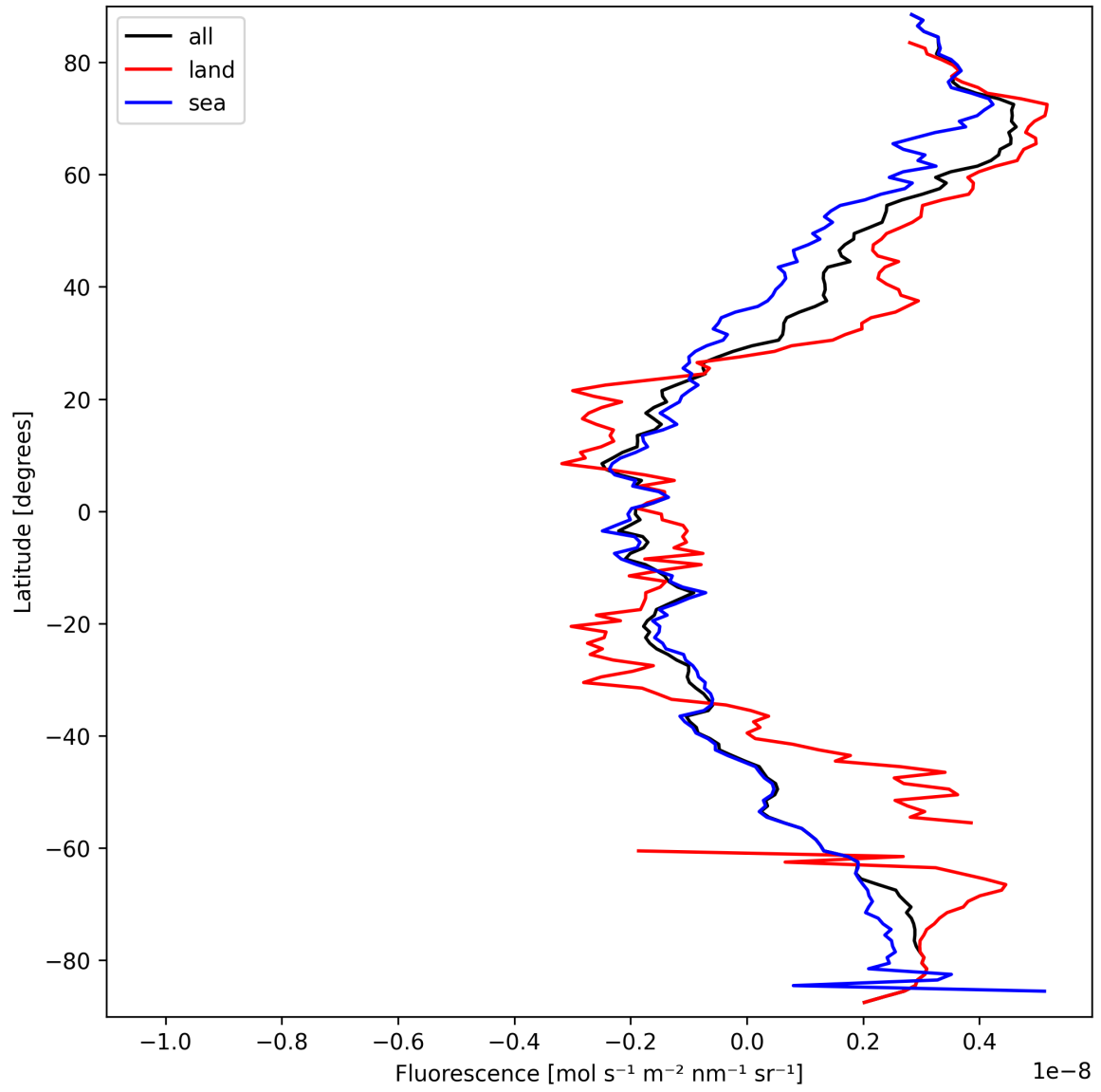
Figure 23: Zonal average of “Fluorescence” for 2025-03-20 to 2025-03-22.
