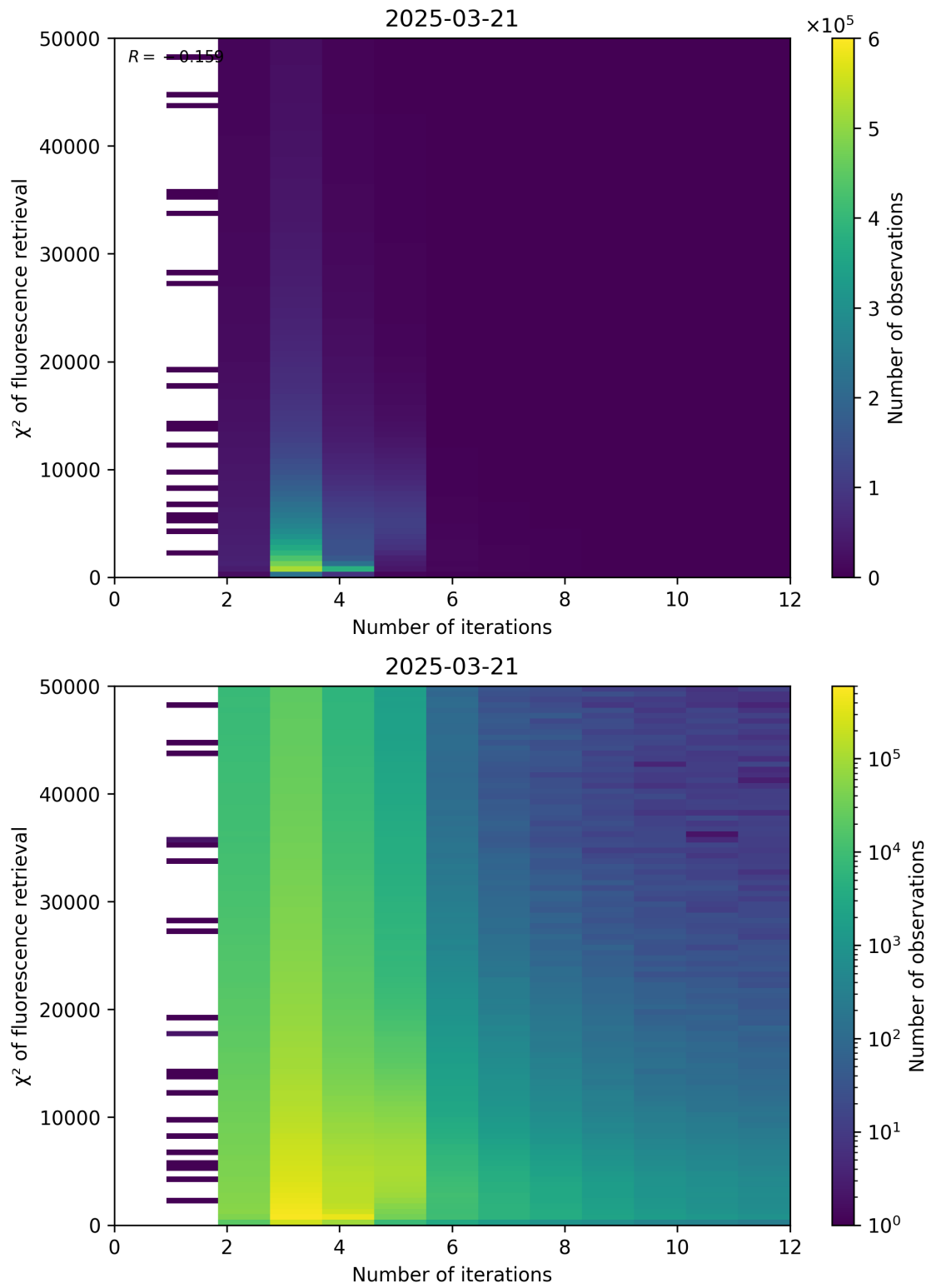
Figure 97: Scatter density plot of “Number of iterations” against “ \chi^2 of fluorescence retrieval” for 2025-03-20 to 2025-03-22.
