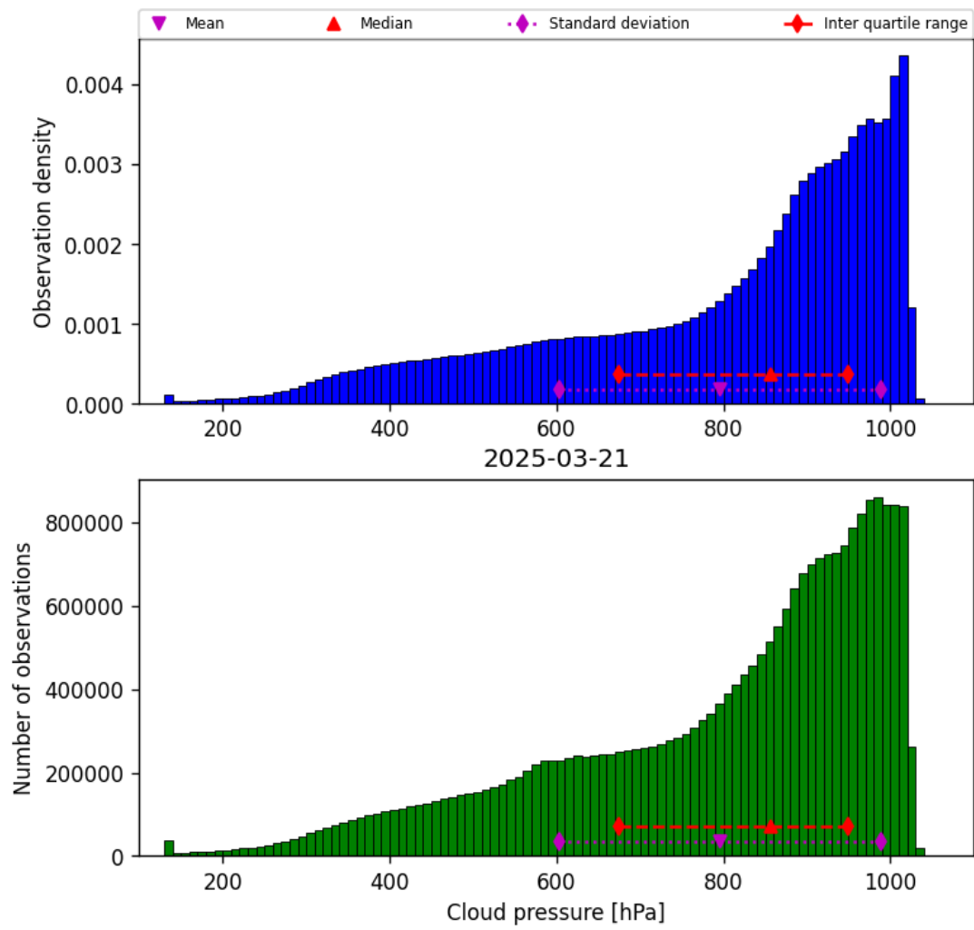
Figure 30: Histogram of “Cloud pressure” for 2025-03-20 to 2025-03-22
