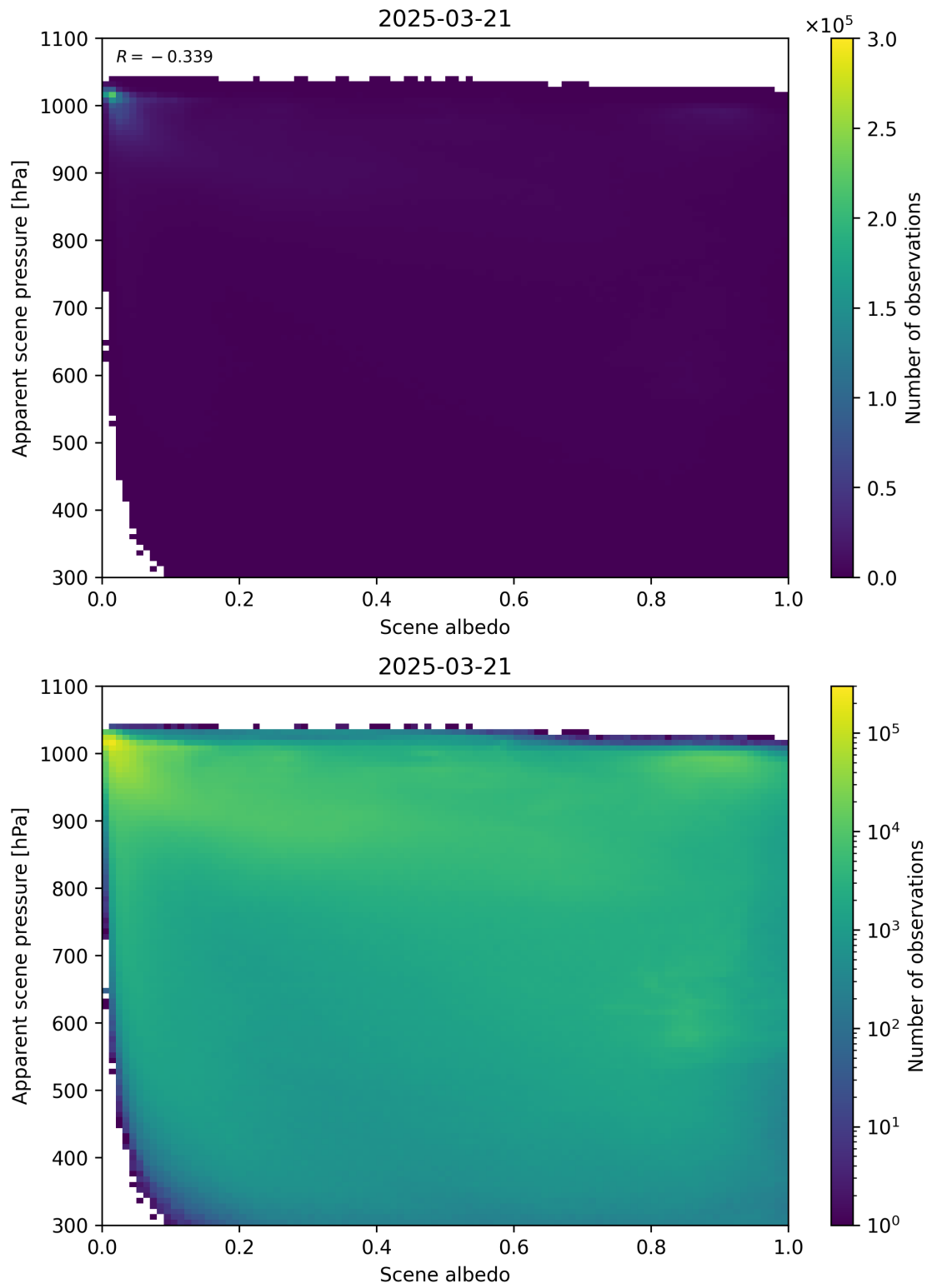
Figure 102: Scatter density plot of “Scene albedo” against “Apparent scene pressure” for 2025-03-20 to 2025-03-22.
