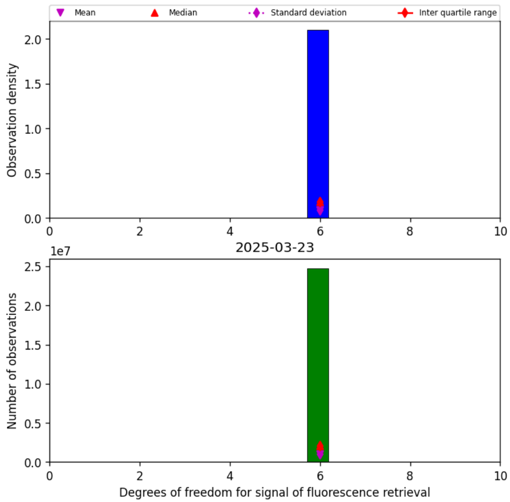
Figure 43: Histogram of “Degrees of freedom for signal of fluorescence retrieval” for 2025-03-23 to 2025-03-24
