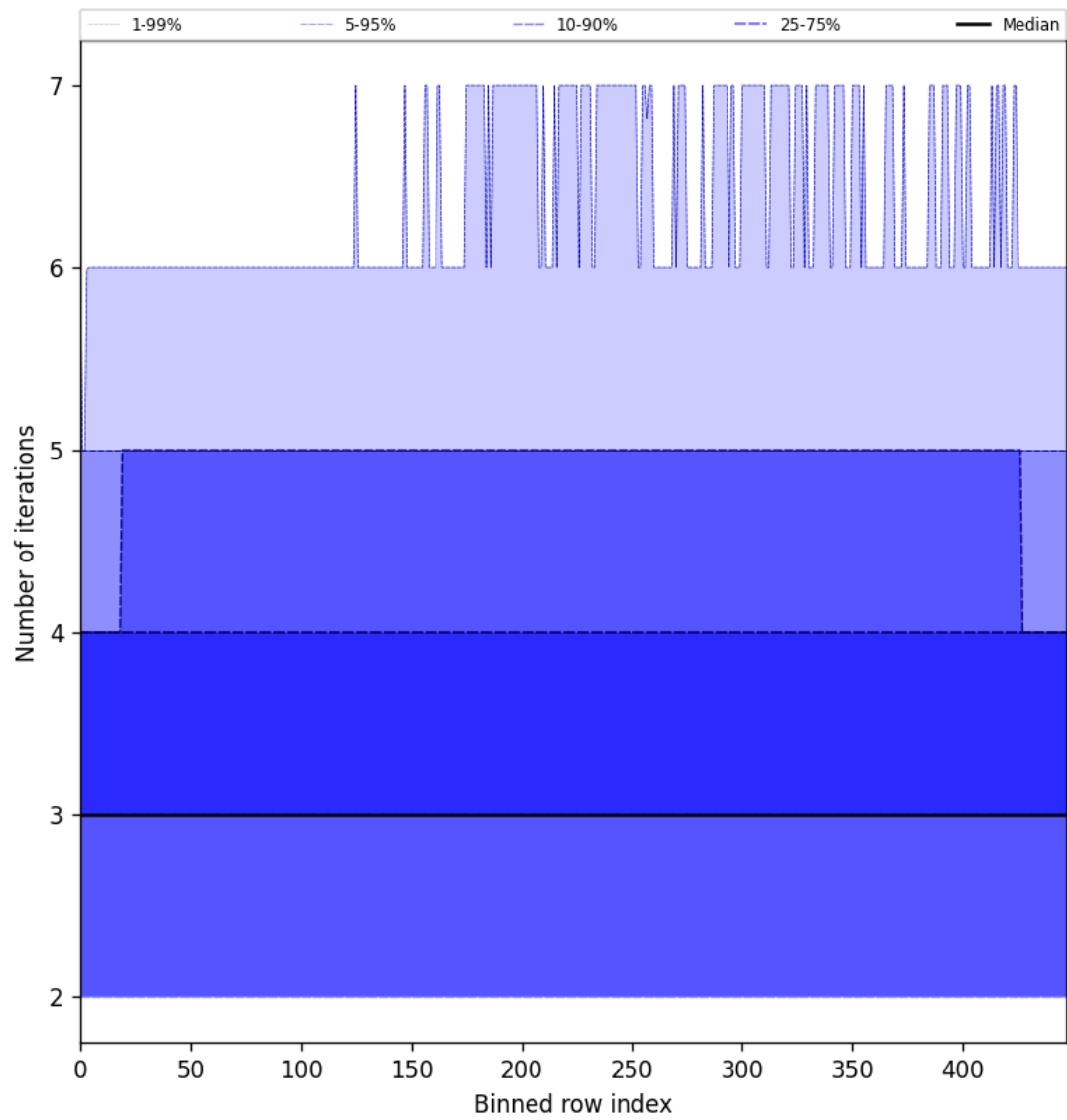
Figure 56: Along track statistics of “Number of iterations” for 2025-03-23 to 2025-03-24
