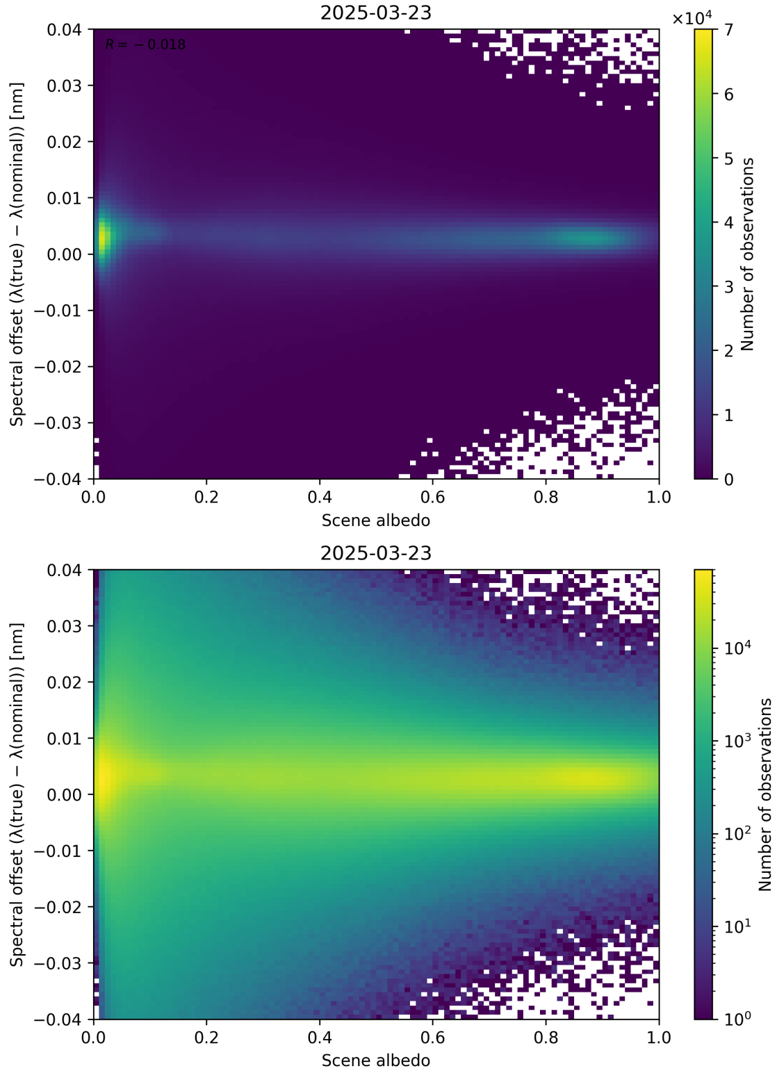
Figure 107: Scatter density plot of “Scene albedo” against “Spectral offset ( \lambda_{\text{true}} - \lambda_{\text{nominal}} )” for 2025-03-23 to 2025-03-24.
