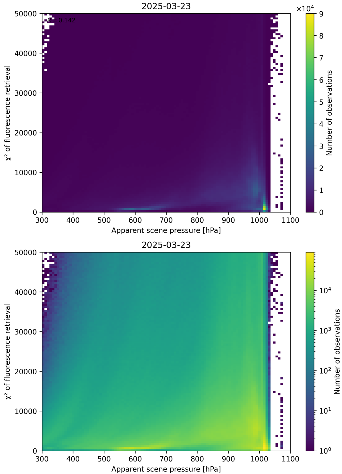
Figure 63: Scatter density plot of “Apparent scene pressure” against “ \chi^2 of fluorescence retrieval” for 2025-03-23 to 2025-03-24.
