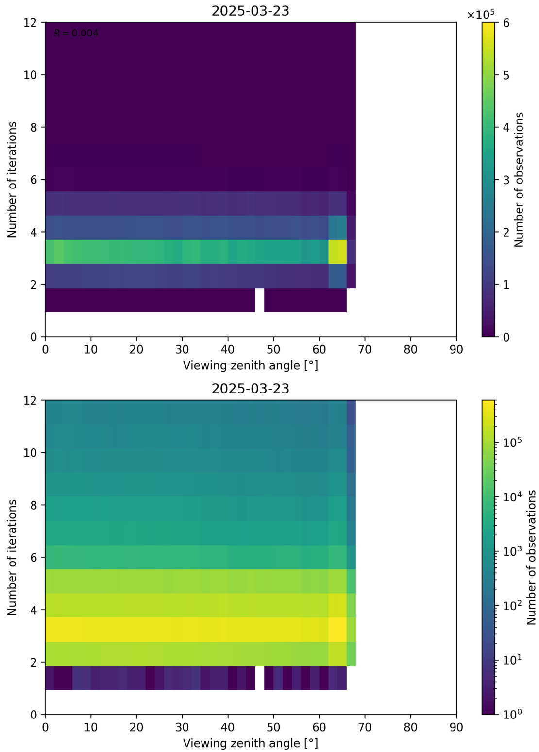
Figure 124: Scatter density plot of “Viewing zenith angle” against “Number of iterations” for 2025-03-23 to 2025-03-24.
