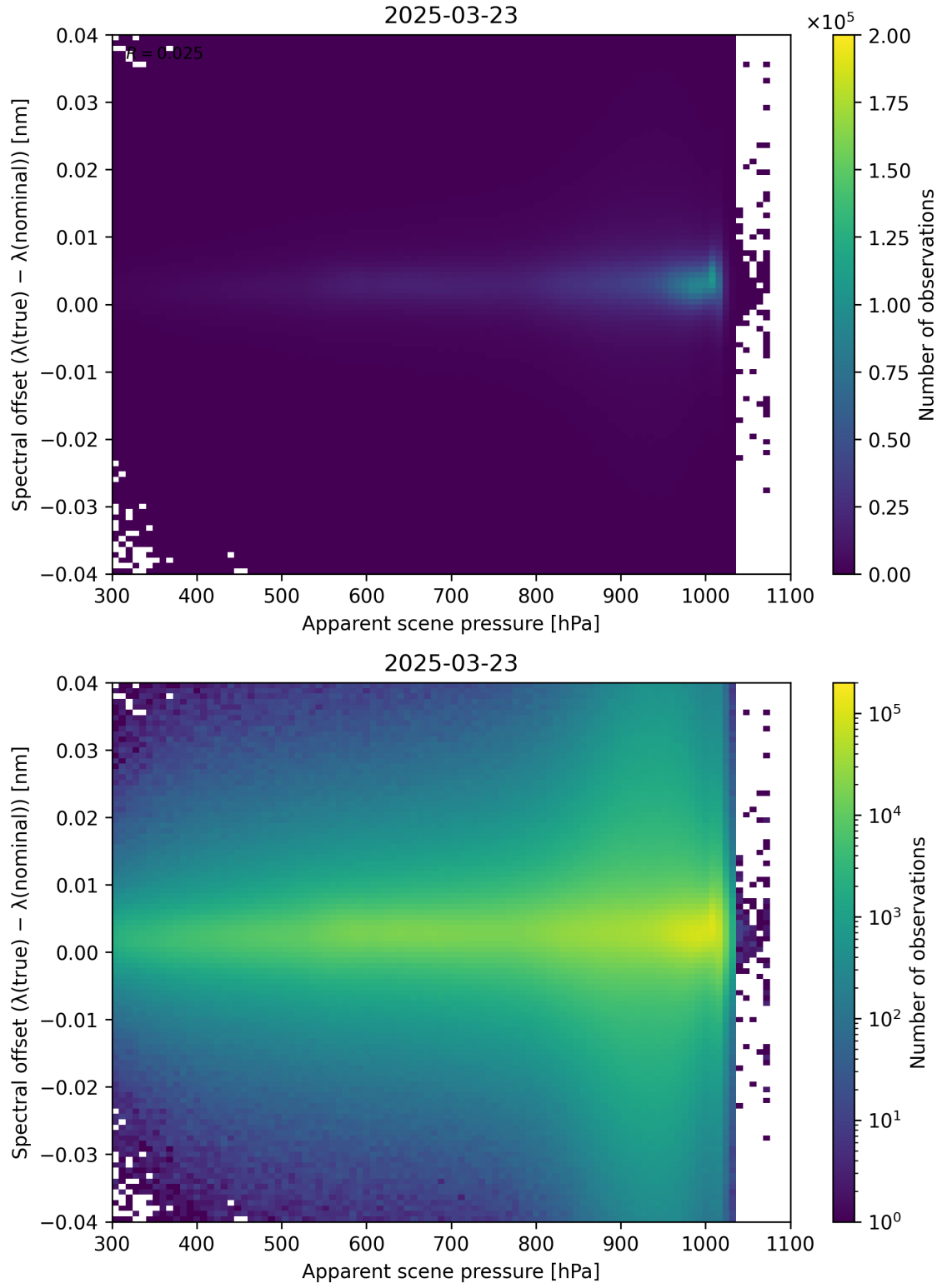
Figure 67: Scatter density plot of “Apparent scene pressure” against “Spectral offset ( \lambda_{\text{true}} - \lambda_{\text{nominal}} )” for 2025-03-23 to 2025-03-24.
