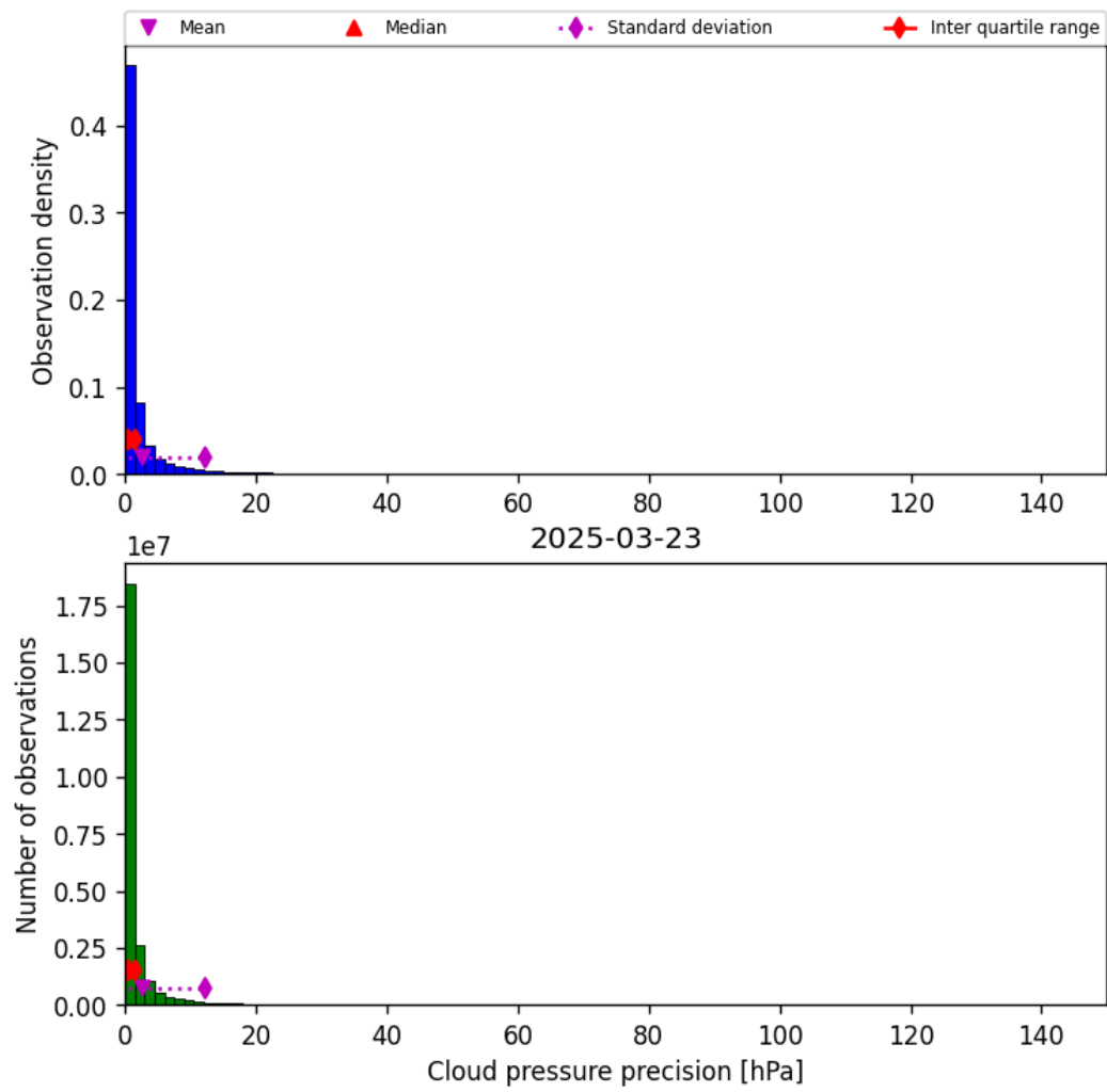
Figure 31: Histogram of “Cloud pressure precision” for 2025-03-23 to 2025-03-24
