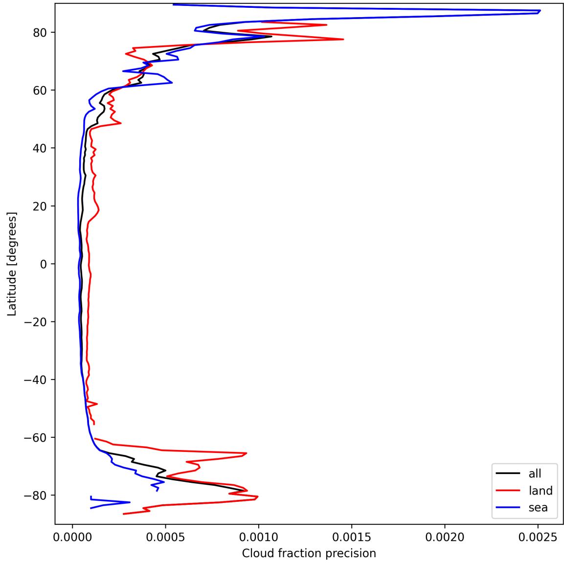
Figure 16: Zonal average of “Cloud fraction precision” for 2025-03-23 to 2025-03-24.
