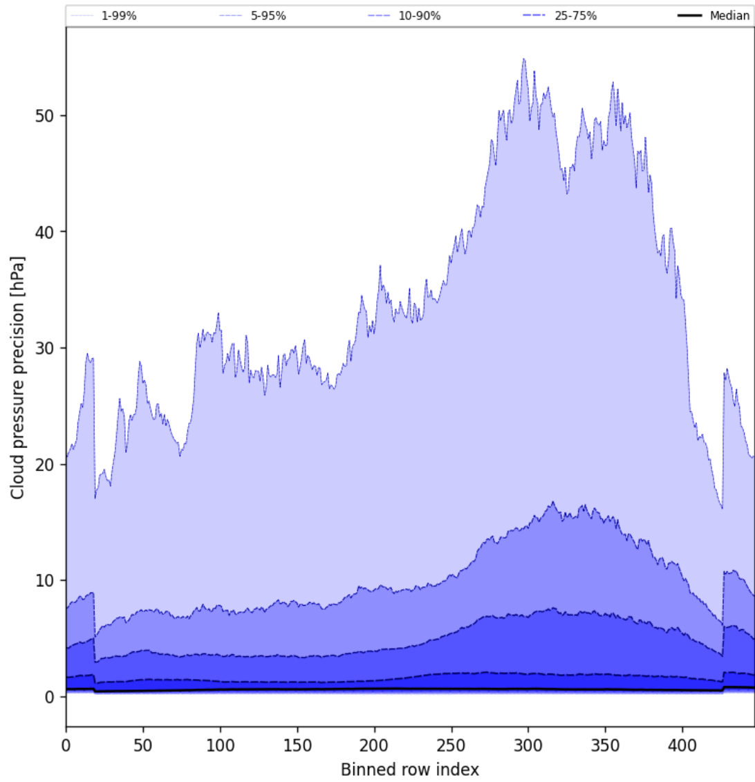
Figure 48: Along track statistics of “Cloud pressure precision” for 2025-03-23 to 2025-03-24
