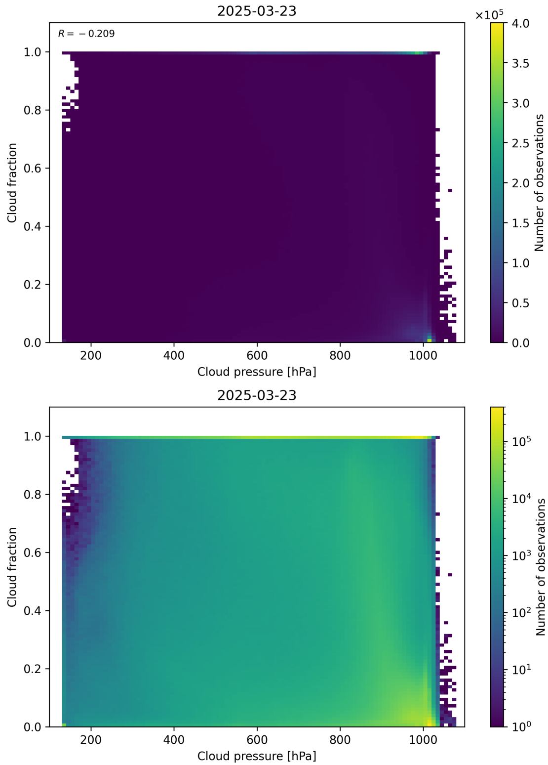
Figure 79: Scatter density plot of “Cloud pressure” against “Cloud fraction” for 2025-03-23 to 2025-03-24.
