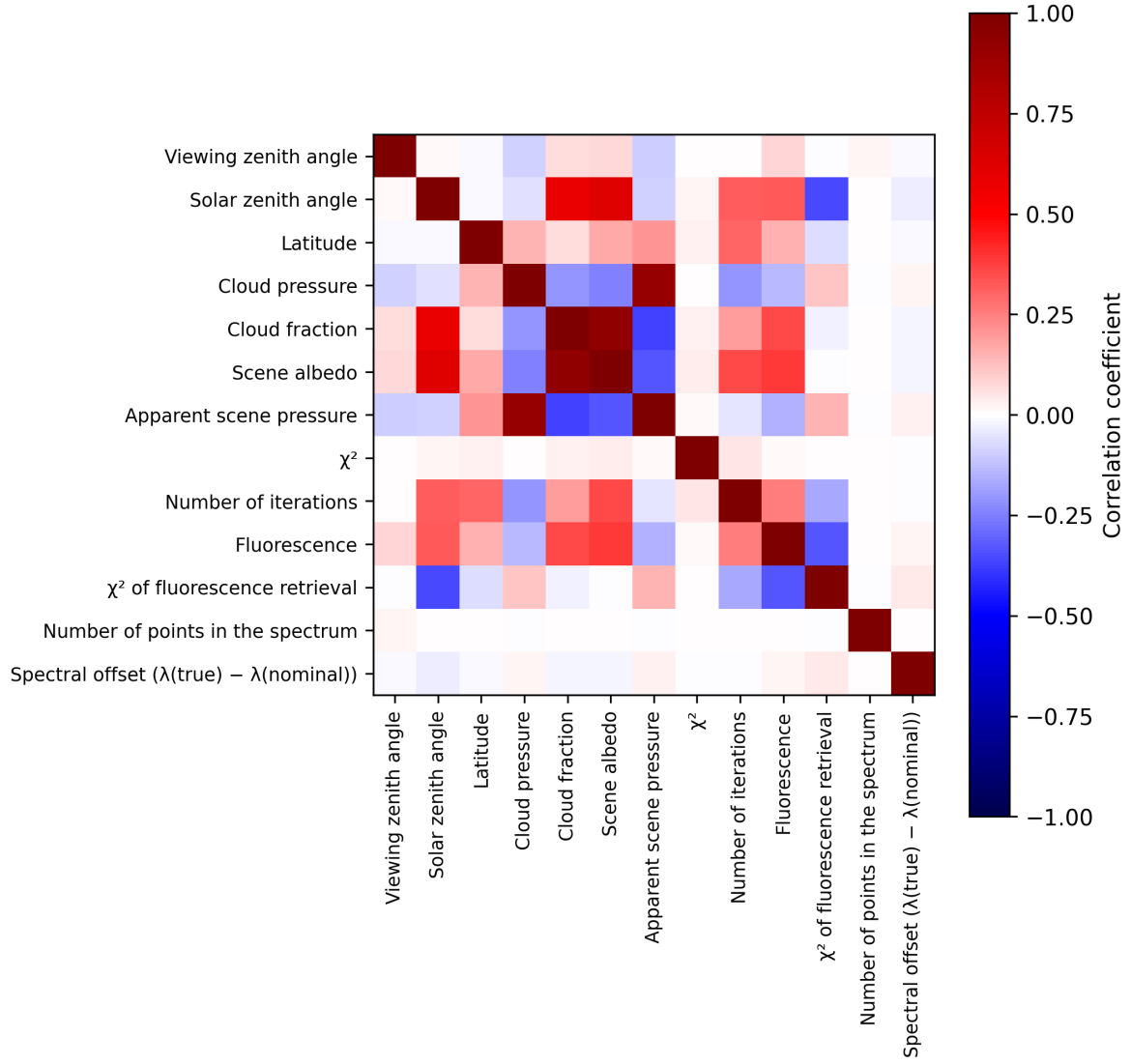
Figure 2: Map of correlation matrix for 2025-03-23 to 2025-03-24.
