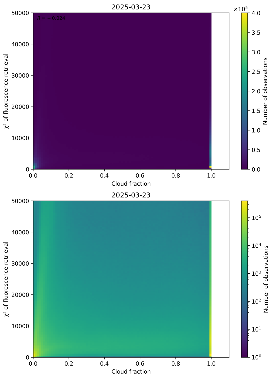
Figure 71: Scatter density plot of “Cloud fraction” against “ \chi^2 of fluorescence retrieval” for 2025-03-23 to 2025-03-24.
