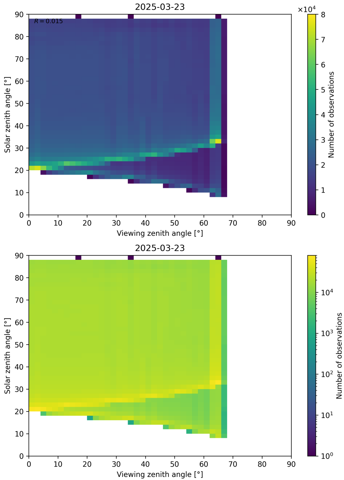
Figure 127: Scatter density plot of “Viewing zenith angle” against “Solar zenith angle” for 2025-03-23 to 2025-03-24.
