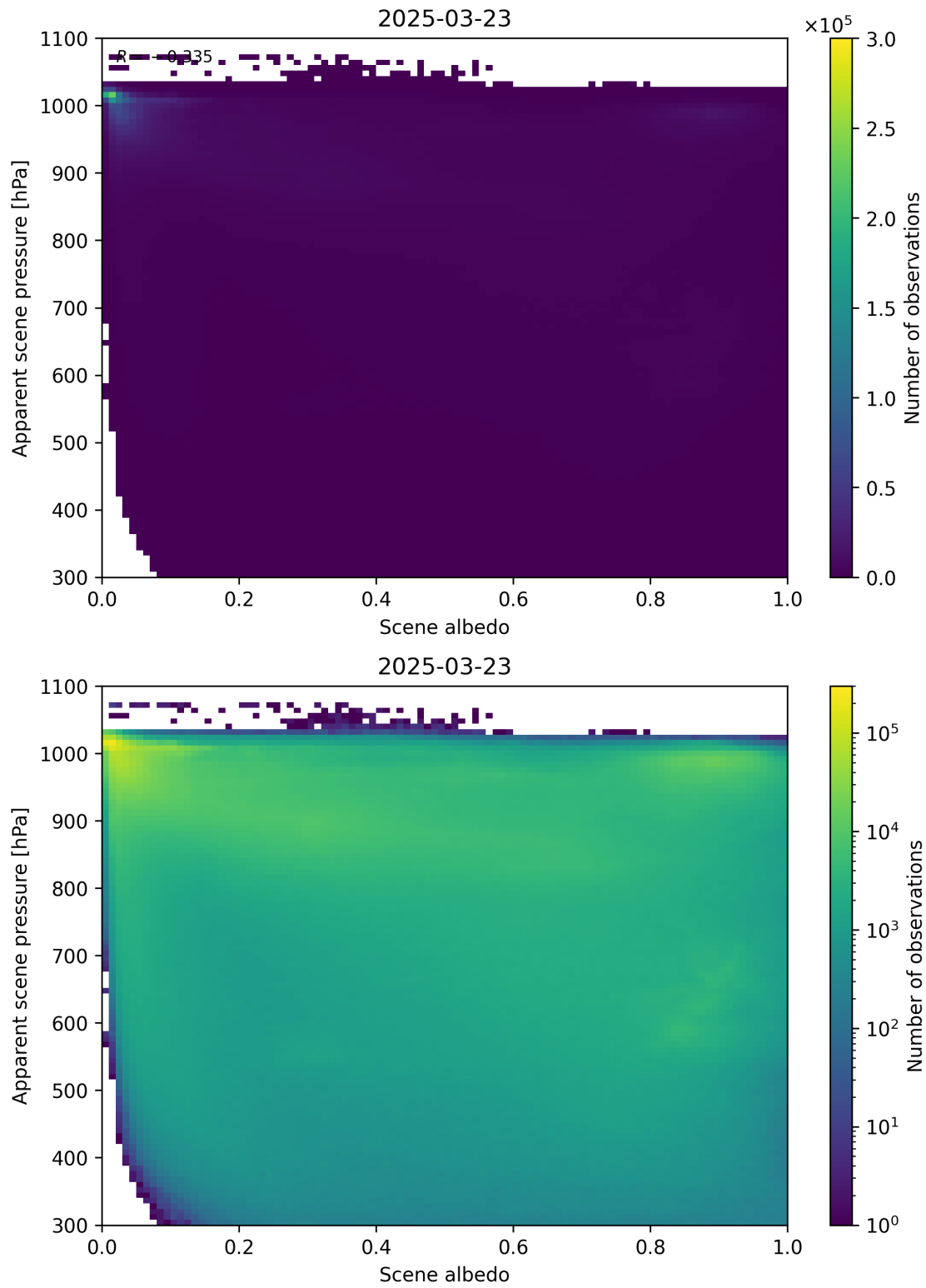
Figure 102: Scatter density plot of “Scene albedo” against “Apparent scene pressure” for 2025-03-23 to 2025-03-24.
