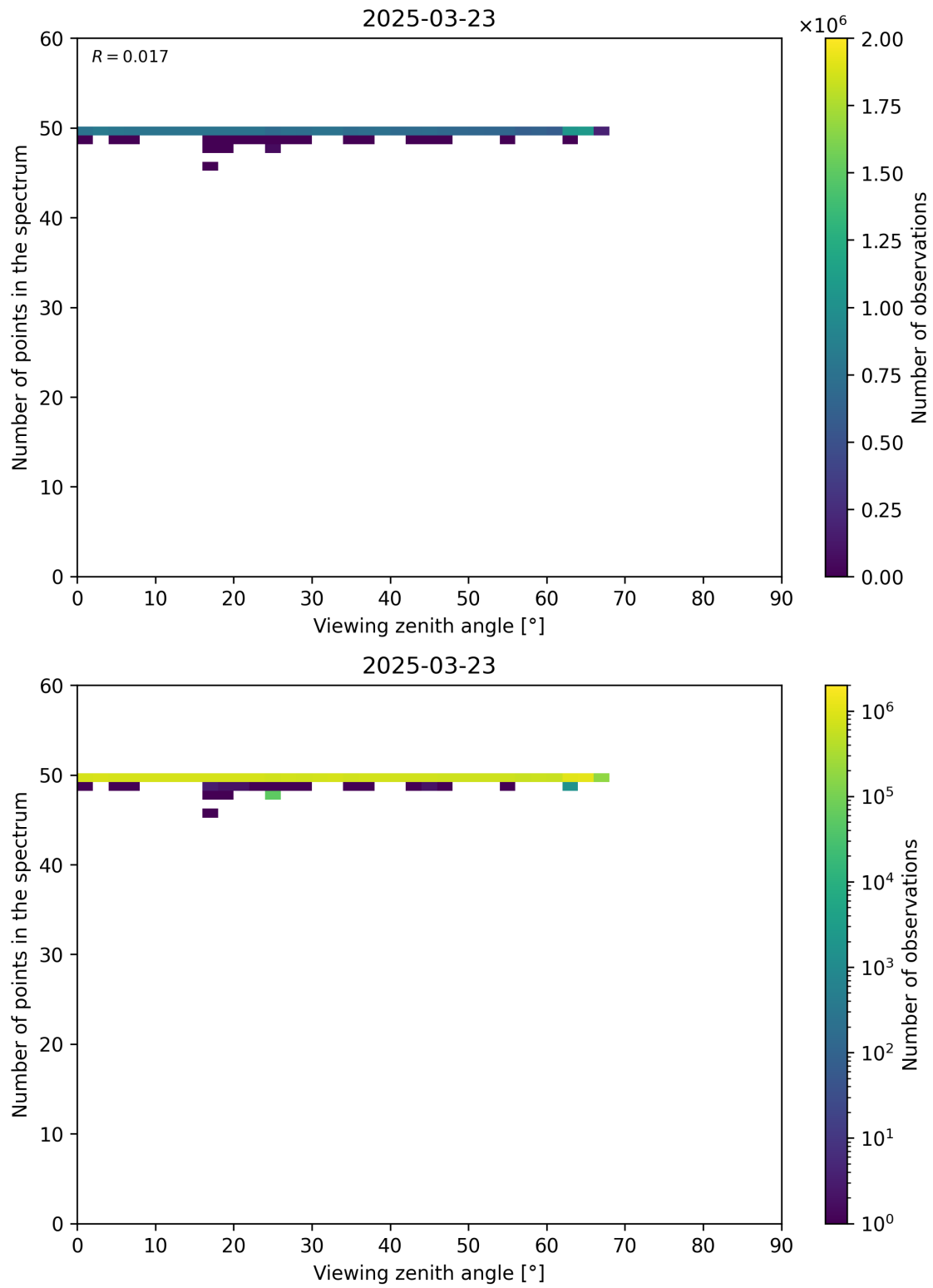
Figure 125: Scatter density plot of “Viewing zenith angle” against “Number of points in the spectrum” for 2025-03-23 to 2025-03-24.
