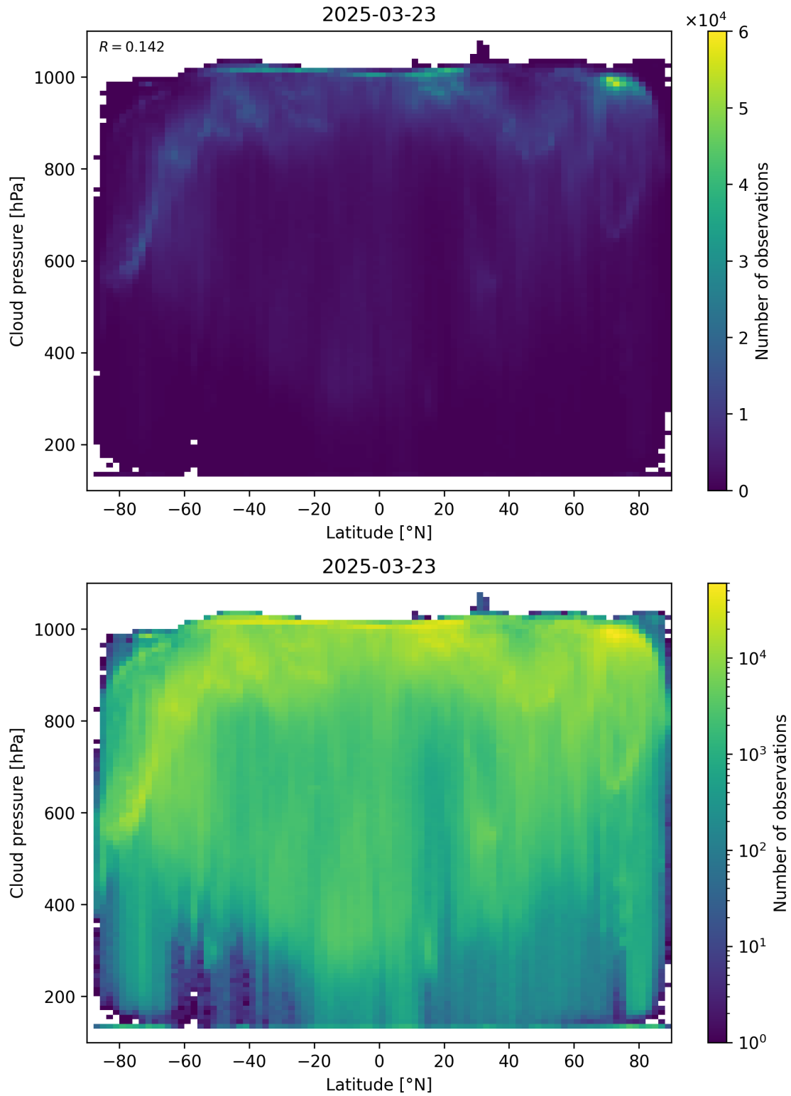
Figure 91: Scatter density plot of “Latitude” against “Cloud pressure” for 2025-03-23 to 2025-03-24.
