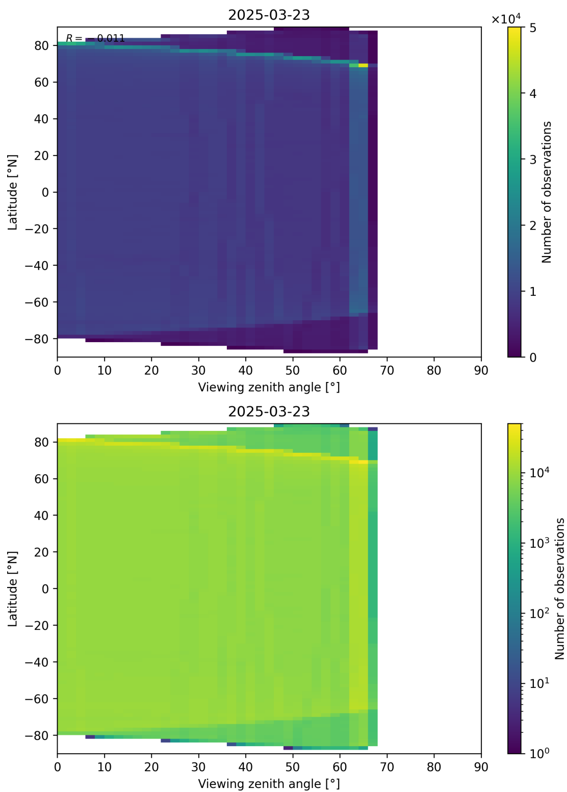
Figure 123: Scatter density plot of “Viewing zenith angle” against “Latitude” for 2025-03-23 to 2025-03-24.
