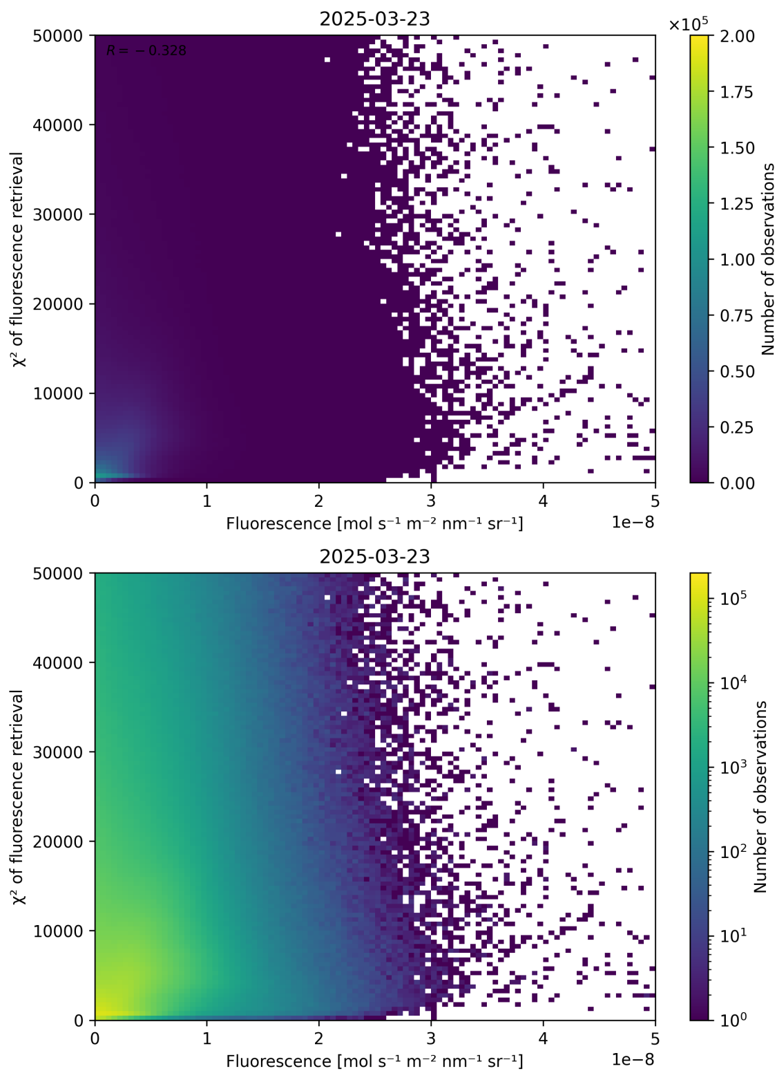
Figure 85: Scatter density plot of “Fluorescence” against “ \chi^2 of fluorescence retrieval” for 2025-03-23 to 2025-03-24.
