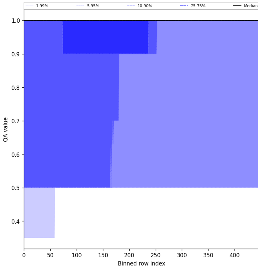
Figure 46: Along track statistics of “QA value” for 2025-03-23 to 2025-03-24
