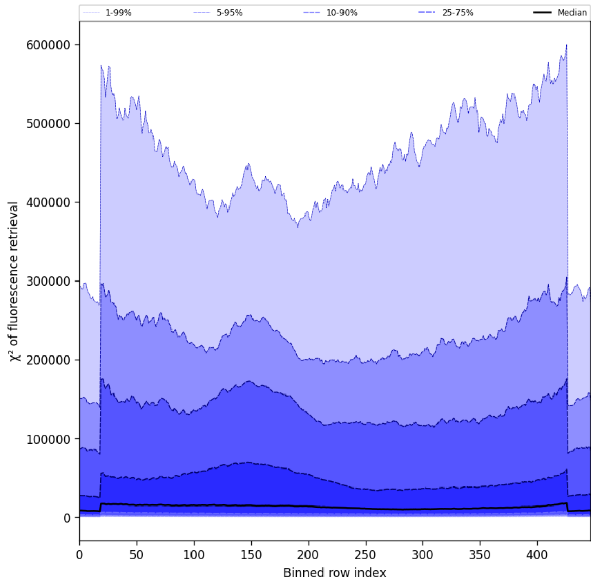
Figure 59: Along track statistics of “ \chi^2 of fluorescence retrieval” for 2025-03-23 to 2025-03-24
