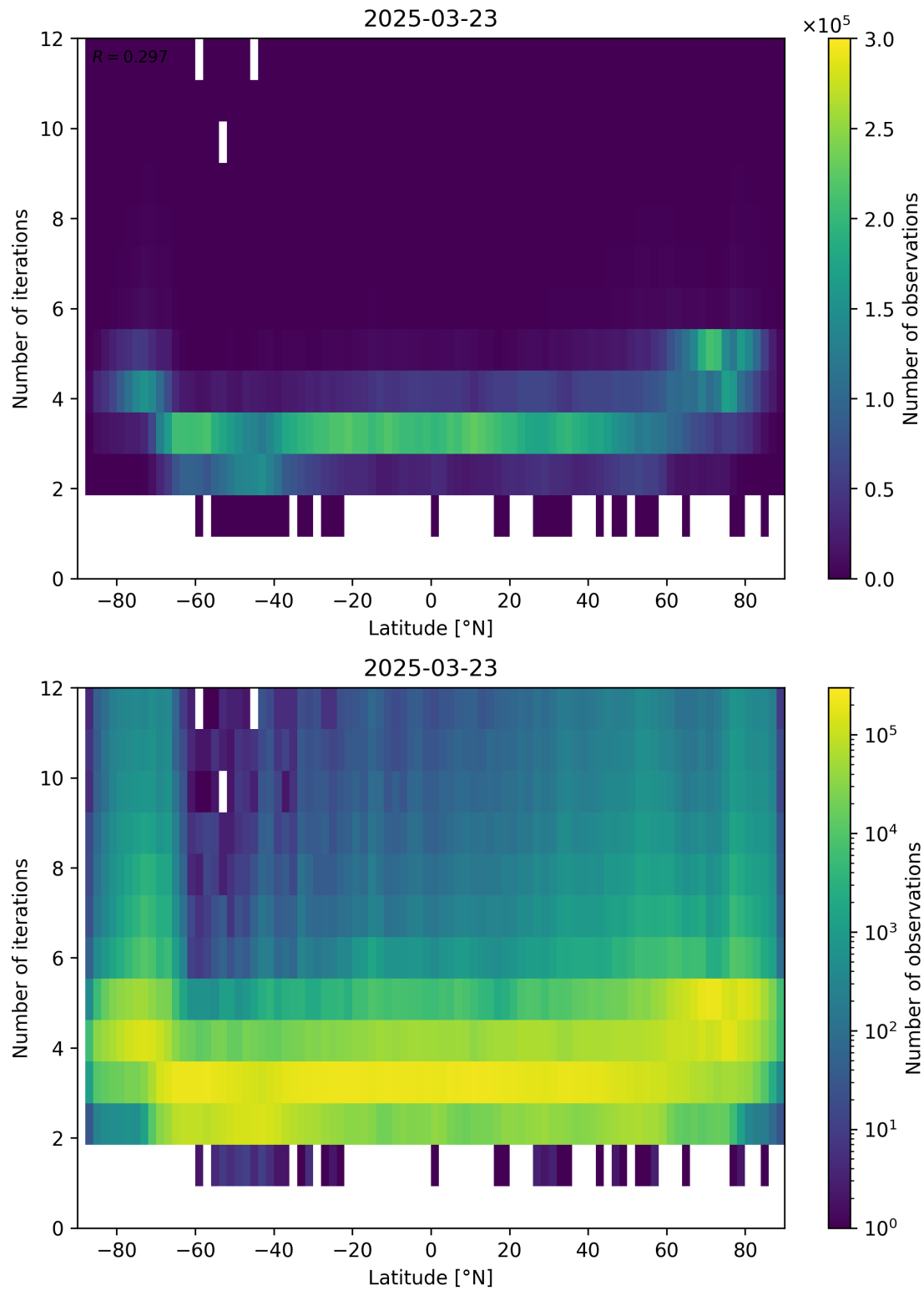
Figure 93: Scatter density plot of “Latitude” against “Number of iterations” for 2025-03-23 to 2025-03-24.
