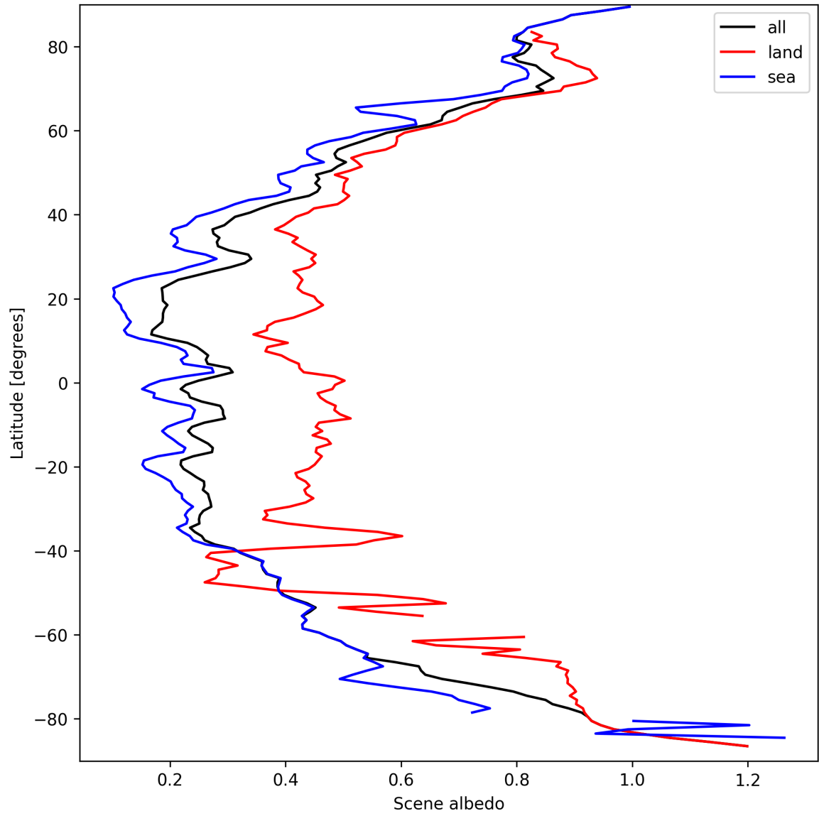
Figure 17: Zonal average of “Scene albedo” for 2025-03-23 to 2025-03-24.
