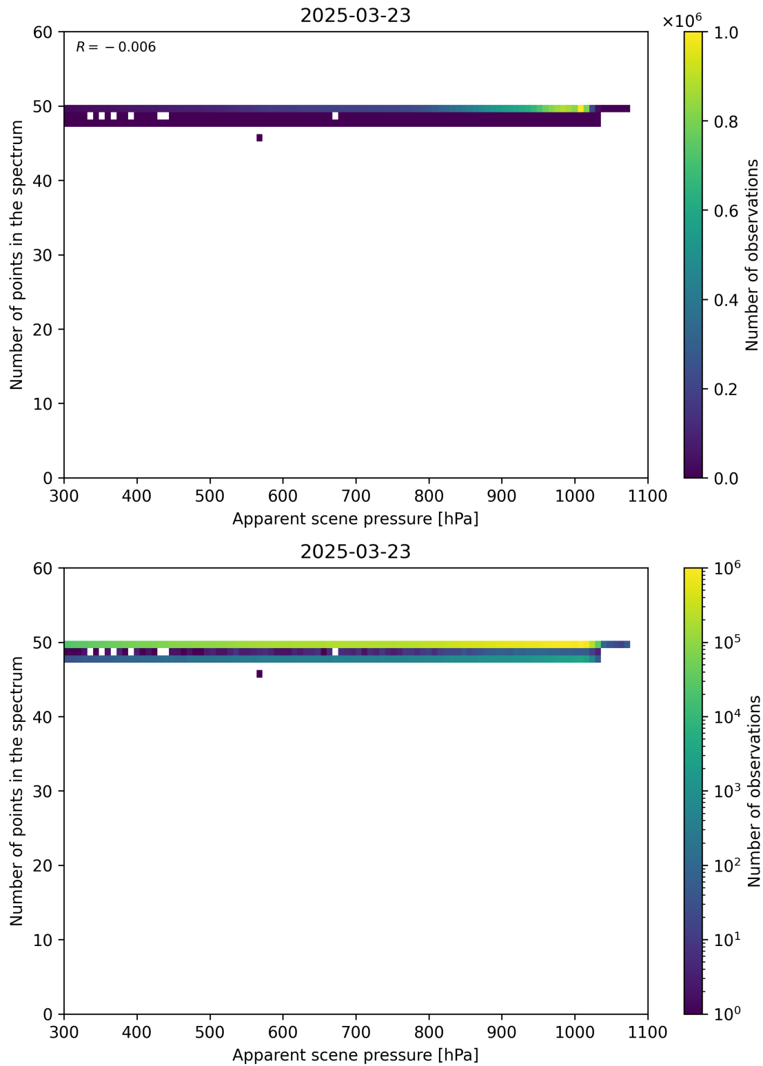
Figure 66: Scatter density plot of “Apparent scene pressure” against “Number of points in the spectrum” for 2025-03-23 to 2025-03-24.
