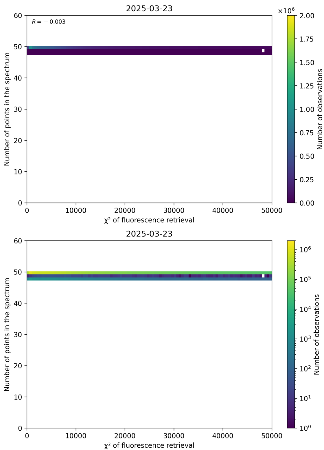
Figure 68: Scatter density plot of “ \chi^2 of fluorescence retrieval” against “Number of points in the spectrum” for 2025-03-23 to 2025-03-24.
