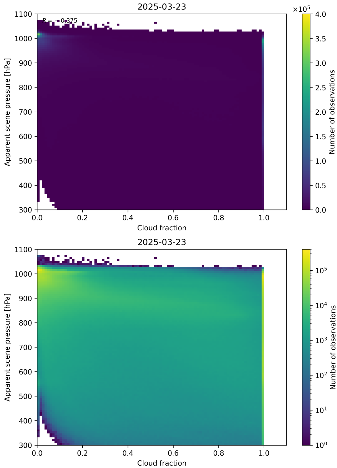
Figure 70: Scatter density plot of “Cloud fraction” against “Apparent scene pressure” for 2025-03-23 to 2025-03-24.
