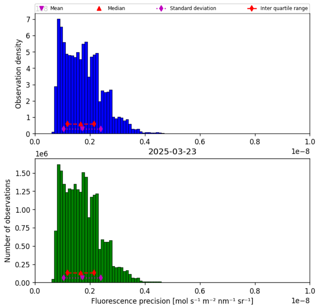
Figure 41: Histogram of “Fluorescence precision” for 2025-03-23 to 2025-03-24
