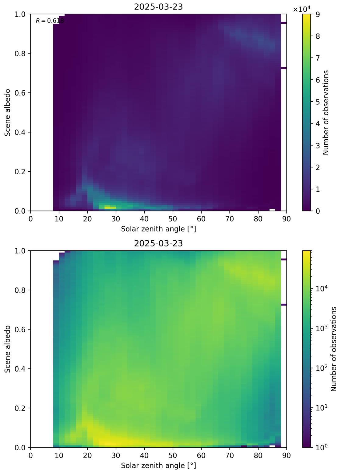
Figure 116: Scatter density plot of “Solar zenith angle” against “Scene albedo” for 2025-03-23 to 2025-03-24.
