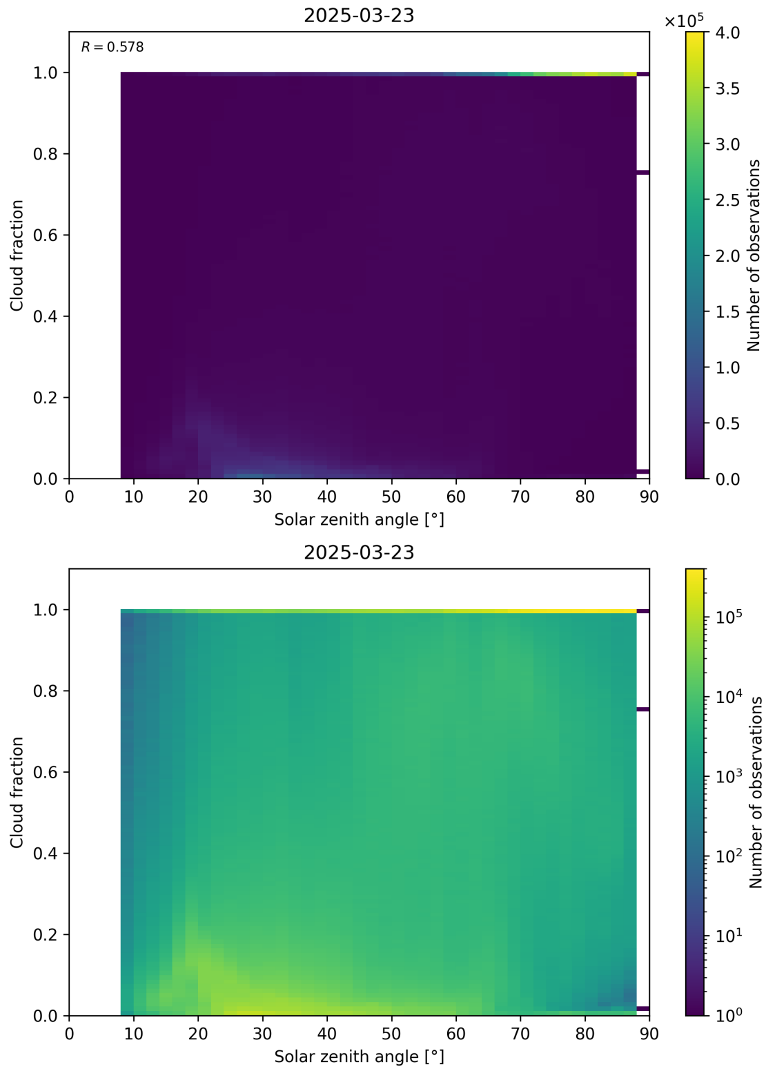
Figure 110: Scatter density plot of “Solar zenith angle” against “Cloud fraction” for 2025-03-23 to 2025-03-24.
