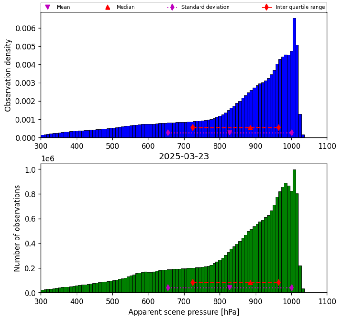
Figure 36: Histogram of “Apparent scene pressure” for 2025-03-23 to 2025-03-24
