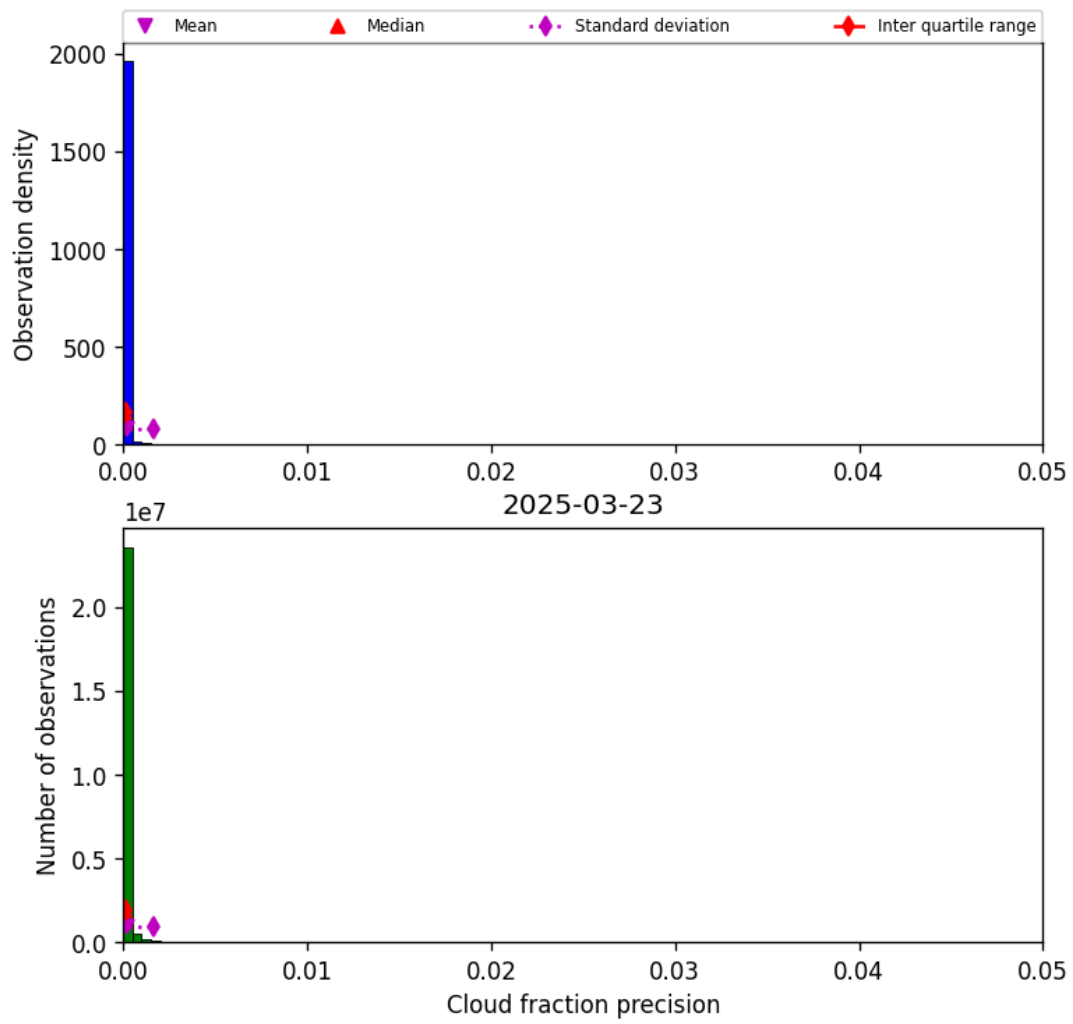
Figure 33: Histogram of “Cloud fraction precision” for 2025-03-23 to 2025-03-24
