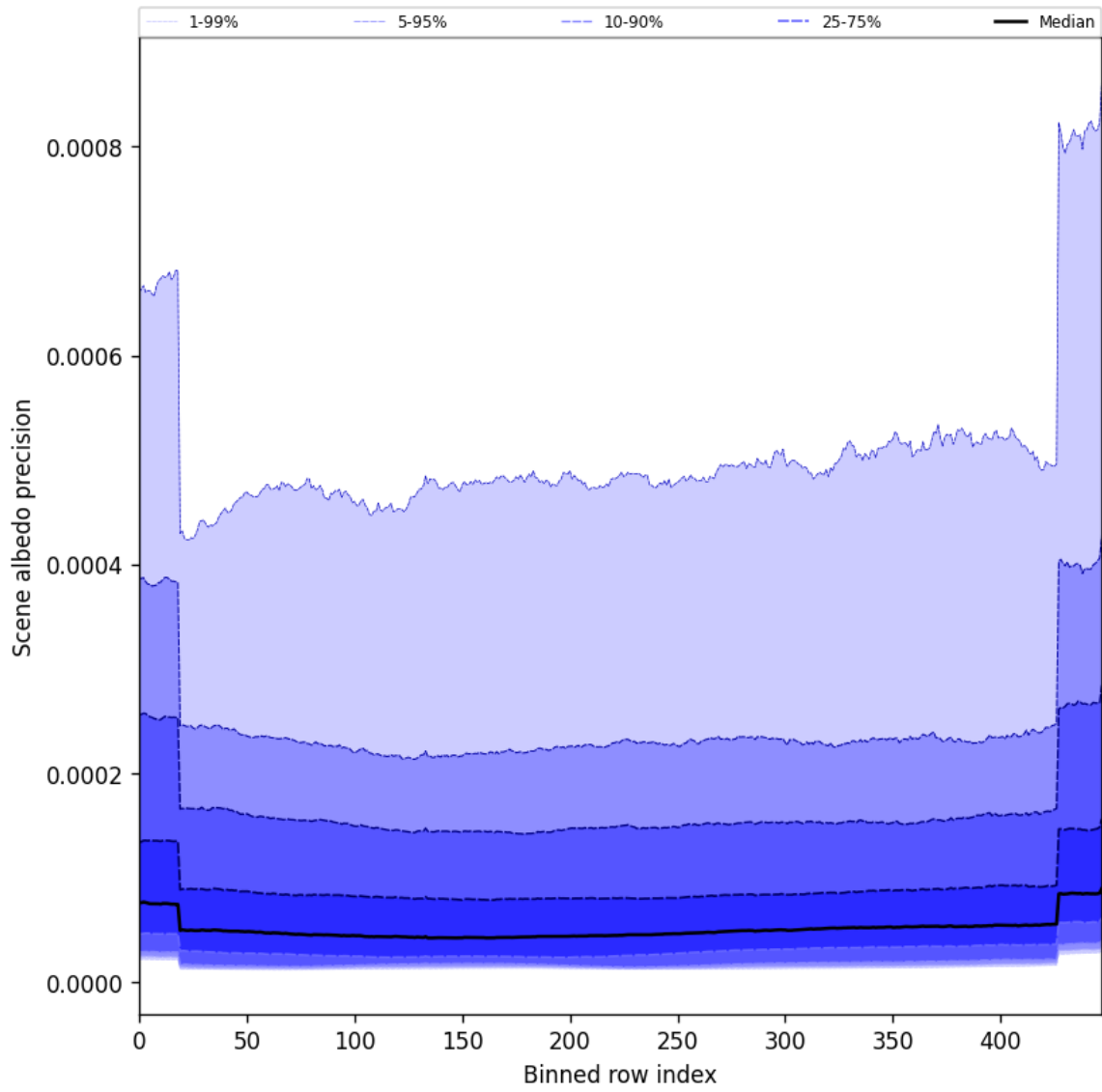
Figure 52: Along track statistics of “Scene albedo precision” for 2025-03-23 to 2025-03-24
