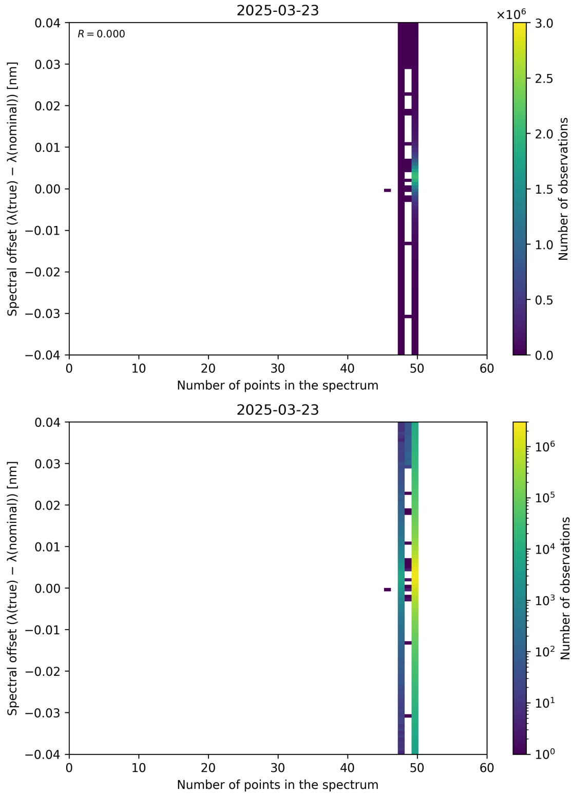
Figure 101: Scatter density plot of “Number of points in the spectrum” against “Spectral offset ( \lambda_{\text{true}} - \lambda_{\text{nominal}} )” for 2025-03-23 to 2025-03-24.
