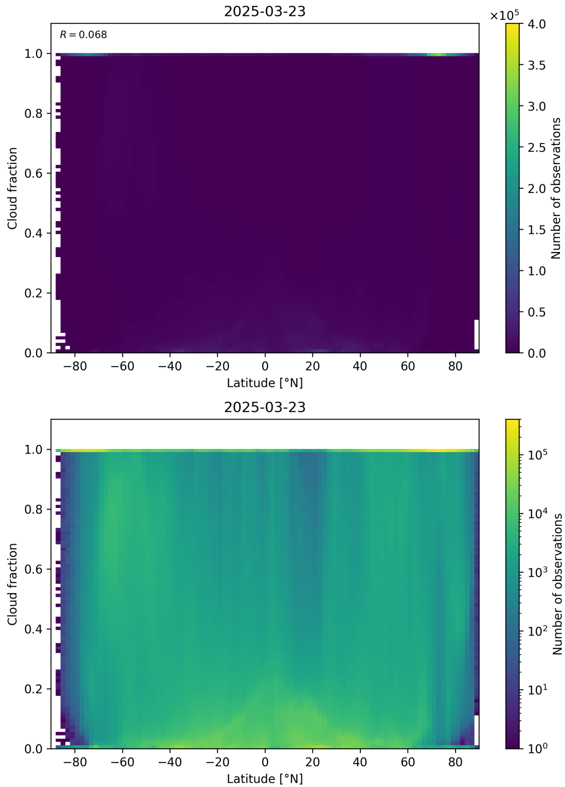
Figure 90: Scatter density plot of “Latitude” against “Cloud fraction” for 2025-03-23 to 2025-03-24.
