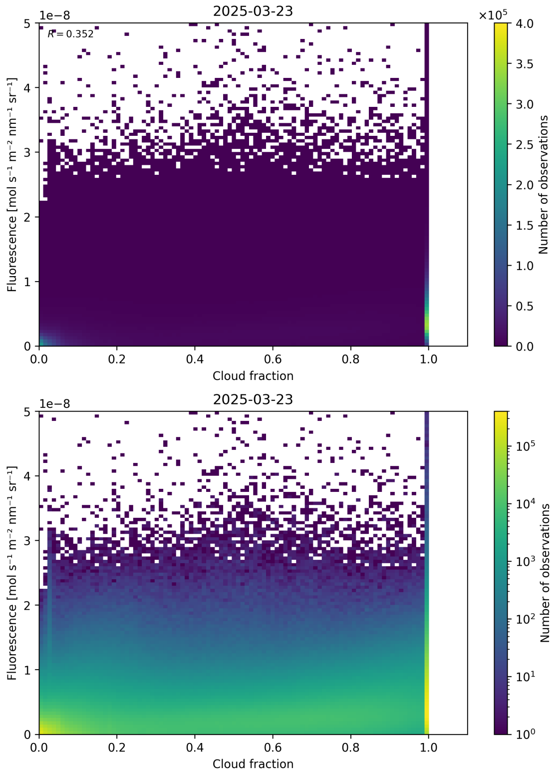
Figure 72: Scatter density plot of “Cloud fraction” against “Fluorescence” for 2025-03-23 to 2025-03-24.
