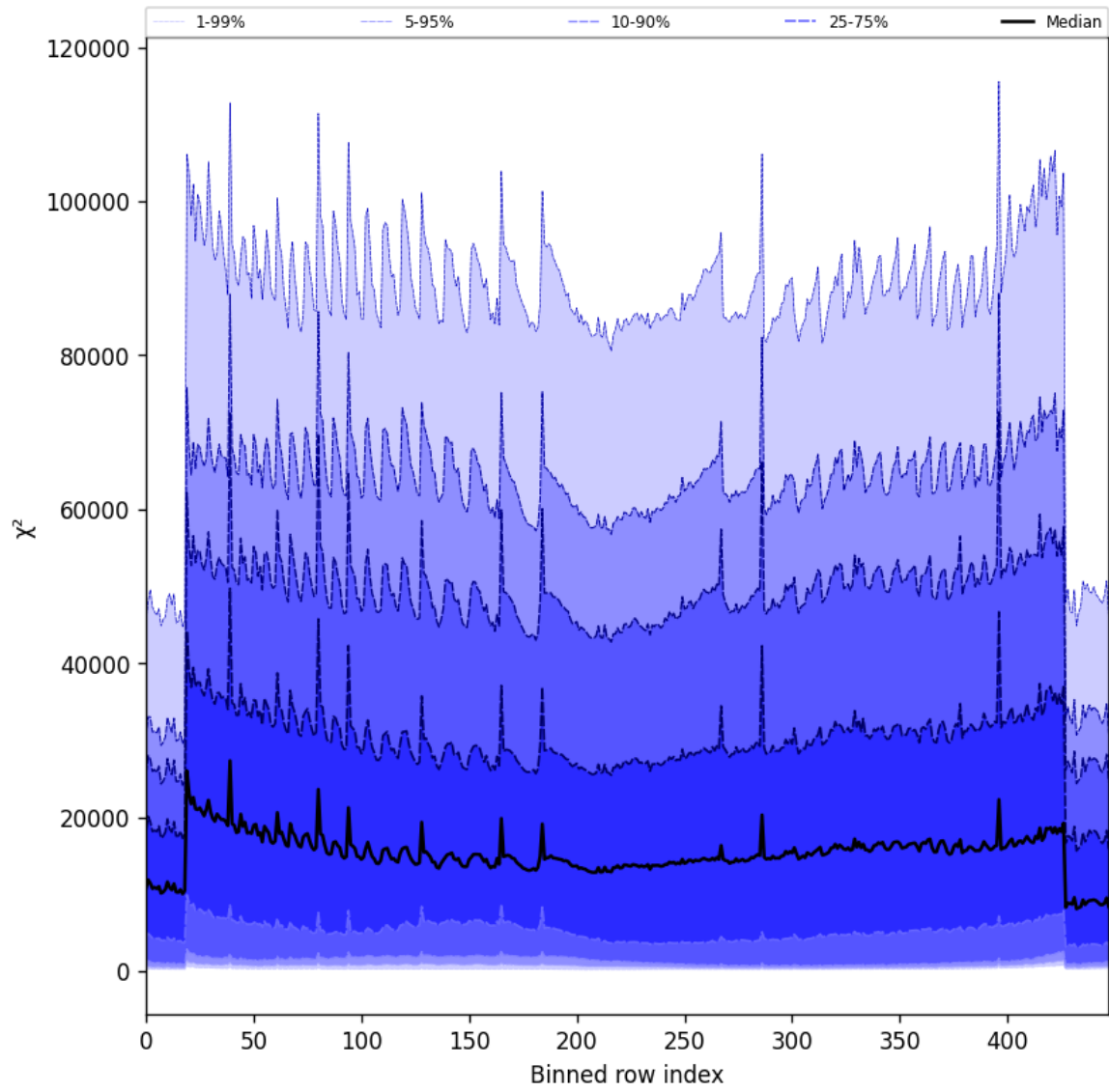
Figure 55: Along track statistics of “ \chi^2 ” for 2025-03-23 to 2025-03-24
