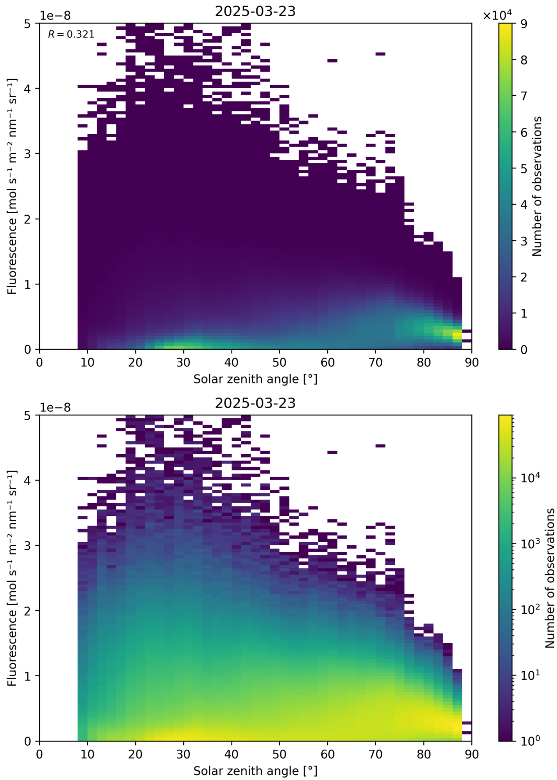
Figure 112: Scatter density plot of “Solar zenith angle” against “Fluorescence” for 2025-03-23 to 2025-03-24.
