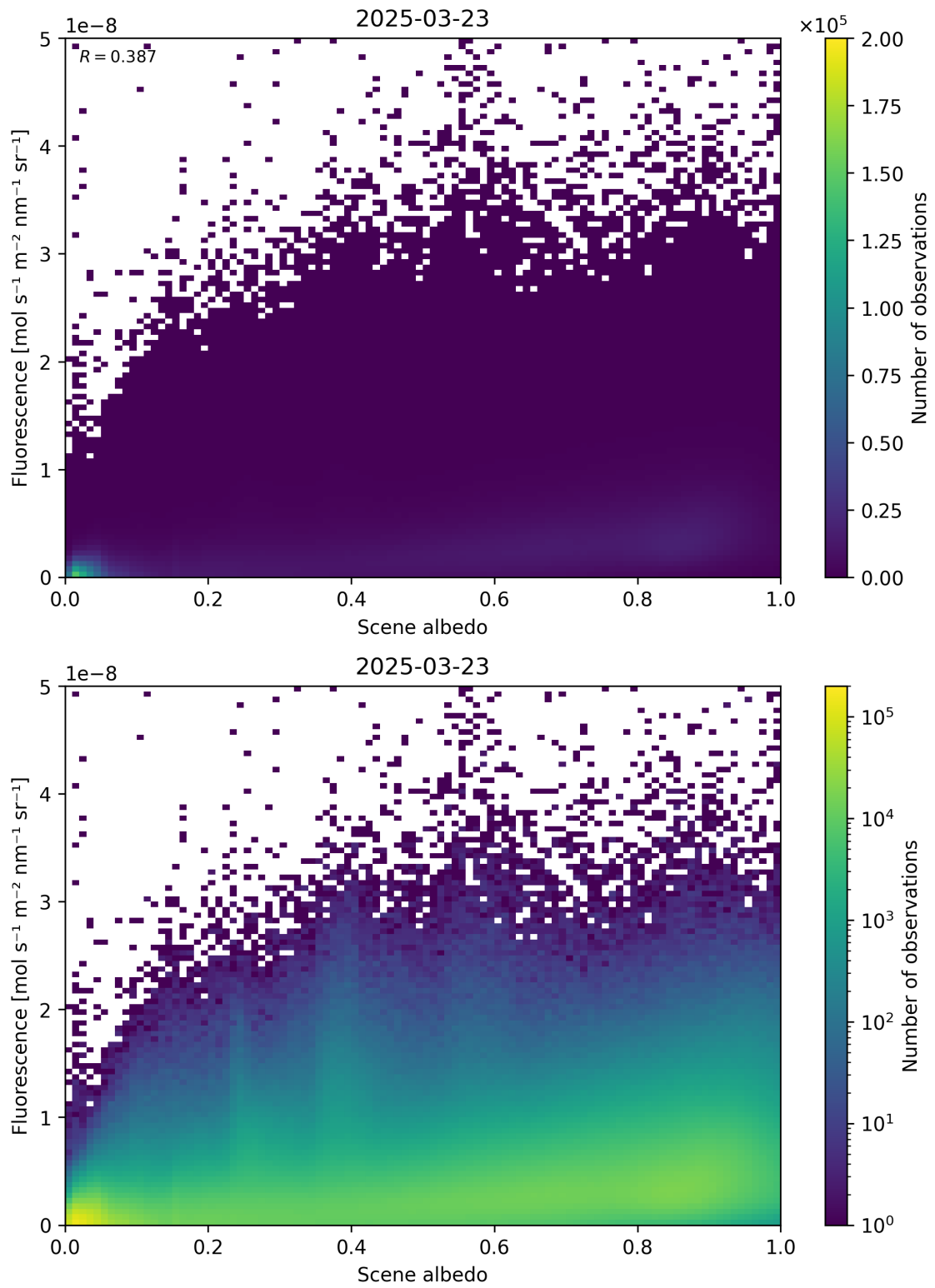
Figure 104: Scatter density plot of “Scene albedo” against “Fluorescence” for 2025-03-23 to 2025-03-24.
