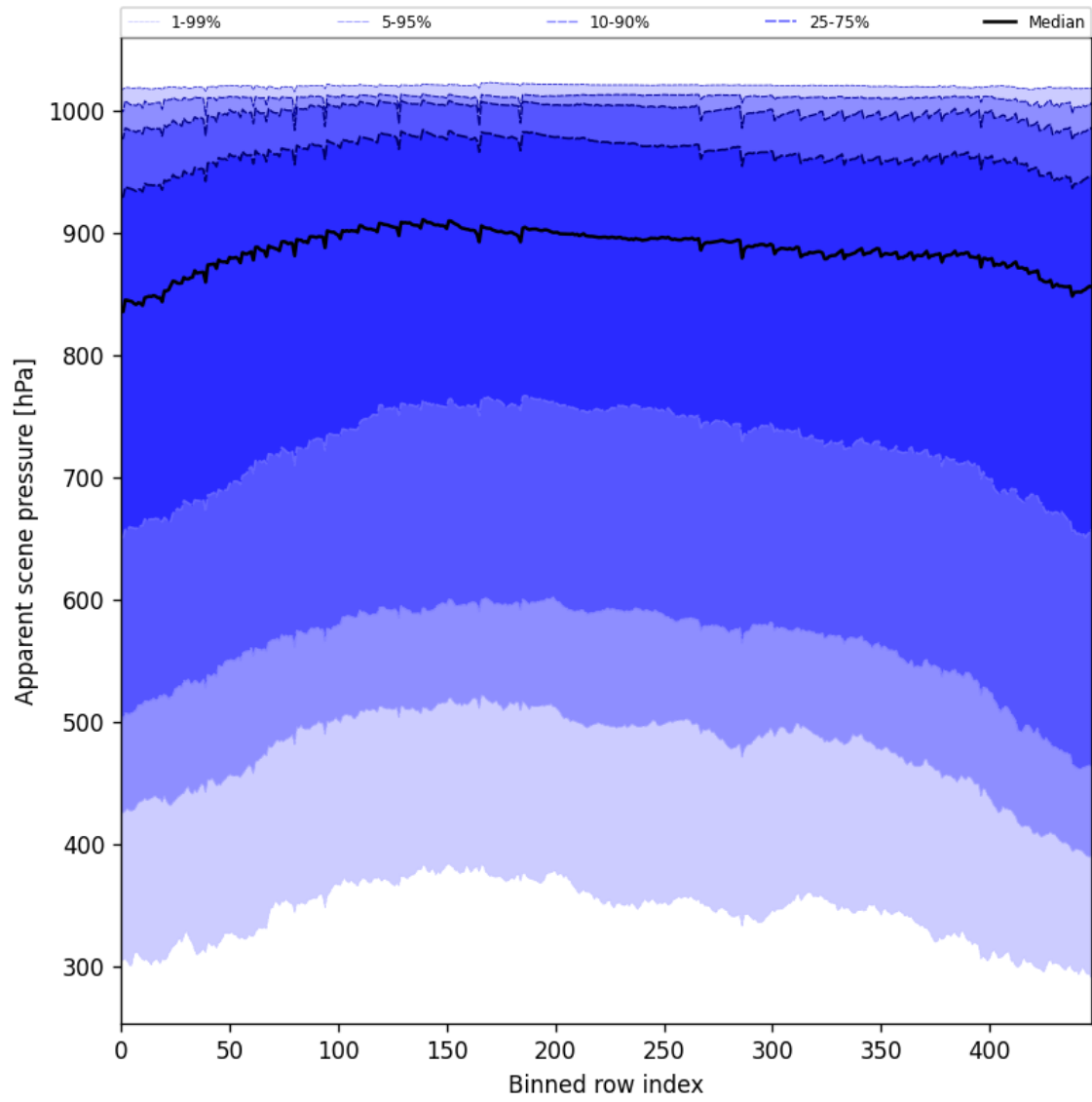
Figure 53: Along track statistics of “Apparent scene pressure” for 2025-03-23 to 2025-03-24
