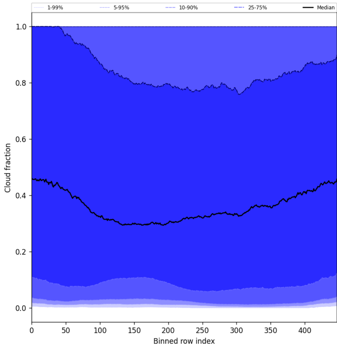
Figure 49: Along track statistics of “Cloud fraction” for 2025-03-23 to 2025-03-24
