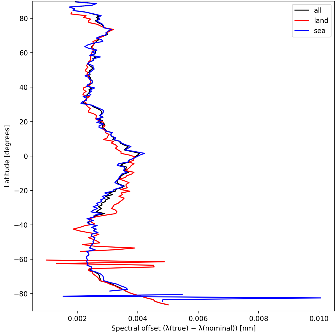
Figure 28: Zonal average of “Spectral offset ( \lambda_{\text{true}} - \lambda_{\text{nominal}} )” for 2025-03-23 to 2025-03-24.
