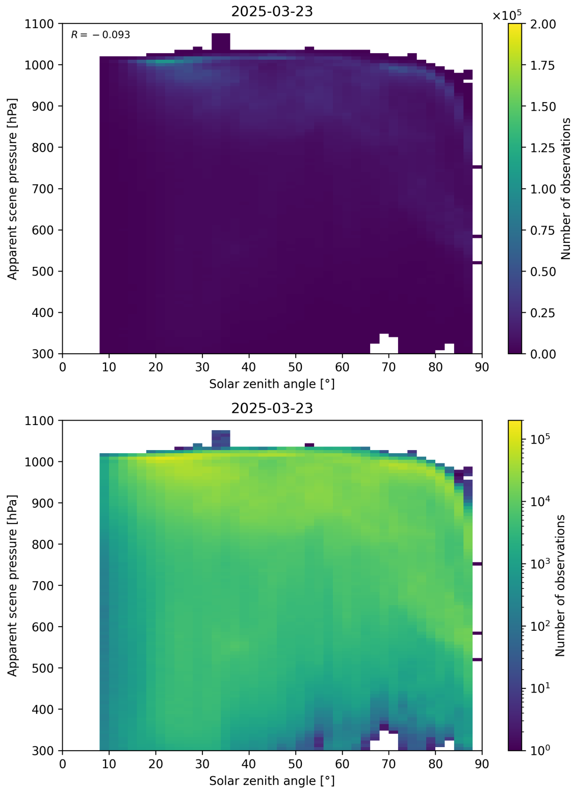
Figure 108: Scatter density plot of “Solar zenith angle” against “Apparent scene pressure” for 2025-03-23 to 2025-03-24.
