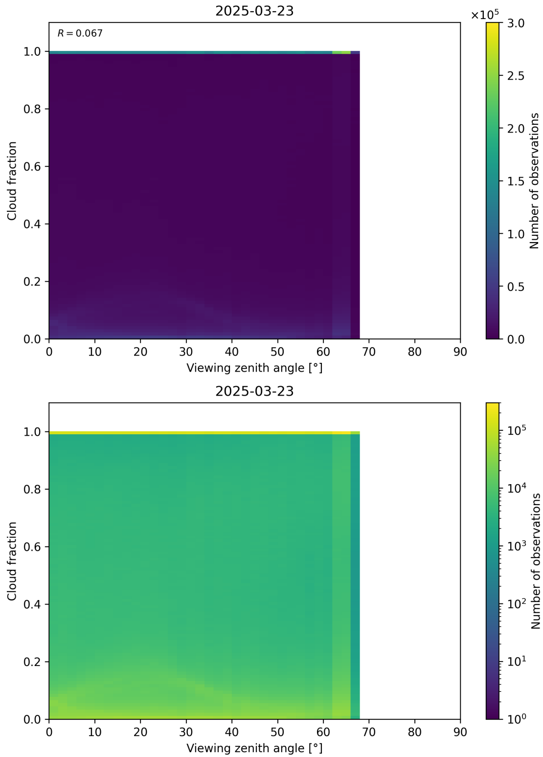
Figure 120: Scatter density plot of “Viewing zenith angle” against “Cloud fraction” for 2025-03-23 to 2025-03-24.
