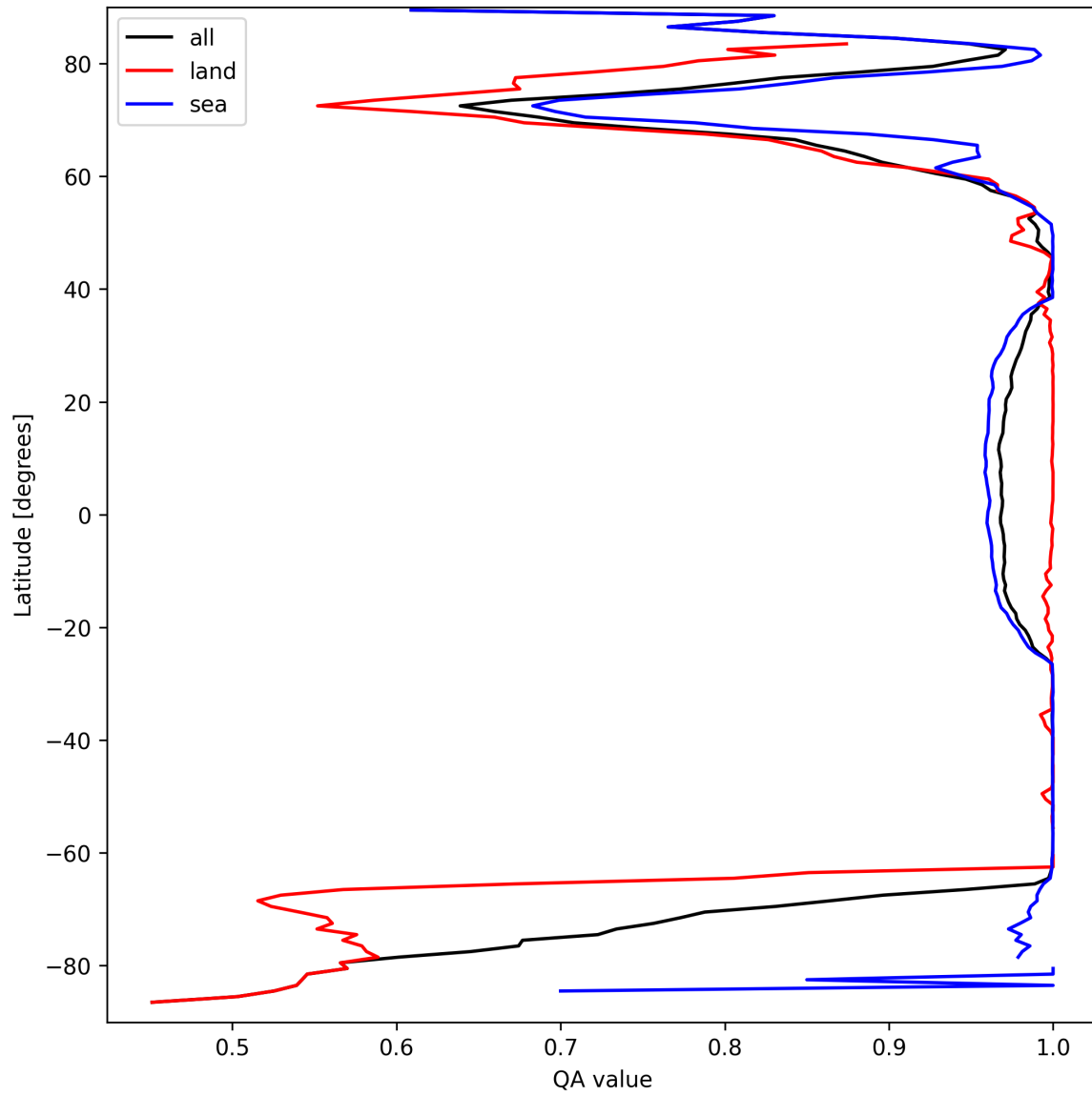
Figure 12: Zonal average of “QA value” for 2025-03-23 to 2025-03-24.
