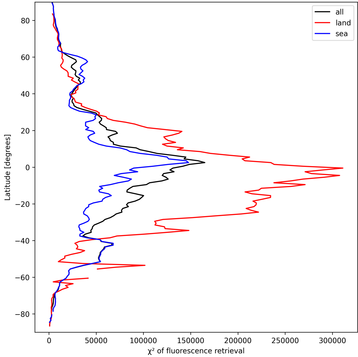
Figure 25: Zonal average of “ \chi^2 of fluorescence retrieval” for 2025-03-23 to 2025-03-24.
