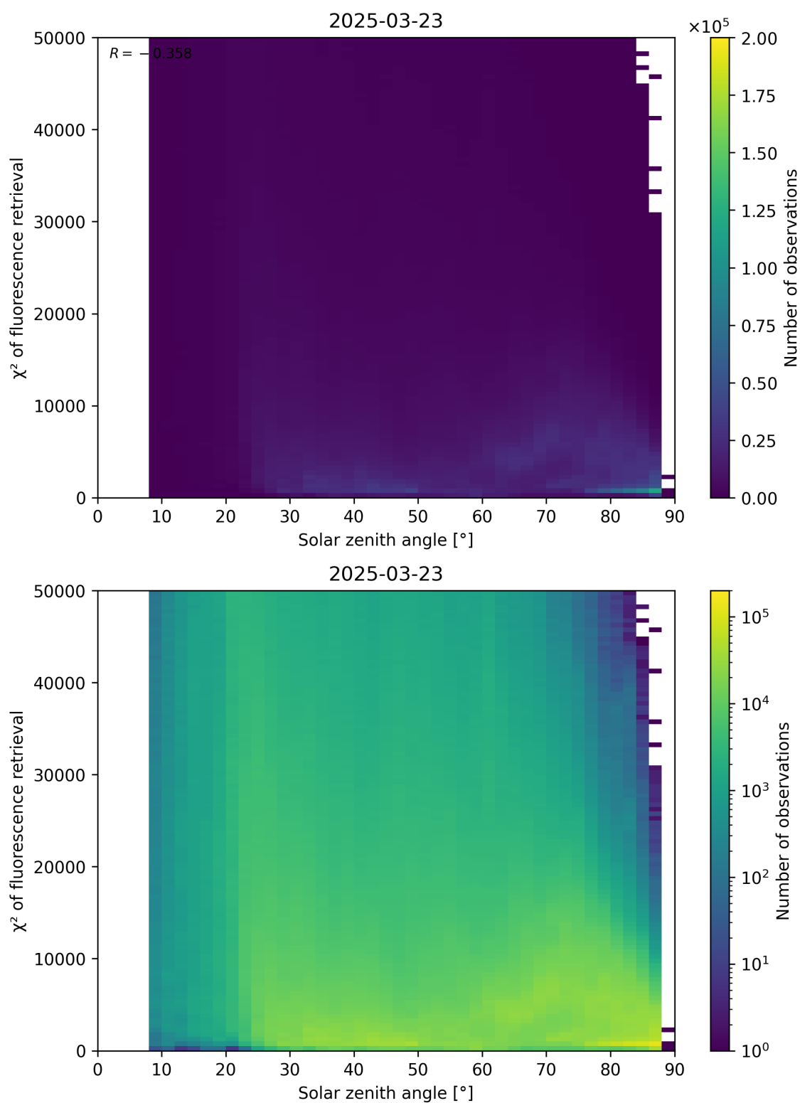
Figure 109: Scatter density plot of “Solar zenith angle” against “ \chi^2 of fluorescence retrieval” for 2025-03-23 to 2025-03-24.
