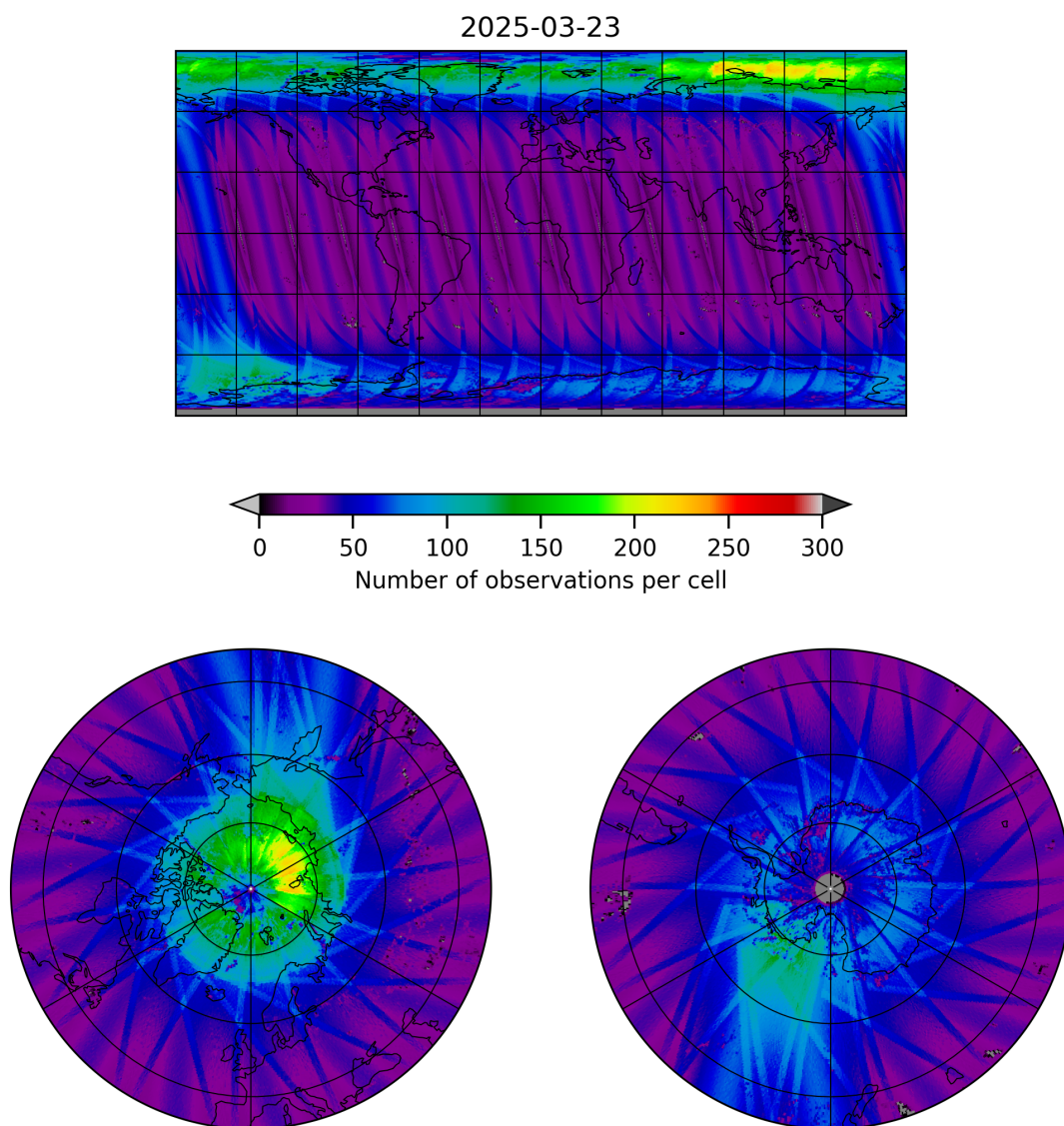
Figure 11: Map of the number of observations for 2025-03-23 to 2025-03-24
