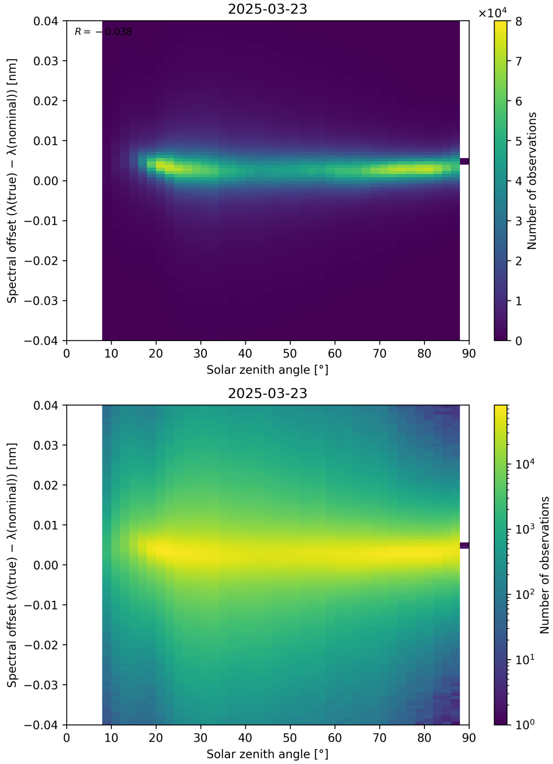
Figure 117: Scatter density plot of “Solar zenith angle” against “Spectral offset ( \lambda_{\text{true}} - \lambda_{\text{nominal}} )” for 2025-03-23 to 2025-03-24.
