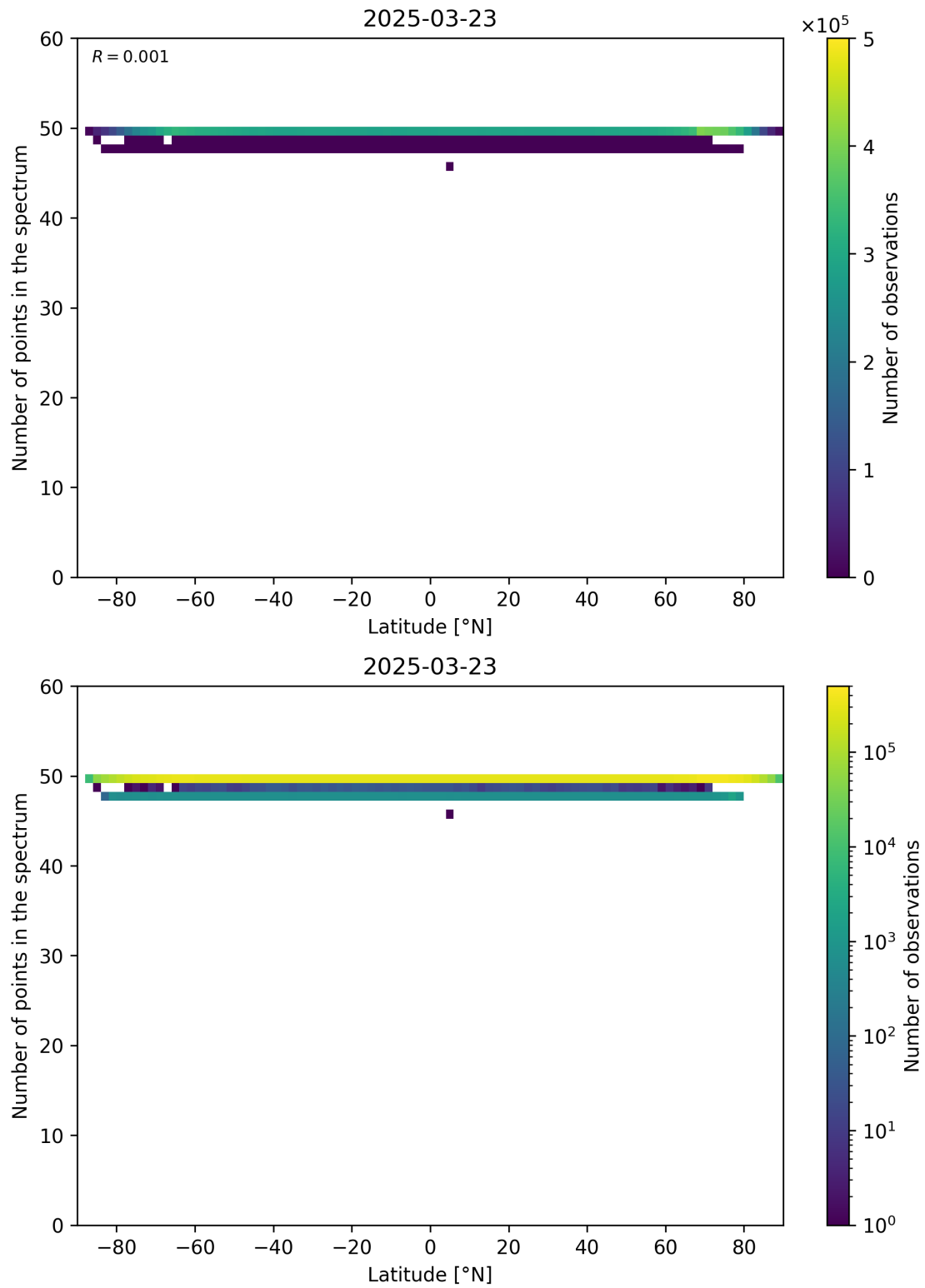
Figure 94: Scatter density plot of “Latitude” against “Number of points in the spectrum” for 2025-03-23 to 2025-03-24.
