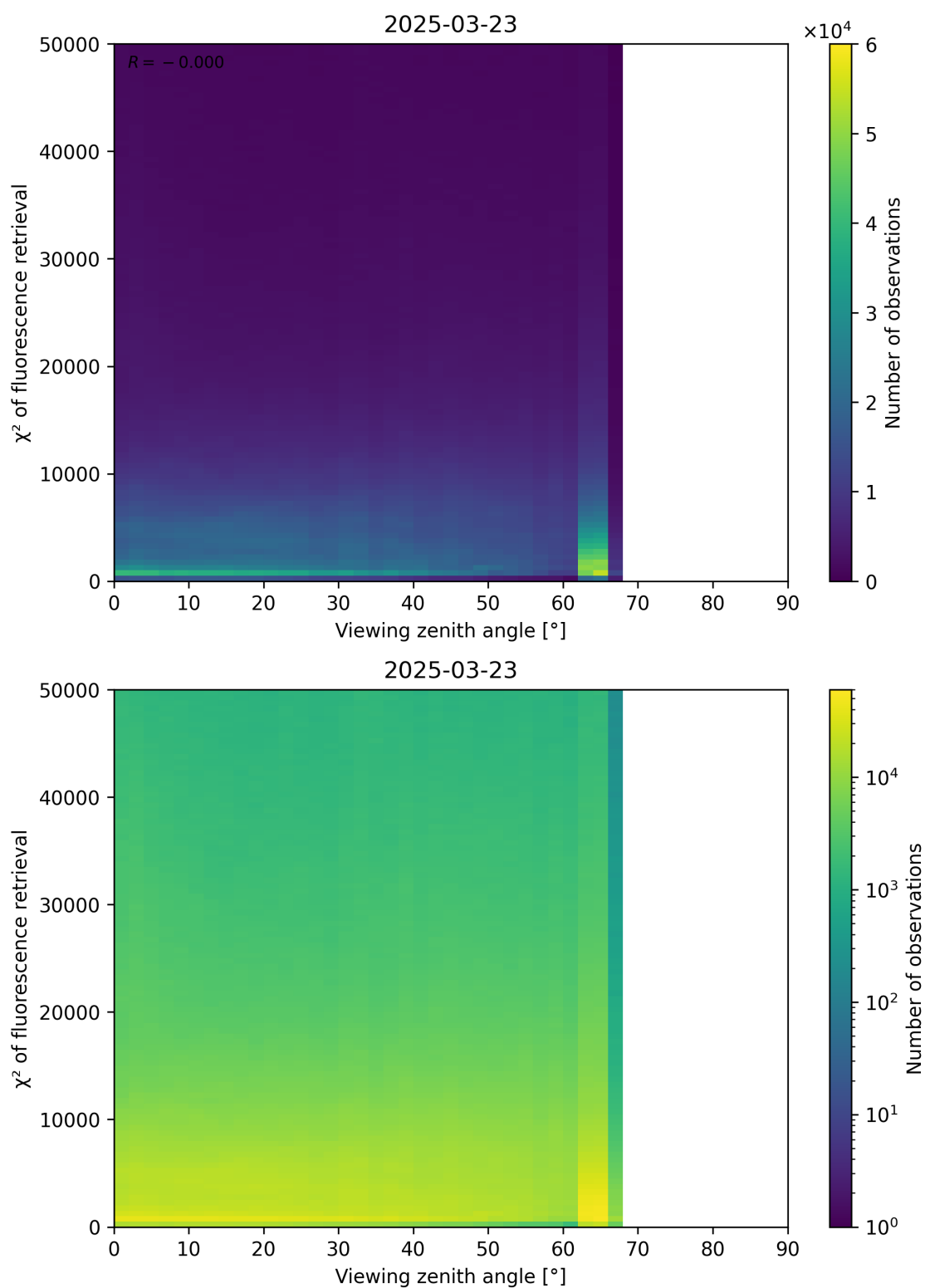
Figure 119: Scatter density plot of “Viewing zenith angle” against “ \chi^2 of fluorescence retrieval” for 2025-03-23 to 2025-03-24.
