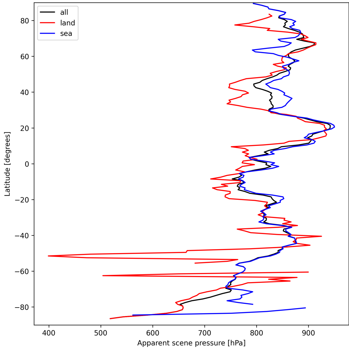
Figure 19: Zonal average of “Apparent scene pressure” for 2025-03-23 to 2025-03-24.
