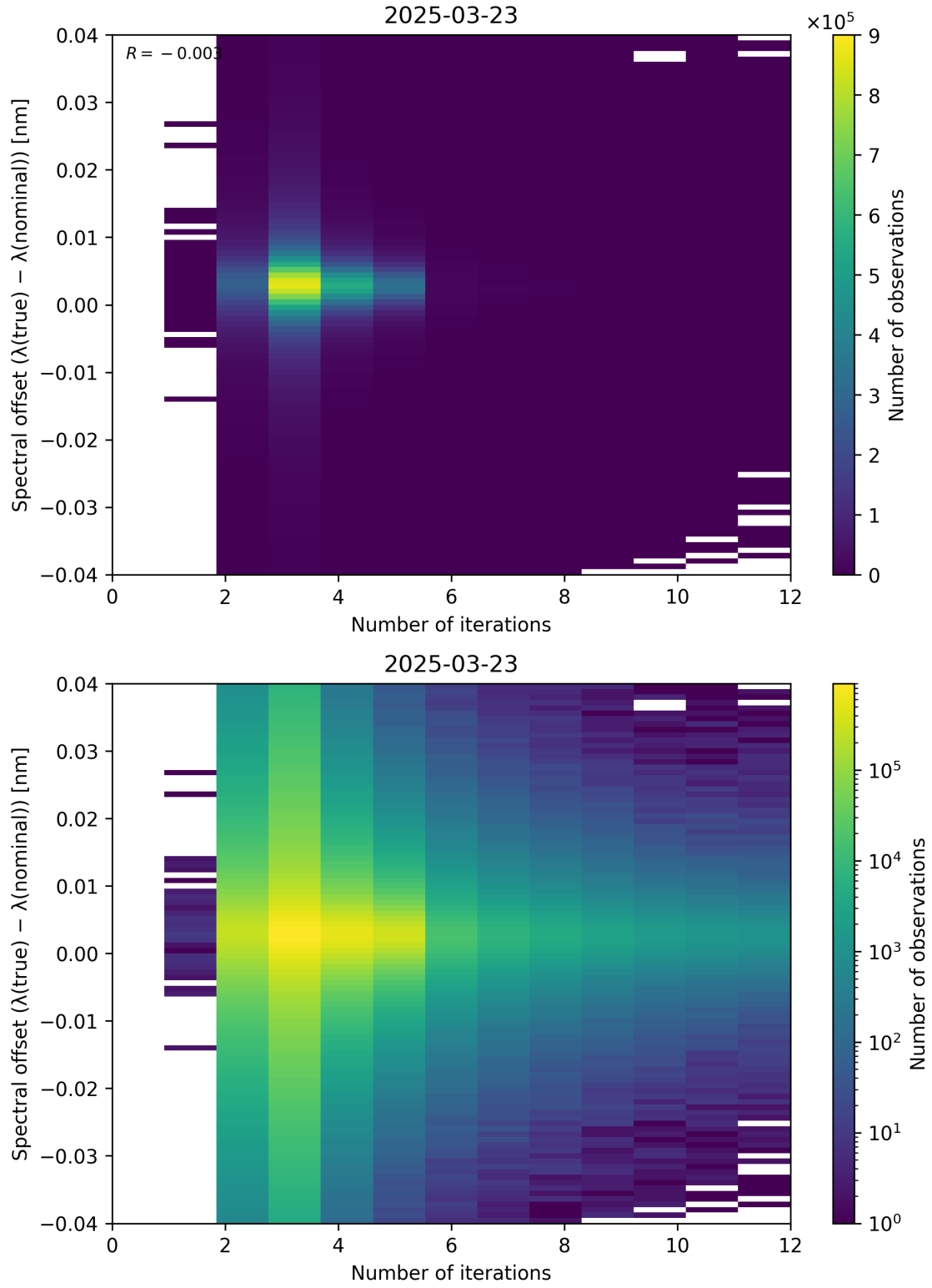
Figure 100: Scatter density plot of “Number of iterations” against “Spectral offset ( \lambda_{\text{true}} - \lambda_{\text{nominal}} )” for 2025-03-23 to 2025-03-24.
