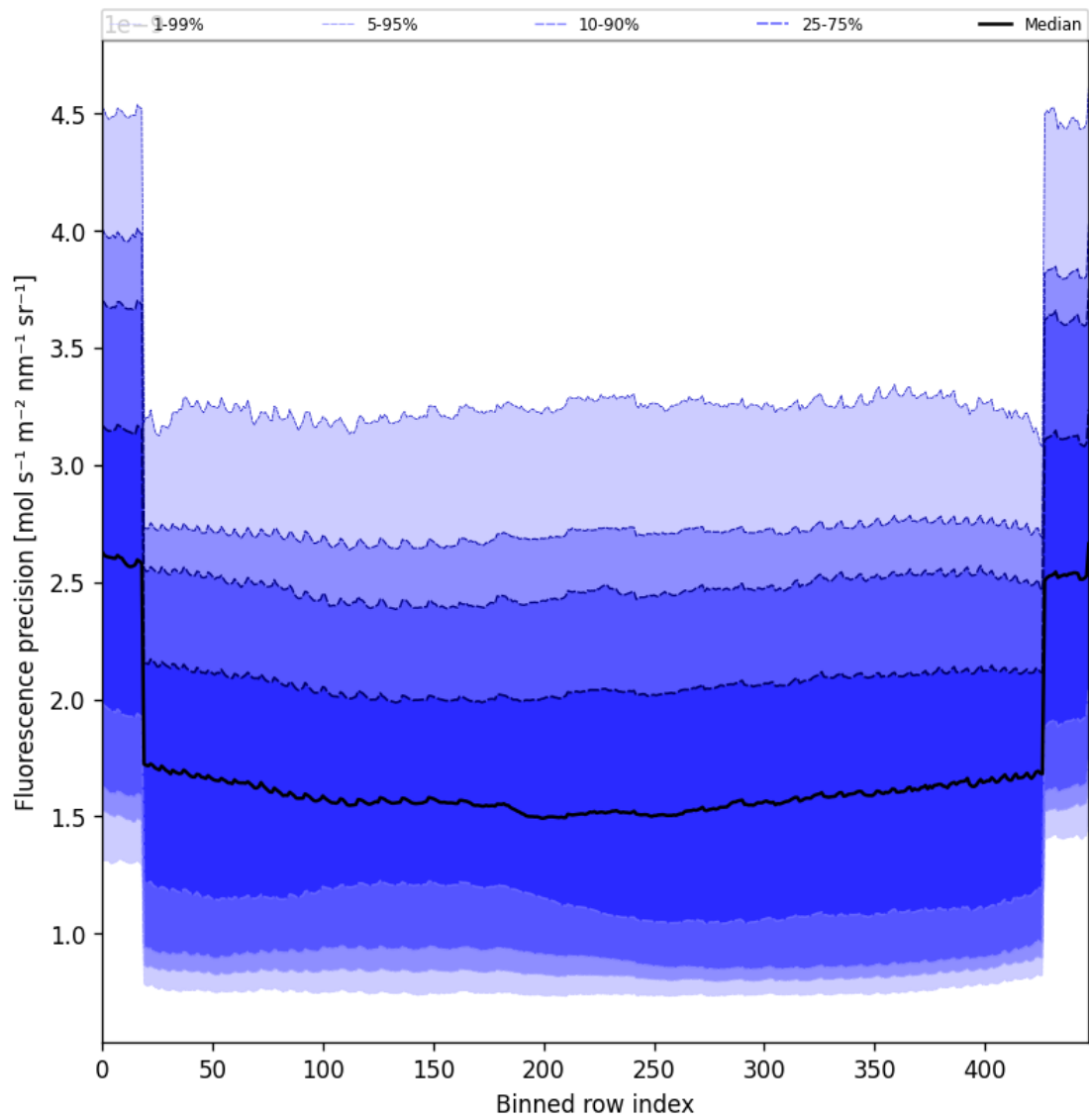
Figure 58: Along track statistics of “Fluorescence precision” for 2025-03-23 to 2025-03-24
