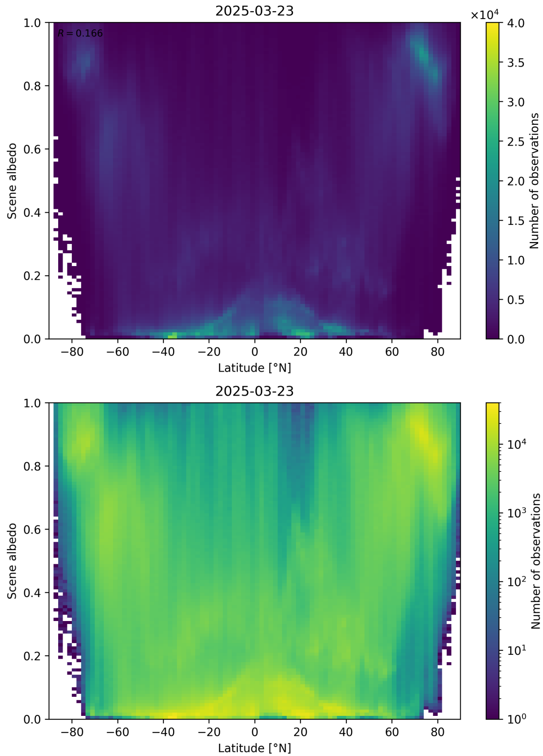
Figure 95: Scatter density plot of “Latitude” against “Scene albedo” for 2025-03-23 to 2025-03-24.
