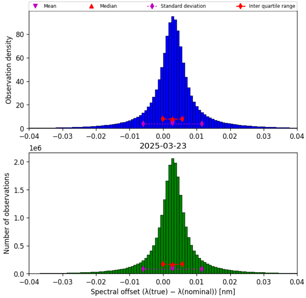
Figure 45: Histogram of “Spectral offset ( \lambda_{\text{true}} - \lambda_{\text{nominal}} )” for 2025-03-23 to 2025-03-24
