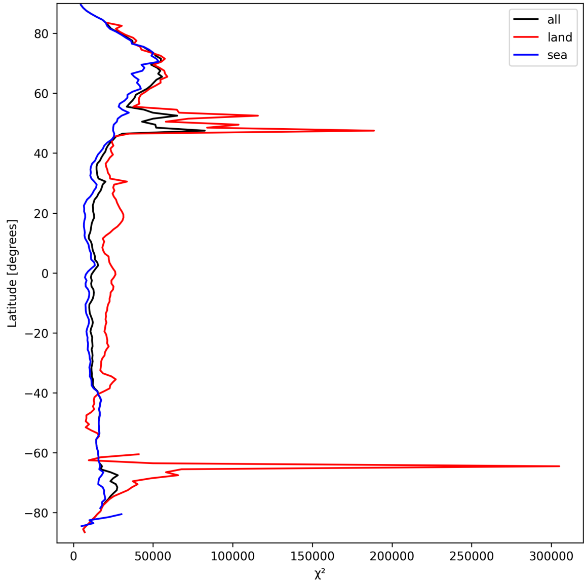
Figure 21: Zonal average of “ \chi^2 ” for 2025-03-23 to 2025-03-24.
