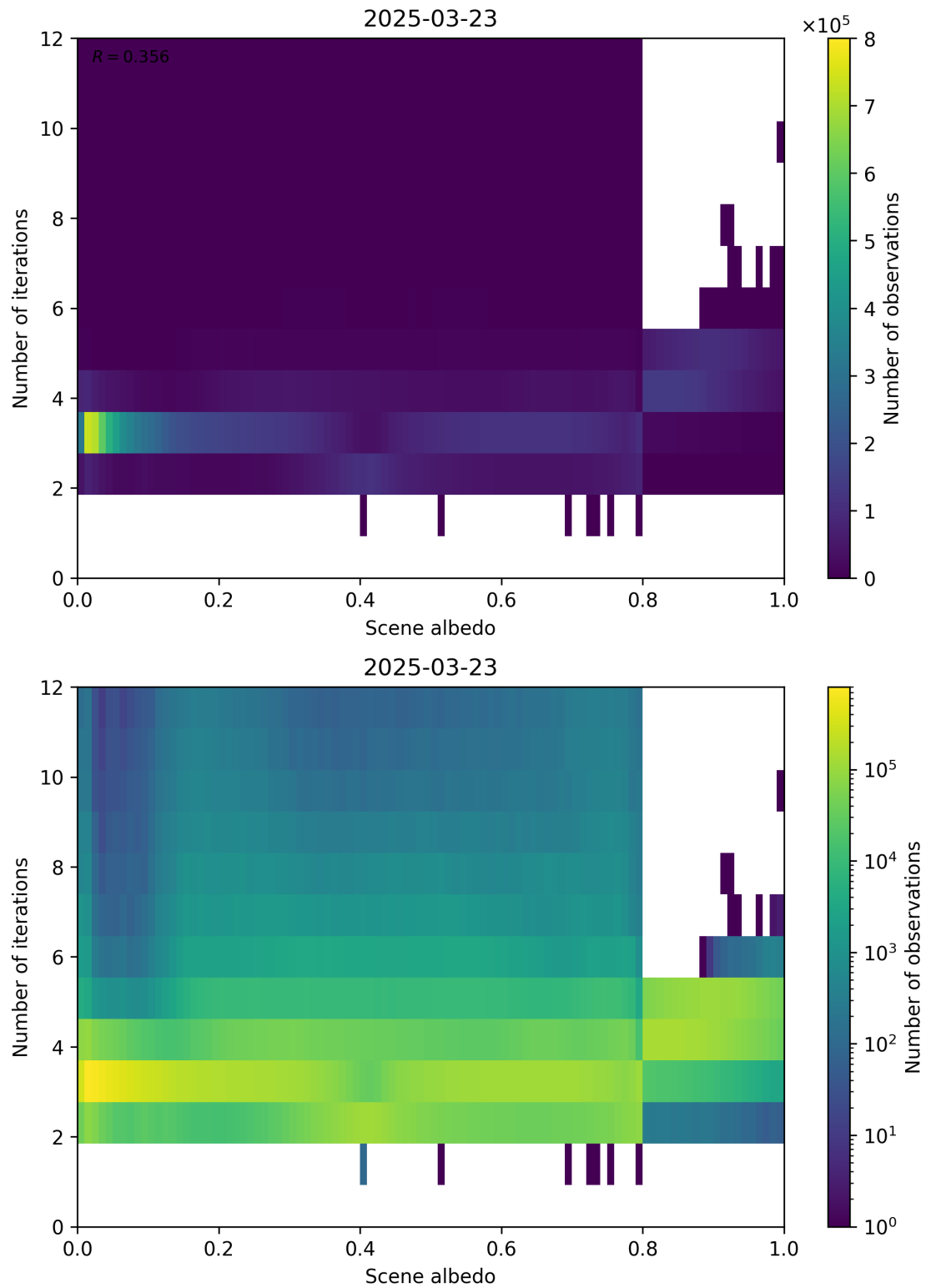
Figure 105: Scatter density plot of “Scene albedo” against “Number of iterations” for 2025-03-23 to 2025-03-24.
