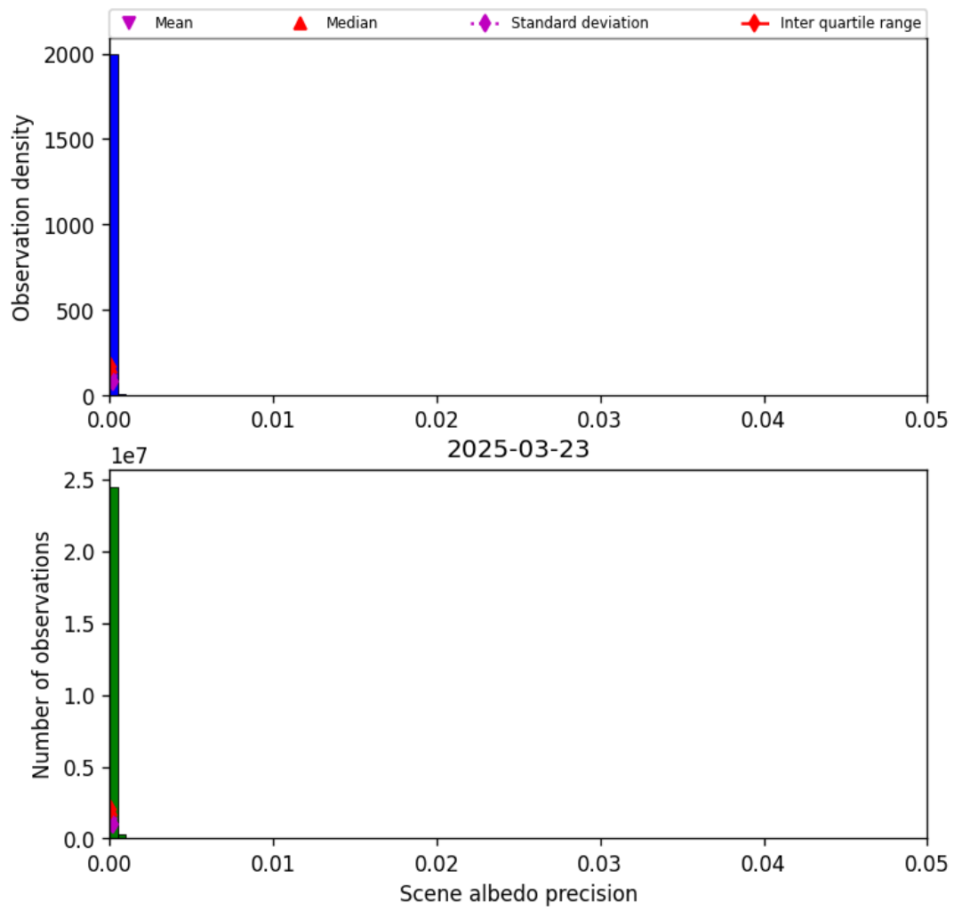
Figure 35: Histogram of “Scene albedo precision” for 2025-03-23 to 2025-03-24
