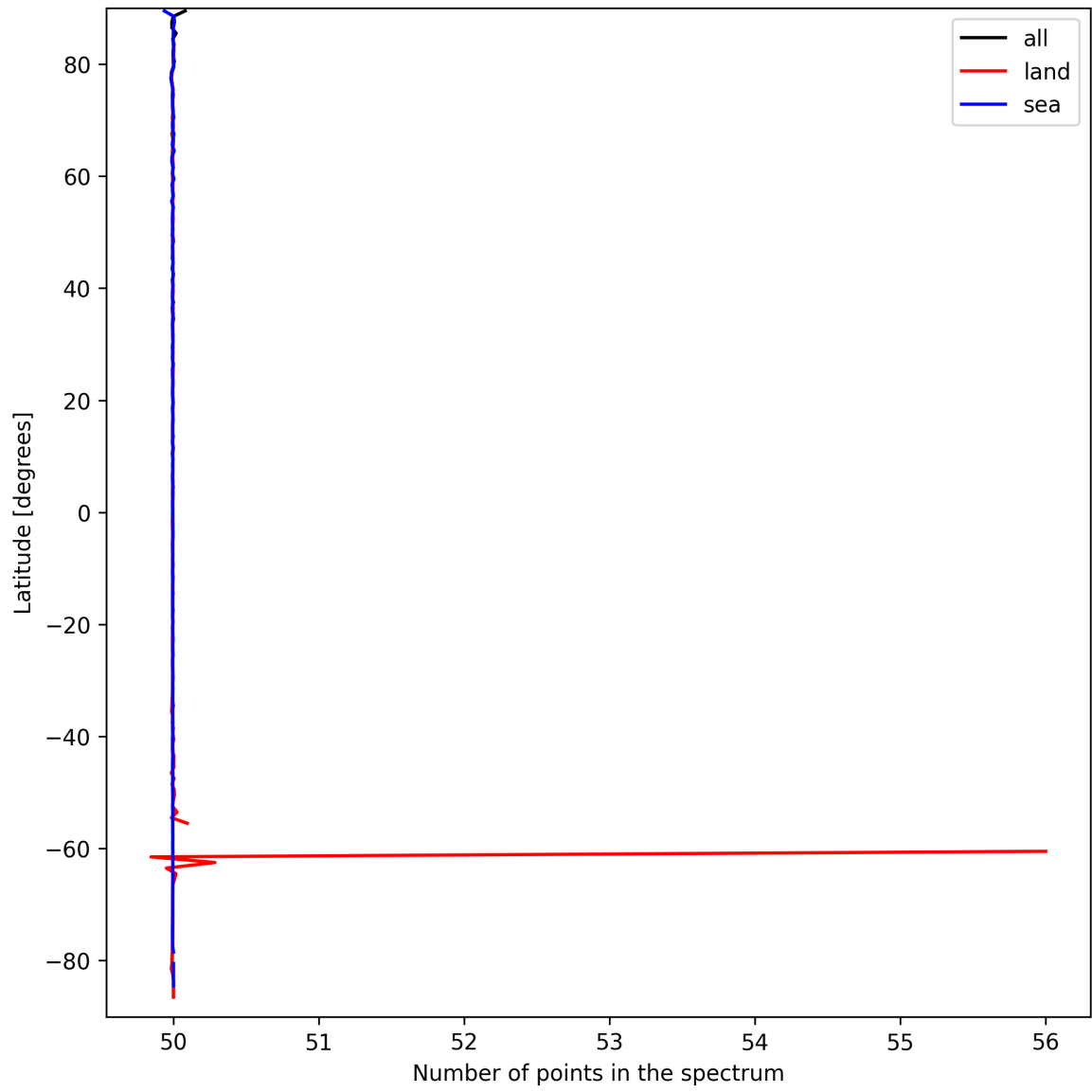
Figure 27: Zonal average of “Number of points in the spectrum” for 2025-03-23 to 2025-03-24.
