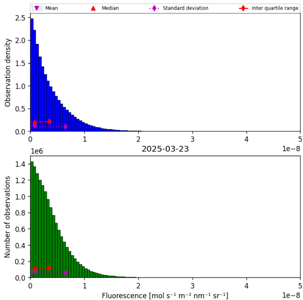
Figure 40: Histogram of “Fluorescence” for 2025-03-23 to 2025-03-24
