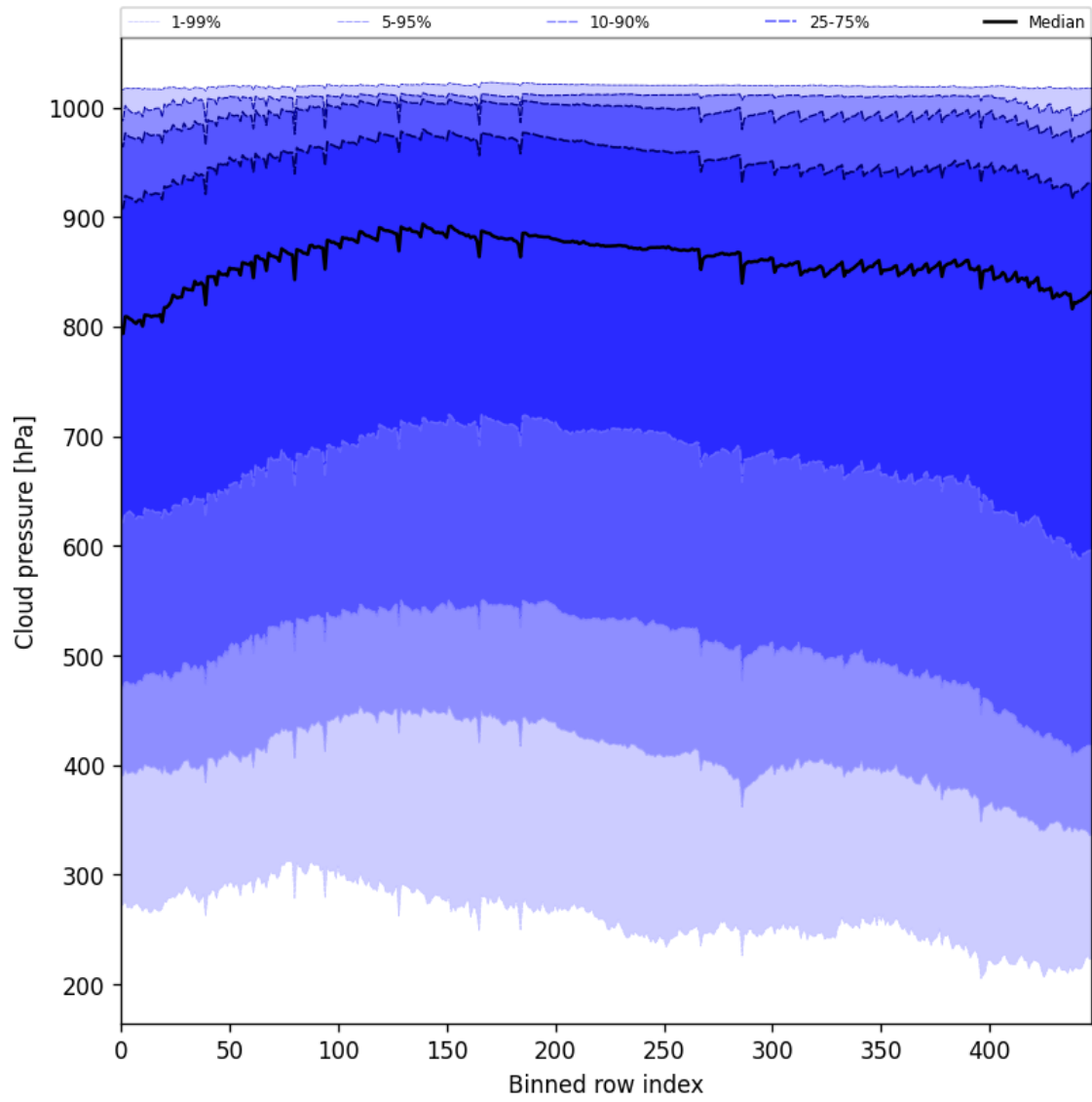
Figure 47: Along track statistics of “Cloud pressure” for 2025-03-23 to 2025-03-24
