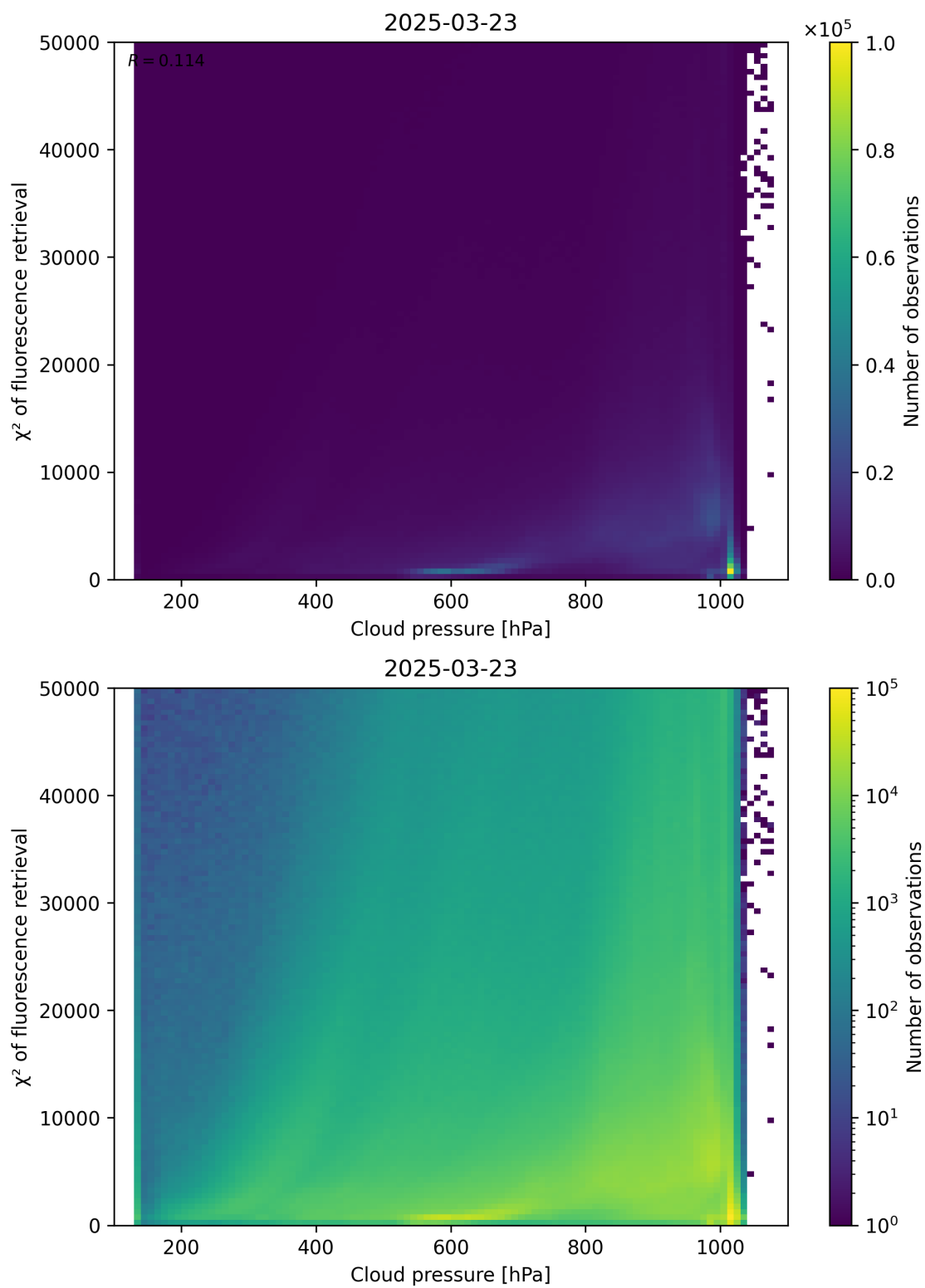
Figure 78: Scatter density plot of “Cloud pressure” against “ \chi^2 of fluorescence retrieval” for 2025-03-23 to 2025-03-24.
