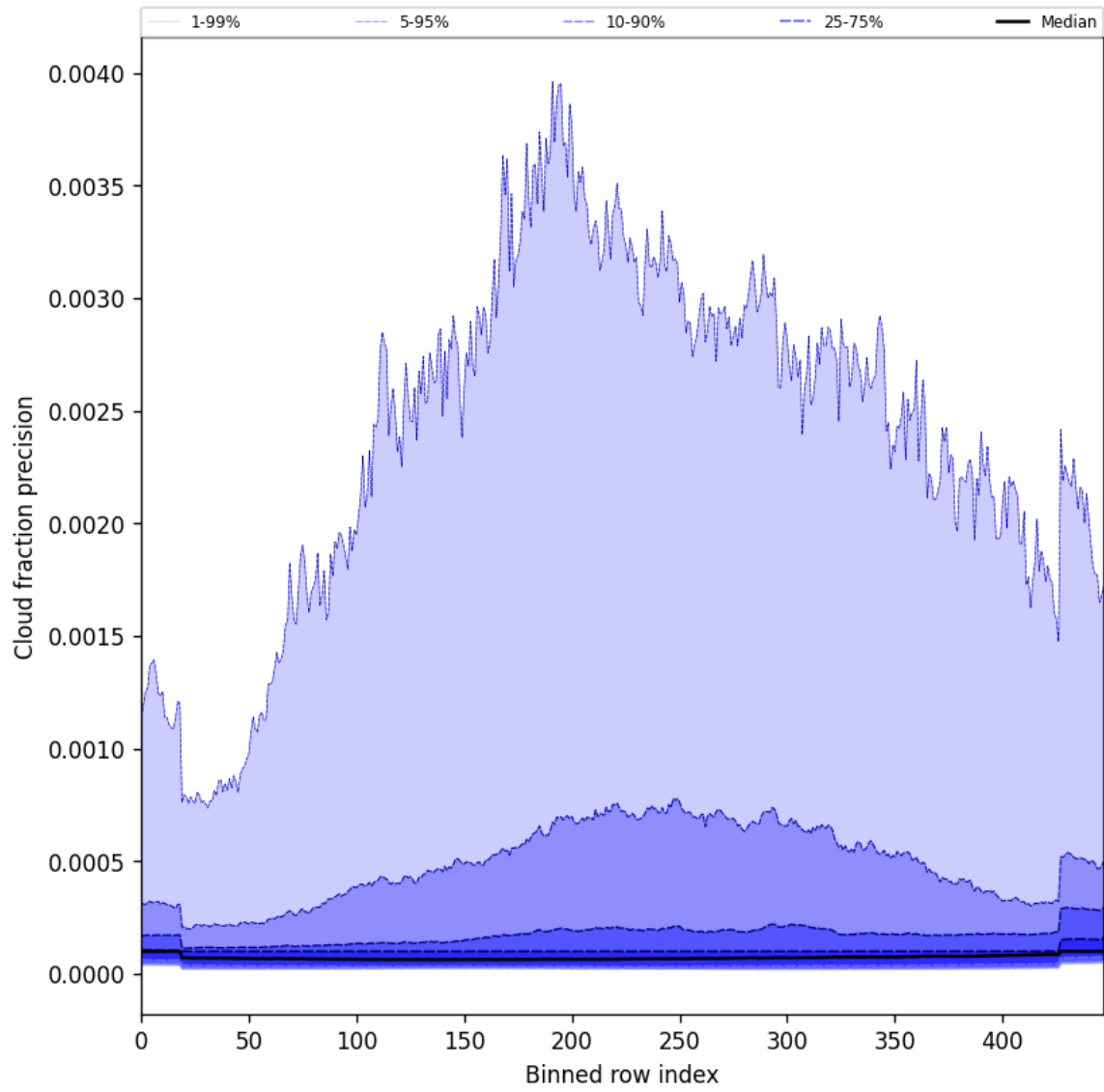
Figure 50: Along track statistics of “Cloud fraction precision” for 2025-03-23 to 2025-03-24
