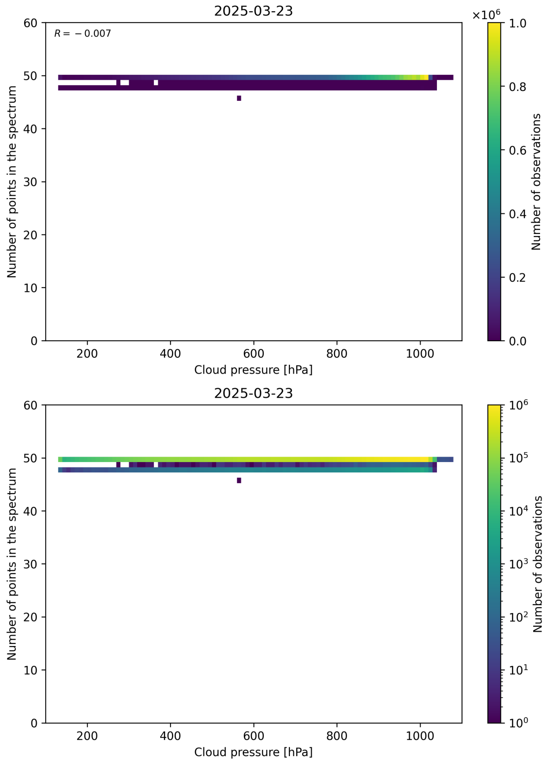
Figure 82: Scatter density plot of “Cloud pressure” against “Number of points in the spectrum” for 2025-03-23 to 2025-03-24.
