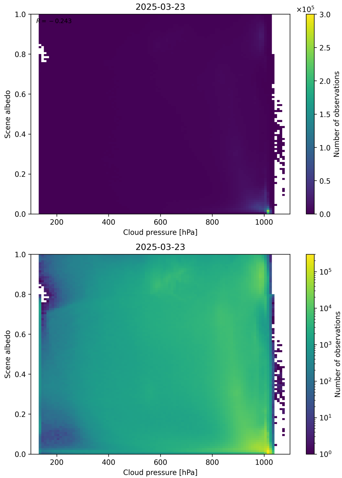
Figure 83: Scatter density plot of “Cloud pressure” against “Scene albedo” for 2025-03-23 to 2025-03-24.
