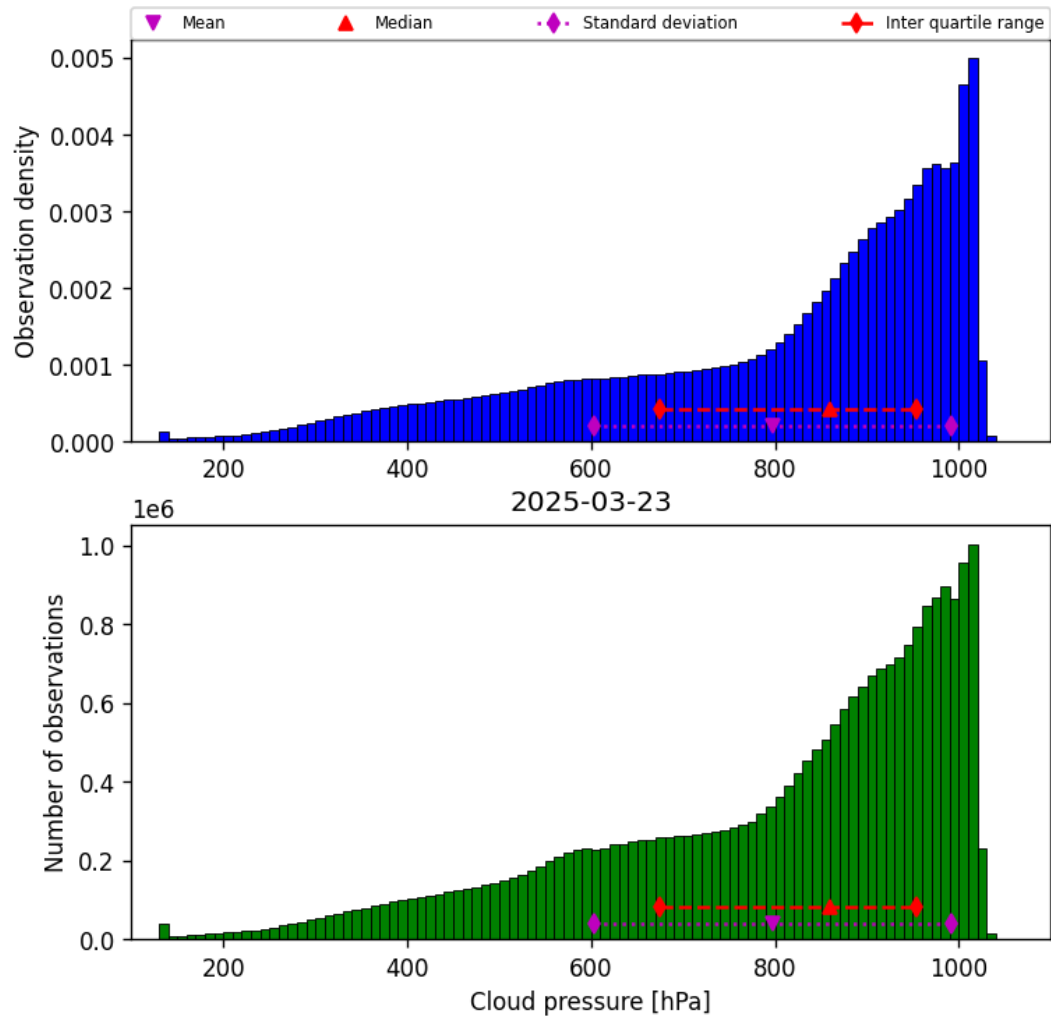
Figure 30: Histogram of “Cloud pressure” for 2025-03-23 to 2025-03-24
