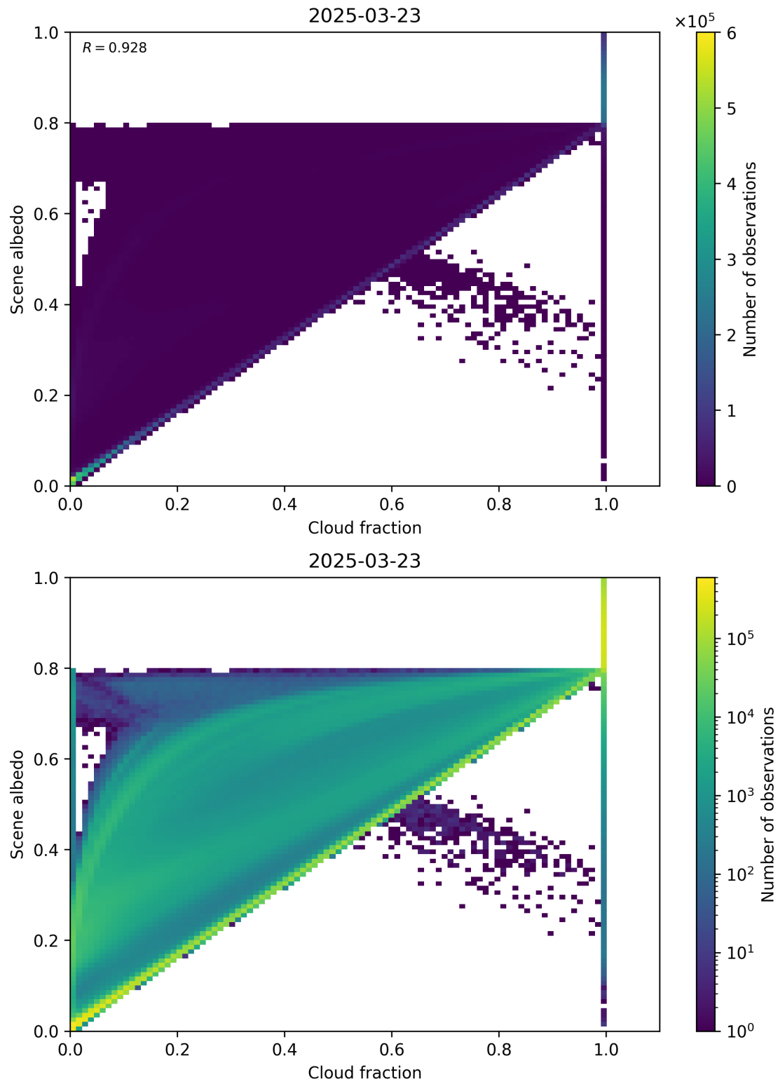
Figure 75: Scatter density plot of “Cloud fraction” against “Scene albedo” for 2025-03-23 to 2025-03-24.
