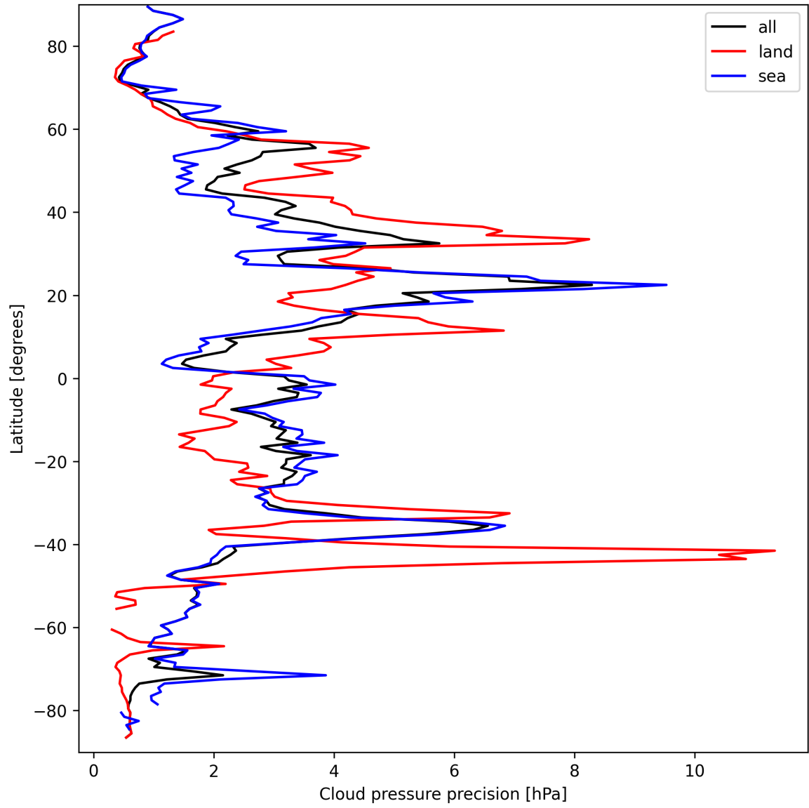
Figure 14: Zonal average of “Cloud pressure precision” for 2025-03-23 to 2025-03-24.
