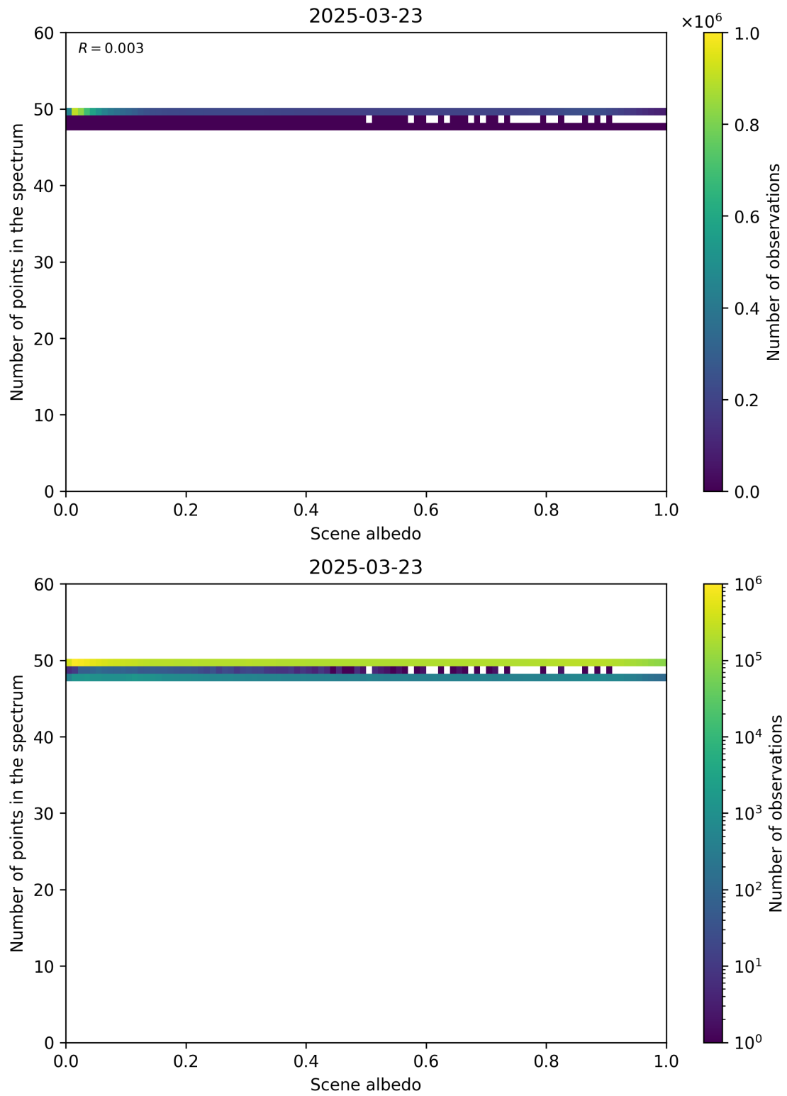
Figure 106: Scatter density plot of “Scene albedo” against “Number of points in the spectrum” for 2025-03-23 to 2025-03-24.
