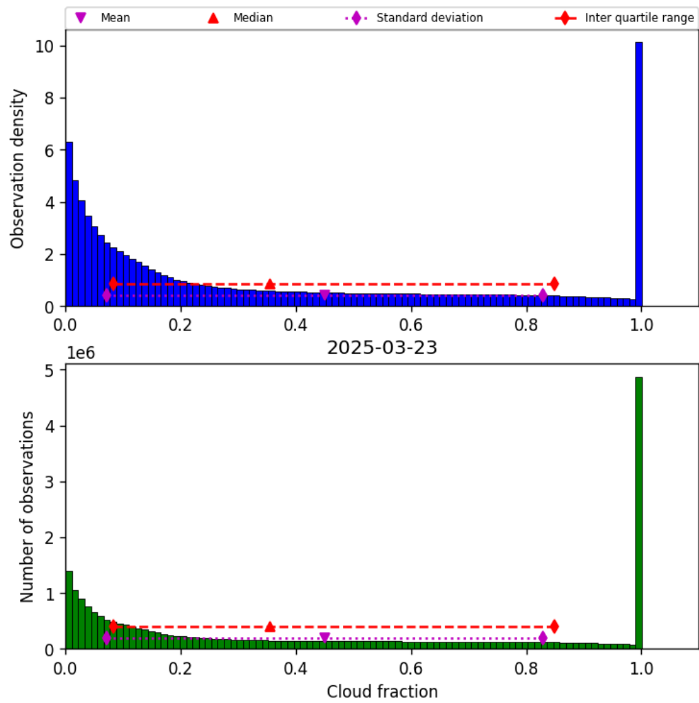
Figure 32: Histogram of “Cloud fraction” for 2025-03-23 to 2025-03-24
