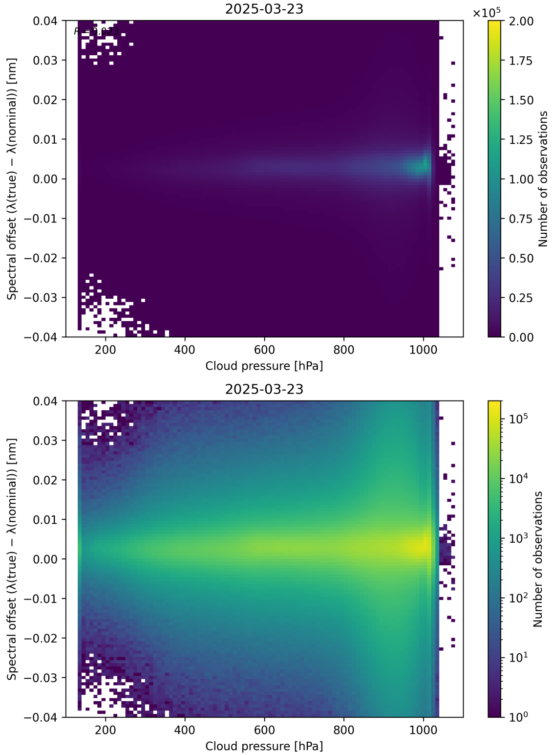
Figure 84: Scatter density plot of “Cloud pressure” against “Spectral offset ( \lambda_{\text{true}} - \lambda_{\text{nominal}} )” for 2025-03-23 to 2025-03-24.
