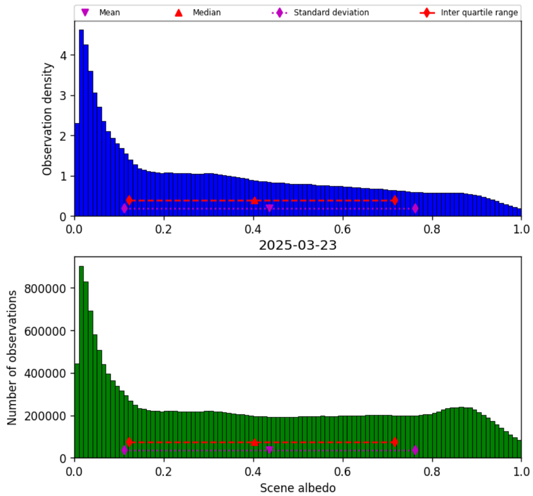
Figure 34: Histogram of “Scene albedo” for 2025-03-23 to 2025-03-24
