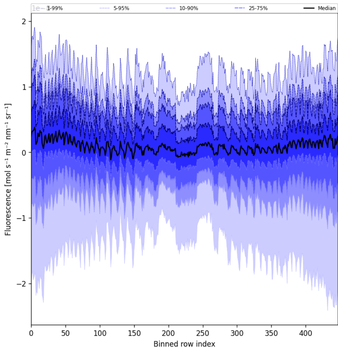
Figure 57: Along track statistics of “Fluorescence” for 2025-03-23 to 2025-03-24
