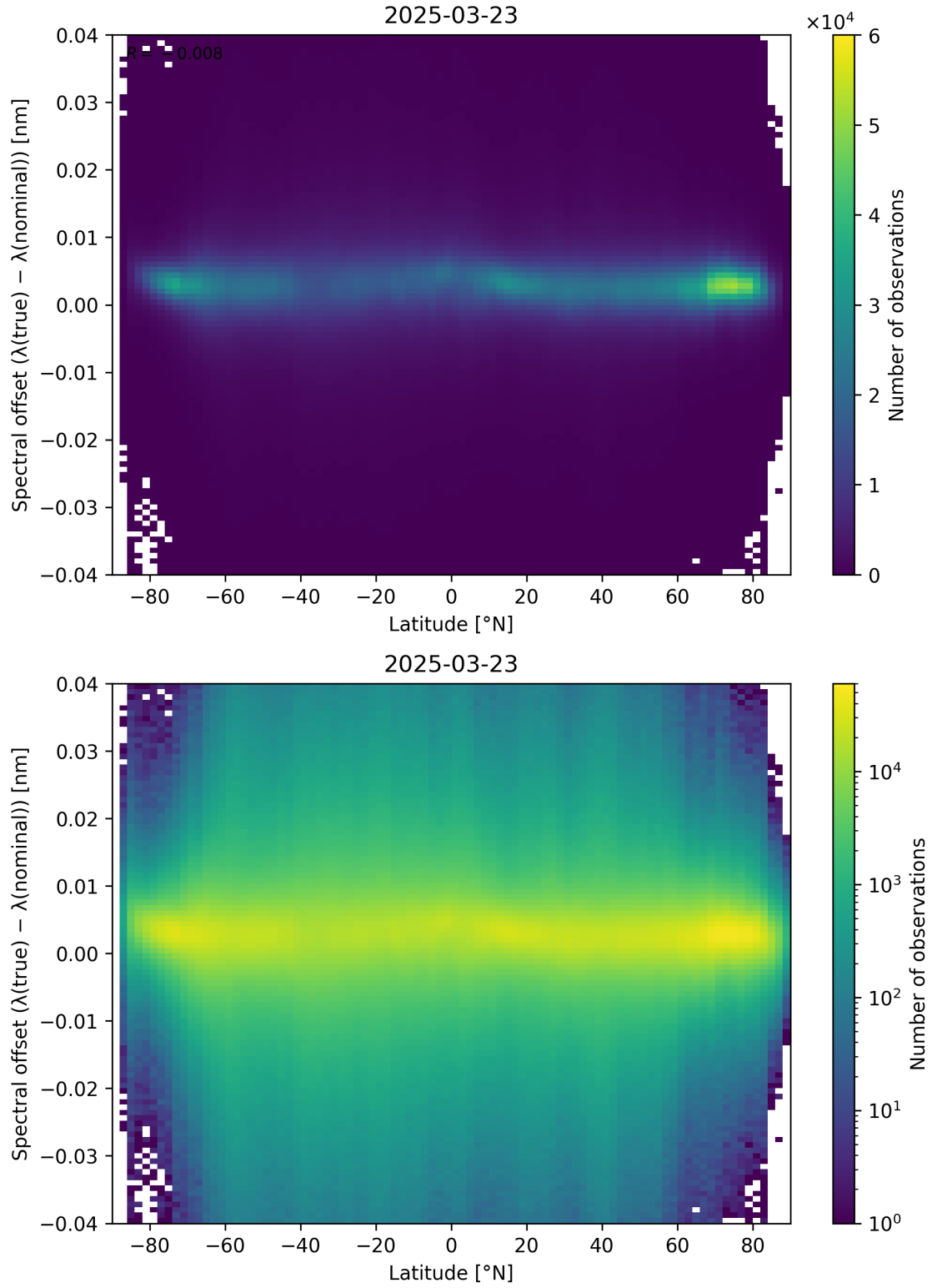
Figure 96: Scatter density plot of “Latitude” against “Spectral offset ( \lambda_{\text{true}} - \lambda_{\text{nominal}} )” for 2025-03-23 to 2025-03-24.
