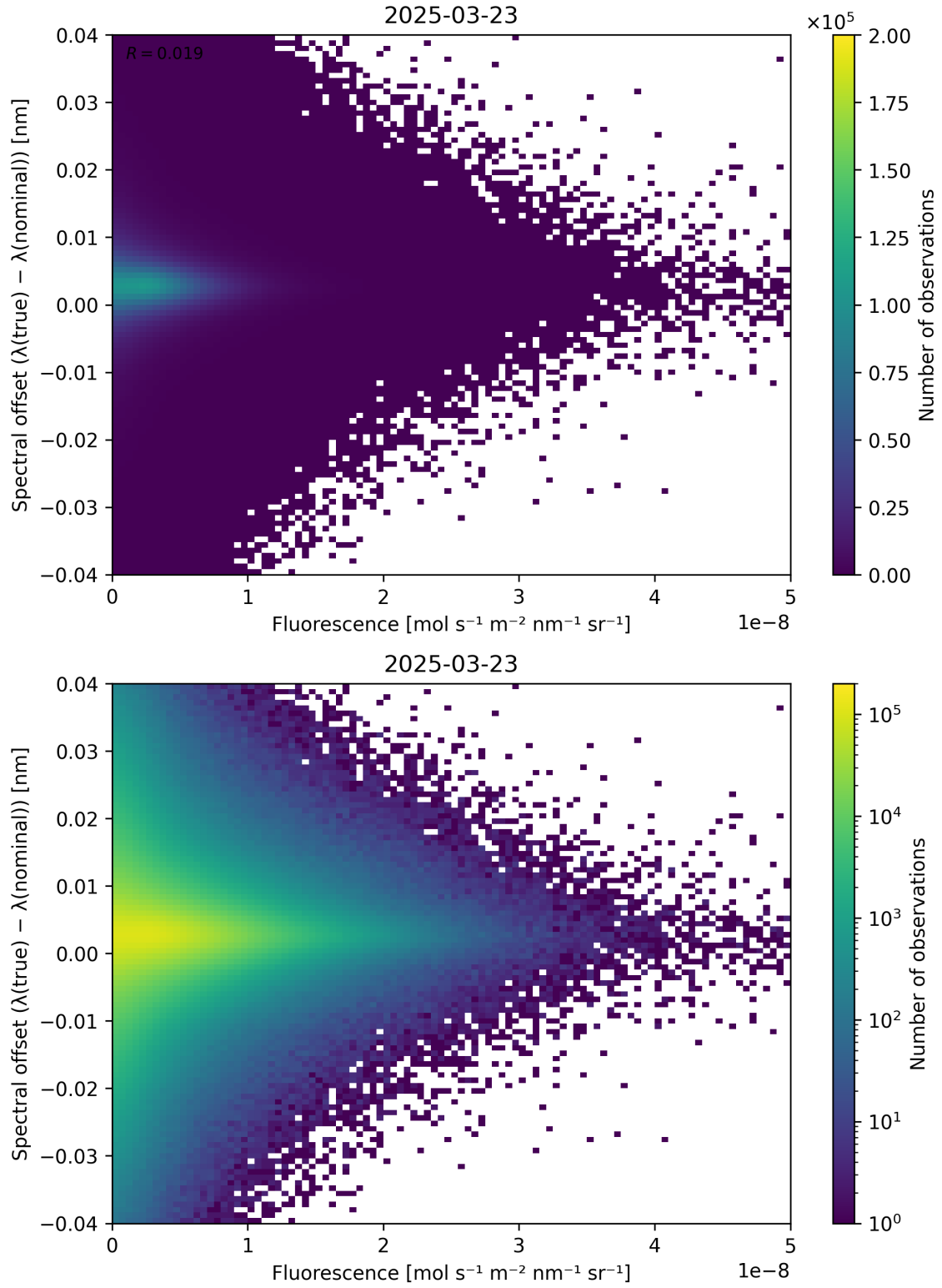
Figure 87: Scatter density plot of “Fluorescence” against “Spectral offset ( \lambda_{\text{true}} - \lambda_{\text{nominal}} )” for 2025-03-23 to 2025-03-24.
