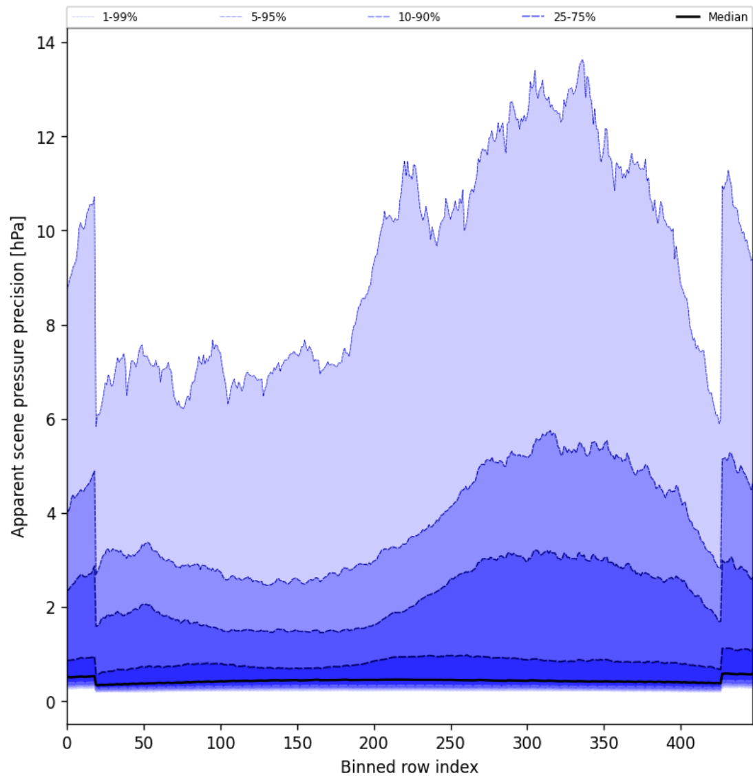
Figure 54: Along track statistics of “Apparent scene pressure precision” for 2025-03-23 to 2025-03-24
