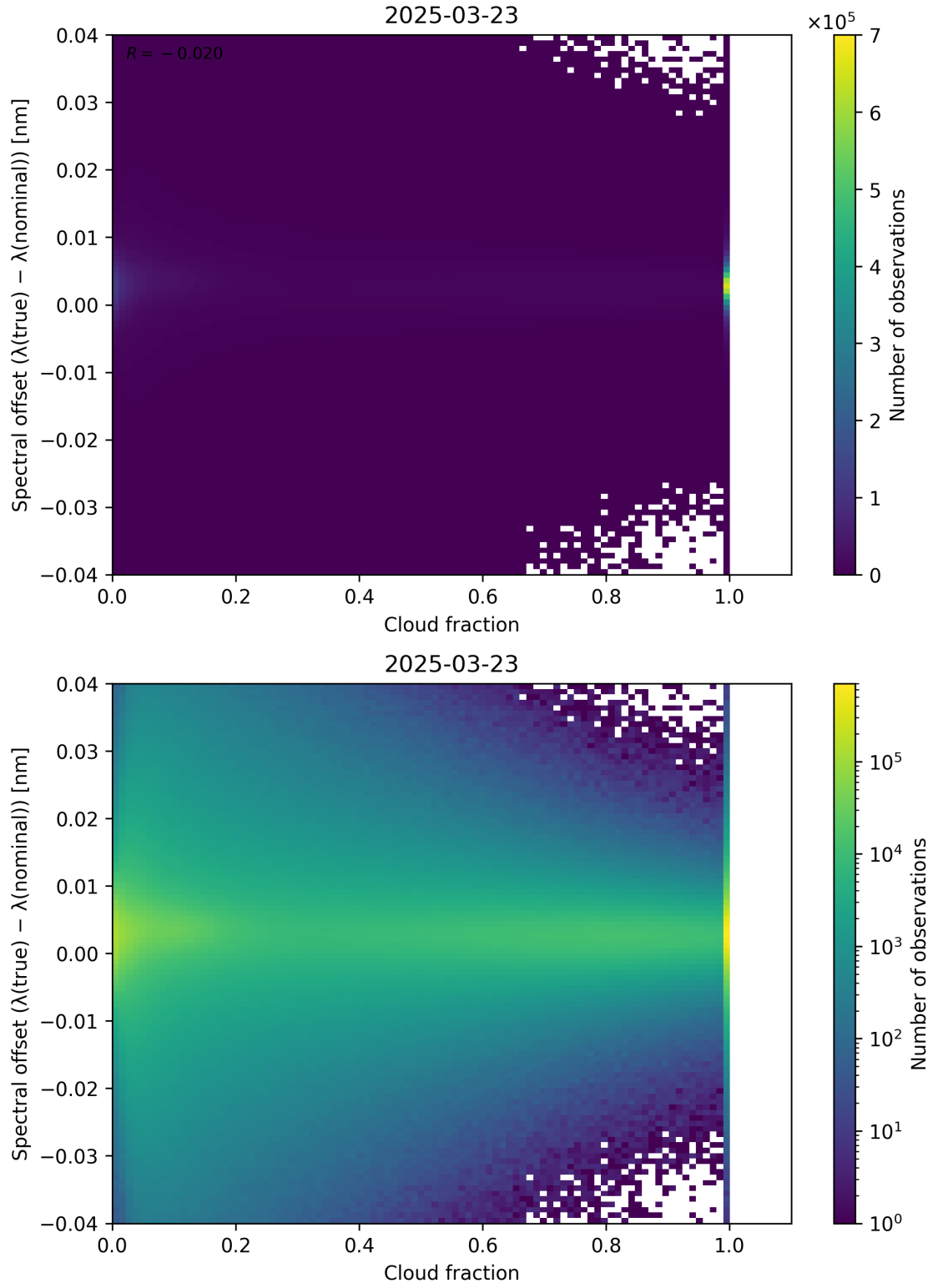
Figure 76: Scatter density plot of “Cloud fraction” against “Spectral offset ( \lambda_{\text{true}} - \lambda_{\text{nominal}} )” for 2025-03-23 to 2025-03-24.
