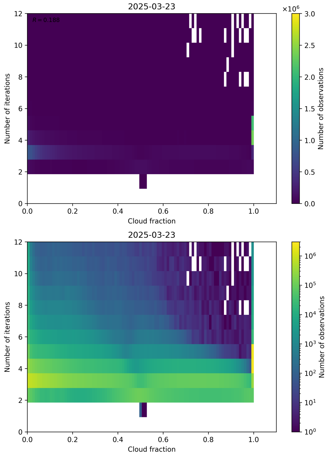
Figure 73: Scatter density plot of “Cloud fraction” against “Number of iterations” for 2025-03-23 to 2025-03-24.
