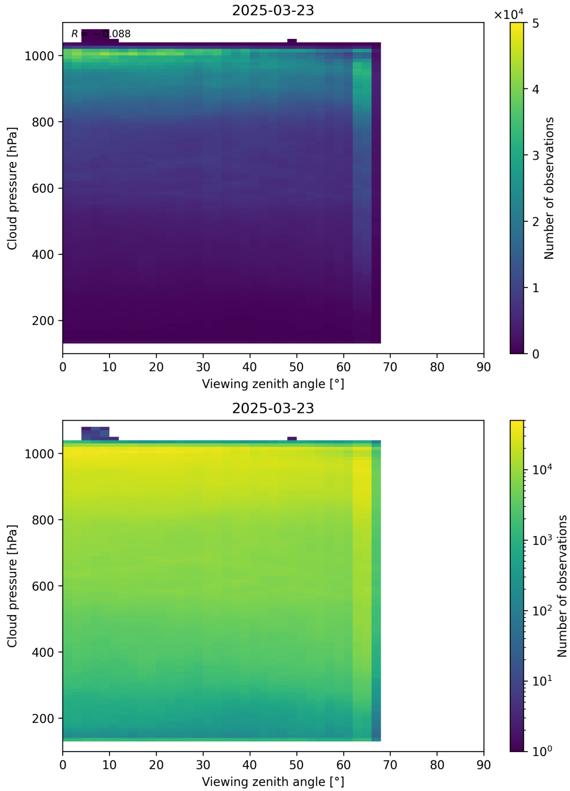
Figure 121: Scatter density plot of “Viewing zenith angle” against “Cloud pressure” for 2025-03-23 to 2025-03-24.
