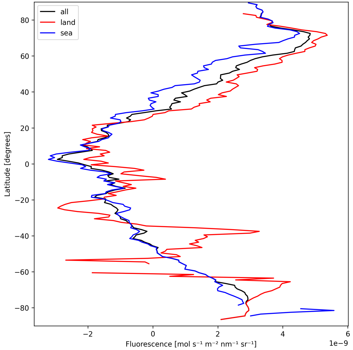
Figure 23: Zonal average of “Fluorescence” for 2025-03-23 to 2025-03-24.
