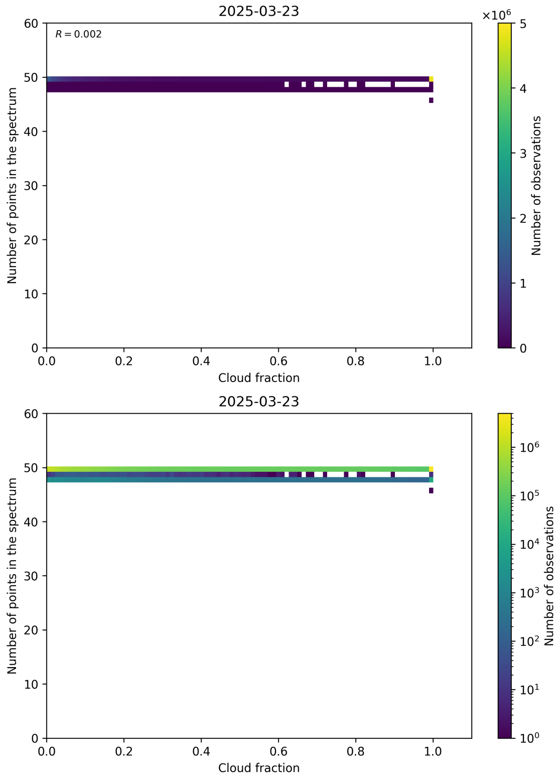
Figure 74: Scatter density plot of “Cloud fraction” against “Number of points in the spectrum” for 2025-03-23 to 2025-03-24.
