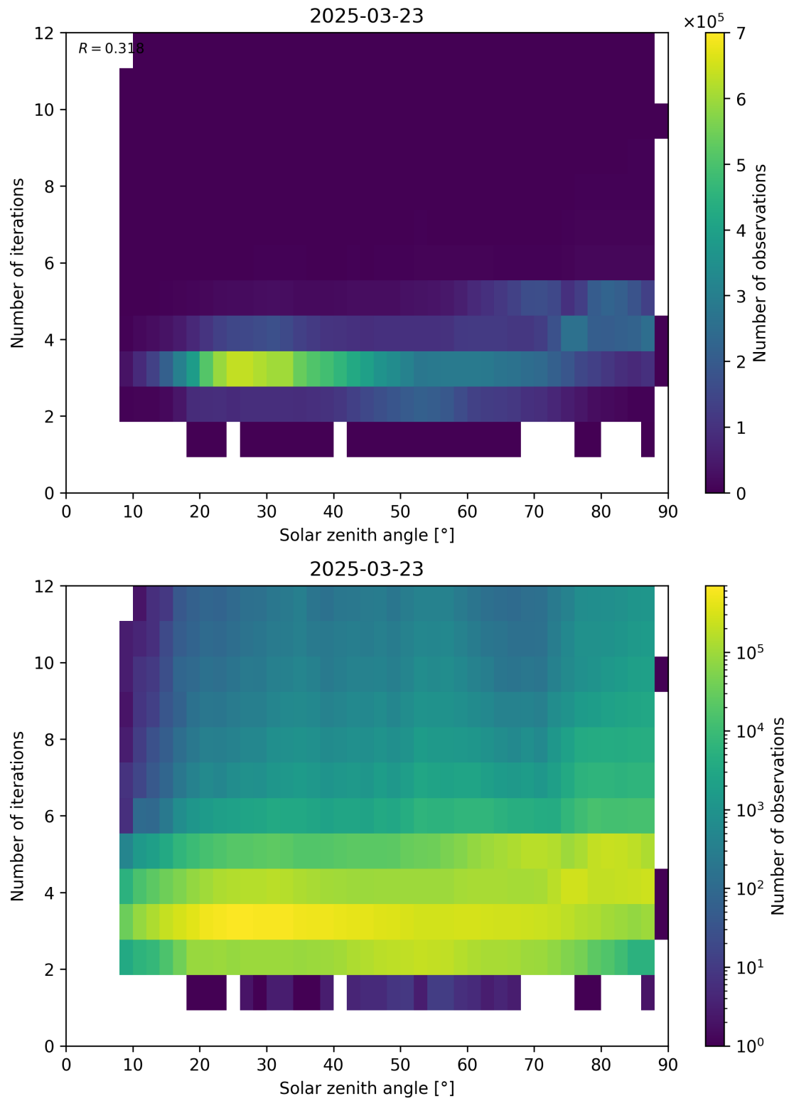
Figure 114: Scatter density plot of “Solar zenith angle” against “Number of iterations” for 2025-03-23 to 2025-03-24.
