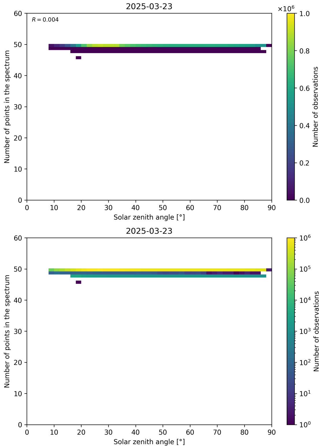
Figure 115: Scatter density plot of “Solar zenith angle” against “Number of points in the spectrum” for 2025-03-23 to 2025-03-24.
