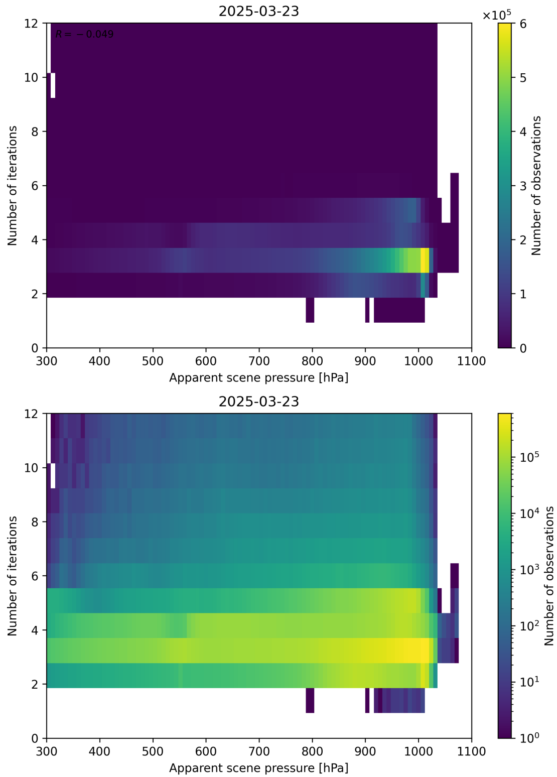
Figure 65: Scatter density plot of “Apparent scene pressure” against “Number of iterations” for 2025-03-23 to 2025-03-24.
