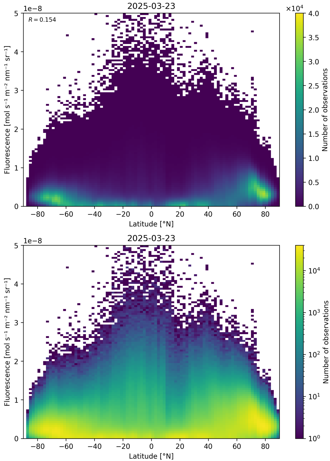
Figure 92: Scatter density plot of “Latitude” against “Fluorescence” for 2025-03-23 to 2025-03-24.
