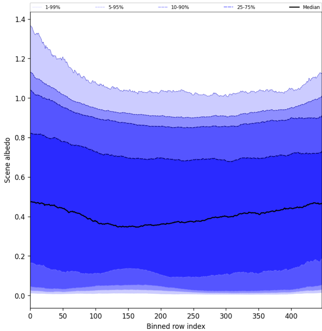
Figure 51: Along track statistics of “Scene albedo” for 2025-03-23 to 2025-03-24
