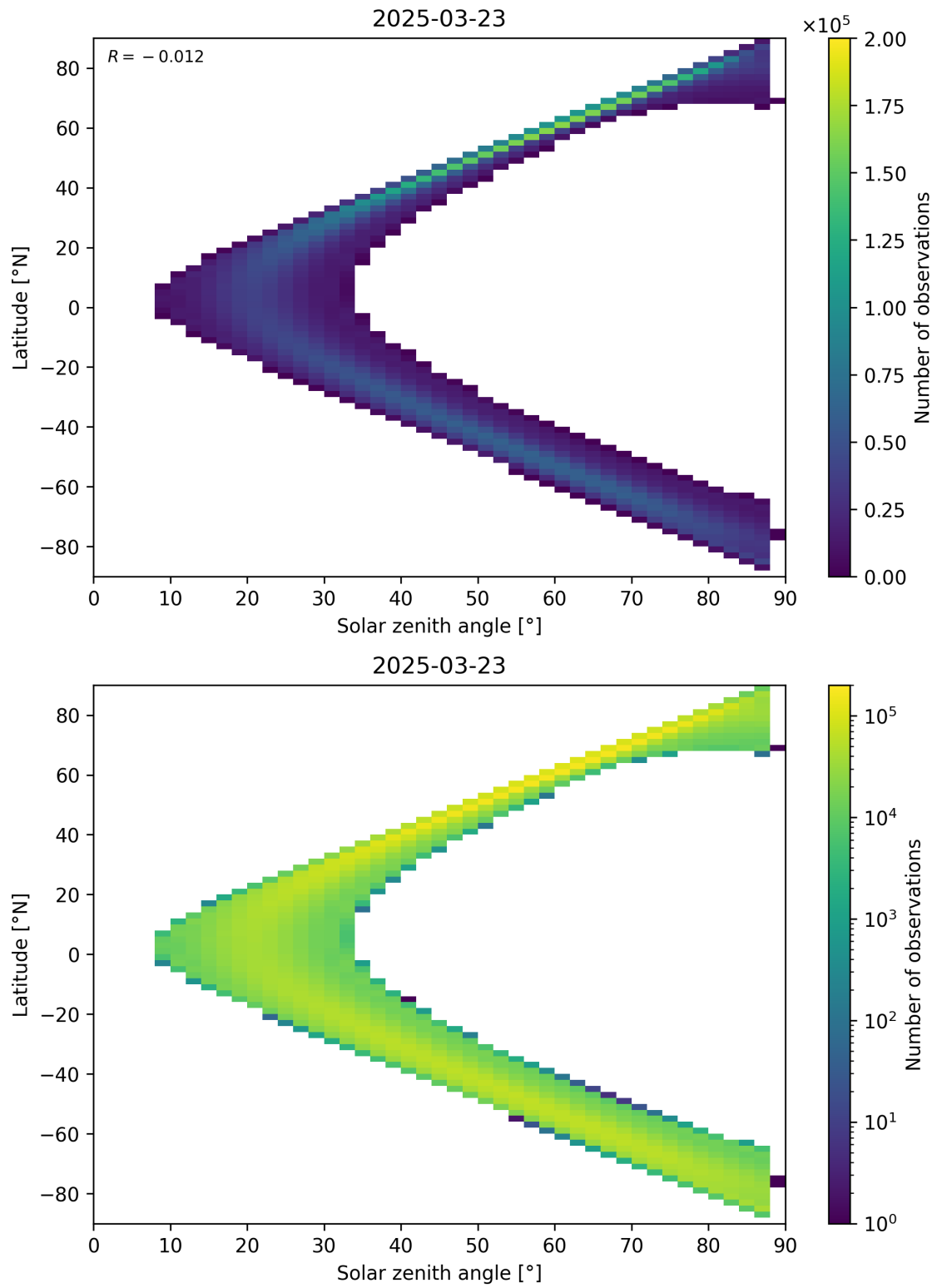
Figure 113: Scatter density plot of “Solar zenith angle” against “Latitude” for 2025-03-23 to 2025-03-24.
