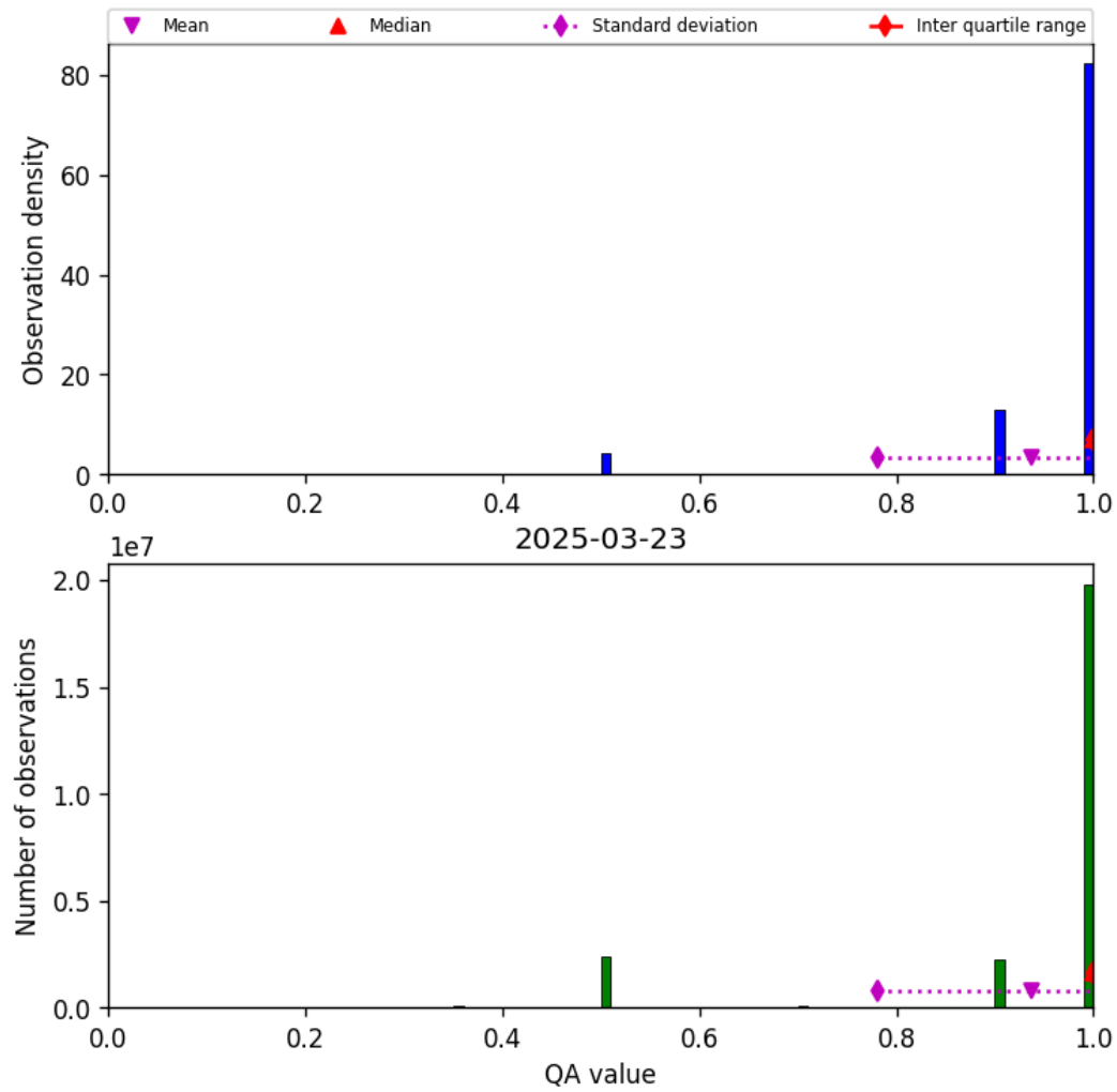
Figure 29: Histogram of “QA value” for 2025-03-23 to 2025-03-24
