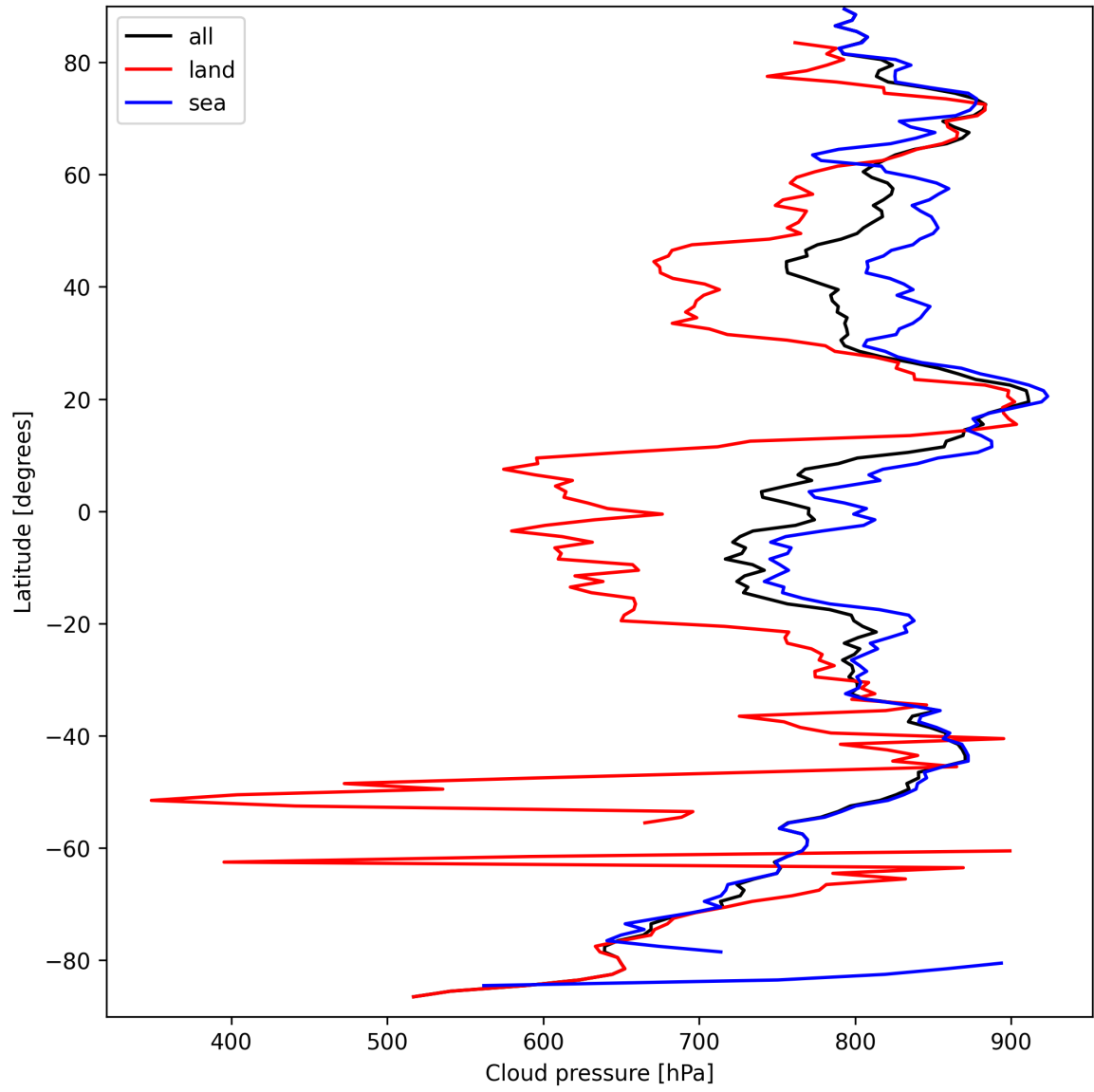
Figure 13: Zonal average of “Cloud pressure” for 2025-03-23 to 2025-03-24.
