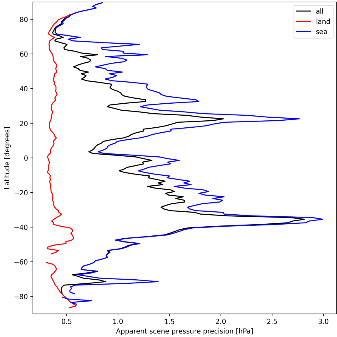
Figure 20: Zonal average of “Apparent scene pressure precision” for 2025-03-23 to 2025-03-24.
