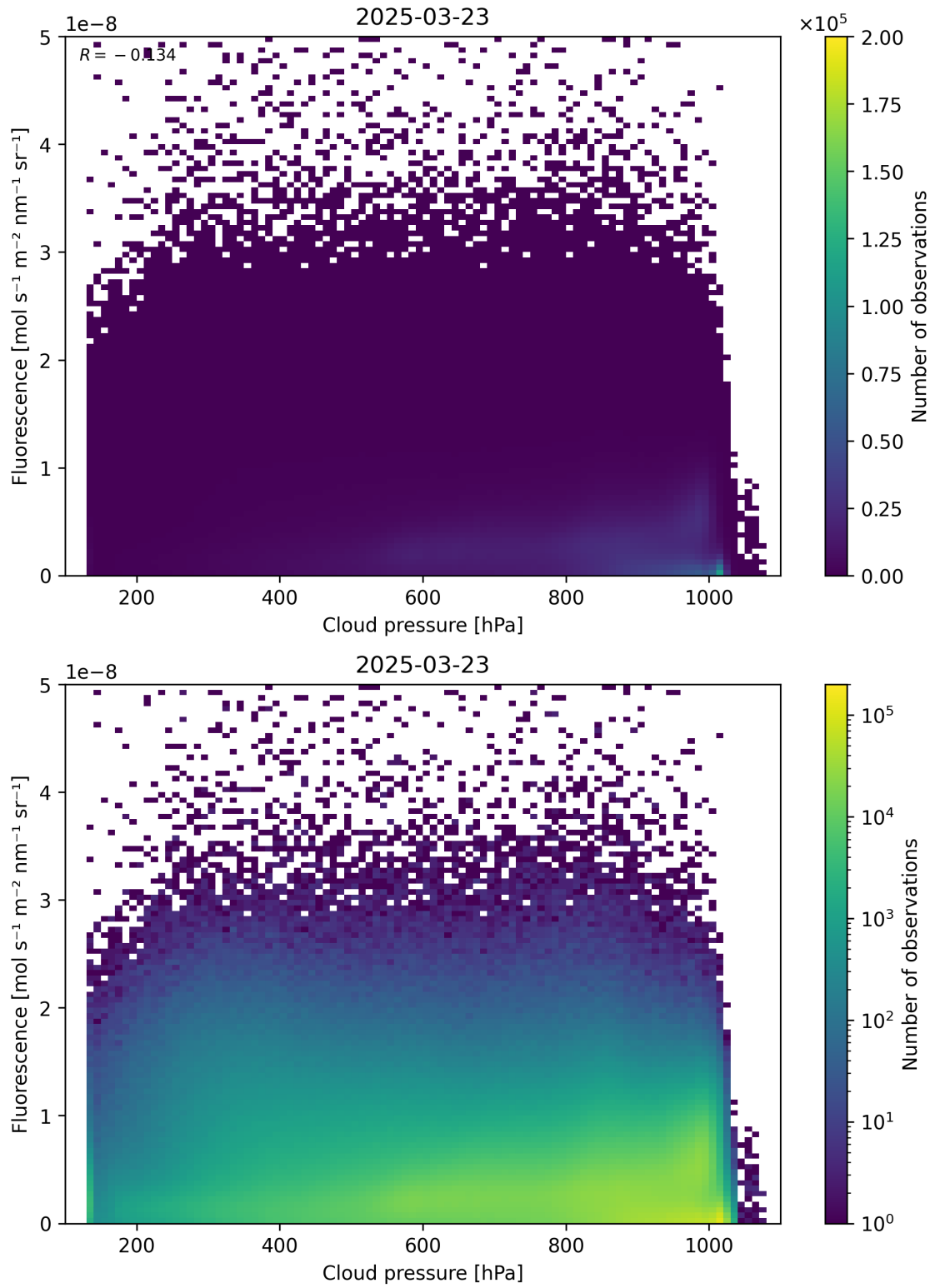
Figure 80: Scatter density plot of “Cloud pressure” against “Fluorescence” for 2025-03-23 to 2025-03-24.
