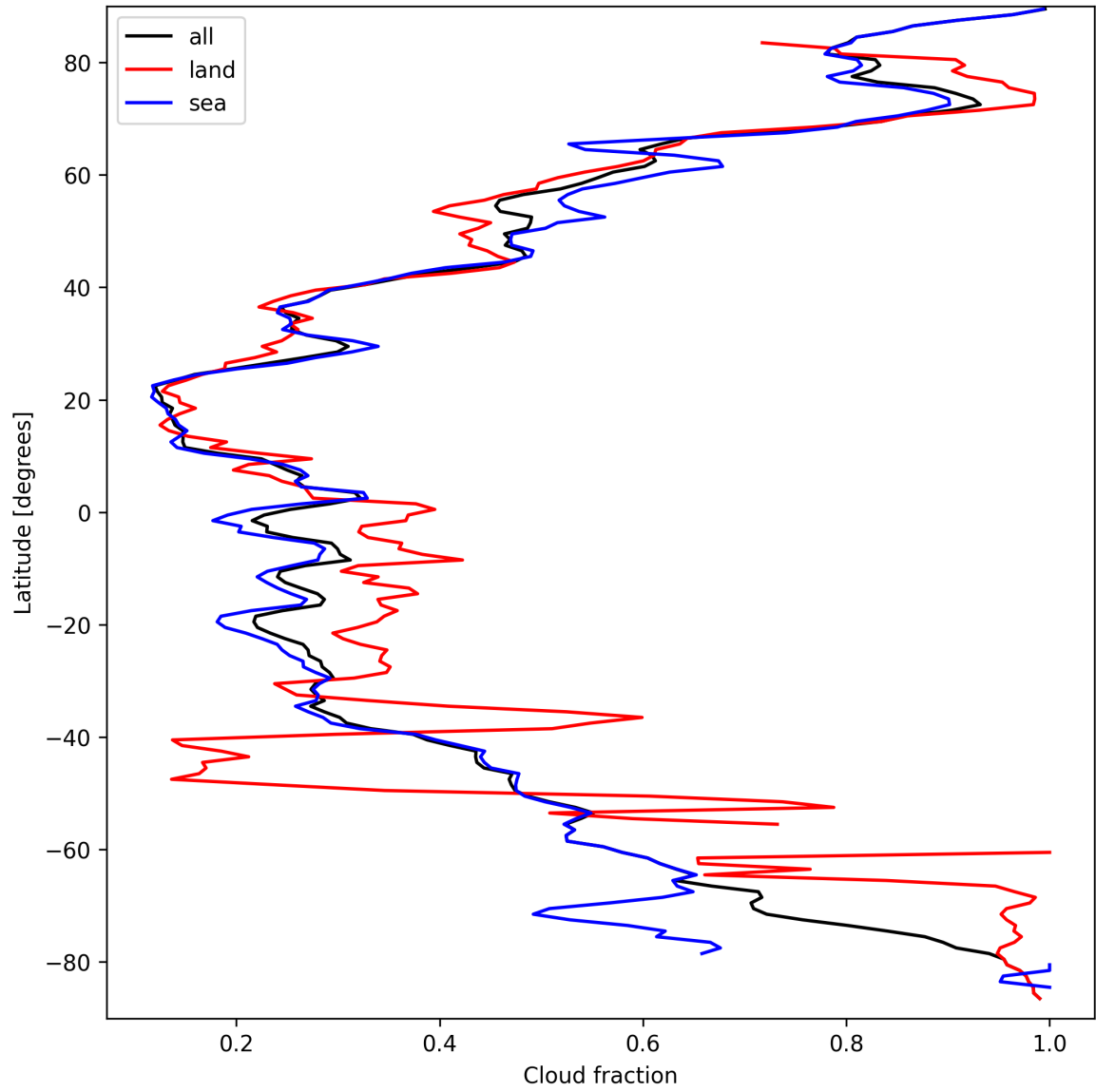
Figure 15: Zonal average of “Cloud fraction” for 2025-03-23 to 2025-03-24.
