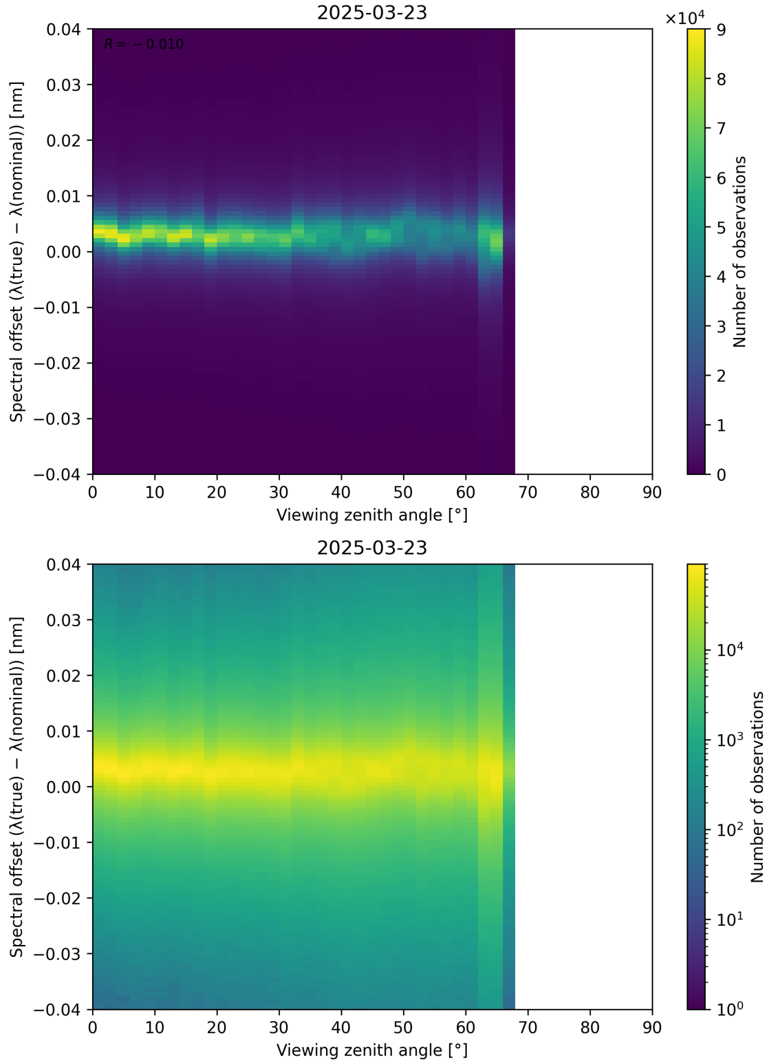
Figure 128: Scatter density plot of “Viewing zenith angle” against “Spectral offset ( \lambda_{\text{true}} - \lambda_{\text{nominal}} )” for 2025-03-23 to 2025-03-24.
