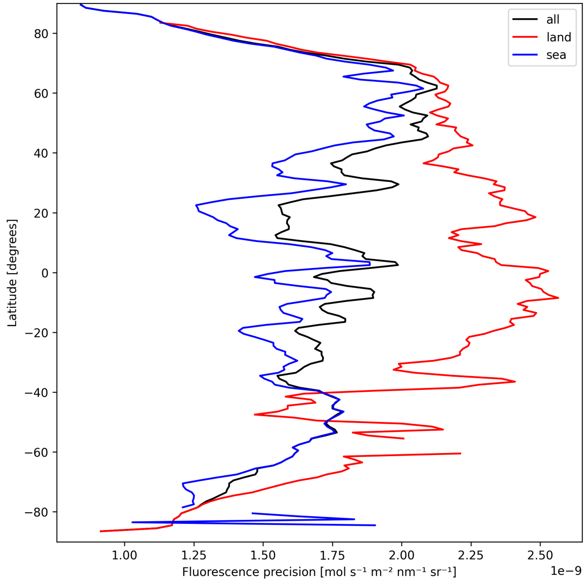
Figure 24: Zonal average of “Fluorescence precision” for 2025-03-23 to 2025-03-24.
