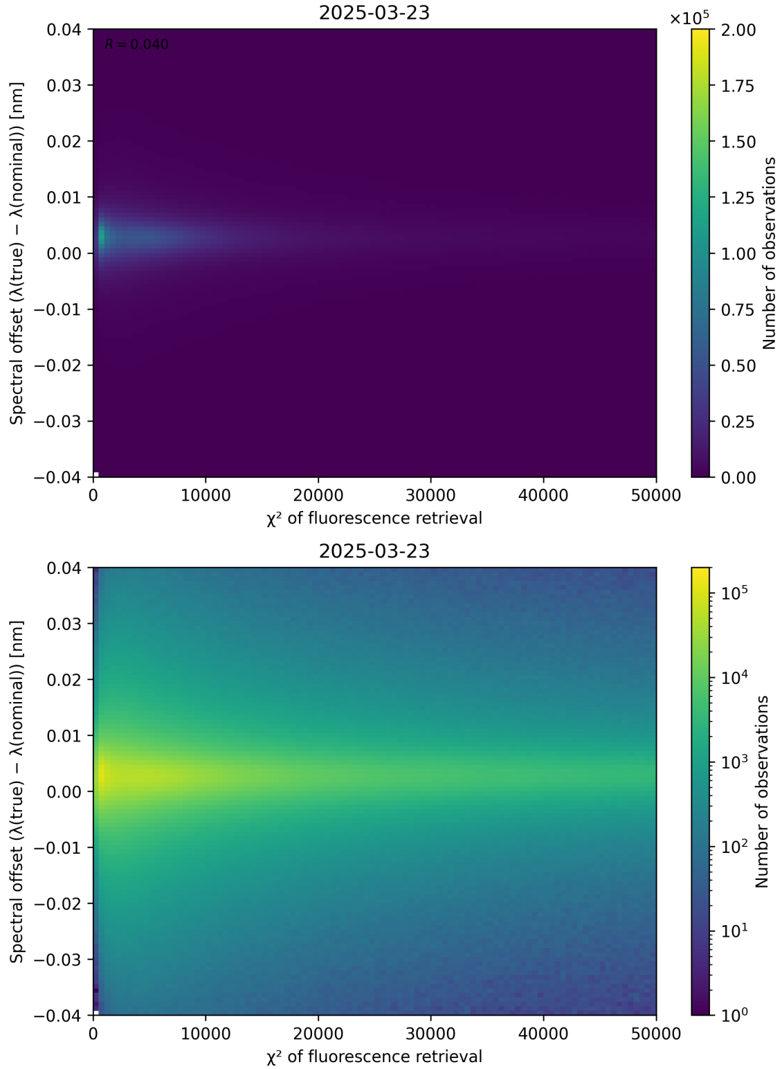
Figure 69: Scatter density plot of “ \chi^2 of fluorescence retrieval” against “Spectral offset ( \lambda_{\text{true}} - \lambda_{\text{nominal}} )” for 2025-03-23 to 2025-03-24.
