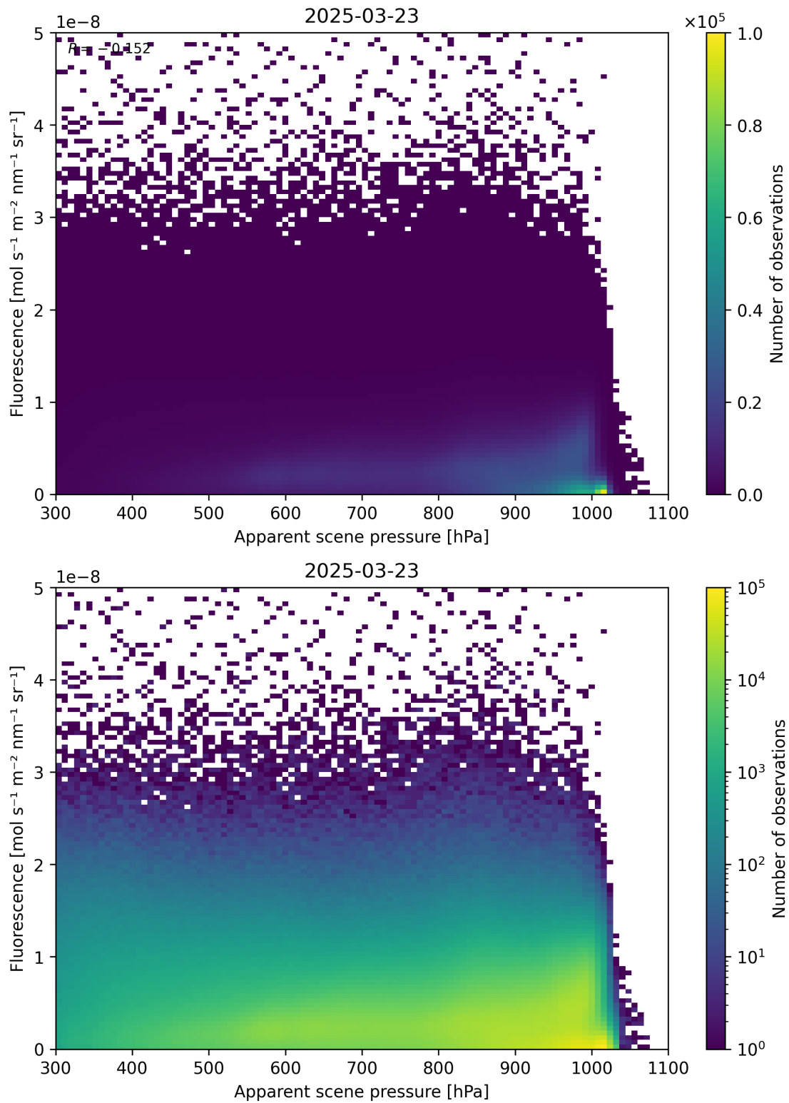
Figure 64: Scatter density plot of “Apparent scene pressure” against “Fluorescence” for 2025-03-23 to 2025-03-24.
