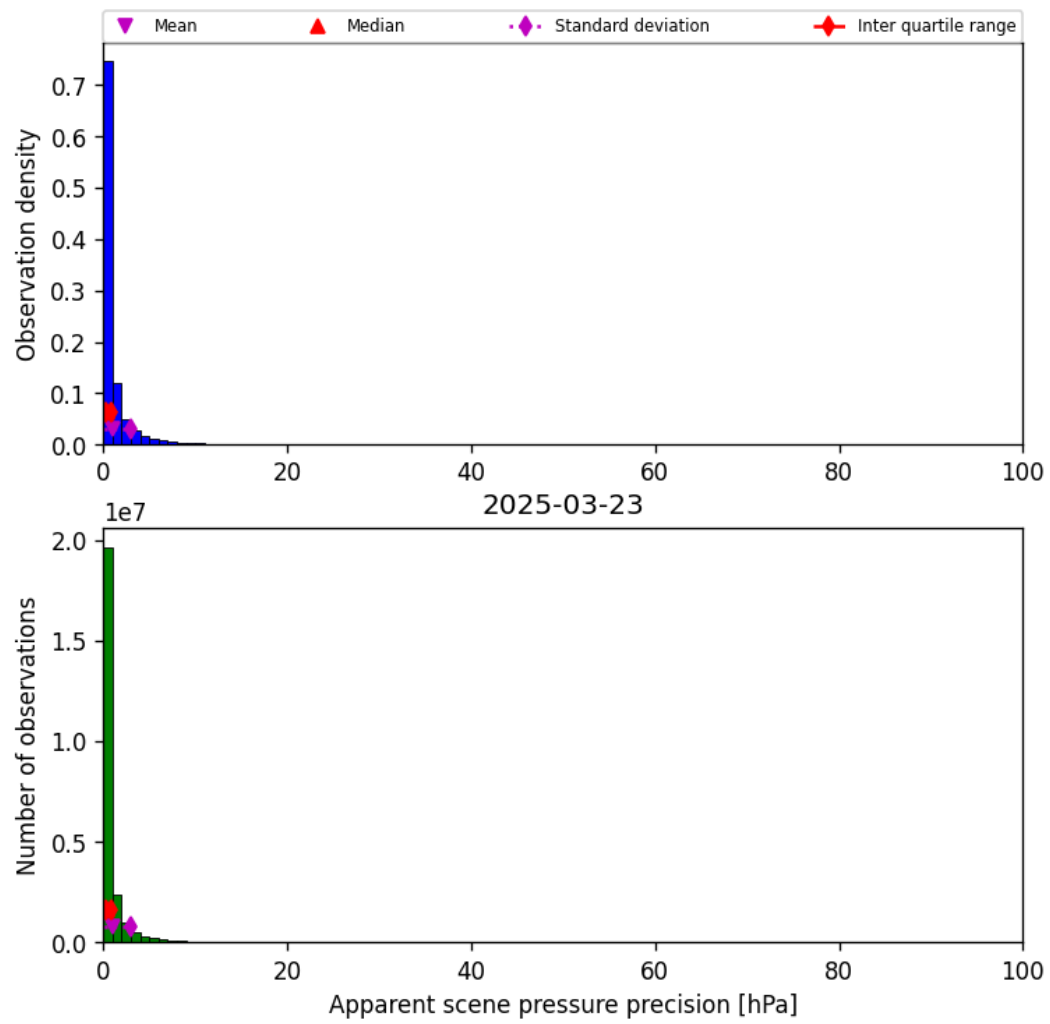
Figure 37: Histogram of “Apparent scene pressure precision” for 2025-03-23 to 2025-03-24
