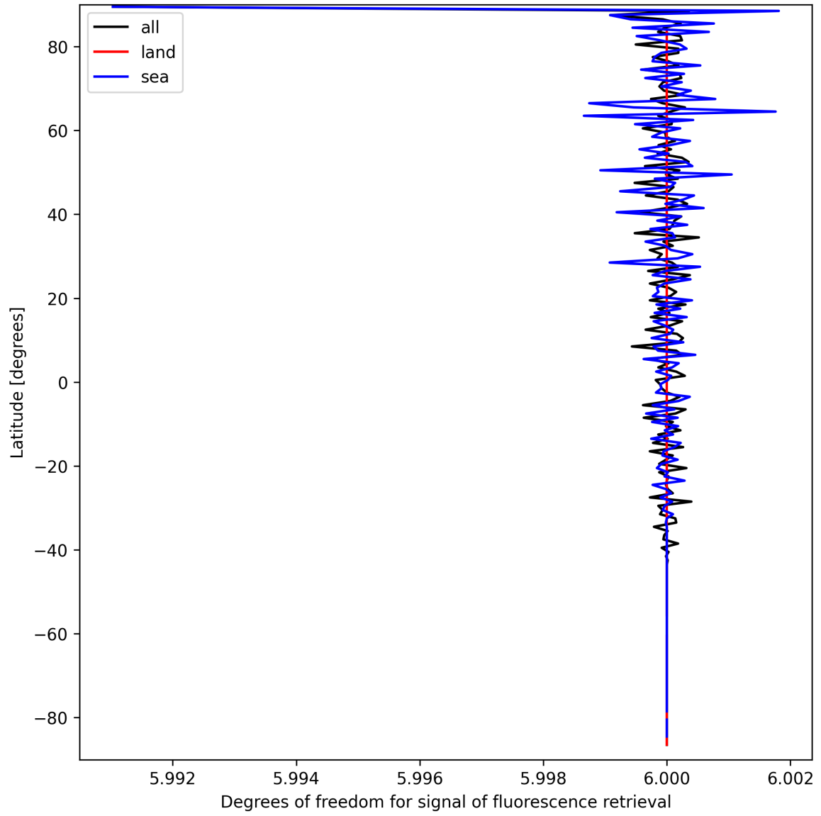
Figure 26: Zonal average of “Degrees of freedom for signal of fluorescence retrieval” for 2025-03-23 to 2025-03-24.
