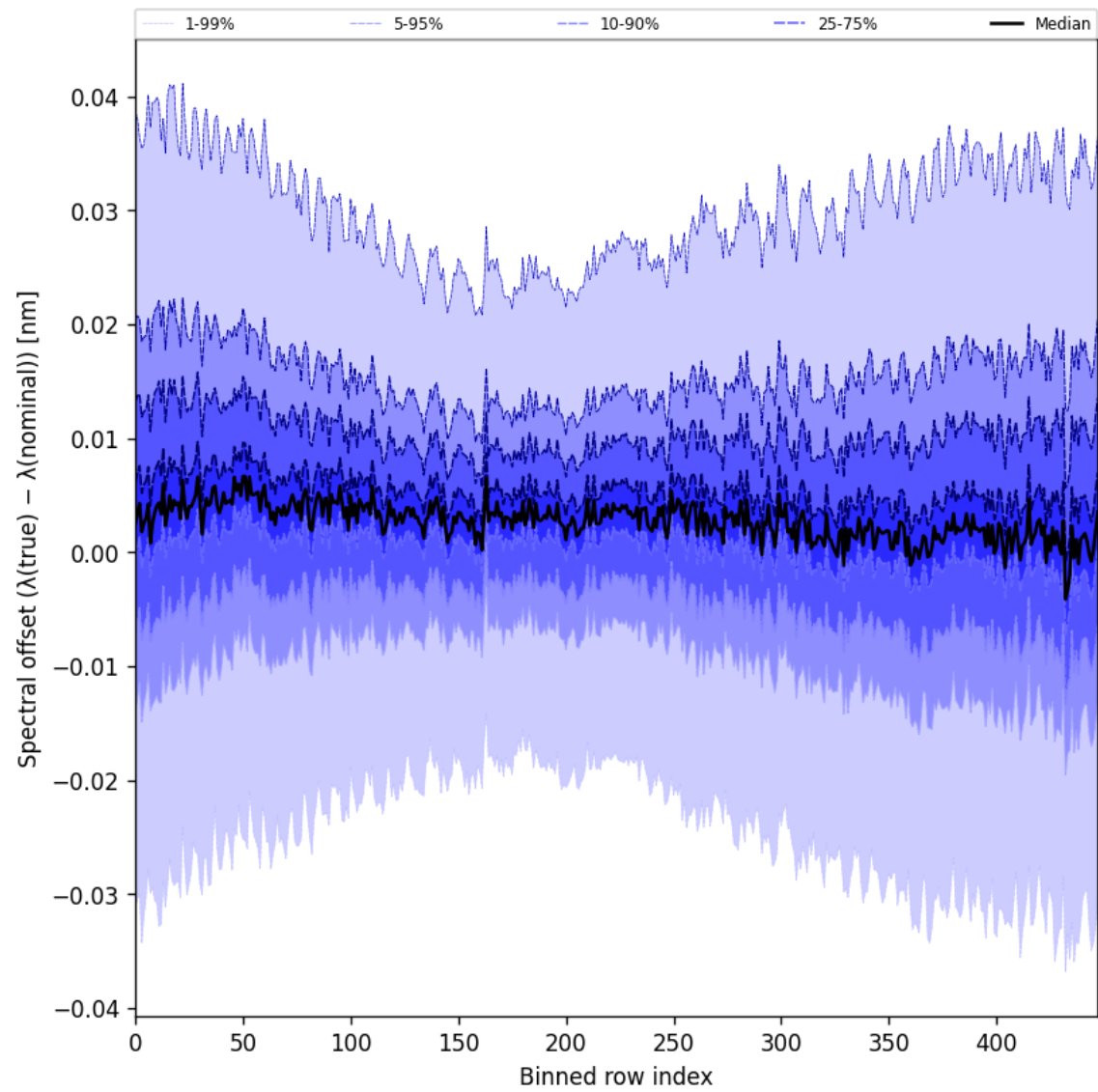
Figure 62: Along track statistics of “Spectral offset ( \lambda_{\text{true}} - \lambda_{\text{nominal}} )” for 2025-03-23 to 2025-03-24
