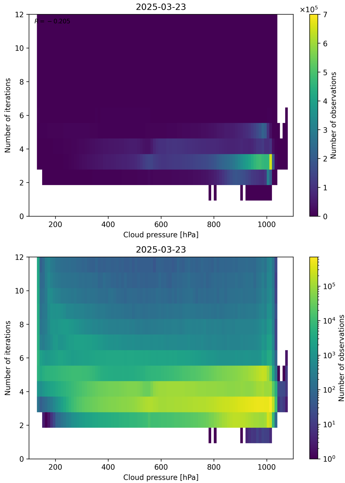
Figure 81: Scatter density plot of “Cloud pressure” against “Number of iterations” for 2025-03-23 to 2025-03-24.
