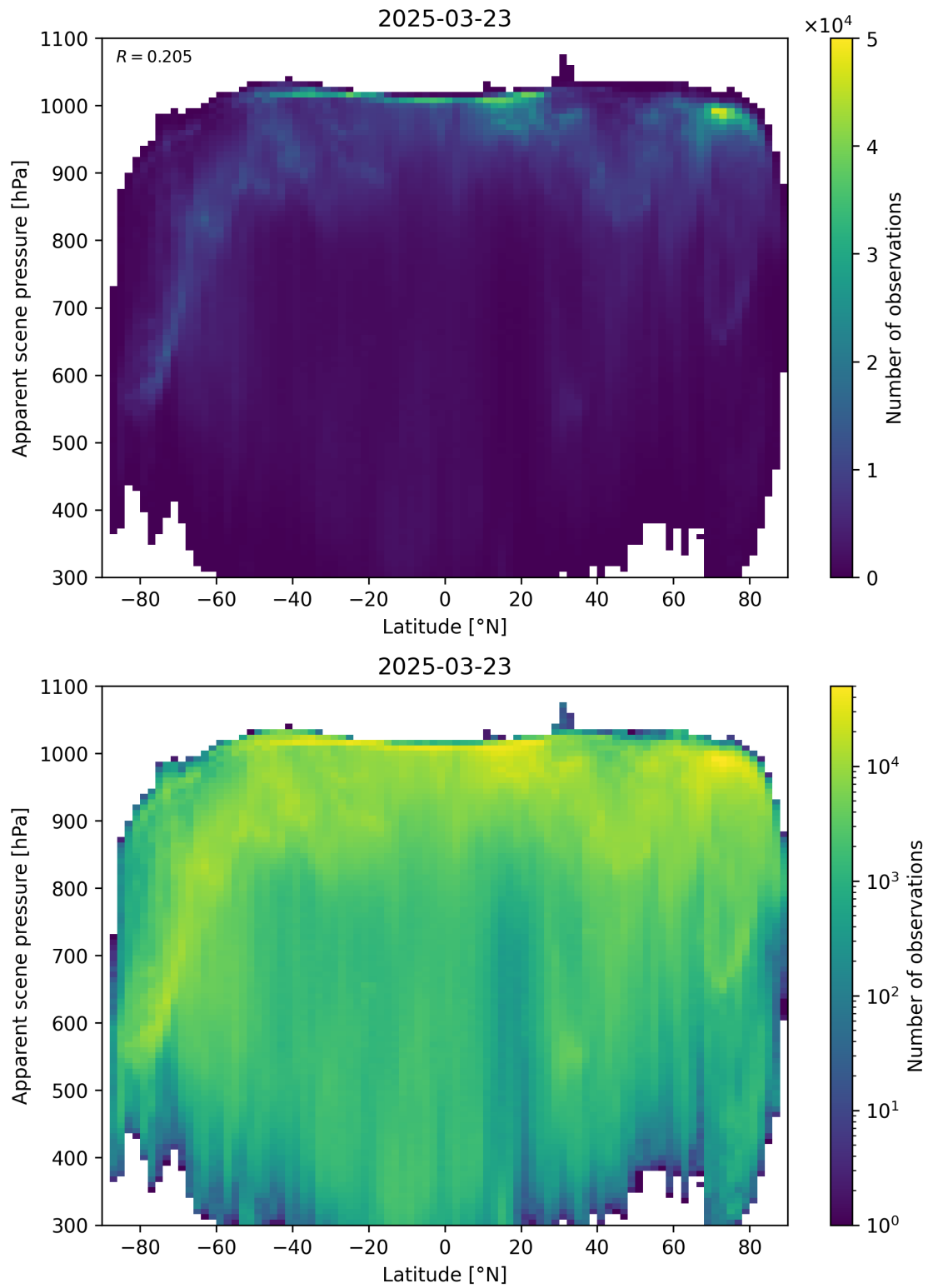
Figure 88: Scatter density plot of “Latitude” against “Apparent scene pressure” for 2025-03-23 to 2025-03-24.
