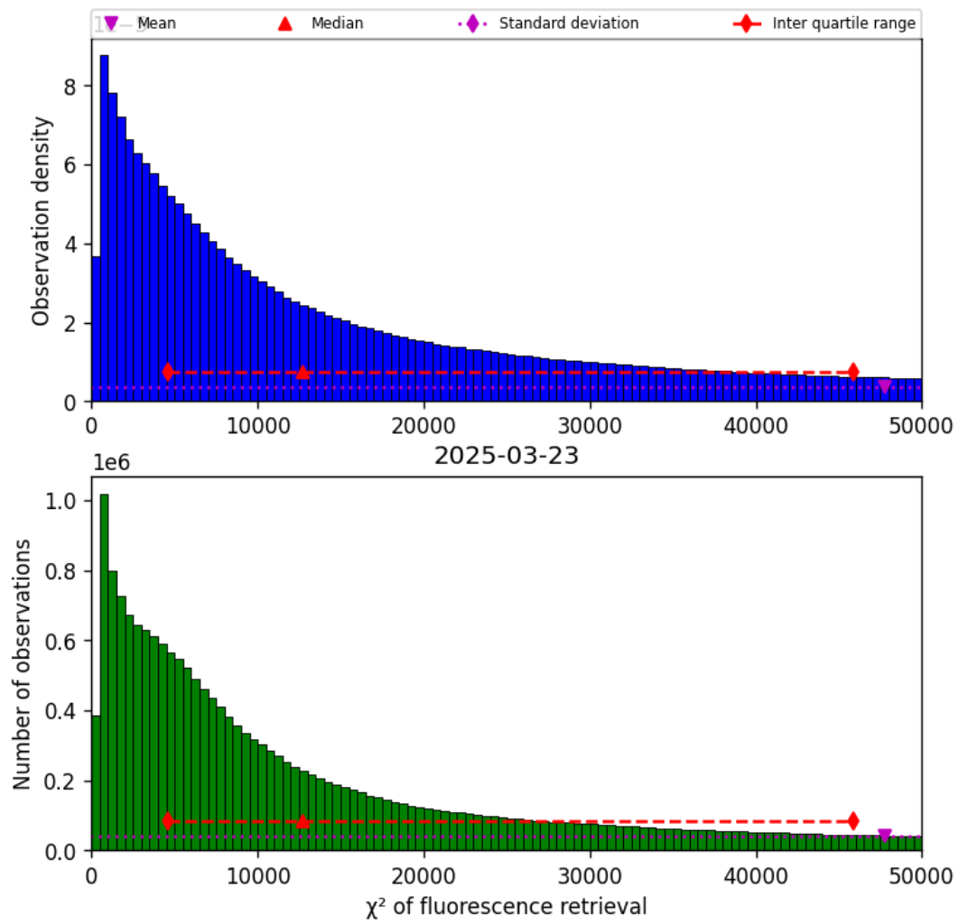
Figure 42: Histogram of “ \chi^2 of fluorescence retrieval” for 2025-03-23 to 2025-03-24
