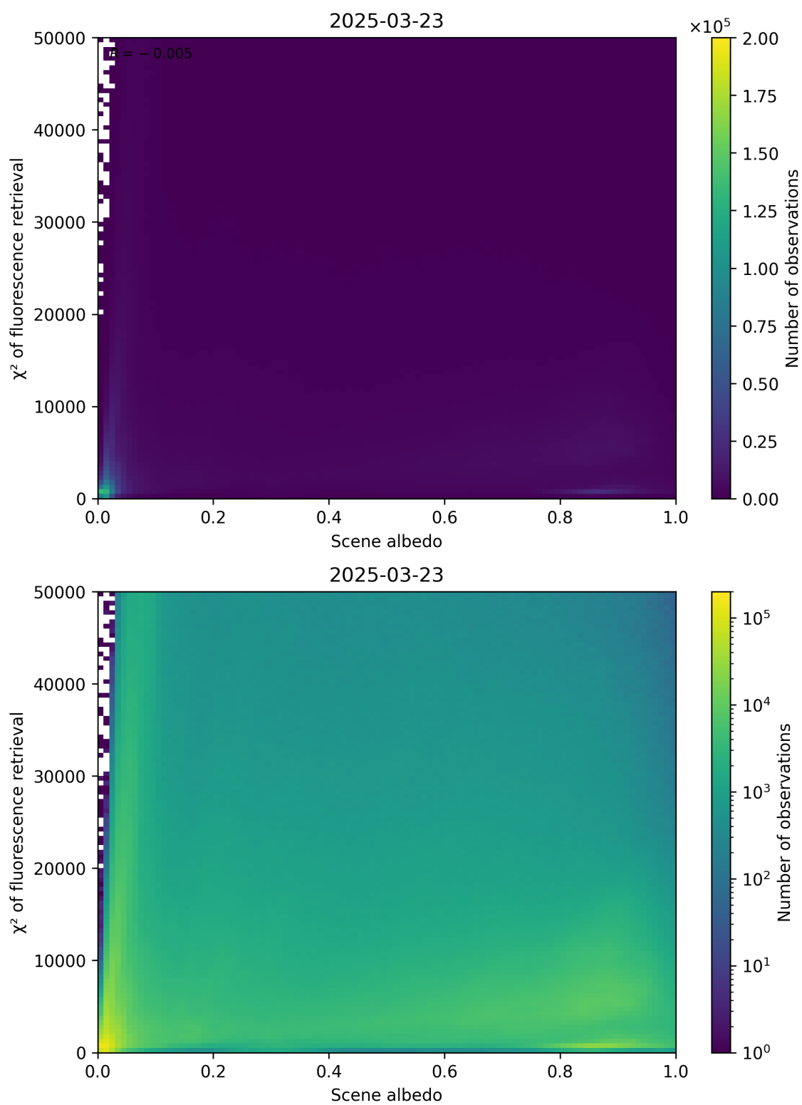
Figure 103: Scatter density plot of “Scene albedo” against “ \chi^2 of fluorescence retrieval” for 2025-03-23 to 2025-03-24.
