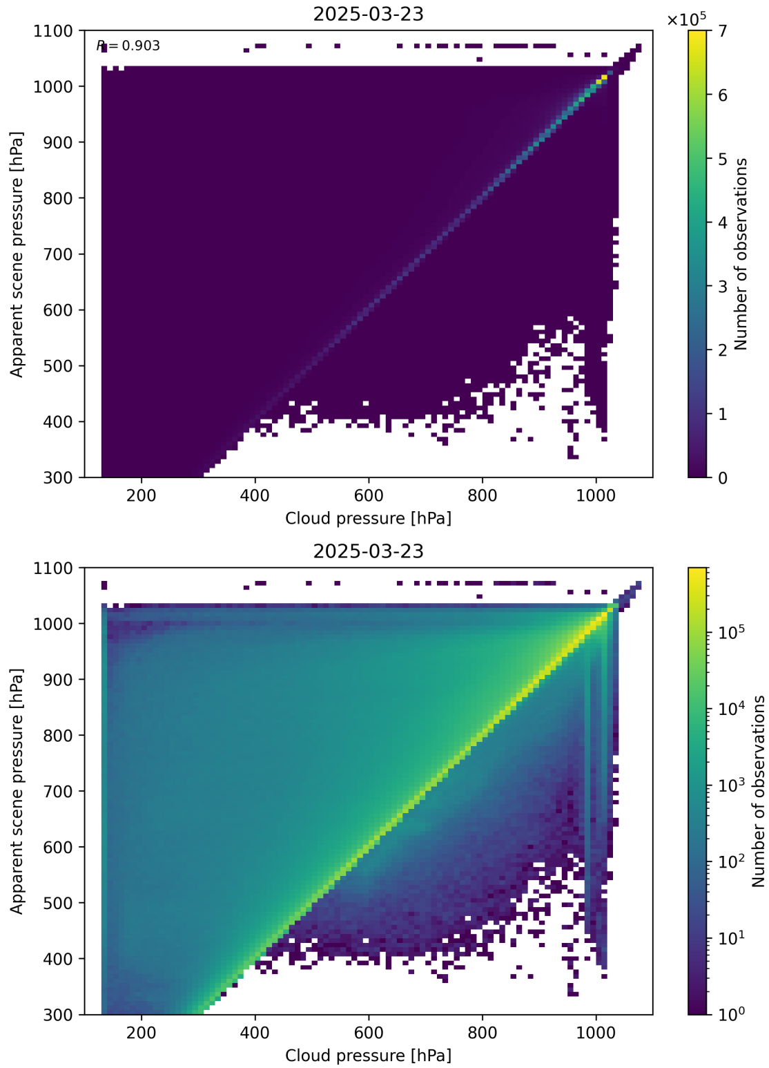
Figure 77: Scatter density plot of “Cloud pressure” against “Apparent scene pressure” for 2025-03-23 to 2025-03-24.
