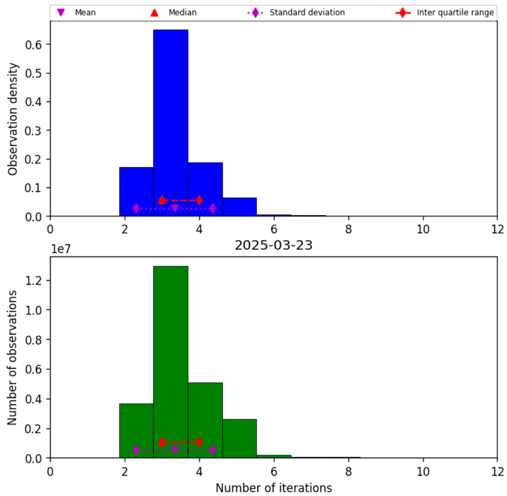
Figure 39: Histogram of “Number of iterations” for 2025-03-23 to 2025-03-24
