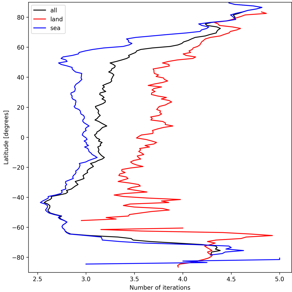
Figure 22: Zonal average of “Number of iterations” for 2025-03-23 to 2025-03-24.
