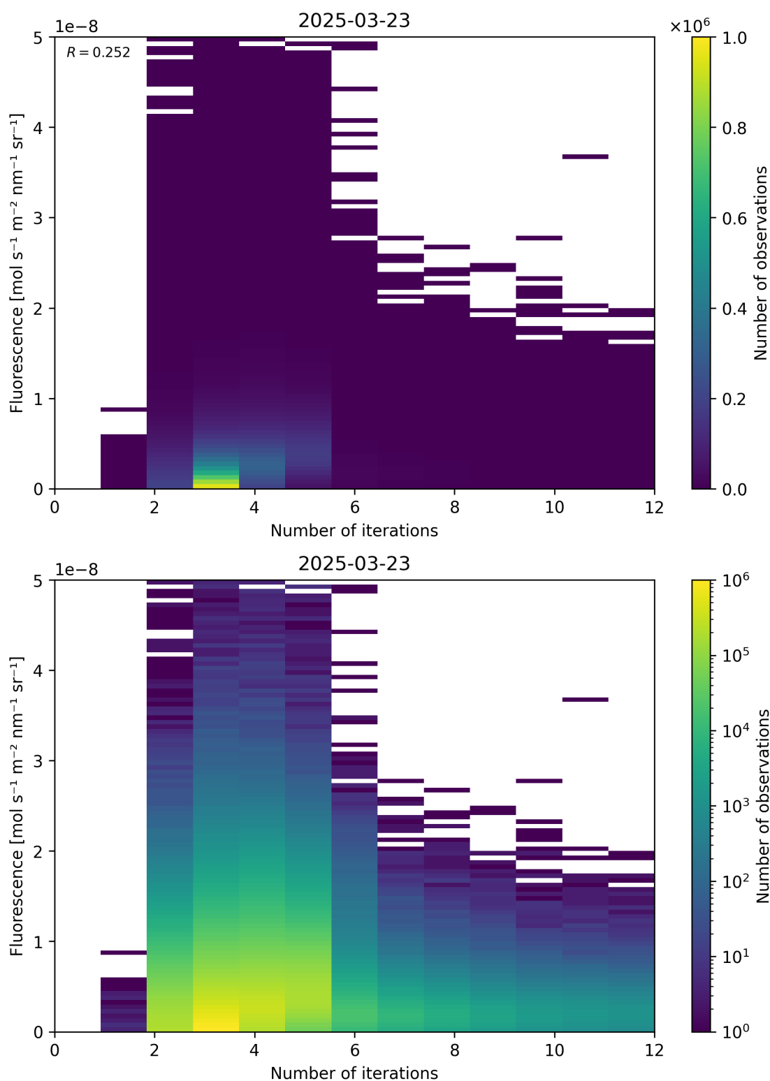
Figure 98: Scatter density plot of “Number of iterations” against “Fluorescence” for 2025-03-23 to 2025-03-24.
