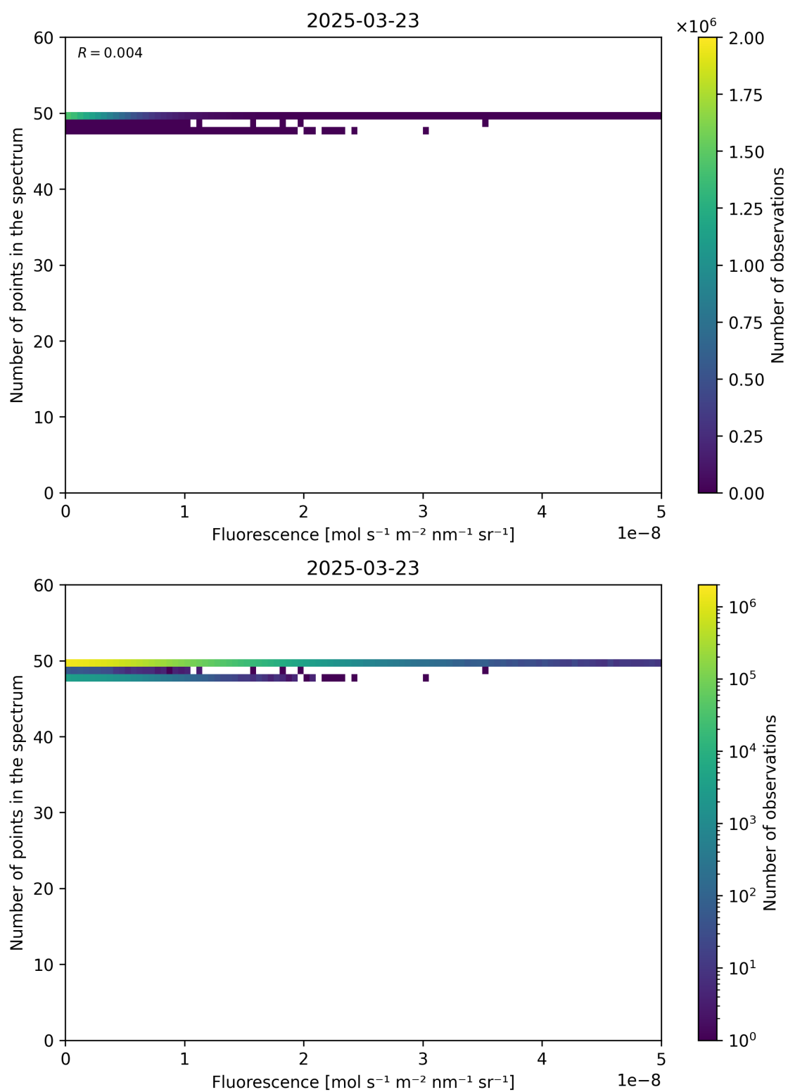
Figure 86: Scatter density plot of “Fluorescence” against “Number of points in the spectrum” for 2025-03-23 to 2025-03-24.
