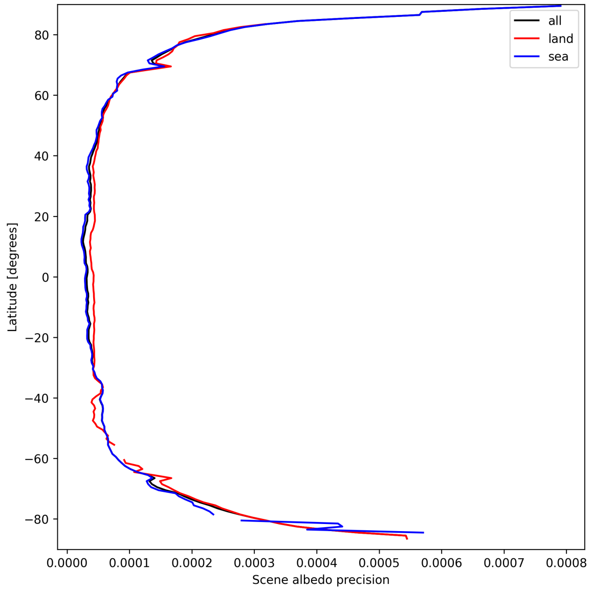
Figure 18: Zonal average of “Scene albedo precision” for 2025-03-23 to 2025-03-24.
