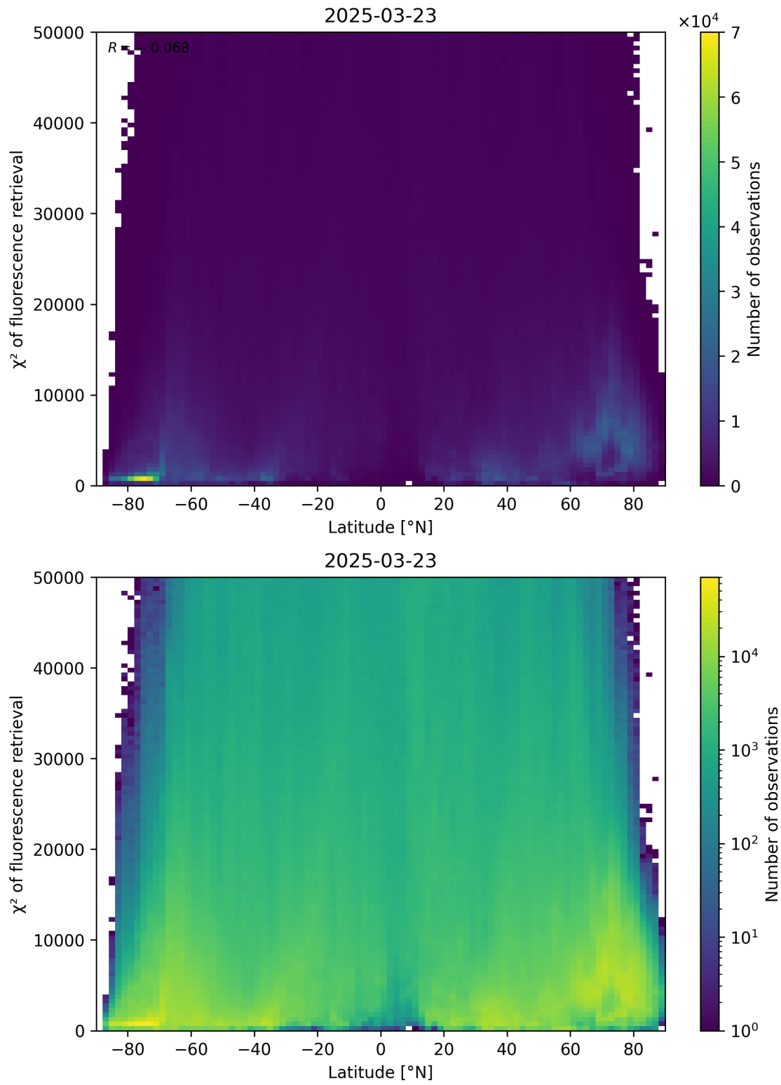
Figure 89: Scatter density plot of “Latitude” against “ \chi^2 of fluorescence retrieval” for 2025-03-23 to 2025-03-24.
