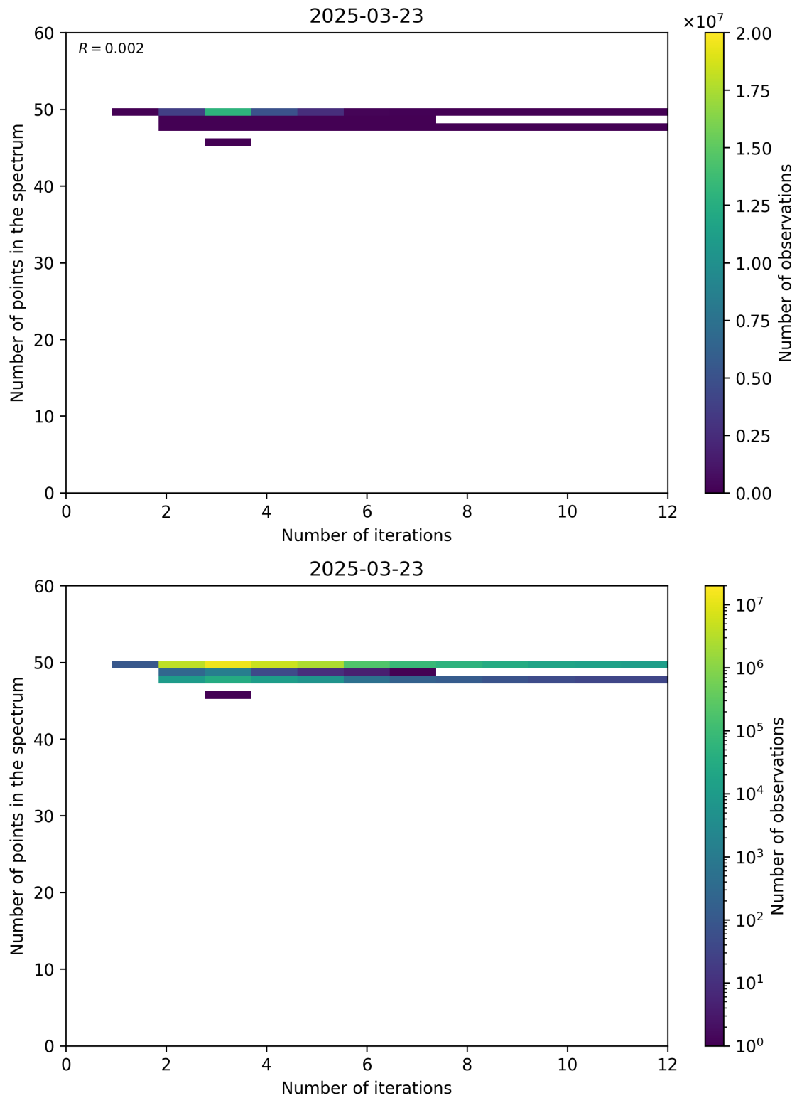
Figure 99: Scatter density plot of “Number of iterations” against “Number of points in the spectrum” for 2025-03-23 to 2025-03-24.
