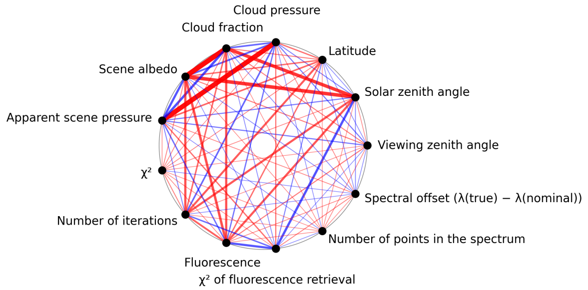
Figure 1: Map of correlation graph for 2025-03-23 to 2025-03-24.
