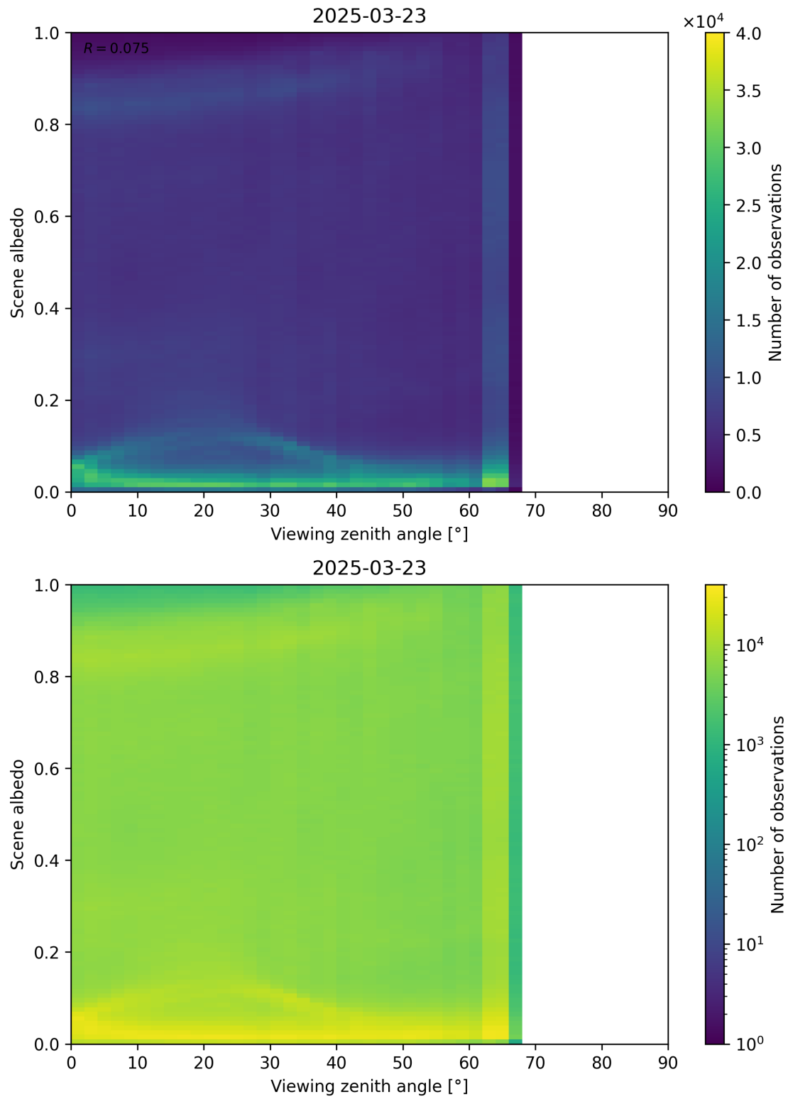
Figure 126: Scatter density plot of “Viewing zenith angle” against “Scene albedo” for 2025-03-23 to 2025-03-24.
