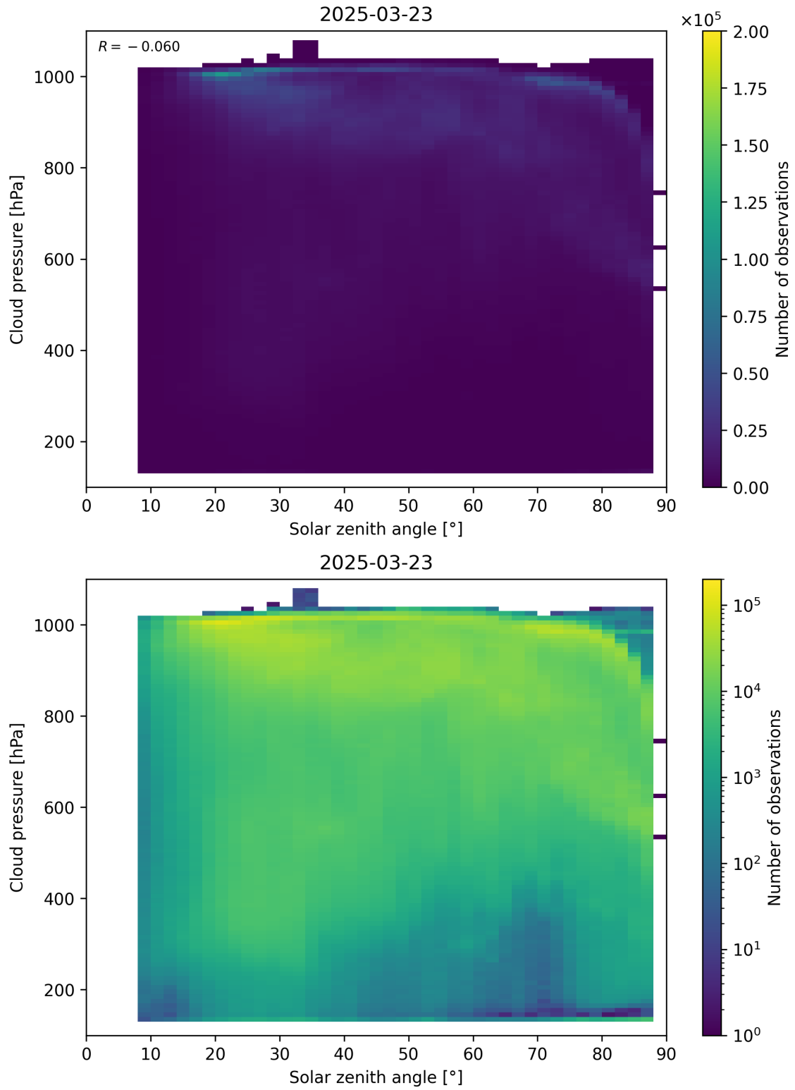
Figure 111: Scatter density plot of “Solar zenith angle” against “Cloud pressure” for 2025-03-23 to 2025-03-24.
