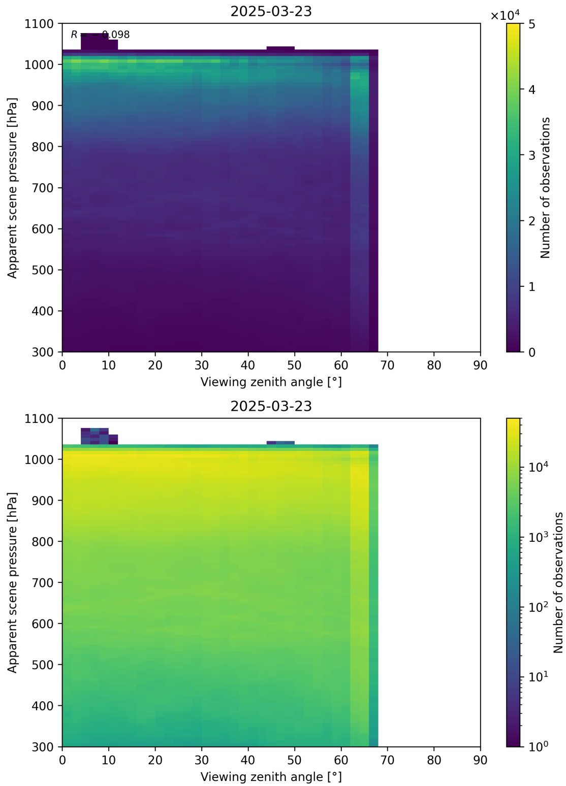
Figure 118: Scatter density plot of “Viewing zenith angle” against “Apparent scene pressure” for 2025-03-23 to 2025-03-24.
