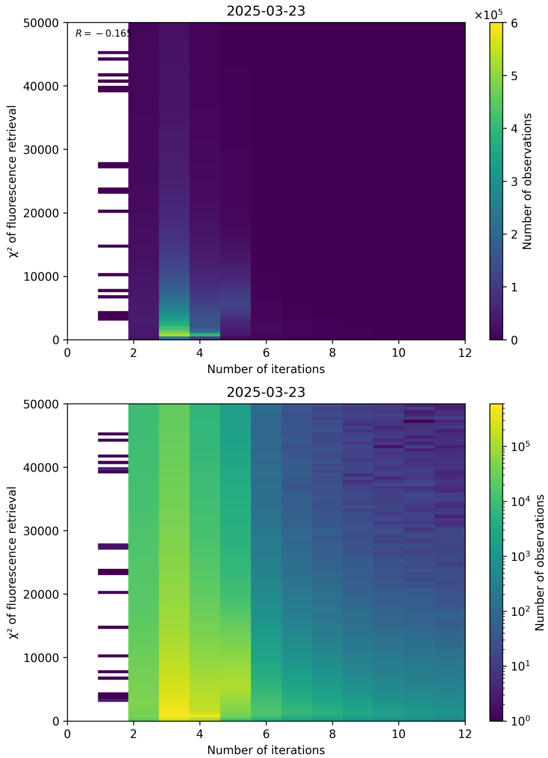
Figure 97: Scatter density plot of “Number of iterations” against “ \chi^2 of fluorescence retrieval” for 2025-03-23 to 2025-03-24.
