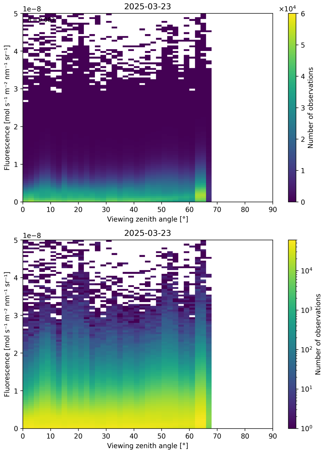
Figure 122: Scatter density plot of “Viewing zenith angle” against “Fluorescence” for 2025-03-23 to 2025-03-24.
