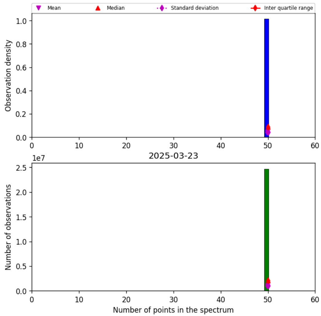
Figure 44: Histogram of “Number of points in the spectrum” for 2025-03-23 to 2025-03-24
