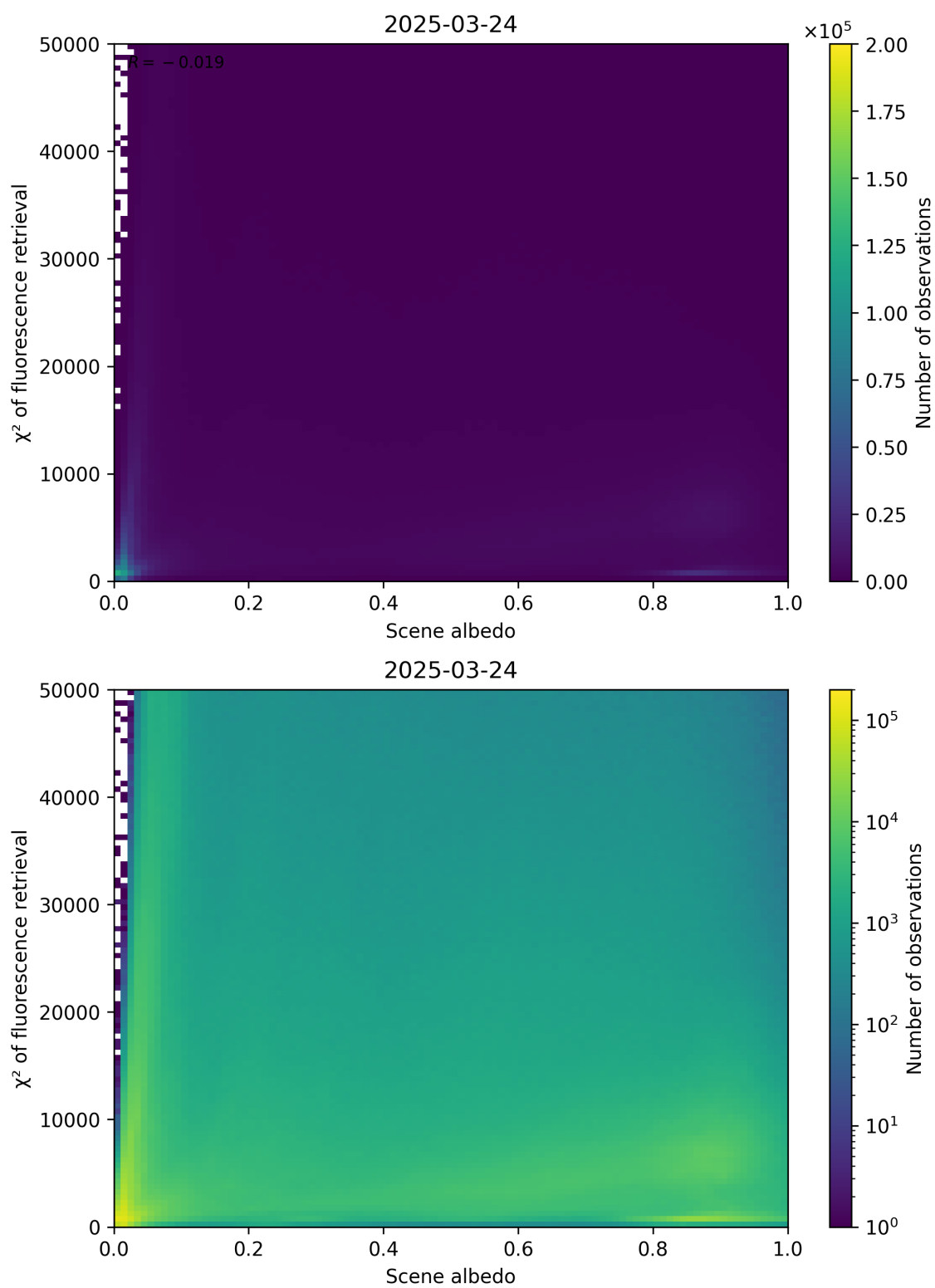
Figure 103: Scatter density plot of “Scene albedo” against “ \chi^2 of fluorescence retrieval” for 2025-03-23 to 2025-03-25.
