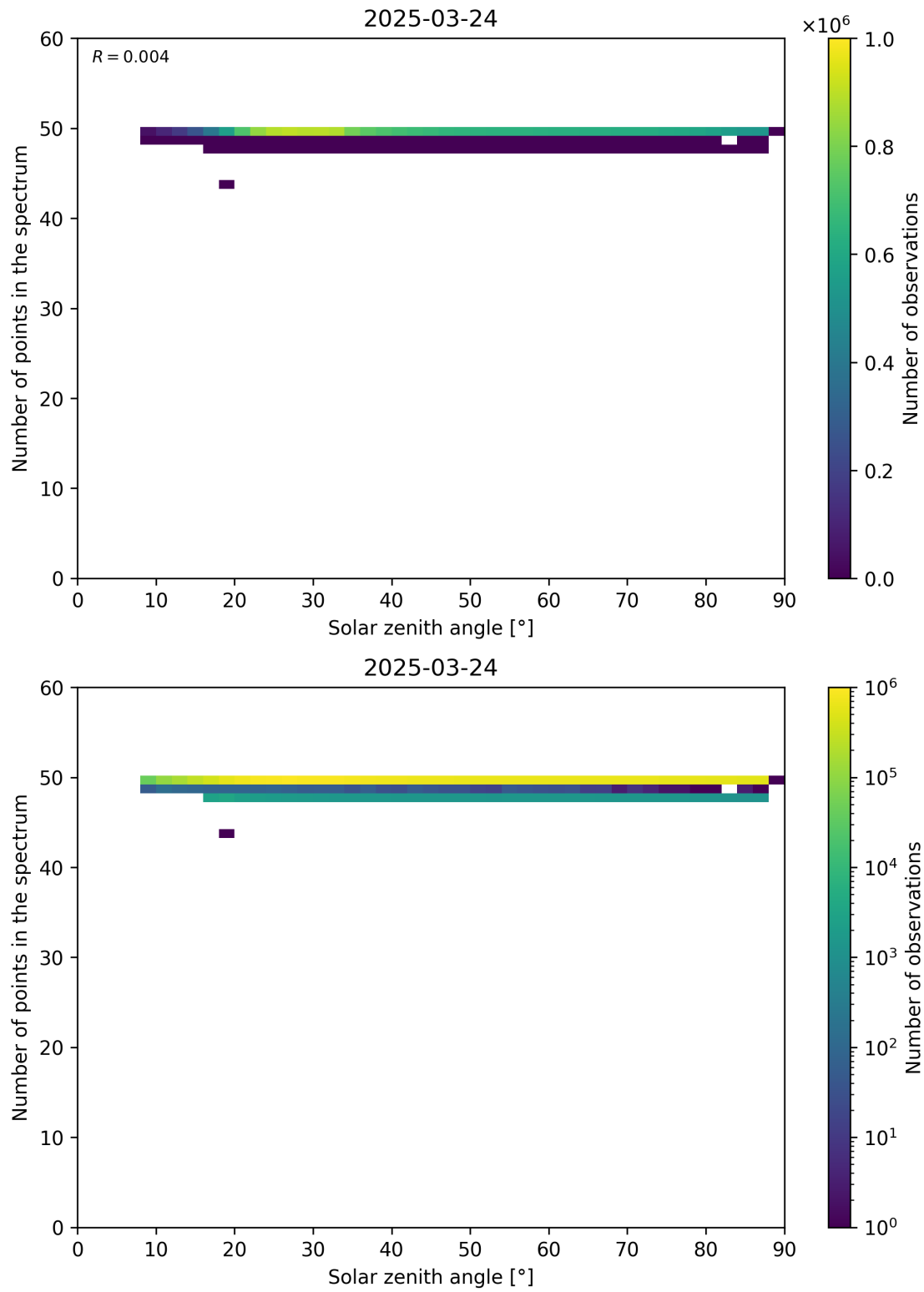
Figure 115: Scatter density plot of “Solar zenith angle” against “Number of points in the spectrum” for 2025-03-23 to 2025-03-25.
