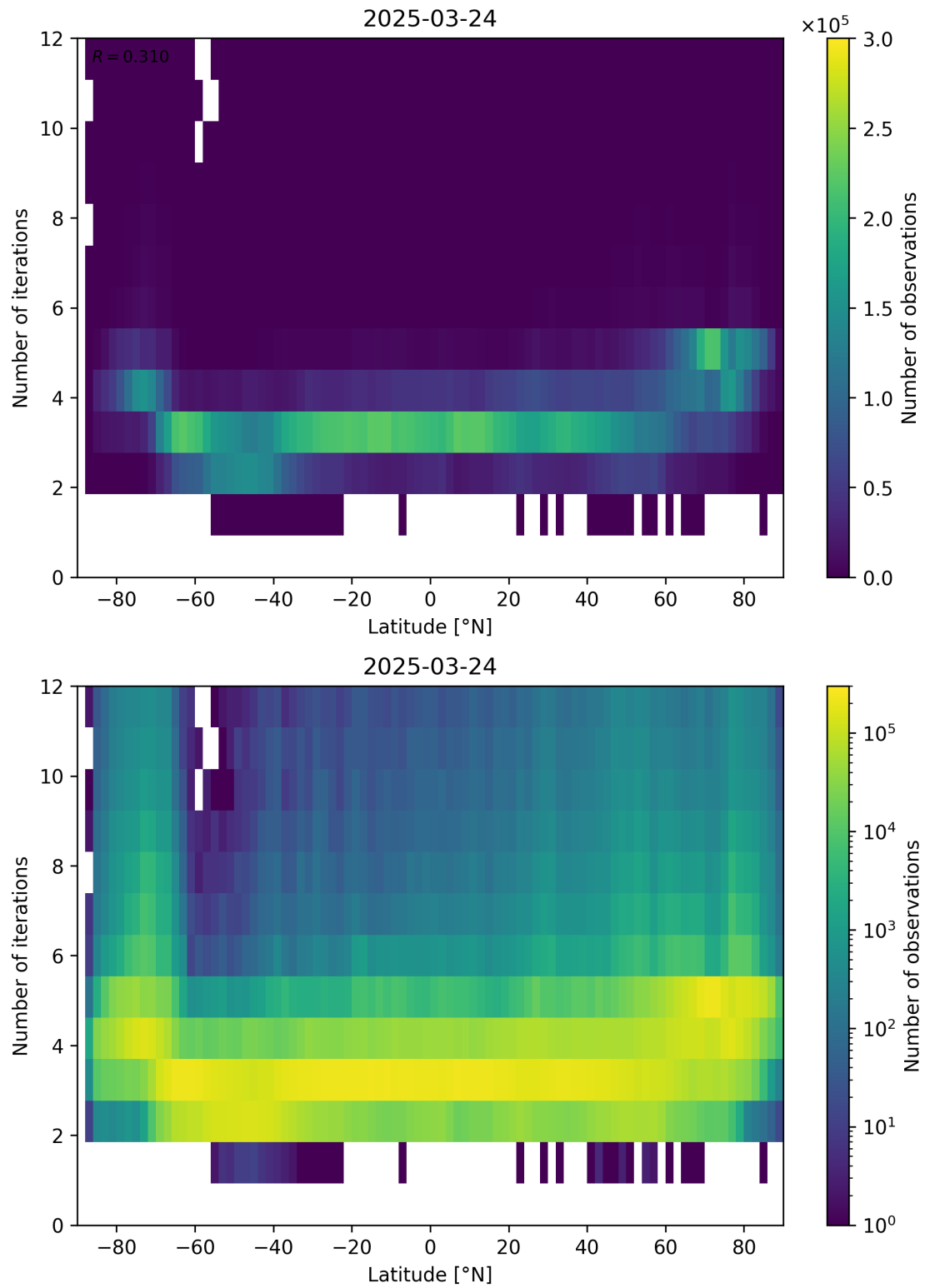
Figure 93: Scatter density plot of “Latitude” against “Number of iterations” for 2025-03-23 to 2025-03-25.
