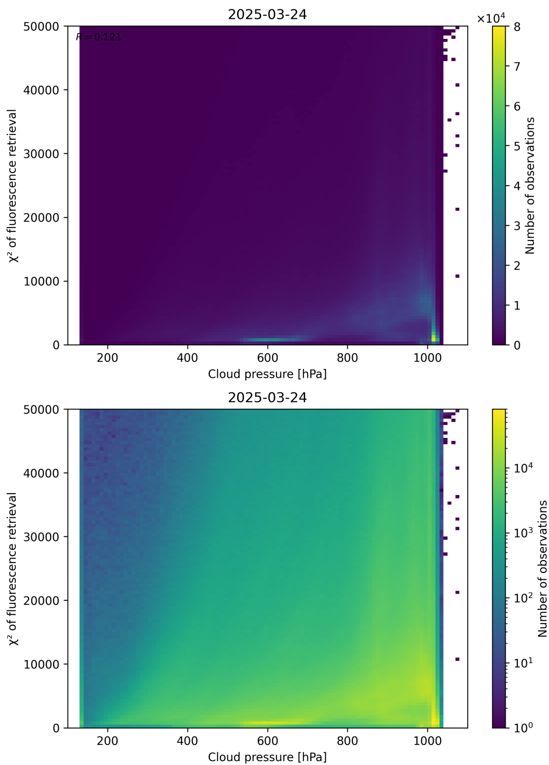
Figure 78: Scatter density plot of “Cloud pressure” against “ \chi^2 of fluorescence retrieval” for 2025-03-23 to 2025-03-25.
