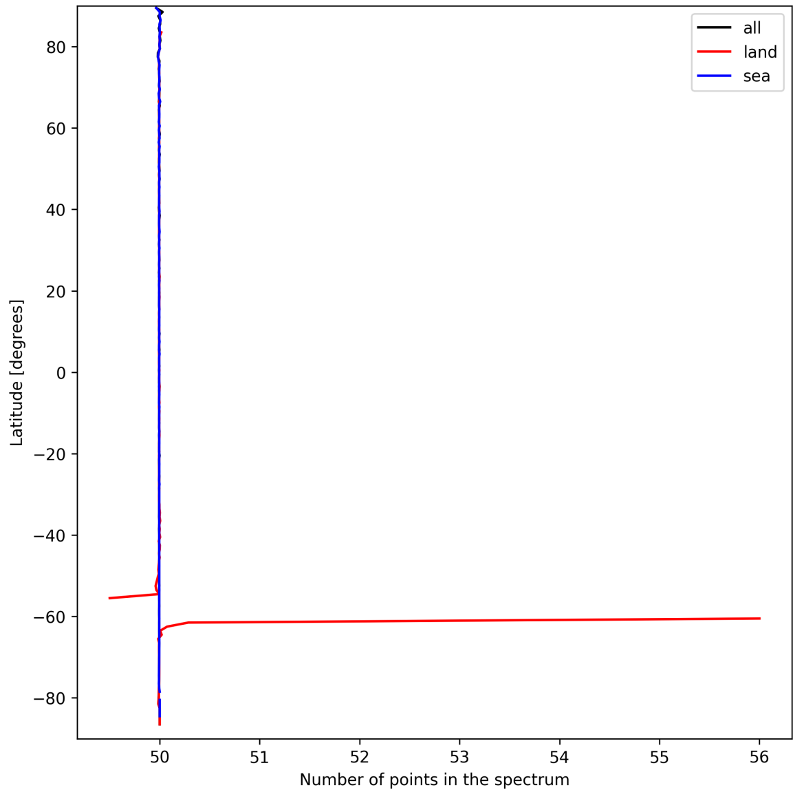
Figure 27: Zonal average of “Number of points in the spectrum” for 2025-03-23 to 2025-03-25.
