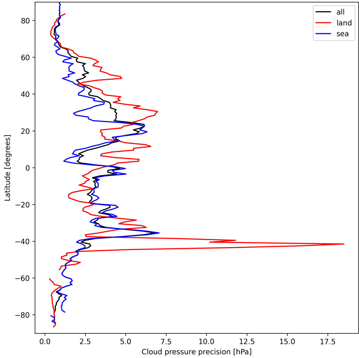
Figure 14: Zonal average of “Cloud pressure precision” for 2025-03-23 to 2025-03-25.
