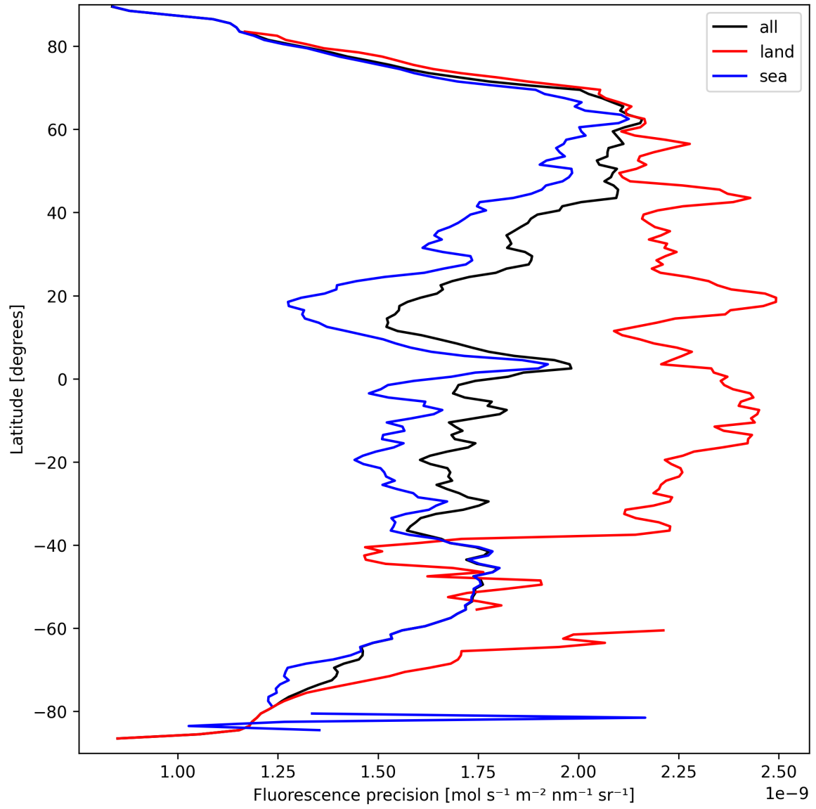
Figure 24: Zonal average of “Fluorescence precision” for 2025-03-23 to 2025-03-25.
