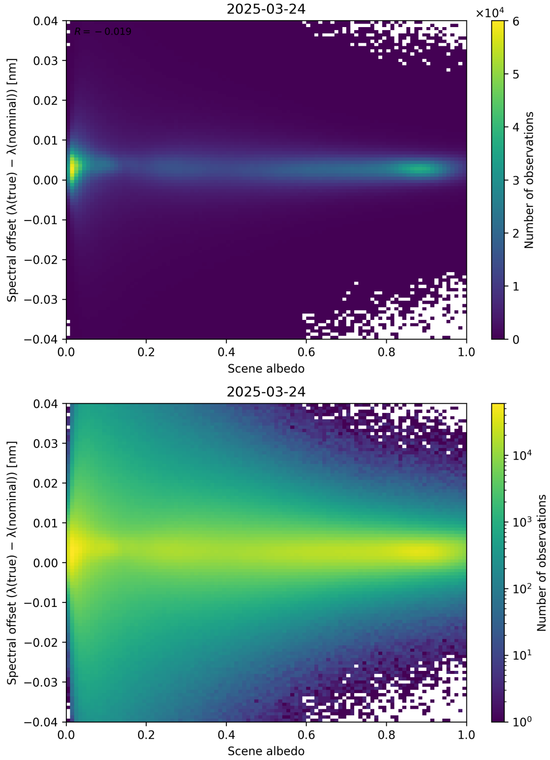
Figure 107: Scatter density plot of “Scene albedo” against “Spectral offset ( \lambda_{\text{true}} - \lambda_{\text{nominal}} )” for 2025-03-23 to 2025-03-25.
