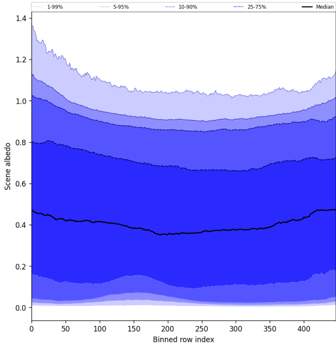
Figure 51: Along track statistics of “Scene albedo” for 2025-03-23 to 2025-03-25
