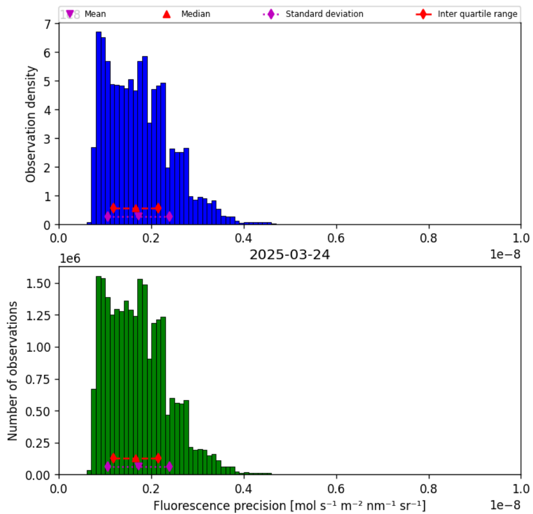
Figure 41: Histogram of “Fluorescence precision” for 2025-03-23 to 2025-03-25
