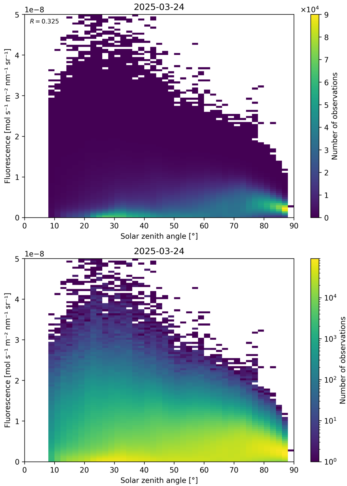
Figure 112: Scatter density plot of “Solar zenith angle” against “Fluorescence” for 2025-03-23 to 2025-03-25.
