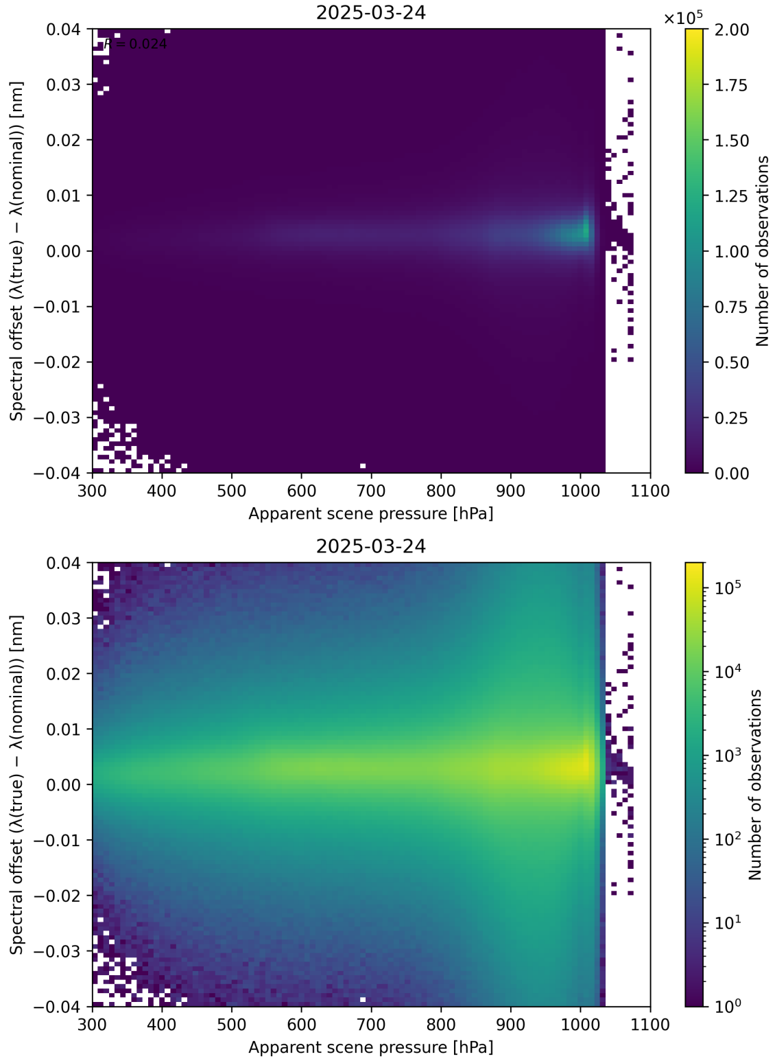
Figure 67: Scatter density plot of “Apparent scene pressure” against “Spectral offset ( \lambda_{\text{true}} - \lambda_{\text{nominal}} )” for 2025-03-23 to 2025-03-25.
