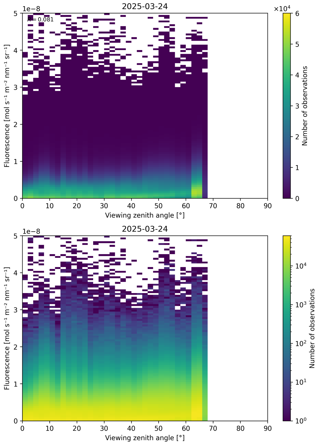
Figure 122: Scatter density plot of “Viewing zenith angle” against “Fluorescence” for 2025-03-23 to 2025-03-25.
