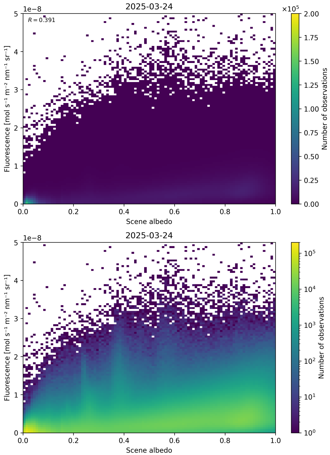
Figure 104: Scatter density plot of "Scene albedo" against "Fluorescence" for 2025-03-23 to 2025-03-25.
