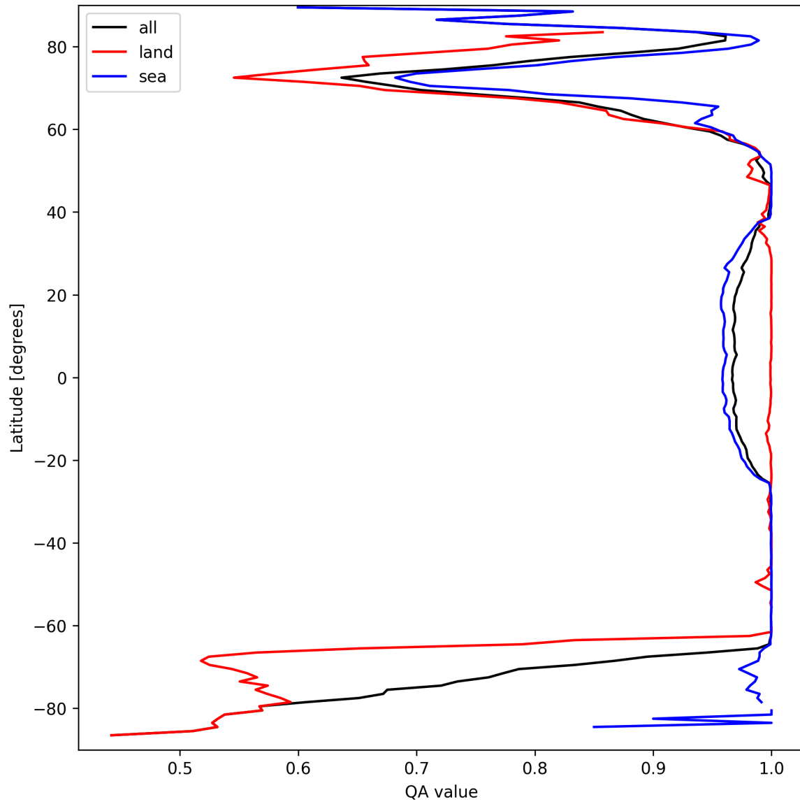
Figure 12: Zonal average of “QA value” for 2025-03-23 to 2025-03-25.
