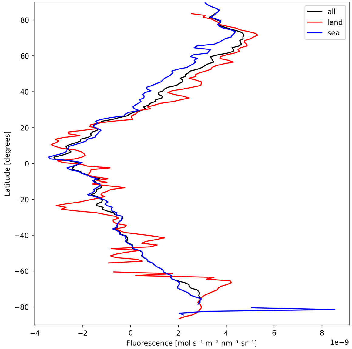
Figure 23: Zonal average of “Fluorescence” for 2025-03-23 to 2025-03-25.
