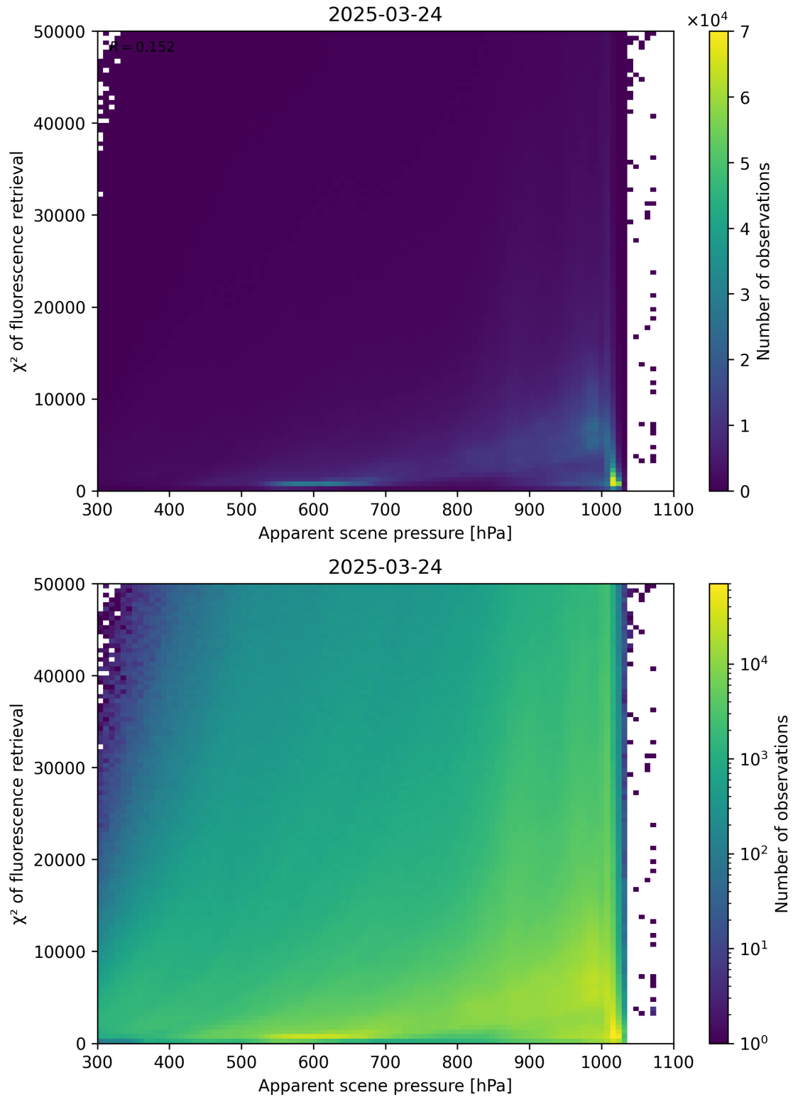
Figure 63: Scatter density plot of “Apparent scene pressure” against “ \chi^2 of fluorescence retrieval” for 2025-03-23 to 2025-03-25.
