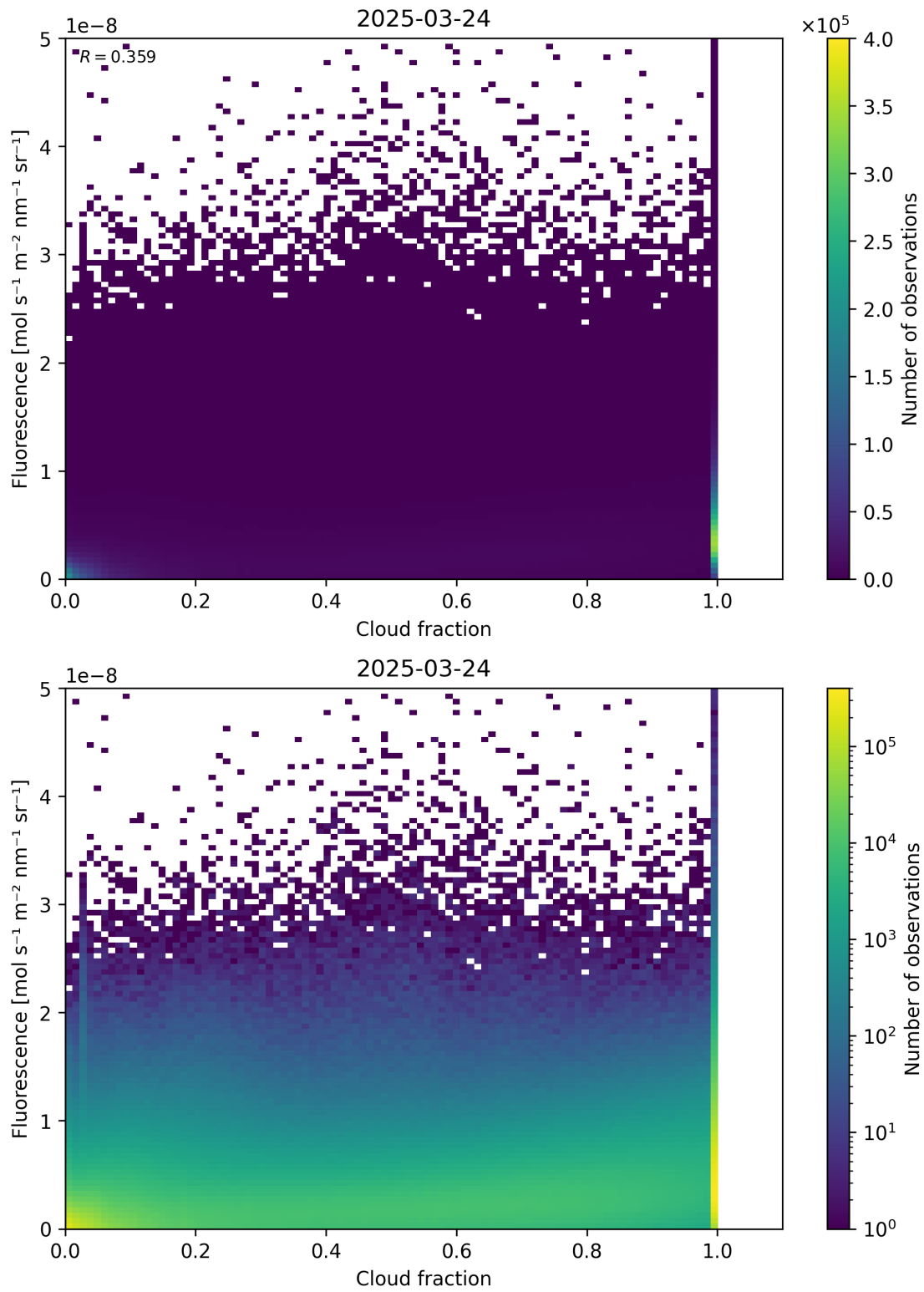
Figure 72: Scatter density plot of “Cloud fraction” against “Fluorescence” for 2025-03-23 to 2025-03-25.
