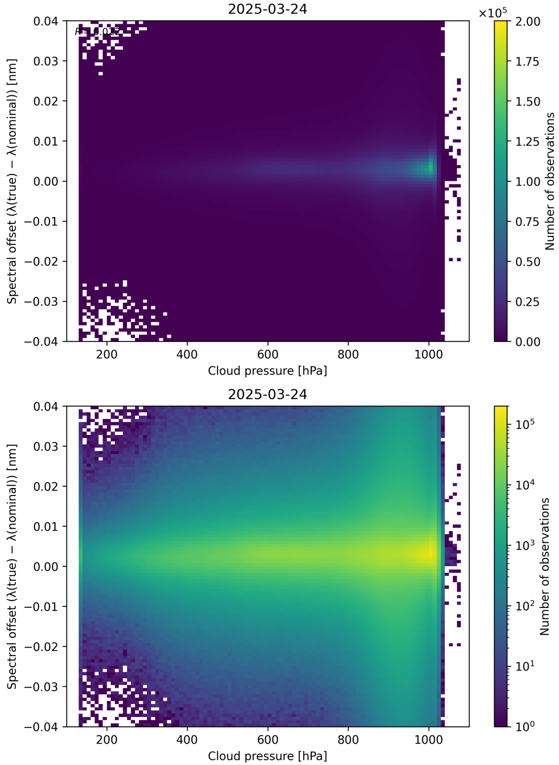
Figure 84: Scatter density plot of “Cloud pressure” against “Spectral offset ( \lambda_{\text{true}} - \lambda_{\text{nominal}} )” for 2025-03-23 to 2025-03-25.
