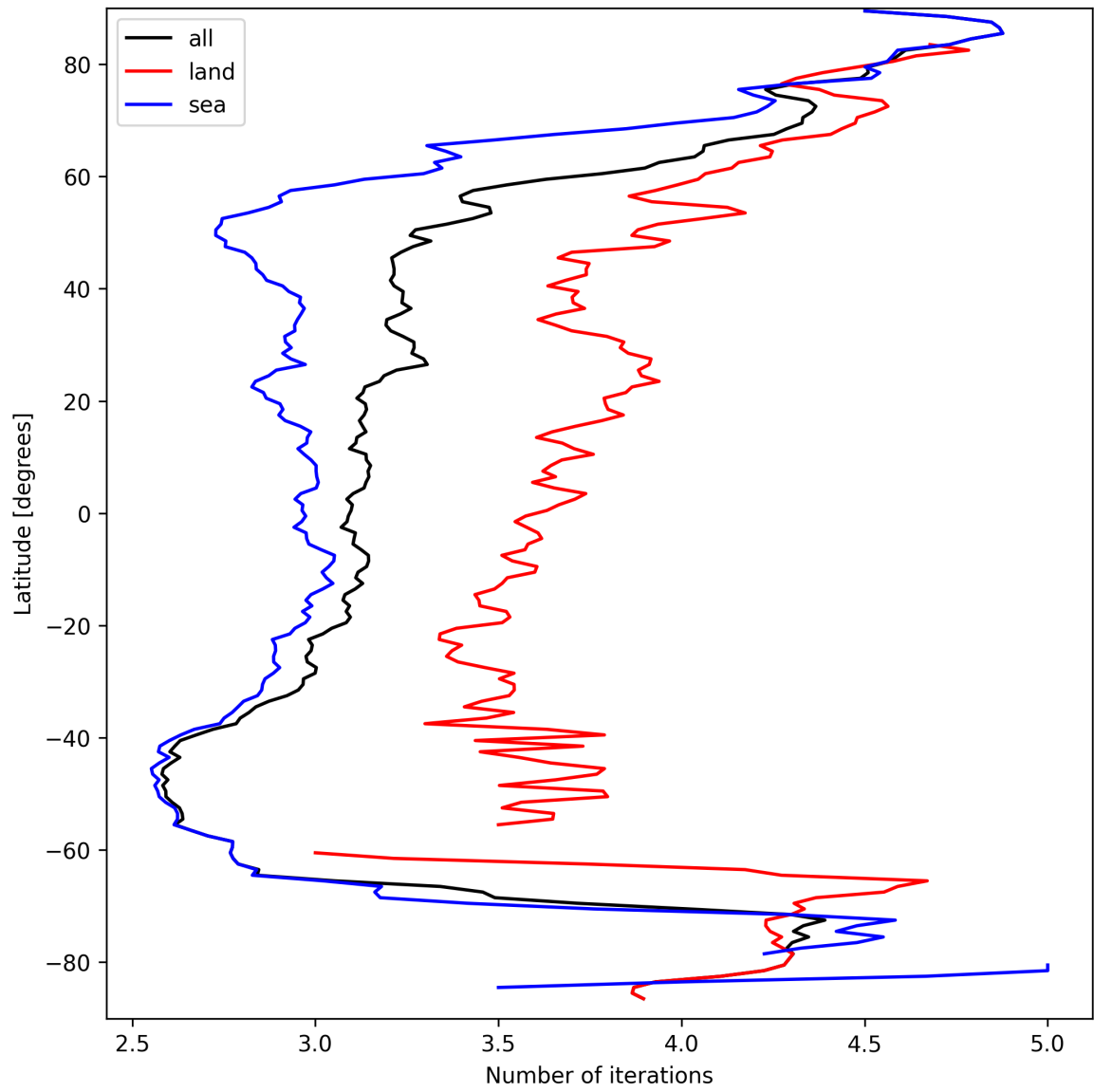
Figure 22: Zonal average of “Number of iterations” for 2025-03-23 to 2025-03-25.
