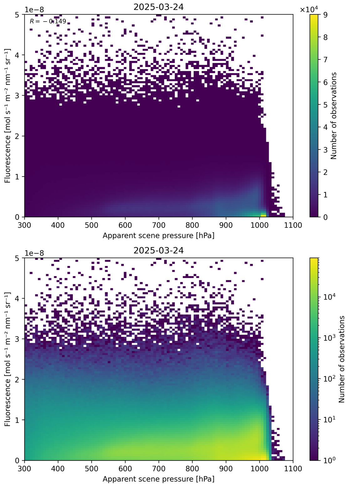
Figure 64: Scatter density plot of “Apparent scene pressure” against “Fluorescence” for 2025-03-23 to 2025-03-25.
