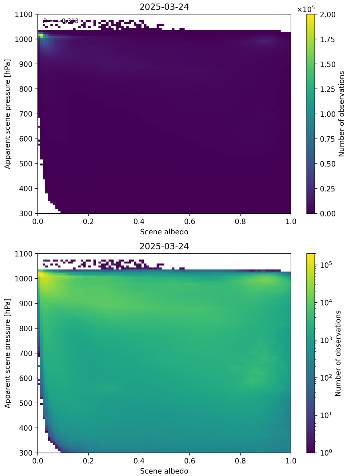
Figure 102: Scatter density plot of “Scene albedo” against “Apparent scene pressure” for 2025-03-23 to 2025-03-25.
