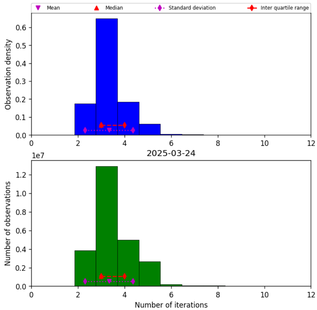
Figure 39: Histogram of “Number of iterations” for 2025-03-23 to 2025-03-25
