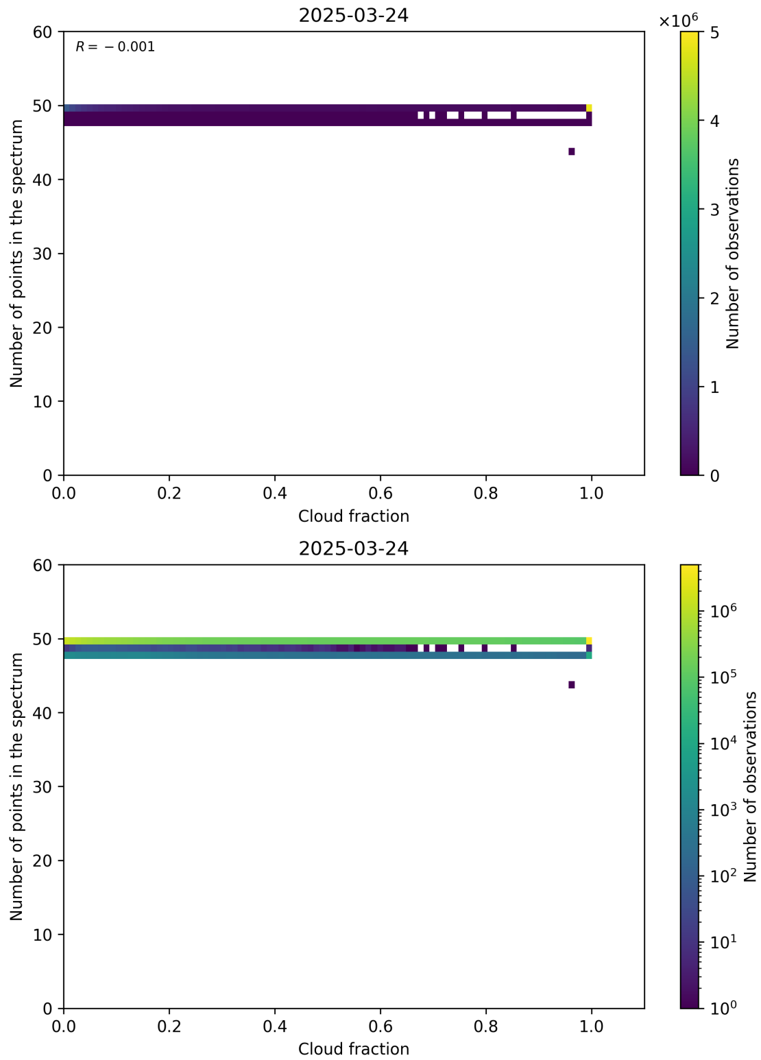
Figure 74: Scatter density plot of “Cloud fraction” against “Number of points in the spectrum” for 2025-03-23 to 2025-03-25.
