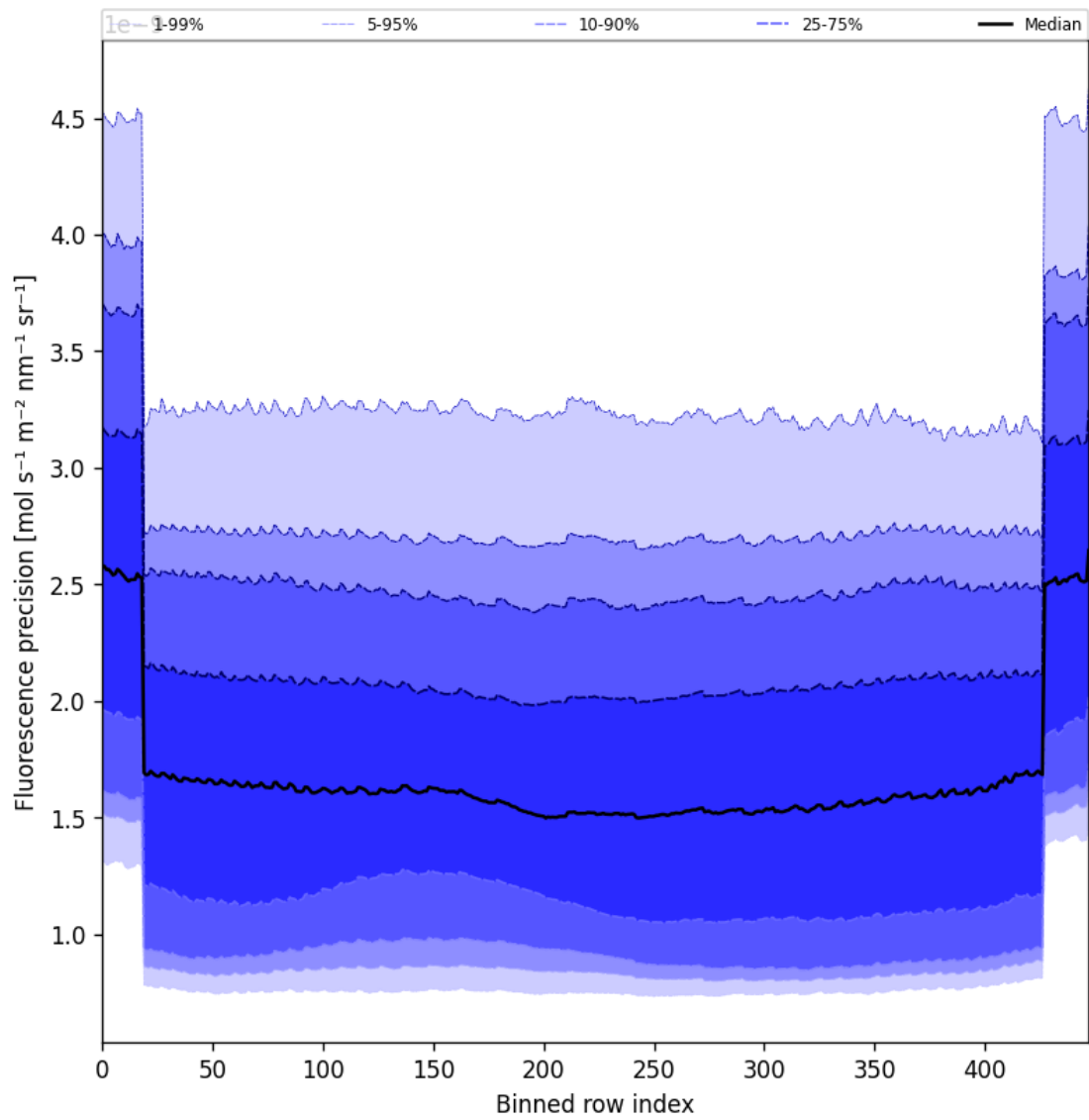
Figure 58: Along track statistics of “Fluorescence precision” for 2025-03-23 to 2025-03-25
