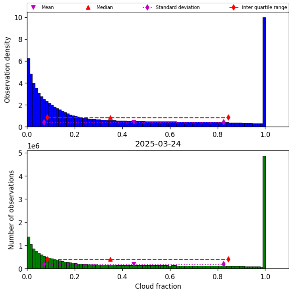
Figure 32: Histogram of “Cloud fraction” for 2025-03-23 to 2025-03-25
