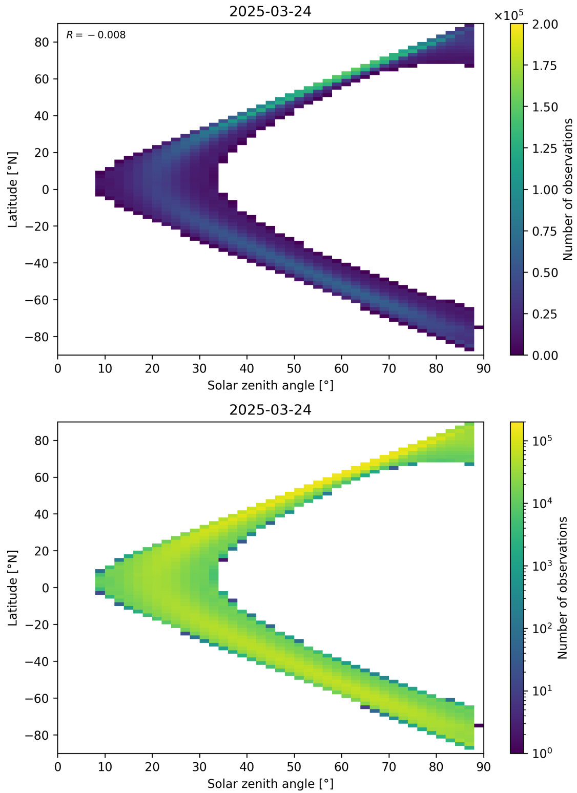
Figure 113: Scatter density plot of “Solar zenith angle” against “Latitude” for 2025-03-23 to 2025-03-25.
