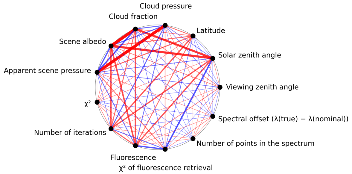
Figure 1: Map of correlation graph for 2025-03-23 to 2025-03-25.
