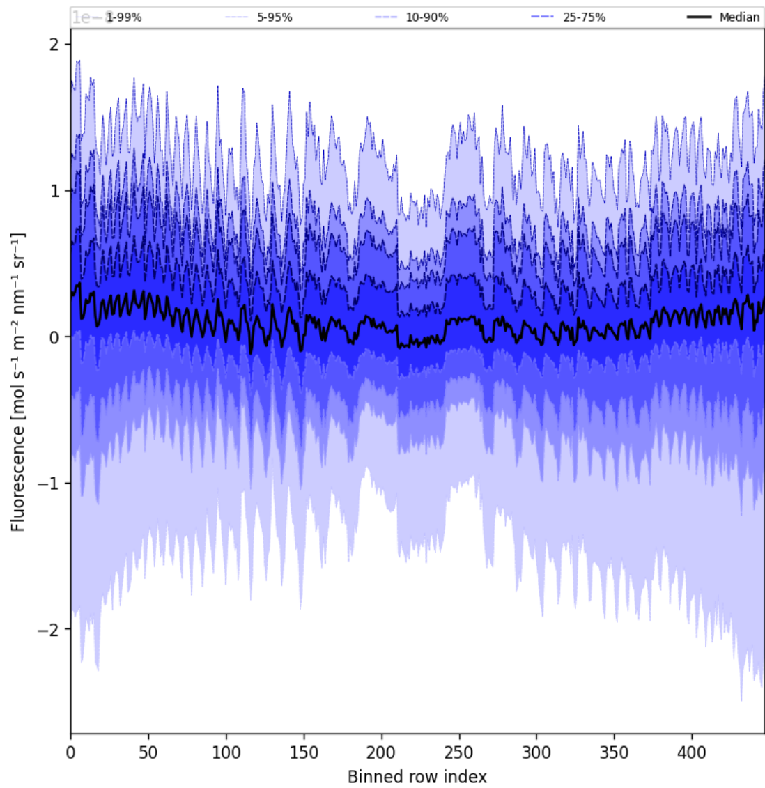
Figure 57: Along track statistics of “Fluorescence” for 2025-03-23 to 2025-03-25
