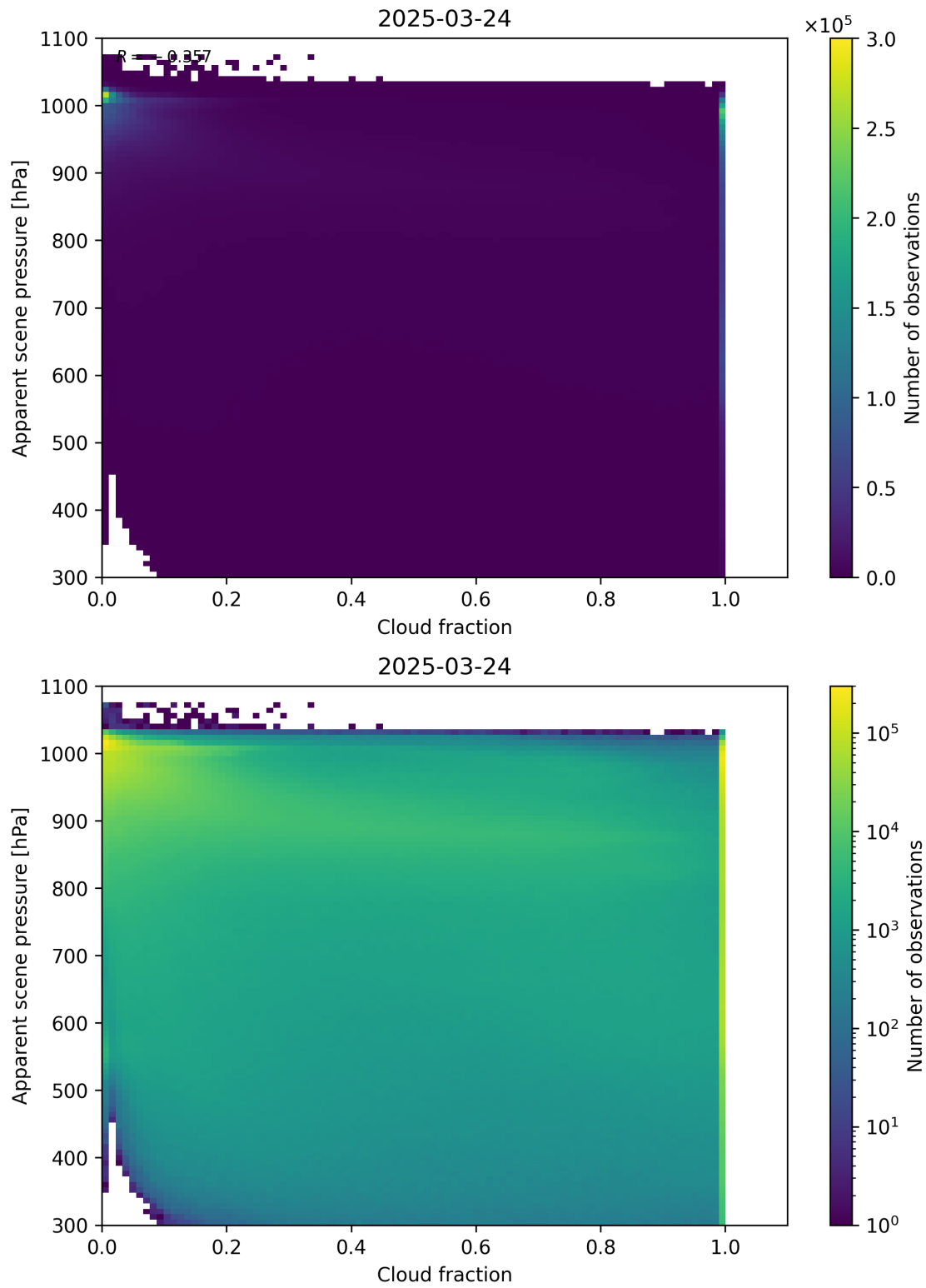
Figure 70: Scatter density plot of “Cloud fraction” against “Apparent scene pressure” for 2025-03-23 to 2025-03-25.
