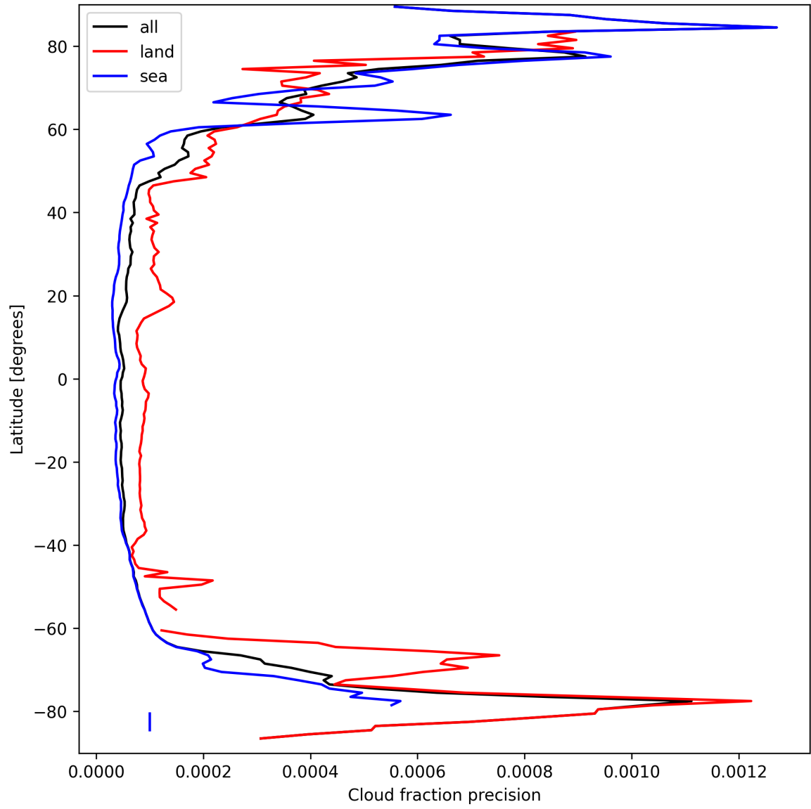
Figure 16: Zonal average of “Cloud fraction precision” for 2025-03-23 to 2025-03-25.
