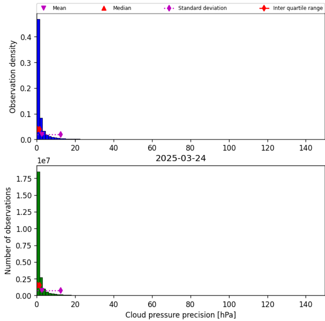
Figure 31: Histogram of “Cloud pressure precision” for 2025-03-23 to 2025-03-25
