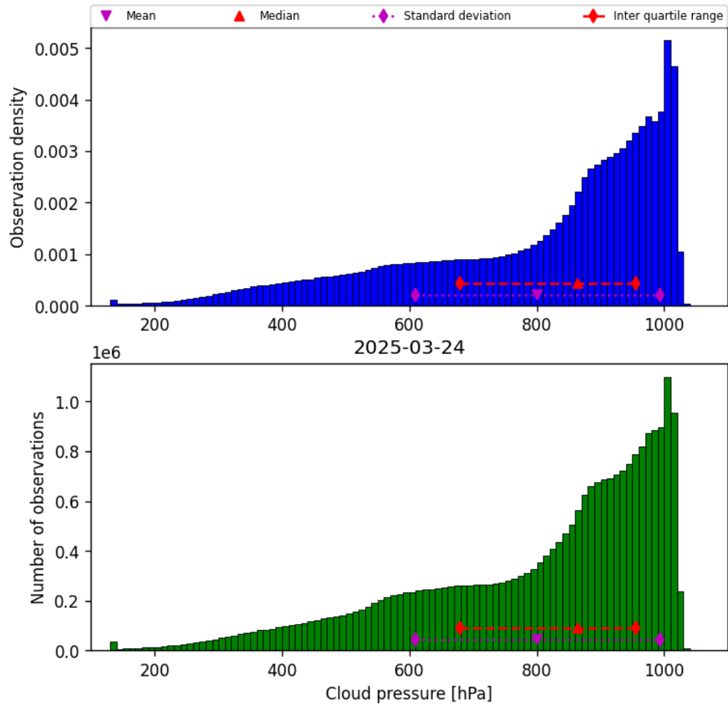
Figure 30: Histogram of “Cloud pressure” for 2025-03-23 to 2025-03-25
