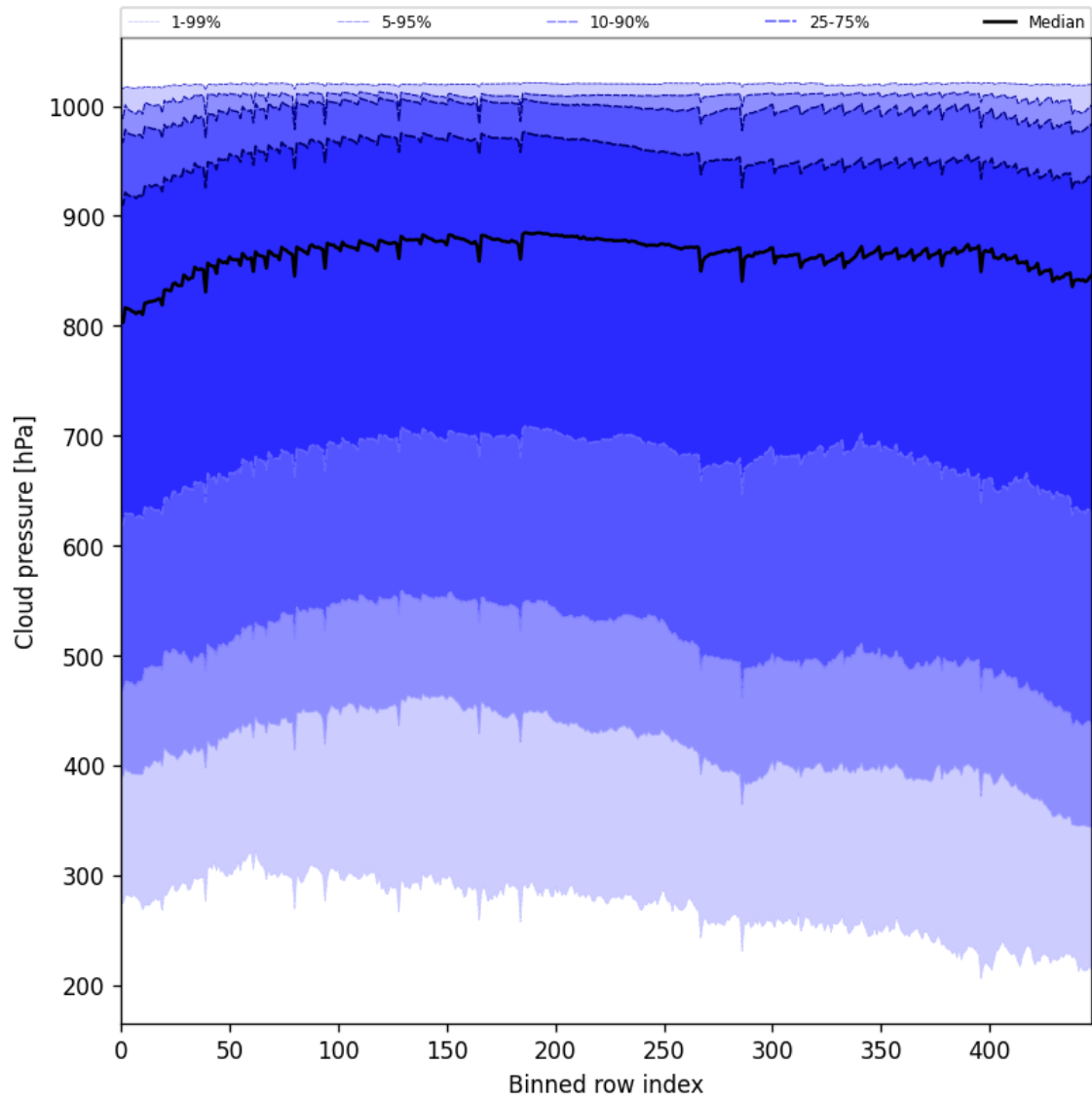
Figure 47: Along track statistics of “Cloud pressure” for 2025-03-23 to 2025-03-25
