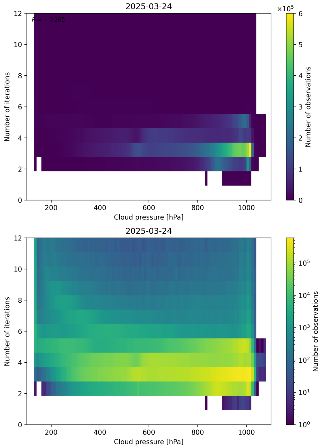
Figure 81: Scatter density plot of “Cloud pressure” against “Number of iterations” for 2025-03-23 to 2025-03-25.
