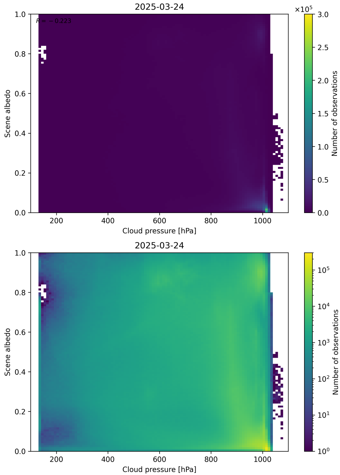
Figure 83: Scatter density plot of “Cloud pressure” against “Scene albedo” for 2025-03-23 to 2025-03-25.
