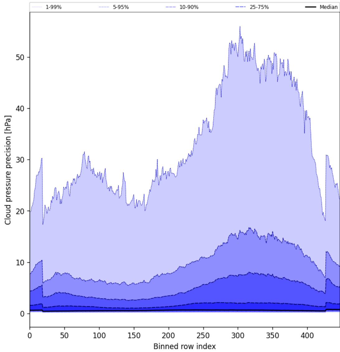
Figure 48: Along track statistics of “Cloud pressure precision” for 2025-03-23 to 2025-03-25
