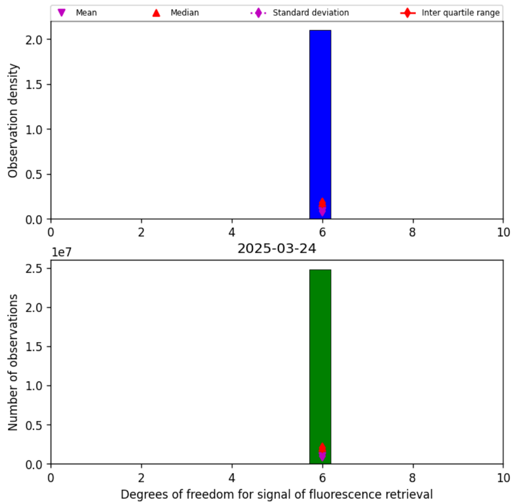
Figure 43: Histogram of “Degrees of freedom for signal of fluorescence retrieval” for 2025-03-23 to 2025-03-25
