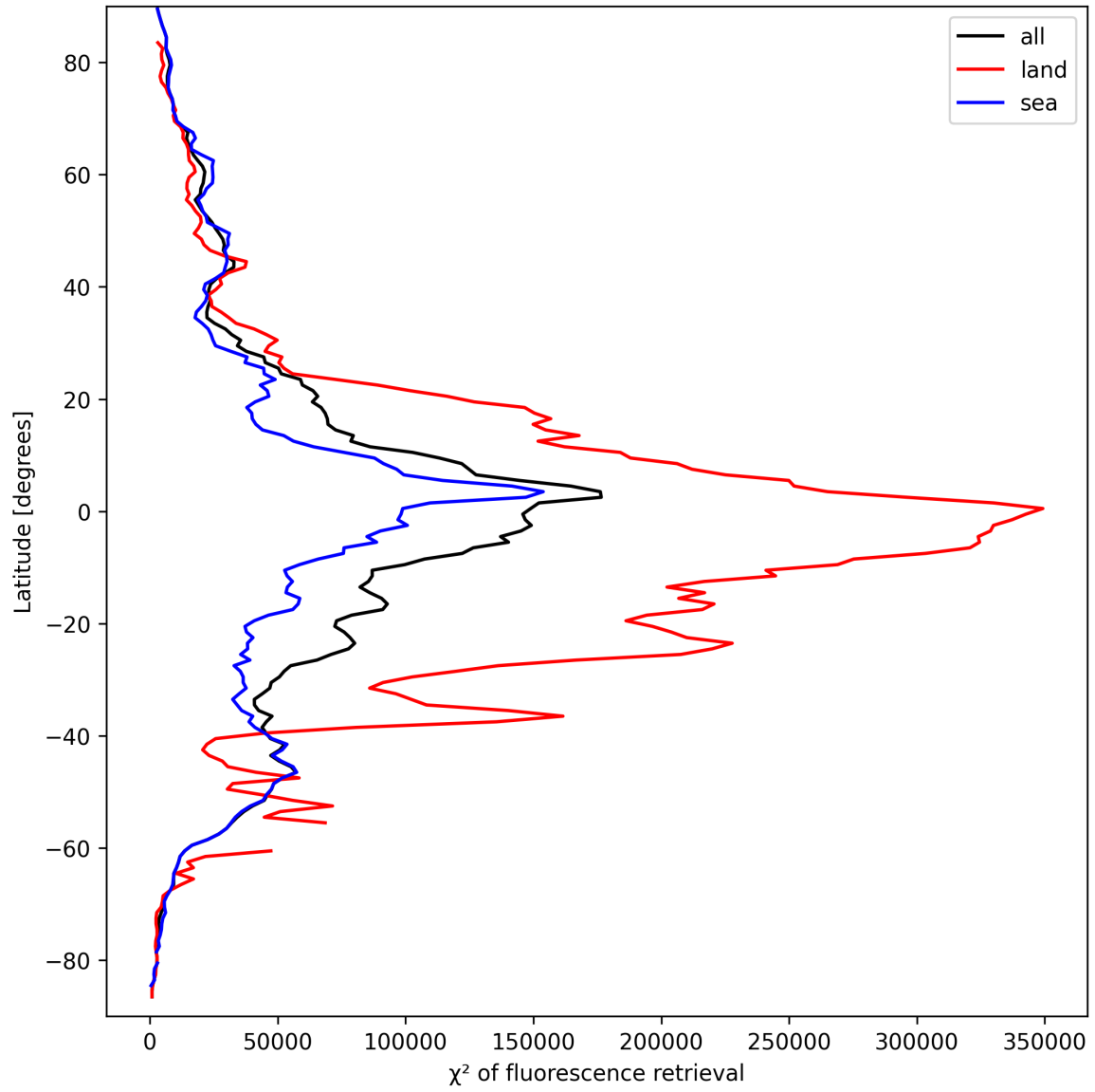
Figure 25: Zonal average of “ \chi^2 of fluorescence retrieval” for 2025-03-23 to 2025-03-25.
