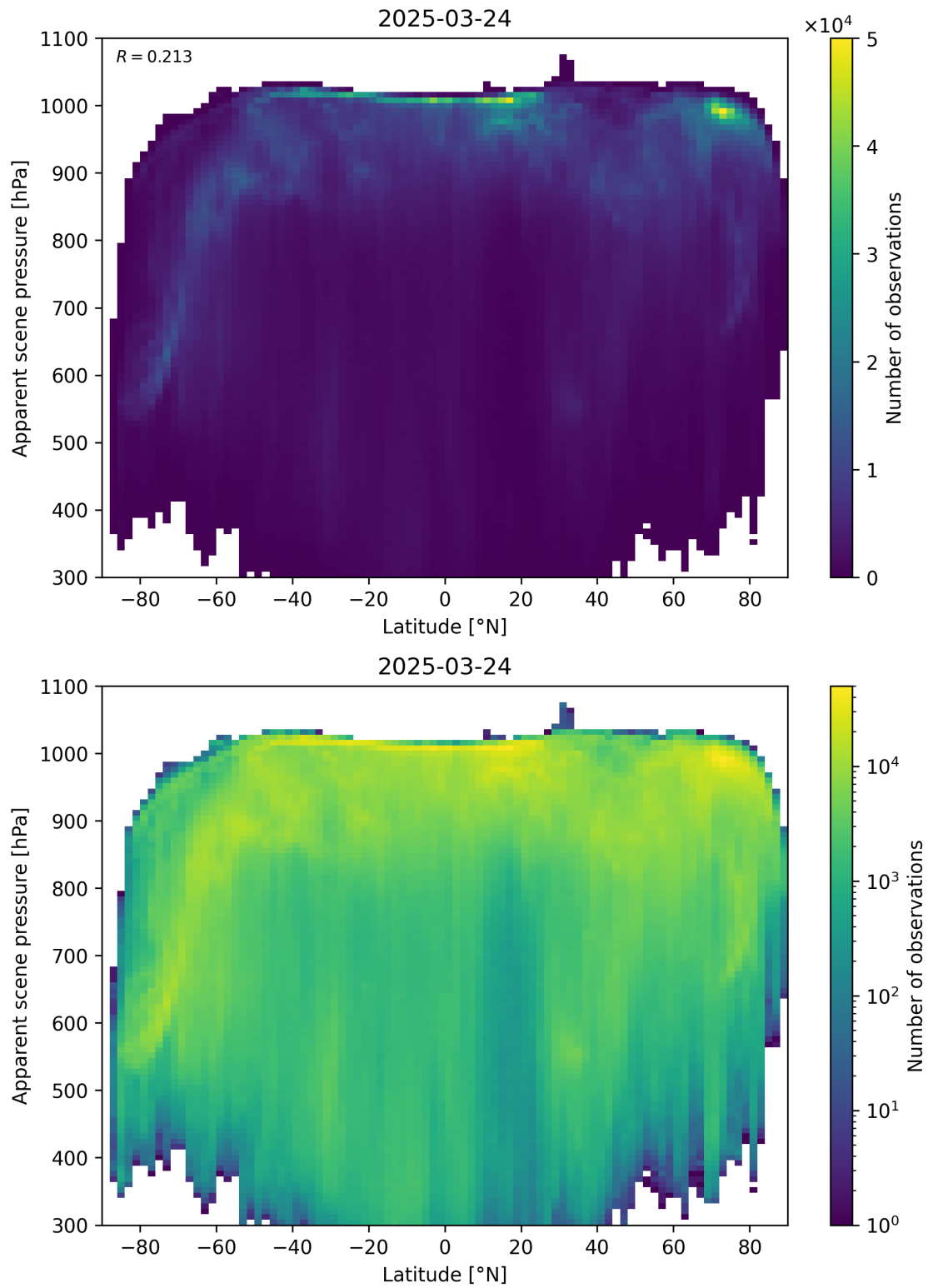
Figure 88: Scatter density plot of “Latitude” against “Apparent scene pressure” for 2025-03-23 to 2025-03-25.
