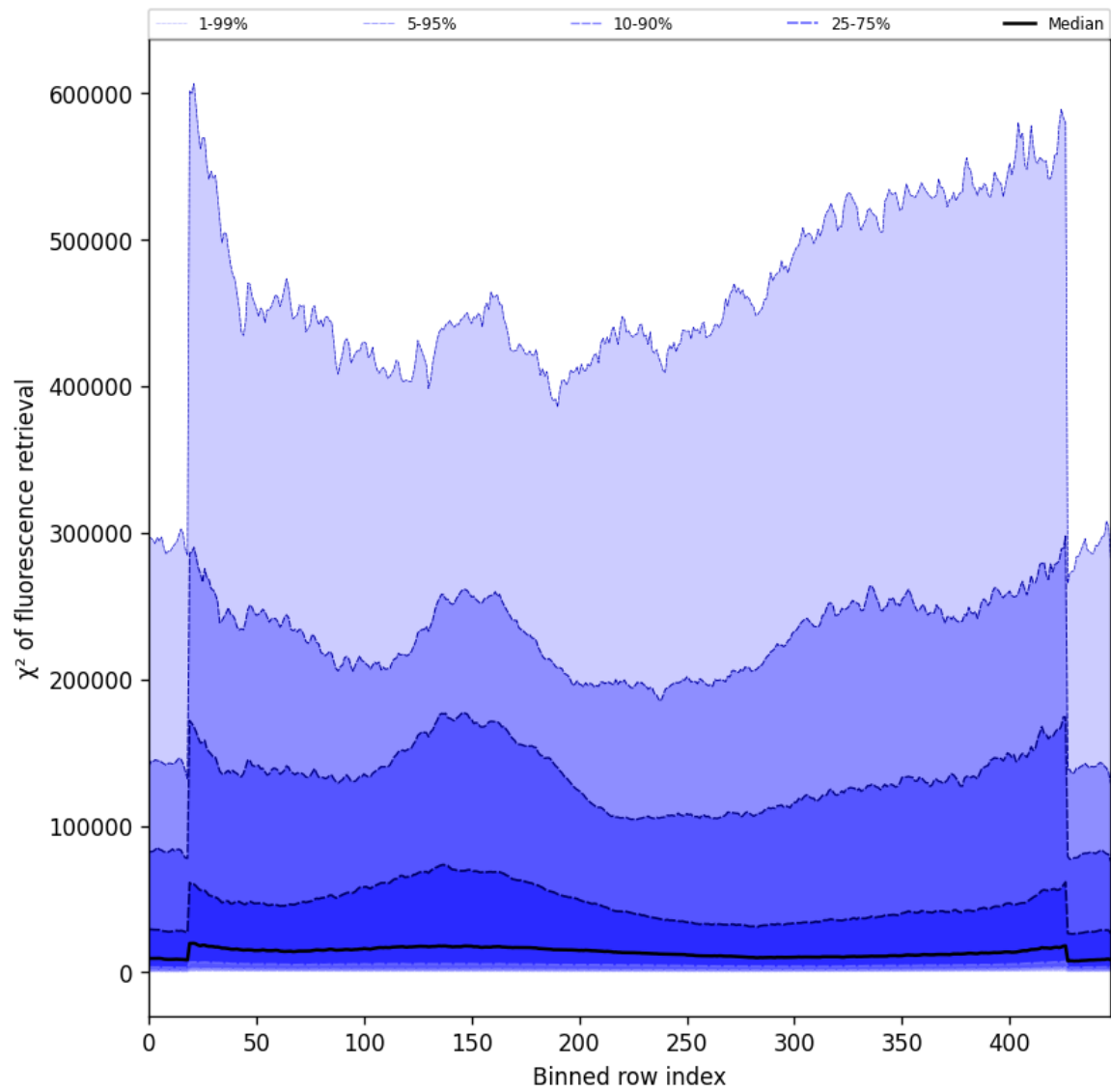
Figure 59: Along track statistics of “ \chi^2 of fluorescence retrieval” for 2025-03-23 to 2025-03-25
