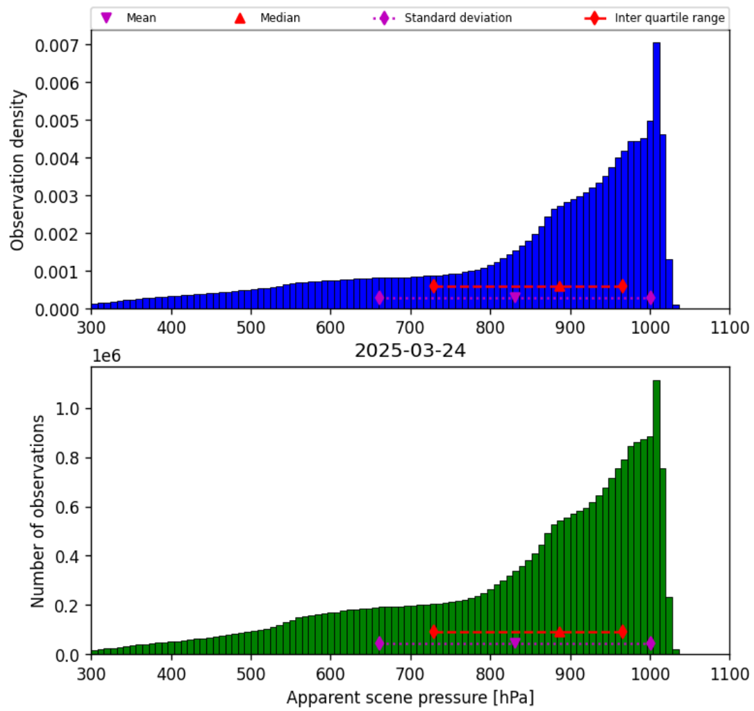
Figure 36: Histogram of “Apparent scene pressure” for 2025-03-23 to 2025-03-25
