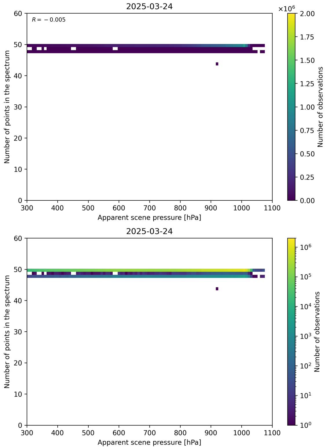
Figure 66: Scatter density plot of “Apparent scene pressure” against “Number of points in the spectrum” for 2025-03-23 to 2025-03-25.
