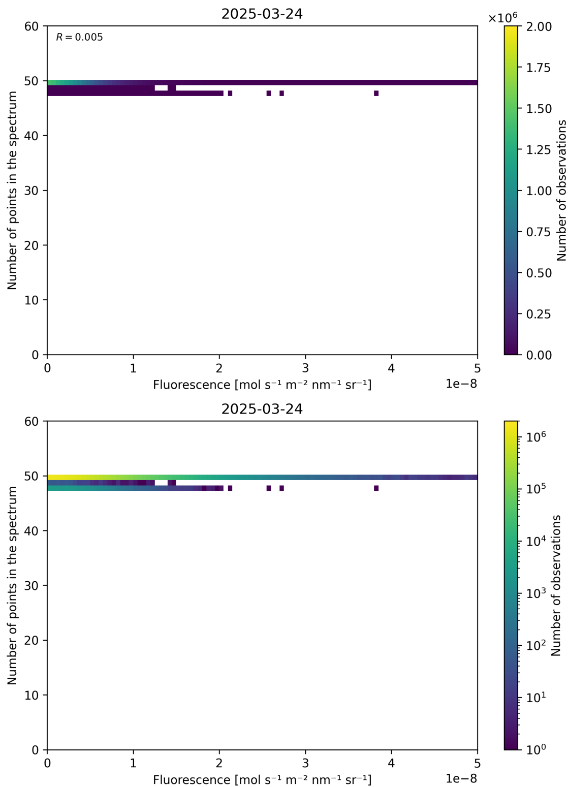
Figure 86: Scatter density plot of “Fluorescence” against “Number of points in the spectrum” for 2025-03-23 to 2025-03-25.
