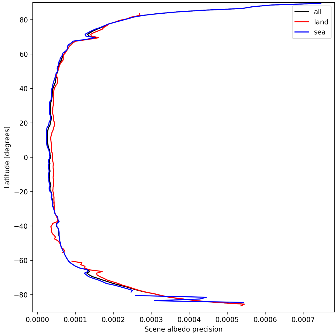
Figure 18: Zonal average of “Scene albedo precision” for 2025-03-23 to 2025-03-25.
