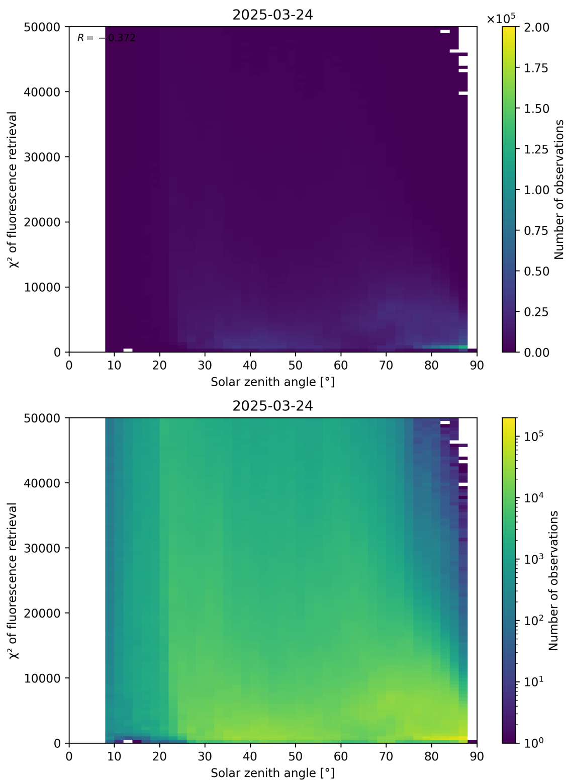
Figure 109: Scatter density plot of “Solar zenith angle” against “ \chi^2 of fluorescence retrieval” for 2025-03-23 to 2025-03-25.
