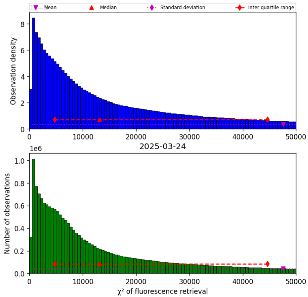
Figure 42: Histogram of “ \chi^2 of fluorescence retrieval” for 2025-03-23 to 2025-03-25
