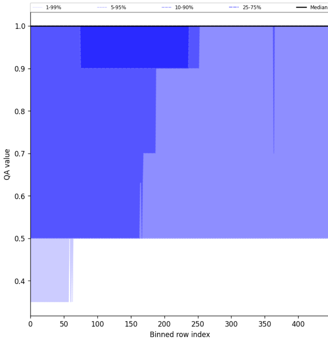
Figure 46: Along track statistics of “QA value” for 2025-03-23 to 2025-03-25
