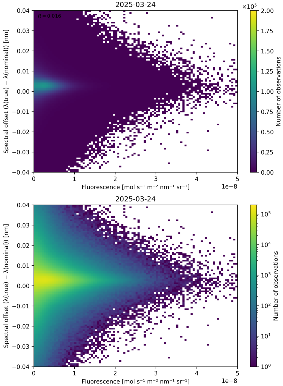
Figure 87: Scatter density plot of “Fluorescence” against “Spectral offset ( \lambda_{\text{true}} - \lambda_{\text{nominal}} )” for 2025-03-23 to 2025-03-25.
