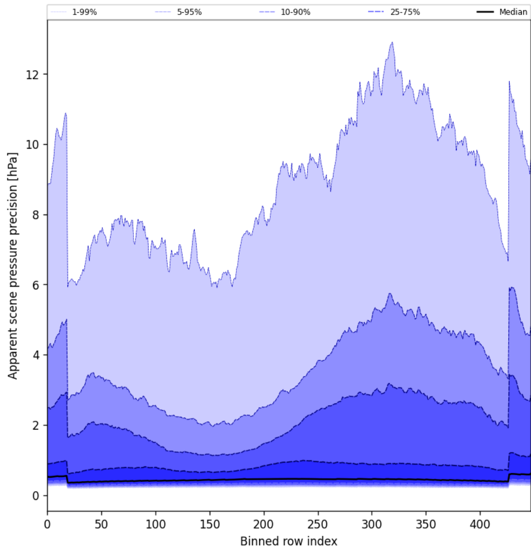
Figure 54: Along track statistics of “Apparent scene pressure precision” for 2025-03-23 to 2025-03-25
