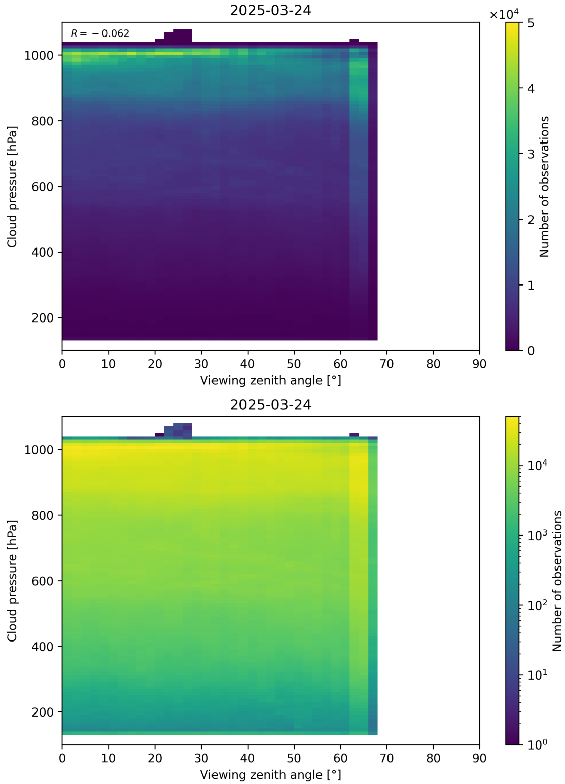
Figure 121: Scatter density plot of “Viewing zenith angle” against “Cloud pressure” for 2025-03-23 to 2025-03-25.
