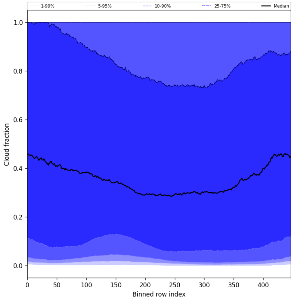
Figure 49: Along track statistics of “Cloud fraction” for 2025-03-23 to 2025-03-25
