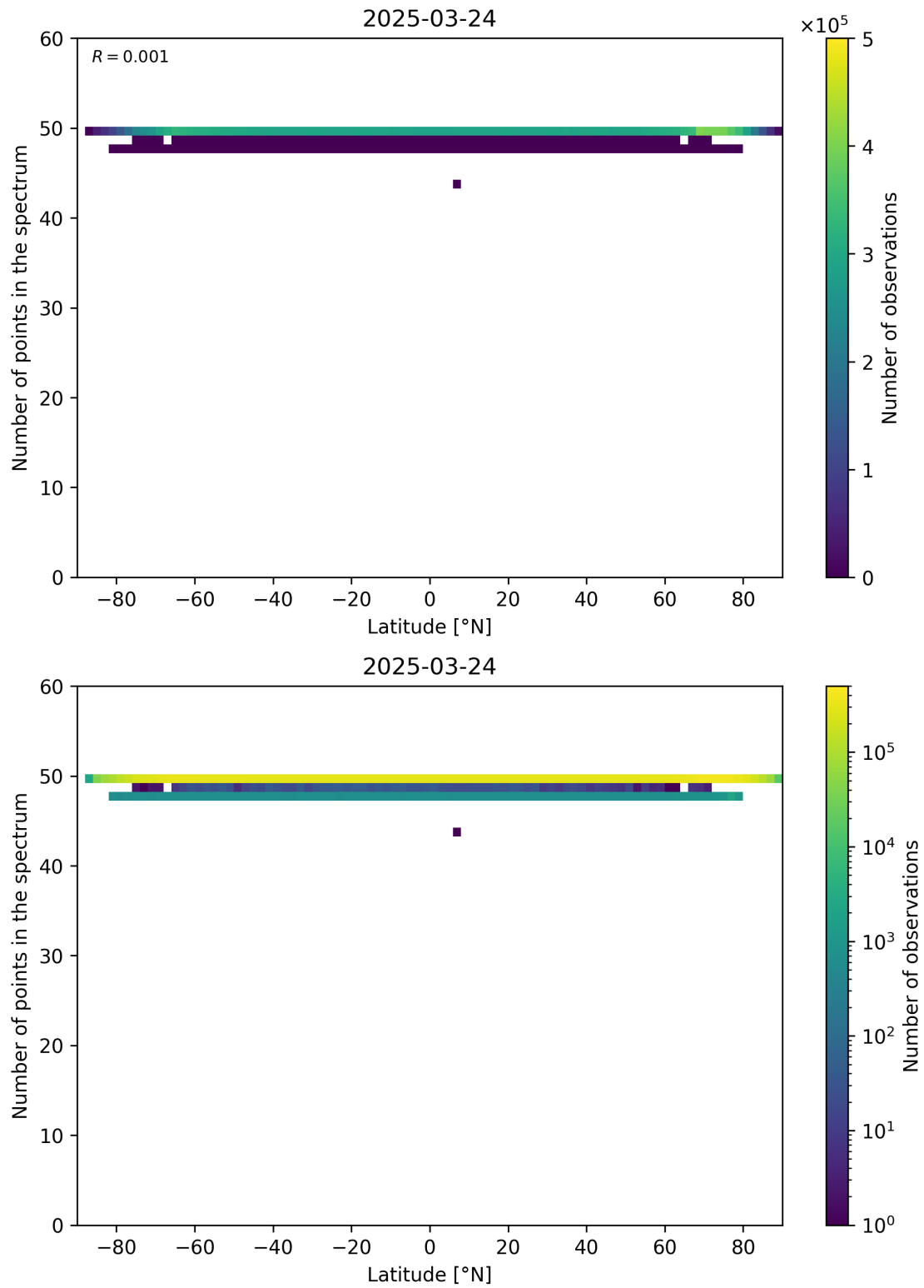
Figure 94: Scatter density plot of “Latitude” against “Number of points in the spectrum” for 2025-03-23 to 2025-03-25.
