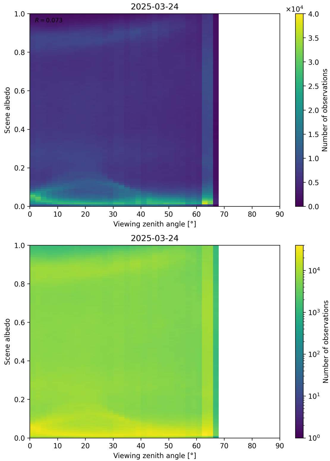
Figure 126: Scatter density plot of “Viewing zenith angle” against “Scene albedo” for 2025-03-23 to 2025-03-25.
