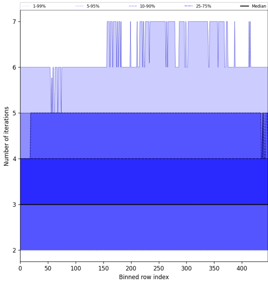
Figure 56: Along track statistics of “Number of iterations” for 2025-03-23 to 2025-03-25
