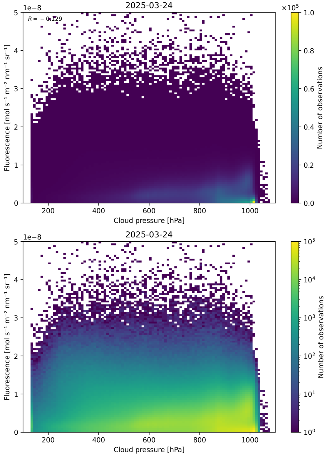
Figure 80: Scatter density plot of “Cloud pressure” against “Fluorescence” for 2025-03-23 to 2025-03-25.
