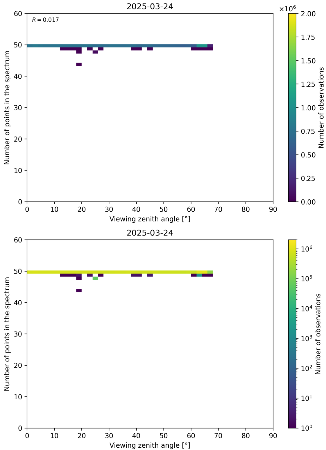
Figure 125: Scatter density plot of “Viewing zenith angle” against “Number of points in the spectrum” for 2025-03-23 to 2025-03-25.
