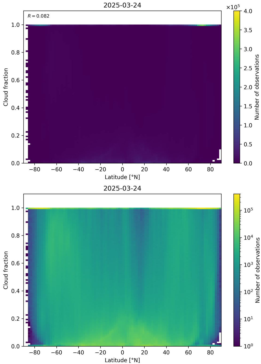
Figure 90: Scatter density plot of “Latitude” against “Cloud fraction” for 2025-03-23 to 2025-03-25.
