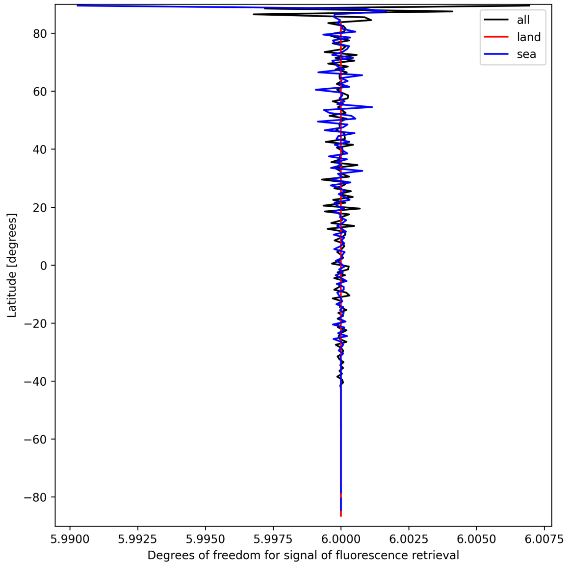
Figure 26: Zonal average of “Degrees of freedom for signal of fluorescence retrieval” for 2025-03-23 to 2025-03-25.
