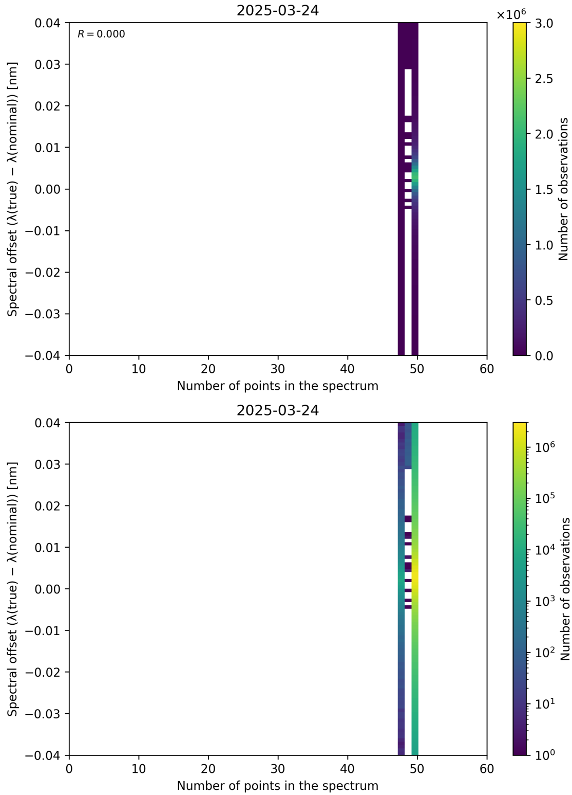
Figure 101: Scatter density plot of “Number of points in the spectrum” against “Spectral offset ( \lambda_{\text{true}} - \lambda_{\text{nominal}} )” for 2025-03-23 to 2025-03-25.
