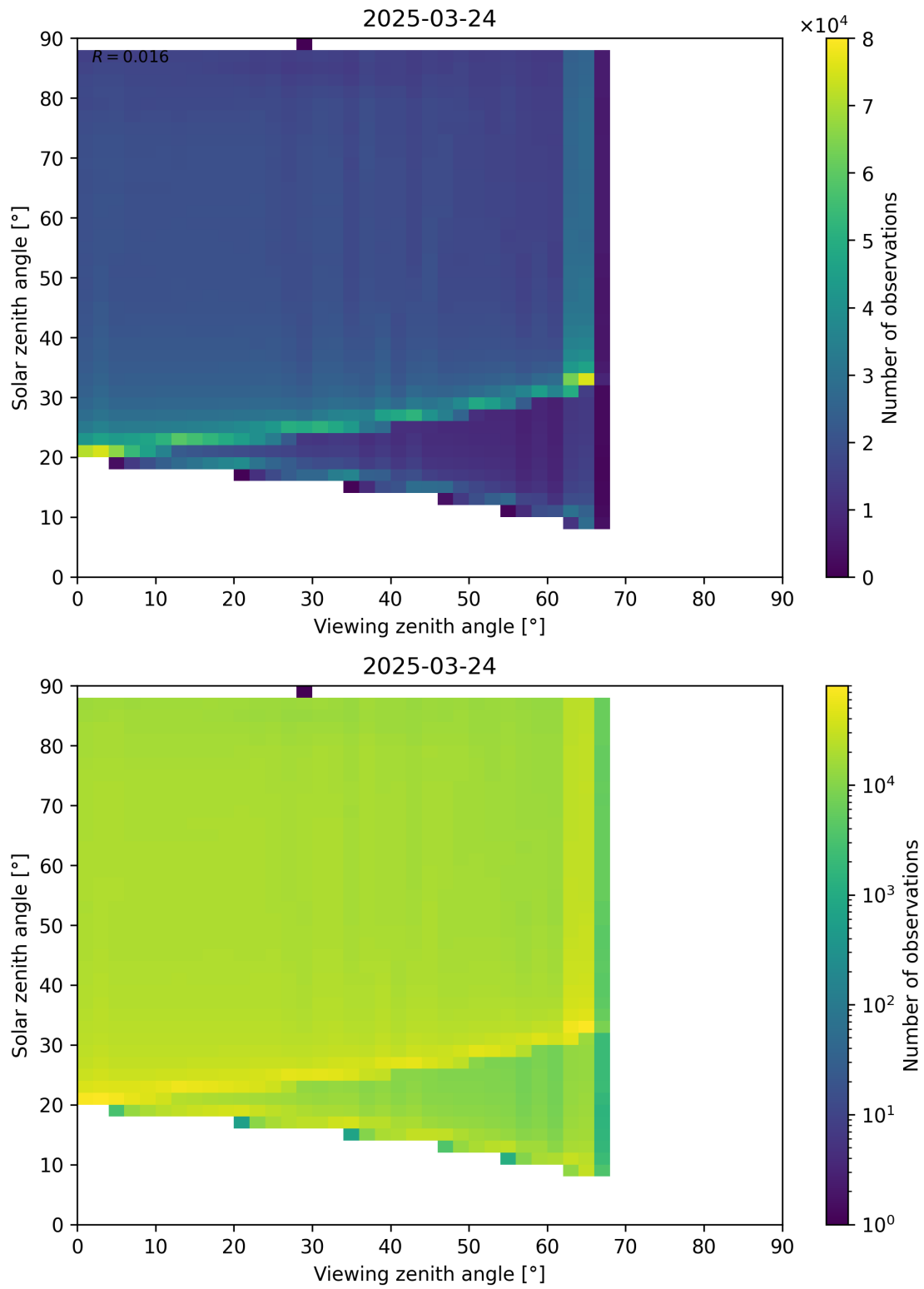
Figure 127: Scatter density plot of “Viewing zenith angle” against “Solar zenith angle” for 2025-03-23 to 2025-03-25.
