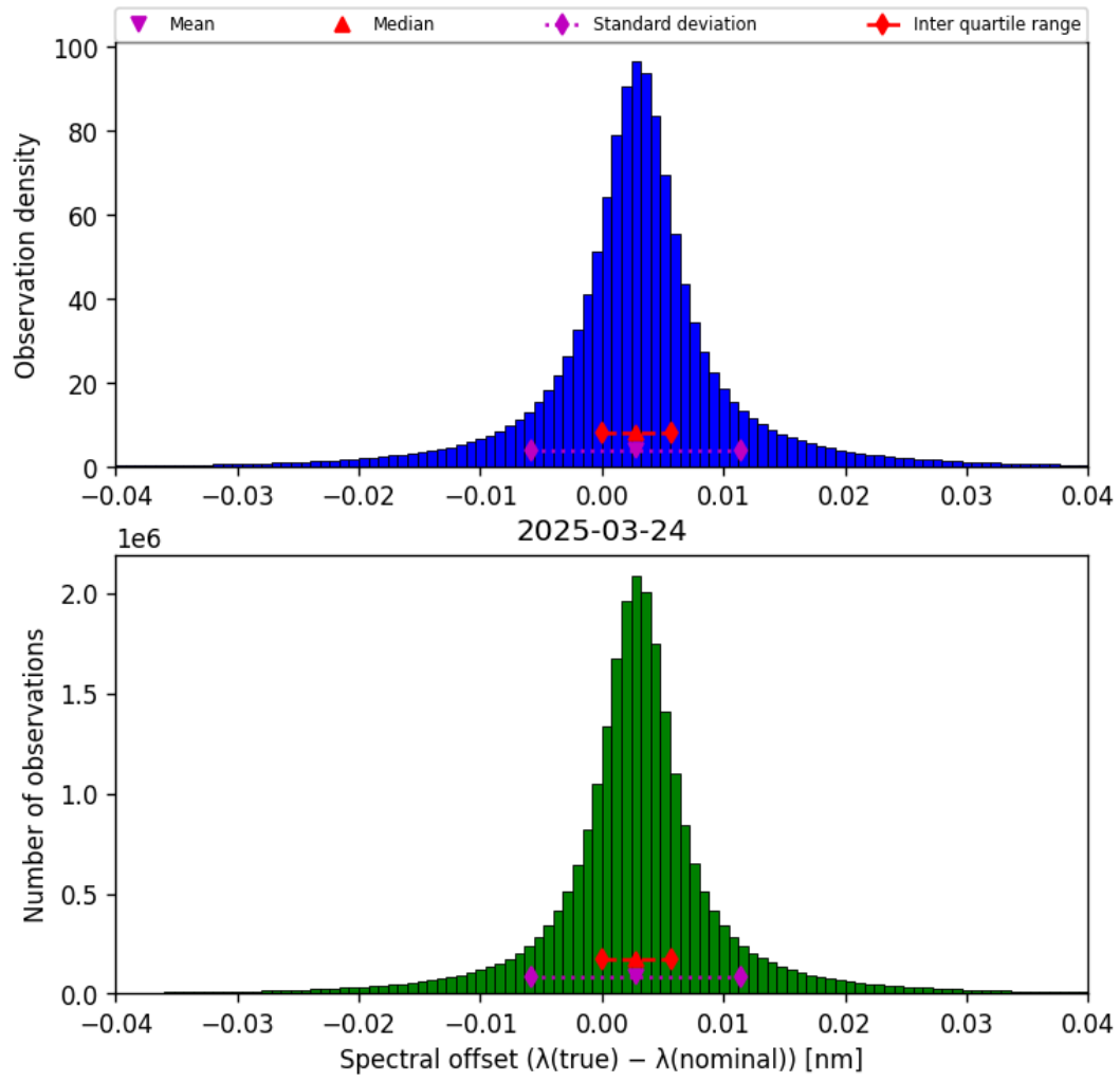
Figure 45: Histogram of “Spectral offset ( \lambda_{\text{true}} - \lambda_{\text{nominal}} )” for 2025-03-23 to 2025-03-25
