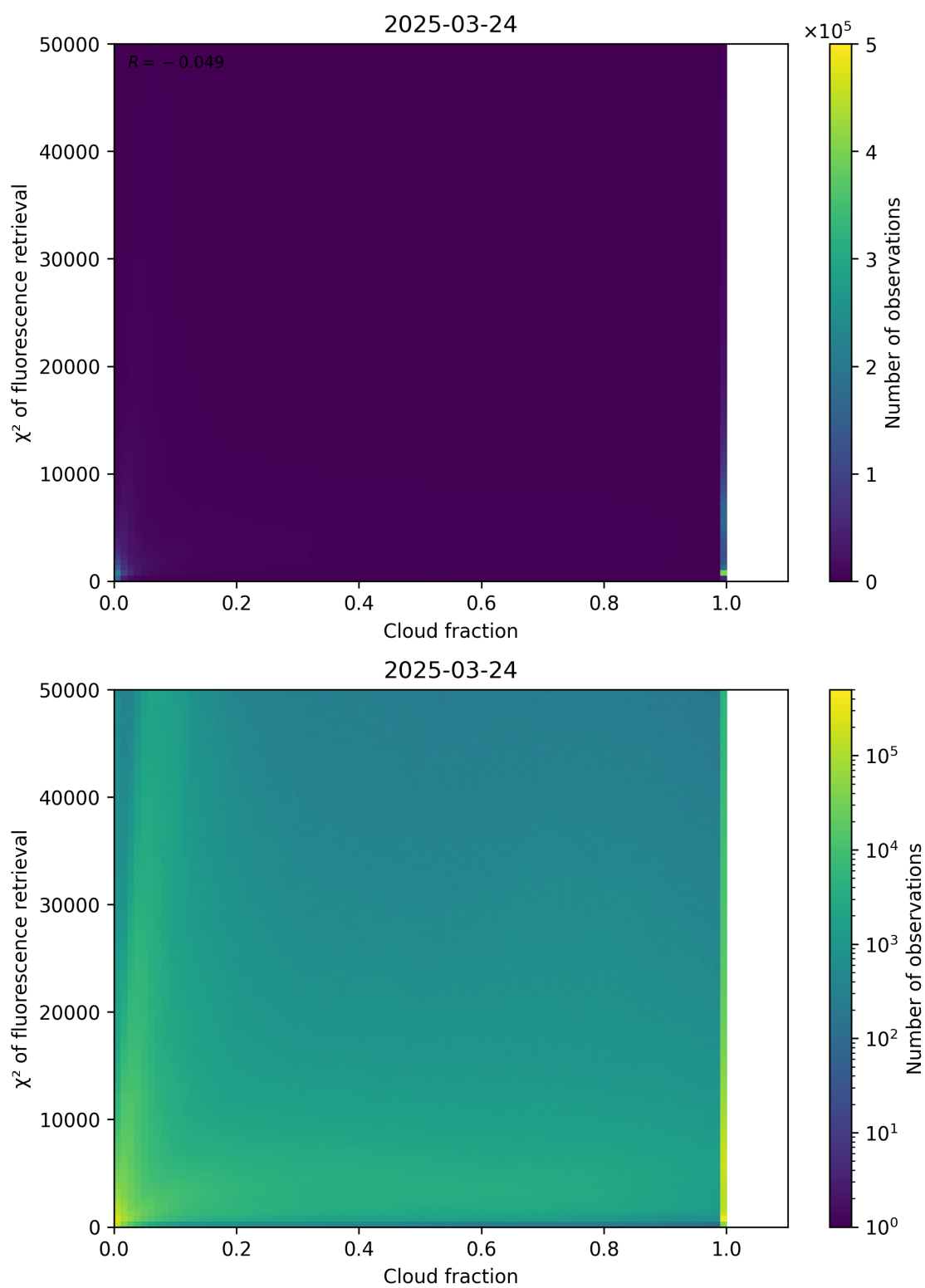
Figure 71: Scatter density plot of “Cloud fraction” against “ \chi^2 of fluorescence retrieval” for 2025-03-23 to 2025-03-25.
