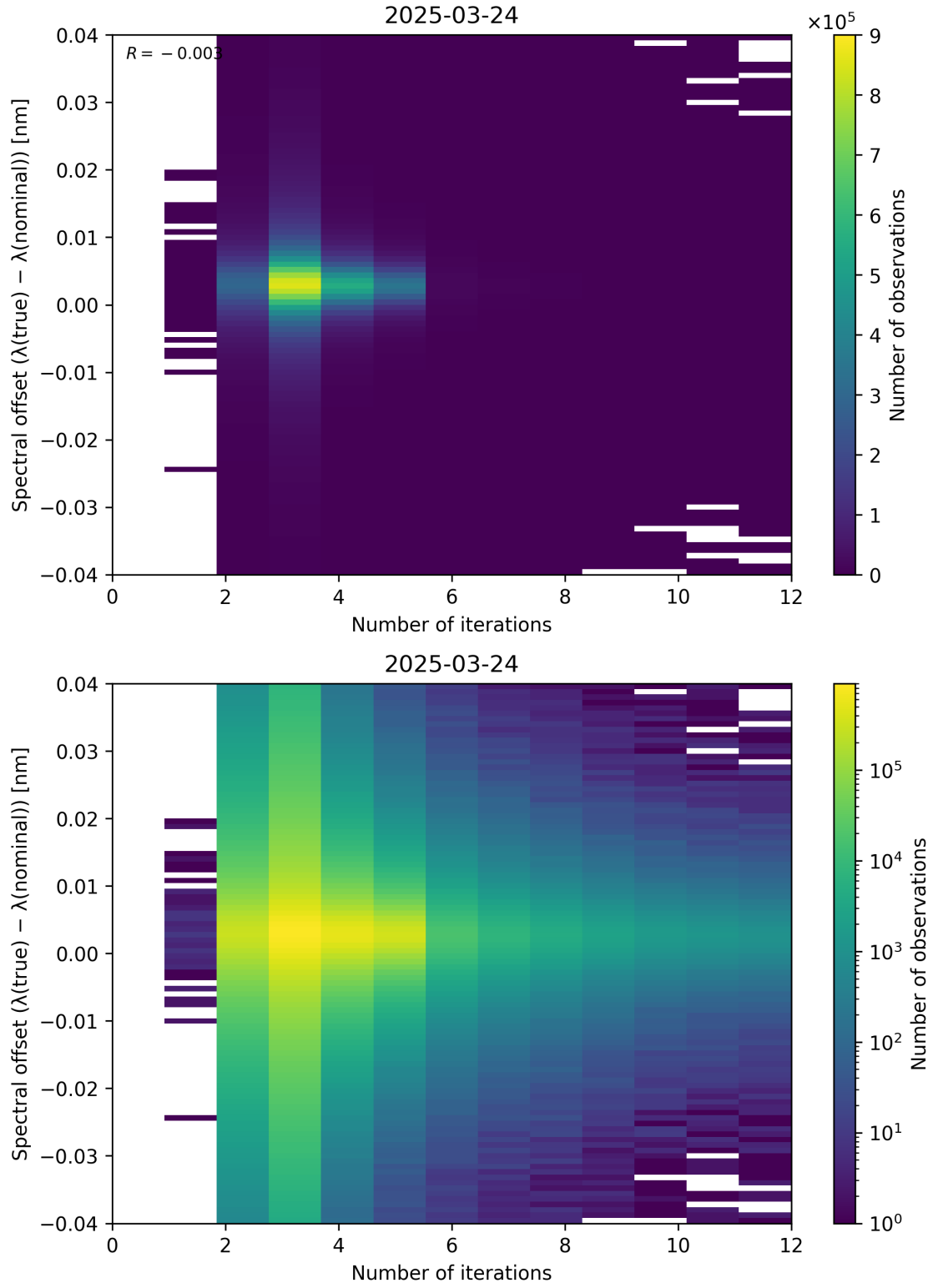
Figure 100: Scatter density plot of “Number of iterations” against “Spectral offset ( \lambda_{\text{true}} - \lambda_{\text{nominal}} )” for 2025-03-23 to 2025-03-25.
