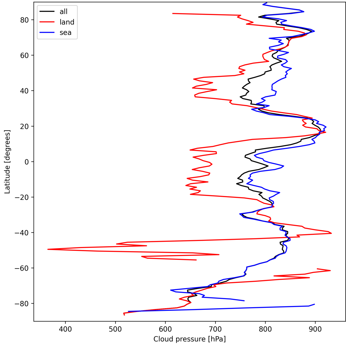
Figure 13: Zonal average of “Cloud pressure” for 2025-03-23 to 2025-03-25.
