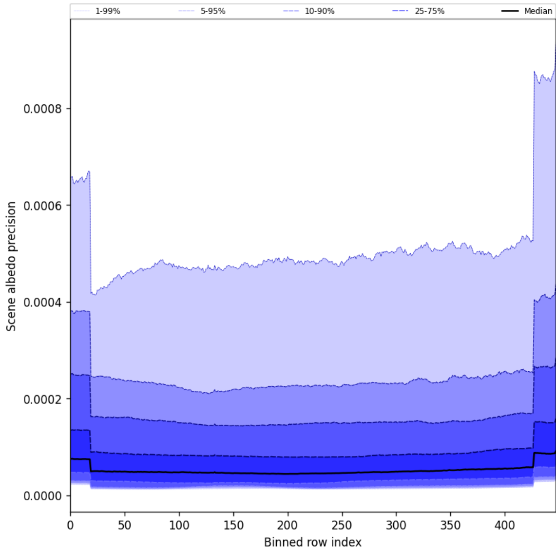
Figure 52: Along track statistics of “Scene albedo precision” for 2025-03-23 to 2025-03-25
