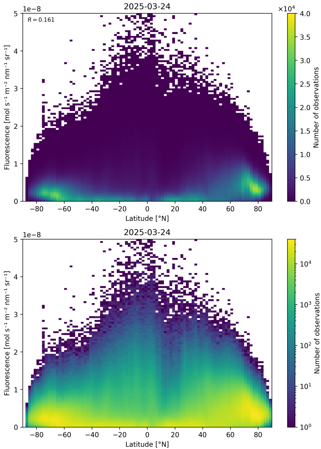
Figure 92: Scatter density plot of “Latitude” against “Fluorescence” for 2025-03-23 to 2025-03-25.
