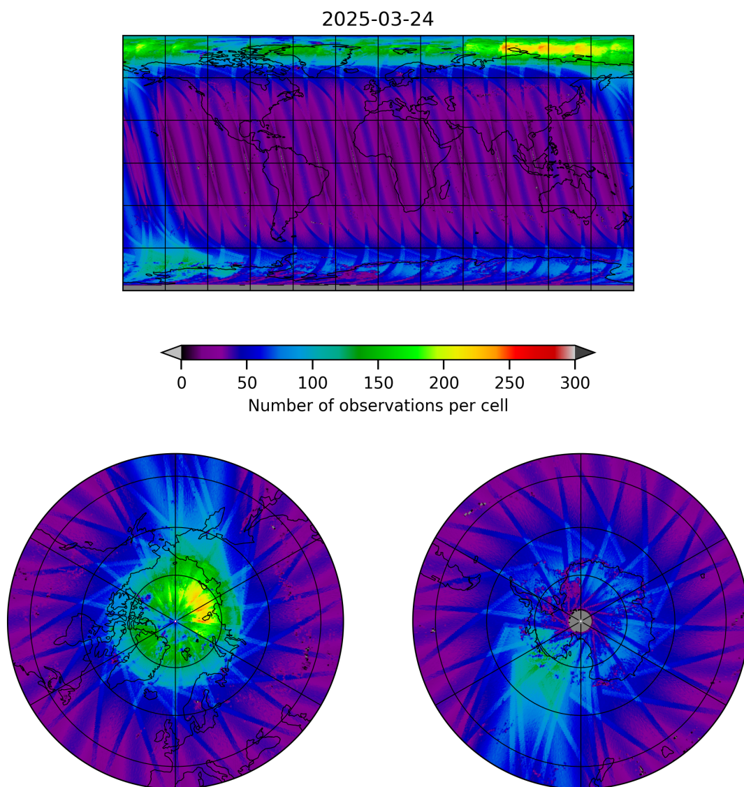
Figure 11: Map of the number of observations for 2025-03-23 to 2025-03-25
