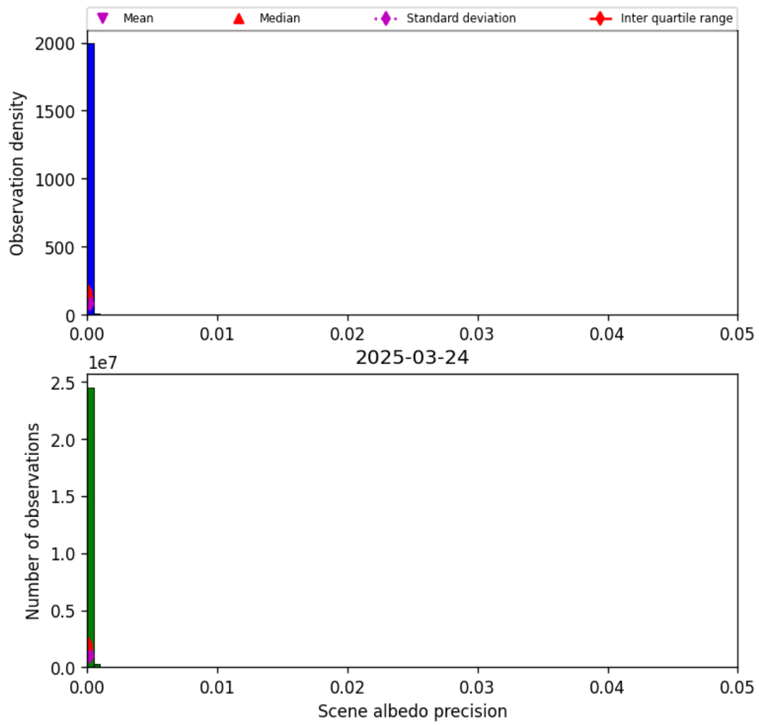
Figure 35: Histogram of “Scene albedo precision” for 2025-03-23 to 2025-03-25
