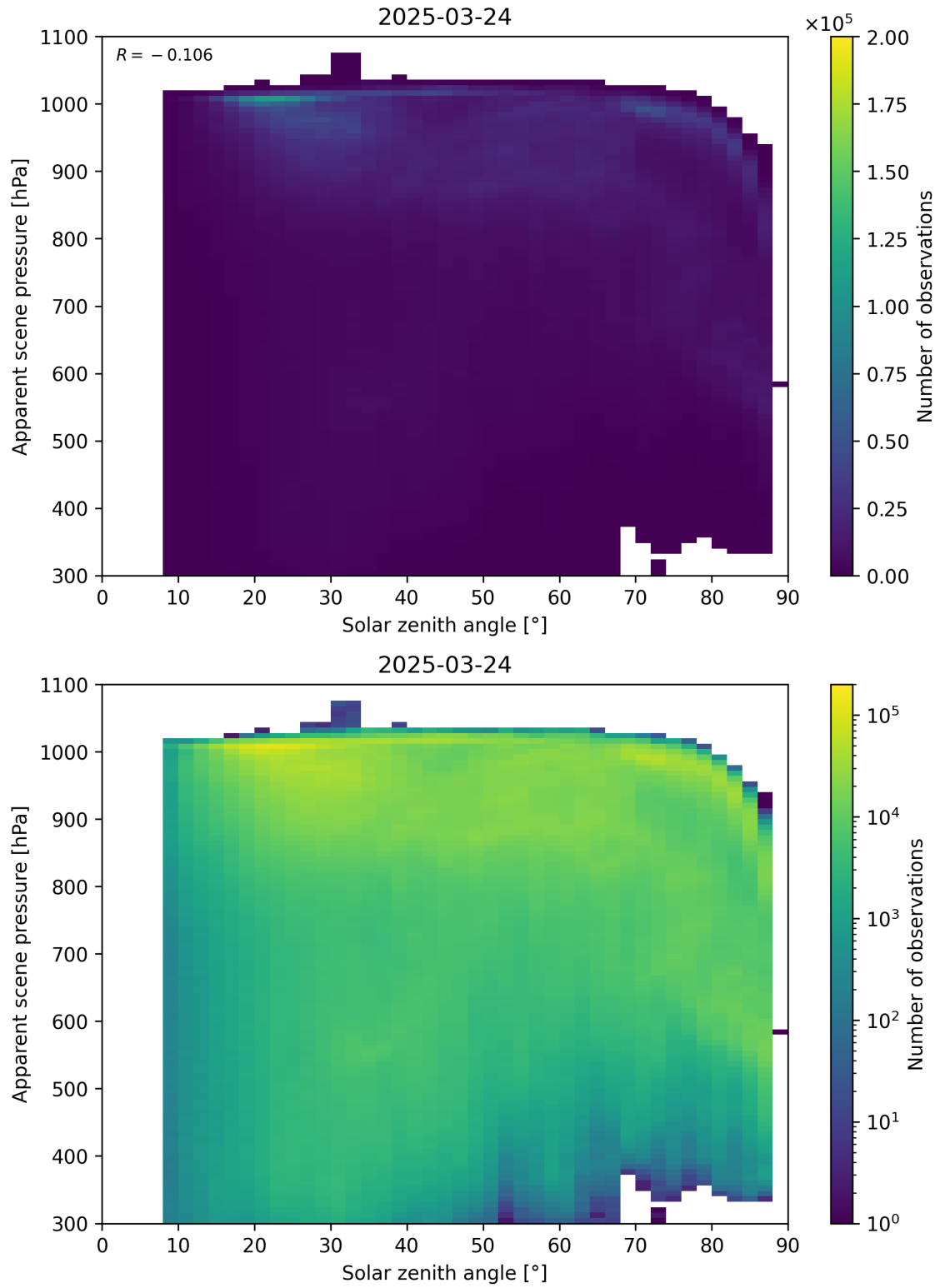
Figure 108: Scatter density plot of “Solar zenith angle” against “Apparent scene pressure” for 2025-03-23 to 2025-03-25.
