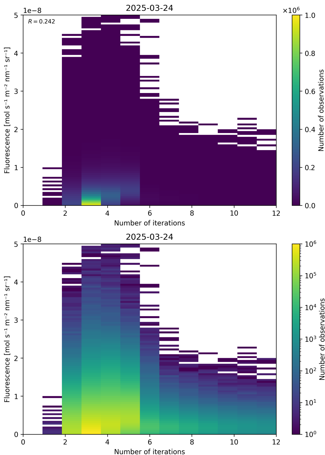
Figure 98: Scatter density plot of “Number of iterations” against “Fluorescence” for 2025-03-23 to 2025-03-25.
