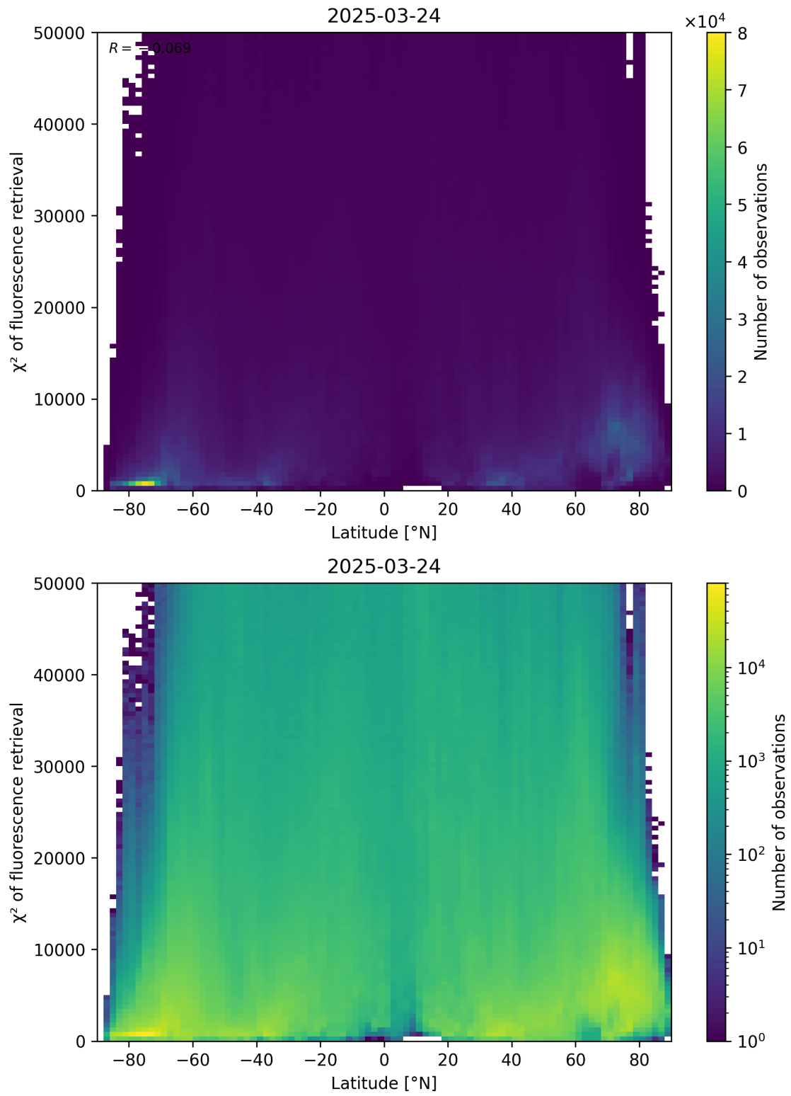
Figure 89: Scatter density plot of “Latitude” against “ \chi^2 of fluorescence retrieval” for 2025-03-23 to 2025-03-25.
