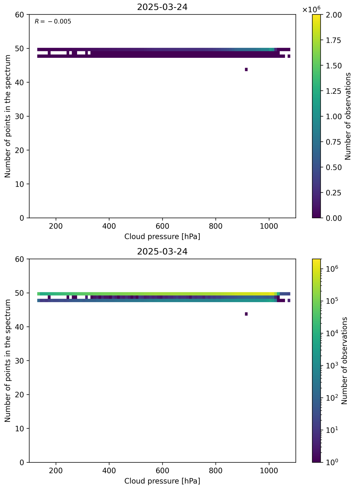
Figure 82: Scatter density plot of “Cloud pressure” against “Number of points in the spectrum” for 2025-03-23 to 2025-03-25.
