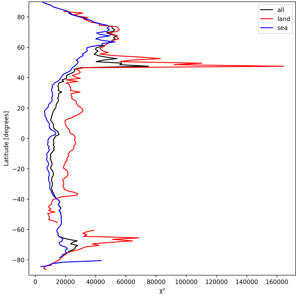
Figure 21: Zonal average of “ \chi^2 ” for 2025-03-23 to 2025-03-25.
