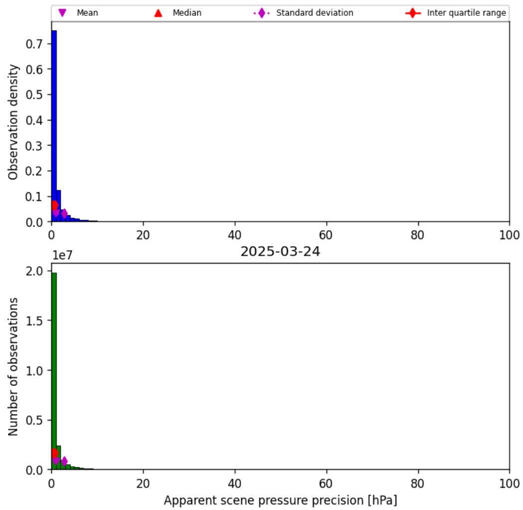
Figure 37: Histogram of “Apparent scene pressure precision” for 2025-03-23 to 2025-03-25
