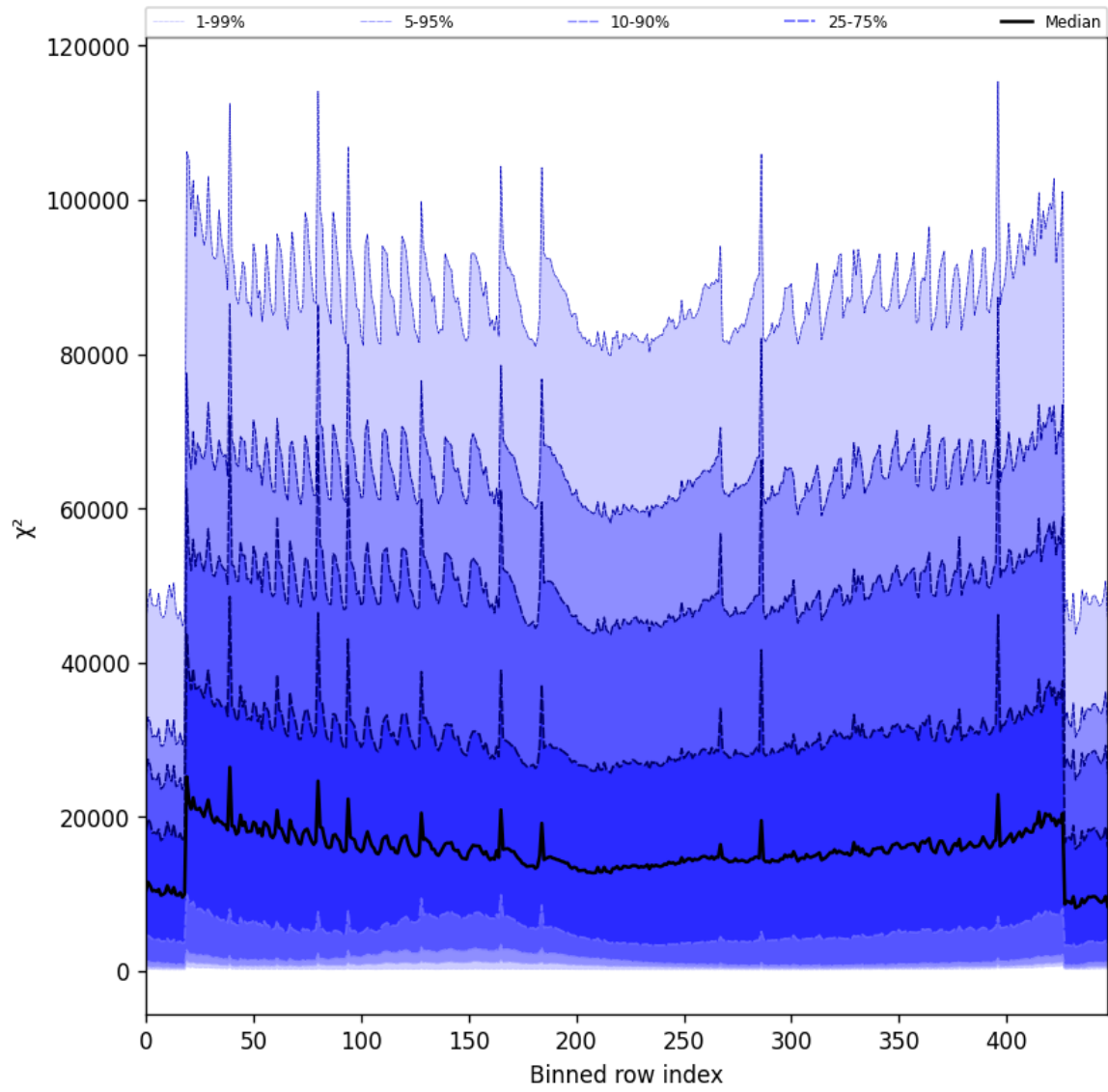
Figure 55: Along track statistics of “ \chi^2 ” for 2025-03-23 to 2025-03-25
