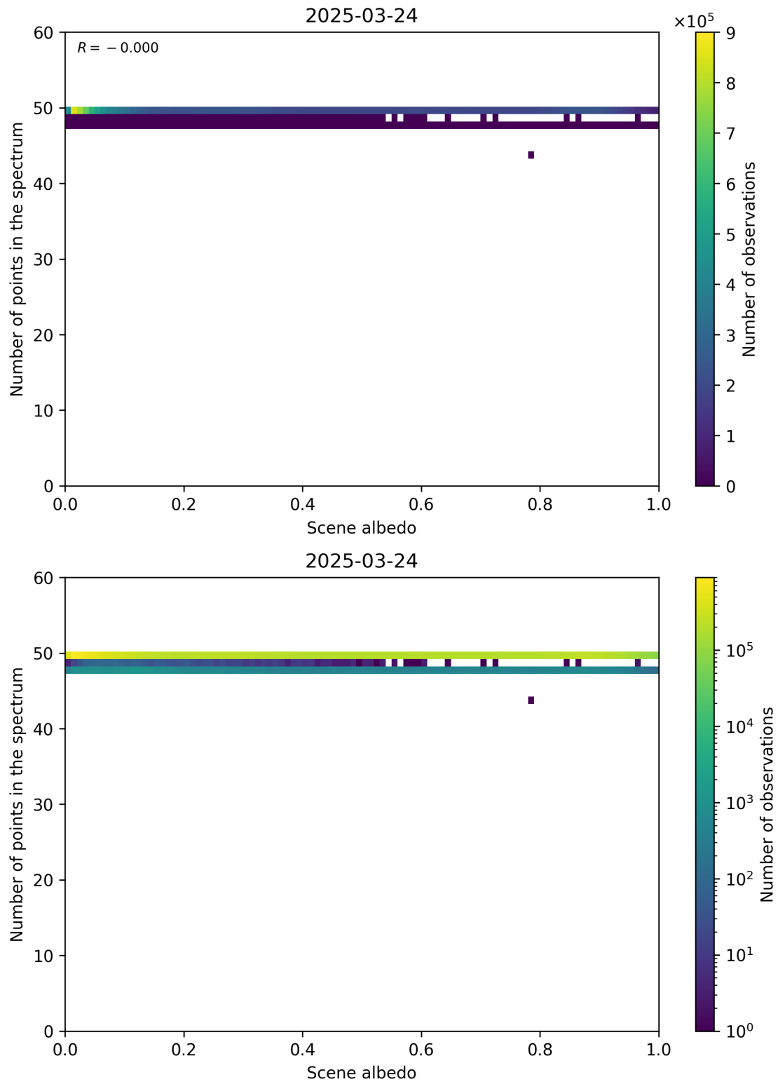
Figure 106: Scatter density plot of “Scene albedo” against “Number of points in the spectrum” for 2025-03-23 to 2025-03-25.
