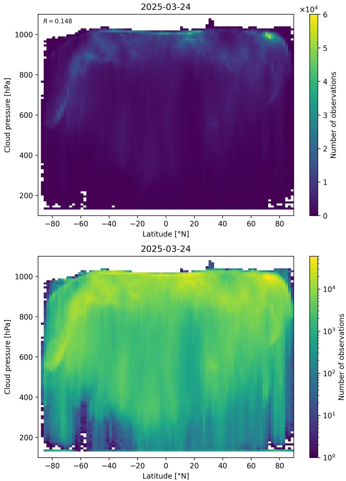
Figure 91: Scatter density plot of “Latitude” against “Cloud pressure” for 2025-03-23 to 2025-03-25.
