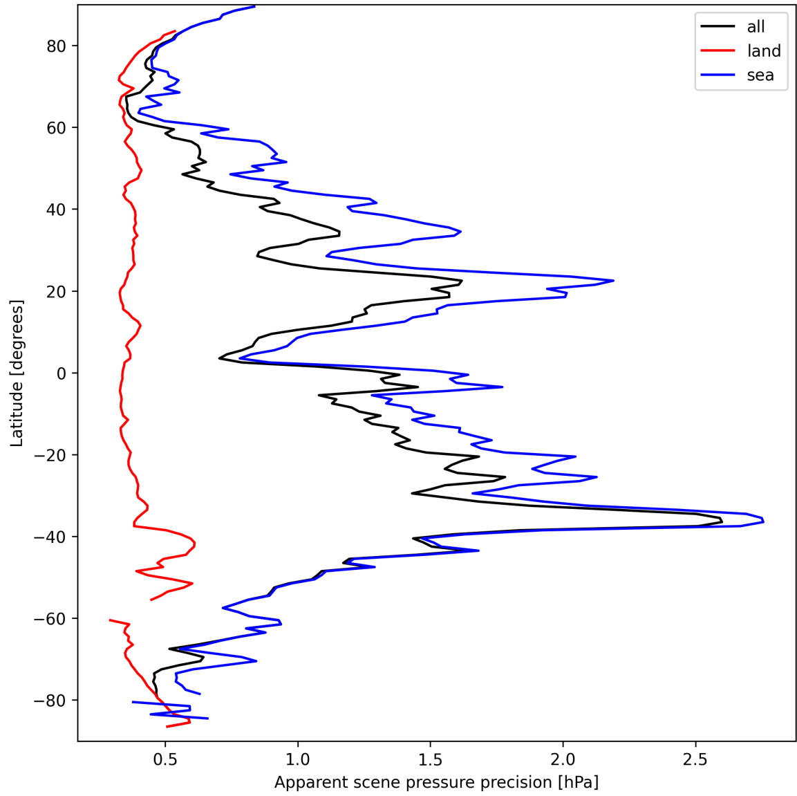
Figure 20: Zonal average of “Apparent scene pressure precision” for 2025-03-23 to 2025-03-25.
