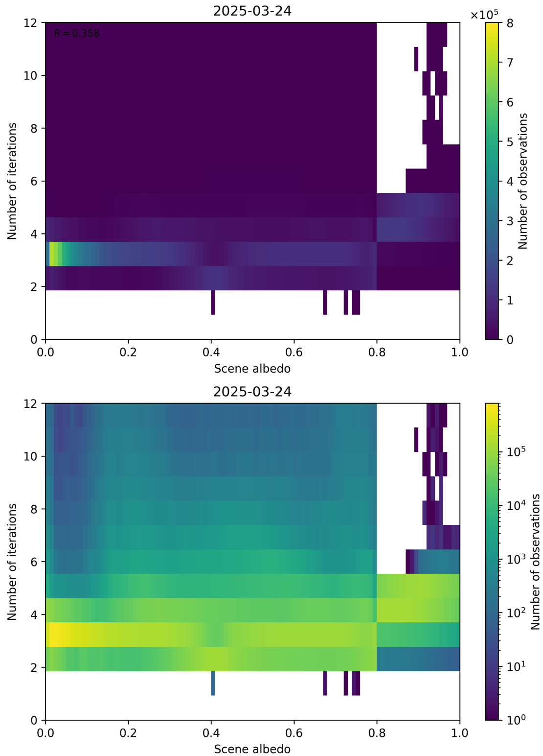
Figure 105: Scatter density plot of “Scene albedo” against “Number of iterations” for 2025-03-23 to 2025-03-25.
