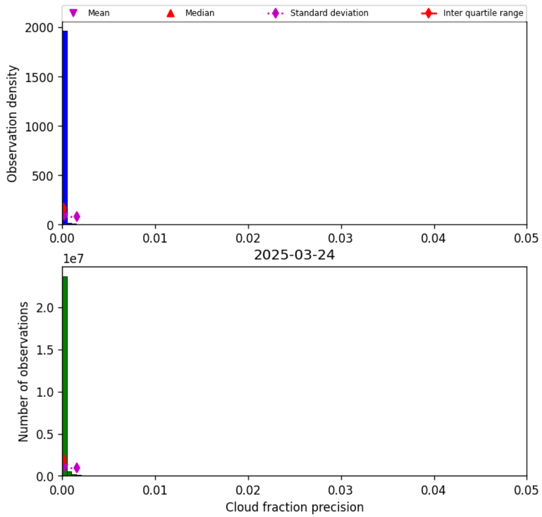
Figure 33: Histogram of “Cloud fraction precision” for 2025-03-23 to 2025-03-25
