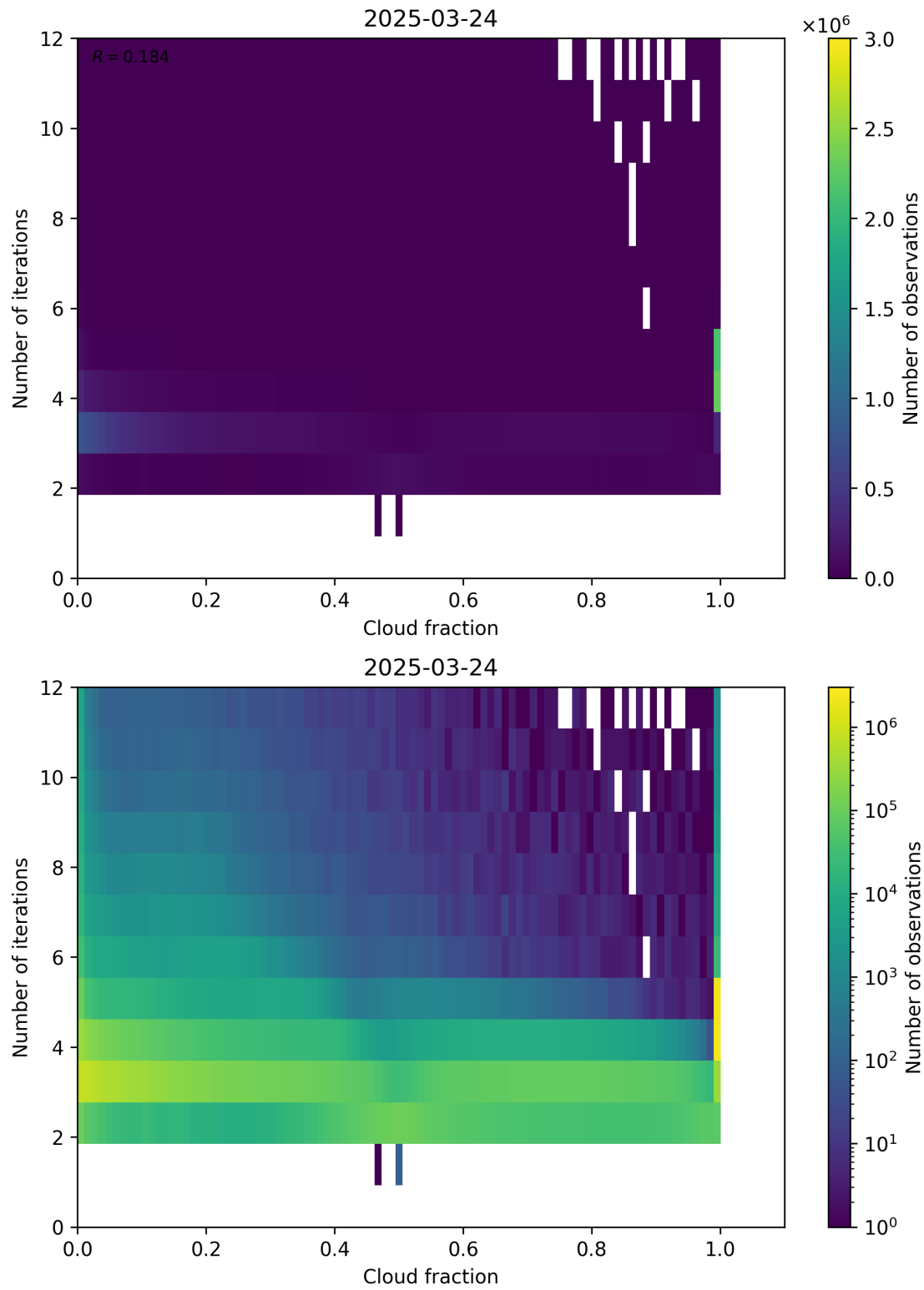
Figure 73: Scatter density plot of “Cloud fraction” against “Number of iterations” for 2025-03-23 to 2025-03-25.
