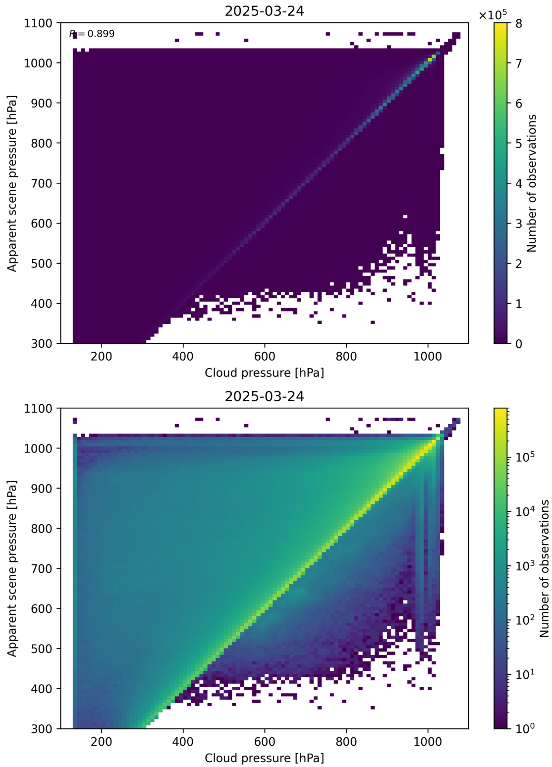
Figure 77: Scatter density plot of “Cloud pressure” against “Apparent scene pressure” for 2025-03-23 to 2025-03-25.
