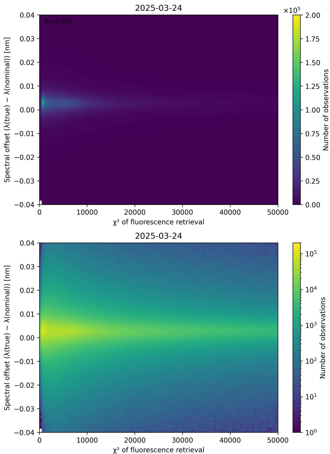
Figure 69: Scatter density plot of “ \chi^2 of fluorescence retrieval” against “Spectral offset ( \lambda_{\text{true}} - \lambda_{\text{nominal}} )” for 2025-03-23 to 2025-03-25.
