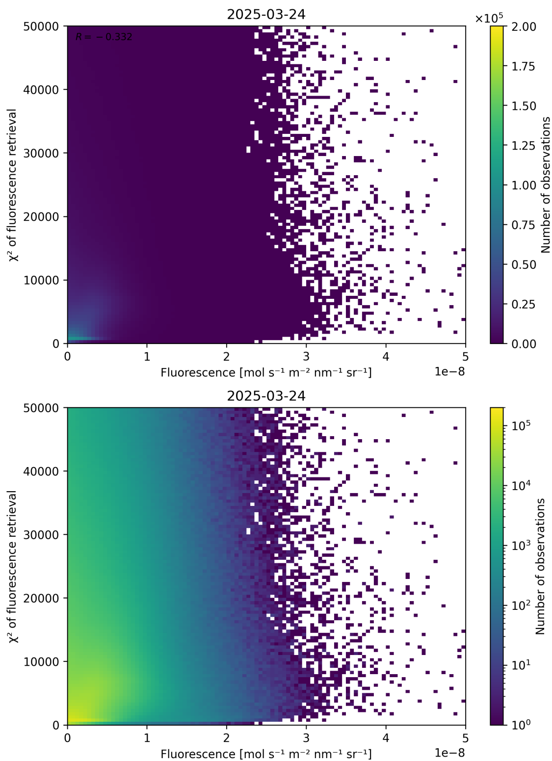
Figure 85: Scatter density plot of “Fluorescence” against “ \chi^2 of fluorescence retrieval” for 2025-03-23 to 2025-03-25.
