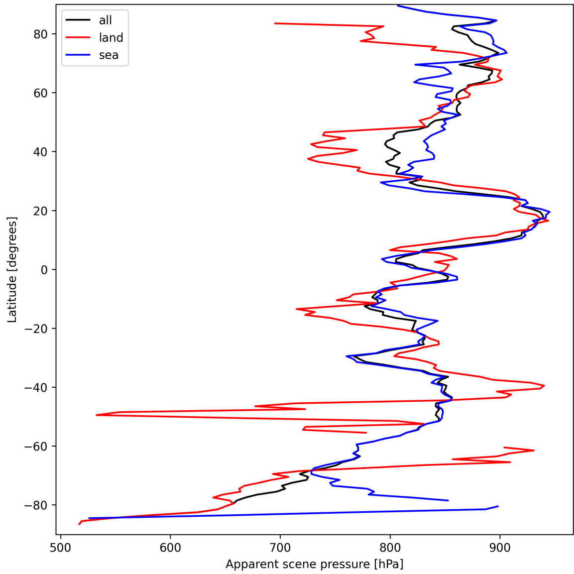
Figure 19: Zonal average of “Apparent scene pressure” for 2025-03-23 to 2025-03-25.
