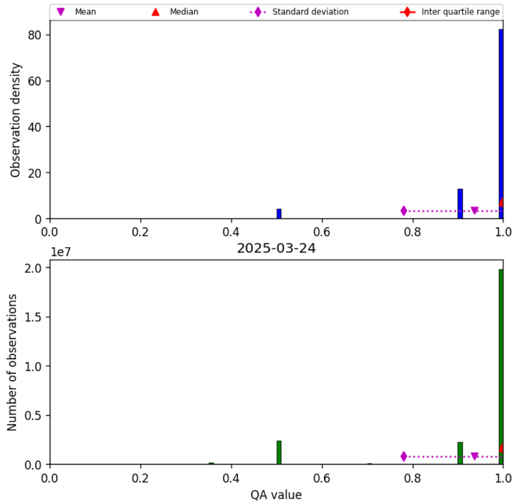
Figure 29: Histogram of “QA value” for 2025-03-23 to 2025-03-25
