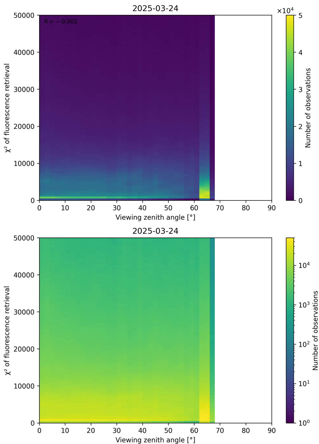
Figure 119: Scatter density plot of “Viewing zenith angle” against “ \chi^2 of fluorescence retrieval” for 2025-03-23 to 2025-03-25.
