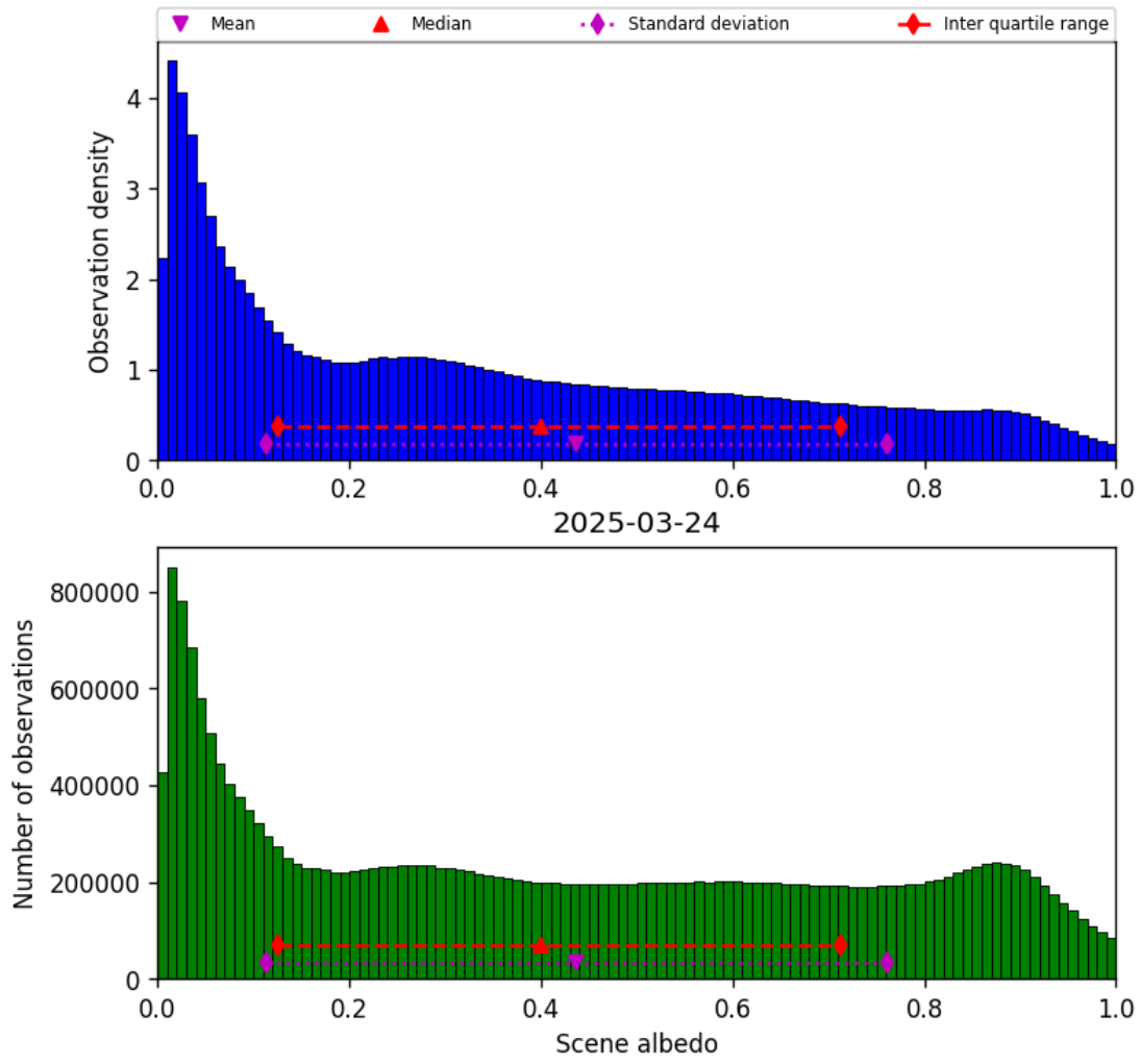
Figure 34: Histogram of “Scene albedo” for 2025-03-23 to 2025-03-25
