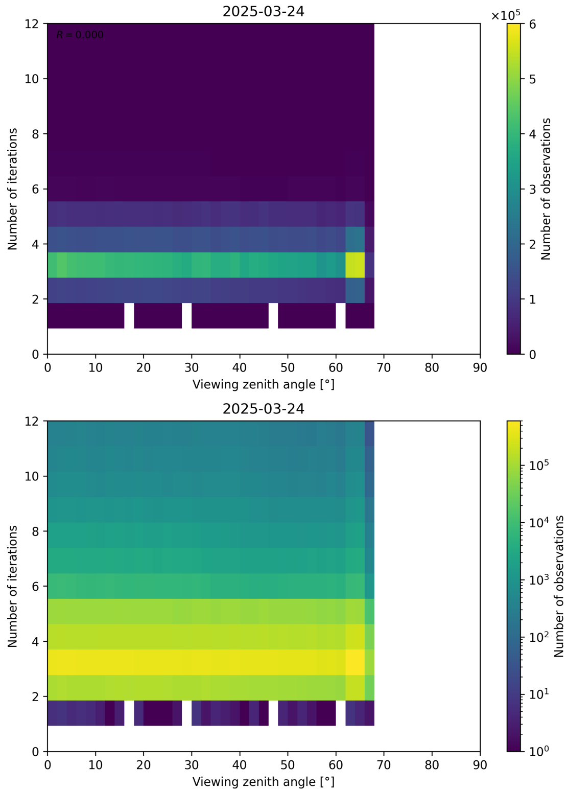
Figure 124: Scatter density plot of “Viewing zenith angle” against “Number of iterations” for 2025-03-23 to 2025-03-25.
