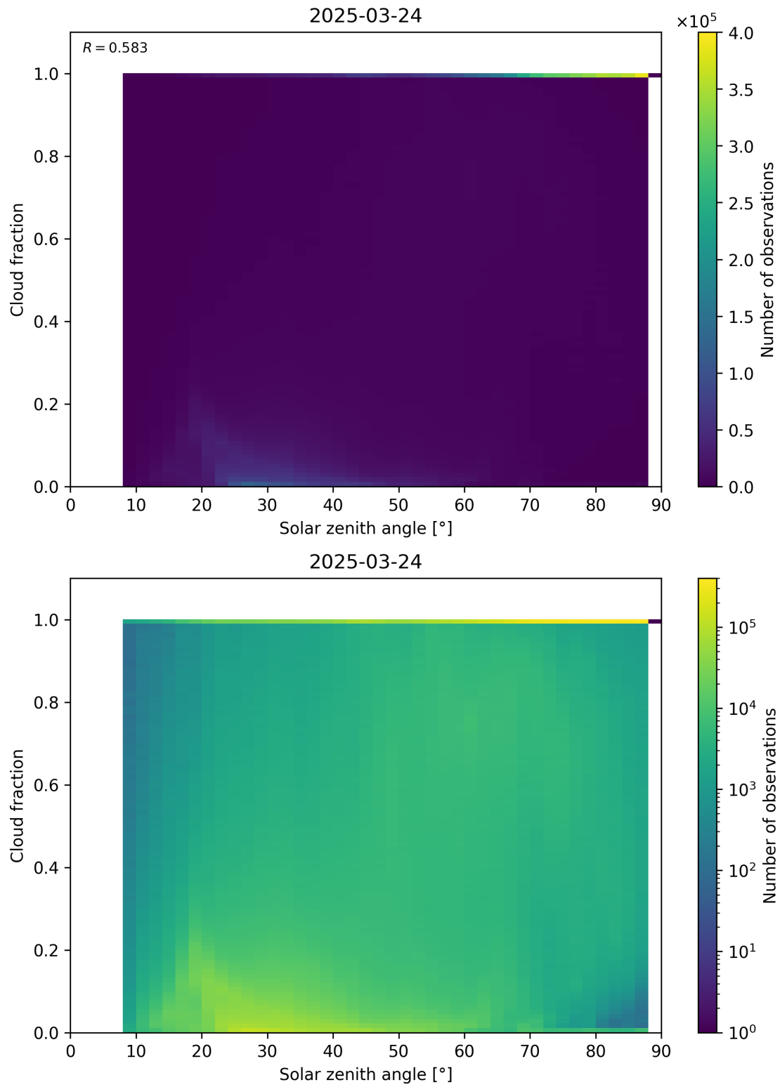
Figure 110: Scatter density plot of “Solar zenith angle” against “Cloud fraction” for 2025-03-23 to 2025-03-25.
