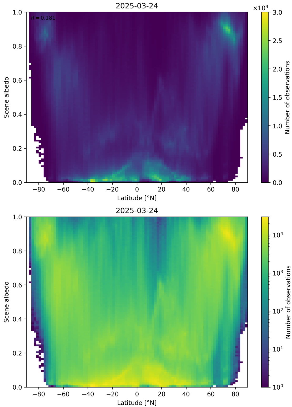
Figure 95: Scatter density plot of “Latitude” against “Scene albedo” for 2025-03-23 to 2025-03-25.
