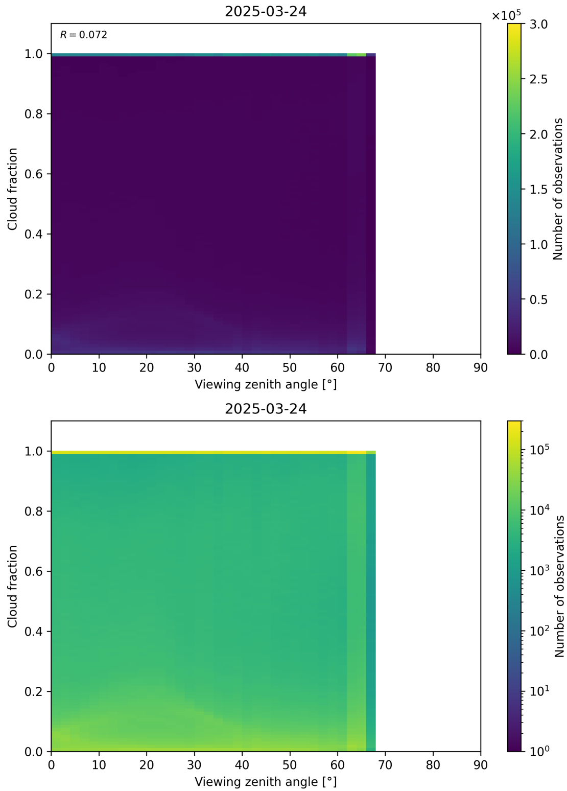
Figure 120: Scatter density plot of “Viewing zenith angle” against “Cloud fraction” for 2025-03-23 to 2025-03-25.
