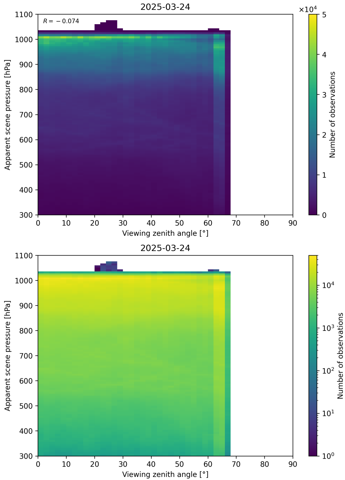
Figure 118: Scatter density plot of “Viewing zenith angle” against “Apparent scene pressure” for 2025-03-23 to 2025-03-25.
