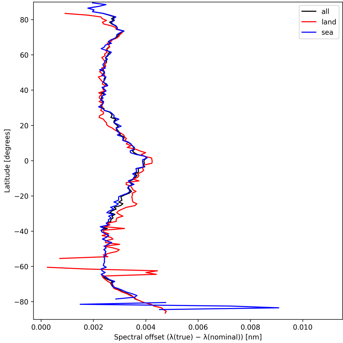
Figure 28: Zonal average of “Spectral offset ( \lambda_{\text{true}} - \lambda_{\text{nominal}} )” for 2025-03-23 to 2025-03-25.
