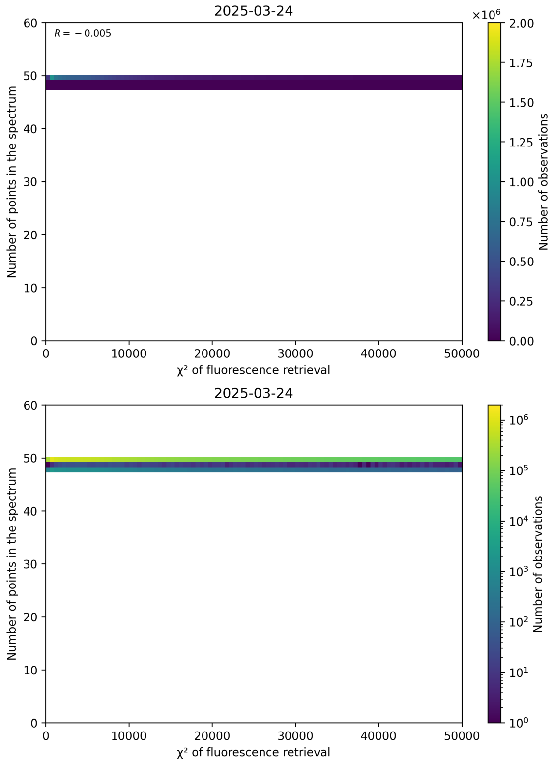
Figure 68: Scatter density plot of " \chi^2 of fluorescence retrieval" against "Number of points in the spectrum" for 2025-03-23 to 2025-03-25.
