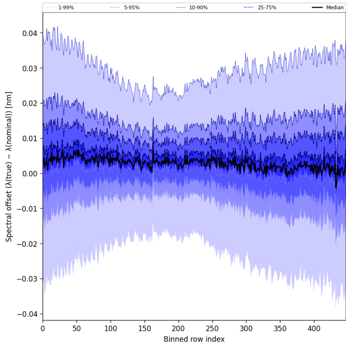
Figure 62: Along track statistics of “Spectral offset ( \lambda_{\text{true}} - \lambda_{\text{nominal}} )” for 2025-03-23 to 2025-03-25
