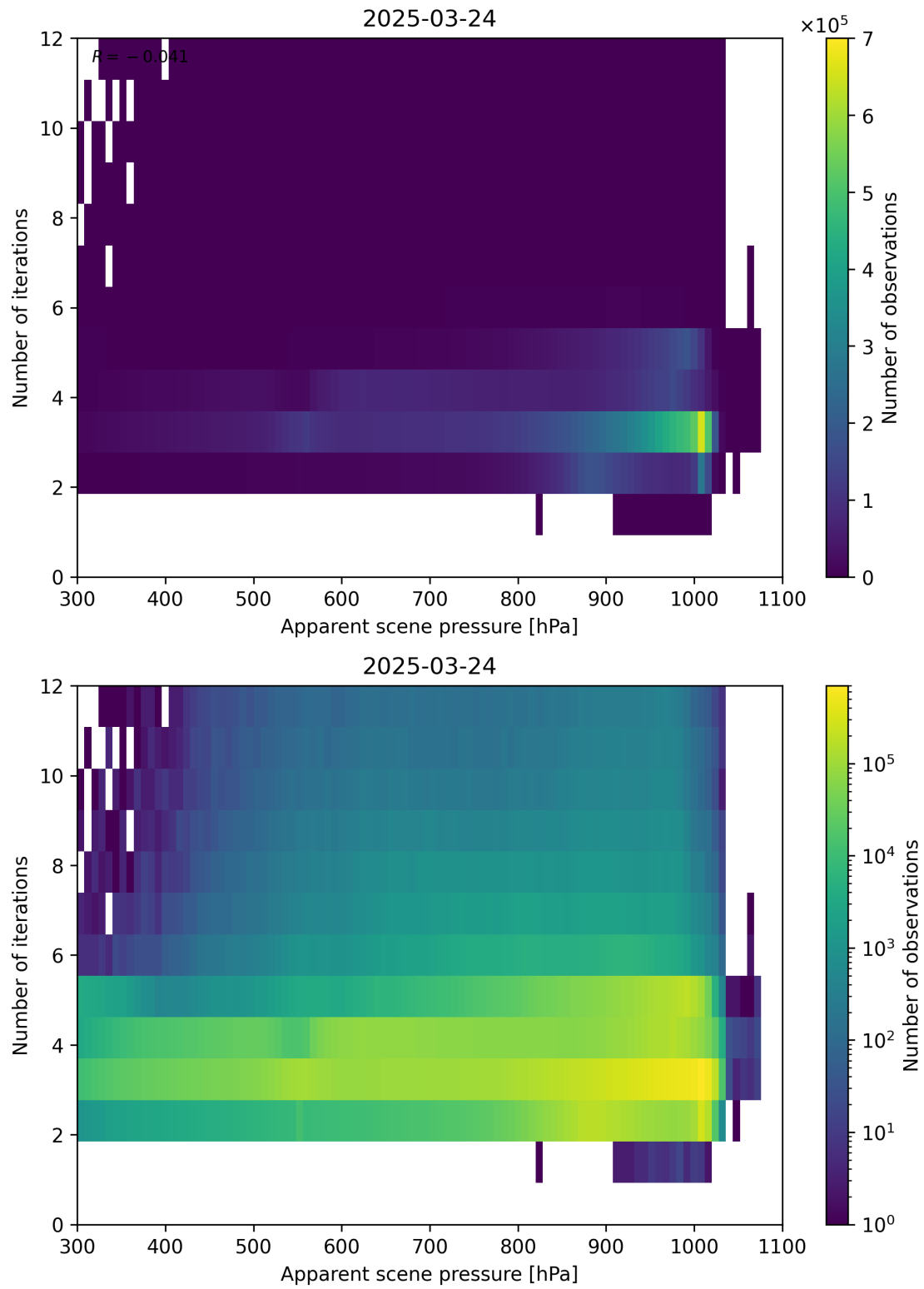
Figure 65: Scatter density plot of “Apparent scene pressure” against “Number of iterations” for 2025-03-23 to 2025-03-25.
