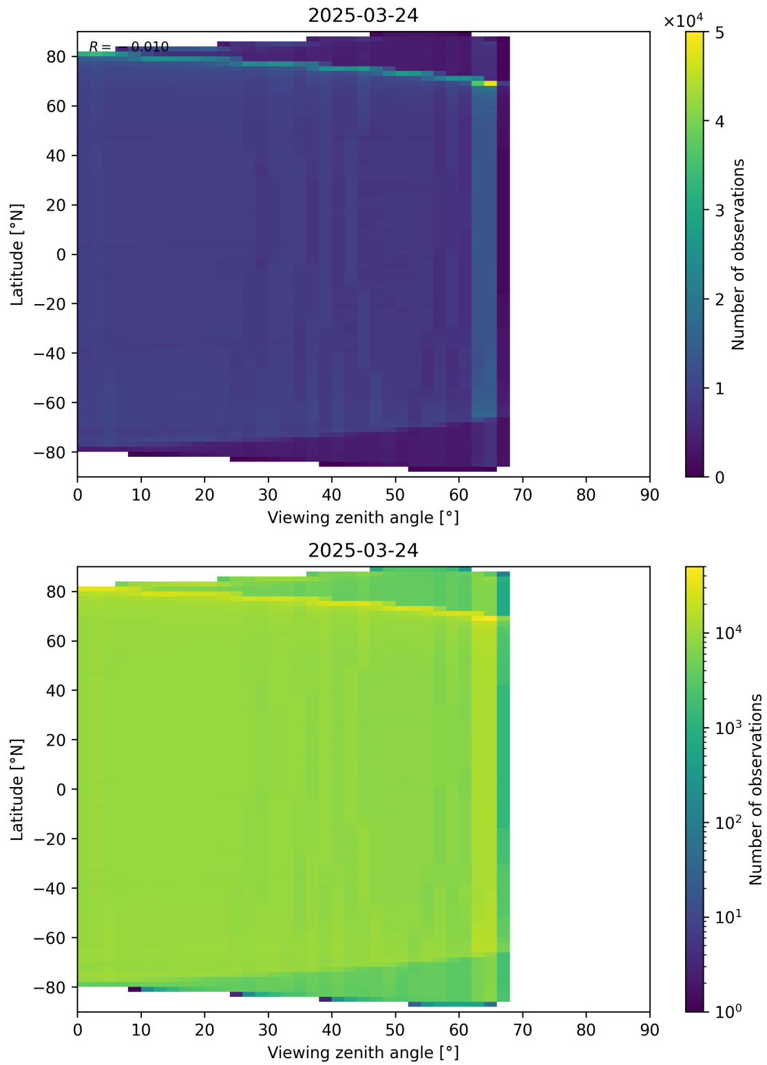
Figure 123: Scatter density plot of “Viewing zenith angle” against “Latitude” for 2025-03-23 to 2025-03-25.
