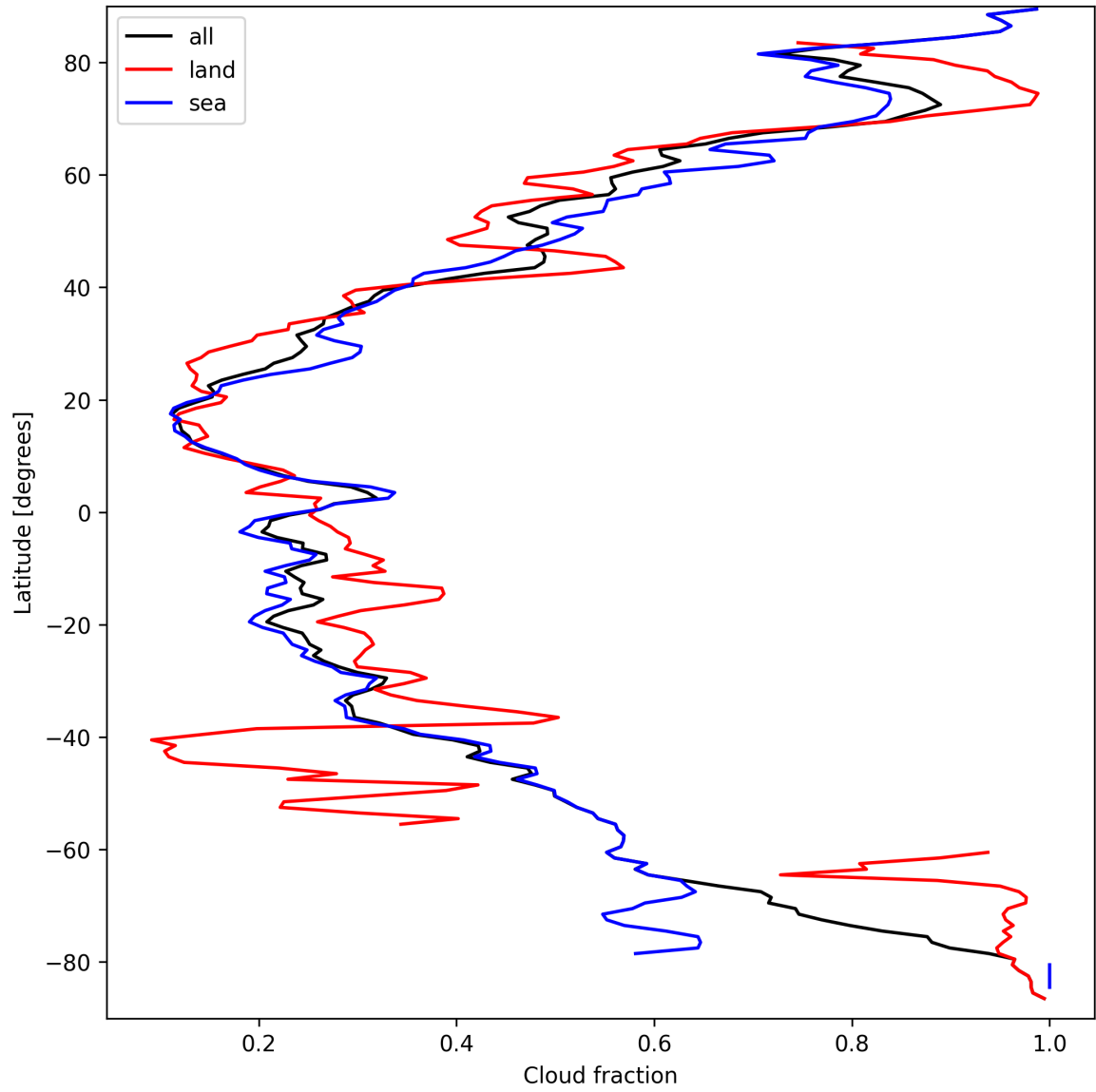
Figure 15: Zonal average of “Cloud fraction” for 2025-03-23 to 2025-03-25.
