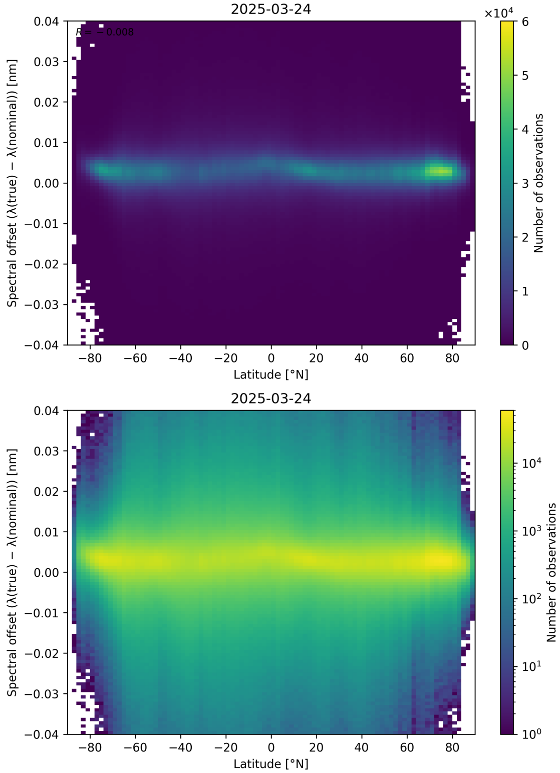
Figure 96: Scatter density plot of “Latitude” against “Spectral offset ( \lambda_{\text{true}} - \lambda_{\text{nominal}} )” for 2025-03-23 to 2025-03-25.
