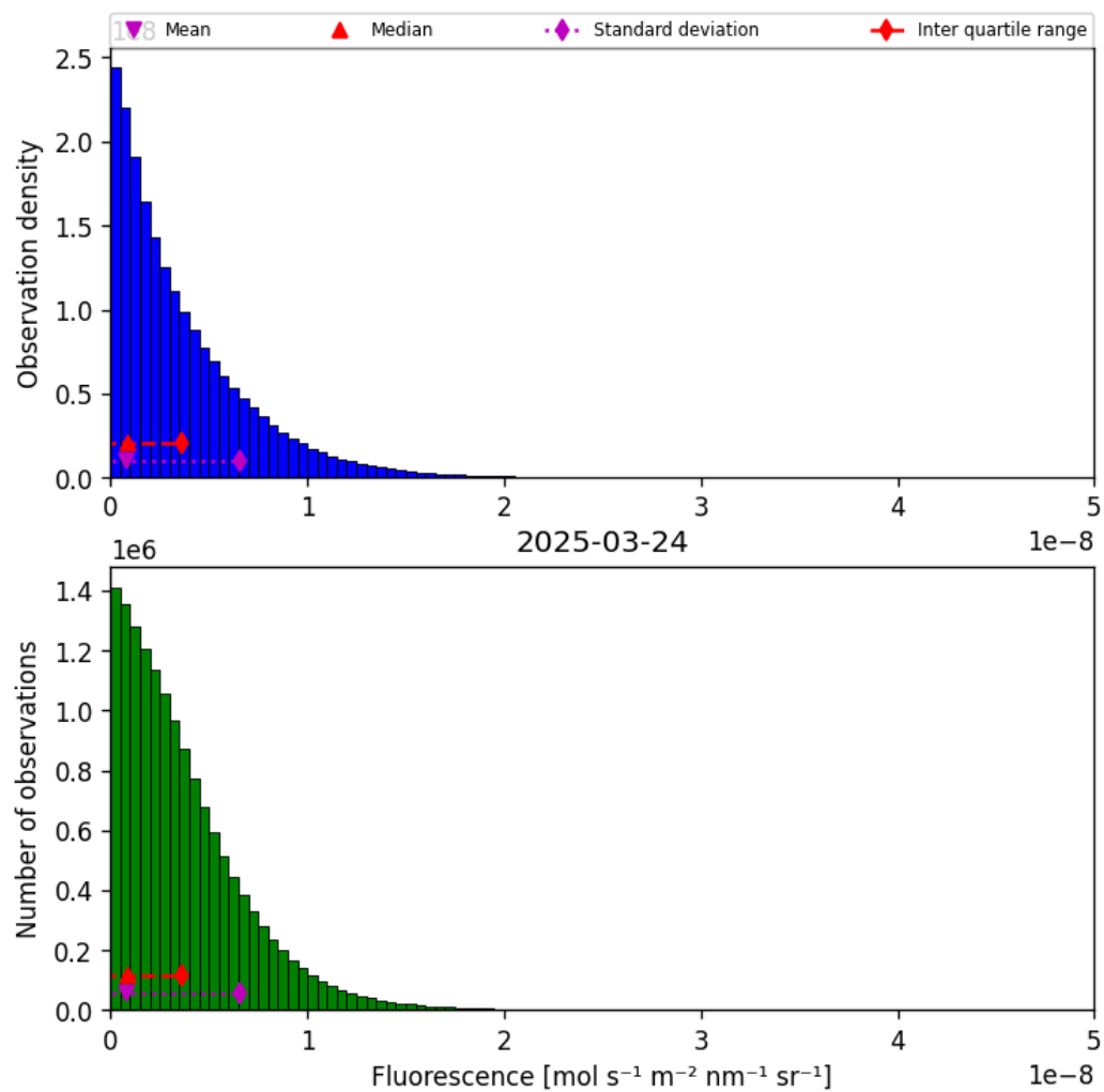
Figure 40: Histogram of “Fluorescence” for 2025-03-23 to 2025-03-25
