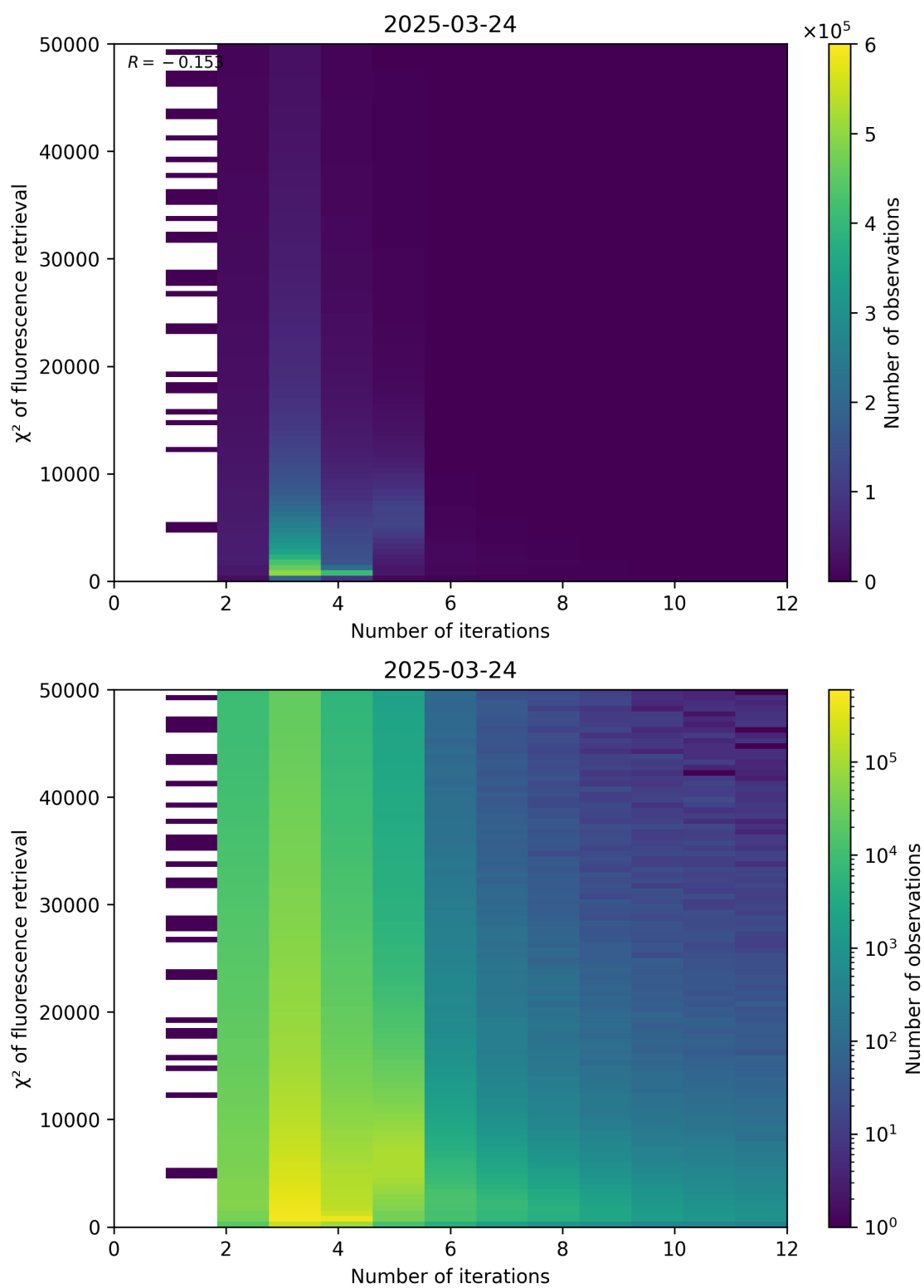
Figure 97: Scatter density plot of “Number of iterations” against “ \chi^2 of fluorescence retrieval” for 2025-03-23 to 2025-03-25.
