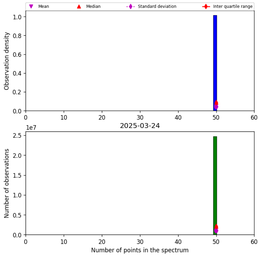
Figure 44: Histogram of “Number of points in the spectrum” for 2025-03-23 to 2025-03-25
