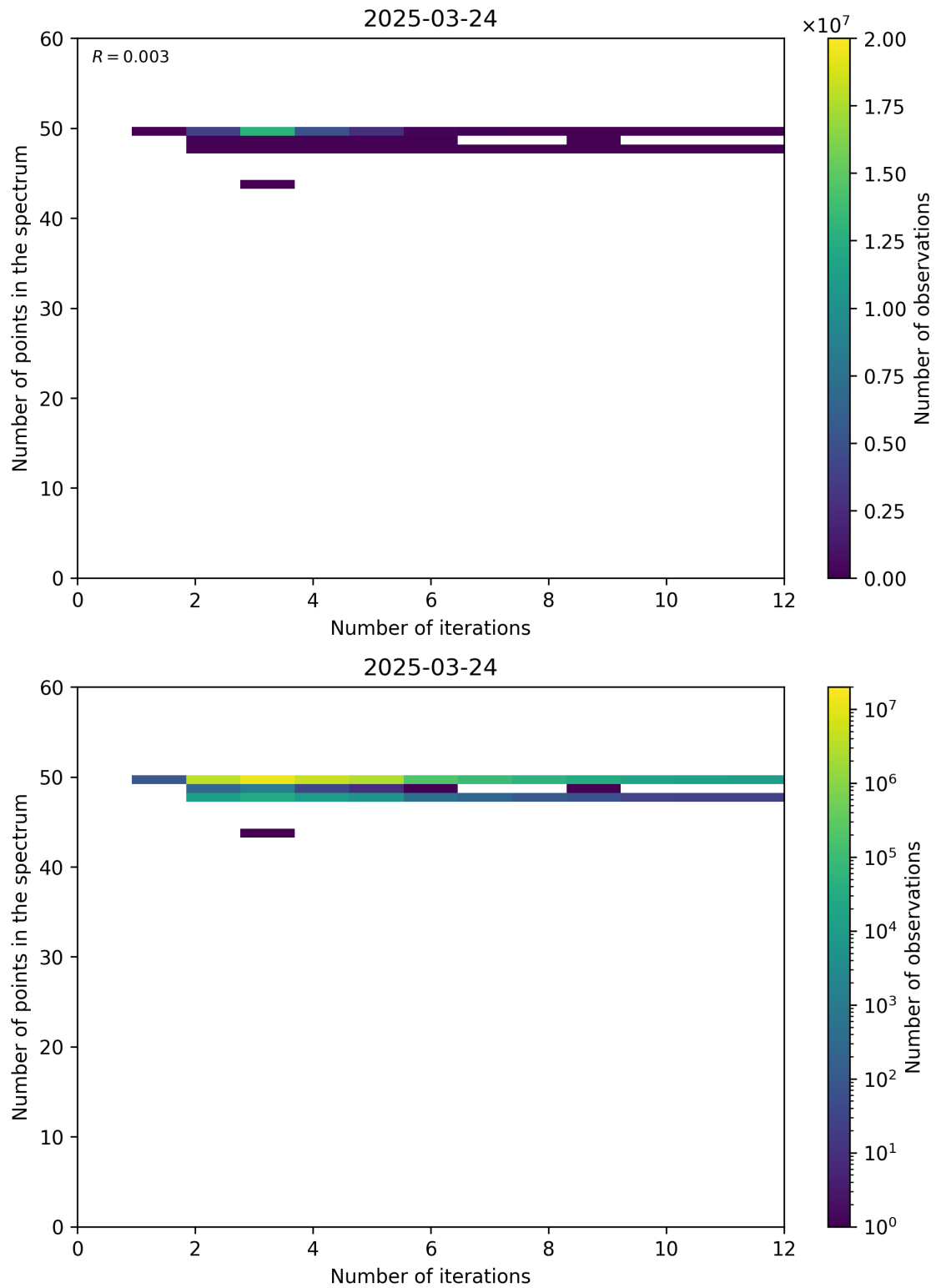
Figure 99: Scatter density plot of “Number of iterations” against “Number of points in the spectrum” for 2025-03-23 to 2025-03-25.
