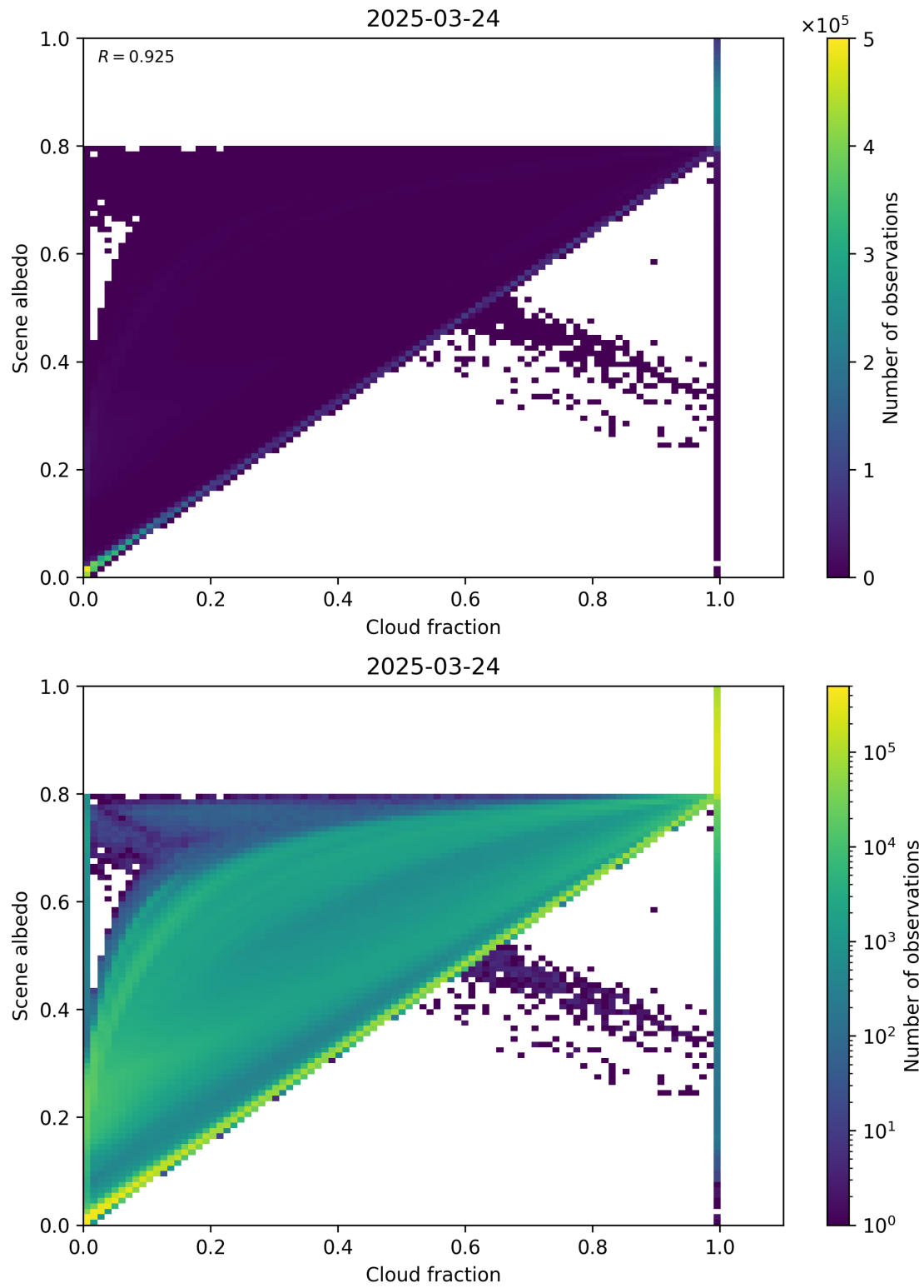
Figure 75: Scatter density plot of “Cloud fraction” against “Scene albedo” for 2025-03-23 to 2025-03-25.
