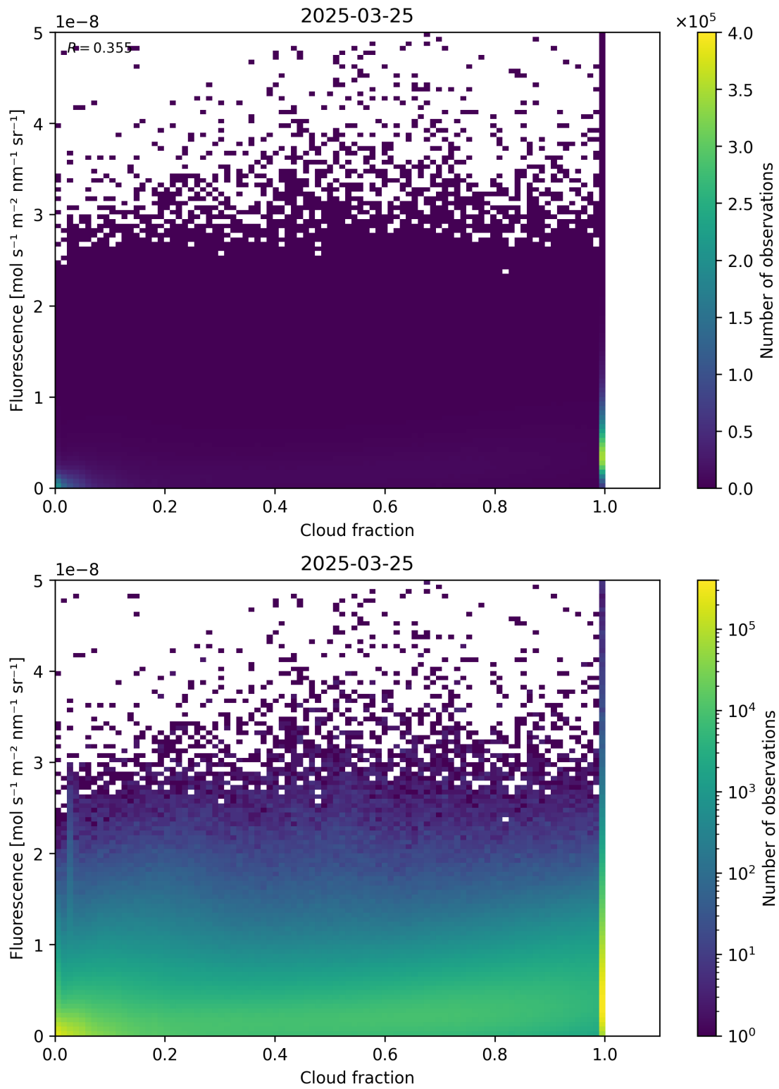
Figure 72: Scatter density plot of “Cloud fraction” against “Fluorescence” for 2025-03-24 to 2025-03-26.
