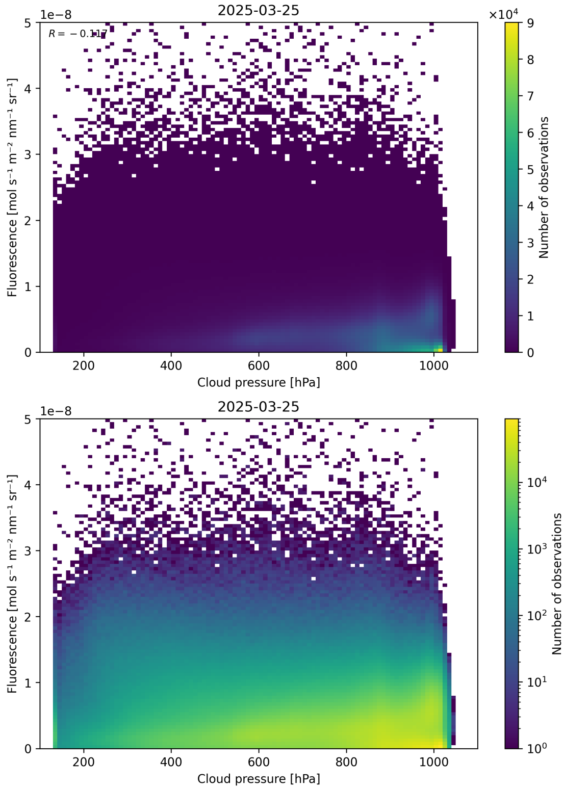
Figure 80: Scatter density plot of “Cloud pressure” against “Fluorescence” for 2025-03-24 to 2025-03-26.
