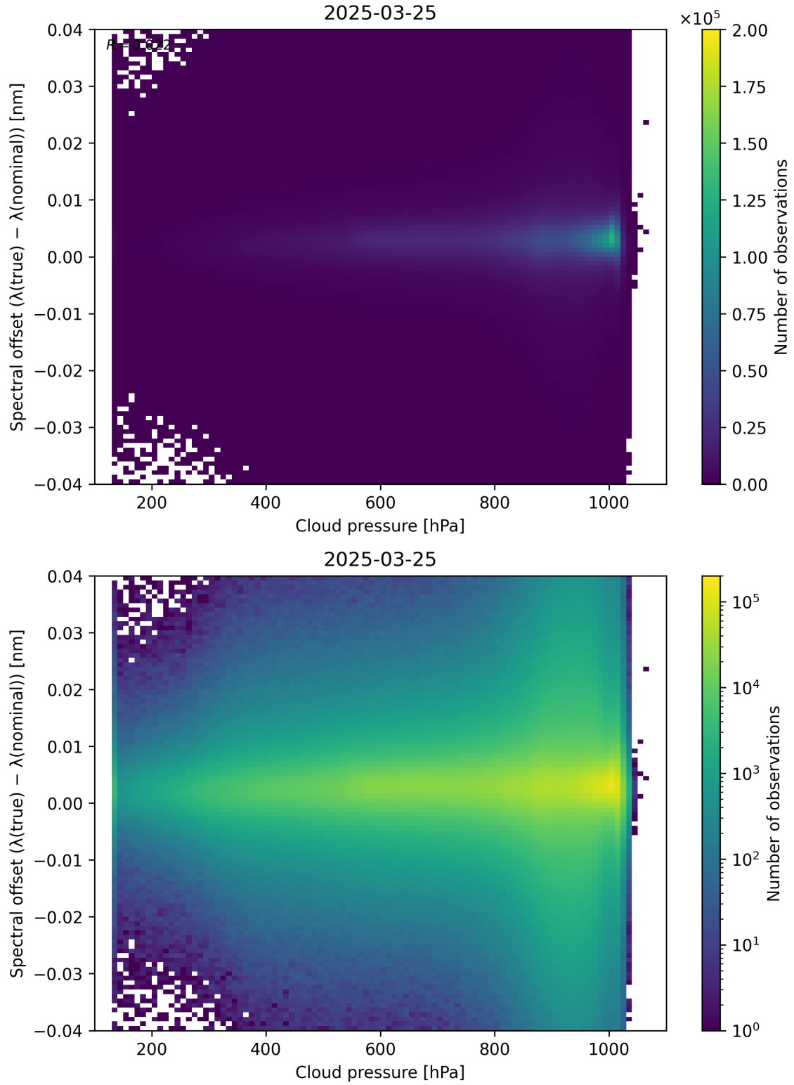
Figure 84: Scatter density plot of “Cloud pressure” against “Spectral offset ( \lambda_{\text{true}} - \lambda_{\text{nominal}} )” for 2025-03-24 to 2025-03-26.
