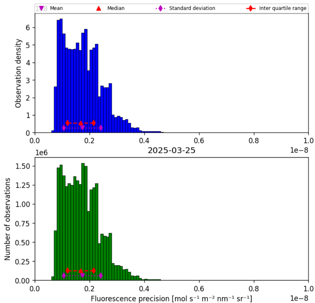
Figure 41: Histogram of “Fluorescence precision” for 2025-03-24 to 2025-03-26
