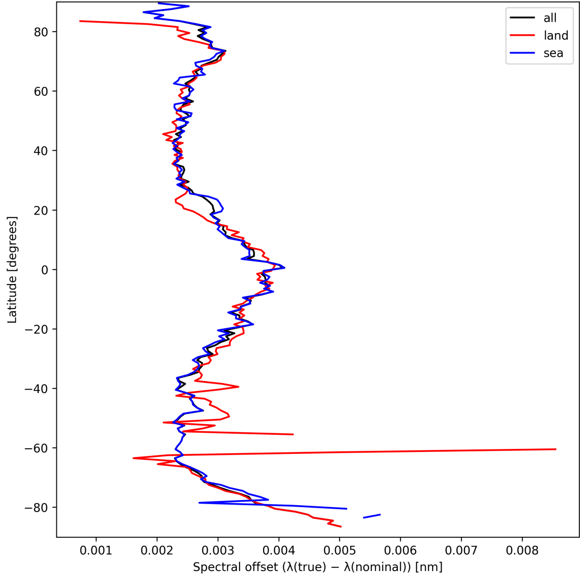
Figure 28: Zonal average of “Spectral offset ( \lambda_{\text{true}} - \lambda_{\text{nominal}} )” for 2025-03-24 to 2025-03-26.
