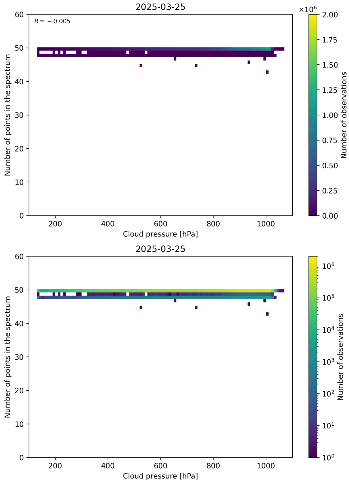
Figure 82: Scatter density plot of “Cloud pressure” against “Number of points in the spectrum” for 2025-03-24 to 2025-03-26.
