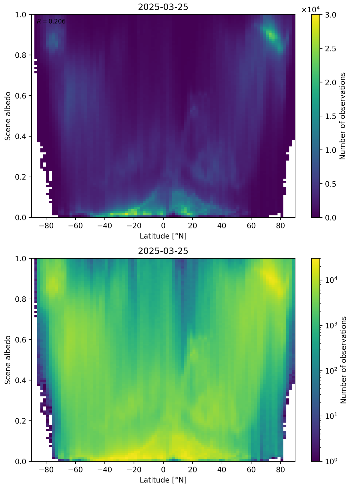
Figure 95: Scatter density plot of “Latitude” against “Scene albedo” for 2025-03-24 to 2025-03-26.
