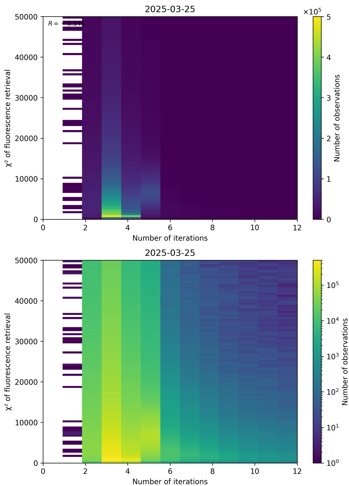
Figure 97: Scatter density plot of “Number of iterations” against “ \chi^2 of fluorescence retrieval” for 2025-03-24 to 2025-03-26.
