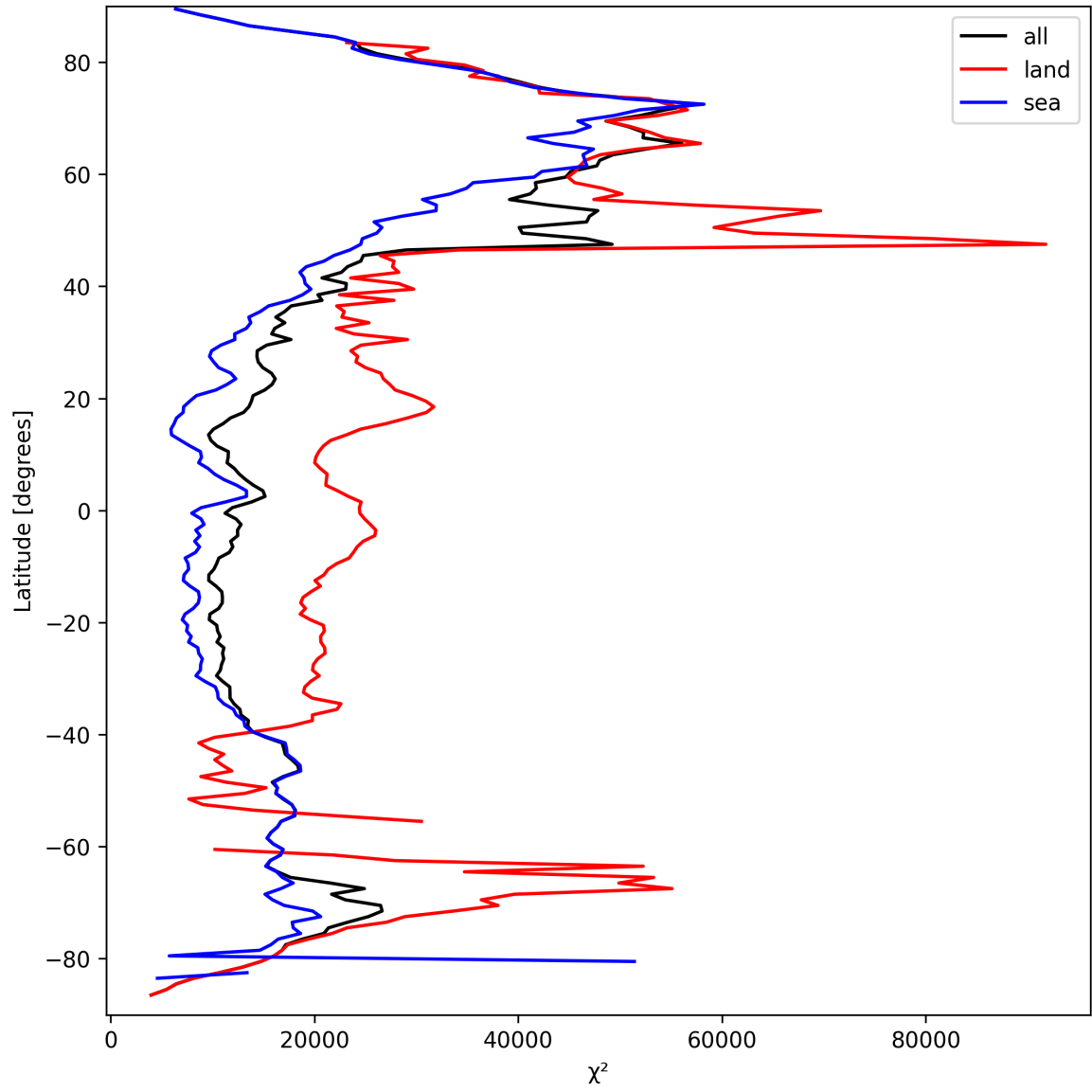
Figure 21: Zonal average of “ \chi^2 ” for 2025-03-24 to 2025-03-26.
