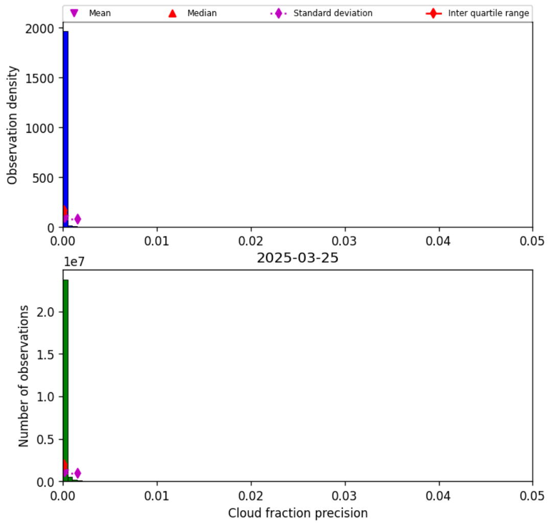
Figure 33: Histogram of “Cloud fraction precision” for 2025-03-24 to 2025-03-26
