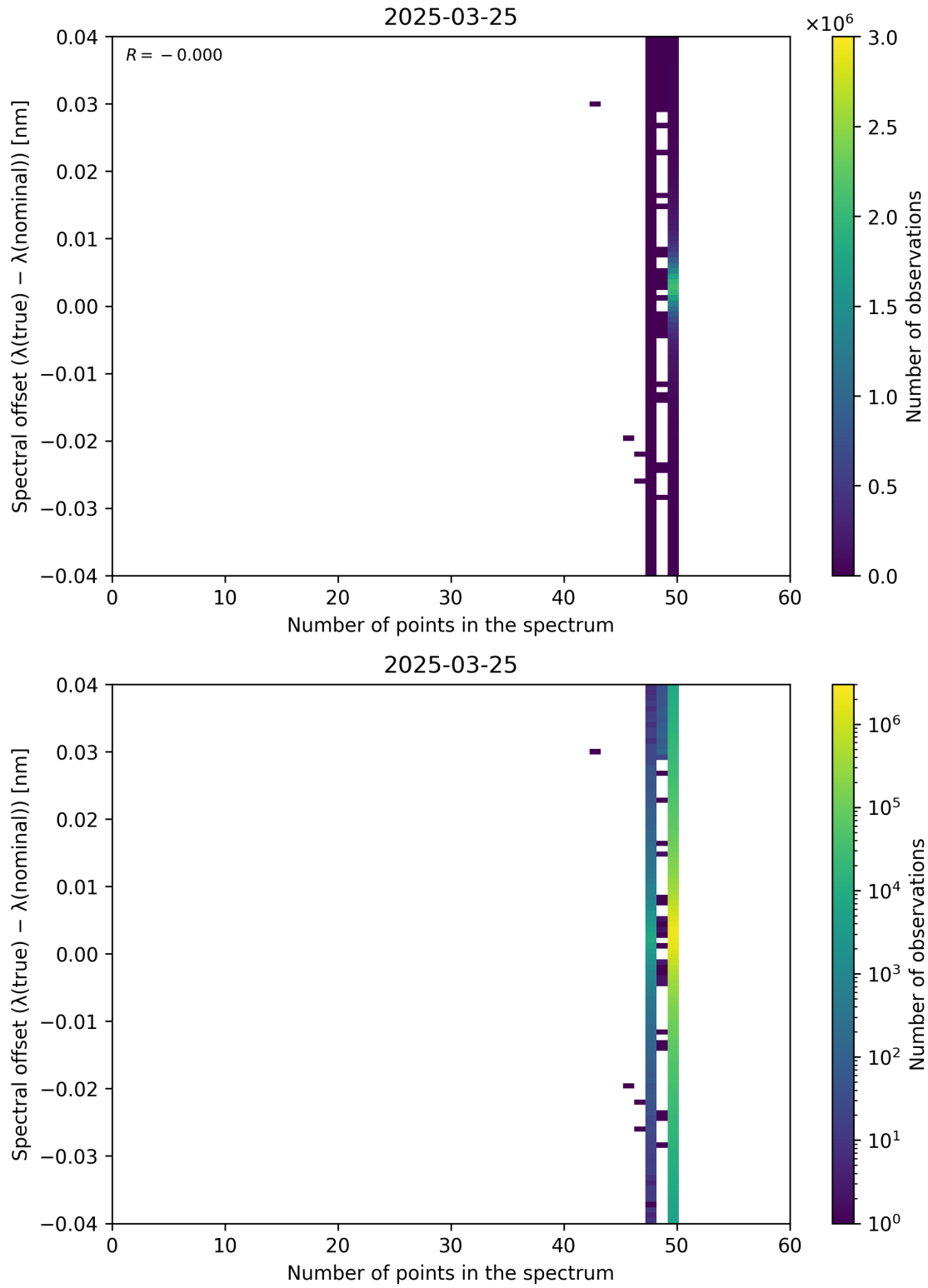
Figure 101: Scatter density plot of “Number of points in the spectrum” against “Spectral offset ( \lambda_{\text{true}} - \lambda_{\text{nominal}} )” for 2025-03-24 to 2025-03-26.
