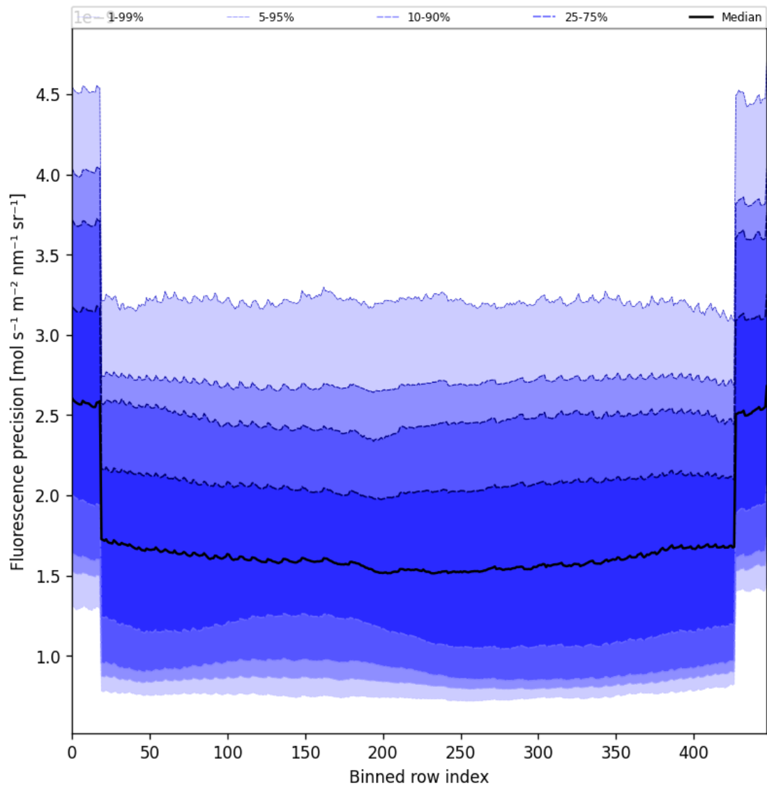
Figure 58: Along track statistics of “Fluorescence precision” for 2025-03-24 to 2025-03-26
