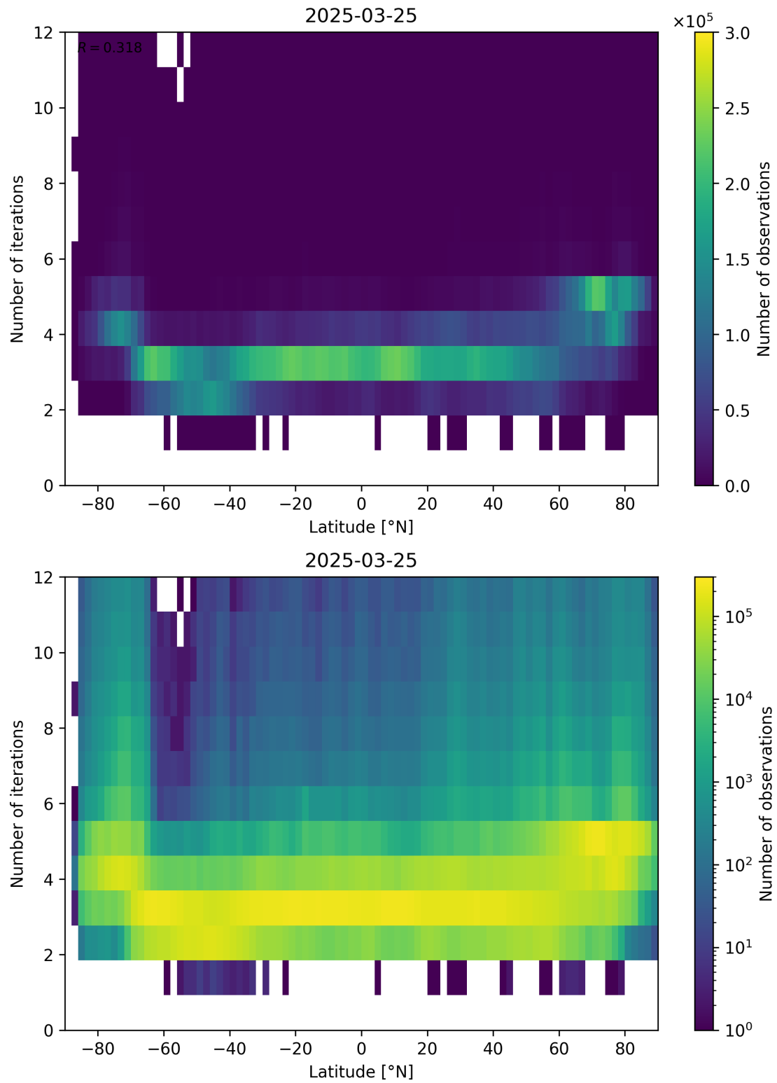
Figure 93: Scatter density plot of “Latitude” against “Number of iterations” for 2025-03-24 to 2025-03-26.
