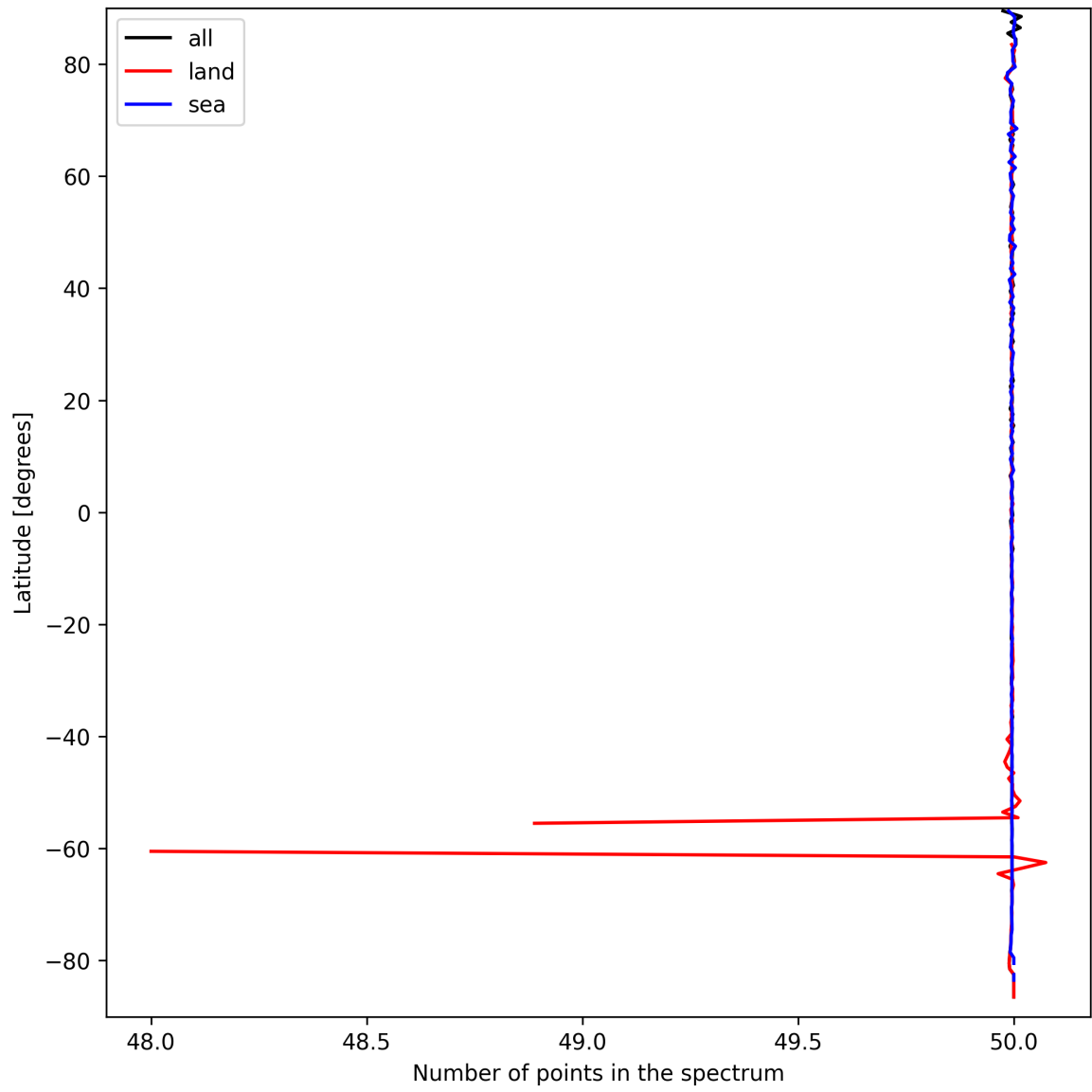
Figure 27: Zonal average of “Number of points in the spectrum” for 2025-03-24 to 2025-03-26.
