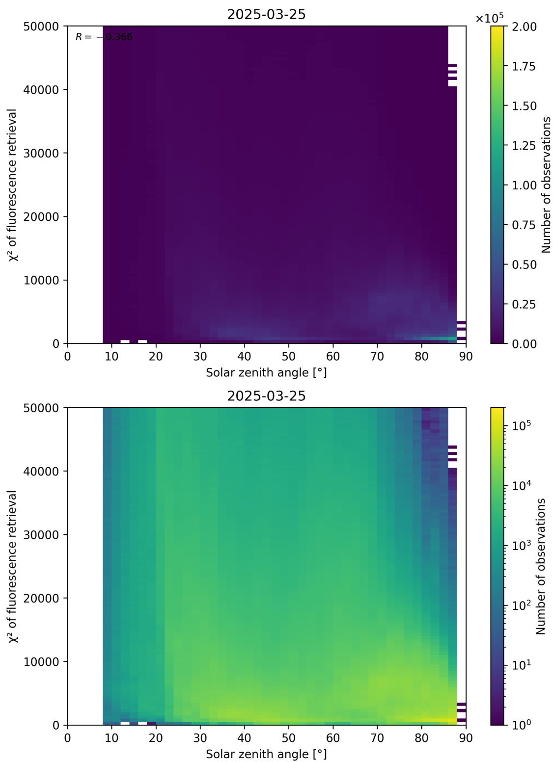
Figure 109: Scatter density plot of “Solar zenith angle” against “ \chi^2 of fluorescence retrieval” for 2025-03-24 to 2025-03-26.
