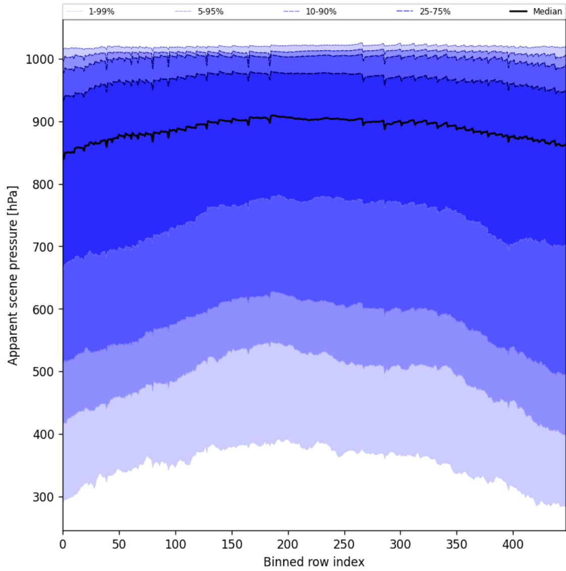
Figure 53: Along track statistics of “Apparent scene pressure” for 2025-03-24 to 2025-03-26
