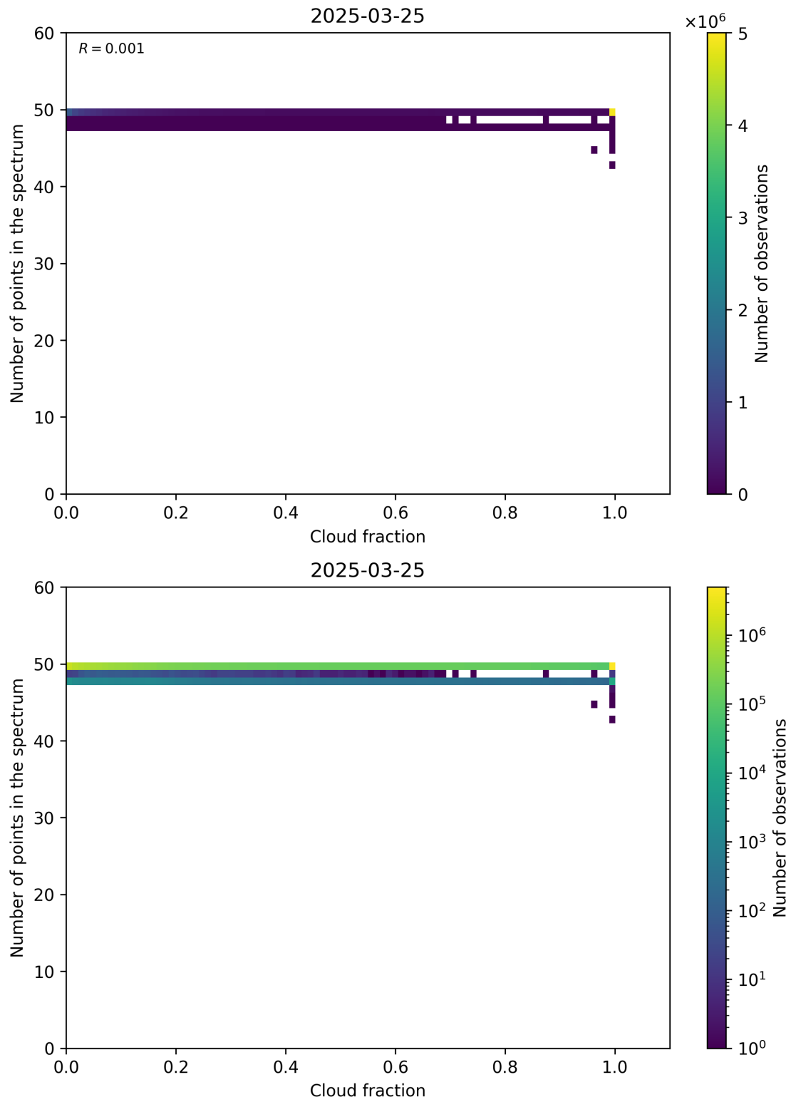
Figure 74: Scatter density plot of “Cloud fraction” against “Number of points in the spectrum” for 2025-03-24 to 2025-03-26.
