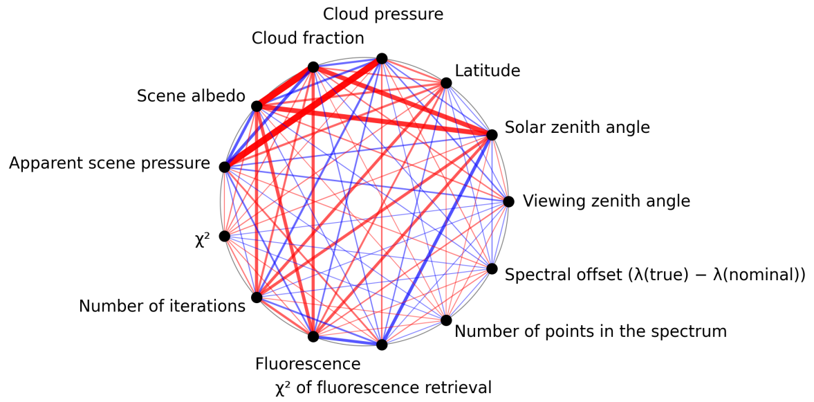
Figure 1: Map of correlation graph for 2025-03-24 to 2025-03-26.
