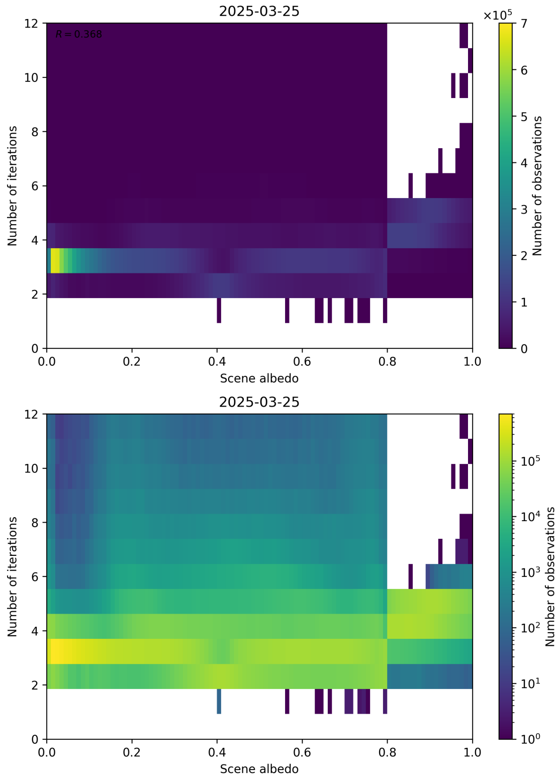
Figure 105: Scatter density plot of “Scene albedo” against “Number of iterations” for 2025-03-24 to 2025-03-26.
