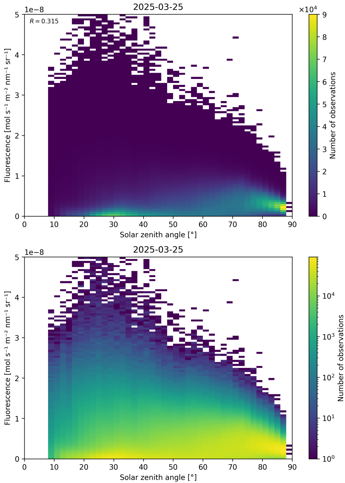
Figure 112: Scatter density plot of “Solar zenith angle” against “Fluorescence” for 2025-03-24 to 2025-03-26.
