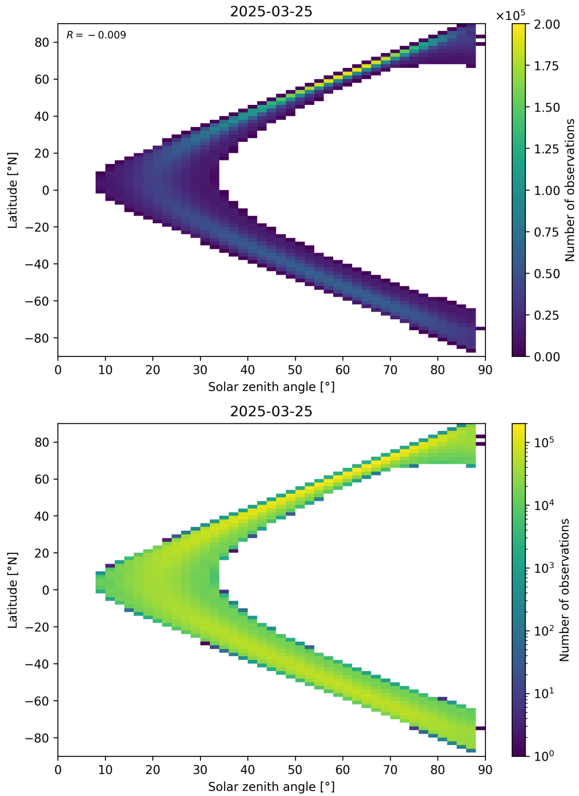
Figure 113: Scatter density plot of “Solar zenith angle” against “Latitude” for 2025-03-24 to 2025-03-26.
