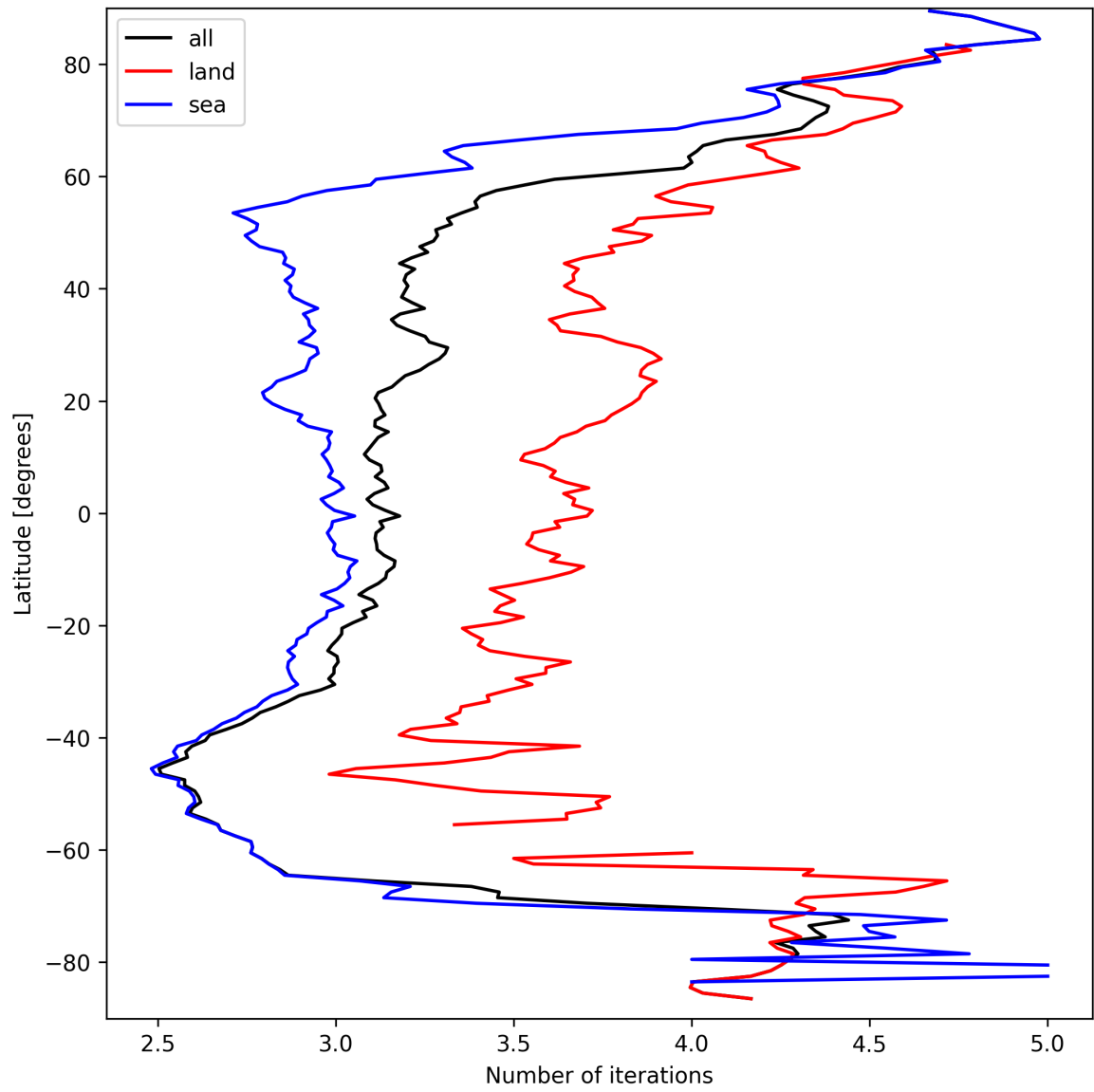
Figure 22: Zonal average of “Number of iterations” for 2025-03-24 to 2025-03-26.
