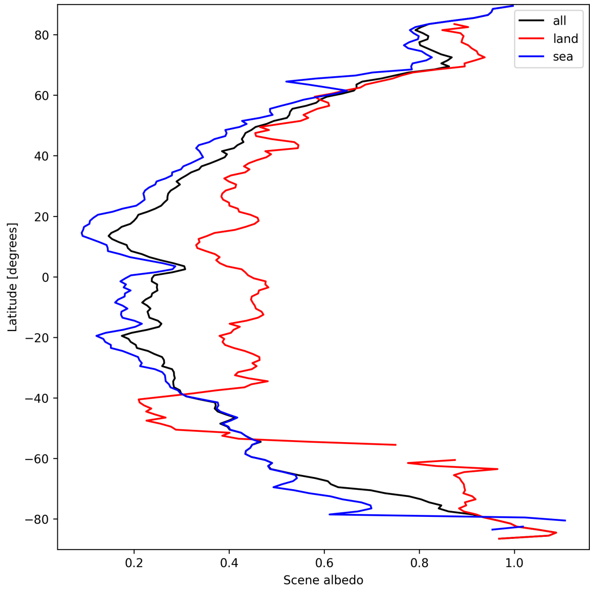
Figure 17: Zonal average of “Scene albedo” for 2025-03-24 to 2025-03-26.
