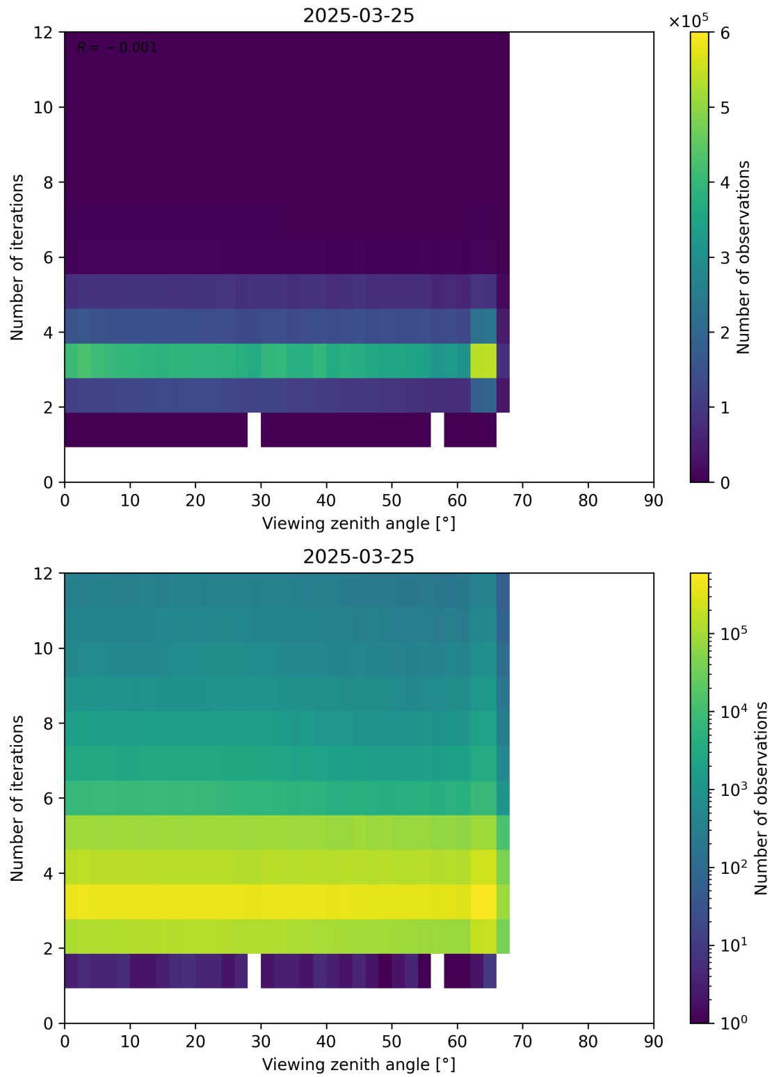
Figure 124: Scatter density plot of “Viewing zenith angle” against “Number of iterations” for 2025-03-24 to 2025-03-26.
