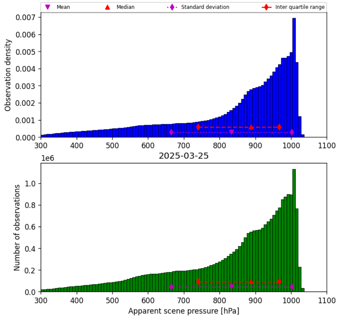
Figure 36: Histogram of “Apparent scene pressure” for 2025-03-24 to 2025-03-26
