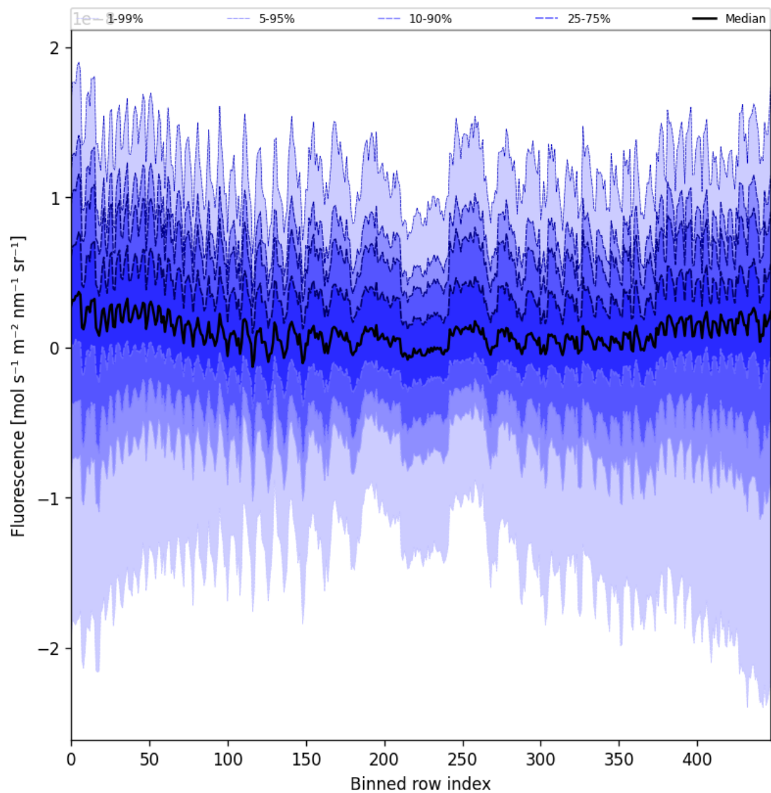
Figure 57: Along track statistics of “Fluorescence” for 2025-03-24 to 2025-03-26
