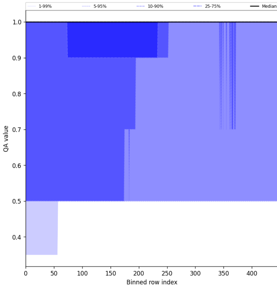
Figure 46: Along track statistics of “QA value” for 2025-03-24 to 2025-03-26
