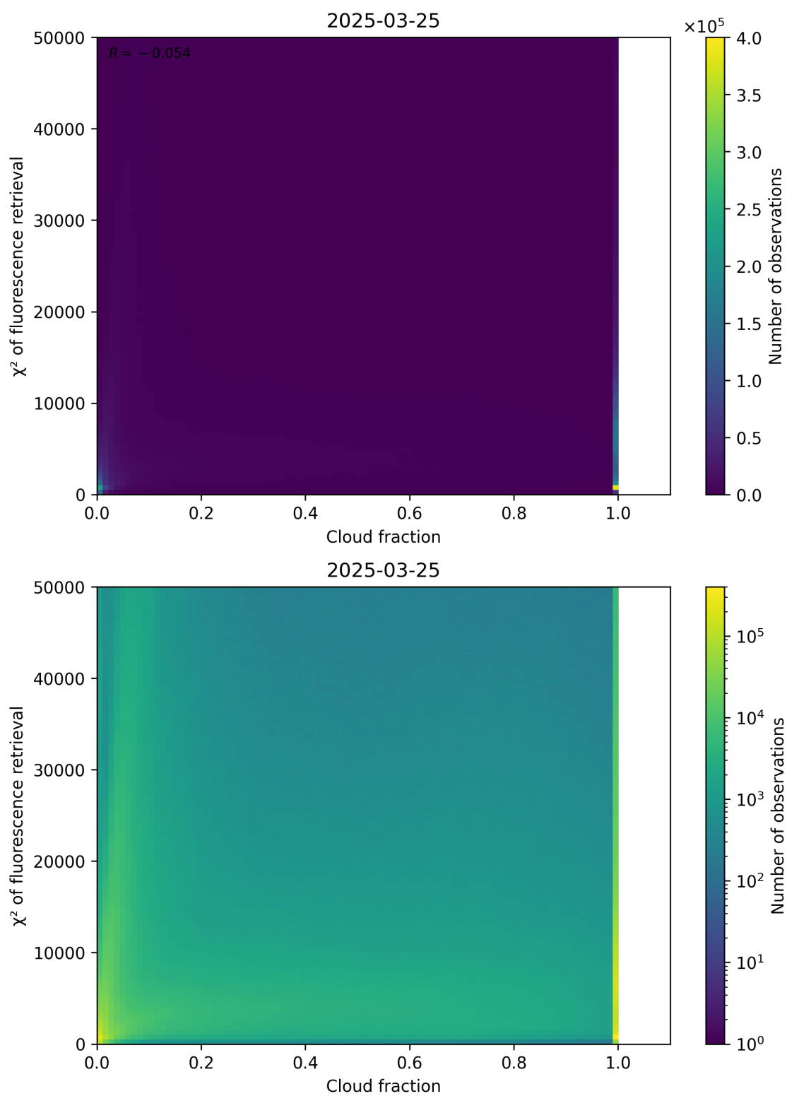
Figure 71: Scatter density plot of “Cloud fraction” against “ \chi^2 of fluorescence retrieval” for 2025-03-24 to 2025-03-26.
