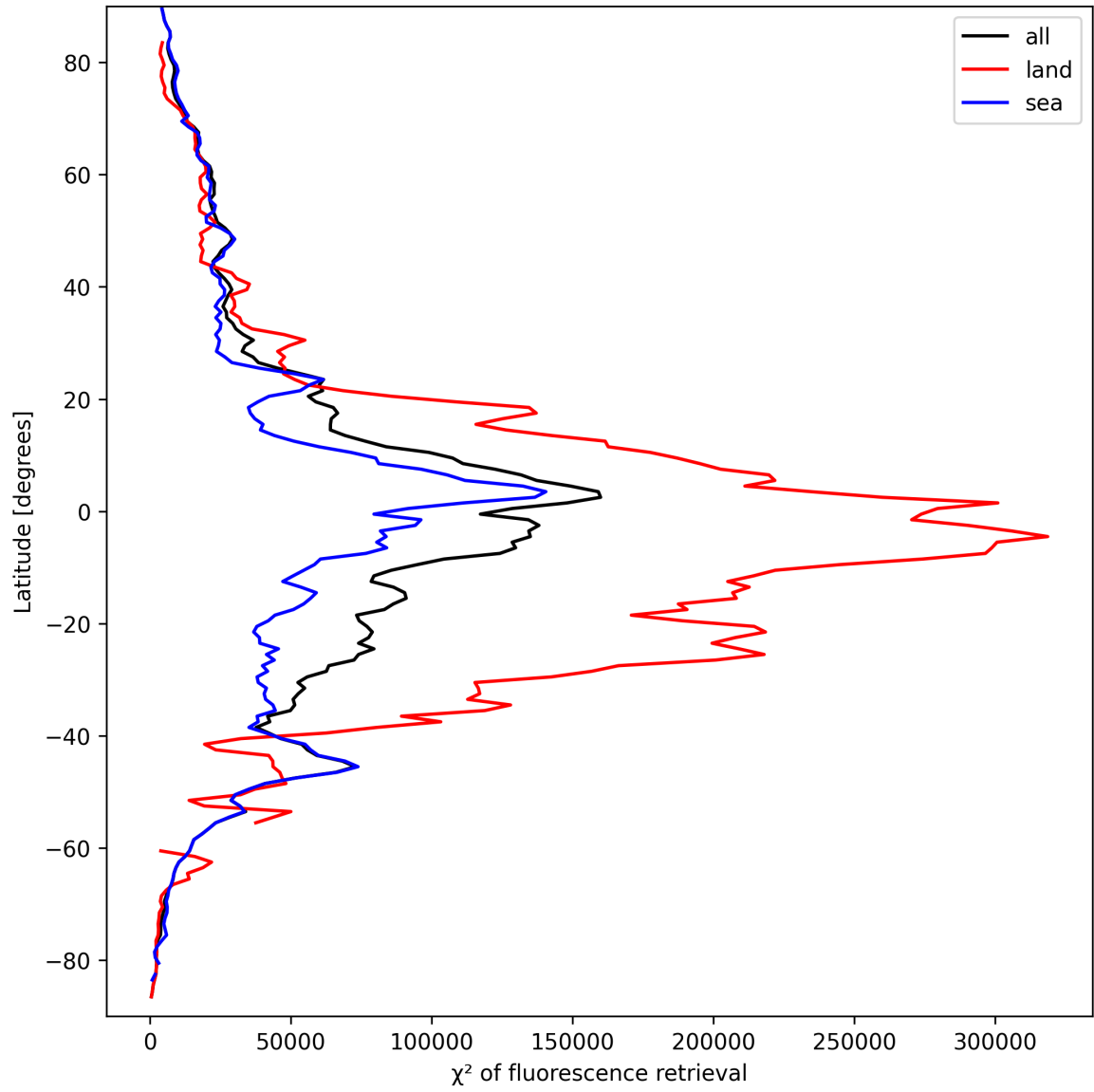
Figure 25: Zonal average of “ \chi^2 of fluorescence retrieval” for 2025-03-24 to 2025-03-26.
