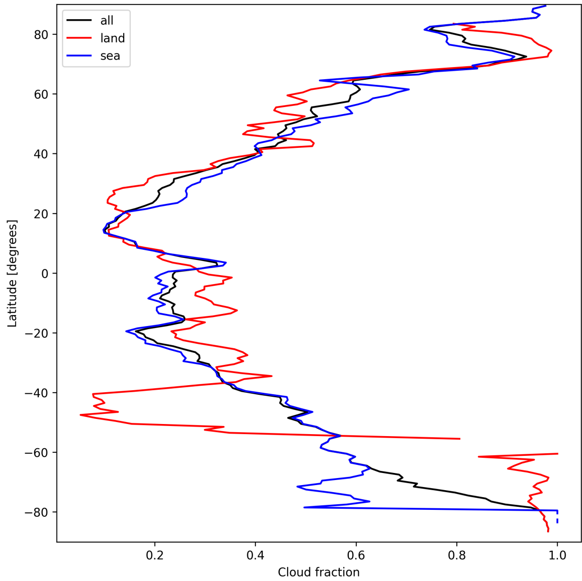
Figure 15: Zonal average of “Cloud fraction” for 2025-03-24 to 2025-03-26.
