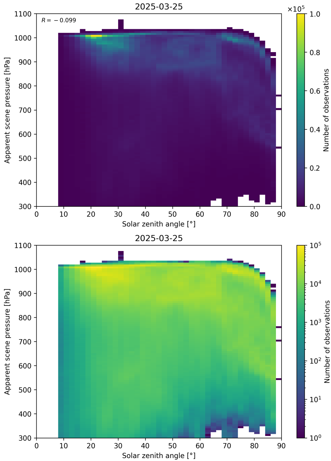
Figure 108: Scatter density plot of “Solar zenith angle” against “Apparent scene pressure” for 2025-03-24 to 2025-03-26.
