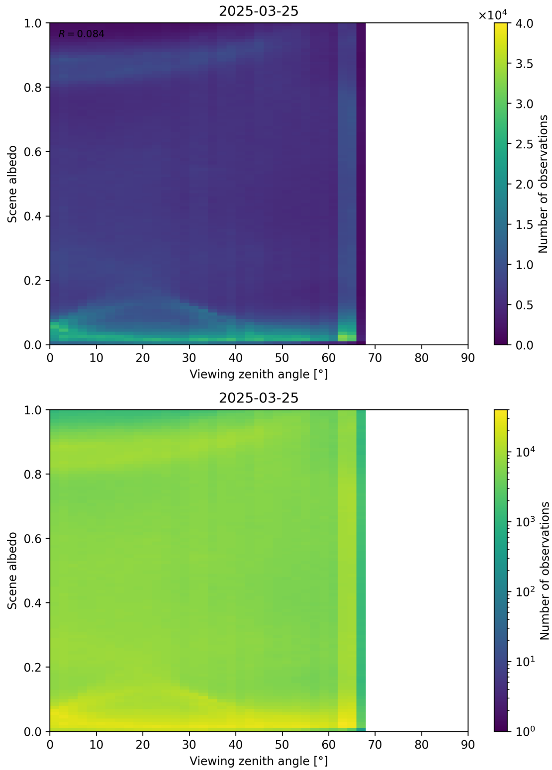
Figure 126: Scatter density plot of “Viewing zenith angle” against “Scene albedo” for 2025-03-24 to 2025-03-26.
