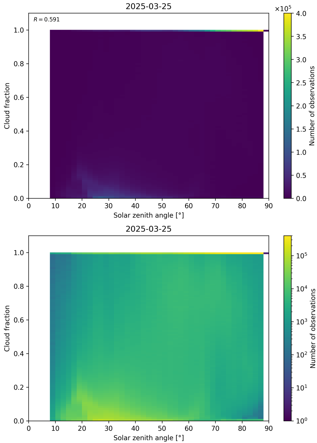
Figure 110: Scatter density plot of “Solar zenith angle” against “Cloud fraction” for 2025-03-24 to 2025-03-26.
