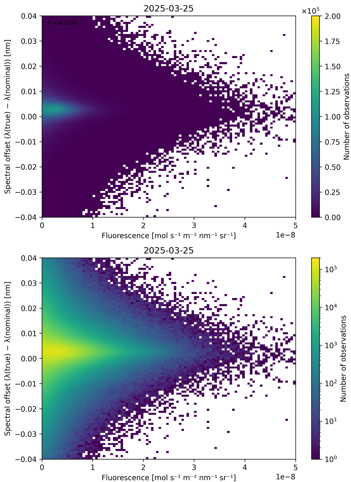
Figure 87: Scatter density plot of “Fluorescence” against “Spectral offset ( \lambda_{\text{true}} - \lambda_{\text{nominal}} )” for 2025-03-24 to 2025-03-26.
