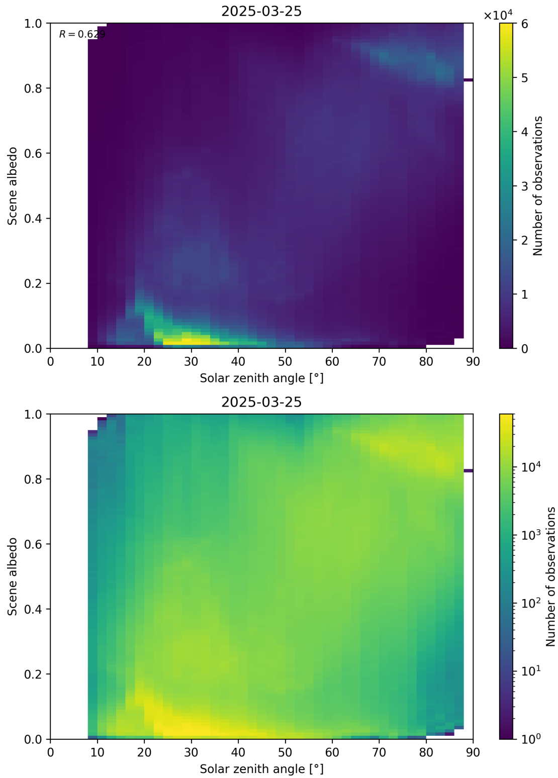
Figure 116: Scatter density plot of “Solar zenith angle” against “Scene albedo” for 2025-03-24 to 2025-03-26.
