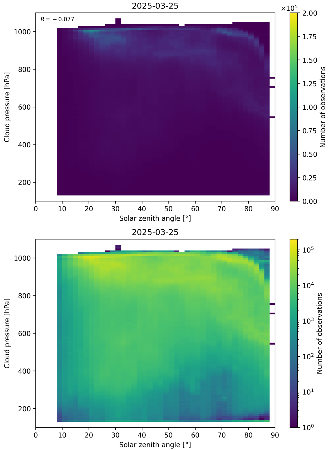
Figure 111: Scatter density plot of “Solar zenith angle” against “Cloud pressure” for 2025-03-24 to 2025-03-26.
