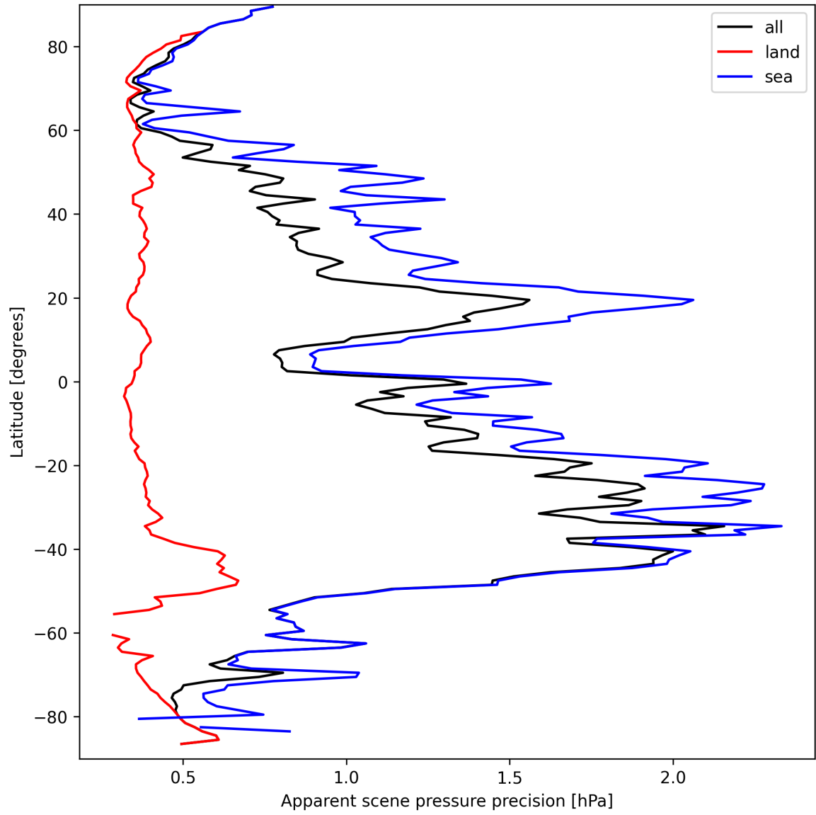
Figure 20: Zonal average of “Apparent scene pressure precision” for 2025-03-24 to 2025-03-26.
