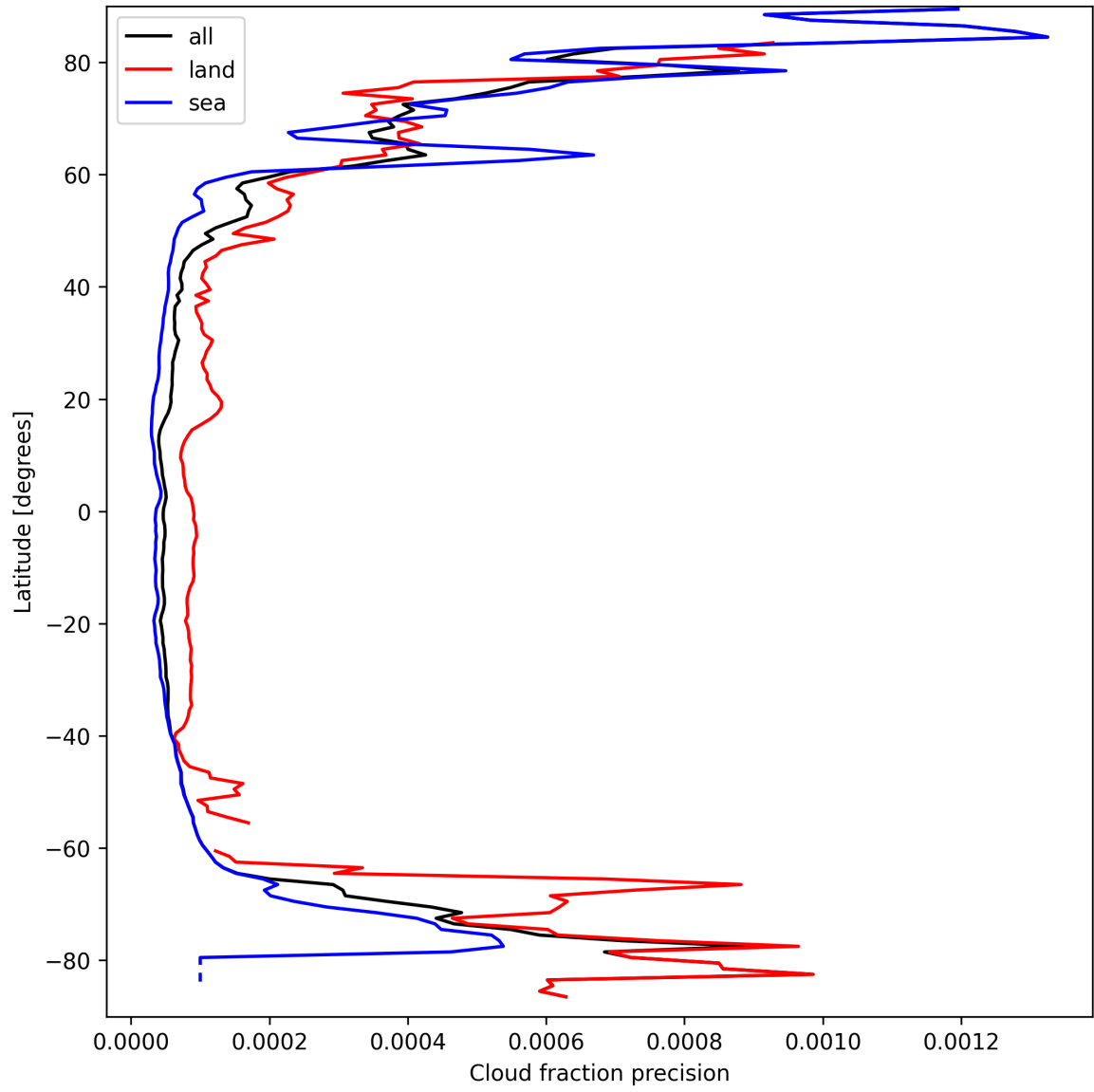
Figure 16: Zonal average of “Cloud fraction precision” for 2025-03-24 to 2025-03-26.
