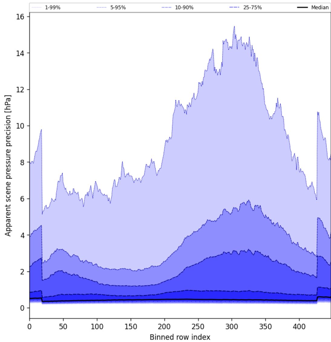
Figure 54: Along track statistics of “Apparent scene pressure precision” for 2025-03-24 to 2025-03-26
