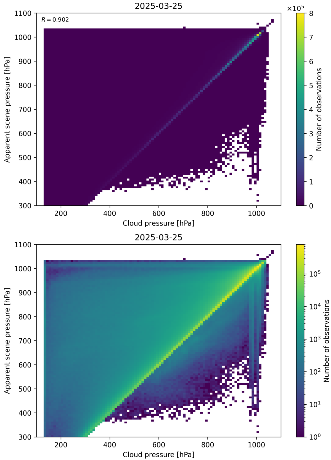
Figure 77: Scatter density plot of “Cloud pressure” against “Apparent scene pressure” for 2025-03-24 to 2025-03-26.
