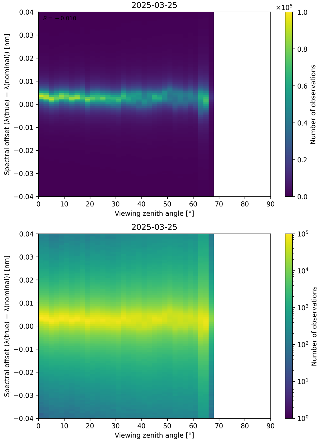
Figure 128: Scatter density plot of “Viewing zenith angle” against “Spectral offset ( \lambda_{\text{true}} - \lambda_{\text{nominal}} )” for 2025-03-24 to 2025-03-26.
