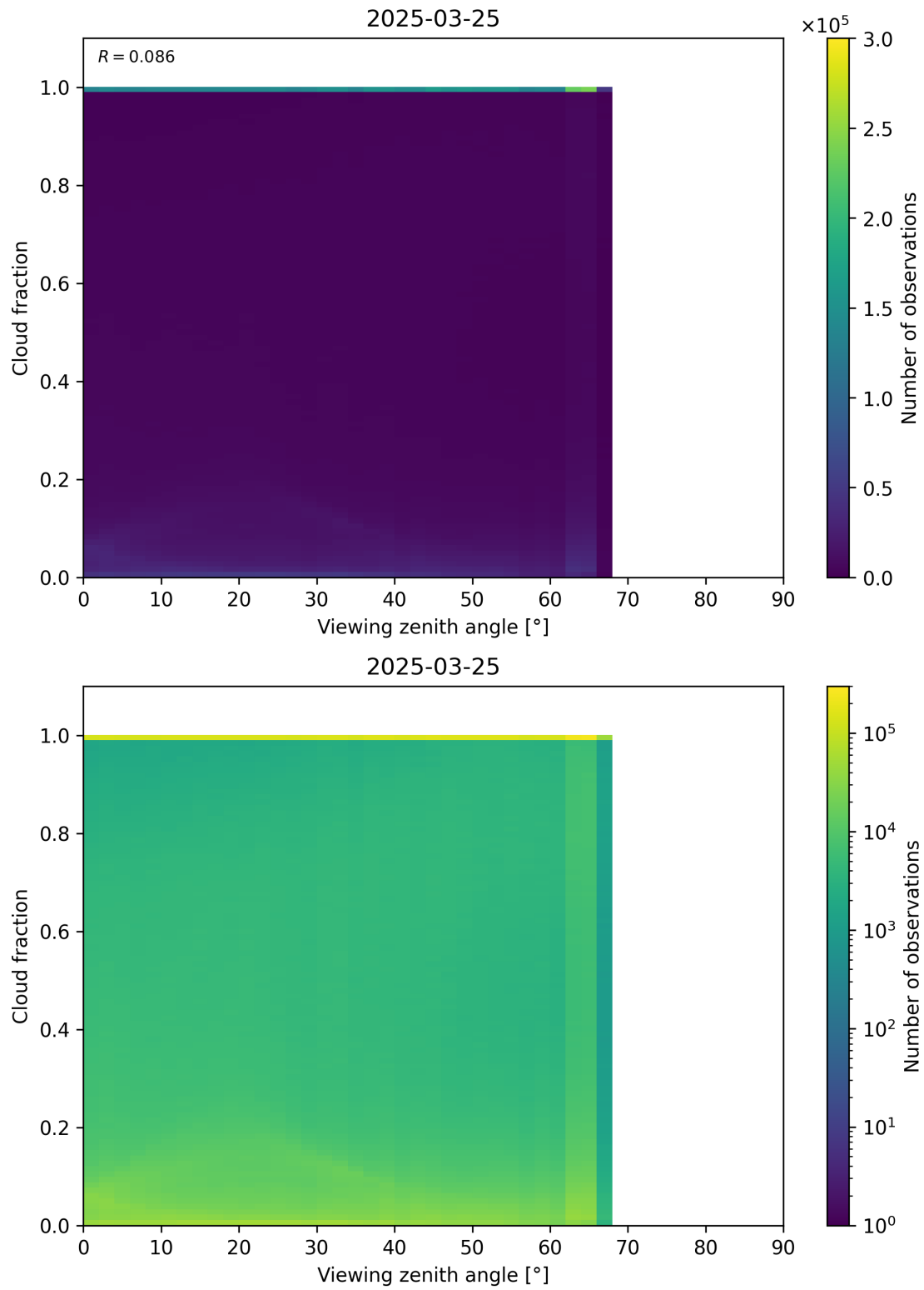
Figure 120: Scatter density plot of “Viewing zenith angle” against “Cloud fraction” for 2025-03-24 to 2025-03-26.
