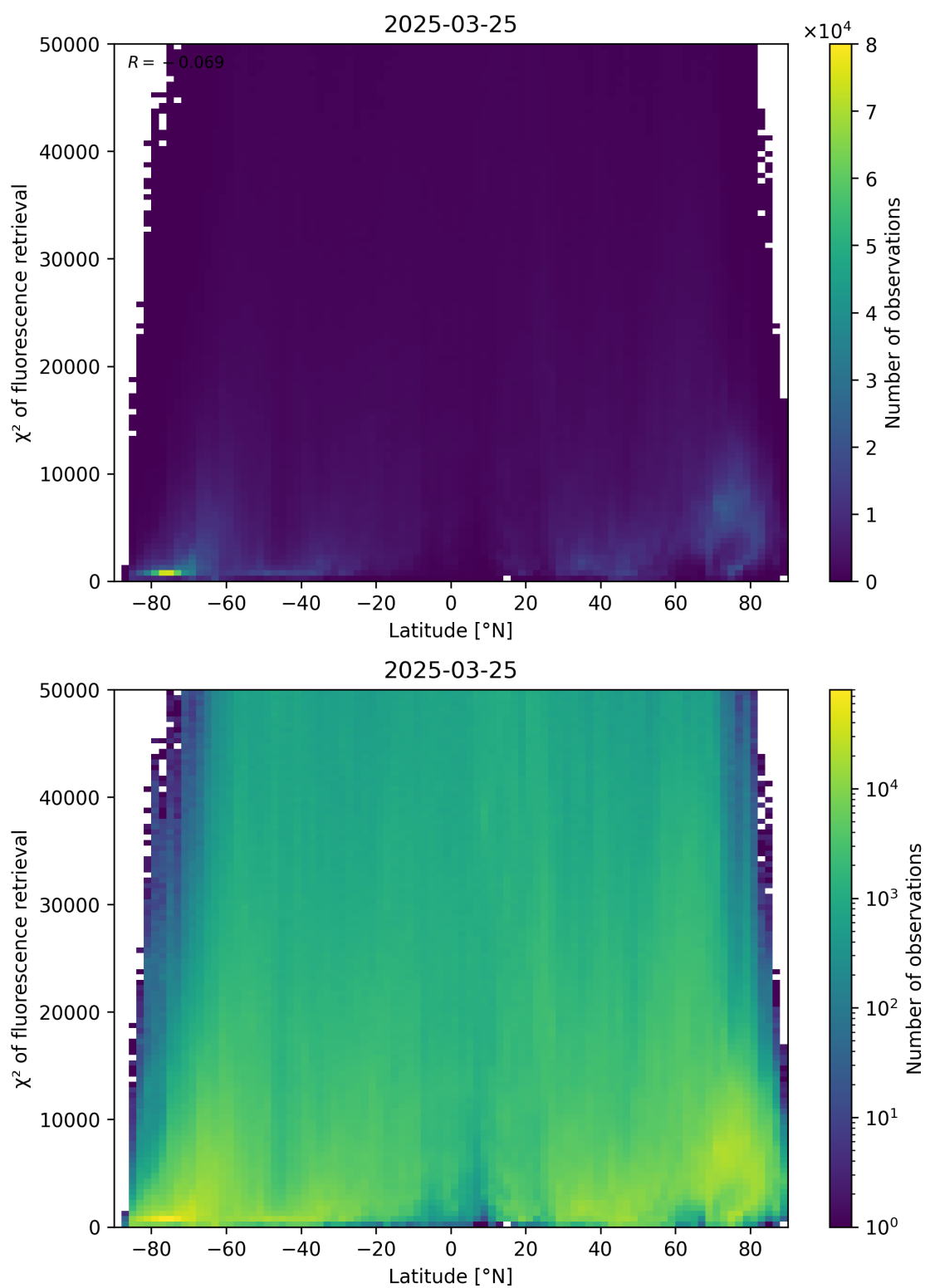
Figure 89: Scatter density plot of “Latitude” against “ \chi^2 of fluorescence retrieval” for 2025-03-24 to 2025-03-26.
