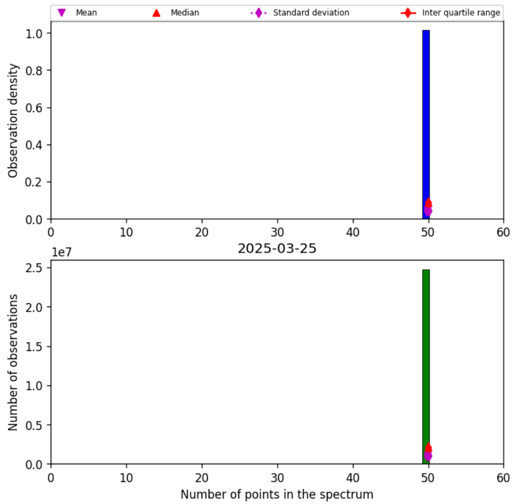
Figure 44: Histogram of “Number of points in the spectrum” for 2025-03-24 to 2025-03-26
