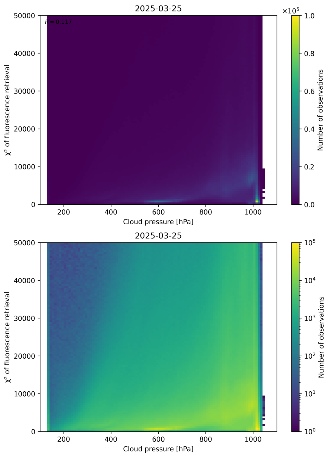
Figure 78: Scatter density plot of “Cloud pressure” against “ \chi^2 of fluorescence retrieval” for 2025-03-24 to 2025-03-26.
