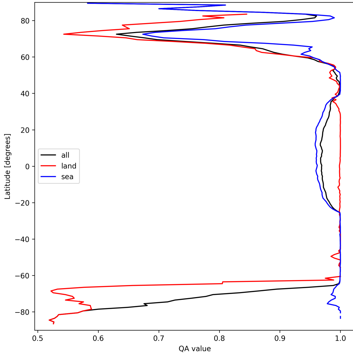
Figure 12: Zonal average of “QA value” for 2025-03-24 to 2025-03-26.
