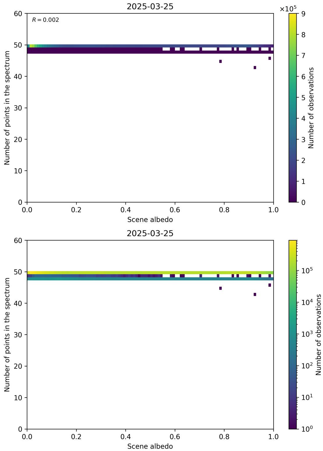
Figure 106: Scatter density plot of “Scene albedo” against “Number of points in the spectrum” for 2025-03-24 to 2025-03-26.
