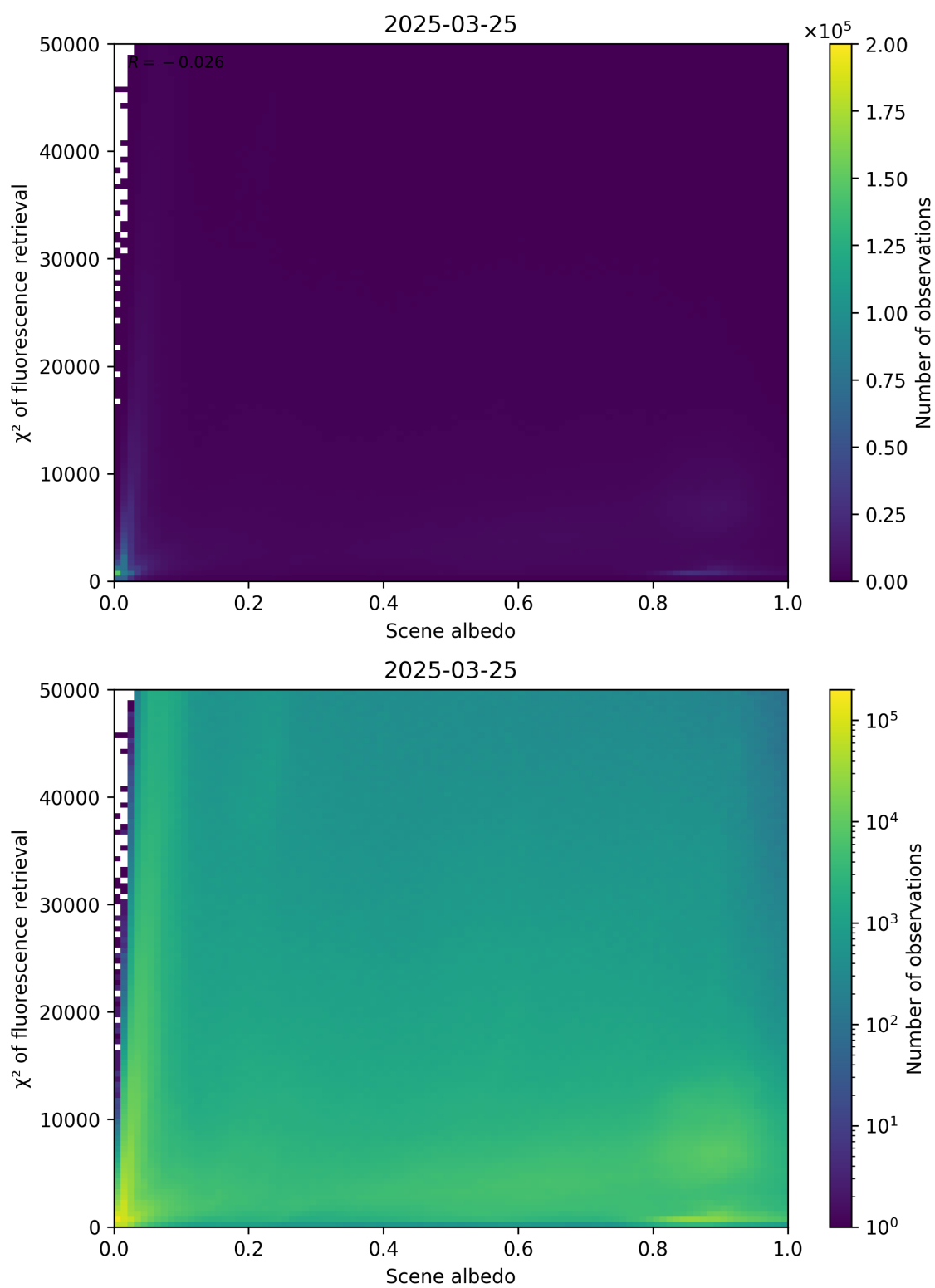
Figure 103: Scatter density plot of “Scene albedo” against “ \chi^2 of fluorescence retrieval” for 2025-03-24 to 2025-03-26.
