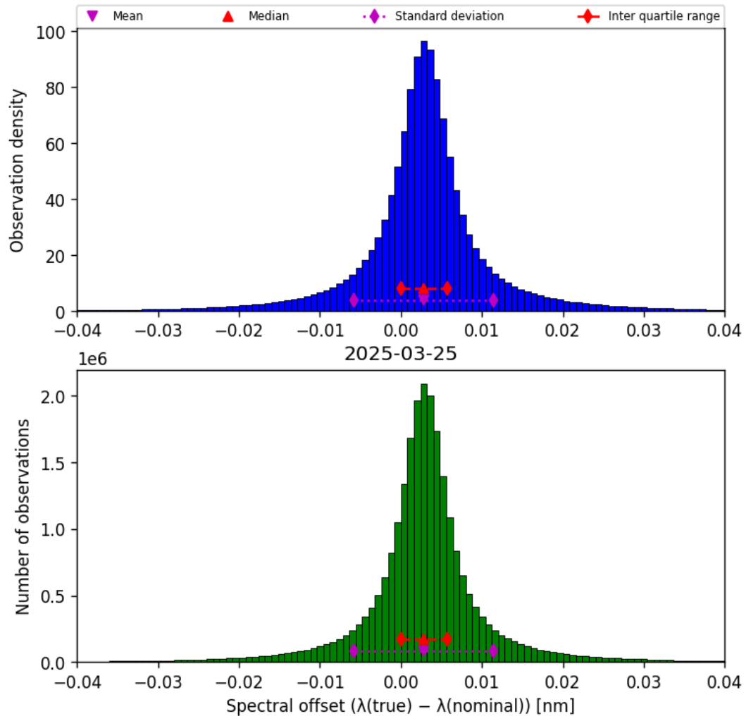
Figure 45: Histogram of “Spectral offset ( \lambda_{\text{true}} - \lambda_{\text{nominal}} )” for 2025-03-24 to 2025-03-26
