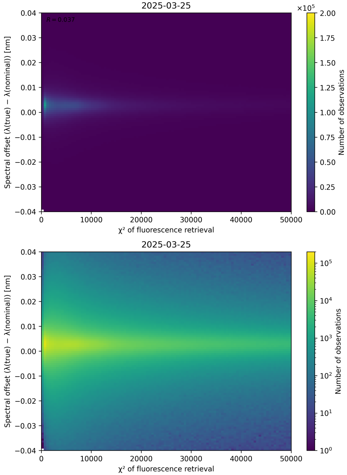
Figure 69: Scatter density plot of “ \chi^2 of fluorescence retrieval” against “Spectral offset ( \lambda_{\text{true}} - \lambda_{\text{nominal}} )” for 2025-03-24 to 2025-03-26.
