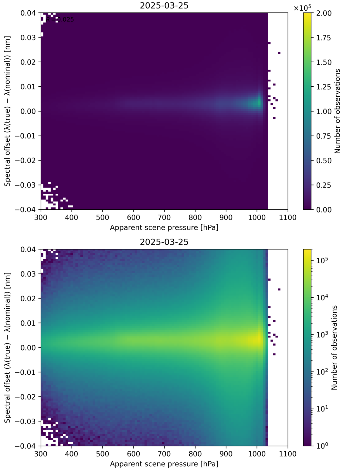
Figure 67: Scatter density plot of “Apparent scene pressure” against “Spectral offset ( \lambda_{\text{true}} - \lambda_{\text{nominal}} )” for 2025-03-24 to 2025-03-26.
