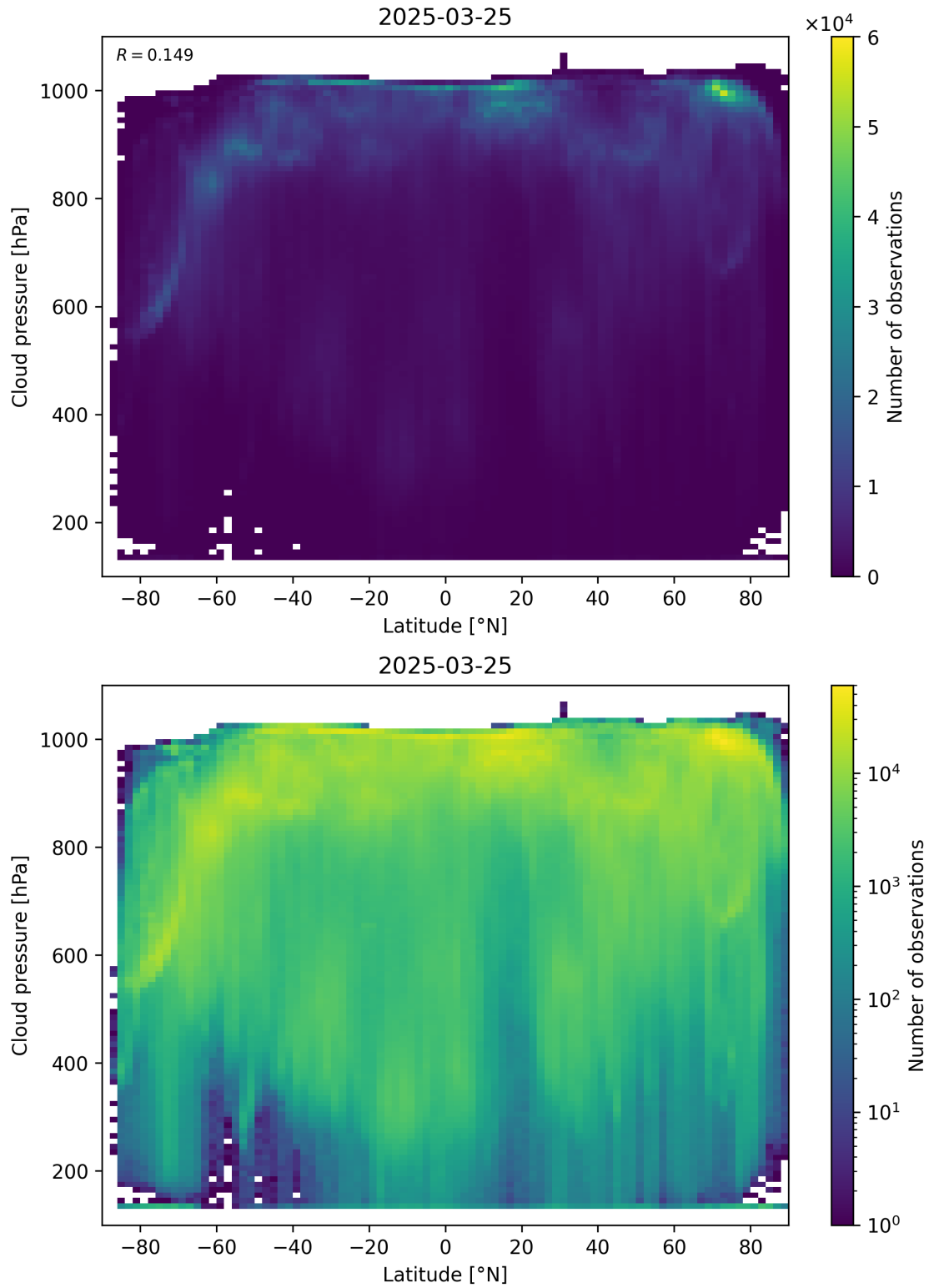
Figure 91: Scatter density plot of “Latitude” against “Cloud pressure” for 2025-03-24 to 2025-03-26.
