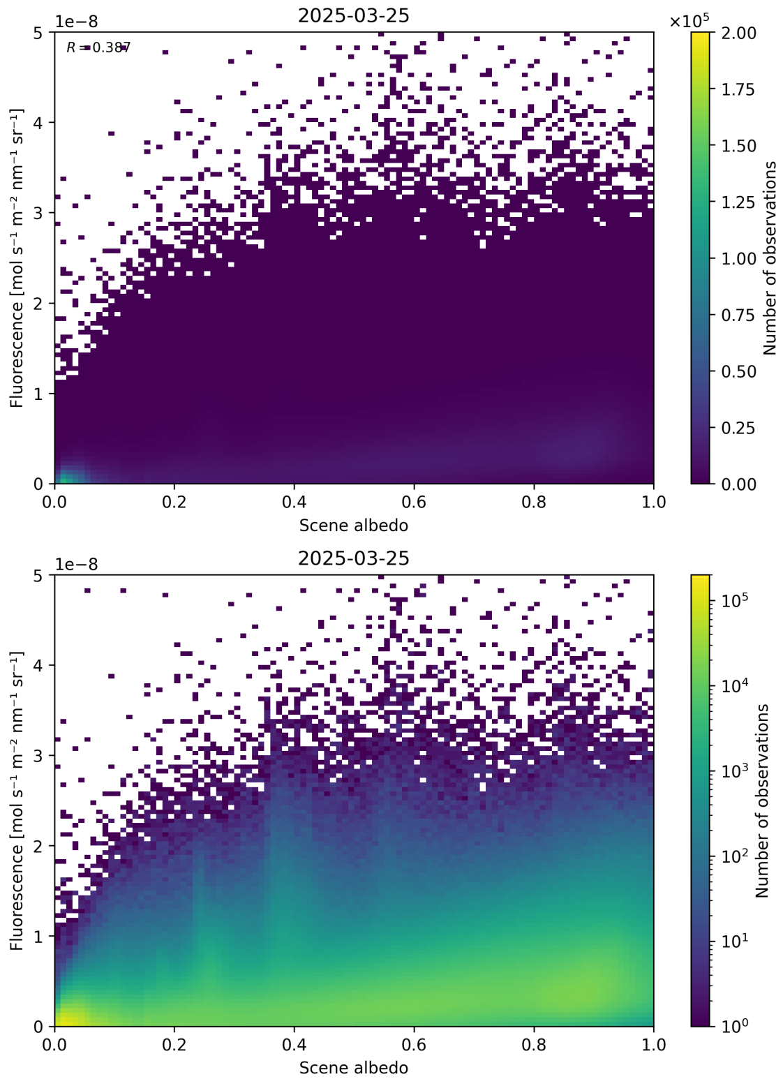
Figure 104: Scatter density plot of “Scene albedo” against “Fluorescence” for 2025-03-24 to 2025-03-26.
