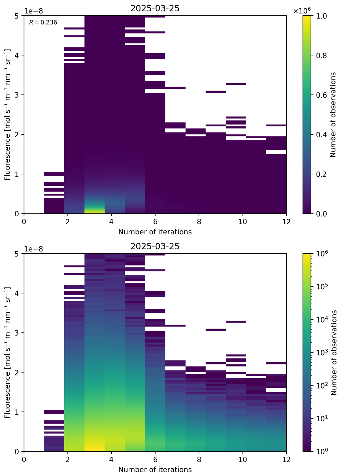
Figure 98: Scatter density plot of “Number of iterations” against “Fluorescence” for 2025-03-24 to 2025-03-26.
