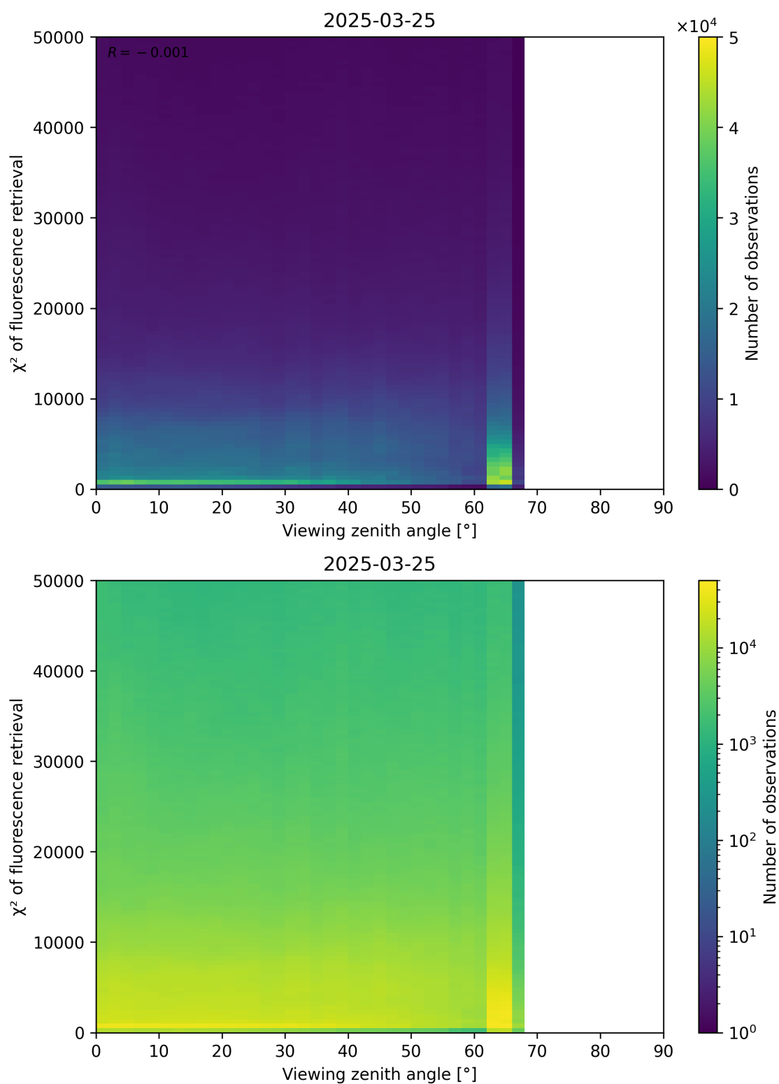
Figure 119: Scatter density plot of “Viewing zenith angle” against “ \chi^2 of fluorescence retrieval” for 2025-03-24 to 2025-03-26.
