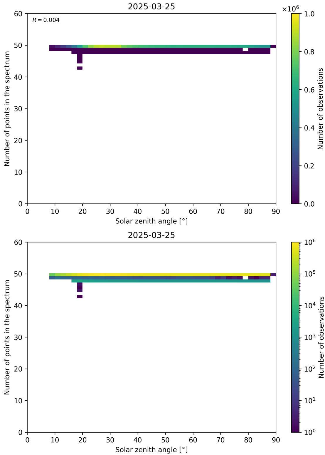
Figure 115: Scatter density plot of “Solar zenith angle” against “Number of points in the spectrum” for 2025-03-24 to 2025-03-26.
