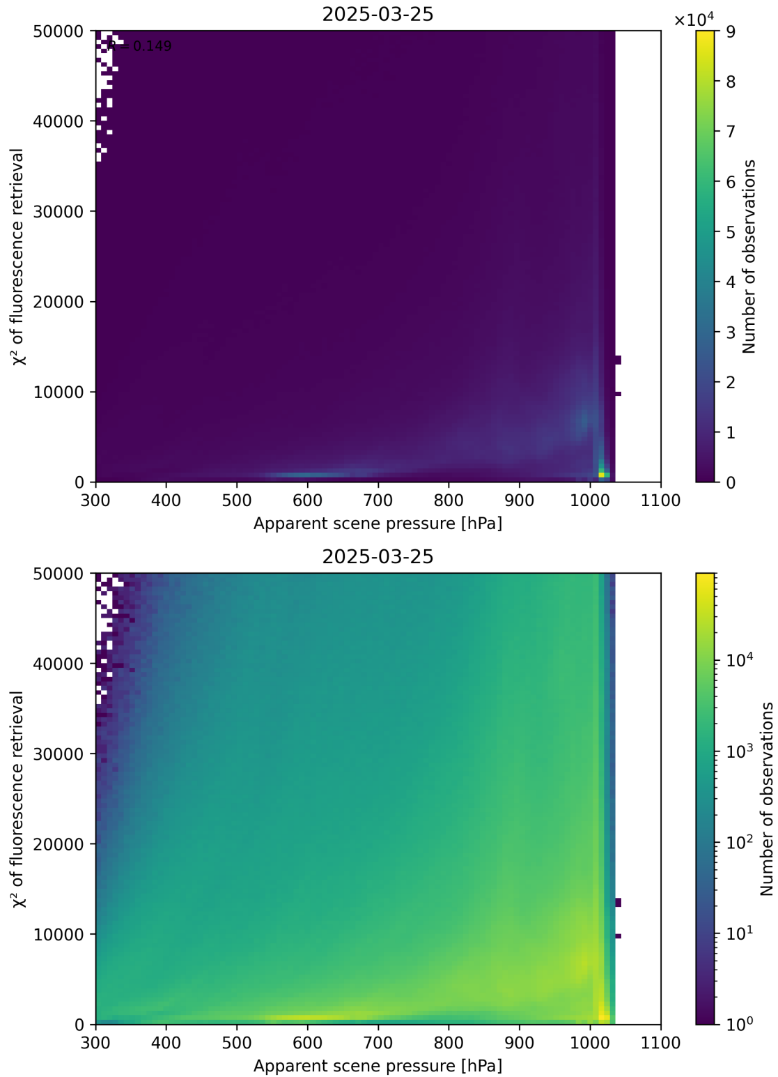
Figure 63: Scatter density plot of “Apparent scene pressure” against “ \chi^2 of fluorescence retrieval” for 2025-03-24 to 2025-03-26.
