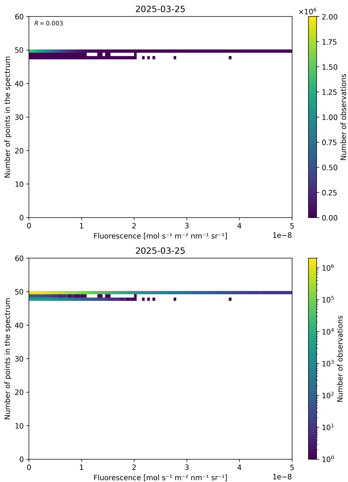
Figure 86: Scatter density plot of “Fluorescence” against “Number of points in the spectrum” for 2025-03-24 to 2025-03-26.
