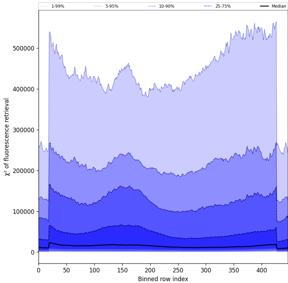
Figure 59: Along track statistics of “ \chi^2 of fluorescence retrieval” for 2025-03-24 to 2025-03-26
