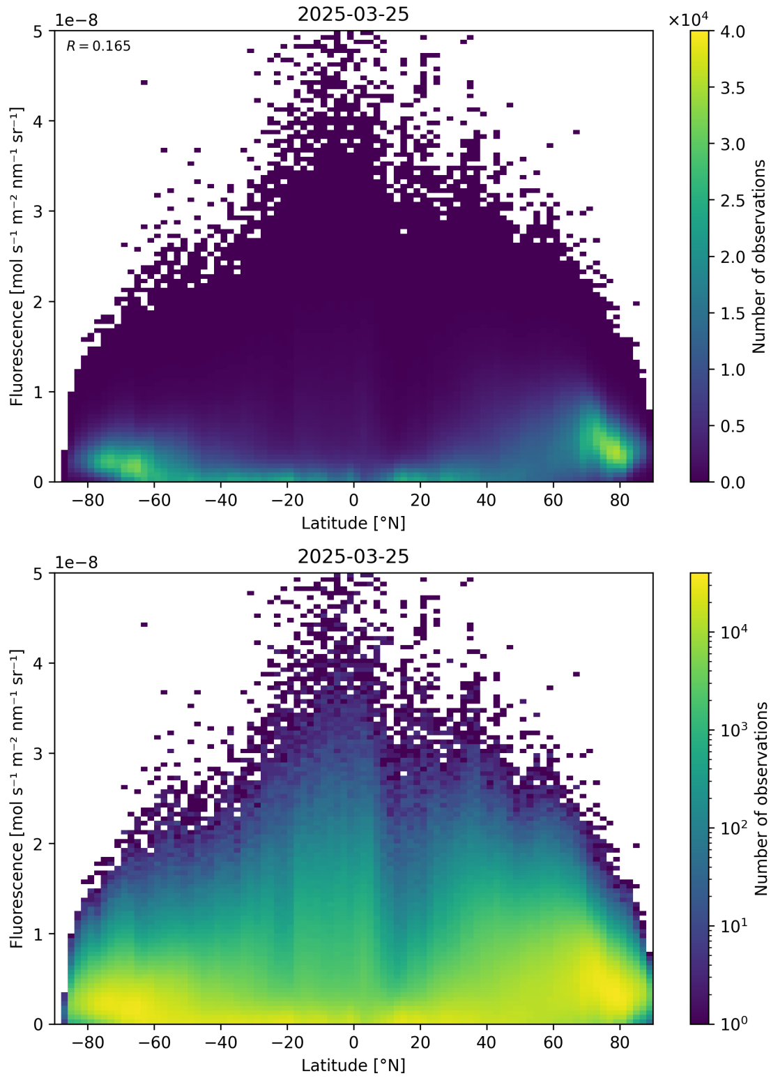
Figure 92: Scatter density plot of “Latitude” against “Fluorescence” for 2025-03-24 to 2025-03-26.
