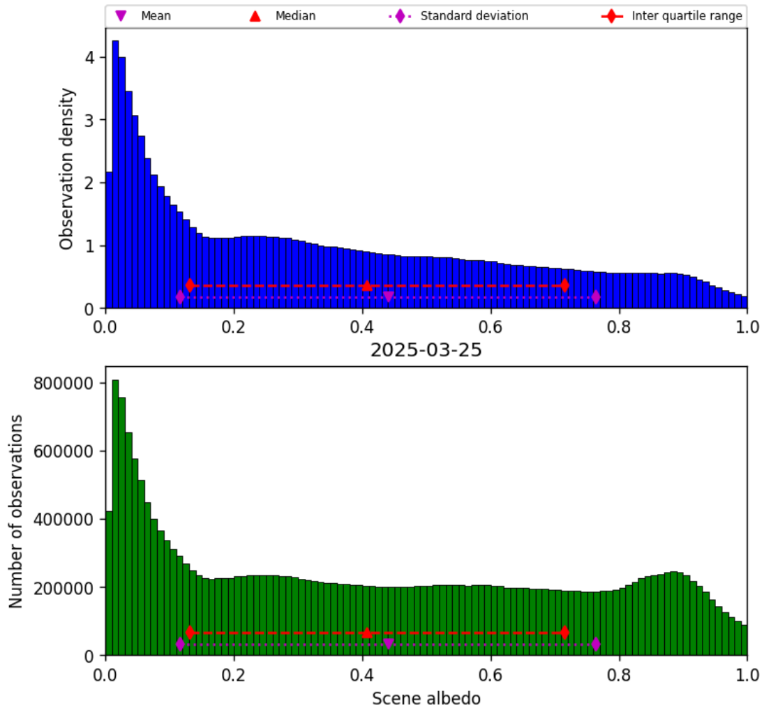
Figure 34: Histogram of “Scene albedo” for 2025-03-24 to 2025-03-26
