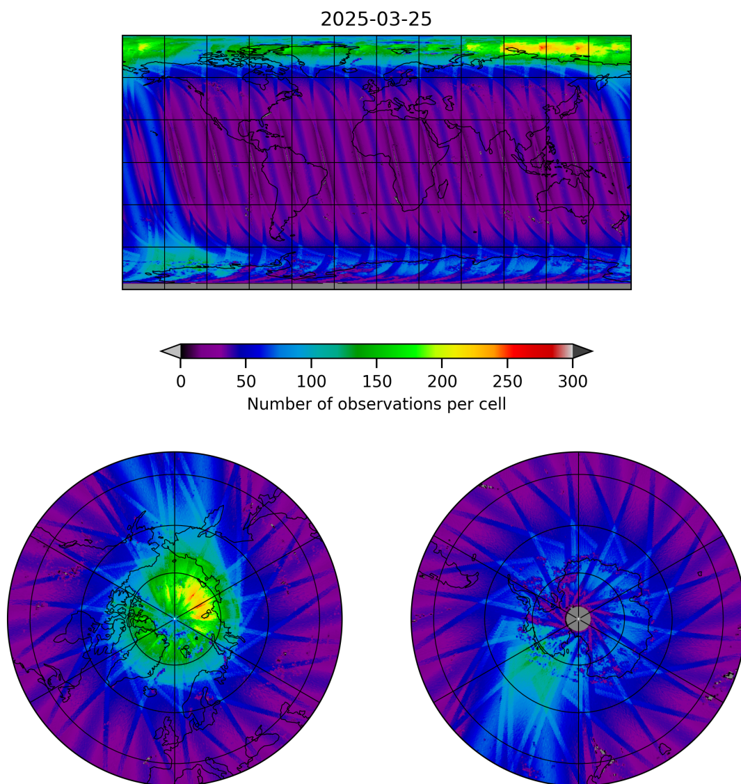
Figure 11: Map of the number of observations for 2025-03-24 to 2025-03-26
