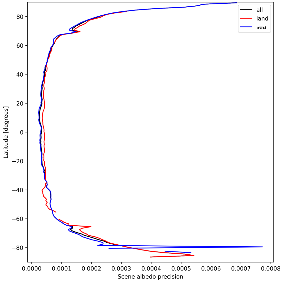
Figure 18: Zonal average of “Scene albedo precision” for 2025-03-24 to 2025-03-26.
