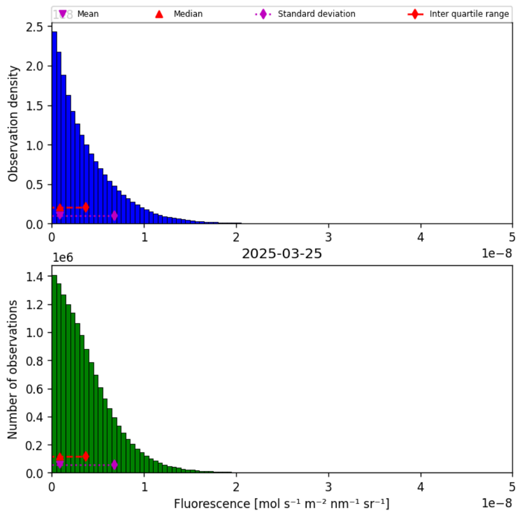
Figure 40: Histogram of “Fluorescence” for 2025-03-24 to 2025-03-26
