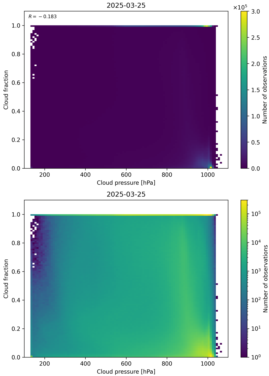
Figure 79: Scatter density plot of “Cloud pressure” against “Cloud fraction” for 2025-03-24 to 2025-03-26.
