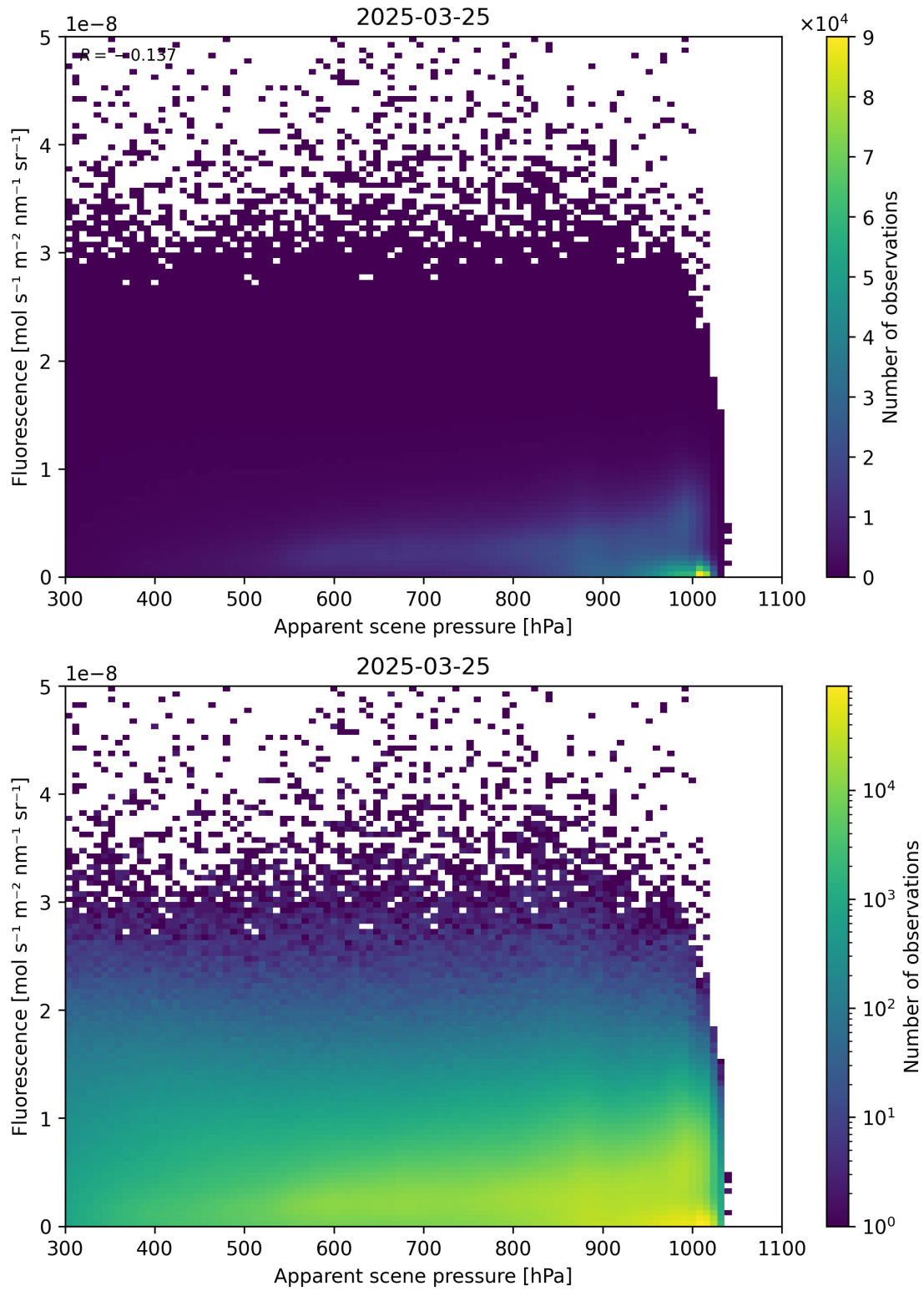
Figure 64: Scatter density plot of “Apparent scene pressure” against “Fluorescence” for 2025-03-24 to 2025-03-26.
