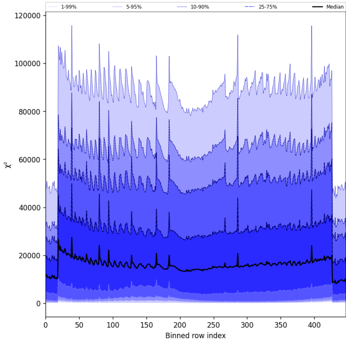
Figure 55: Along track statistics of “ \chi^2 ” for 2025-03-24 to 2025-03-26
