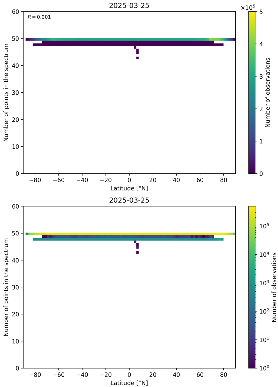
Figure 94: Scatter density plot of “Latitude” against “Number of points in the spectrum” for 2025-03-24 to 2025-03-26.
