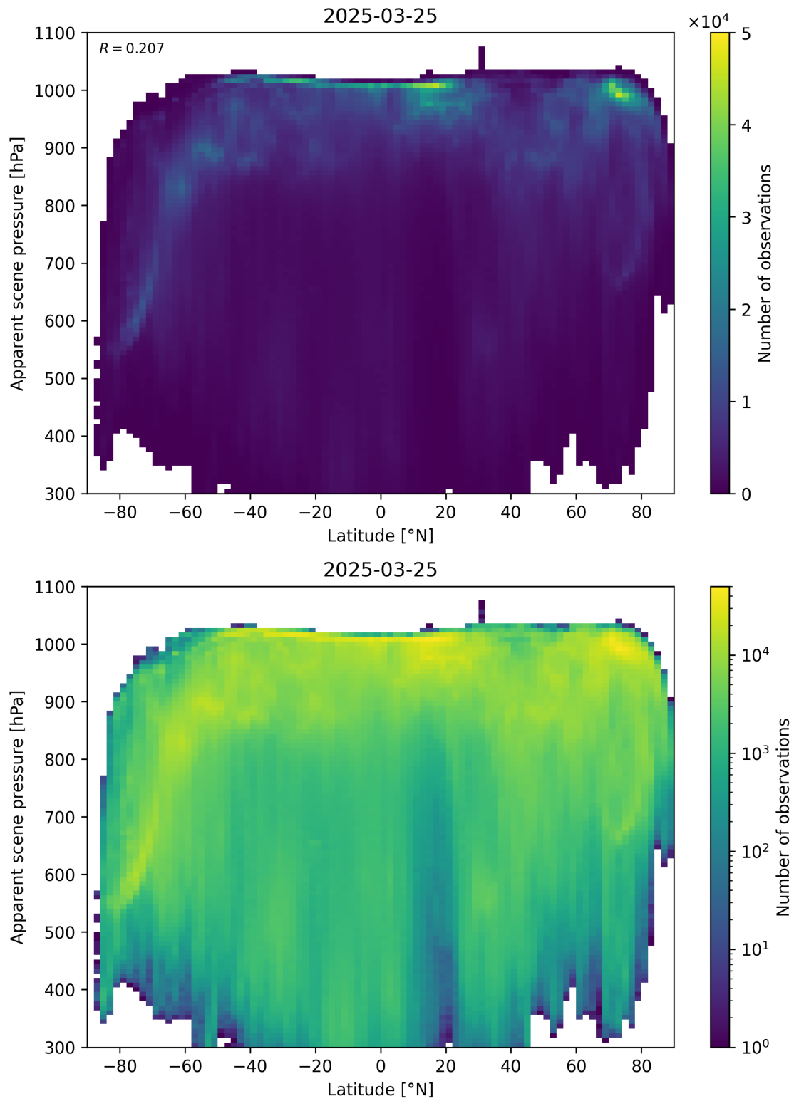
Figure 88: Scatter density plot of “Latitude” against “Apparent scene pressure” for 2025-03-24 to 2025-03-26.
