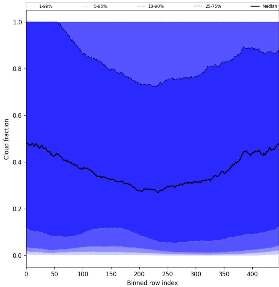
Figure 49: Along track statistics of “Cloud fraction” for 2025-03-24 to 2025-03-26
