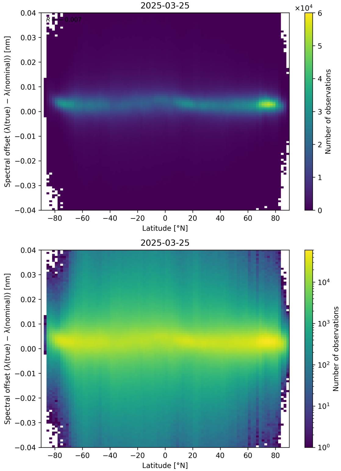
Figure 96: Scatter density plot of “Latitude” against “Spectral offset ( \lambda_{\text{true}} - \lambda_{\text{nominal}} )” for 2025-03-24 to 2025-03-26.
