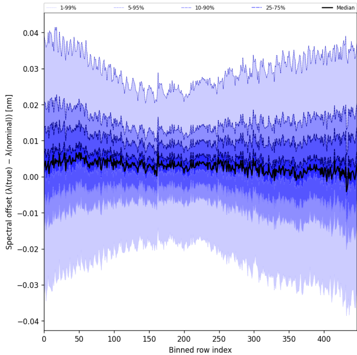
Figure 62: Along track statistics of “Spectral offset ( \lambda_{\text{true}} - \lambda_{\text{nominal}} )” for 2025-03-24 to 2025-03-26
