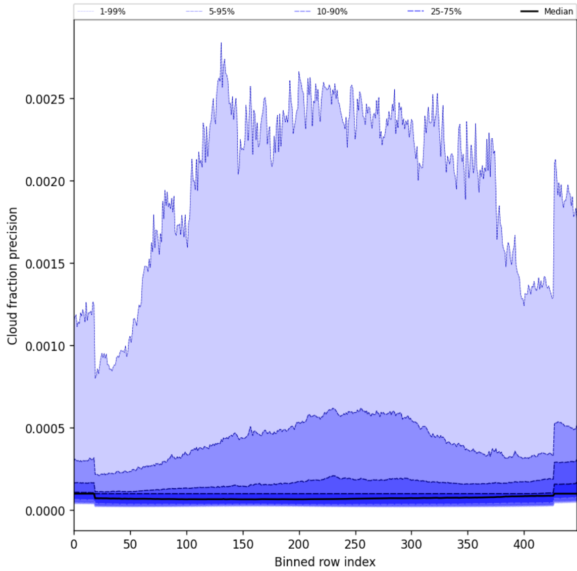
Figure 50: Along track statistics of “Cloud fraction precision” for 2025-03-24 to 2025-03-26
