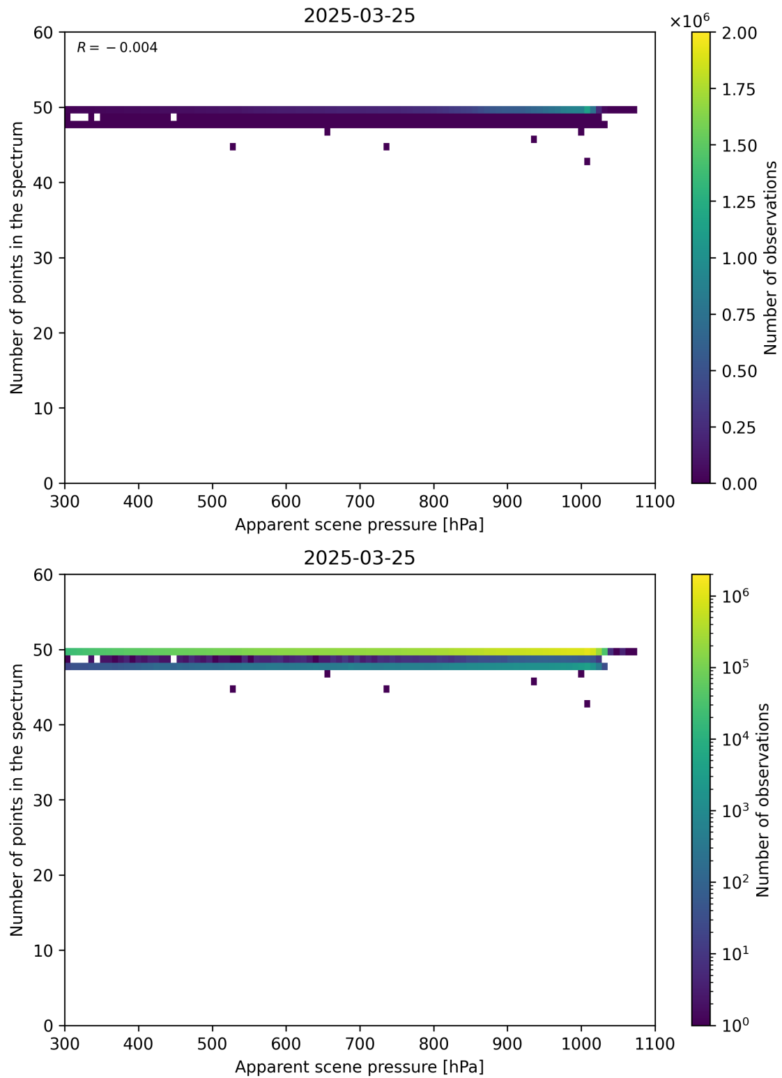
Figure 66: Scatter density plot of “Apparent scene pressure” against “Number of points in the spectrum” for 2025-03-24 to 2025-03-26.
