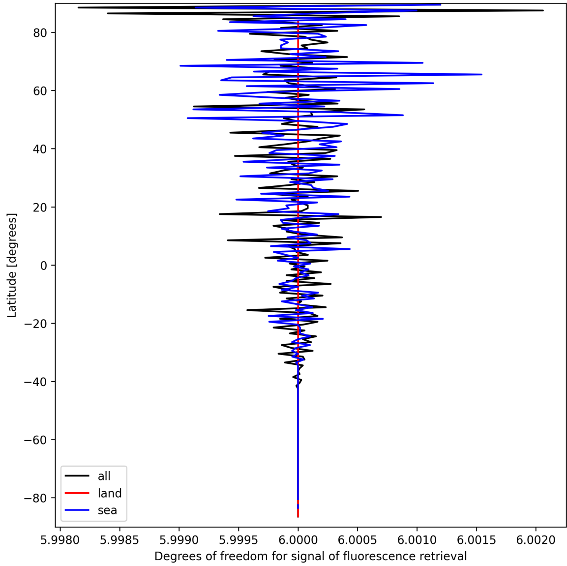
Figure 26: Zonal average of “Degrees of freedom for signal of fluorescence retrieval” for 2025-03-24 to 2025-03-26.
