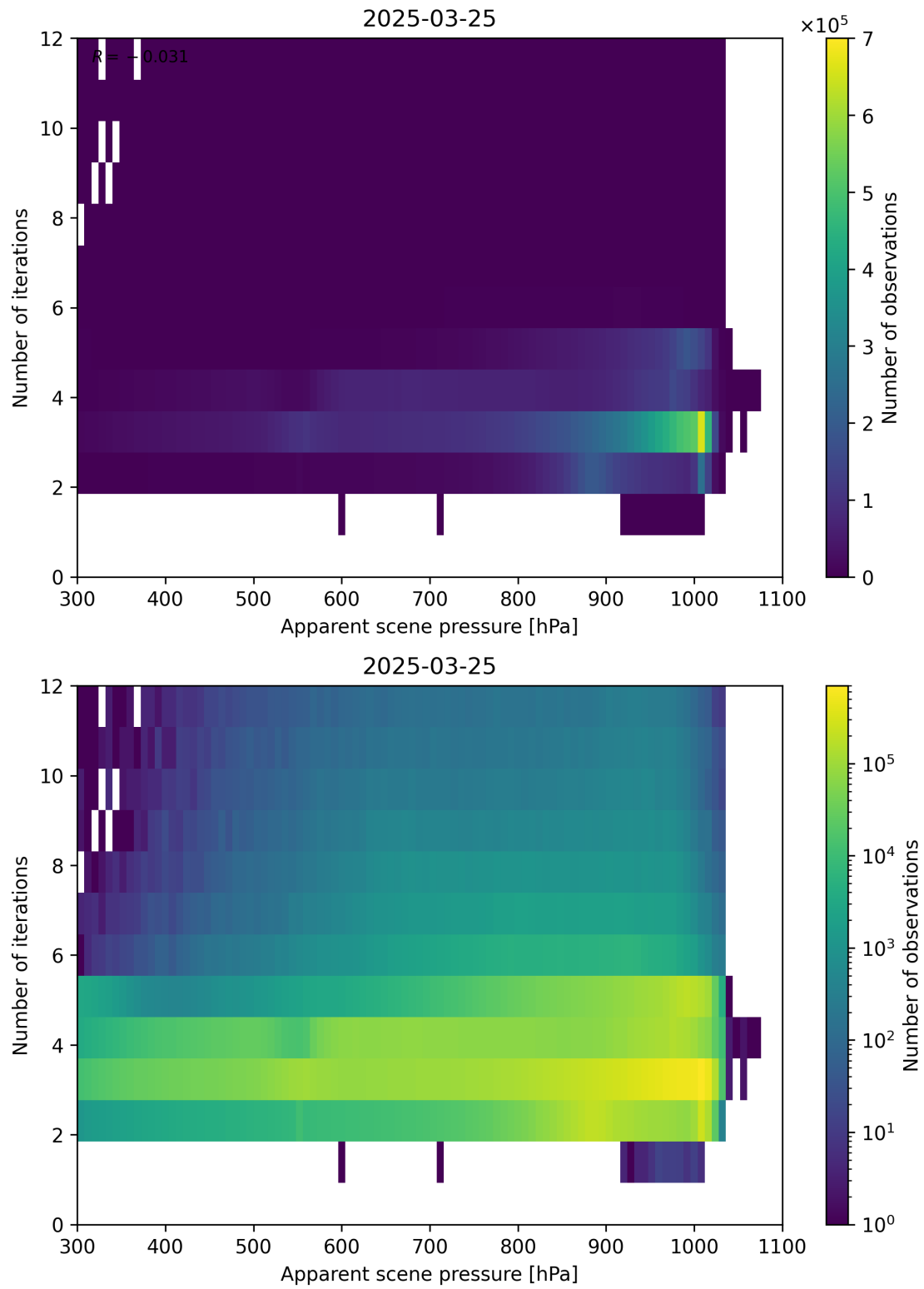
Figure 65: Scatter density plot of “Apparent scene pressure” against “Number of iterations” for 2025-03-24 to 2025-03-26.
