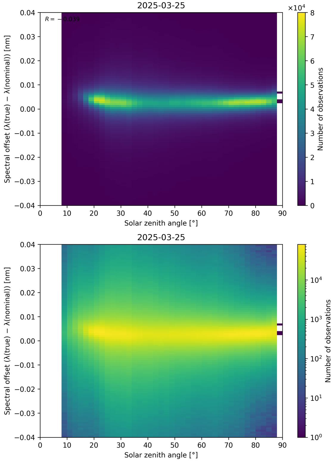
Figure 117: Scatter density plot of “Solar zenith angle” against “Spectral offset ( \lambda_{\text{true}} - \lambda_{\text{nominal}} )” for 2025-03-24 to 2025-03-26.
