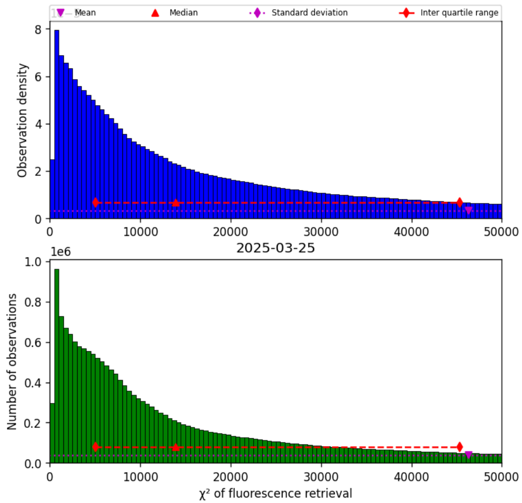
Figure 42: Histogram of “ \chi^2 of fluorescence retrieval” for 2025-03-24 to 2025-03-26
