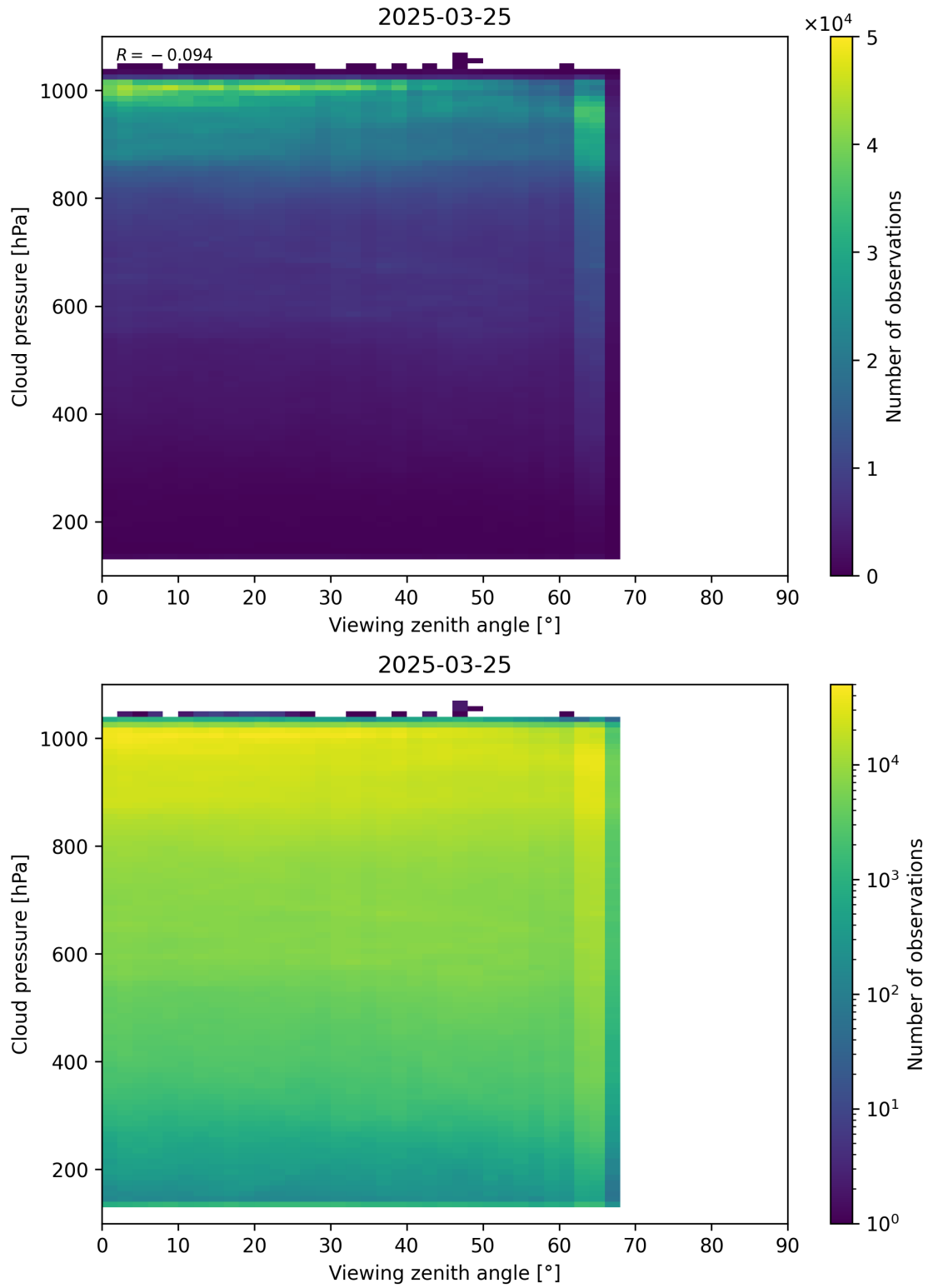
Figure 121: Scatter density plot of “Viewing zenith angle” against “Cloud pressure” for 2025-03-24 to 2025-03-26.
