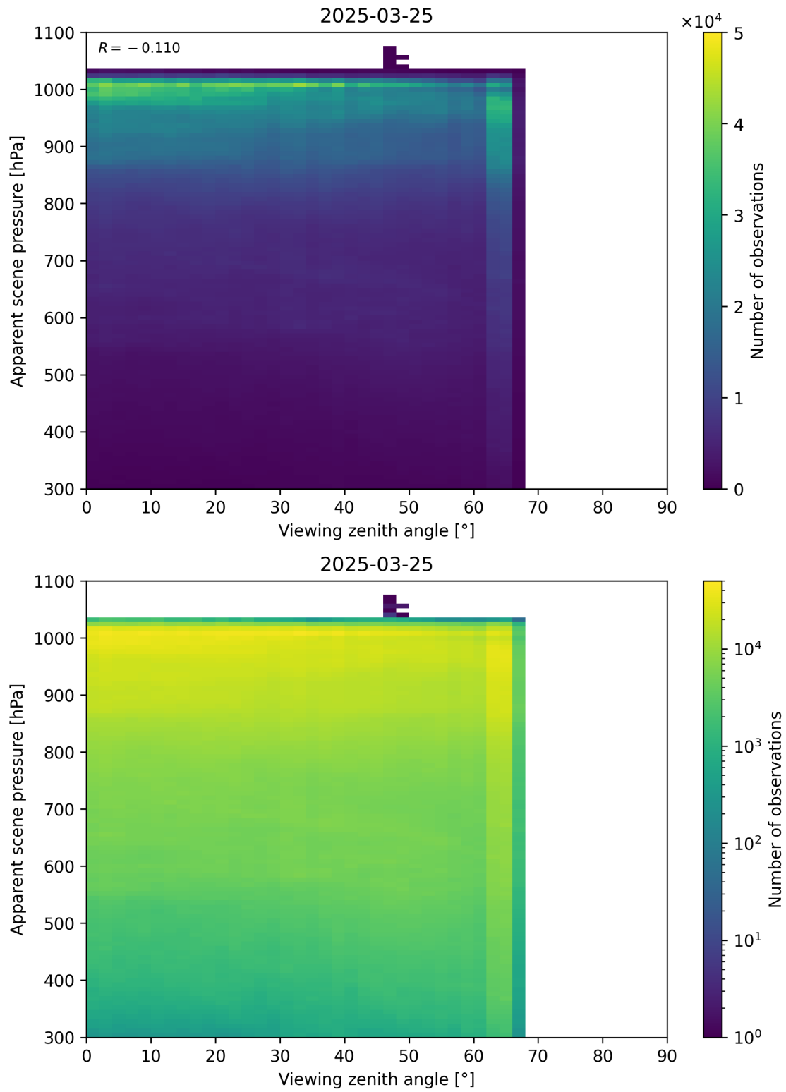
Figure 118: Scatter density plot of “Viewing zenith angle” against “Apparent scene pressure” for 2025-03-24 to 2025-03-26.
