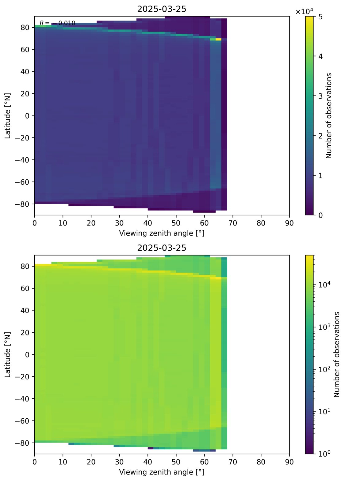
Figure 123: Scatter density plot of “Viewing zenith angle” against “Latitude” for 2025-03-24 to 2025-03-26.
