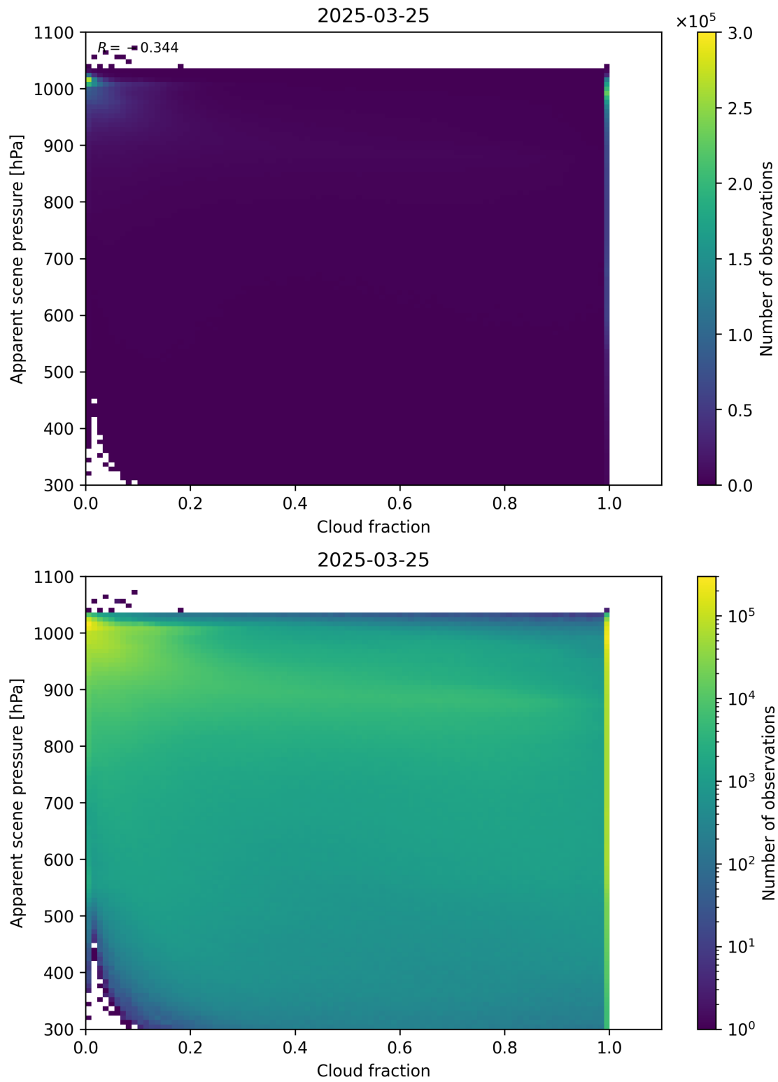
Figure 70: Scatter density plot of “Cloud fraction” against “Apparent scene pressure” for 2025-03-24 to 2025-03-26.
