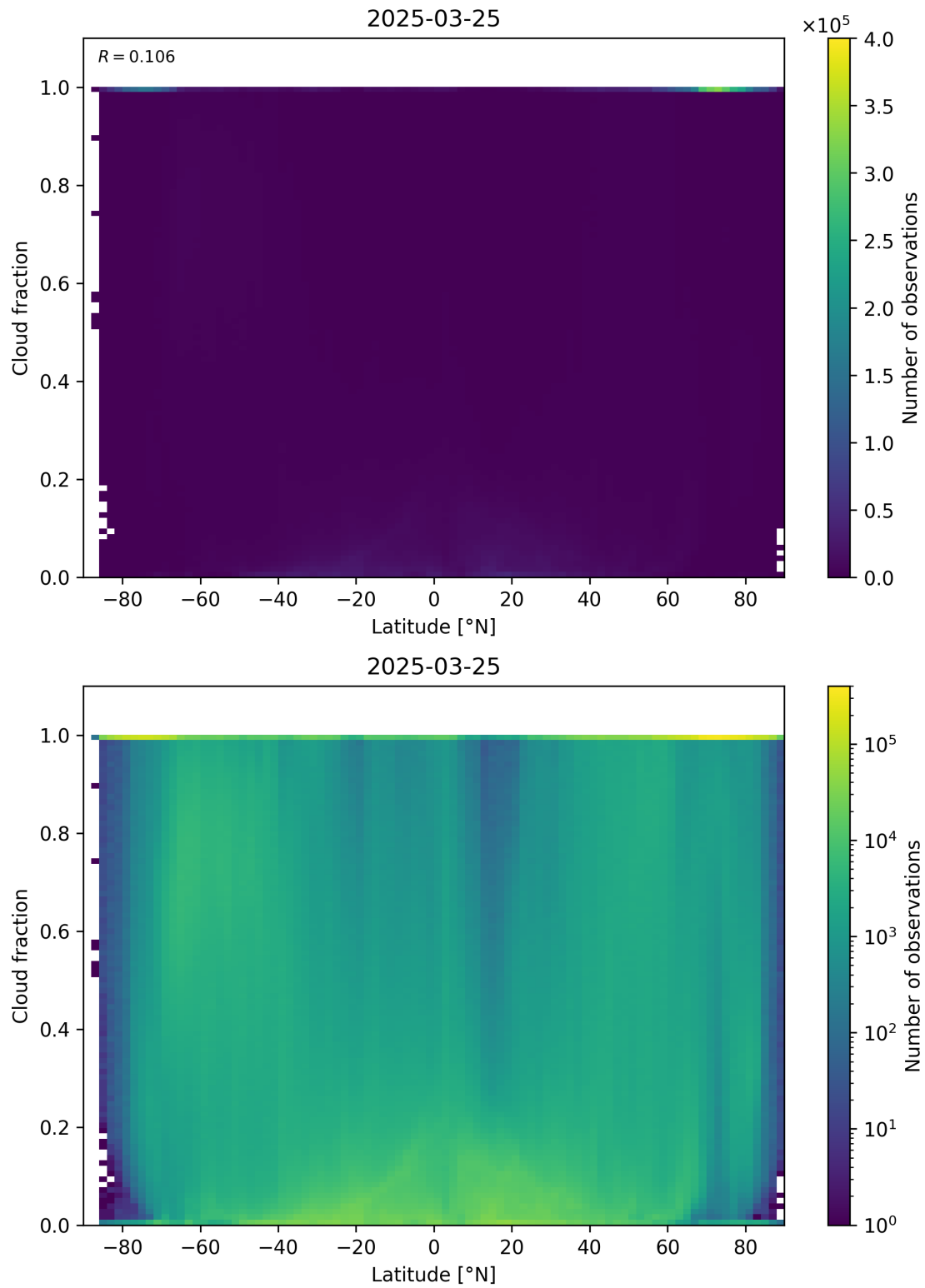
Figure 90: Scatter density plot of “Latitude” against “Cloud fraction” for 2025-03-24 to 2025-03-26.
