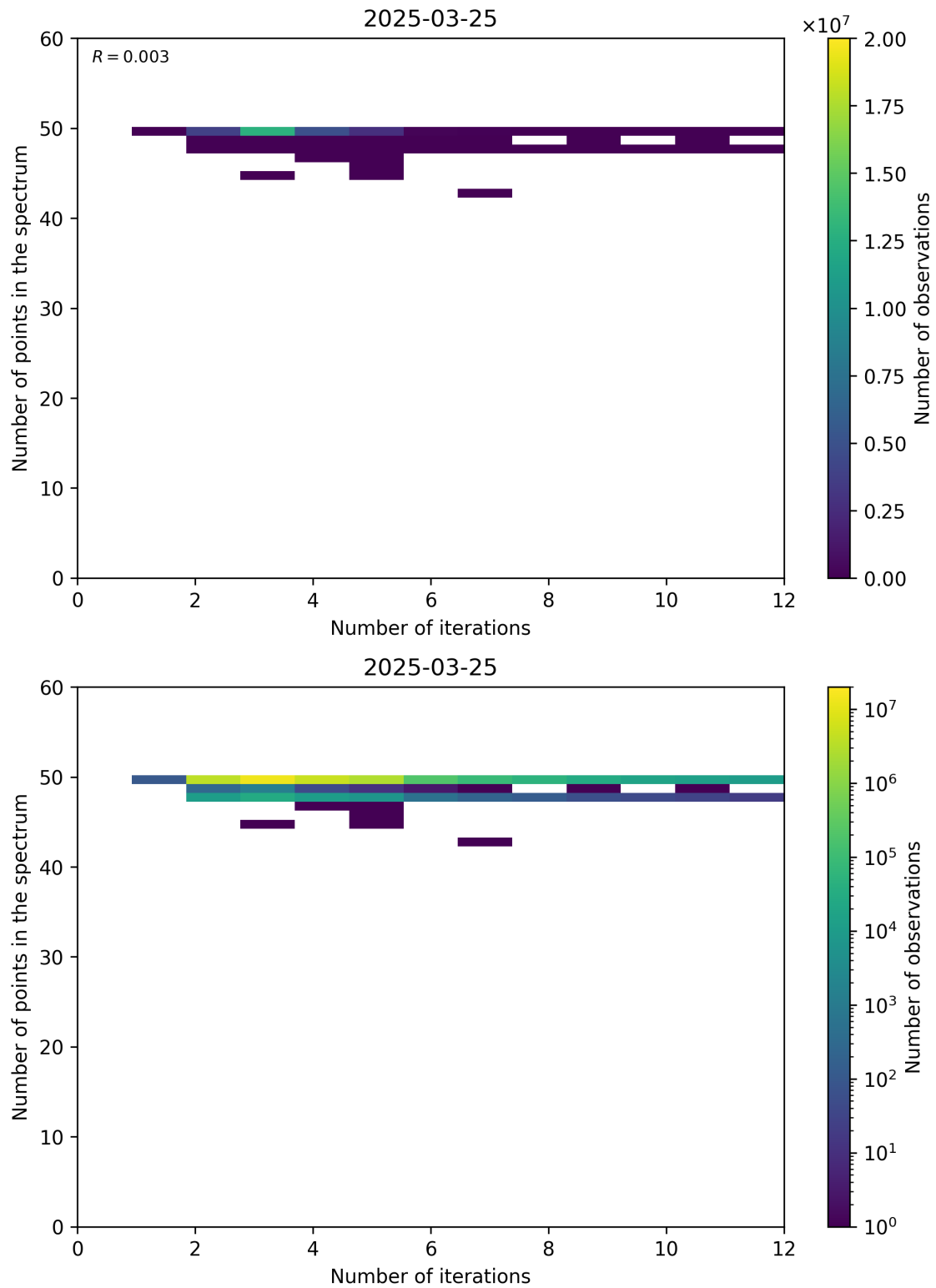
Figure 99: Scatter density plot of “Number of iterations” against “Number of points in the spectrum” for 2025-03-24 to 2025-03-26.
