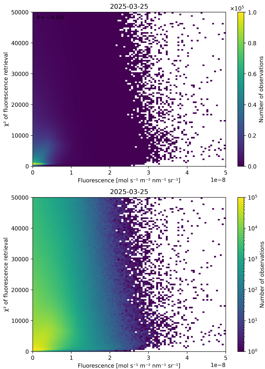
Figure 85: Scatter density plot of “Fluorescence” against “ \chi^2 of fluorescence retrieval” for 2025-03-24 to 2025-03-26.
