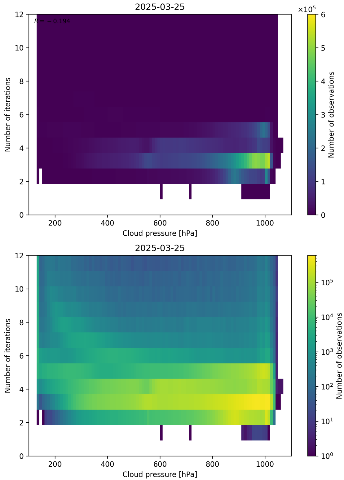
Figure 81: Scatter density plot of “Cloud pressure” against “Number of iterations” for 2025-03-24 to 2025-03-26.
