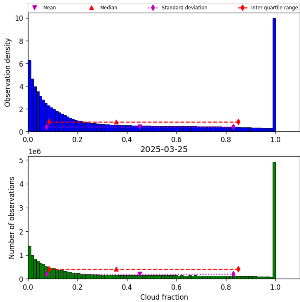
Figure 32: Histogram of “Cloud fraction” for 2025-03-24 to 2025-03-26
