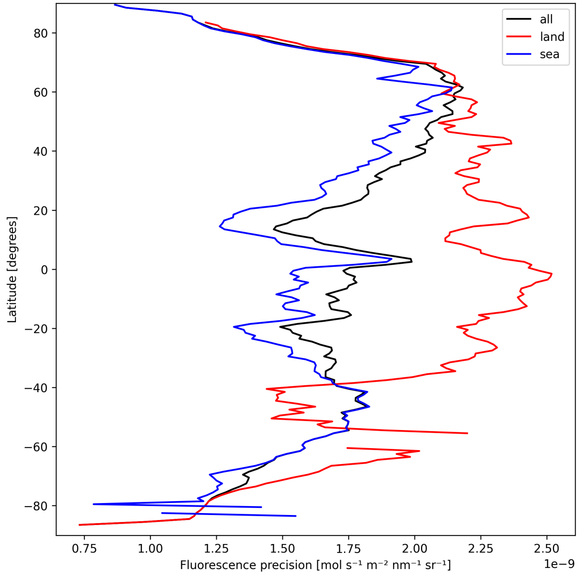
Figure 24: Zonal average of “Fluorescence precision” for 2025-03-24 to 2025-03-26.
