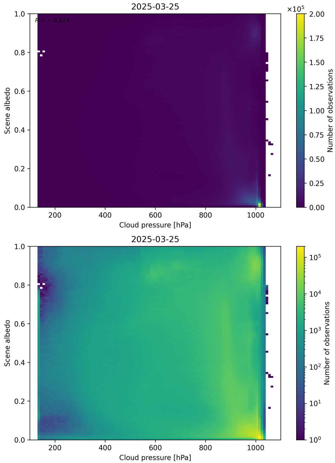
Figure 83: Scatter density plot of “Cloud pressure” against “Scene albedo” for 2025-03-24 to 2025-03-26.
