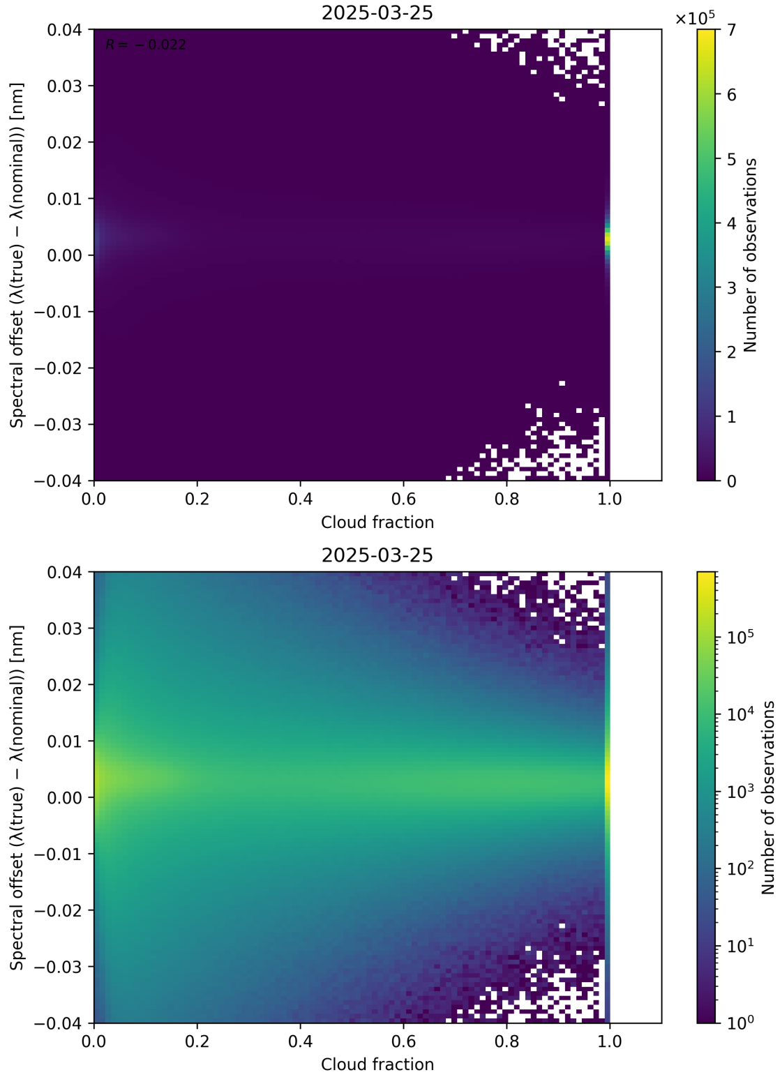
Figure 76: Scatter density plot of “Cloud fraction” against “Spectral offset ( \lambda_{\text{true}} - \lambda_{\text{nominal}} )” for 2025-03-24 to 2025-03-26.
