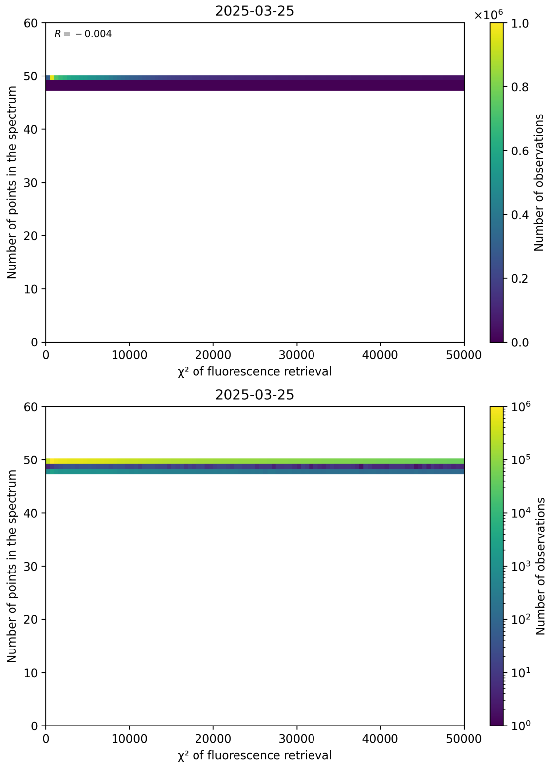
Figure 68: Scatter density plot of “ \chi^2 of fluorescence retrieval” against “Number of points in the spectrum” for 2025-03-24 to 2025-03-26.
