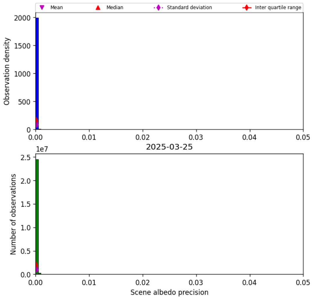
Figure 35: Histogram of “Scene albedo precision” for 2025-03-24 to 2025-03-26
