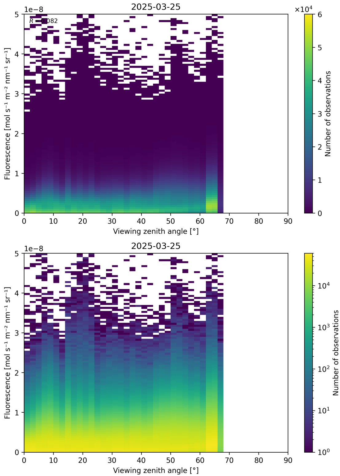
Figure 122: Scatter density plot of “Viewing zenith angle” against “Fluorescence” for 2025-03-24 to 2025-03-26.
