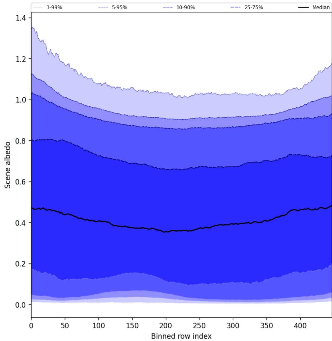
Figure 51: Along track statistics of “Scene albedo” for 2025-03-24 to 2025-03-26
