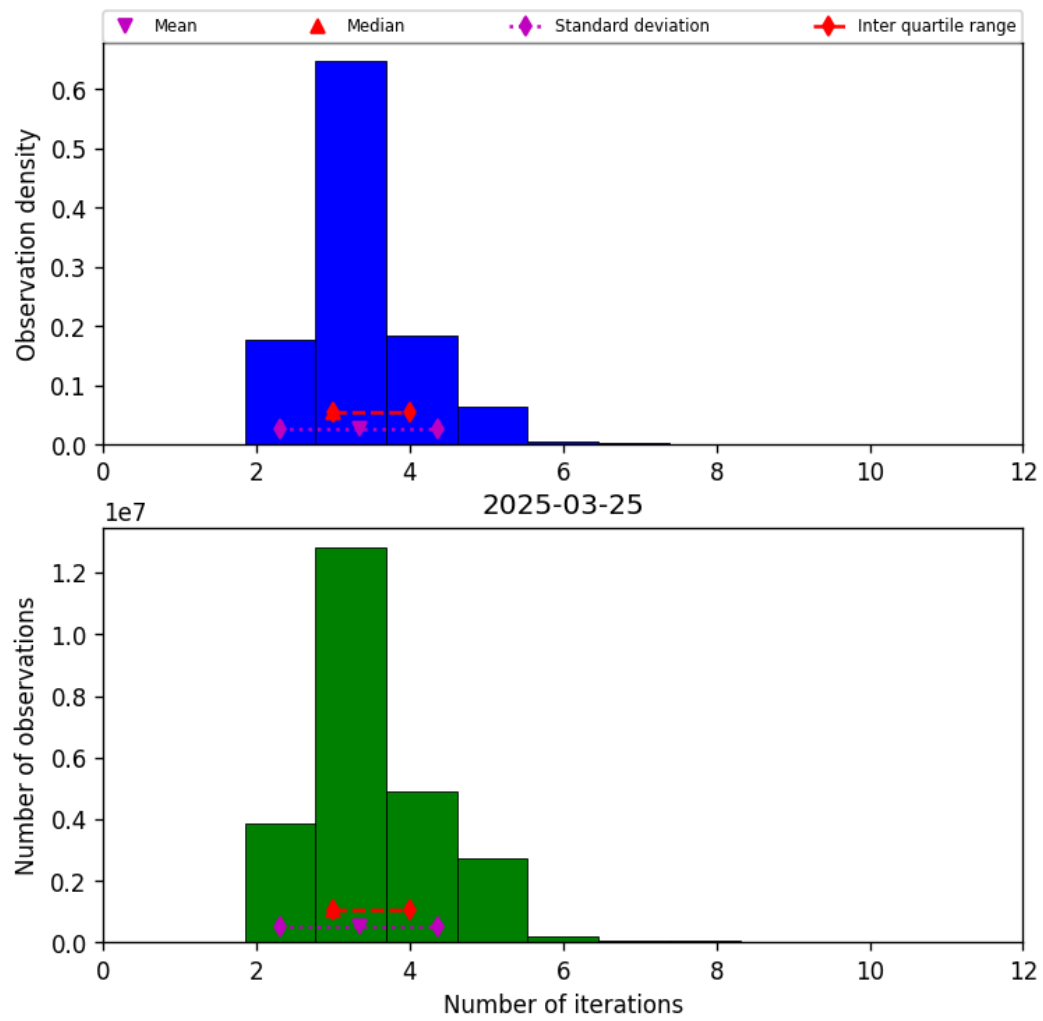
Figure 39: Histogram of “Number of iterations” for 2025-03-24 to 2025-03-26
