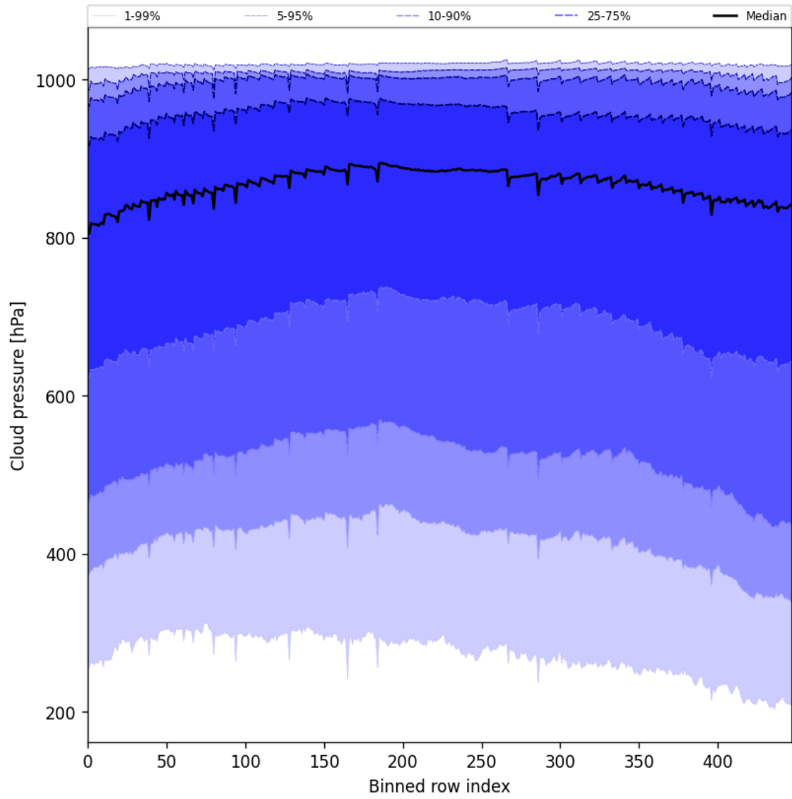
Figure 47: Along track statistics of “Cloud pressure” for 2025-03-24 to 2025-03-26
