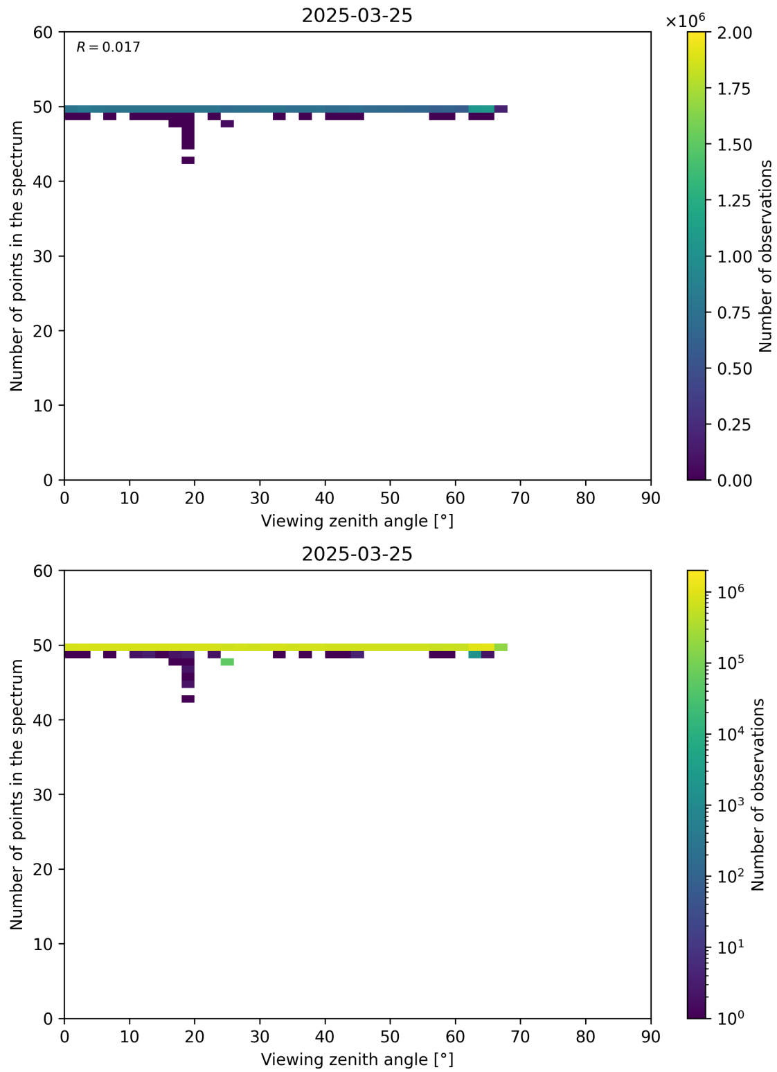
Figure 125: Scatter density plot of “Viewing zenith angle” against “Number of points in the spectrum” for 2025-03-24 to 2025-03-26.
