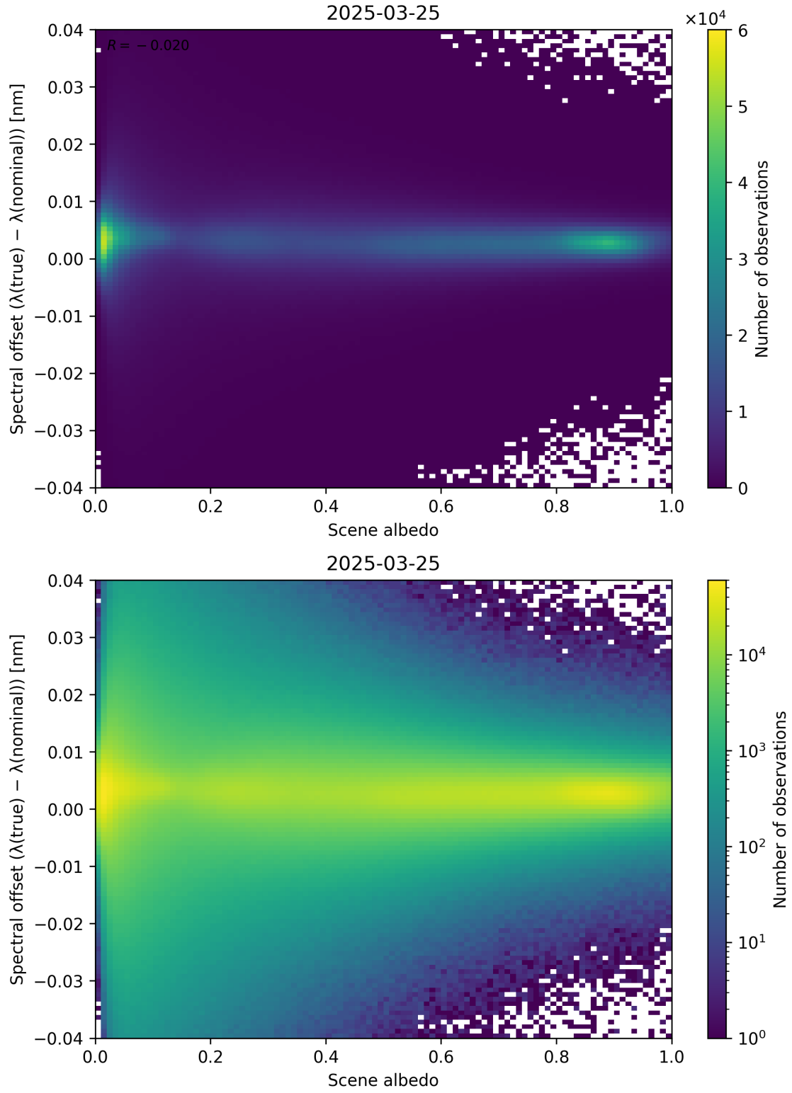
Figure 107: Scatter density plot of “Scene albedo” against “Spectral offset ( \lambda_{\text{true}} - \lambda_{\text{nominal}} )” for 2025-03-24 to 2025-03-26.
