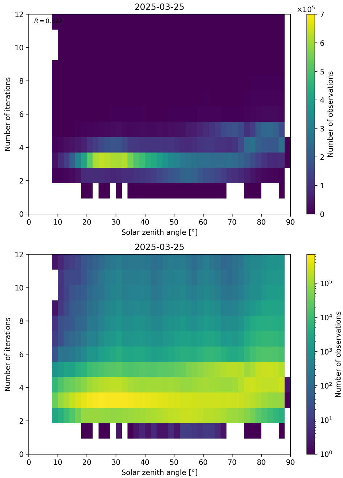
Figure 114: Scatter density plot of “Solar zenith angle” against “Number of iterations” for 2025-03-24 to 2025-03-26.
