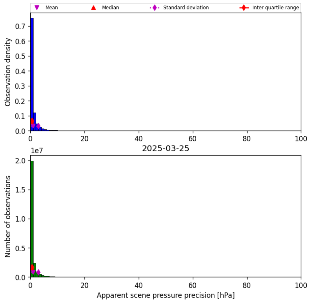
Figure 37: Histogram of “Apparent scene pressure precision” for 2025-03-24 to 2025-03-26
