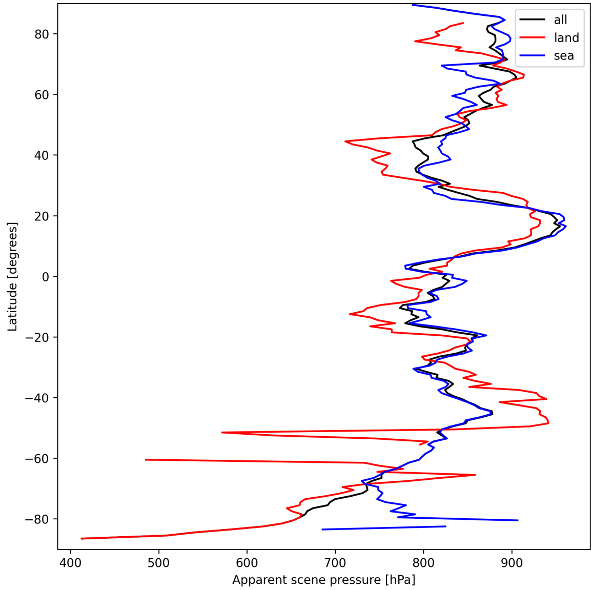
Figure 19: Zonal average of “Apparent scene pressure” for 2025-03-24 to 2025-03-26.
