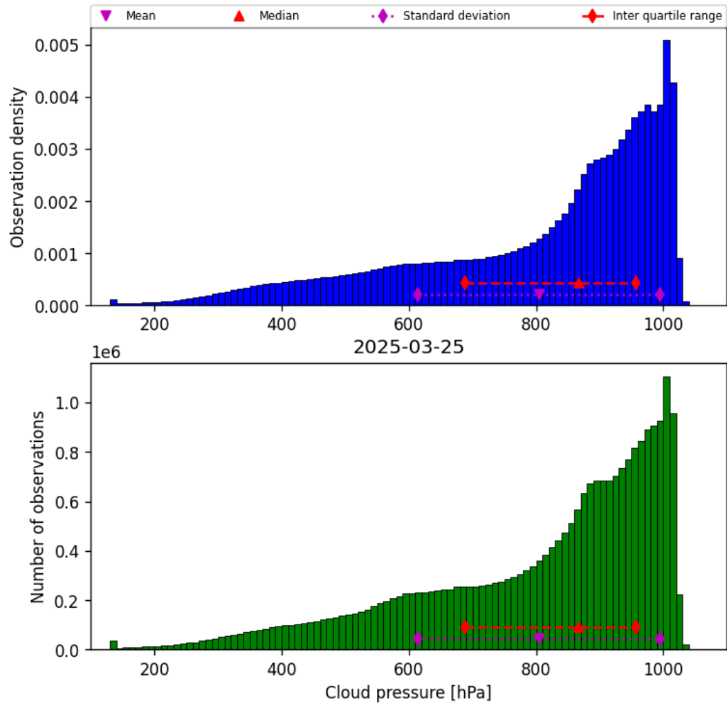
Figure 30: Histogram of “Cloud pressure” for 2025-03-24 to 2025-03-26
