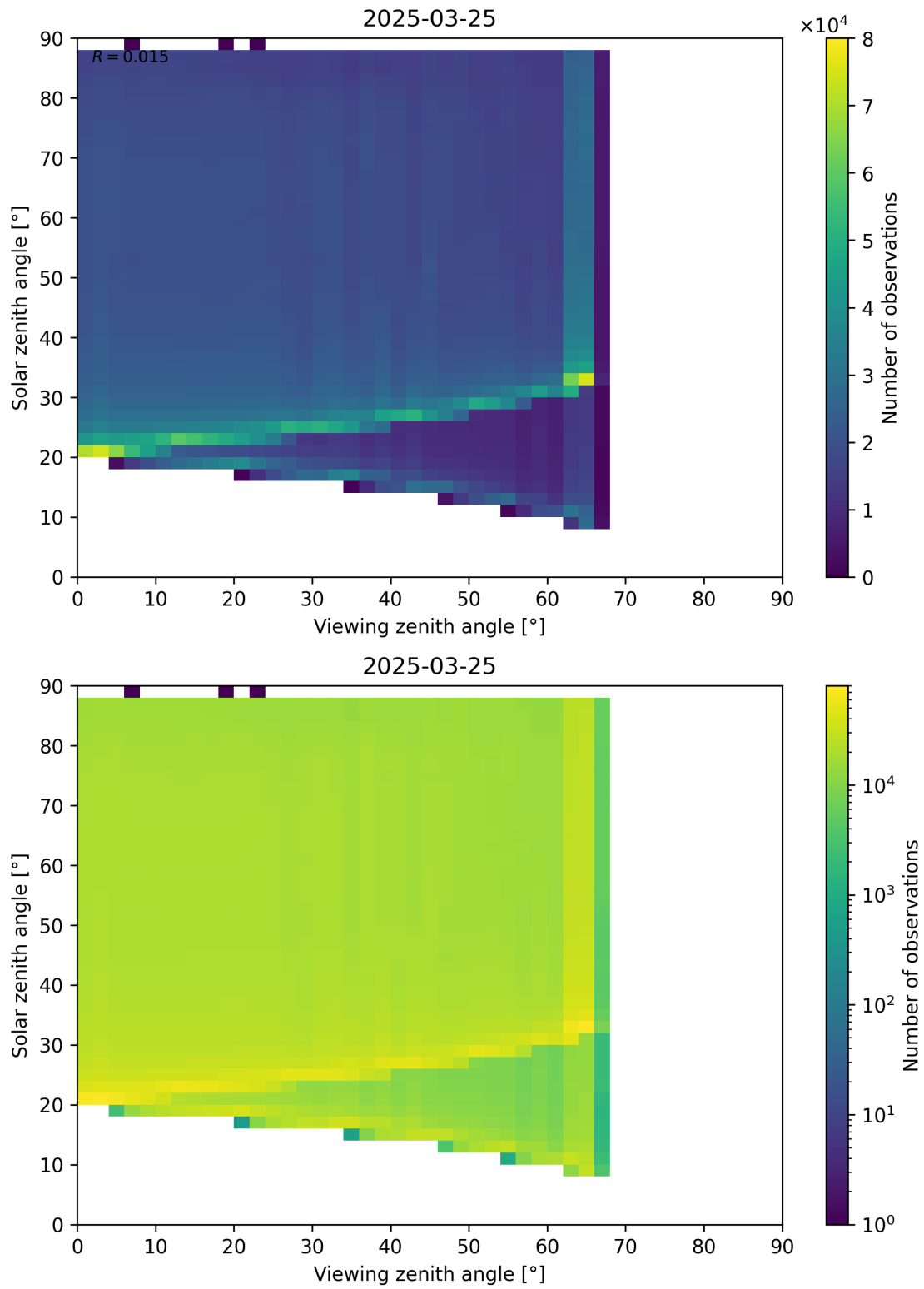
Figure 127: Scatter density plot of “Viewing zenith angle” against “Solar zenith angle” for 2025-03-24 to 2025-03-26.
