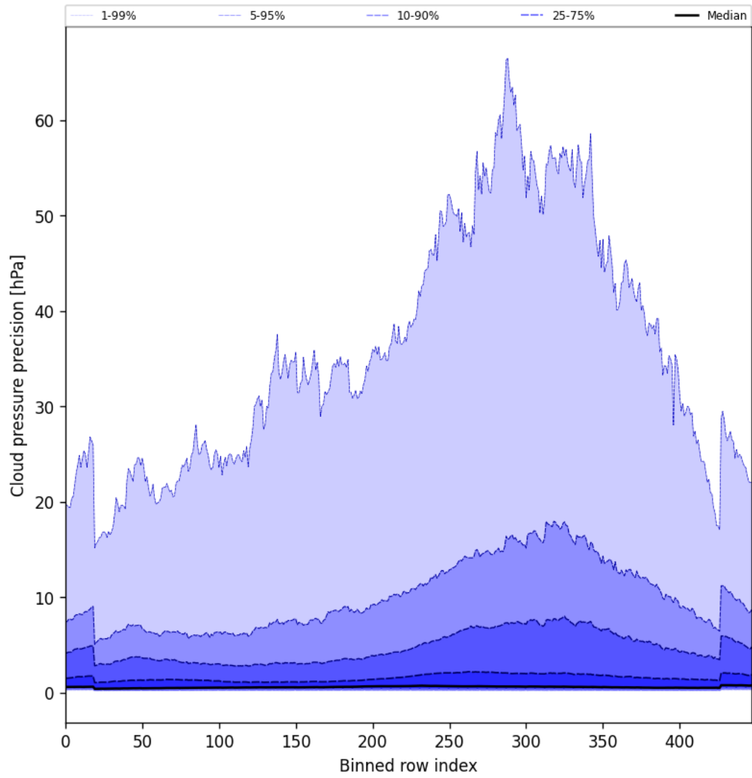
Figure 48: Along track statistics of “Cloud pressure precision” for 2025-03-24 to 2025-03-26
