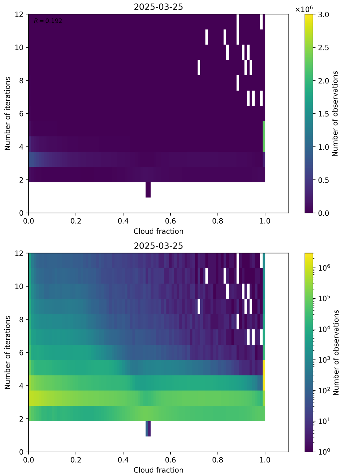
Figure 73: Scatter density plot of “Cloud fraction” against “Number of iterations” for 2025-03-24 to 2025-03-26.
