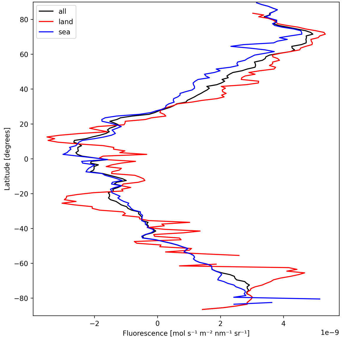
Figure 23: Zonal average of “Fluorescence” for 2025-03-24 to 2025-03-26.
