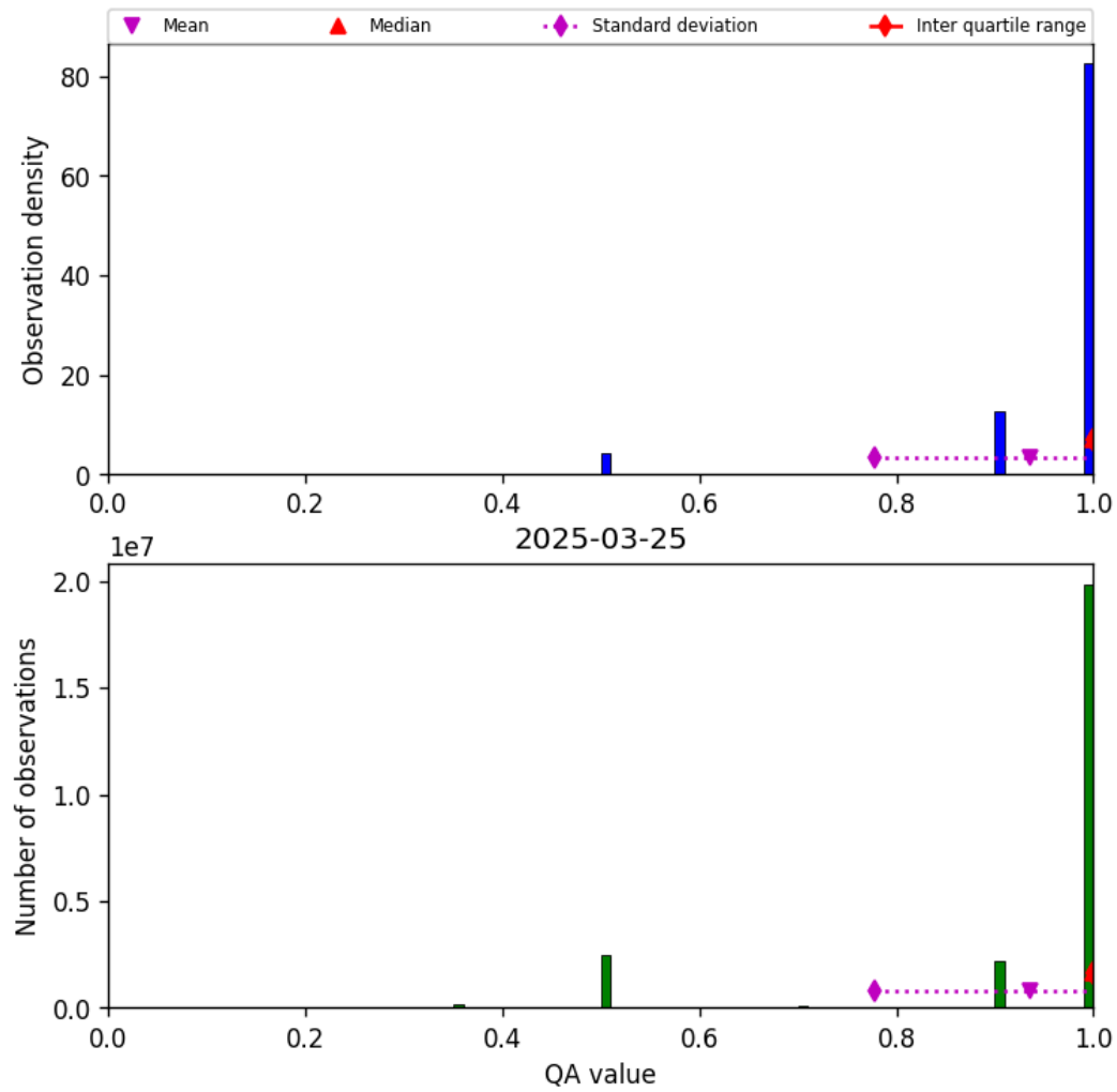
Figure 29: Histogram of “QA value” for 2025-03-24 to 2025-03-26
