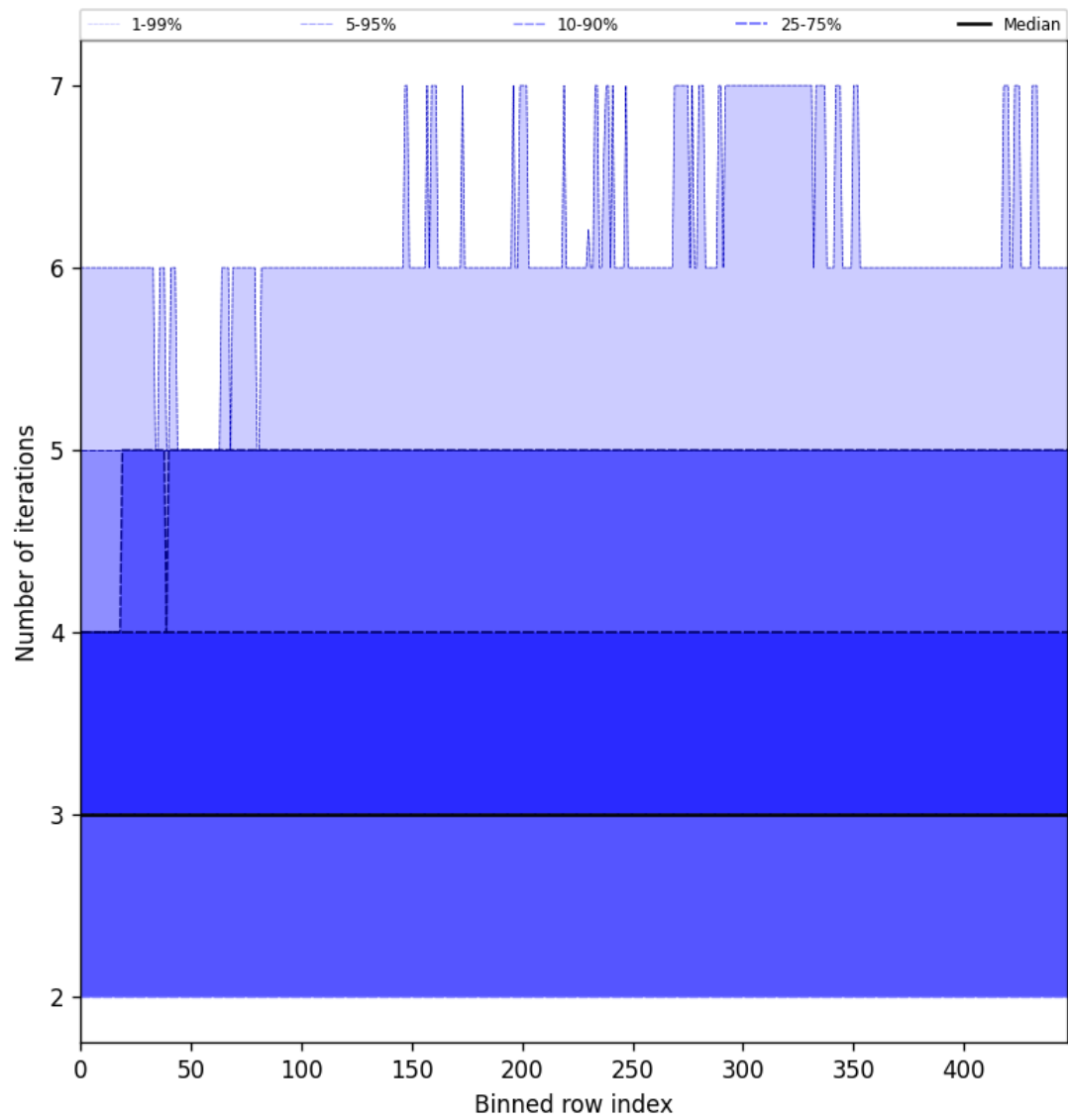
Figure 56: Along track statistics of “Number of iterations” for 2025-03-24 to 2025-03-26
