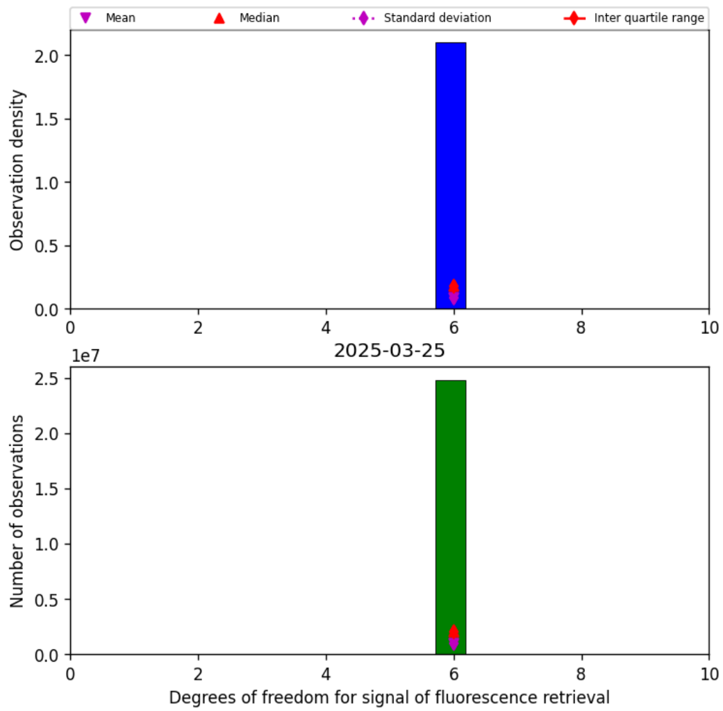
Figure 43: Histogram of "Degrees of freedom for signal of fluorescence retrieval" for 2025-03-24 to 2025-03-26
