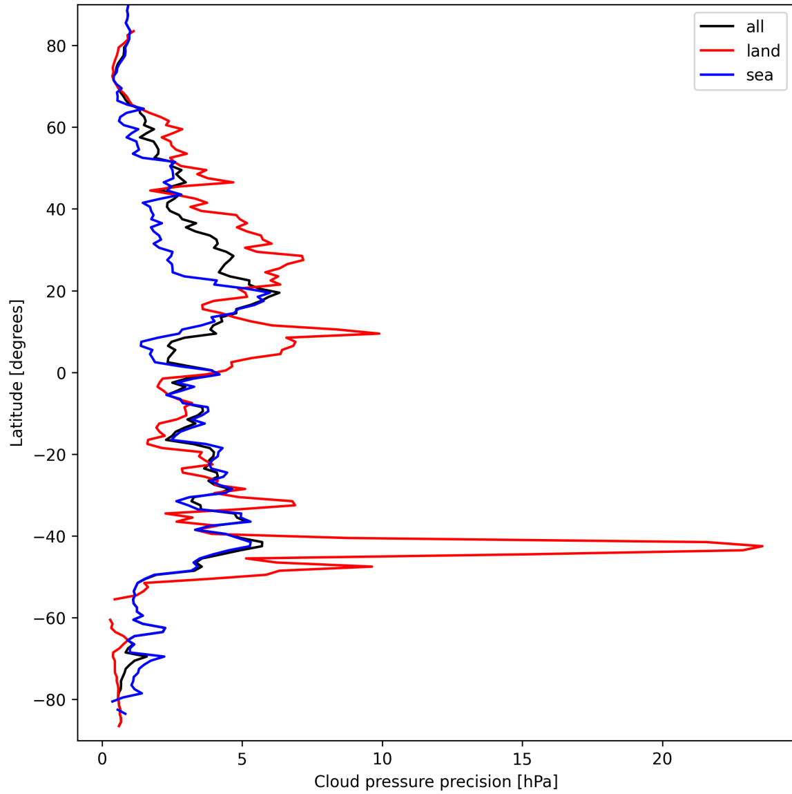
Figure 14: Zonal average of “Cloud pressure precision” for 2025-03-24 to 2025-03-26.
