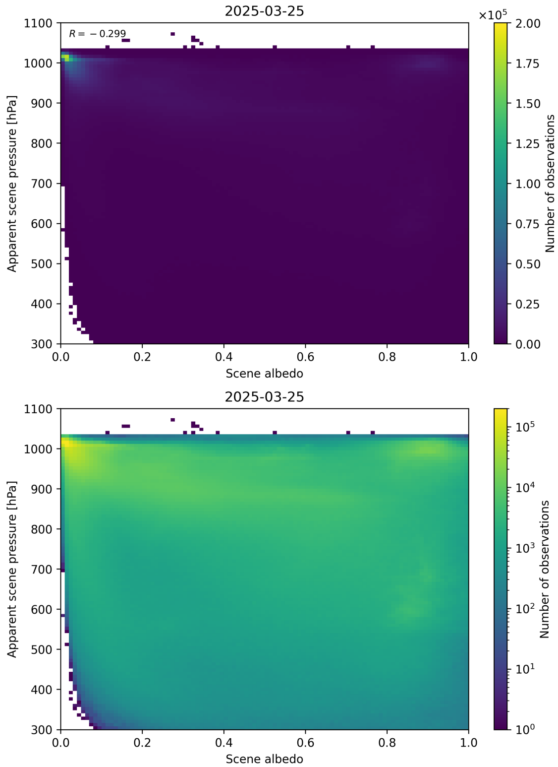
Figure 102: Scatter density plot of “Scene albedo” against “Apparent scene pressure” for 2025-03-24 to 2025-03-26.
