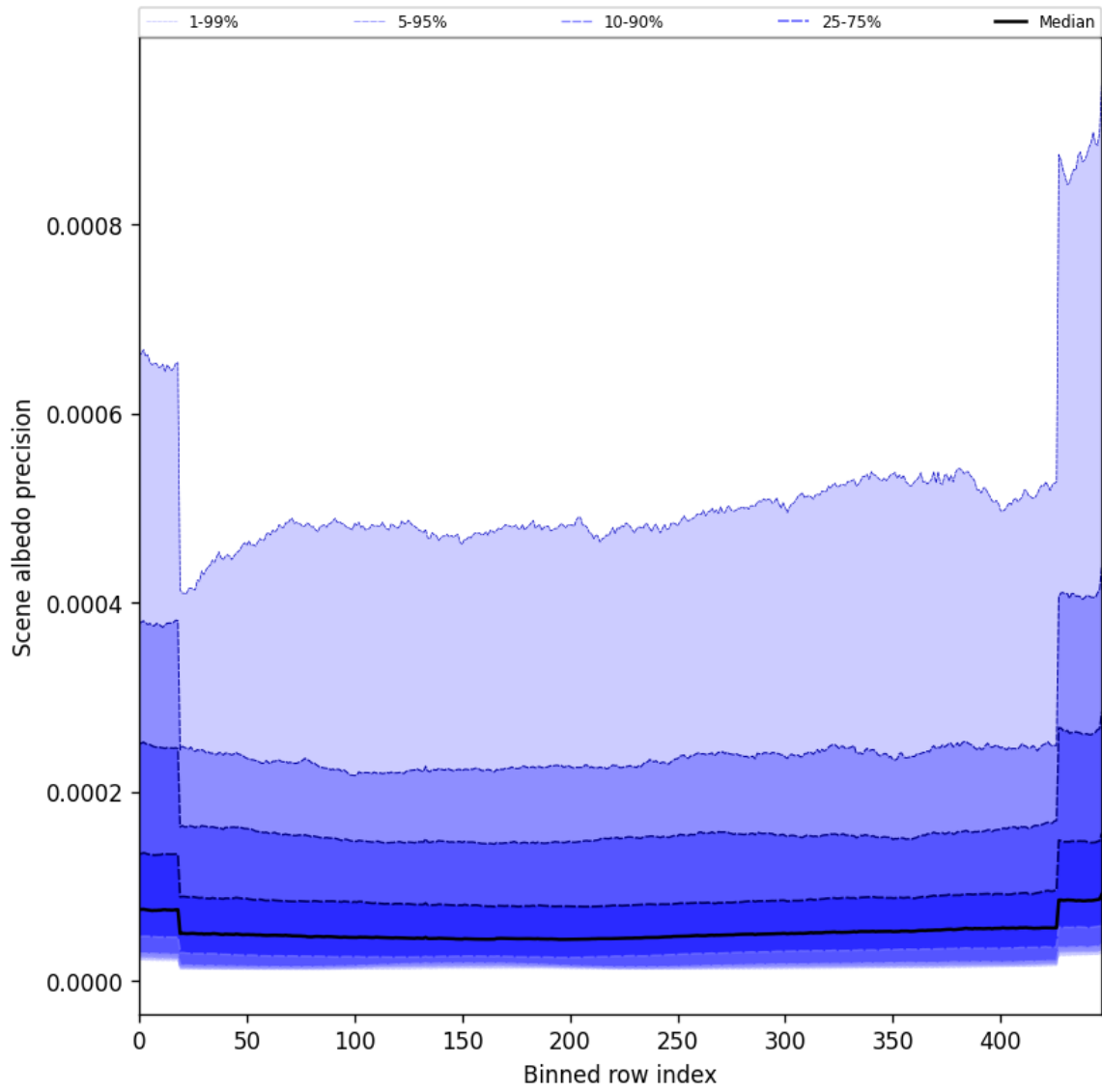
Figure 52: Along track statistics of “Scene albedo precision” for 2025-03-24 to 2025-03-26
