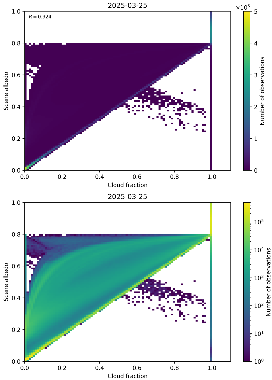
Figure 75: Scatter density plot of “Cloud fraction” against “Scene albedo” for 2025-03-24 to 2025-03-26.
