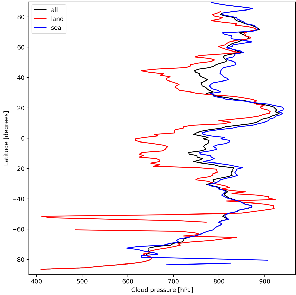
Figure 13: Zonal average of “Cloud pressure” for 2025-03-24 to 2025-03-26.
