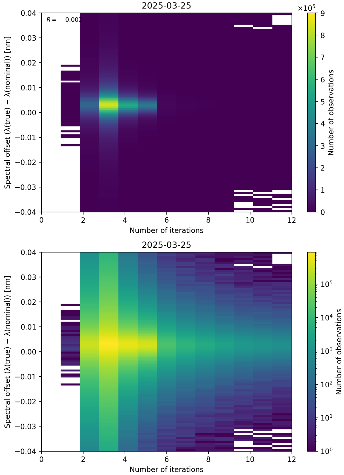
Figure 100: Scatter density plot of “Number of iterations” against “Spectral offset ( \lambda_{\text{true}} - \lambda_{\text{nominal}} )” for 2025-03-24 to 2025-03-26.
