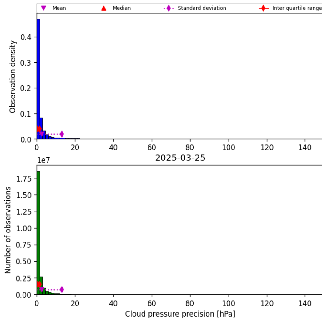
Figure 31: Histogram of “Cloud pressure precision” for 2025-03-24 to 2025-03-26
