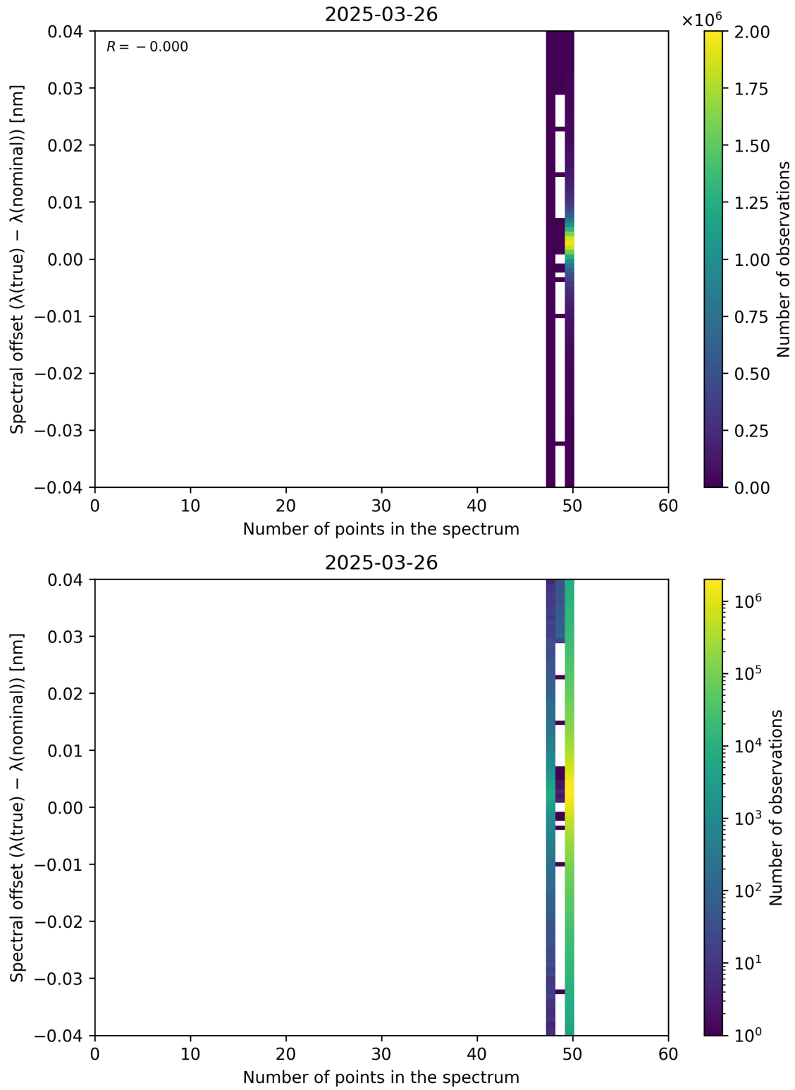
Figure 101: Scatter density plot of “Number of points in the spectrum” against “Spectral offset ( \lambda_{\text{true}} - \lambda_{\text{nominal}} )” for 2025-03-25 to 2025-03-27.
