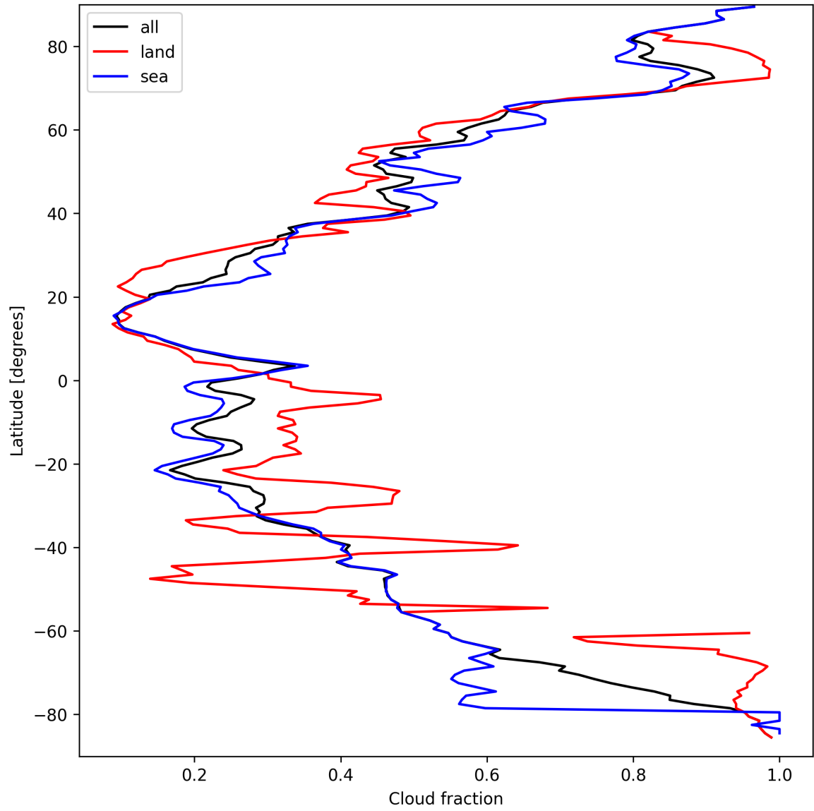
Figure 15: Zonal average of “Cloud fraction” for 2025-03-25 to 2025-03-27.
