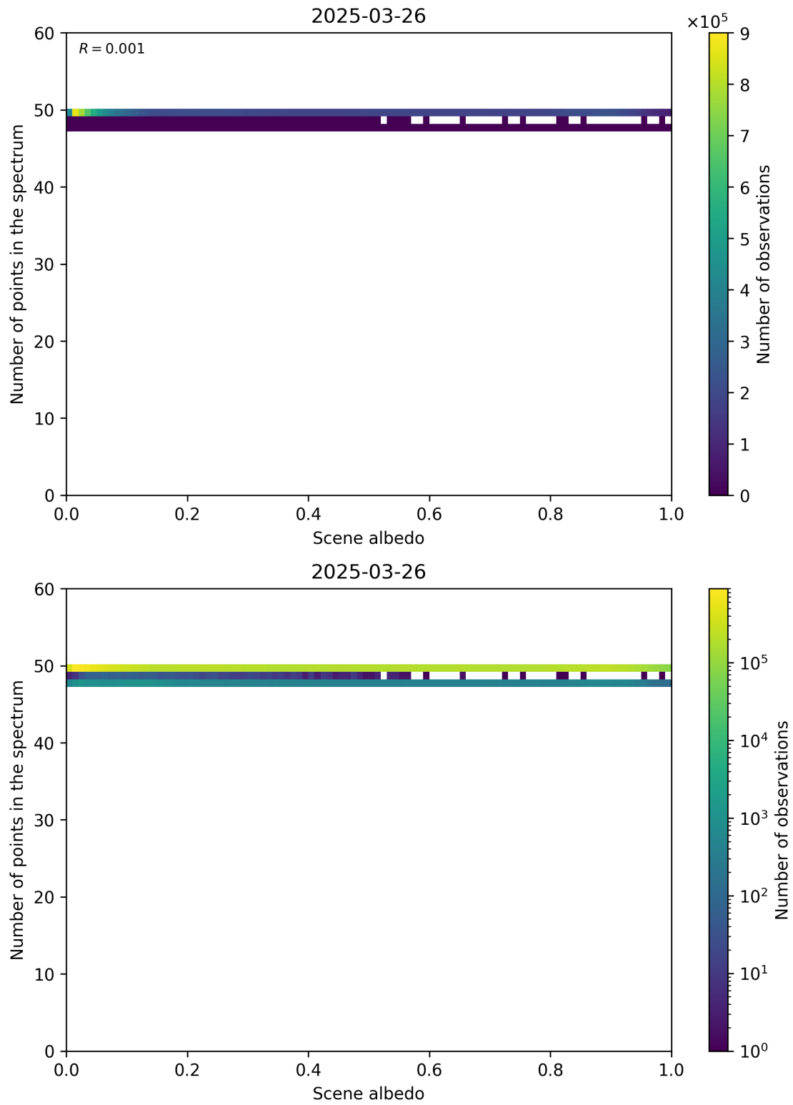
Figure 106: Scatter density plot of “Scene albedo” against “Number of points in the spectrum” for 2025-03-25 to 2025-03-27.
