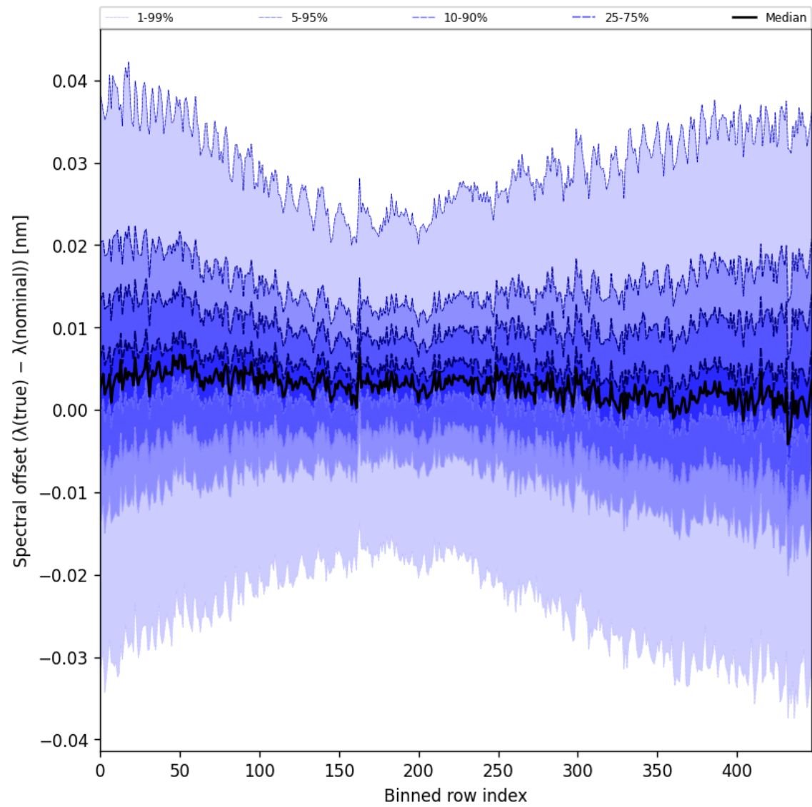
Figure 62: Along track statistics of “Spectral offset ( \lambda_{\text{true}} - \lambda_{\text{nominal}} )” for 2025-03-25 to 2025-03-27
