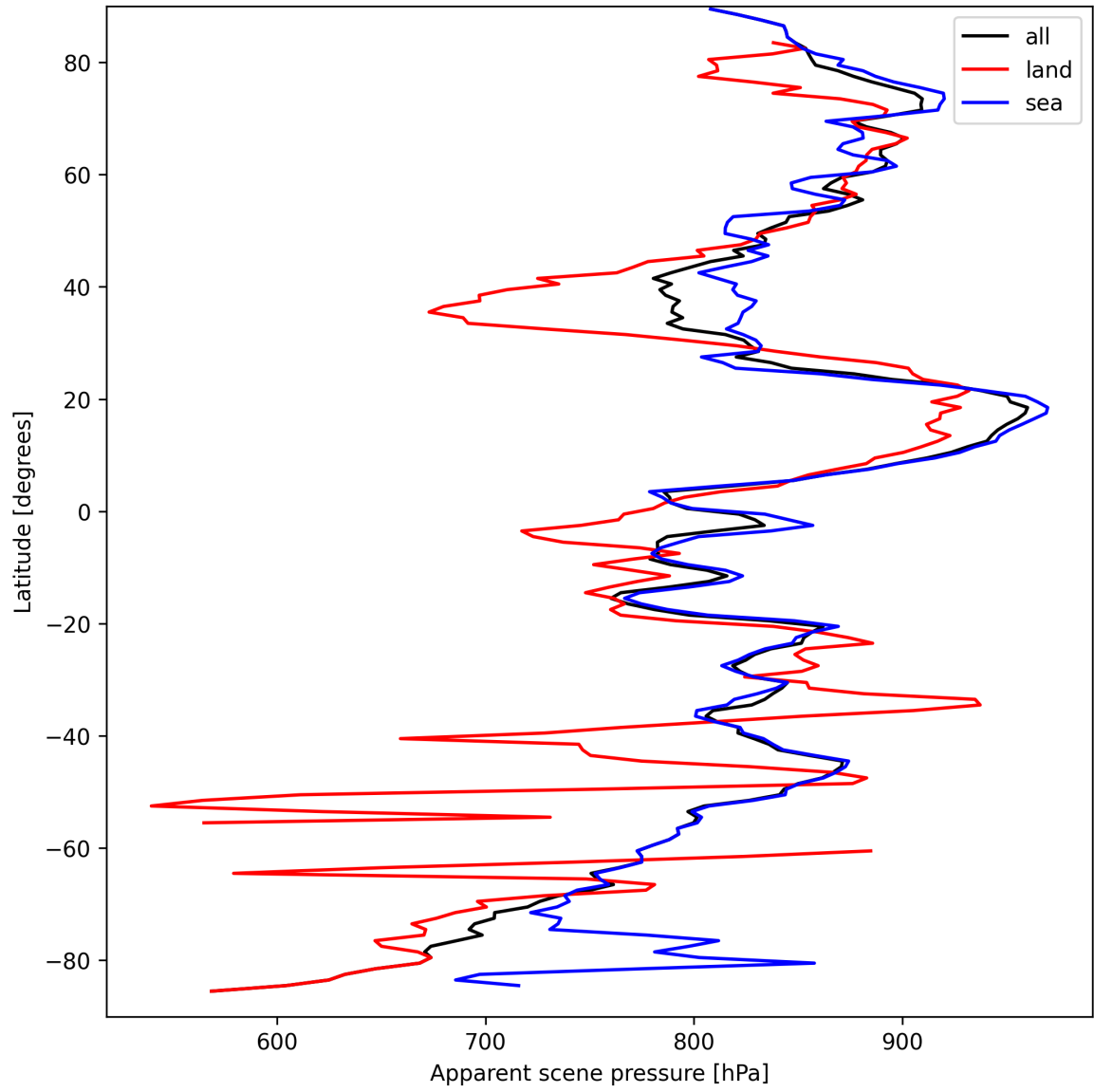
Figure 19: Zonal average of “Apparent scene pressure” for 2025-03-25 to 2025-03-27.
