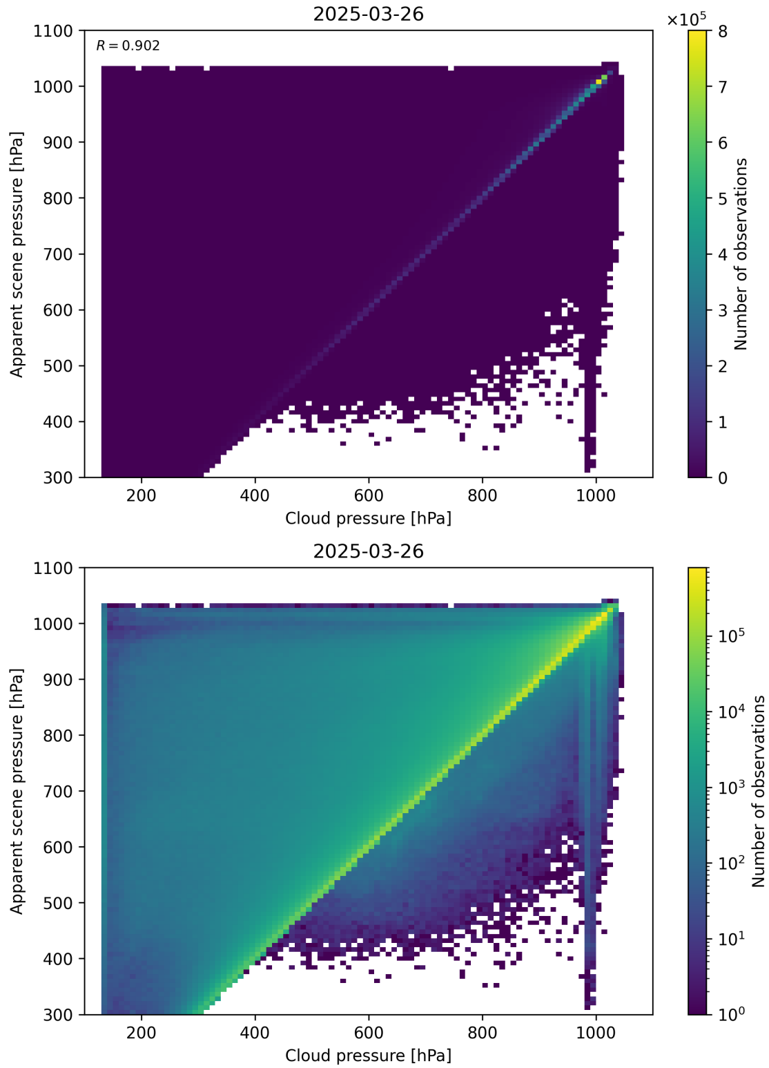
Figure 77: Scatter density plot of “Cloud pressure” against “Apparent scene pressure” for 2025-03-25 to 2025-03-27.
