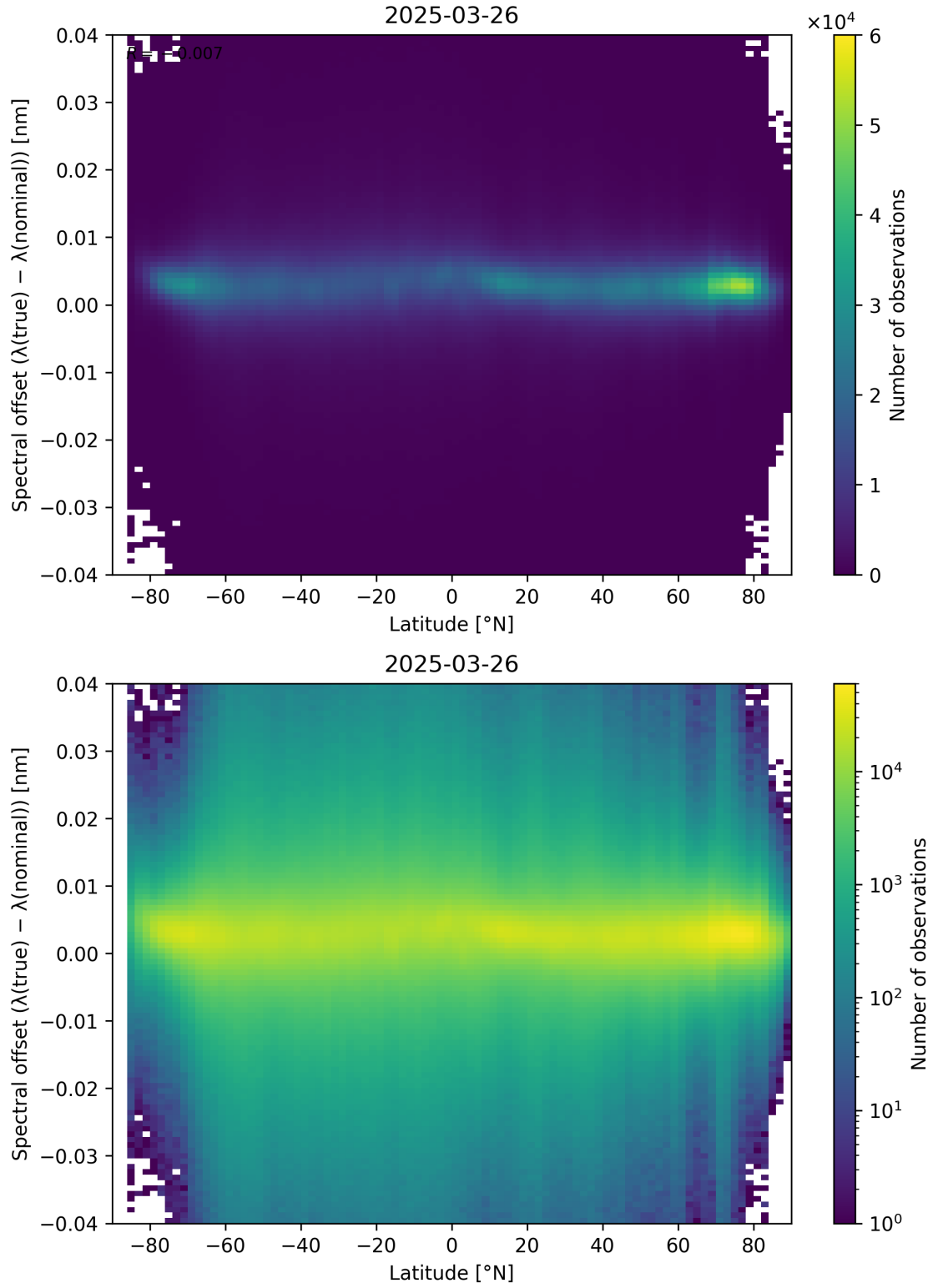
Figure 96: Scatter density plot of “Latitude” against “Spectral offset ( \lambda_{\text{true}} - \lambda_{\text{nominal}} )” for 2025-03-25 to 2025-03-27.
