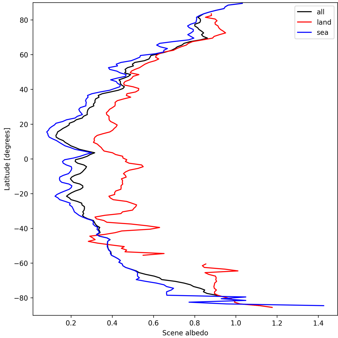
Figure 17: Zonal average of “Scene albedo” for 2025-03-25 to 2025-03-27.
