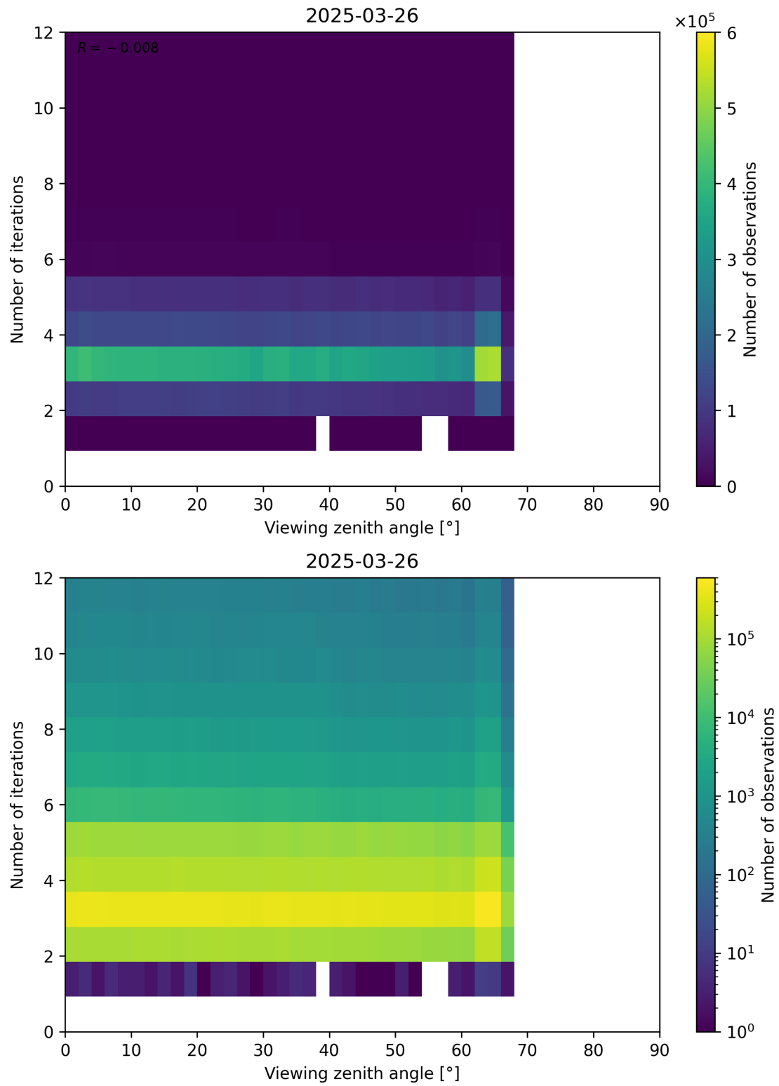
Figure 124: Scatter density plot of “Viewing zenith angle” against “Number of iterations” for 2025-03-25 to 2025-03-27.
