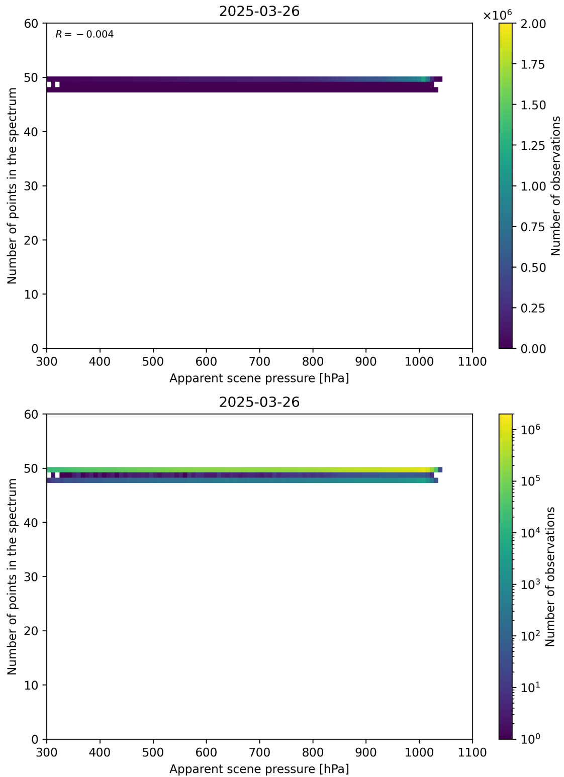
Figure 66: Scatter density plot of “Apparent scene pressure” against “Number of points in the spectrum” for 2025-03-25 to 2025-03-27.
