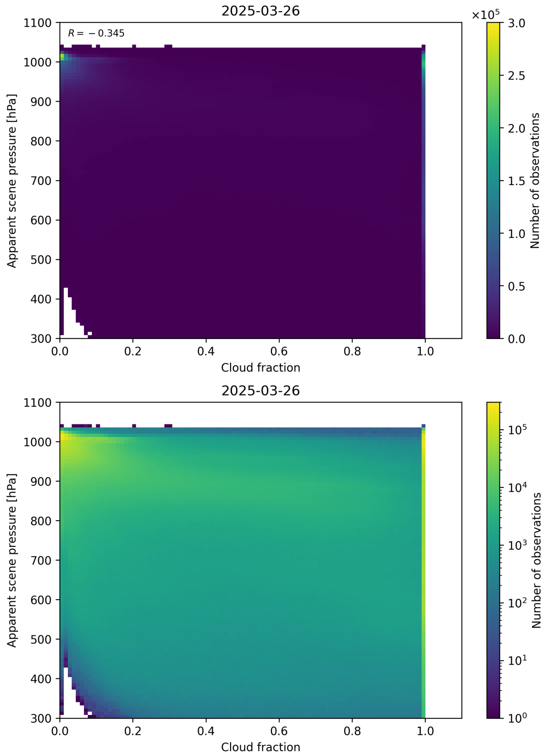
Figure 70: Scatter density plot of “Cloud fraction” against “Apparent scene pressure” for 2025-03-25 to 2025-03-27.
