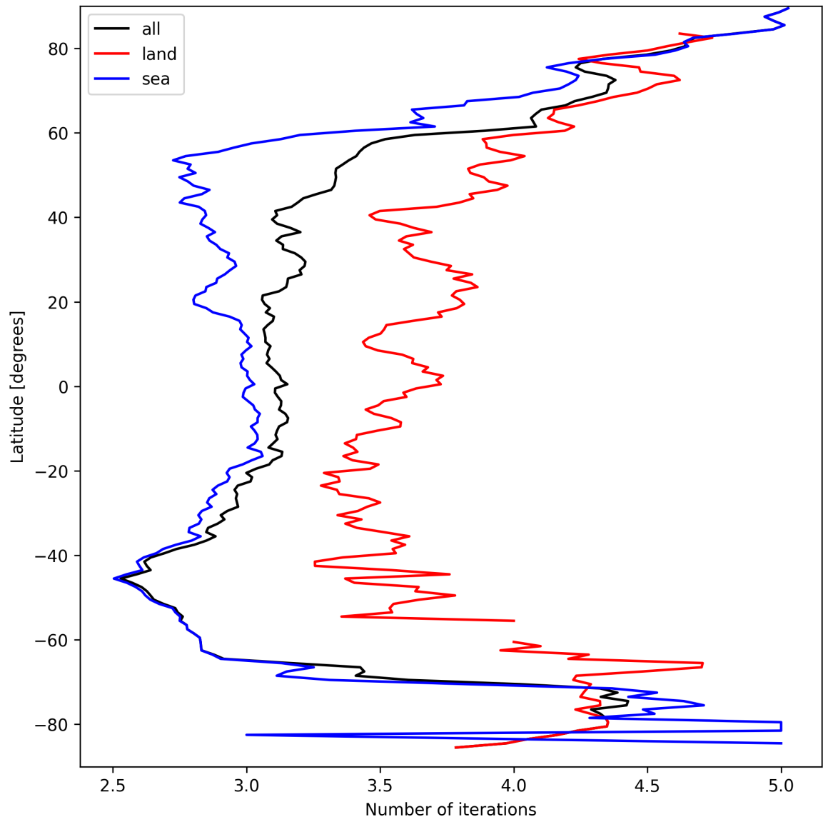
Figure 22: Zonal average of “Number of iterations” for 2025-03-25 to 2025-03-27.
