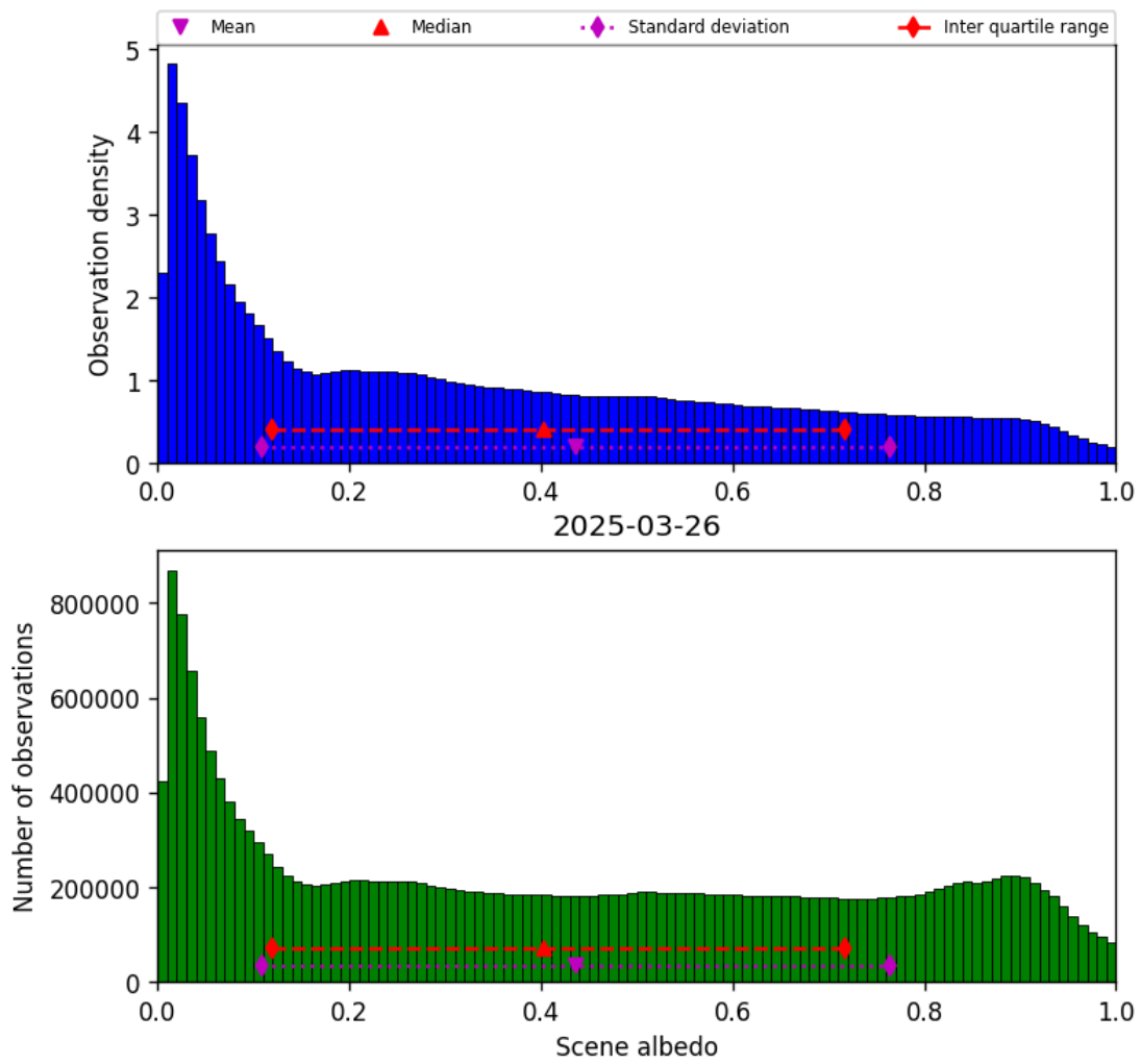
Figure 34: Histogram of “Scene albedo” for 2025-03-25 to 2025-03-27
