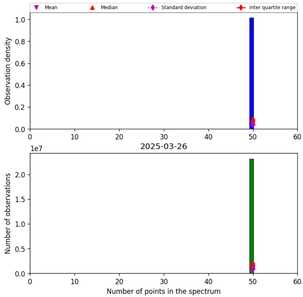
Figure 44: Histogram of “Number of points in the spectrum” for 2025-03-25 to 2025-03-27
