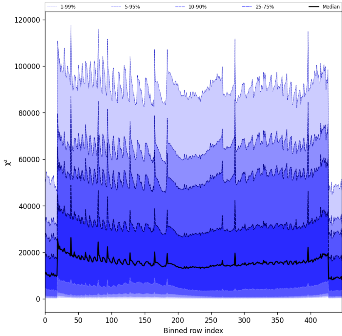
Figure 55: Along track statistics of “ \chi^2 ” for 2025-03-25 to 2025-03-27
