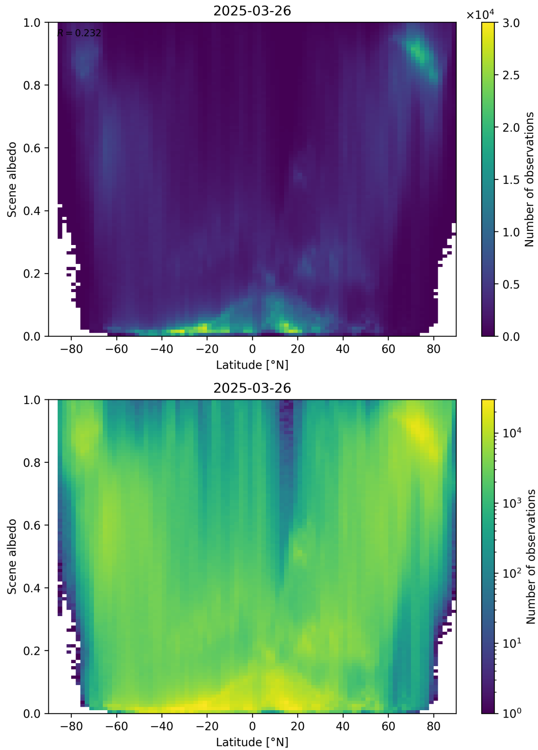
Figure 95: Scatter density plot of “Latitude” against “Scene albedo” for 2025-03-25 to 2025-03-27.
