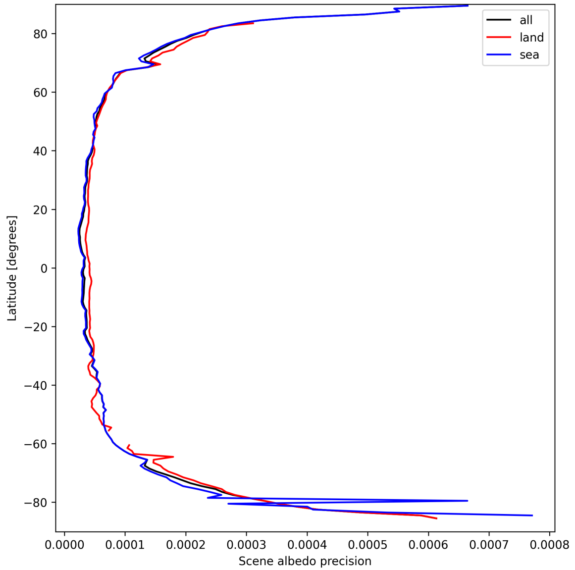
Figure 18: Zonal average of “Scene albedo precision” for 2025-03-25 to 2025-03-27.
