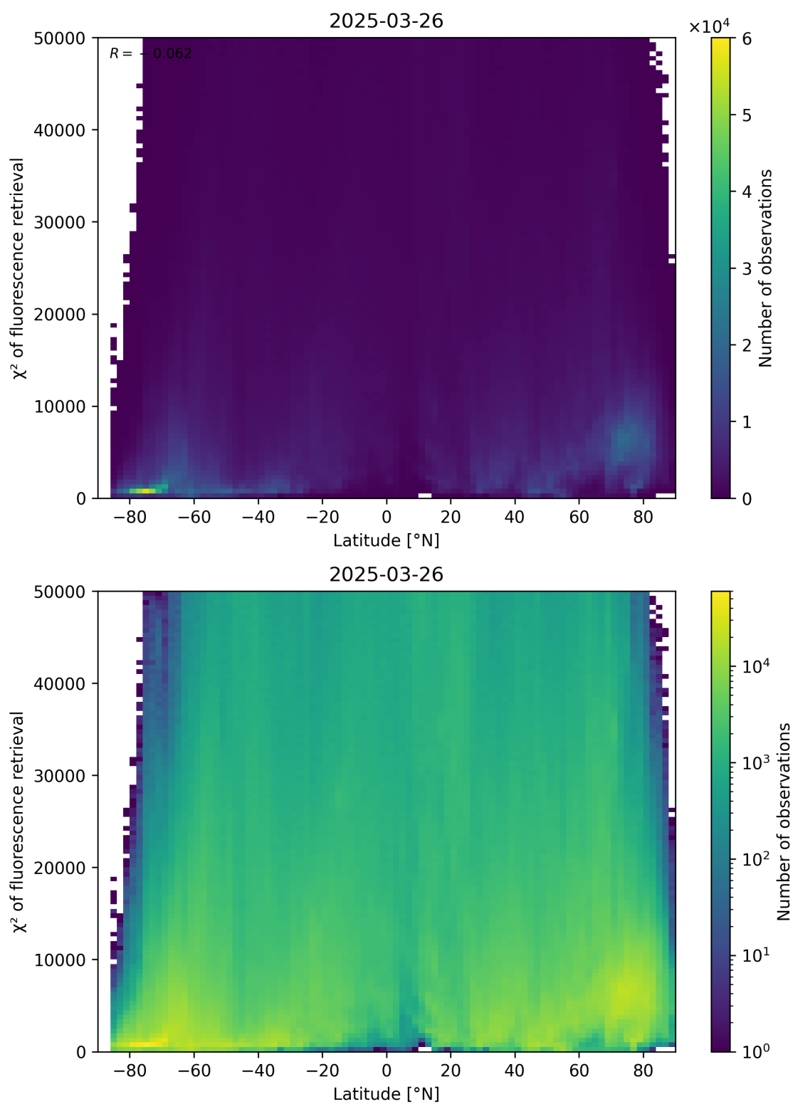
Figure 89: Scatter density plot of “Latitude” against “ \chi^2 of fluorescence retrieval” for 2025-03-25 to 2025-03-27.
