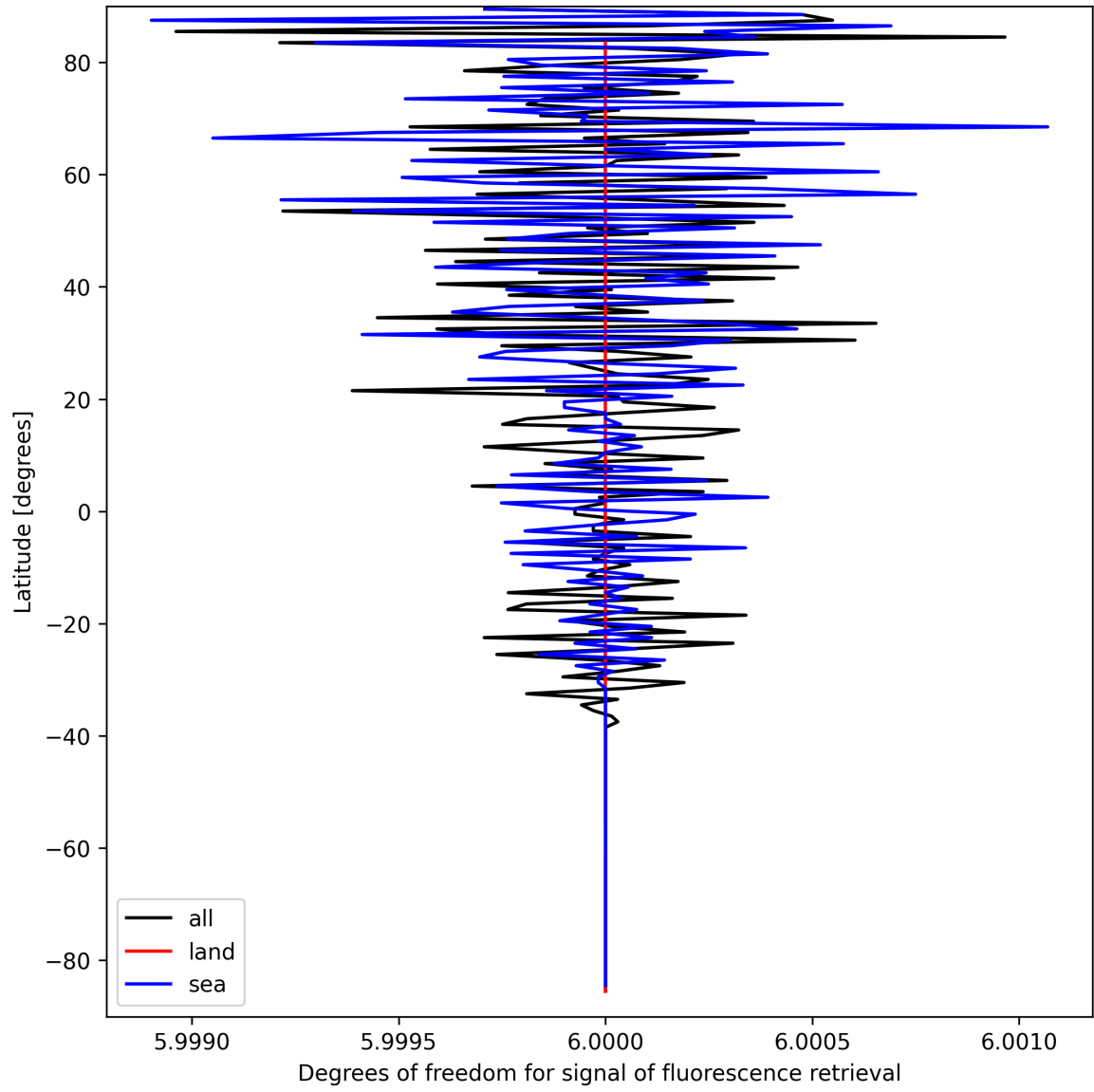
Figure 26: Zonal average of “Degrees of freedom for signal of fluorescence retrieval” for 2025-03-25 to 2025-03-27.
