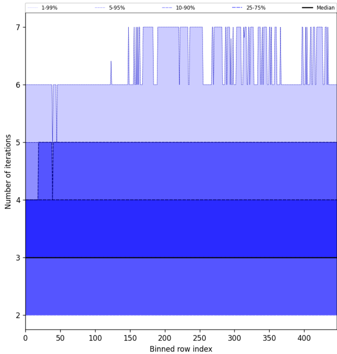
Figure 56: Along track statistics of “Number of iterations” for 2025-03-25 to 2025-03-27
