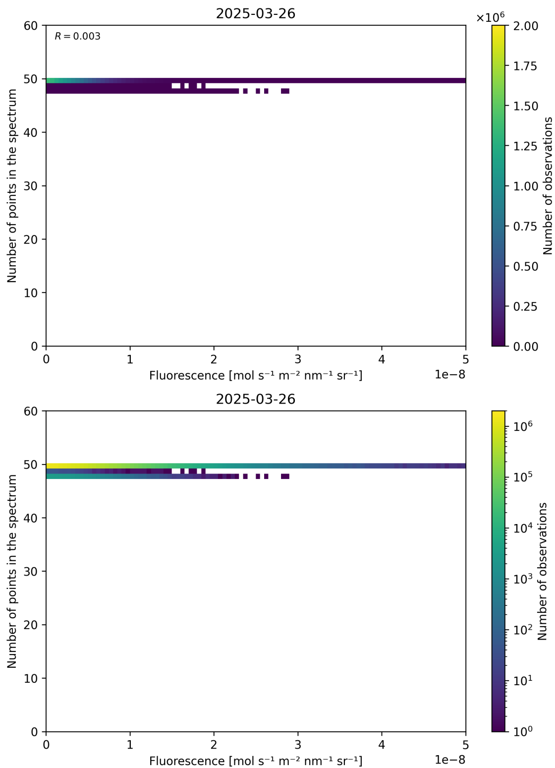
Figure 86: Scatter density plot of “Fluorescence” against “Number of points in the spectrum” for 2025-03-25 to 2025-03-27.
