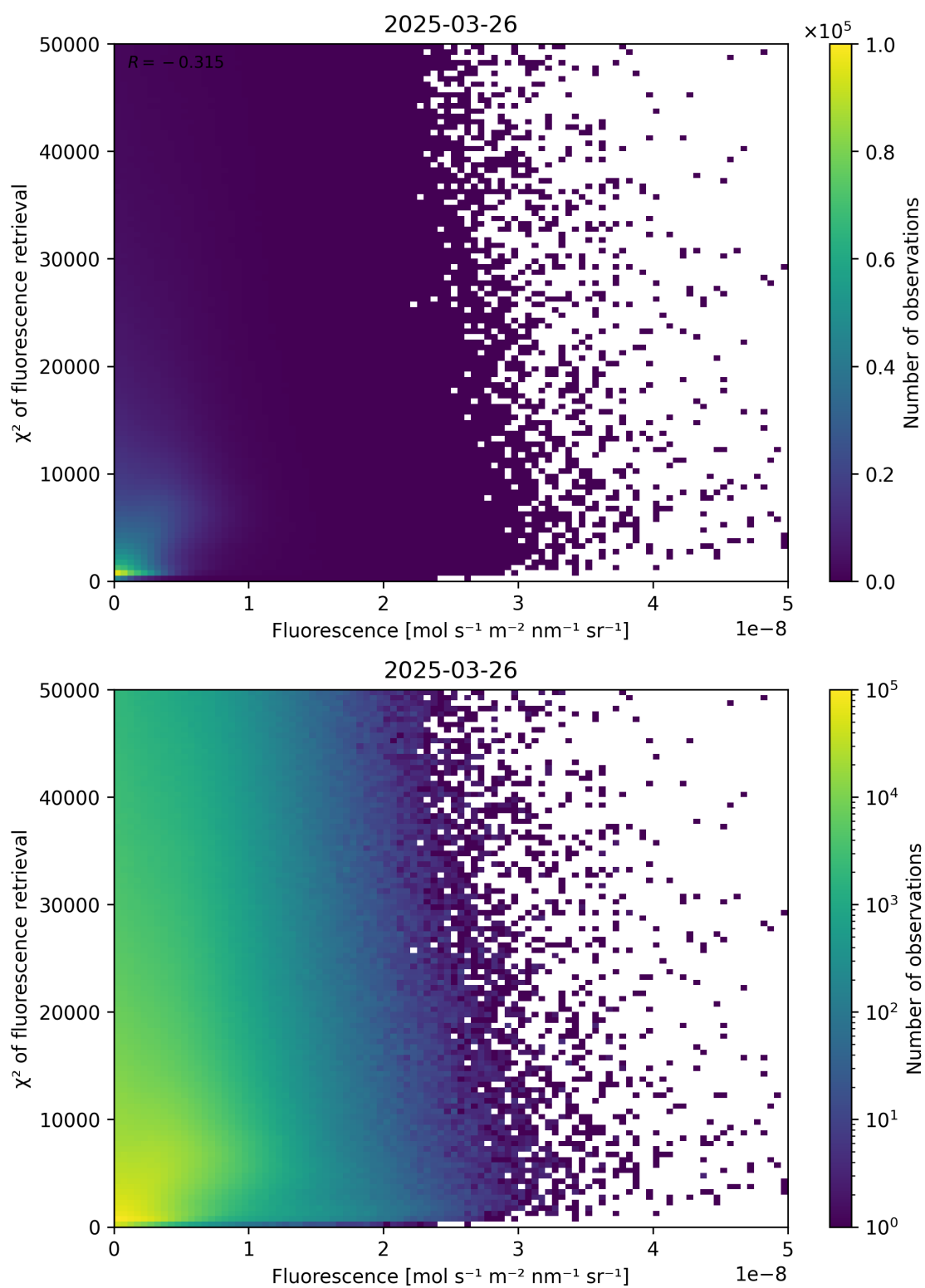
Figure 85: Scatter density plot of “Fluorescence” against “ \chi^2 of fluorescence retrieval” for 2025-03-25 to 2025-03-27.
