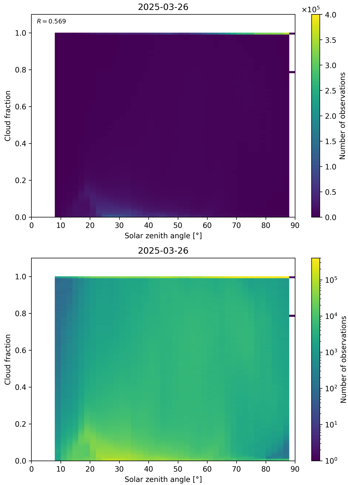
Figure 110: Scatter density plot of “Solar zenith angle” against “Cloud fraction” for 2025-03-25 to 2025-03-27.
