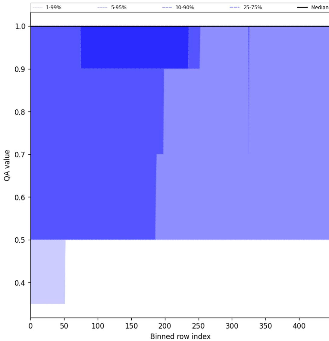
Figure 46: Along track statistics of “QA value” for 2025-03-25 to 2025-03-27
