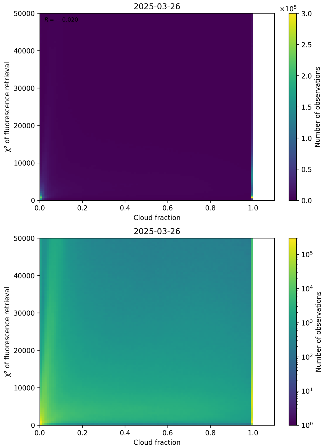
Figure 71: Scatter density plot of “Cloud fraction” against “ \chi^2 of fluorescence retrieval” for 2025-03-25 to 2025-03-27.
