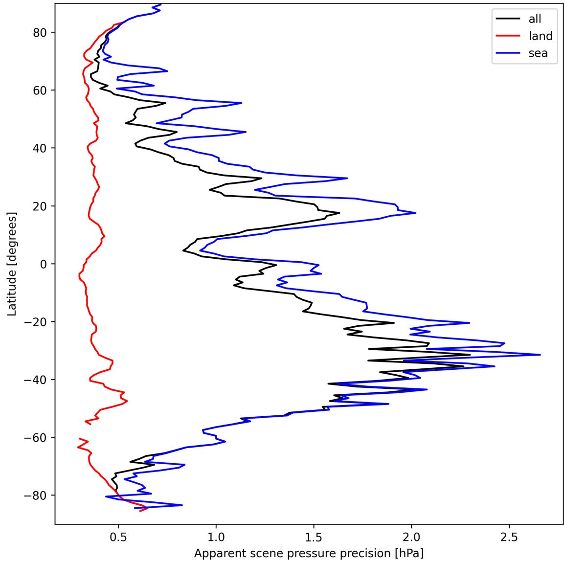
Figure 20: Zonal average of “Apparent scene pressure precision” for 2025-03-25 to 2025-03-27.
