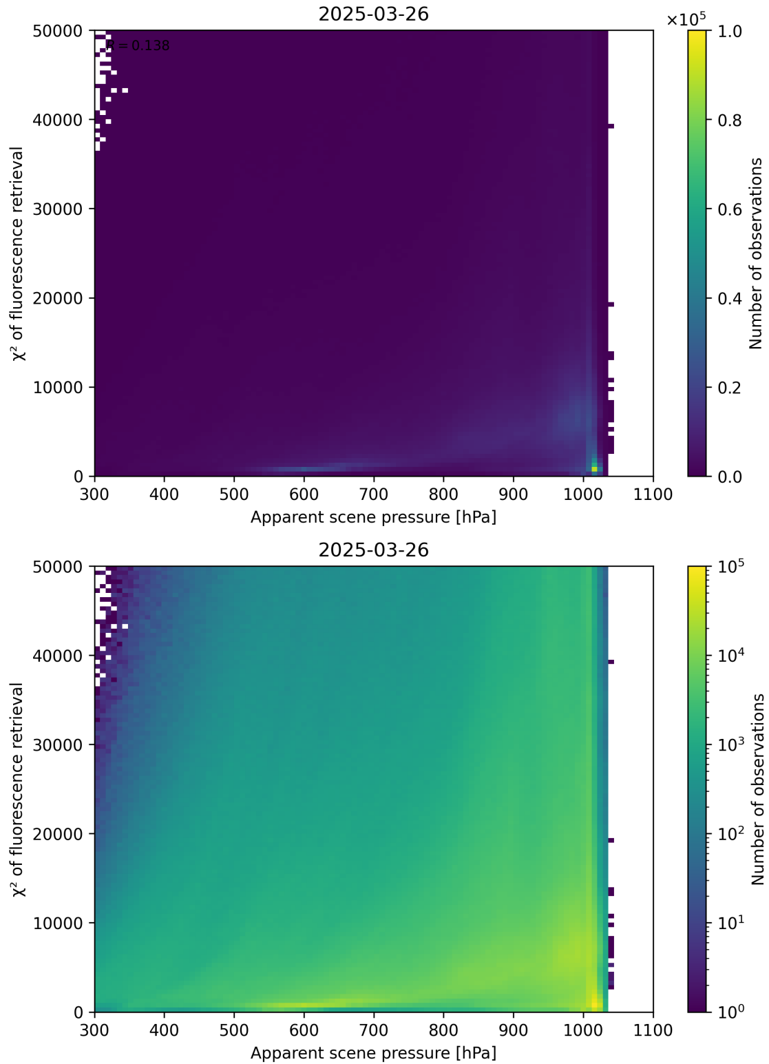
Figure 63: Scatter density plot of “Apparent scene pressure” against “ \chi^2 of fluorescence retrieval” for 2025-03-25 to 2025-03-27.
