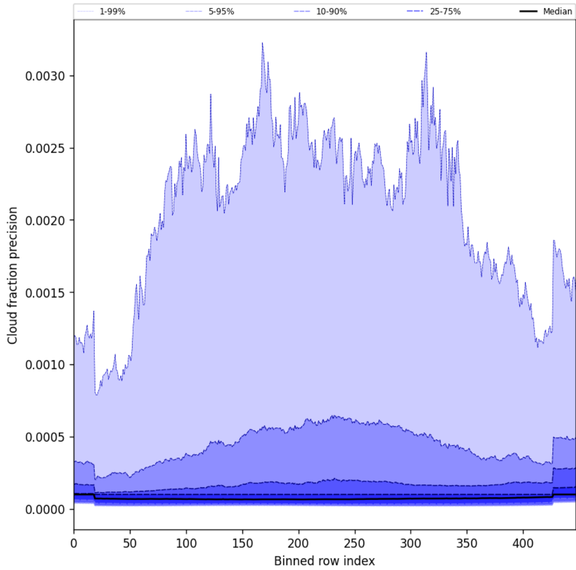
Figure 50: Along track statistics of “Cloud fraction precision” for 2025-03-25 to 2025-03-27
