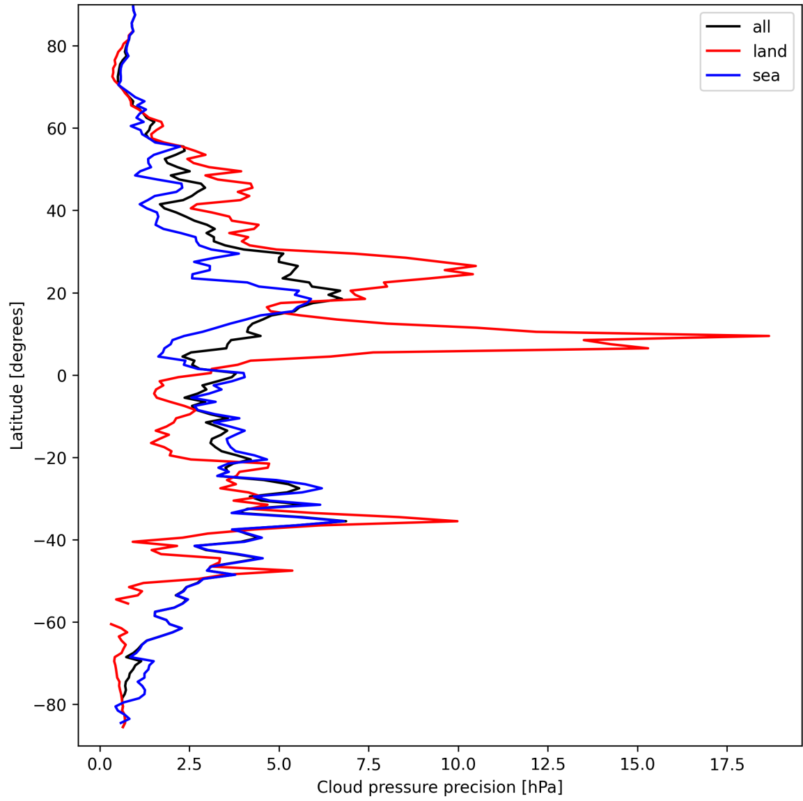
Figure 14: Zonal average of “Cloud pressure precision” for 2025-03-25 to 2025-03-27.
