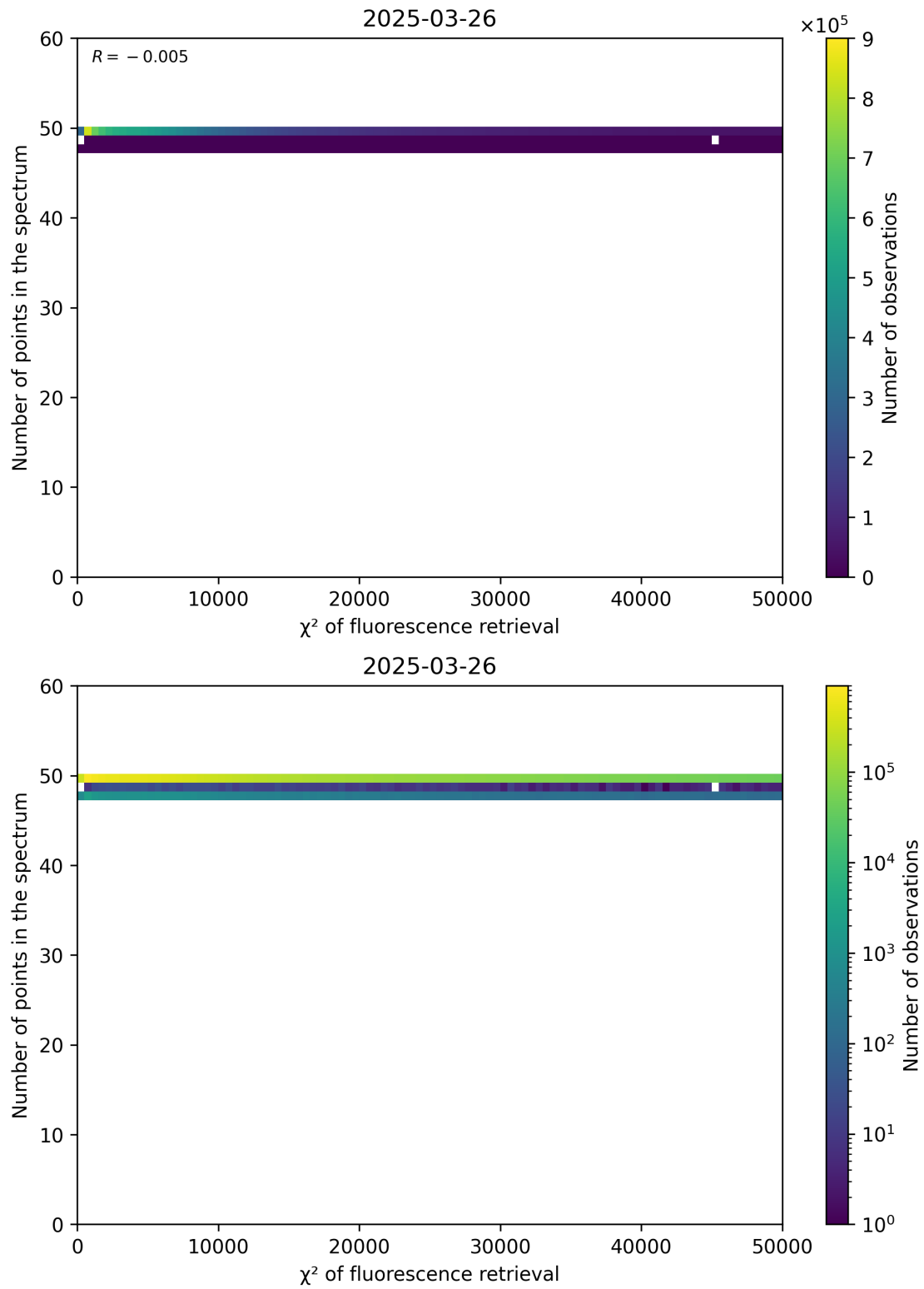
Figure 68: Scatter density plot of “ \chi^2 of fluorescence retrieval” against “Number of points in the spectrum” for 2025-03-25 to 2025-03-27.
