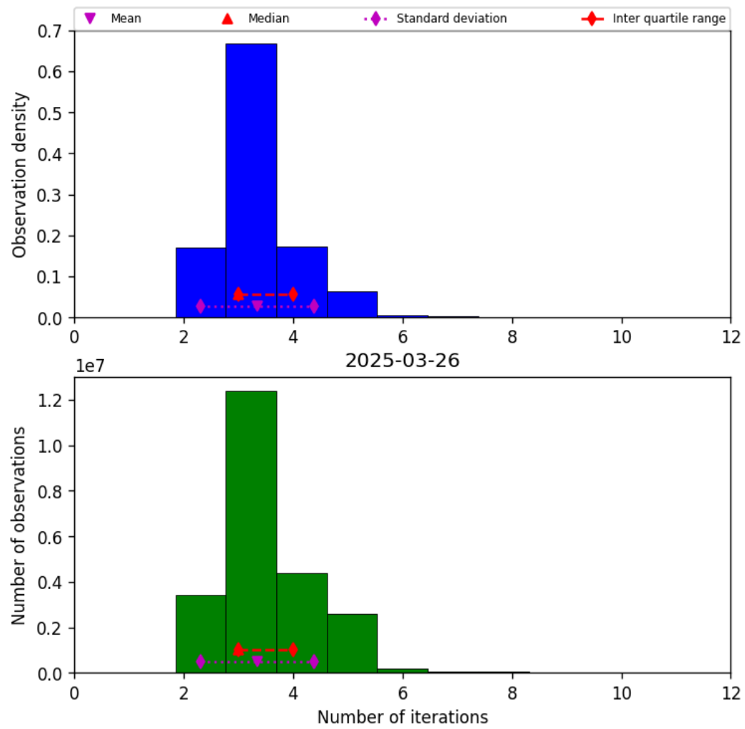
Figure 39: Histogram of “Number of iterations” for 2025-03-25 to 2025-03-27
