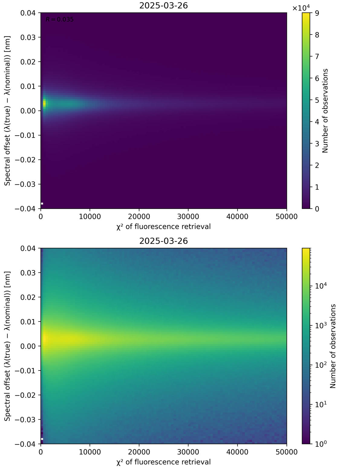
Figure 69: Scatter density plot of “ \chi^2 of fluorescence retrieval” against “Spectral offset ( \lambda_{\text{true}} - \lambda_{\text{nominal}} )” for 2025-03-25 to 2025-03-27.
