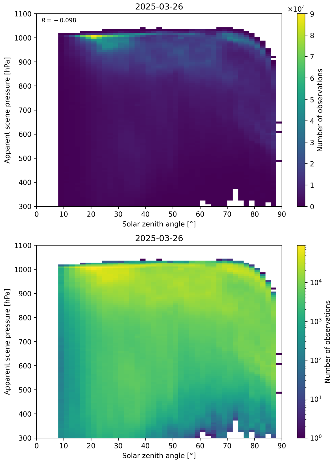
Figure 108: Scatter density plot of “Solar zenith angle” against “Apparent scene pressure” for 2025-03-25 to 2025-03-27.
