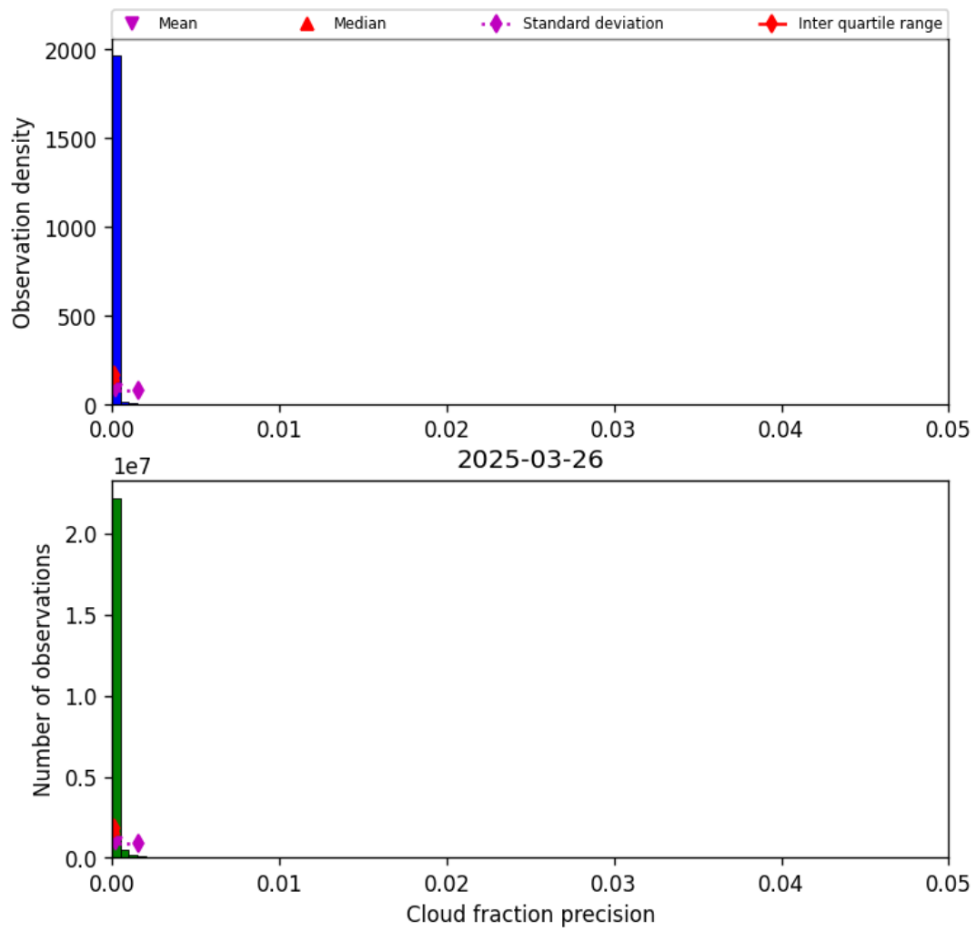
Figure 33: Histogram of “Cloud fraction precision” for 2025-03-25 to 2025-03-27
