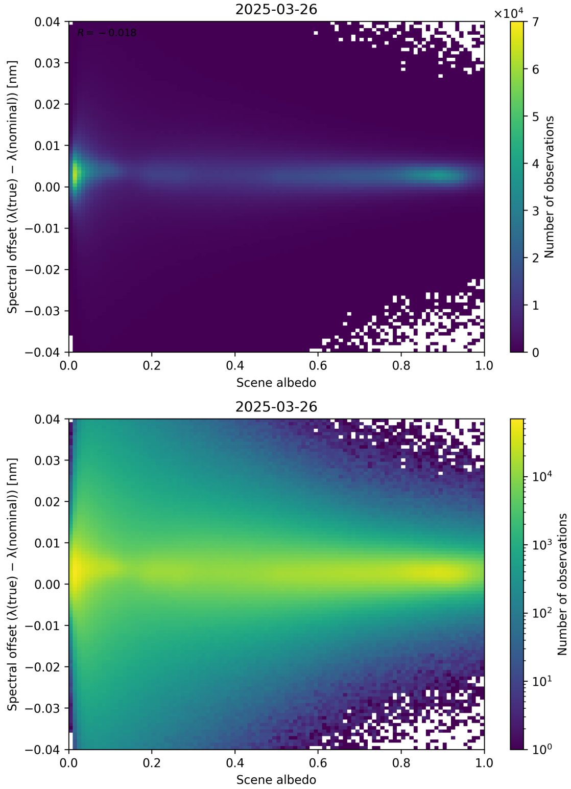
Figure 107: Scatter density plot of “Scene albedo” against “Spectral offset ( \lambda_{\text{true}} - \lambda_{\text{nominal}} )” for 2025-03-25 to 2025-03-27.
