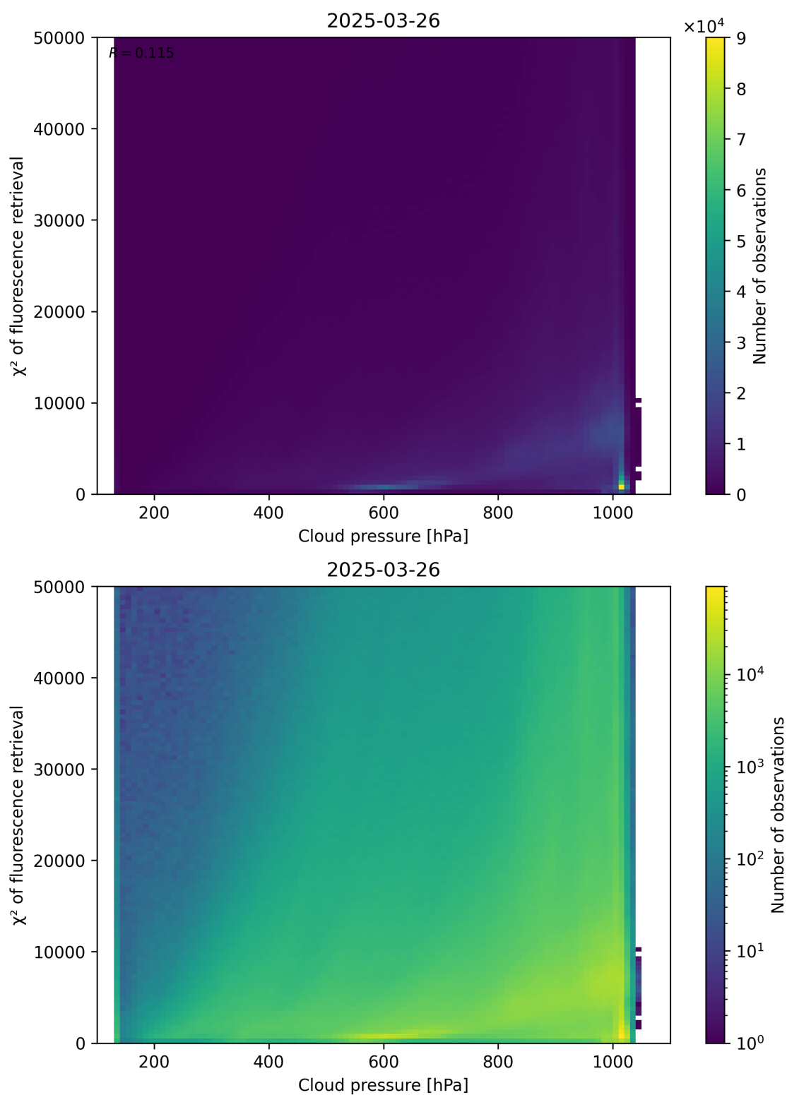
Figure 78: Scatter density plot of “Cloud pressure” against “ \chi^2 of fluorescence retrieval” for 2025-03-25 to 2025-03-27.
