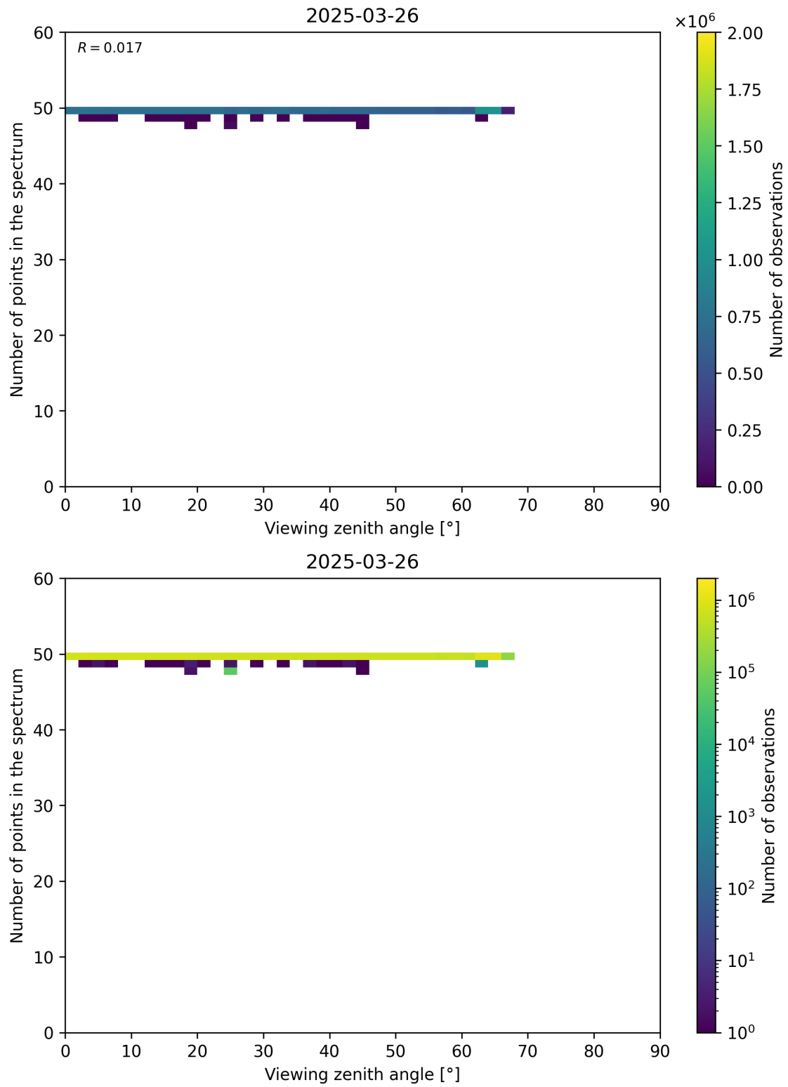
Figure 125: Scatter density plot of “Viewing zenith angle” against “Number of points in the spectrum” for 2025-03-25 to 2025-03-27.
