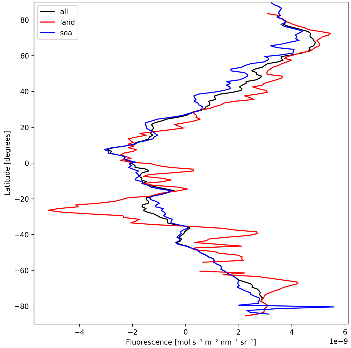
Figure 23: Zonal average of “Fluorescence” for 2025-03-25 to 2025-03-27.
