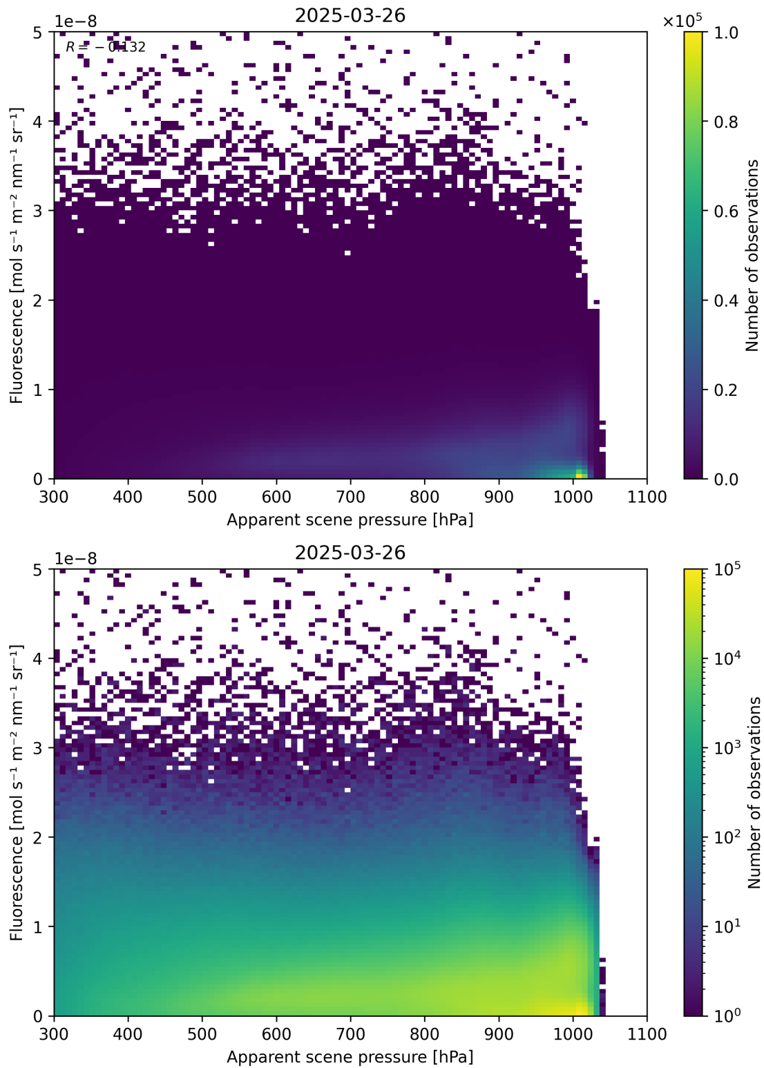
Figure 64: Scatter density plot of “Apparent scene pressure” against “Fluorescence” for 2025-03-25 to 2025-03-27.
