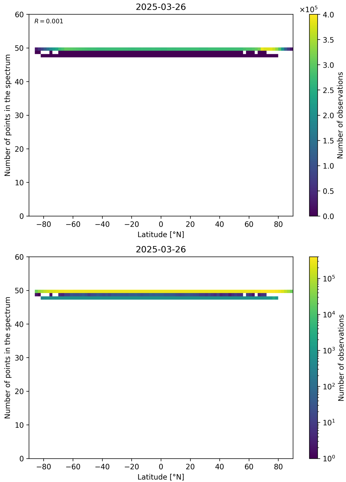
Figure 94: Scatter density plot of “Latitude” against “Number of points in the spectrum” for 2025-03-25 to 2025-03-27.
