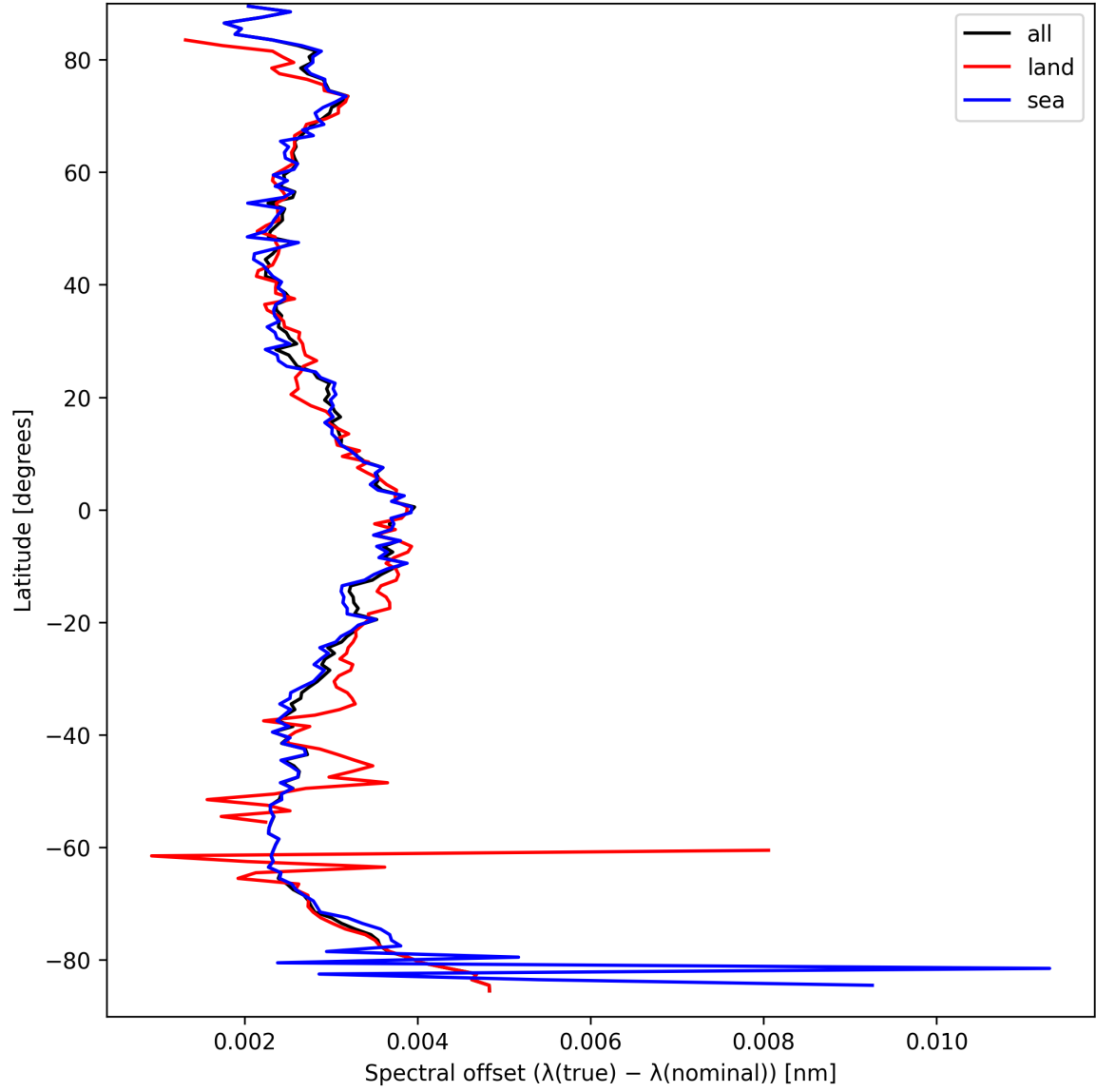
Figure 28: Zonal average of “Spectral offset ( \lambda_{\text{true}} - \lambda_{\text{nominal}} )” for 2025-03-25 to 2025-03-27.
