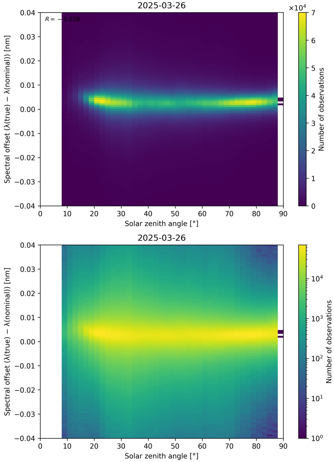
Figure 117: Scatter density plot of “Solar zenith angle” against “Spectral offset ( \lambda_{\text{true}} - \lambda_{\text{nominal}} )” for 2025-03-25 to 2025-03-27.
