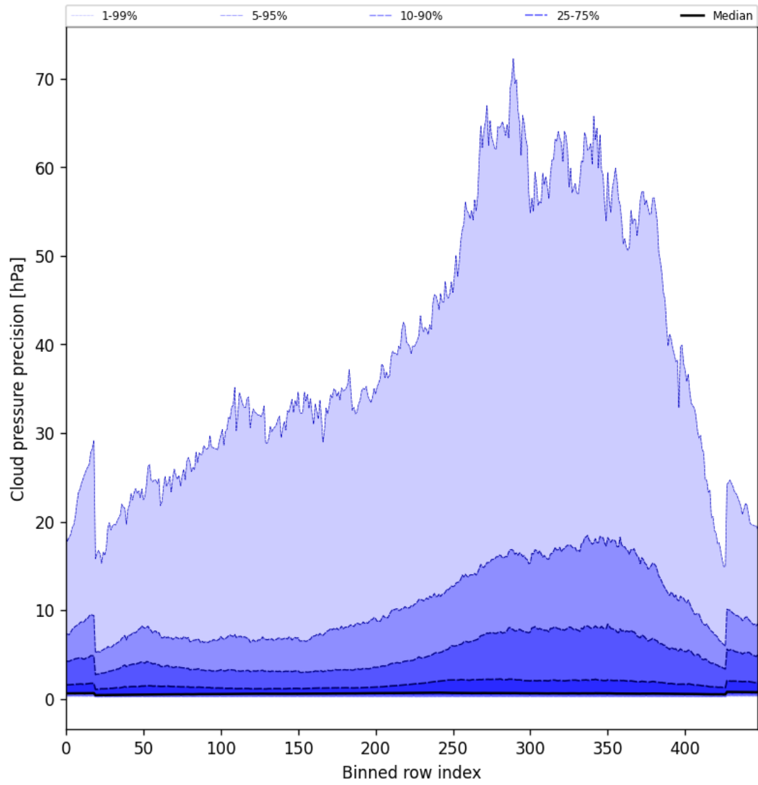
Figure 48: Along track statistics of “Cloud pressure precision” for 2025-03-25 to 2025-03-27
