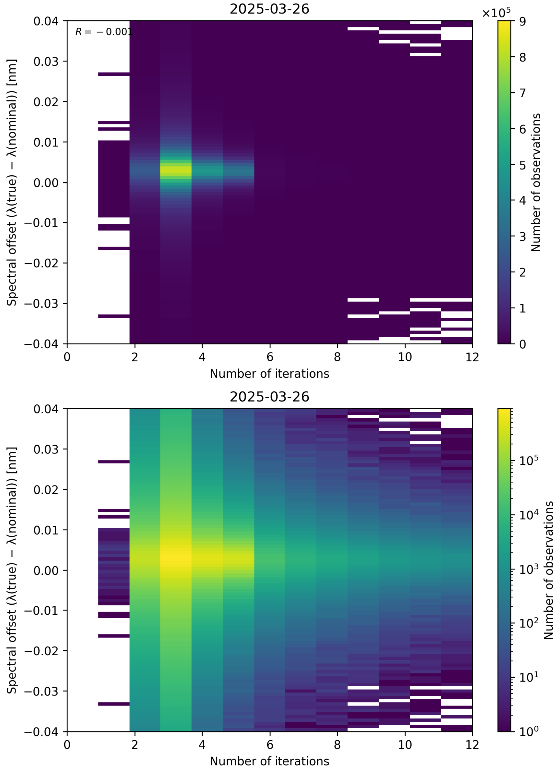
Figure 100: Scatter density plot of “Number of iterations” against “Spectral offset ( \lambda_{\text{true}} - \lambda_{\text{nominal}} )” for 2025-03-25 to 2025-03-27.
