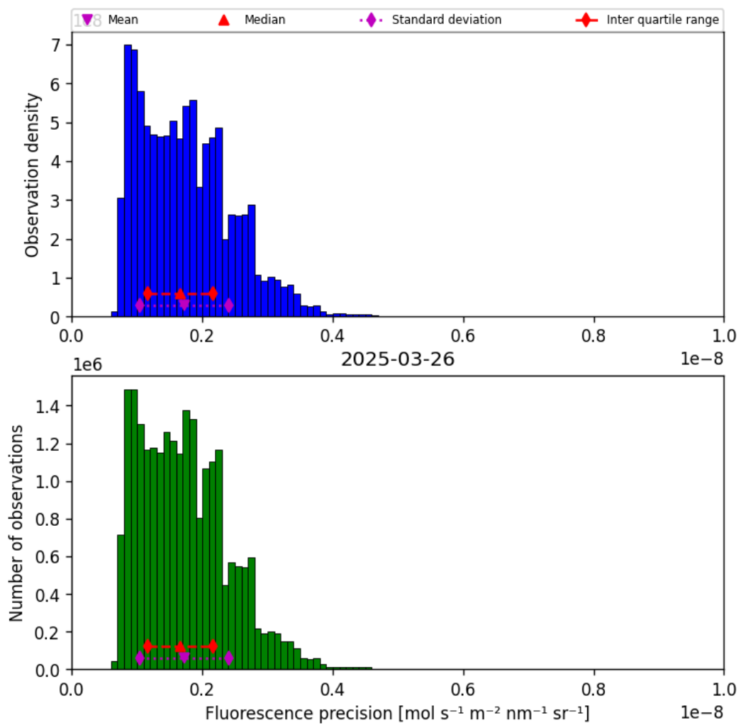
Figure 41: Histogram of “Fluorescence precision” for 2025-03-25 to 2025-03-27
