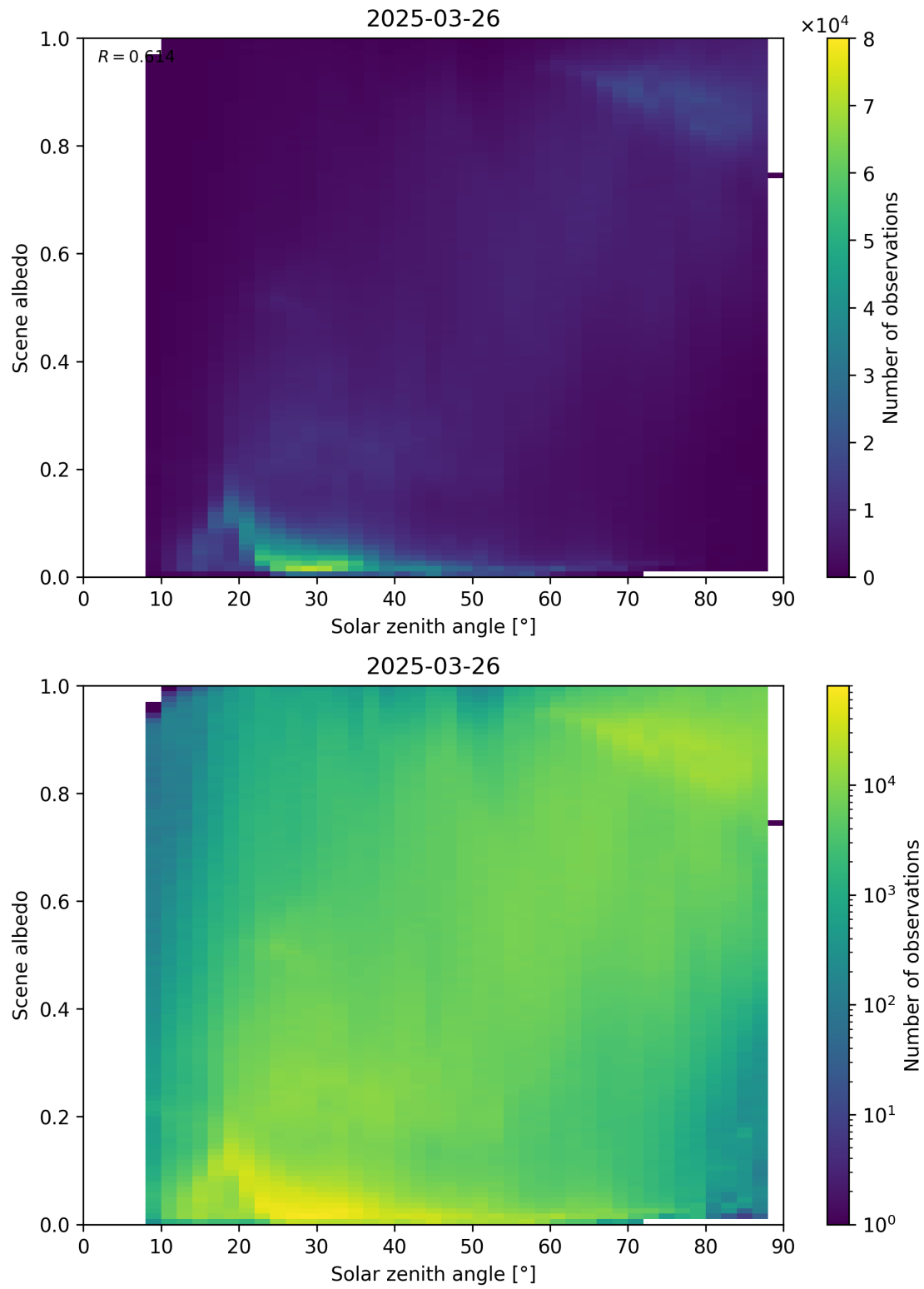
Figure 116: Scatter density plot of “Solar zenith angle” against “Scene albedo” for 2025-03-25 to 2025-03-27.
