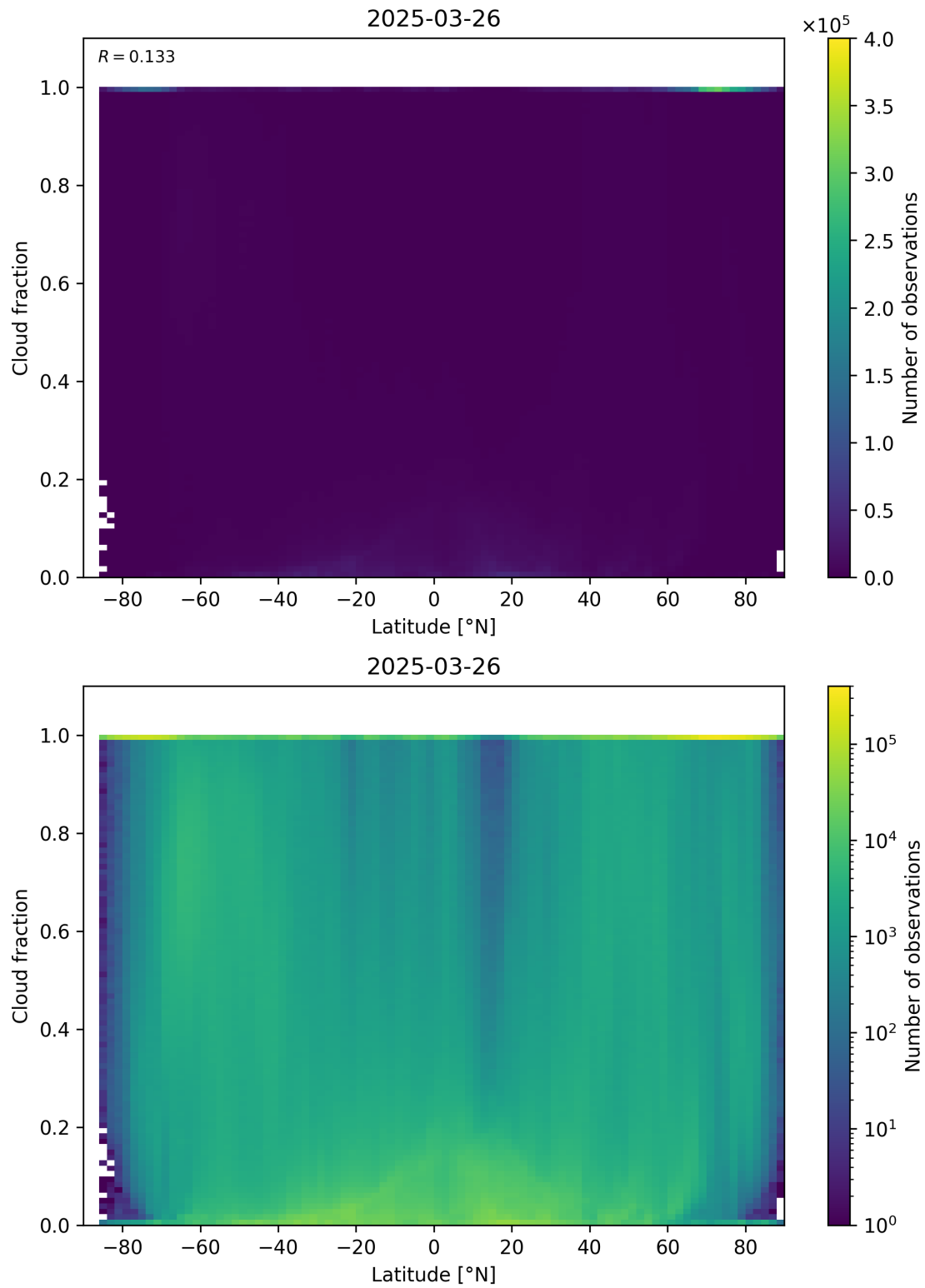
Figure 90: Scatter density plot of “Latitude” against “Cloud fraction” for 2025-03-25 to 2025-03-27.
