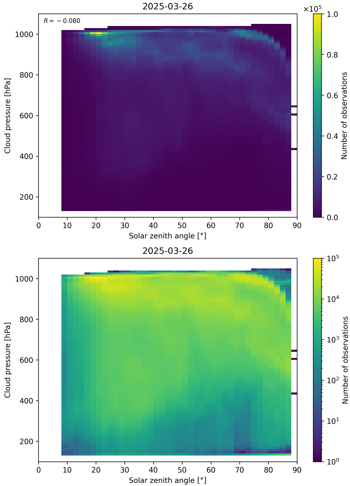
Figure 111: Scatter density plot of “Solar zenith angle” against “Cloud pressure” for 2025-03-25 to 2025-03-27.
