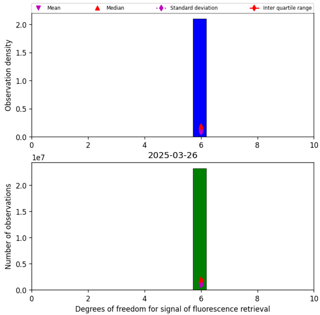
Figure 43: Histogram of “Degrees of freedom for signal of fluorescence retrieval” for 2025-03-25 to 2025-03-27
