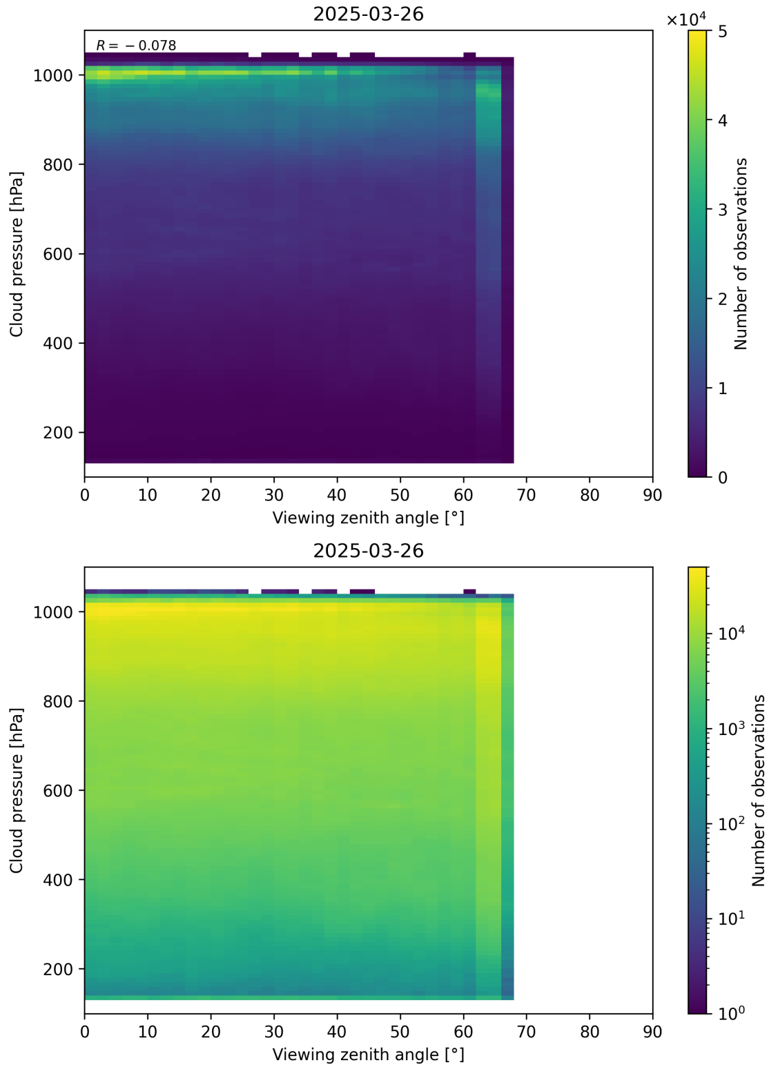
Figure 121: Scatter density plot of “Viewing zenith angle” against “Cloud pressure” for 2025-03-25 to 2025-03-27.
