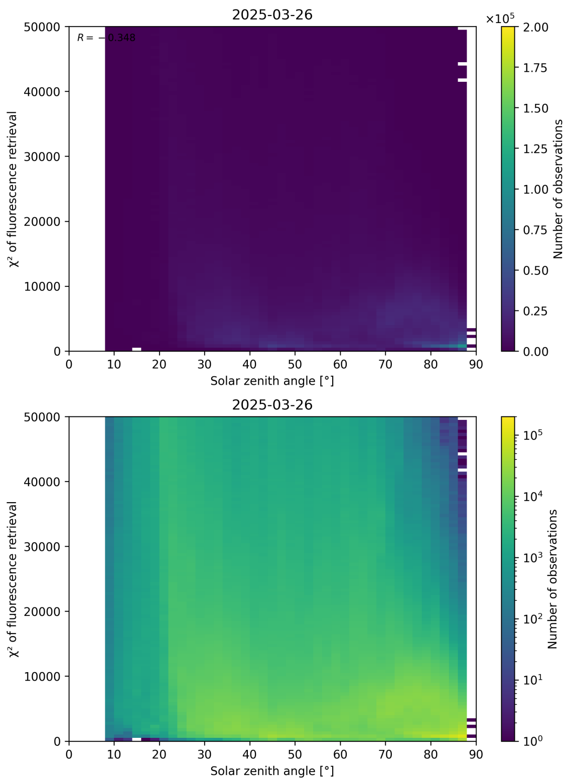
Figure 109: Scatter density plot of “Solar zenith angle” against “ \chi^2 of fluorescence retrieval” for 2025-03-25 to 2025-03-27.
