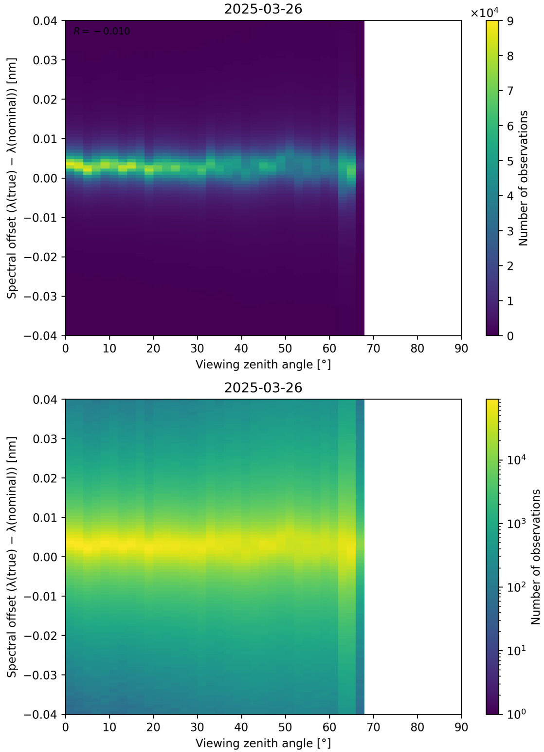
Figure 128: Scatter density plot of “Viewing zenith angle” against “Spectral offset ( \lambda_{\text{true}} - \lambda_{\text{nominal}} )” for 2025-03-25 to 2025-03-27.
