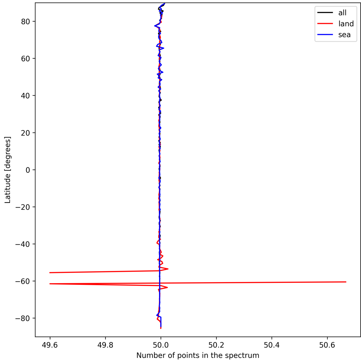
Figure 27: Zonal average of “Number of points in the spectrum” for 2025-03-25 to 2025-03-27.
