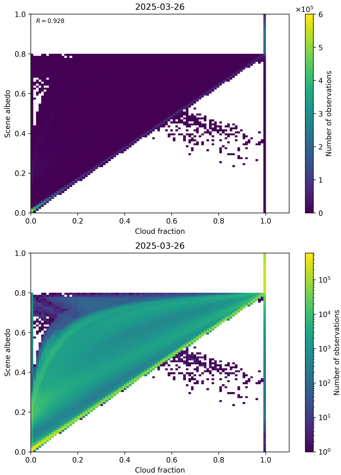
Figure 75: Scatter density plot of “Cloud fraction” against “Scene albedo” for 2025-03-25 to 2025-03-27.
