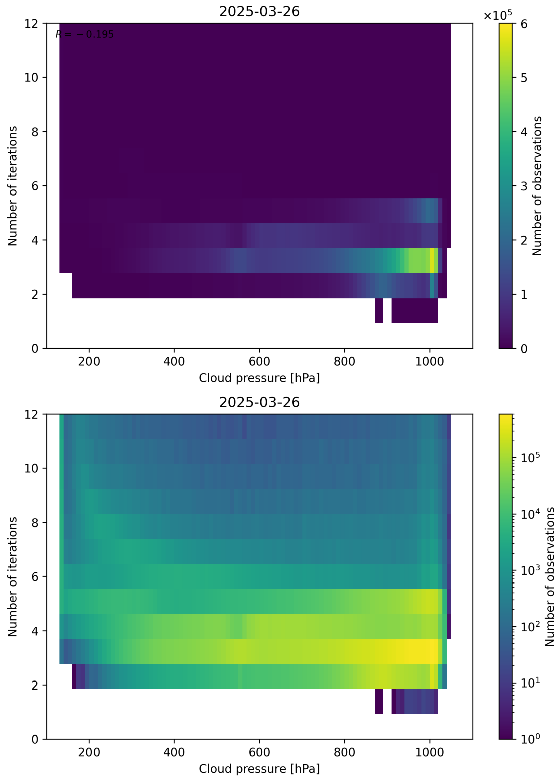
Figure 81: Scatter density plot of “Cloud pressure” against “Number of iterations” for 2025-03-25 to 2025-03-27.
