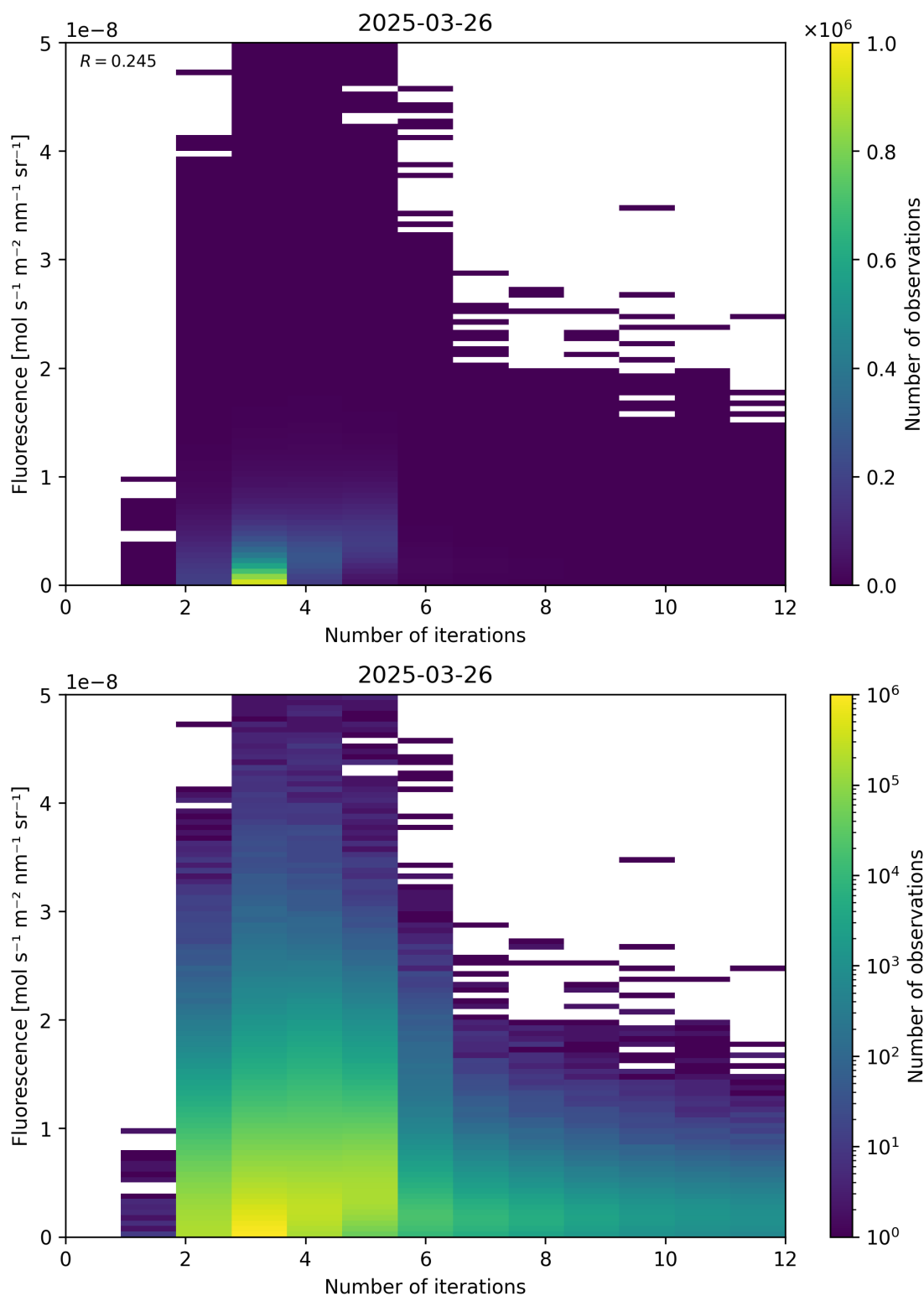
Figure 98: Scatter density plot of “Number of iterations” against “Fluorescence” for 2025-03-25 to 2025-03-27.
