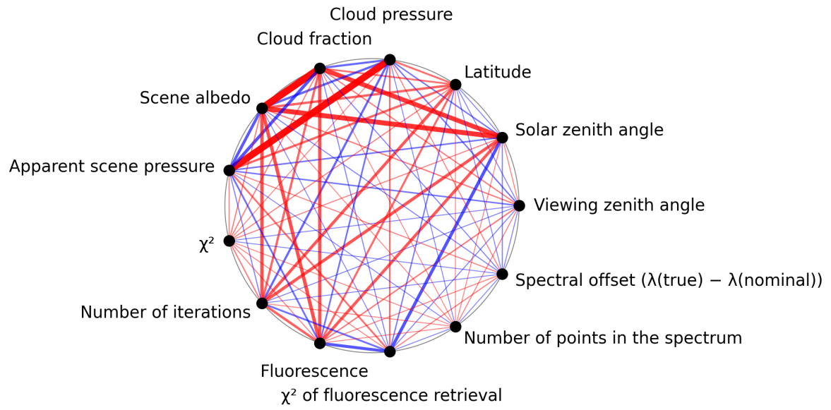
Figure 1: Map of correlation graph for 2025-03-25 to 2025-03-27.
