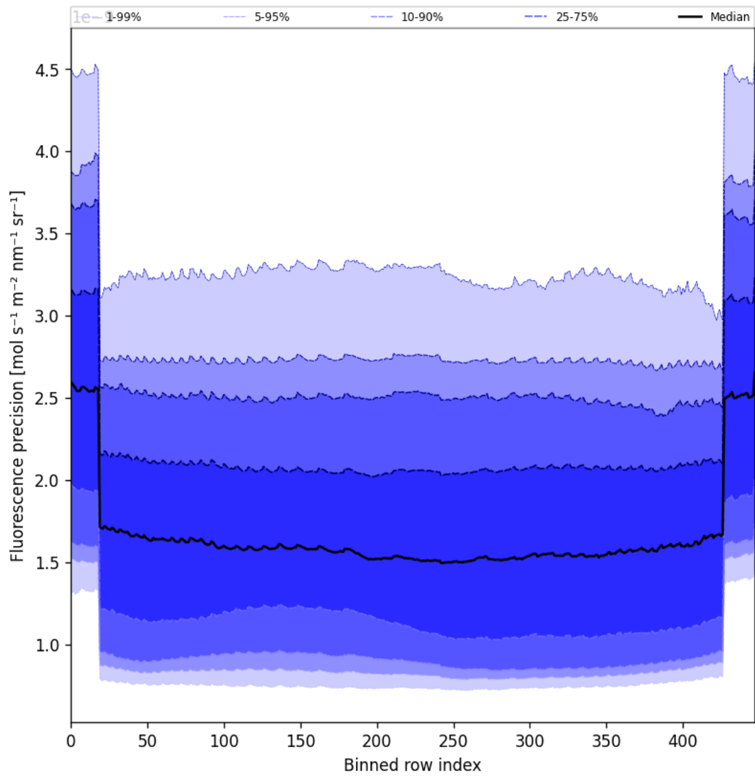
Figure 58: Along track statistics of “Fluorescence precision” for 2025-03-25 to 2025-03-27
