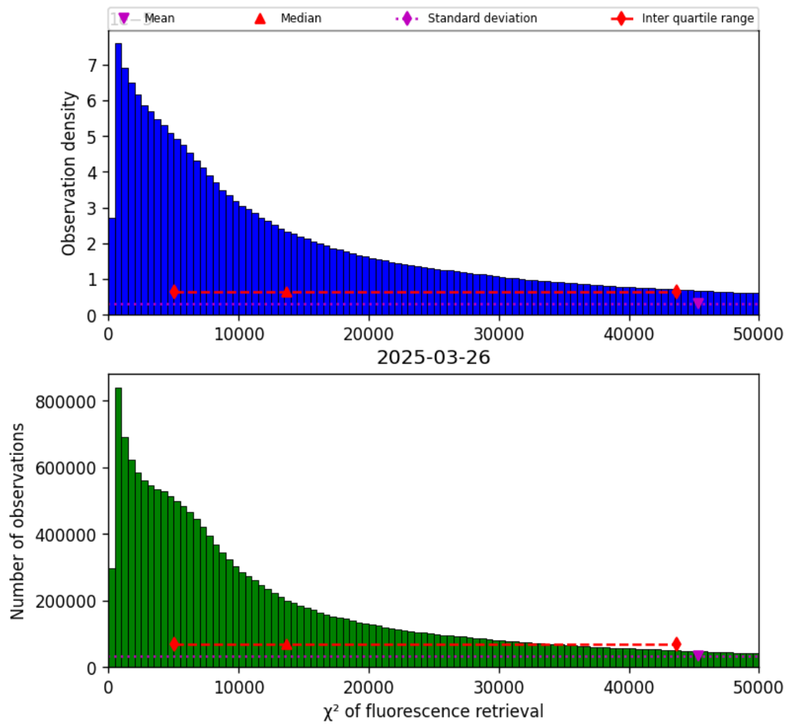
Figure 42: Histogram of “ \chi^2 of fluorescence retrieval” for 2025-03-25 to 2025-03-27
