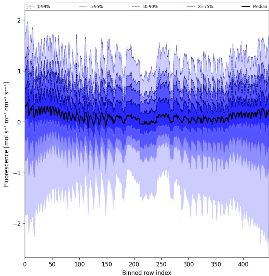
Figure 57: Along track statistics of “Fluorescence” for 2025-03-25 to 2025-03-27
