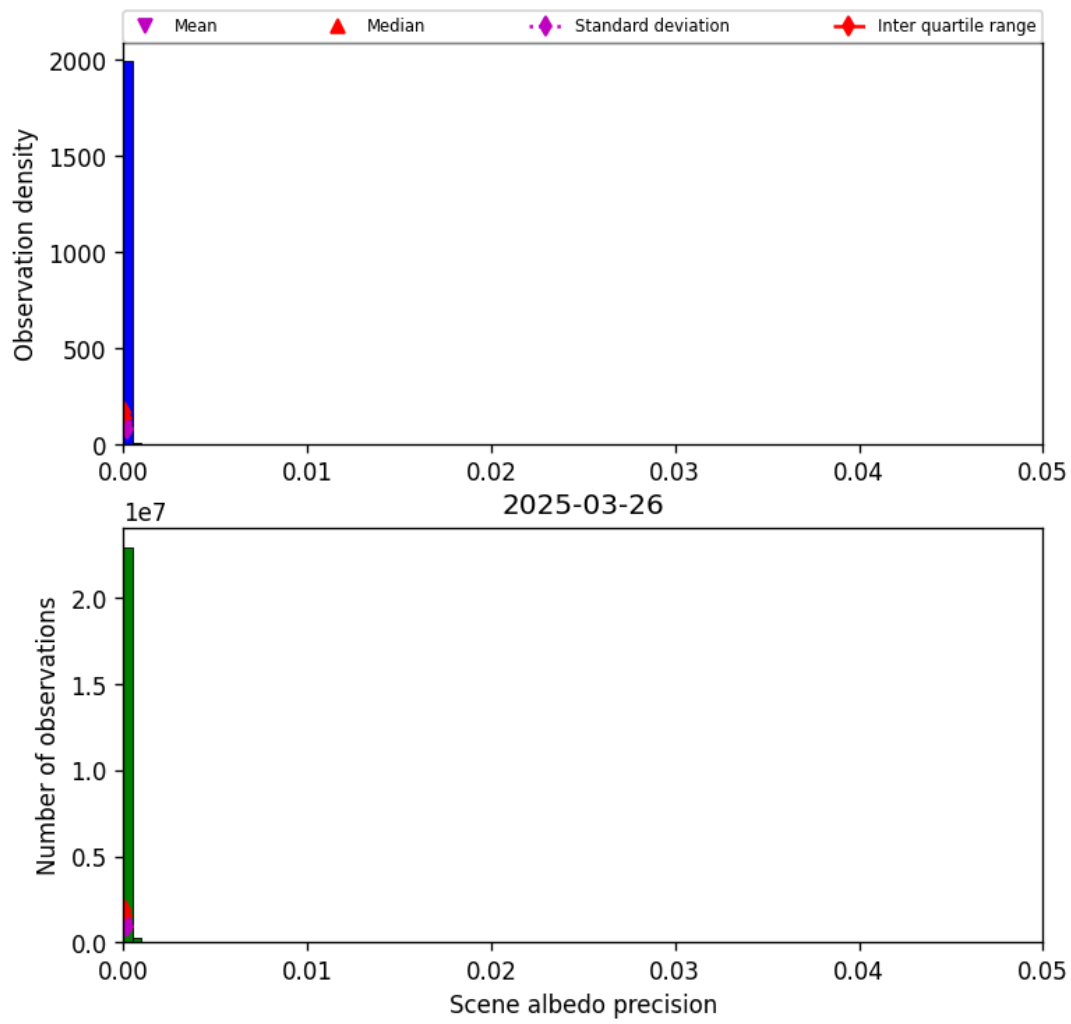
Figure 35: Histogram of “Scene albedo precision” for 2025-03-25 to 2025-03-27
