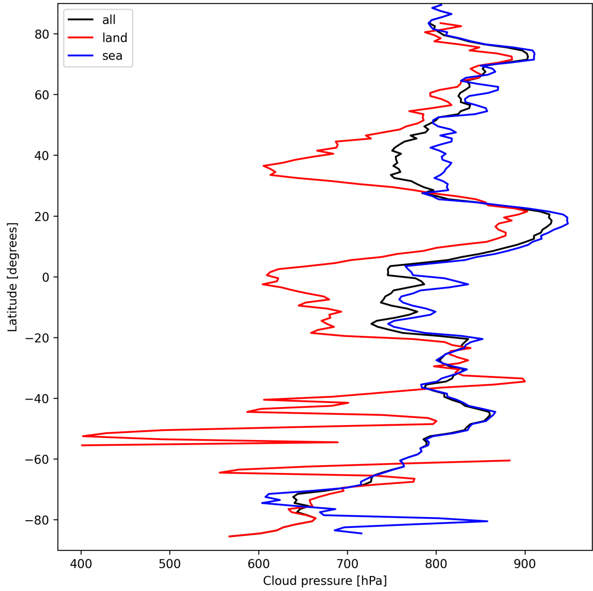
Figure 13: Zonal average of “Cloud pressure” for 2025-03-25 to 2025-03-27.
