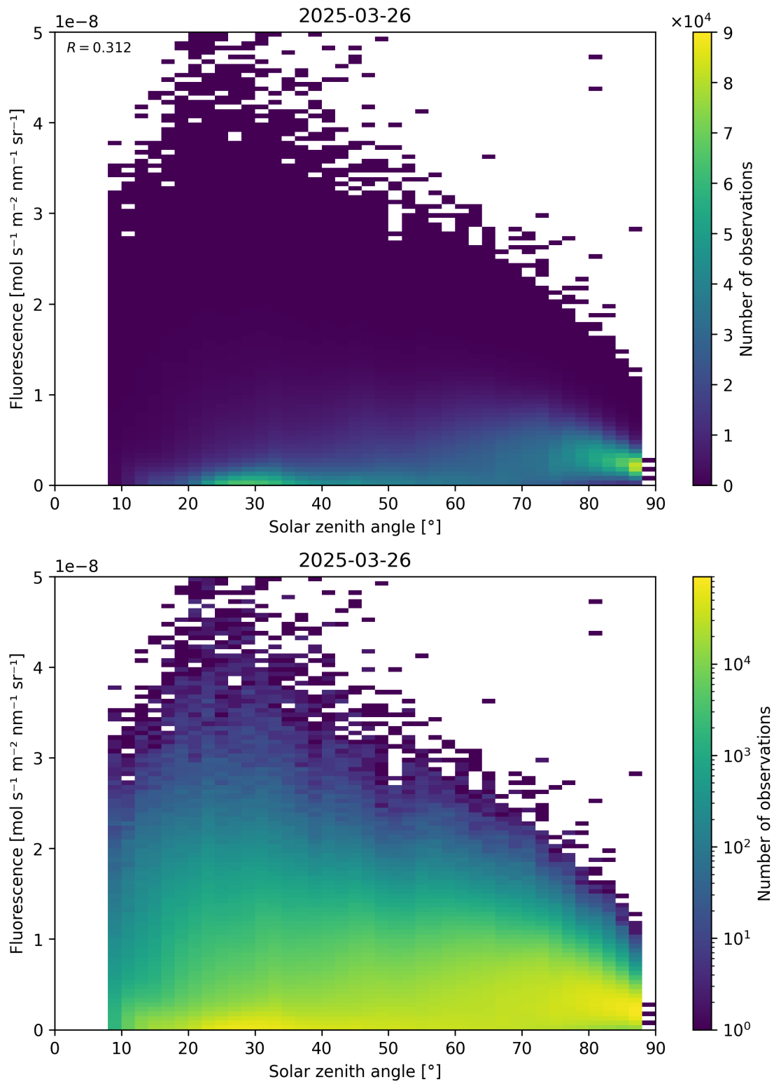
Figure 112: Scatter density plot of “Solar zenith angle” against “Fluorescence” for 2025-03-25 to 2025-03-27.
