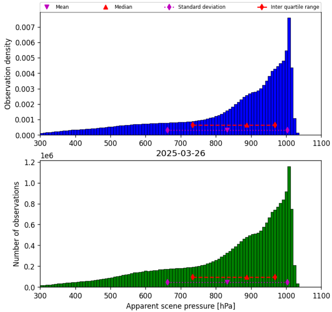
Figure 36: Histogram of “Apparent scene pressure” for 2025-03-25 to 2025-03-27
