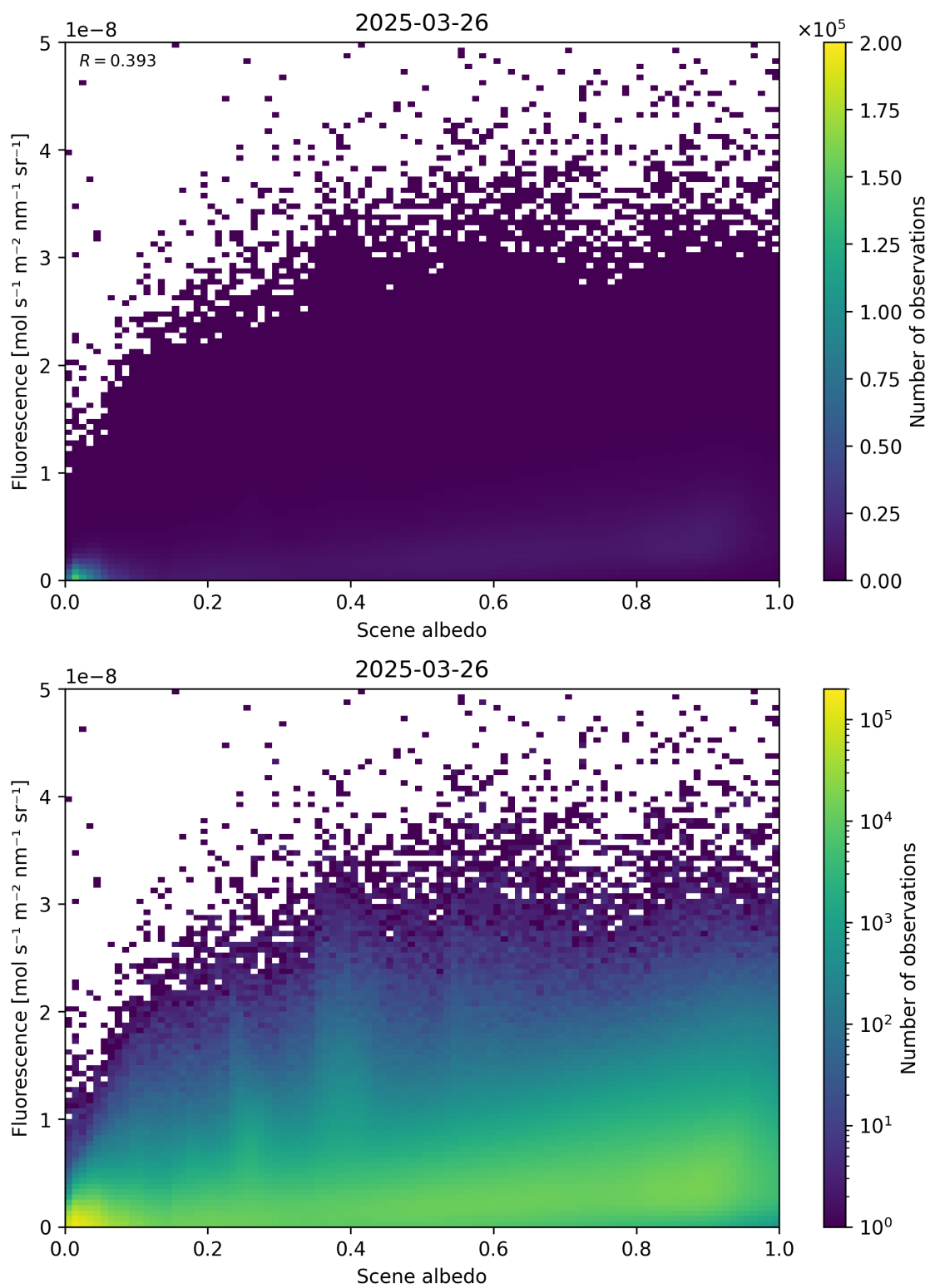
Figure 104: Scatter density plot of “Scene albedo” against “Fluorescence” for 2025-03-25 to 2025-03-27.
