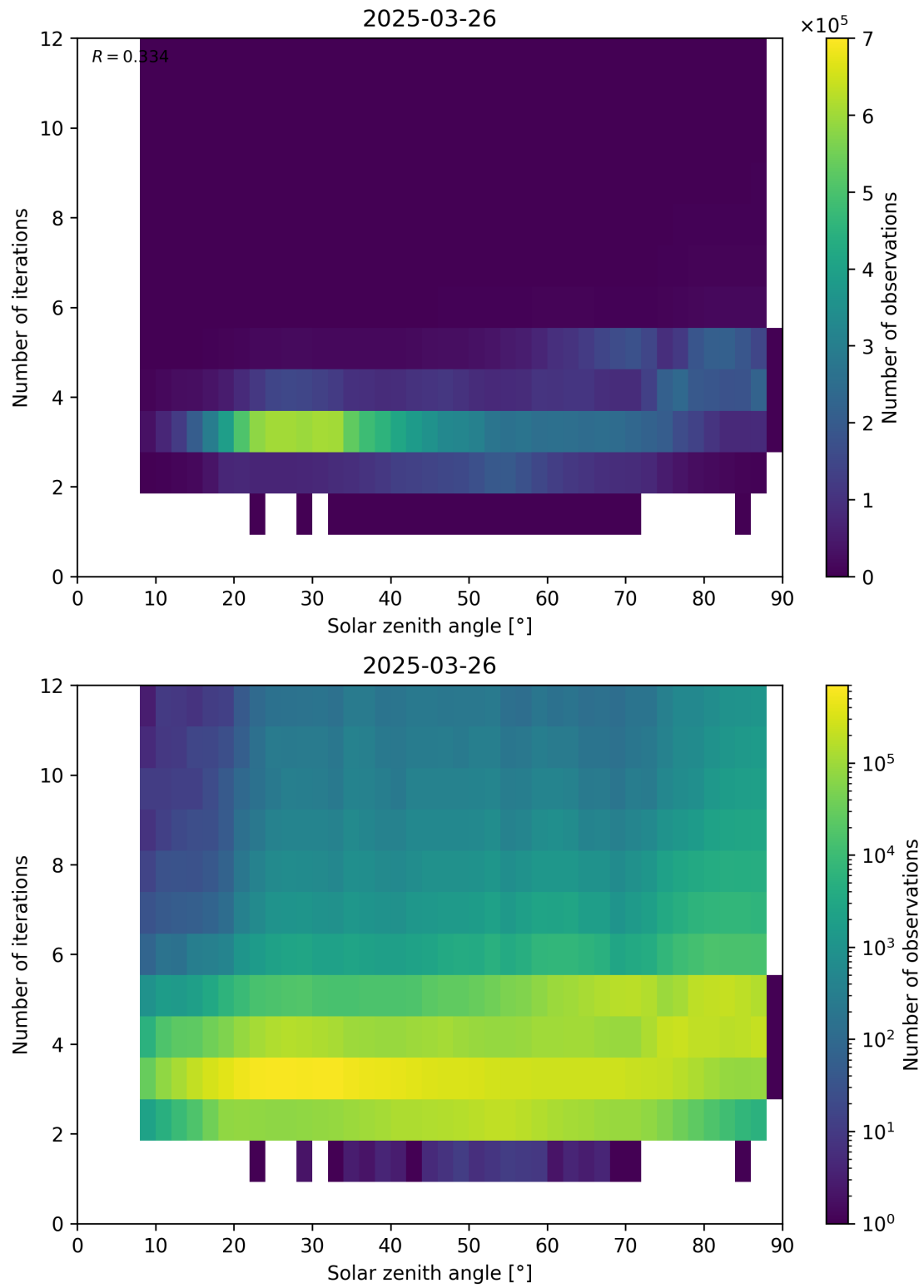
Figure 114: Scatter density plot of “Solar zenith angle” against “Number of iterations” for 2025-03-25 to 2025-03-27.
