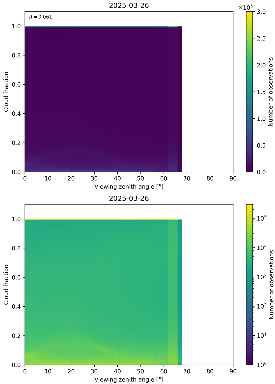
Figure 120: Scatter density plot of “Viewing zenith angle” against “Cloud fraction” for 2025-03-25 to 2025-03-27.
