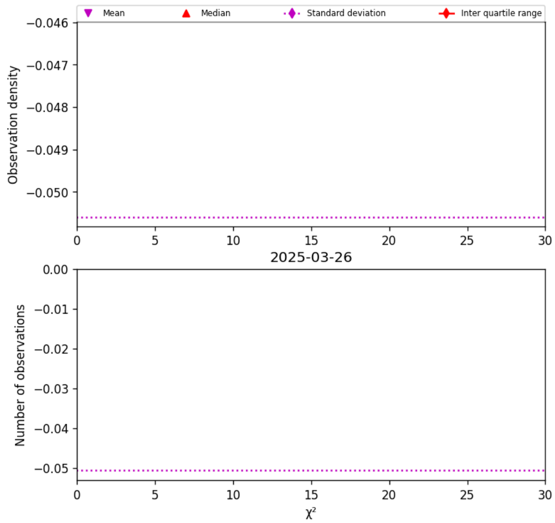
Figure 38: Histogram of " \chi^2 " for 2025-03-25 to 2025-03-27
