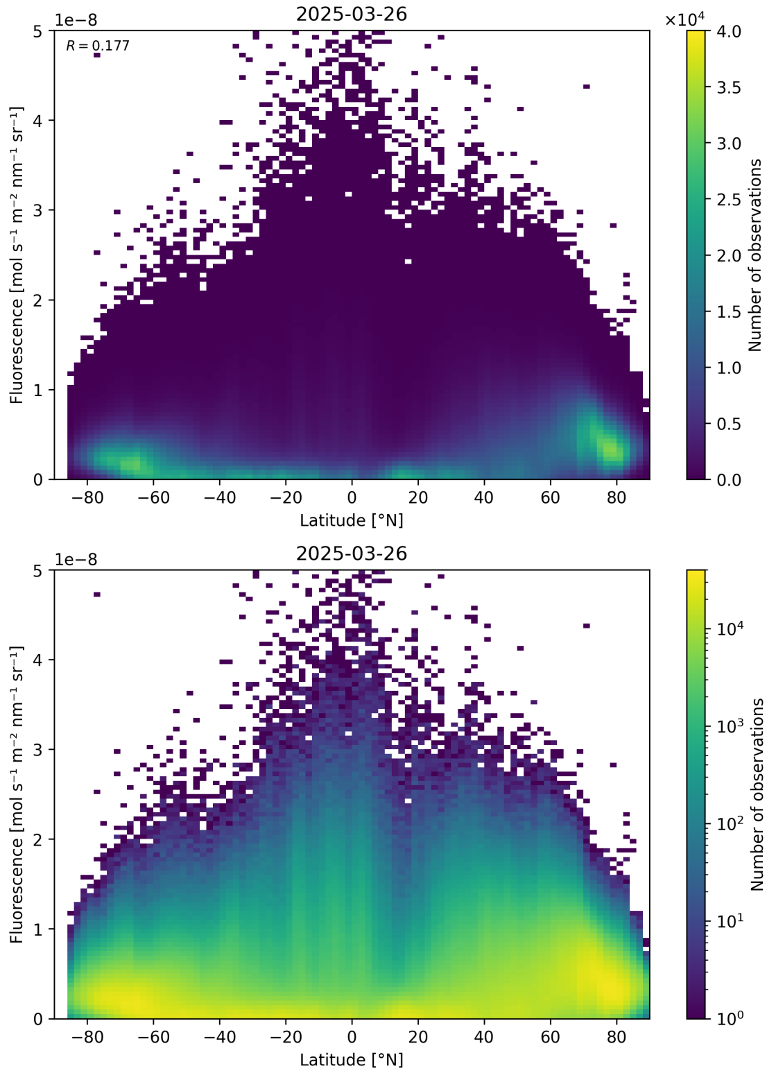
Figure 92: Scatter density plot of “Latitude” against “Fluorescence” for 2025-03-25 to 2025-03-27.
