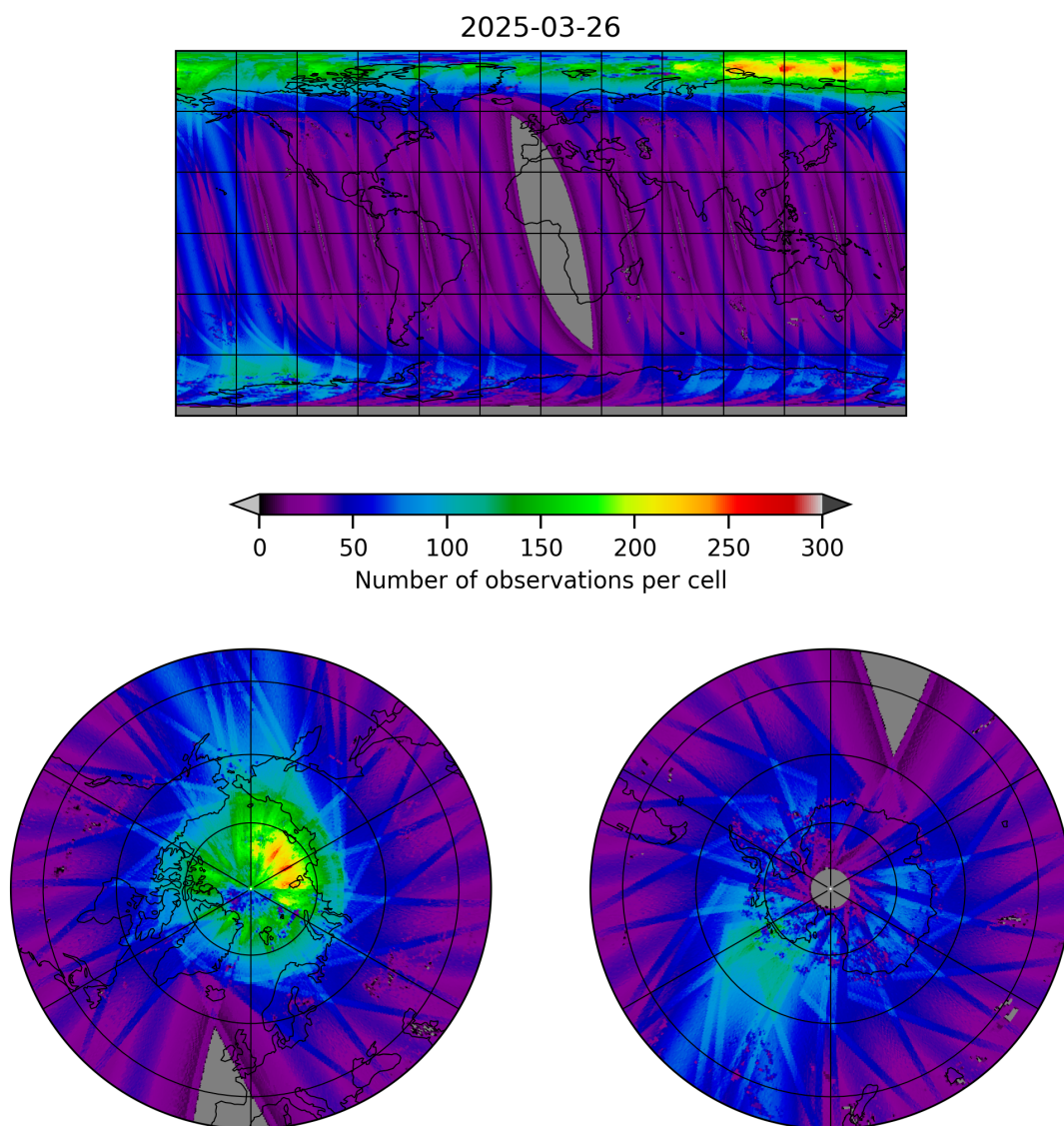
Figure 11: Map of the number of observations for 2025-03-25 to 2025-03-27
