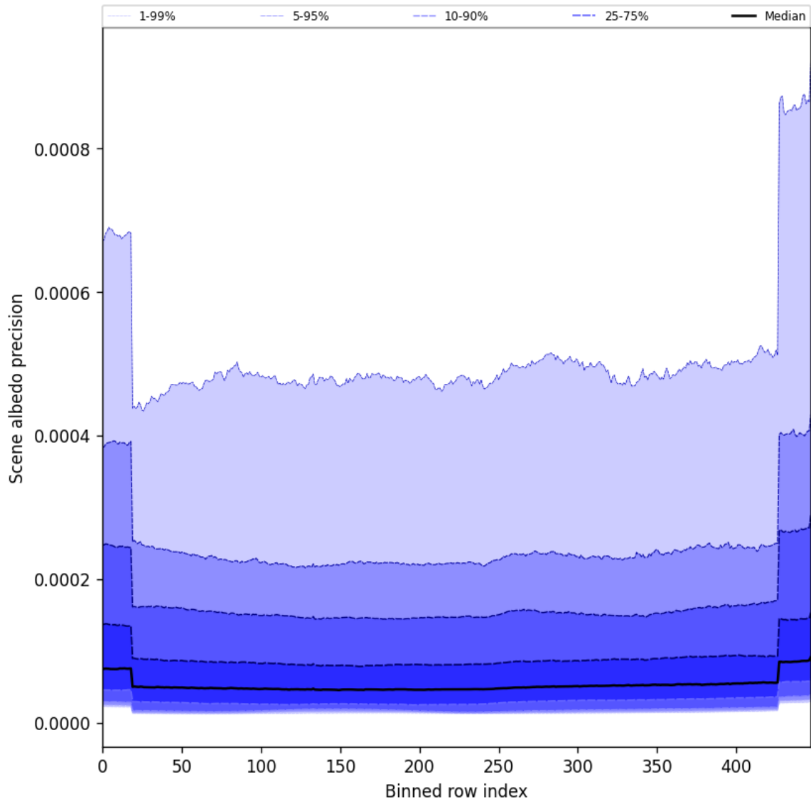
Figure 52: Along track statistics of “Scene albedo precision” for 2025-03-25 to 2025-03-27
