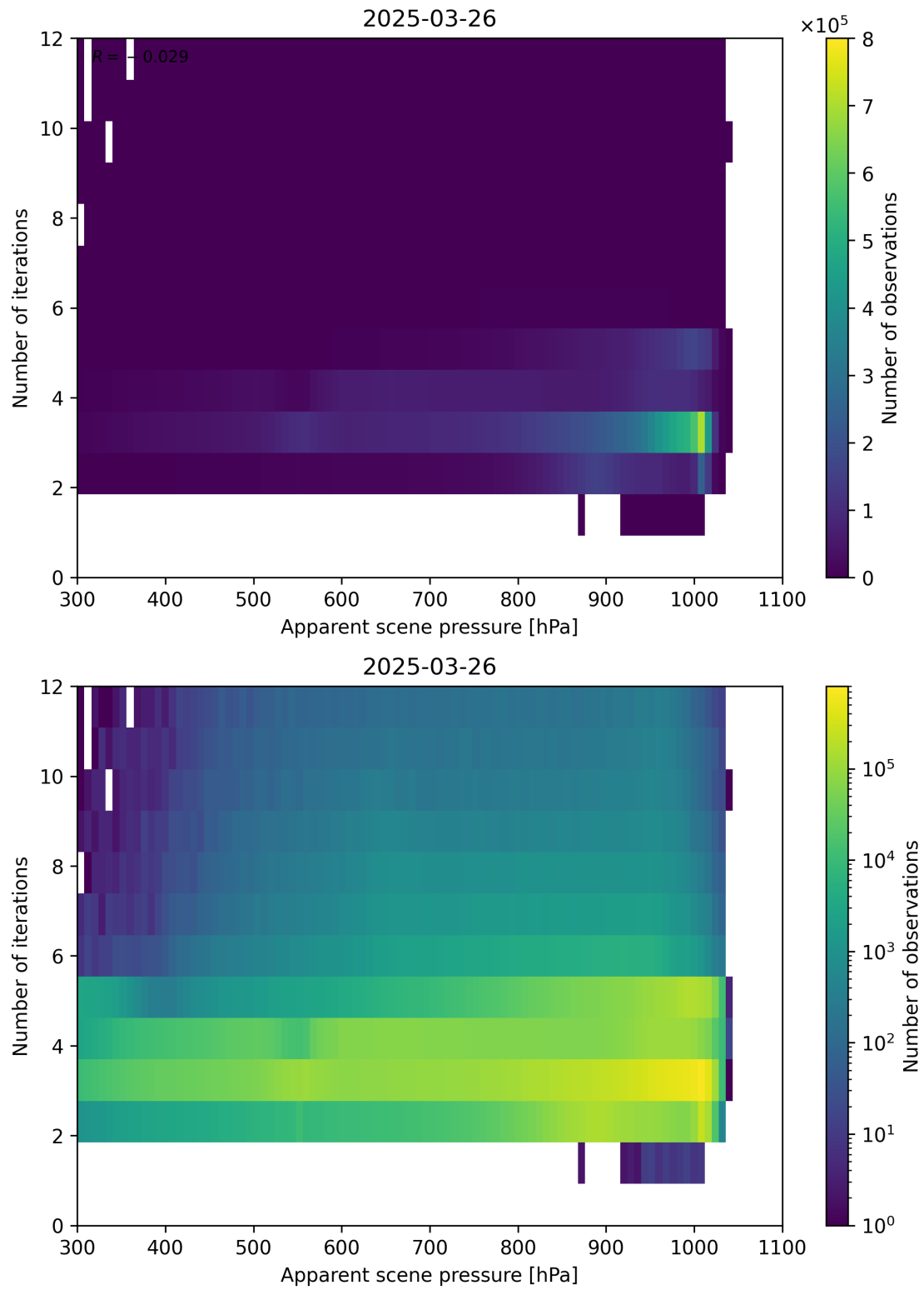
Figure 65: Scatter density plot of “Apparent scene pressure” against “Number of iterations” for 2025-03-25 to 2025-03-27.
