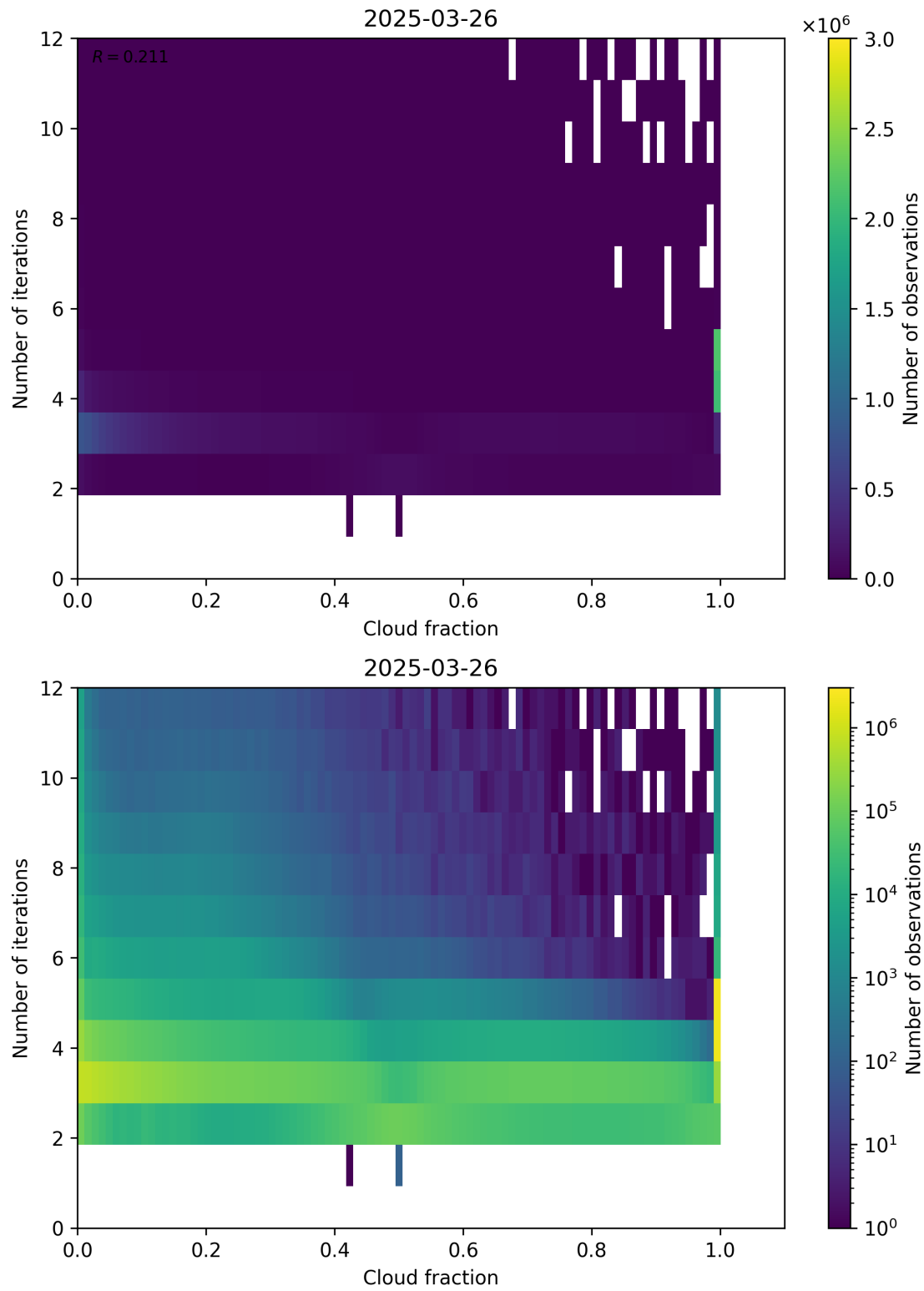
Figure 73: Scatter density plot of “Cloud fraction” against “Number of iterations” for 2025-03-25 to 2025-03-27.
