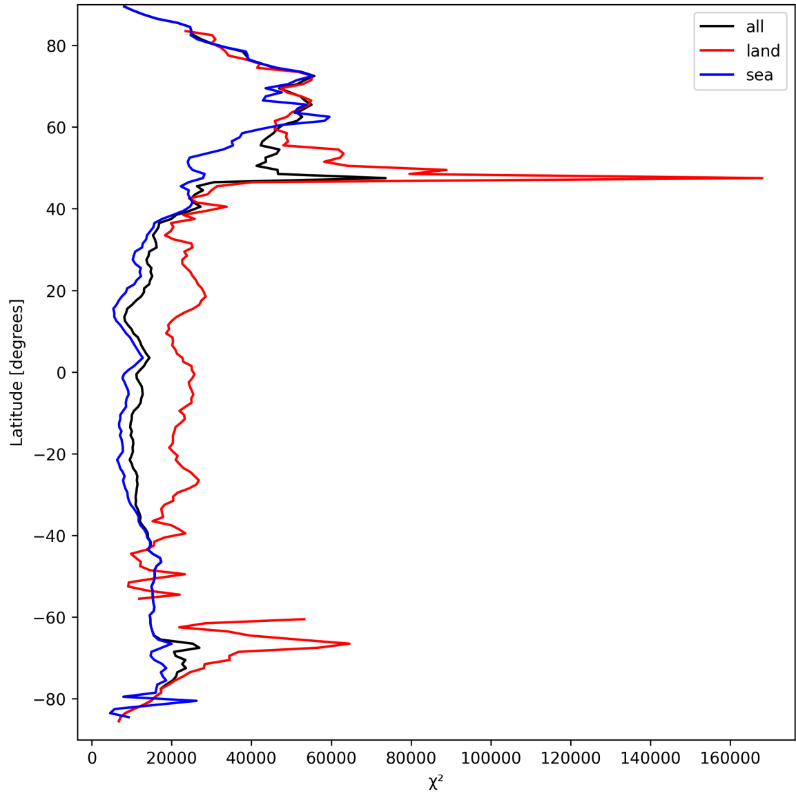
Figure 21: Zonal average of “ \chi^2 ” for 2025-03-25 to 2025-03-27.
