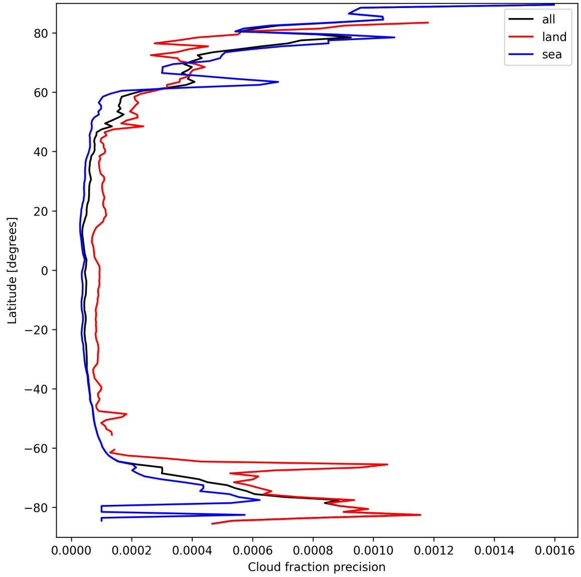
Figure 16: Zonal average of “Cloud fraction precision” for 2025-03-25 to 2025-03-27.
