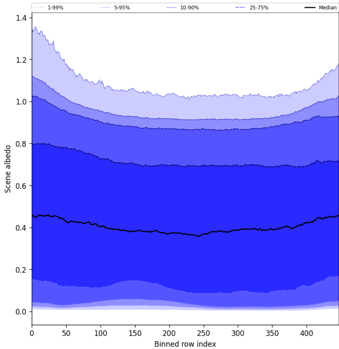
Figure 51: Along track statistics of “Scene albedo” for 2025-03-25 to 2025-03-27
