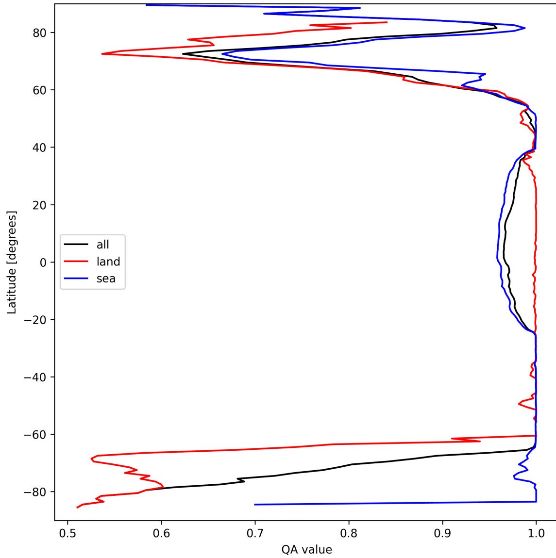
Figure 12: Zonal average of “QA value” for 2025-03-25 to 2025-03-27.
