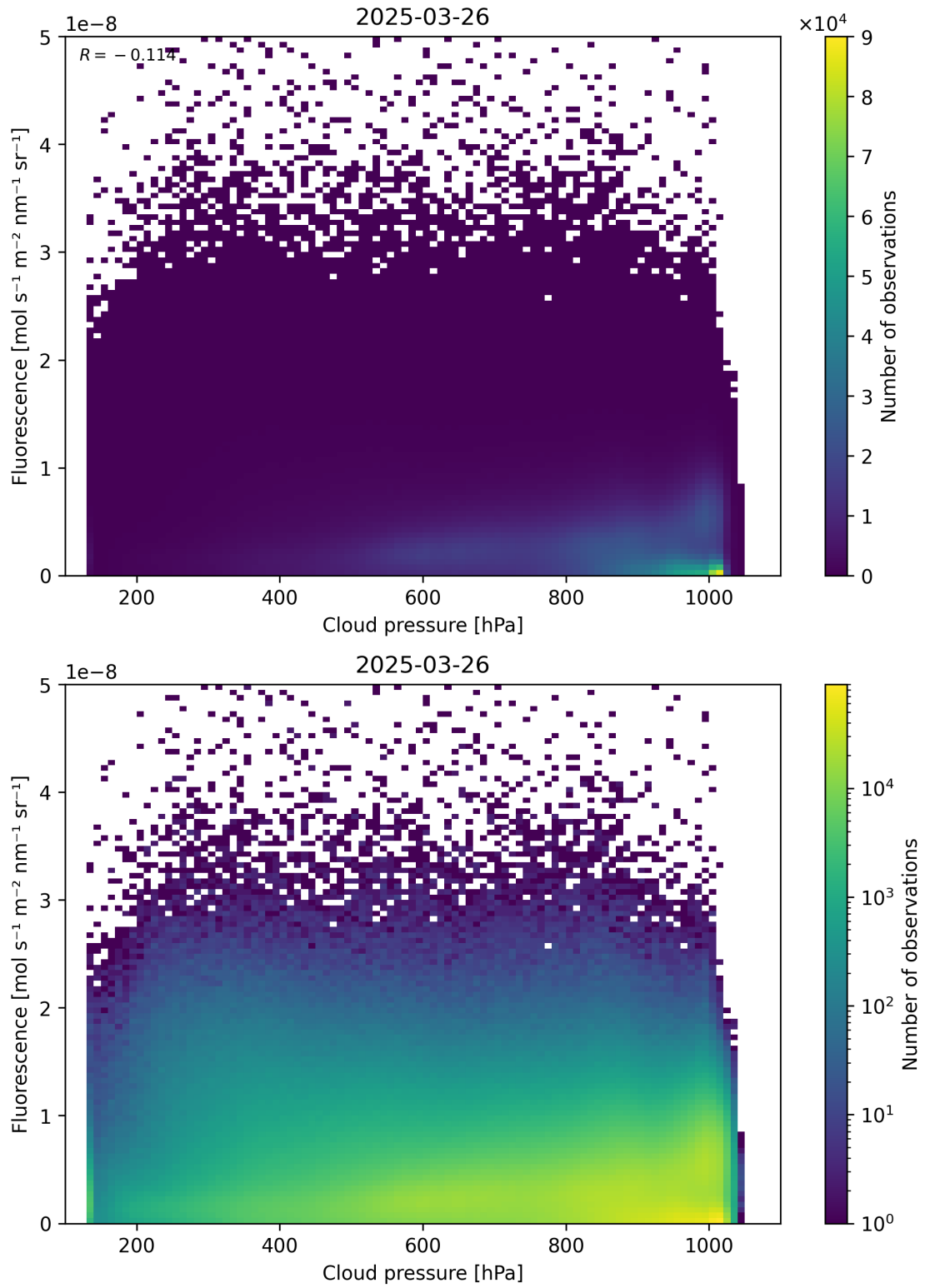
Figure 80: Scatter density plot of “Cloud pressure” against “Fluorescence” for 2025-03-25 to 2025-03-27.
