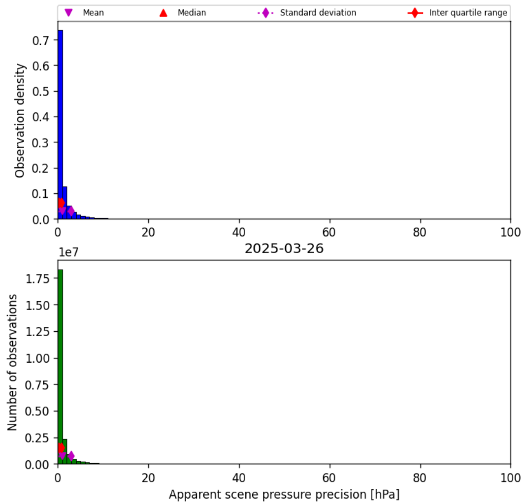
Figure 37: Histogram of “Apparent scene pressure precision” for 2025-03-25 to 2025-03-27
