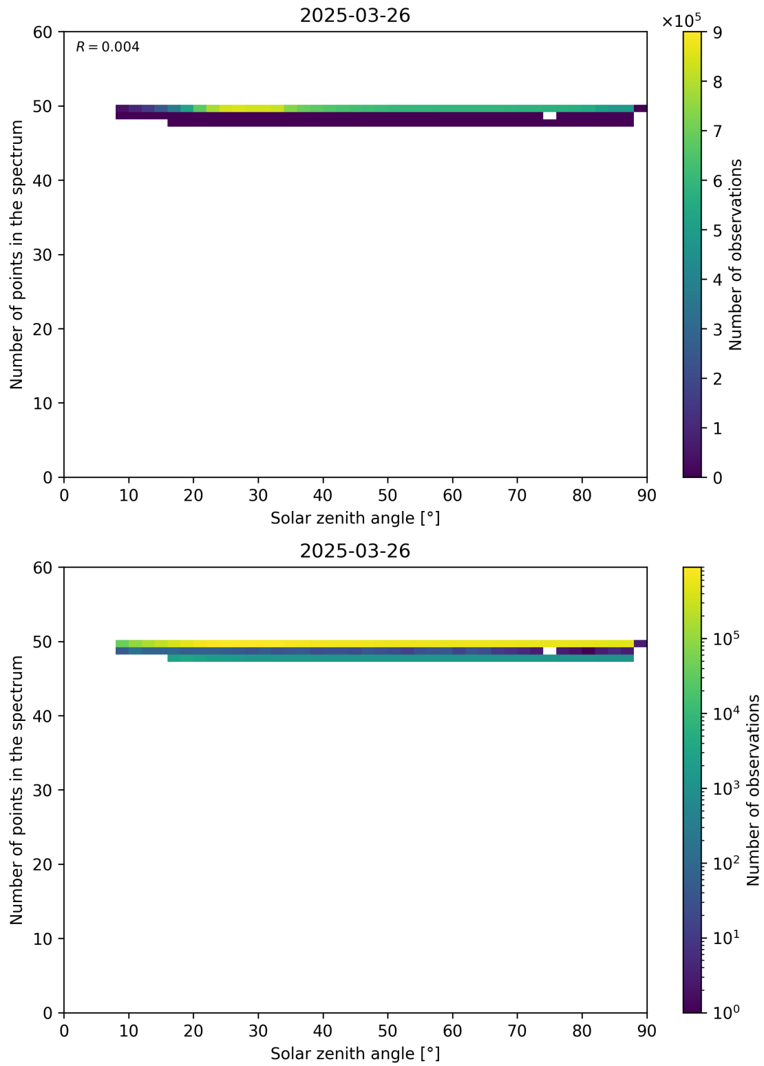
Figure 115: Scatter density plot of “Solar zenith angle” against “Number of points in the spectrum” for 2025-03-25 to 2025-03-27.
