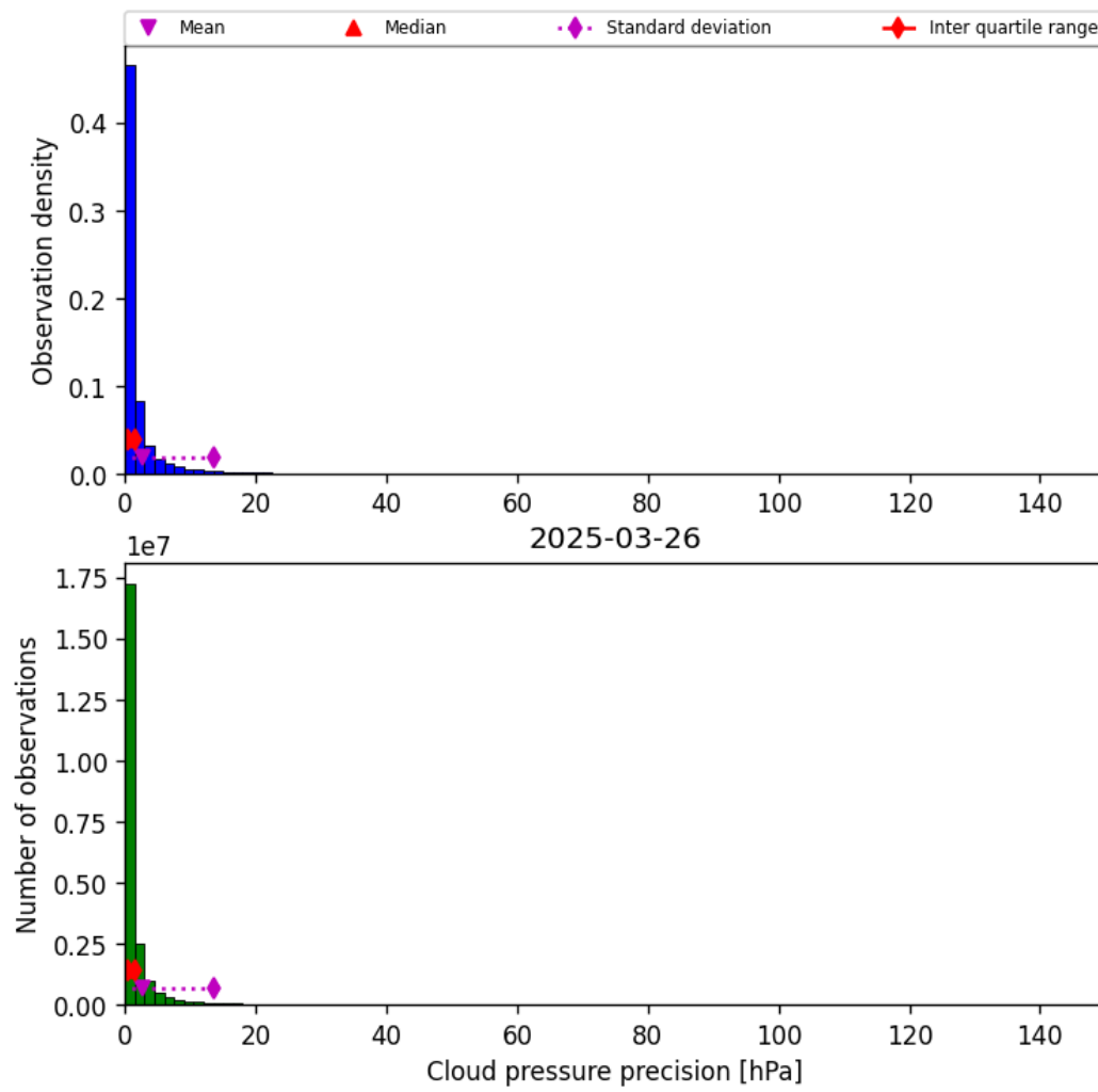
Figure 31: Histogram of “Cloud pressure precision” for 2025-03-25 to 2025-03-27
