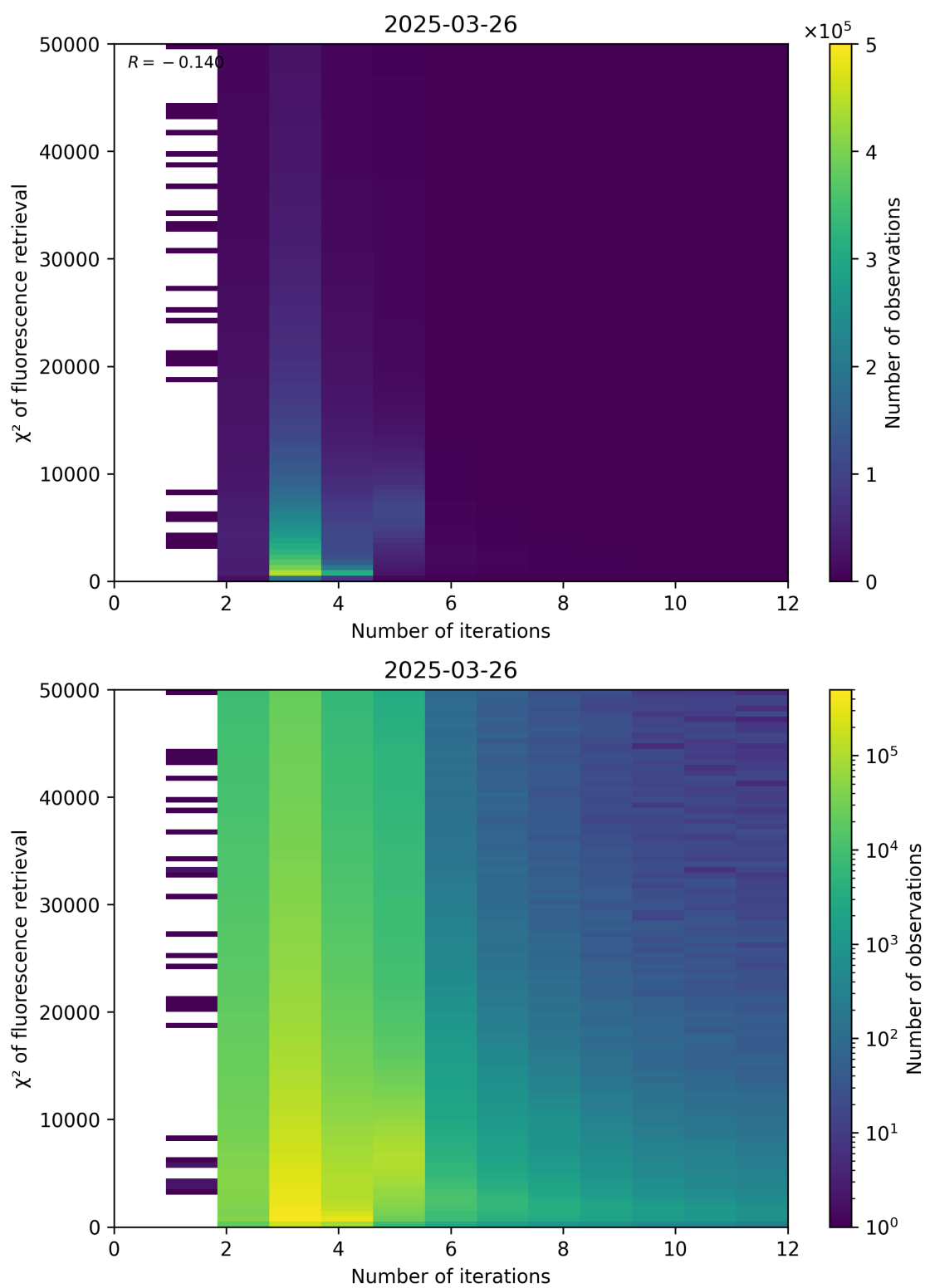
Figure 97: Scatter density plot of “Number of iterations” against “ \chi^2 of fluorescence retrieval” for 2025-03-25 to 2025-03-27.
