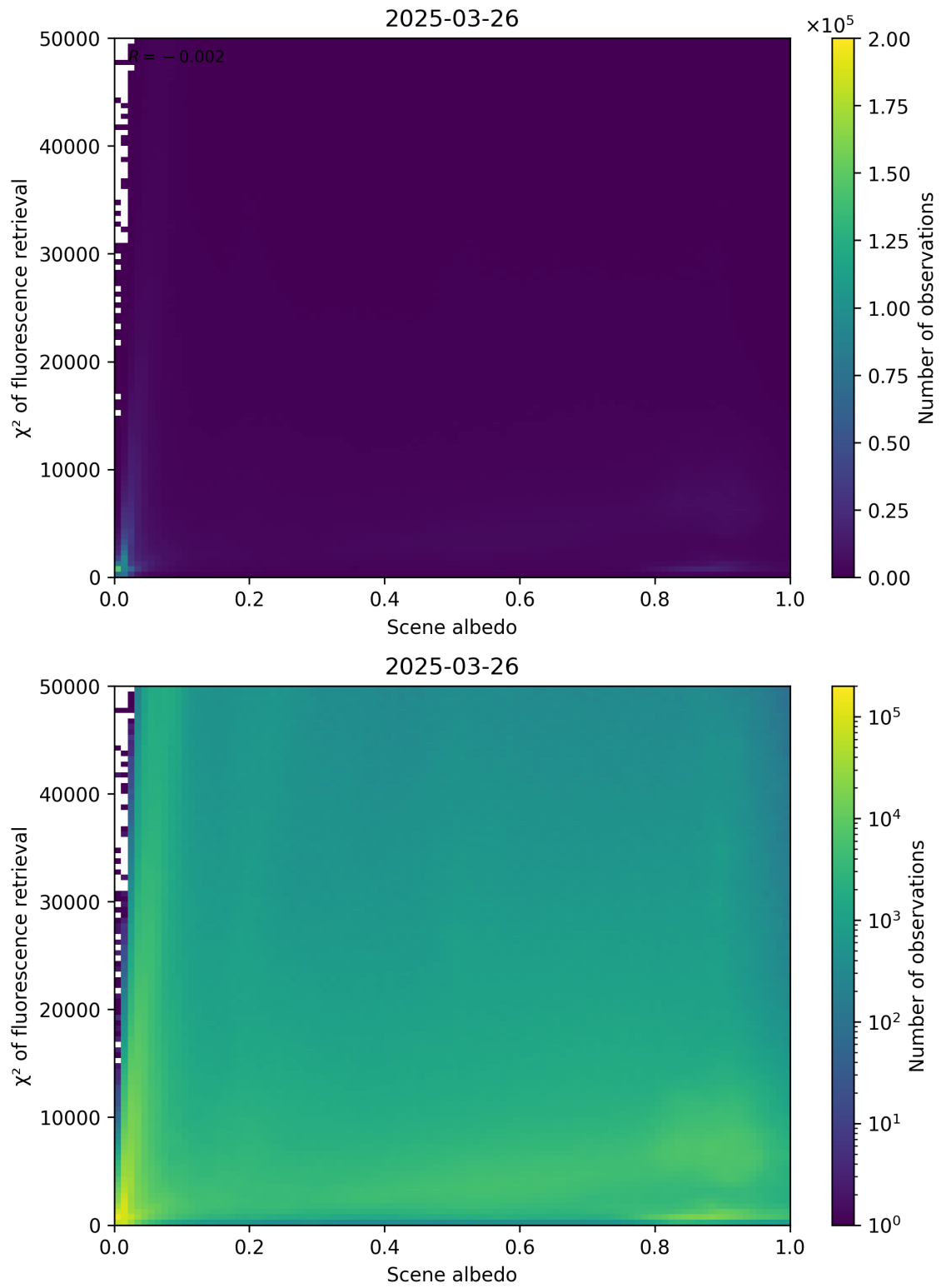
Figure 103: Scatter density plot of “Scene albedo” against “ \chi^2 of fluorescence retrieval” for 2025-03-25 to 2025-03-27.
