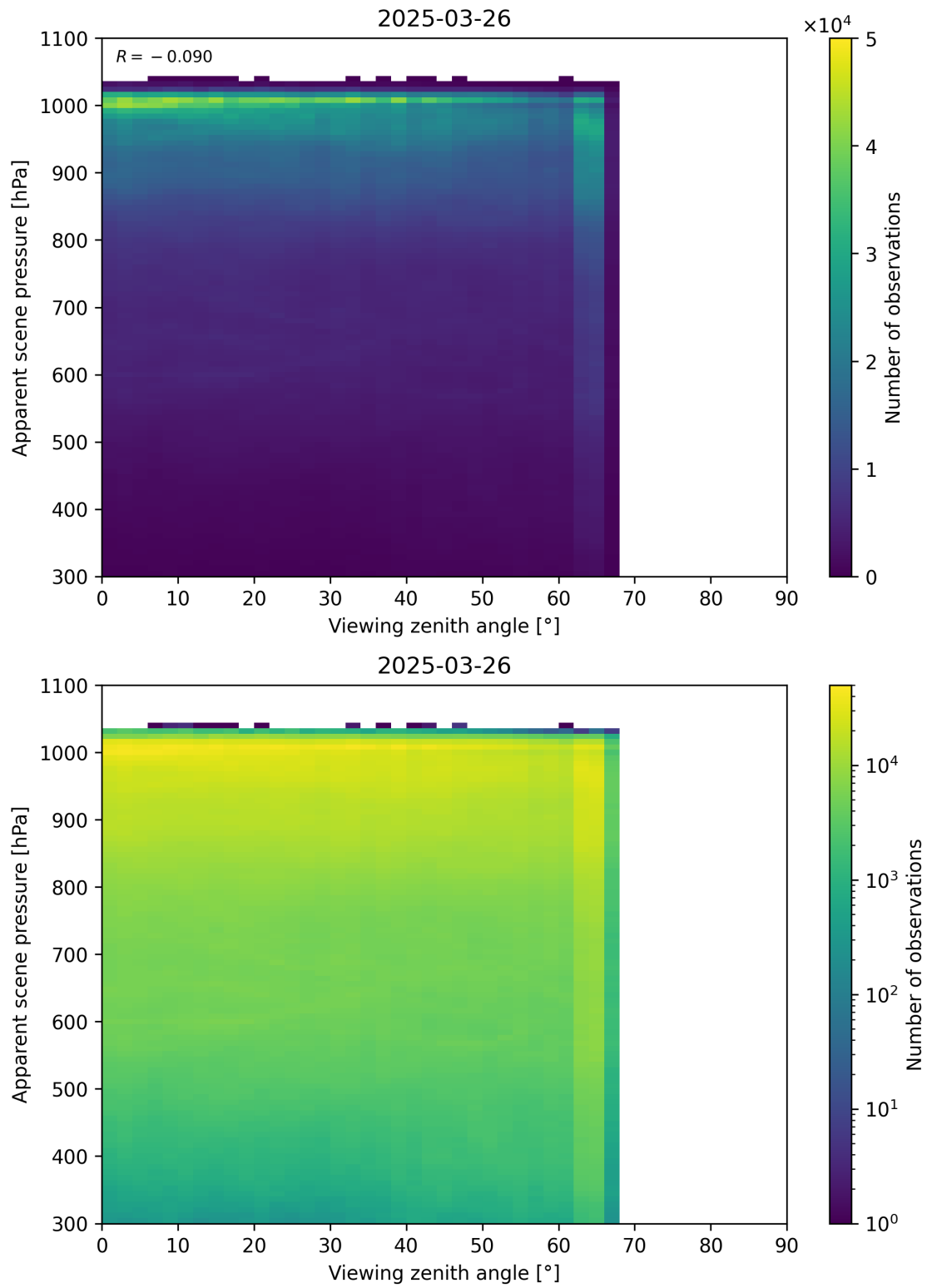
Figure 118: Scatter density plot of “Viewing zenith angle” against “Apparent scene pressure” for 2025-03-25 to 2025-03-27.
