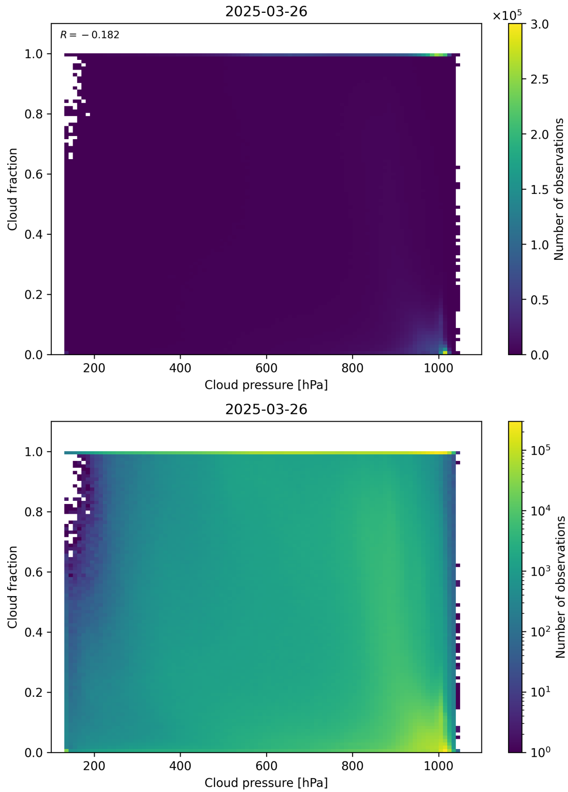
Figure 79: Scatter density plot of “Cloud pressure” against “Cloud fraction” for 2025-03-25 to 2025-03-27.
