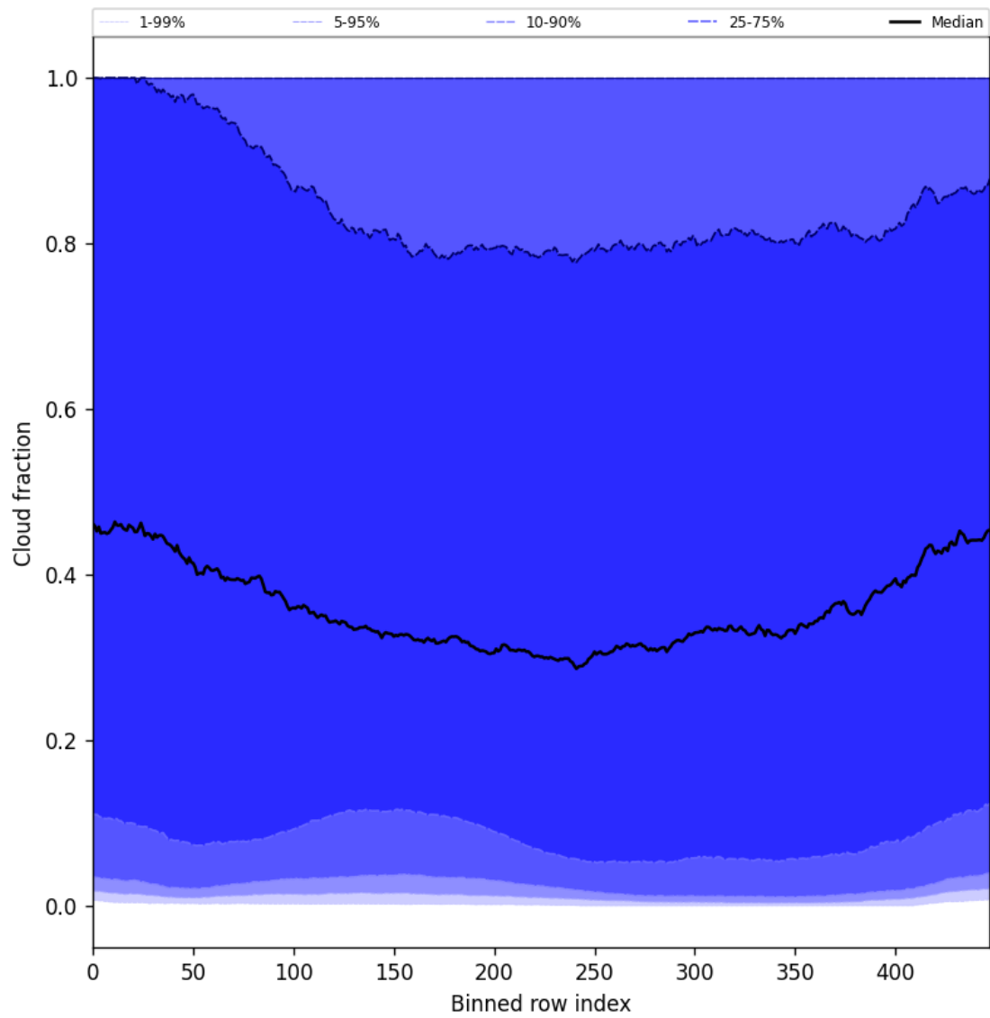
Figure 49: Along track statistics of “Cloud fraction” for 2025-03-25 to 2025-03-27
