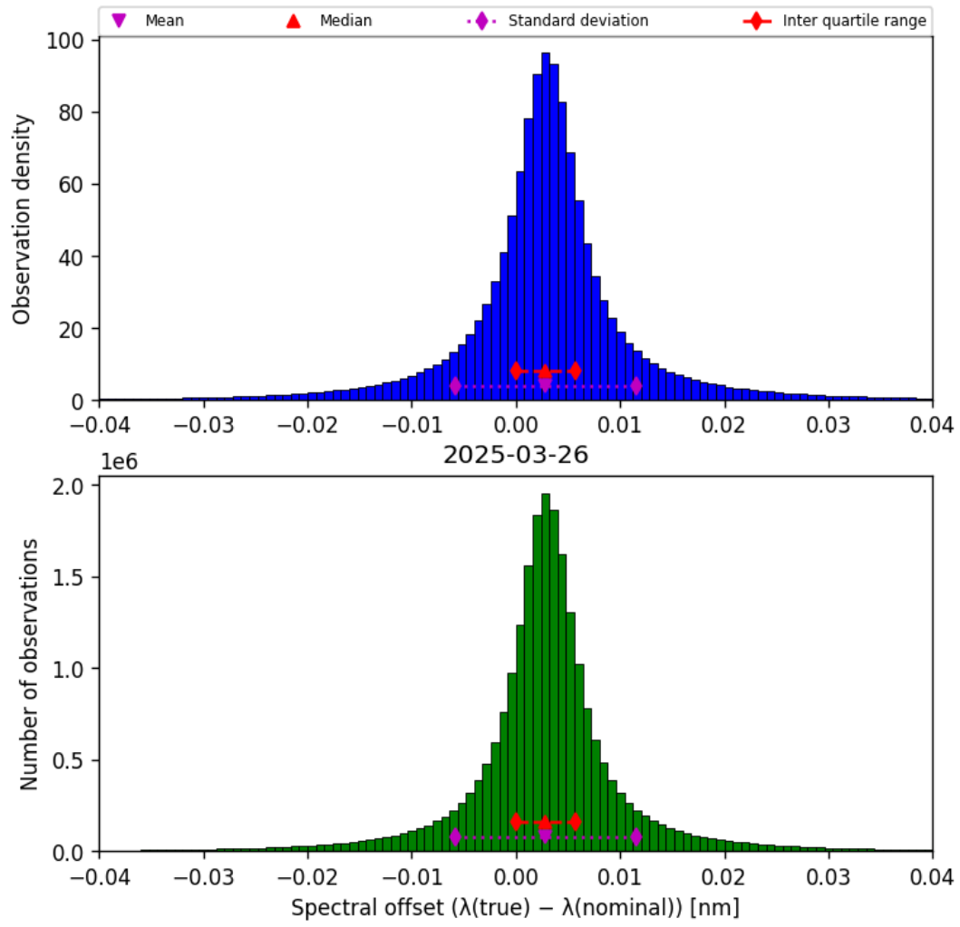
Figure 45: Histogram of “Spectral offset ( \lambda_{\text{true}} - \lambda_{\text{nominal}} )” for 2025-03-25 to 2025-03-27
