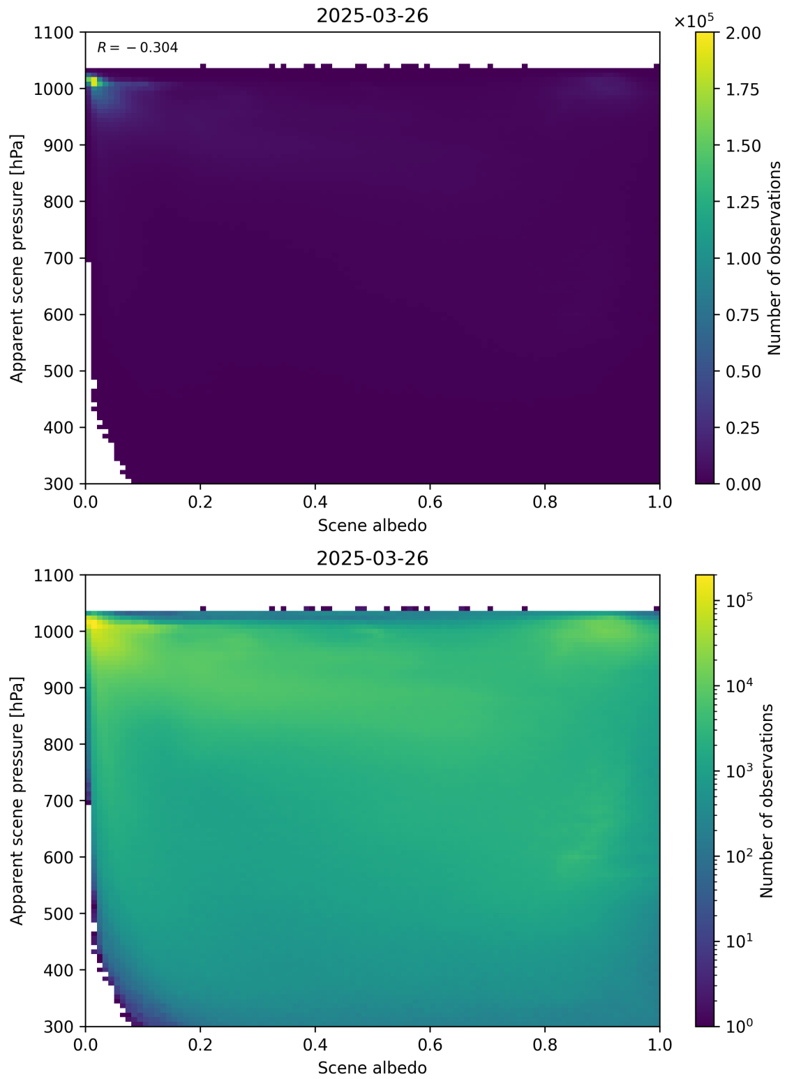
Figure 102: Scatter density plot of “Scene albedo” against “Apparent scene pressure” for 2025-03-25 to 2025-03-27.
