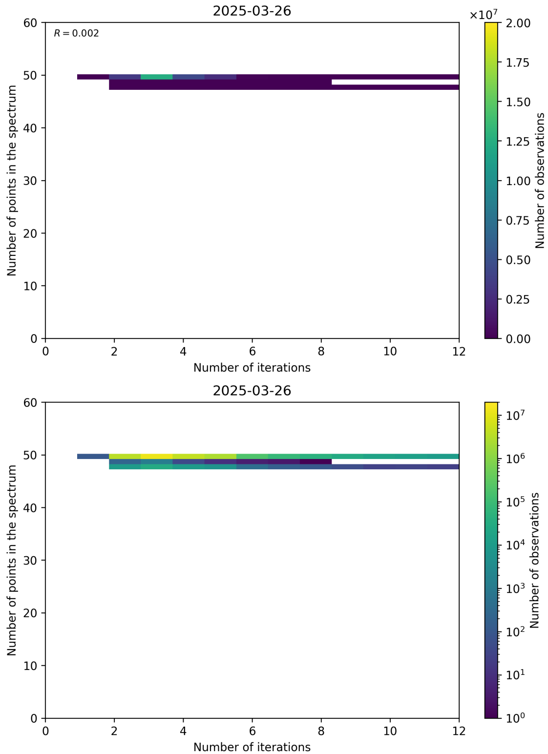
Figure 99: Scatter density plot of “Number of iterations” against “Number of points in the spectrum” for 2025-03-25 to 2025-03-27.
