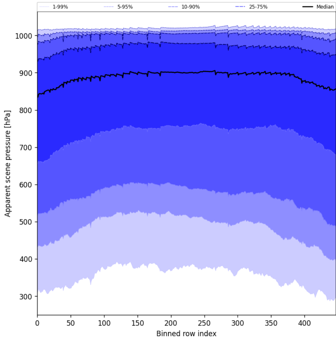
Figure 53: Along track statistics of “Apparent scene pressure” for 2025-03-25 to 2025-03-27
