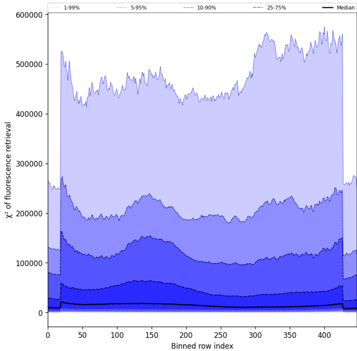
Figure 59: Along track statistics of “ \chi^2 of fluorescence retrieval” for 2025-03-25 to 2025-03-27
