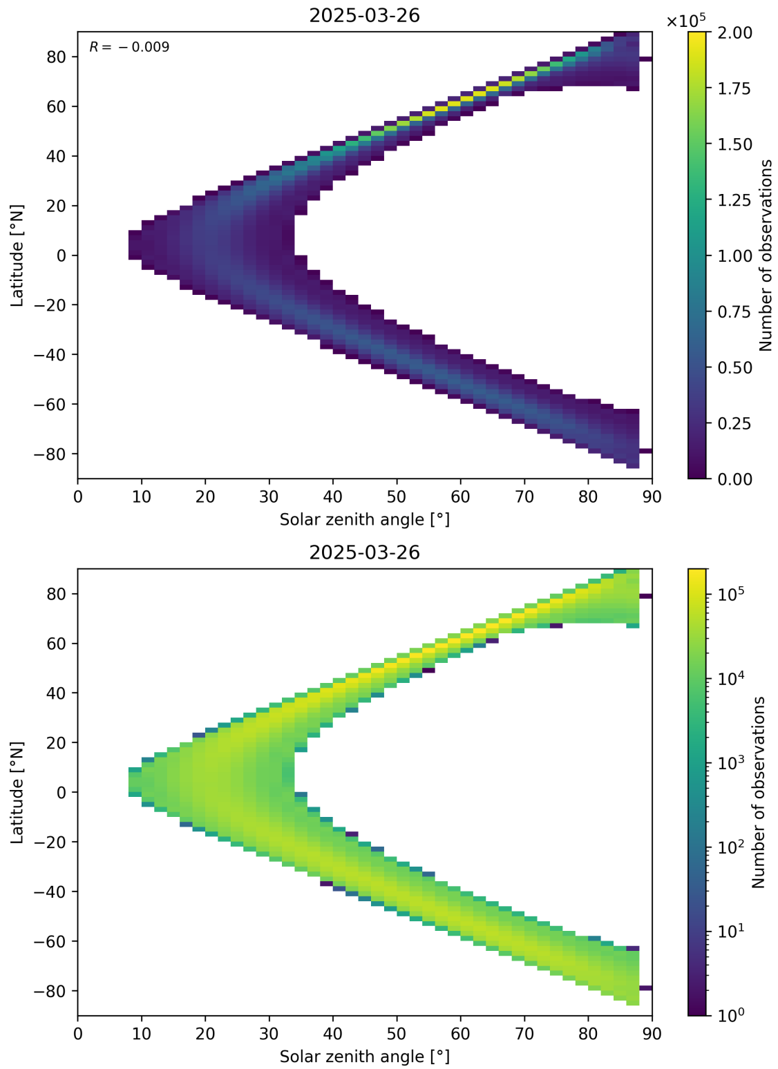
Figure 113: Scatter density plot of “Solar zenith angle” against “Latitude” for 2025-03-25 to 2025-03-27.
