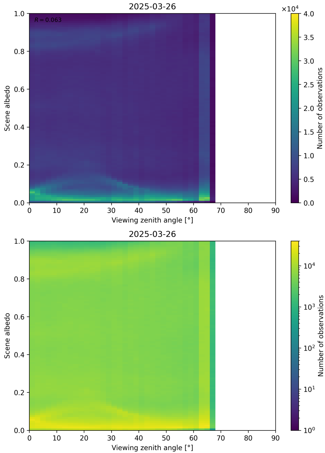
Figure 126: Scatter density plot of “Viewing zenith angle” against “Scene albedo” for 2025-03-25 to 2025-03-27.
