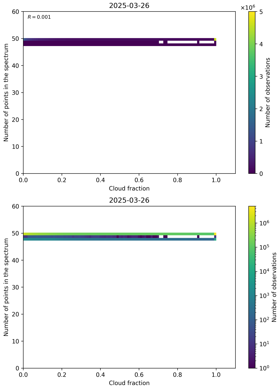
Figure 74: Scatter density plot of “Cloud fraction” against “Number of points in the spectrum” for 2025-03-25 to 2025-03-27.
