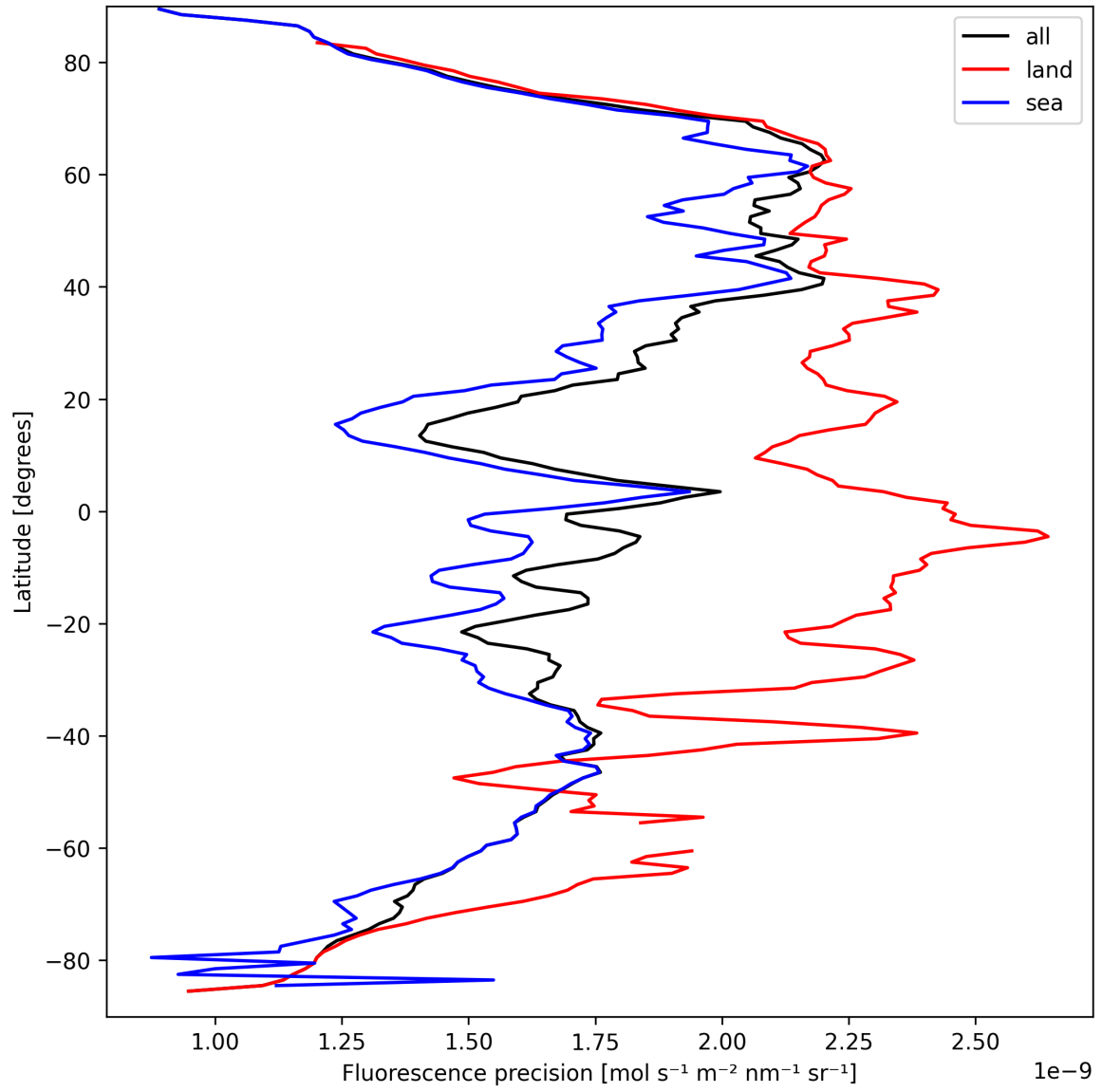
Figure 24: Zonal average of “Fluorescence precision” for 2025-03-25 to 2025-03-27.
