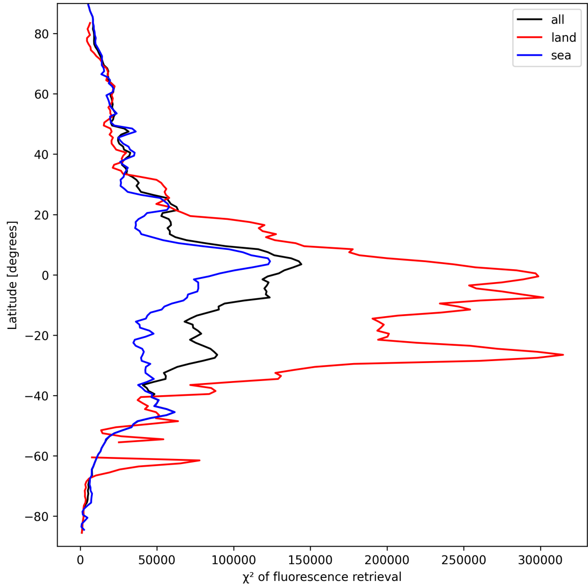
Figure 25: Zonal average of “ \chi^2 of fluorescence retrieval” for 2025-03-25 to 2025-03-27.
