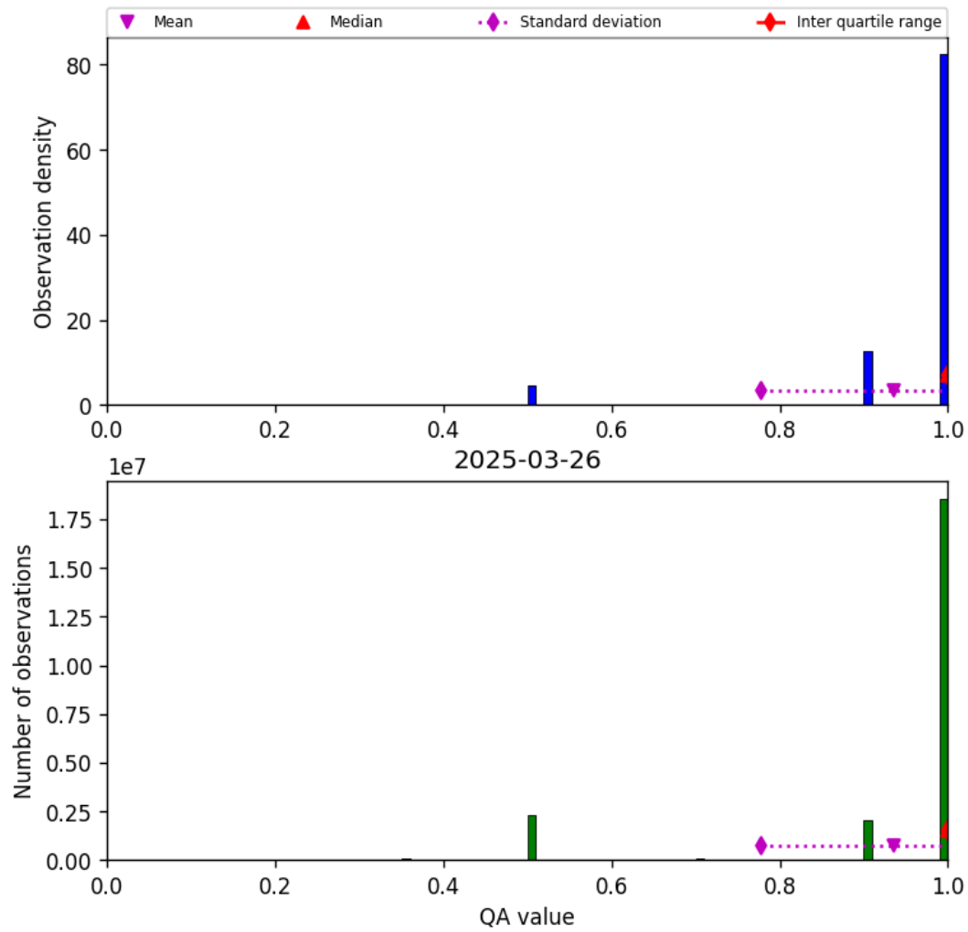
Figure 29: Histogram of “QA value” for 2025-03-25 to 2025-03-27
