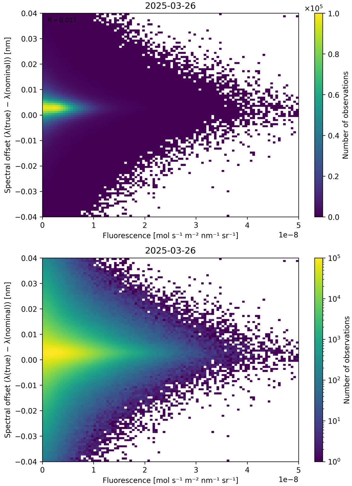
Figure 87: Scatter density plot of “Fluorescence” against “Spectral offset ( \lambda_{\text{true}} - \lambda_{\text{nominal}} )” for 2025-03-25 to 2025-03-27.
