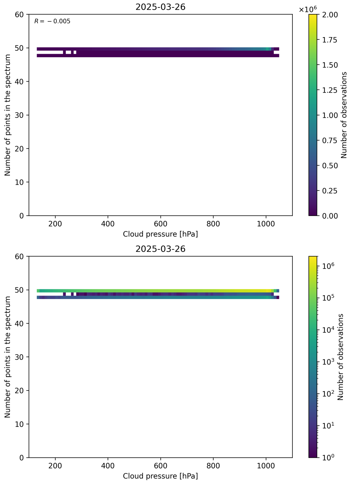
Figure 82: Scatter density plot of “Cloud pressure” against “Number of points in the spectrum” for 2025-03-25 to 2025-03-27.
