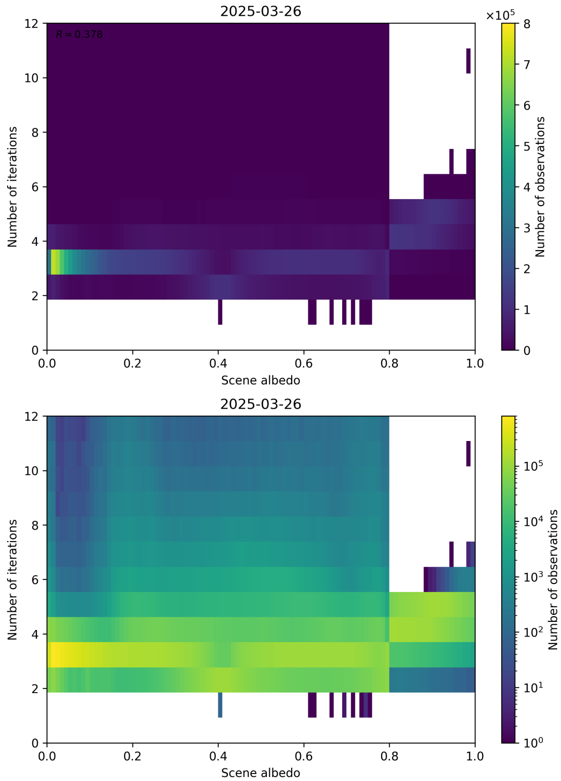
Figure 105: Scatter density plot of “Scene albedo” against “Number of iterations” for 2025-03-25 to 2025-03-27.
