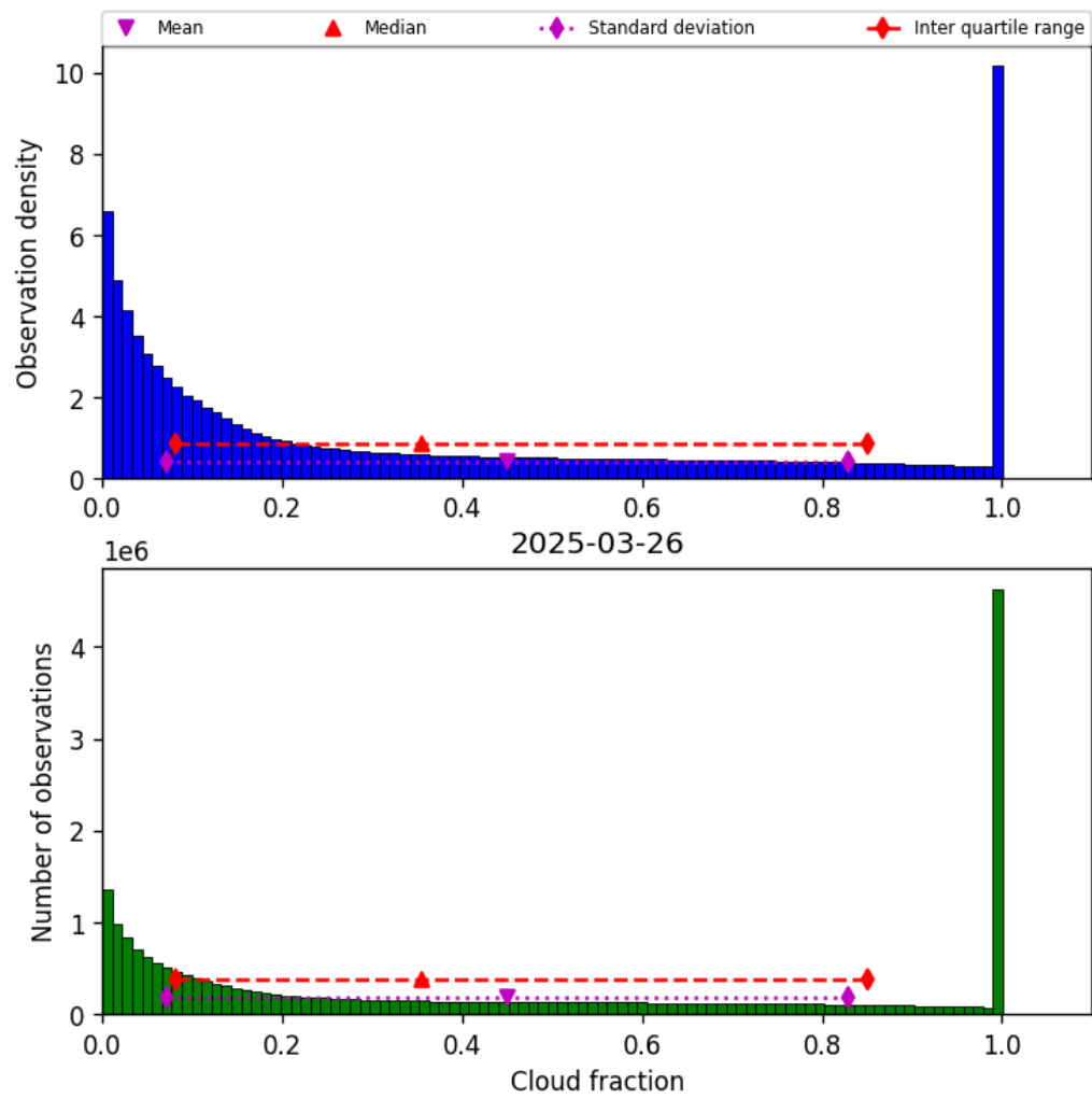
Figure 32: Histogram of “Cloud fraction” for 2025-03-25 to 2025-03-27
