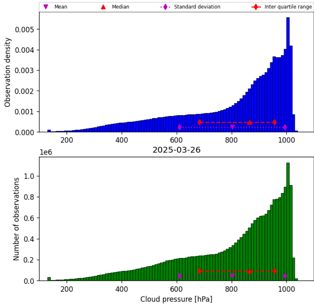
Figure 30: Histogram of “Cloud pressure” for 2025-03-25 to 2025-03-27
