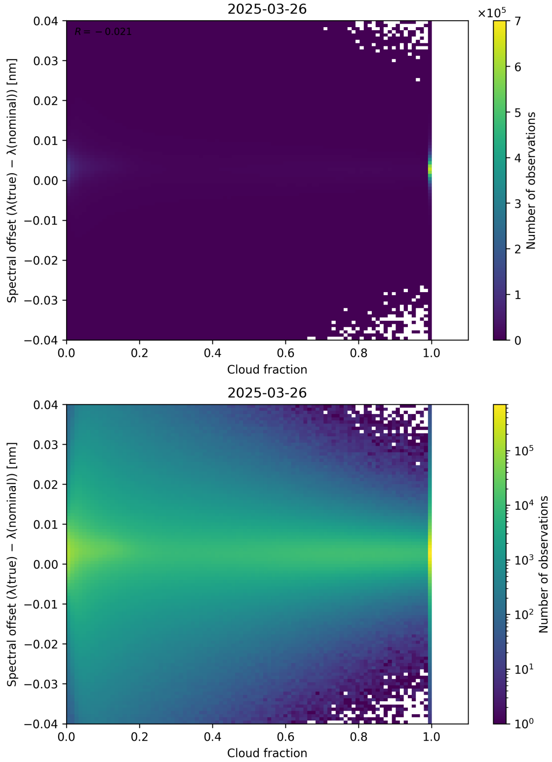
Figure 76: Scatter density plot of “Cloud fraction” against “Spectral offset ( \lambda_{\text{true}} - \lambda_{\text{nominal}} )” for 2025-03-25 to 2025-03-27.
