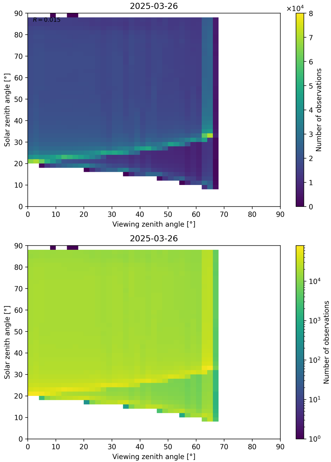
Figure 127: Scatter density plot of “Viewing zenith angle” against “Solar zenith angle” for 2025-03-25 to 2025-03-27.
