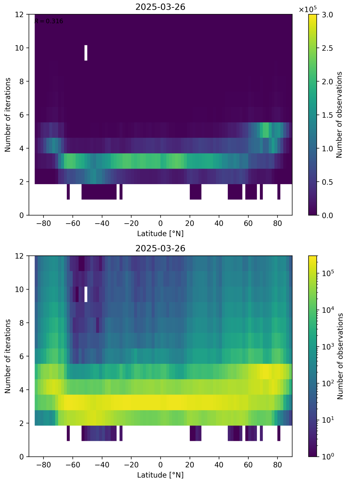
Figure 93: Scatter density plot of “Latitude” against “Number of iterations” for 2025-03-25 to 2025-03-27.
