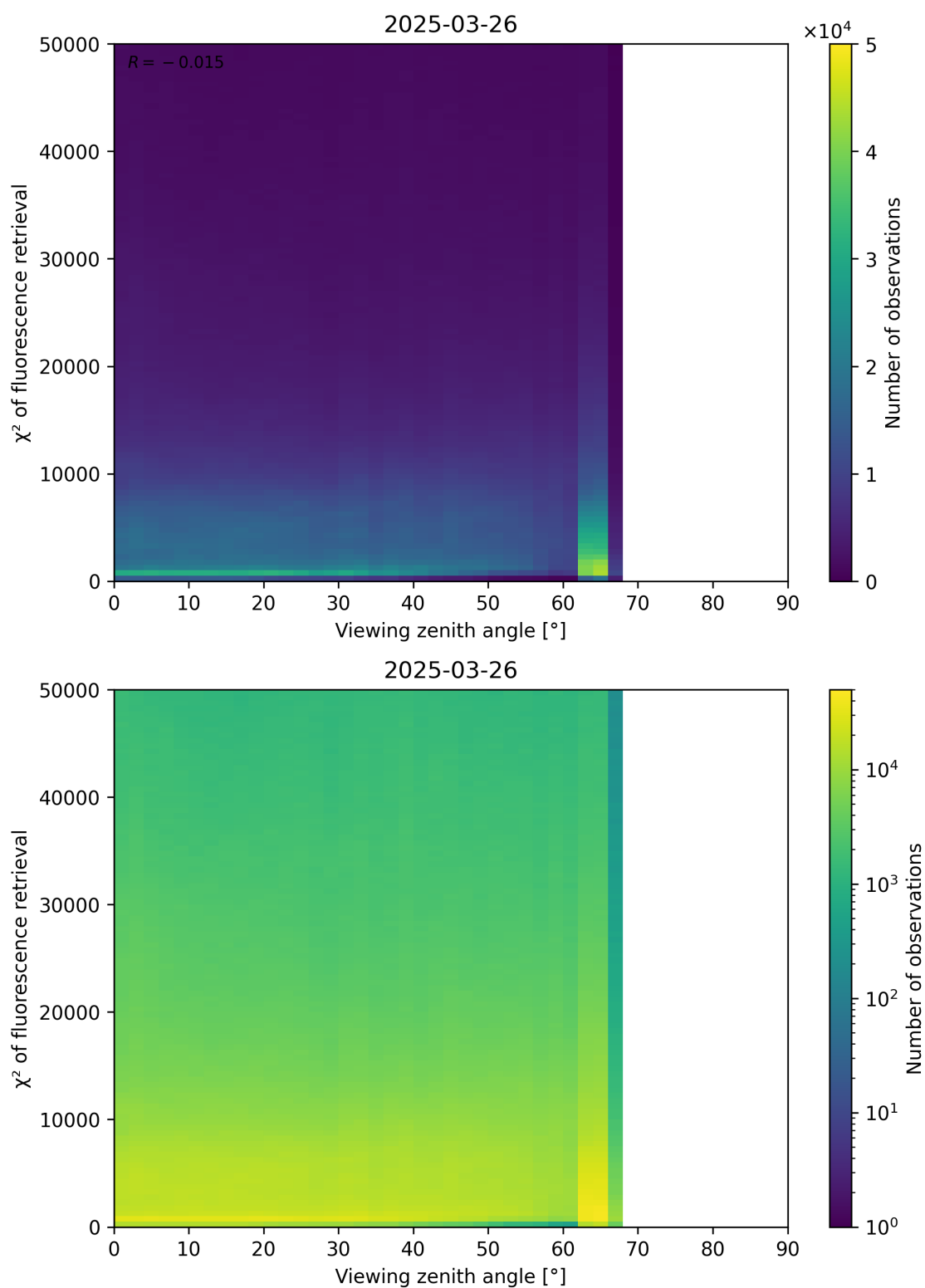
Figure 119: Scatter density plot of “Viewing zenith angle” against “ \chi^2 of fluorescence retrieval” for 2025-03-25 to 2025-03-27.
