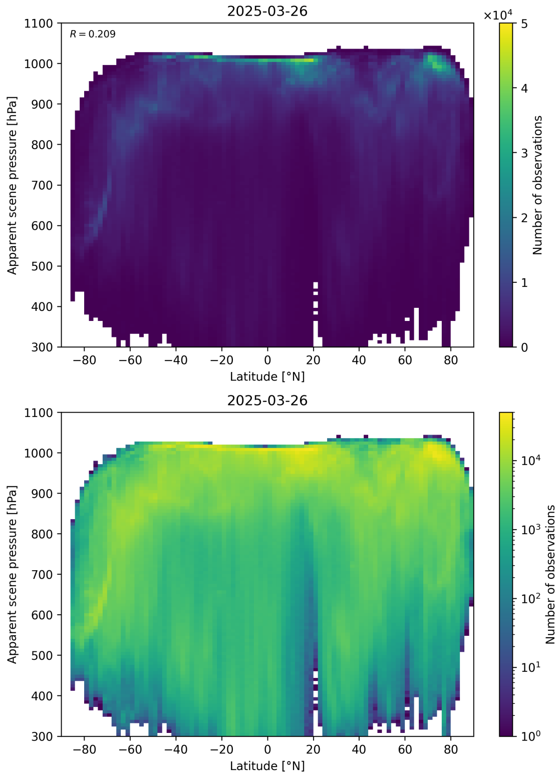
Figure 88: Scatter density plot of “Latitude” against “Apparent scene pressure” for 2025-03-25 to 2025-03-27.
