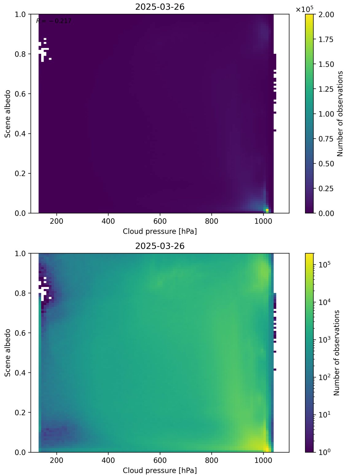
Figure 83: Scatter density plot of “Cloud pressure” against “Scene albedo” for 2025-03-25 to 2025-03-27.
