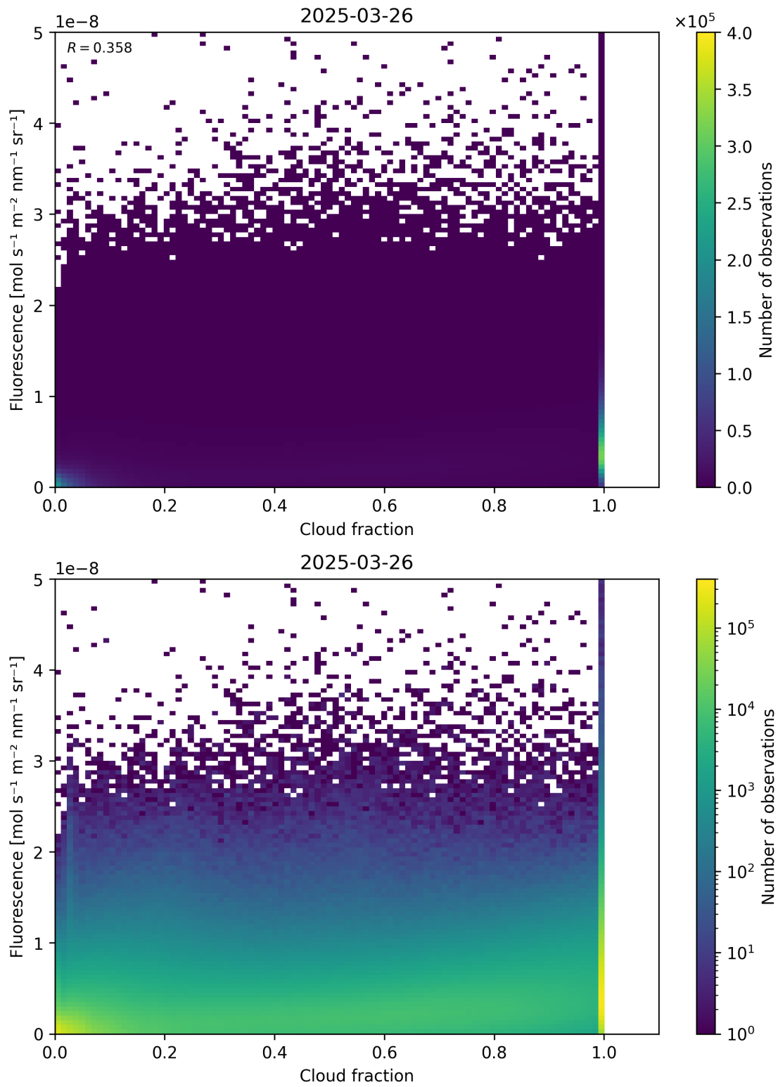
Figure 72: Scatter density plot of “Cloud fraction” against “Fluorescence” for 2025-03-25 to 2025-03-27.
