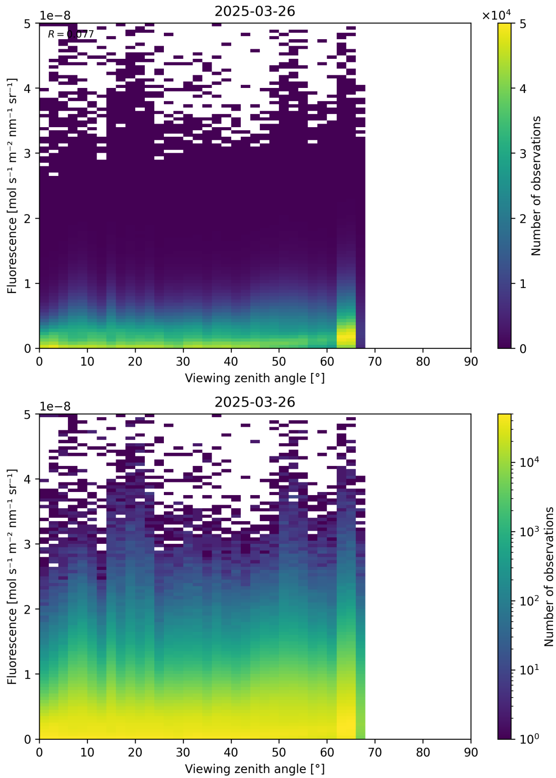
Figure 122: Scatter density plot of “Viewing zenith angle” against “Fluorescence” for 2025-03-25 to 2025-03-27.
