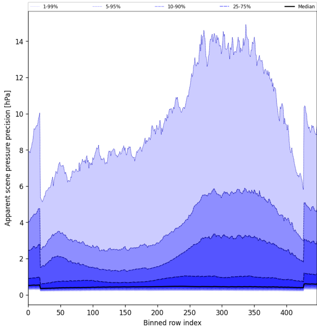
Figure 54: Along track statistics of “Apparent scene pressure precision” for 2025-03-25 to 2025-03-27
