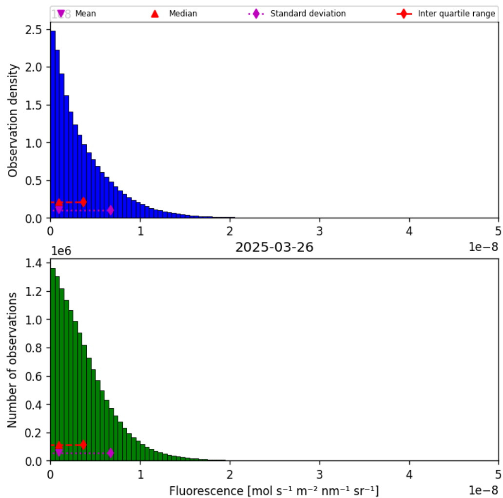
Figure 40: Histogram of “Fluorescence” for 2025-03-25 to 2025-03-27
