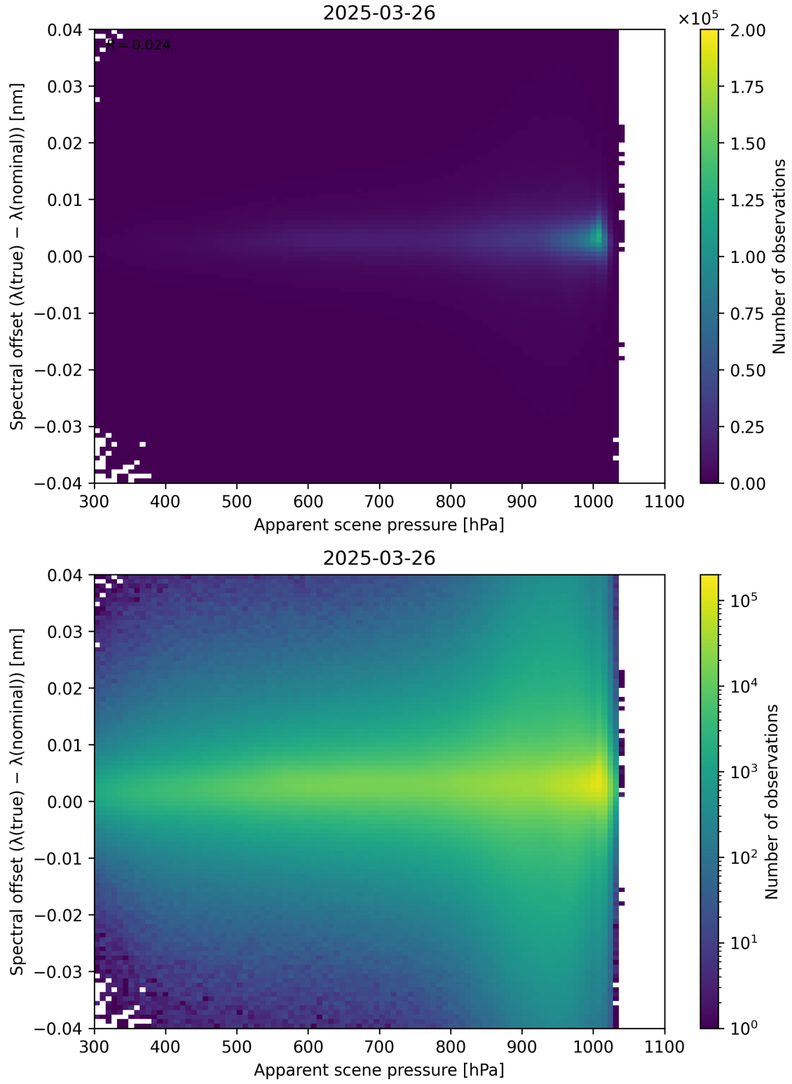
Figure 67: Scatter density plot of “Apparent scene pressure” against “Spectral offset ( \lambda_{\text{true}} - \lambda_{\text{nominal}} )” for 2025-03-25 to 2025-03-27.
