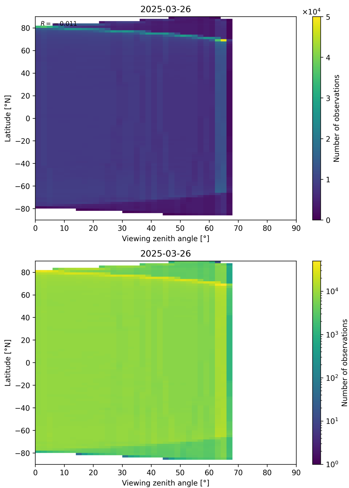
Figure 123: Scatter density plot of “Viewing zenith angle” against “Latitude” for 2025-03-25 to 2025-03-27.
