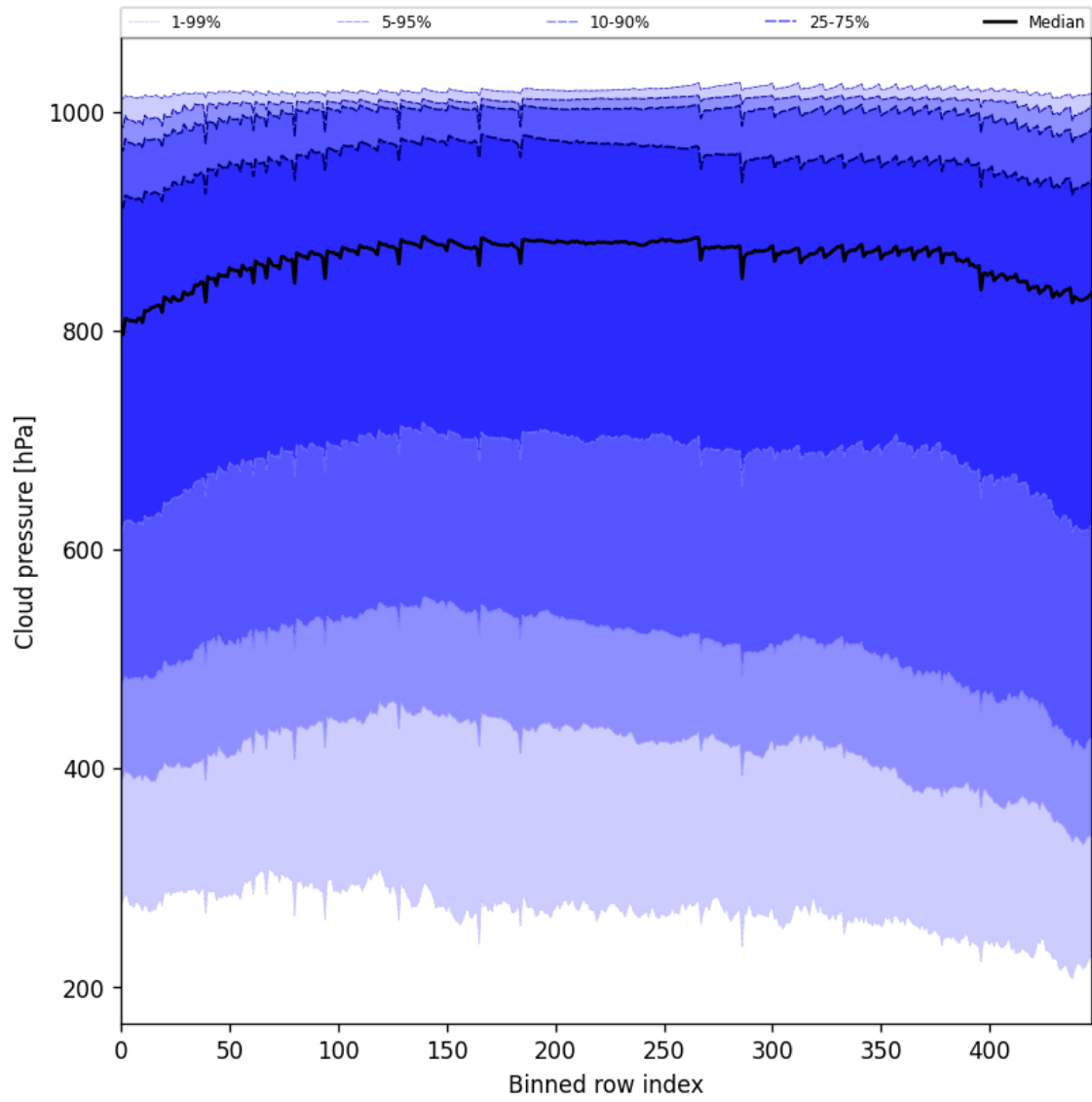
Figure 47: Along track statistics of “Cloud pressure” for 2025-03-25 to 2025-03-27
