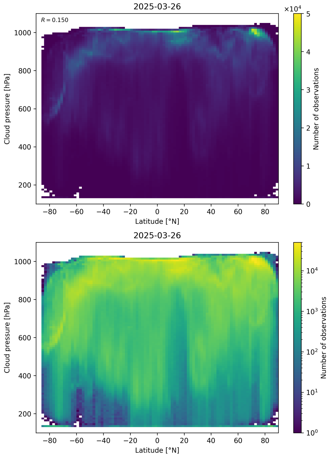
Figure 91: Scatter density plot of “Latitude” against “Cloud pressure” for 2025-03-25 to 2025-03-27.
