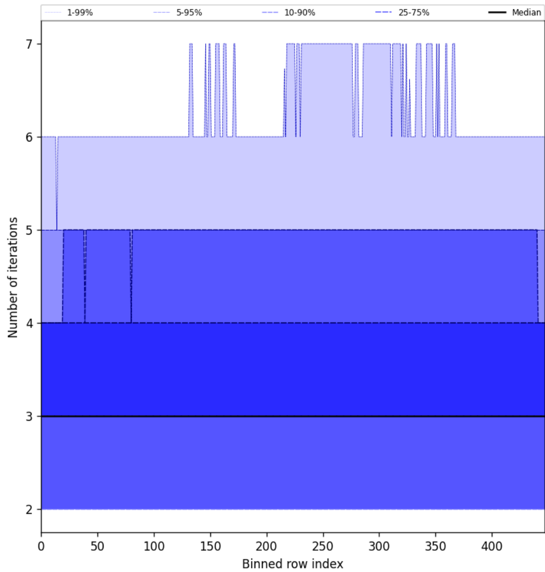
Figure 56: Along track statistics of “Number of iterations” for 2025-03-26 to 2025-03-28
