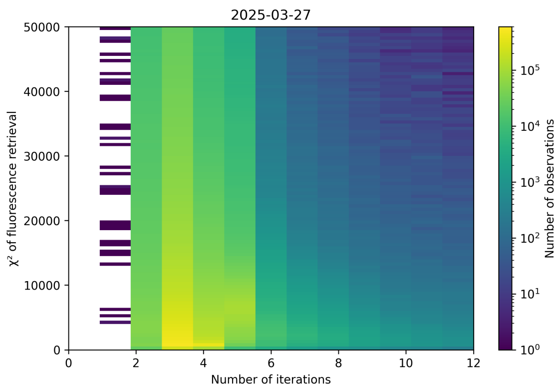
Figure 97: Scatter density plot of “Number of iterations” against “ \chi^2 of fluorescence retrieval” for 2025-03-26 to 2025-03-28.
