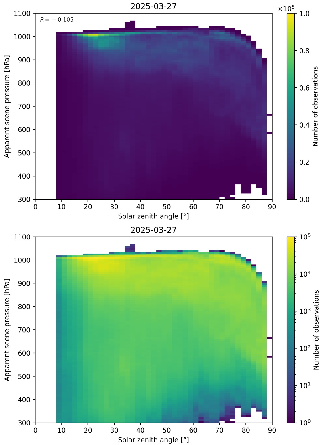
Figure 108: Scatter density plot of “Solar zenith angle” against “Apparent scene pressure” for 2025-03-26 to 2025-03-28.
