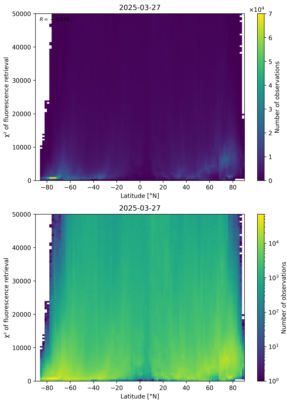
Figure 89: Scatter density plot of “Latitude” against “ \chi^2 of fluorescence retrieval” for 2025-03-26 to 2025-03-28.
