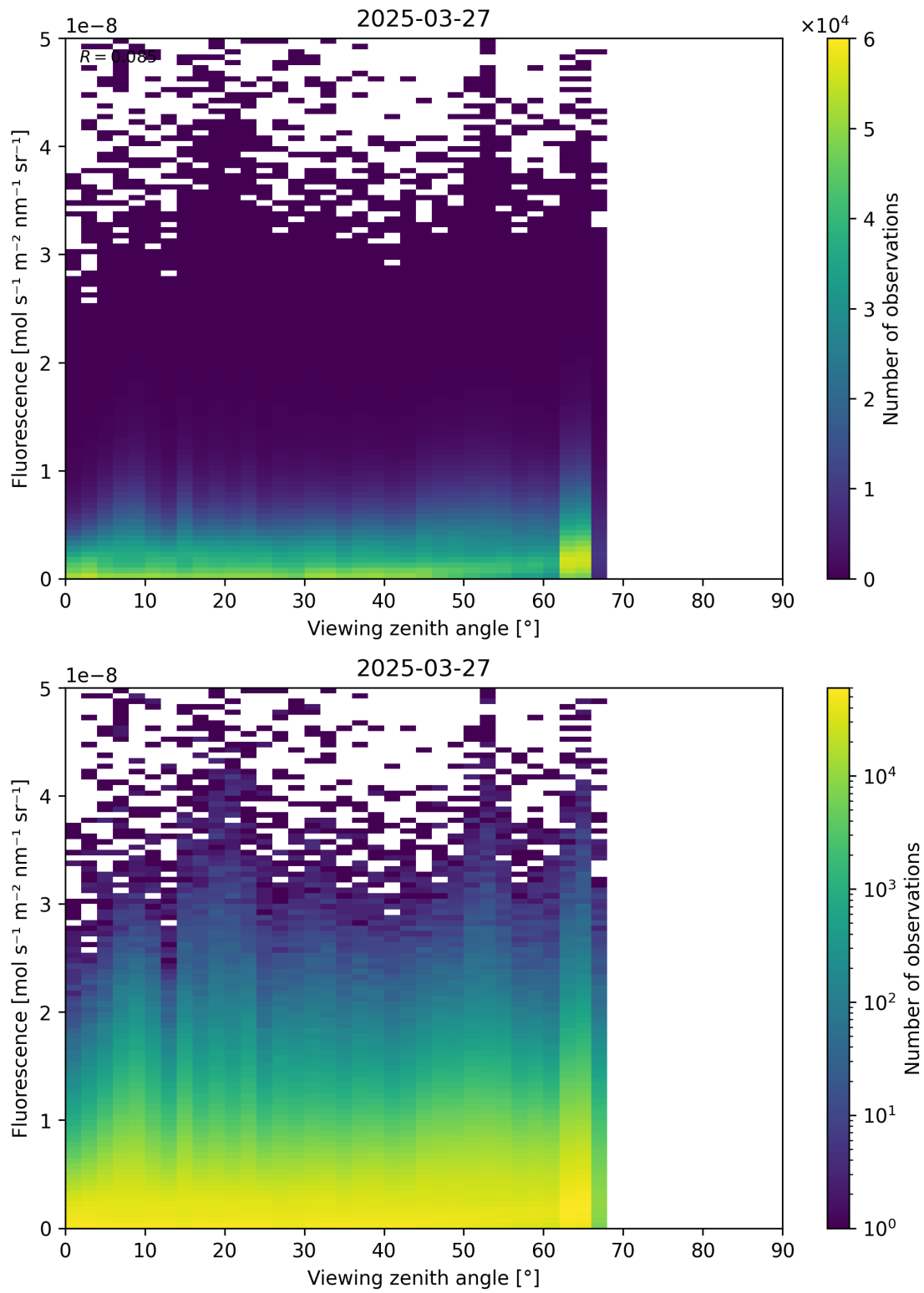
Figure 122: Scatter density plot of “Viewing zenith angle” against “Fluorescence” for 2025-03-26 to 2025-03-28.
