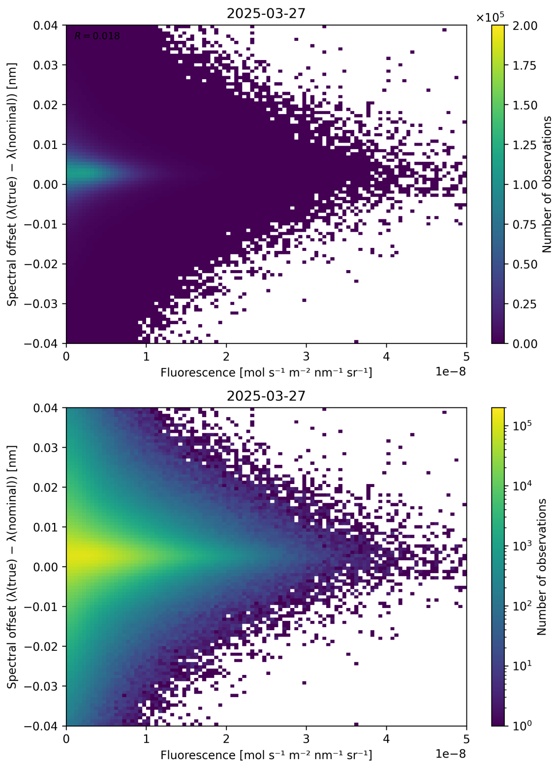
Figure 87: Scatter density plot of “Fluorescence” against “Spectral offset ( \lambda_{\text{true}} - \lambda_{\text{nominal}} )” for 2025-03-26 to 2025-03-28.
