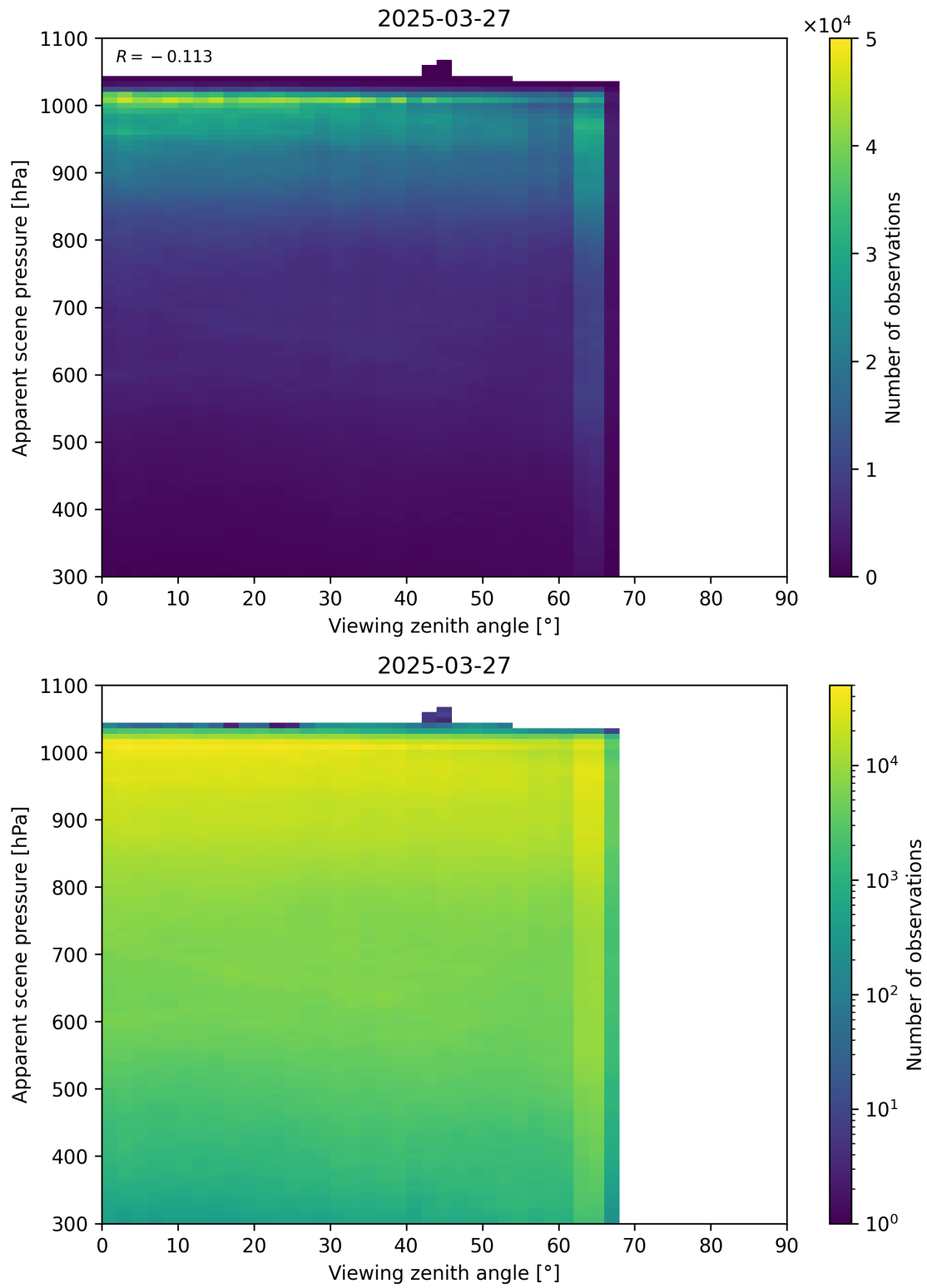
Figure 118: Scatter density plot of “Viewing zenith angle” against “Apparent scene pressure” for 2025-03-26 to 2025-03-28.
