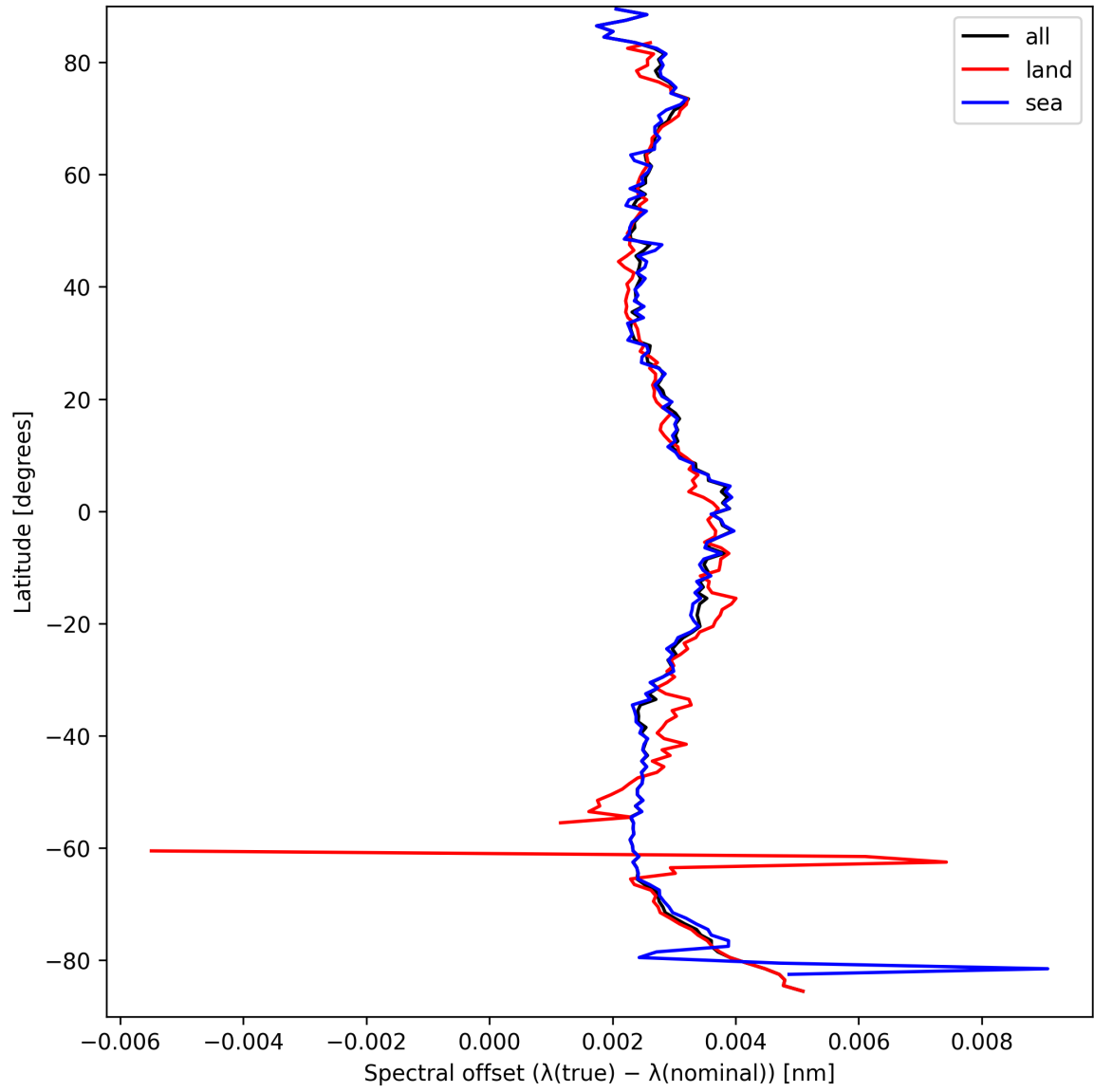
Figure 28: Zonal average of “Spectral offset ( \lambda_{\text{true}} - \lambda_{\text{nominal}} )” for 2025-03-26 to 2025-03-28.
