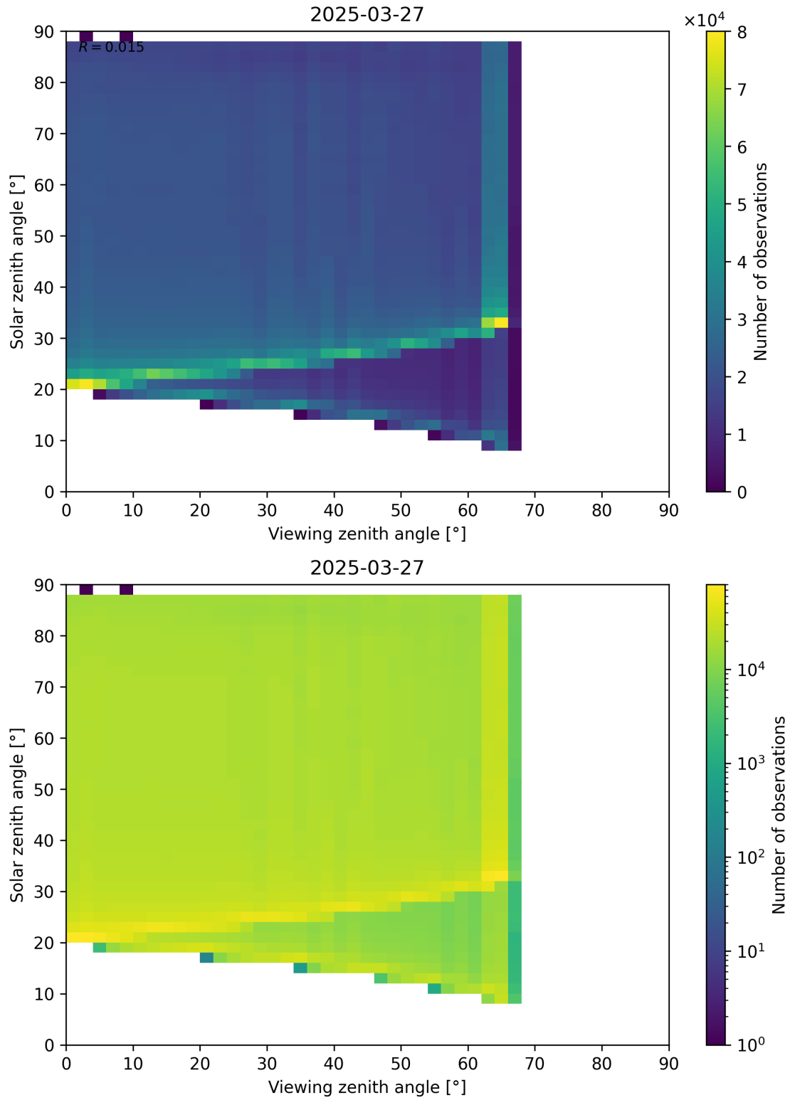
Figure 127: Scatter density plot of “Viewing zenith angle” against “Solar zenith angle” for 2025-03-26 to 2025-03-28.
