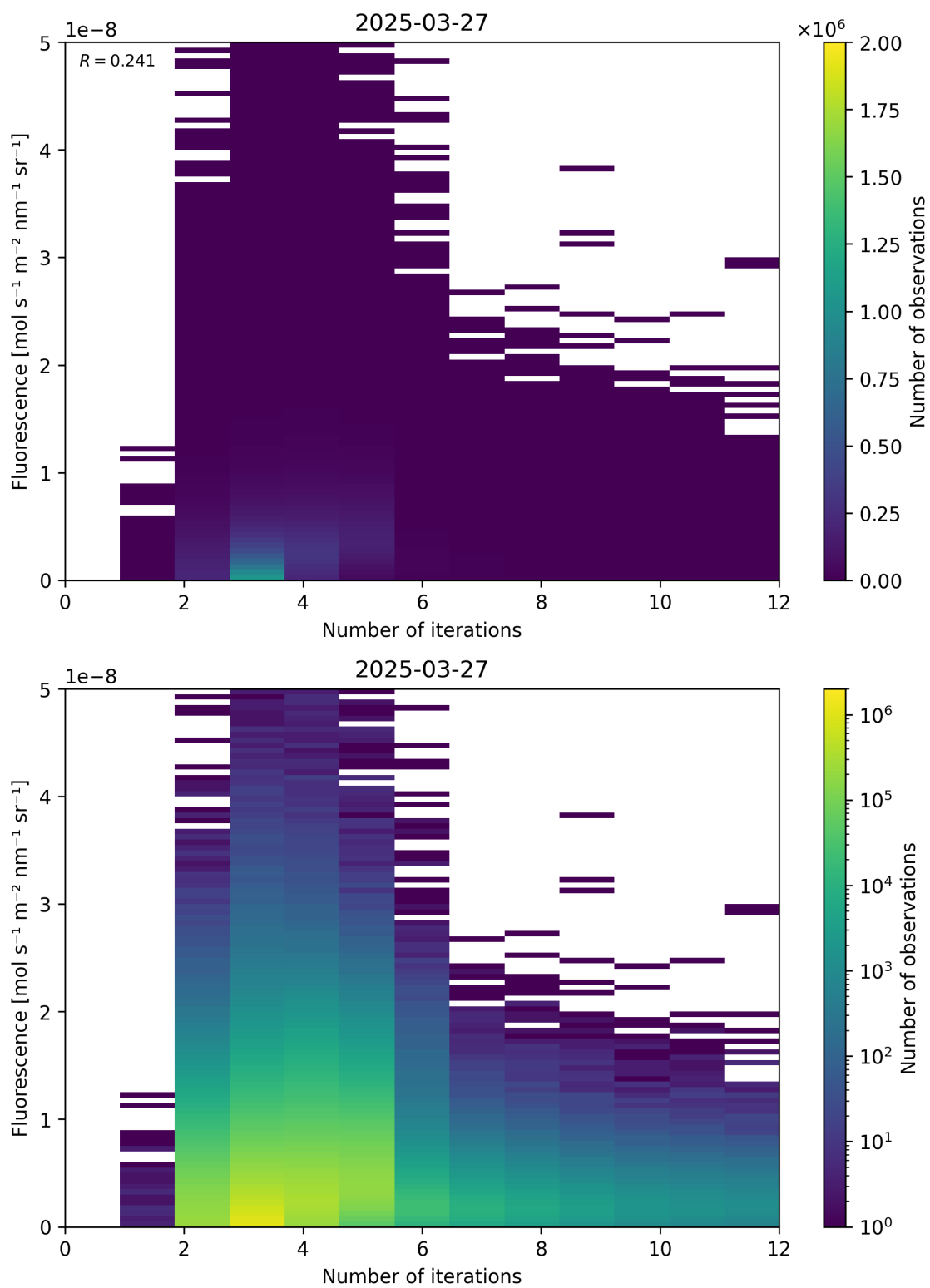
Figure 98: Scatter density plot of “Number of iterations” against “Fluorescence” for 2025-03-26 to 2025-03-28.
