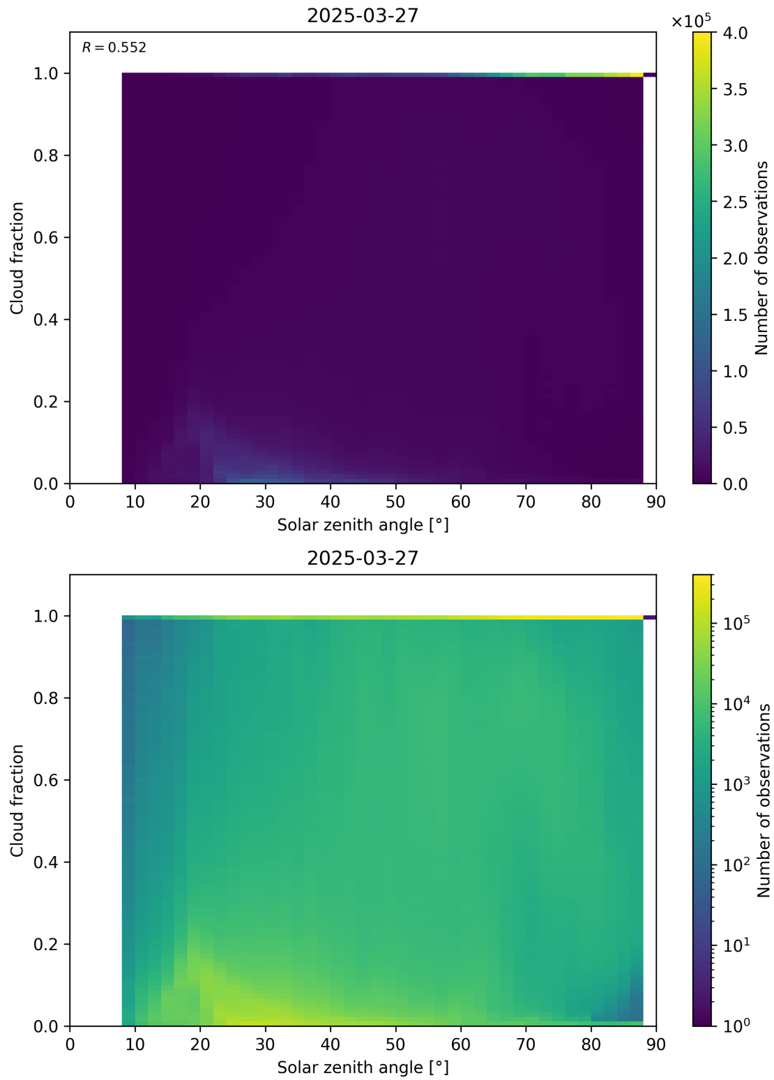
Figure 110: Scatter density plot of “Solar zenith angle” against “Cloud fraction” for 2025-03-26 to 2025-03-28.
