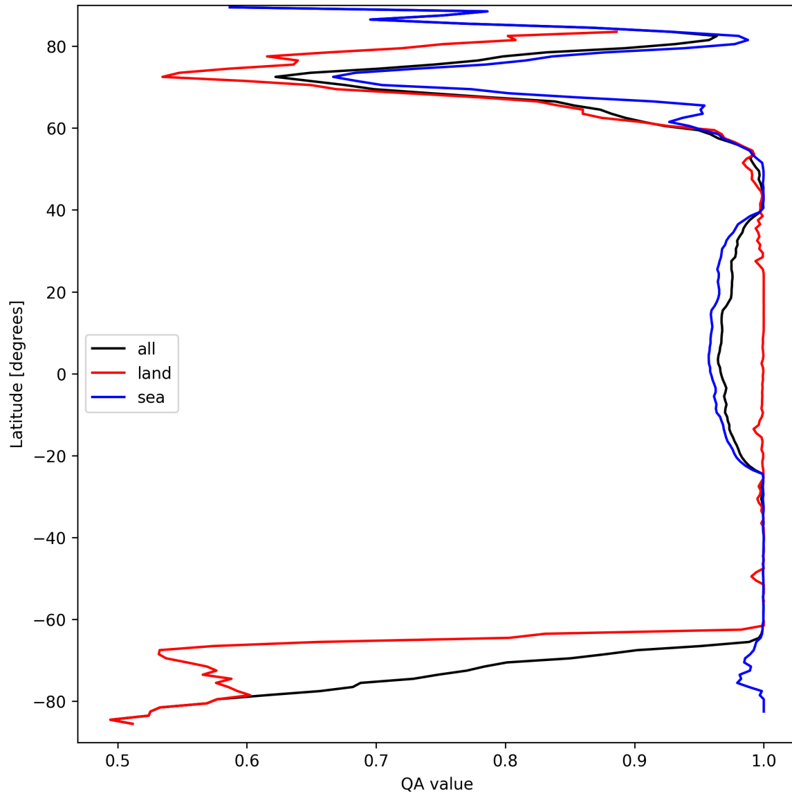
Figure 12: Zonal average of "QA value" for 2025-03-26 to 2025-03-28.
