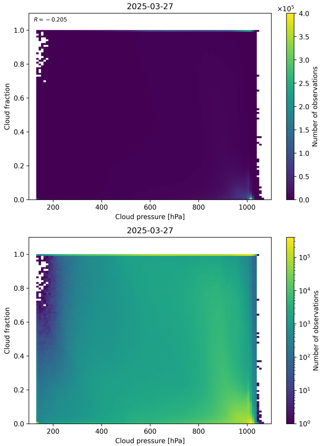
Figure 79: Scatter density plot of “Cloud pressure” against “Cloud fraction” for 2025-03-26 to 2025-03-28.
