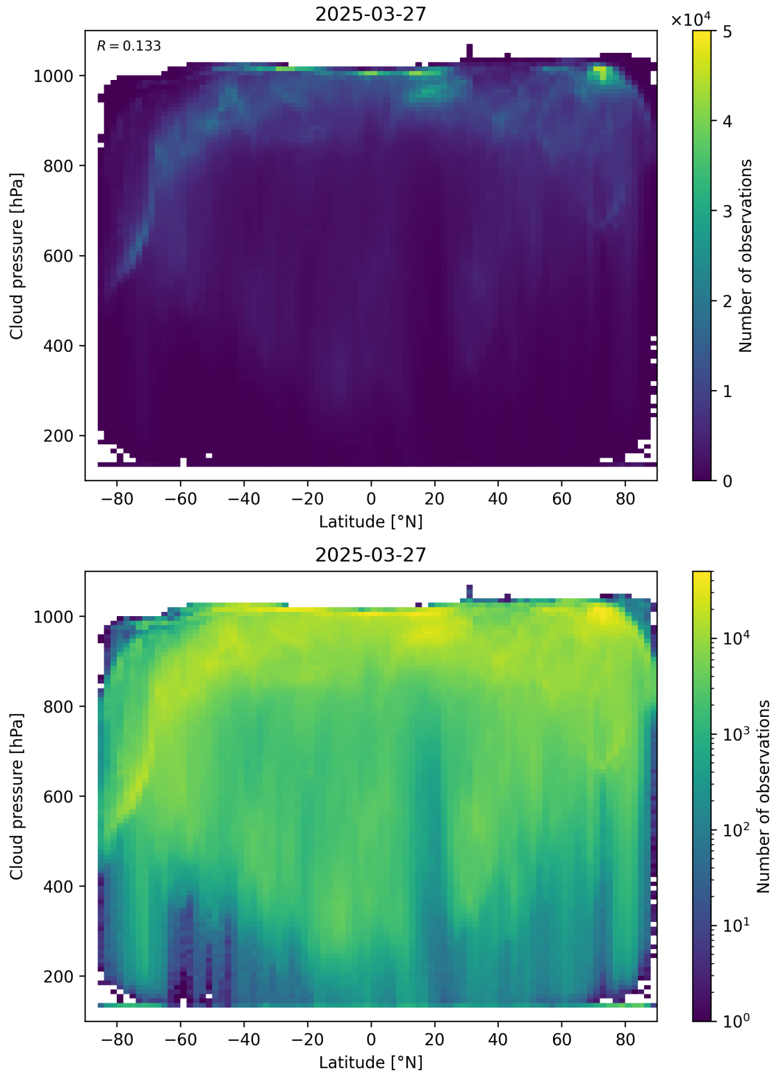
Figure 91: Scatter density plot of “Latitude” against “Cloud pressure” for 2025-03-26 to 2025-03-28.
