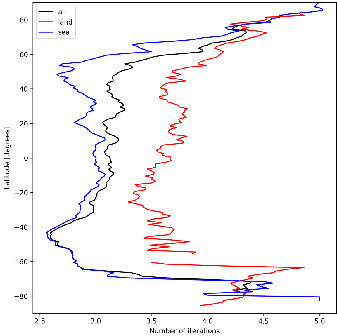
Figure 22: Zonal average of “Number of iterations” for 2025-03-26 to 2025-03-28.
