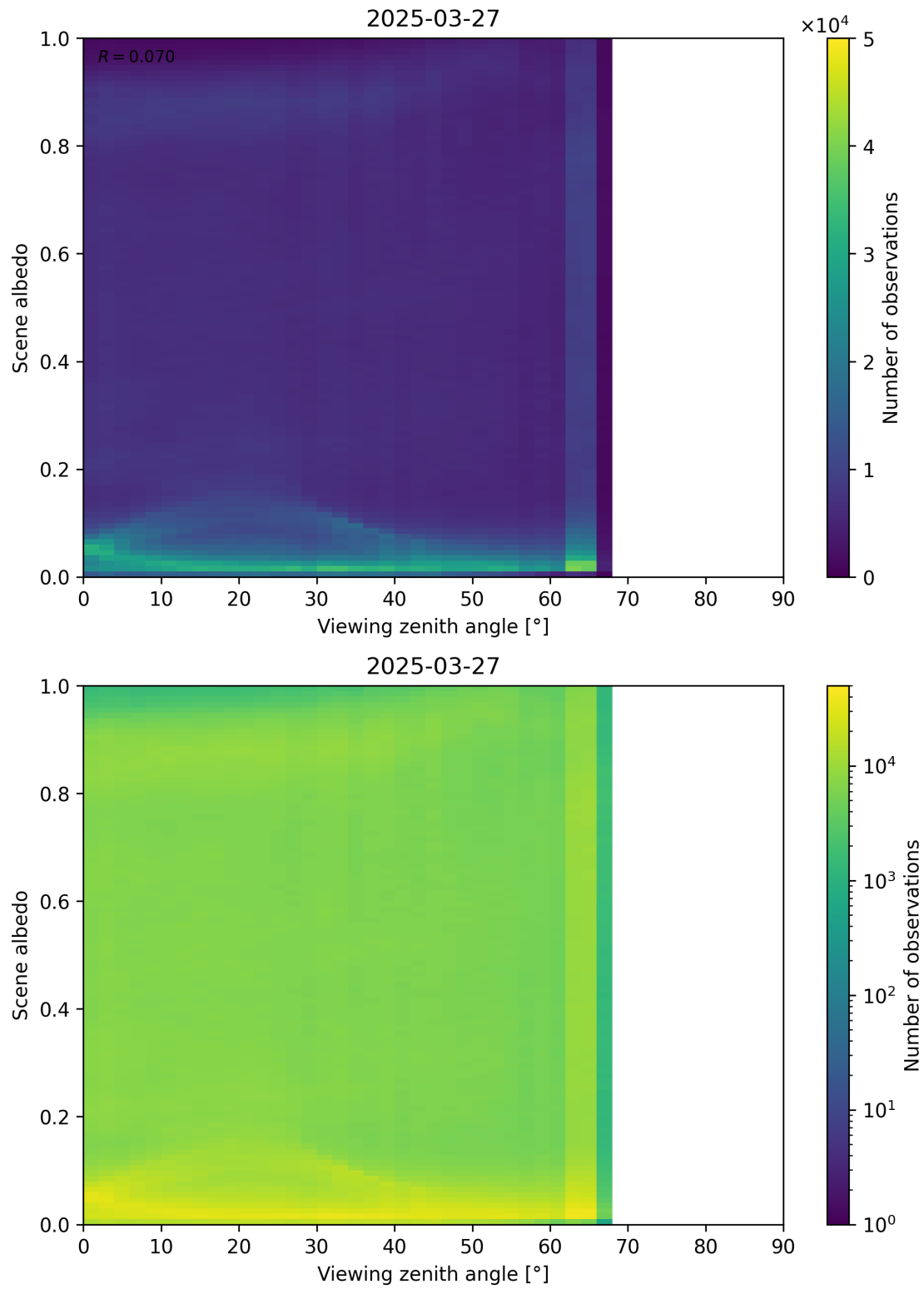
Figure 126: Scatter density plot of “Viewing zenith angle” against “Scene albedo” for 2025-03-26 to 2025-03-28.
