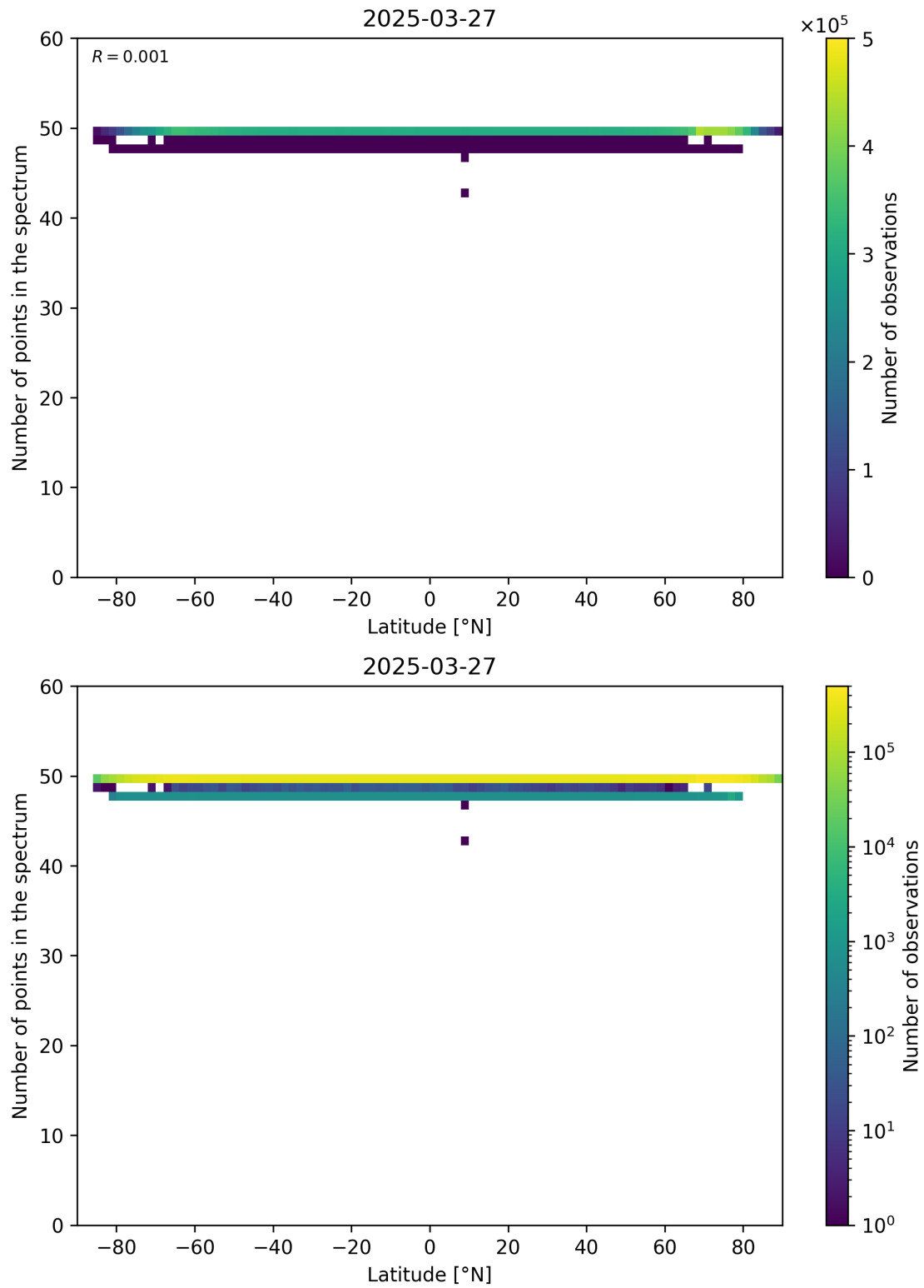
Figure 94: Scatter density plot of “Latitude” against “Number of points in the spectrum” for 2025-03-26 to 2025-03-28.
