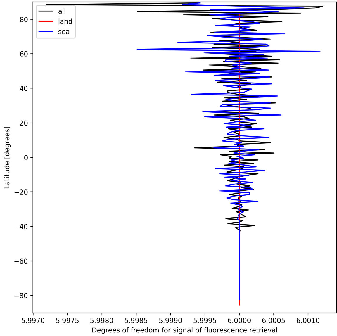
Figure 26: Zonal average of “Degrees of freedom for signal of fluorescence retrieval” for 2025-03-26 to 2025-03-28.
