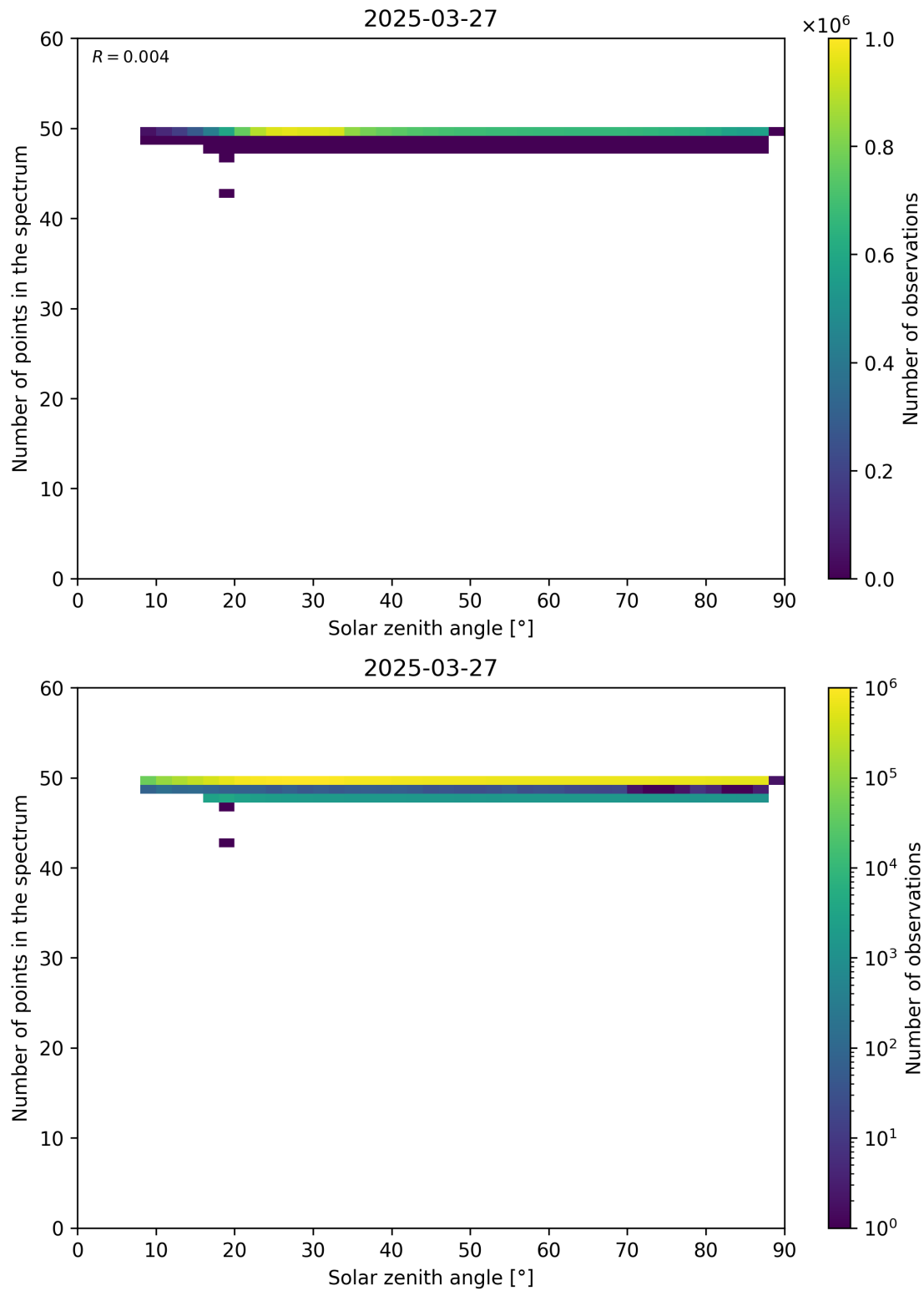
Figure 115: Scatter density plot of “Solar zenith angle” against “Number of points in the spectrum” for 2025-03-26 to 2025-03-28.
