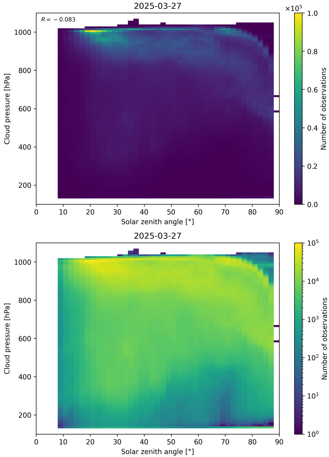
Figure 111: Scatter density plot of “Solar zenith angle” against “Cloud pressure” for 2025-03-26 to 2025-03-28.
