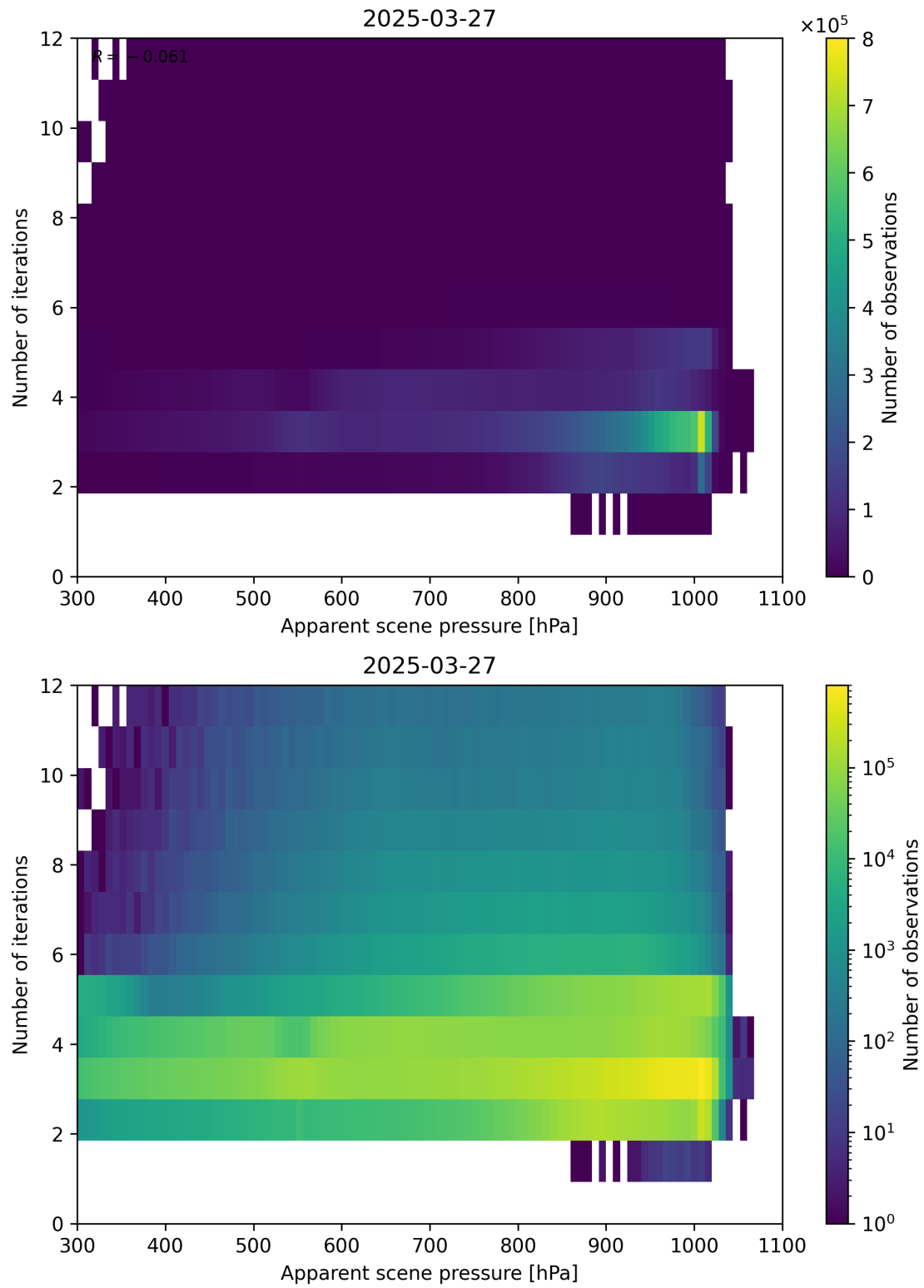
Figure 65: Scatter density plot of “Apparent scene pressure” against “Number of iterations” for 2025-03-26 to 2025-03-28.
