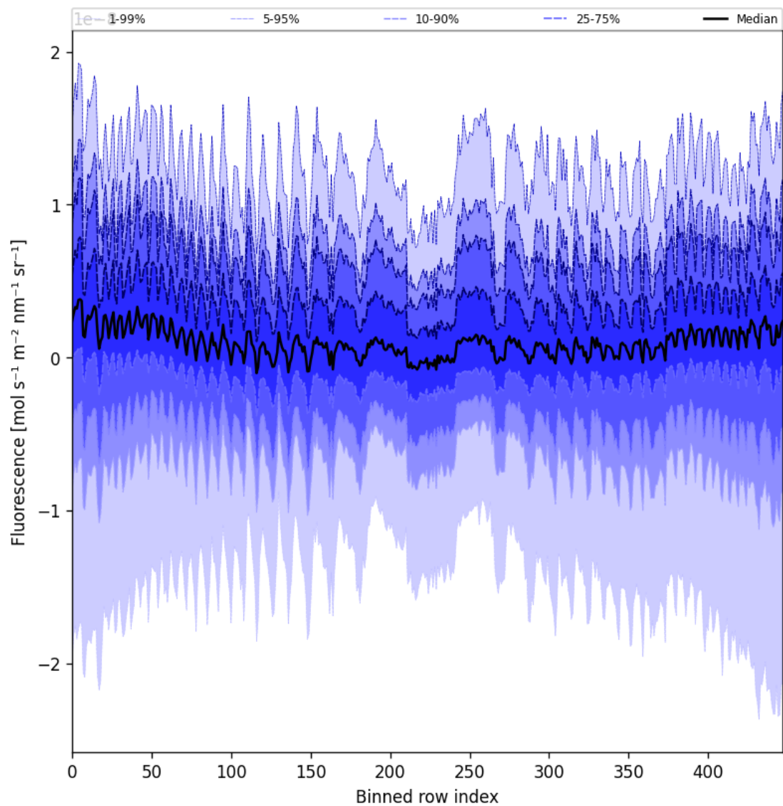
Figure 57: Along track statistics of “Fluorescence” for 2025-03-26 to 2025-03-28
