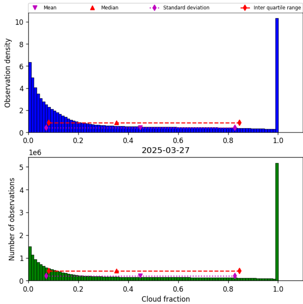
Figure 32: Histogram of “Cloud fraction” for 2025-03-26 to 2025-03-28
