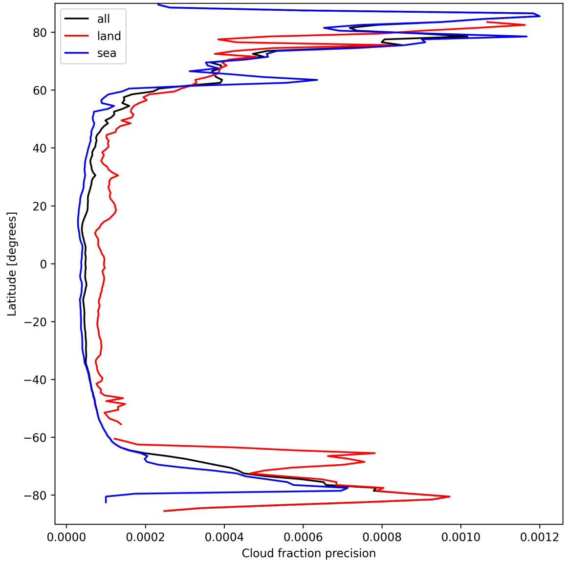
Figure 16: Zonal average of “Cloud fraction precision” for 2025-03-26 to 2025-03-28.
