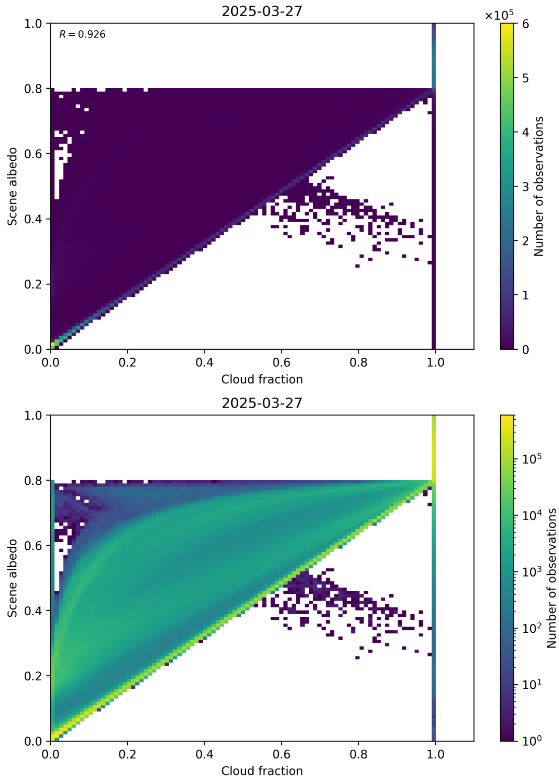
Figure 75: Scatter density plot of “Cloud fraction” against “Scene albedo” for 2025-03-26 to 2025-03-28.
