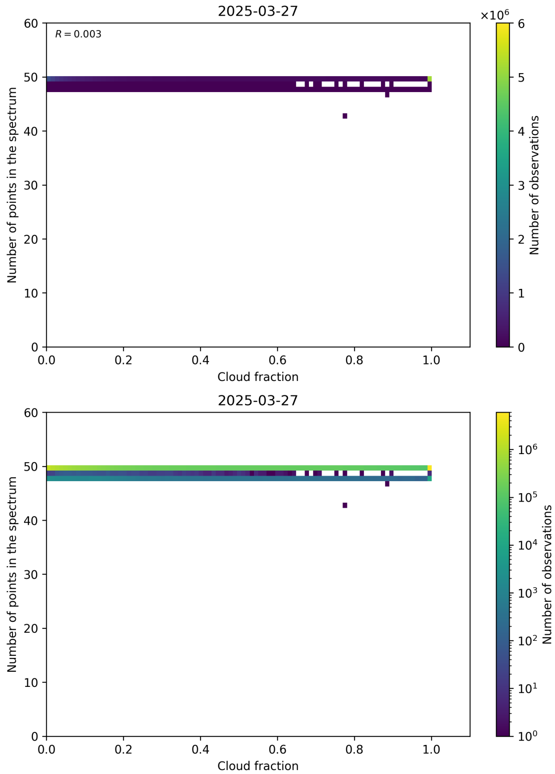
Figure 74: Scatter density plot of “Cloud fraction” against “Number of points in the spectrum” for 2025-03-26 to 2025-03-28.
