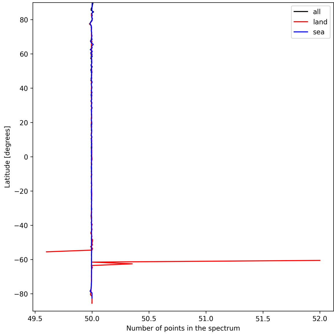
Figure 27: Zonal average of “Number of points in the spectrum” for 2025-03-26 to 2025-03-28.
