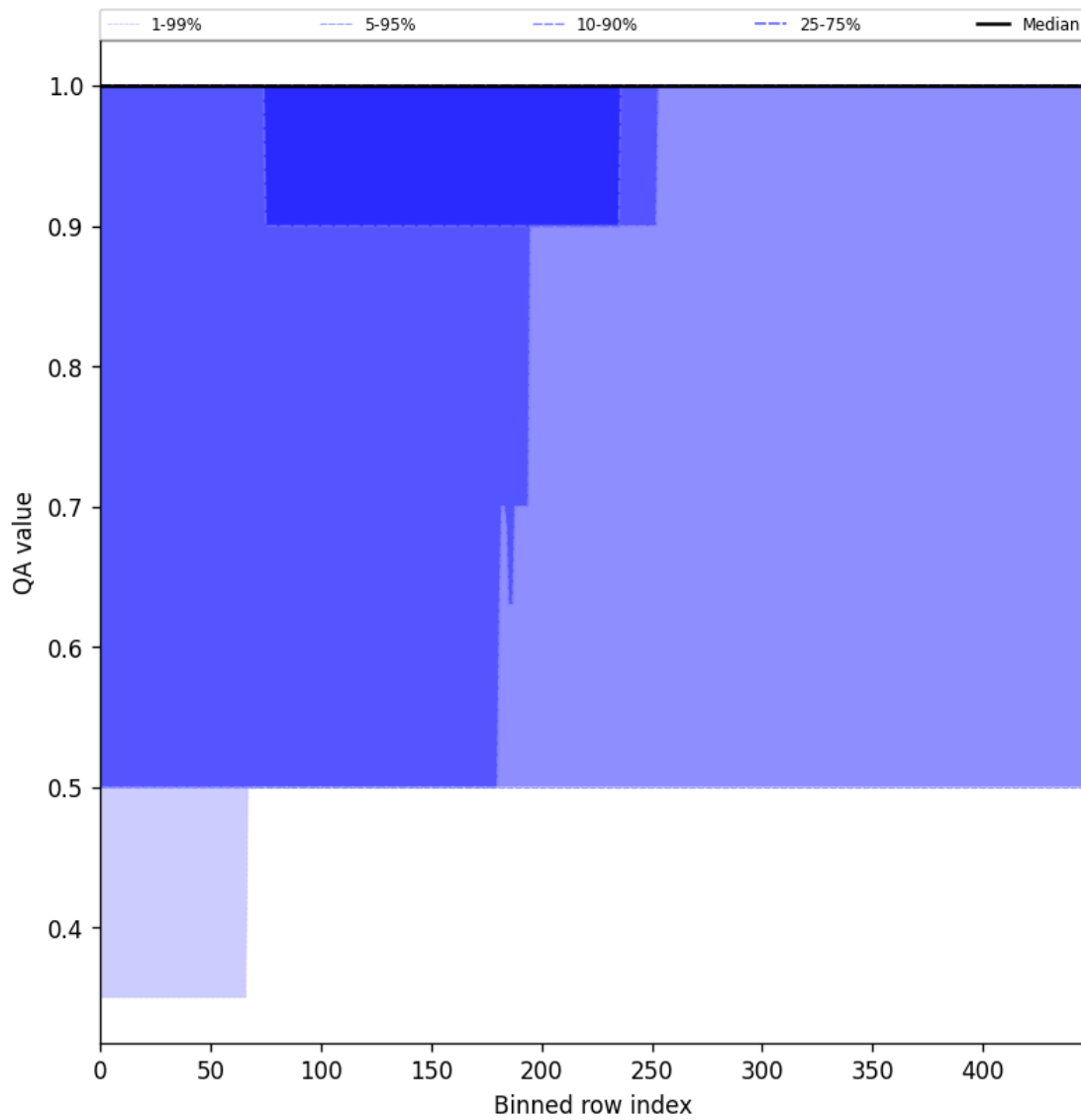
Figure 46: Along track statistics of “QA value” for 2025-03-26 to 2025-03-28
