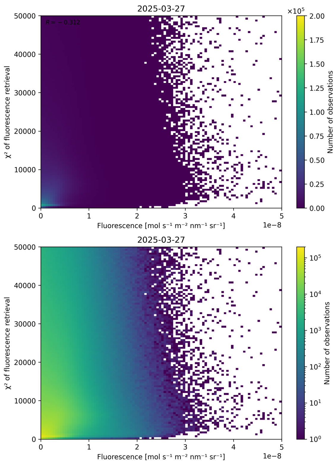
Figure 85: Scatter density plot of “Fluorescence” against “ \chi^2 of fluorescence retrieval” for 2025-03-26 to 2025-03-28.
