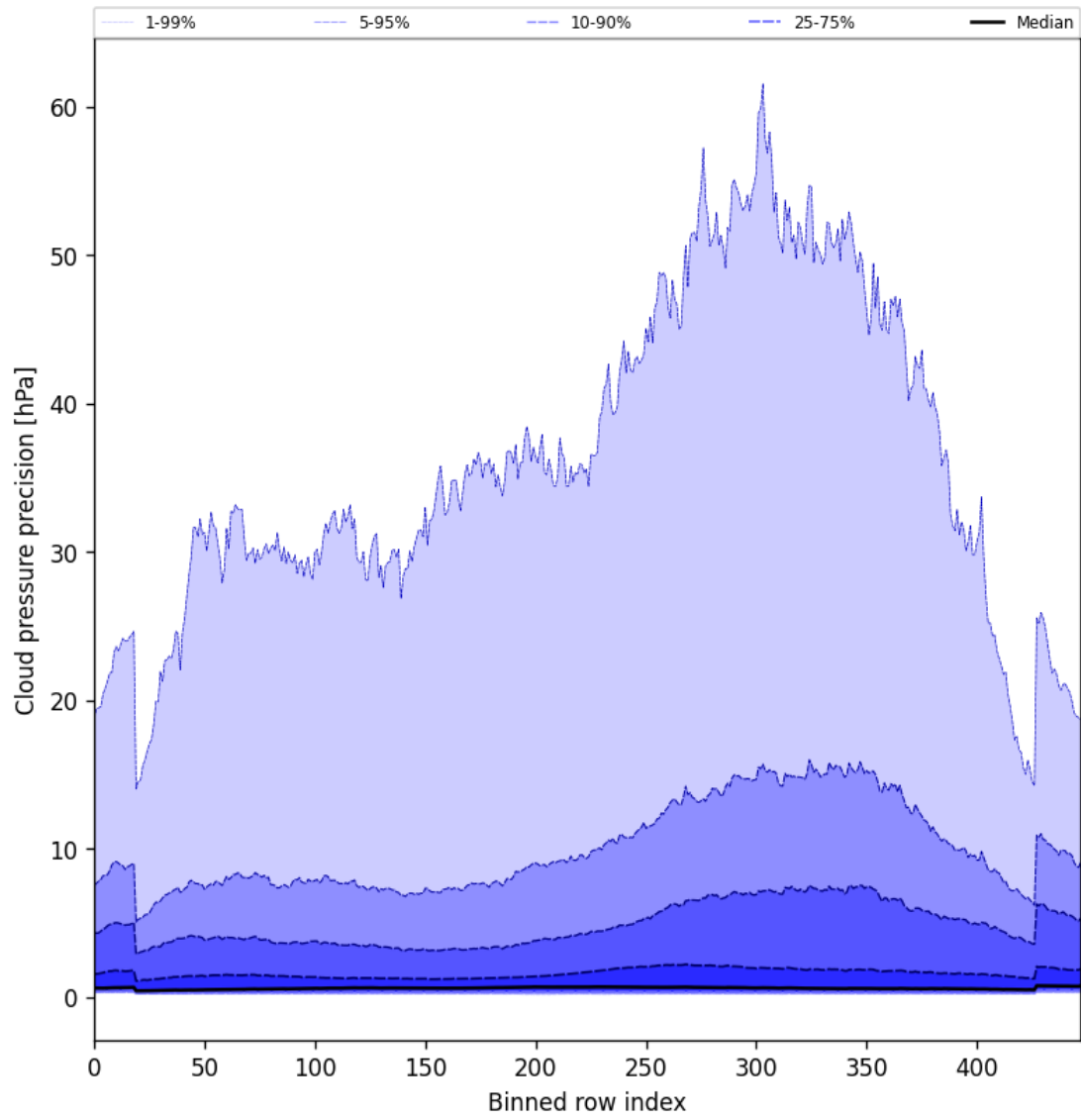
Figure 48: Along track statistics of “Cloud pressure precision” for 2025-03-26 to 2025-03-28
