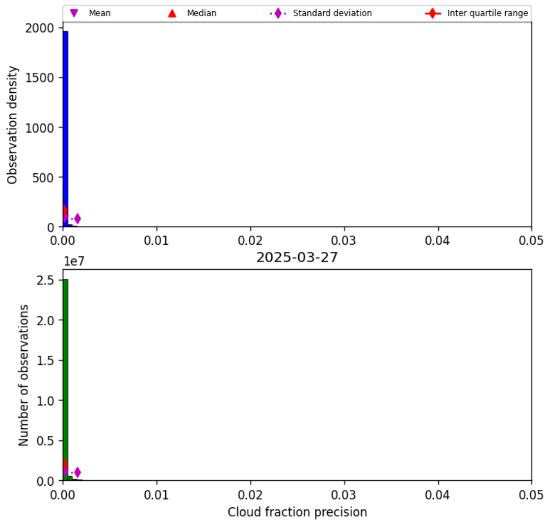
Figure 33: Histogram of “Cloud fraction precision” for 2025-03-26 to 2025-03-28
