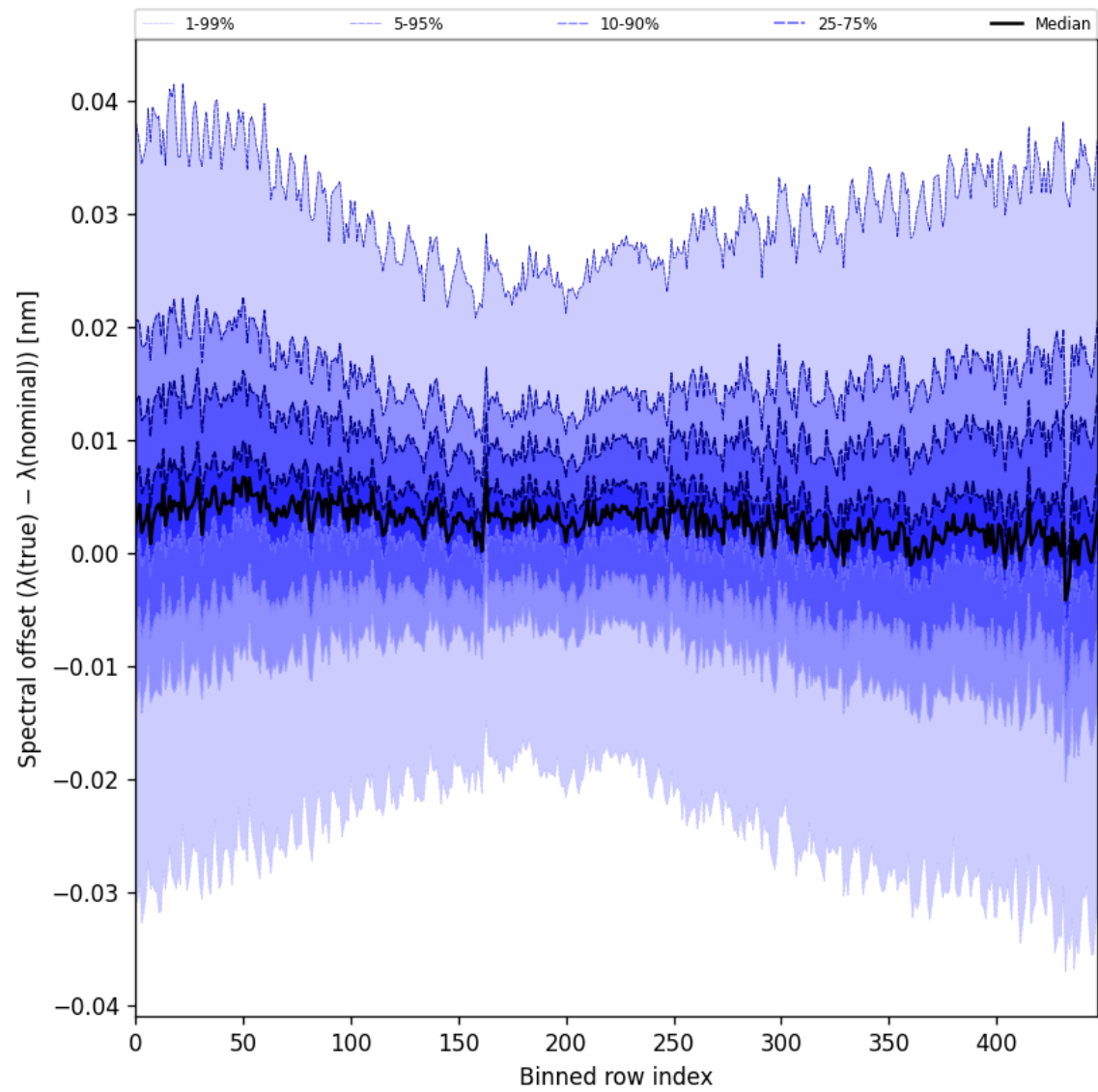
Figure 62: Along track statistics of “Spectral offset ( \lambda_{\text{true}} - \lambda_{\text{nominal}} )” for 2025-03-26 to 2025-03-28
