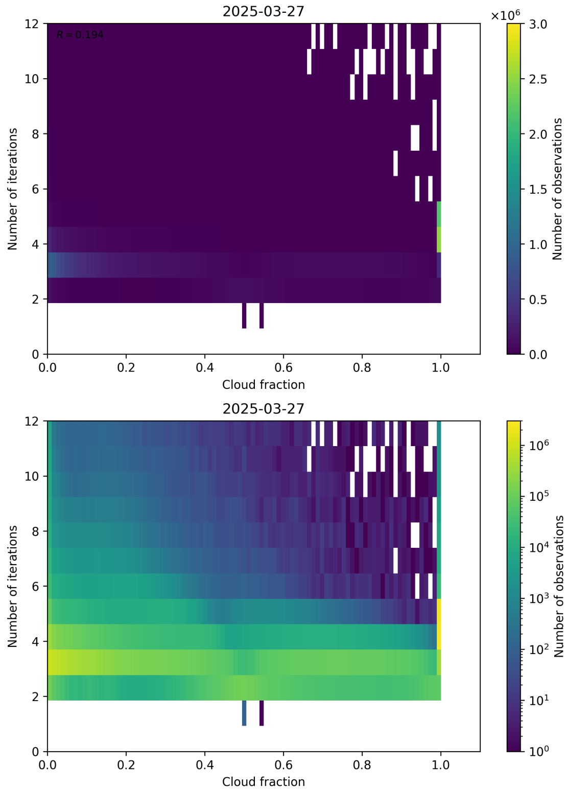
Figure 73: Scatter density plot of “Cloud fraction” against “Number of iterations” for 2025-03-26 to 2025-03-28.
