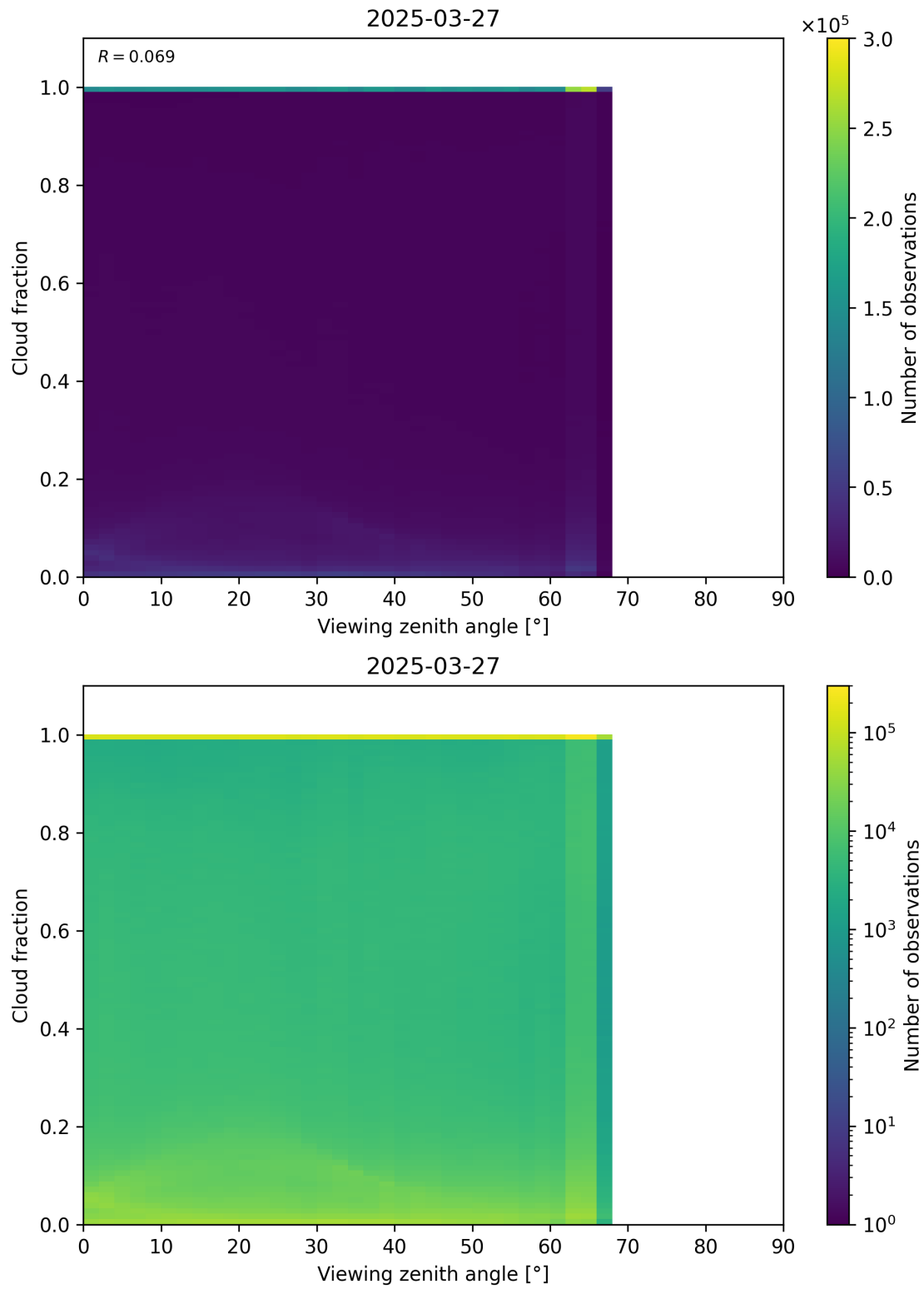
Figure 120: Scatter density plot of “Viewing zenith angle” against “Cloud fraction” for 2025-03-26 to 2025-03-28.
