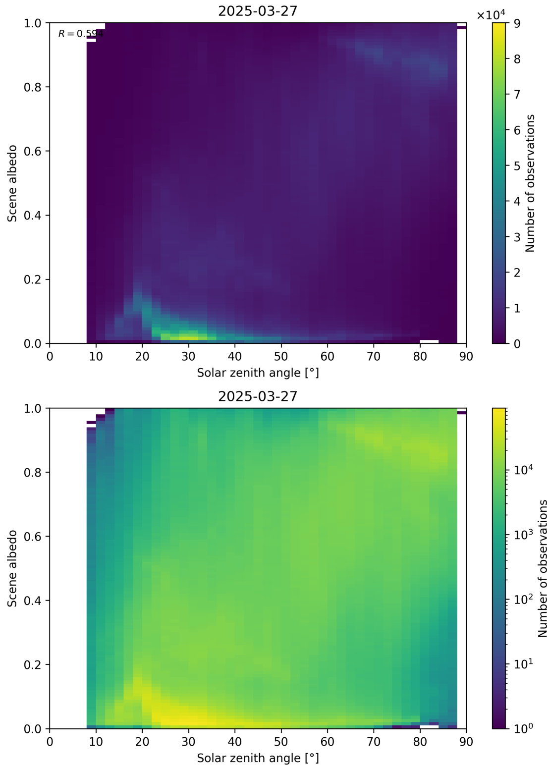
Figure 116: Scatter density plot of “Solar zenith angle” against “Scene albedo” for 2025-03-26 to 2025-03-28.
