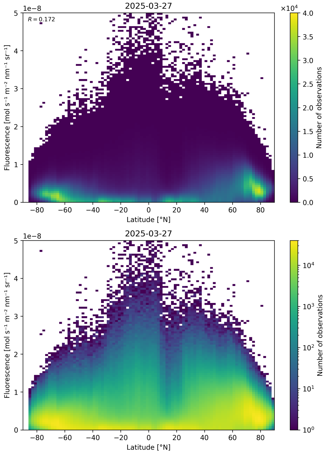
Figure 92: Scatter density plot of “Latitude” against “Fluorescence” for 2025-03-26 to 2025-03-28.
