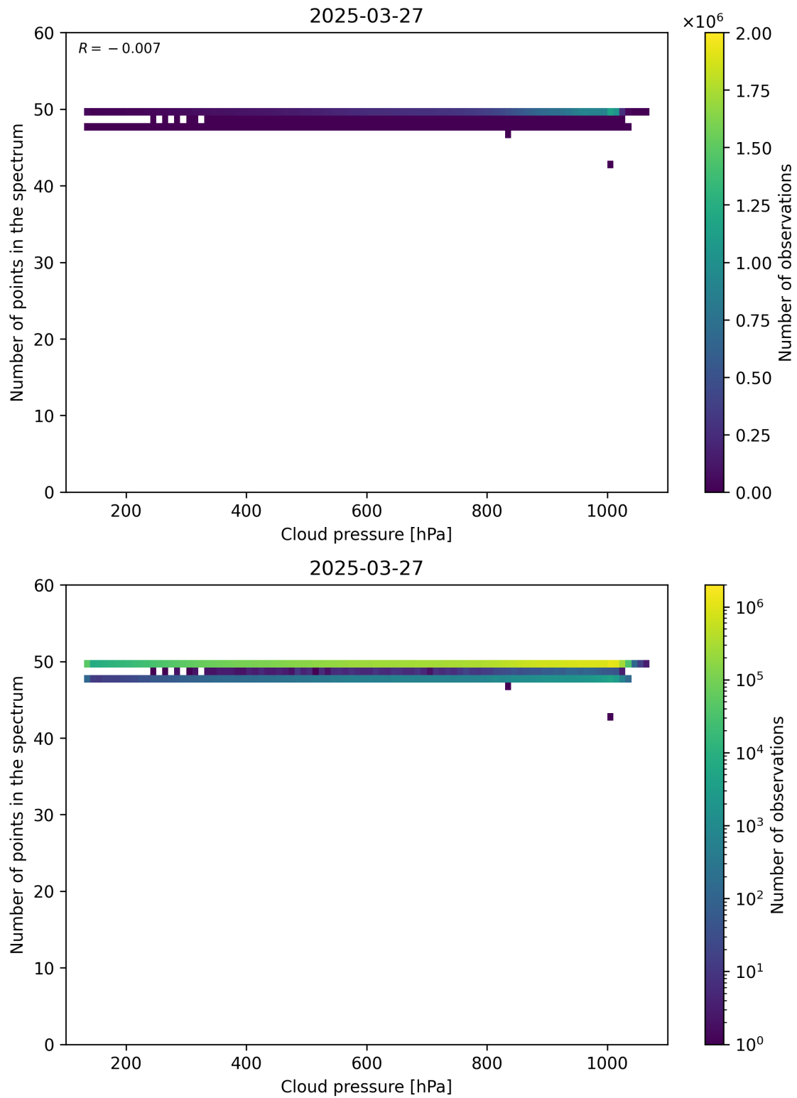
Figure 82: Scatter density plot of “Cloud pressure” against “Number of points in the spectrum” for 2025-03-26 to 2025-03-28.
