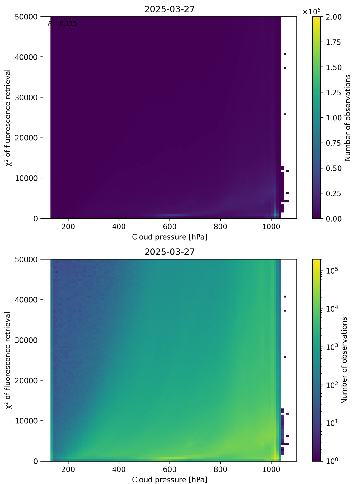
Figure 78: Scatter density plot of “Cloud pressure” against “ \chi^2 of fluorescence retrieval” for 2025-03-26 to 2025-03-28.
