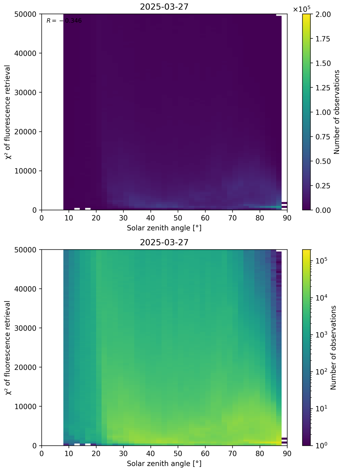
Figure 109: Scatter density plot of “Solar zenith angle” against “ \chi^2 of fluorescence retrieval” for 2025-03-26 to 2025-03-28.
