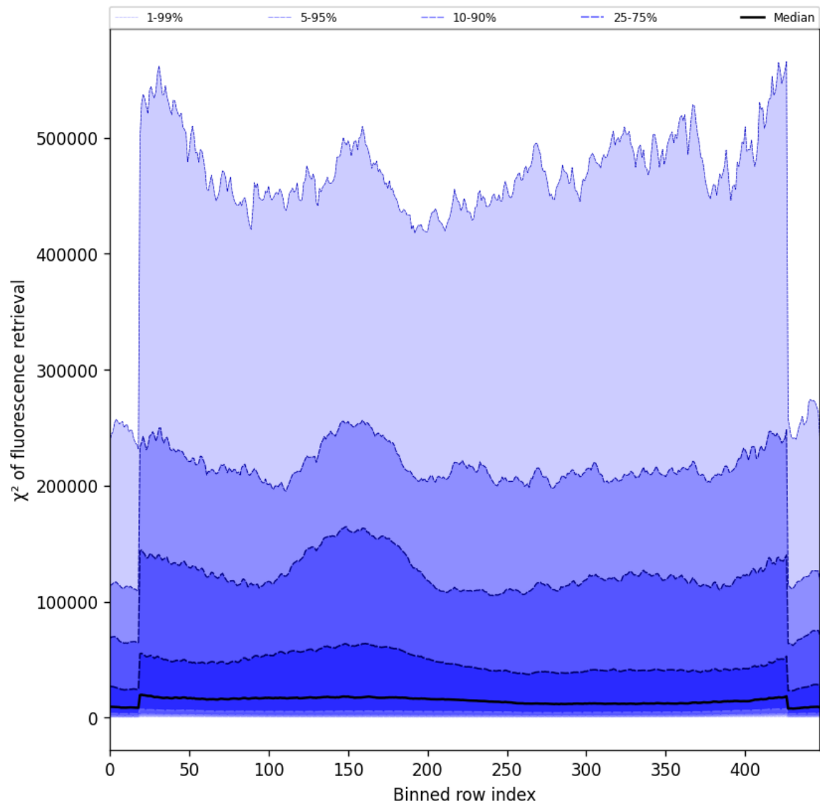
Figure 59: Along track statistics of “ \chi^2 of fluorescence retrieval” for 2025-03-26 to 2025-03-28
