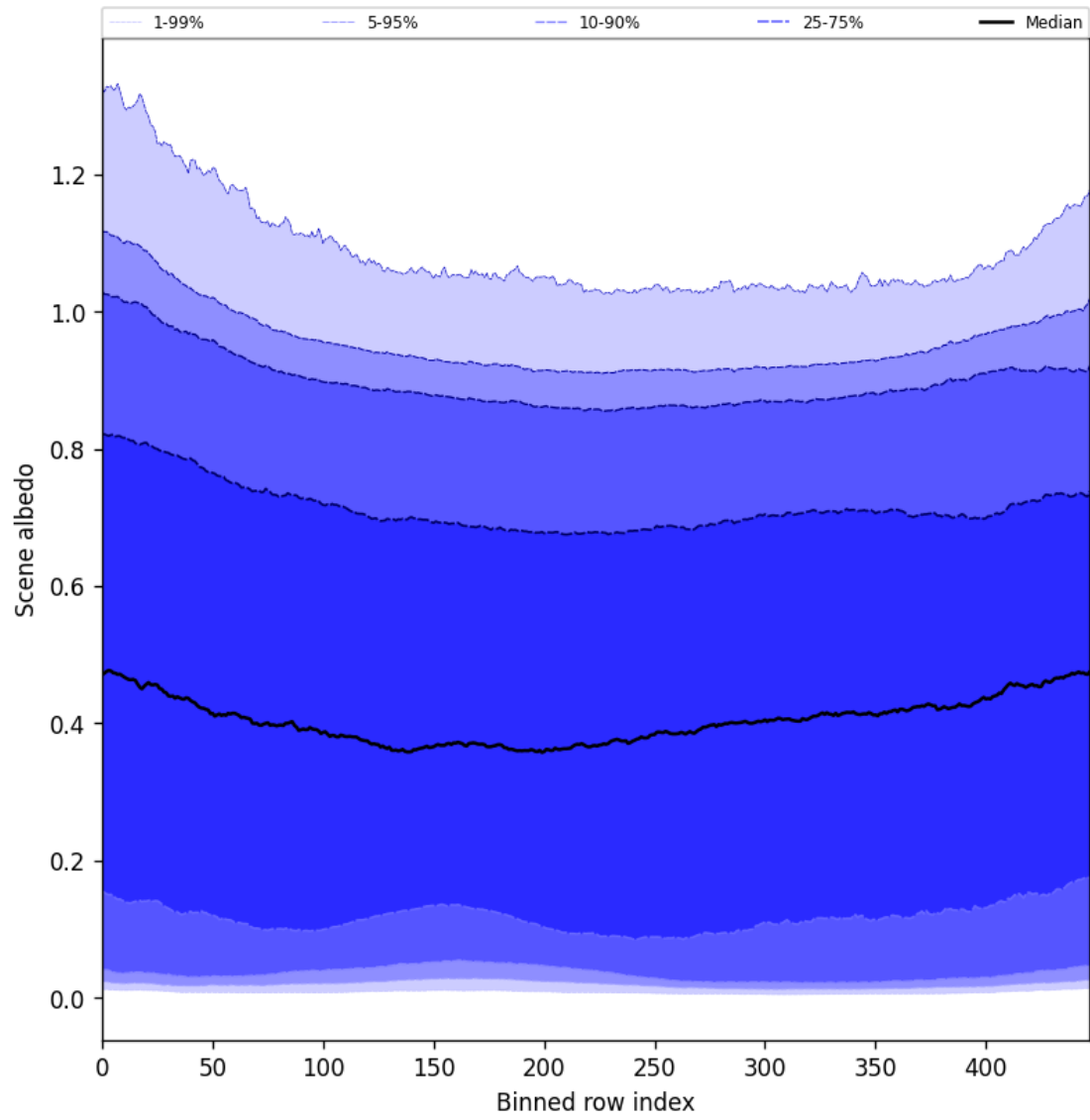
Figure 51: Along track statistics of “Scene albedo” for 2025-03-26 to 2025-03-28
