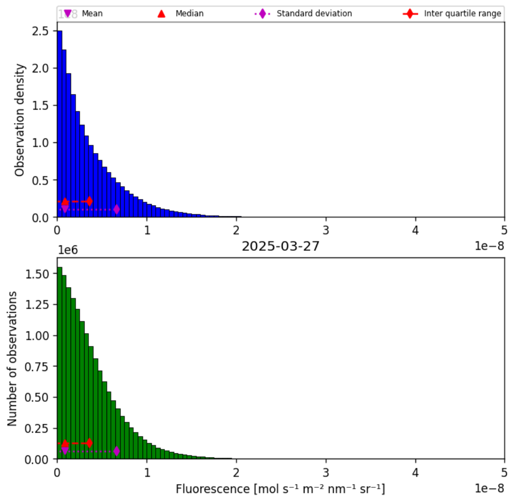
Figure 40: Histogram of “Fluorescence” for 2025-03-26 to 2025-03-28
