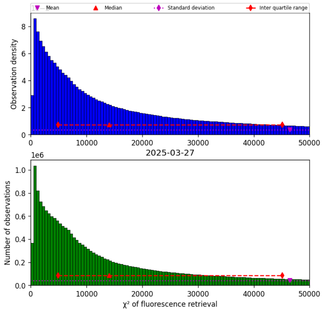
Figure 42: Histogram of “ \chi^2 of fluorescence retrieval” for 2025-03-26 to 2025-03-28
