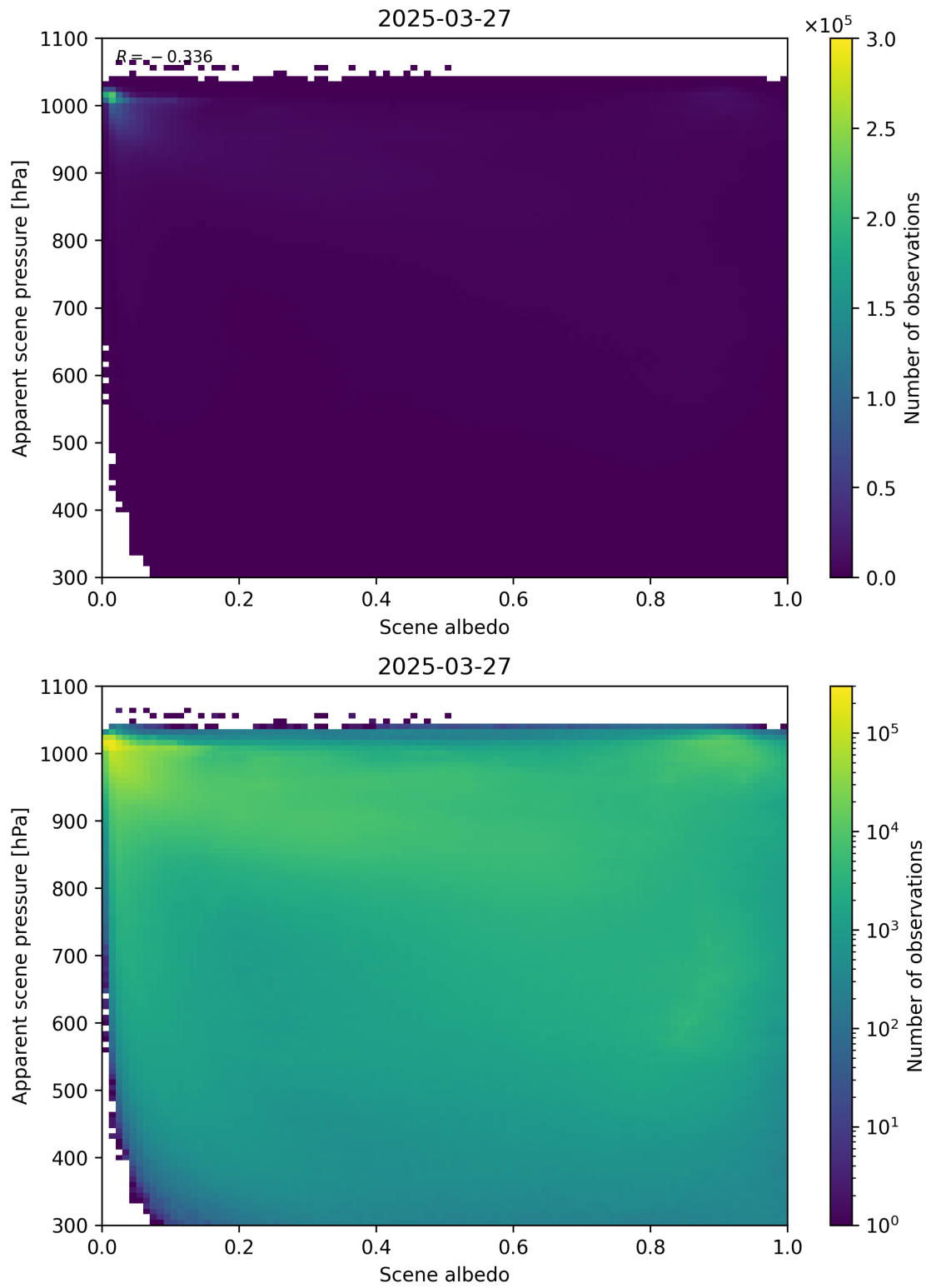
Figure 102: Scatter density plot of “Scene albedo” against “Apparent scene pressure” for 2025-03-26 to 2025-03-28.
