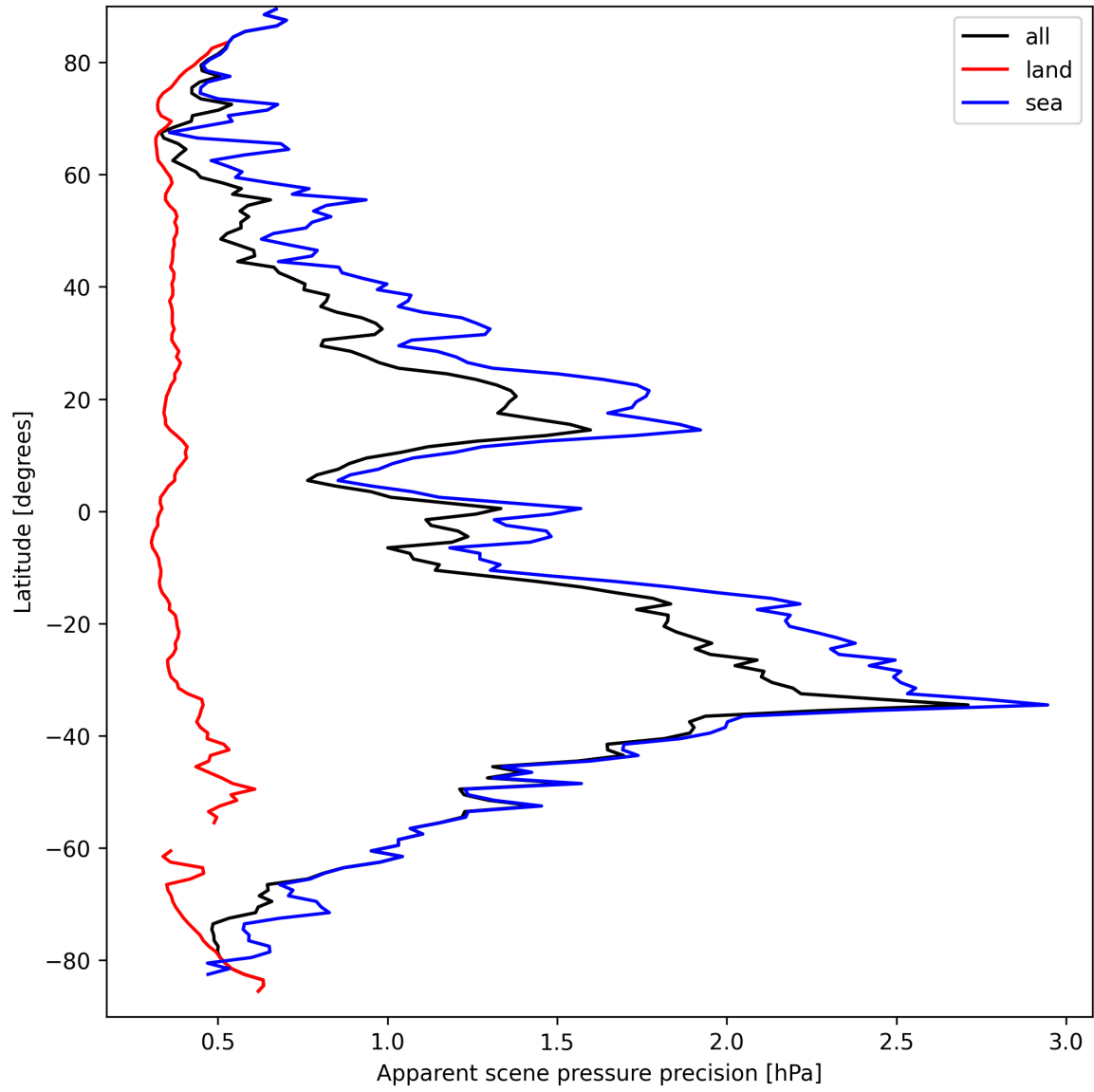
Figure 20: Zonal average of “Apparent scene pressure precision” for 2025-03-26 to 2025-03-28.
