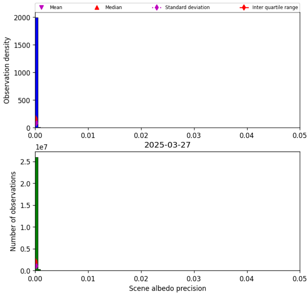
Figure 35: Histogram of “Scene albedo precision” for 2025-03-26 to 2025-03-28
