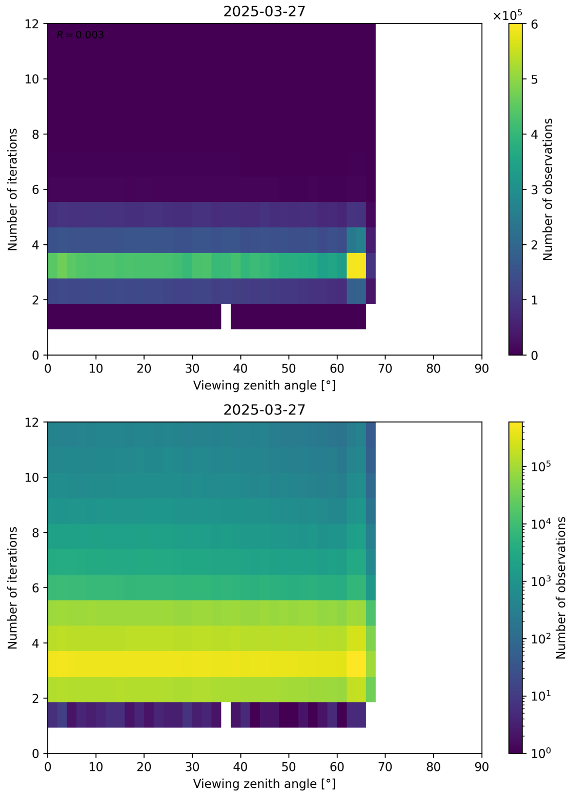
Figure 124: Scatter density plot of “Viewing zenith angle” against “Number of iterations” for 2025-03-26 to 2025-03-28.
