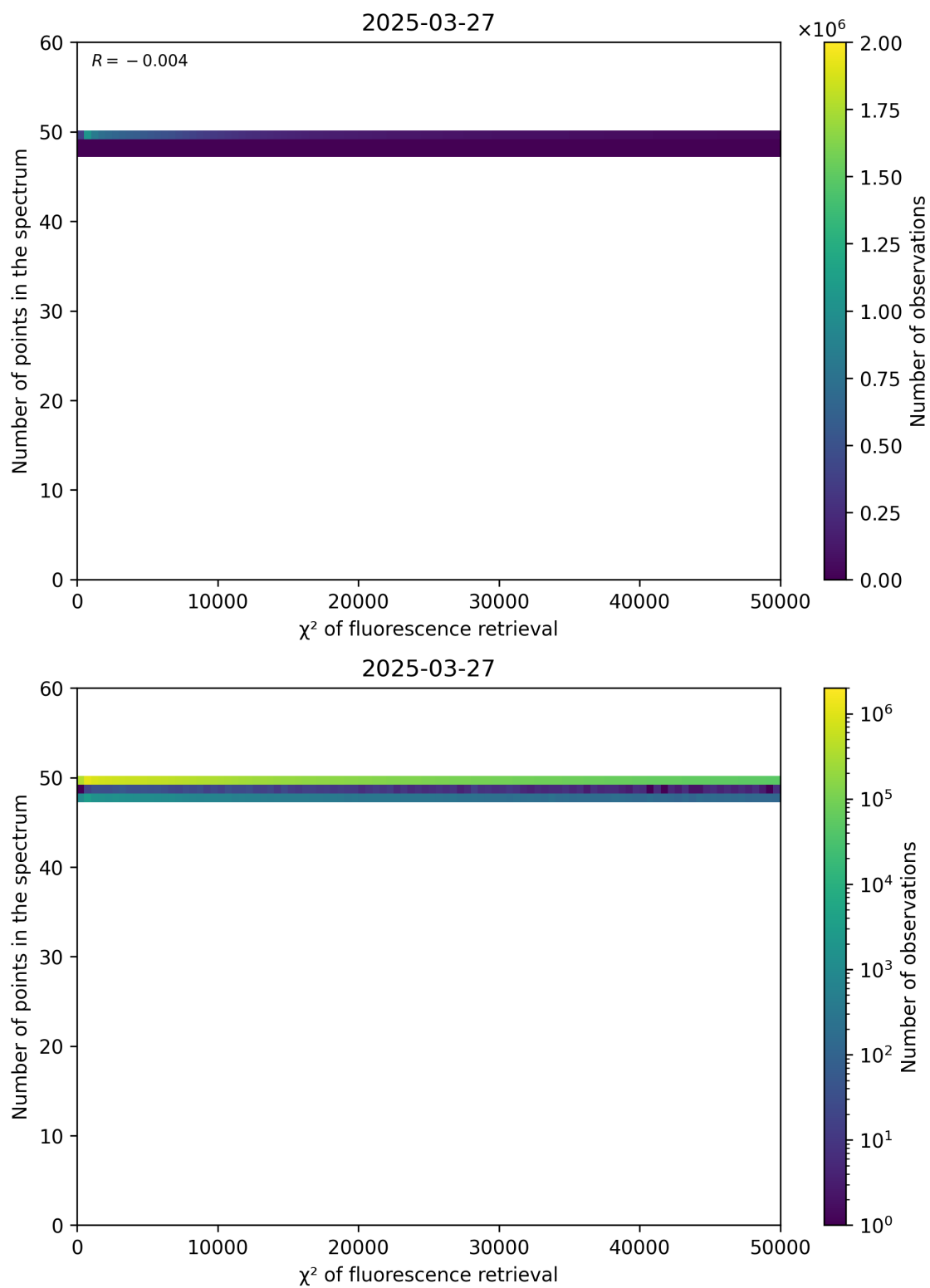
Figure 68: Scatter density plot of " \chi^2 of fluorescence retrieval" against "Number of points in the spectrum" for 2025-03-26 to 2025-03-28.
