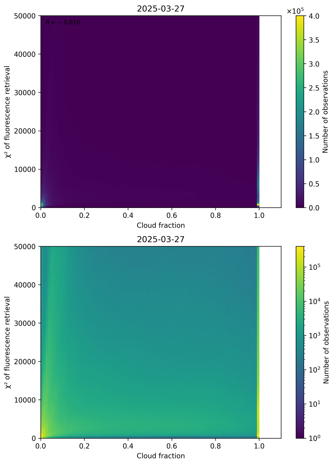
Figure 71: Scatter density plot of “Cloud fraction” against “ \chi^2 of fluorescence retrieval” for 2025-03-26 to 2025-03-28.
