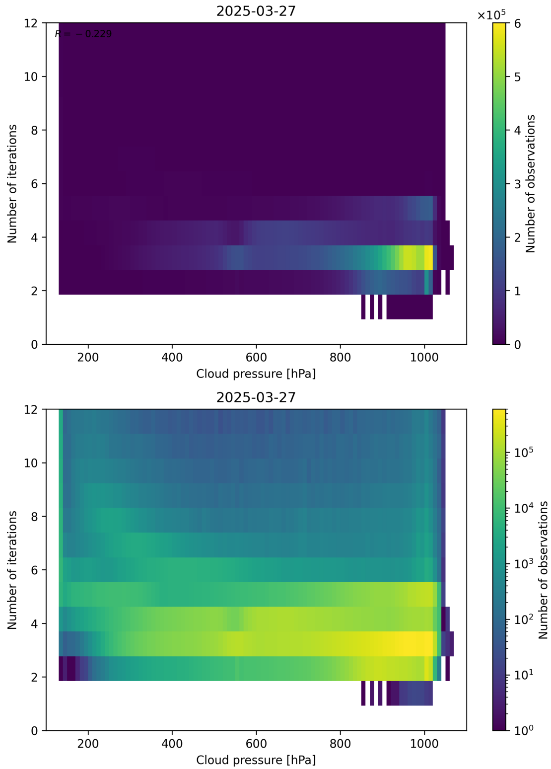
Figure 81: Scatter density plot of “Cloud pressure” against “Number of iterations” for 2025-03-26 to 2025-03-28.
