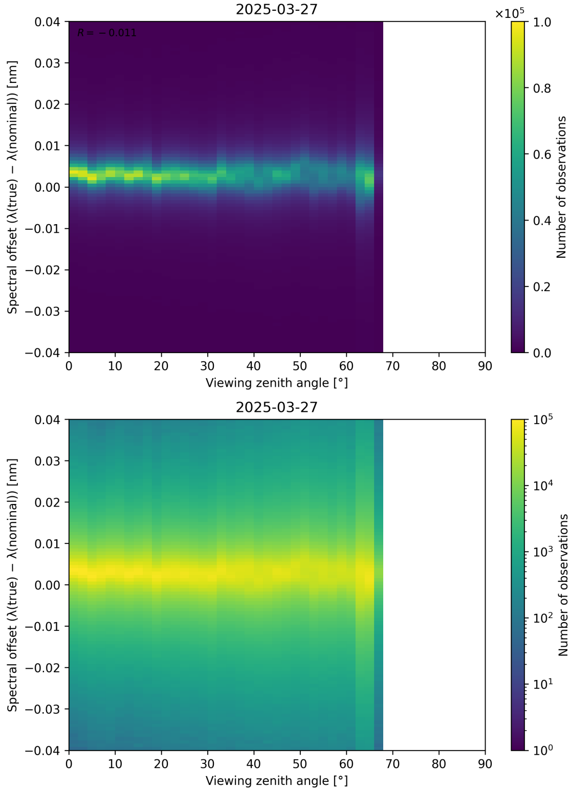
Figure 128: Scatter density plot of “Viewing zenith angle” against “Spectral offset ( \lambda_{\text{true}} - \lambda_{\text{nominal}} )” for 2025-03-26 to 2025-03-28.
