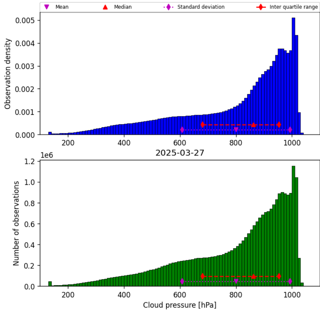
Figure 30: Histogram of “Cloud pressure” for 2025-03-26 to 2025-03-28
