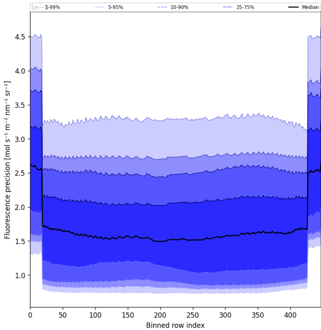
Figure 58: Along track statistics of “Fluorescence precision” for 2025-03-26 to 2025-03-28
