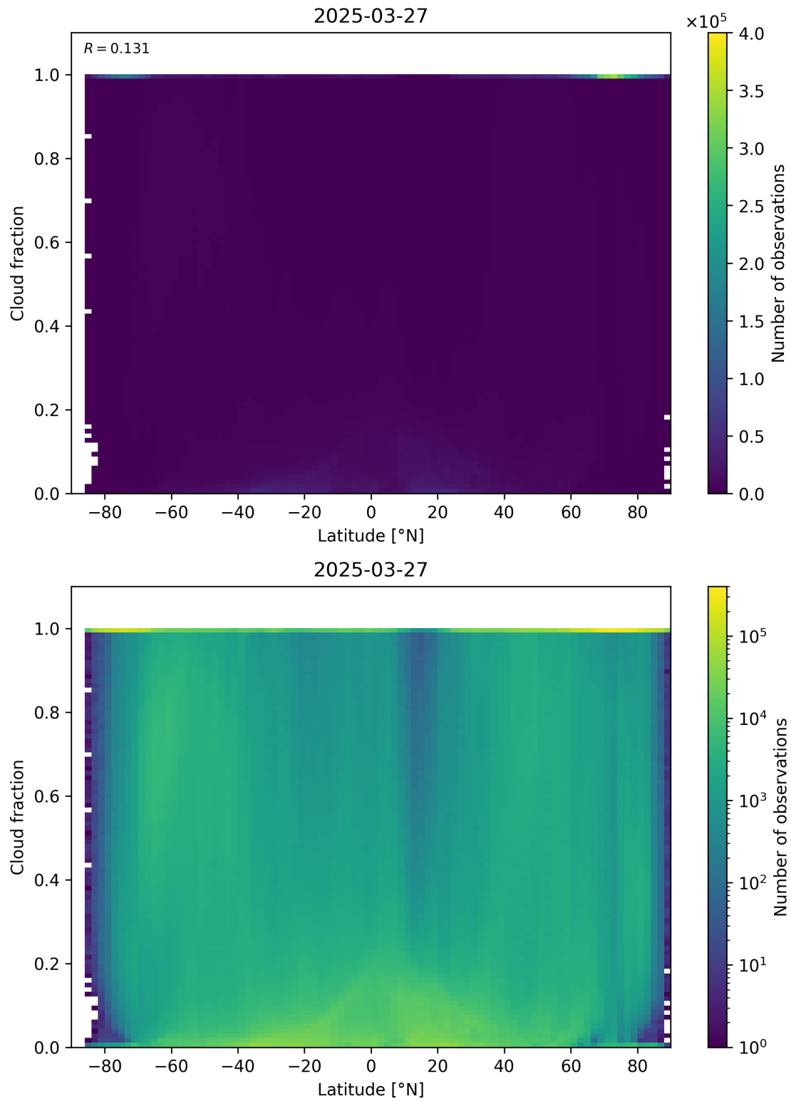
Figure 90: Scatter density plot of “Latitude” against “Cloud fraction” for 2025-03-26 to 2025-03-28.
