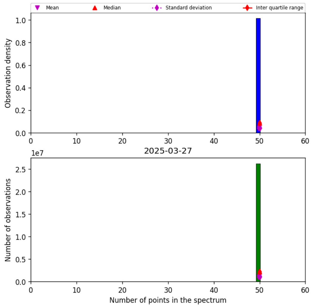
Figure 44: Histogram of "Number of points in the spectrum" for 2025-03-26 to 2025-03-28
