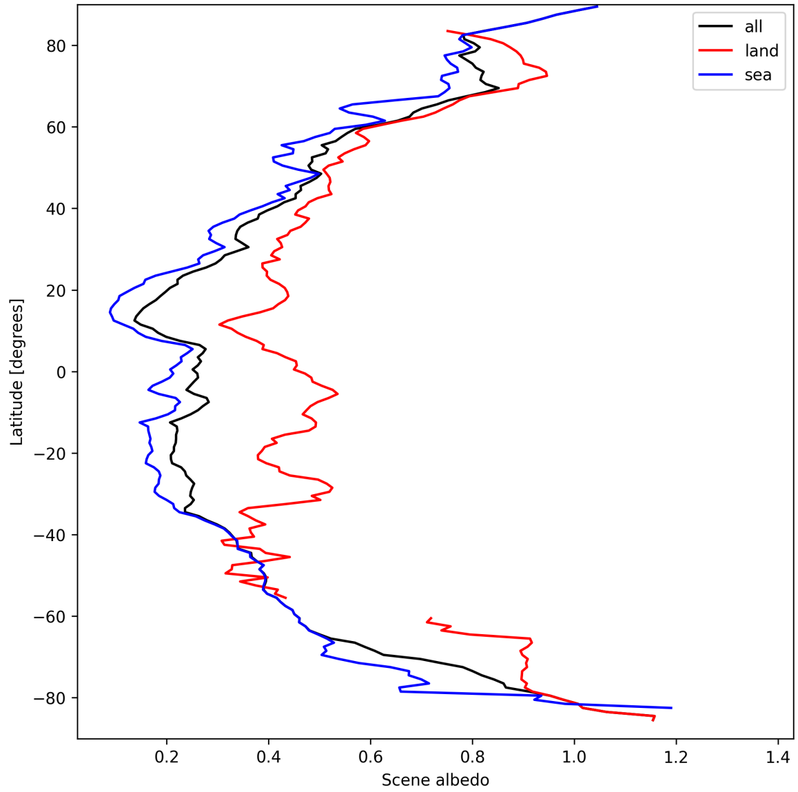
Figure 17: Zonal average of “Scene albedo” for 2025-03-26 to 2025-03-28.
