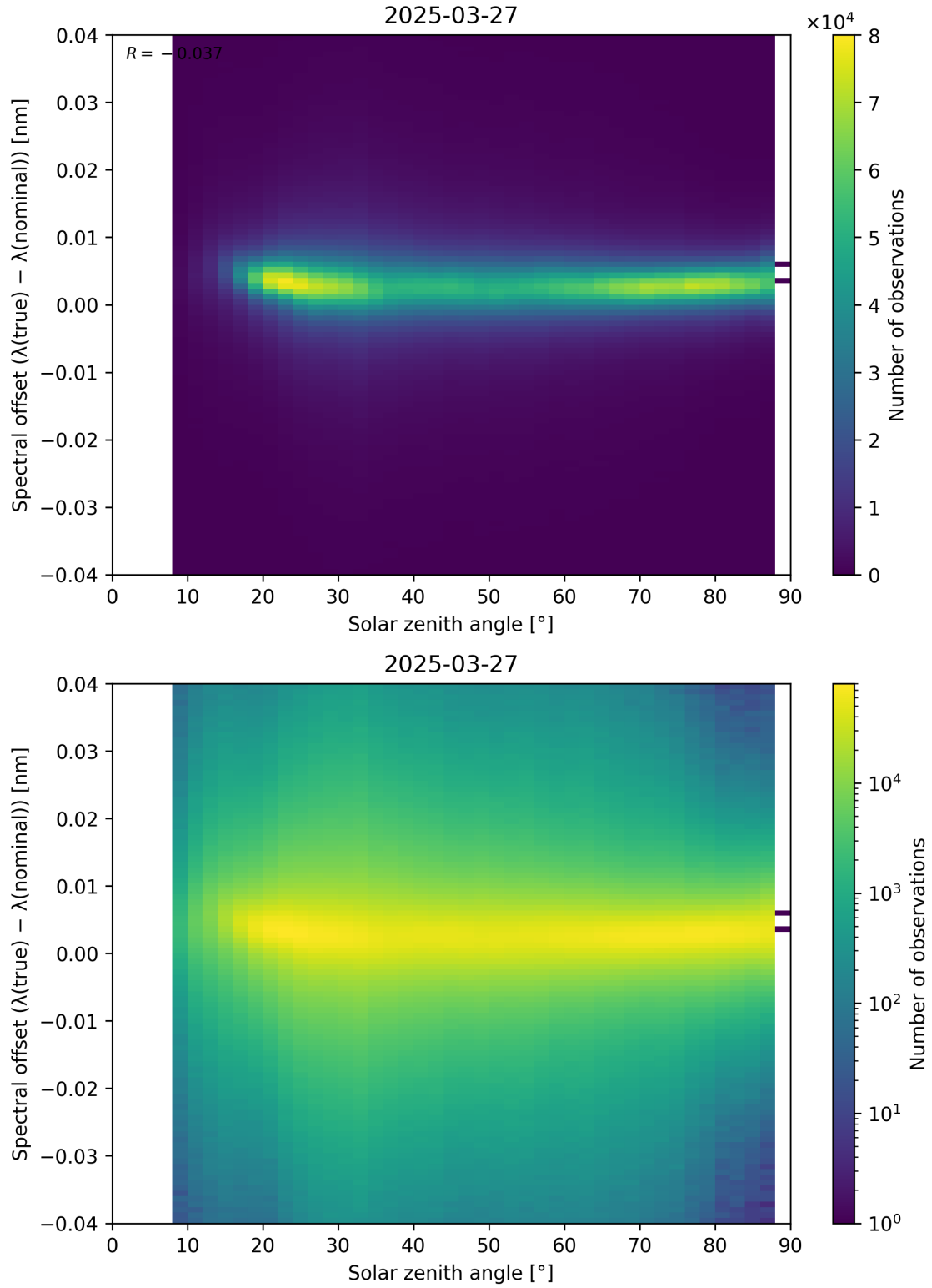
Figure 117: Scatter density plot of “Solar zenith angle” against “Spectral offset ( \lambda_{\text{true}} - \lambda_{\text{nominal}} )” for 2025-03-26 to 2025-03-28.
