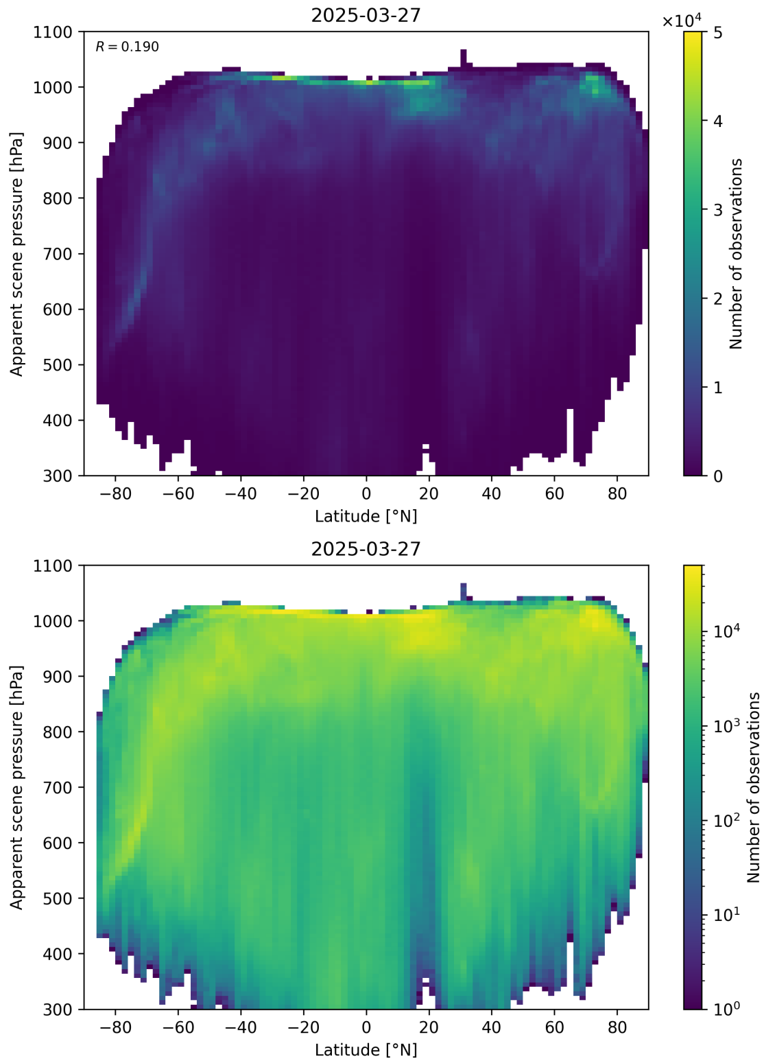
Figure 88: Scatter density plot of “Latitude” against “Apparent scene pressure” for 2025-03-26 to 2025-03-28.
