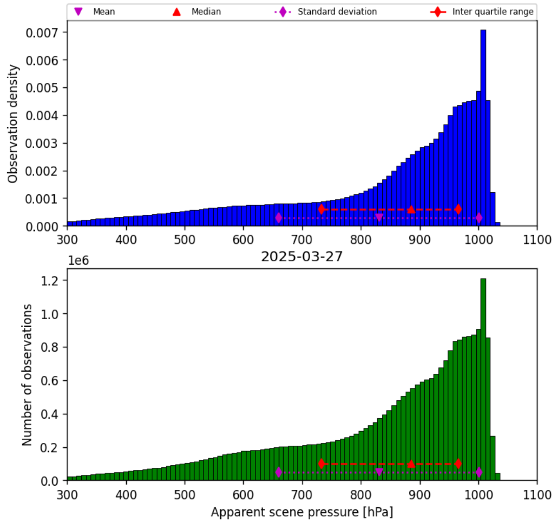
Figure 36: Histogram of “Apparent scene pressure” for 2025-03-26 to 2025-03-28
