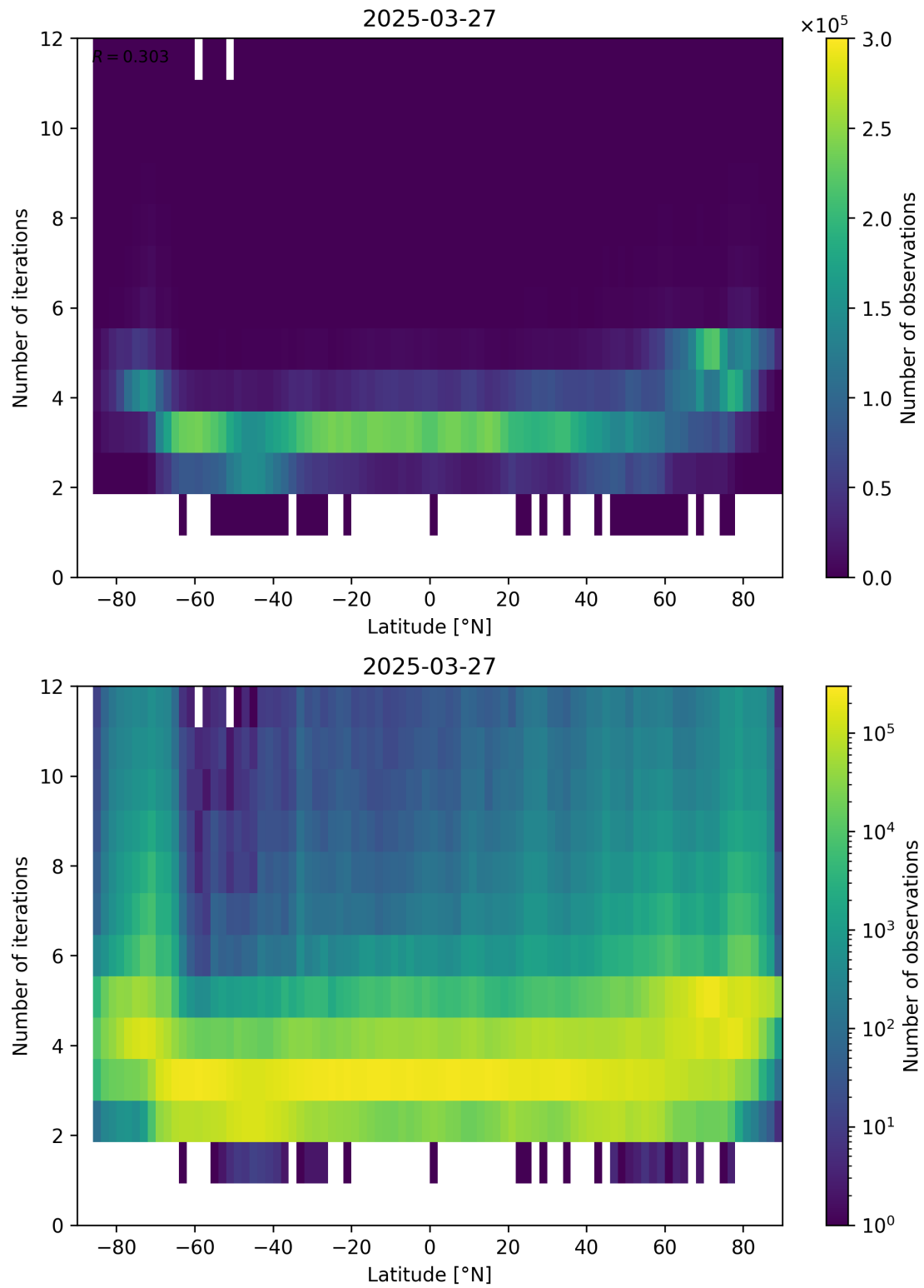
Figure 93: Scatter density plot of “Latitude” against “Number of iterations” for 2025-03-26 to 2025-03-28.
