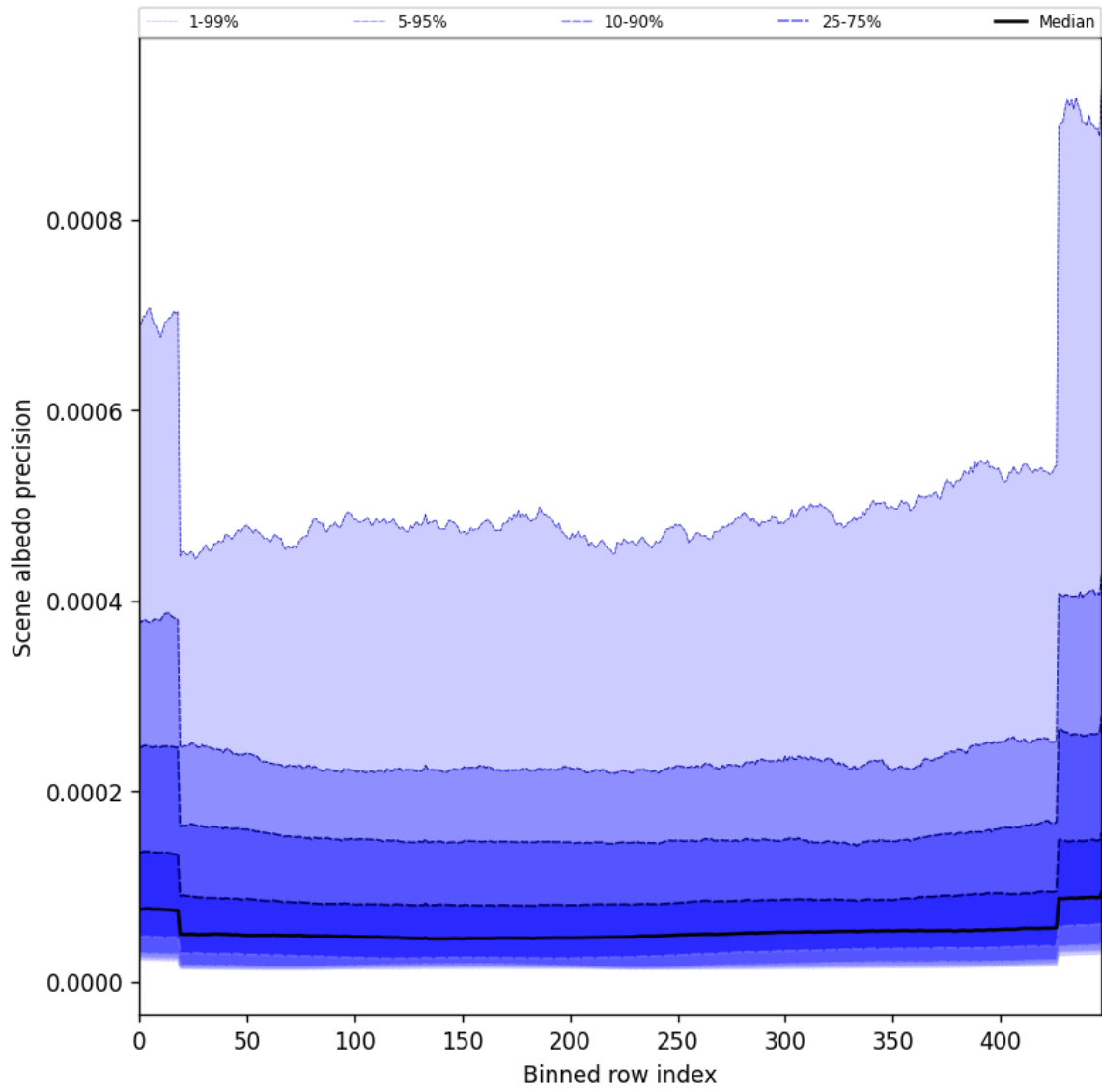
Figure 52: Along track statistics of “Scene albedo precision” for 2025-03-26 to 2025-03-28
