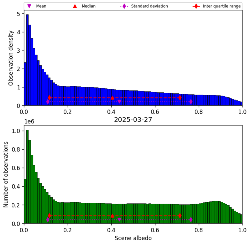
Figure 34: Histogram of “Scene albedo” for 2025-03-26 to 2025-03-28
