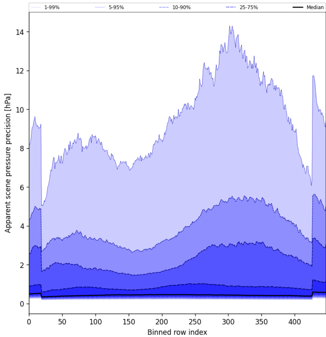
Figure 54: Along track statistics of “Apparent scene pressure precision” for 2025-03-26 to 2025-03-28
