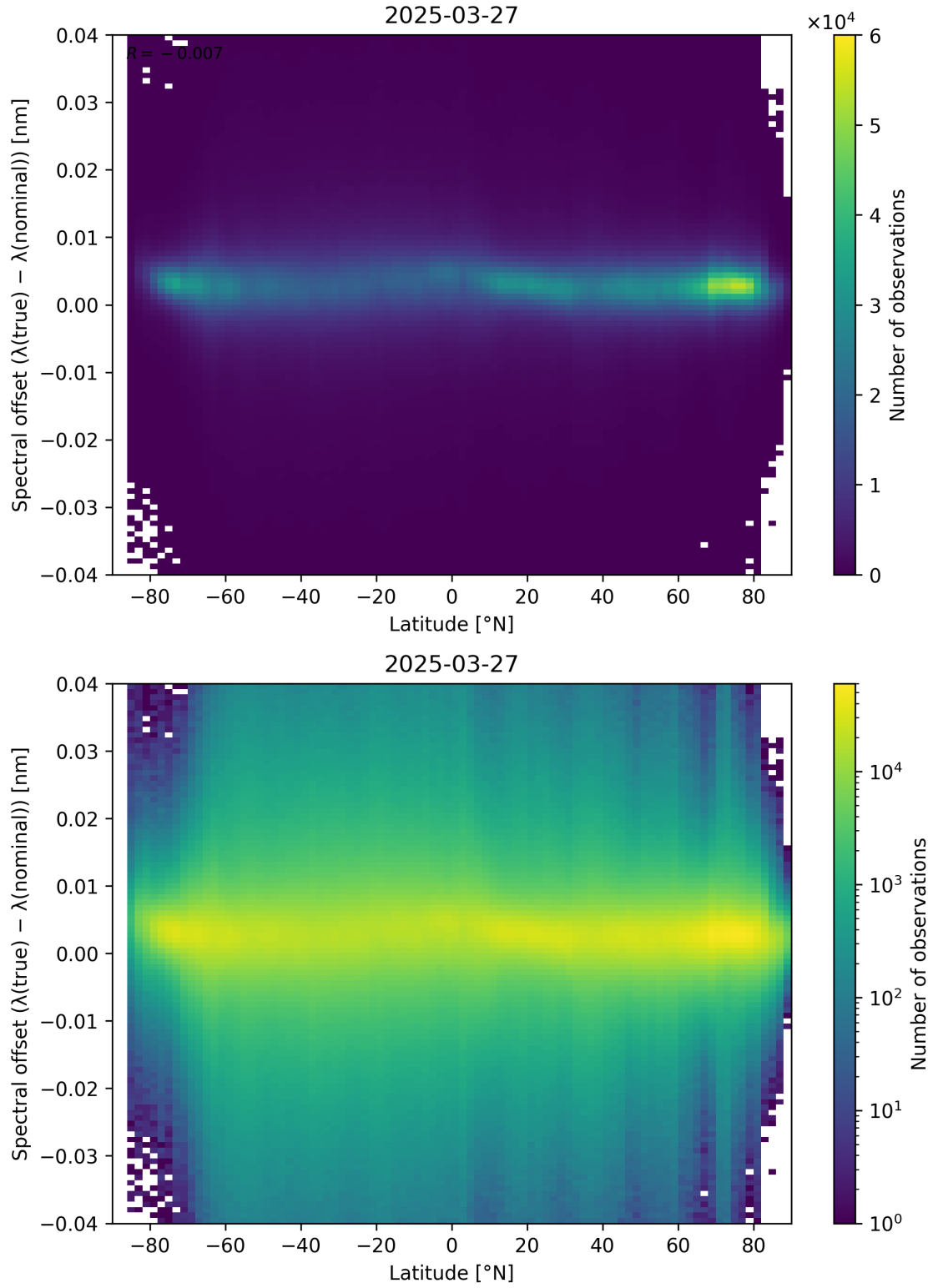
Figure 96: Scatter density plot of “Latitude” against “Spectral offset ( \lambda_{\text{true}} - \lambda_{\text{nominal}} )” for 2025-03-26 to 2025-03-28.
