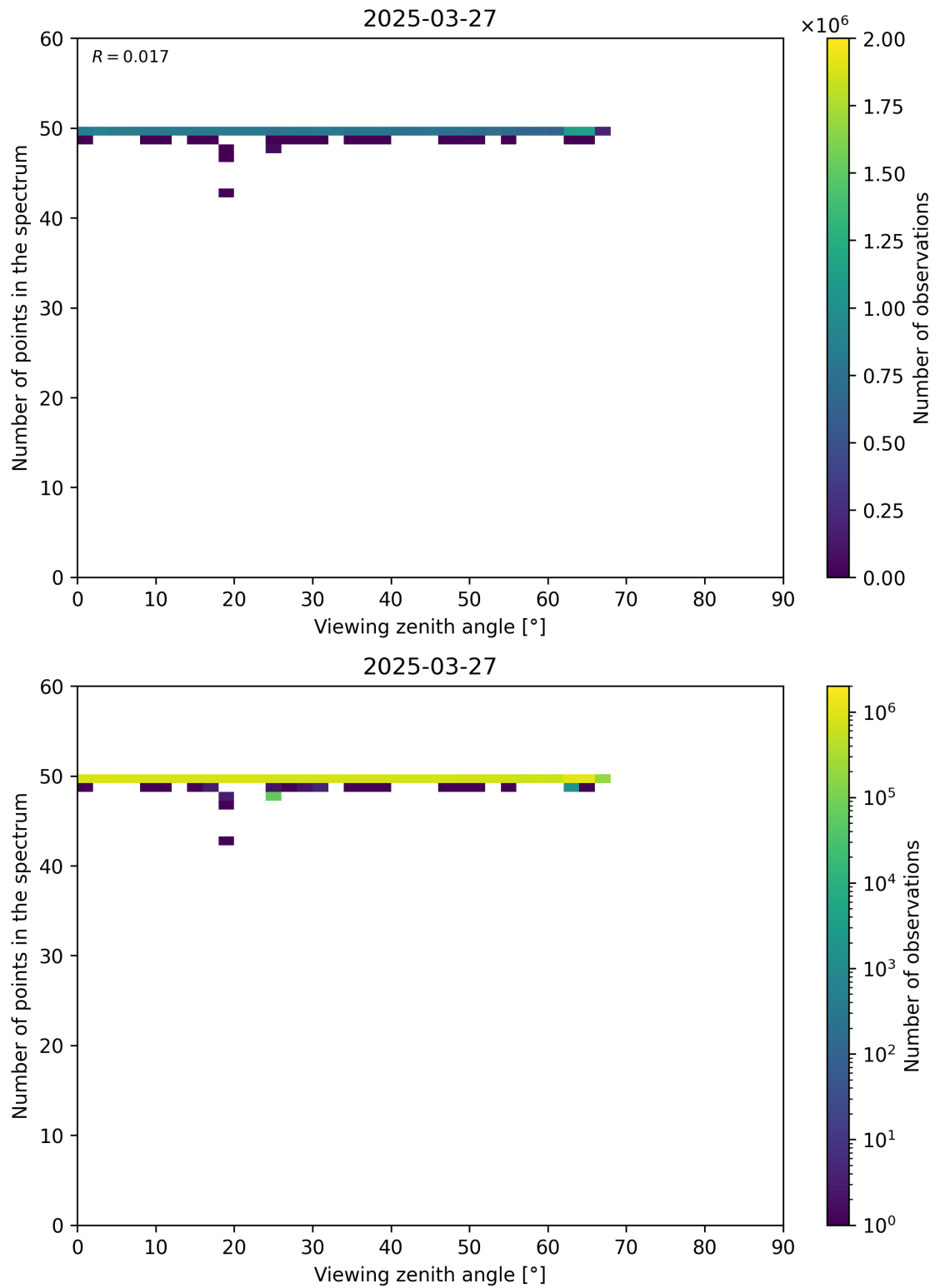
Figure 125: Scatter density plot of “Viewing zenith angle” against “Number of points in the spectrum” for 2025-03-26 to 2025-03-28.
