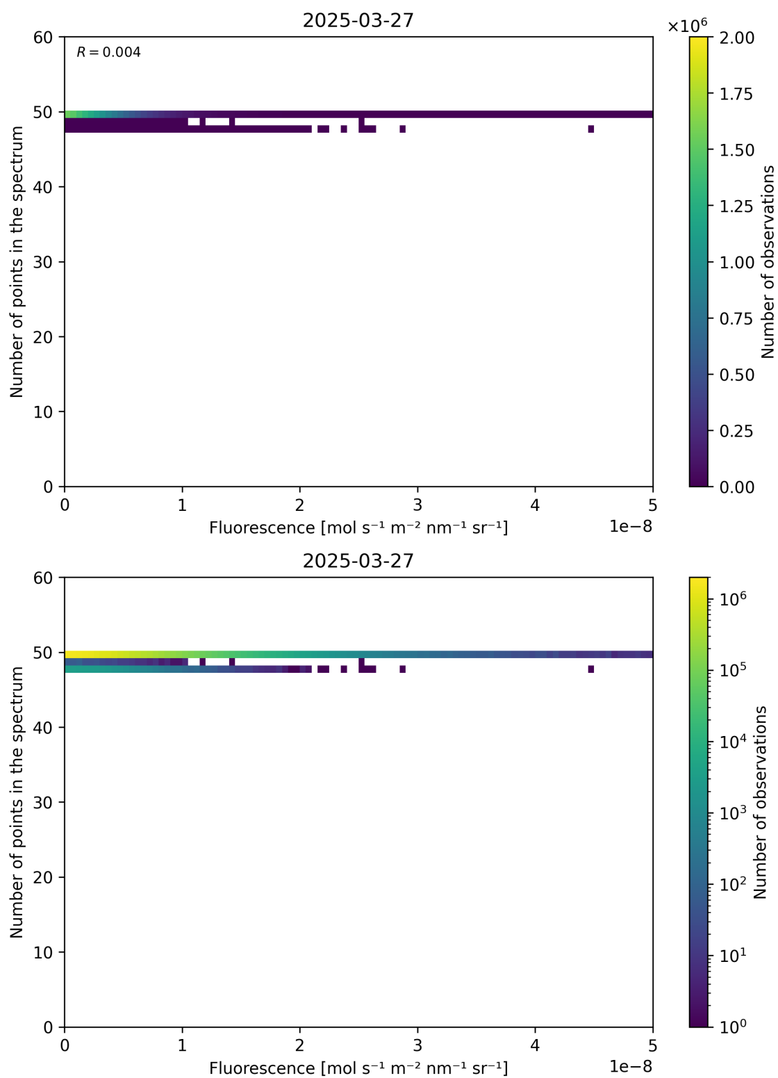
Figure 86: Scatter density plot of “Fluorescence” against “Number of points in the spectrum” for 2025-03-26 to 2025-03-28.
