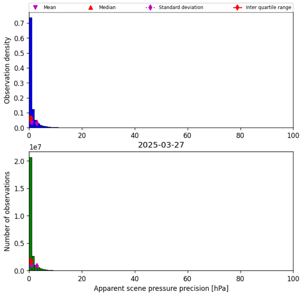
Figure 37: Histogram of “Apparent scene pressure precision” for 2025-03-26 to 2025-03-28
