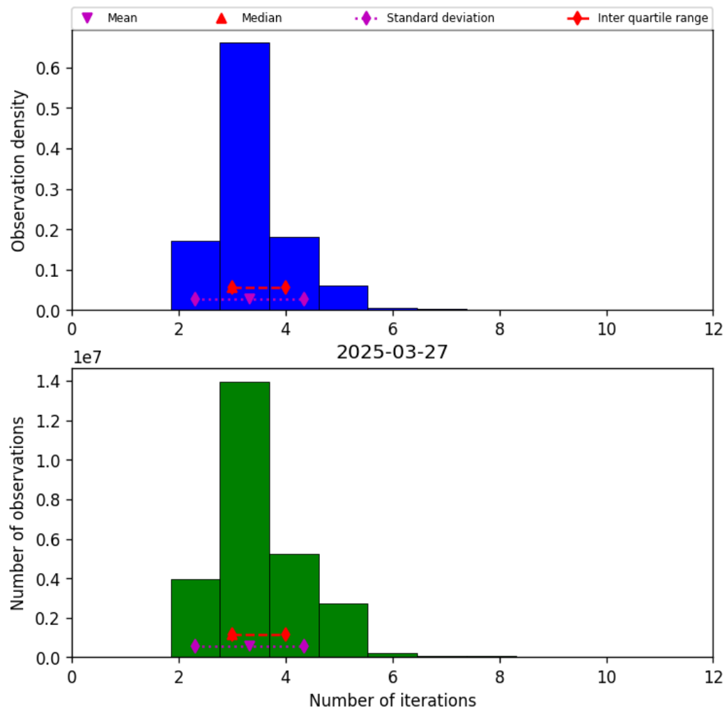
Figure 39: Histogram of “Number of iterations” for 2025-03-26 to 2025-03-28
