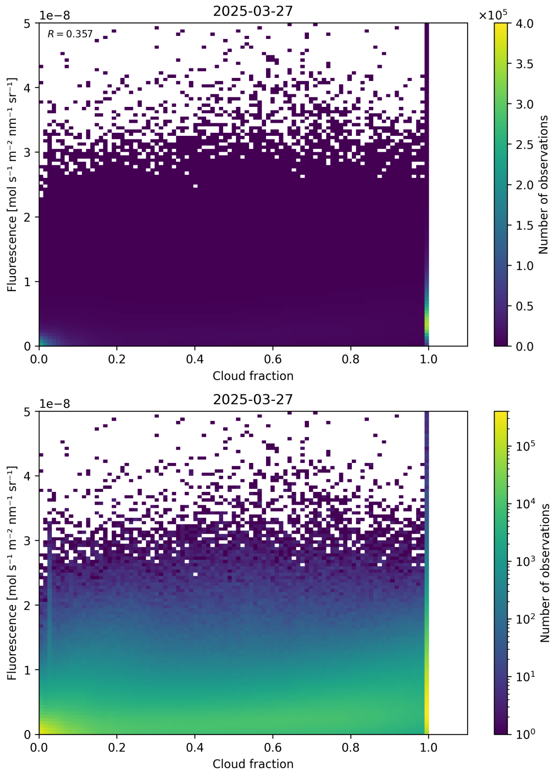
Figure 72: Scatter density plot of “Cloud fraction” against “Fluorescence” for 2025-03-26 to 2025-03-28.
