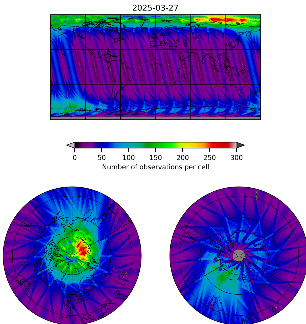
Figure 11: Map of the number of observations for 2025-03-26 to 2025-03-28
