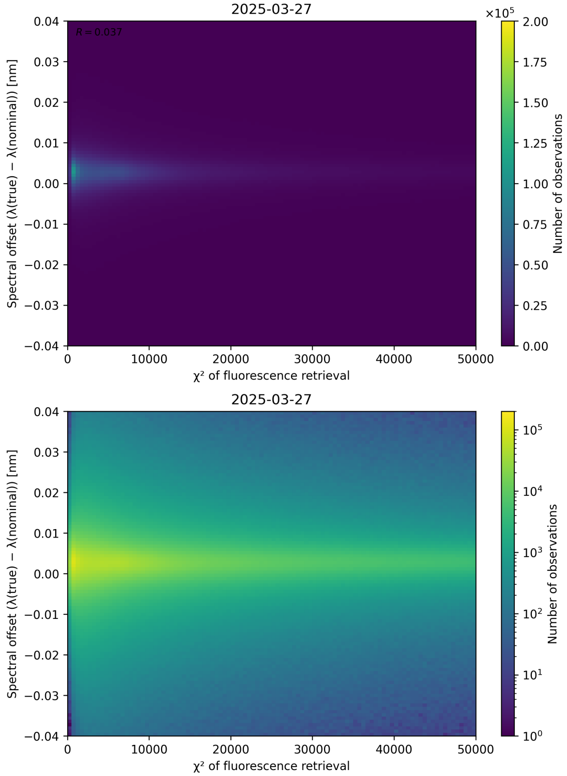
Figure 69: Scatter density plot of “ \chi^2 of fluorescence retrieval” against “Spectral offset ( \lambda_{\text{true}} - \lambda_{\text{nominal}} )” for 2025-03-26 to 2025-03-28.
