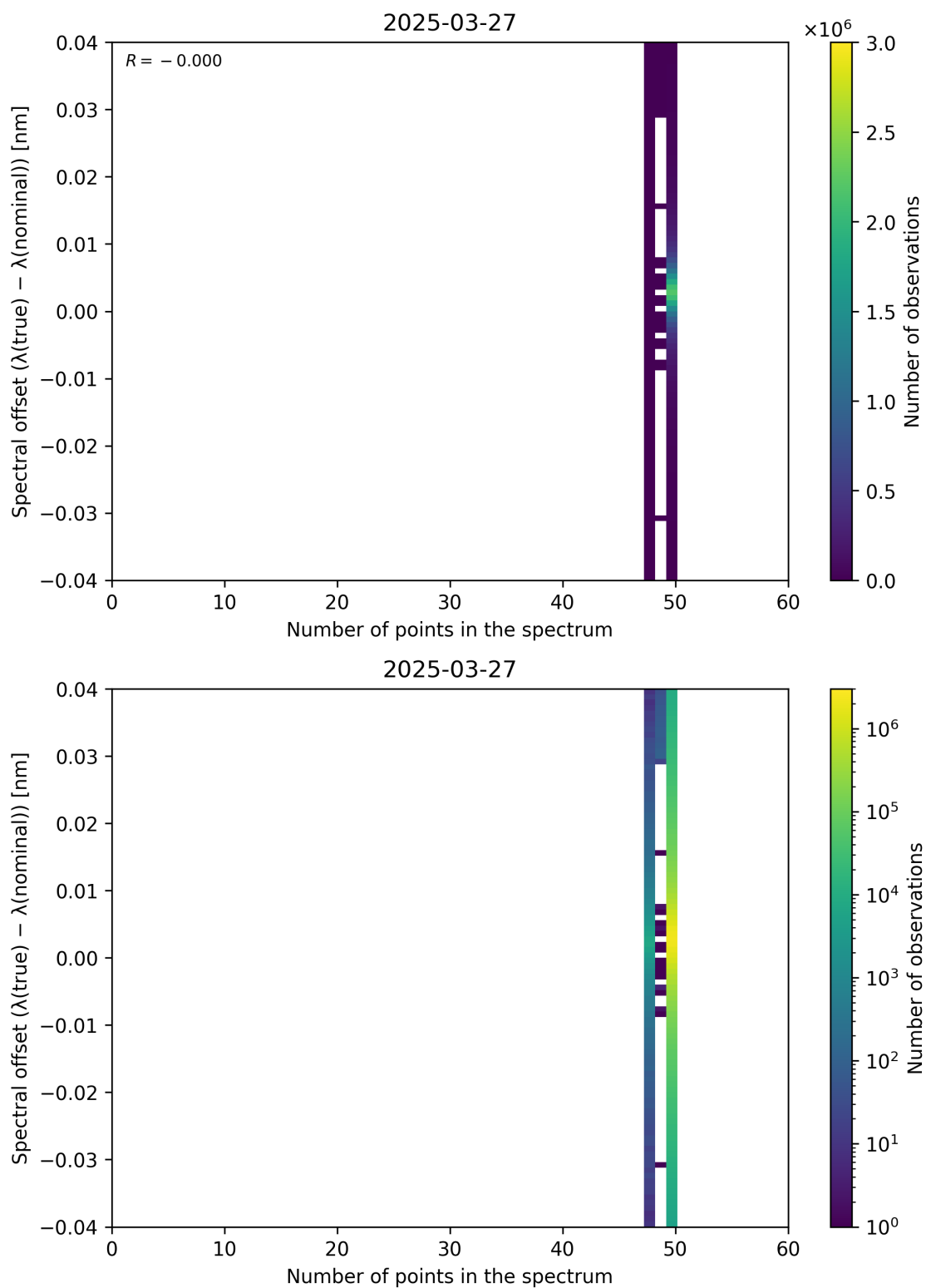
Figure 101: Scatter density plot of “Number of points in the spectrum” against “Spectral offset ( \lambda_{\text{true}} - \lambda_{\text{nominal}} )” for 2025-03-26 to 2025-03-28.
