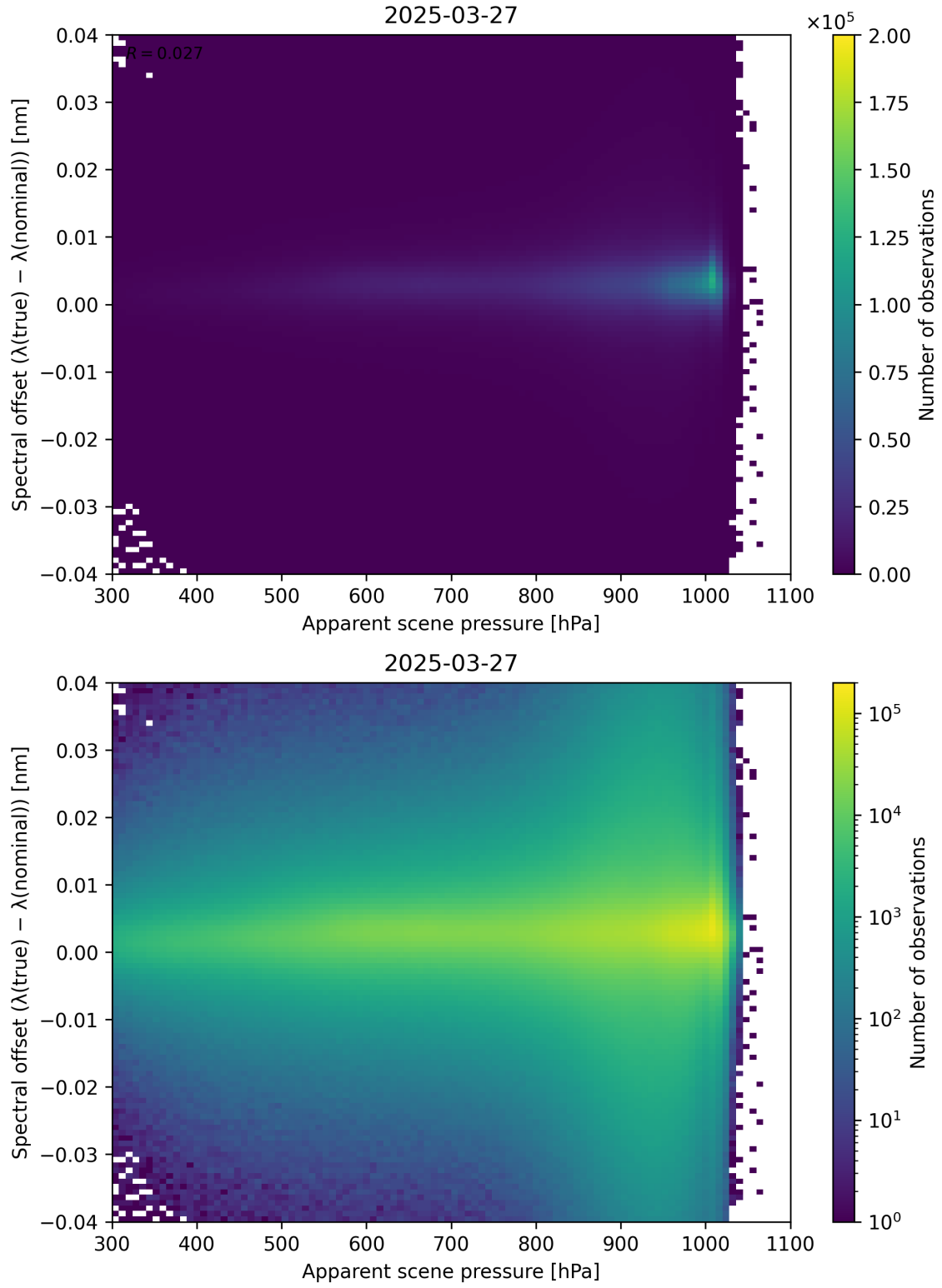
Figure 67: Scatter density plot of “Apparent scene pressure” against “Spectral offset ( \lambda_{\text{true}} - \lambda_{\text{nominal}} )” for 2025-03-26 to 2025-03-28.
