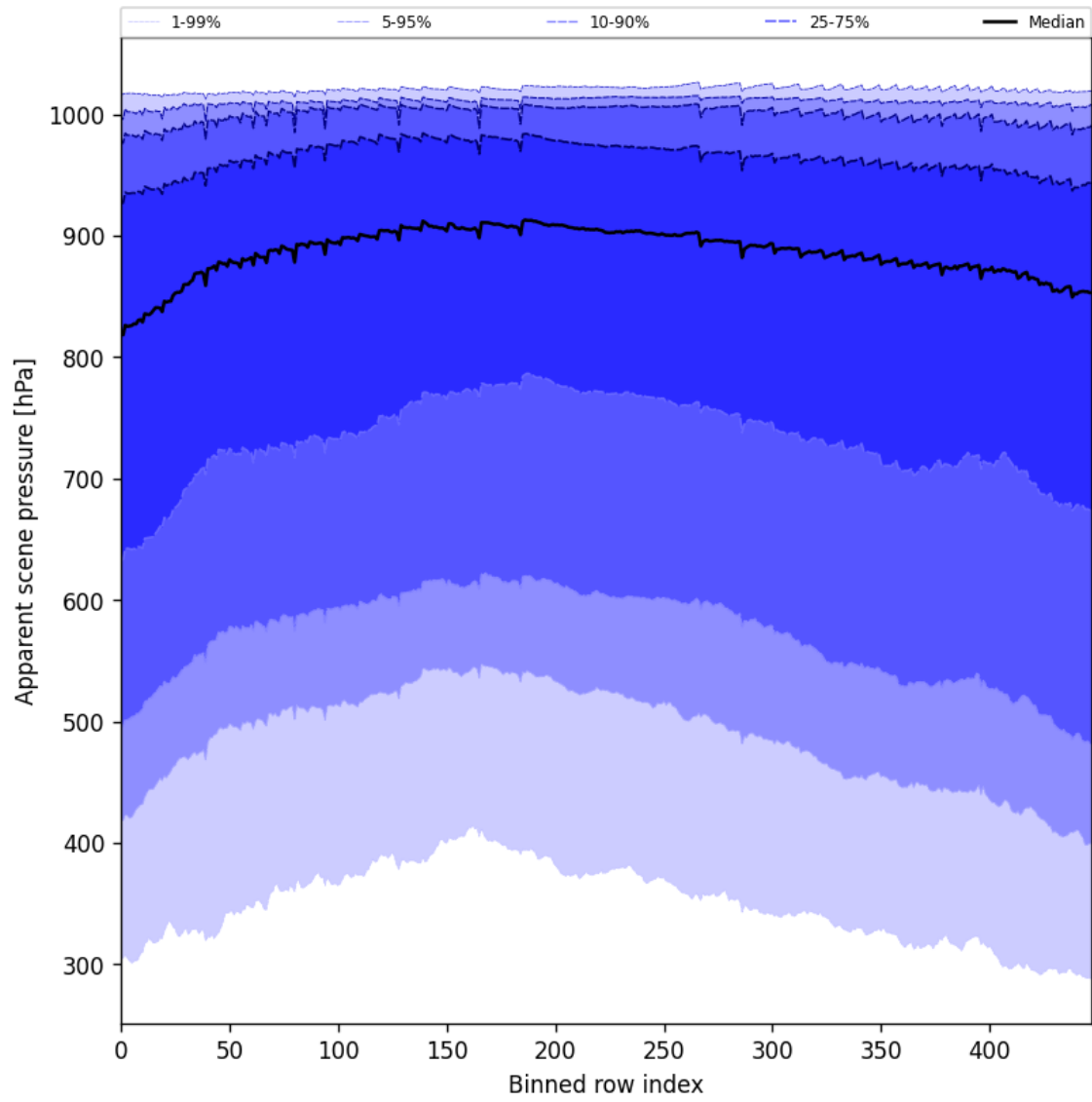
Figure 53: Along track statistics of “Apparent scene pressure” for 2025-03-26 to 2025-03-28
