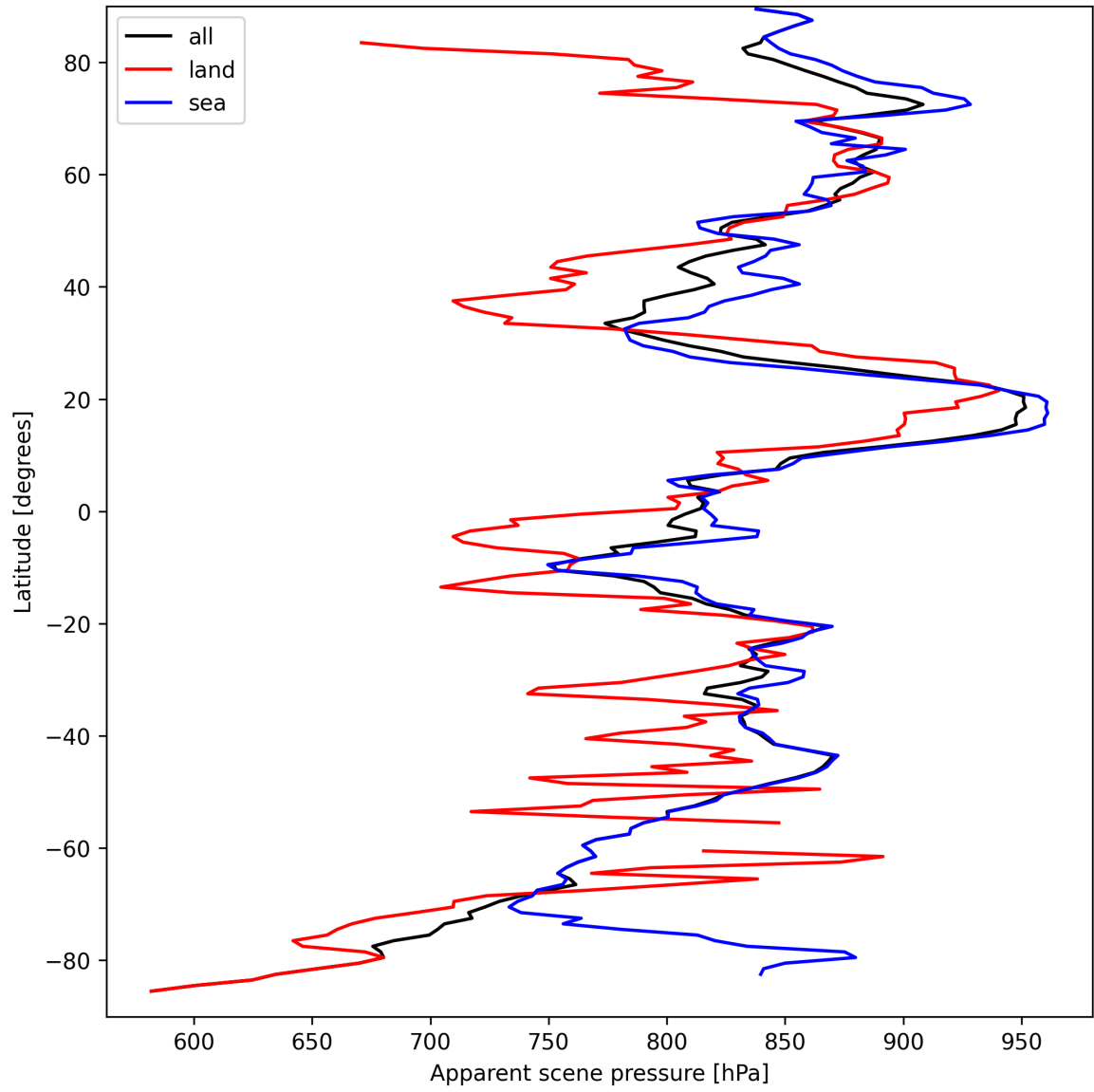
Figure 19: Zonal average of “Apparent scene pressure” for 2025-03-26 to 2025-03-28.
