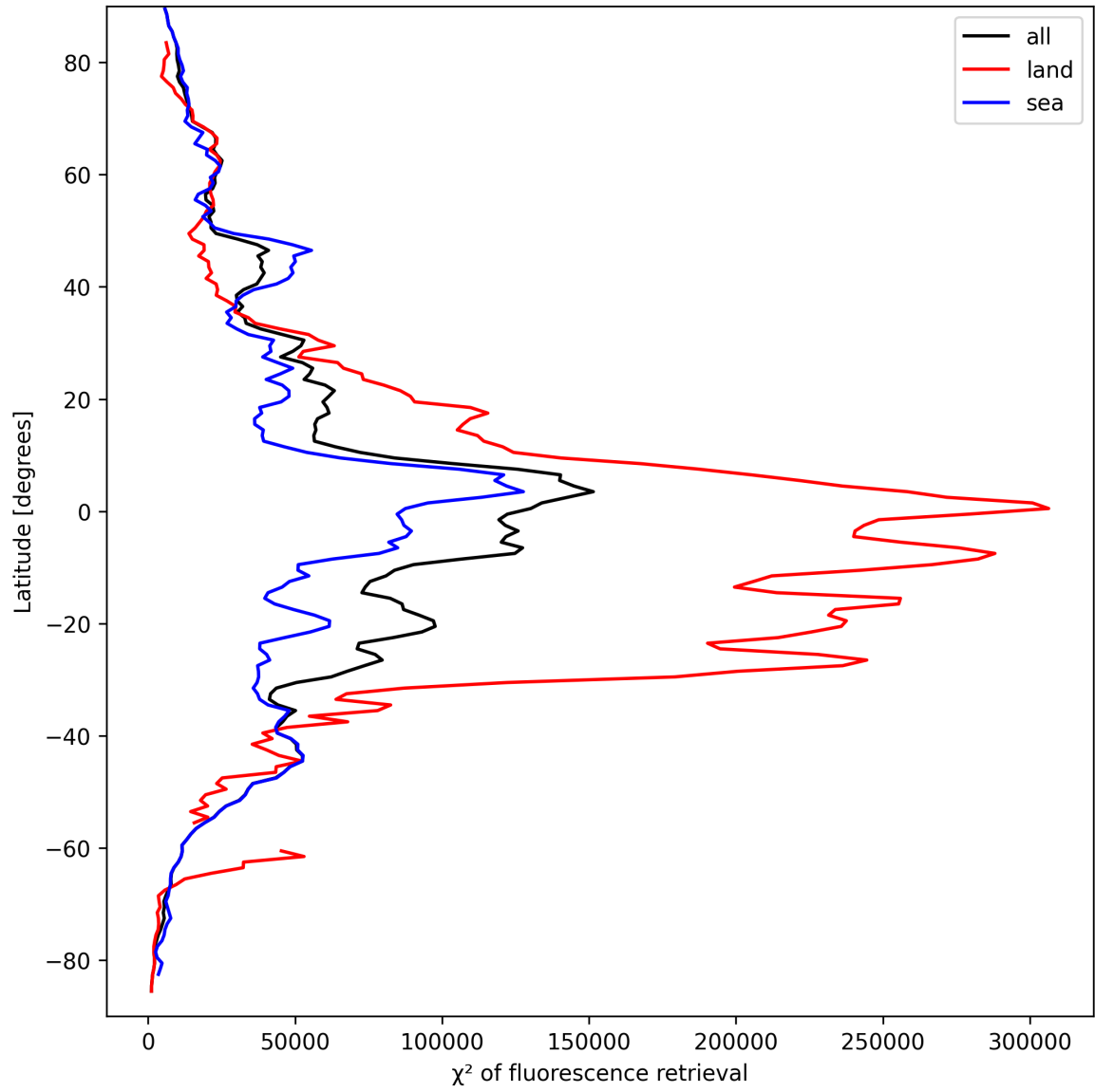
Figure 25: Zonal average of “ \chi^2 of fluorescence retrieval” for 2025-03-26 to 2025-03-28.
