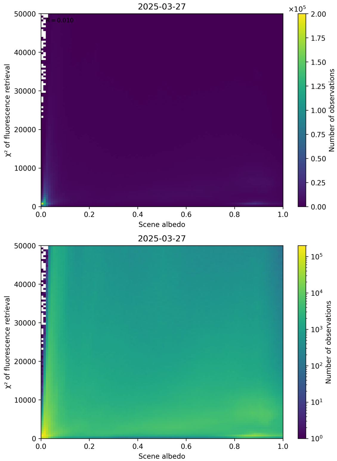
Figure 103: Scatter density plot of “Scene albedo” against “ \chi^2 of fluorescence retrieval” for 2025-03-26 to 2025-03-28.
