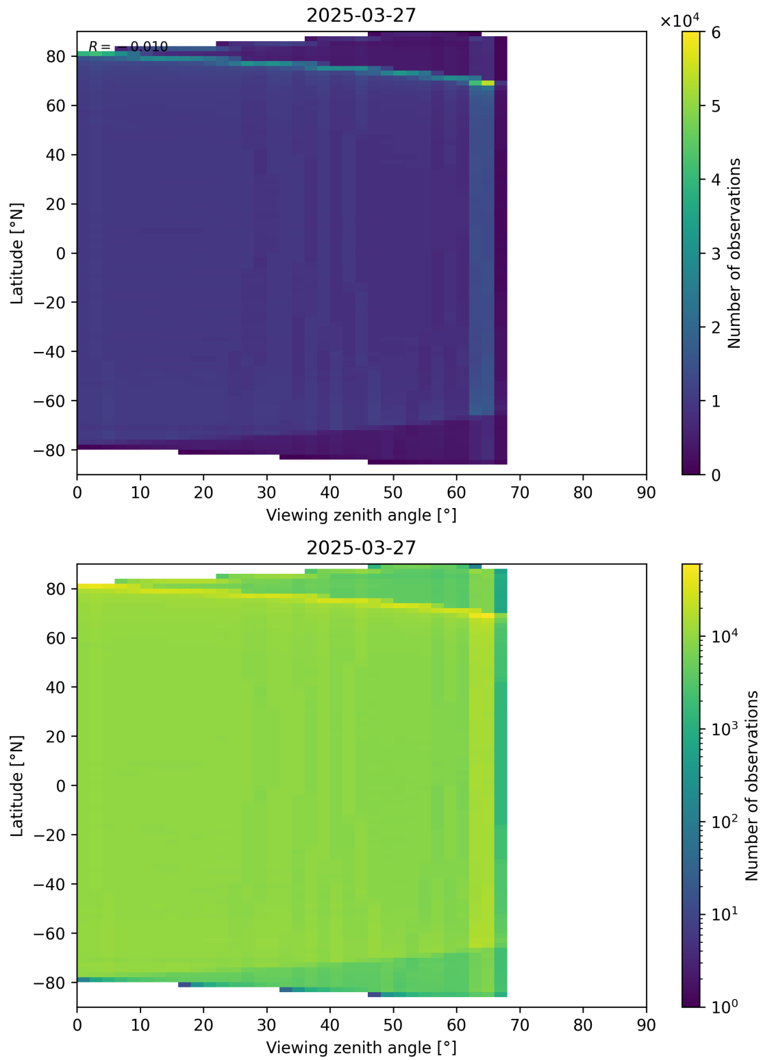
Figure 123: Scatter density plot of “Viewing zenith angle” against “Latitude” for 2025-03-26 to 2025-03-28.
