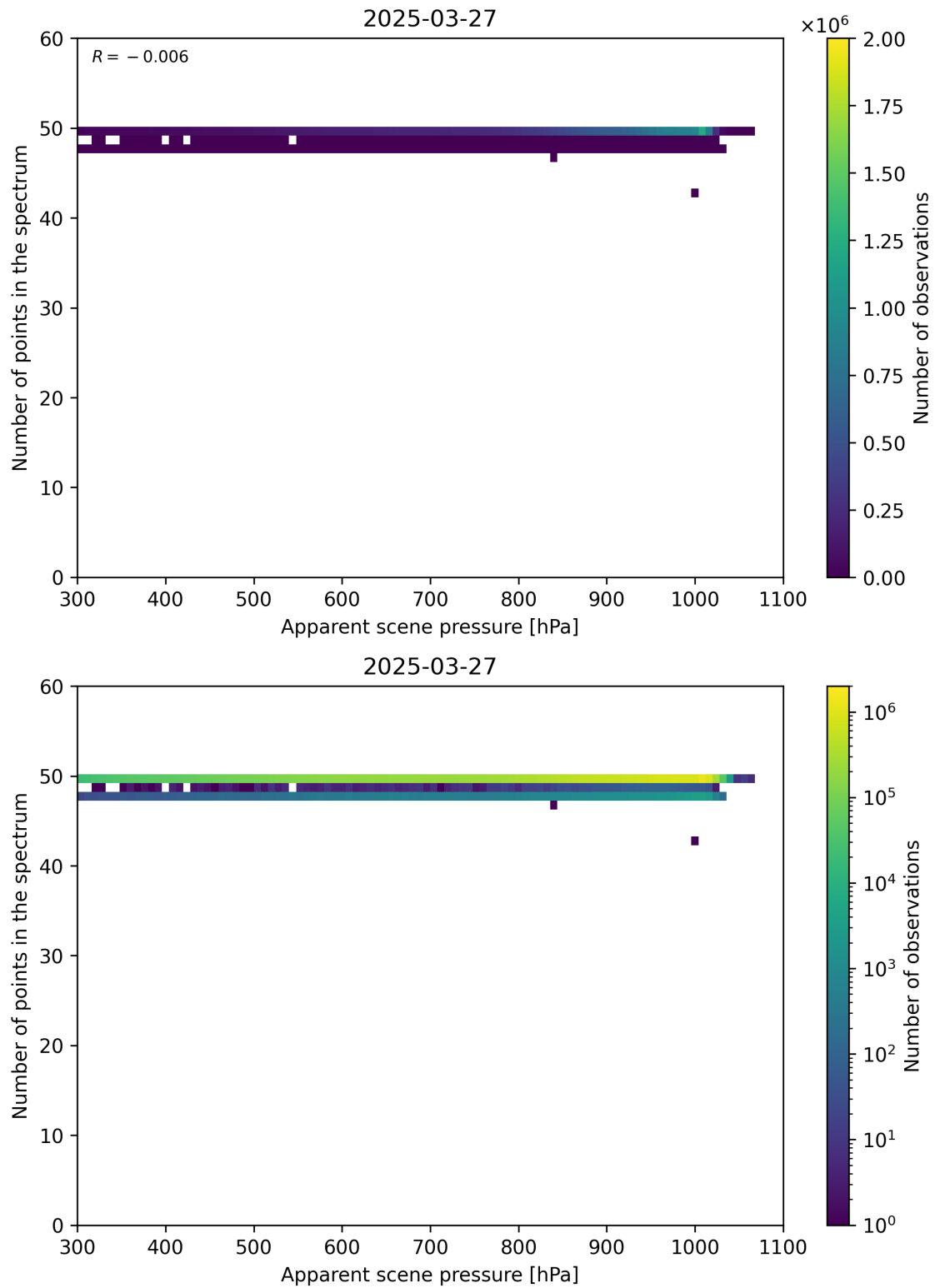
Figure 66: Scatter density plot of “Apparent scene pressure” against “Number of points in the spectrum” for 2025-03-26 to 2025-03-28.
