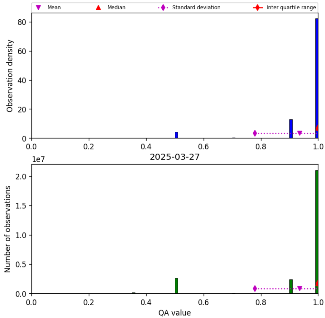
Figure 29: Histogram of “QA value” for 2025-03-26 to 2025-03-28
