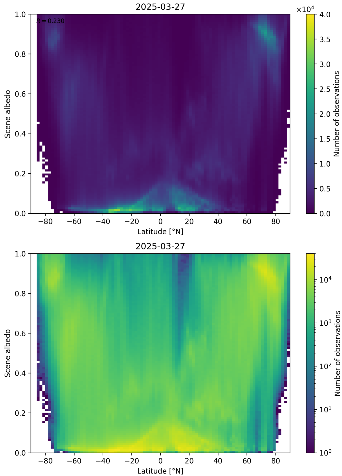
Figure 95: Scatter density plot of “Latitude” against “Scene albedo” for 2025-03-26 to 2025-03-28.
