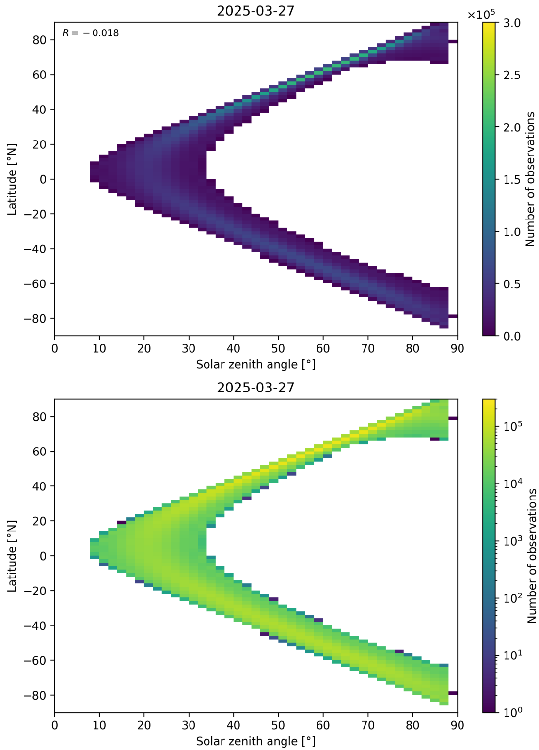
Figure 113: Scatter density plot of “Solar zenith angle” against “Latitude” for 2025-03-26 to 2025-03-28.
