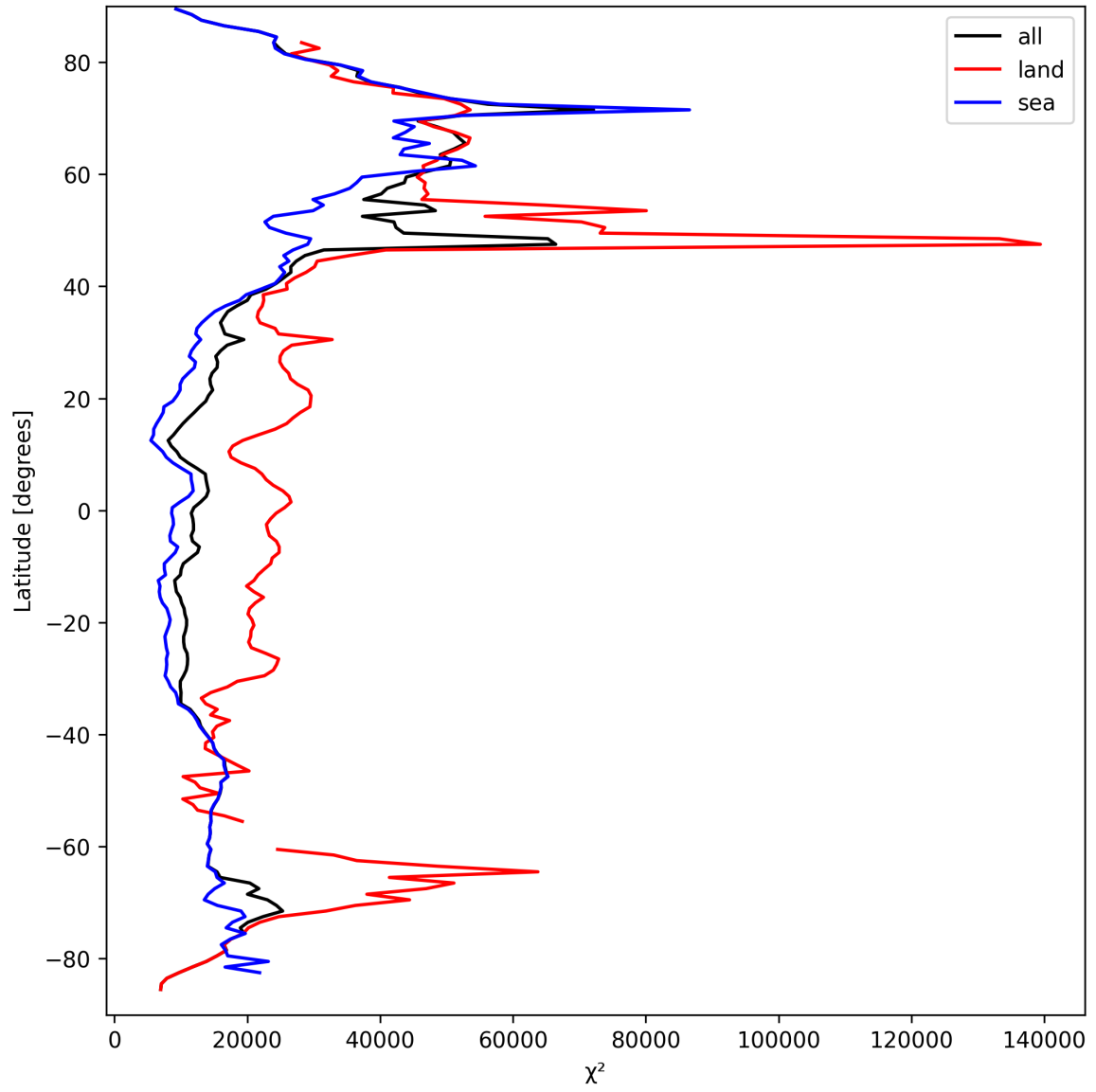
Figure 21: Zonal average of “ \chi^2 ” for 2025-03-26 to 2025-03-28.
