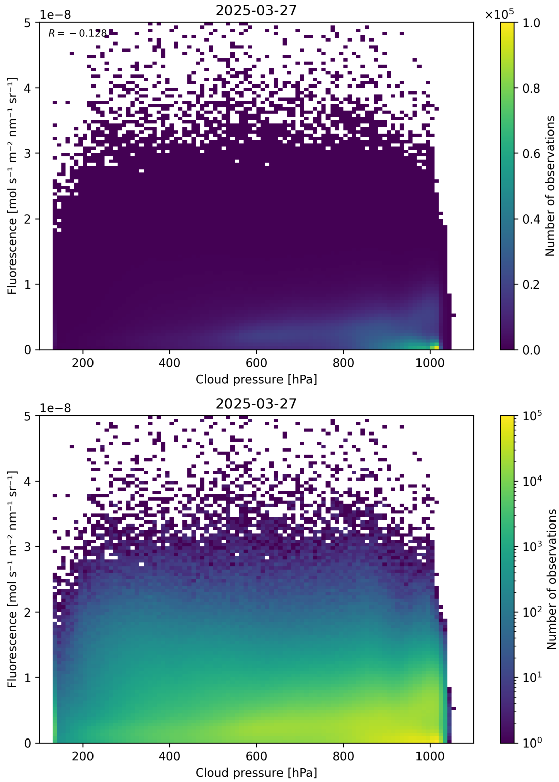
Figure 80: Scatter density plot of “Cloud pressure” against “Fluorescence” for 2025-03-26 to 2025-03-28.
