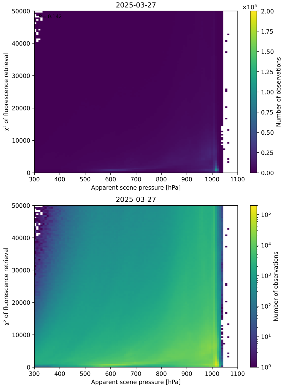
Figure 63: Scatter density plot of “Apparent scene pressure” against “ \chi^2 of fluorescence retrieval” for 2025-03-26 to 2025-03-28.
