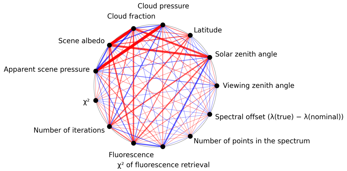
Figure 1: Map of correlation graph for 2025-03-26 to 2025-03-28.
