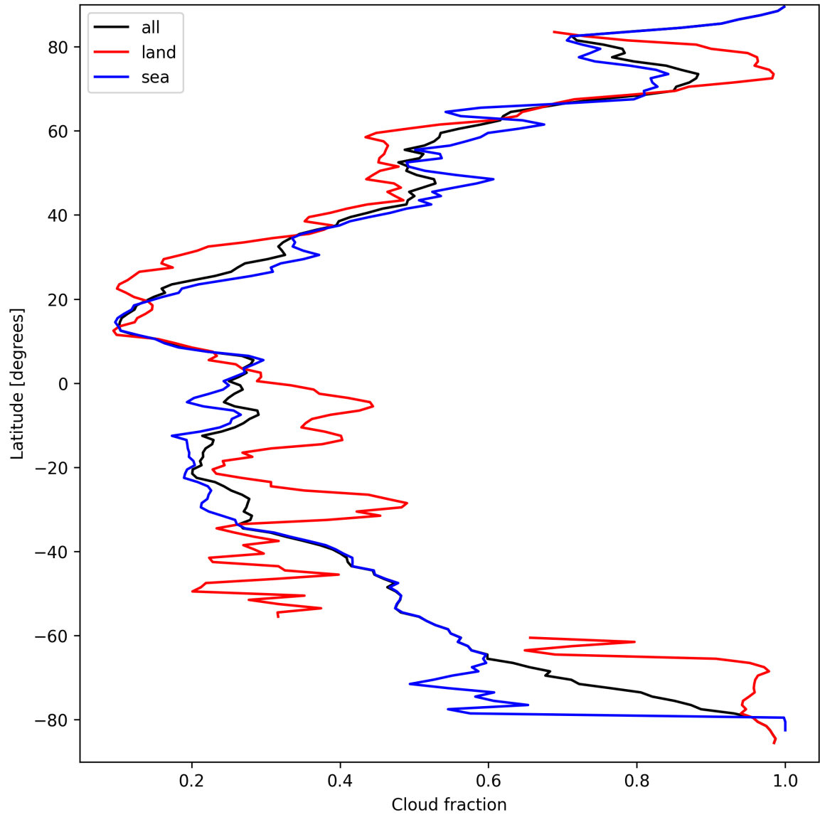
Figure 15: Zonal average of “Cloud fraction” for 2025-03-26 to 2025-03-28.
