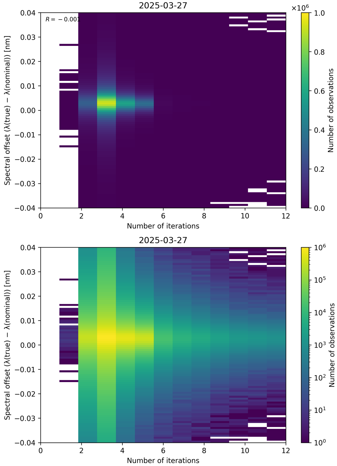
Figure 100: Scatter density plot of “Number of iterations” against “Spectral offset ( \lambda_{\text{true}} - \lambda_{\text{nominal}} )” for 2025-03-26 to 2025-03-28.
