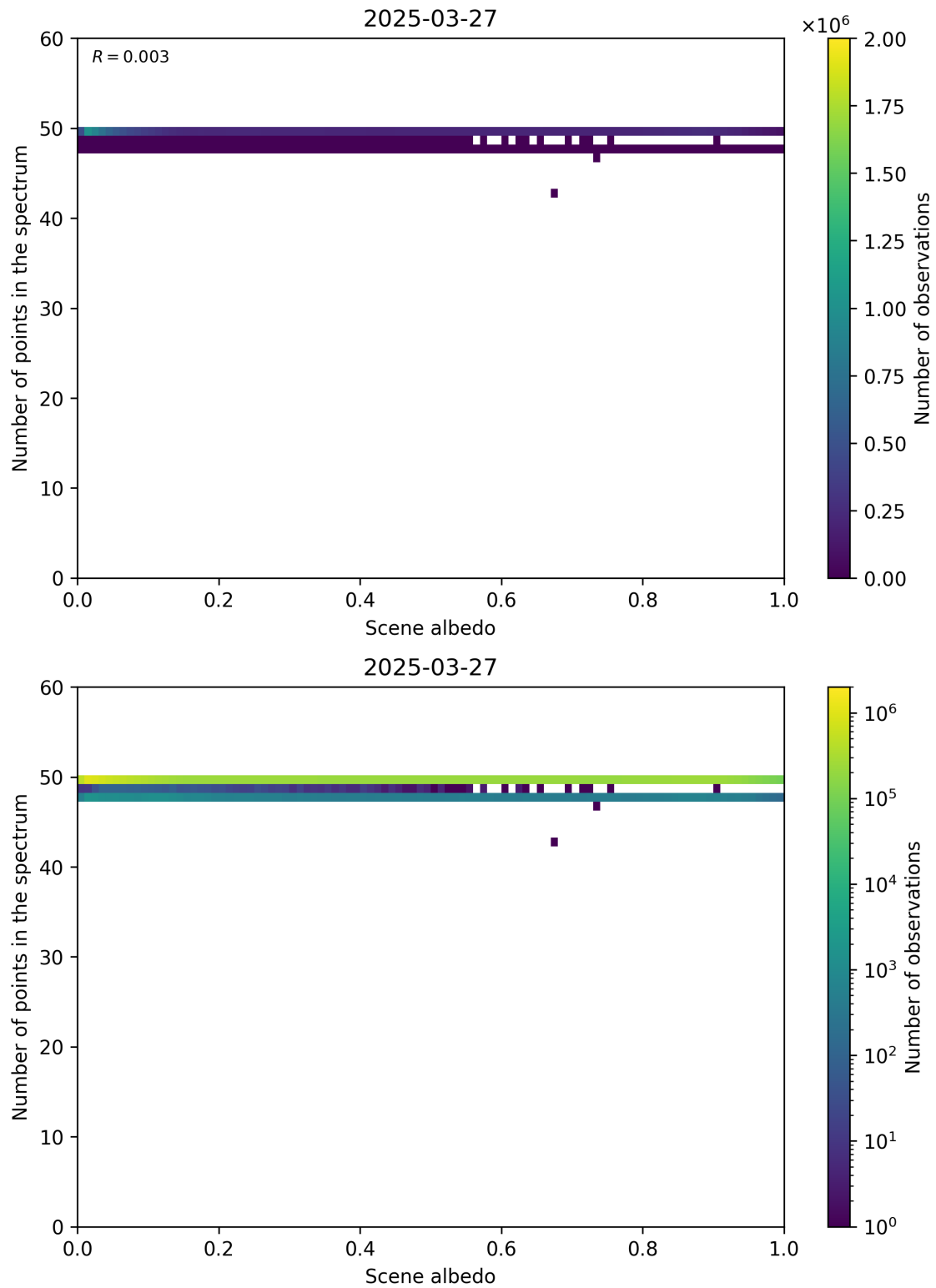
Figure 106: Scatter density plot of “Scene albedo” against “Number of points in the spectrum” for 2025-03-26 to 2025-03-28.
