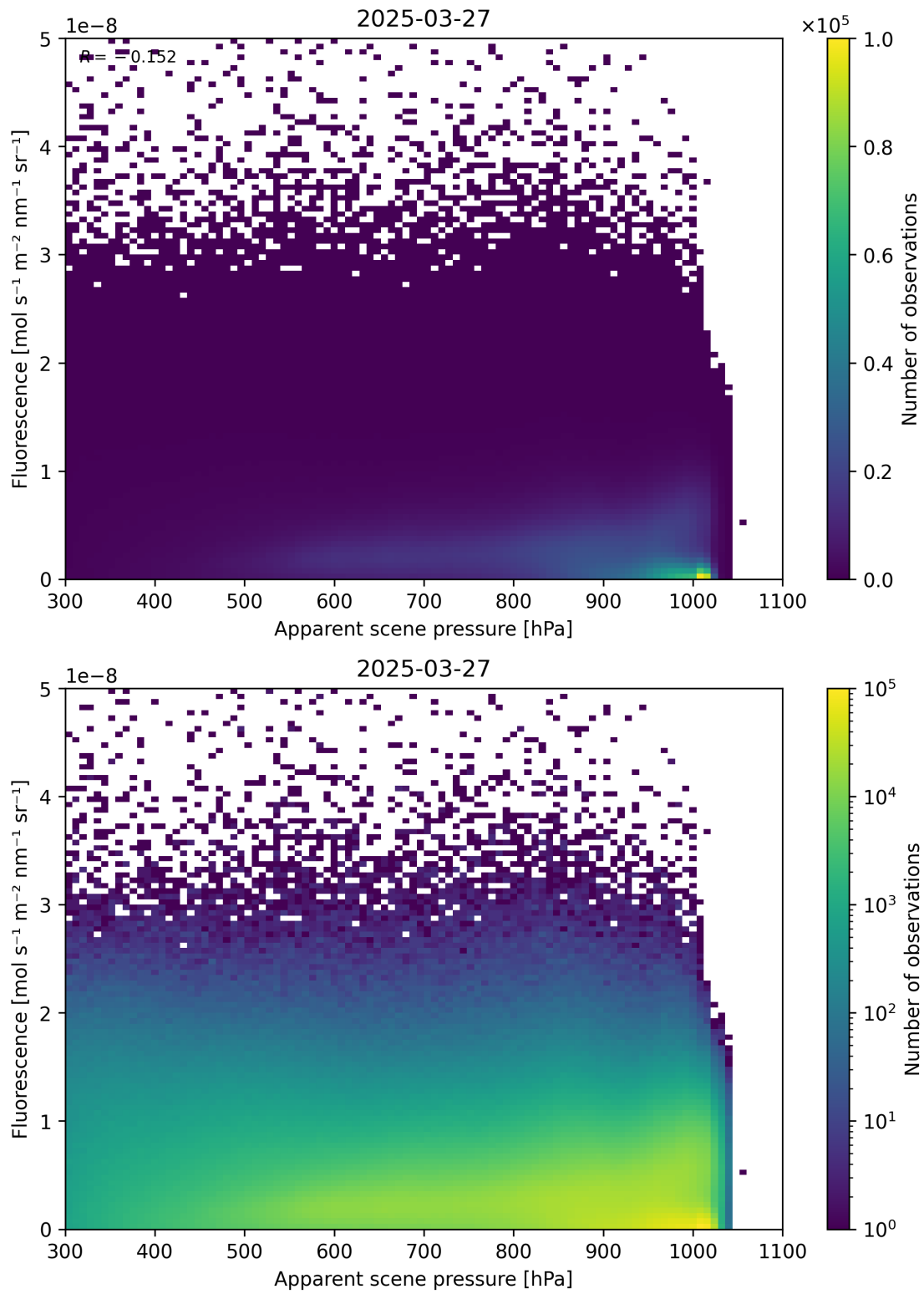
Figure 64: Scatter density plot of “Apparent scene pressure” against “Fluorescence” for 2025-03-26 to 2025-03-28.
