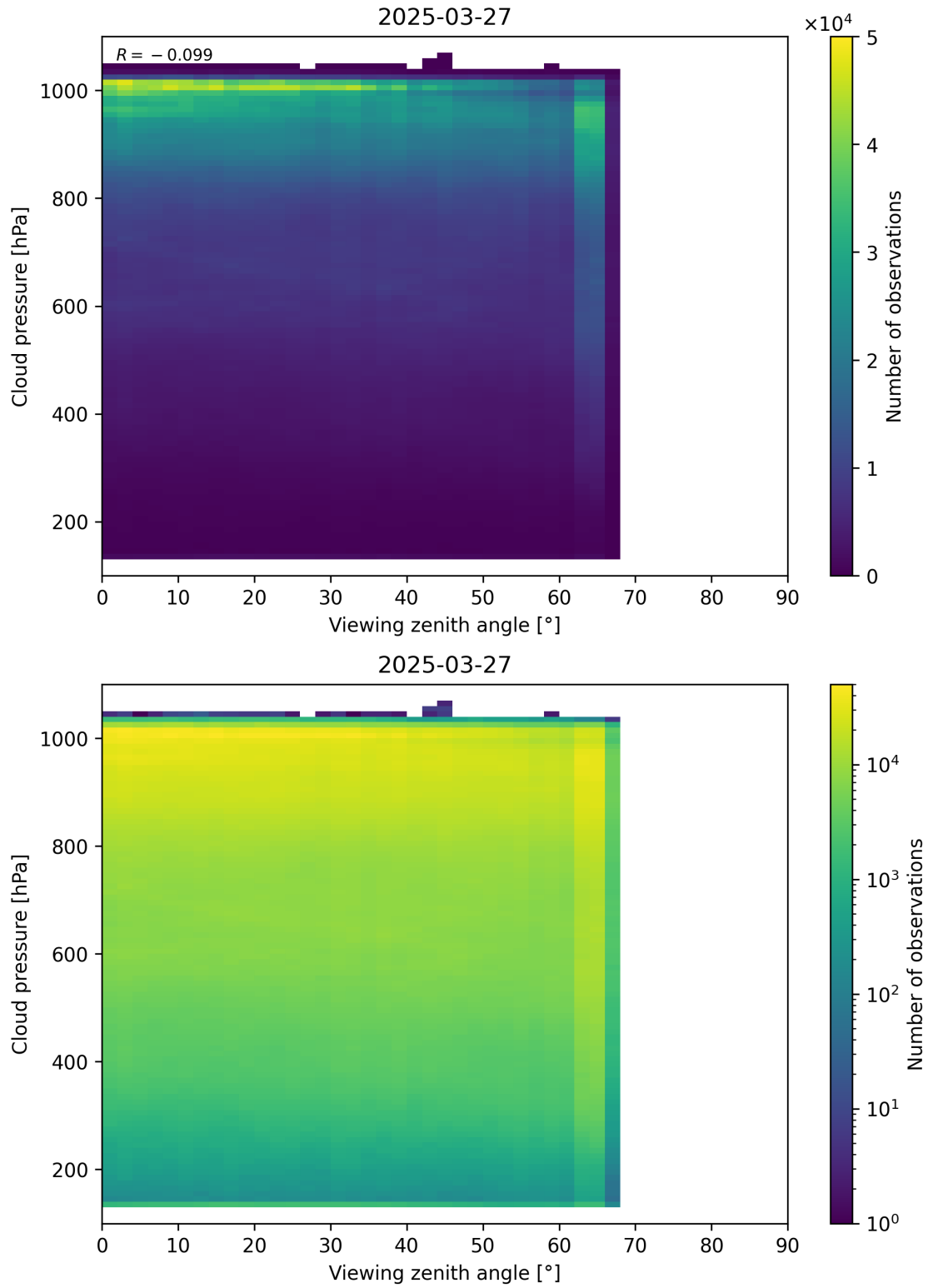
Figure 121: Scatter density plot of “Viewing zenith angle” against “Cloud pressure” for 2025-03-26 to 2025-03-28.
