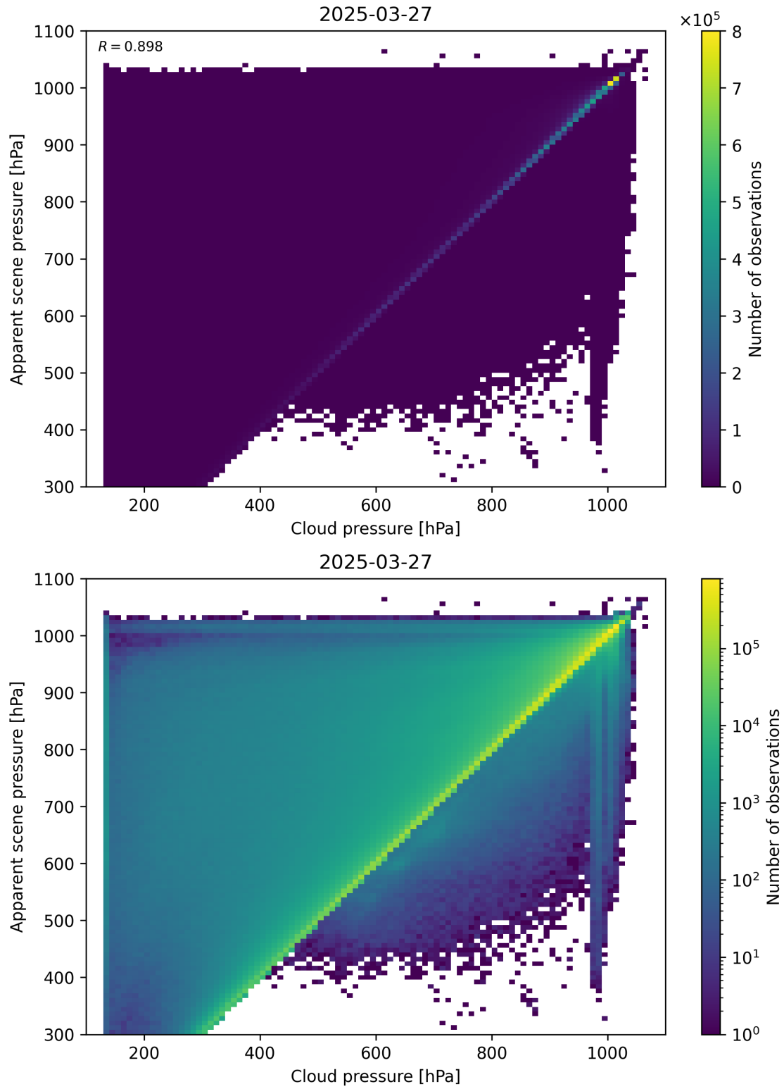
Figure 77: Scatter density plot of “Cloud pressure” against “Apparent scene pressure” for 2025-03-26 to 2025-03-28.
