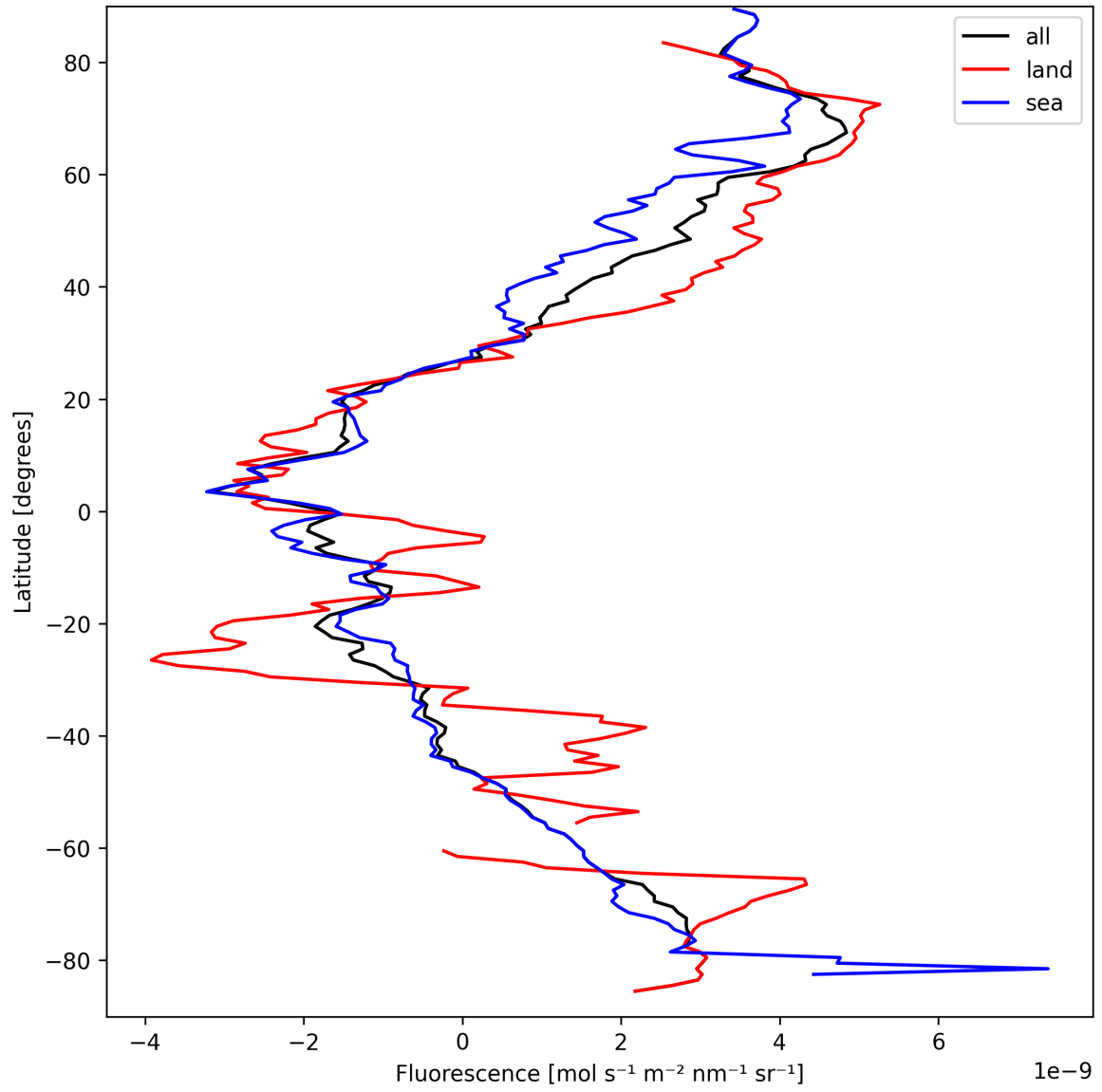
Figure 23: Zonal average of “Fluorescence” for 2025-03-26 to 2025-03-28.
