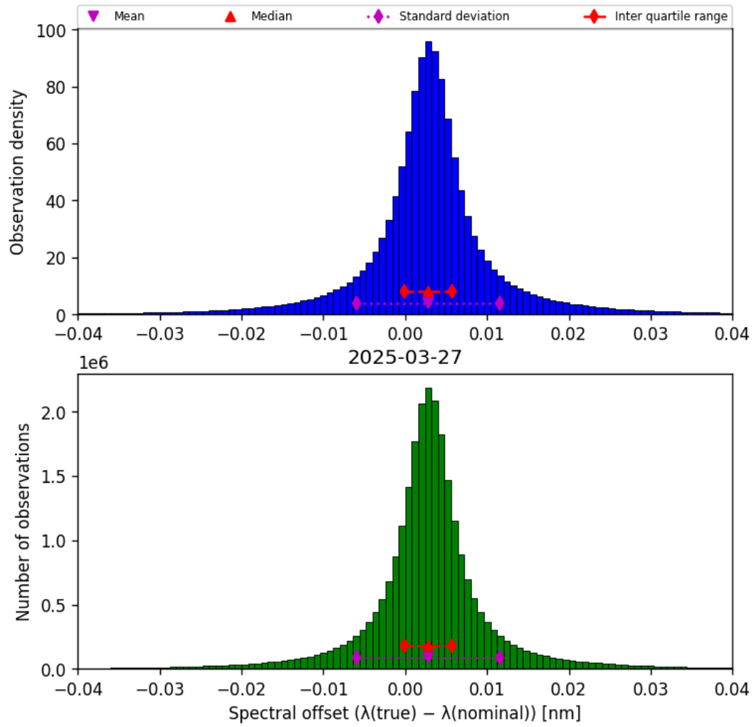
Figure 45: Histogram of “Spectral offset ( \lambda_{\text{true}} - \lambda_{\text{nominal}} )” for 2025-03-26 to 2025-03-28
