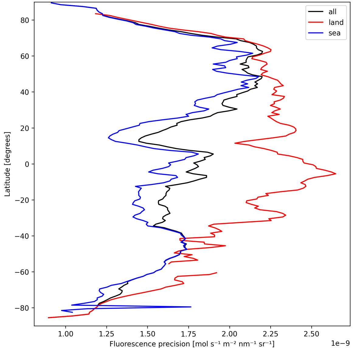
Figure 24: Zonal average of “Fluorescence precision” for 2025-03-26 to 2025-03-28.
