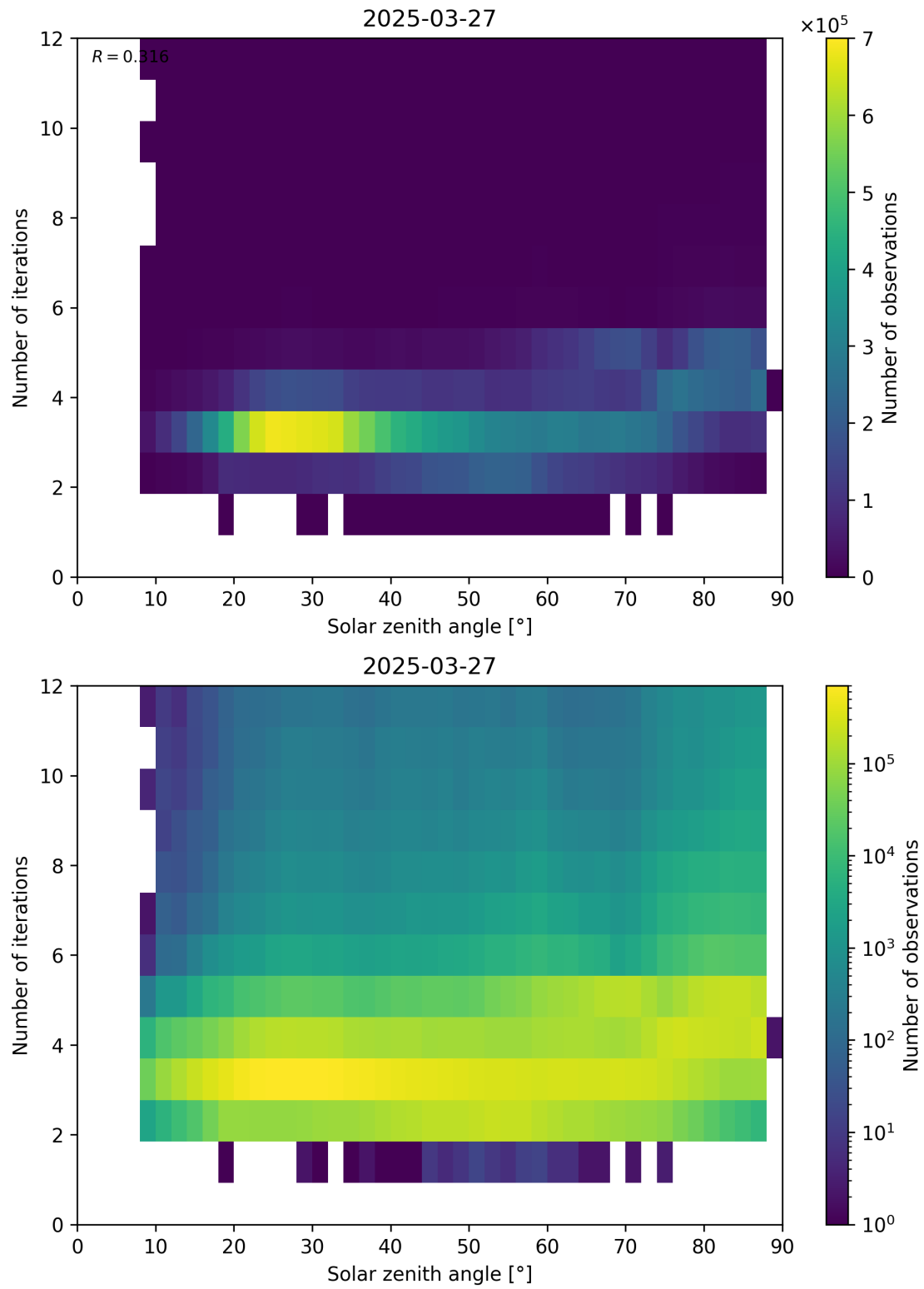
Figure 114: Scatter density plot of “Solar zenith angle” against “Number of iterations” for 2025-03-26 to 2025-03-28.
