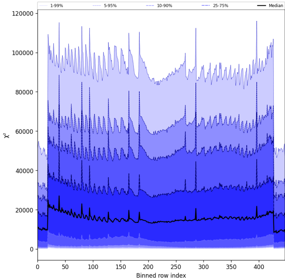
Figure 55: Along track statistics of “ \chi^2 ” for 2025-03-26 to 2025-03-28
