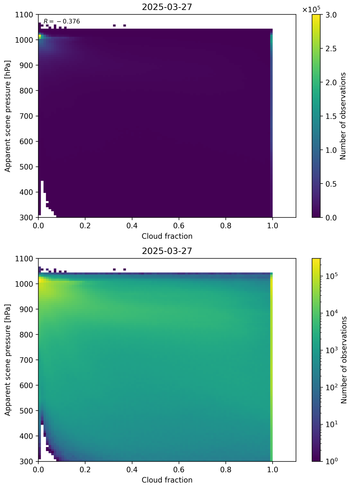
Figure 70: Scatter density plot of “Cloud fraction” against “Apparent scene pressure” for 2025-03-26 to 2025-03-28.
