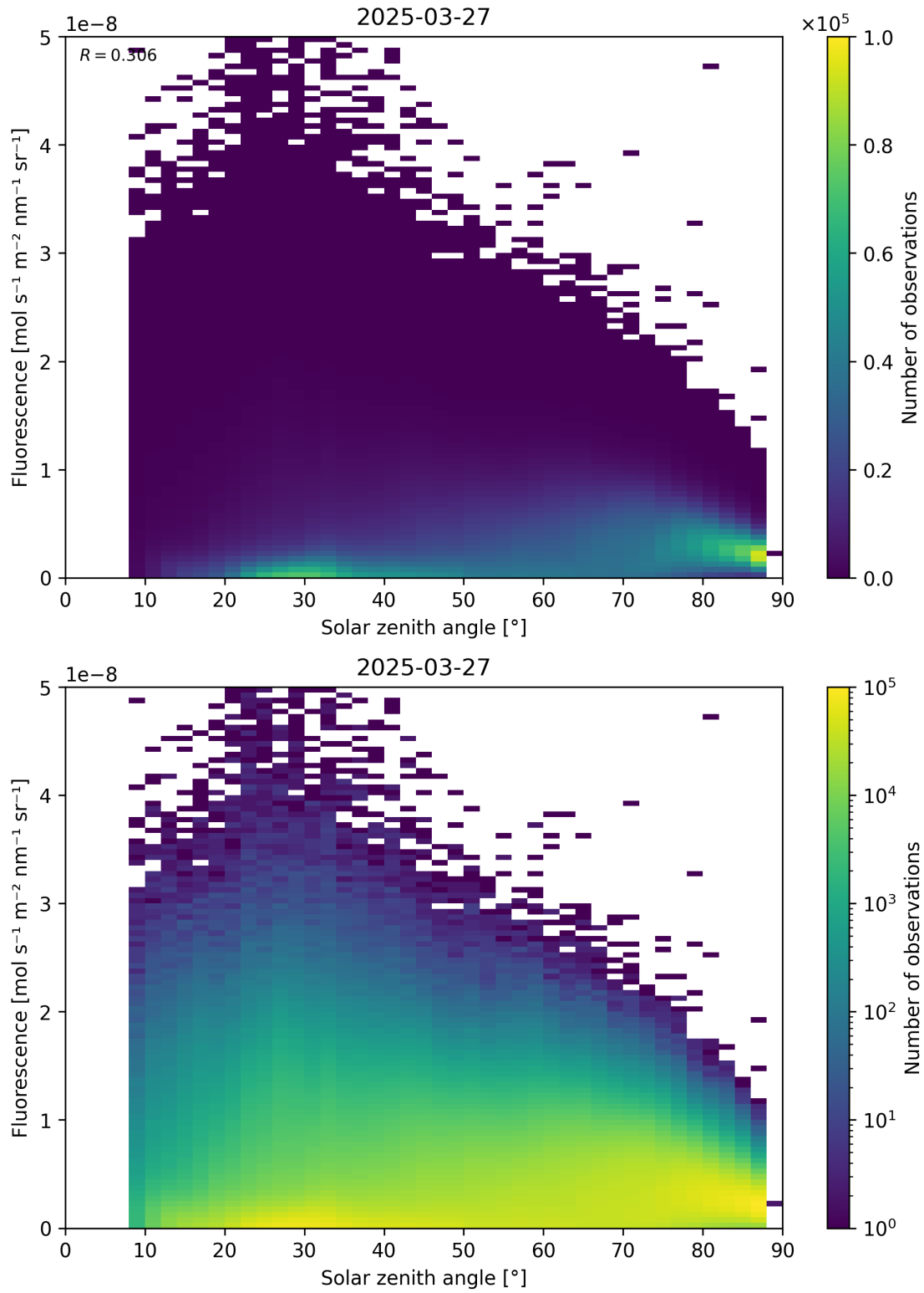
Figure 112: Scatter density plot of “Solar zenith angle” against “Fluorescence” for 2025-03-26 to 2025-03-28.
