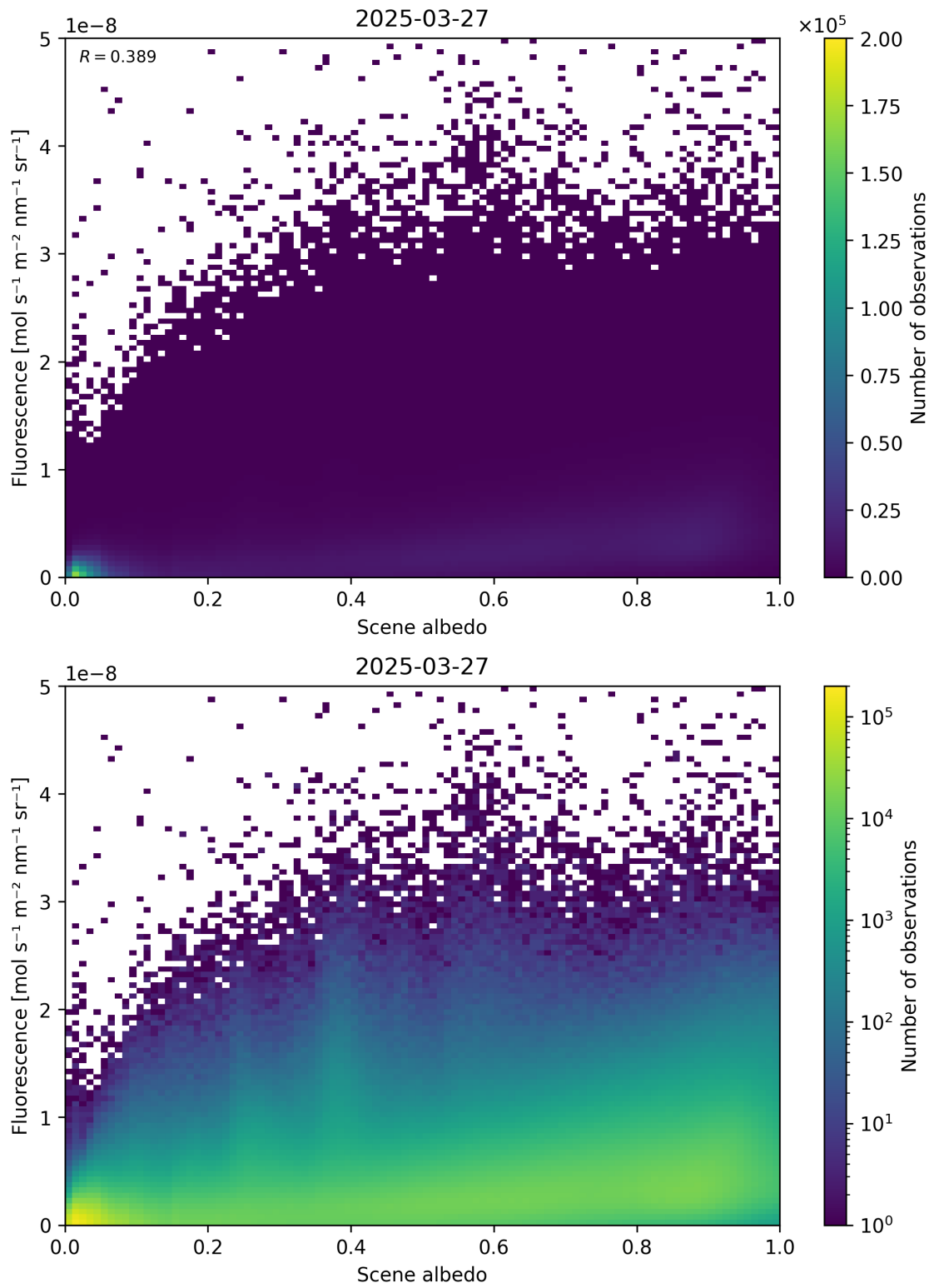
Figure 104: Scatter density plot of “Scene albedo” against “Fluorescence” for 2025-03-26 to 2025-03-28.
