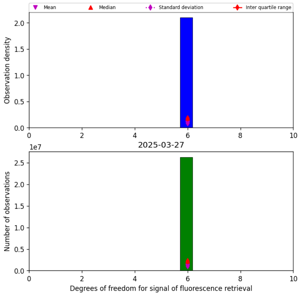
Figure 43: Histogram of “Degrees of freedom for signal of fluorescence retrieval” for 2025-03-26 to 2025-03-28
