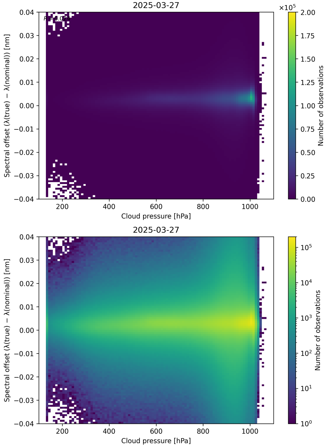
Figure 84: Scatter density plot of “Cloud pressure” against “Spectral offset ( \lambda_{\text{true}} - \lambda_{\text{nominal}} )” for 2025-03-26 to 2025-03-28.
