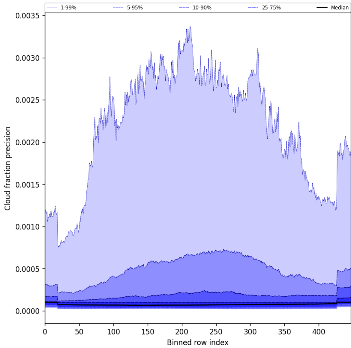
Figure 50: Along track statistics of “Cloud fraction precision” for 2025-03-26 to 2025-03-28
