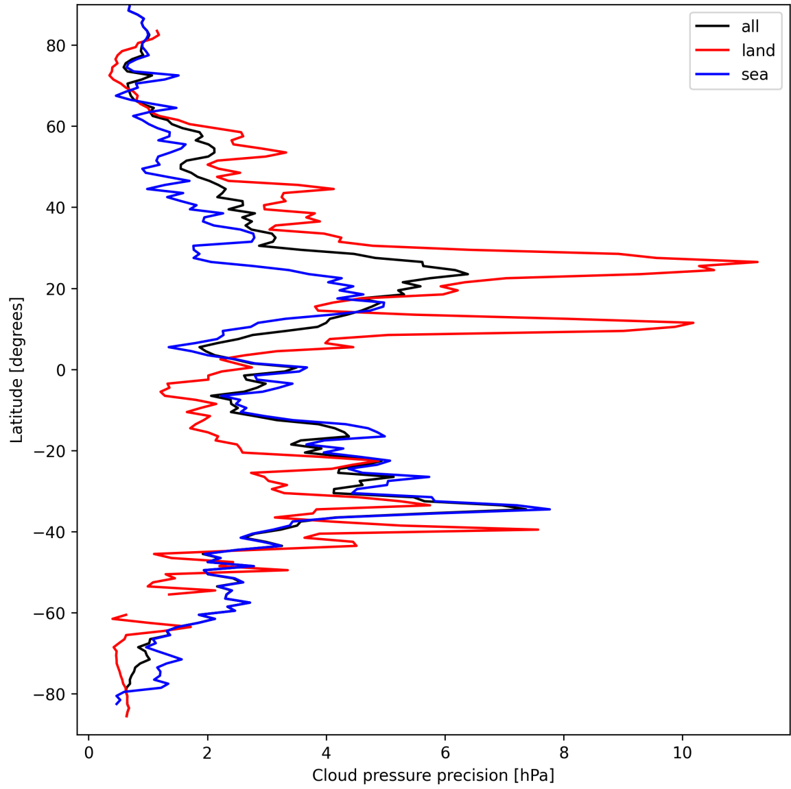
Figure 14: Zonal average of “Cloud pressure precision” for 2025-03-26 to 2025-03-28.
