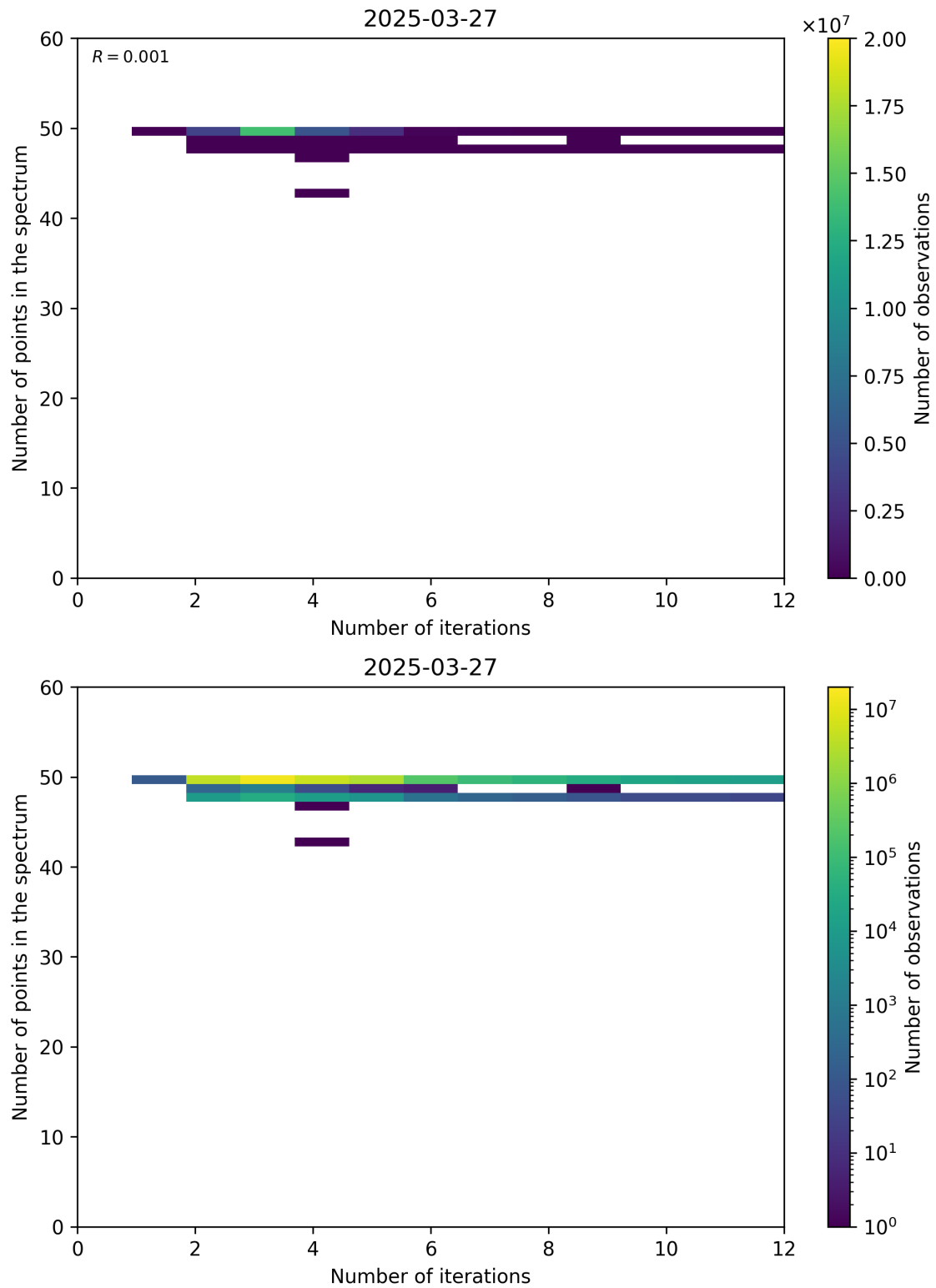
Figure 99: Scatter density plot of “Number of iterations” against “Number of points in the spectrum” for 2025-03-26 to 2025-03-28.
