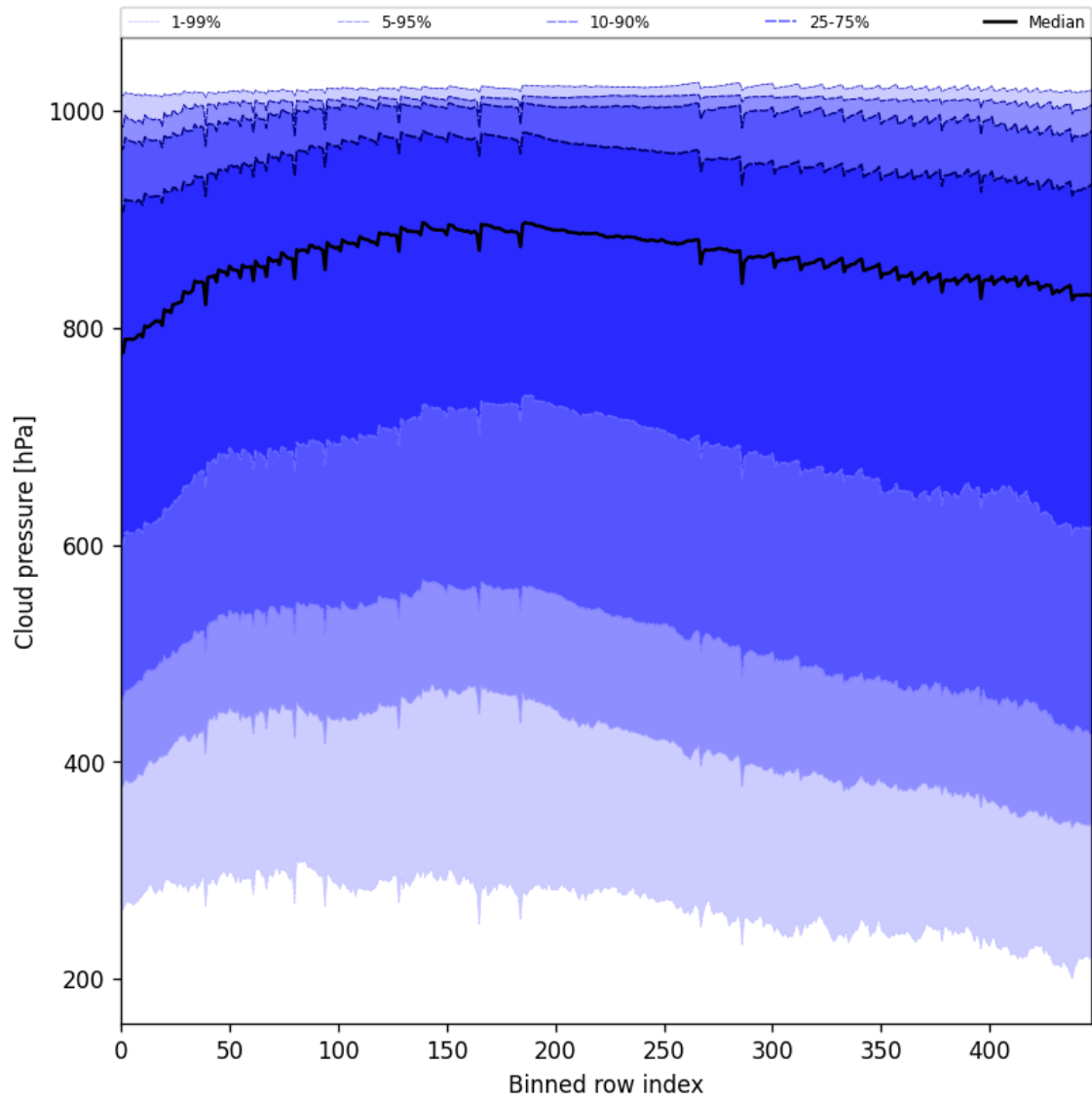
Figure 47: Along track statistics of “Cloud pressure” for 2025-03-26 to 2025-03-28
