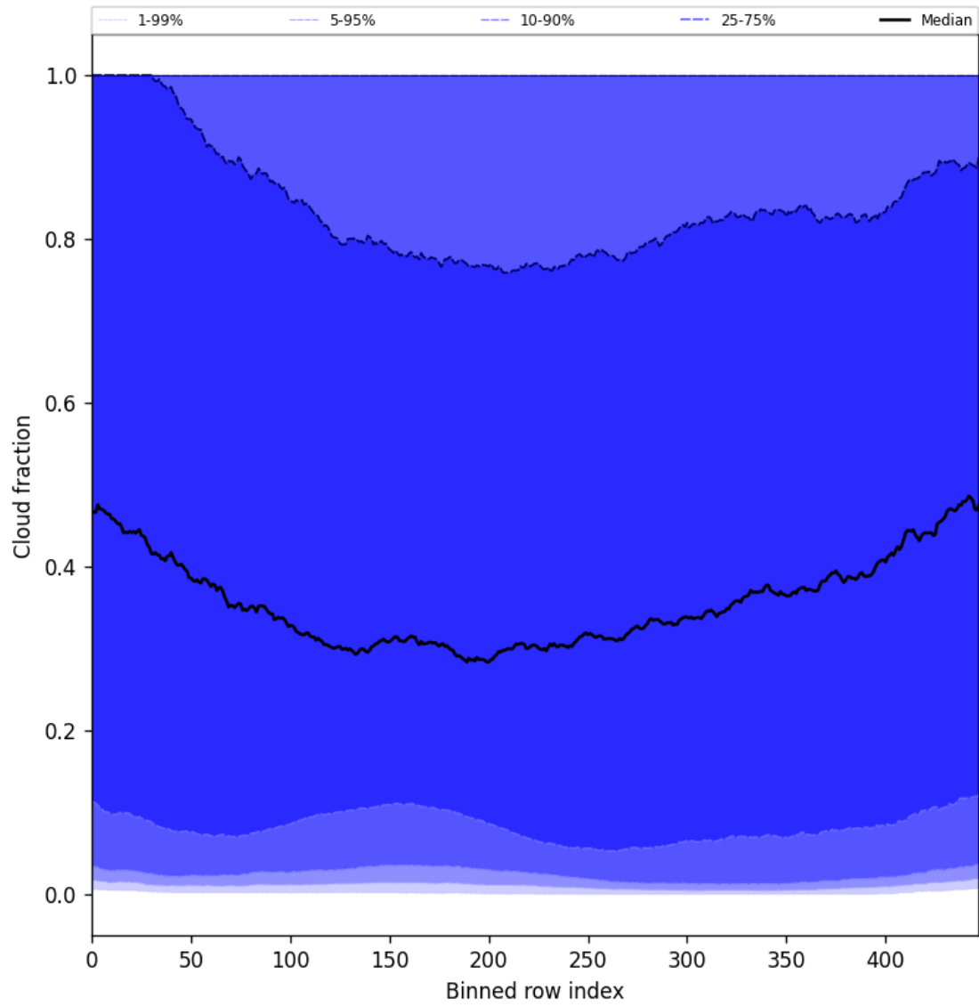
Figure 49: Along track statistics of “Cloud fraction” for 2025-03-26 to 2025-03-28
