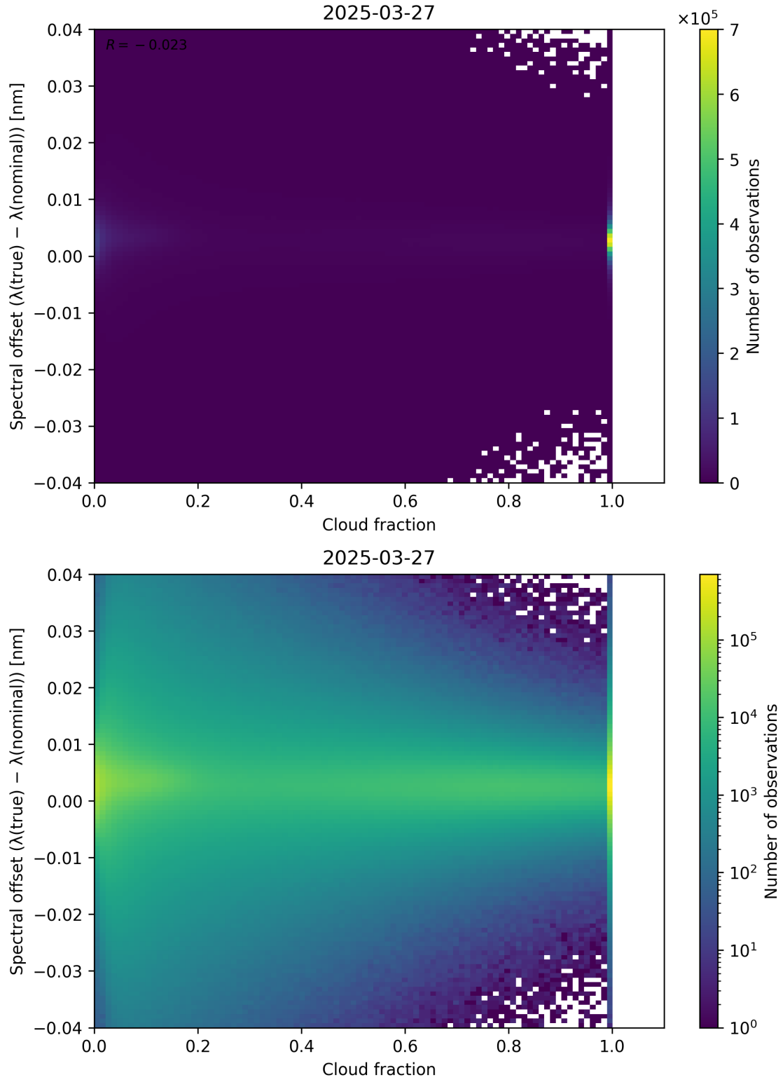
Figure 76: Scatter density plot of “Cloud fraction” against “Spectral offset ( \lambda_{\text{true}} - \lambda_{\text{nominal}} )” for 2025-03-26 to 2025-03-28.
