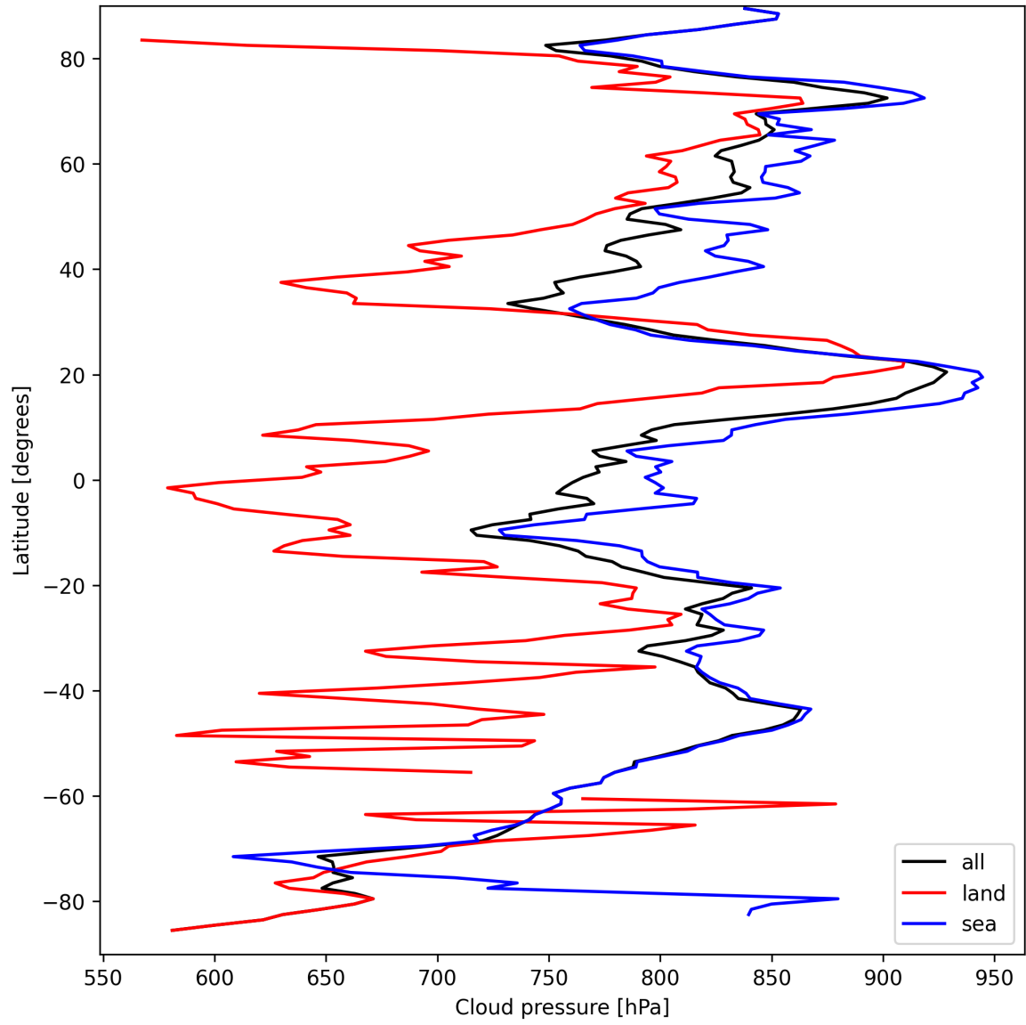
Figure 13: Zonal average of “Cloud pressure” for 2025-03-26 to 2025-03-28.
