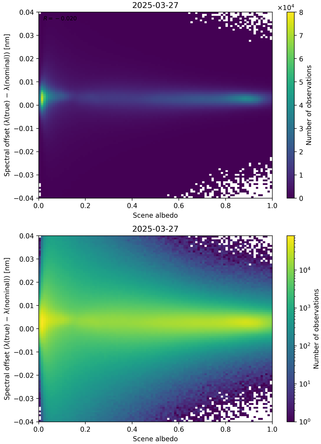
Figure 107: Scatter density plot of “Scene albedo” against “Spectral offset ( \lambda_{\text{true}} - \lambda_{\text{nominal}} )” for 2025-03-26 to 2025-03-28.
