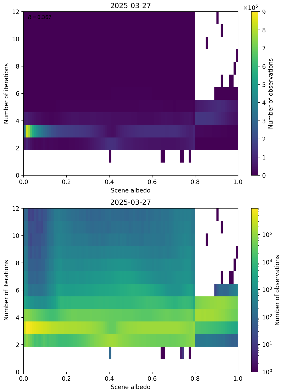
Figure 105: Scatter density plot of “Scene albedo” against “Number of iterations” for 2025-03-26 to 2025-03-28.
