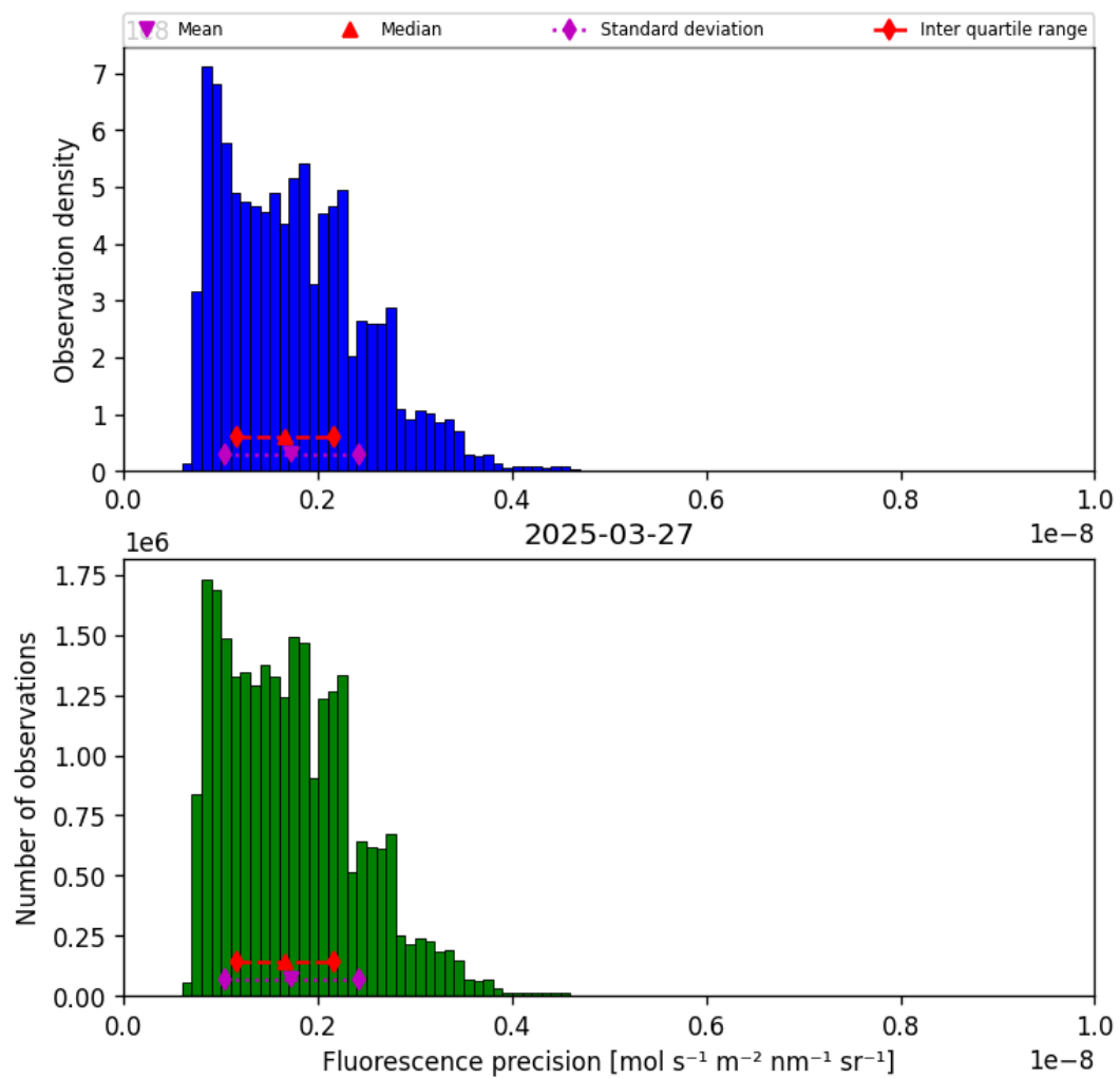
Figure 41: Histogram of “Fluorescence precision” for 2025-03-26 to 2025-03-28
