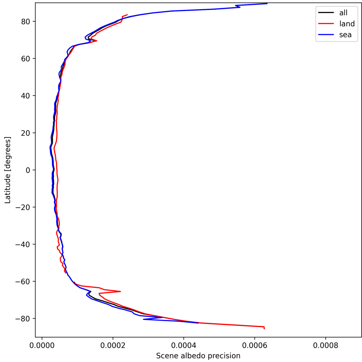
Figure 18: Zonal average of “Scene albedo precision” for 2025-03-26 to 2025-03-28.
