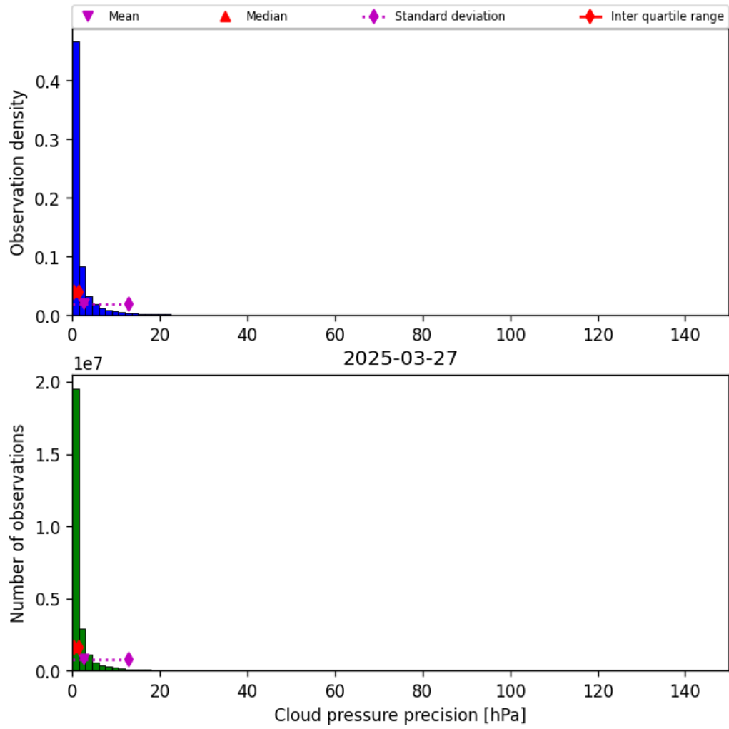
Figure 31: Histogram of “Cloud pressure precision” for 2025-03-26 to 2025-03-28
