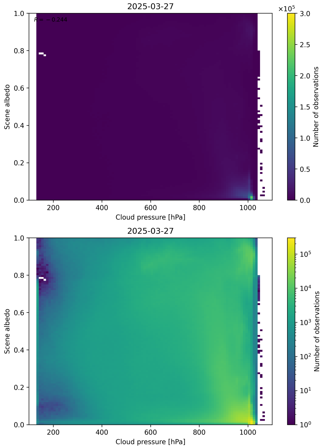
Figure 83: Scatter density plot of “Cloud pressure” against “Scene albedo” for 2025-03-26 to 2025-03-28.
