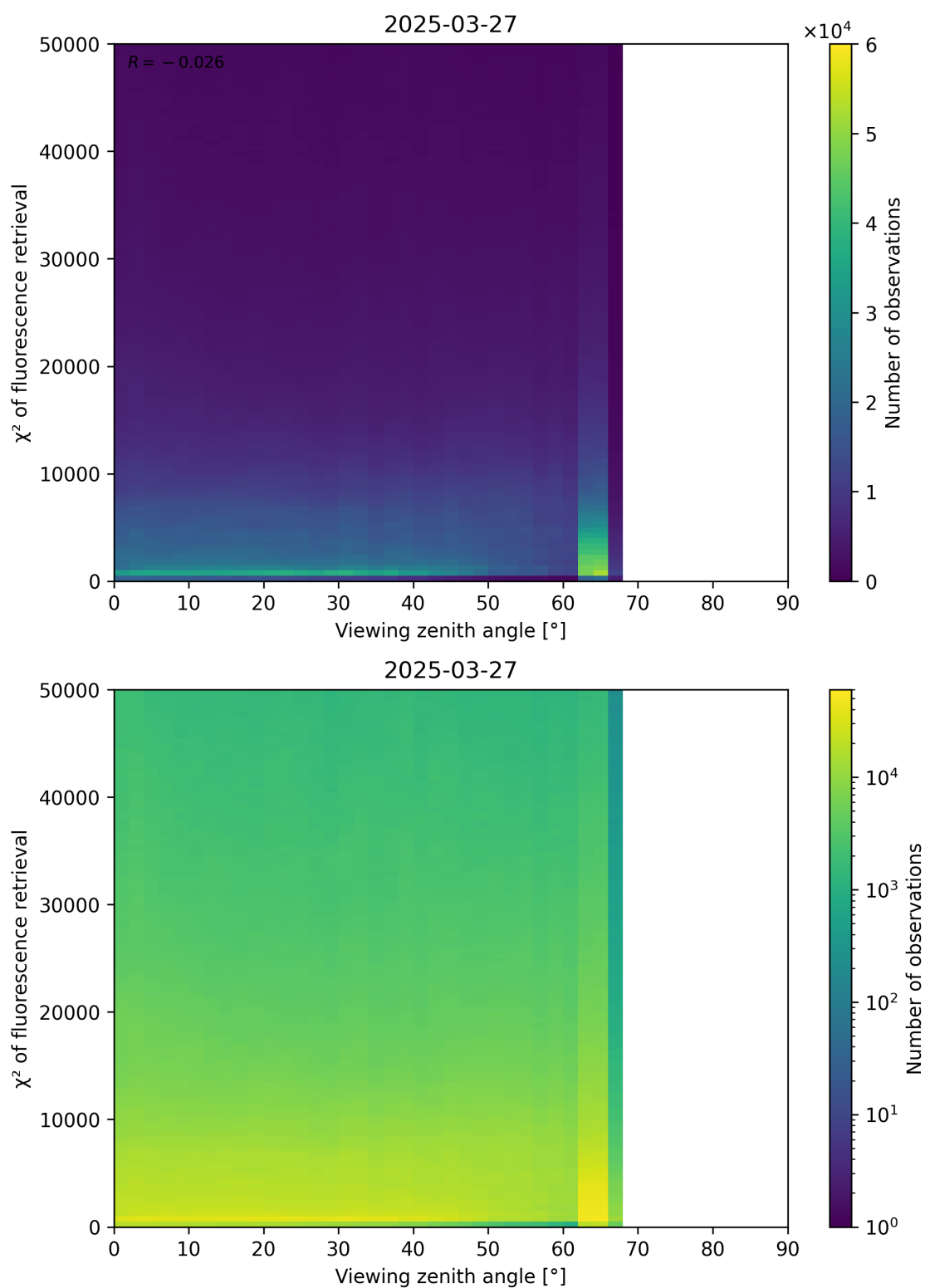
Figure 119: Scatter density plot of “Viewing zenith angle” against “ \chi^2 of fluorescence retrieval” for 2025-03-26 to 2025-03-28.
