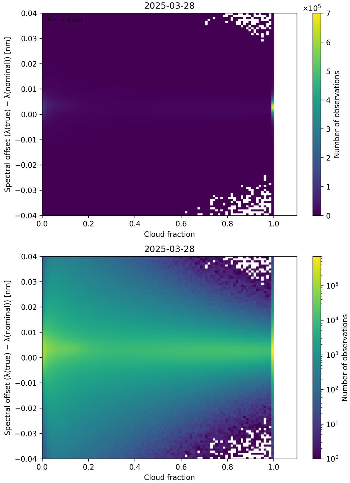
Figure 76: Scatter density plot of “Cloud fraction” against “Spectral offset ( \lambda_{\text{true}} - \lambda_{\text{nominal}} )” for 2025-03-28 to 2025-03-29.
