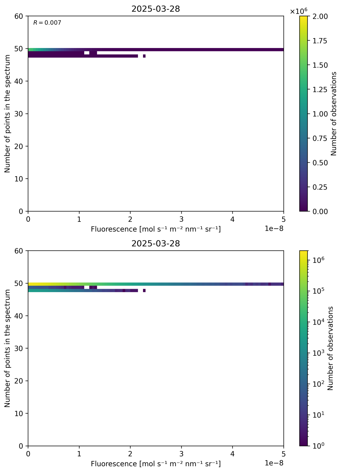
Figure 86: Scatter density plot of “Fluorescence” against “Number of points in the spectrum” for 2025-03-28 to 2025-03-29.
