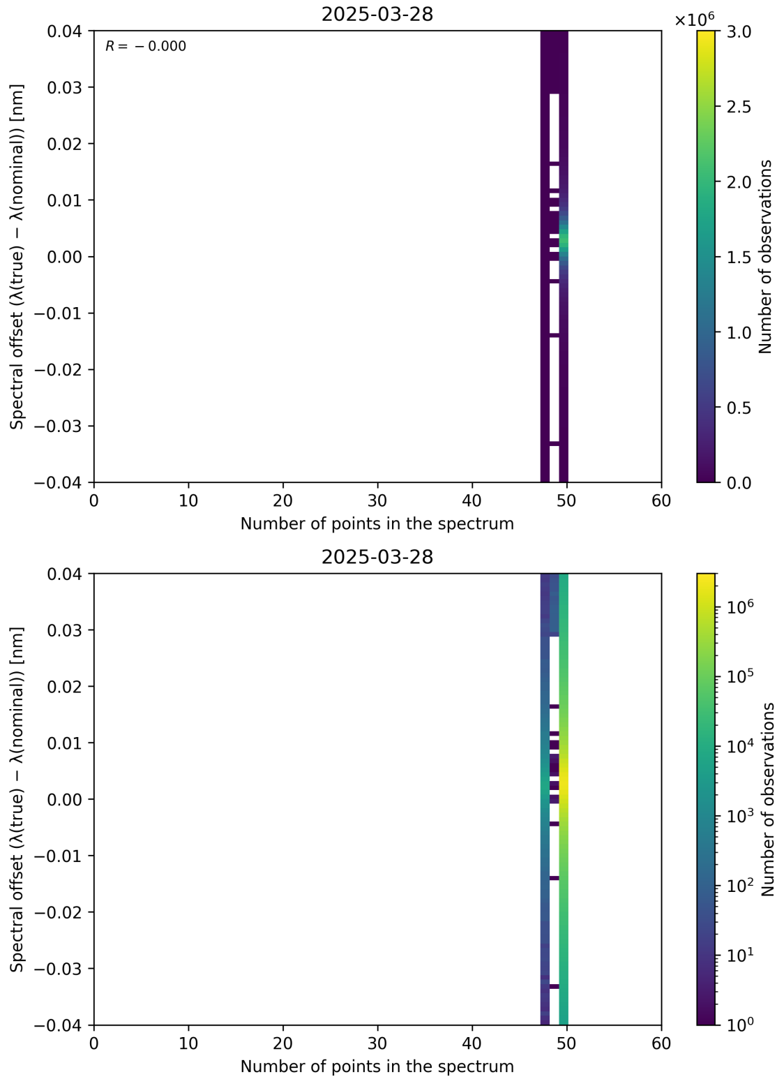
Figure 101: Scatter density plot of “Number of points in the spectrum” against “Spectral offset ( \lambda_{\text{true}} - \lambda_{\text{nominal}} )” for 2025-03-28 to 2025-03-29.
