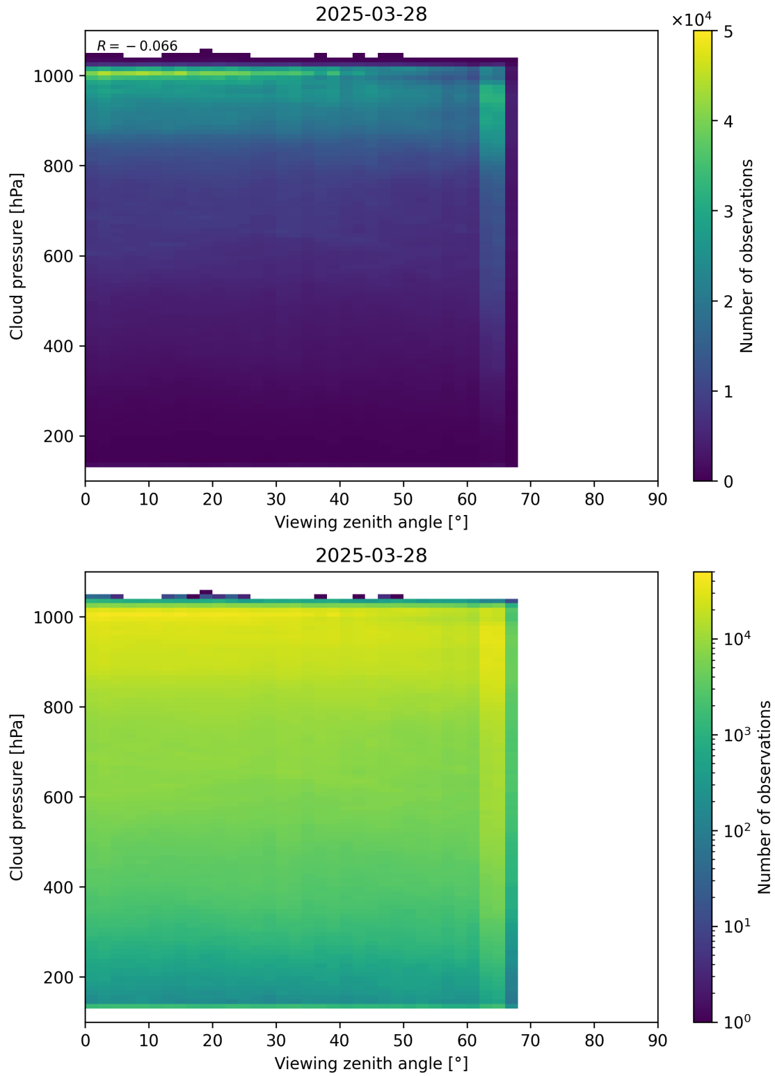
Figure 121: Scatter density plot of “Viewing zenith angle” against “Cloud pressure” for 2025-03-28 to 2025-03-29.
