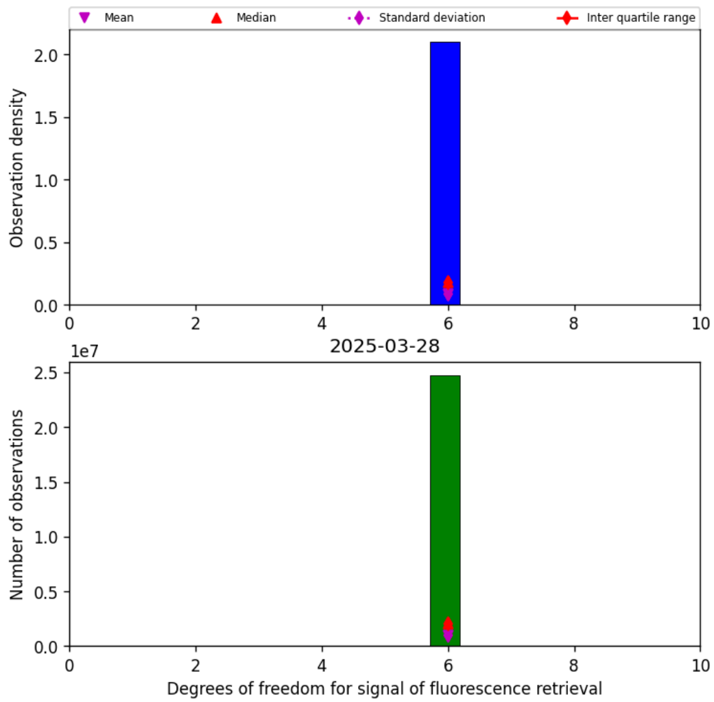
Figure 43: Histogram of “Degrees of freedom for signal of fluorescence retrieval” for 2025-03-28 to 2025-03-29
