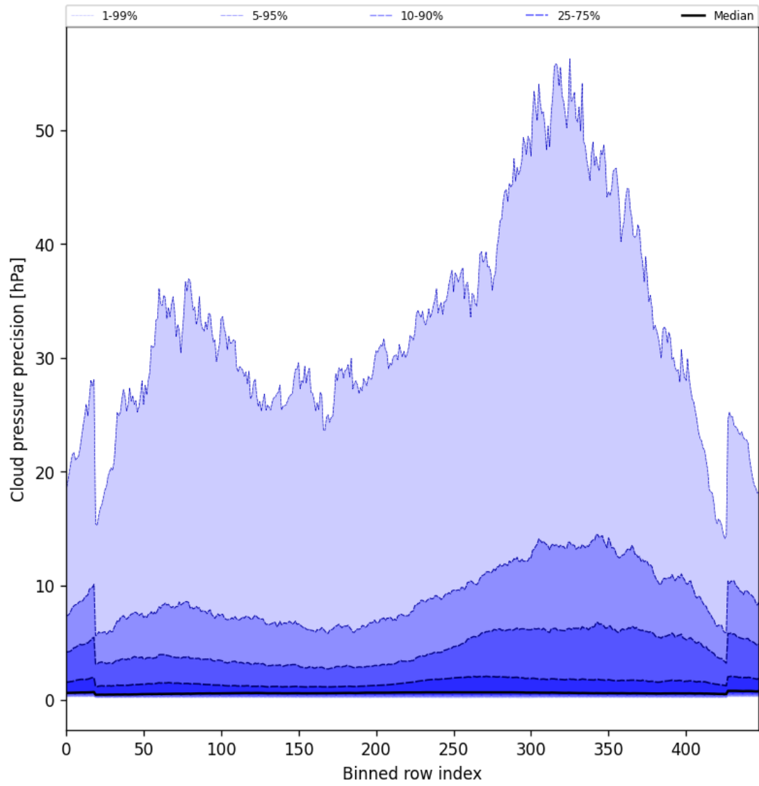
Figure 48: Along track statistics of “Cloud pressure precision” for 2025-03-28 to 2025-03-29
