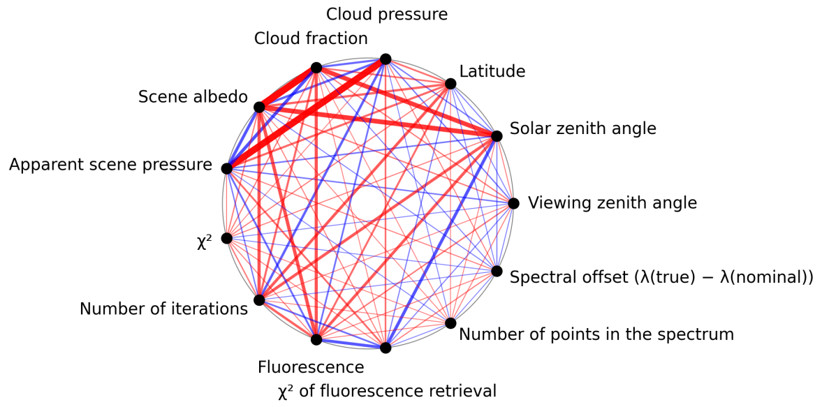
Figure 1: Map of correlation graph for 2025-03-28 to 2025-03-29.
