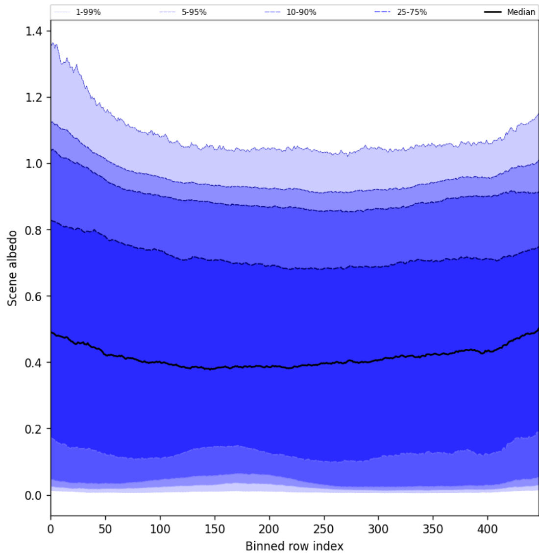
Figure 51: Along track statistics of “Scene albedo” for 2025-03-28 to 2025-03-29
