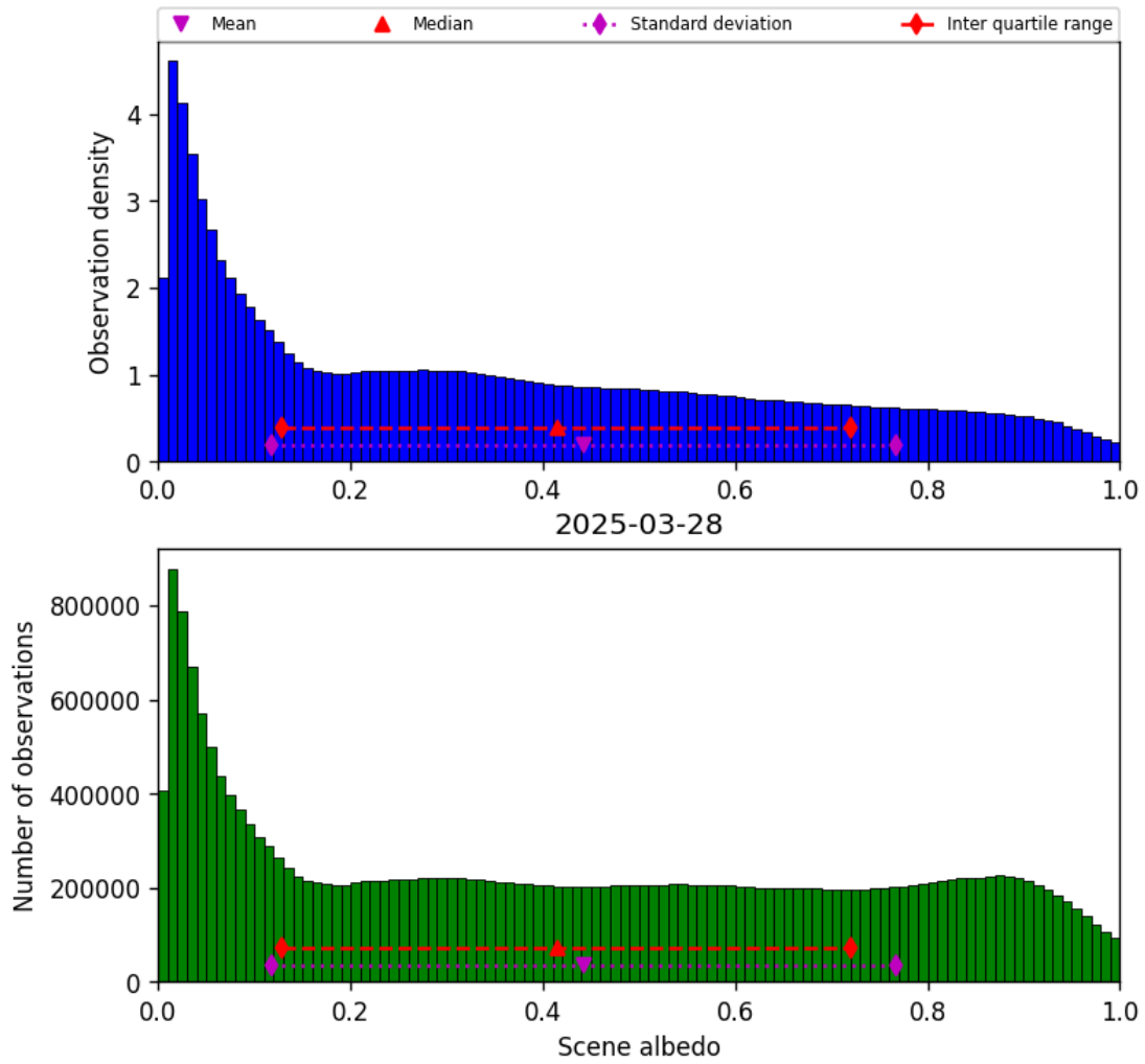
Figure 34: Histogram of “Scene albedo” for 2025-03-28 to 2025-03-29
