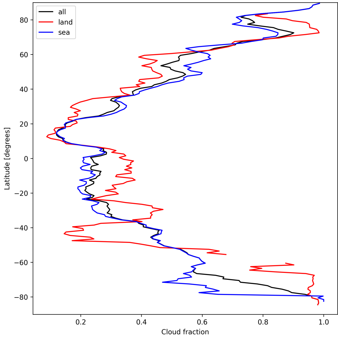
Figure 15: Zonal average of “Cloud fraction” for 2025-03-28 to 2025-03-29.
