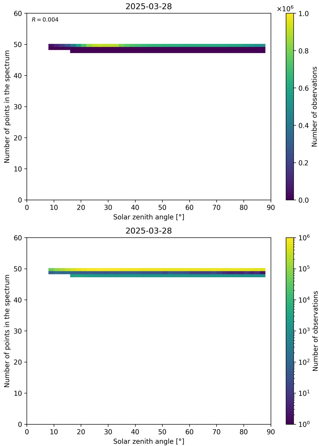
Figure 115: Scatter density plot of “Solar zenith angle” against “Number of points in the spectrum” for 2025-03-28 to 2025-03-29.
