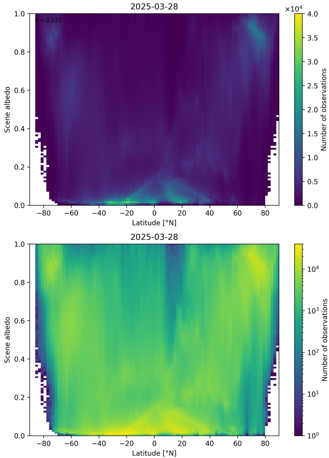
Figure 95: Scatter density plot of “Latitude” against “Scene albedo” for 2025-03-28 to 2025-03-29.
