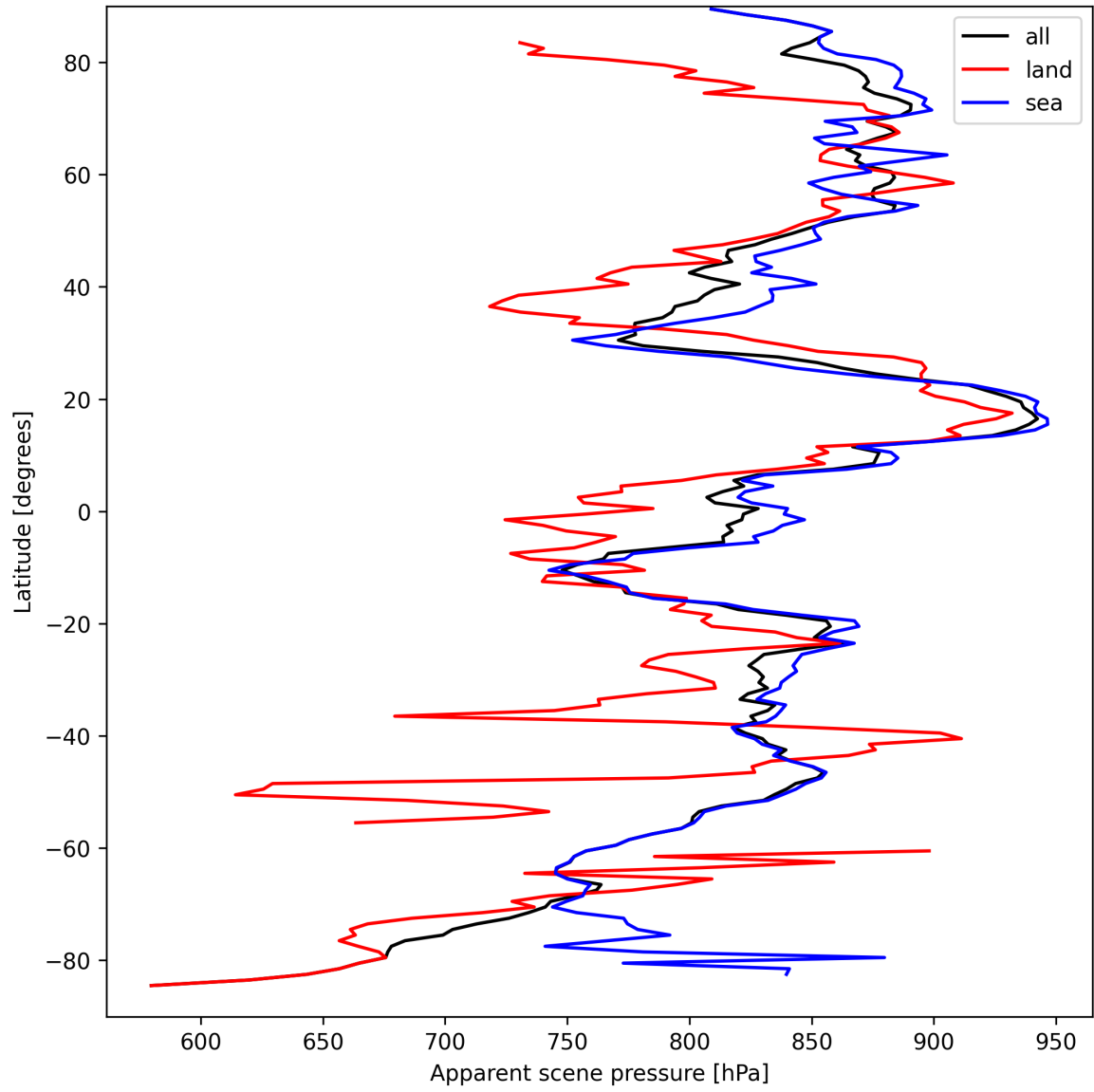
Figure 19: Zonal average of “Apparent scene pressure” for 2025-03-28 to 2025-03-29.
