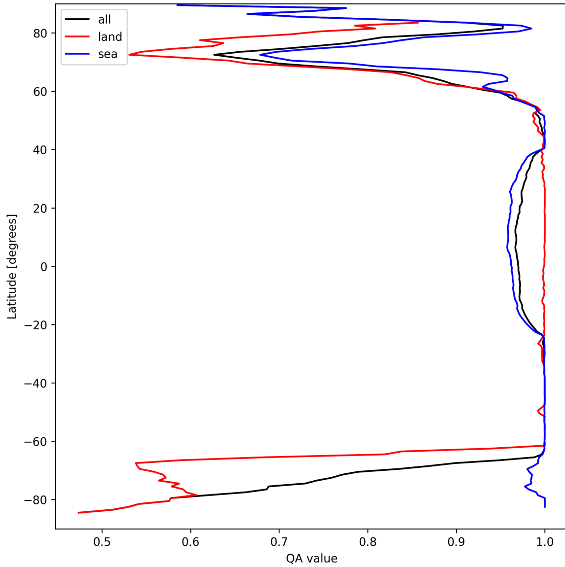
Figure 12: Zonal average of “QA value” for 2025-03-28 to 2025-03-29.
