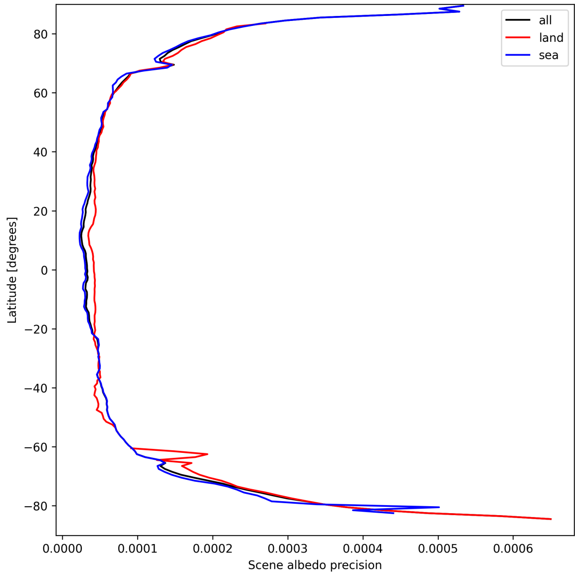
Figure 18: Zonal average of “Scene albedo precision” for 2025-03-28 to 2025-03-29.
