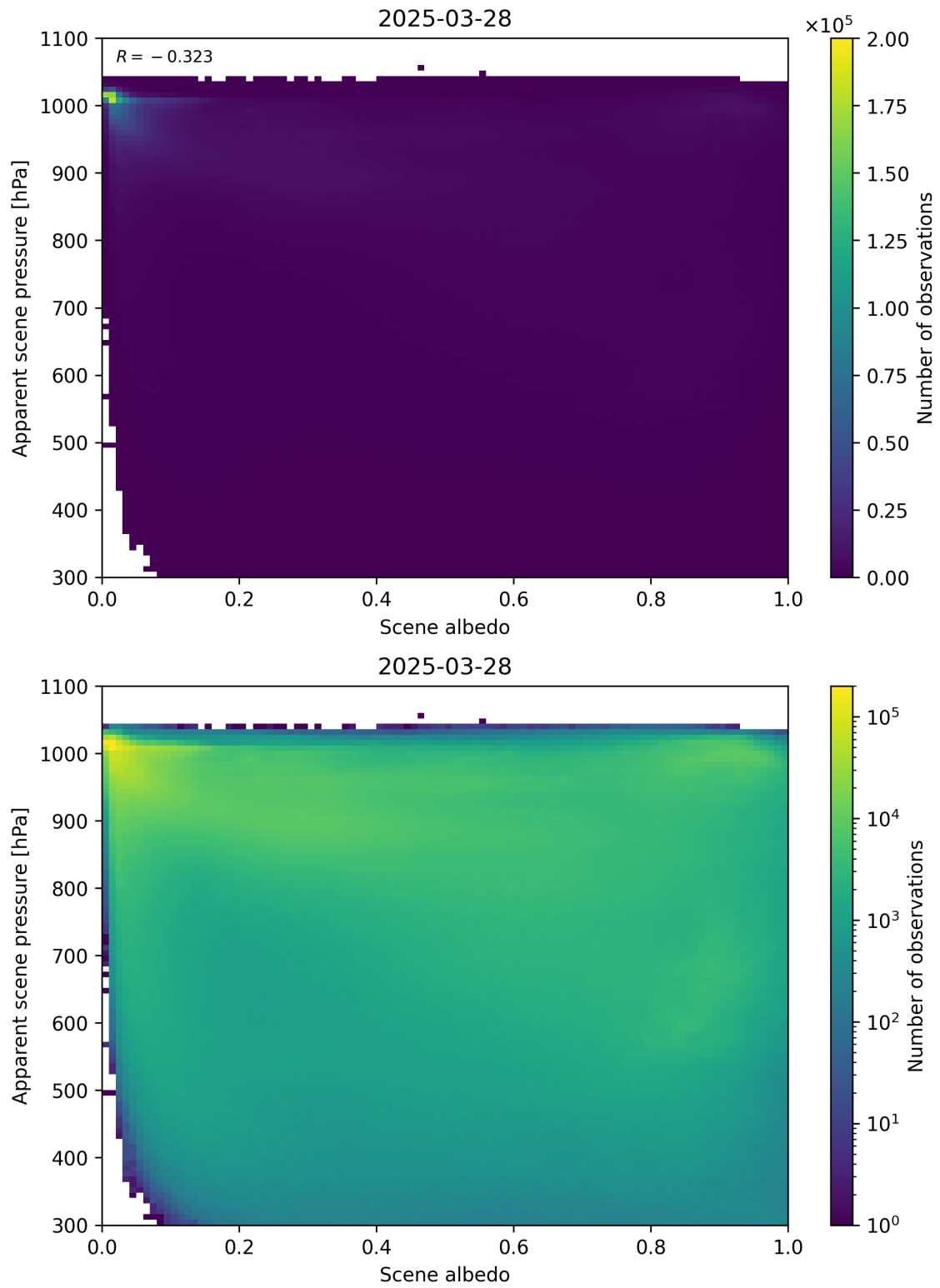
Figure 102: Scatter density plot of “Scene albedo” against “Apparent scene pressure” for 2025-03-28 to 2025-03-29.
