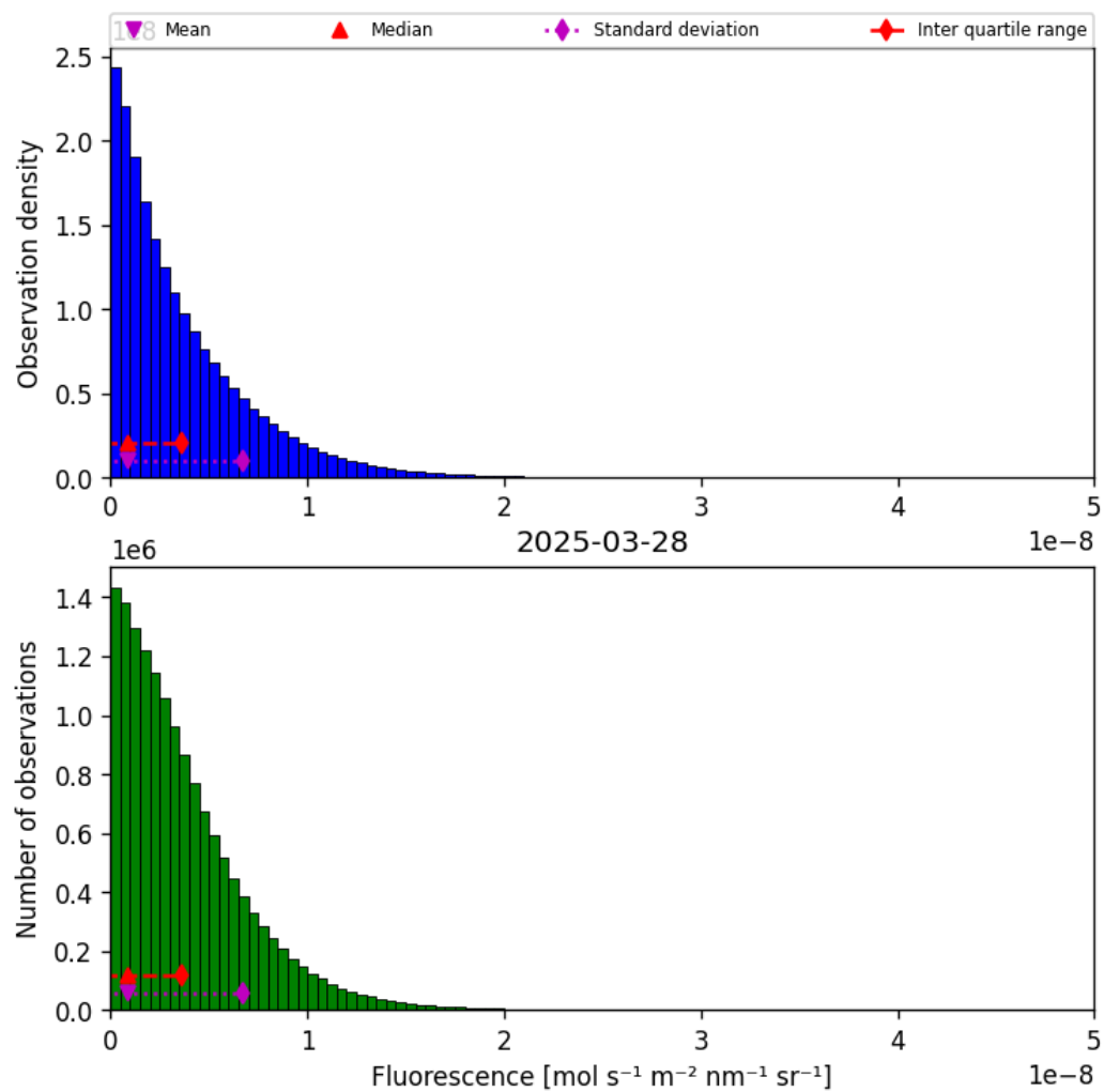
Figure 40: Histogram of “Fluorescence” for 2025-03-28 to 2025-03-29
