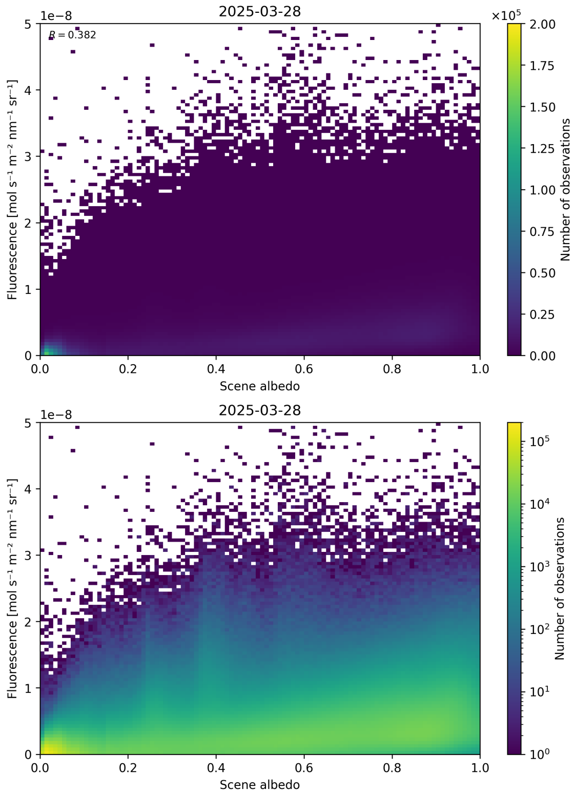
Figure 104: Scatter density plot of “Scene albedo” against “Fluorescence” for 2025-03-28 to 2025-03-29.
