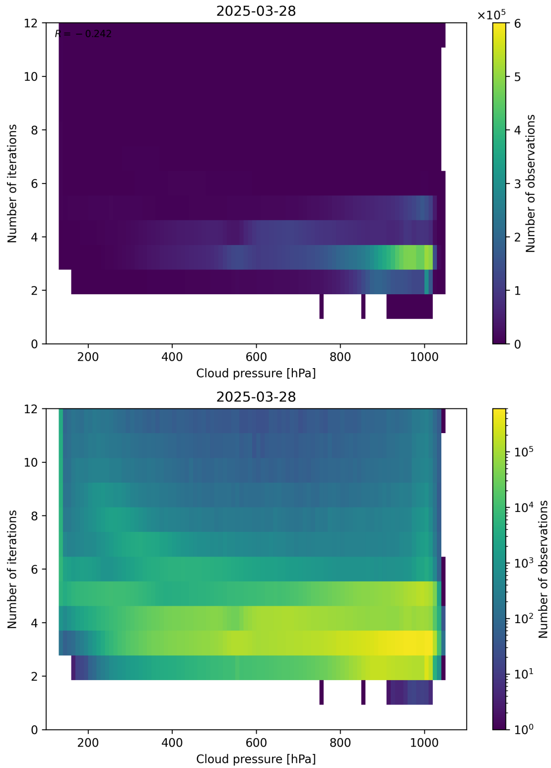
Figure 81: Scatter density plot of “Cloud pressure” against “Number of iterations” for 2025-03-28 to 2025-03-29.
