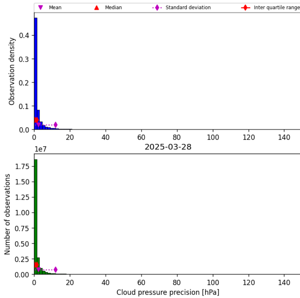
Figure 31: Histogram of “Cloud pressure precision” for 2025-03-28 to 2025-03-29
