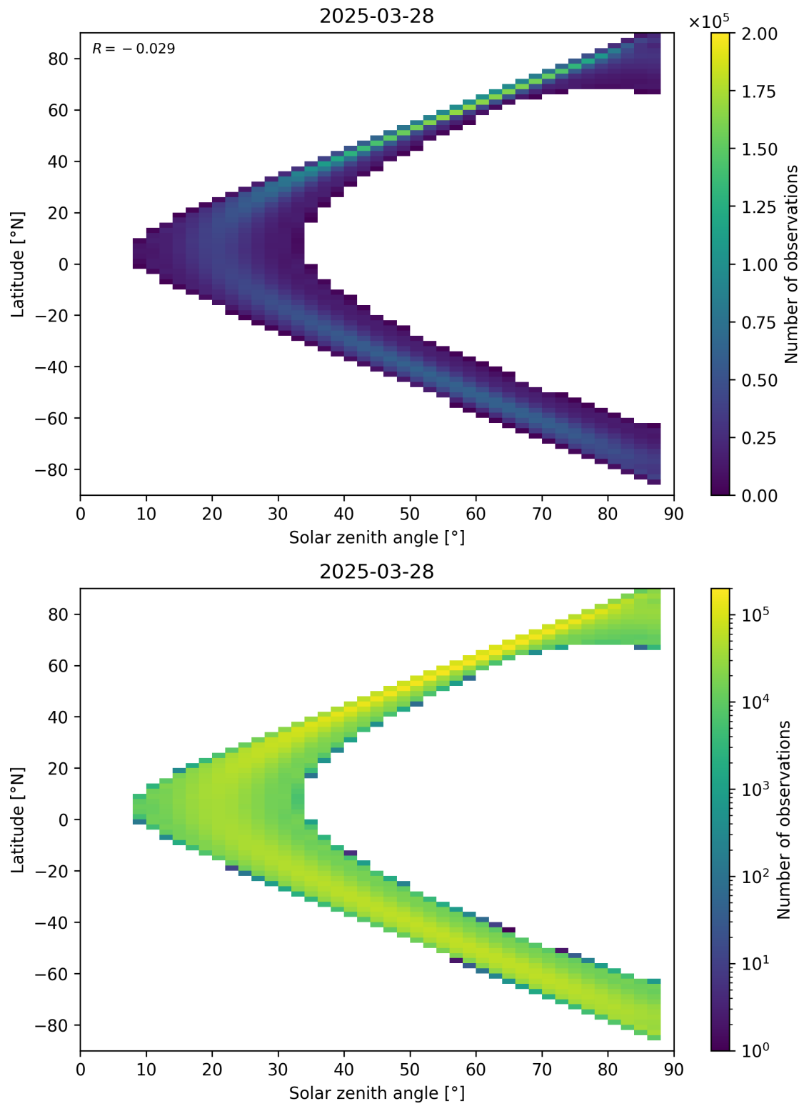
Figure 113: Scatter density plot of “Solar zenith angle” against “Latitude” for 2025-03-28 to 2025-03-29.
