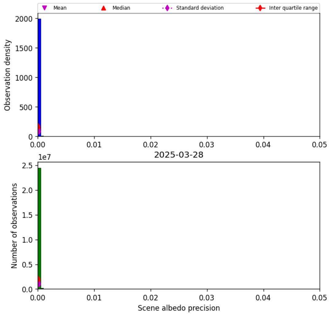
Figure 35: Histogram of “Scene albedo precision” for 2025-03-28 to 2025-03-29
