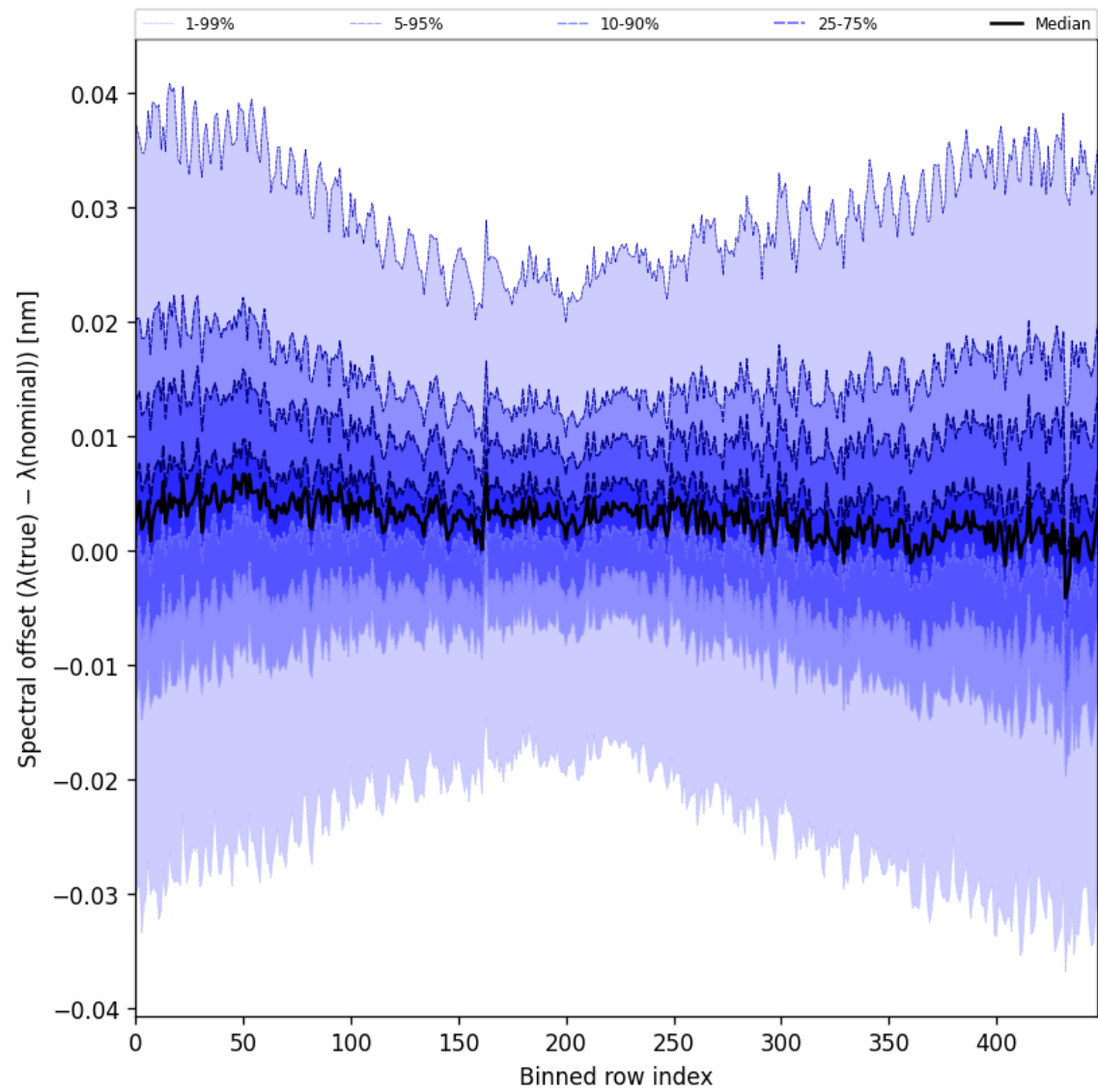
Figure 62: Along track statistics of “Spectral offset ( \lambda_{\text{true}} - \lambda_{\text{nominal}} )” for 2025-03-28 to 2025-03-29
