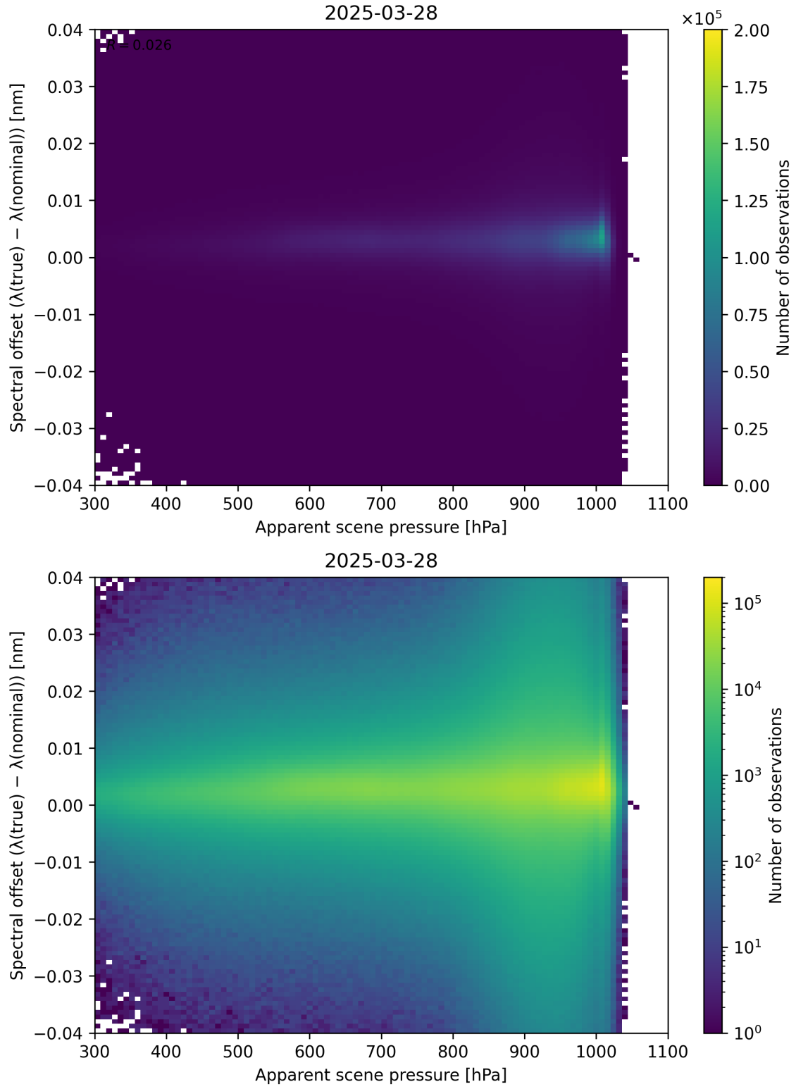
Figure 67: Scatter density plot of “Apparent scene pressure” against “Spectral offset ( \lambda_{\text{true}} - \lambda_{\text{nominal}} )” for 2025-03-28 to 2025-03-29.
