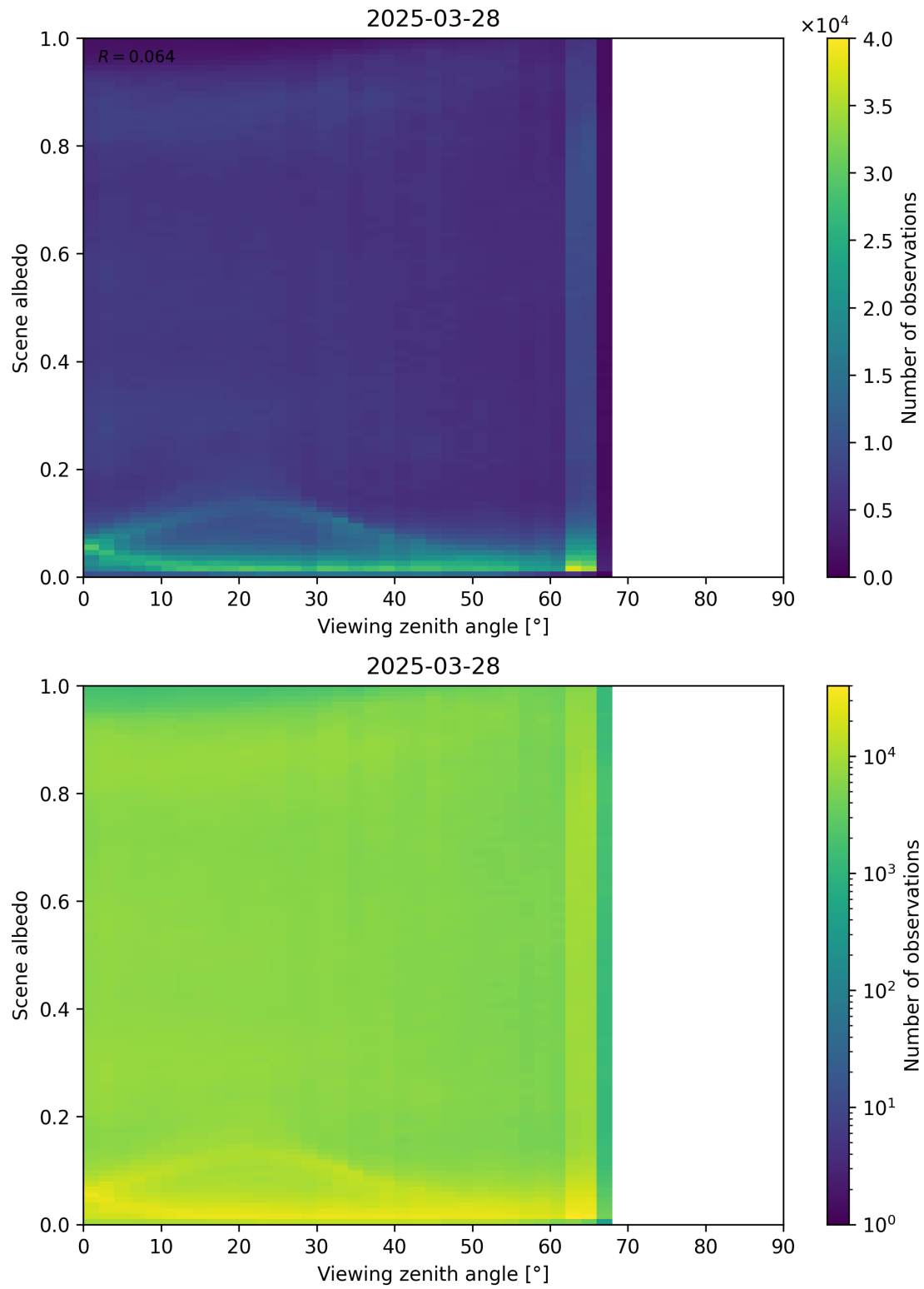
Figure 126: Scatter density plot of “Viewing zenith angle” against “Scene albedo” for 2025-03-28 to 2025-03-29.
