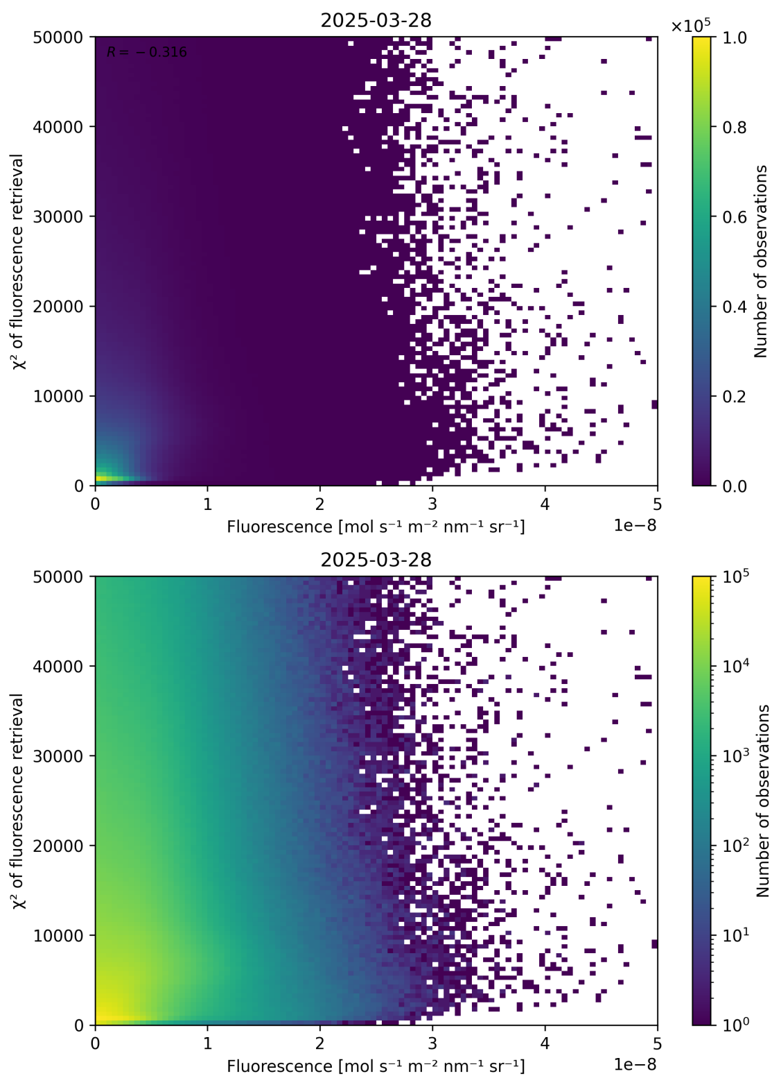
Figure 85: Scatter density plot of “Fluorescence” against “ \chi^2 of fluorescence retrieval” for 2025-03-28 to 2025-03-29.
