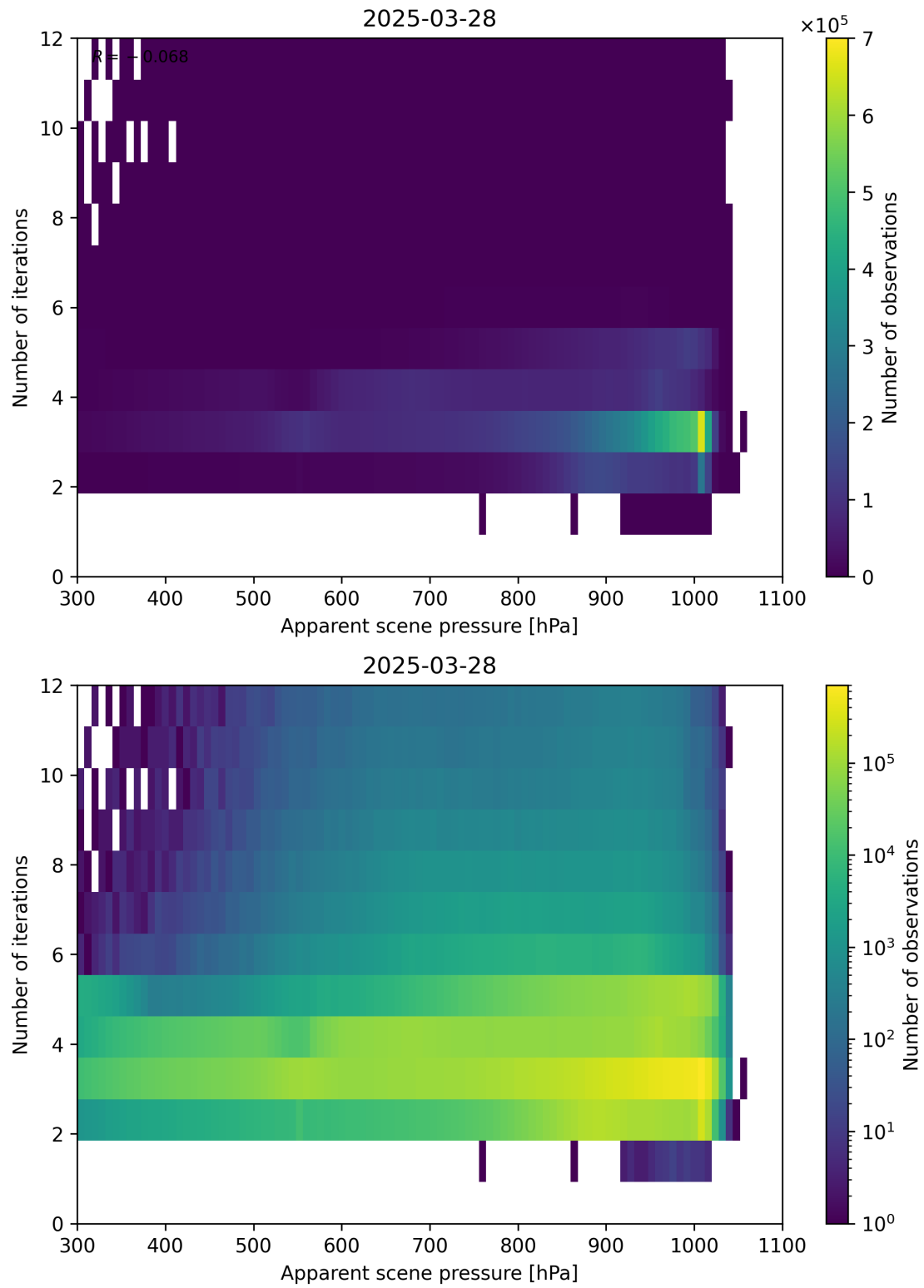
Figure 65: Scatter density plot of “Apparent scene pressure” against “Number of iterations” for 2025-03-28 to 2025-03-29.
