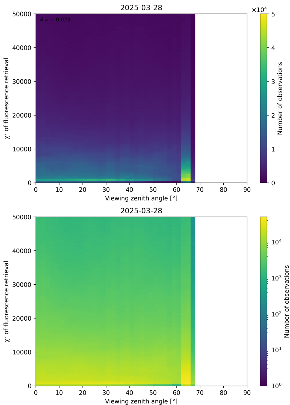
Figure 119: Scatter density plot of “Viewing zenith angle” against “ \chi^2 of fluorescence retrieval” for 2025-03-28 to 2025-03-29.
