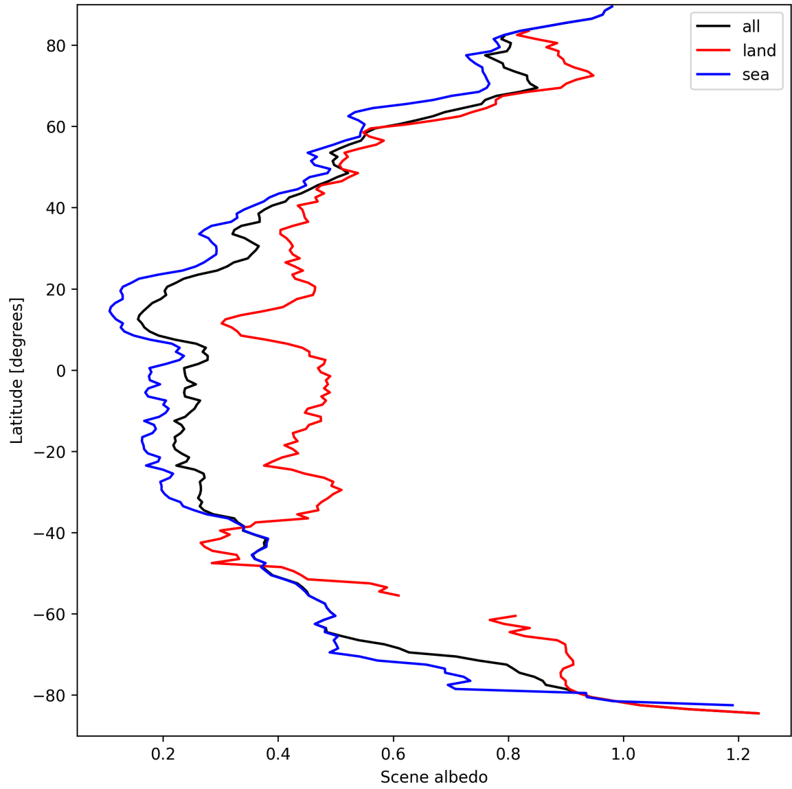
Figure 17: Zonal average of “Scene albedo” for 2025-03-28 to 2025-03-29.
