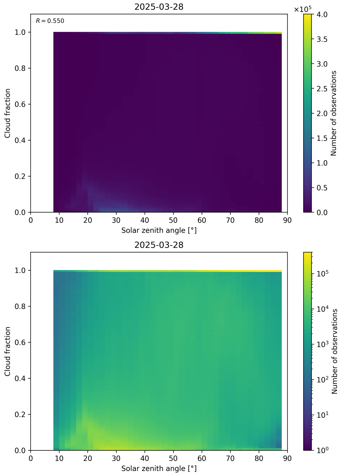
Figure 110: Scatter density plot of “Solar zenith angle” against “Cloud fraction” for 2025-03-28 to 2025-03-29.
