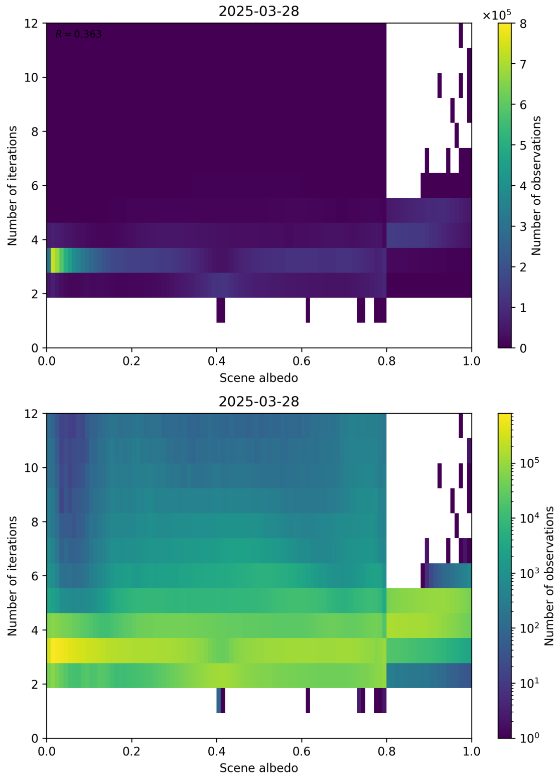
Figure 105: Scatter density plot of “Scene albedo” against “Number of iterations” for 2025-03-28 to 2025-03-29.
