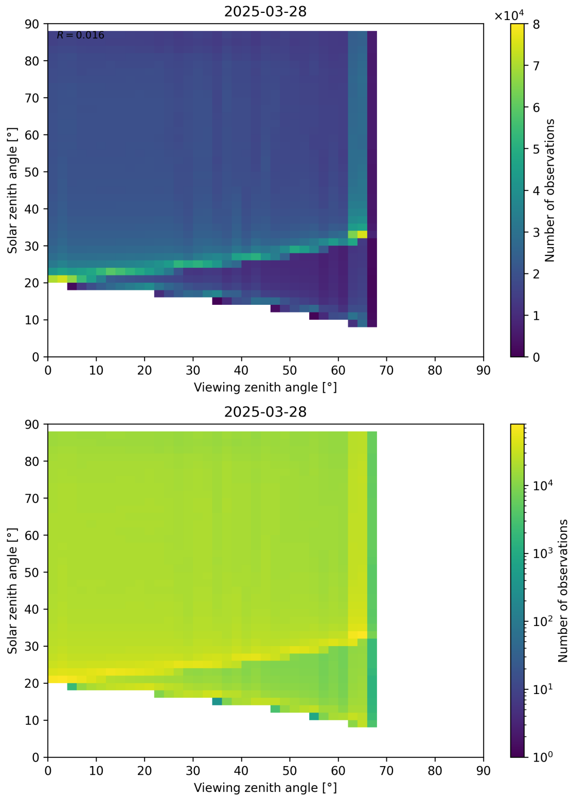
Figure 127: Scatter density plot of “Viewing zenith angle” against “Solar zenith angle” for 2025-03-28 to 2025-03-29.
