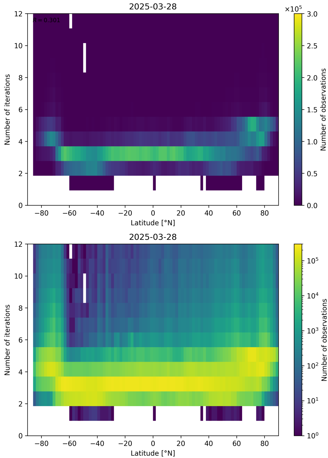
Figure 93: Scatter density plot of “Latitude” against “Number of iterations” for 2025-03-28 to 2025-03-29.
