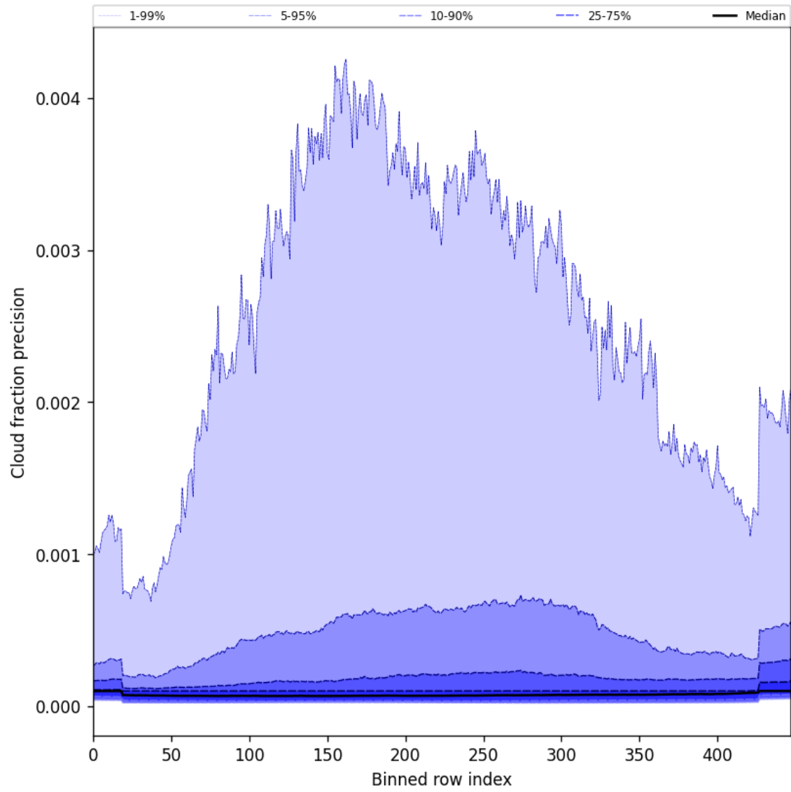
Figure 50: Along track statistics of “Cloud fraction precision” for 2025-03-28 to 2025-03-29
