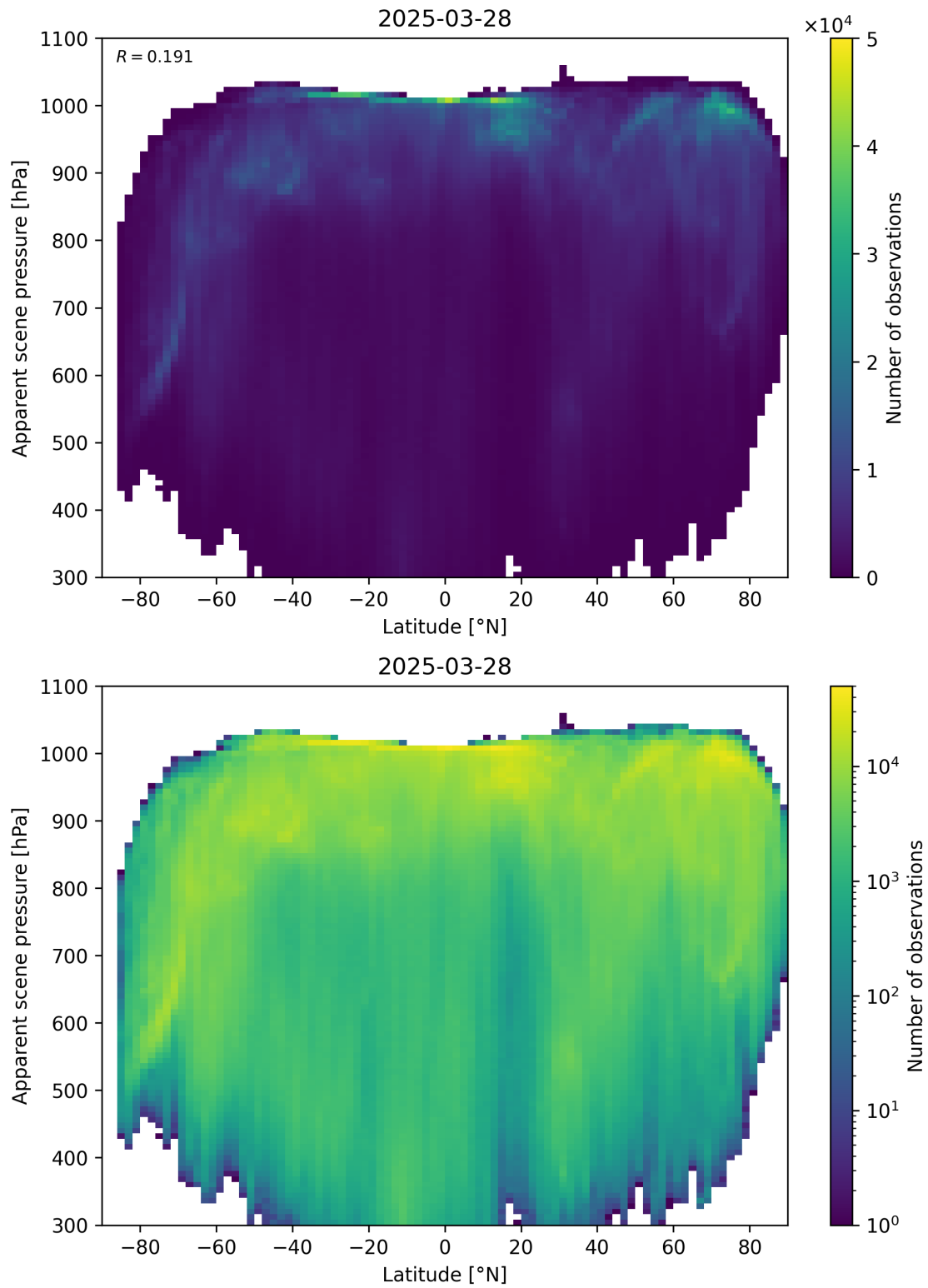
Figure 88: Scatter density plot of “Latitude” against “Apparent scene pressure” for 2025-03-28 to 2025-03-29.
