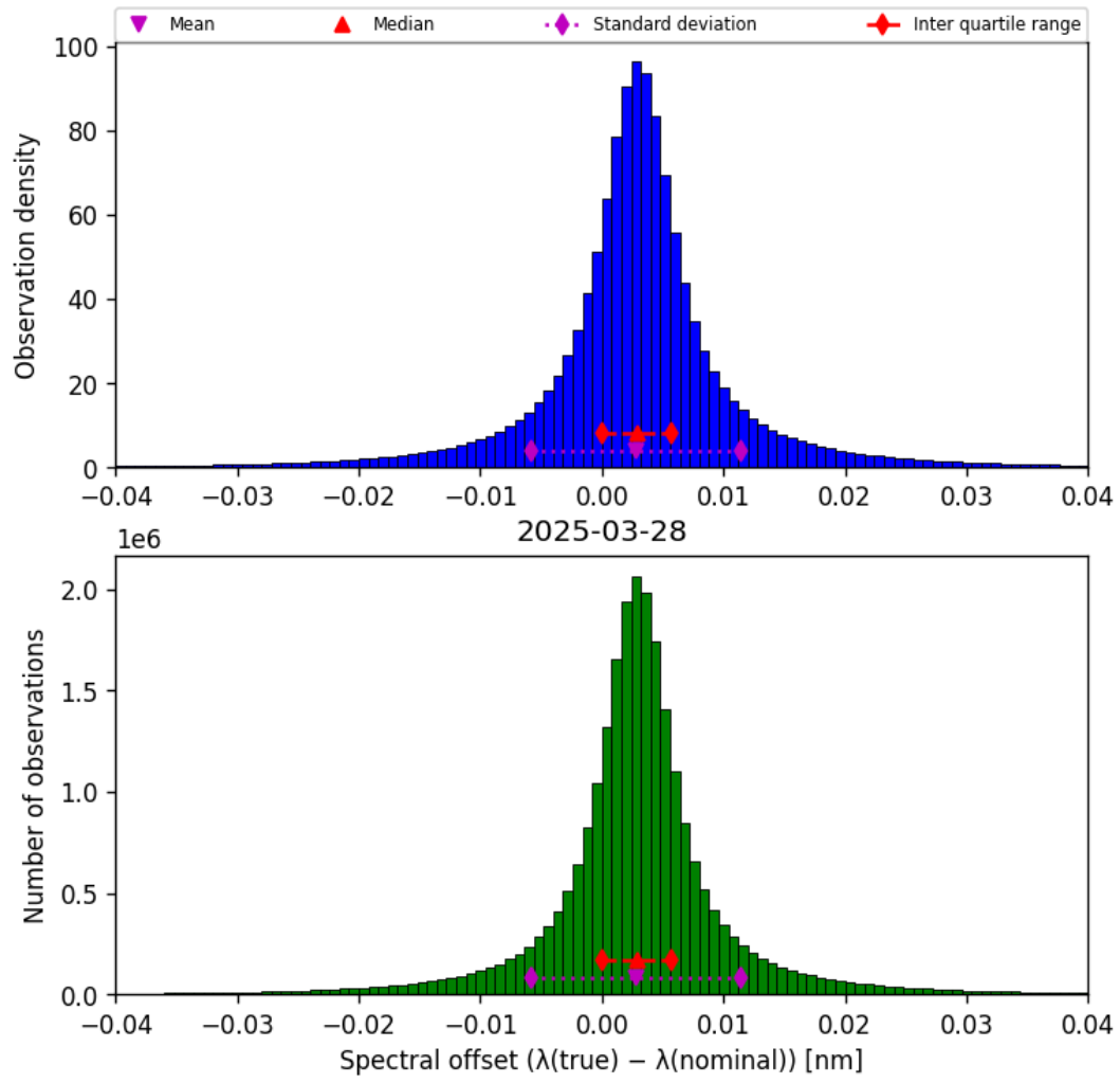
Figure 45: Histogram of “Spectral offset ( \lambda_{\text{true}} - \lambda_{\text{nominal}} )” for 2025-03-28 to 2025-03-29
