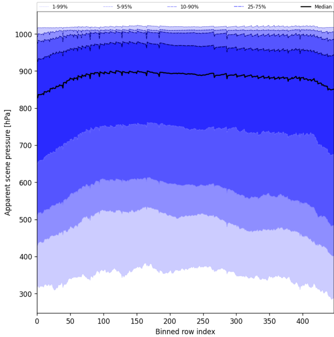
Figure 53: Along track statistics of “Apparent scene pressure” for 2025-03-28 to 2025-03-29
