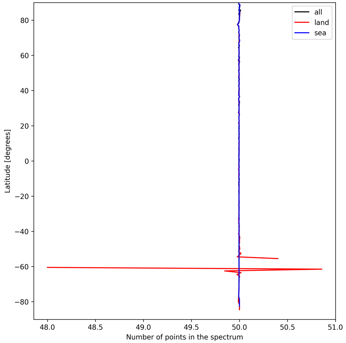
Figure 27: Zonal average of “Number of points in the spectrum” for 2025-03-28 to 2025-03-29.
