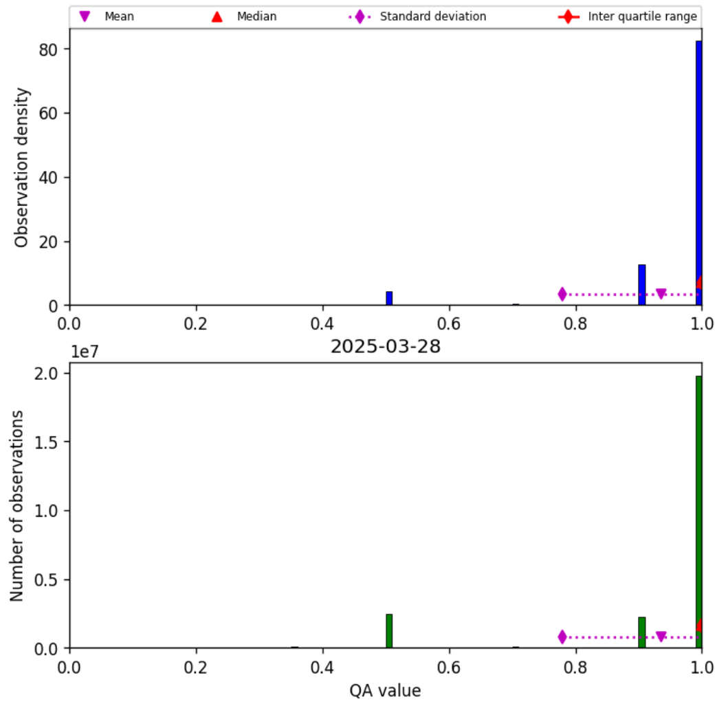
Figure 29: Histogram of “QA value” for 2025-03-28 to 2025-03-29
