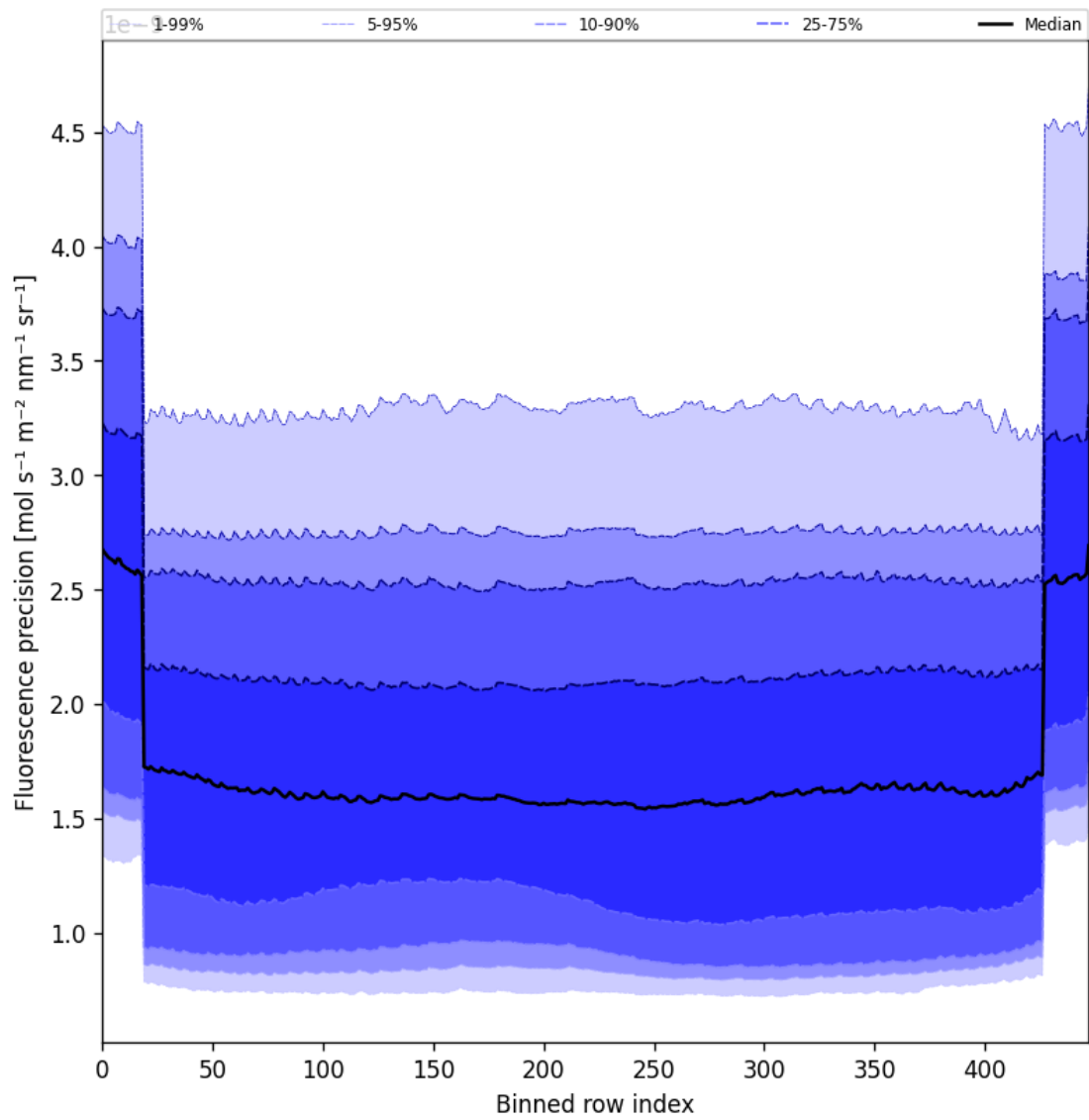
Figure 58: Along track statistics of “Fluorescence precision” for 2025-03-28 to 2025-03-29
