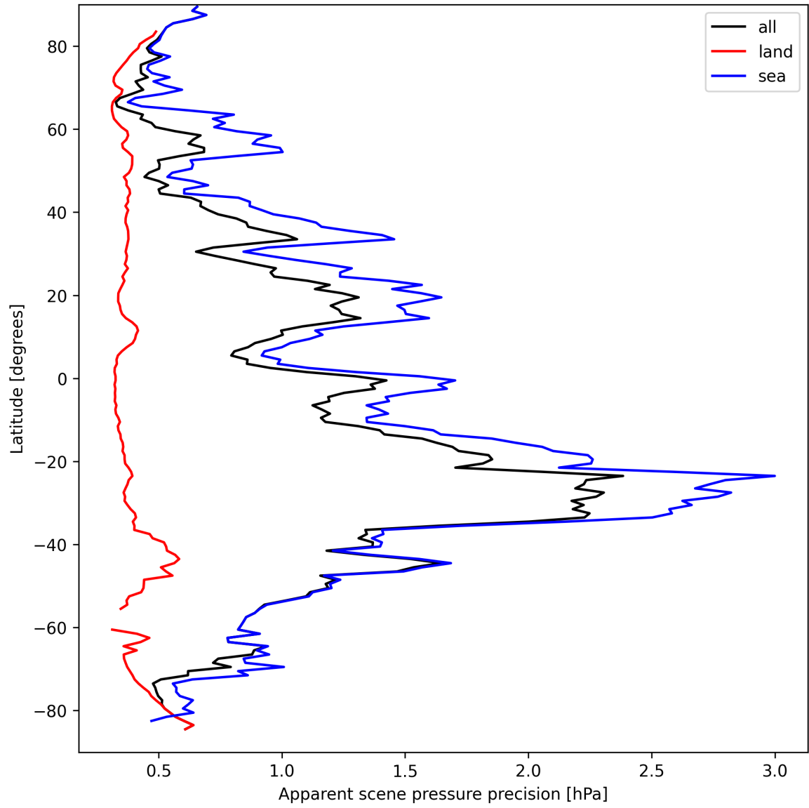
Figure 20: Zonal average of “Apparent scene pressure precision” for 2025-03-28 to 2025-03-29.
