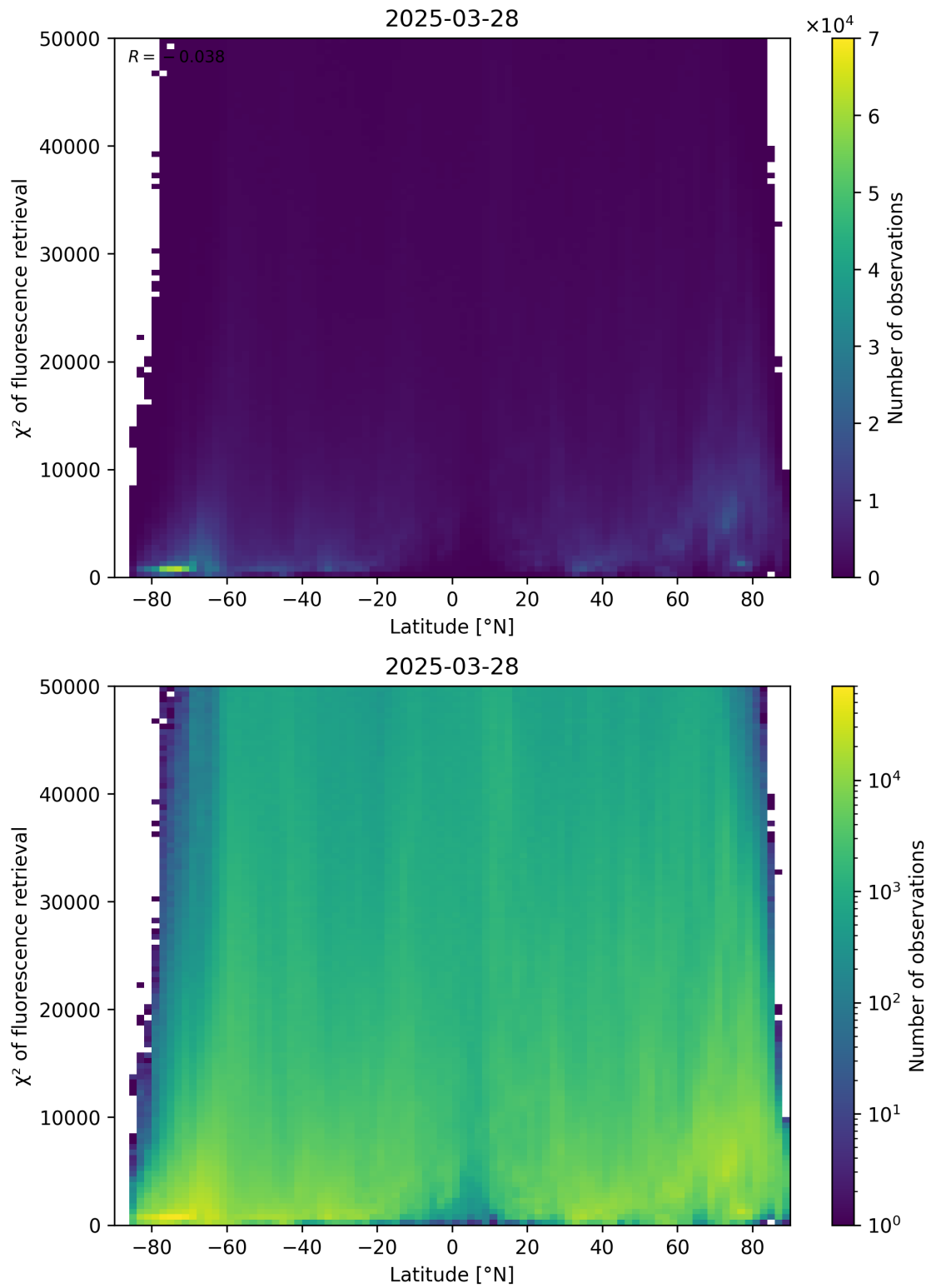
Figure 89: Scatter density plot of “Latitude” against “ \chi^2 of fluorescence retrieval” for 2025-03-28 to 2025-03-29.
