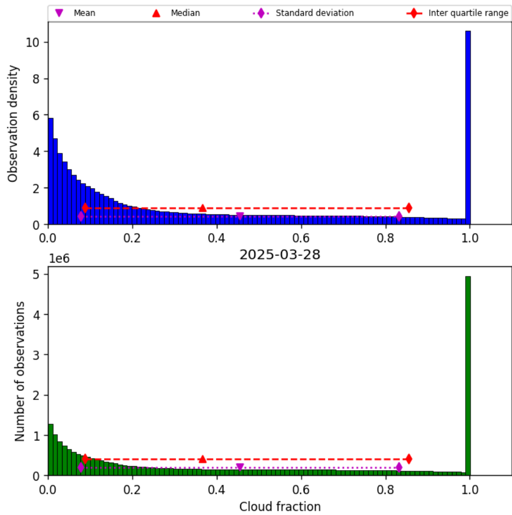
Figure 32: Histogram of “Cloud fraction” for 2025-03-28 to 2025-03-29
