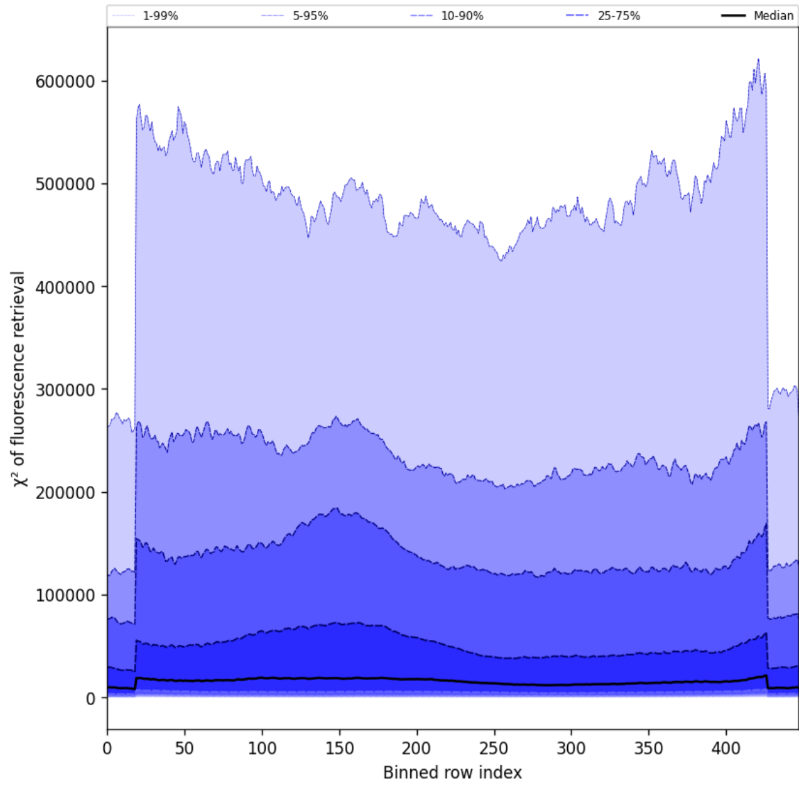
Figure 59: Along track statistics of “ \chi^2 of fluorescence retrieval” for 2025-03-28 to 2025-03-29
