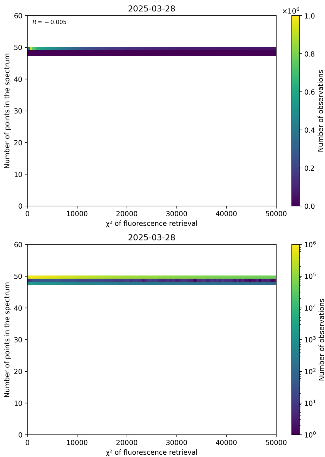
Figure 68: Scatter density plot of " \chi^2 of fluorescence retrieval" against "Number of points in the spectrum" for 2025-03-28 to 2025-03-29.
