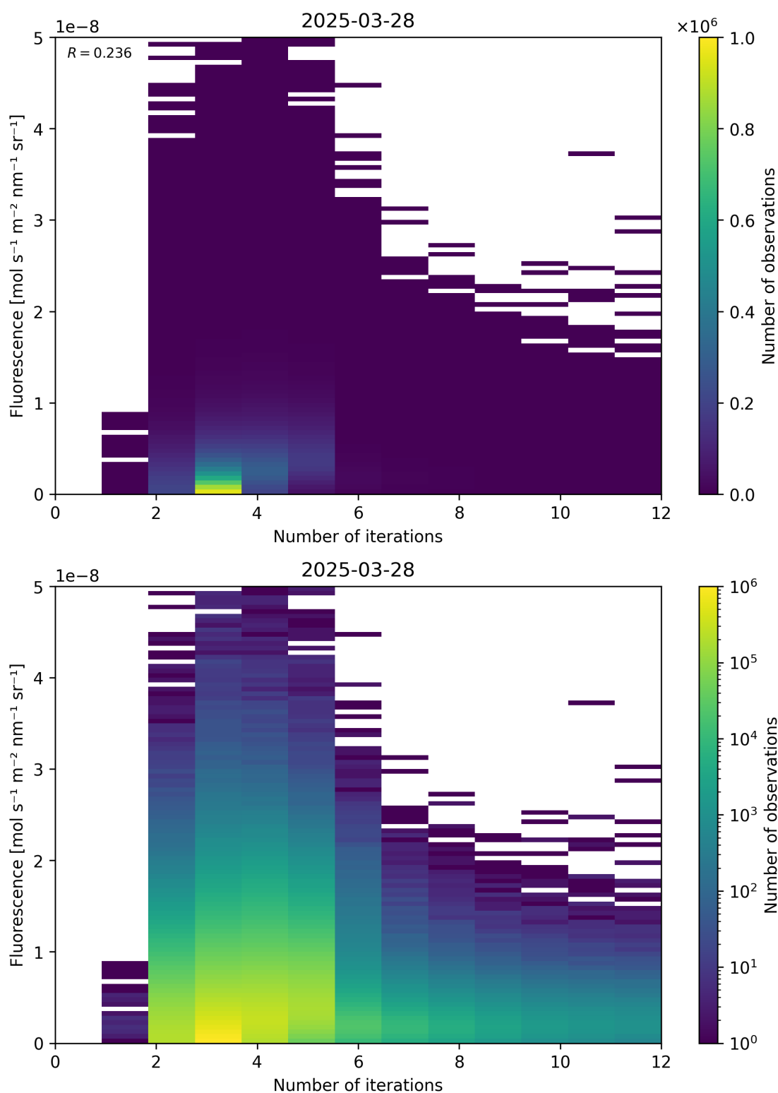
Figure 98: Scatter density plot of “Number of iterations” against “Fluorescence” for 2025-03-28 to 2025-03-29.
