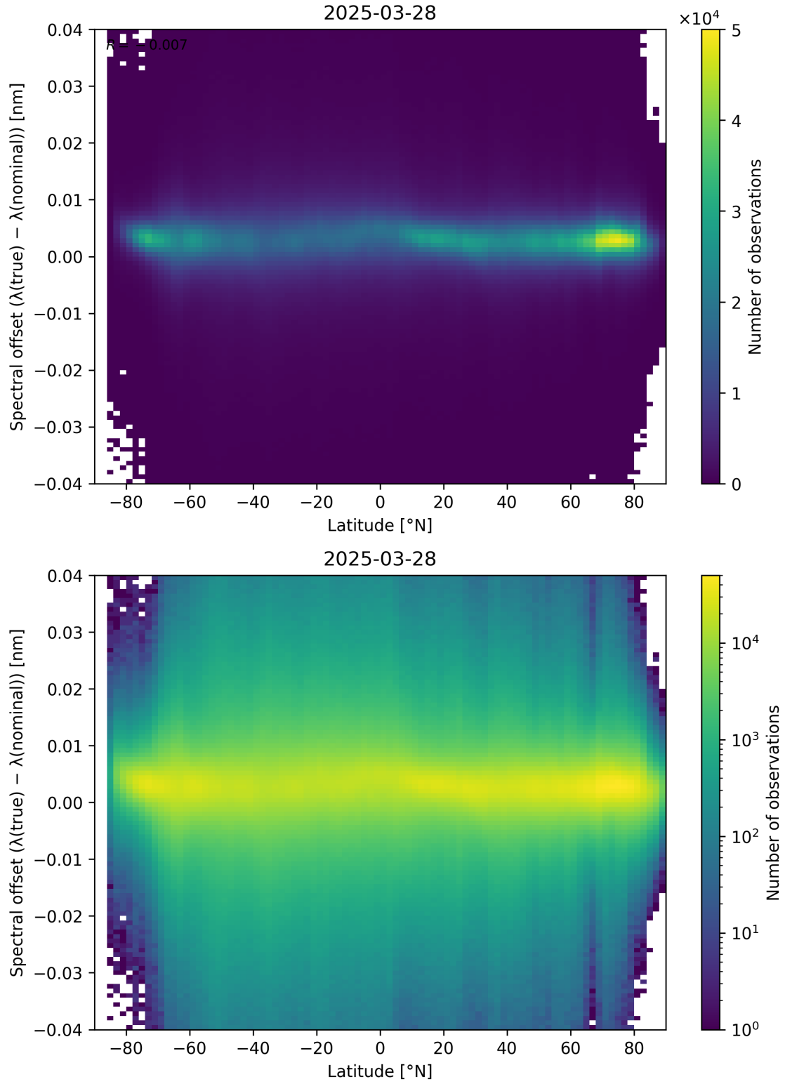
Figure 96: Scatter density plot of “Latitude” against “Spectral offset ( \lambda_{\text{true}} - \lambda_{\text{nominal}} )” for 2025-03-28 to 2025-03-29.
