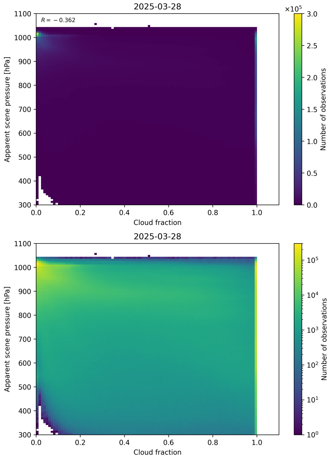
Figure 70: Scatter density plot of “Cloud fraction” against “Apparent scene pressure” for 2025-03-28 to 2025-03-29.
