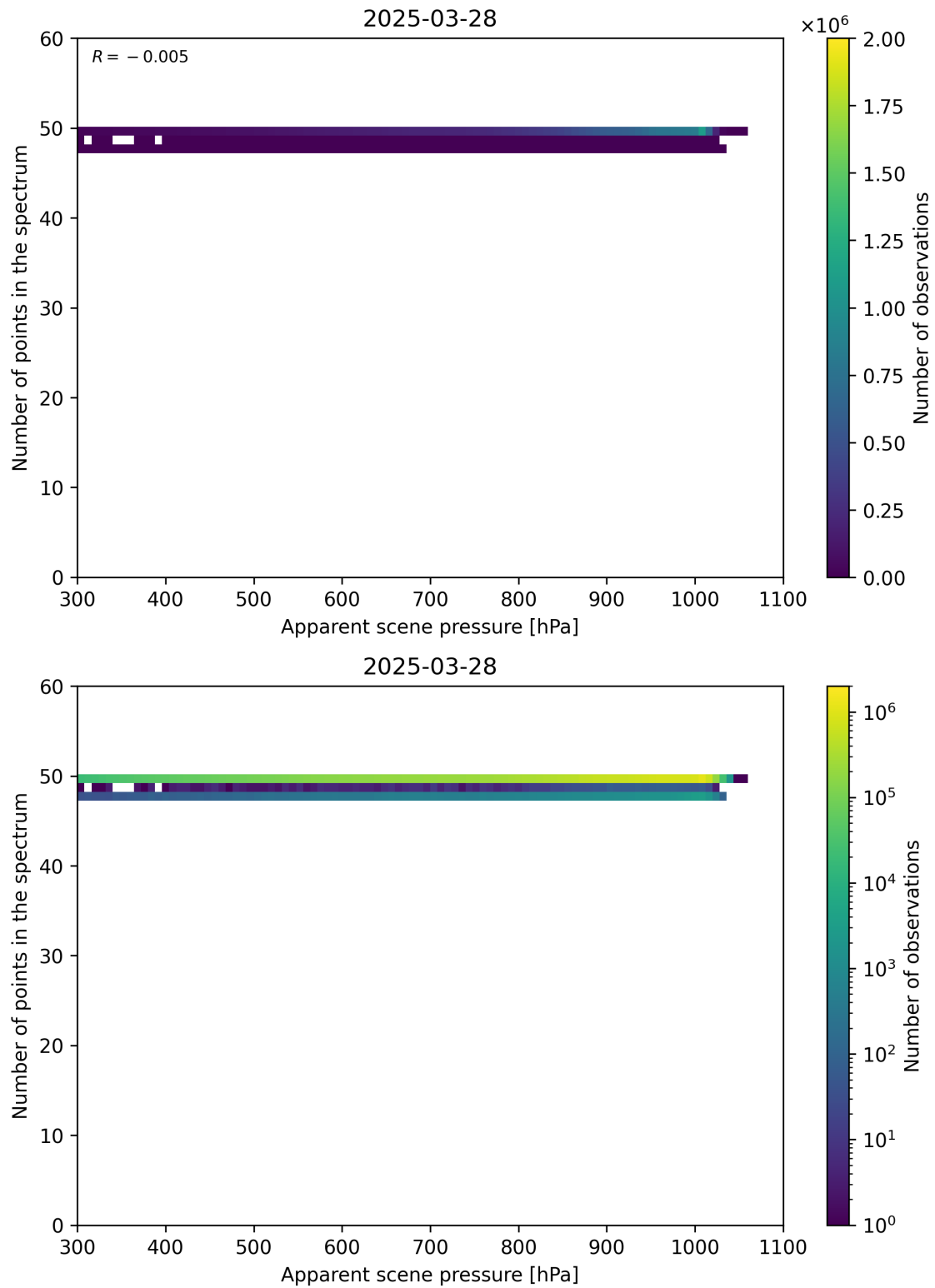
Figure 66: Scatter density plot of “Apparent scene pressure” against “Number of points in the spectrum” for 2025-03-28 to 2025-03-29.
