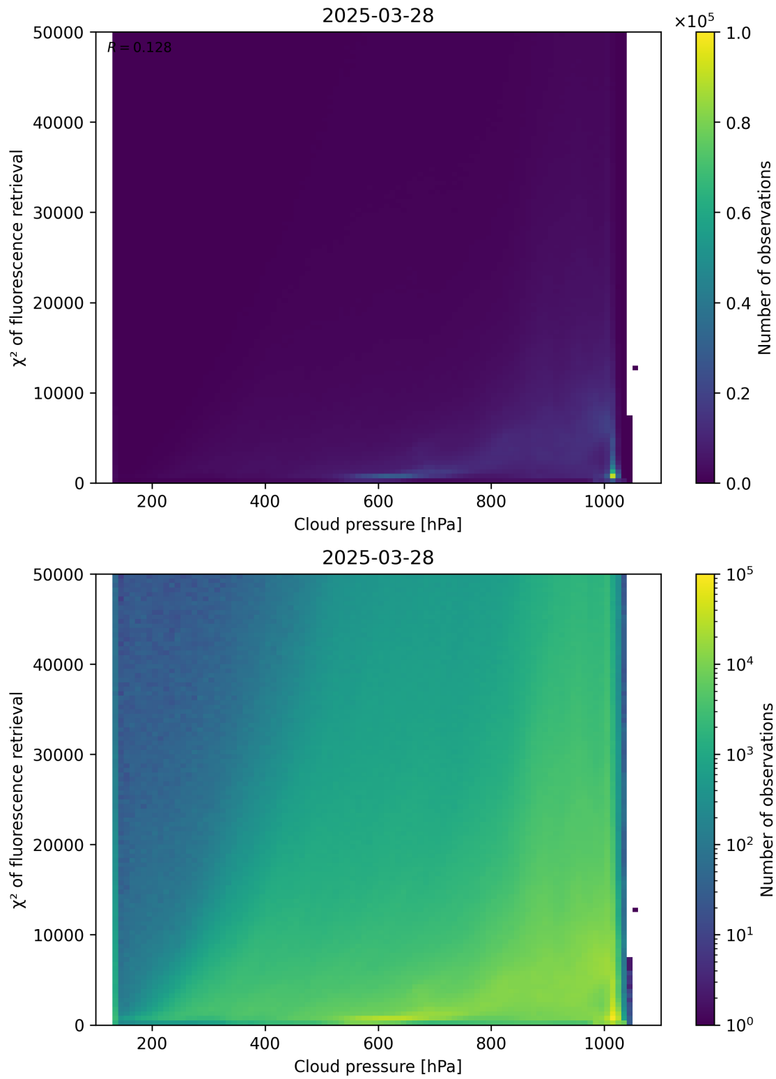
Figure 78: Scatter density plot of “Cloud pressure” against “ \chi^2 of fluorescence retrieval” for 2025-03-28 to 2025-03-29.
