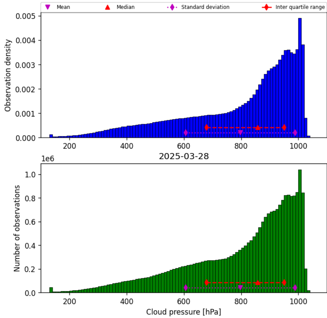
Figure 30: Histogram of “Cloud pressure” for 2025-03-28 to 2025-03-29
