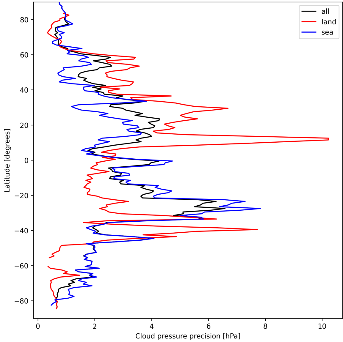
Figure 14: Zonal average of "Cloud pressure precision" for 2025-03-28 to 2025-03-29.
