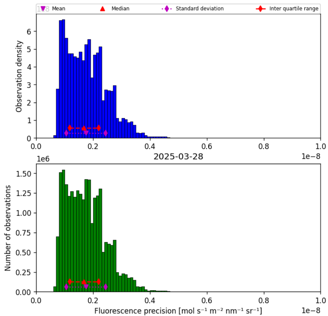
Figure 41: Histogram of “Fluorescence precision” for 2025-03-28 to 2025-03-29
