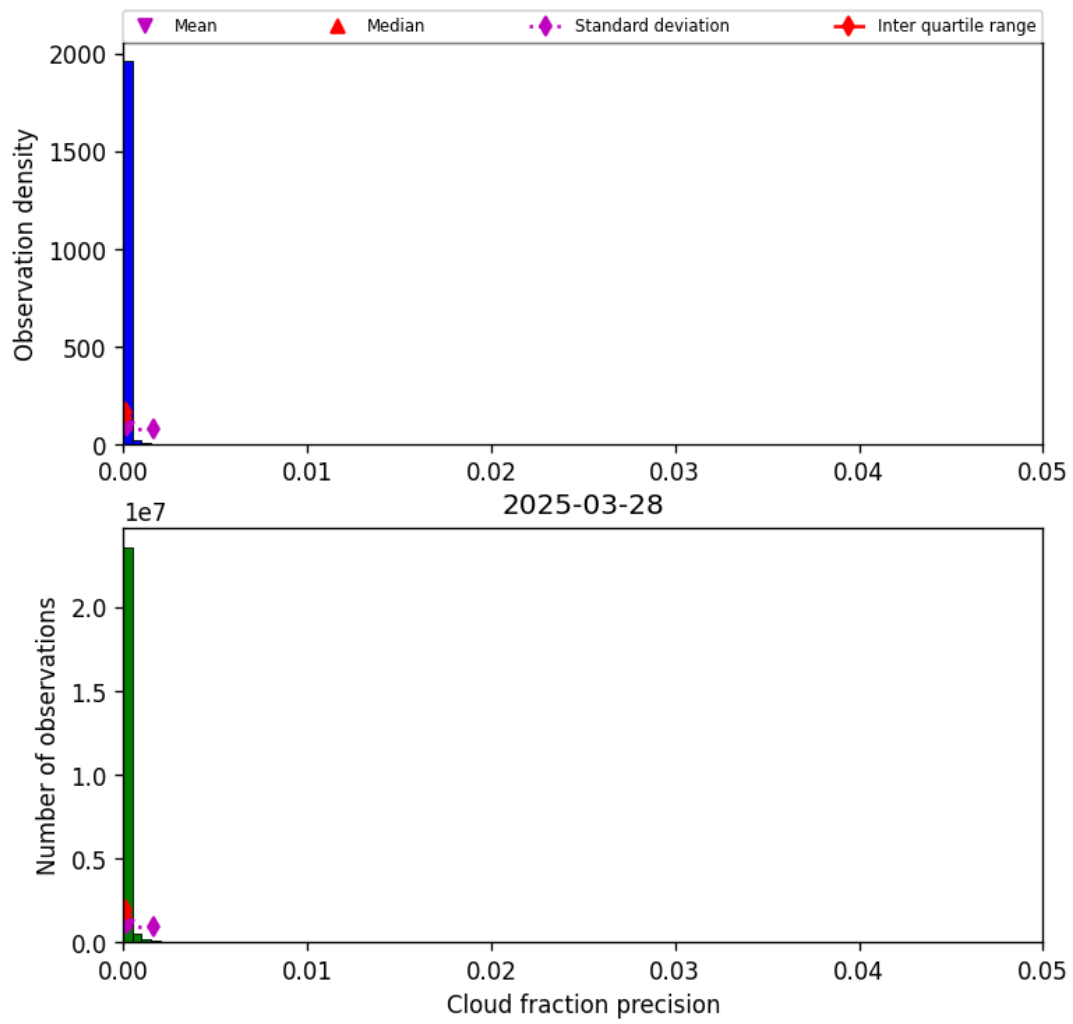
Figure 33: Histogram of “Cloud fraction precision” for 2025-03-28 to 2025-03-29
