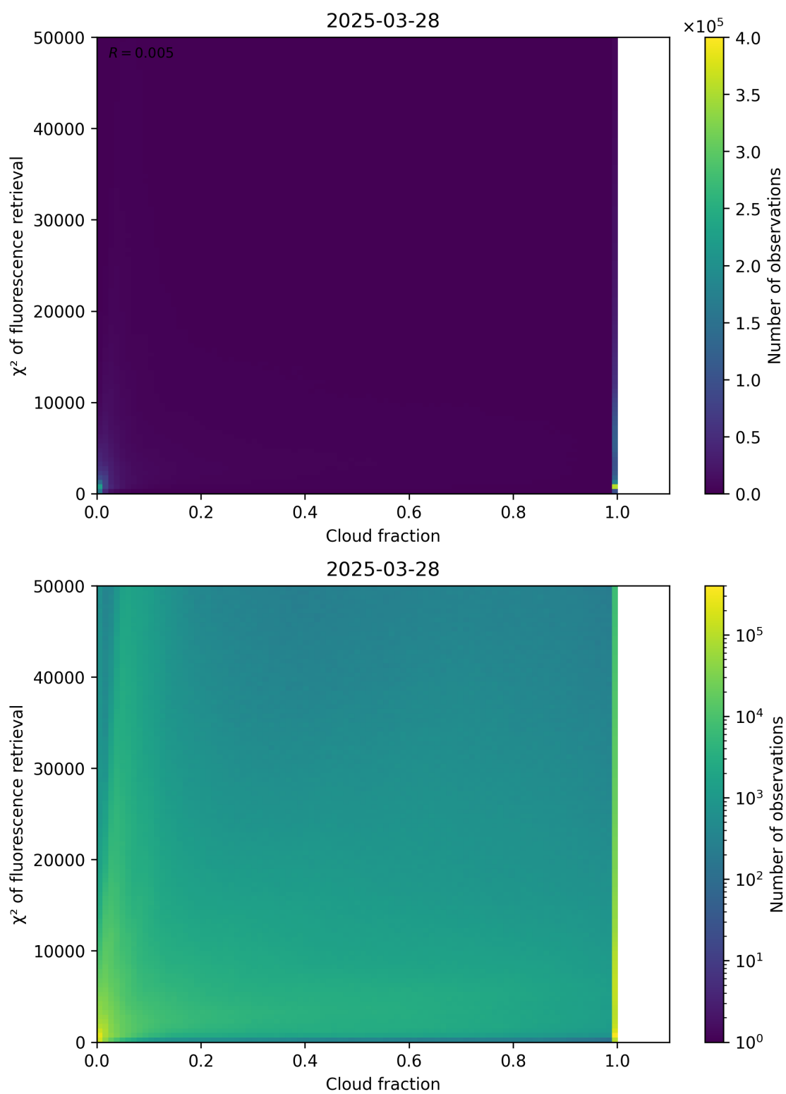
Figure 71: Scatter density plot of “Cloud fraction” against “ \chi^2 of fluorescence retrieval” for 2025-03-28 to 2025-03-29.
