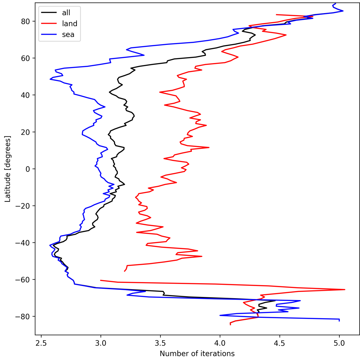
Figure 22: Zonal average of “Number of iterations” for 2025-03-28 to 2025-03-29.
