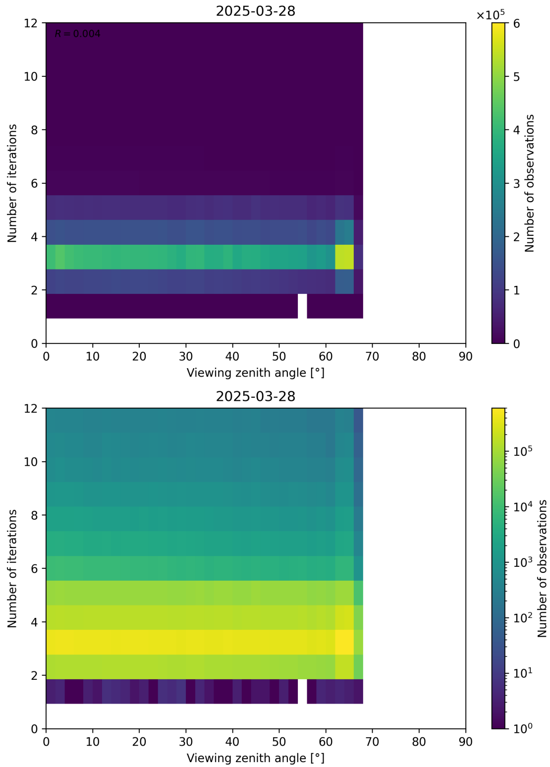
Figure 124: Scatter density plot of “Viewing zenith angle” against “Number of iterations” for 2025-03-28 to 2025-03-29.
