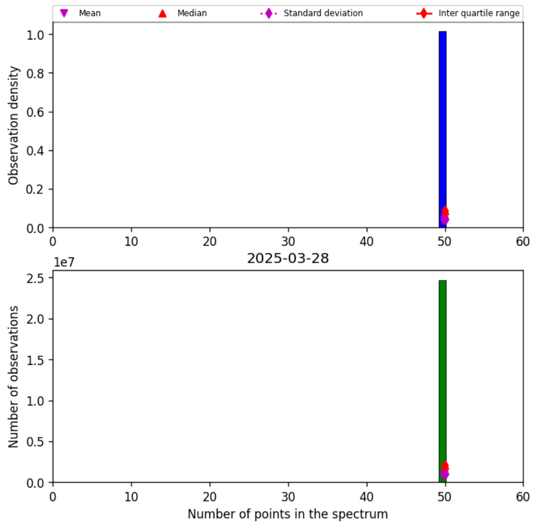
Figure 44: Histogram of “Number of points in the spectrum” for 2025-03-28 to 2025-03-29
