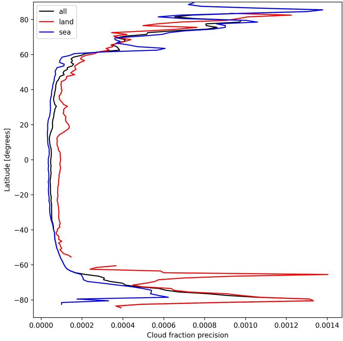
Figure 16: Zonal average of “Cloud fraction precision” for 2025-03-28 to 2025-03-29.
