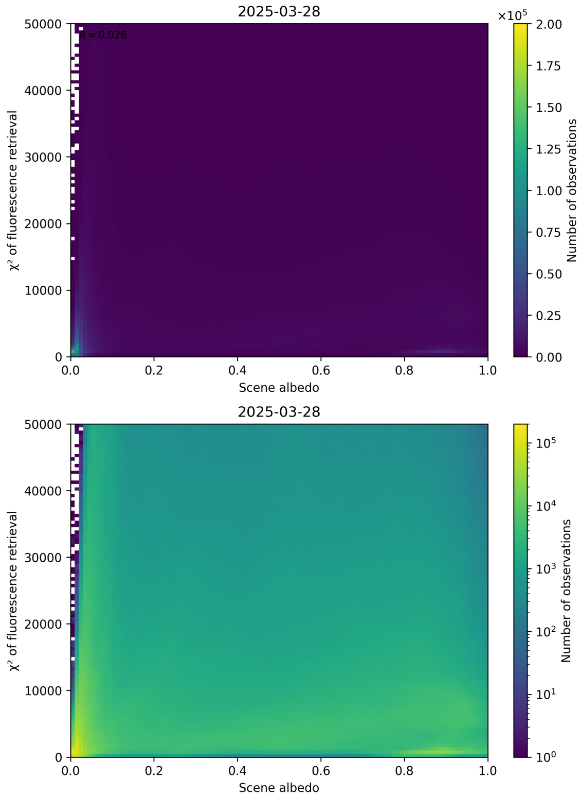
Figure 103: Scatter density plot of “Scene albedo” against “ \chi^2 of fluorescence retrieval” for 2025-03-28 to 2025-03-29.
