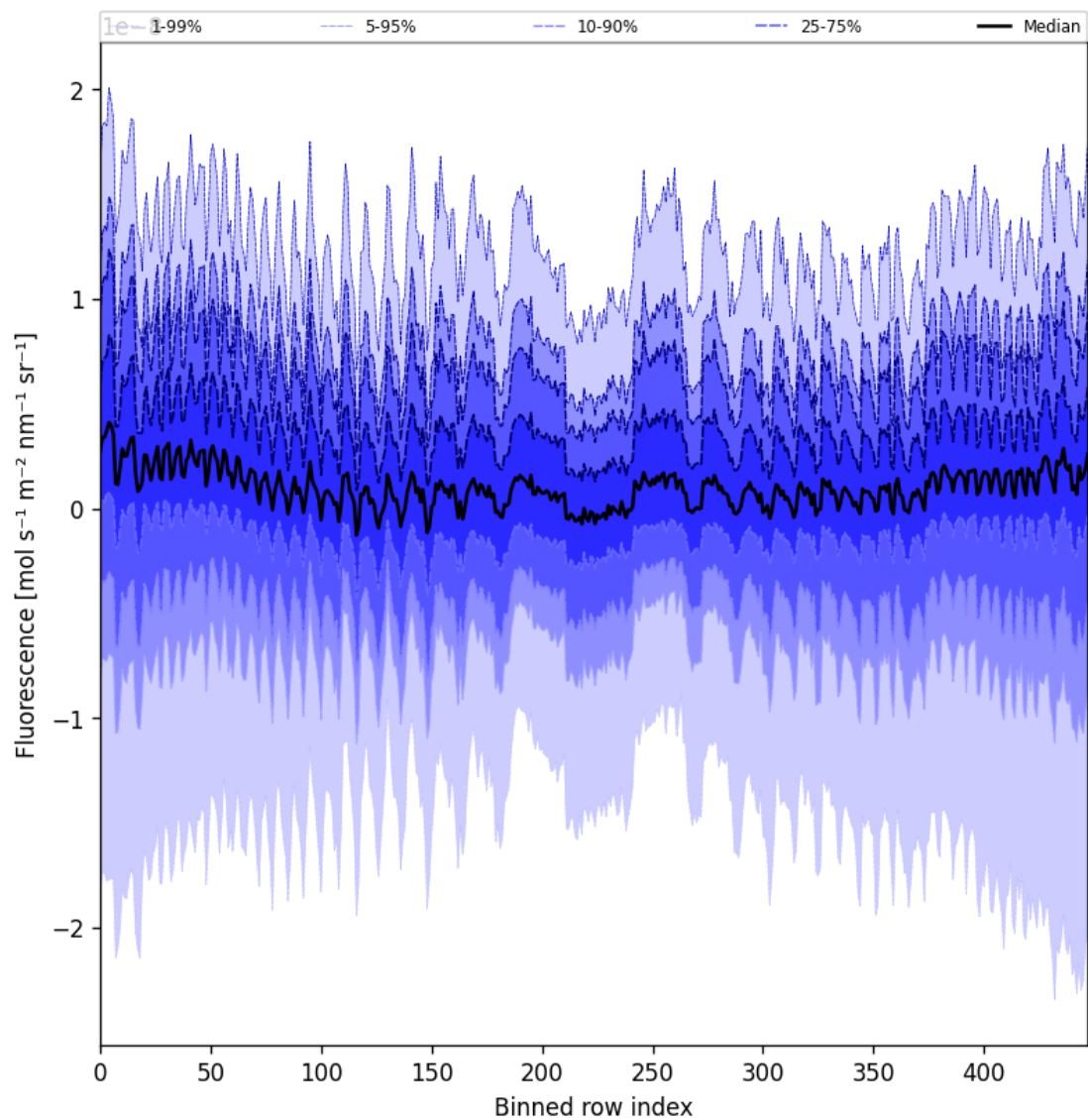
Figure 57: Along track statistics of “Fluorescence” for 2025-03-28 to 2025-03-29
