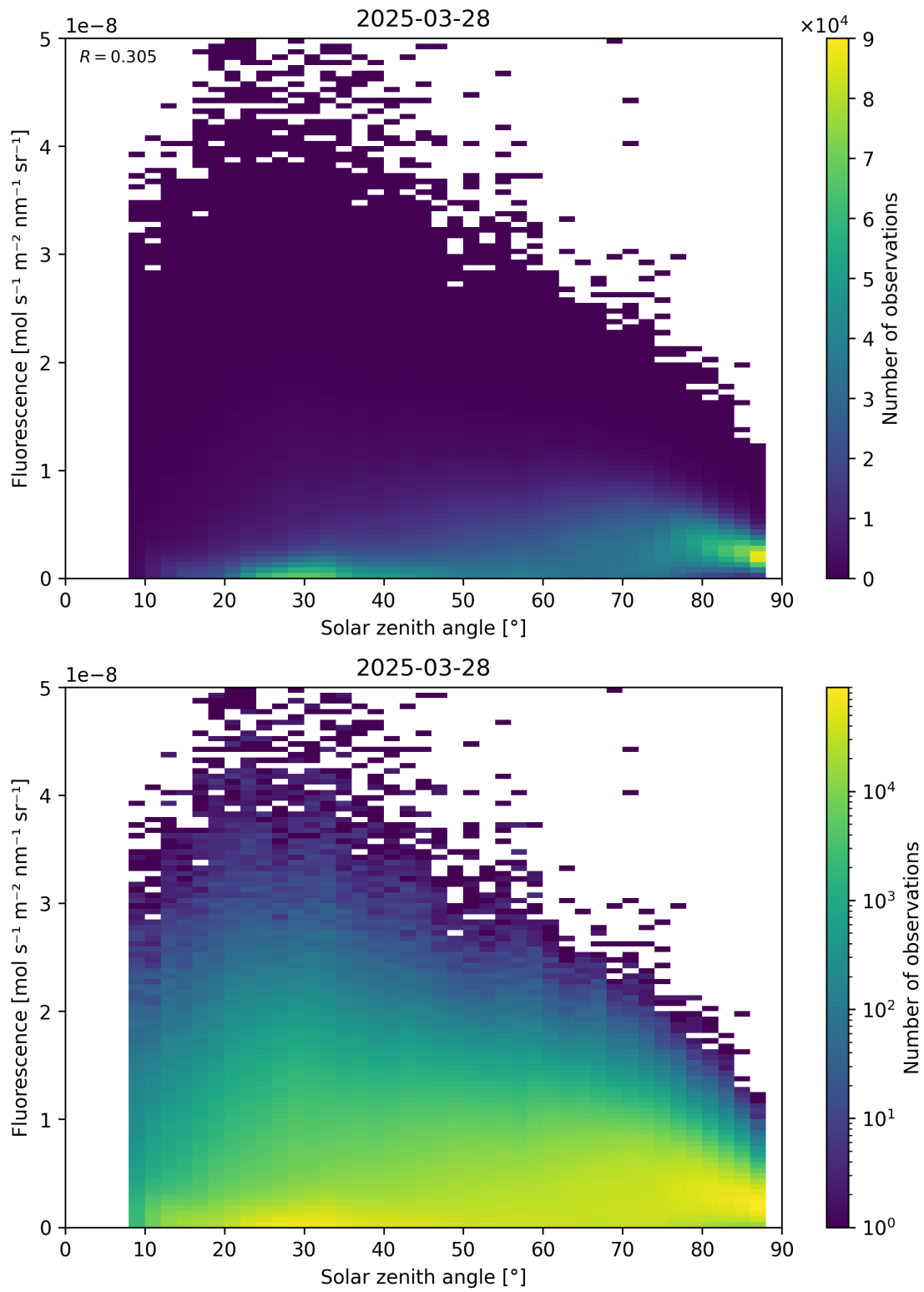
Figure 112: Scatter density plot of “Solar zenith angle” against “Fluorescence” for 2025-03-28 to 2025-03-29.
