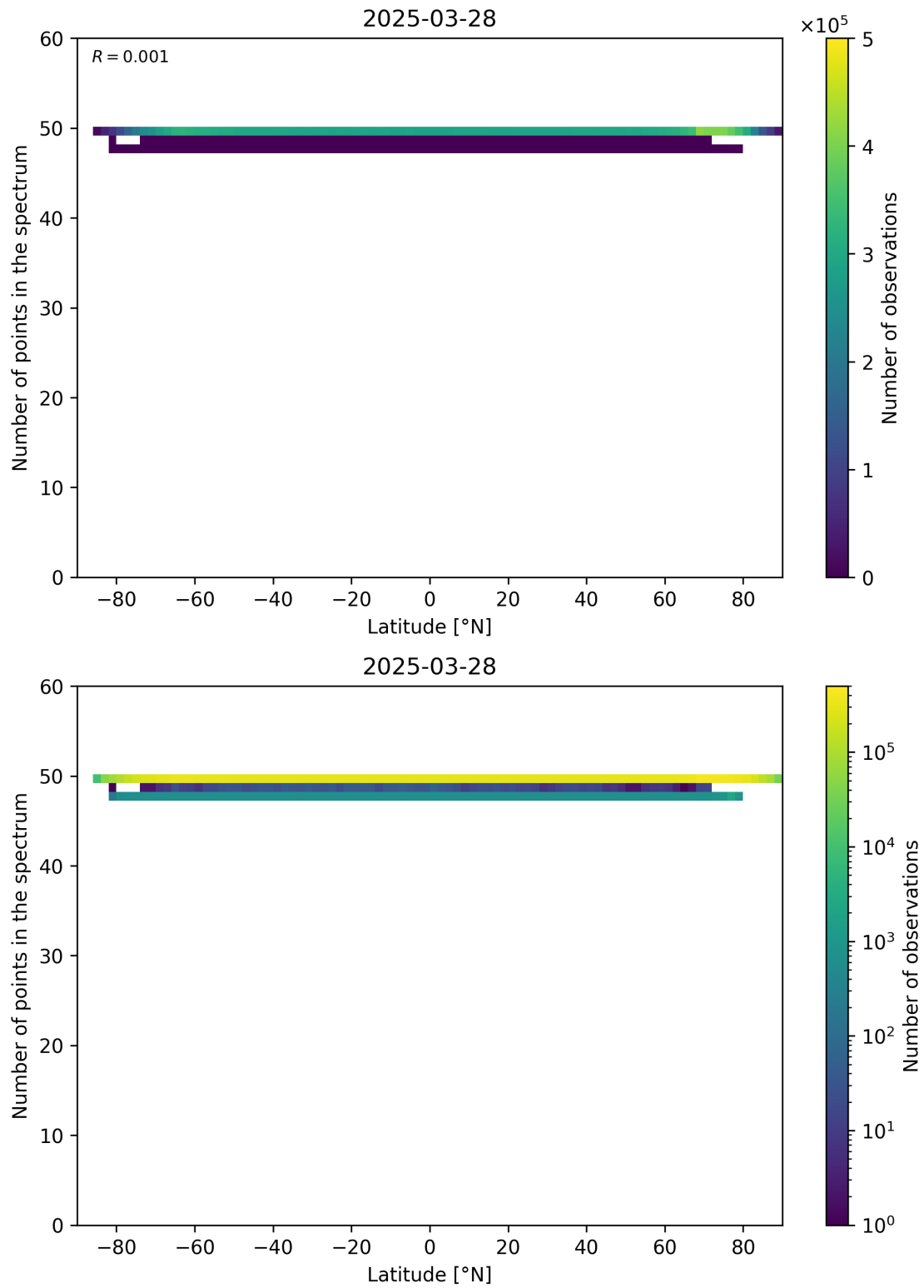
Figure 94: Scatter density plot of “Latitude” against “Number of points in the spectrum” for 2025-03-28 to 2025-03-29.
