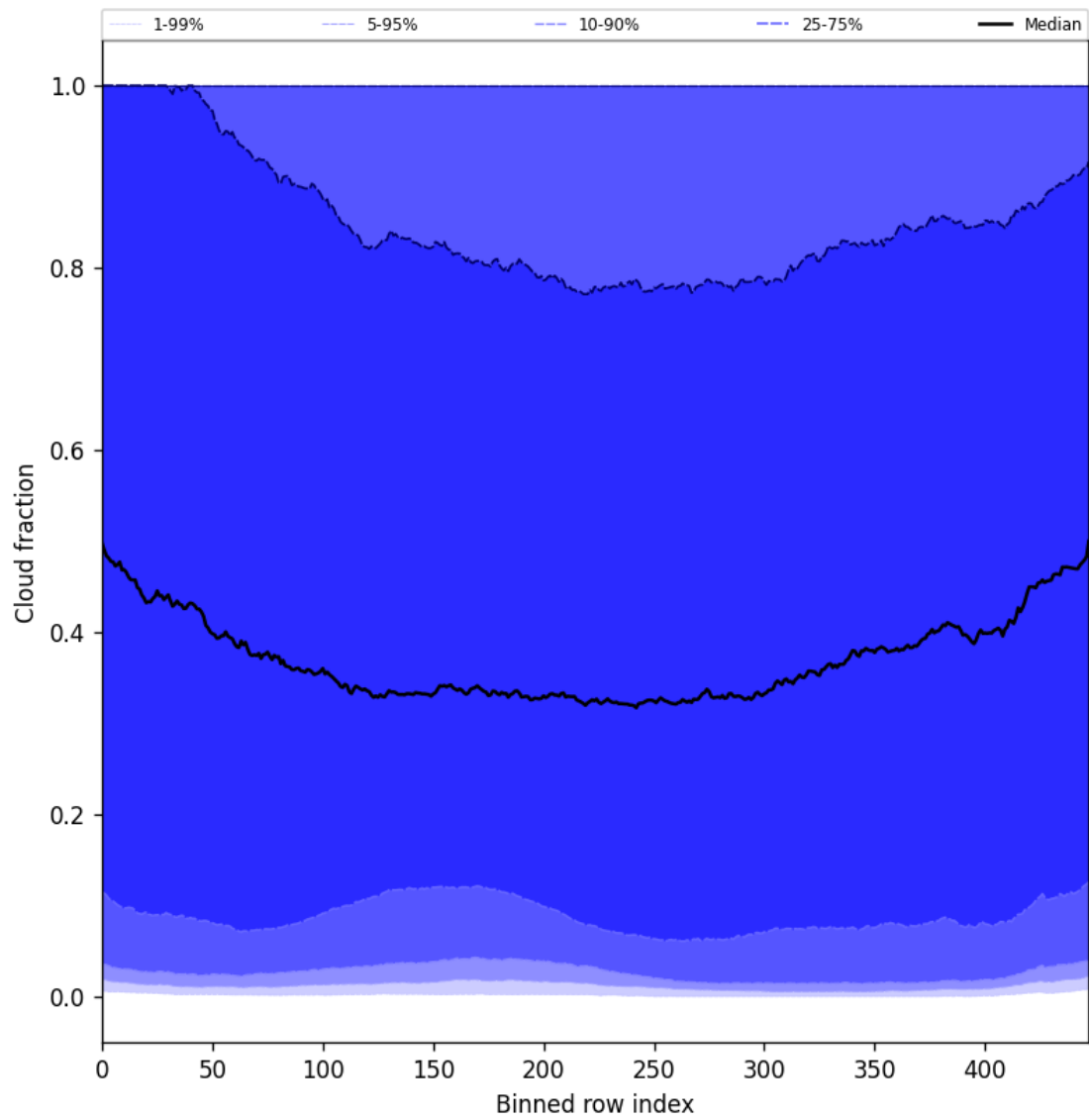
Figure 49: Along track statistics of “Cloud fraction” for 2025-03-28 to 2025-03-29
