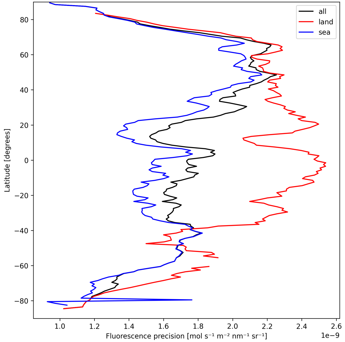
Figure 24: Zonal average of “Fluorescence precision” for 2025-03-28 to 2025-03-29.
