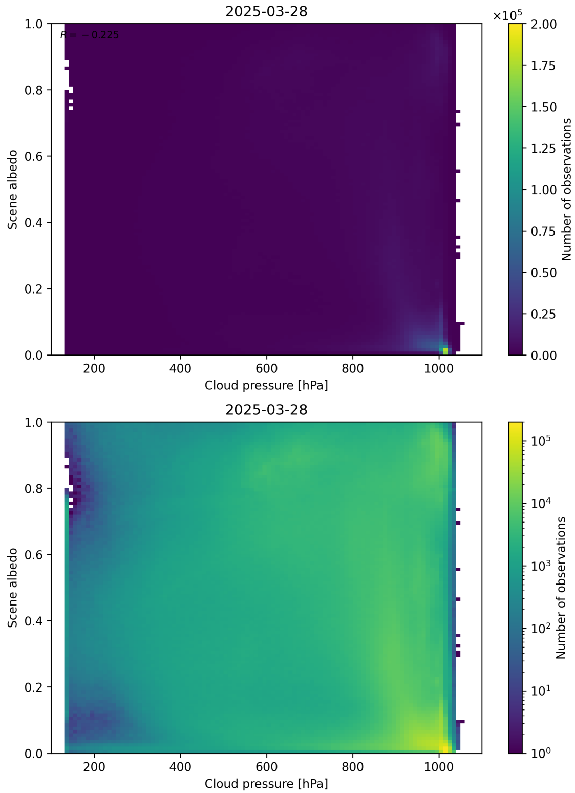
Figure 83: Scatter density plot of “Cloud pressure” against “Scene albedo” for 2025-03-28 to 2025-03-29.
