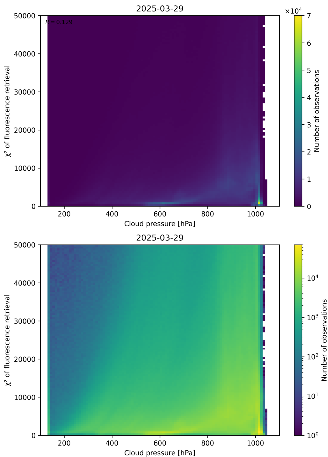
Figure 78: Scatter density plot of “Cloud pressure” against “ \chi^2 of fluorescence retrieval” for 2025-03-28 to 2025-03-30.
