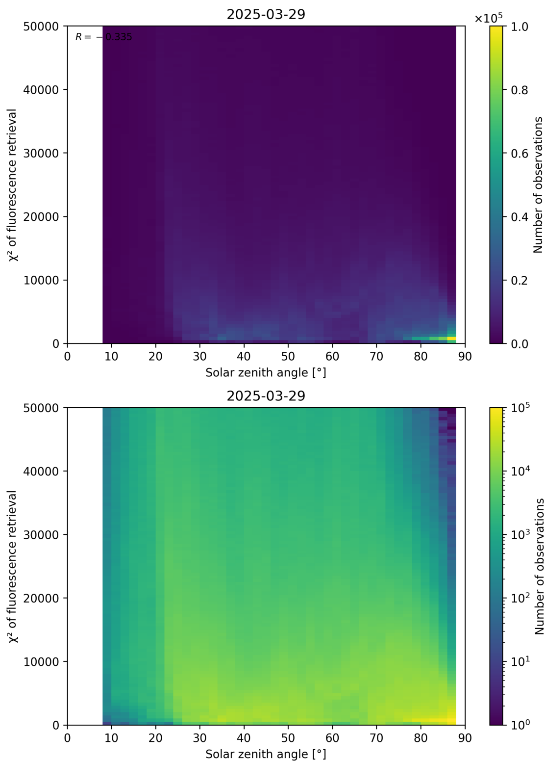
Figure 109: Scatter density plot of “Solar zenith angle” against “ \chi^2 of fluorescence retrieval” for 2025-03-28 to 2025-03-30.
