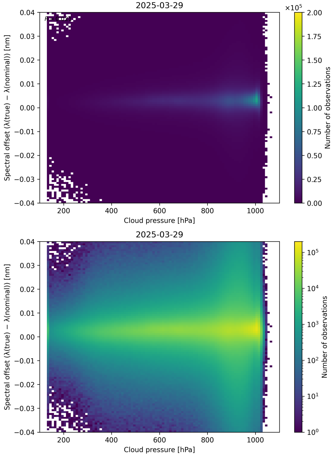
Figure 84: Scatter density plot of “Cloud pressure” against “Spectral offset ( \lambda_{\text{true}} - \lambda_{\text{nominal}} )” for 2025-03-28 to 2025-03-30.
