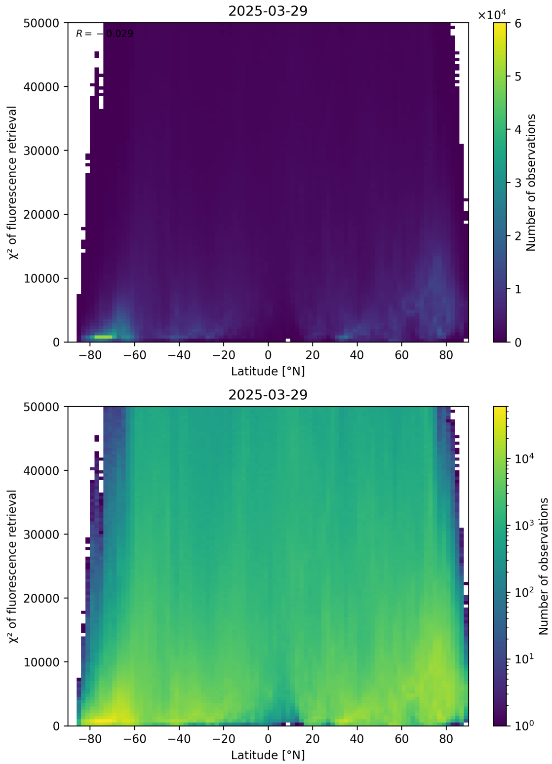
Figure 89: Scatter density plot of “Latitude” against “ \chi^2 of fluorescence retrieval” for 2025-03-28 to 2025-03-30.
