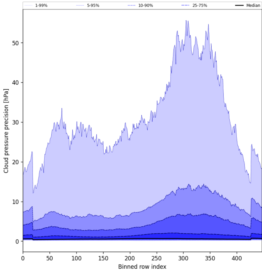
Figure 48: Along track statistics of “Cloud pressure precision” for 2025-03-28 to 2025-03-30
