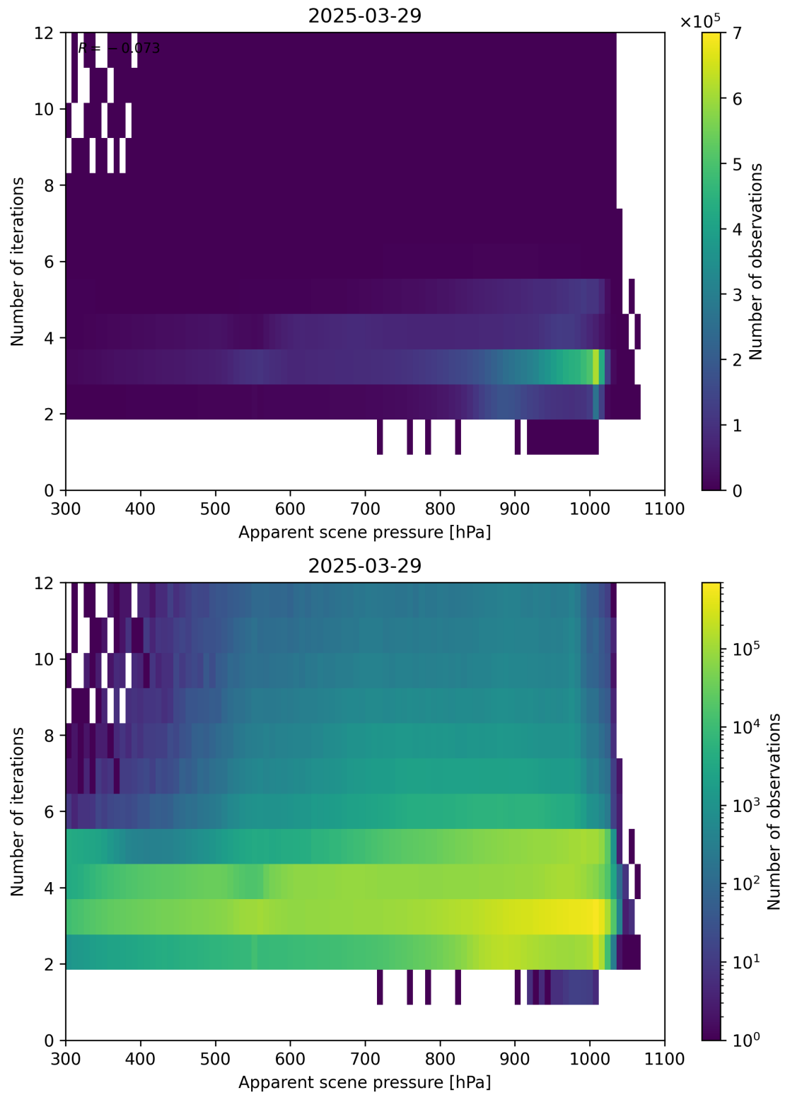
Figure 65: Scatter density plot of “Apparent scene pressure” against “Number of iterations” for 2025-03-28 to 2025-03-30.
