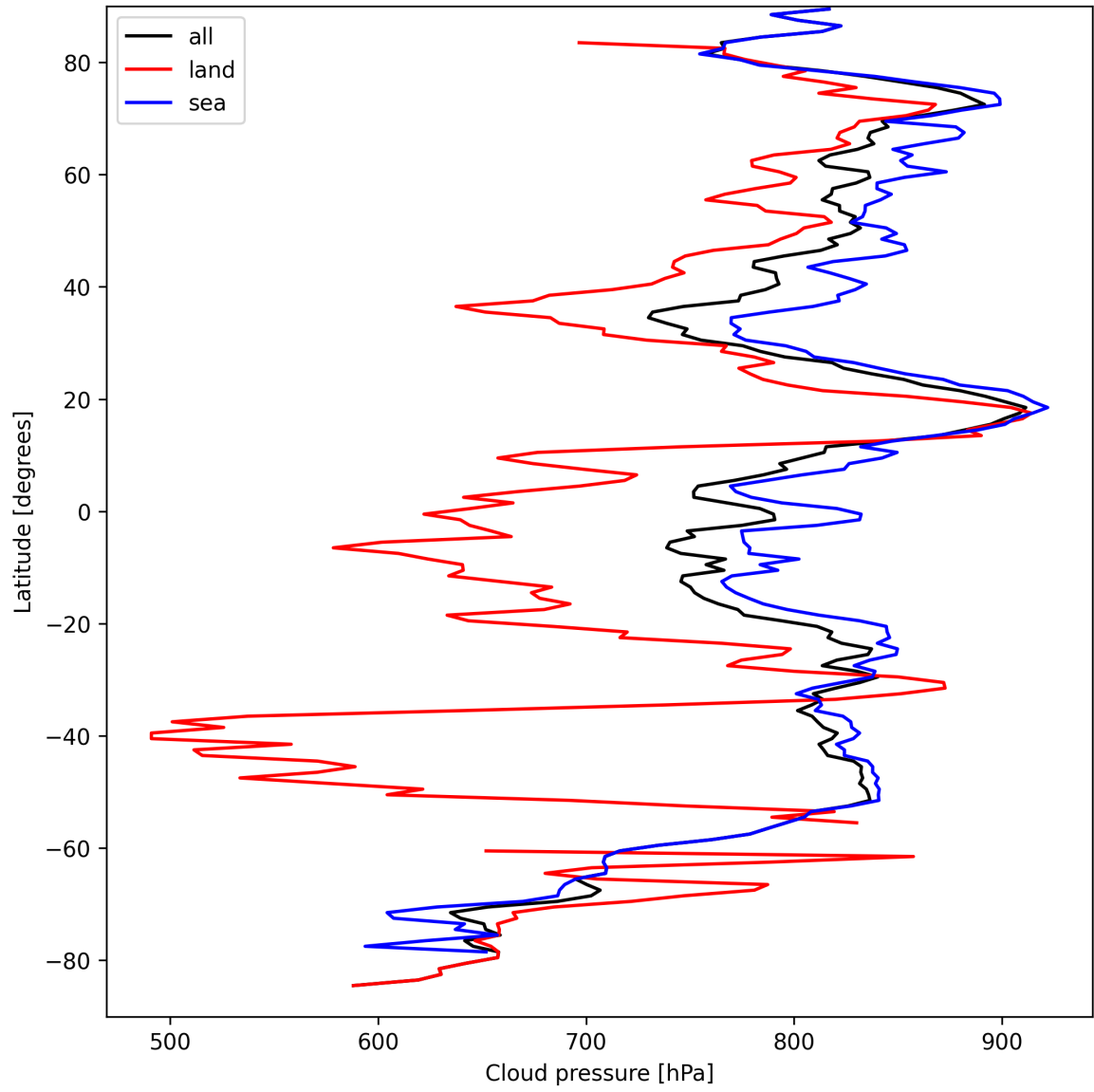
Figure 13: Zonal average of “Cloud pressure” for 2025-03-28 to 2025-03-30.
