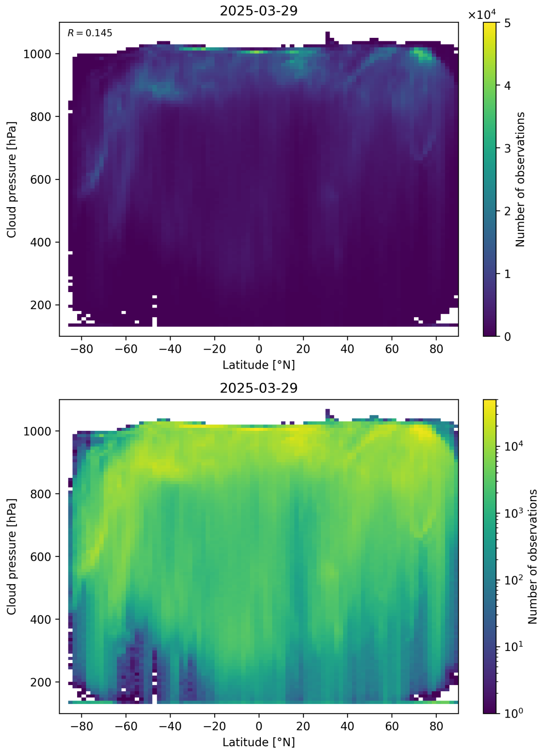
Figure 91: Scatter density plot of “Latitude” against “Cloud pressure” for 2025-03-28 to 2025-03-30.
