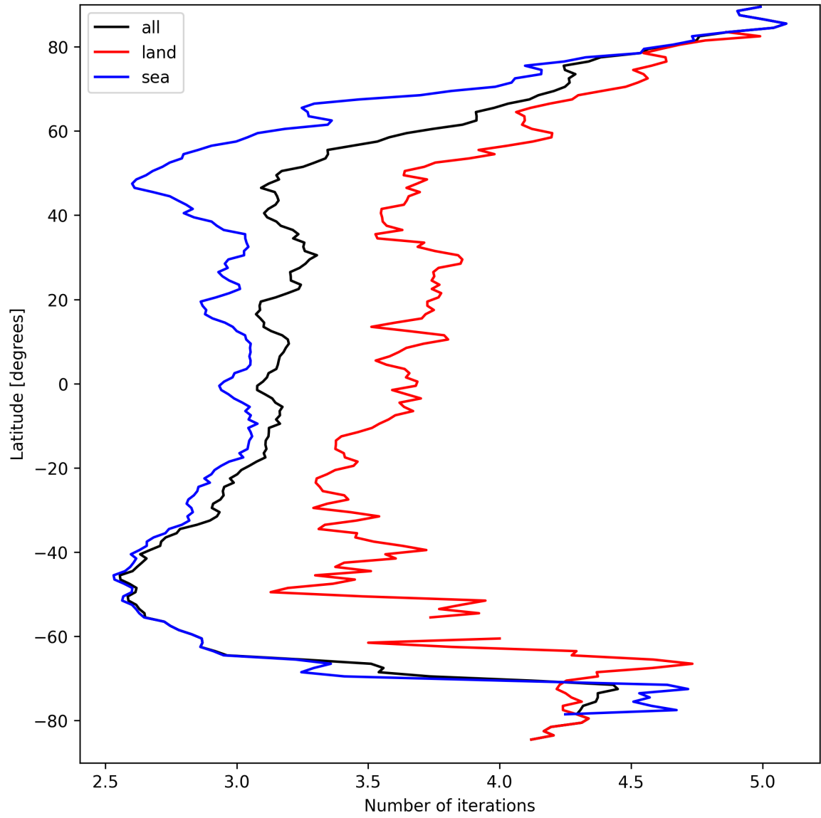
Figure 22: Zonal average of “Number of iterations” for 2025-03-28 to 2025-03-30.
