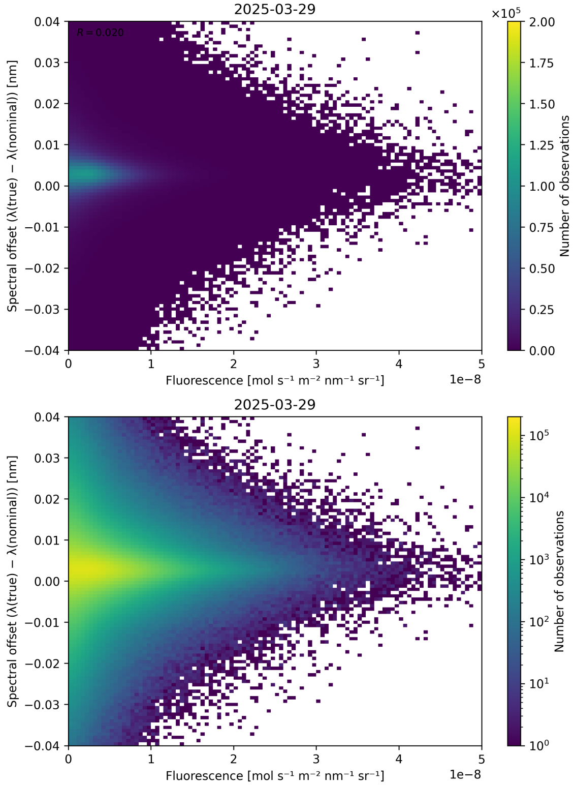
Figure 87: Scatter density plot of “Fluorescence” against “Spectral offset ( \lambda_{\text{true}} - \lambda_{\text{nominal}} )” for 2025-03-28 to 2025-03-30.
