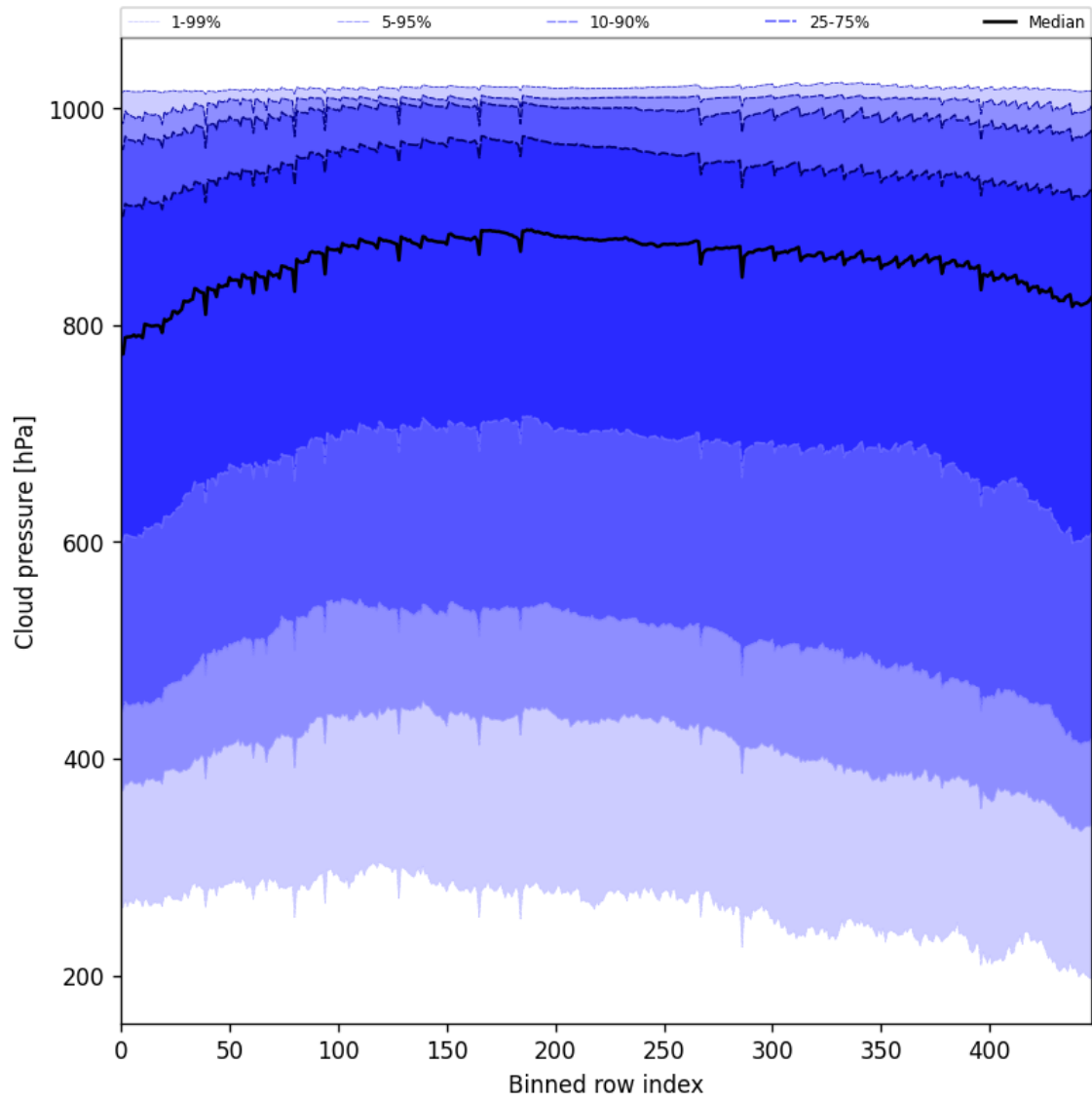
Figure 47: Along track statistics of “Cloud pressure” for 2025-03-28 to 2025-03-30
