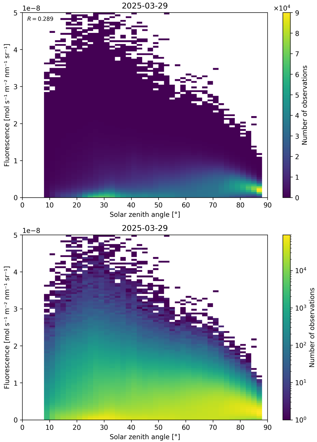
Figure 112: Scatter density plot of “Solar zenith angle” against “Fluorescence” for 2025-03-28 to 2025-03-30.
