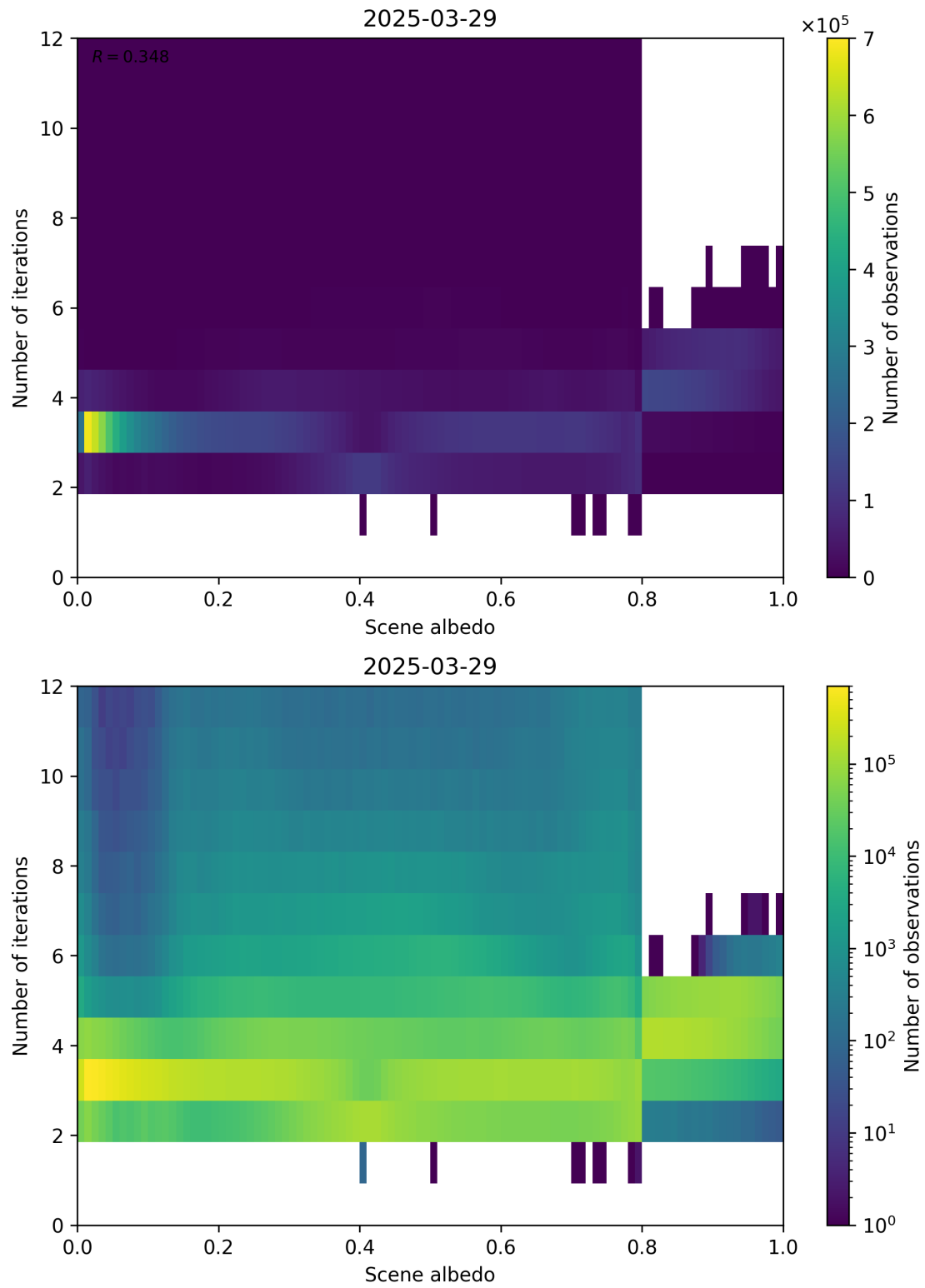
Figure 105: Scatter density plot of “Scene albedo” against “Number of iterations” for 2025-03-28 to 2025-03-30.
