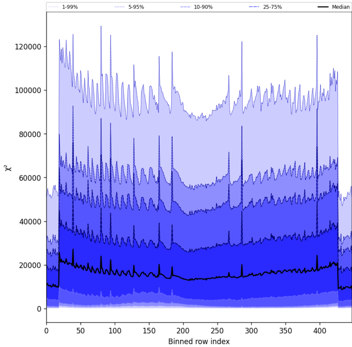
Figure 55: Along track statistics of “ \chi^2 ” for 2025-03-28 to 2025-03-30
