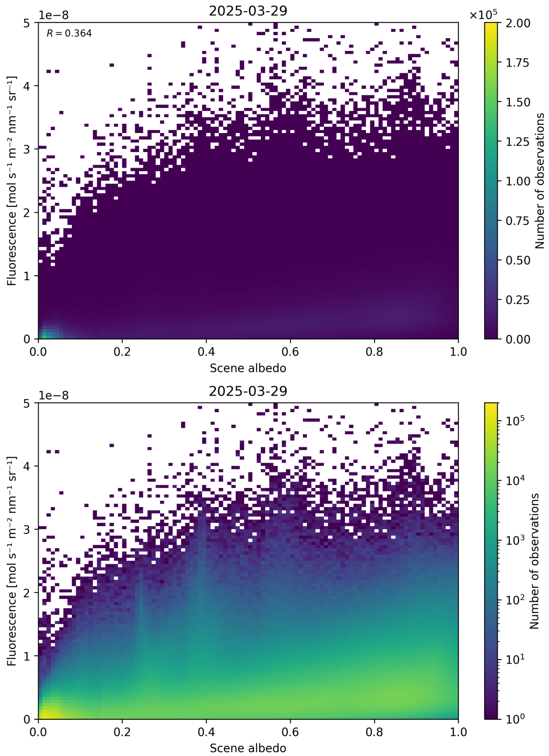
Figure 104: Scatter density plot of “Scene albedo” against “Fluorescence” for 2025-03-28 to 2025-03-30.
