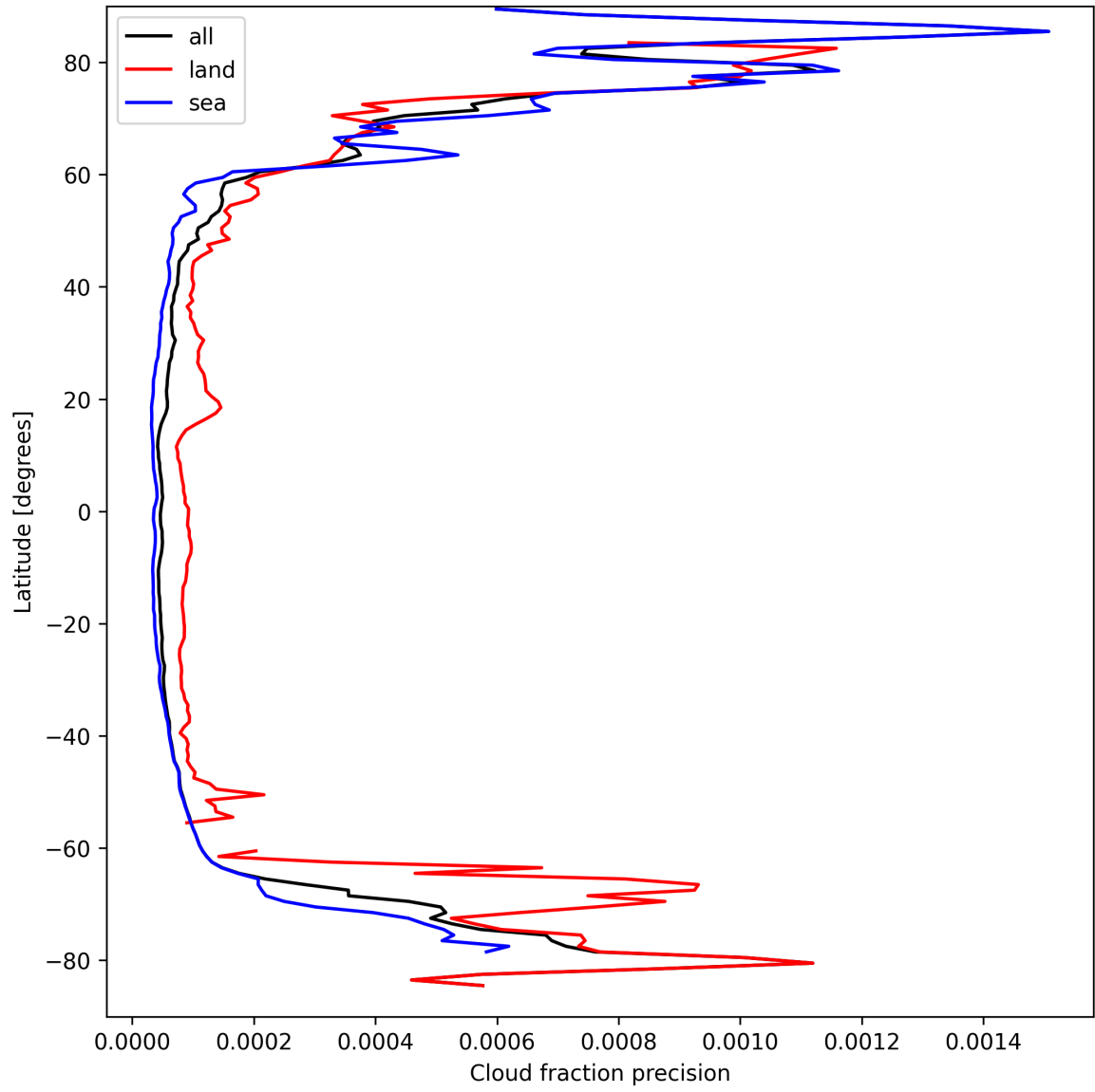
Figure 16: Zonal average of “Cloud fraction precision” for 2025-03-28 to 2025-03-30.
