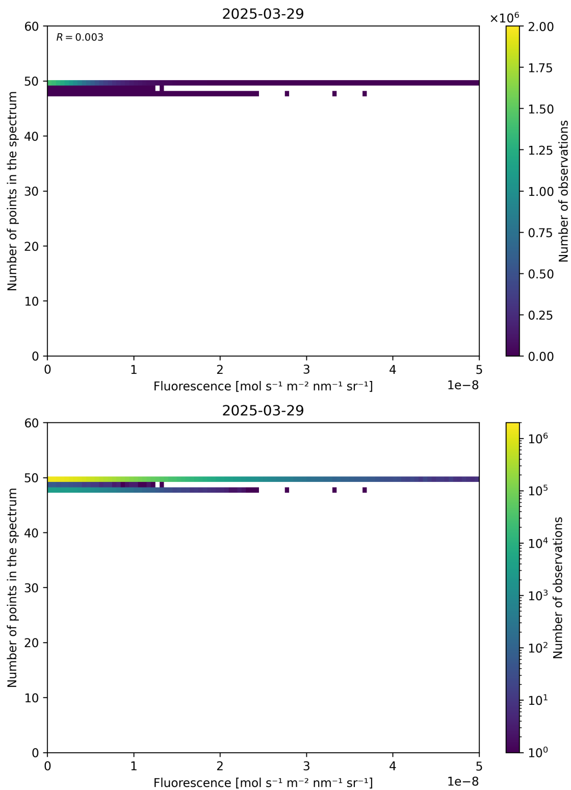
Figure 86: Scatter density plot of “Fluorescence” against “Number of points in the spectrum” for 2025-03-28 to 2025-03-30.
