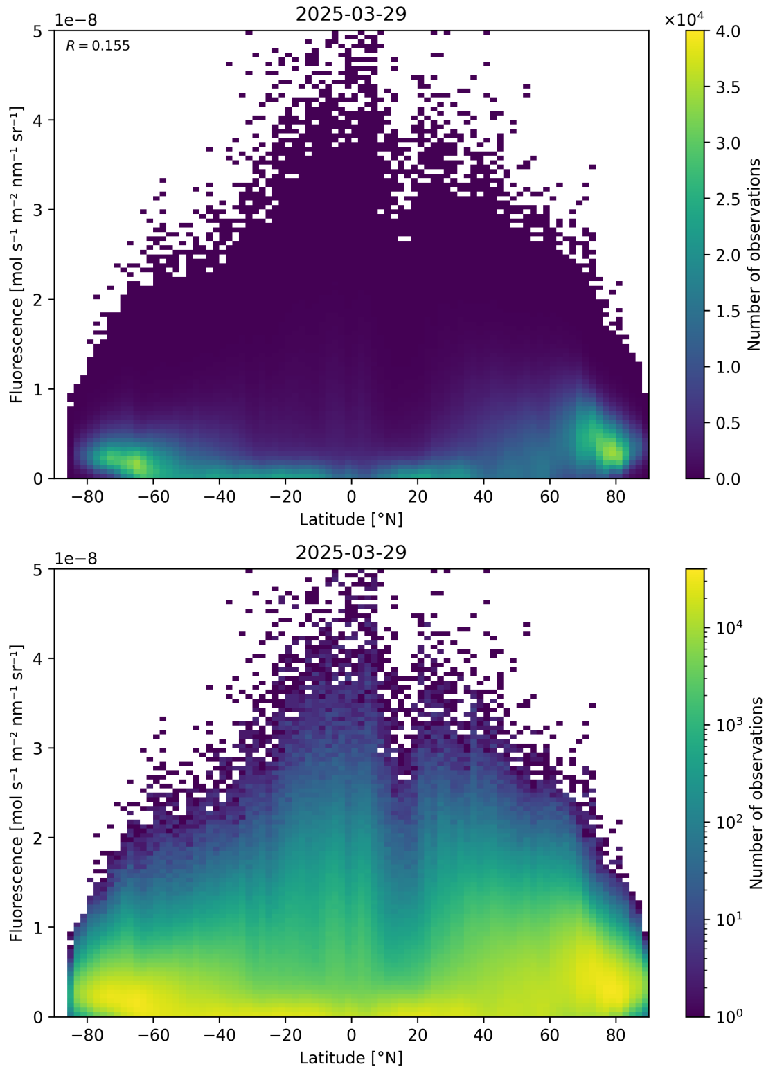
Figure 92: Scatter density plot of “Latitude” against “Fluorescence” for 2025-03-28 to 2025-03-30.
