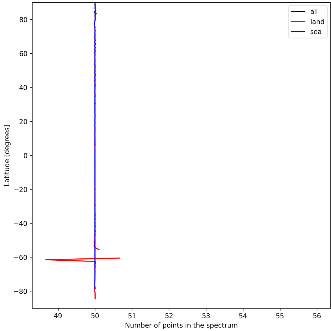
Figure 27: Zonal average of “Number of points in the spectrum” for 2025-03-28 to 2025-03-30.
