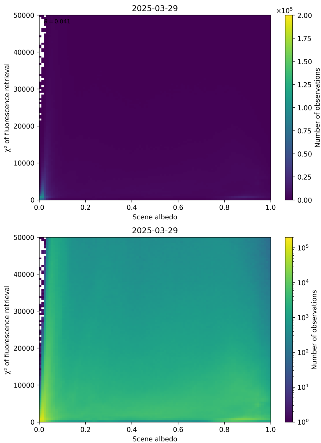
Figure 103: Scatter density plot of “Scene albedo” against “ \chi^2 of fluorescence retrieval” for 2025-03-28 to 2025-03-30.
