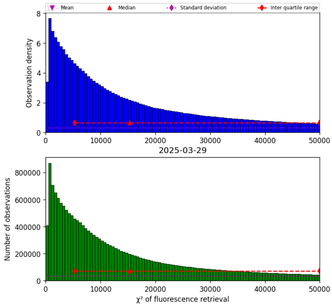
Figure 42: Histogram of “ \chi^2 of fluorescence retrieval” for 2025-03-28 to 2025-03-30
