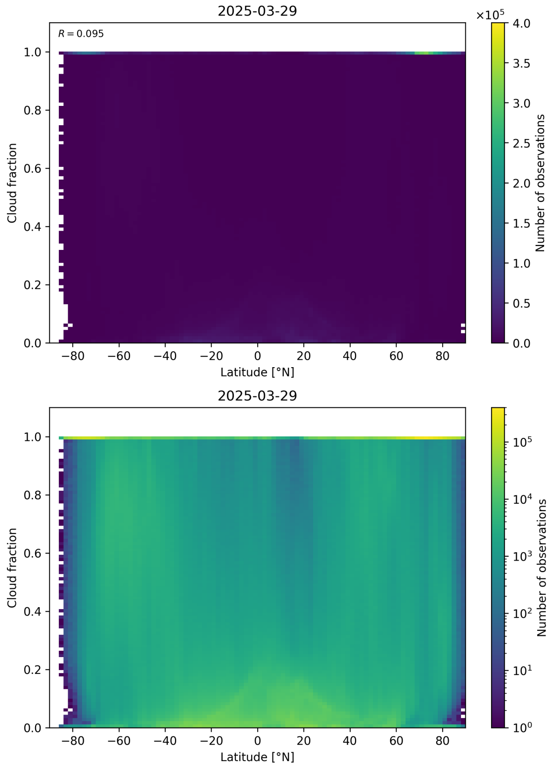
Figure 90: Scatter density plot of “Latitude” against “Cloud fraction” for 2025-03-28 to 2025-03-30.
