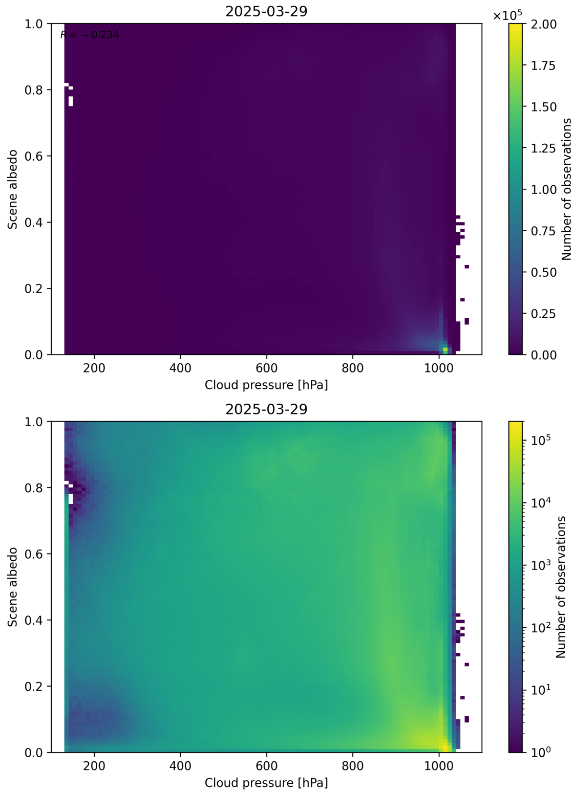
Figure 83: Scatter density plot of “Cloud pressure” against “Scene albedo” for 2025-03-28 to 2025-03-30.
