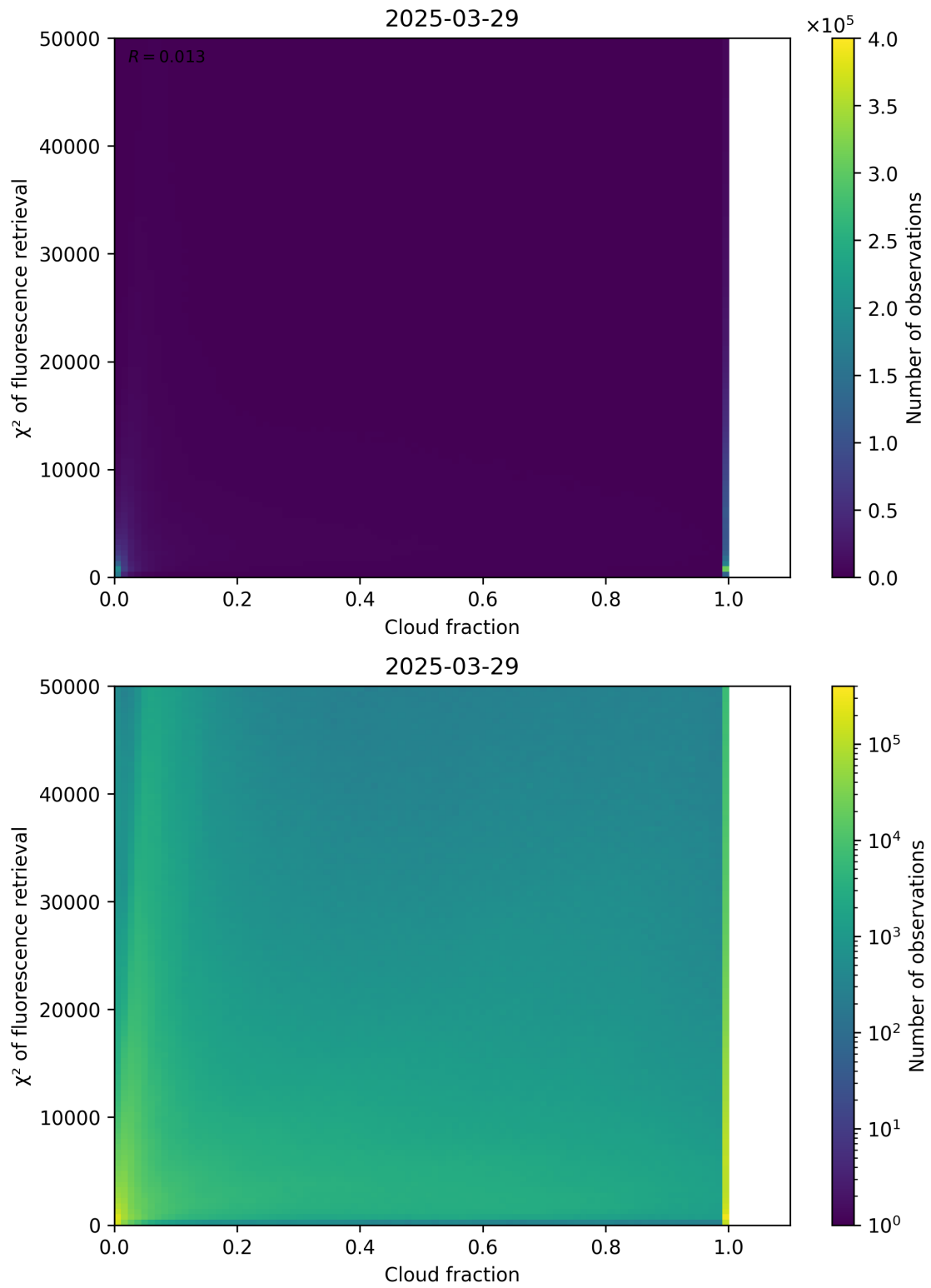
Figure 71: Scatter density plot of “Cloud fraction” against “ \chi^2 of fluorescence retrieval” for 2025-03-28 to 2025-03-30.
