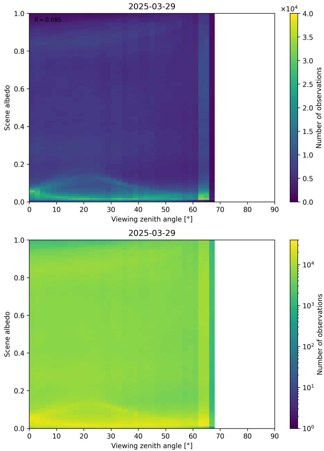
Figure 126: Scatter density plot of “Viewing zenith angle” against “Scene albedo” for 2025-03-28 to 2025-03-30.
