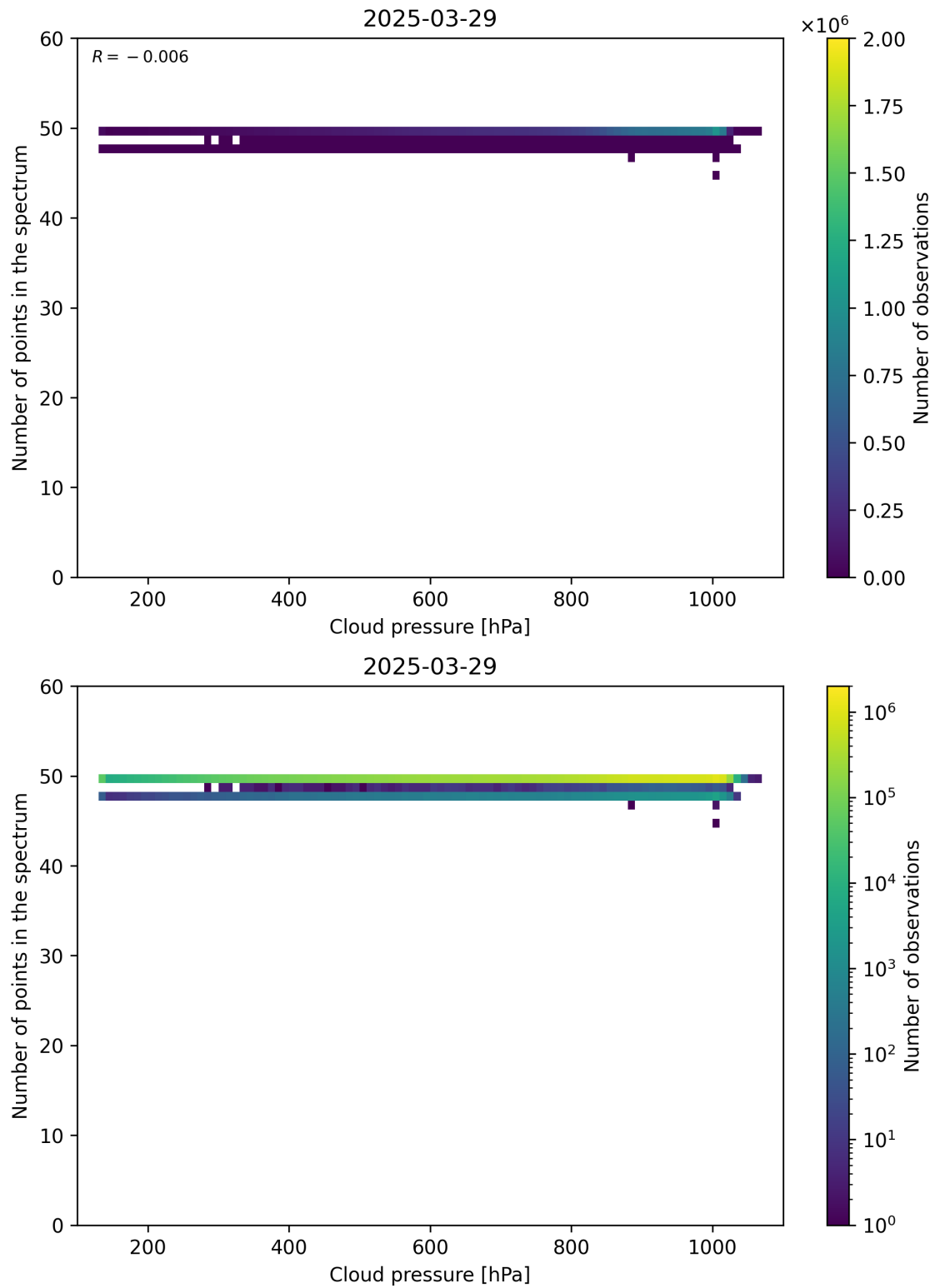
Figure 82: Scatter density plot of “Cloud pressure” against “Number of points in the spectrum” for 2025-03-28 to 2025-03-30.
