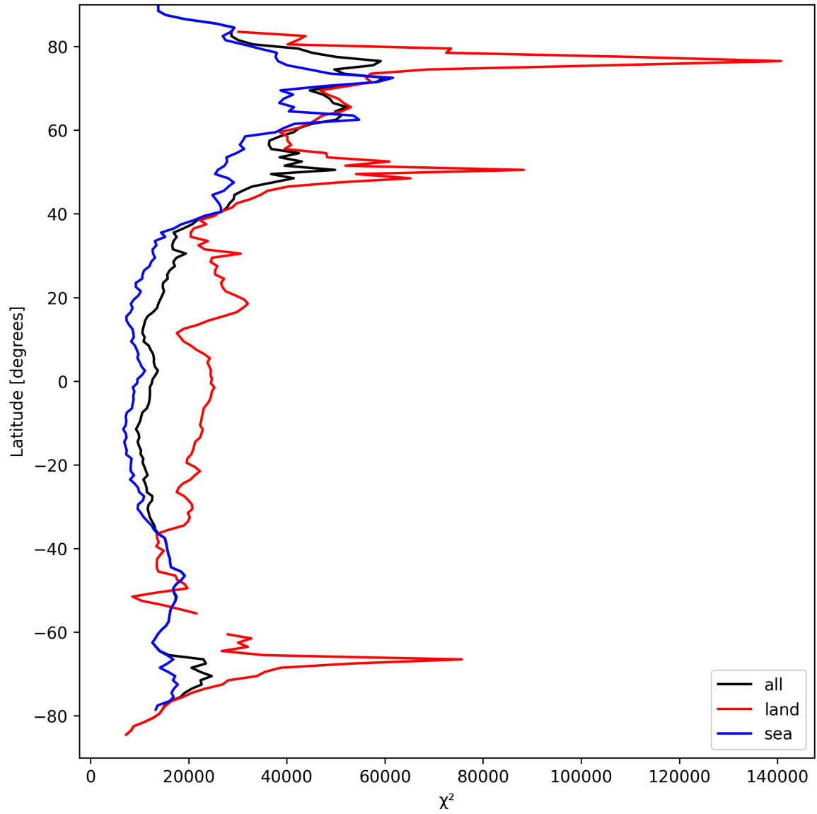
Figure 21: Zonal average of “ \chi^2 ” for 2025-03-28 to 2025-03-30.
