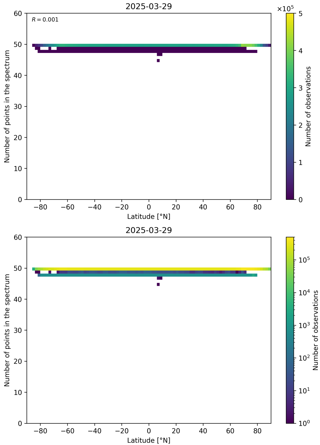
Figure 94: Scatter density plot of “Latitude” against “Number of points in the spectrum” for 2025-03-28 to 2025-03-30.
