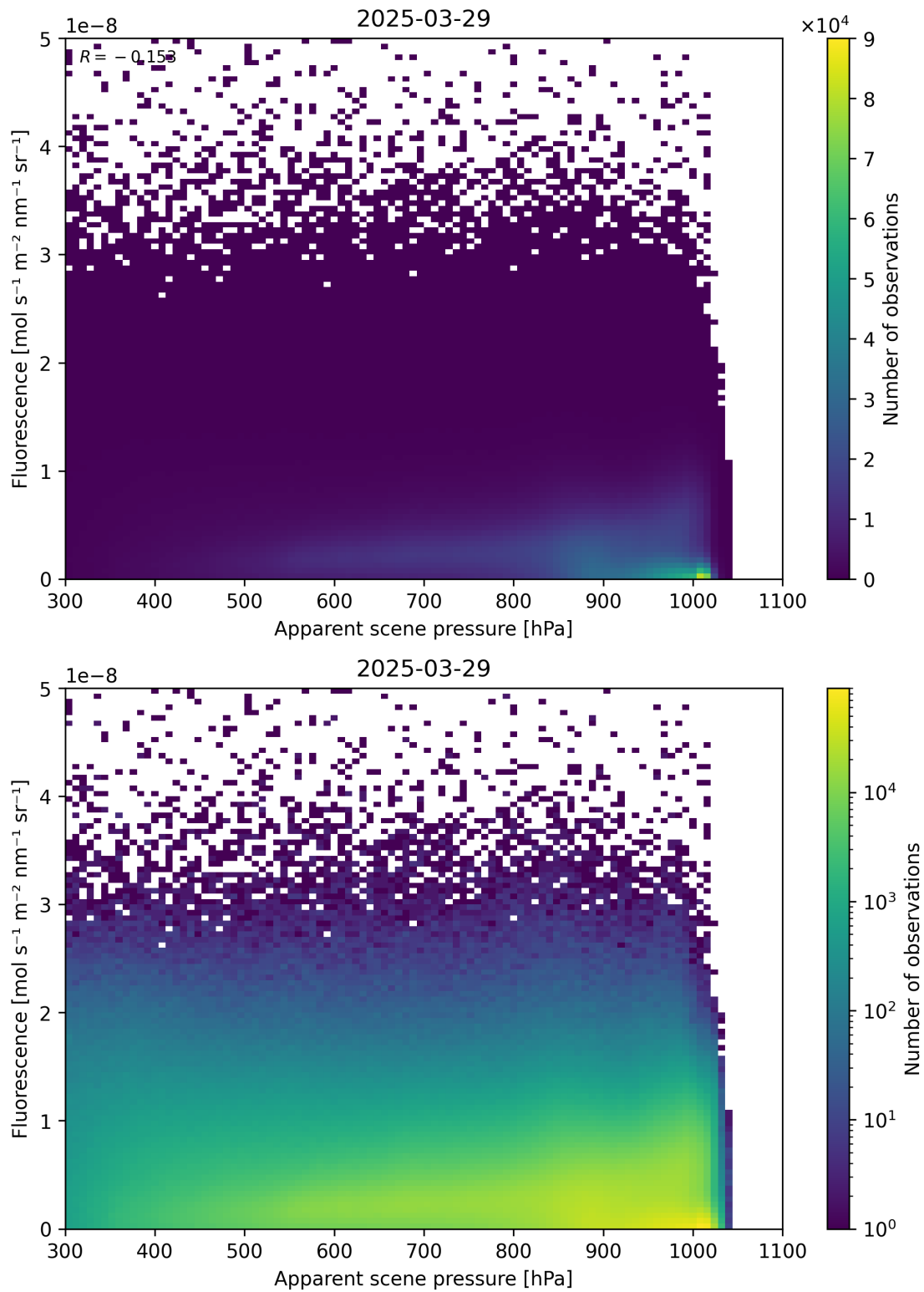
Figure 64: Scatter density plot of “Apparent scene pressure” against “Fluorescence” for 2025-03-28 to 2025-03-30.
