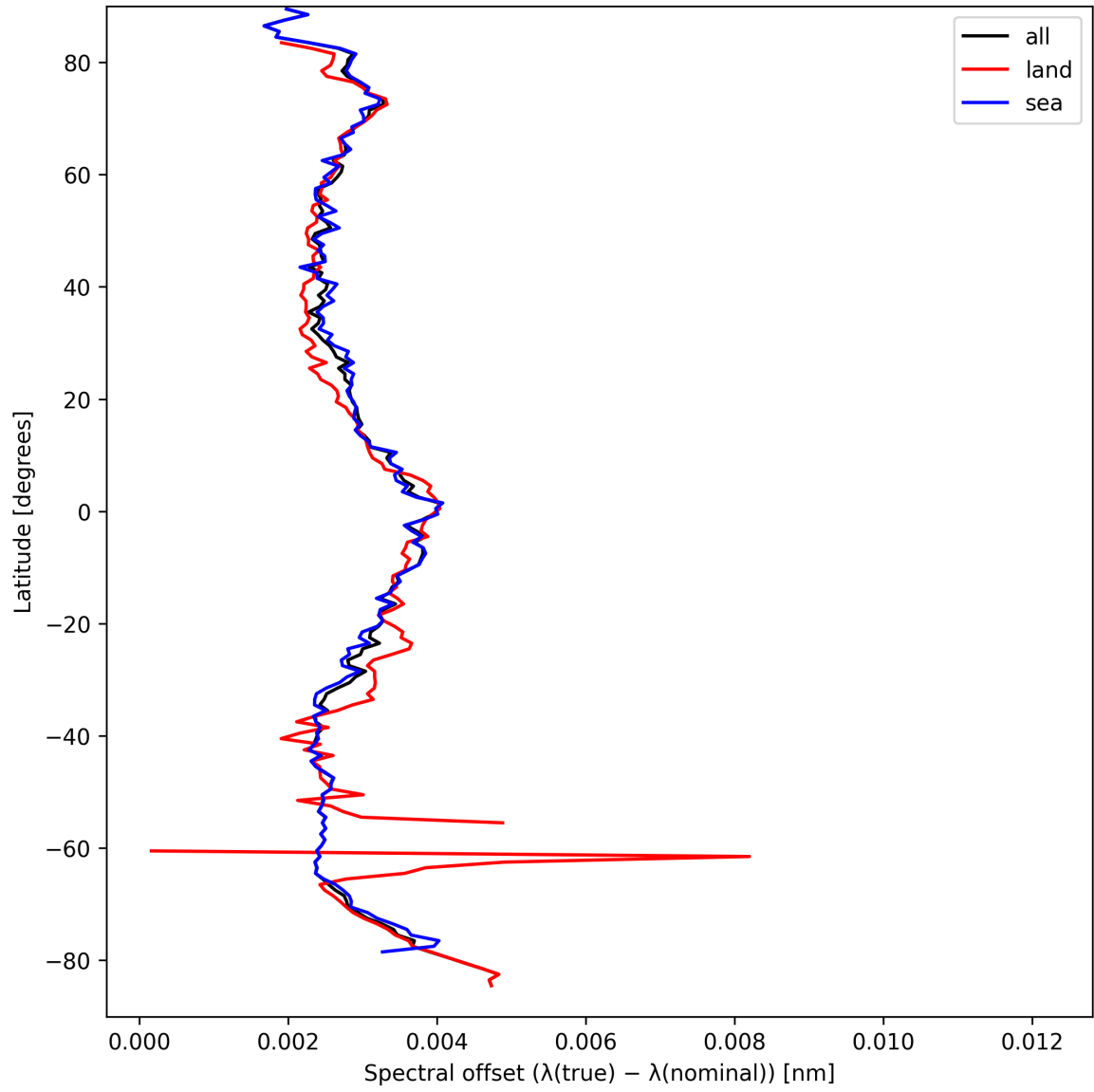
Figure 28: Zonal average of “Spectral offset ( \lambda_{\text{true}} - \lambda_{\text{nominal}} )” for 2025-03-28 to 2025-03-30.
