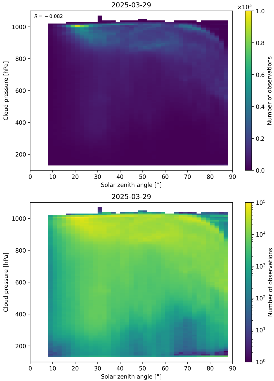
Figure 111: Scatter density plot of “Solar zenith angle” against “Cloud pressure” for 2025-03-28 to 2025-03-30.
