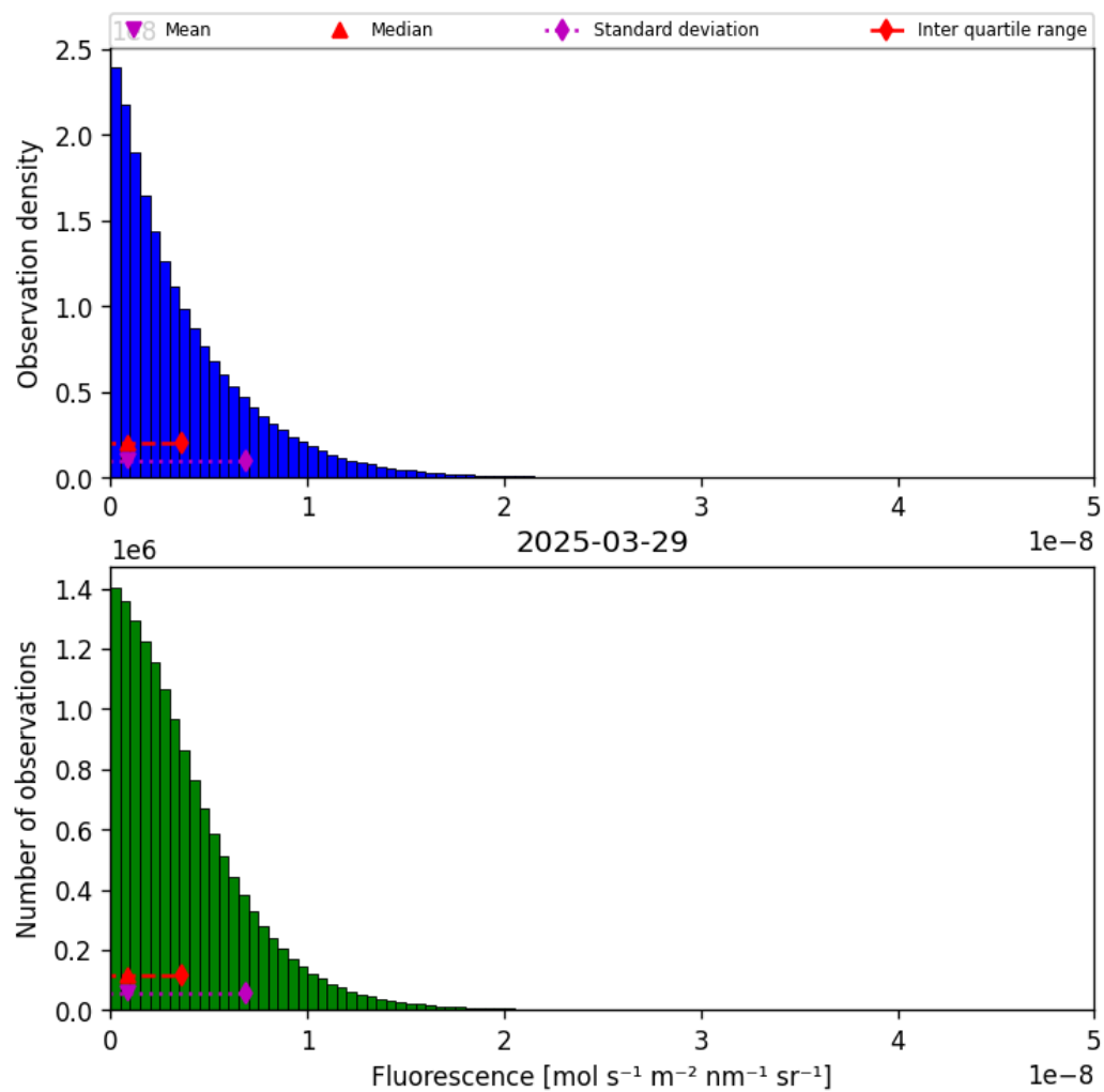
Figure 40: Histogram of “Fluorescence” for 2025-03-28 to 2025-03-30
