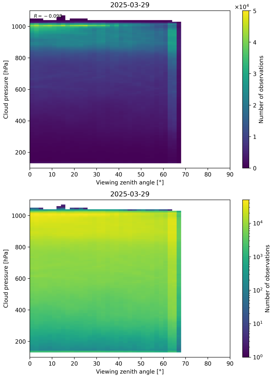
Figure 121: Scatter density plot of “Viewing zenith angle” against “Cloud pressure” for 2025-03-28 to 2025-03-30.
