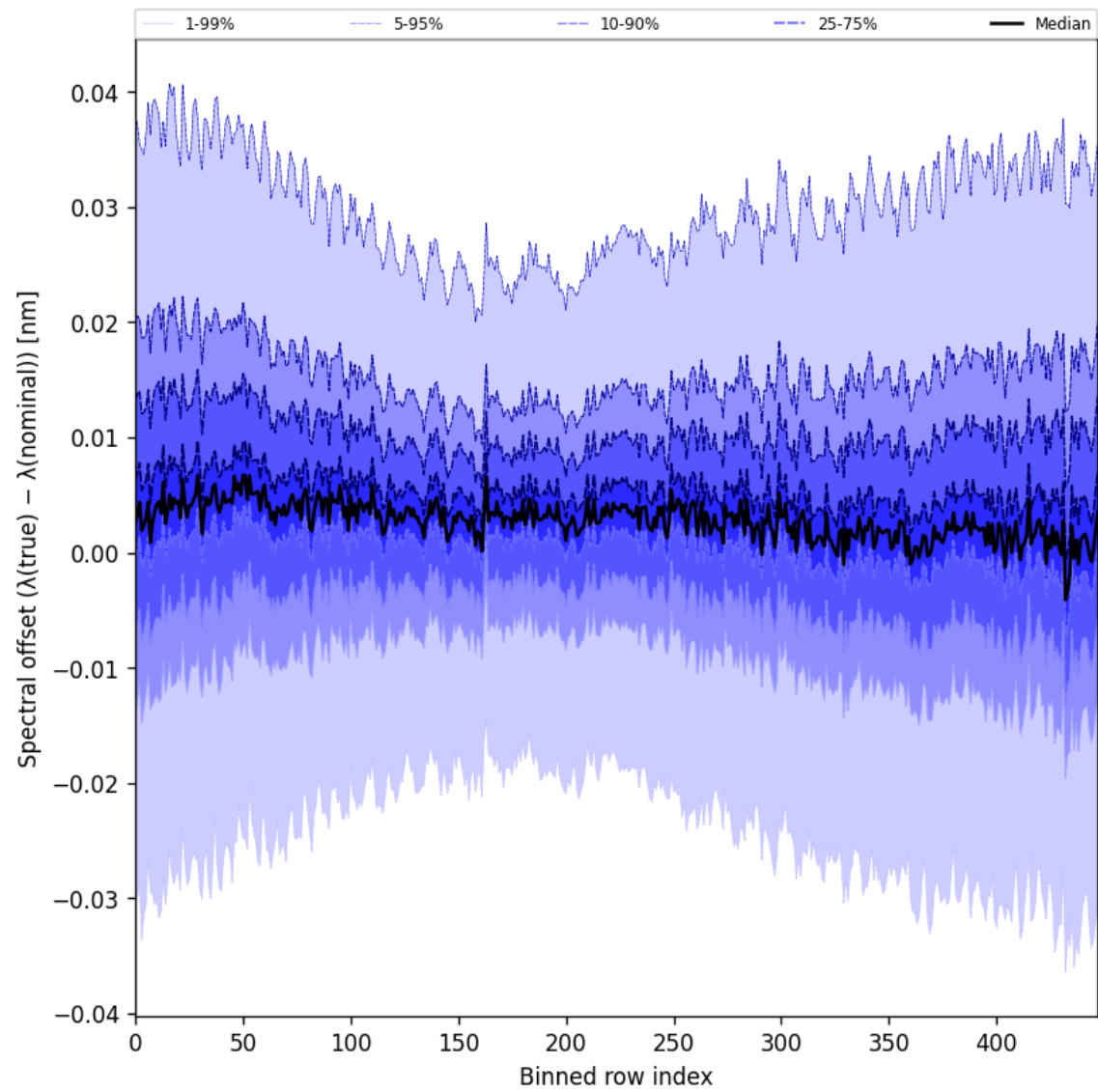
Figure 62: Along track statistics of “Spectral offset ( \lambda_{\text{true}} - \lambda_{\text{nominal}} )” for 2025-03-28 to 2025-03-30
