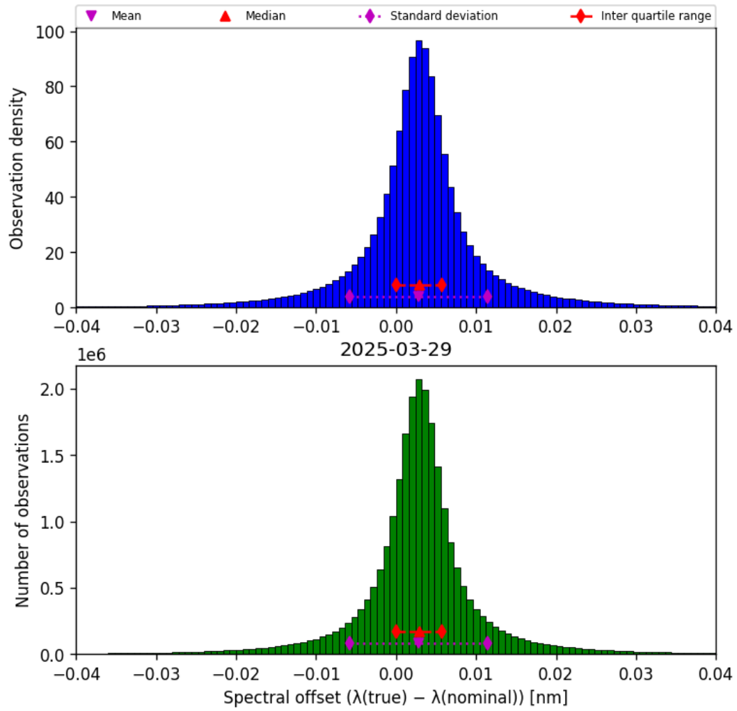
Figure 45: Histogram of “Spectral offset ( \lambda_{\text{true}} - \lambda_{\text{nominal}} )” for 2025-03-28 to 2025-03-30
