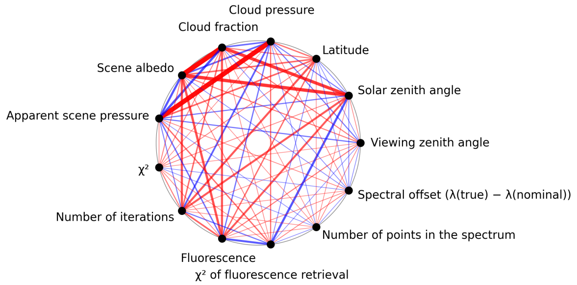
Figure 1: Map of correlation graph for 2025-03-28 to 2025-03-30.
