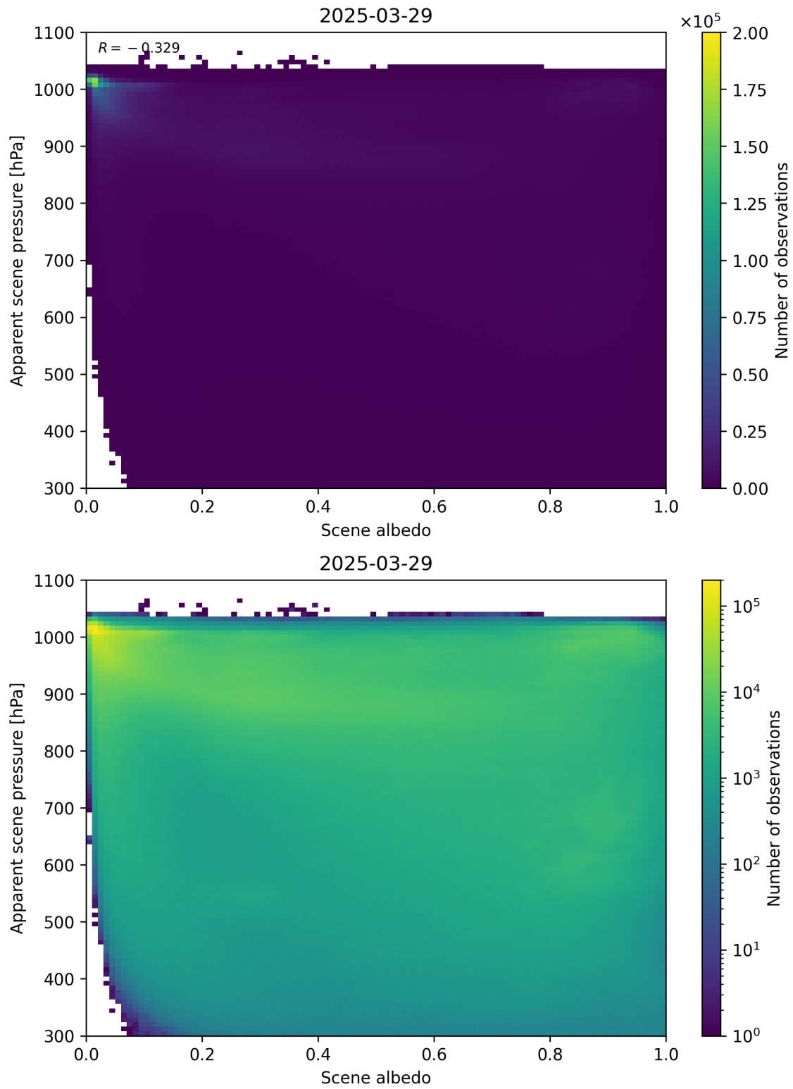
Figure 102: Scatter density plot of “Scene albedo” against “Apparent scene pressure” for 2025-03-28 to 2025-03-30.
