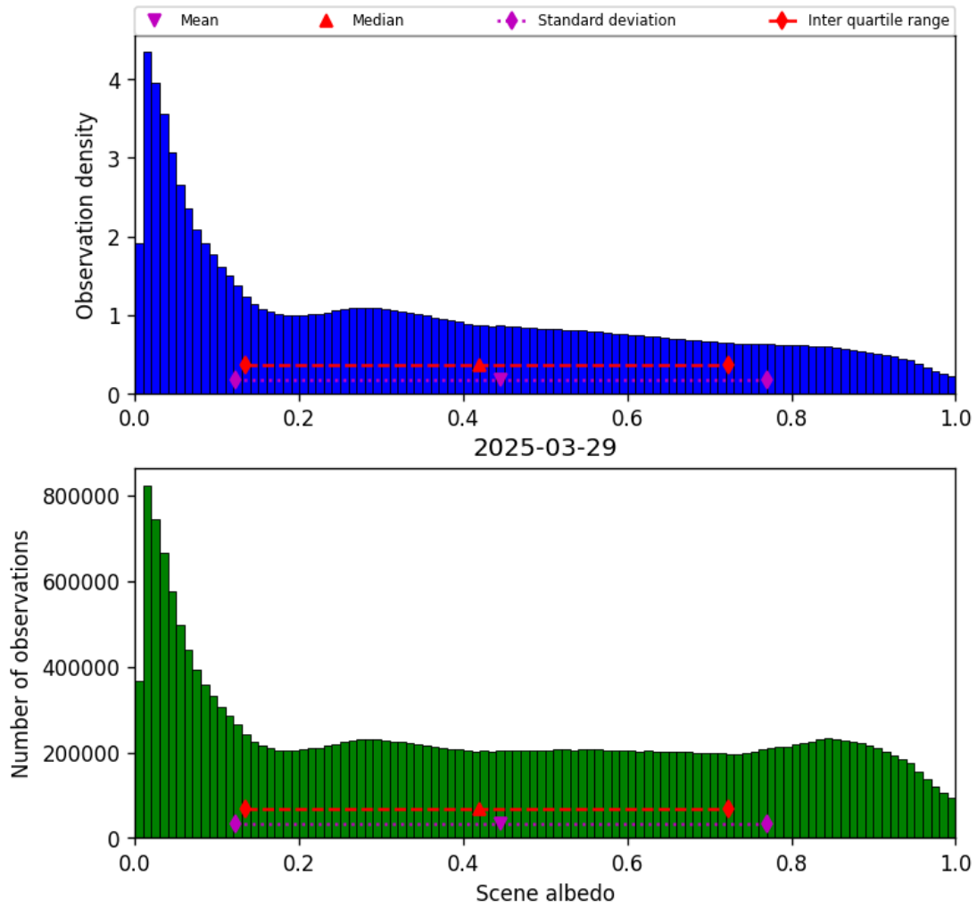
Figure 34: Histogram of “Scene albedo” for 2025-03-28 to 2025-03-30
