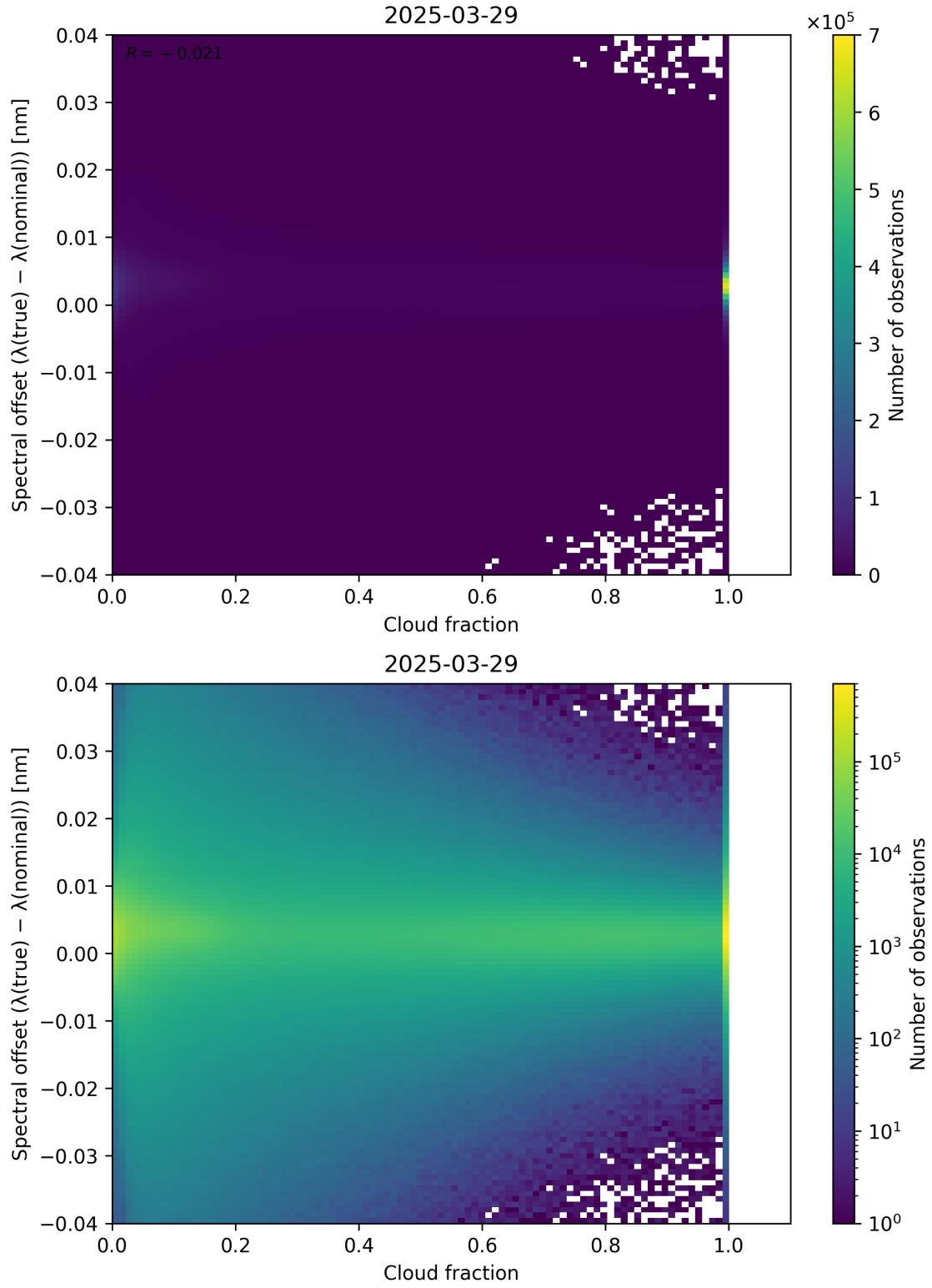
Figure 76: Scatter density plot of “Cloud fraction” against “Spectral offset ( \lambda_{\text{true}} - \lambda_{\text{nominal}} )” for 2025-03-28 to 2025-03-30.
