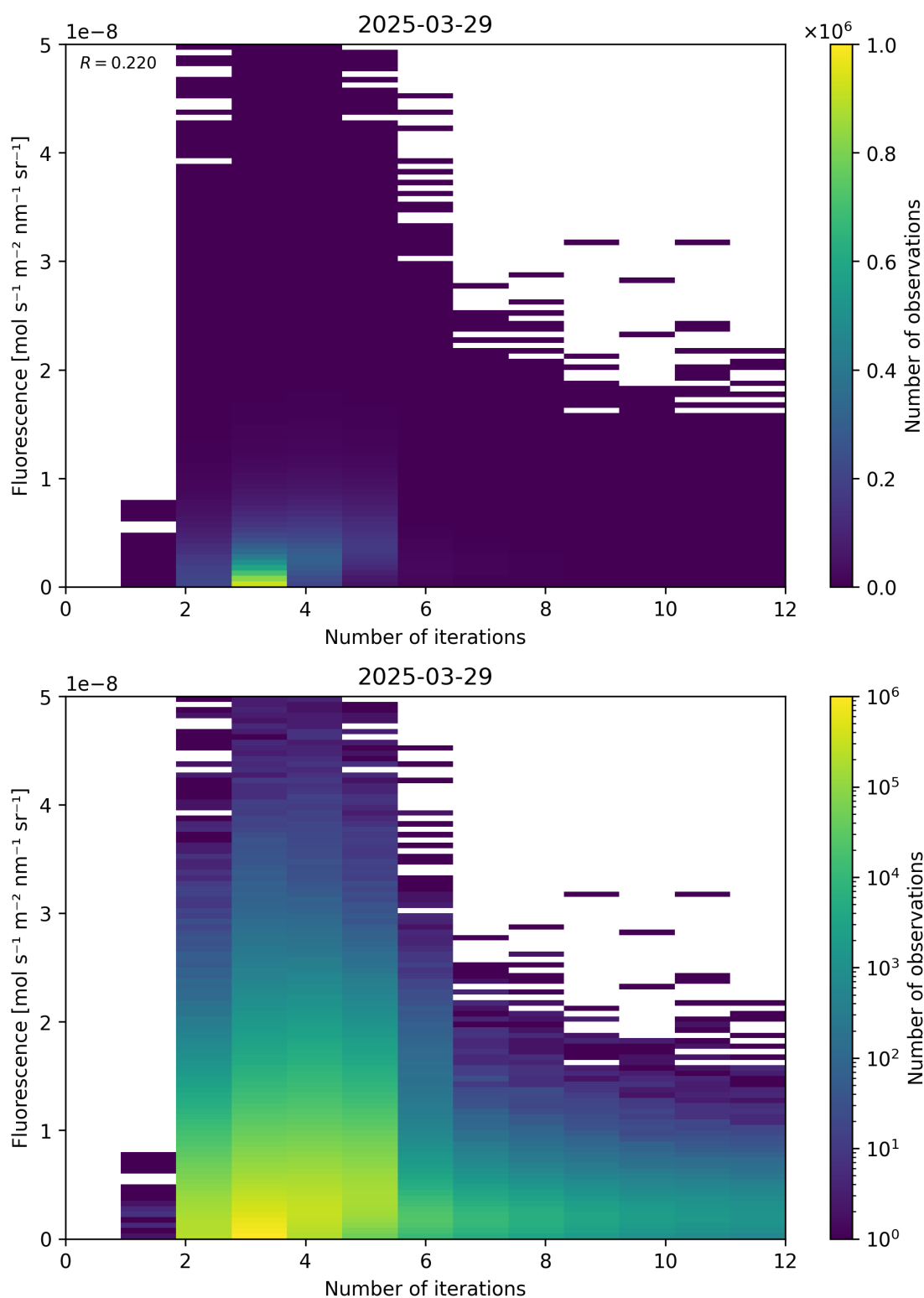
Figure 98: Scatter density plot of “Number of iterations” against “Fluorescence” for 2025-03-28 to 2025-03-30.
