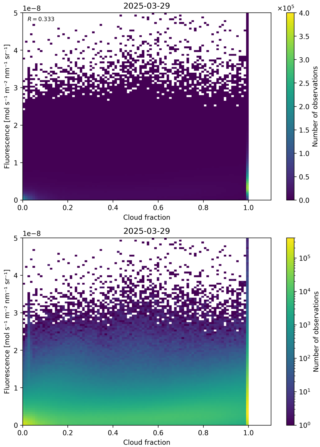
Figure 72: Scatter density plot of “Cloud fraction” against “Fluorescence” for 2025-03-28 to 2025-03-30.
