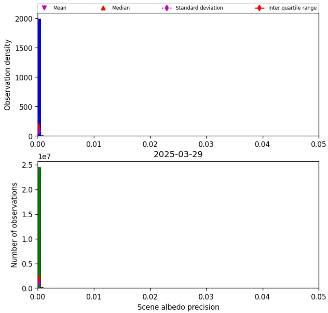
Figure 35: Histogram of “Scene albedo precision” for 2025-03-28 to 2025-03-30
