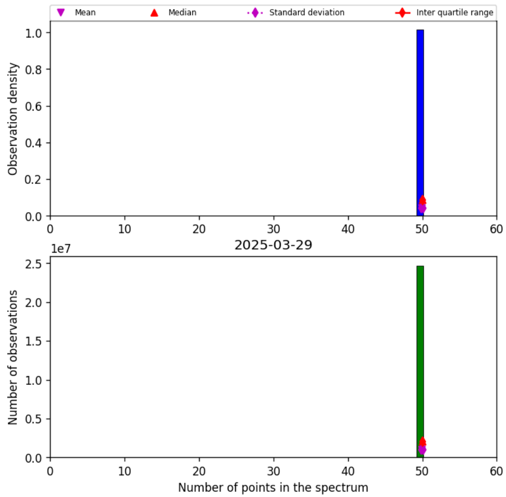
Figure 44: Histogram of “Number of points in the spectrum” for 2025-03-28 to 2025-03-30
