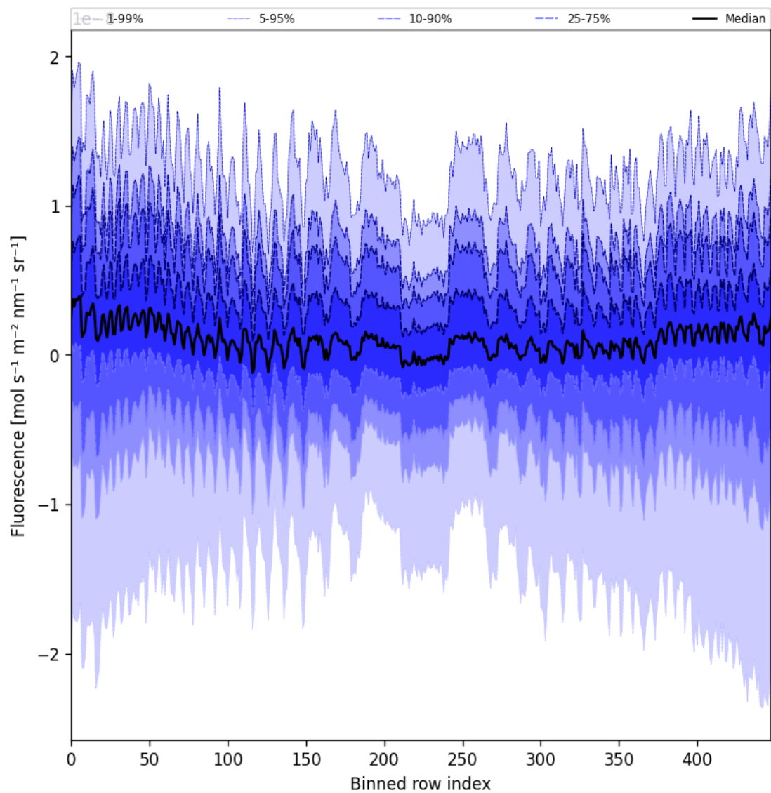
Figure 57: Along track statistics of “Fluorescence” for 2025-03-28 to 2025-03-30
