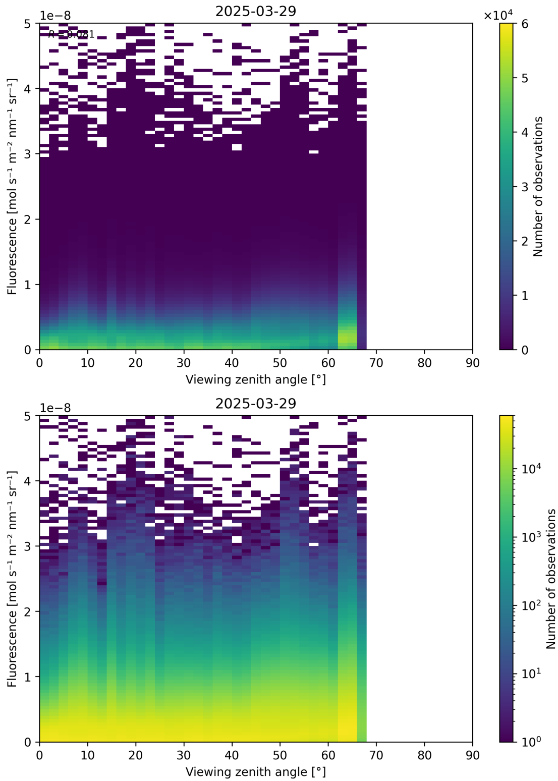
Figure 122: Scatter density plot of “Viewing zenith angle” against “Fluorescence” for 2025-03-28 to 2025-03-30.
