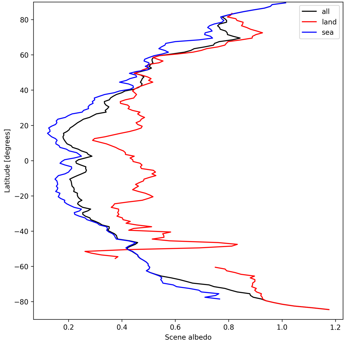
Figure 17: Zonal average of “Scene albedo” for 2025-03-28 to 2025-03-30.
