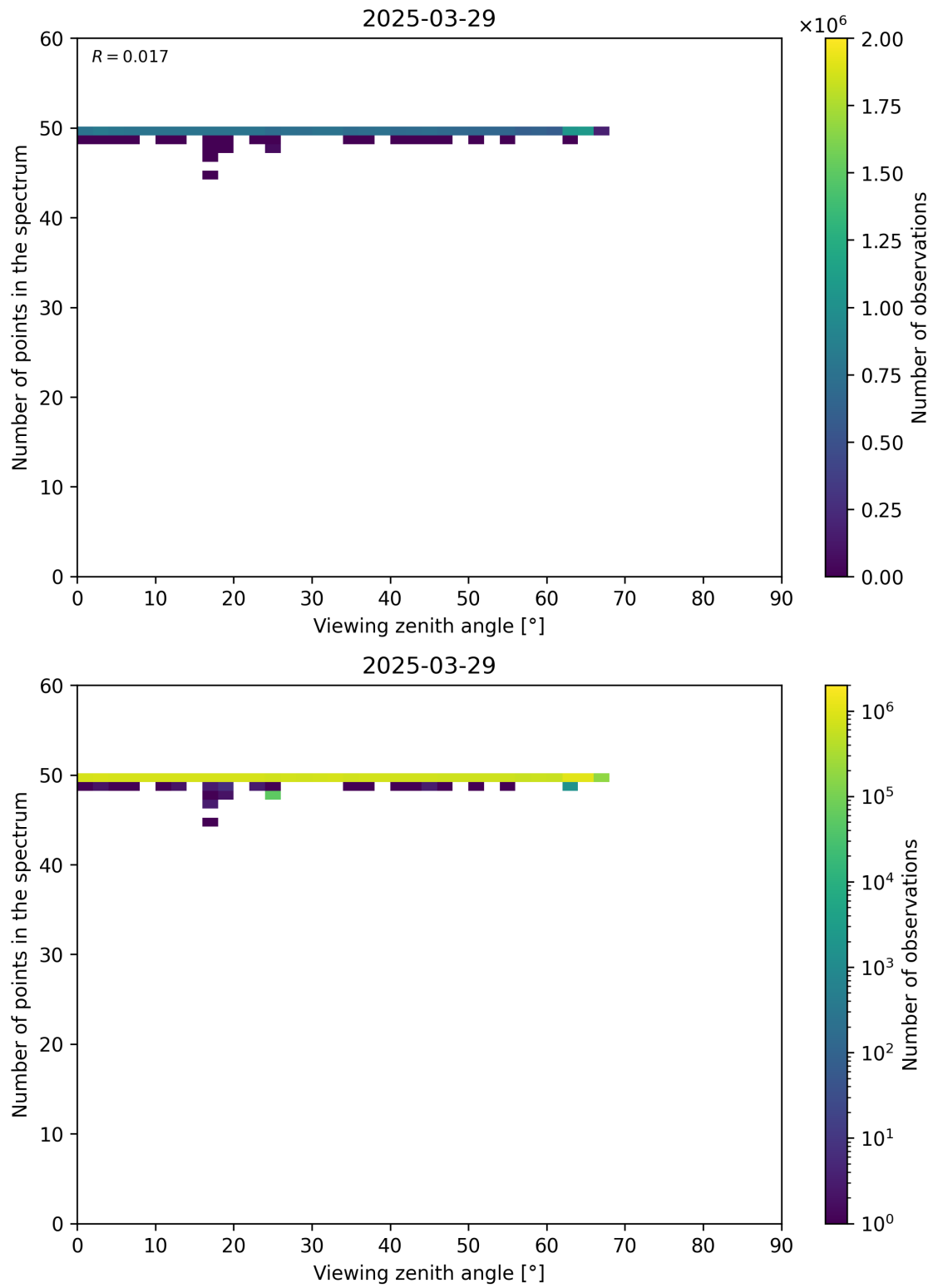
Figure 125: Scatter density plot of “Viewing zenith angle” against “Number of points in the spectrum” for 2025-03-28 to 2025-03-30.
