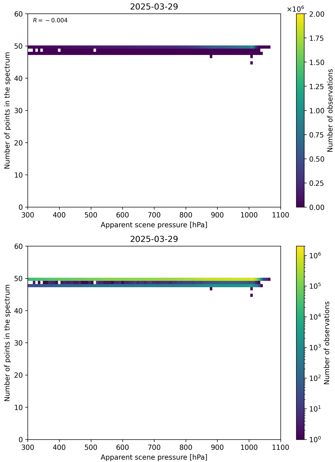
Figure 66: Scatter density plot of “Apparent scene pressure” against “Number of points in the spectrum” for 2025-03-28 to 2025-03-30.
