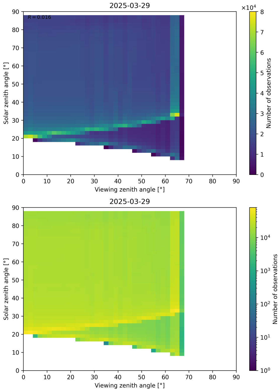
Figure 127: Scatter density plot of “Viewing zenith angle” against “Solar zenith angle” for 2025-03-28 to 2025-03-30.
