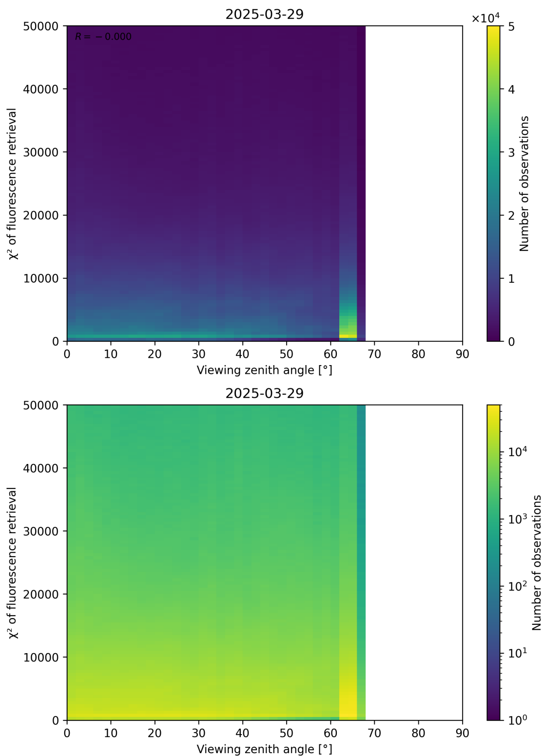
Figure 119: Scatter density plot of “Viewing zenith angle” against “ \chi^2 of fluorescence retrieval” for 2025-03-28 to 2025-03-30.
