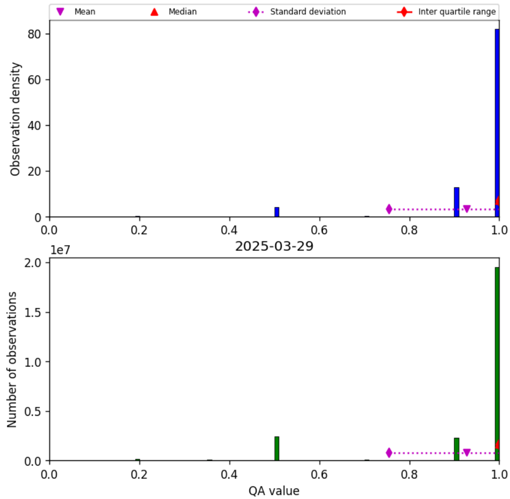
Figure 29: Histogram of “QA value” for 2025-03-28 to 2025-03-30
