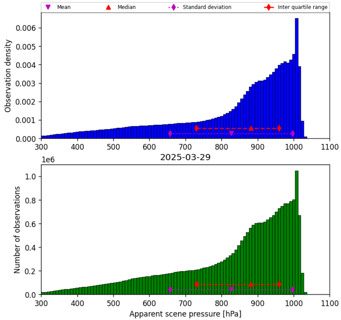
Figure 36: Histogram of “Apparent scene pressure” for 2025-03-28 to 2025-03-30
