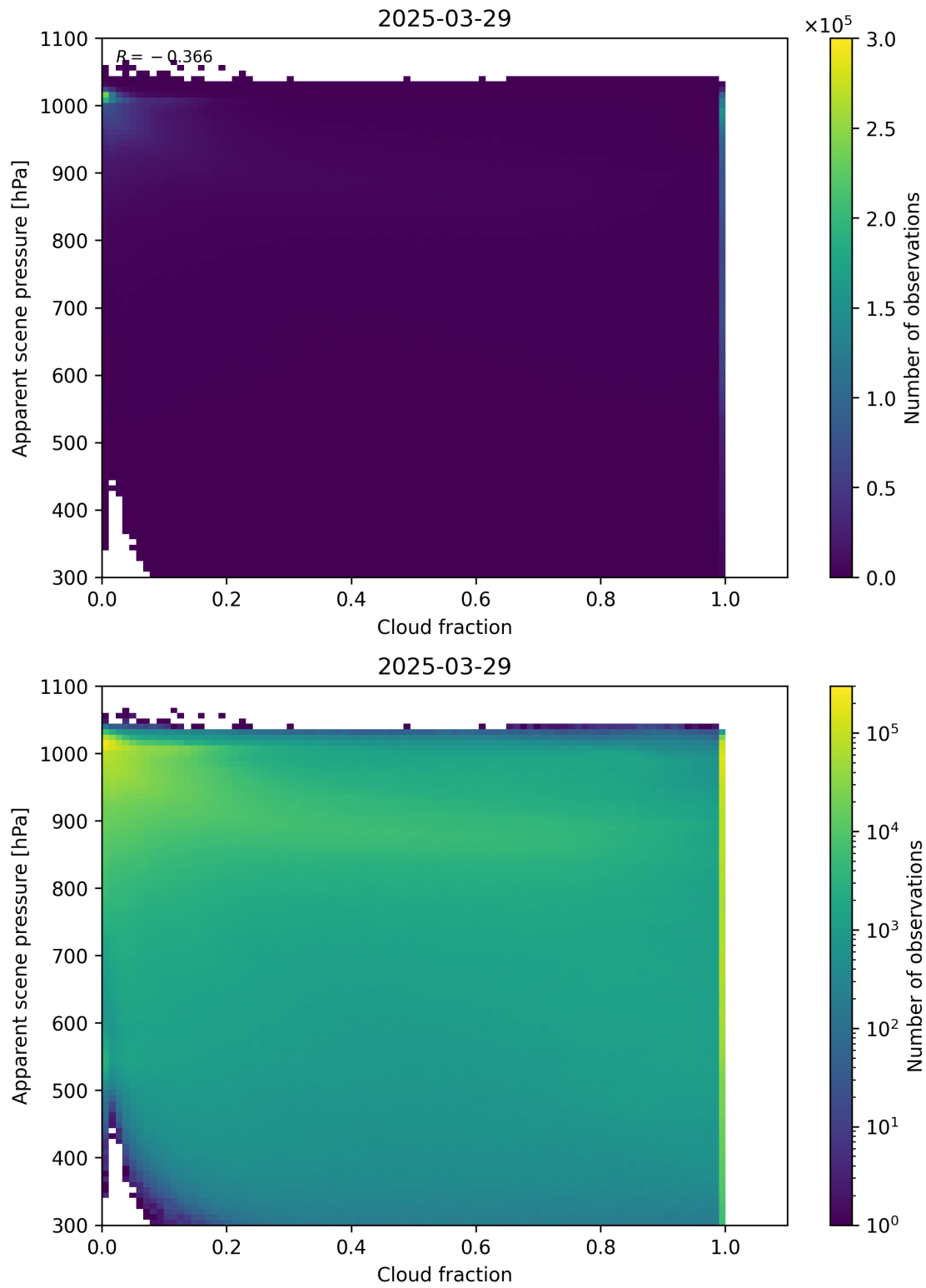
Figure 70: Scatter density plot of “Cloud fraction” against “Apparent scene pressure” for 2025-03-28 to 2025-03-30.
