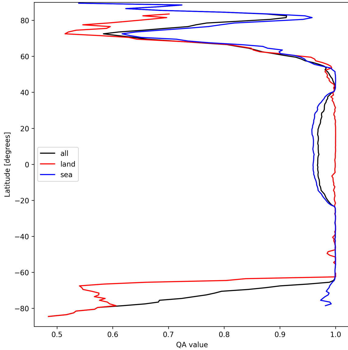
Figure 12: Zonal average of “QA value” for 2025-03-28 to 2025-03-30.
