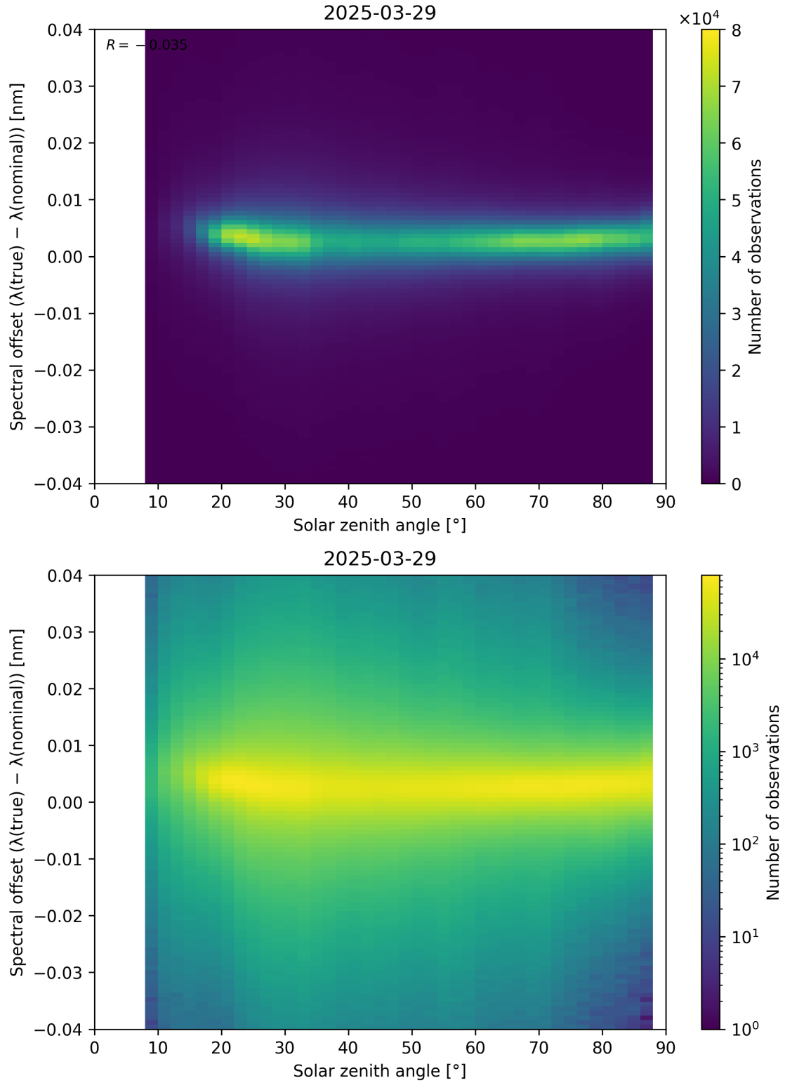
Figure 117: Scatter density plot of “Solar zenith angle” against “Spectral offset ( \lambda_{\text{true}} - \lambda_{\text{nominal}} )” for 2025-03-28 to 2025-03-30.
