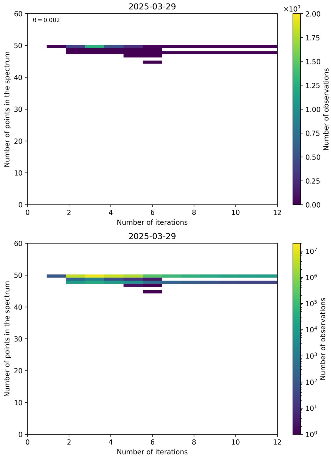
Figure 99: Scatter density plot of “Number of iterations” against “Number of points in the spectrum” for 2025-03-28 to 2025-03-30.
