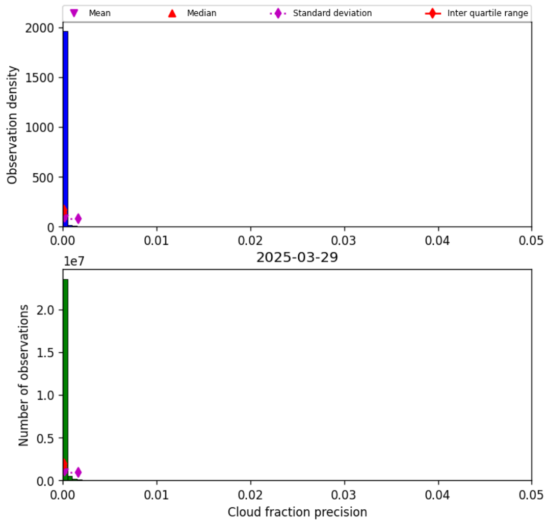
Figure 33: Histogram of “Cloud fraction precision” for 2025-03-28 to 2025-03-30
