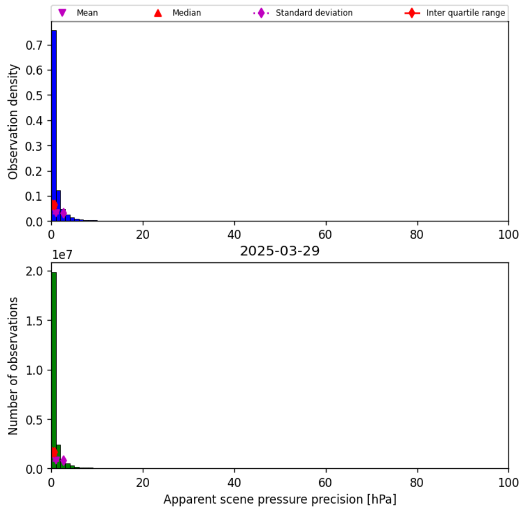
Figure 37: Histogram of “Apparent scene pressure precision” for 2025-03-28 to 2025-03-30
