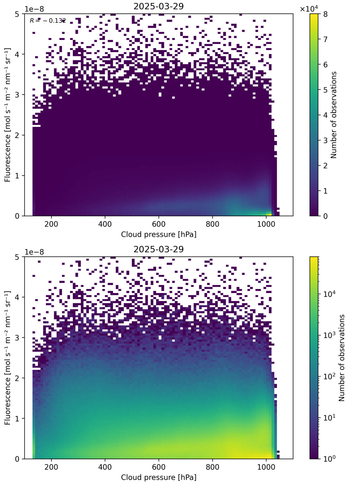
Figure 80: Scatter density plot of “Cloud pressure” against “Fluorescence” for 2025-03-28 to 2025-03-30.
