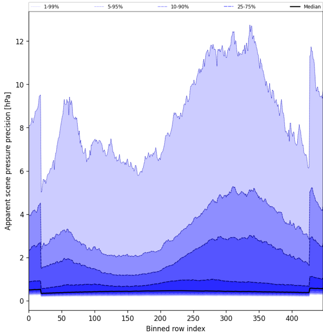
Figure 54: Along track statistics of “Apparent scene pressure precision” for 2025-03-28 to 2025-03-30
