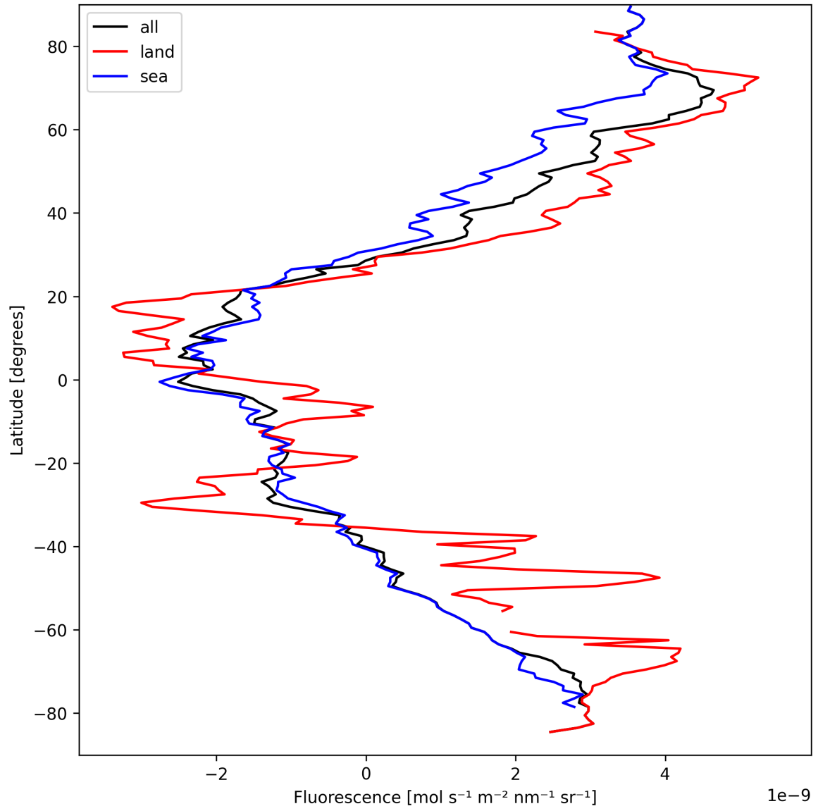
Figure 23: Zonal average of “Fluorescence” for 2025-03-28 to 2025-03-30.
