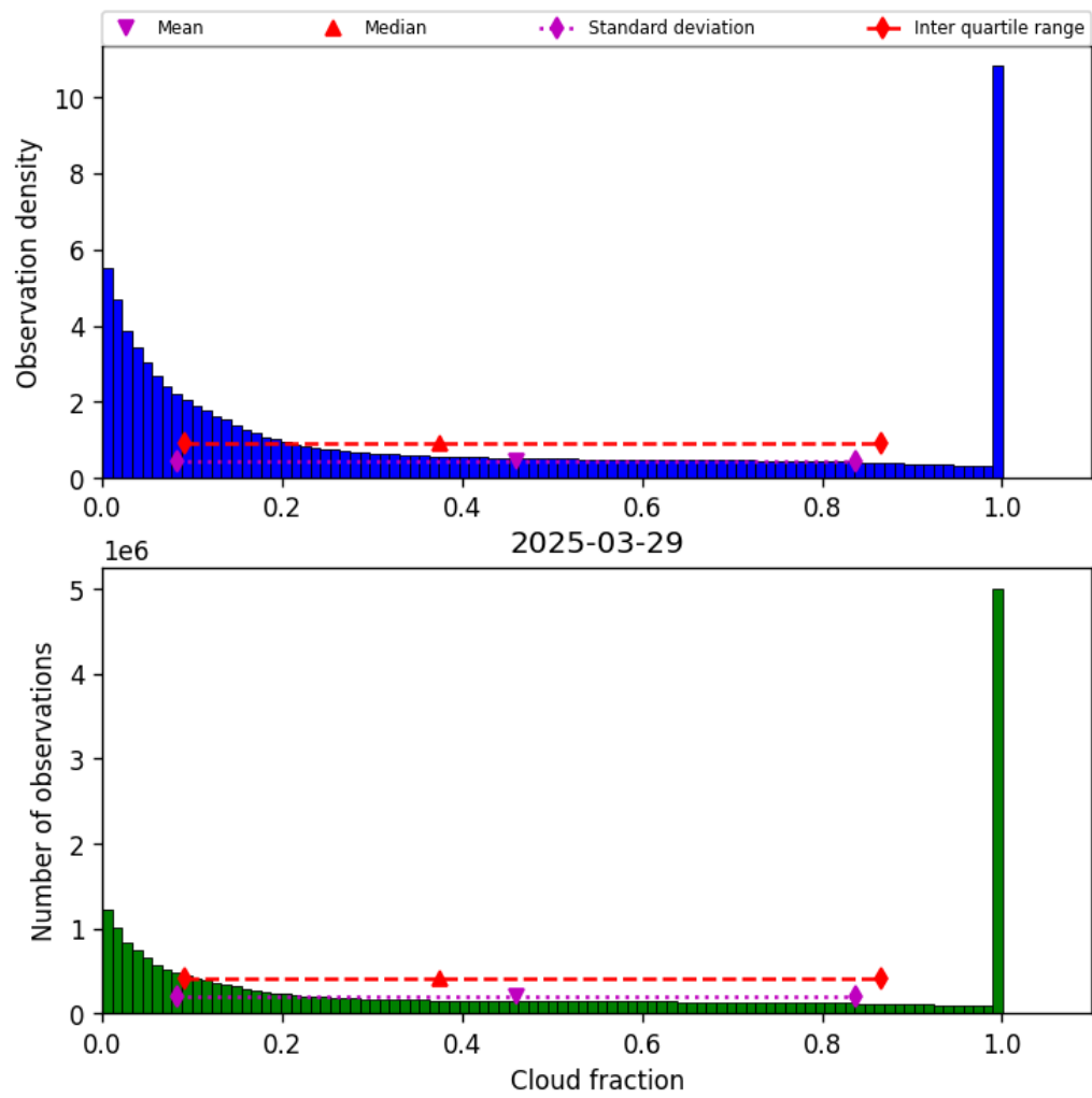
Figure 32: Histogram of “Cloud fraction” for 2025-03-28 to 2025-03-30
