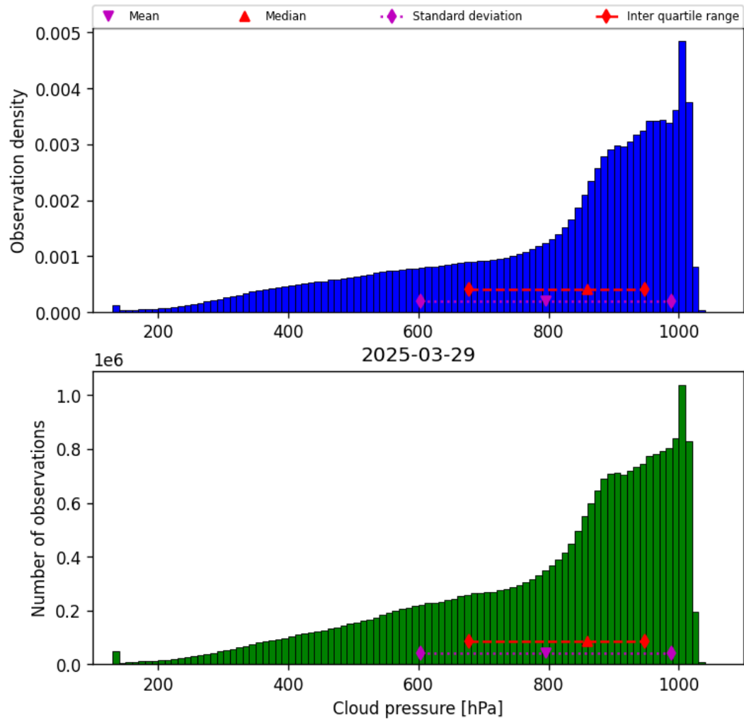
Figure 30: Histogram of “Cloud pressure” for 2025-03-28 to 2025-03-30
