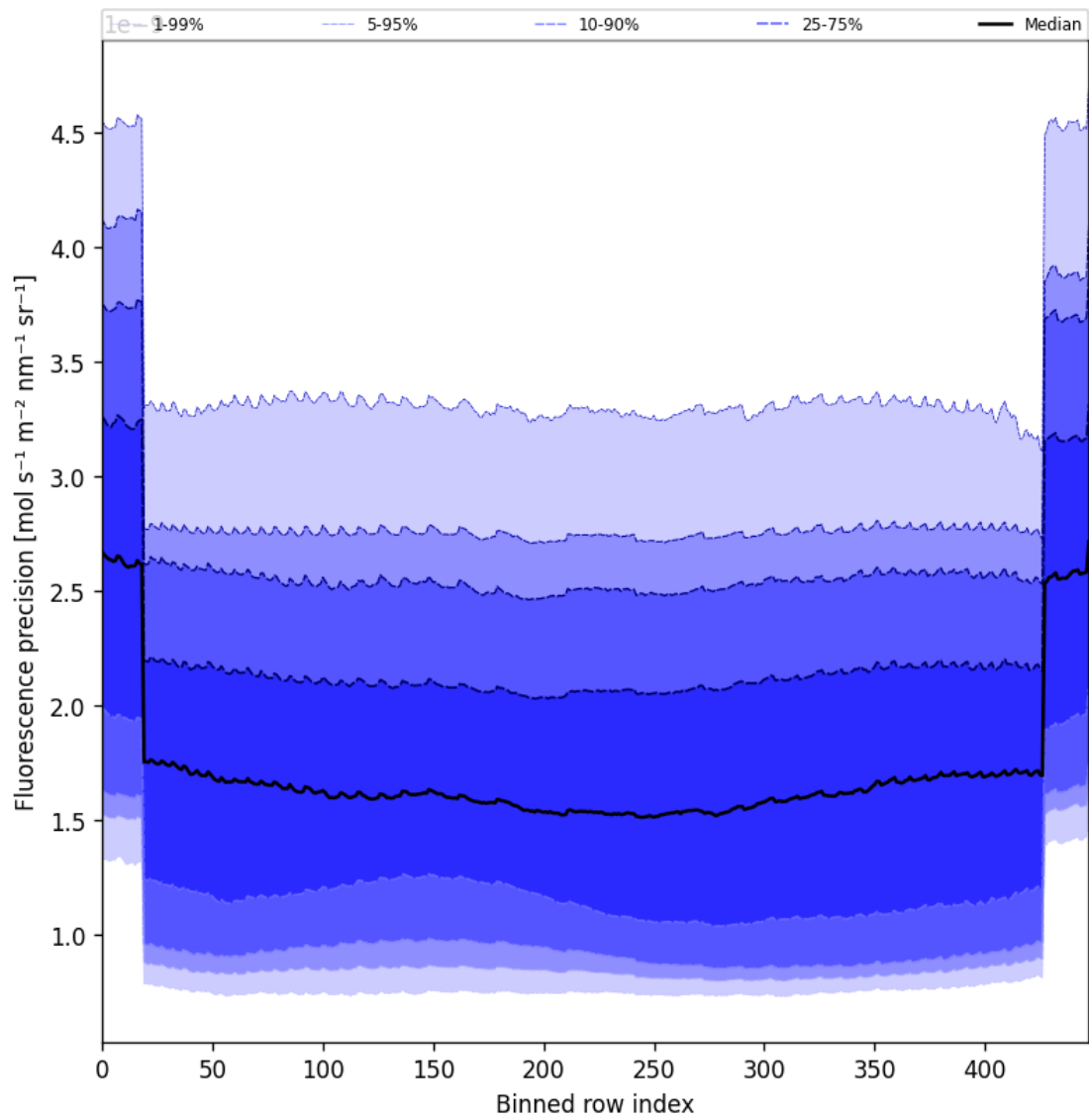
Figure 58: Along track statistics of “Fluorescence precision” for 2025-03-28 to 2025-03-30
