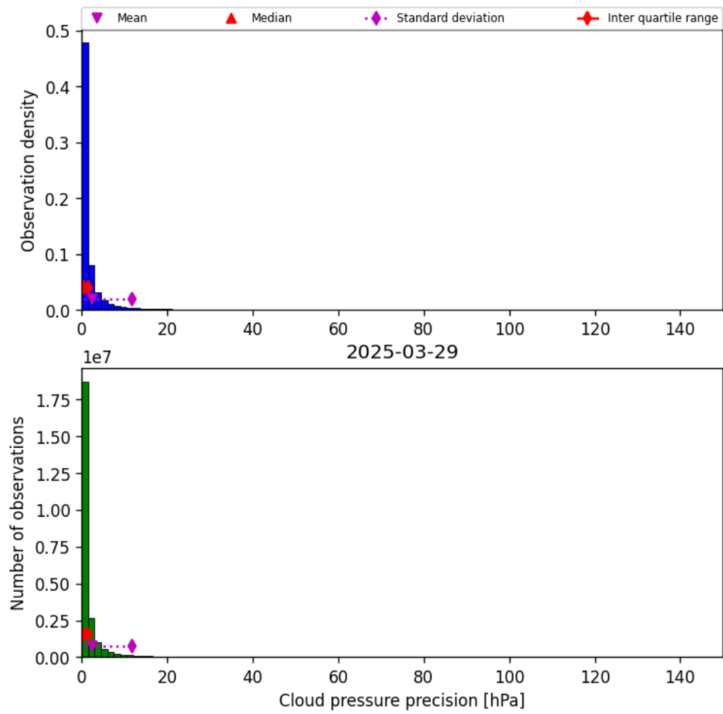
Figure 31: Histogram of “Cloud pressure precision” for 2025-03-28 to 2025-03-30
