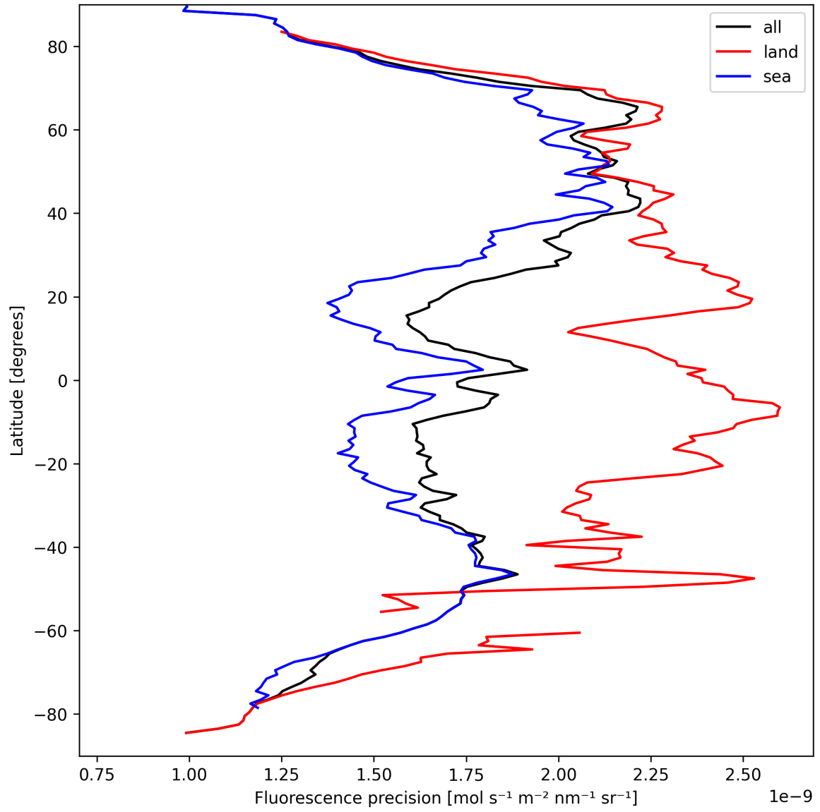
Figure 24: Zonal average of “Fluorescence precision” for 2025-03-28 to 2025-03-30.
