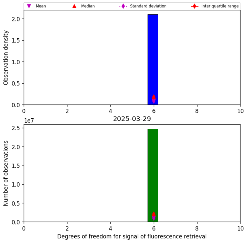
Figure 43: Histogram of “Degrees of freedom for signal of fluorescence retrieval” for 2025-03-28 to 2025-03-30
