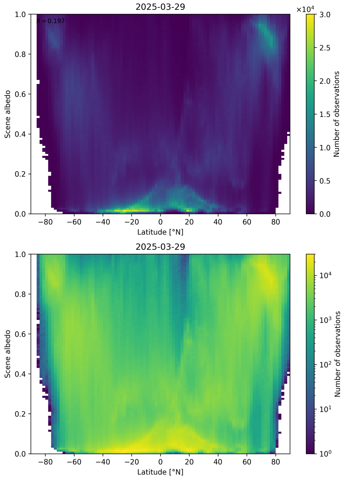
Figure 95: Scatter density plot of “Latitude” against “Scene albedo” for 2025-03-28 to 2025-03-30.
