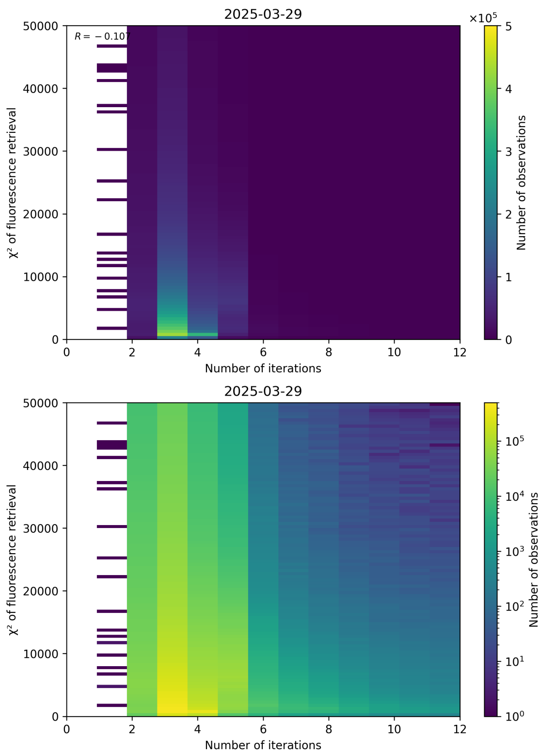
Figure 97: Scatter density plot of “Number of iterations” against “ \chi^2 of fluorescence retrieval” for 2025-03-28 to 2025-03-30.
