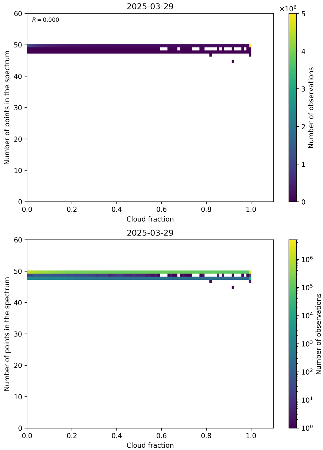
Figure 74: Scatter density plot of “Cloud fraction” against “Number of points in the spectrum” for 2025-03-28 to 2025-03-30.
