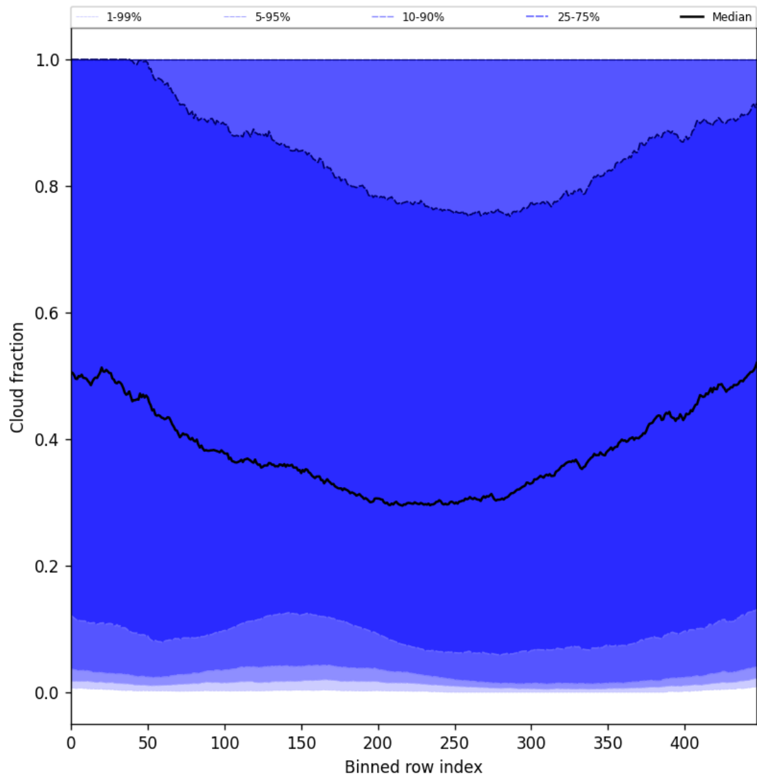
Figure 49: Along track statistics of “Cloud fraction” for 2025-03-28 to 2025-03-30
