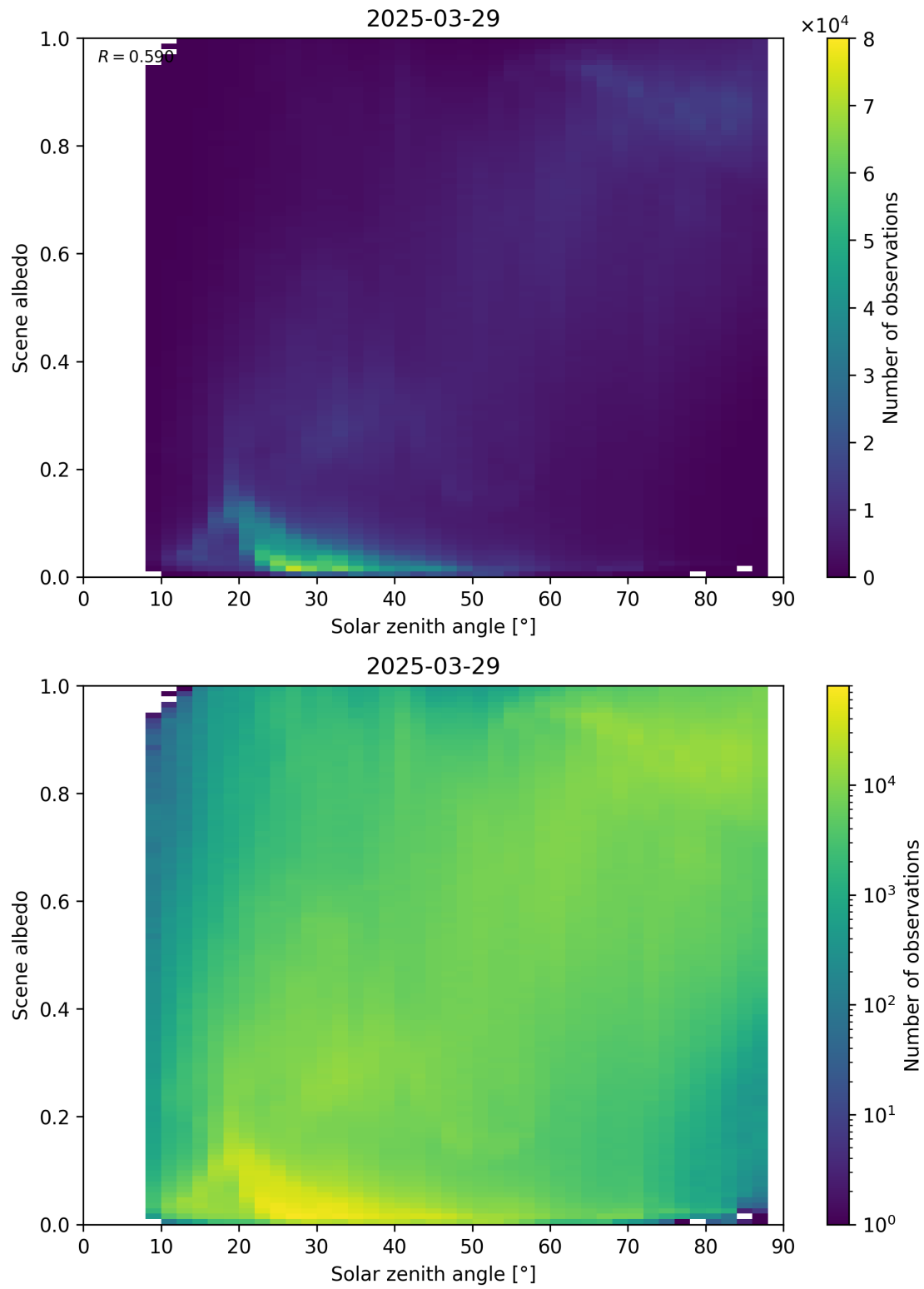
Figure 116: Scatter density plot of “Solar zenith angle” against “Scene albedo” for 2025-03-28 to 2025-03-30.
