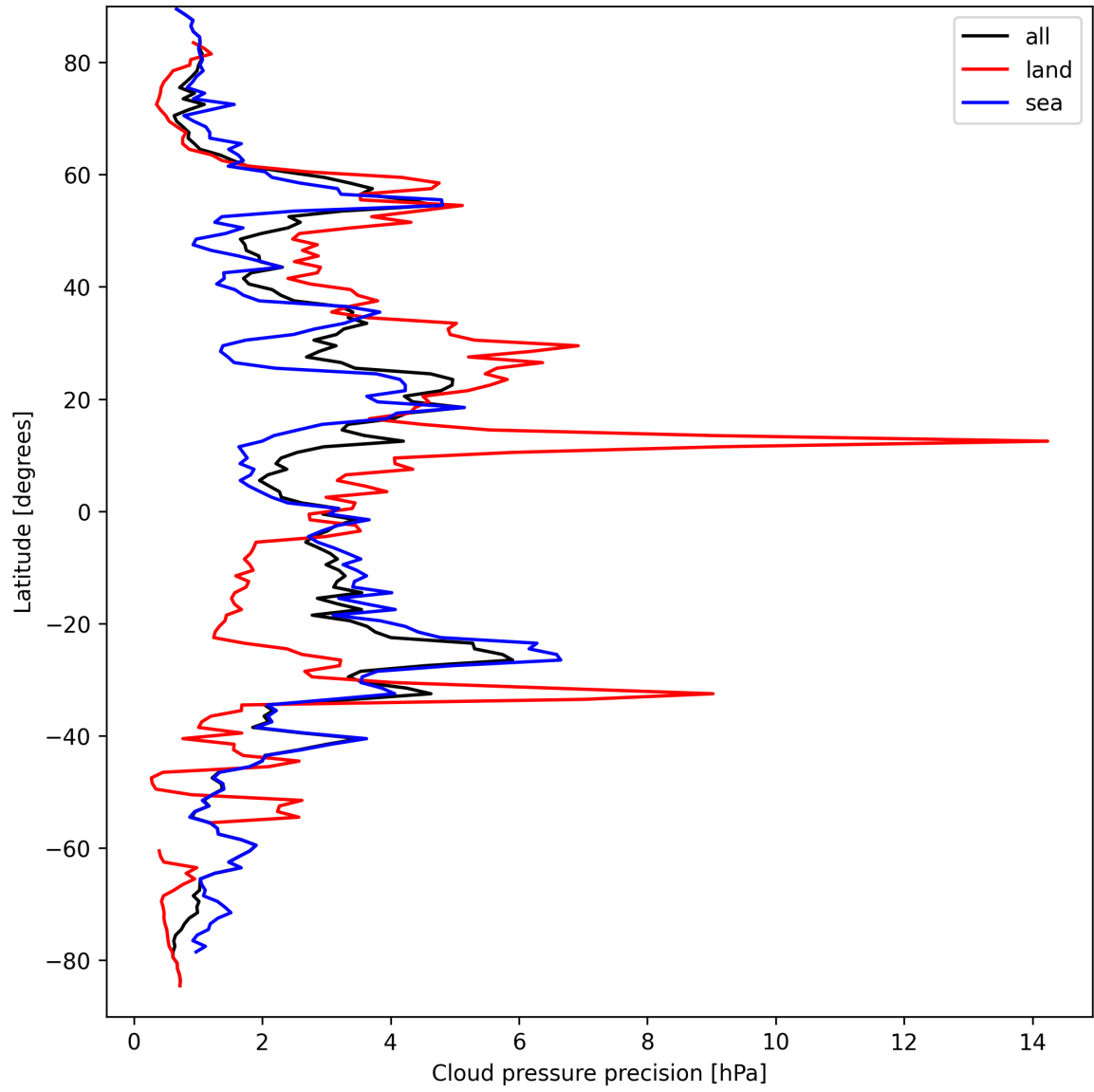
Figure 14: Zonal average of “Cloud pressure precision” for 2025-03-28 to 2025-03-30.
