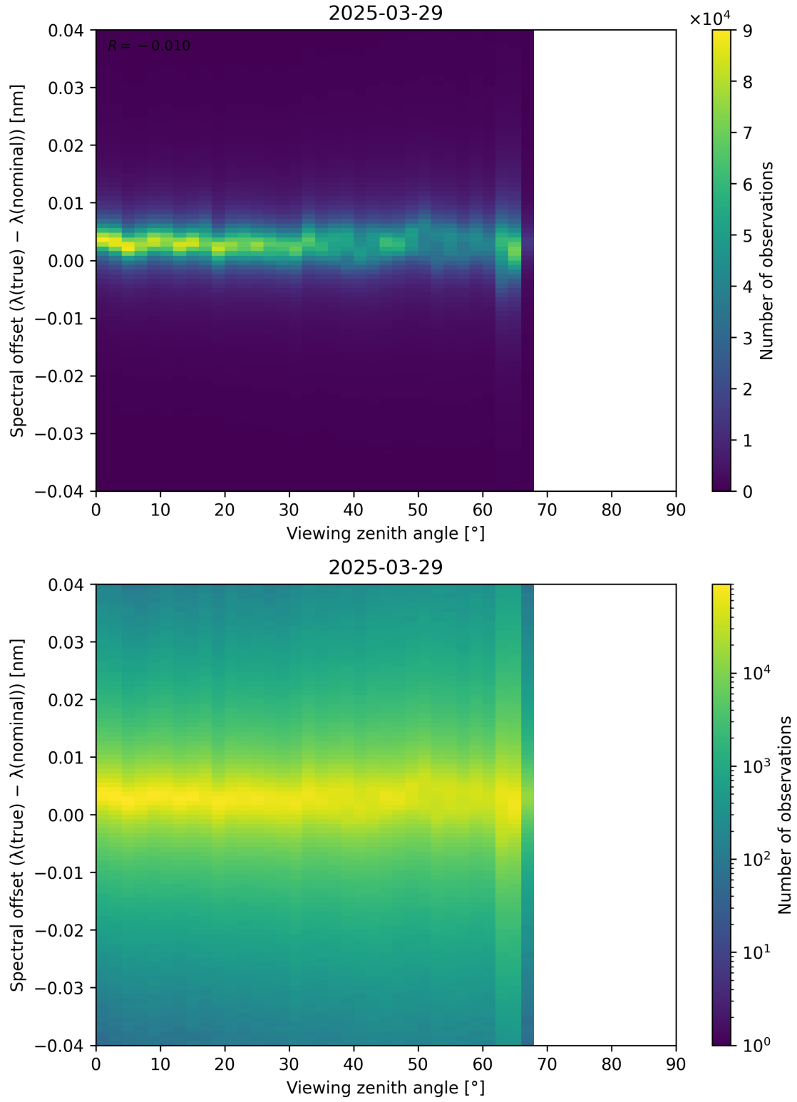
Figure 128: Scatter density plot of “Viewing zenith angle” against “Spectral offset ( \lambda_{\text{true}} - \lambda_{\text{nominal}} )” for 2025-03-28 to 2025-03-30.
