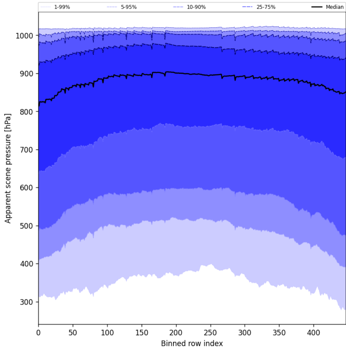
Figure 53: Along track statistics of “Apparent scene pressure” for 2025-03-28 to 2025-03-30
