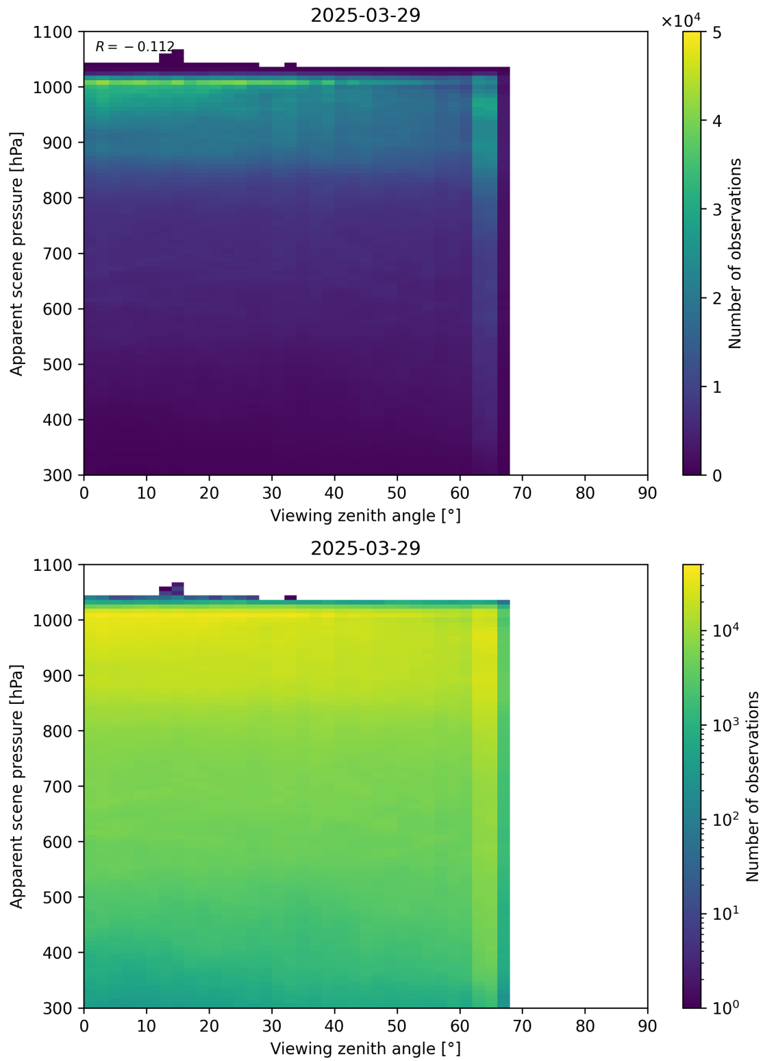
Figure 118: Scatter density plot of “Viewing zenith angle” against “Apparent scene pressure” for 2025-03-28 to 2025-03-30.
