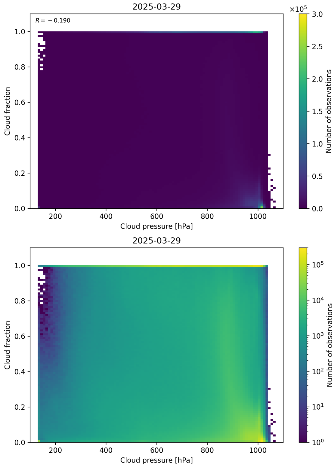
Figure 79: Scatter density plot of “Cloud pressure” against “Cloud fraction” for 2025-03-28 to 2025-03-30.
