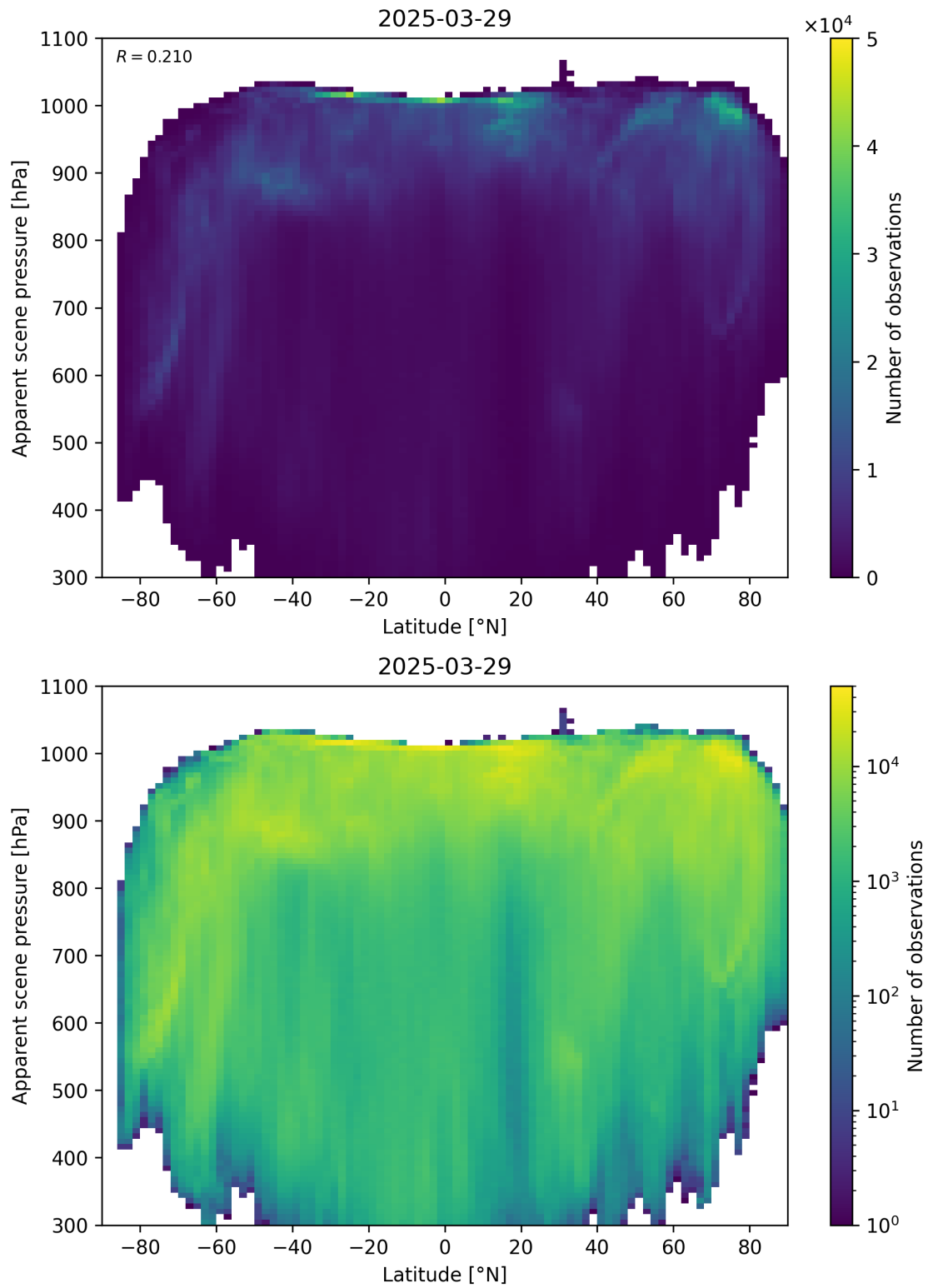
Figure 88: Scatter density plot of “Latitude” against “Apparent scene pressure” for 2025-03-28 to 2025-03-30.
