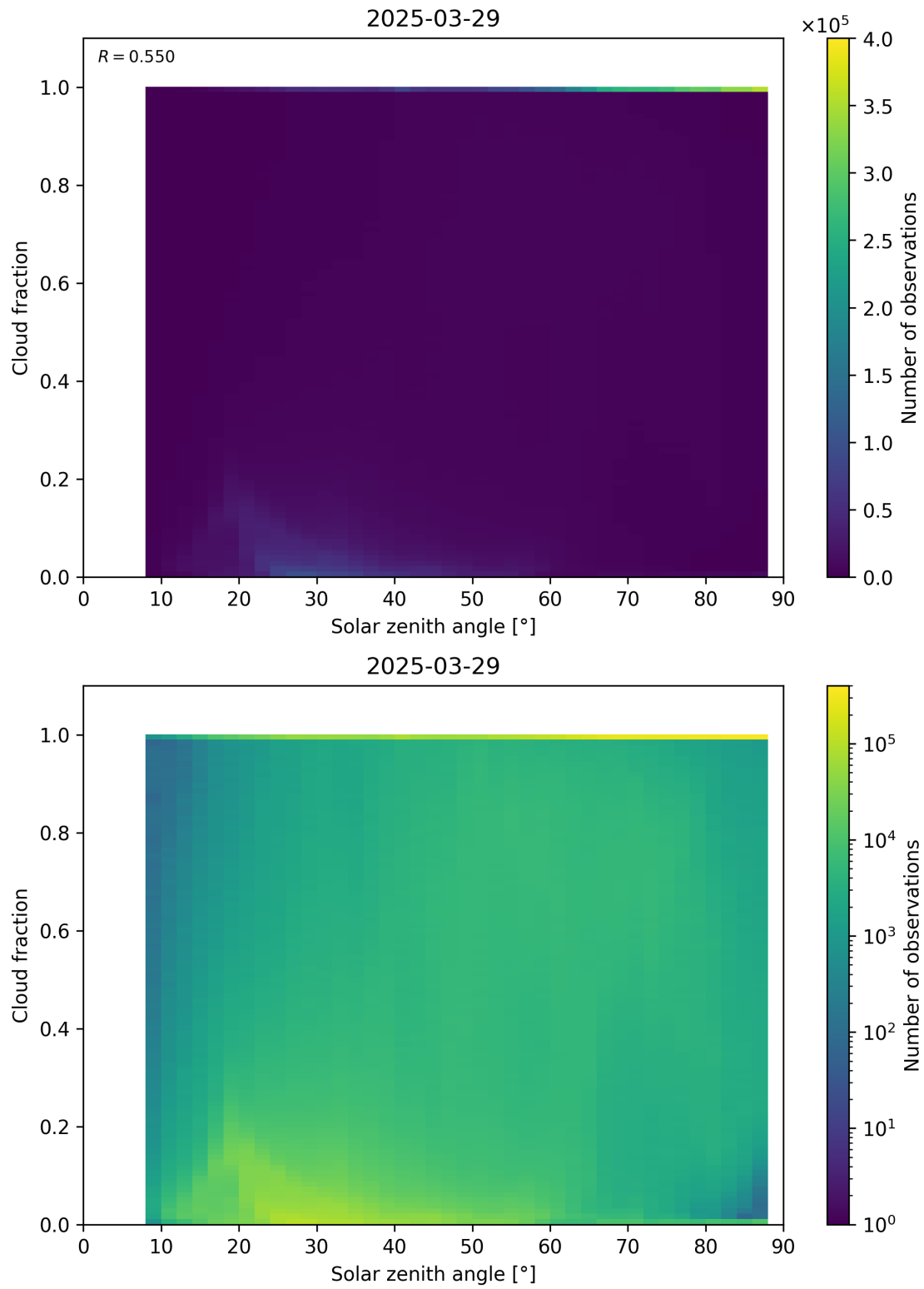
Figure 110: Scatter density plot of “Solar zenith angle” against “Cloud fraction” for 2025-03-28 to 2025-03-30.
