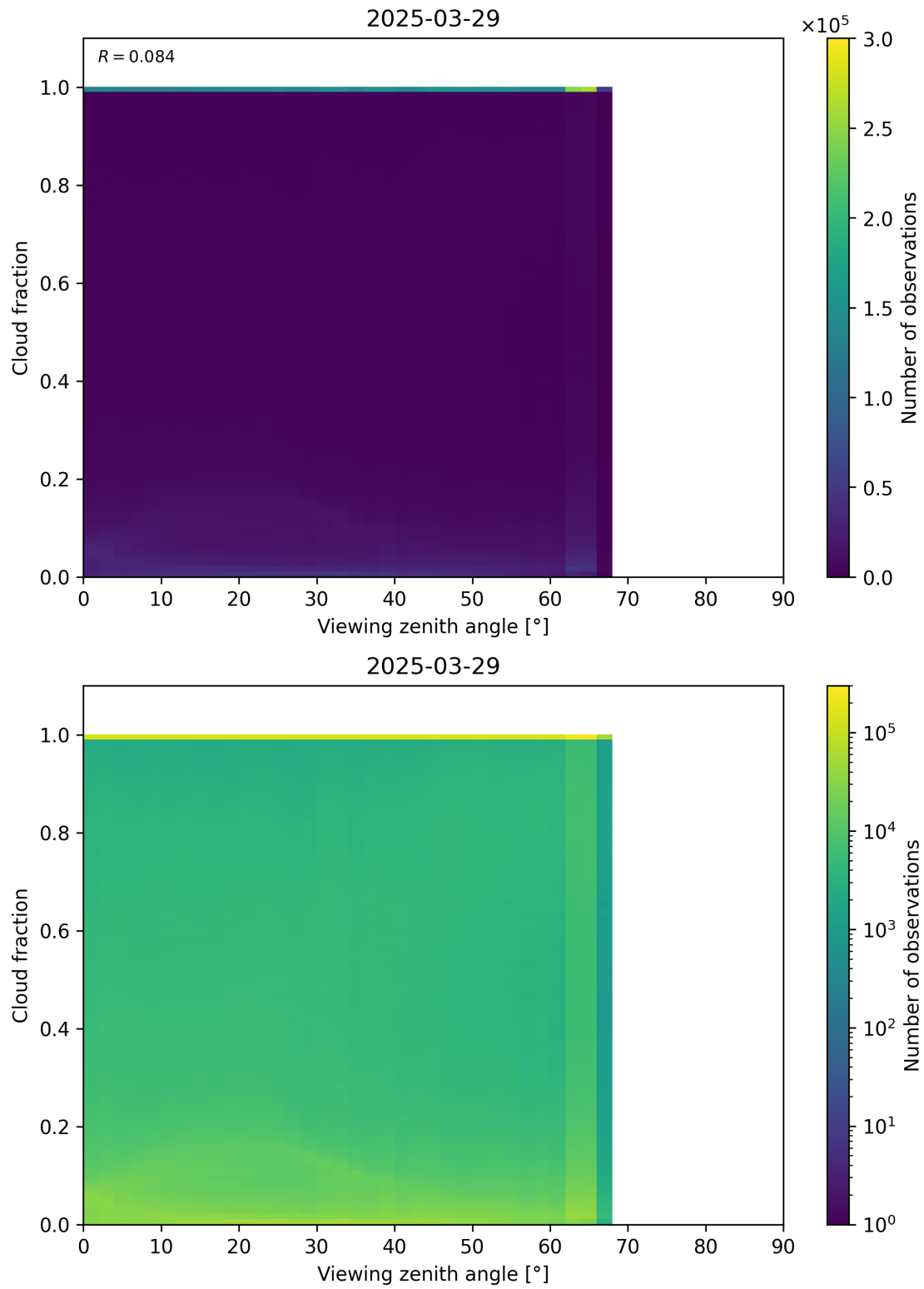
Figure 120: Scatter density plot of “Viewing zenith angle” against “Cloud fraction” for 2025-03-28 to 2025-03-30.
