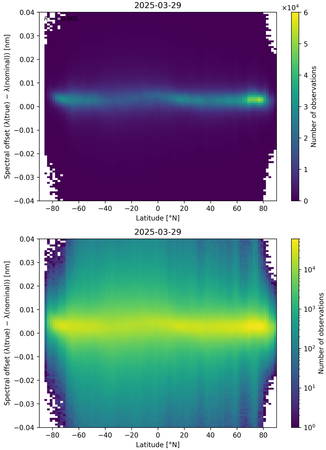
Figure 96: Scatter density plot of “Latitude” against “Spectral offset ( \lambda_{\text{true}} - \lambda_{\text{nominal}} )” for 2025-03-28 to 2025-03-30.
