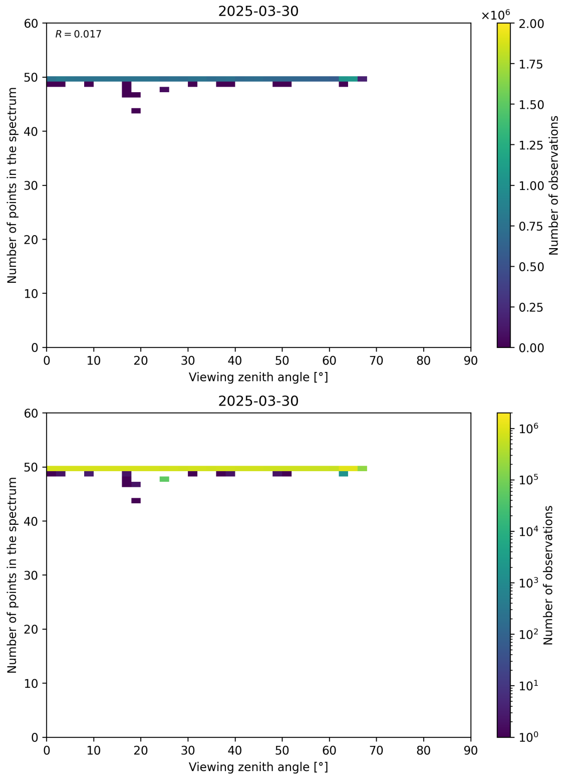
Figure 125: Scatter density plot of “Viewing zenith angle” against “Number of points in the spectrum” for 2025-03-29 to 2025-03-31.
