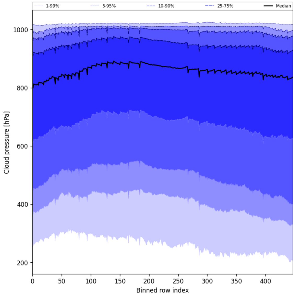
Figure 47: Along track statistics of “Cloud pressure” for 2025-03-29 to 2025-03-31
