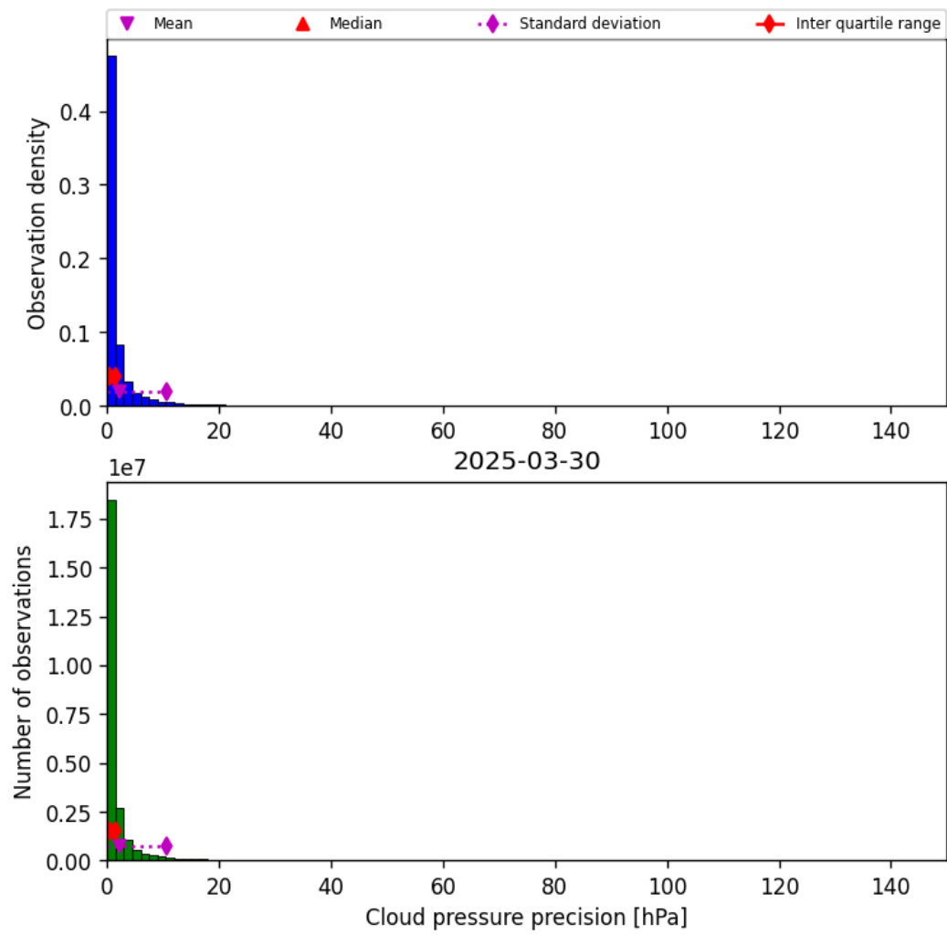
Figure 31: Histogram of “Cloud pressure precision” for 2025-03-29 to 2025-03-31
