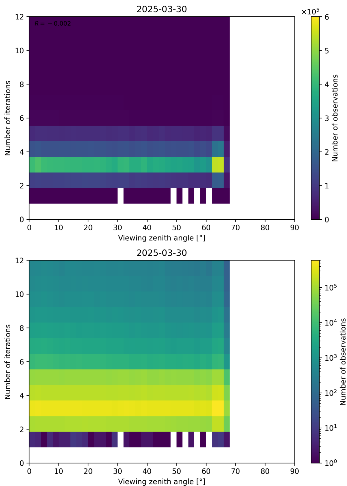
Figure 124: Scatter density plot of “Viewing zenith angle” against “Number of iterations” for 2025-03-29 to 2025-03-31.
