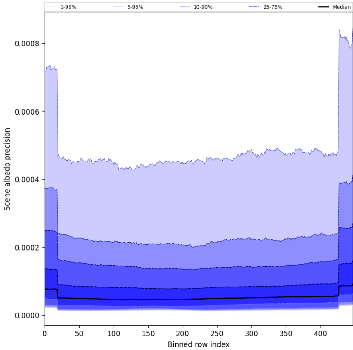
Figure 52: Along track statistics of “Scene albedo precision” for 2025-03-29 to 2025-03-31
