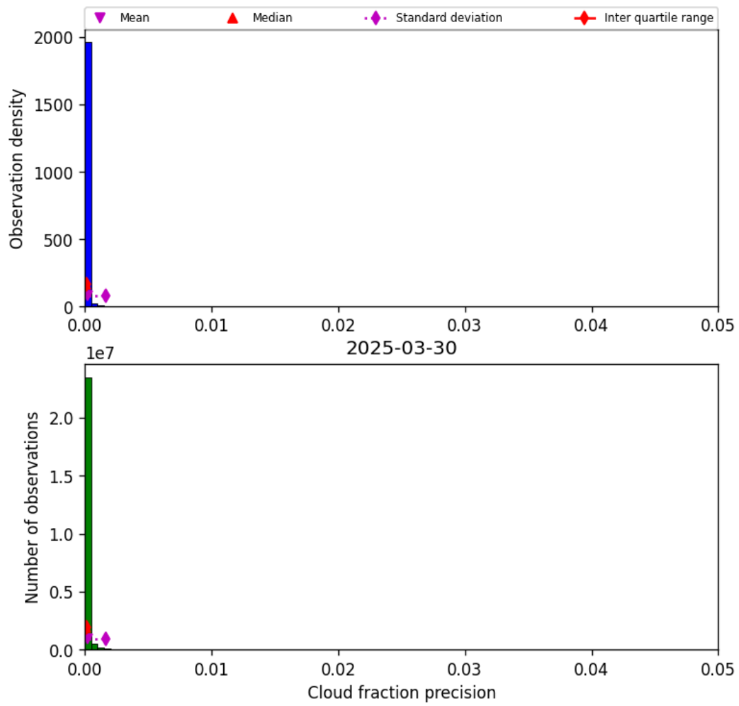
Figure 33: Histogram of “Cloud fraction precision” for 2025-03-29 to 2025-03-31
