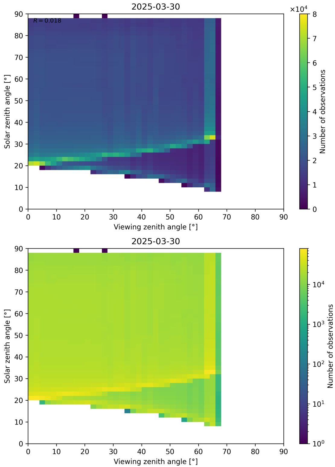
Figure 127: Scatter density plot of “Viewing zenith angle” against “Solar zenith angle” for 2025-03-29 to 2025-03-31.
