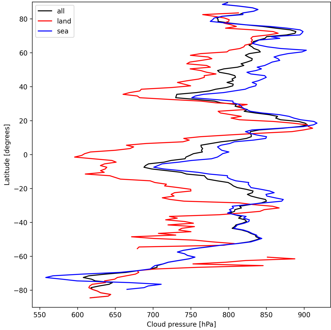
Figure 13: Zonal average of “Cloud pressure” for 2025-03-29 to 2025-03-31.
