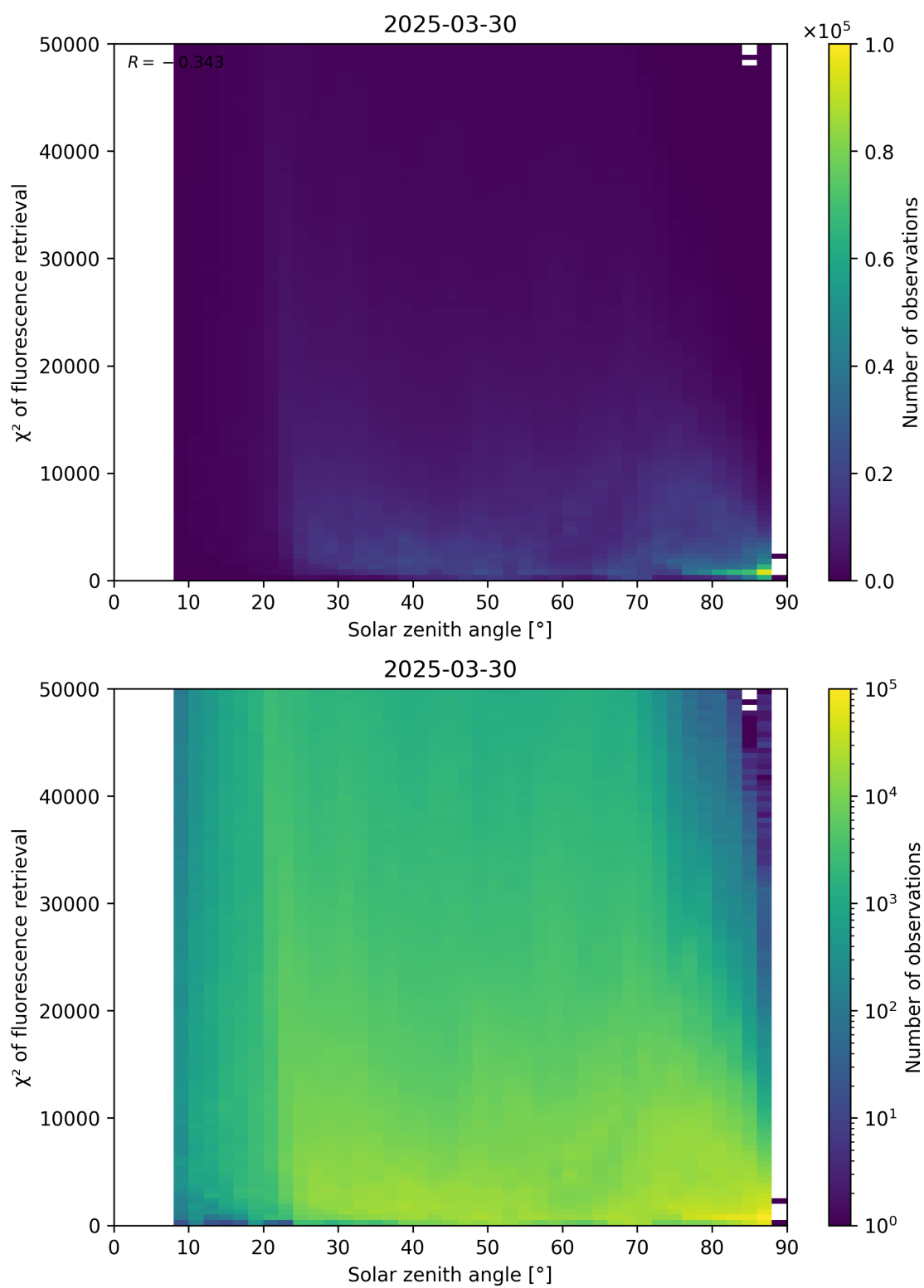
Figure 109: Scatter density plot of “Solar zenith angle” against “ \chi^2 of fluorescence retrieval” for 2025-03-29 to 2025-03-31.
