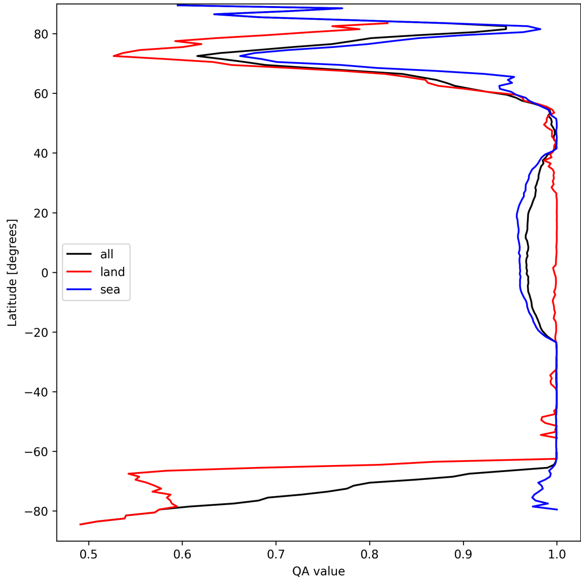
Figure 12: Zonal average of “QA value” for 2025-03-29 to 2025-03-31.
