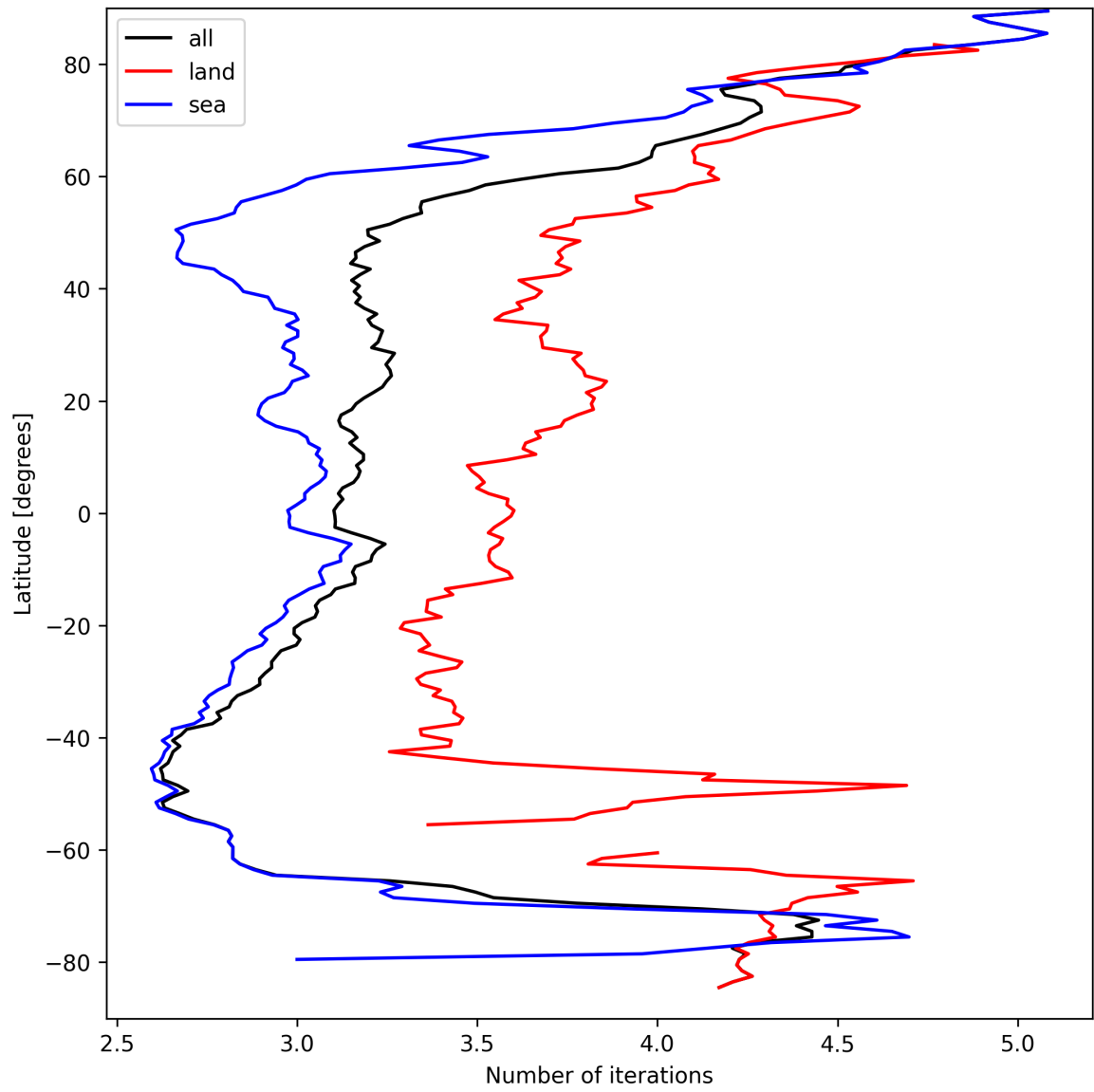
Figure 22: Zonal average of “Number of iterations” for 2025-03-29 to 2025-03-31.
