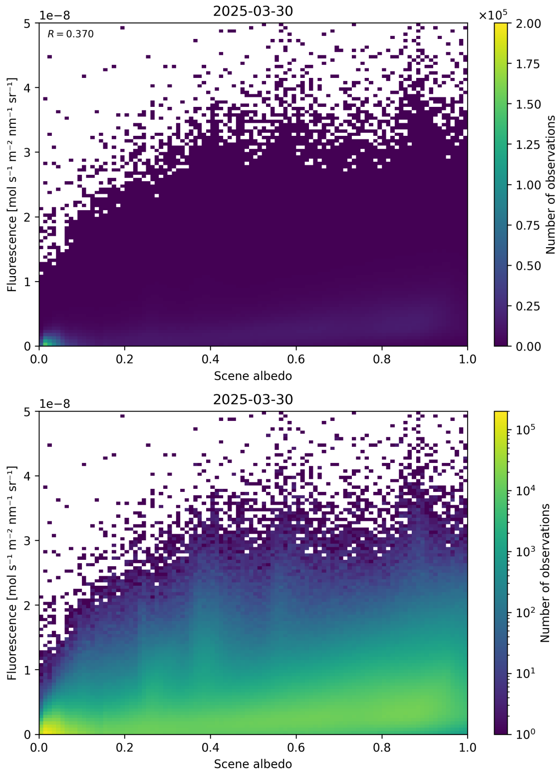
Figure 104: Scatter density plot of “Scene albedo” against “Fluorescence” for 2025-03-29 to 2025-03-31.
