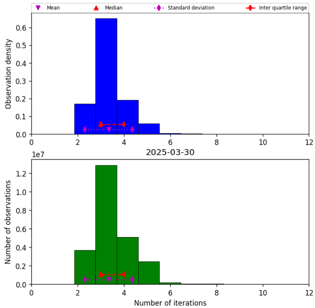
Figure 39: Histogram of “Number of iterations” for 2025-03-29 to 2025-03-31
