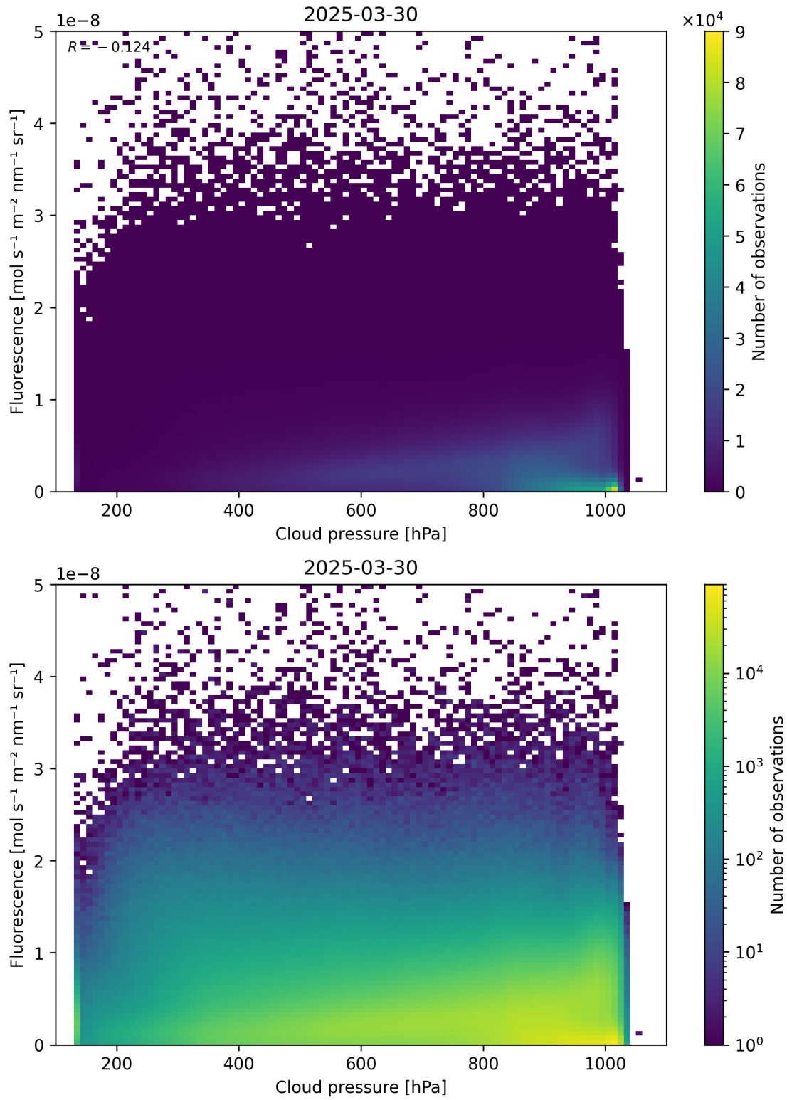
Figure 80: Scatter density plot of “Cloud pressure” against “Fluorescence” for 2025-03-29 to 2025-03-31.
