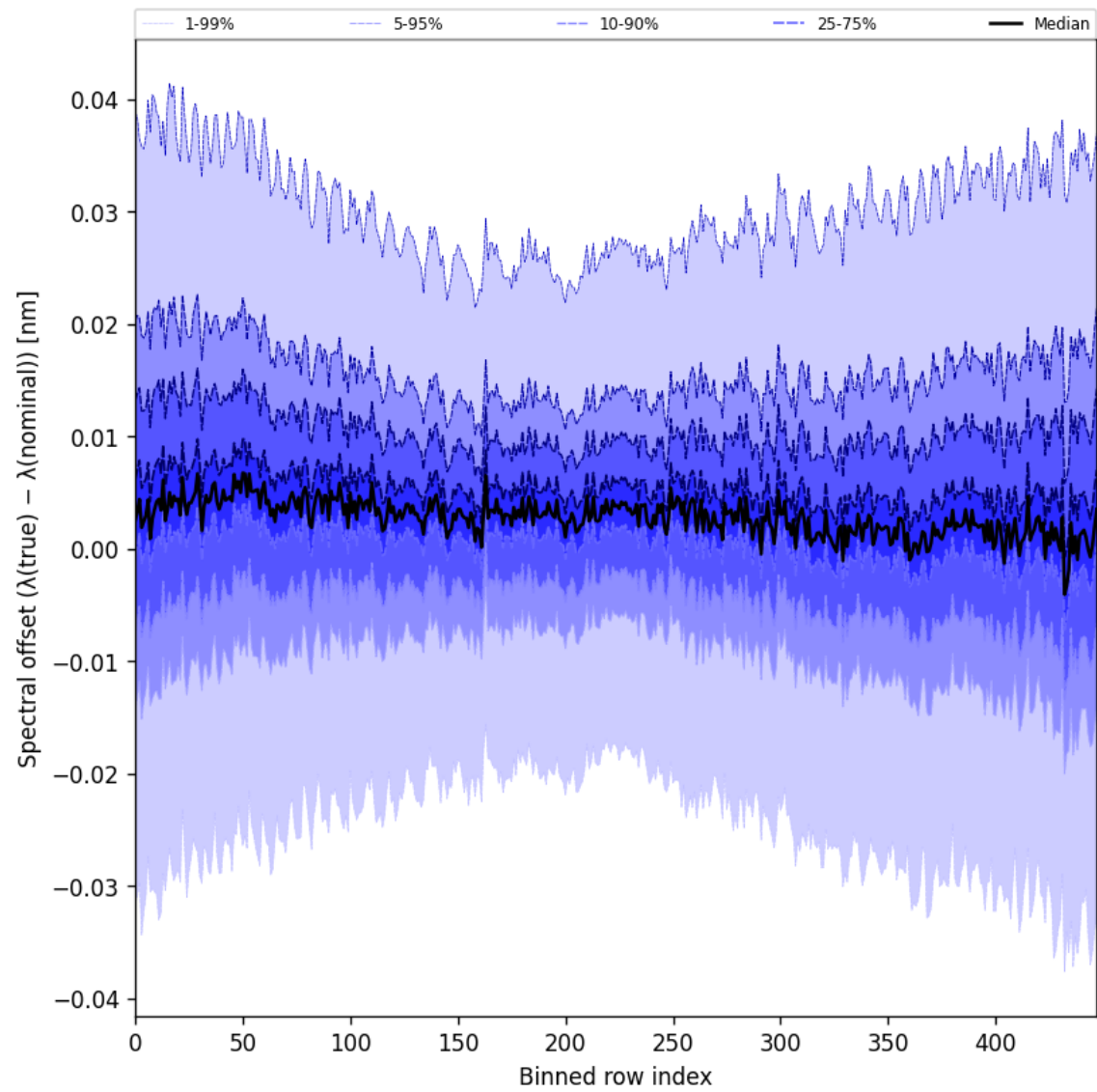
Figure 62: Along track statistics of “Spectral offset ( \lambda_{\text{true}} - \lambda_{\text{nominal}} )” for 2025-03-29 to 2025-03-31
