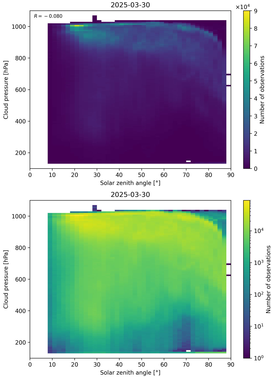
Figure 111: Scatter density plot of “Solar zenith angle” against “Cloud pressure” for 2025-03-29 to 2025-03-31.
