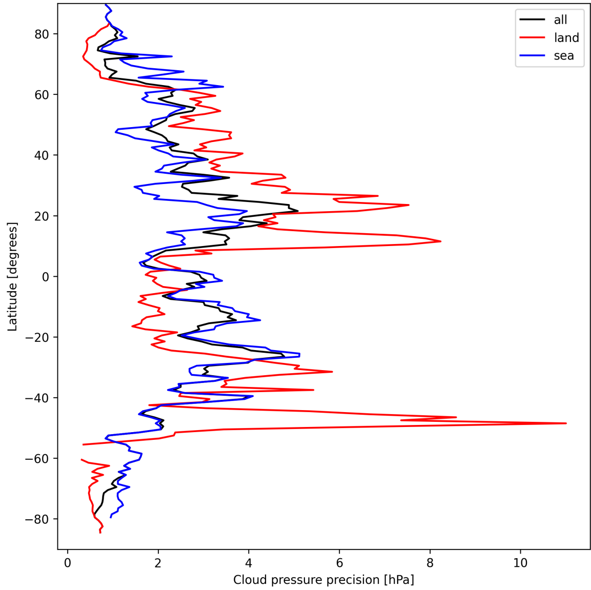
Figure 14: Zonal average of “Cloud pressure precision” for 2025-03-29 to 2025-03-31.
