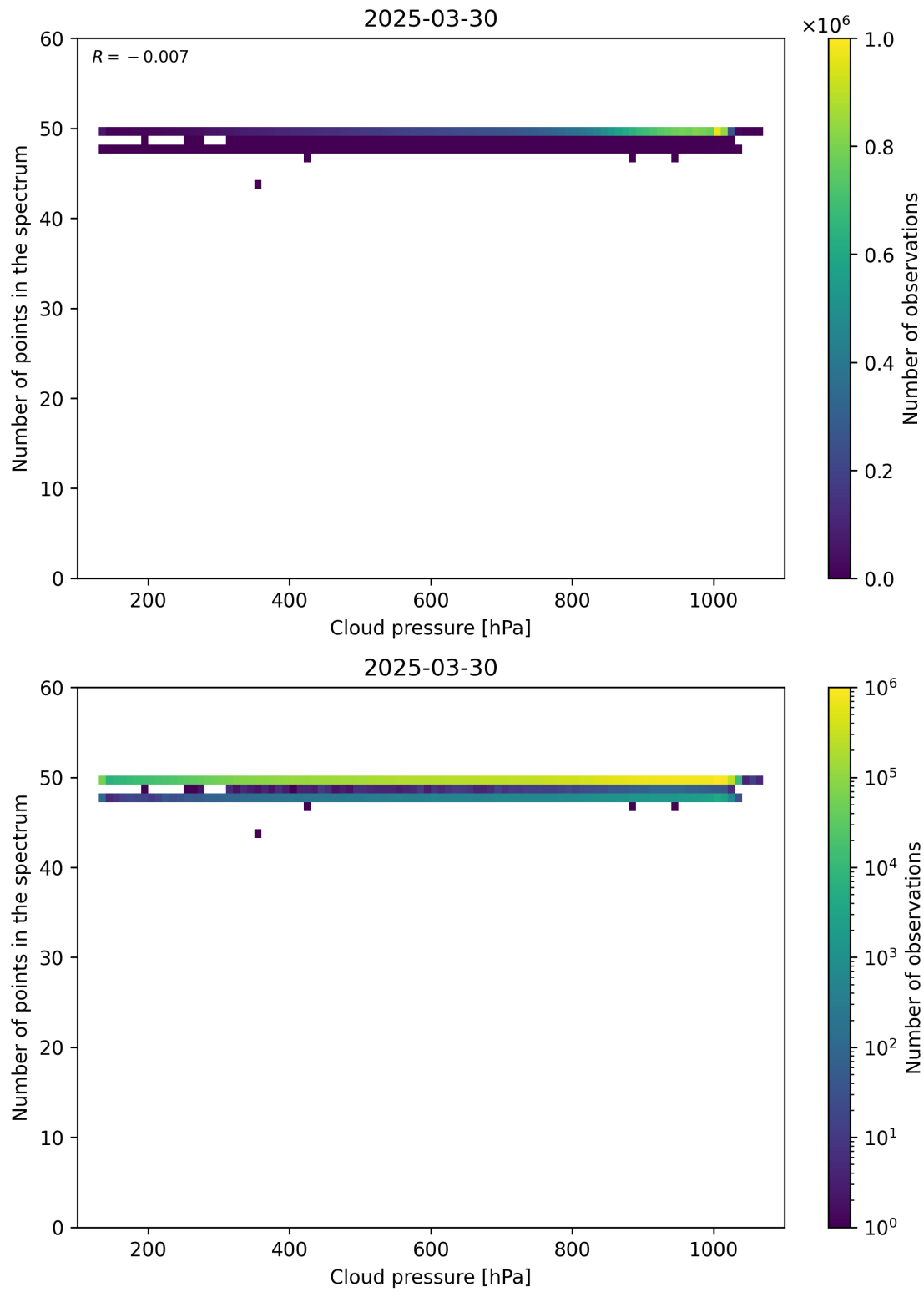
Figure 82: Scatter density plot of “Cloud pressure” against “Number of points in the spectrum” for 2025-03-29 to 2025-03-31.
