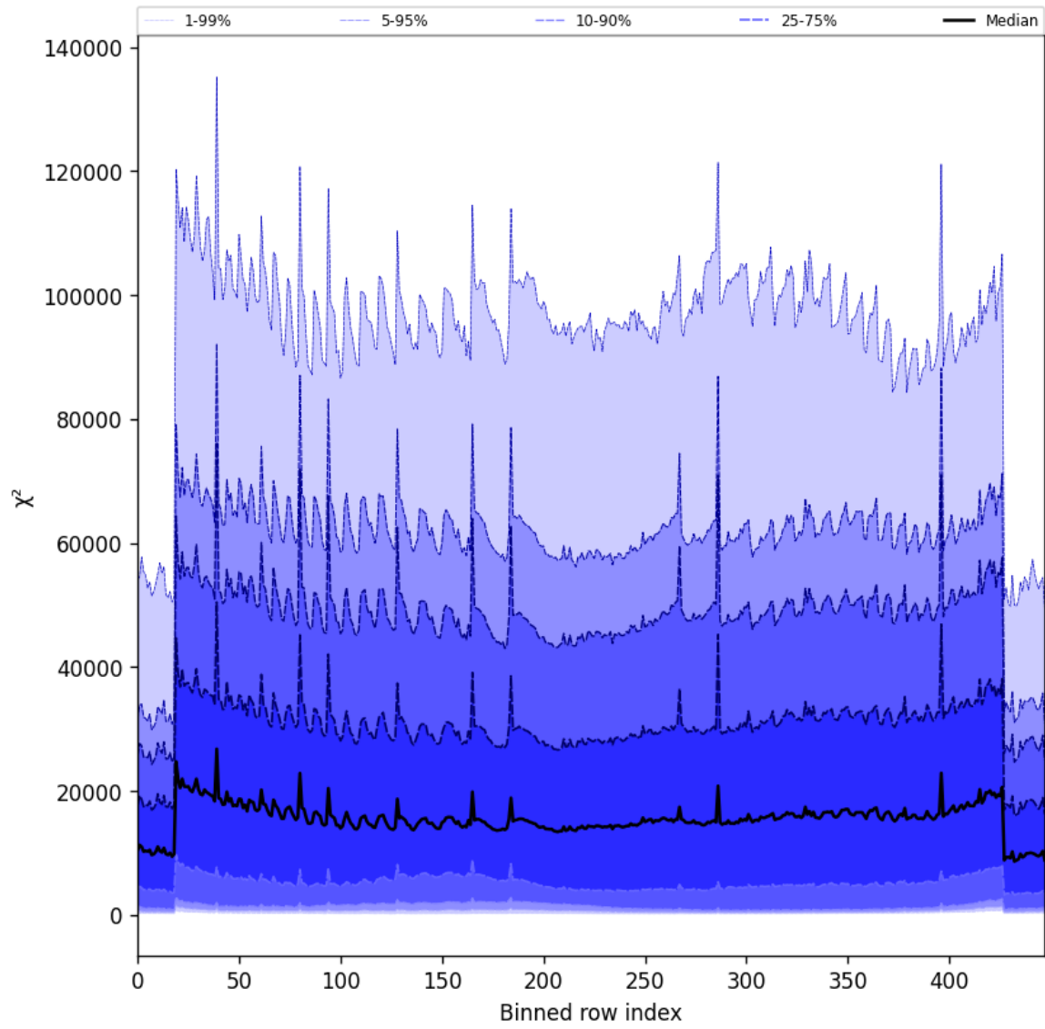
Figure 55: Along track statistics of “ \chi^2 ” for 2025-03-29 to 2025-03-31
