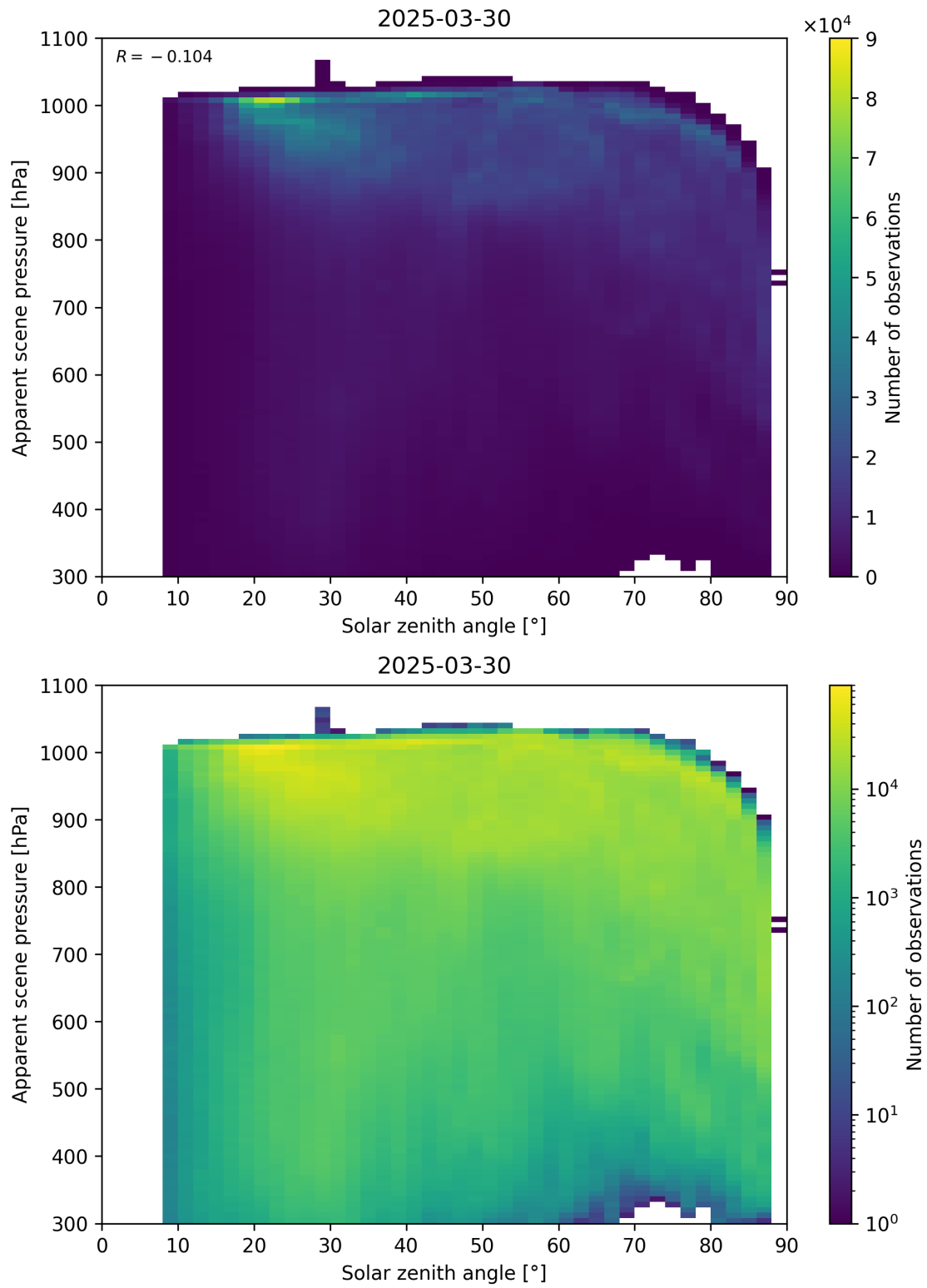
Figure 108: Scatter density plot of “Solar zenith angle” against “Apparent scene pressure” for 2025-03-29 to 2025-03-31.
