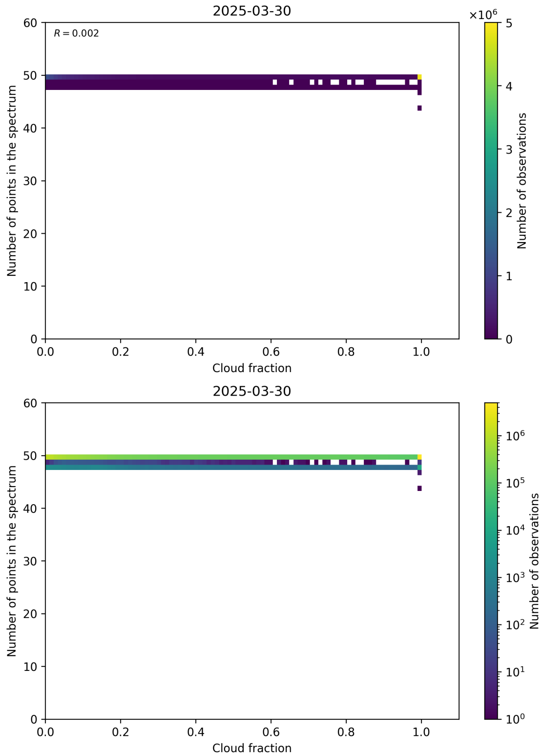
Figure 74: Scatter density plot of “Cloud fraction” against “Number of points in the spectrum” for 2025-03-29 to 2025-03-31.
