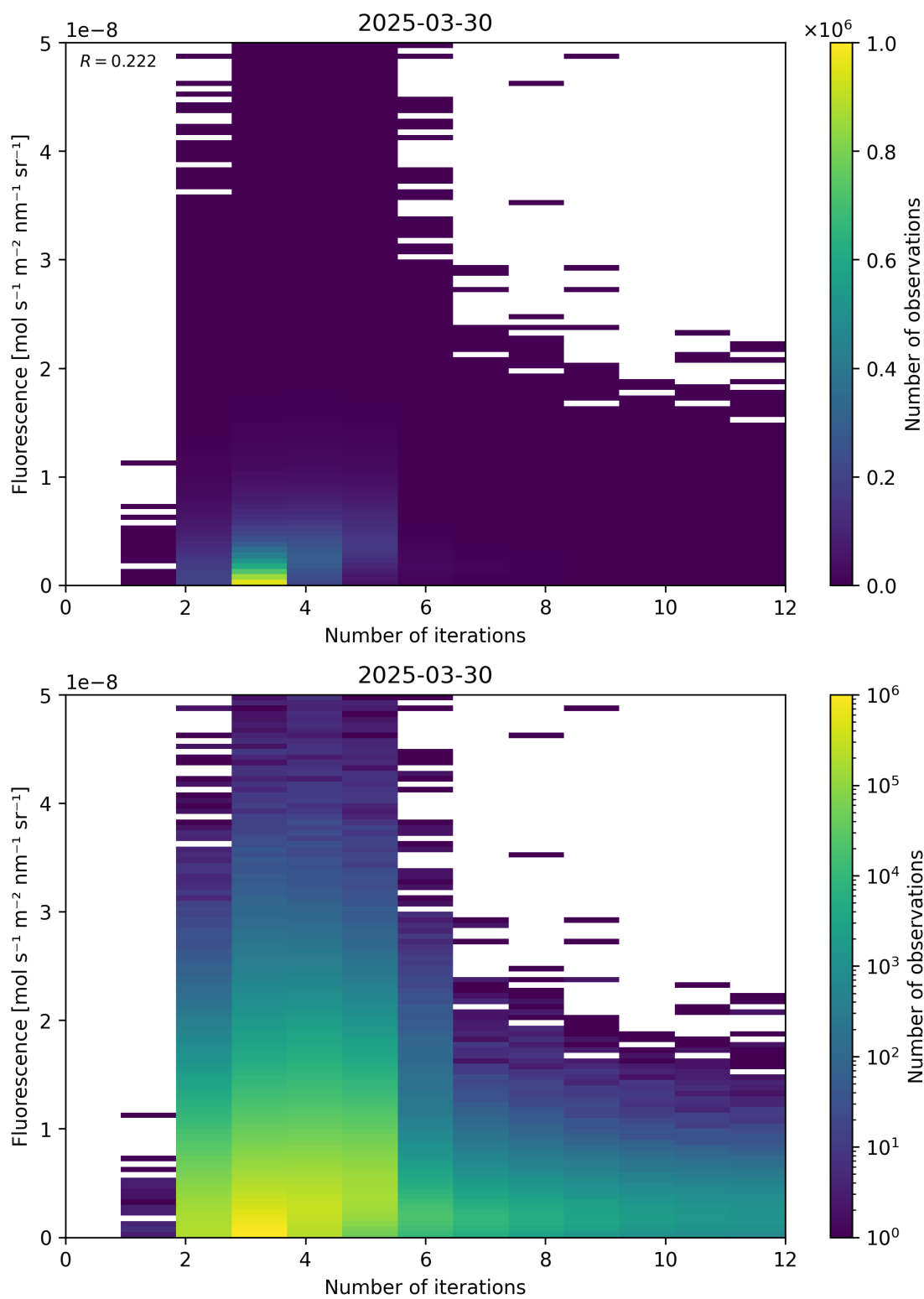
Figure 98: Scatter density plot of “Number of iterations” against “Fluorescence” for 2025-03-29 to 2025-03-31.
