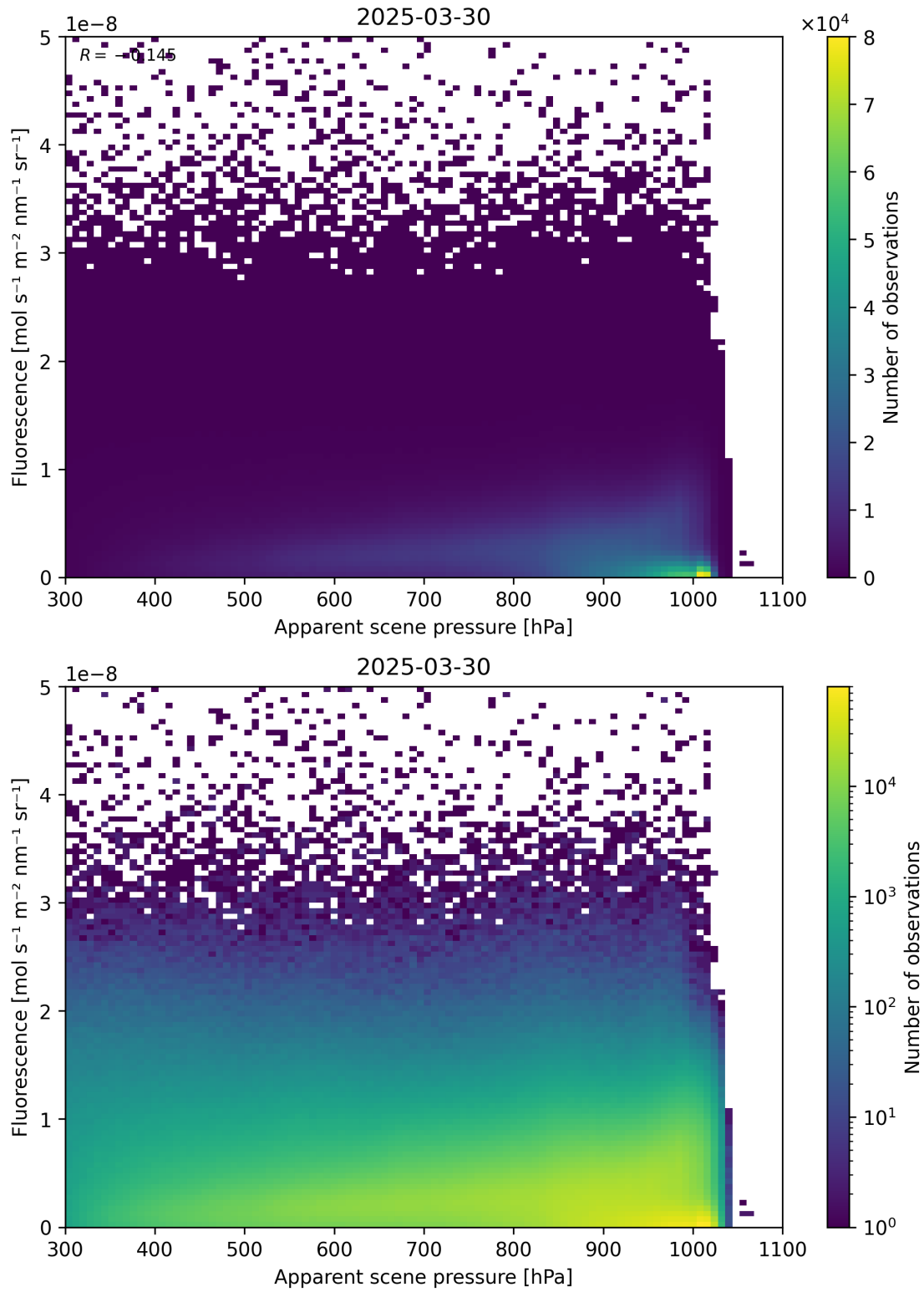
Figure 64: Scatter density plot of “Apparent scene pressure” against “Fluorescence” for 2025-03-29 to 2025-03-31.
