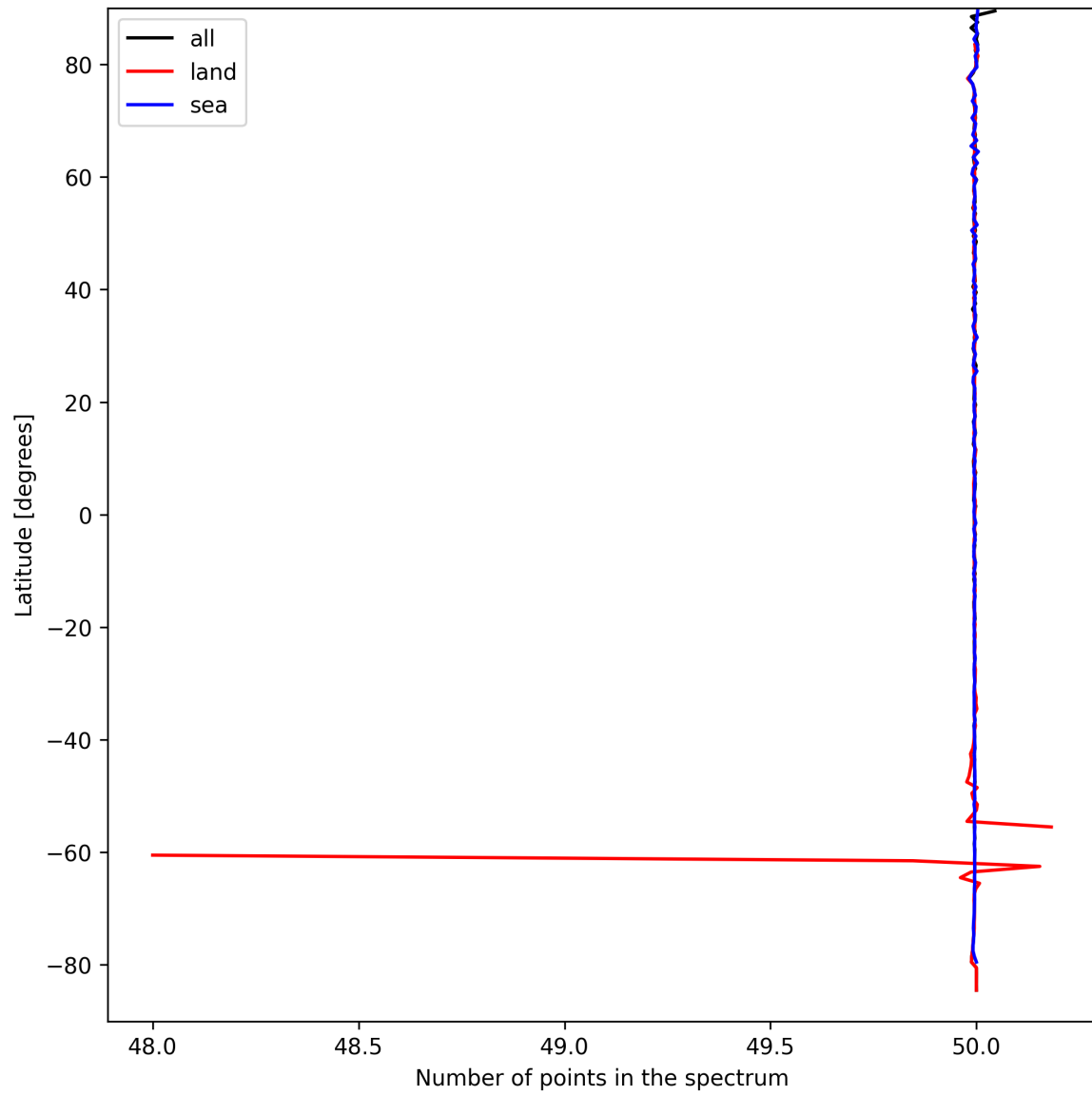
Figure 27: Zonal average of “Number of points in the spectrum” for 2025-03-29 to 2025-03-31.
