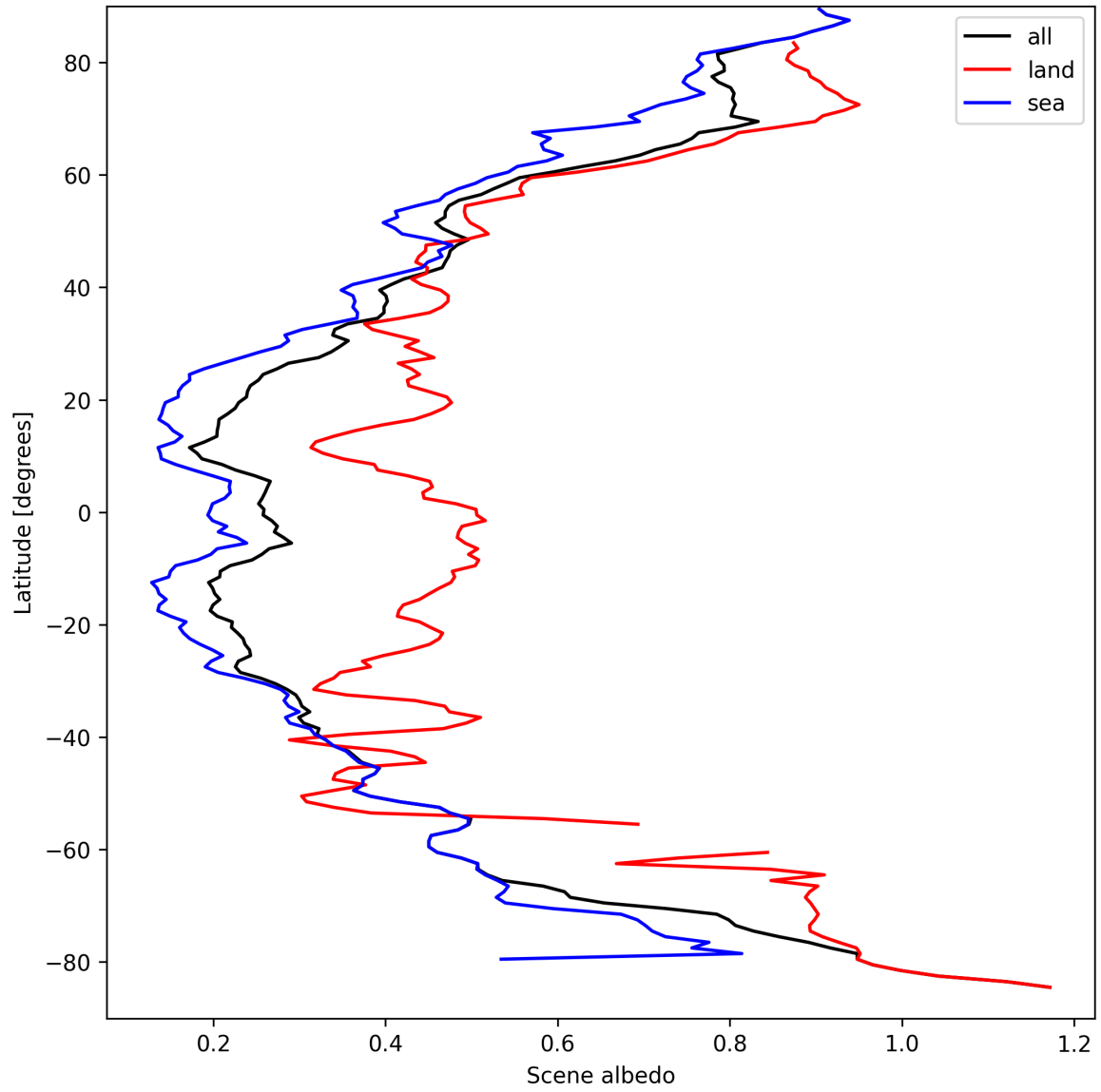
Figure 17: Zonal average of “Scene albedo” for 2025-03-29 to 2025-03-31.
