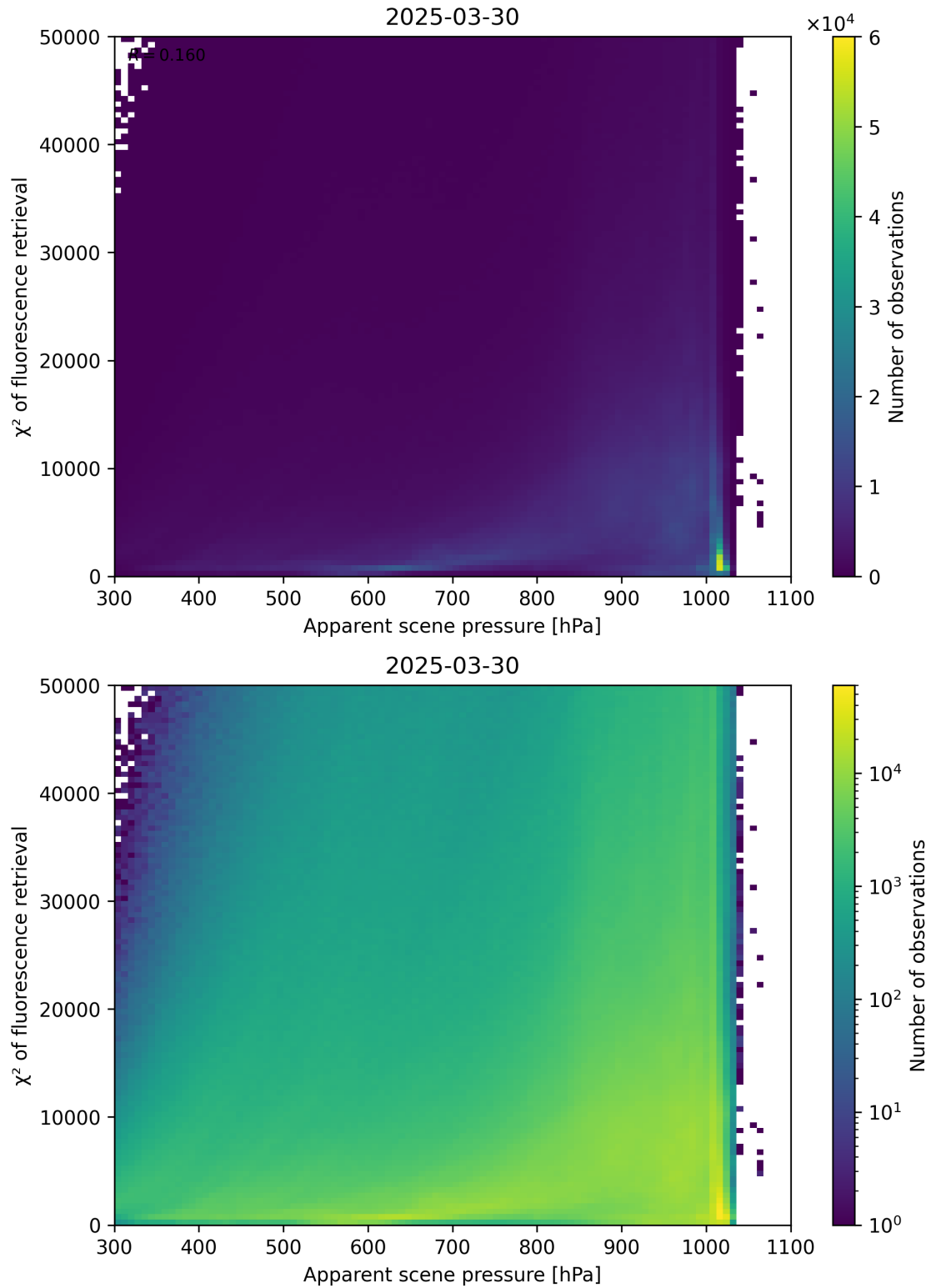
Figure 63: Scatter density plot of “Apparent scene pressure” against “ \chi^2 of fluorescence retrieval” for 2025-03-29 to 2025-03-31.
