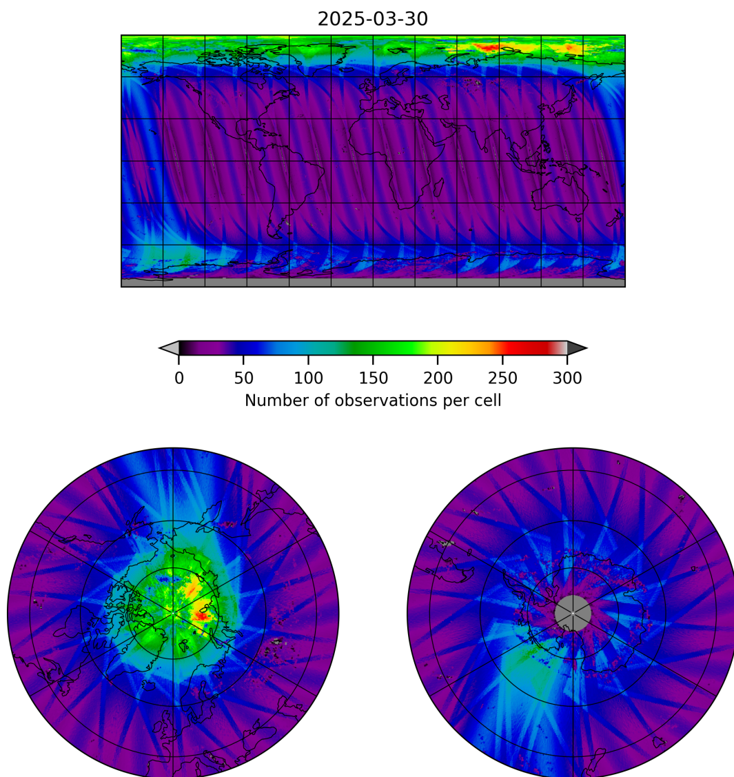
Figure 11: Map of the number of observations for 2025-03-29 to 2025-03-31
