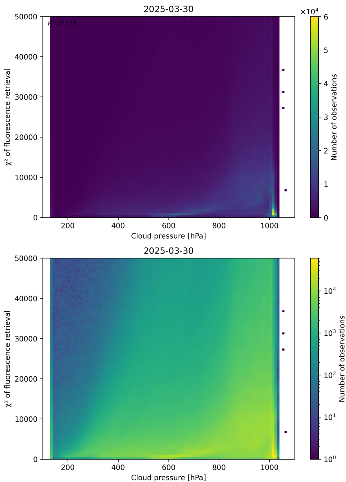
Figure 78: Scatter density plot of “Cloud pressure” against “ \chi^2 of fluorescence retrieval” for 2025-03-29 to 2025-03-31.
