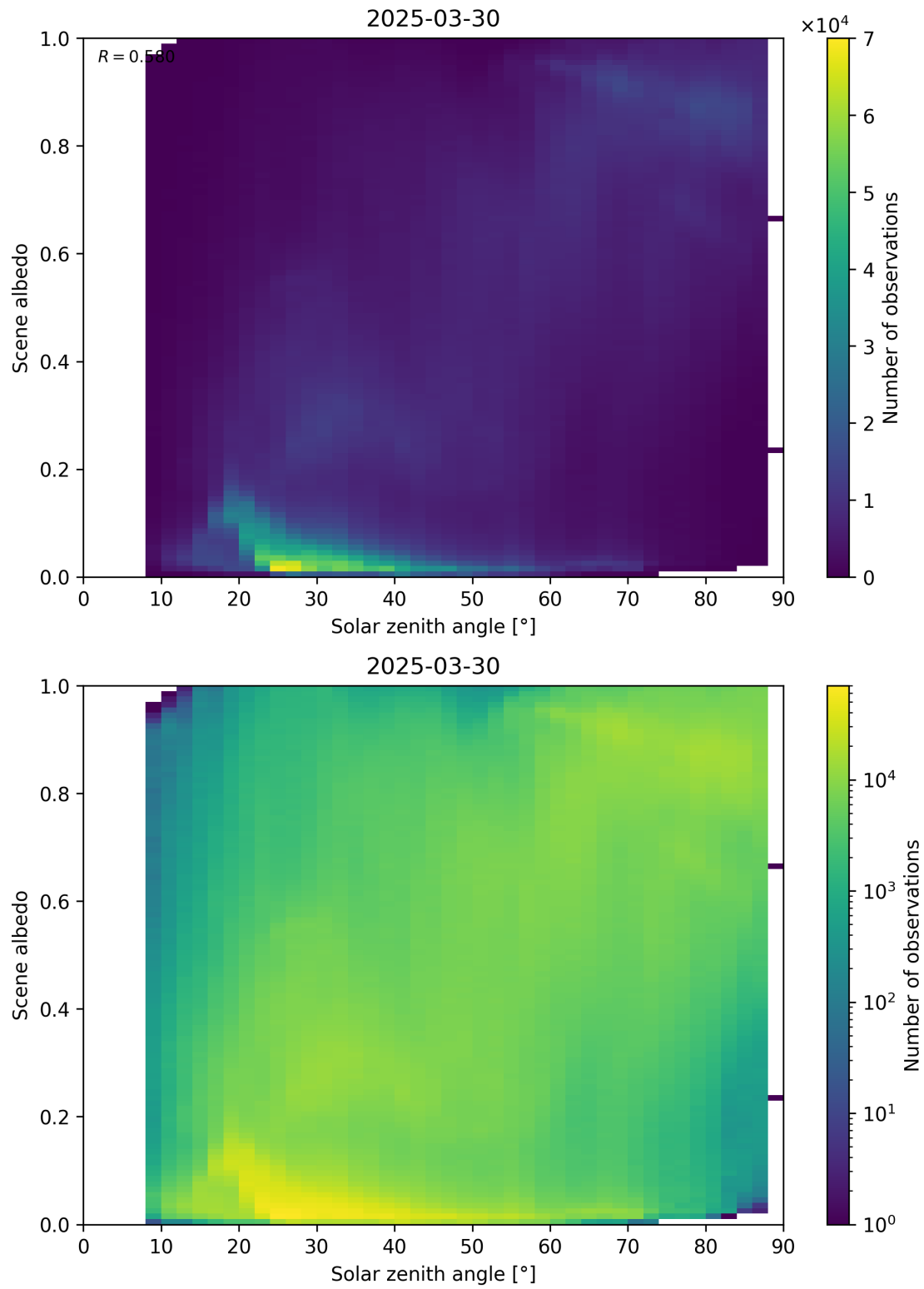
Figure 116: Scatter density plot of “Solar zenith angle” against “Scene albedo” for 2025-03-29 to 2025-03-31.
