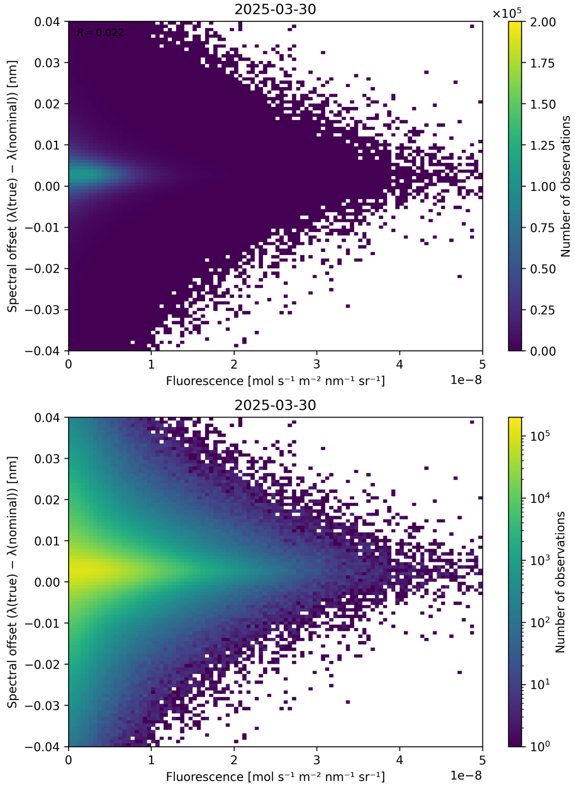
Figure 87: Scatter density plot of “Fluorescence” against “Spectral offset ( \lambda_{\text{true}} - \lambda_{\text{nominal}} )” for 2025-03-29 to 2025-03-31.
