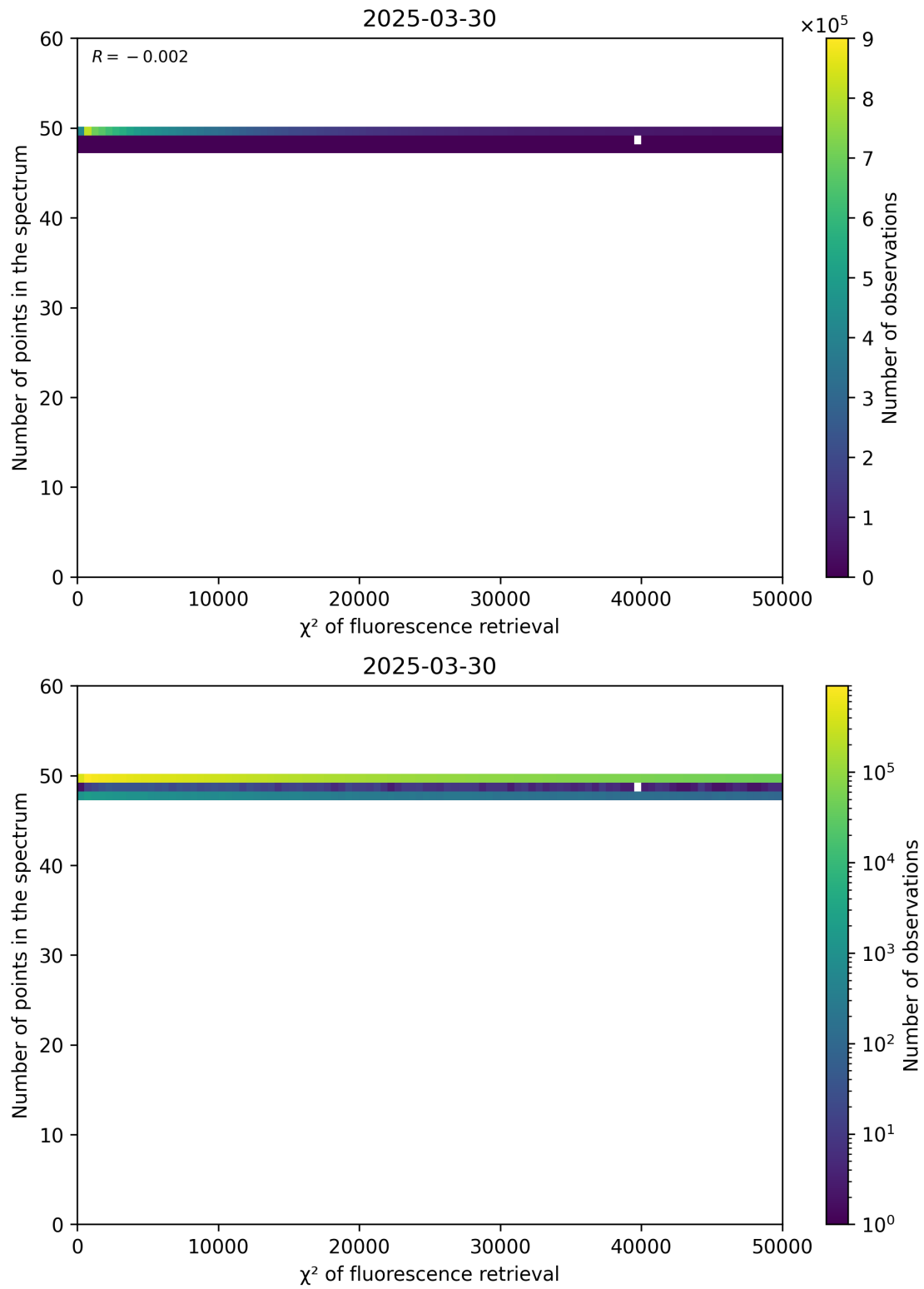
Figure 68: Scatter density plot of “ \chi^2 of fluorescence retrieval” against “Number of points in the spectrum” for 2025-03-29 to 2025-03-31.
