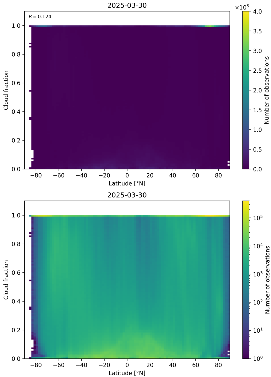
Figure 90: Scatter density plot of “Latitude” against “Cloud fraction” for 2025-03-29 to 2025-03-31.
