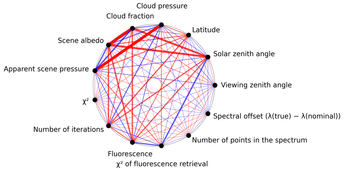
Figure 1: Map of correlation graph for 2025-03-29 to 2025-03-31.
