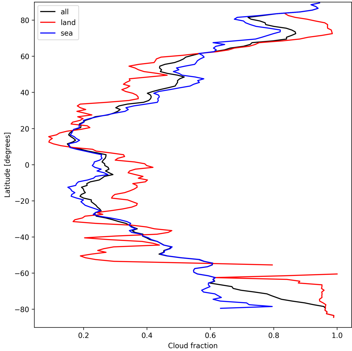
Figure 15: Zonal average of “Cloud fraction” for 2025-03-29 to 2025-03-31.
