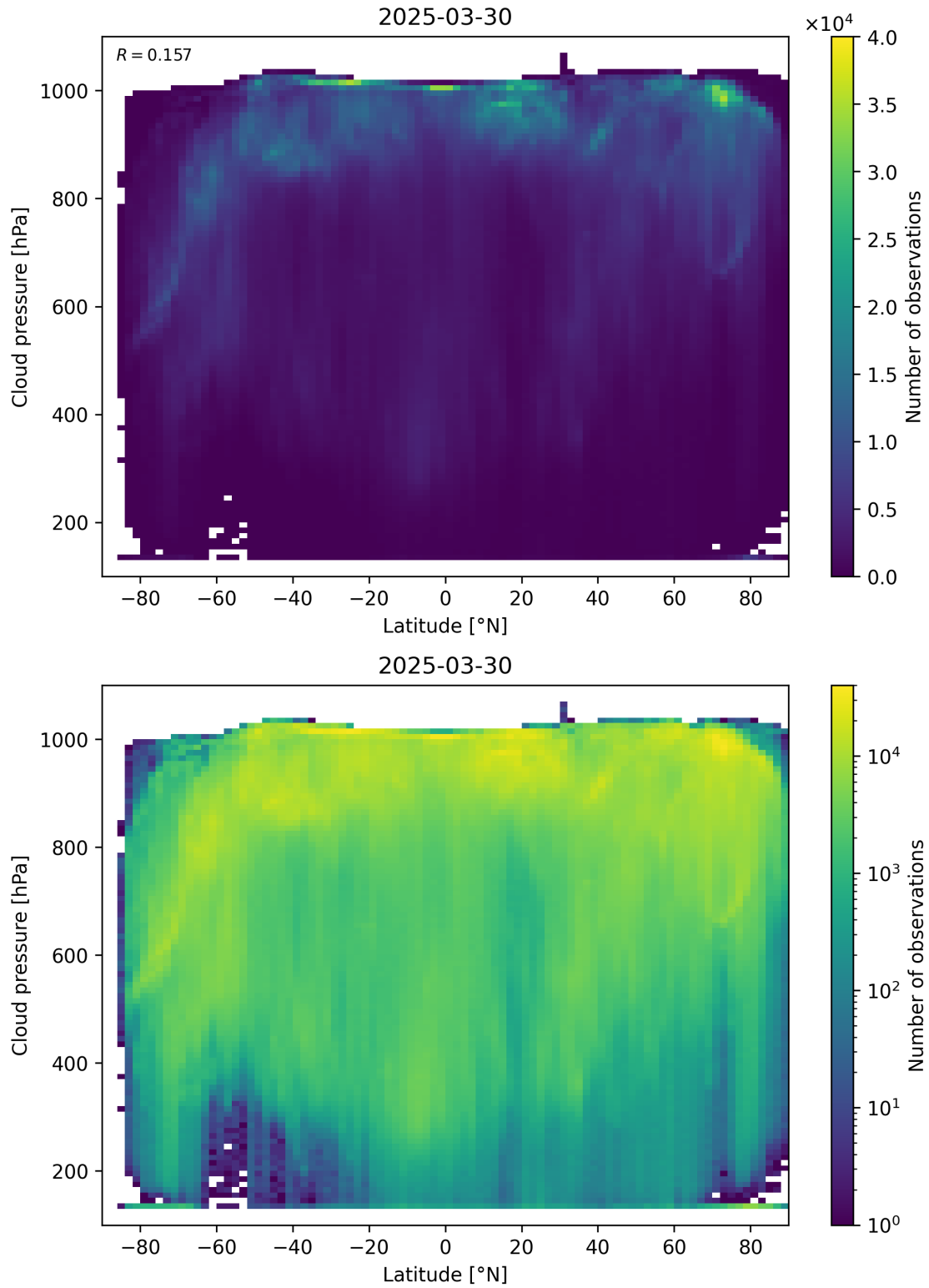
Figure 91: Scatter density plot of “Latitude” against “Cloud pressure” for 2025-03-29 to 2025-03-31.
