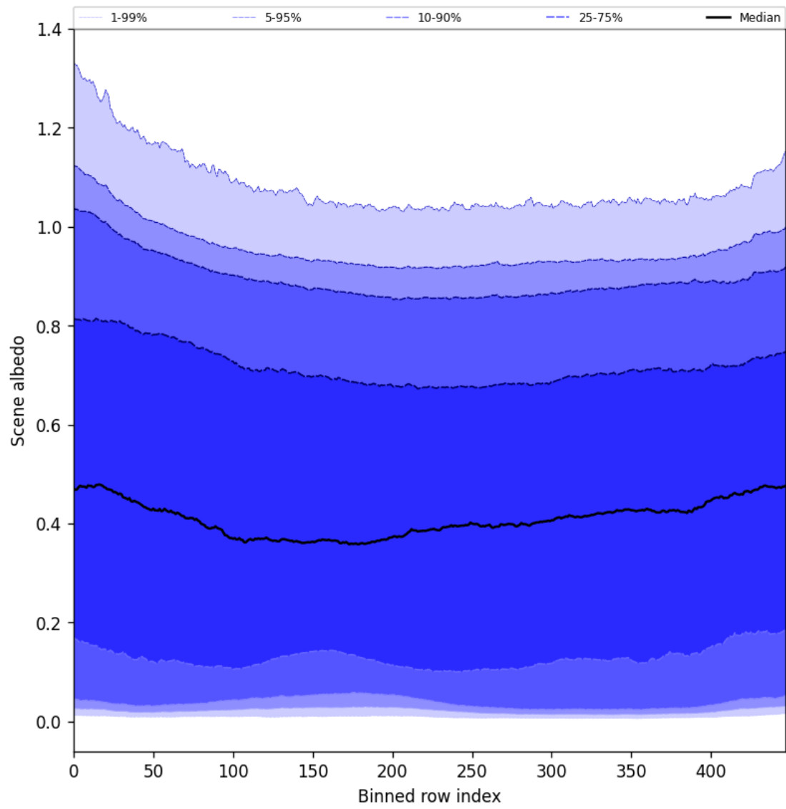
Figure 51: Along track statistics of “Scene albedo” for 2025-03-29 to 2025-03-31
