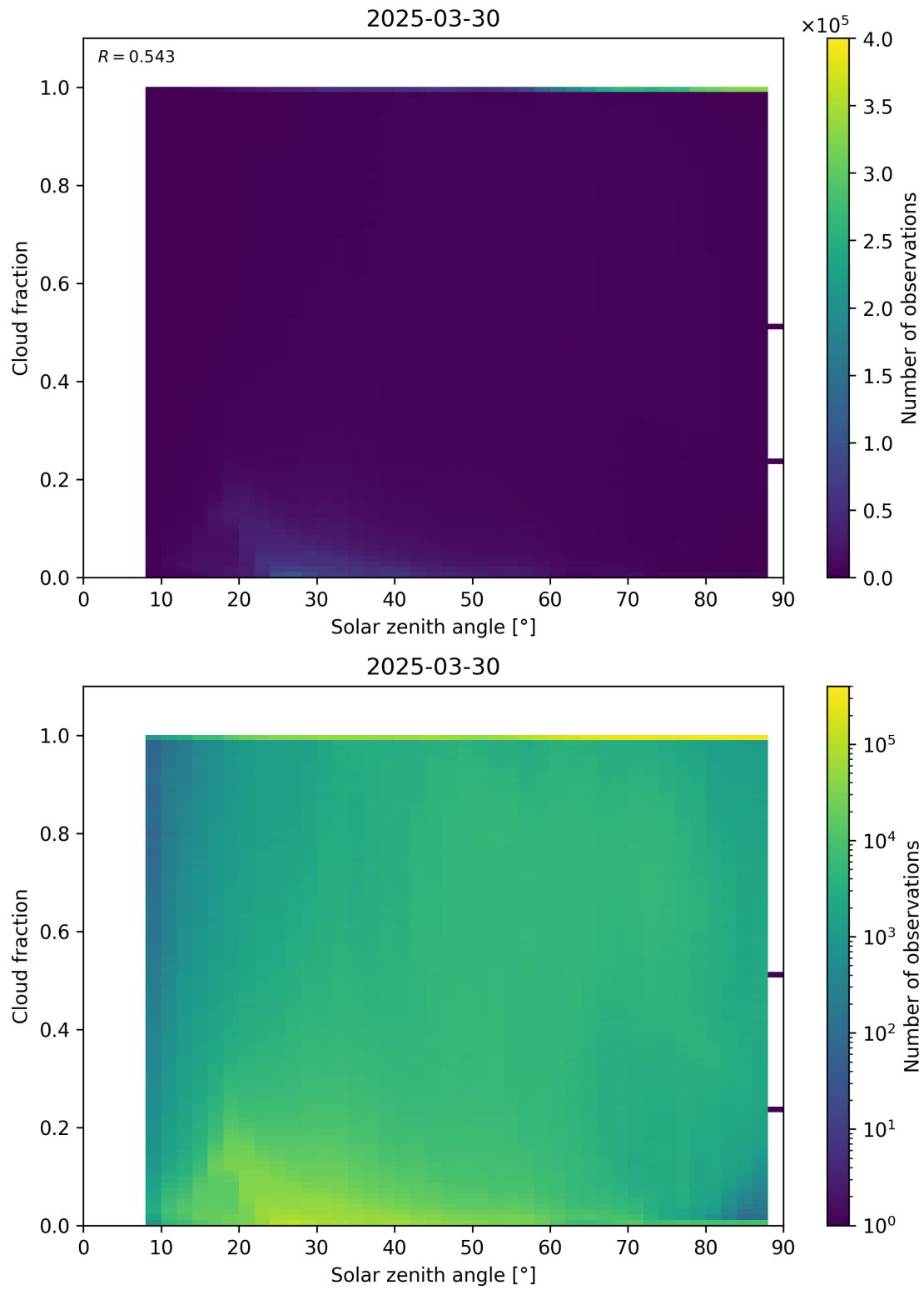
Figure 110: Scatter density plot of “Solar zenith angle” against “Cloud fraction” for 2025-03-29 to 2025-03-31.
