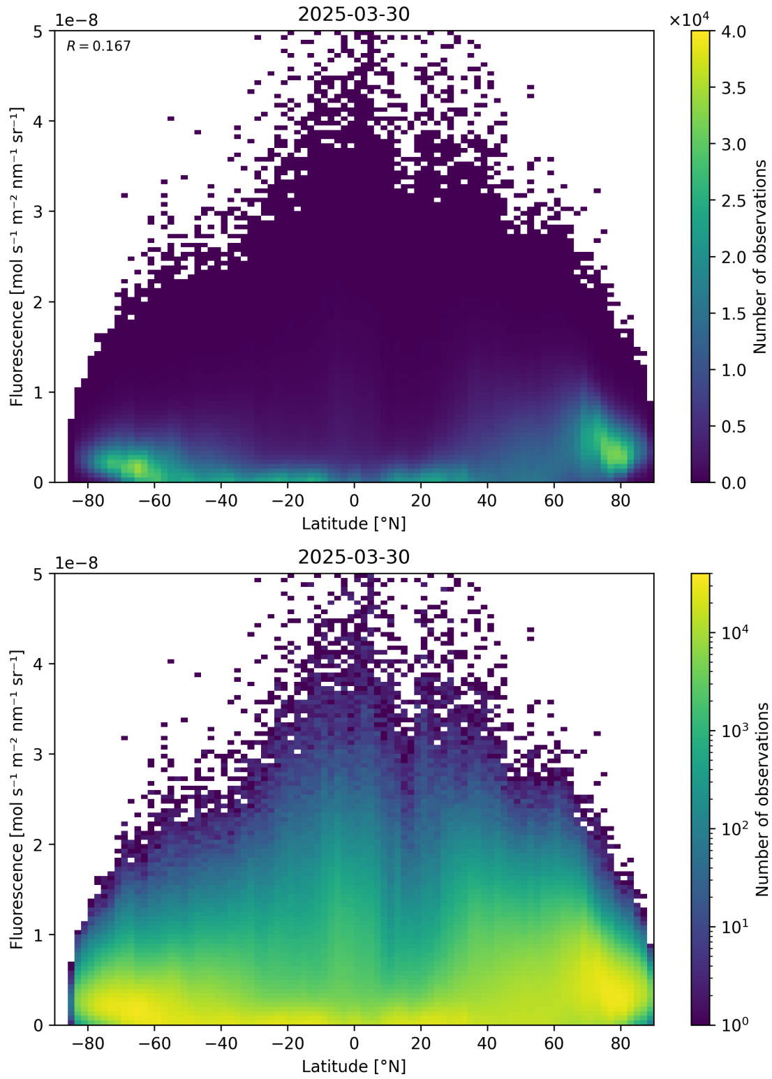
Figure 92: Scatter density plot of “Latitude” against “Fluorescence” for 2025-03-29 to 2025-03-31.
