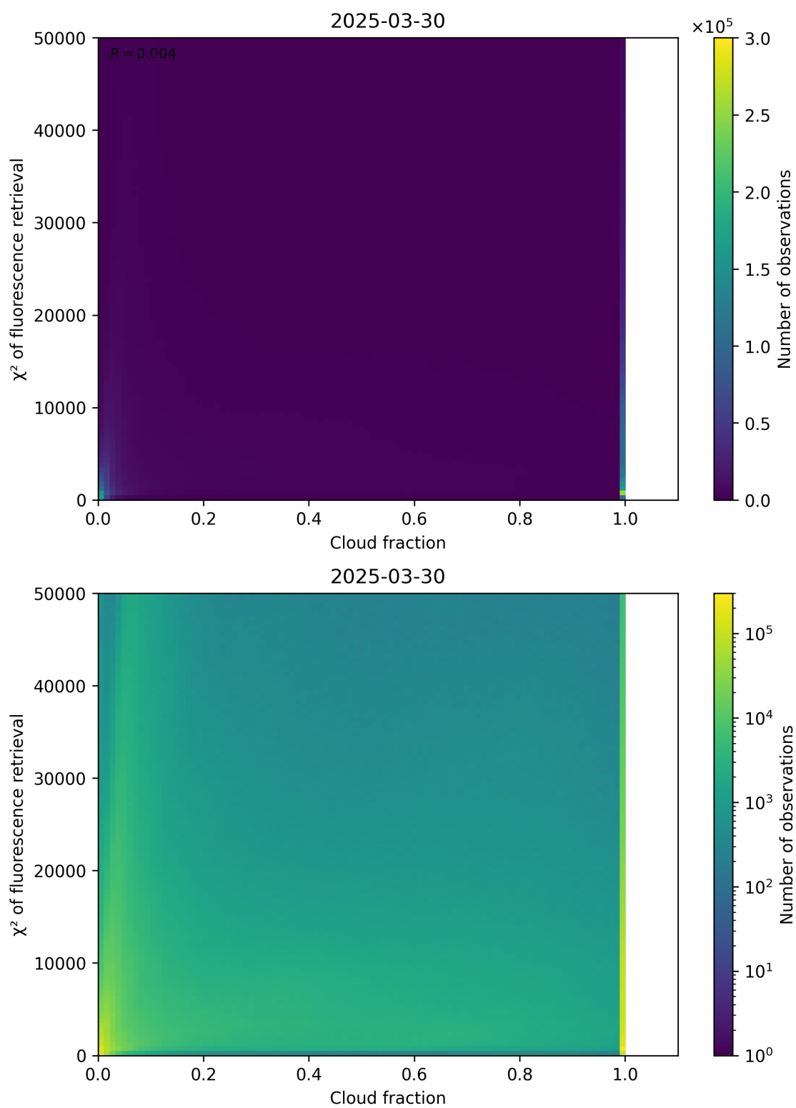
Figure 71: Scatter density plot of “Cloud fraction” against “ \chi^2 of fluorescence retrieval” for 2025-03-29 to 2025-03-31.
