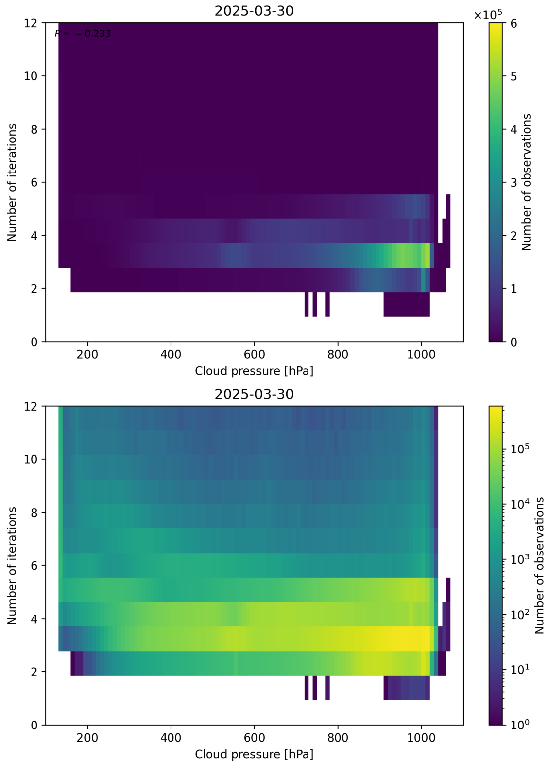
Figure 81: Scatter density plot of “Cloud pressure” against “Number of iterations” for 2025-03-29 to 2025-03-31.
