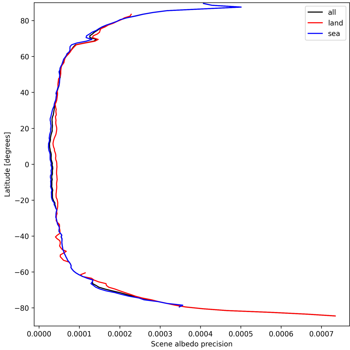
Figure 18: Zonal average of “Scene albedo precision” for 2025-03-29 to 2025-03-31.
