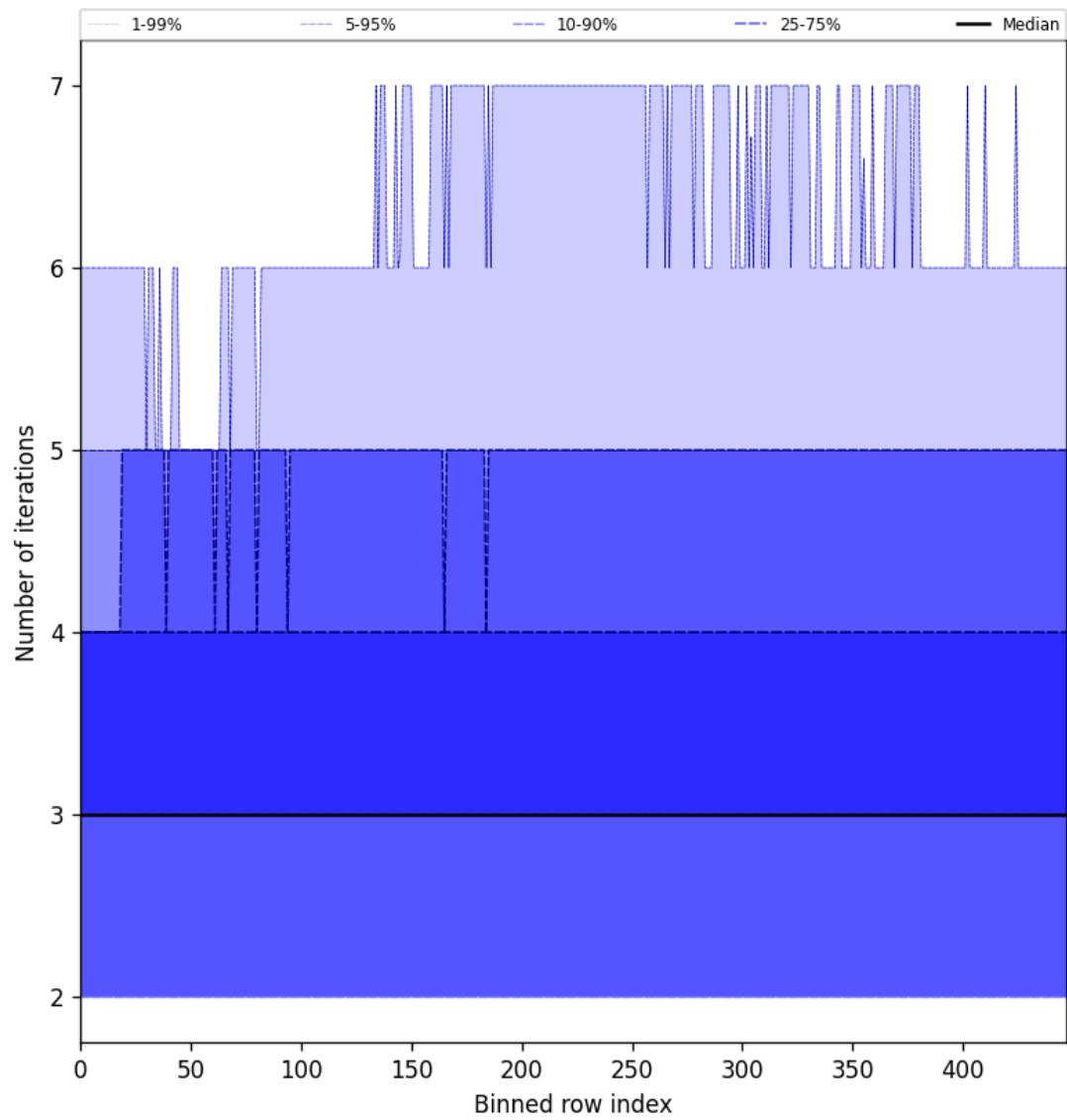
Figure 56: Along track statistics of “Number of iterations” for 2025-03-29 to 2025-03-31
