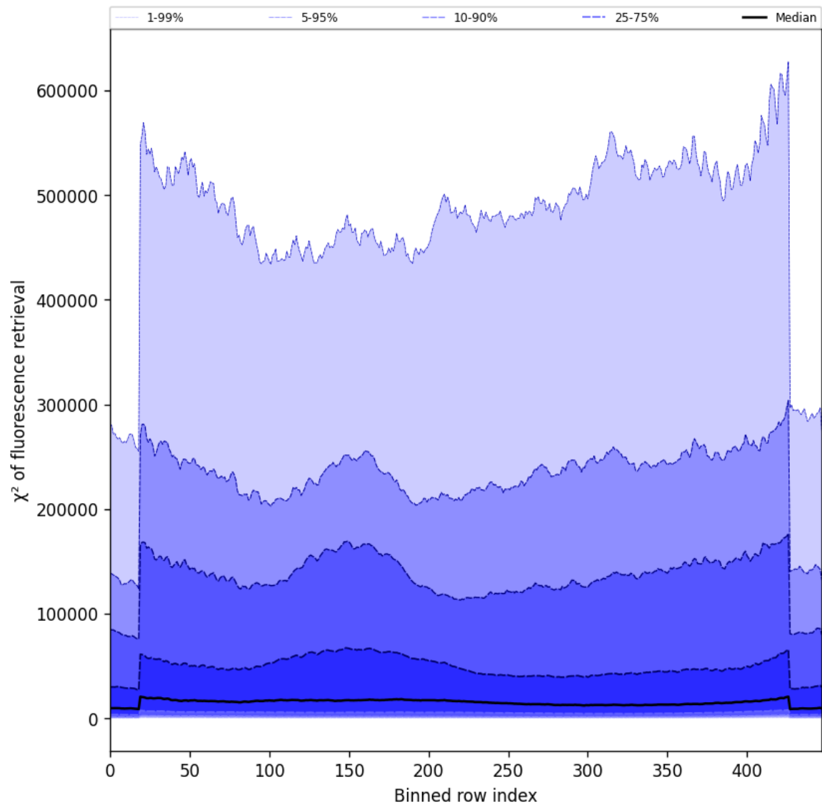
Figure 59: Along track statistics of “ \chi^2 of fluorescence retrieval” for 2025-03-29 to 2025-03-31
