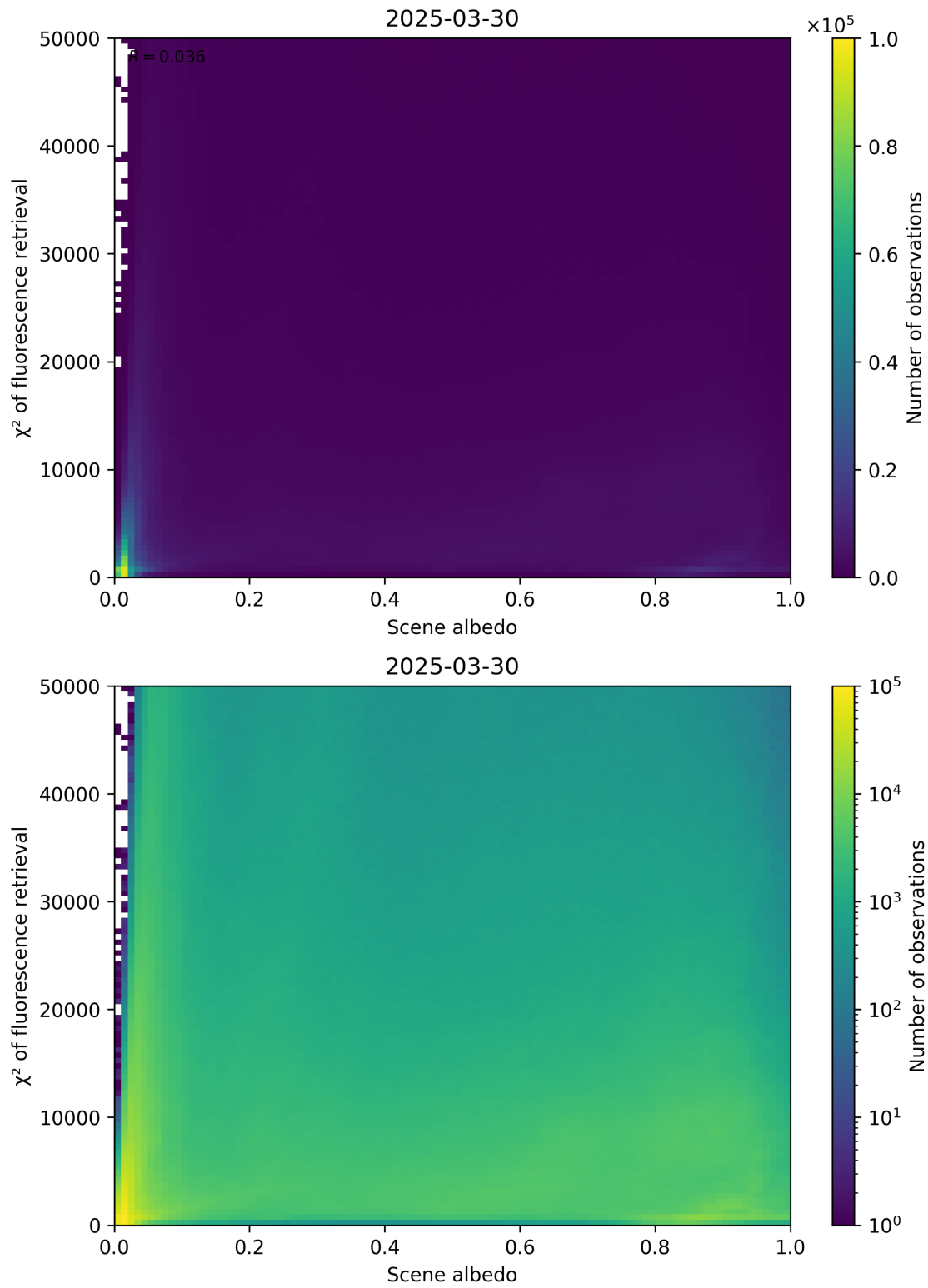
Figure 103: Scatter density plot of “Scene albedo” against “ \chi^2 of fluorescence retrieval” for 2025-03-29 to 2025-03-31.
