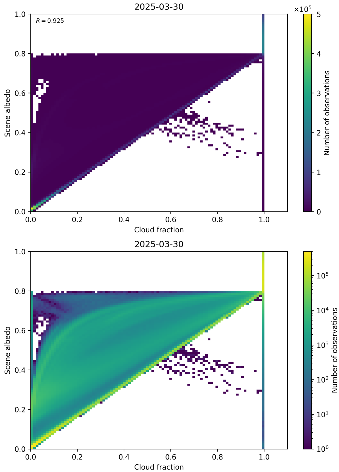
Figure 75: Scatter density plot of “Cloud fraction” against “Scene albedo” for 2025-03-29 to 2025-03-31.
