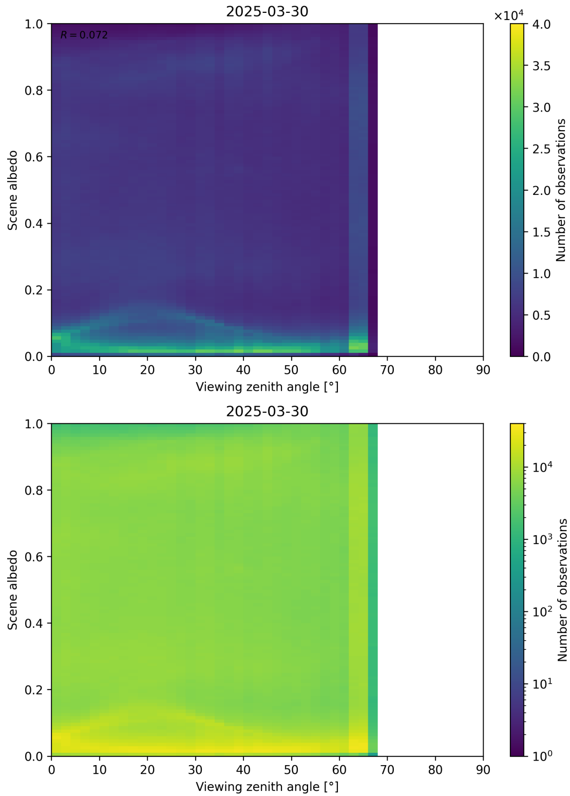
Figure 126: Scatter density plot of “Viewing zenith angle” against “Scene albedo” for 2025-03-29 to 2025-03-31.
