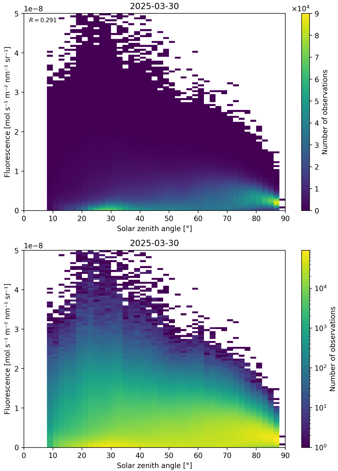
Figure 112: Scatter density plot of “Solar zenith angle” against “Fluorescence” for 2025-03-29 to 2025-03-31.
