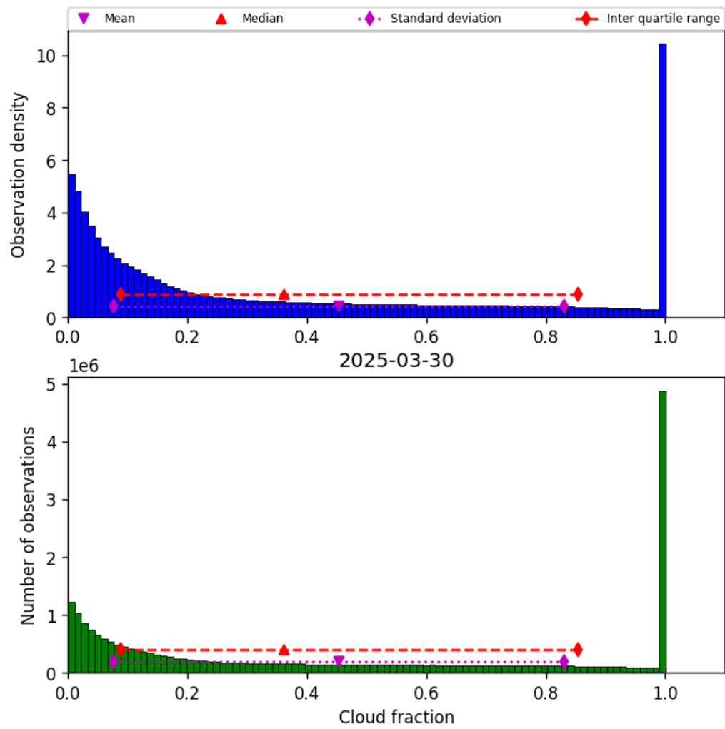
Figure 32: Histogram of “Cloud fraction” for 2025-03-29 to 2025-03-31
