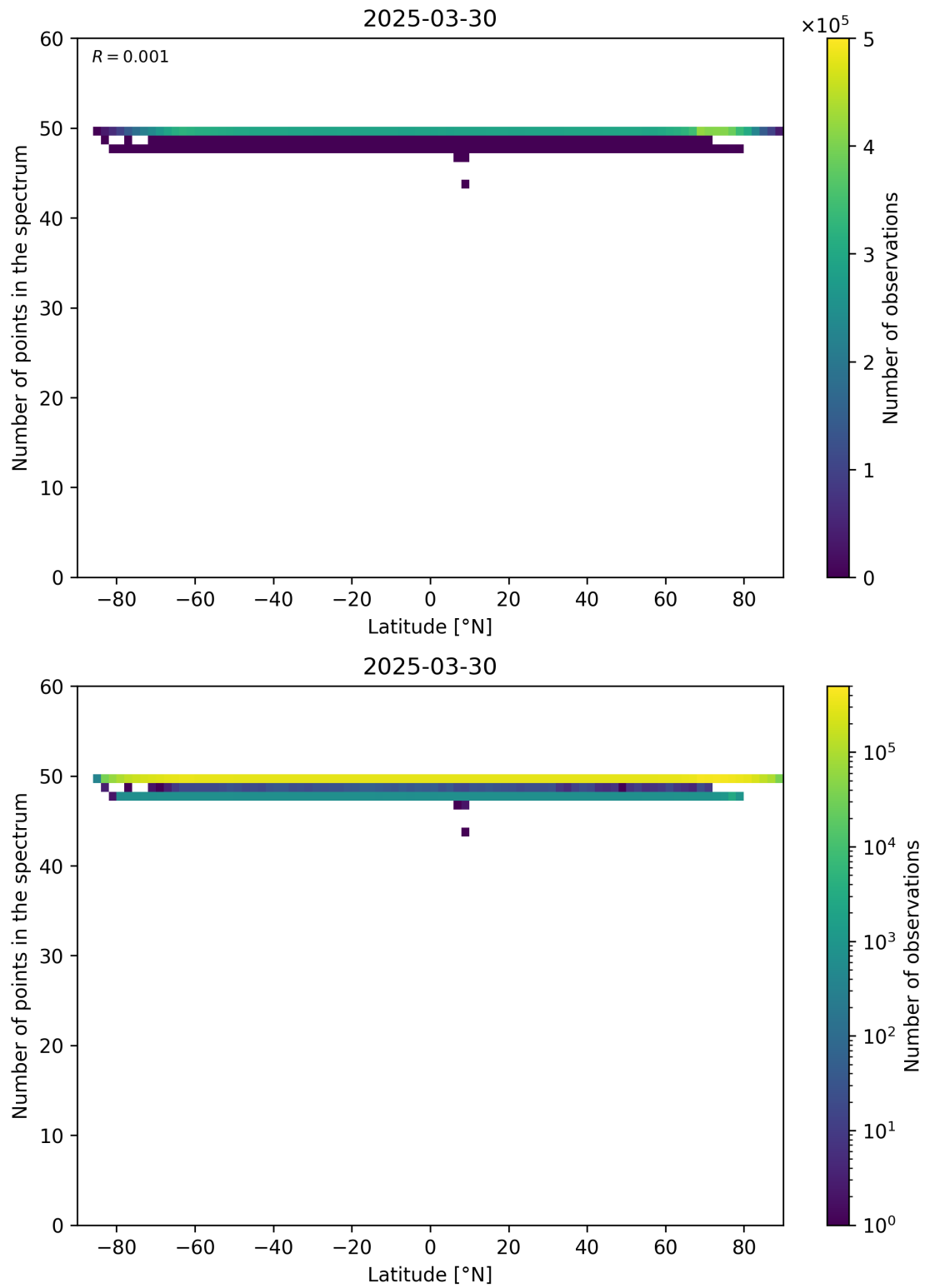
Figure 94: Scatter density plot of “Latitude” against “Number of points in the spectrum” for 2025-03-29 to 2025-03-31.
