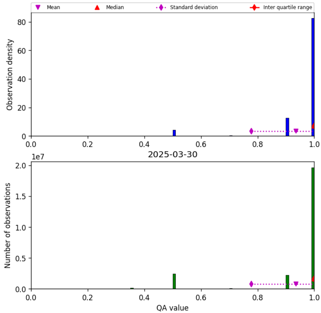
Figure 29: Histogram of “QA value” for 2025-03-29 to 2025-03-31
