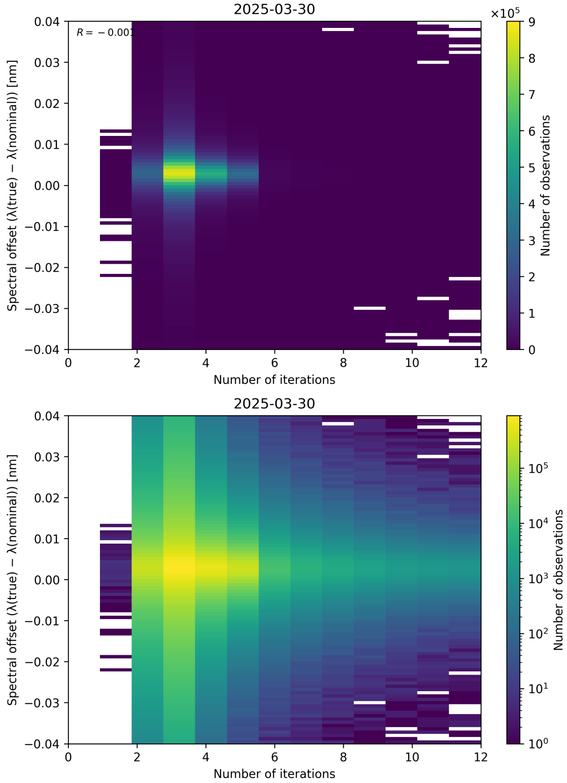
Figure 100: Scatter density plot of “Number of iterations” against “Spectral offset ( \lambda_{\text{true}} - \lambda_{\text{nominal}} )” for 2025-03-29 to 2025-03-31.
