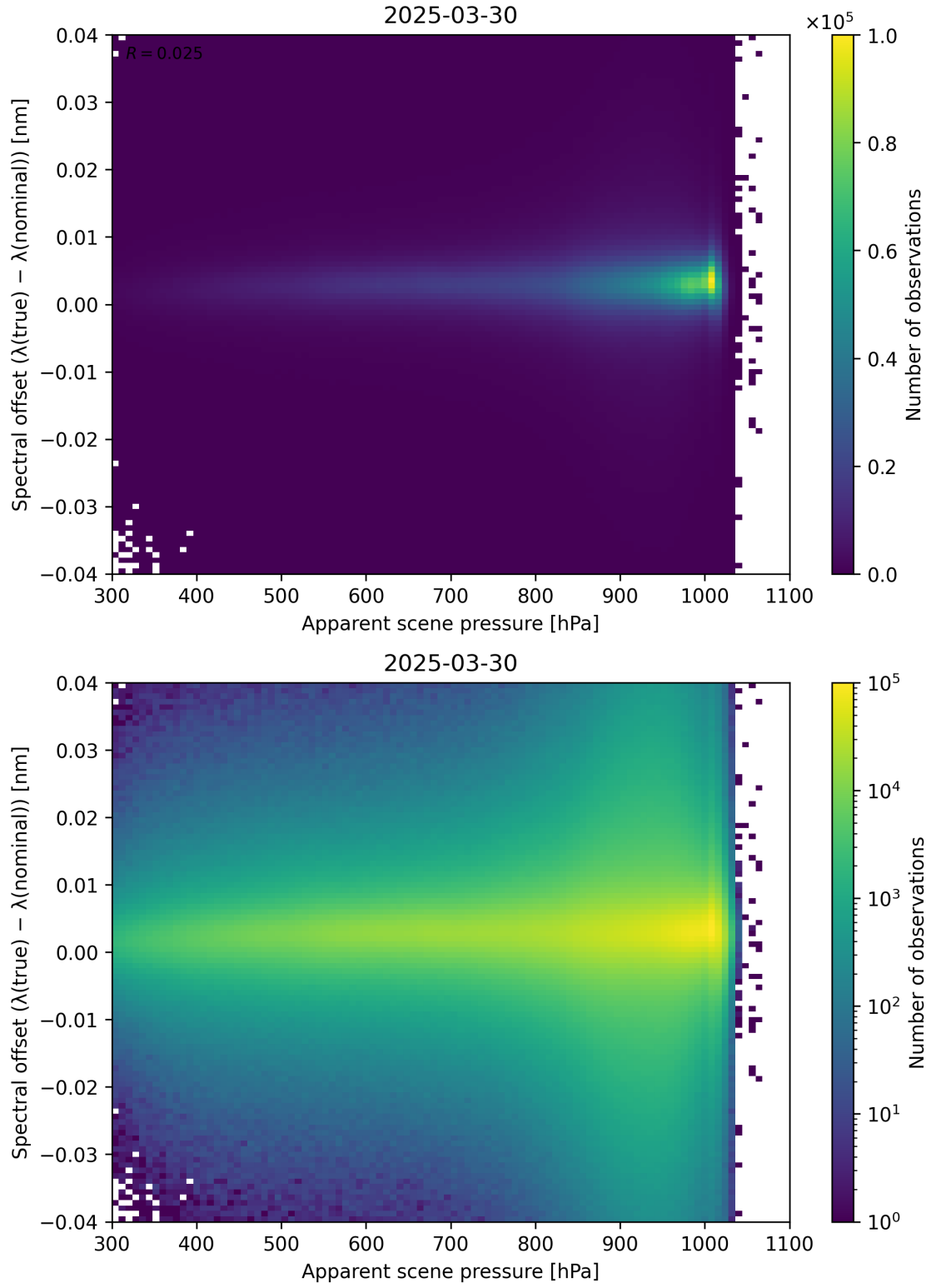
Figure 67: Scatter density plot of “Apparent scene pressure” against “Spectral offset ( \lambda_{\text{true}} - \lambda_{\text{nominal}} )” for 2025-03-29 to 2025-03-31.
