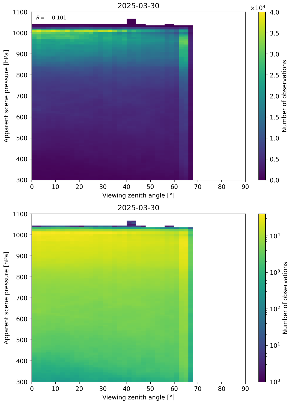
Figure 118: Scatter density plot of “Viewing zenith angle” against “Apparent scene pressure” for 2025-03-29 to 2025-03-31.
