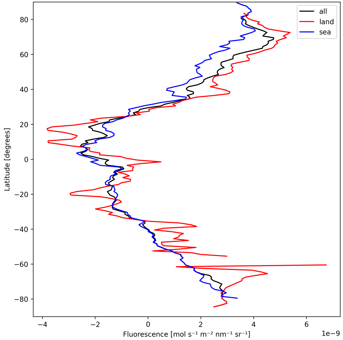
Figure 23: Zonal average of “Fluorescence” for 2025-03-29 to 2025-03-31.
