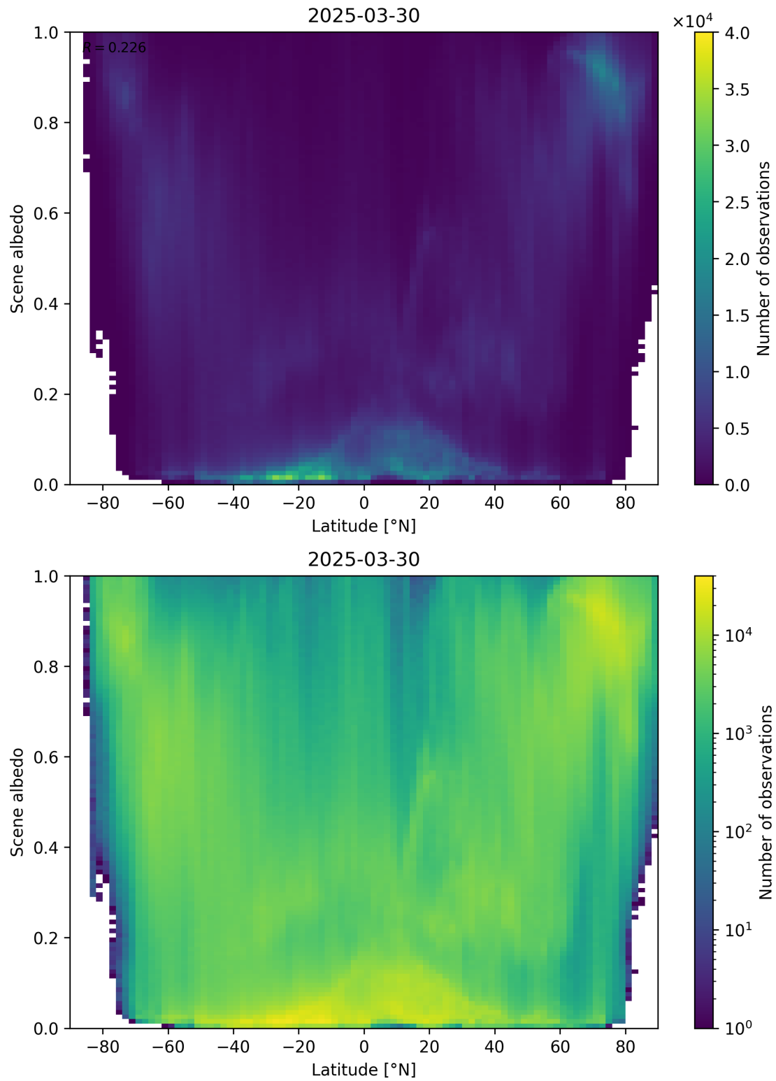
Figure 95: Scatter density plot of “Latitude” against “Scene albedo” for 2025-03-29 to 2025-03-31.
