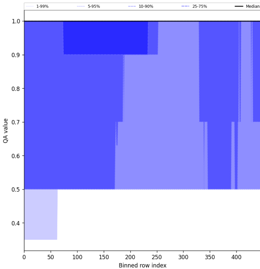
Figure 46: Along track statistics of “QA value” for 2025-03-29 to 2025-03-31
