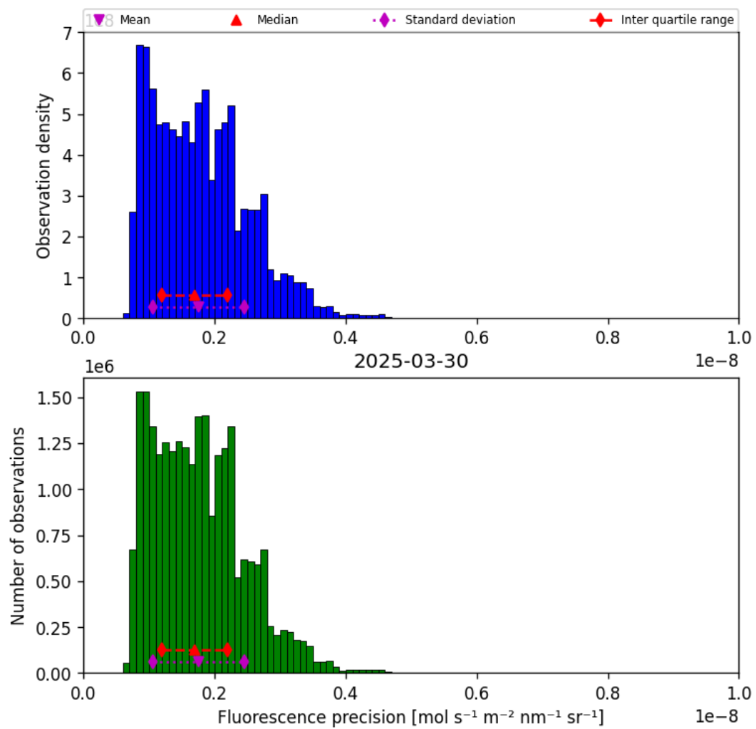
Figure 41: Histogram of “Fluorescence precision” for 2025-03-29 to 2025-03-31
