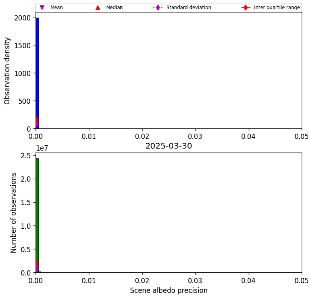
Figure 35: Histogram of “Scene albedo precision” for 2025-03-29 to 2025-03-31
