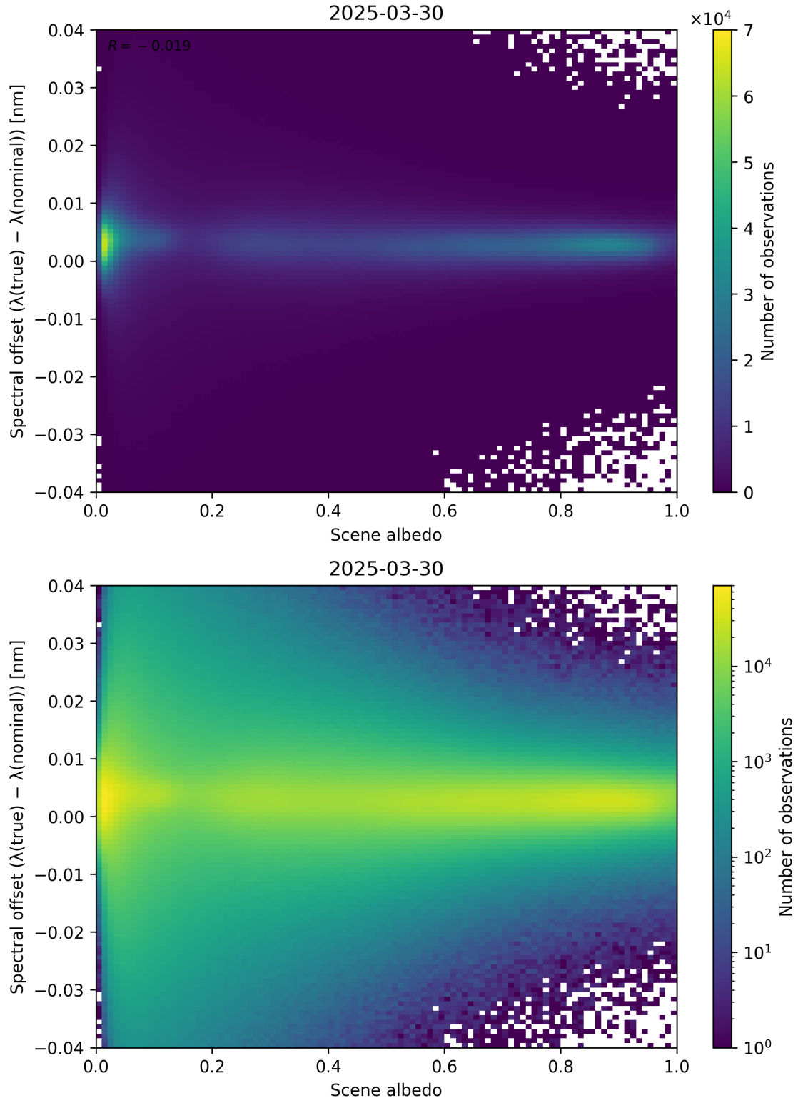
Figure 107: Scatter density plot of “Scene albedo” against “Spectral offset ( \lambda_{\text{true}} - \lambda_{\text{nominal}} )” for 2025-03-29 to 2025-03-31.
