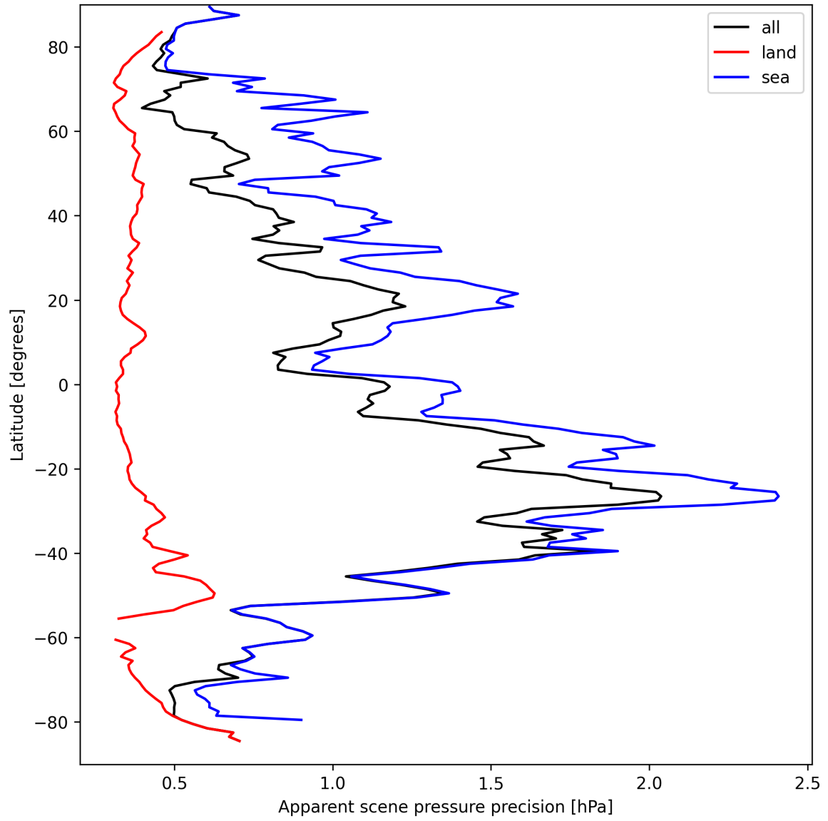
Figure 20: Zonal average of “Apparent scene pressure precision” for 2025-03-29 to 2025-03-31.
