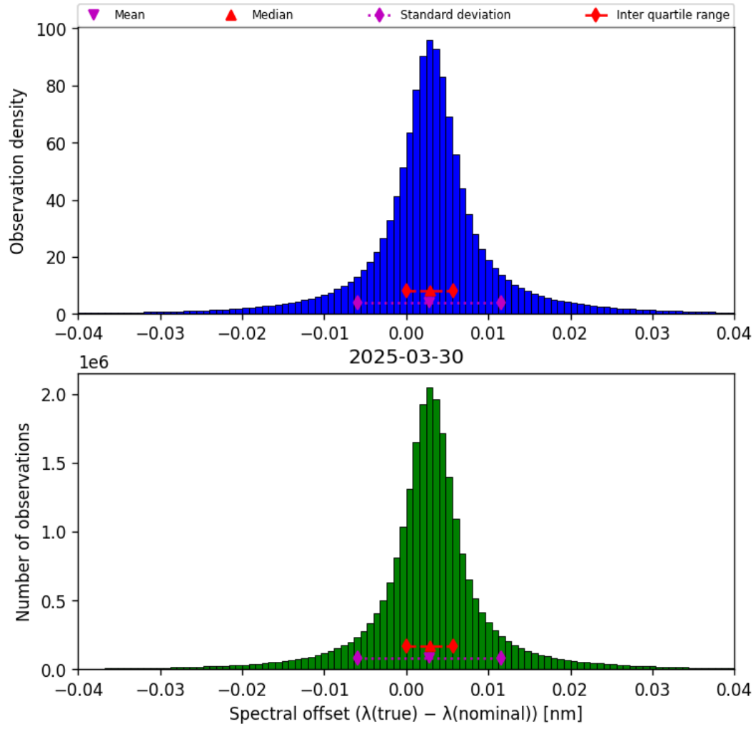
Figure 45: Histogram of “Spectral offset ( \lambda_{\text{true}} - \lambda_{\text{nominal}} )” for 2025-03-29 to 2025-03-31
