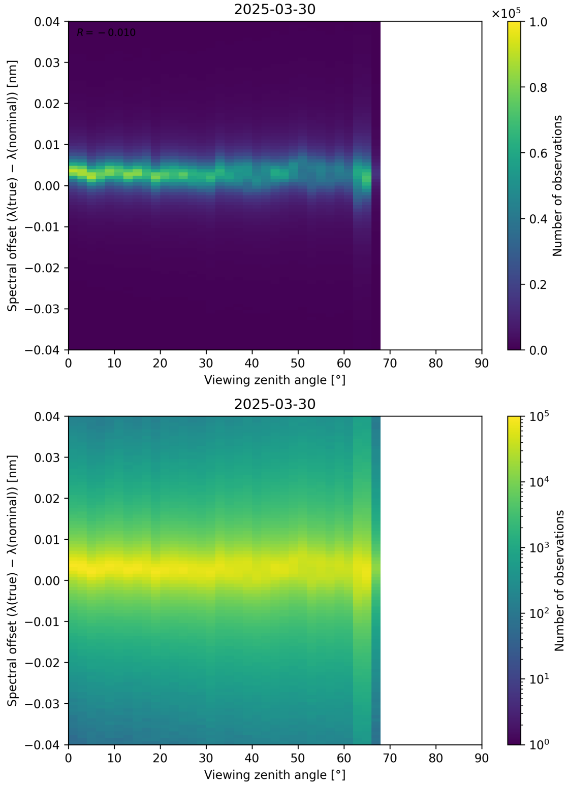
Figure 128: Scatter density plot of “Viewing zenith angle” against “Spectral offset ( \lambda_{\text{true}} - \lambda_{\text{nominal}} )” for 2025-03-29 to 2025-03-31.
