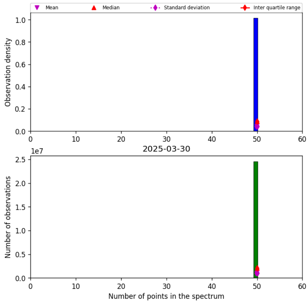
Figure 44: Histogram of “Number of points in the spectrum” for 2025-03-29 to 2025-03-31
