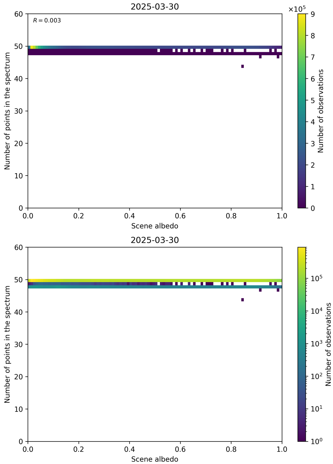
Figure 106: Scatter density plot of “Scene albedo” against “Number of points in the spectrum” for 2025-03-29 to 2025-03-31.
