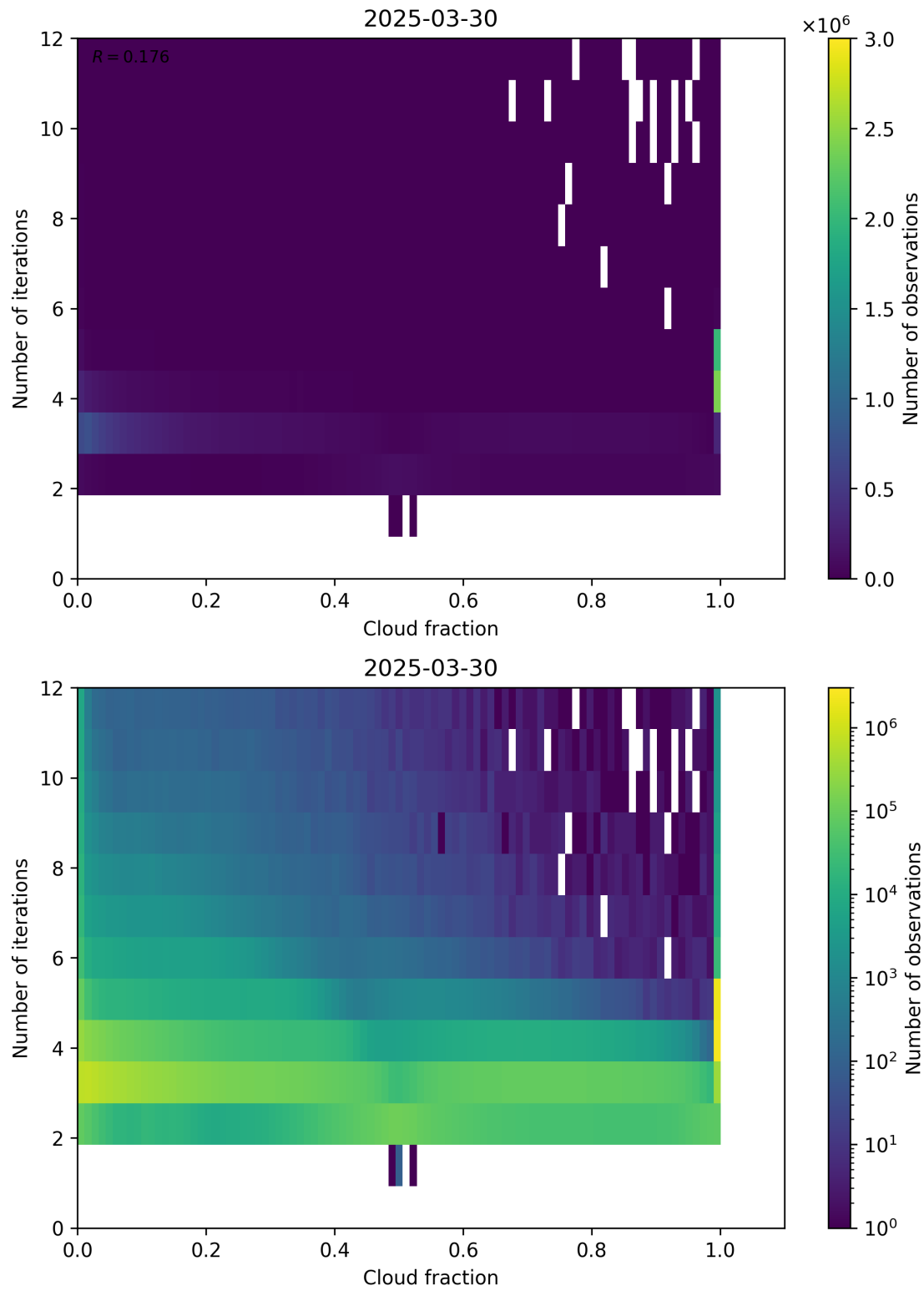
Figure 73: Scatter density plot of “Cloud fraction” against “Number of iterations” for 2025-03-29 to 2025-03-31.
