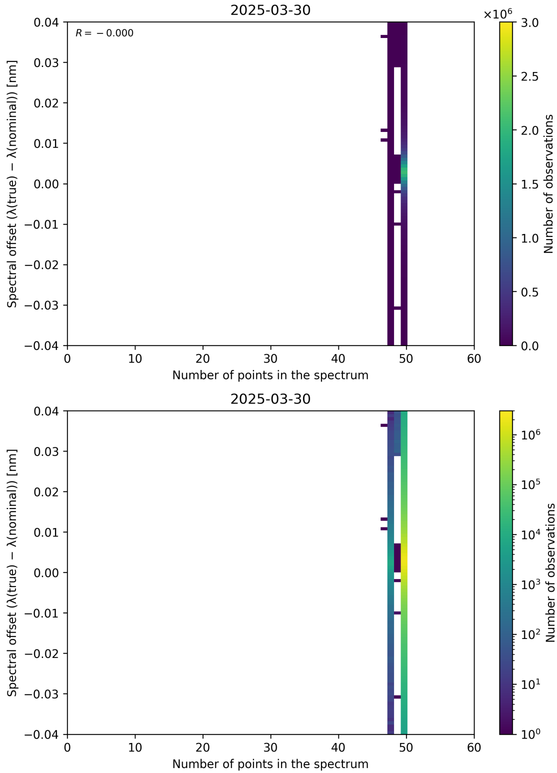
Figure 101: Scatter density plot of “Number of points in the spectrum” against “Spectral offset ( \lambda_{\text{true}} - \lambda_{\text{nominal}} )” for 2025-03-29 to 2025-03-31.
