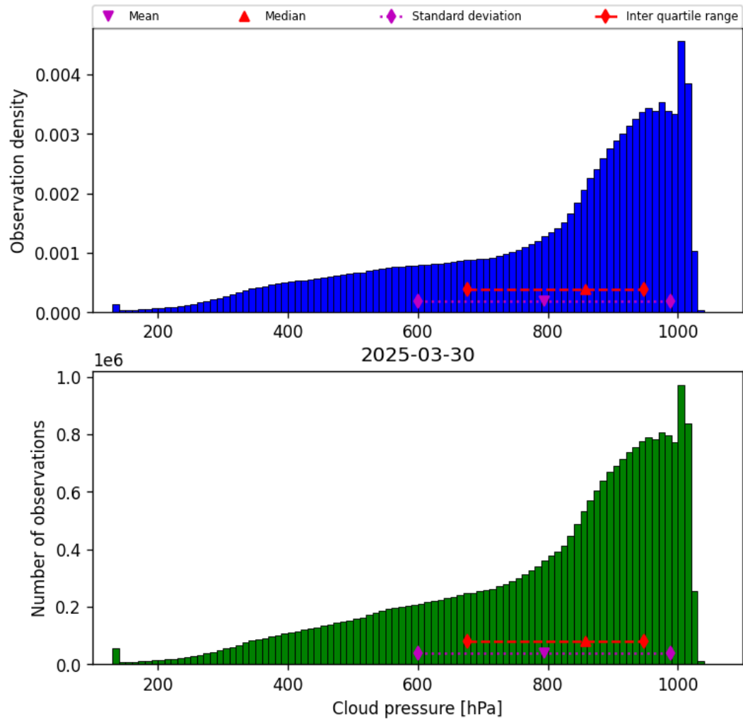
Figure 30: Histogram of “Cloud pressure” for 2025-03-29 to 2025-03-31
