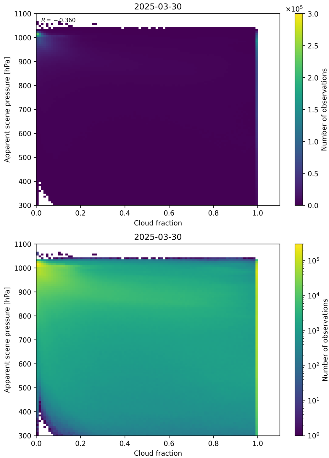
Figure 70: Scatter density plot of “Cloud fraction” against “Apparent scene pressure” for 2025-03-29 to 2025-03-31.
