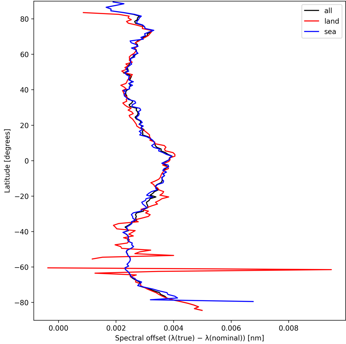
Figure 28: Zonal average of “Spectral offset ( \lambda_{\text{true}} - \lambda_{\text{nominal}} )” for 2025-03-29 to 2025-03-31.
