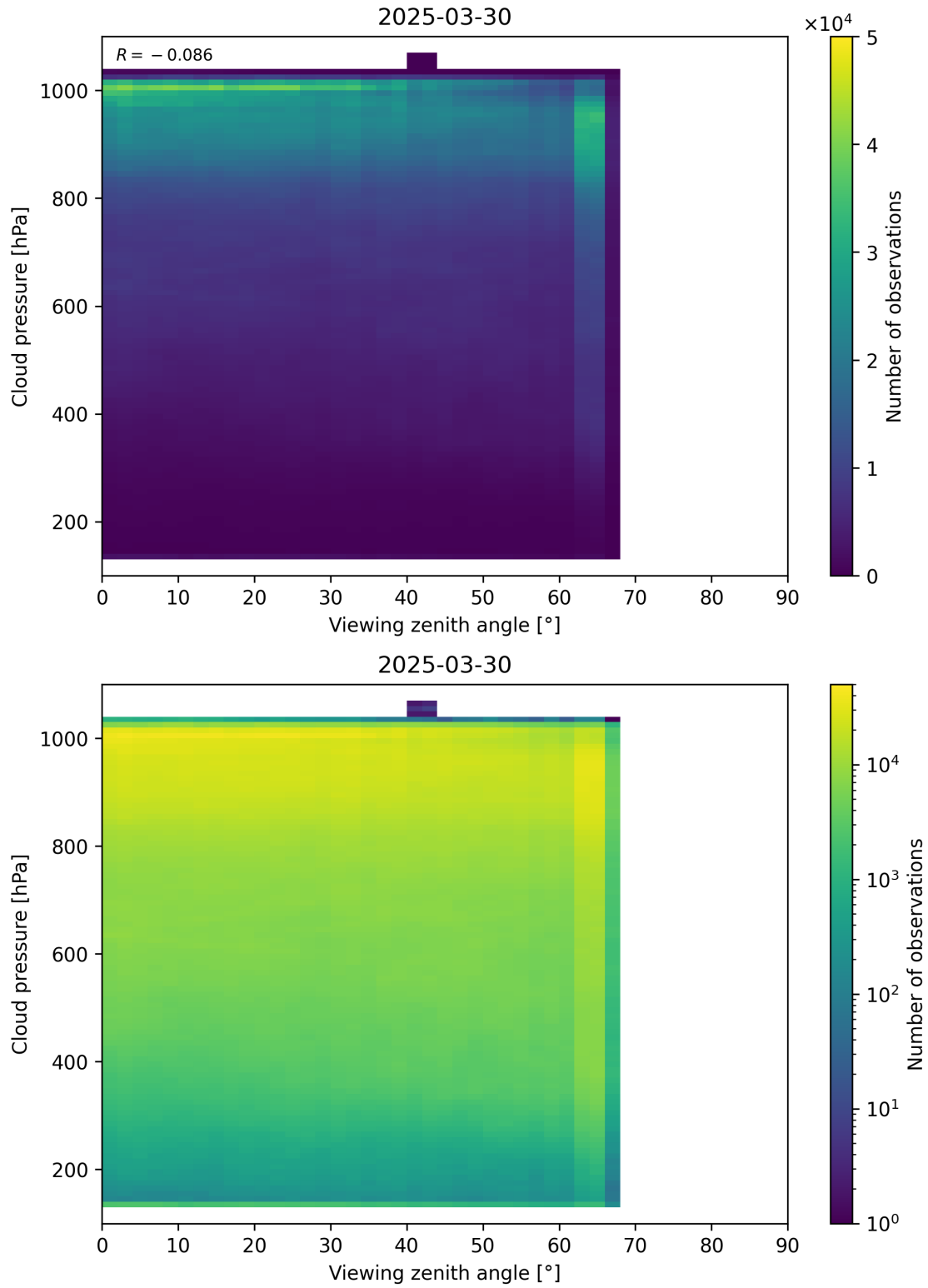
Figure 121: Scatter density plot of “Viewing zenith angle” against “Cloud pressure” for 2025-03-29 to 2025-03-31.
