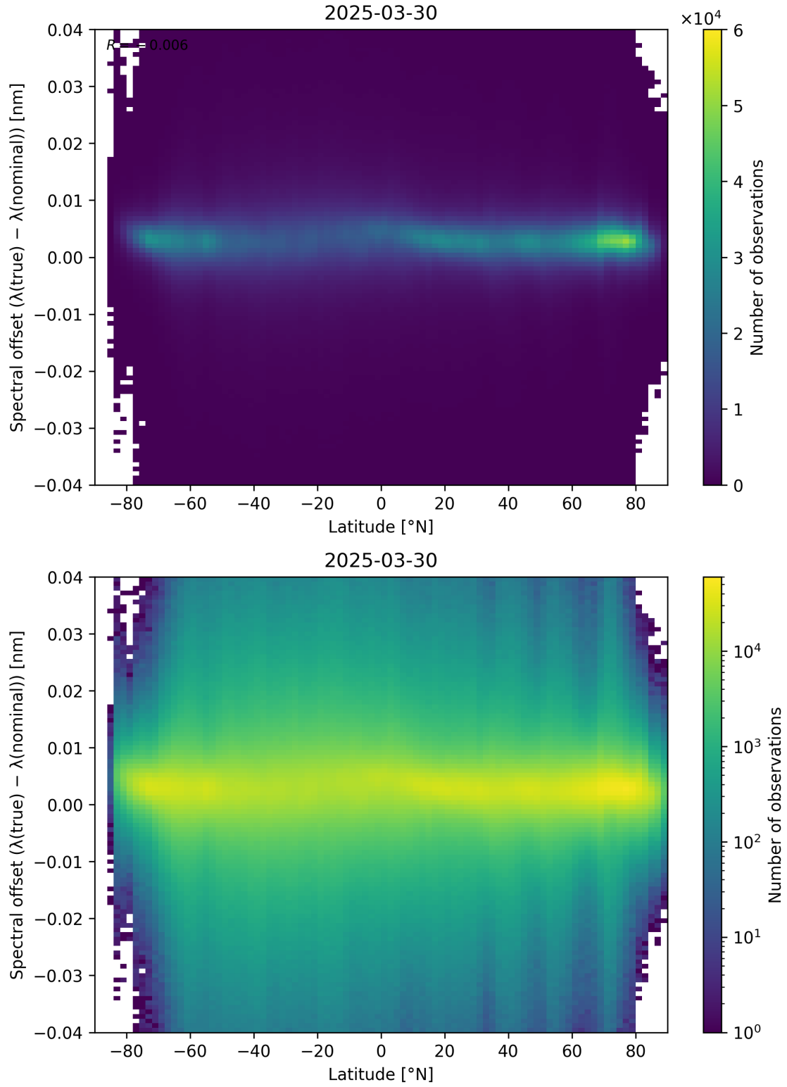
Figure 96: Scatter density plot of “Latitude” against “Spectral offset ( \lambda_{\text{true}} - \lambda_{\text{nominal}} )” for 2025-03-29 to 2025-03-31.
