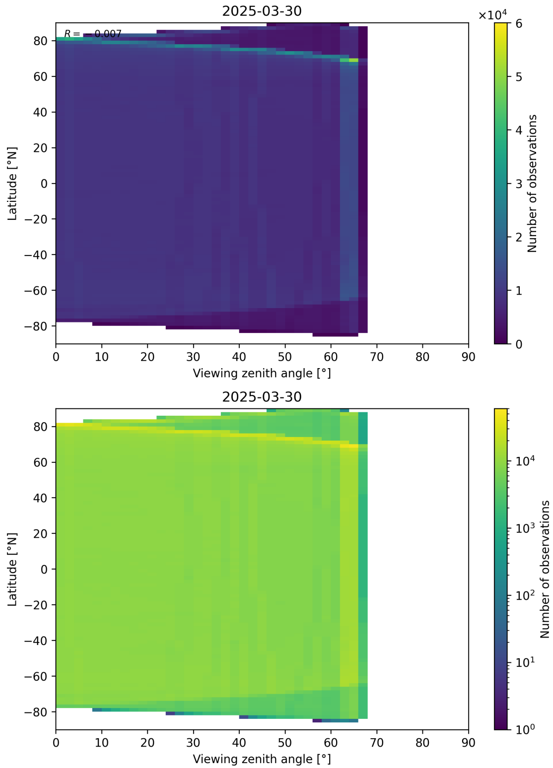
Figure 123: Scatter density plot of “Viewing zenith angle” against “Latitude” for 2025-03-29 to 2025-03-31.
