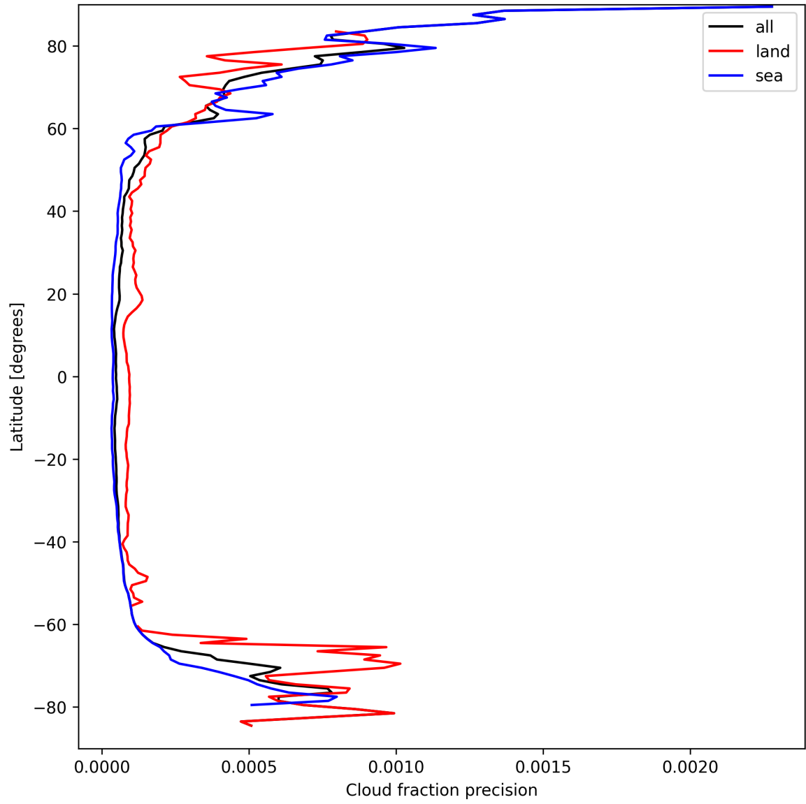
Figure 16: Zonal average of “Cloud fraction precision” for 2025-03-29 to 2025-03-31.
