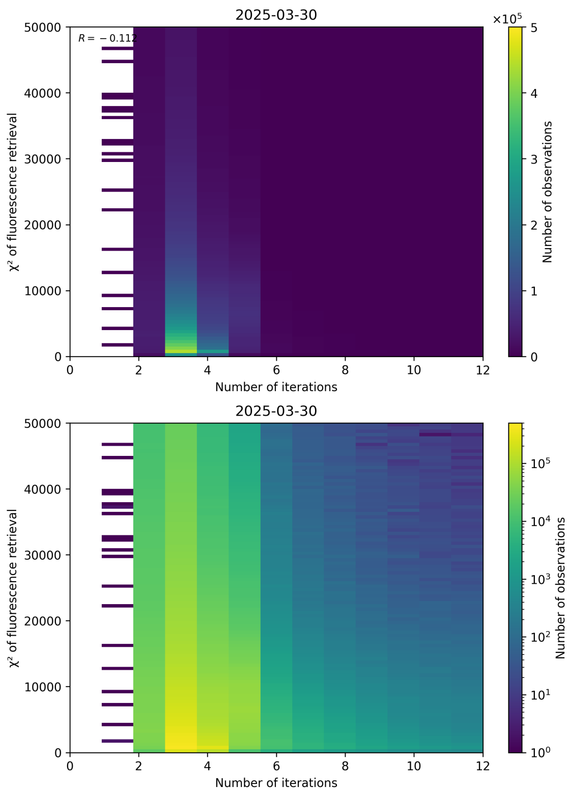
Figure 97: Scatter density plot of “Number of iterations” against “ \chi^2 of fluorescence retrieval” for 2025-03-29 to 2025-03-31.
