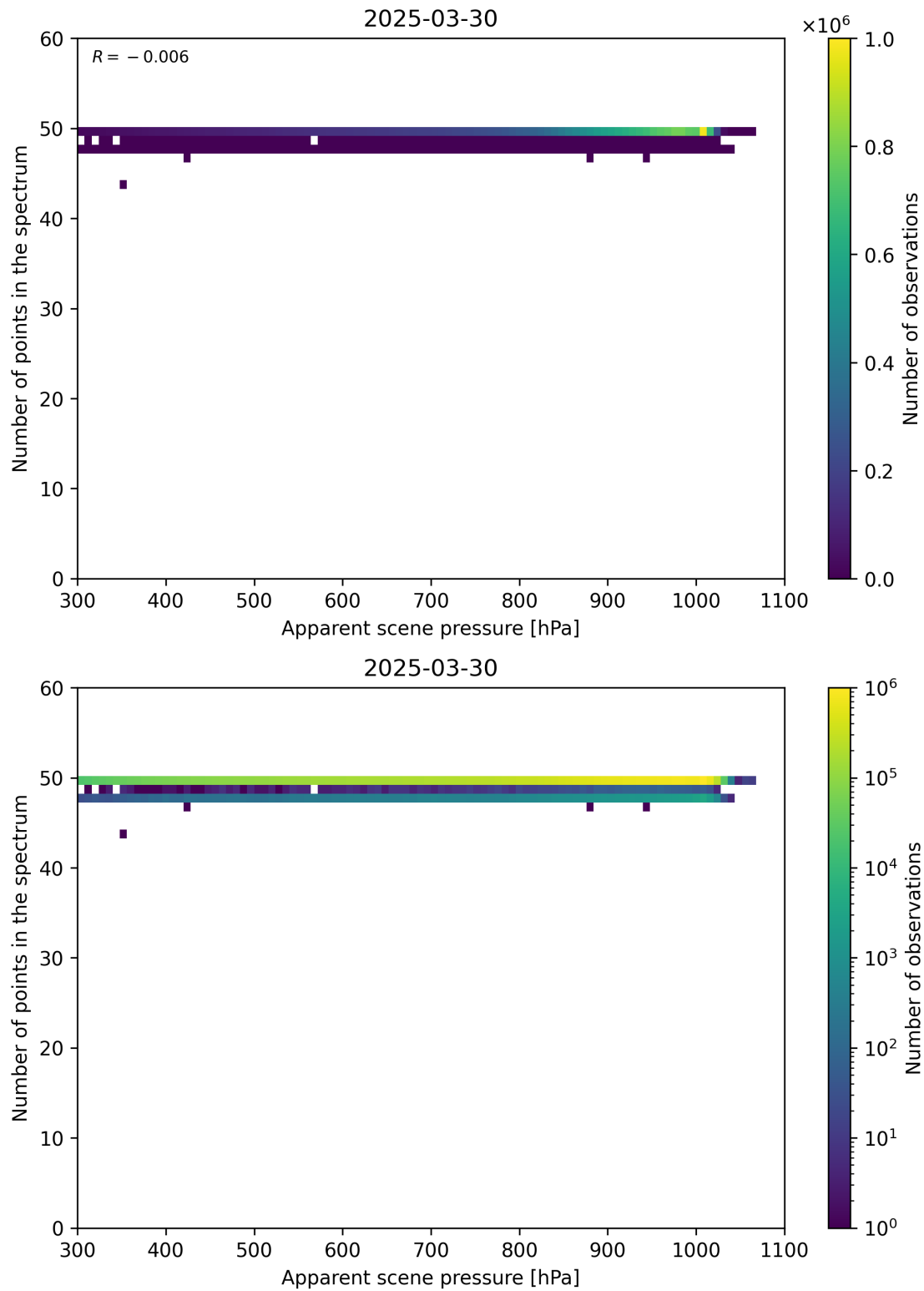
Figure 66: Scatter density plot of “Apparent scene pressure” against “Number of points in the spectrum” for 2025-03-29 to 2025-03-31.
