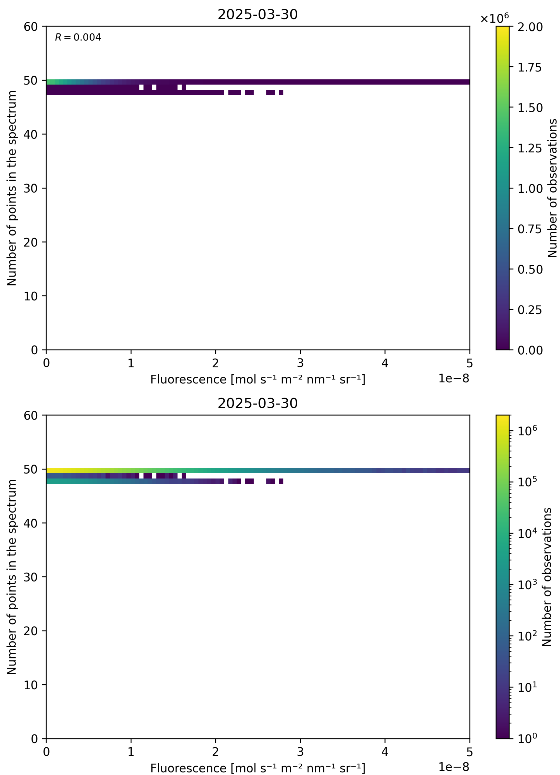
Figure 86: Scatter density plot of “Fluorescence” against “Number of points in the spectrum” for 2025-03-29 to 2025-03-31.
