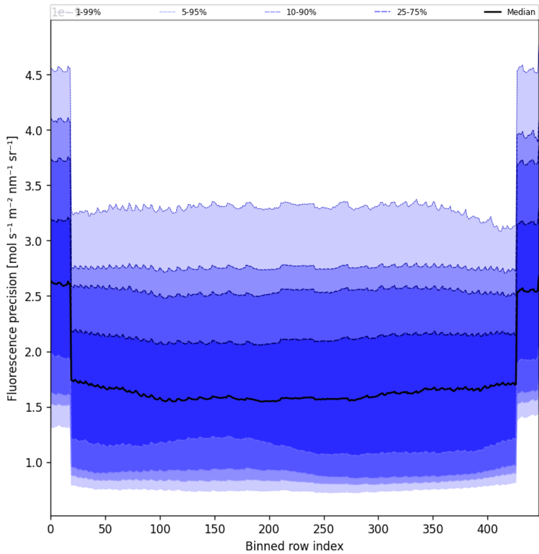
Figure 58: Along track statistics of “Fluorescence precision” for 2025-03-29 to 2025-03-31
