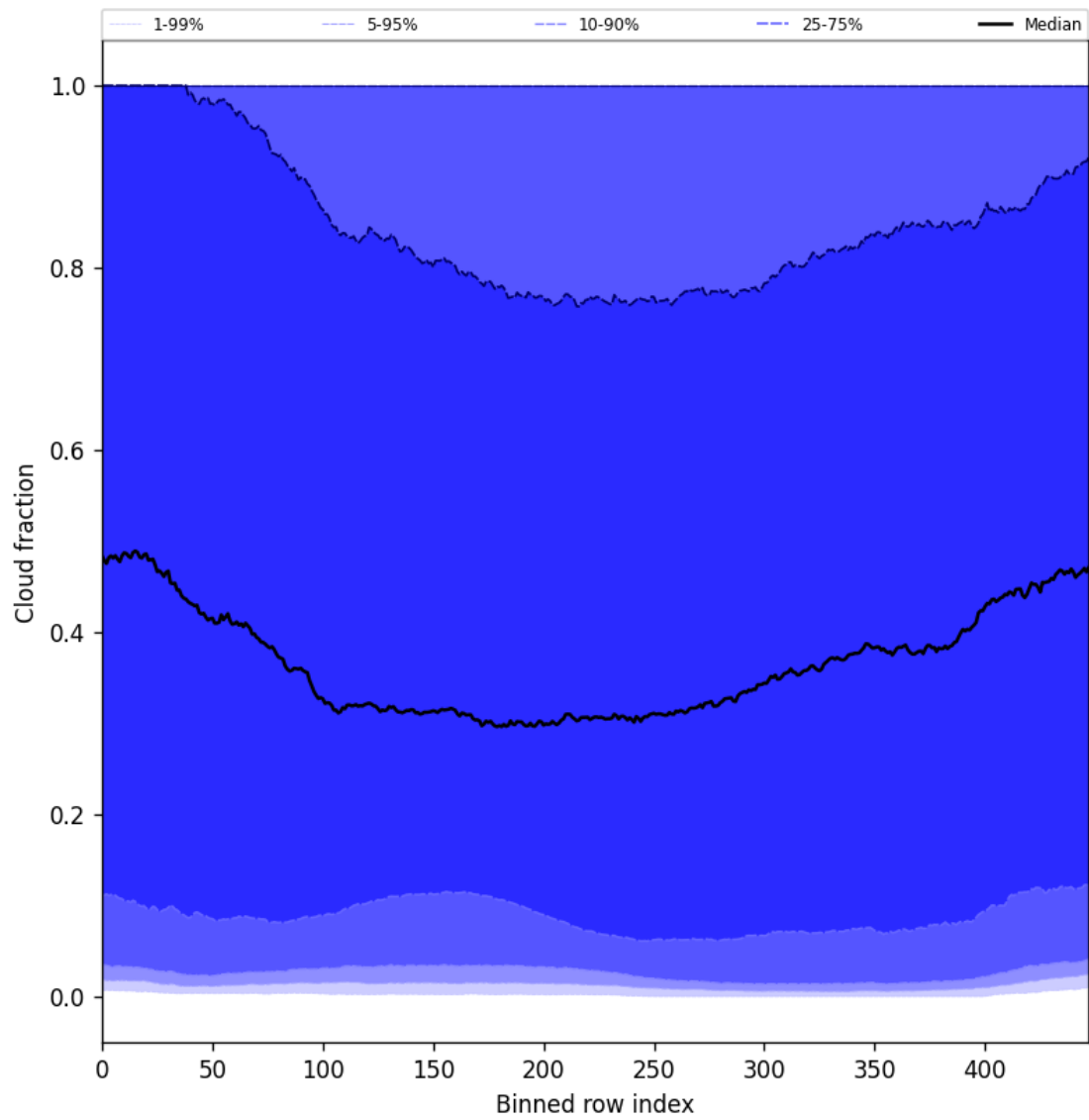
Figure 49: Along track statistics of “Cloud fraction” for 2025-03-29 to 2025-03-31
