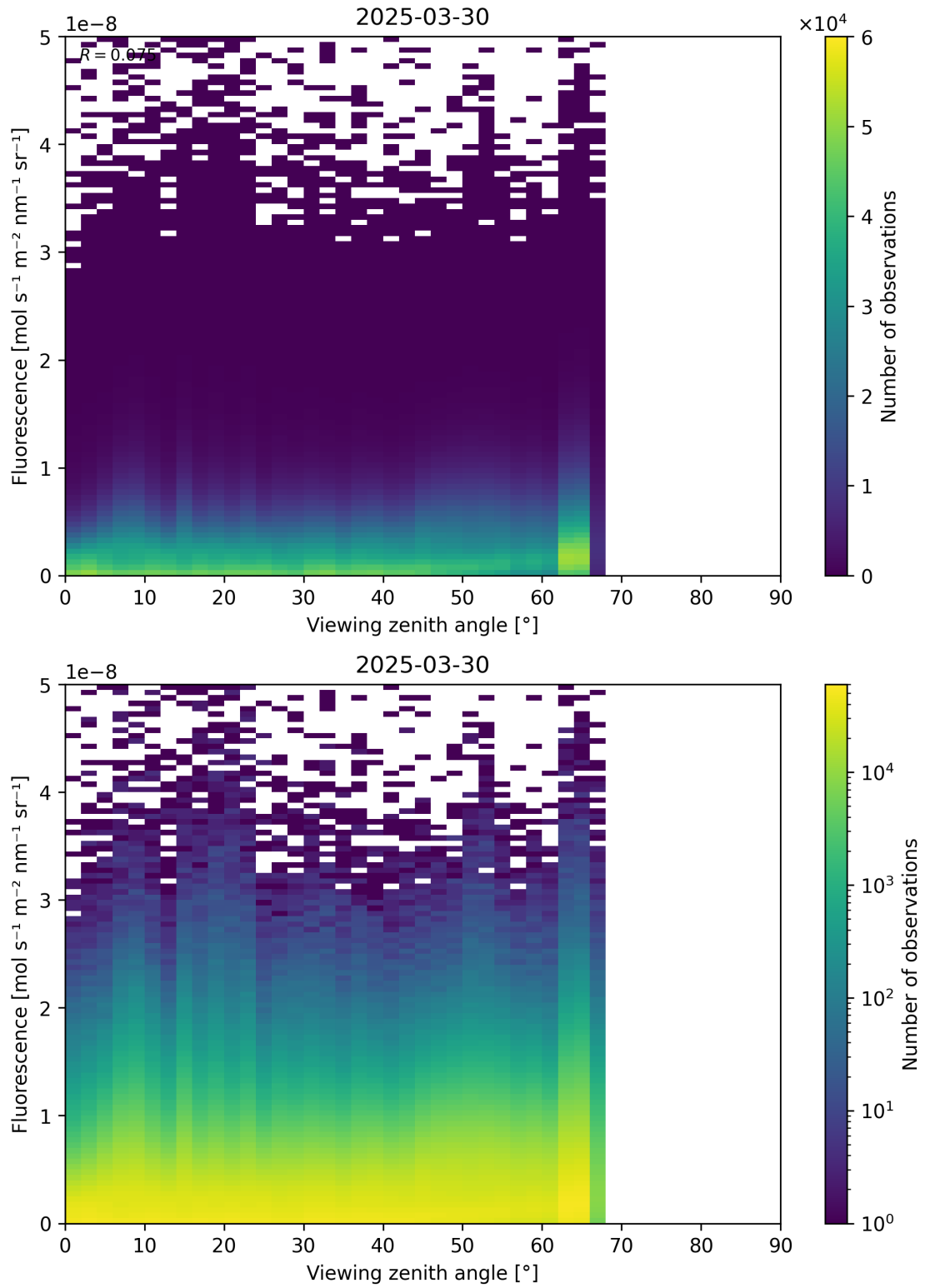
Figure 122: Scatter density plot of “Viewing zenith angle” against “Fluorescence” for 2025-03-29 to 2025-03-31.
