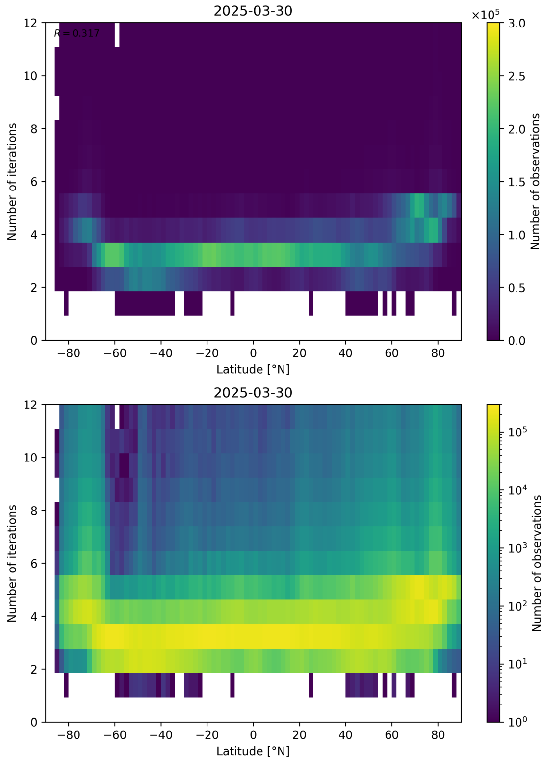
Figure 93: Scatter density plot of “Latitude” against “Number of iterations” for 2025-03-29 to 2025-03-31.
