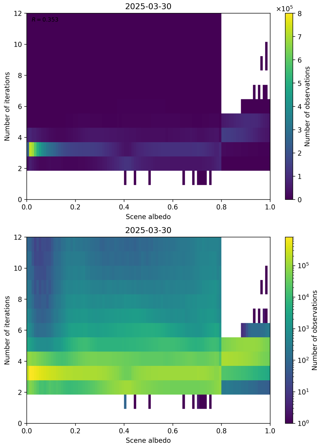
Figure 105: Scatter density plot of “Scene albedo” against “Number of iterations” for 2025-03-29 to 2025-03-31.
