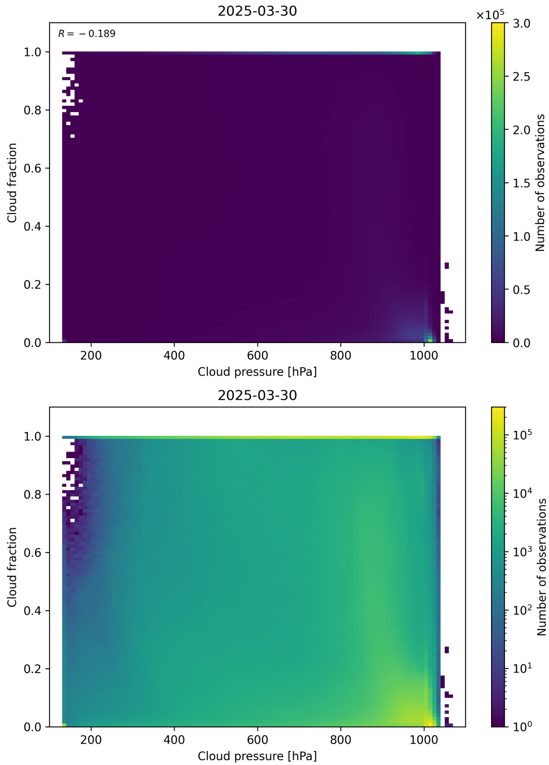
Figure 79: Scatter density plot of “Cloud pressure” against “Cloud fraction” for 2025-03-29 to 2025-03-31.
