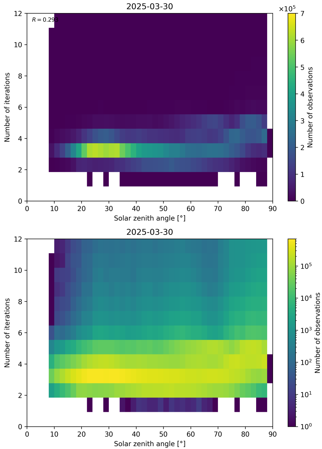
Figure 114: Scatter density plot of “Solar zenith angle” against “Number of iterations” for 2025-03-29 to 2025-03-31.
