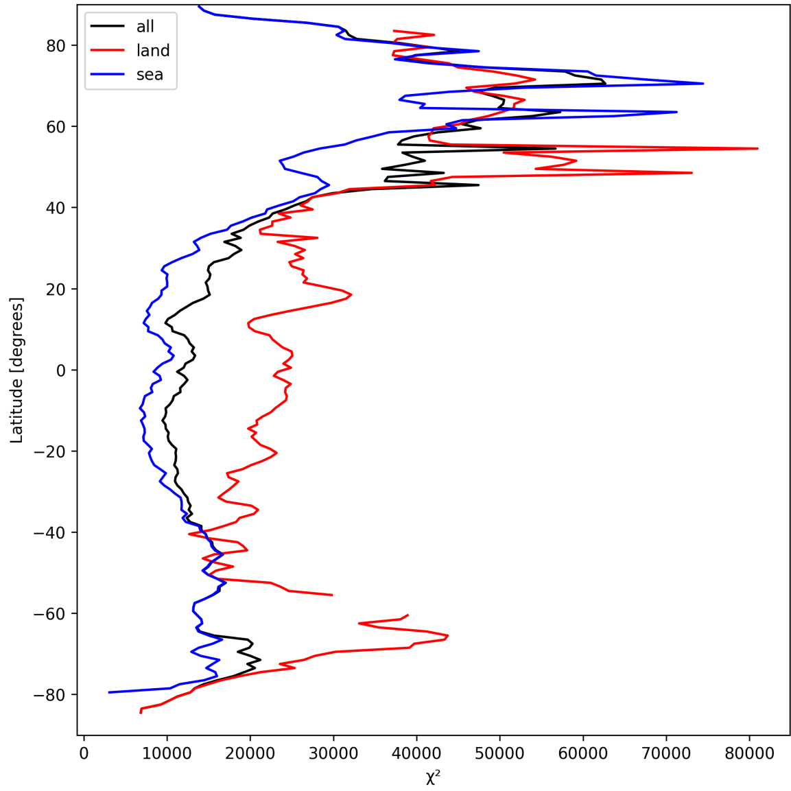
Figure 21: Zonal average of “ \chi^2 ” for 2025-03-29 to 2025-03-31.
