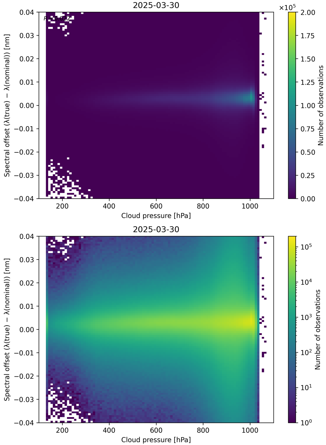
Figure 84: Scatter density plot of “Cloud pressure” against “Spectral offset ( \lambda_{\text{true}} - \lambda_{\text{nominal}} )” for 2025-03-29 to 2025-03-31.
