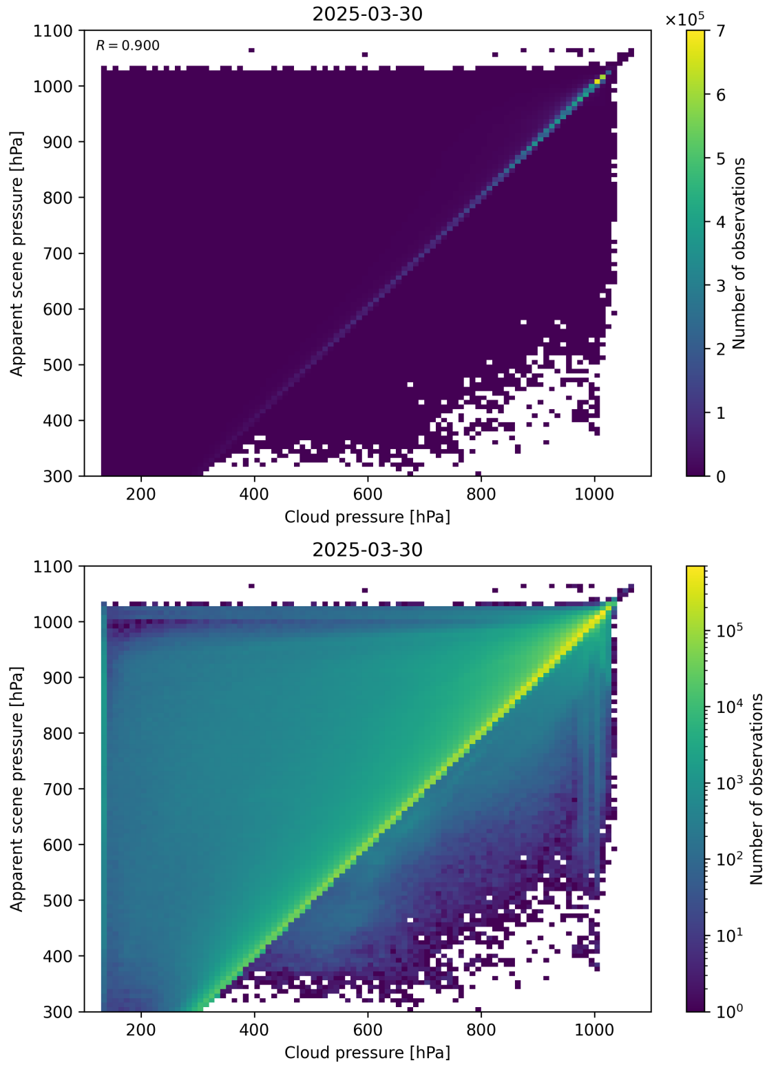
Figure 77: Scatter density plot of “Cloud pressure” against “Apparent scene pressure” for 2025-03-29 to 2025-03-31.
