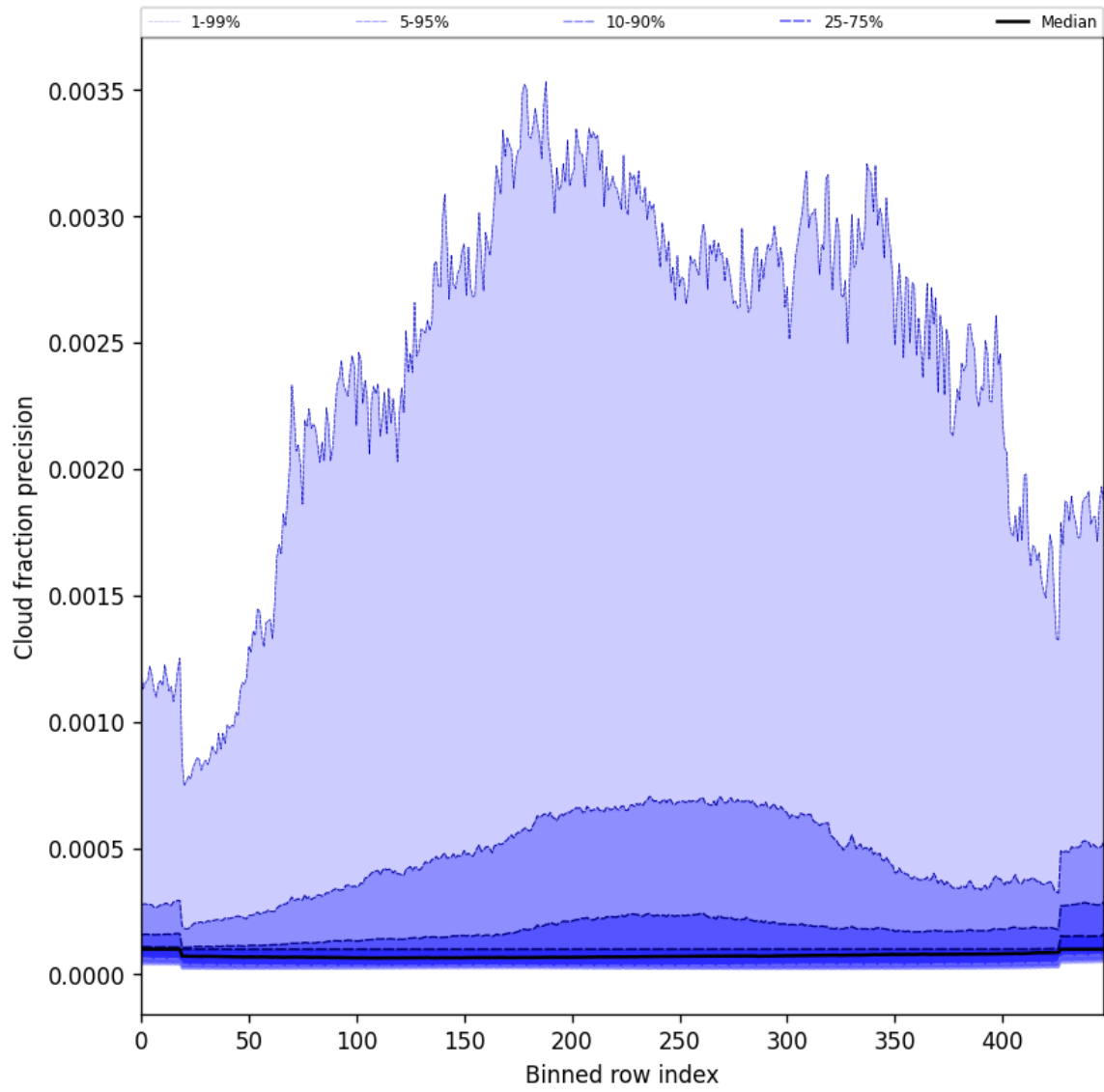
Figure 50: Along track statistics of “Cloud fraction precision” for 2025-03-29 to 2025-03-31
