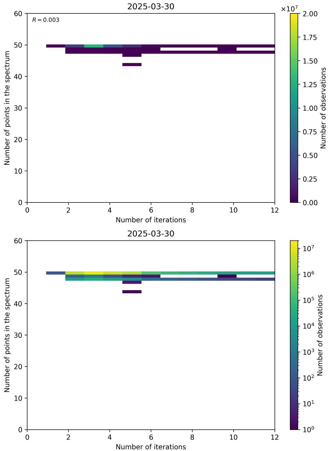
Figure 99: Scatter density plot of “Number of iterations” against “Number of points in the spectrum” for 2025-03-29 to 2025-03-31.
