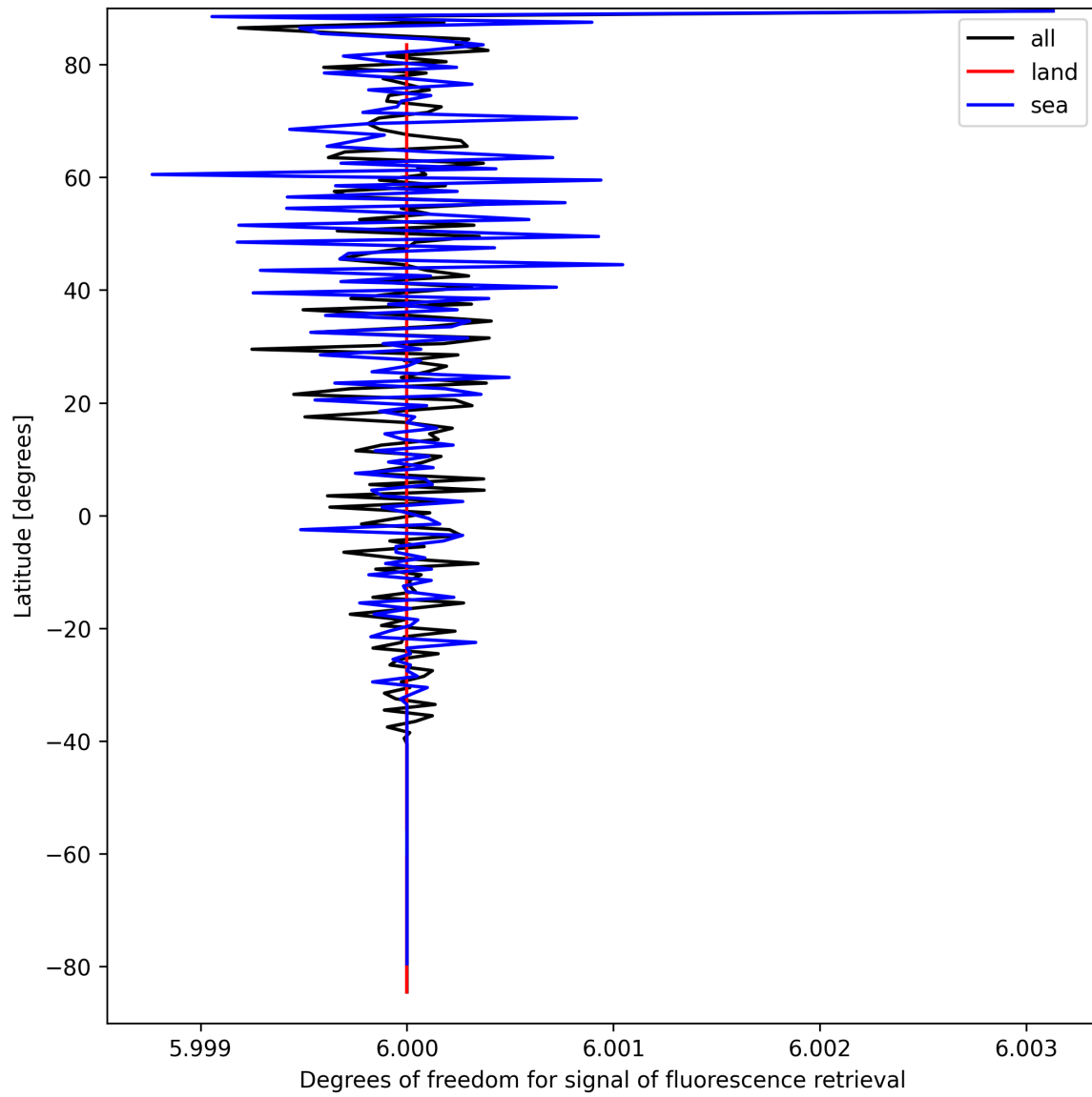
Figure 26: Zonal average of “Degrees of freedom for signal of fluorescence retrieval” for 2025-03-29 to 2025-03-31.
