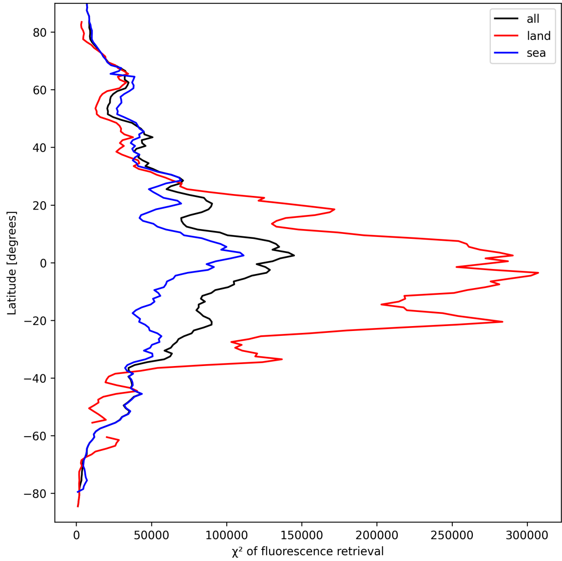
Figure 25: Zonal average of “ \chi^2 of fluorescence retrieval” for 2025-03-29 to 2025-03-31.
