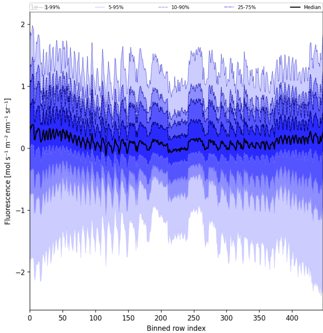
Figure 57: Along track statistics of “Fluorescence” for 2025-03-29 to 2025-03-31
