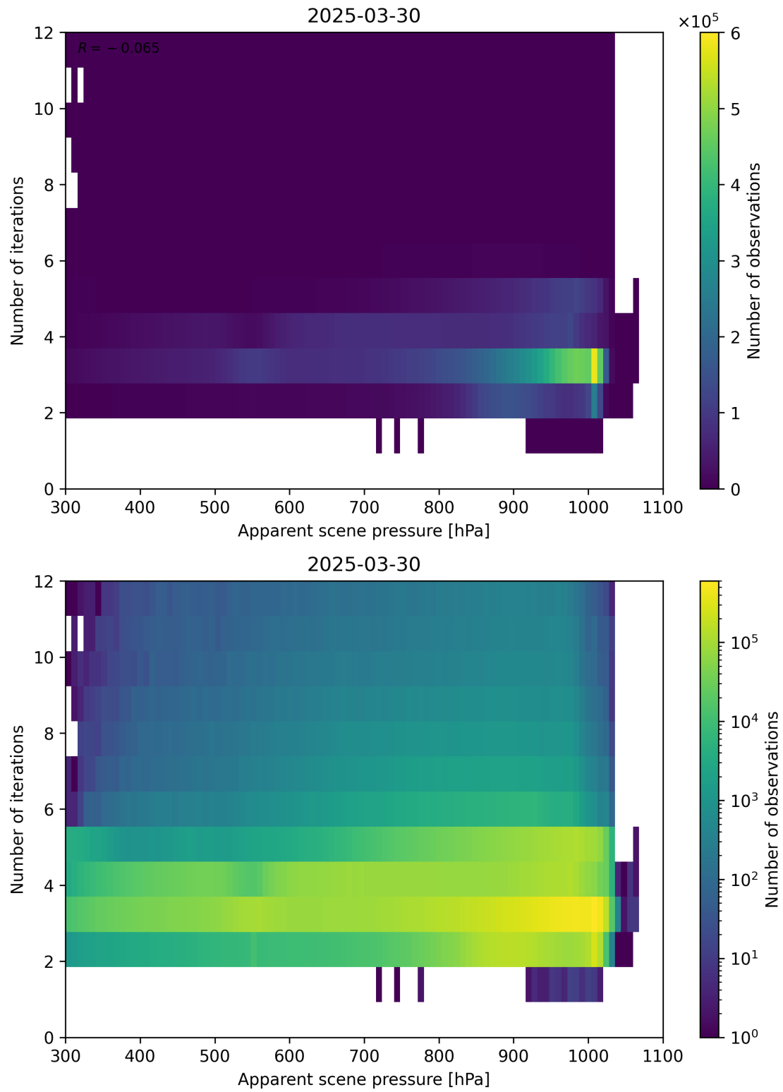
Figure 65: Scatter density plot of “Apparent scene pressure” against “Number of iterations” for 2025-03-29 to 2025-03-31.
