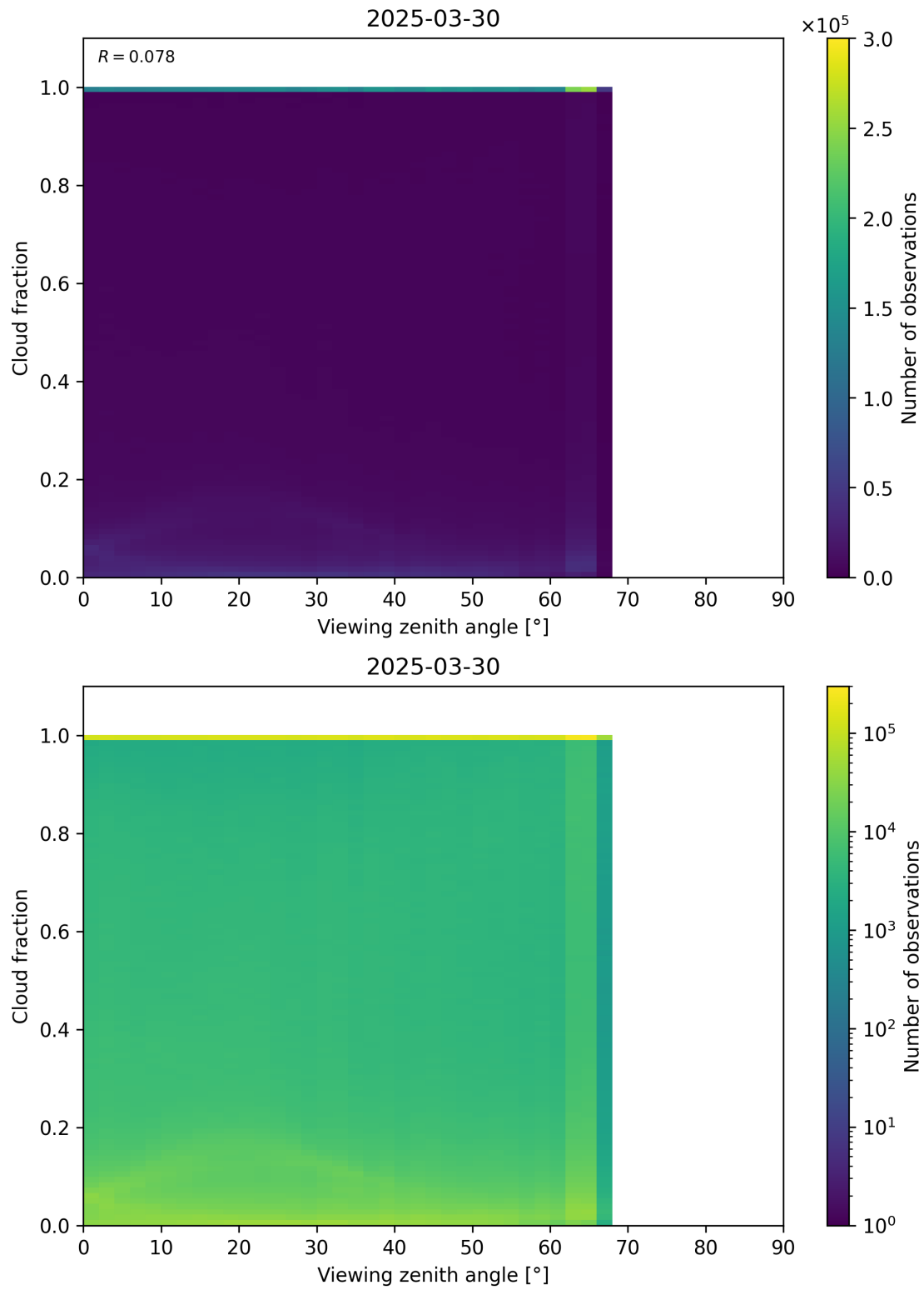
Figure 120: Scatter density plot of “Viewing zenith angle” against “Cloud fraction” for 2025-03-29 to 2025-03-31.
