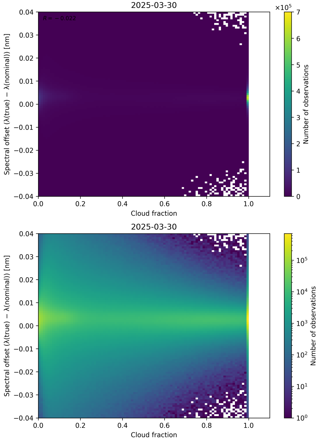
Figure 76: Scatter density plot of “Cloud fraction” against “Spectral offset ( \lambda_{\text{true}} - \lambda_{\text{nominal}} )” for 2025-03-29 to 2025-03-31.
