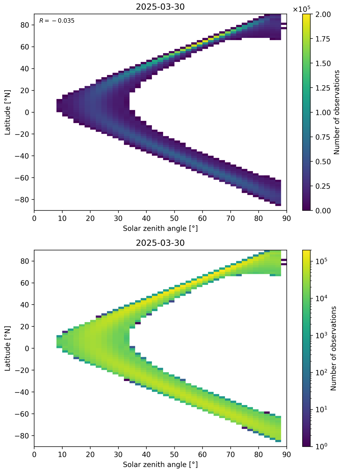
Figure 113: Scatter density plot of “Solar zenith angle” against “Latitude” for 2025-03-29 to 2025-03-31.
