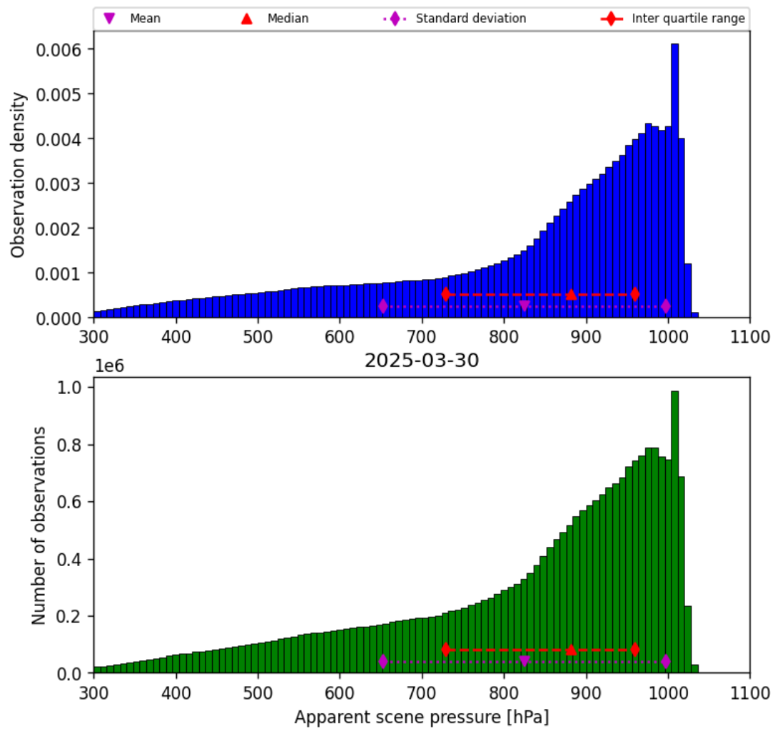
Figure 36: Histogram of “Apparent scene pressure” for 2025-03-29 to 2025-03-31
