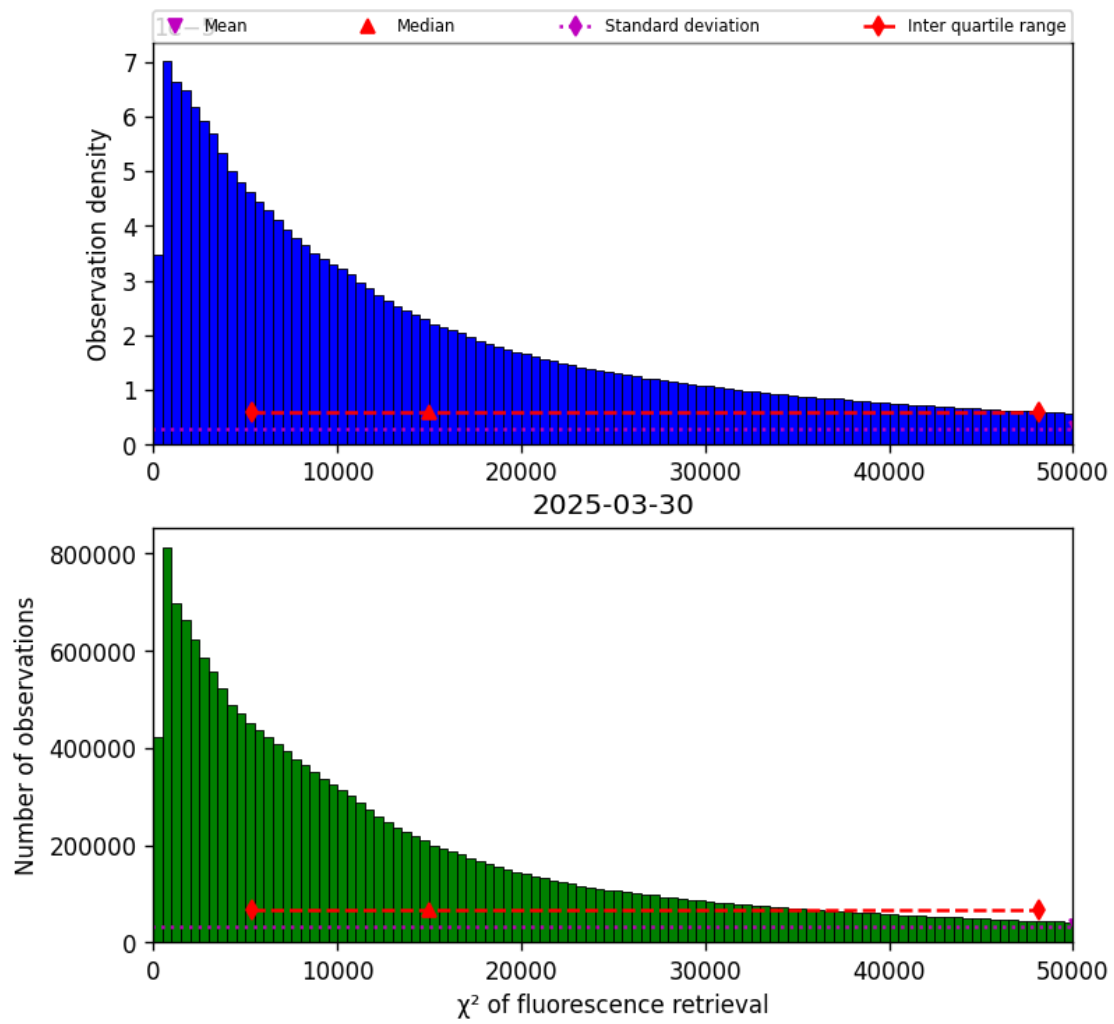
Figure 42: Histogram of “ \chi^2 of fluorescence retrieval” for 2025-03-29 to 2025-03-31
