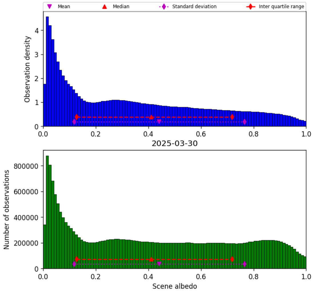
Figure 34: Histogram of “Scene albedo” for 2025-03-29 to 2025-03-31
