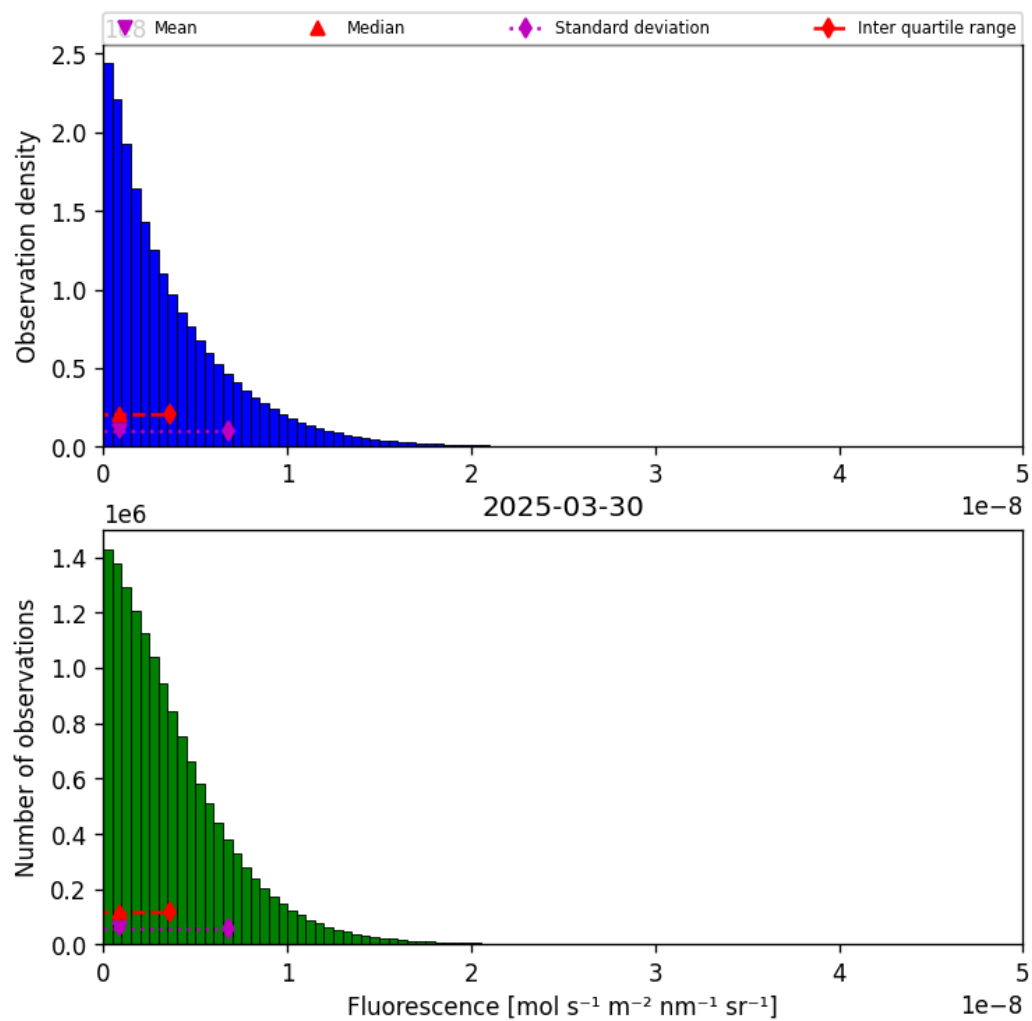
Figure 40: Histogram of “Fluorescence” for 2025-03-29 to 2025-03-31
