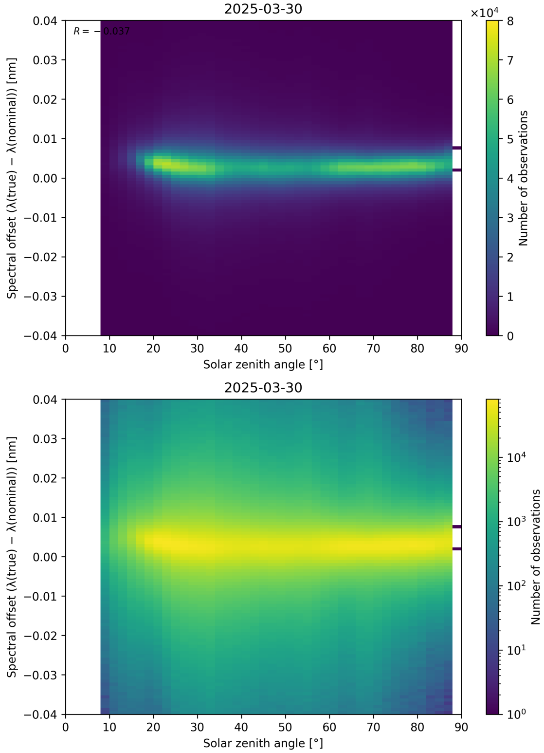
Figure 117: Scatter density plot of “Solar zenith angle” against “Spectral offset ( \lambda_{\text{true}} - \lambda_{\text{nominal}} )” for 2025-03-29 to 2025-03-31.
