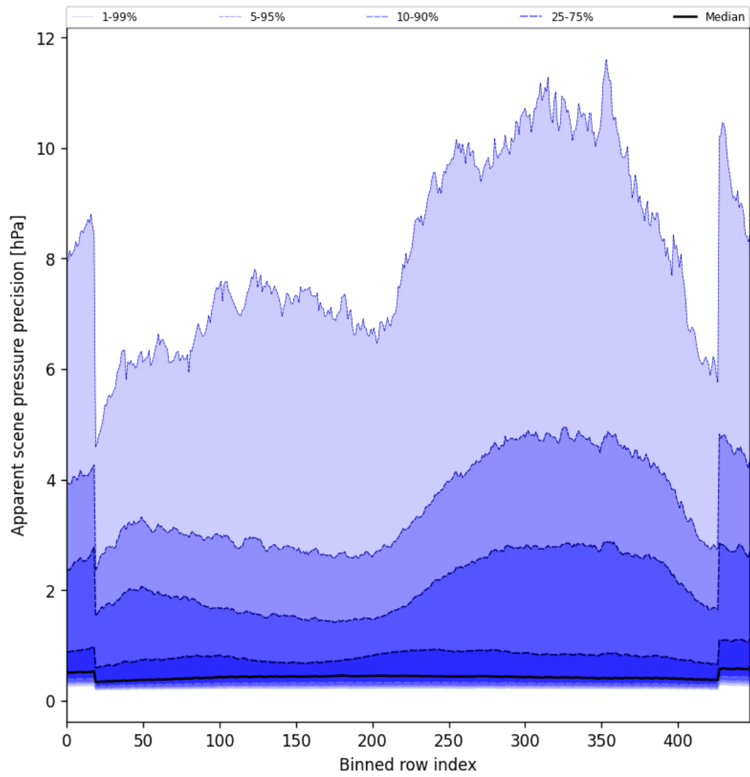
Figure 54: Along track statistics of “Apparent scene pressure precision” for 2025-03-29 to 2025-03-31
