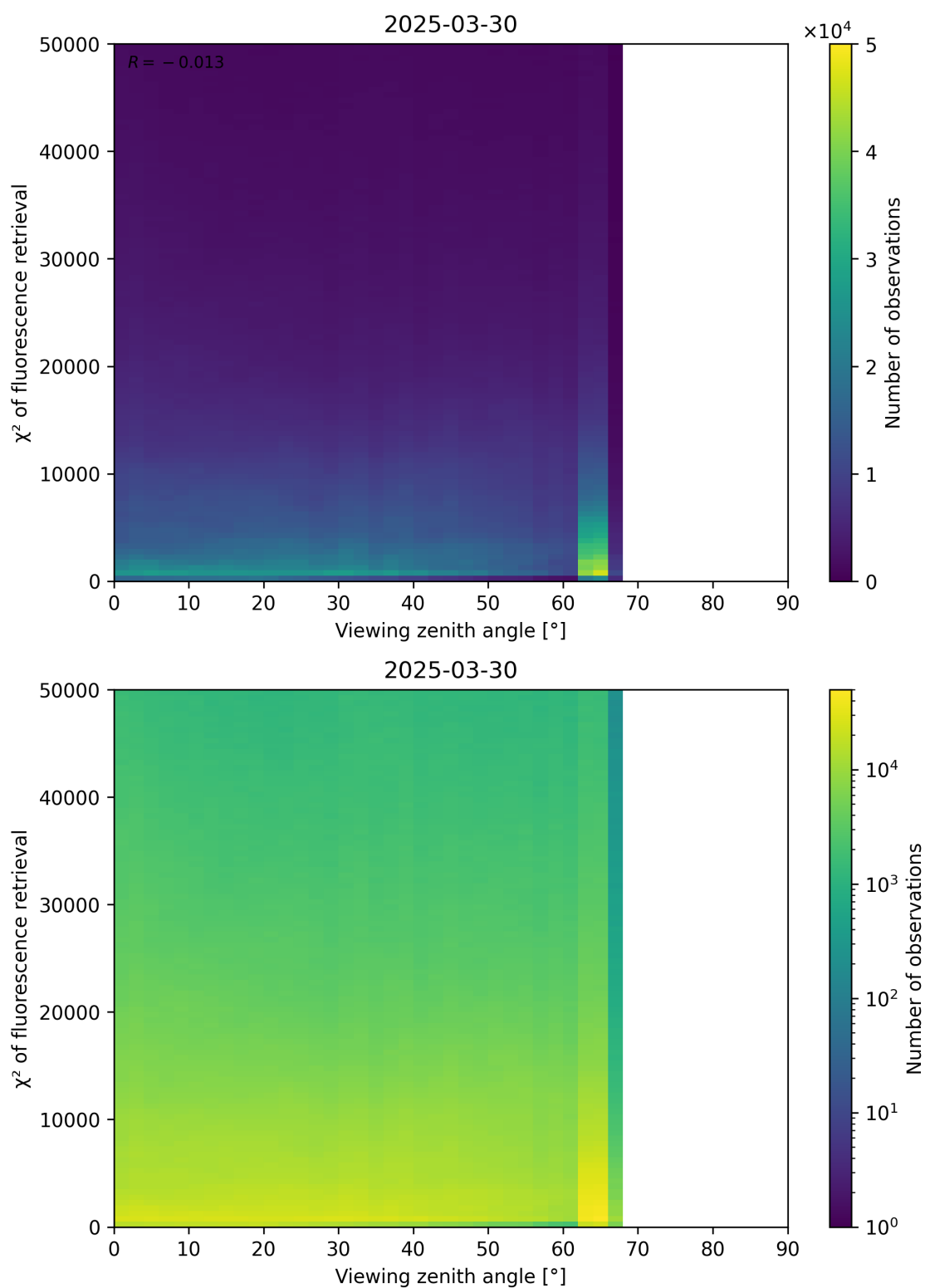
Figure 119: Scatter density plot of “Viewing zenith angle” against “ \chi^2 of fluorescence retrieval” for 2025-03-29 to 2025-03-31.
