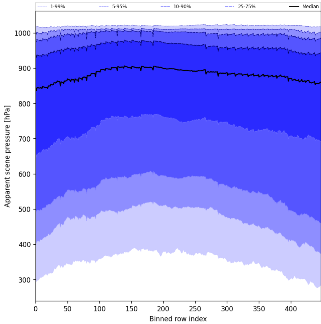
Figure 53: Along track statistics of “Apparent scene pressure” for 2025-03-29 to 2025-03-31
