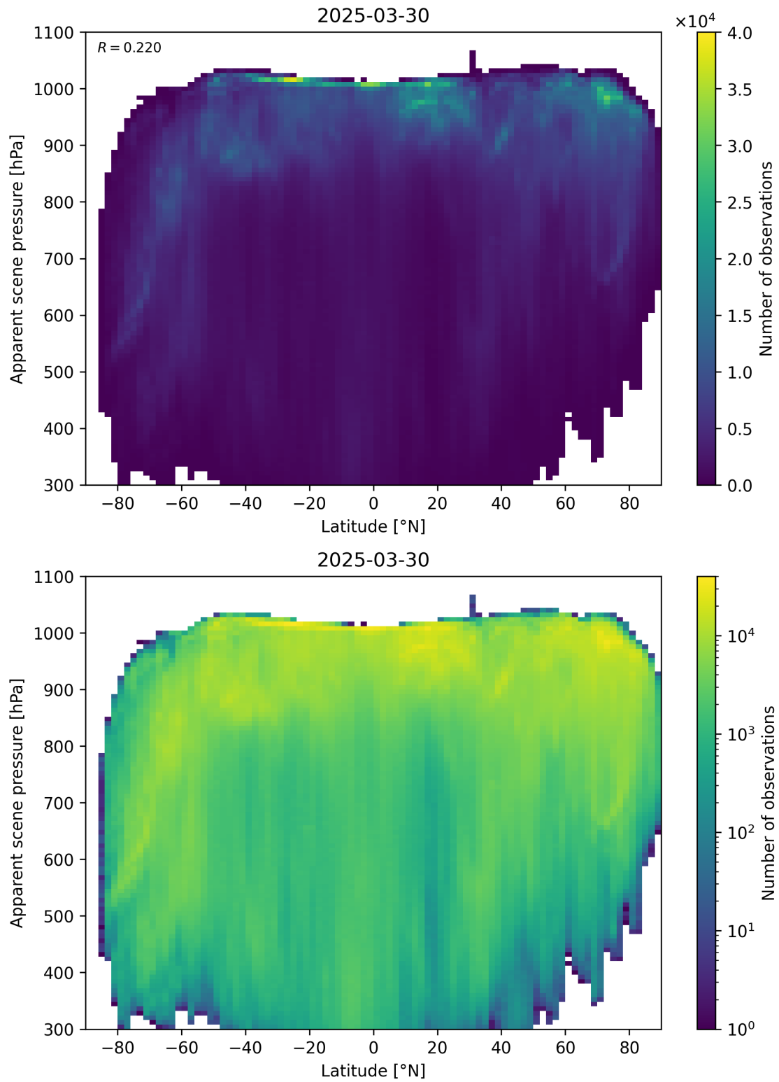
Figure 88: Scatter density plot of “Latitude” against “Apparent scene pressure” for 2025-03-29 to 2025-03-31.
