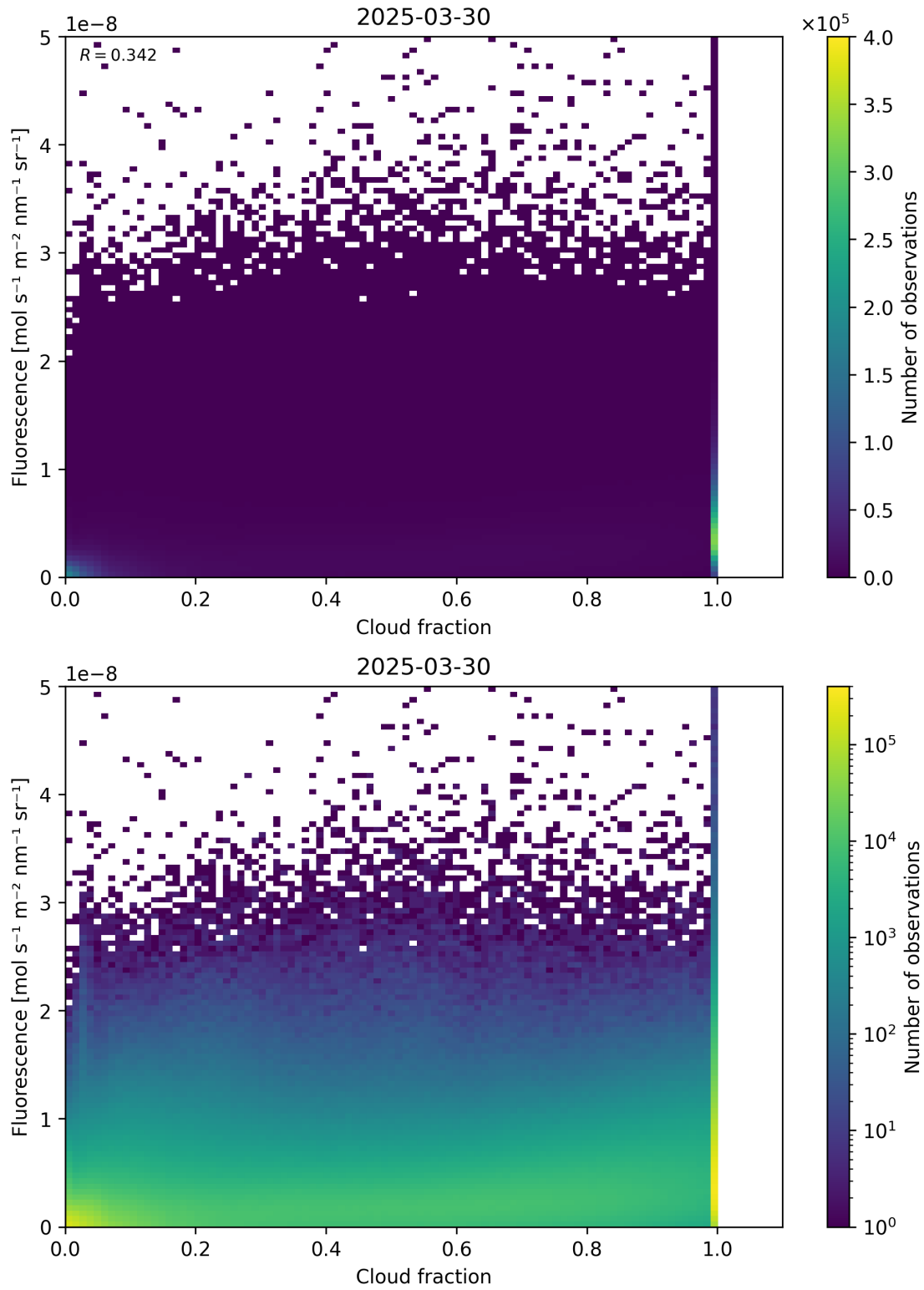
Figure 72: Scatter density plot of “Cloud fraction” against “Fluorescence” for 2025-03-29 to 2025-03-31.
