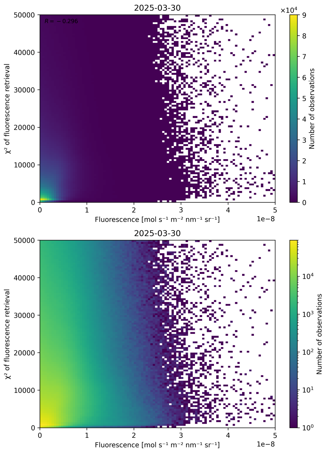
Figure 85: Scatter density plot of “Fluorescence” against “ \chi^2 of fluorescence retrieval” for 2025-03-29 to 2025-03-31.
