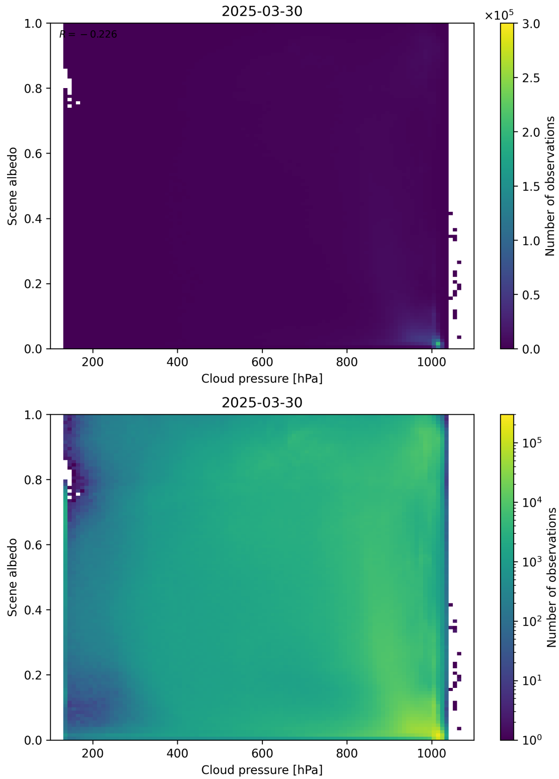
Figure 83: Scatter density plot of “Cloud pressure” against “Scene albedo” for 2025-03-29 to 2025-03-31.
