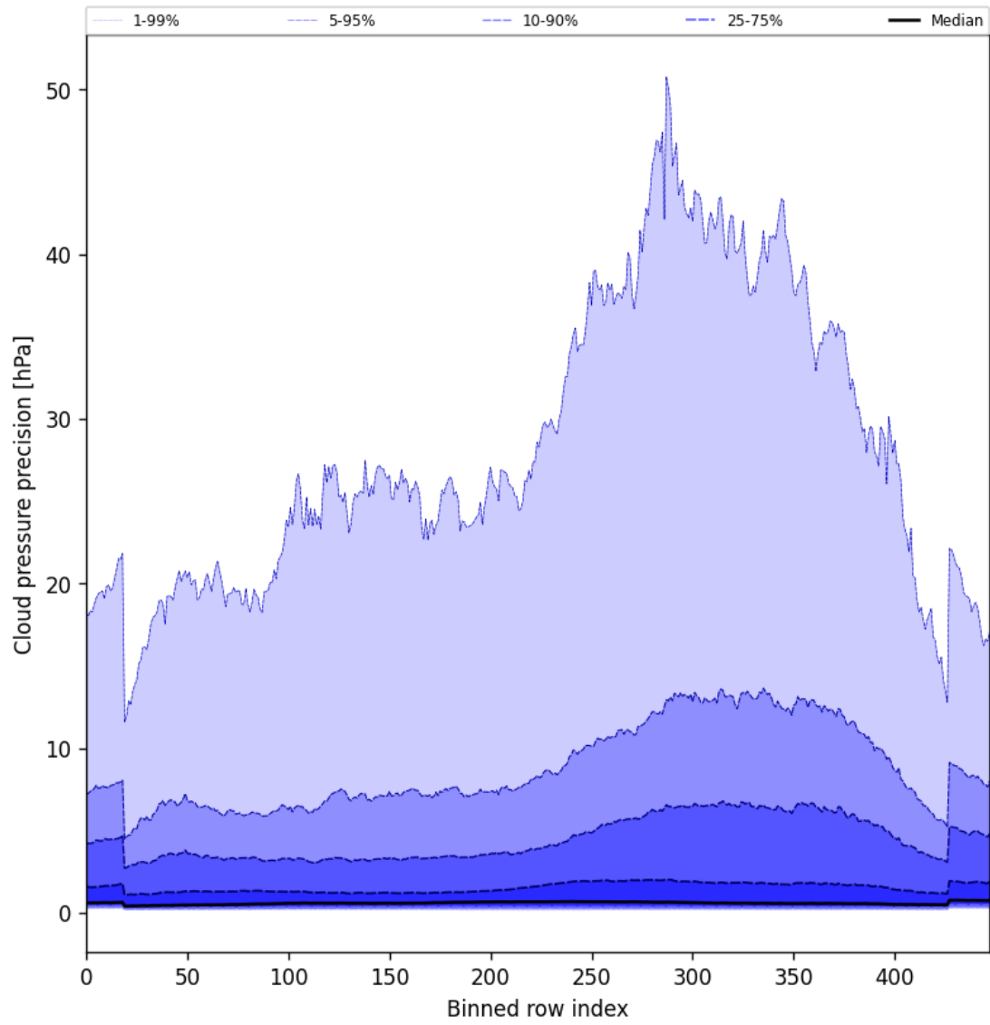
Figure 48: Along track statistics of “Cloud pressure precision” for 2025-03-29 to 2025-03-31
