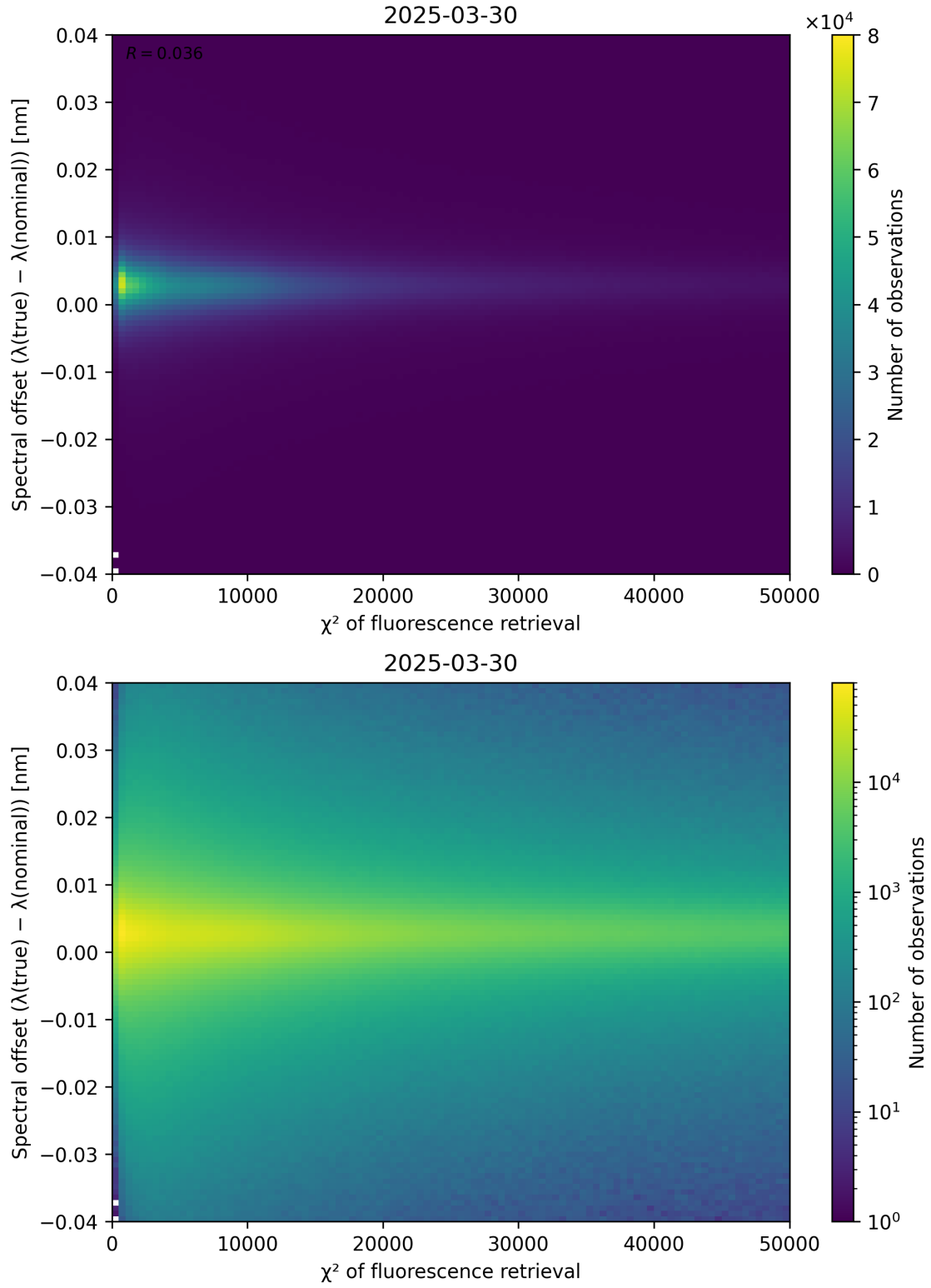
Figure 69: Scatter density plot of “ \chi^2 of fluorescence retrieval” against “Spectral offset ( \lambda_{\text{true}} - \lambda_{\text{nominal}} )” for 2025-03-29 to 2025-03-31.
