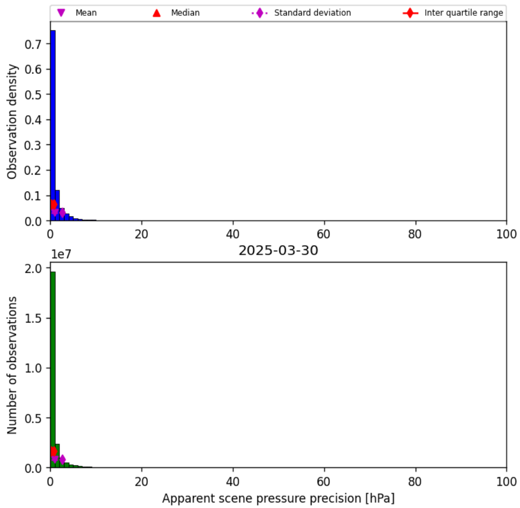
Figure 37: Histogram of “Apparent scene pressure precision” for 2025-03-29 to 2025-03-31
