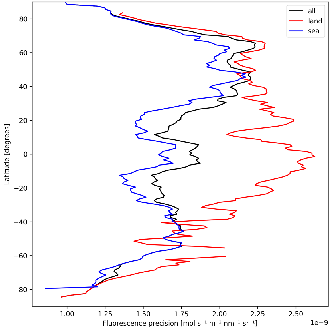
Figure 24: Zonal average of “Fluorescence precision” for 2025-03-29 to 2025-03-31.
