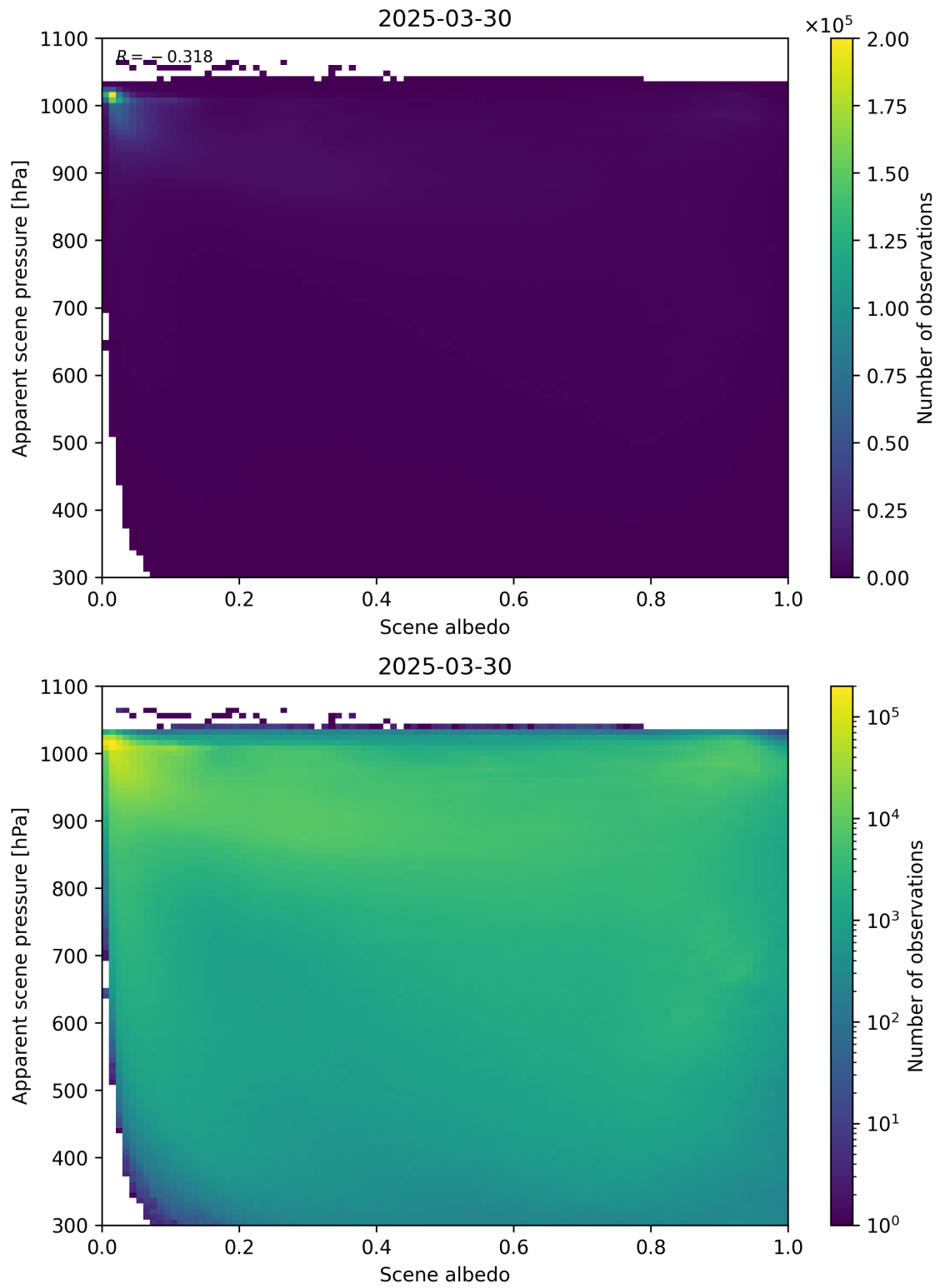
Figure 102: Scatter density plot of “Scene albedo” against “Apparent scene pressure” for 2025-03-29 to 2025-03-31.
