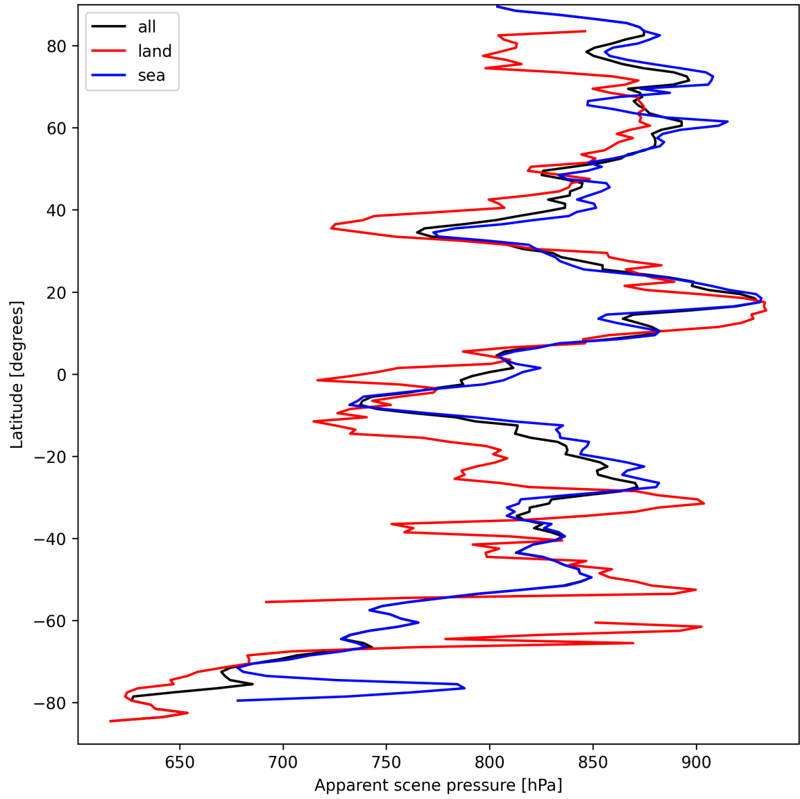
Figure 19: Zonal average of “Apparent scene pressure” for 2025-03-29 to 2025-03-31.
