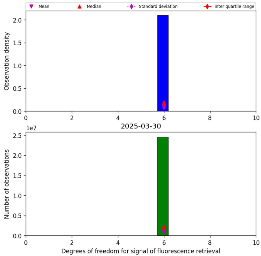
Figure 43: Histogram of “Degrees of freedom for signal of fluorescence retrieval” for 2025-03-29 to 2025-03-31
