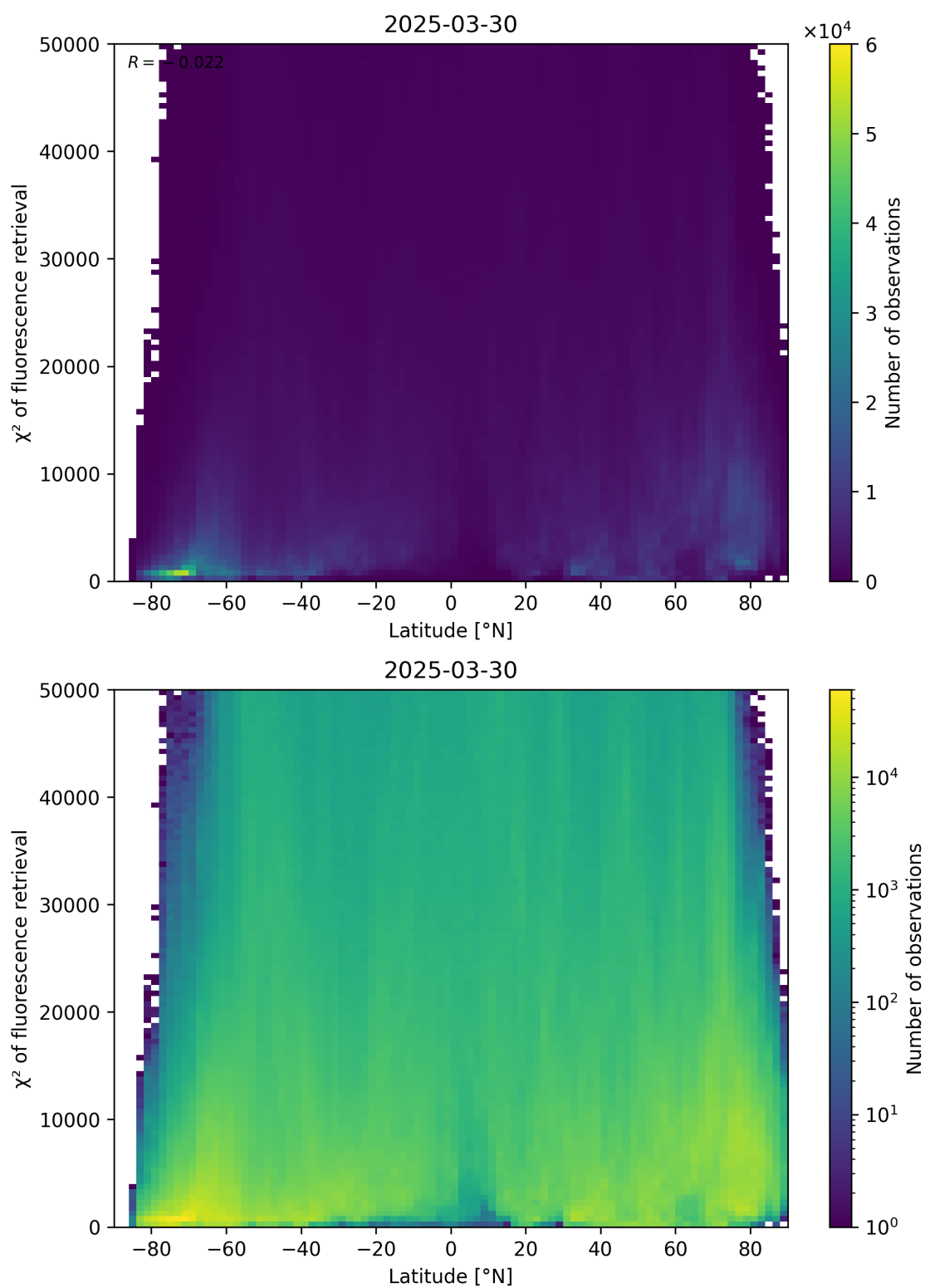
Figure 89: Scatter density plot of “Latitude” against “ \chi^2 of fluorescence retrieval” for 2025-03-29 to 2025-03-31.
