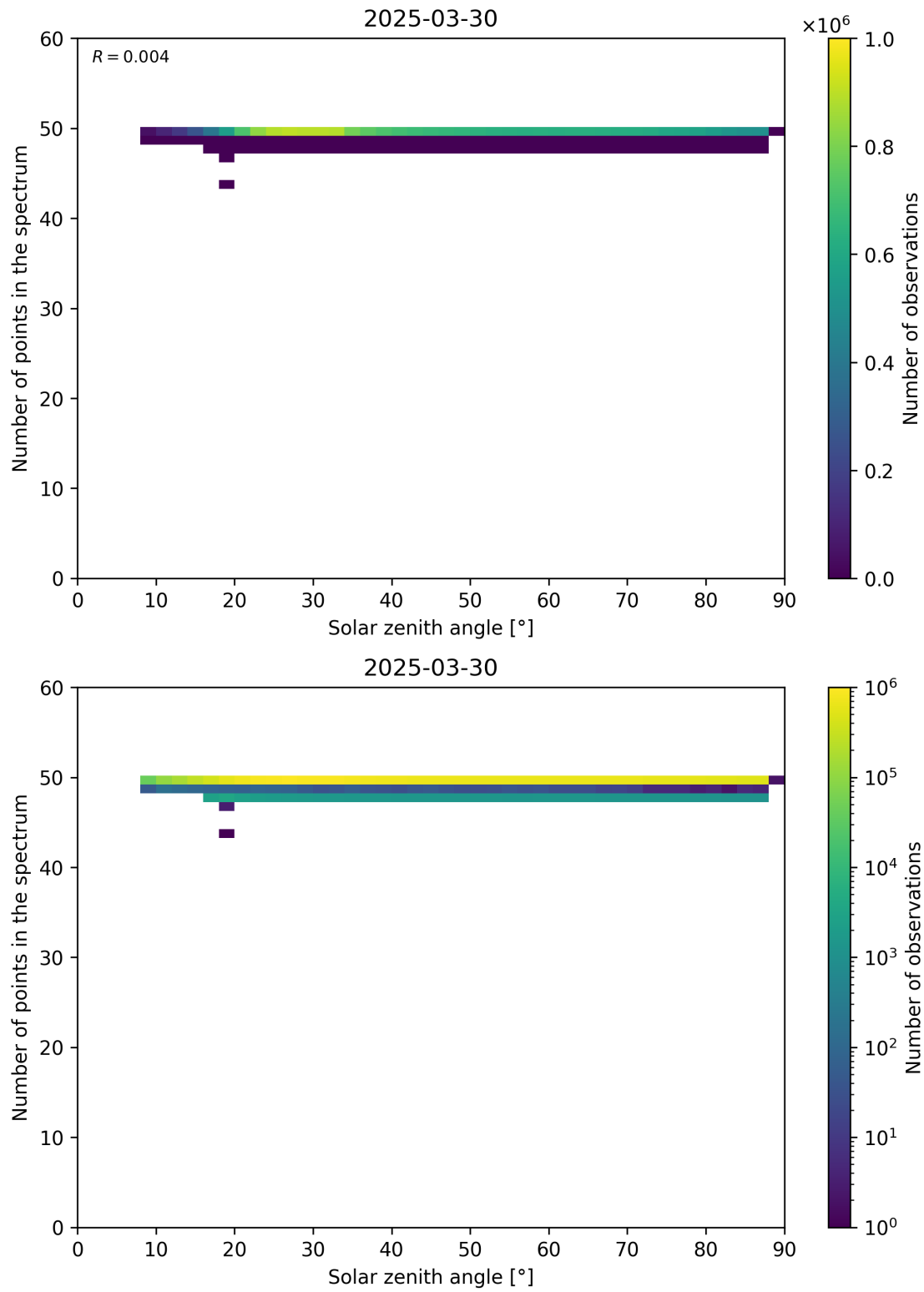
Figure 115: Scatter density plot of “Solar zenith angle” against “Number of points in the spectrum” for 2025-03-29 to 2025-03-31.
