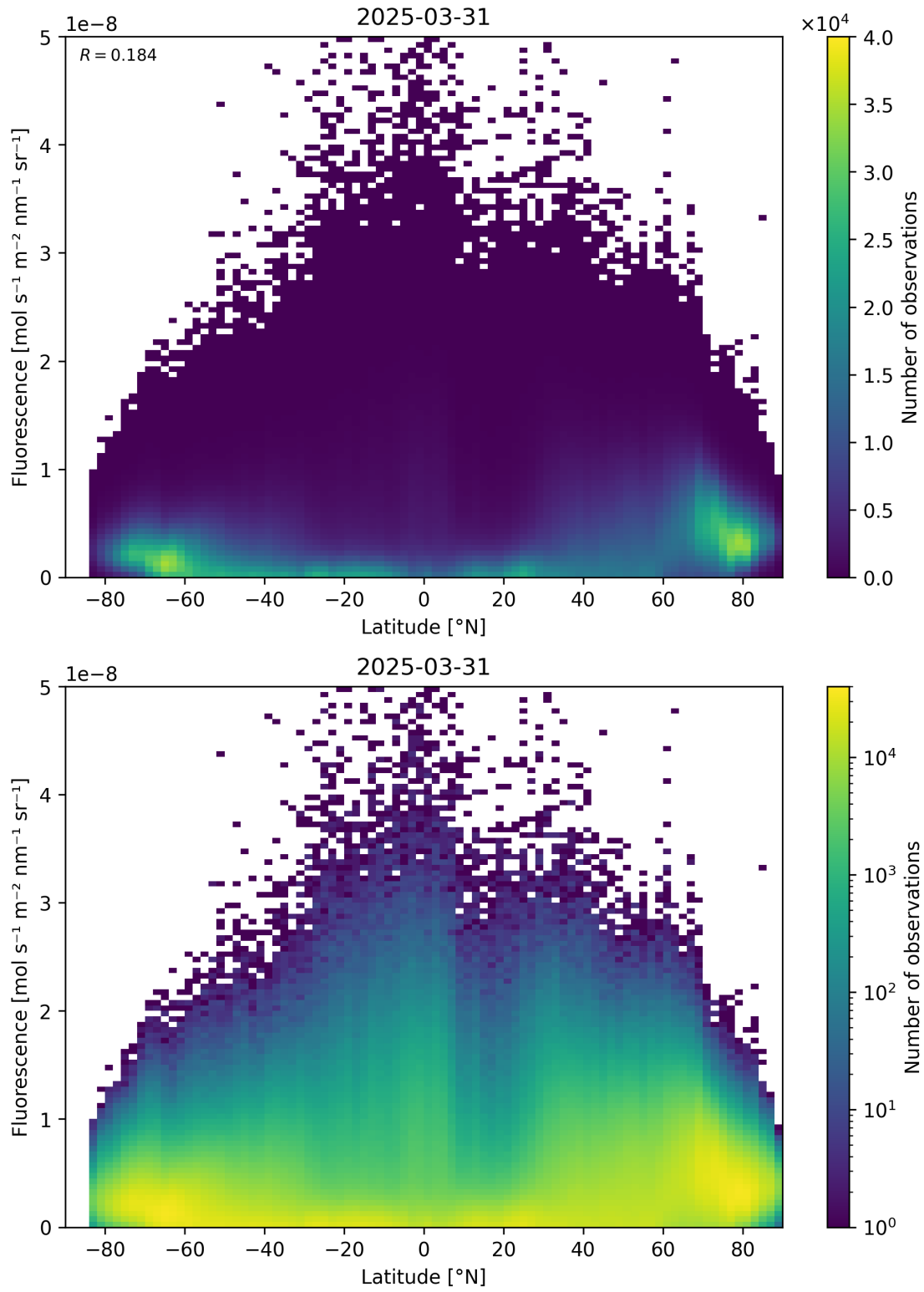
Figure 92: Scatter density plot of “Latitude” against “Fluorescence” for 2025-03-30 to 2025-04-01.
