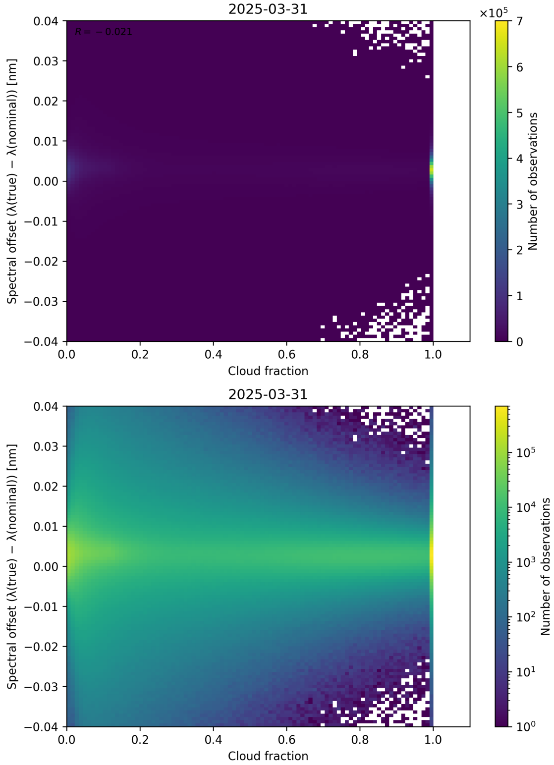
Figure 76: Scatter density plot of “Cloud fraction” against “Spectral offset ( \lambda_{\text{true}} - \lambda_{\text{nominal}} )” for 2025-03-30 to 2025-04-01.
