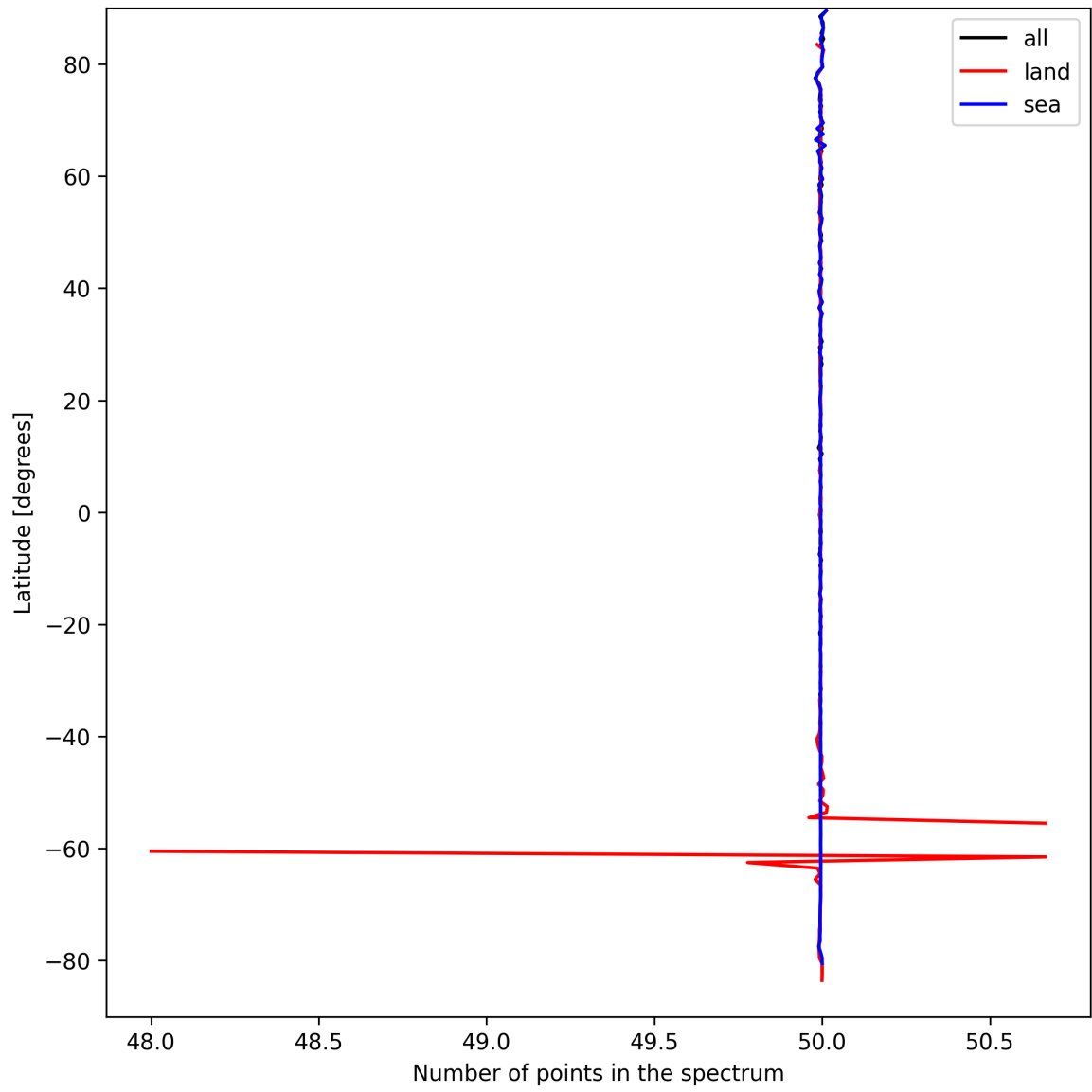
Figure 27: Zonal average of “Number of points in the spectrum” for 2025-03-30 to 2025-04-01.
