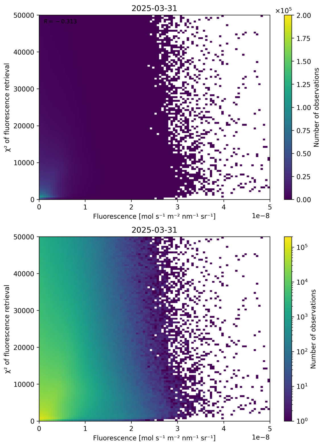
Figure 85: Scatter density plot of “Fluorescence” against “ \chi^2 of fluorescence retrieval” for 2025-03-30 to 2025-04-01.
