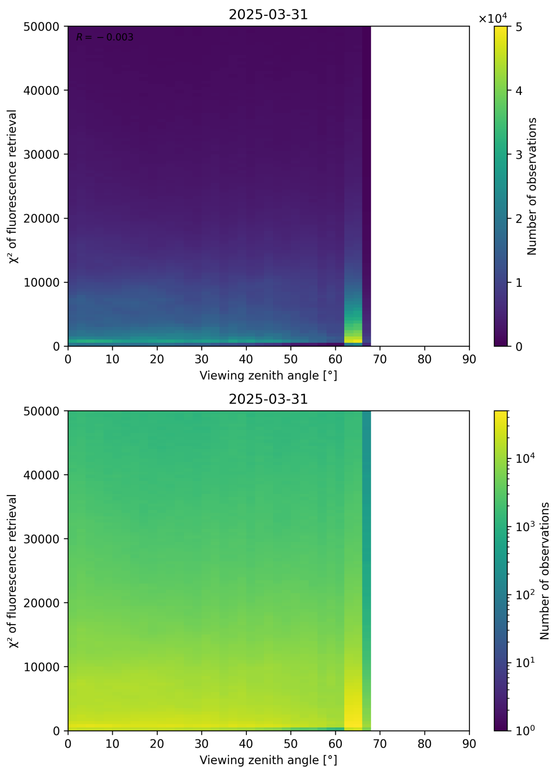
Figure 119: Scatter density plot of “Viewing zenith angle” against “ \chi^2 of fluorescence retrieval” for 2025-03-30 to 2025-04-01.
