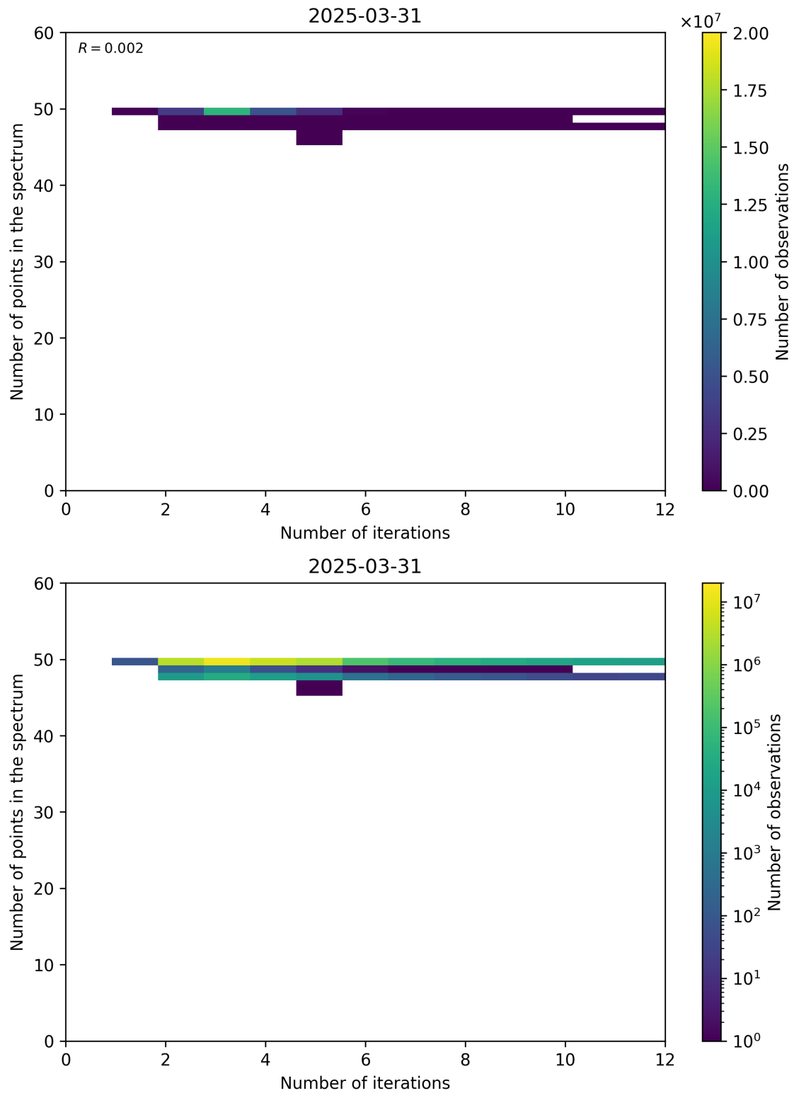
Figure 99: Scatter density plot of “Number of iterations” against “Number of points in the spectrum” for 2025-03-30 to 2025-04-01.
