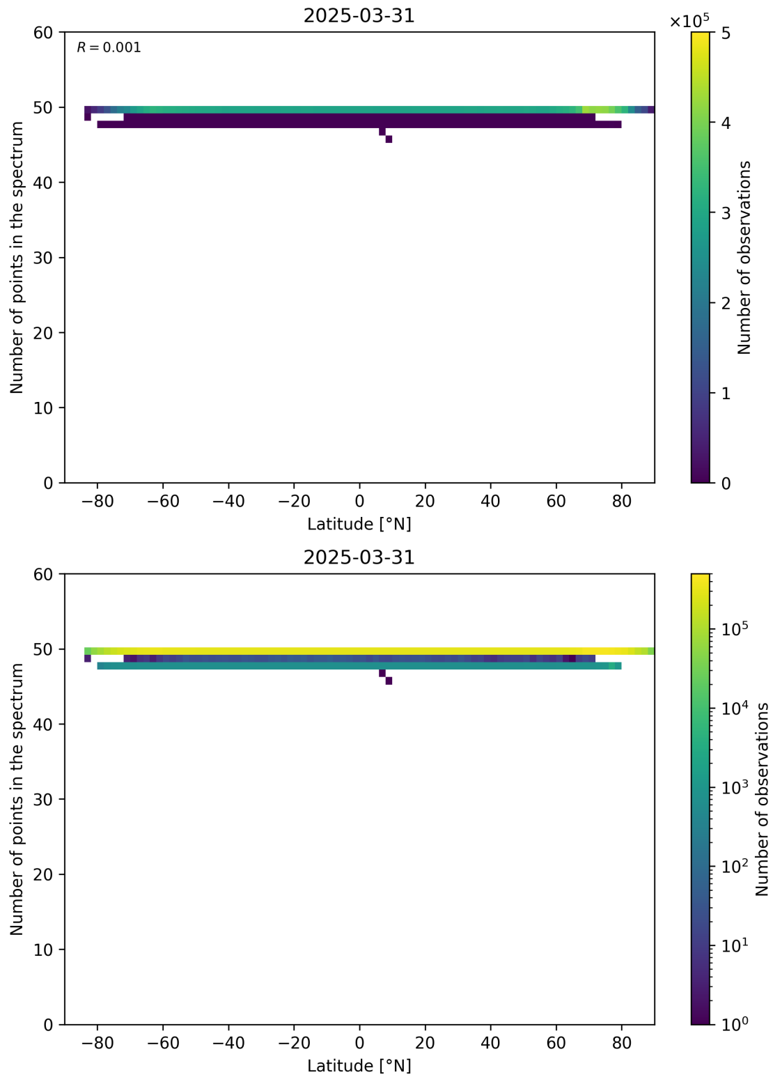
Figure 94: Scatter density plot of “Latitude” against “Number of points in the spectrum” for 2025-03-30 to 2025-04-01.
