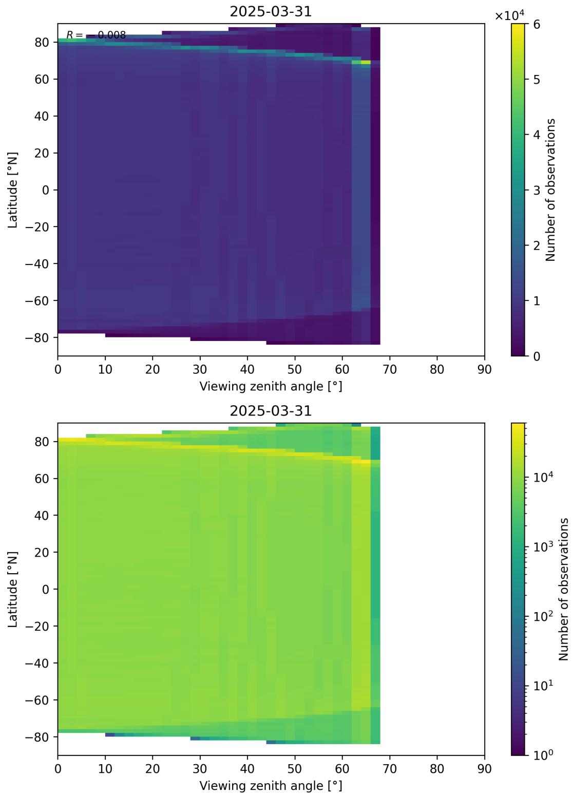
Figure 123: Scatter density plot of “Viewing zenith angle” against “Latitude” for 2025-03-30 to 2025-04-01.
