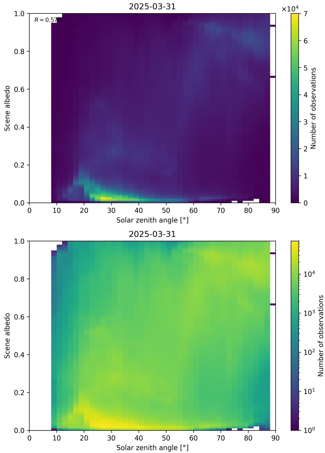
Figure 116: Scatter density plot of “Solar zenith angle” against “Scene albedo” for 2025-03-30 to 2025-04-01.
