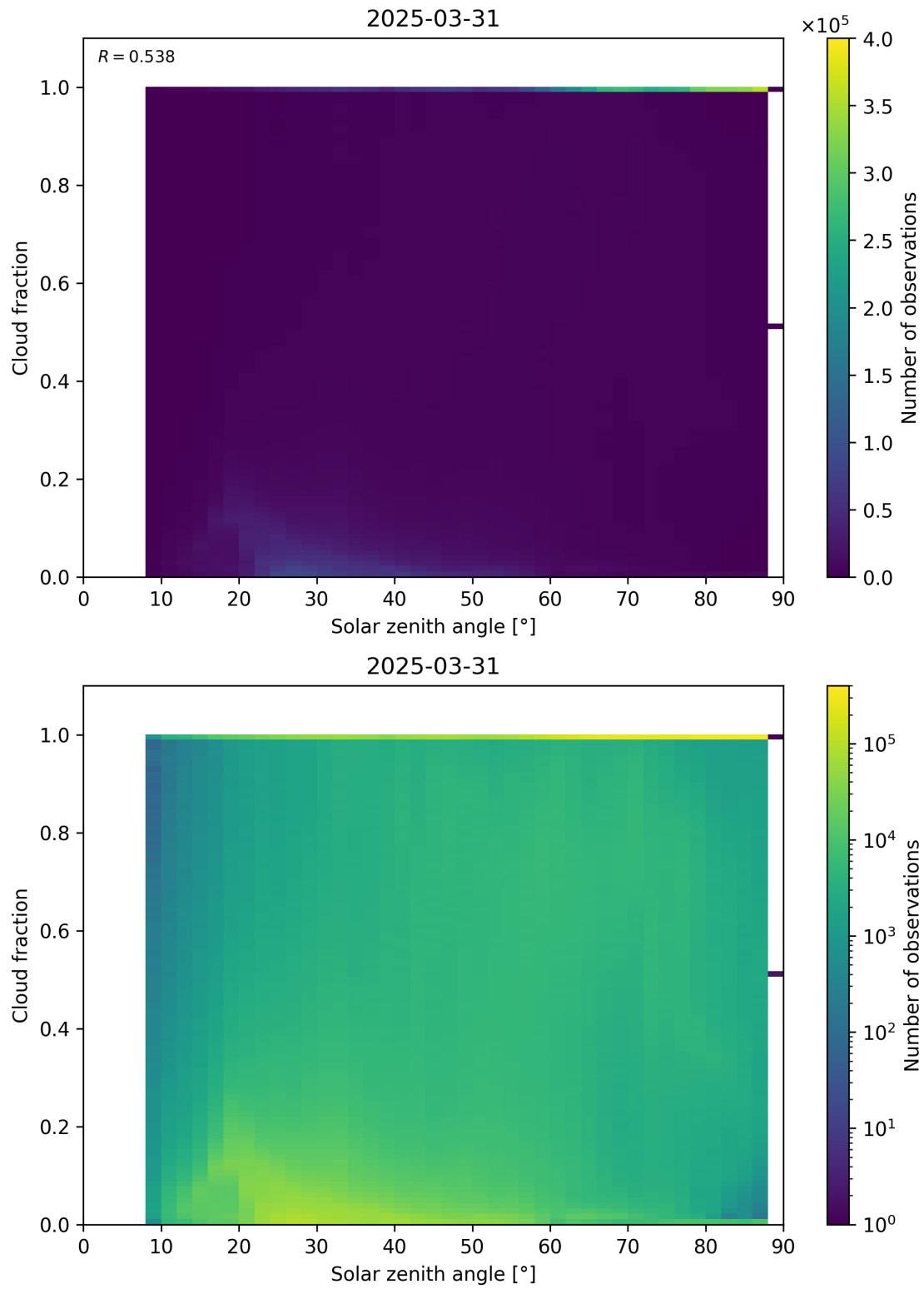
Figure 110: Scatter density plot of “Solar zenith angle” against “Cloud fraction” for 2025-03-30 to 2025-04-01.
