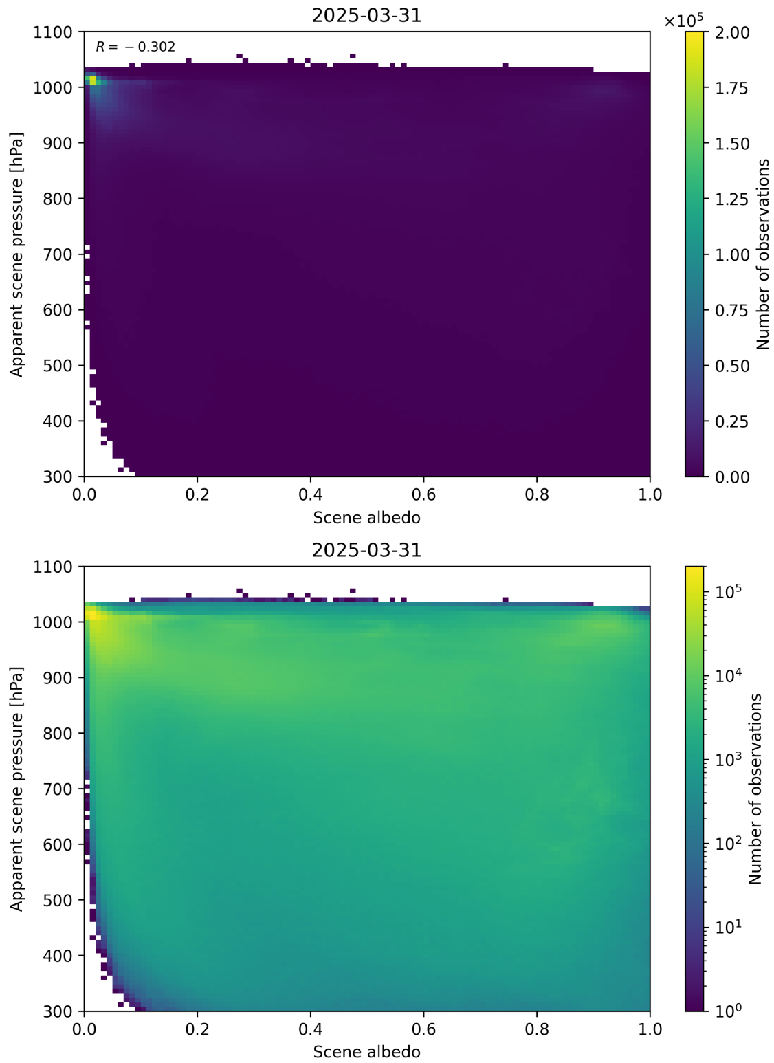
Figure 102: Scatter density plot of “Scene albedo” against “Apparent scene pressure” for 2025-03-30 to 2025-04-01.
