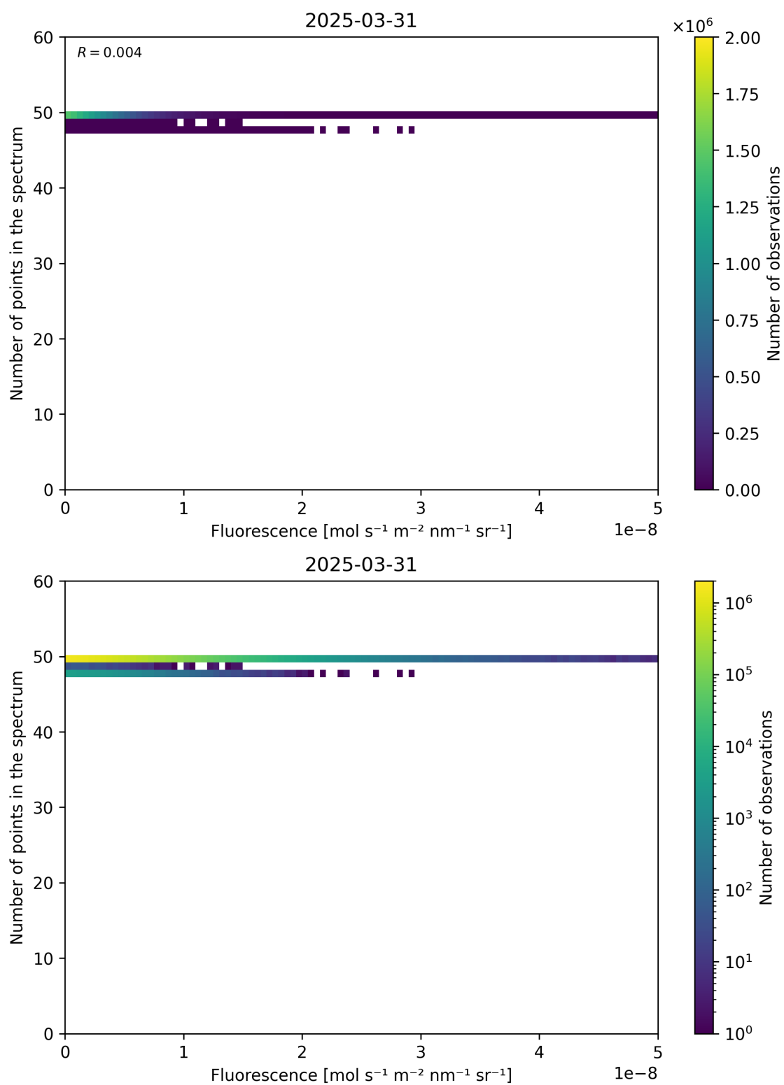
Figure 86: Scatter density plot of “Fluorescence” against “Number of points in the spectrum” for 2025-03-30 to 2025-04-01.
