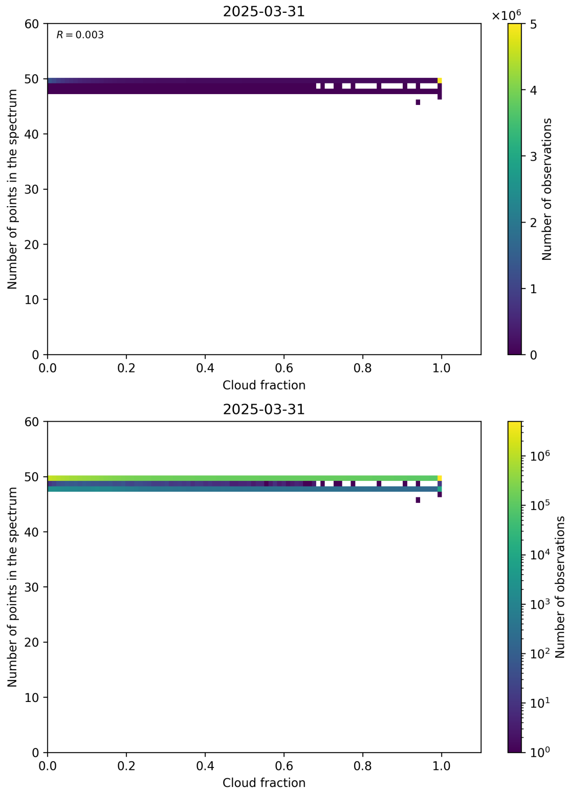
Figure 74: Scatter density plot of “Cloud fraction” against “Number of points in the spectrum” for 2025-03-30 to 2025-04-01.
