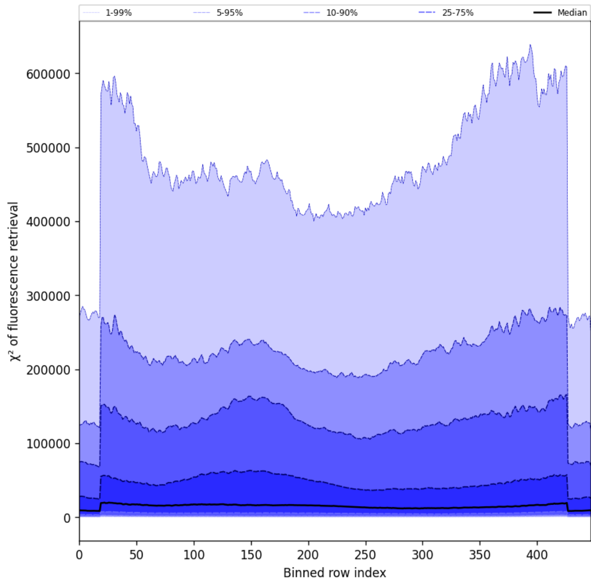
Figure 59: Along track statistics of “ \chi^2 of fluorescence retrieval” for 2025-03-30 to 2025-04-01
