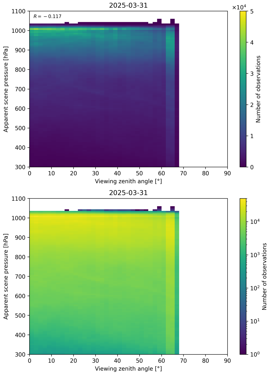
Figure 118: Scatter density plot of “Viewing zenith angle” against “Apparent scene pressure” for 2025-03-30 to 2025-04-01.
