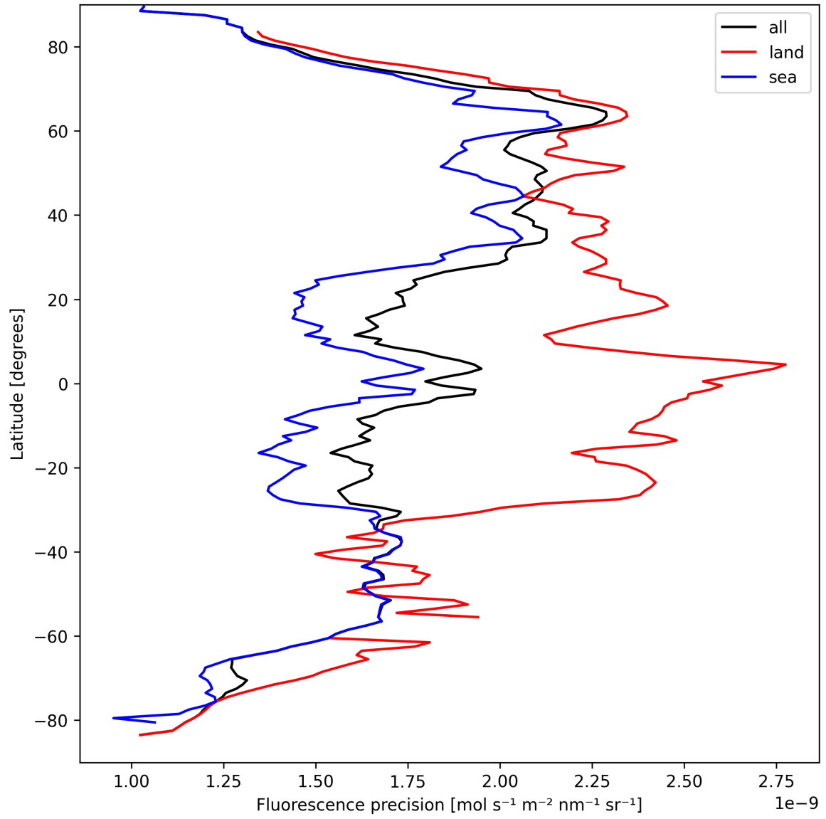
Figure 24: Zonal average of “Fluorescence precision” for 2025-03-30 to 2025-04-01.
