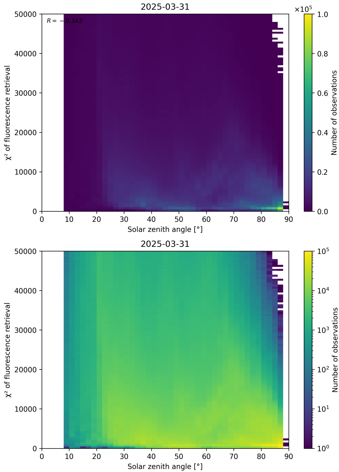
Figure 109: Scatter density plot of “Solar zenith angle” against “ \chi^2 of fluorescence retrieval” for 2025-03-30 to 2025-04-01.
