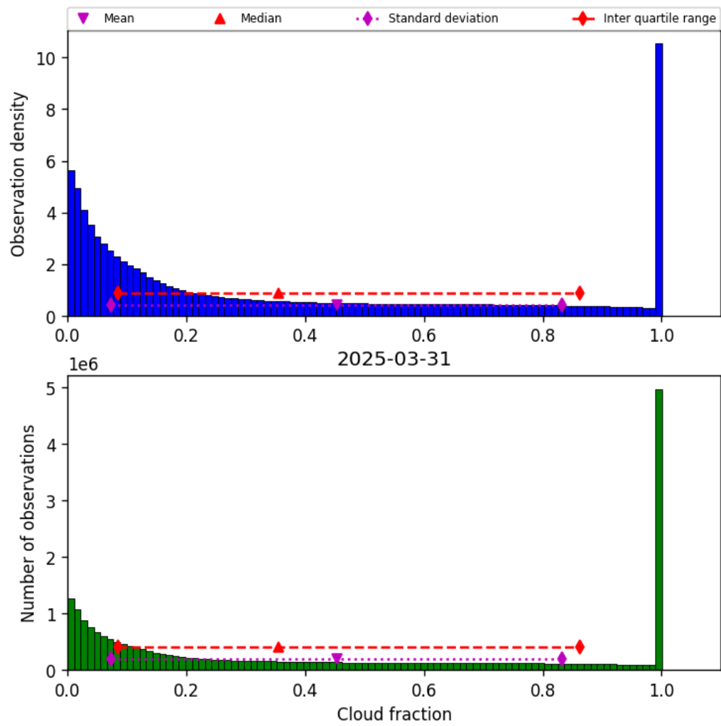
Figure 32: Histogram of “Cloud fraction” for 2025-03-30 to 2025-04-01
