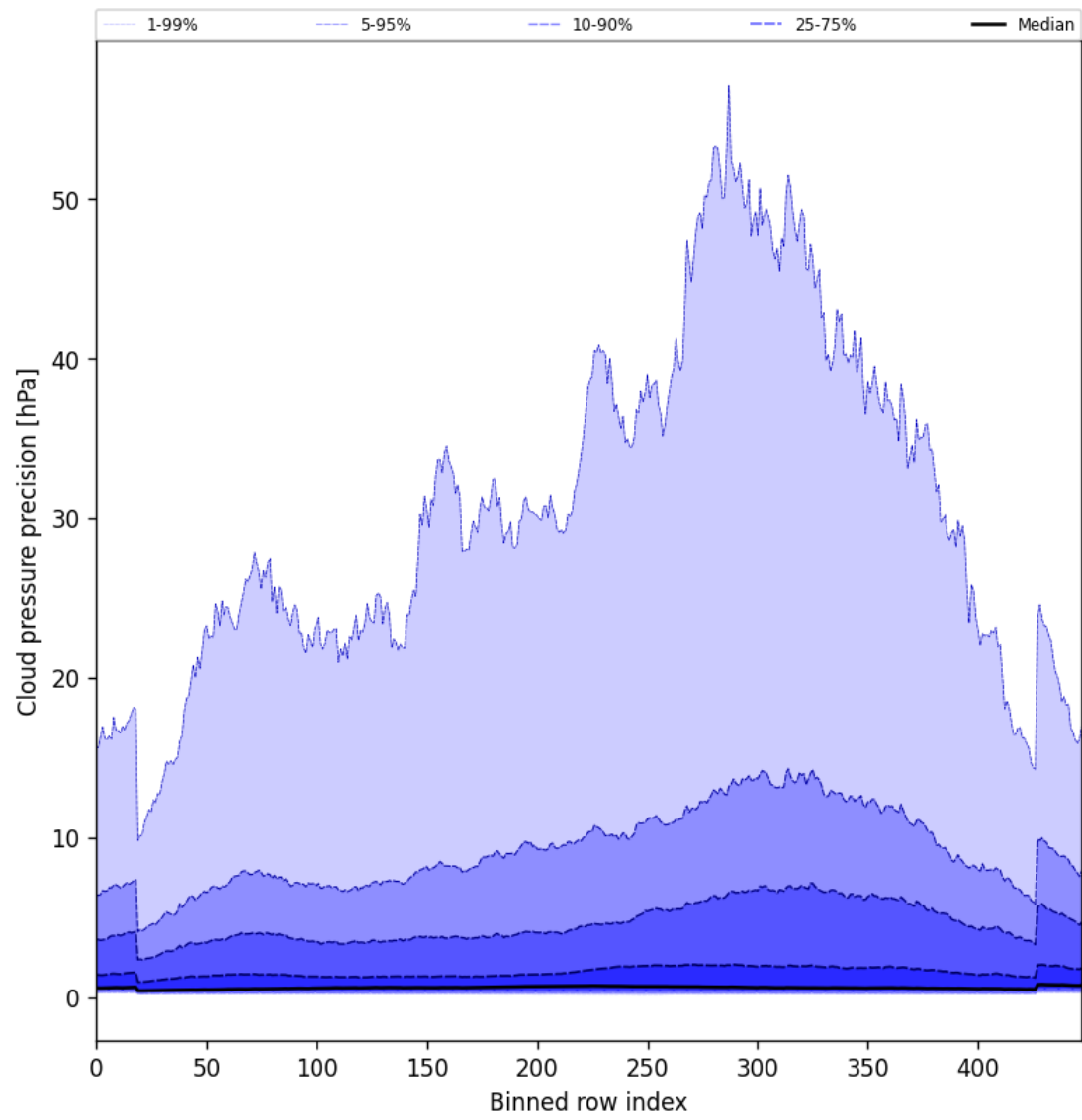
Figure 48: Along track statistics of “Cloud pressure precision” for 2025-03-30 to 2025-04-01
