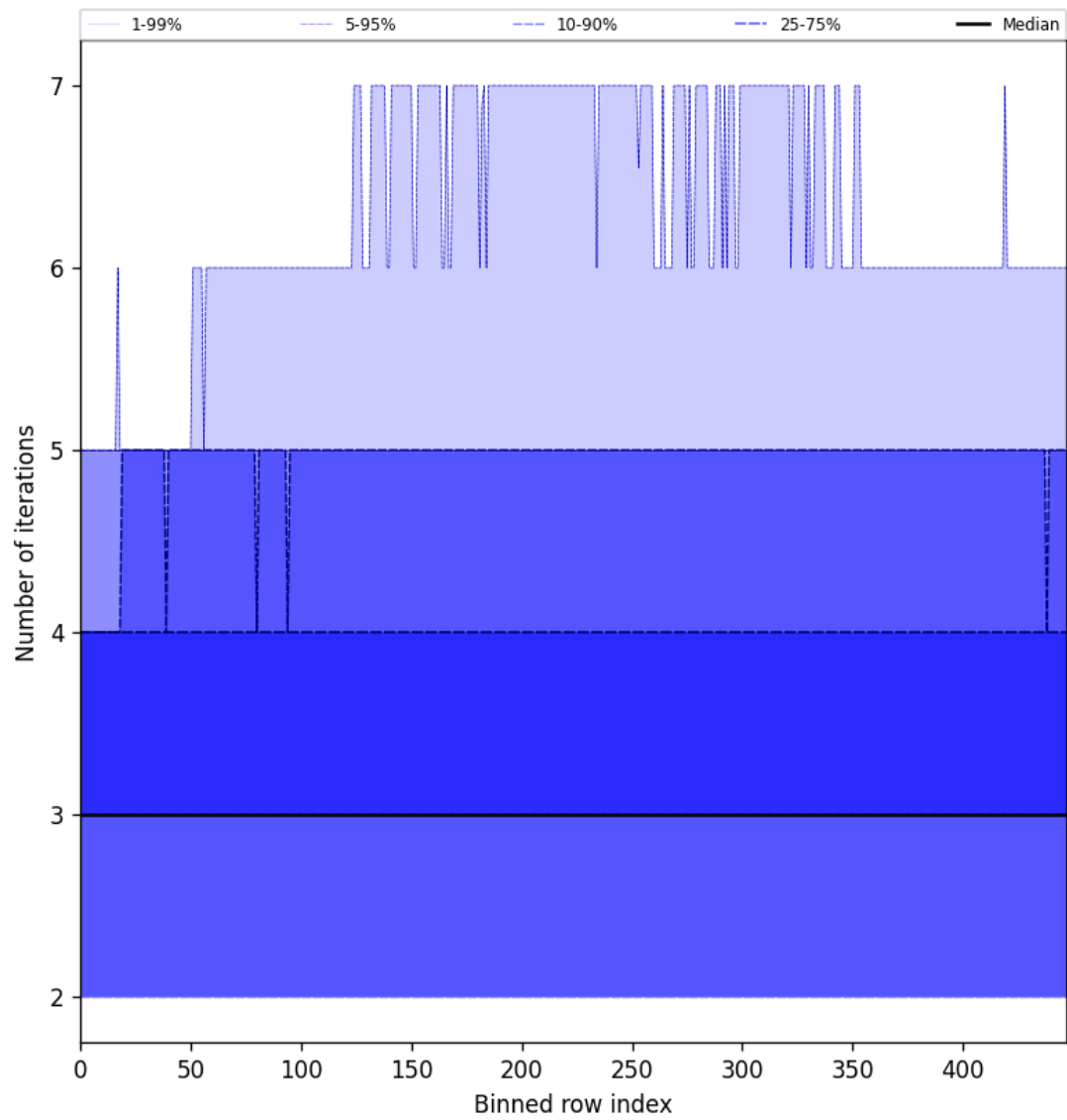
Figure 56: Along track statistics of “Number of iterations” for 2025-03-30 to 2025-04-01
