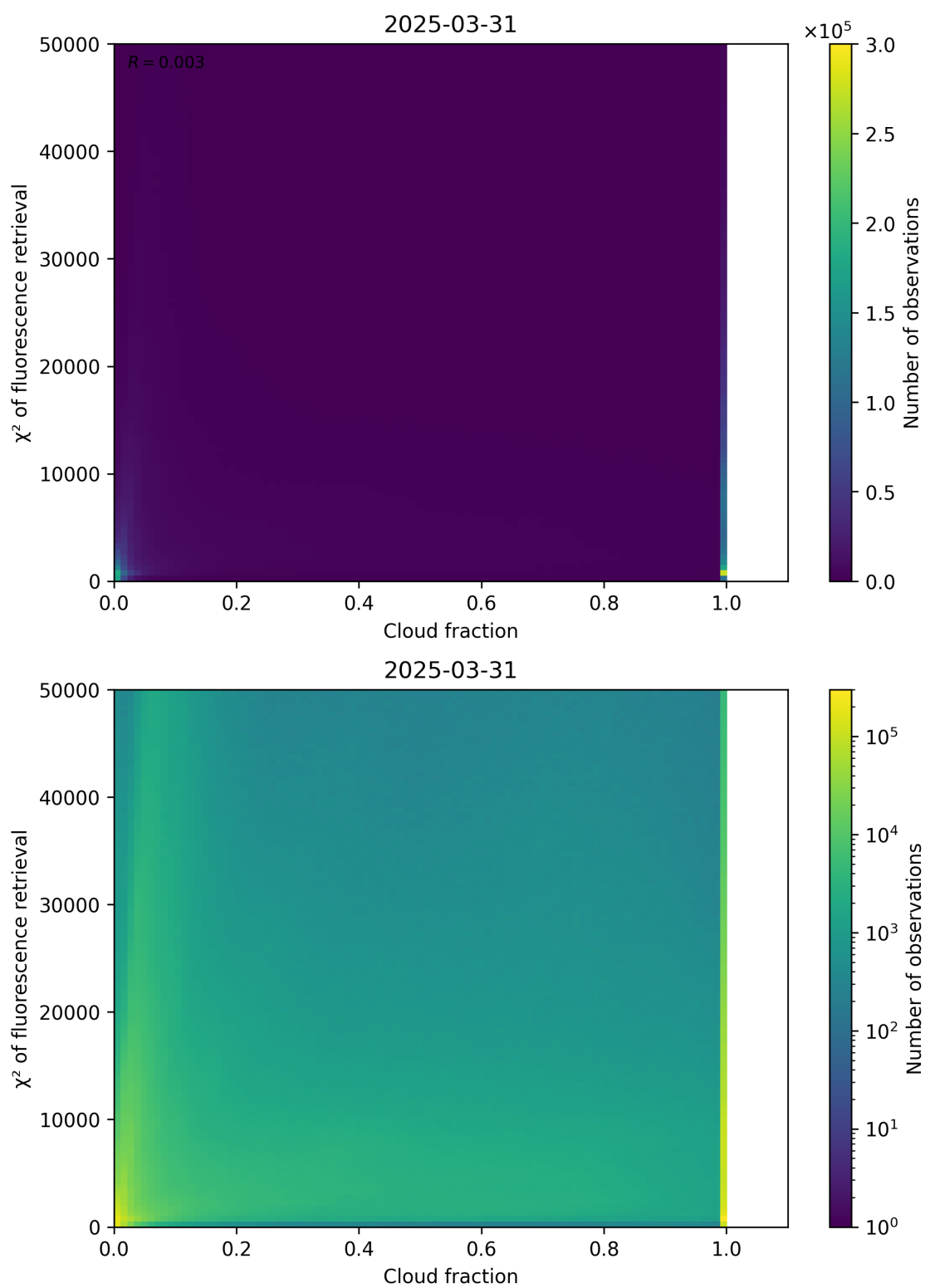
Figure 71: Scatter density plot of “Cloud fraction” against “ \chi^2 of fluorescence retrieval” for 2025-03-30 to 2025-04-01.
