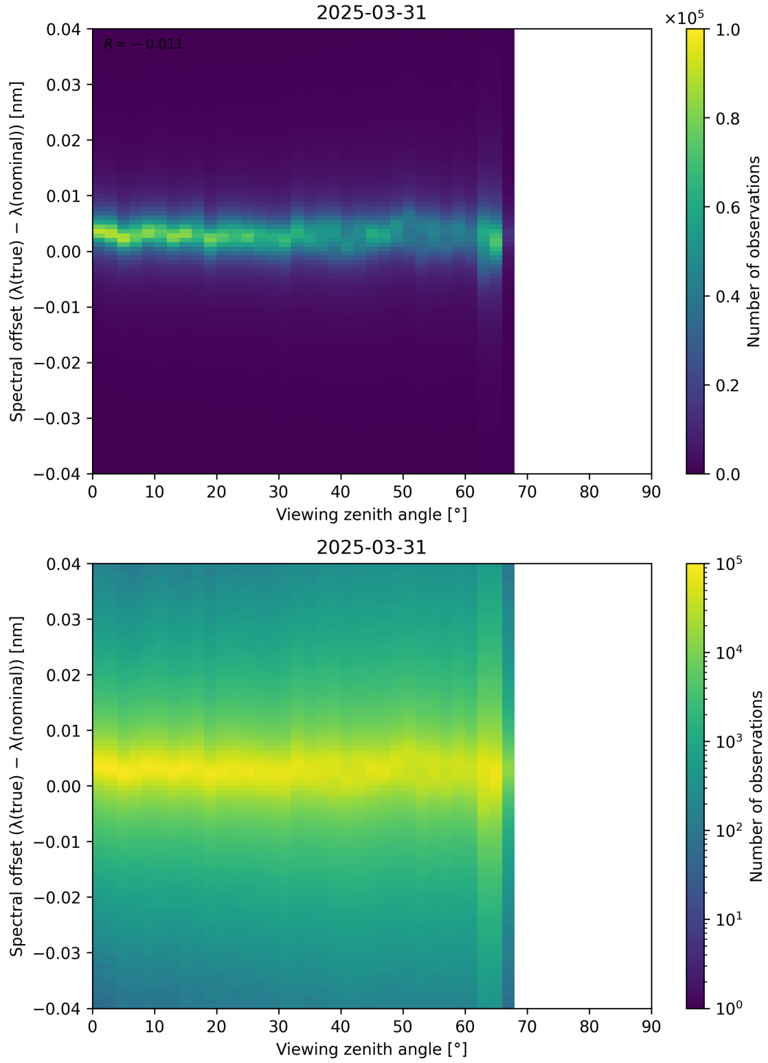
Figure 128: Scatter density plot of “Viewing zenith angle” against “Spectral offset ( \lambda_{\text{true}} - \lambda_{\text{nominal}} )” for 2025-03-30 to 2025-04-01.
