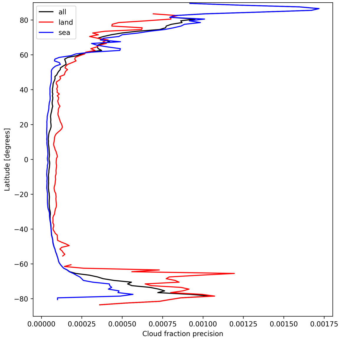
Figure 16: Zonal average of “Cloud fraction precision” for 2025-03-30 to 2025-04-01.
