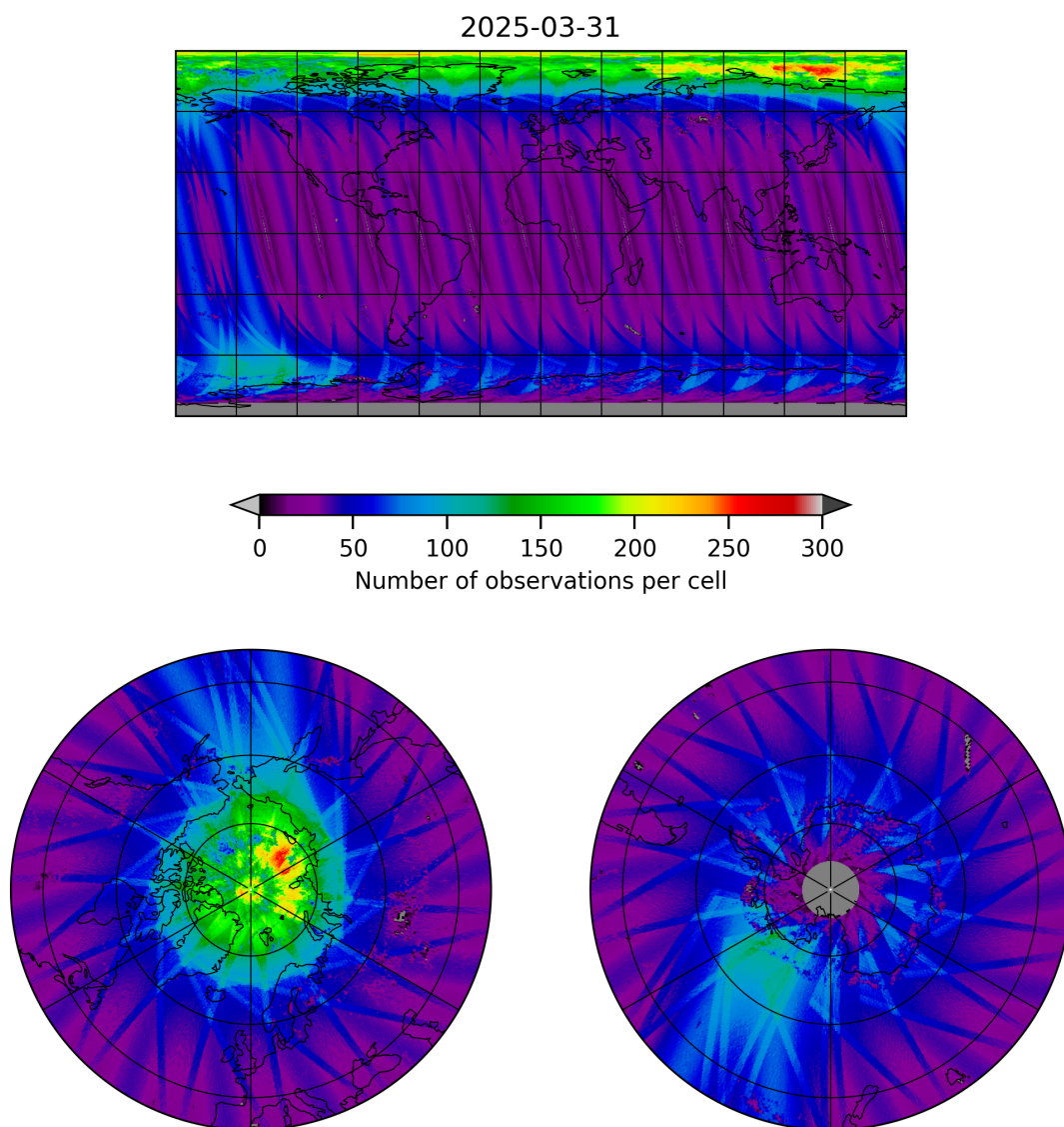
Figure 11: Map of the number of observations for 2025-03-30 to 2025-04-01
