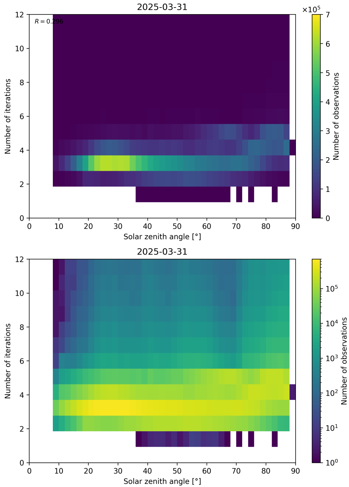
Figure 114: Scatter density plot of “Solar zenith angle” against “Number of iterations” for 2025-03-30 to 2025-04-01.
