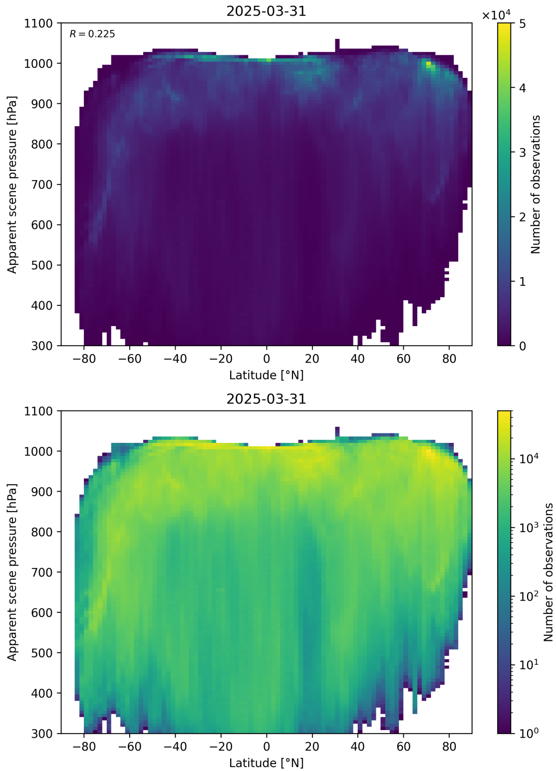
Figure 88: Scatter density plot of “Latitude” against “Apparent scene pressure” for 2025-03-30 to 2025-04-01.
