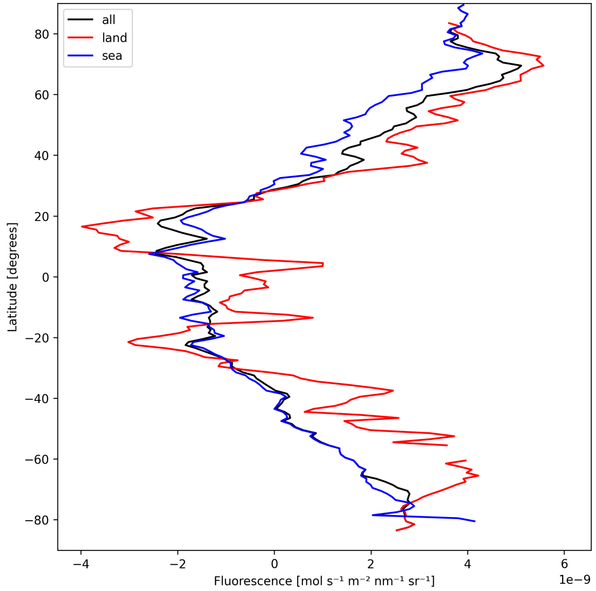
Figure 23: Zonal average of “Fluorescence” for 2025-03-30 to 2025-04-01.
