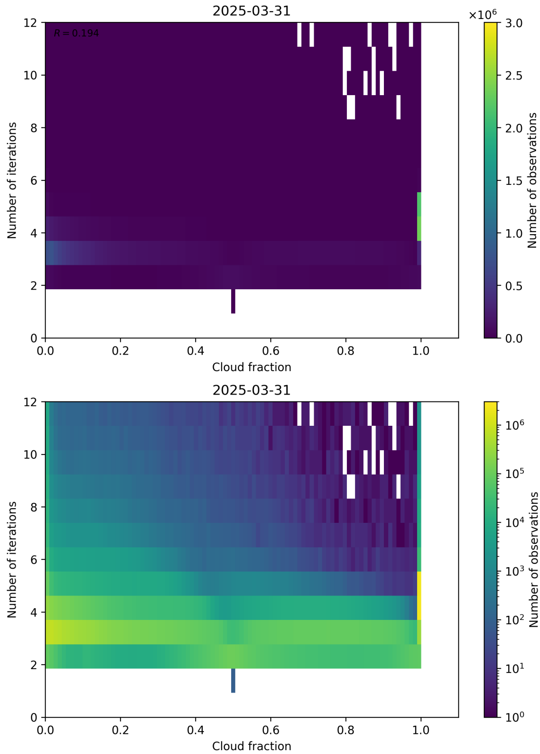
Figure 73: Scatter density plot of “Cloud fraction” against “Number of iterations” for 2025-03-30 to 2025-04-01.
