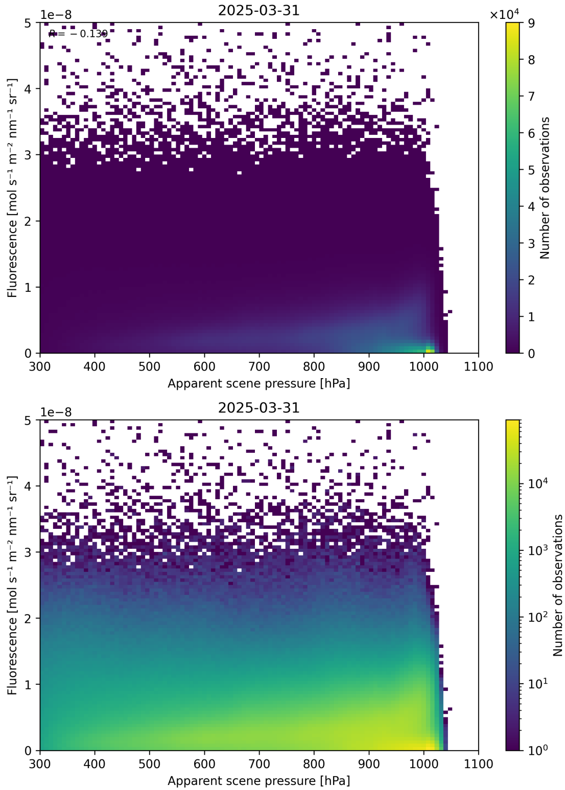
Figure 64: Scatter density plot of “Apparent scene pressure” against “Fluorescence” for 2025-03-30 to 2025-04-01.
