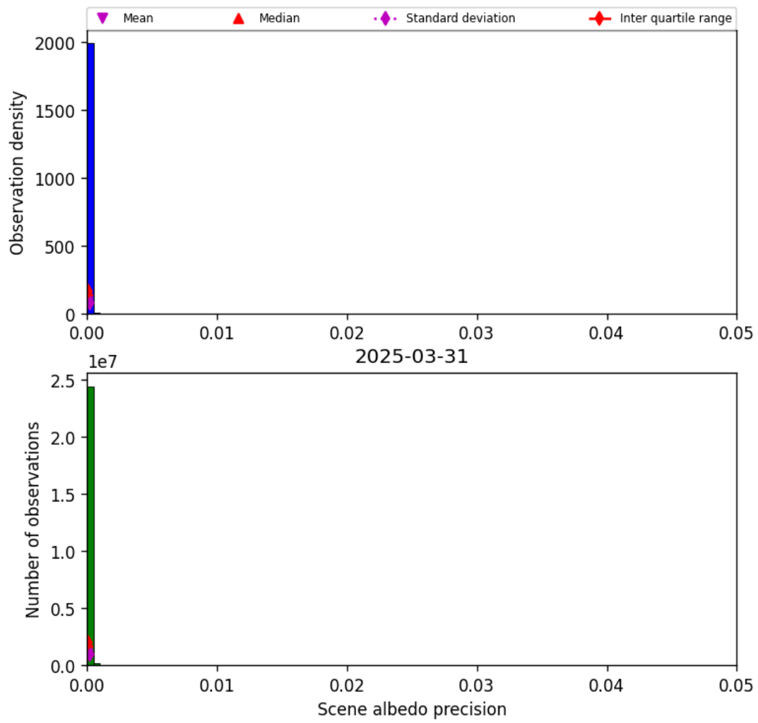
Figure 35: Histogram of “Scene albedo precision” for 2025-03-30 to 2025-04-01
