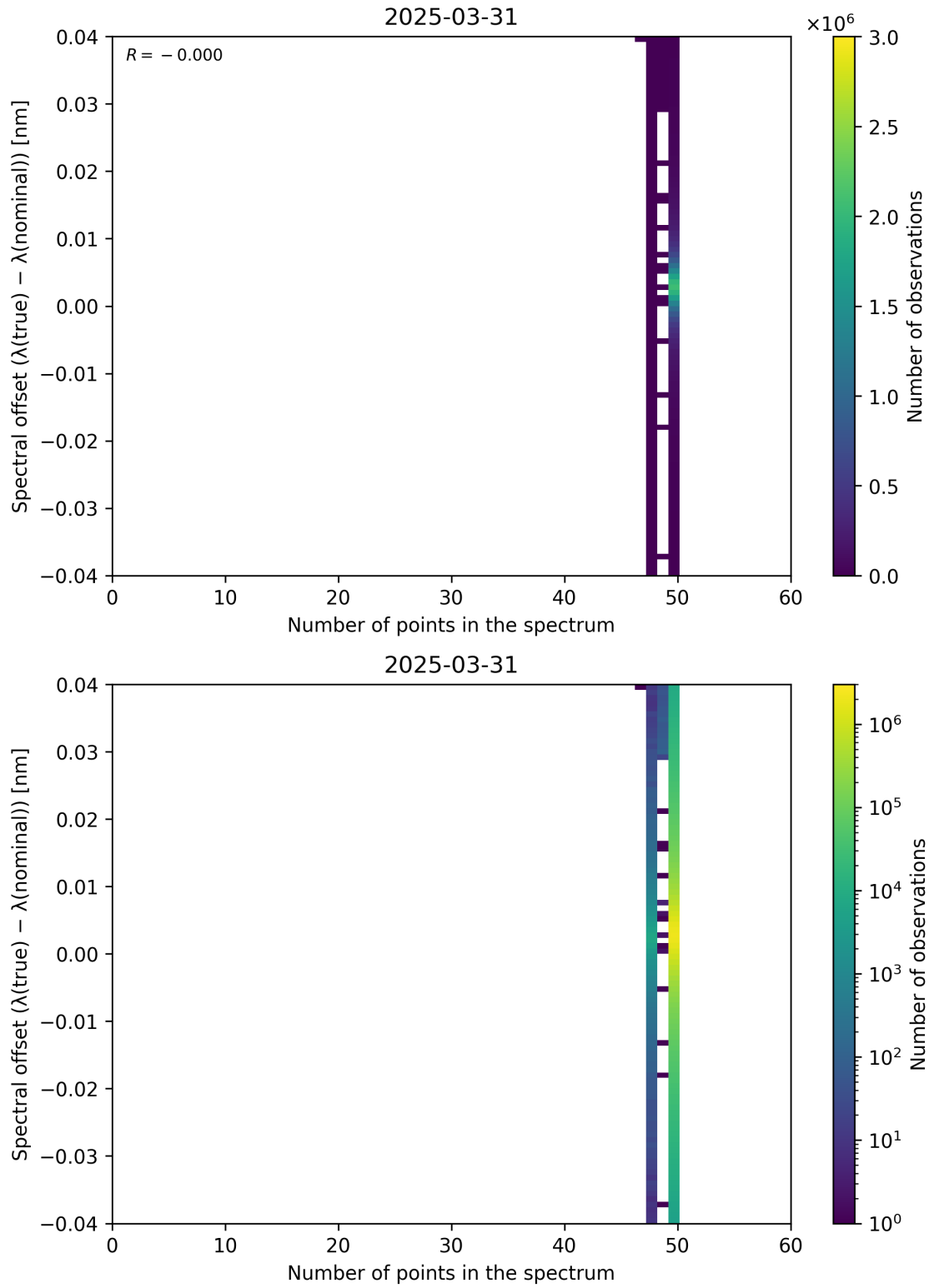
Figure 101: Scatter density plot of “Number of points in the spectrum” against “Spectral offset ( \lambda_{\text{true}} - \lambda_{\text{nominal}} )” for 2025-03-30 to 2025-04-01.
