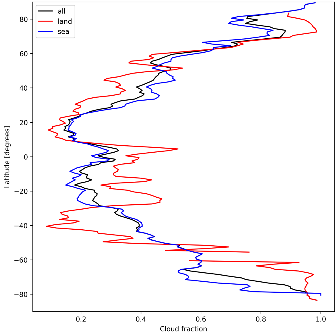
Figure 15: Zonal average of “Cloud fraction” for 2025-03-30 to 2025-04-01.
