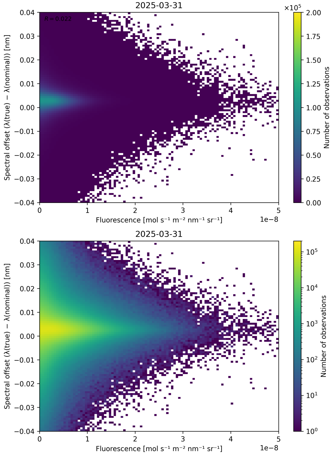
Figure 87: Scatter density plot of “Fluorescence” against “Spectral offset ( \lambda_{\text{true}} - \lambda_{\text{nominal}} )” for 2025-03-30 to 2025-04-01.
