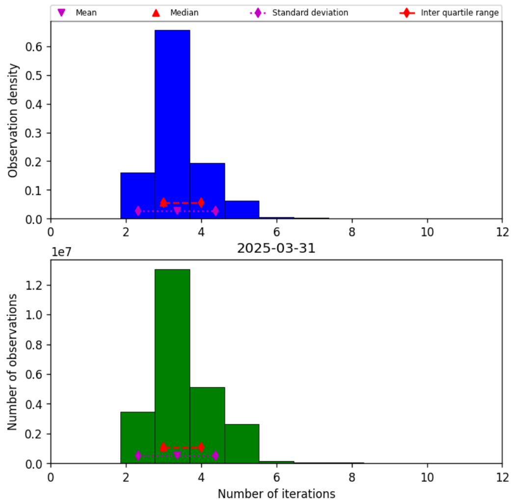
Figure 39: Histogram of “Number of iterations” for 2025-03-30 to 2025-04-01
