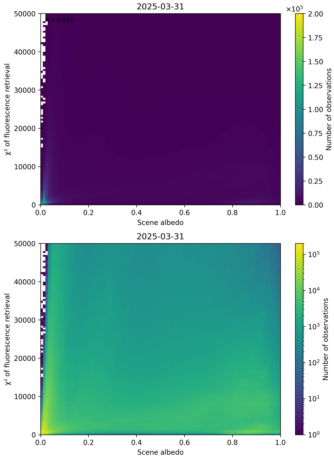
Figure 103: Scatter density plot of “Scene albedo” against “ \chi^2 of fluorescence retrieval” for 2025-03-30 to 2025-04-01.
