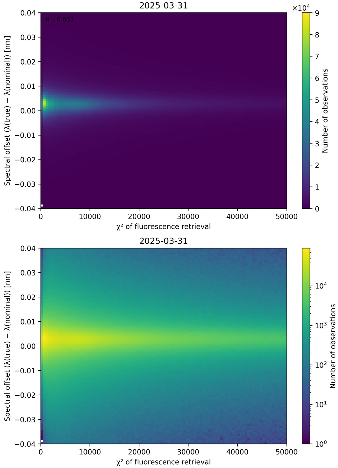
Figure 69: Scatter density plot of “ \chi^2 of fluorescence retrieval” against “Spectral offset ( \lambda_{\text{true}} - \lambda_{\text{nominal}} )” for 2025-03-30 to 2025-04-01.
