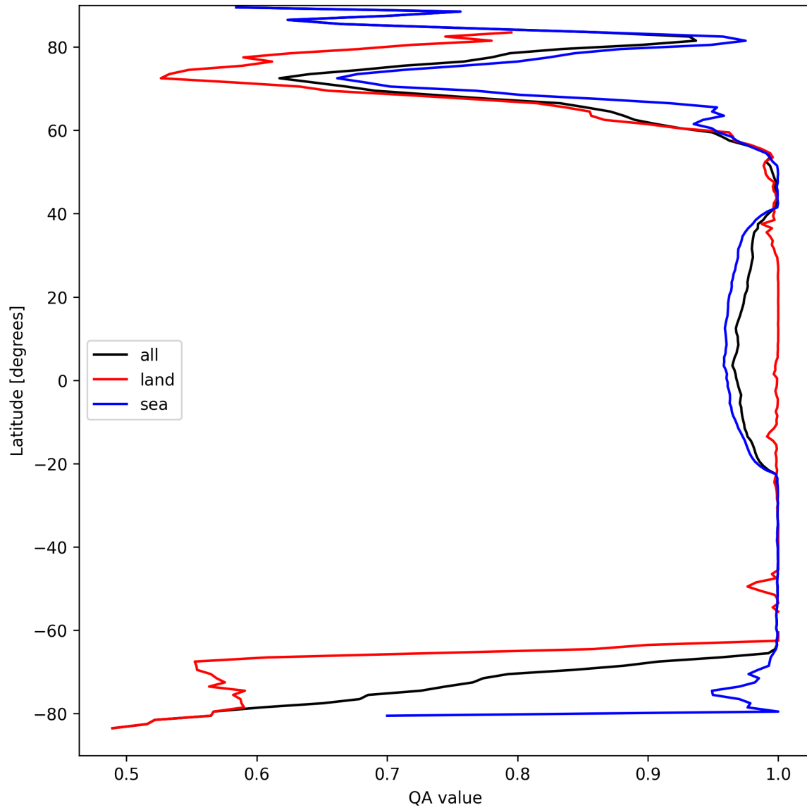
Figure 12: Zonal average of “QA value” for 2025-03-30 to 2025-04-01.
