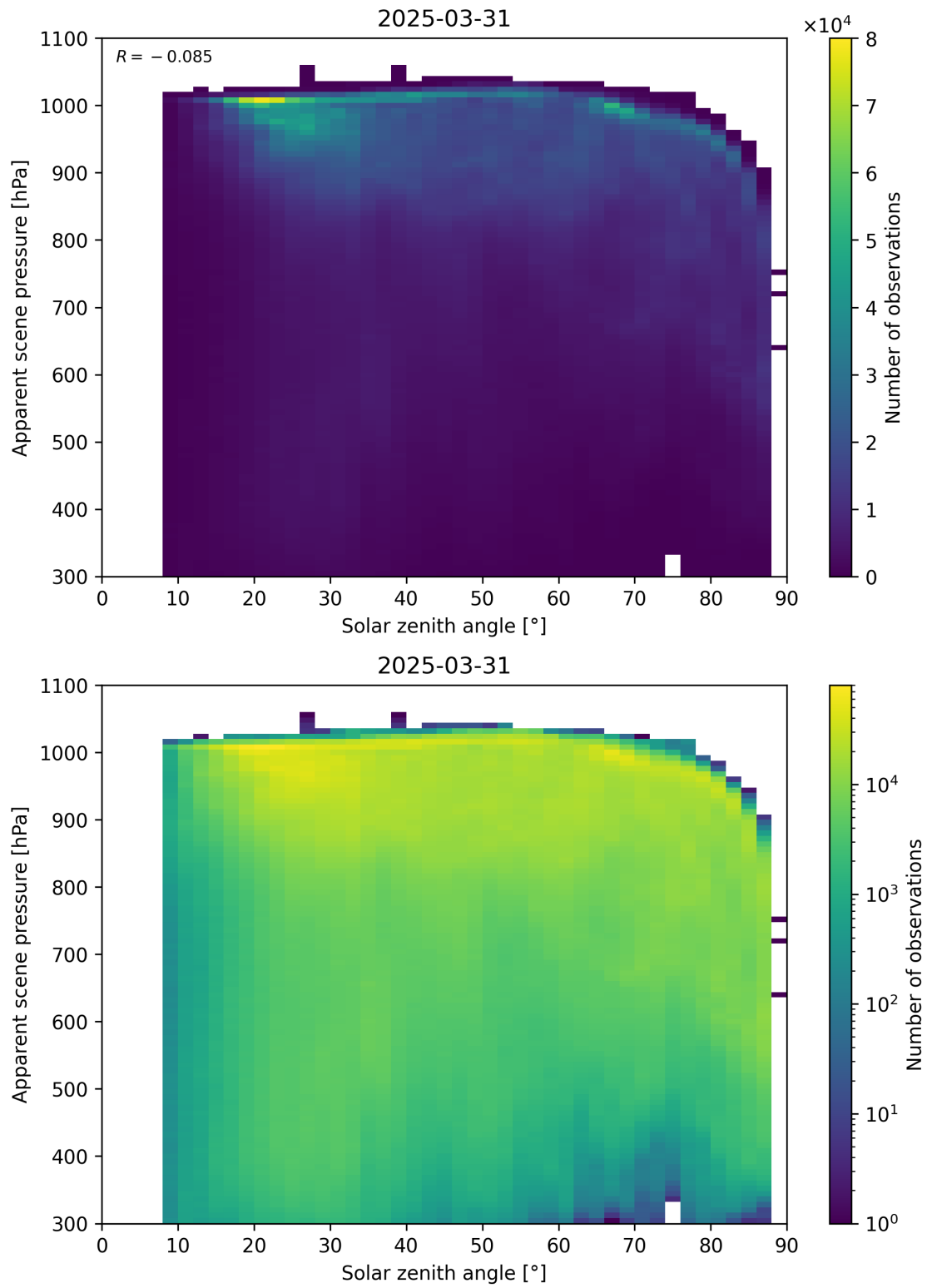
Figure 108: Scatter density plot of “Solar zenith angle” against “Apparent scene pressure” for 2025-03-30 to 2025-04-01.
