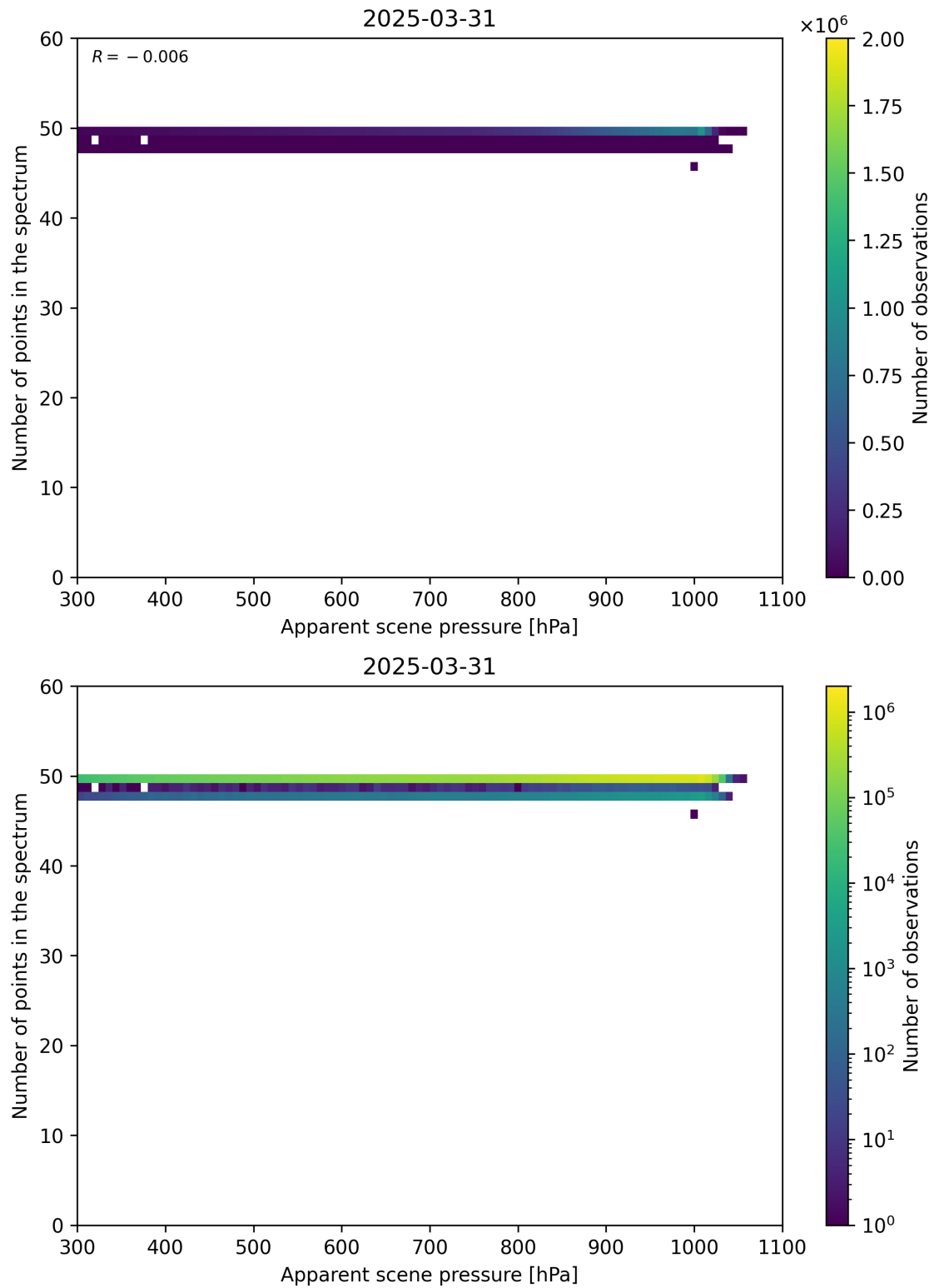
Figure 66: Scatter density plot of “Apparent scene pressure” against “Number of points in the spectrum” for 2025-03-30 to 2025-04-01.
