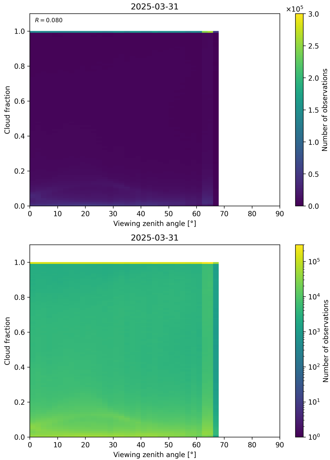
Figure 120: Scatter density plot of “Viewing zenith angle” against “Cloud fraction” for 2025-03-30 to 2025-04-01.
