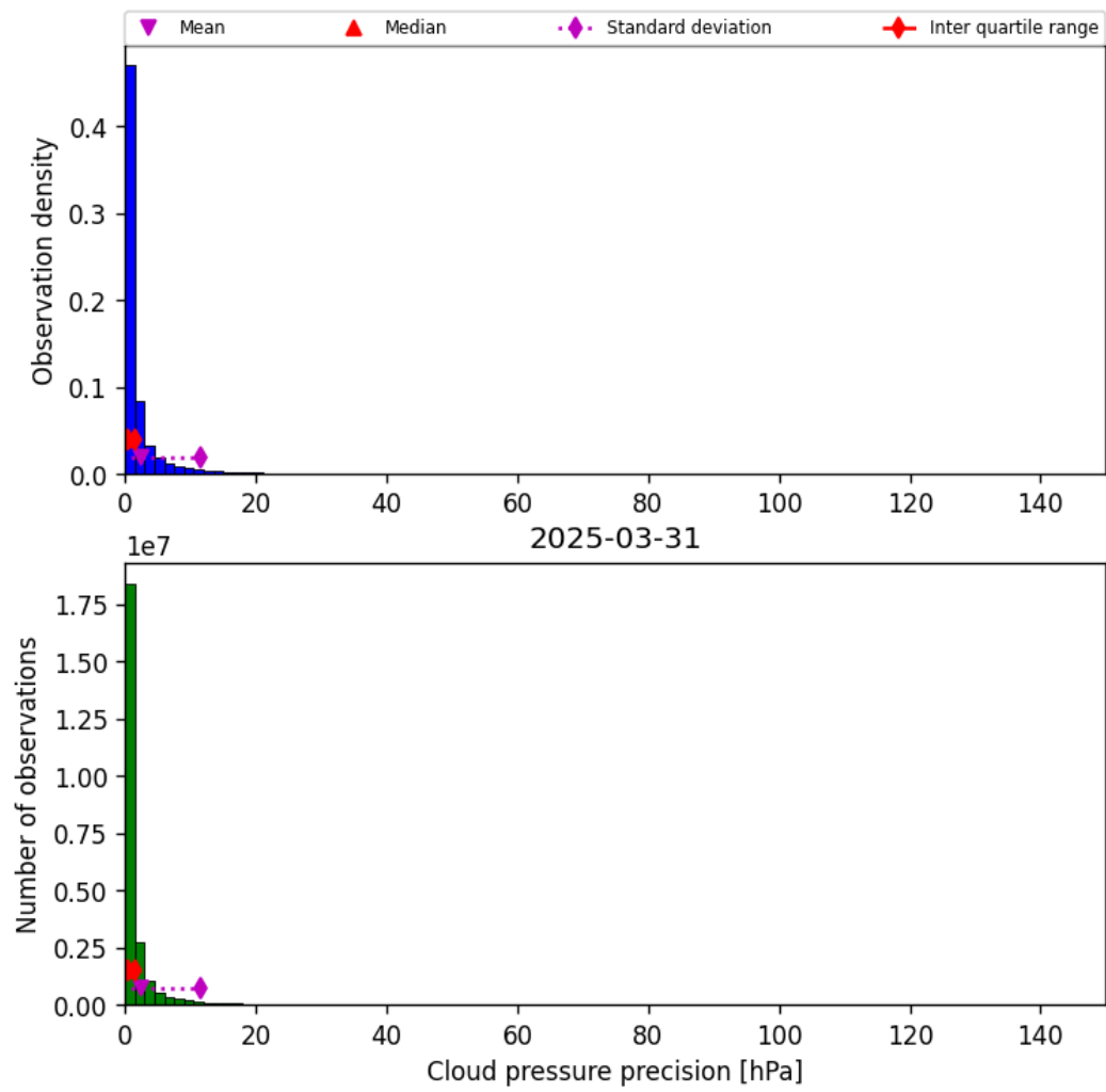
Figure 31: Histogram of “Cloud pressure precision” for 2025-03-30 to 2025-04-01
