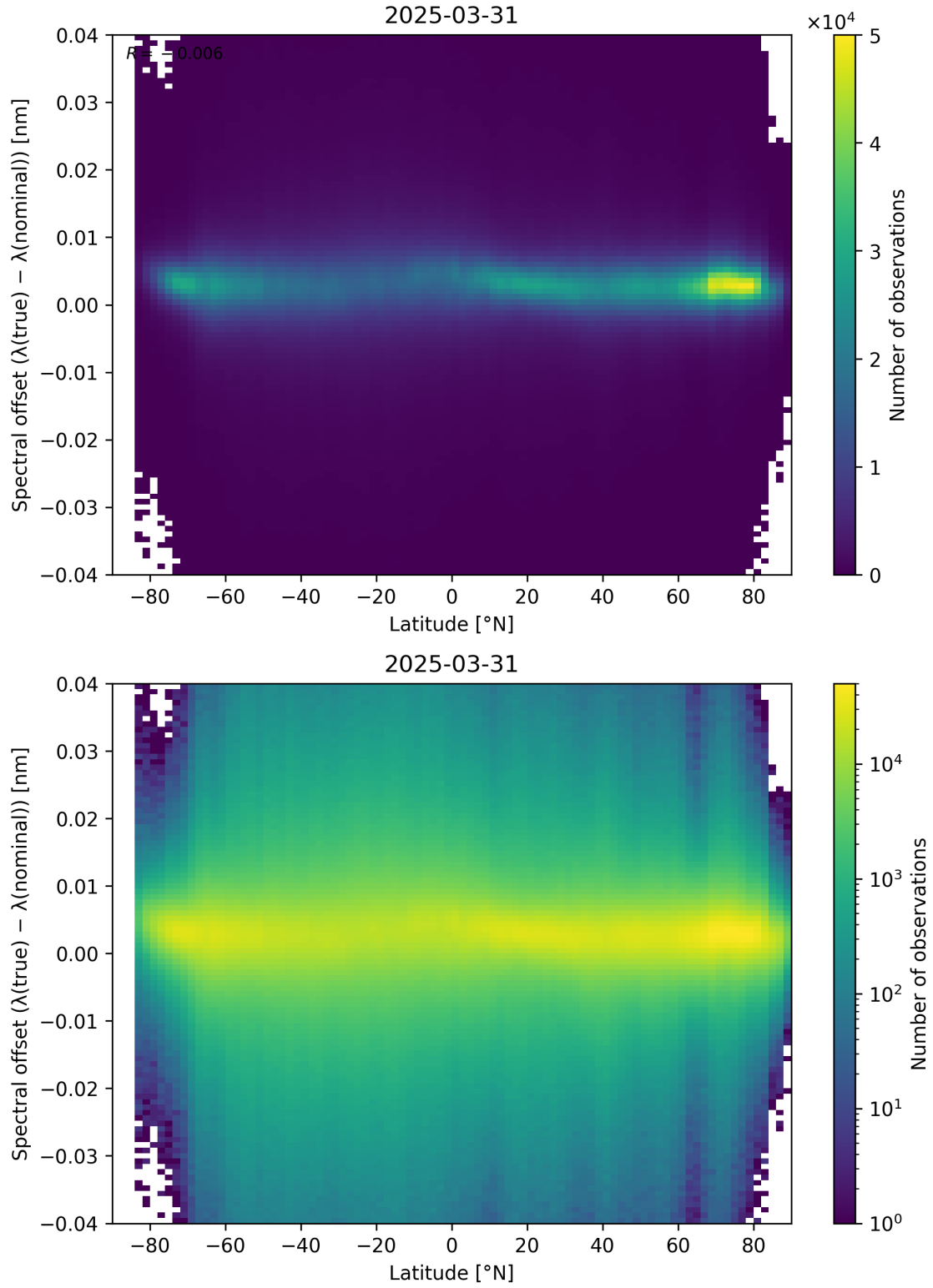
Figure 96: Scatter density plot of “Latitude” against “Spectral offset ( \lambda_{\text{true}} - \lambda_{\text{nominal}} )” for 2025-03-30 to 2025-04-01.
