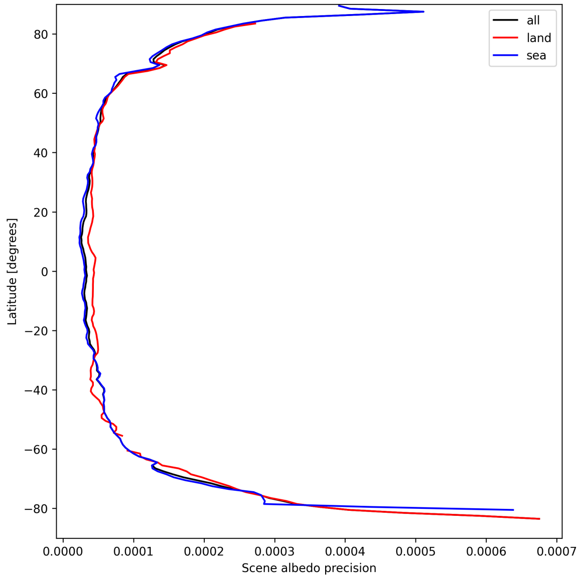
Figure 18: Zonal average of “Scene albedo precision” for 2025-03-30 to 2025-04-01.
