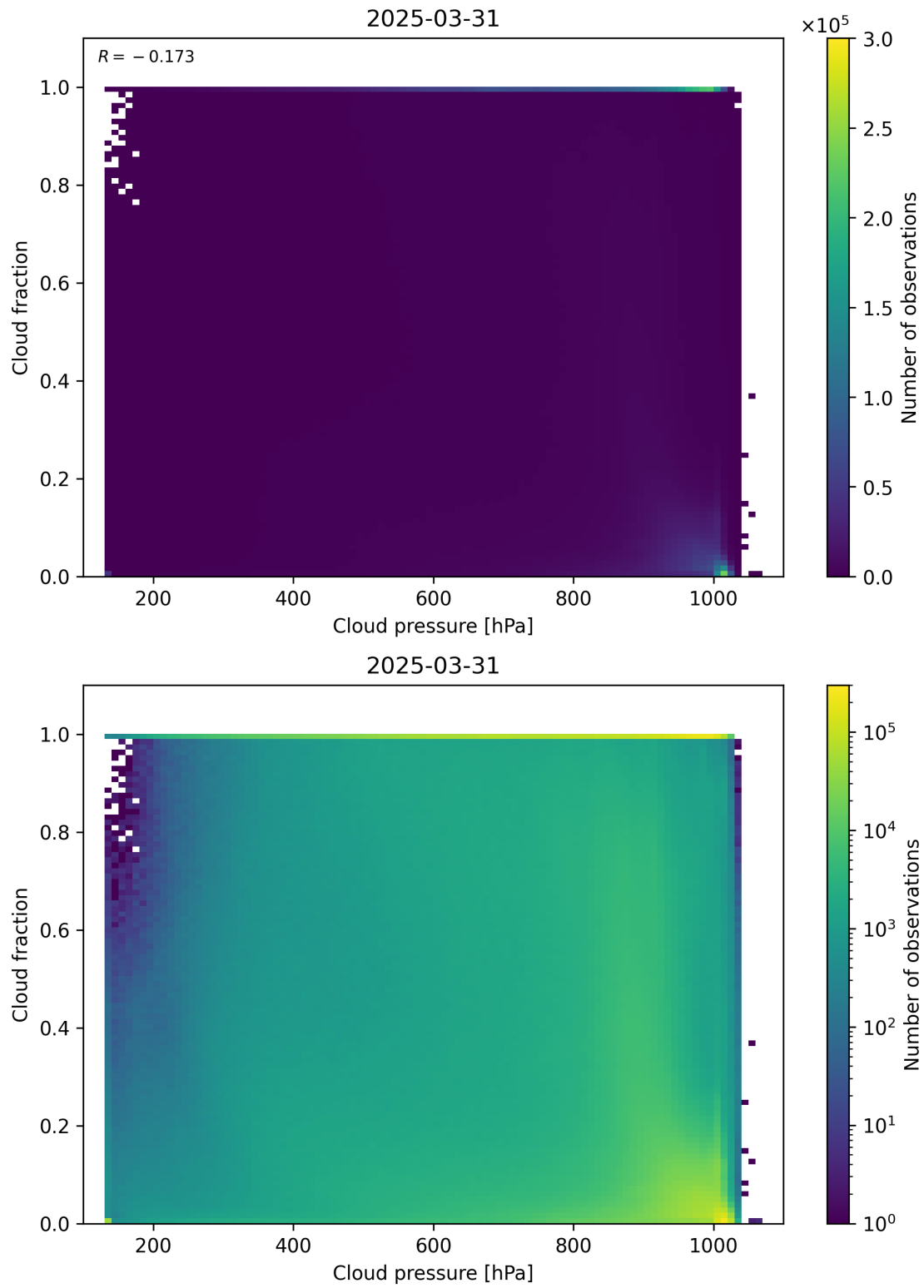
Figure 79: Scatter density plot of “Cloud pressure” against “Cloud fraction” for 2025-03-30 to 2025-04-01.
