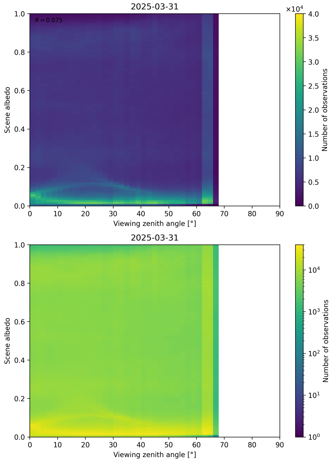
Figure 126: Scatter density plot of “Viewing zenith angle” against “Scene albedo” for 2025-03-30 to 2025-04-01.
