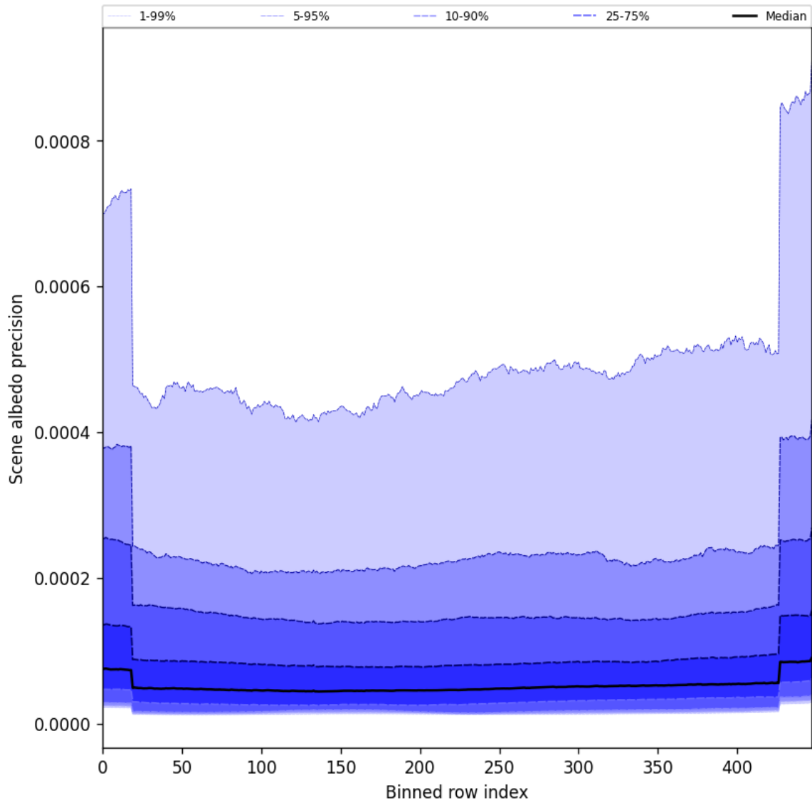
Figure 52: Along track statistics of “Scene albedo precision” for 2025-03-30 to 2025-04-01
