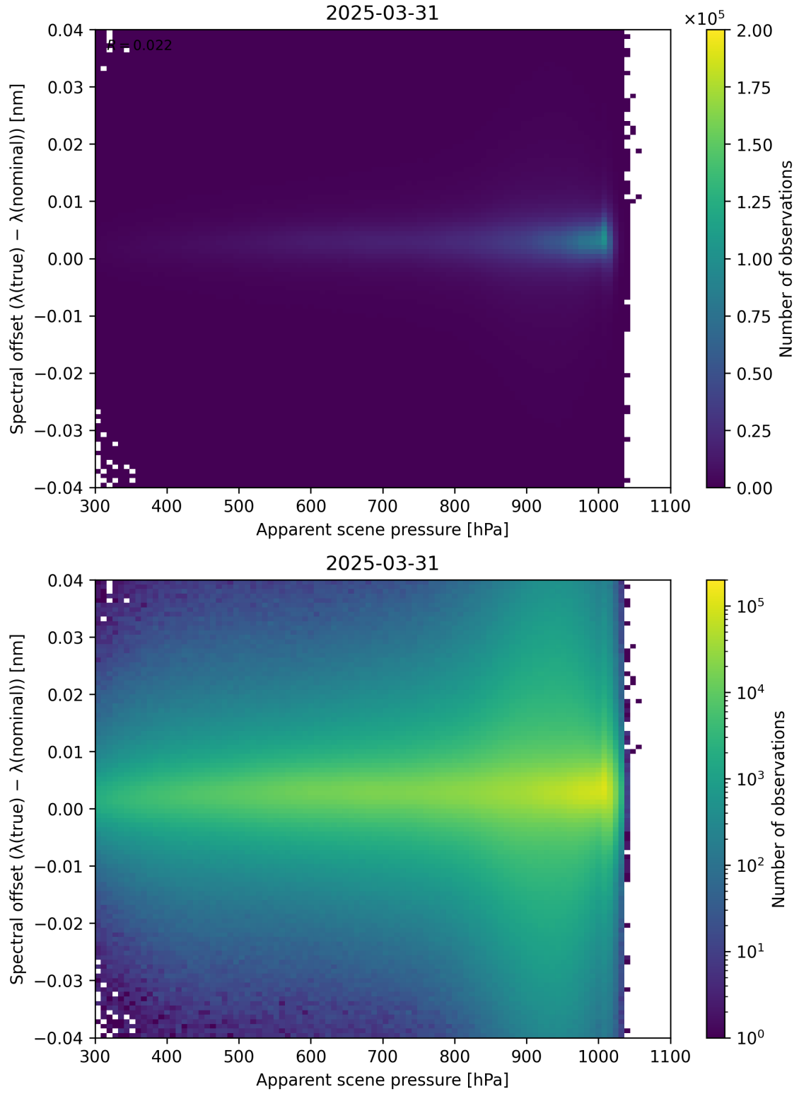
Figure 67: Scatter density plot of “Apparent scene pressure” against “Spectral offset ( \lambda_{\text{true}} - \lambda_{\text{nominal}} )” for 2025-03-30 to 2025-04-01.
