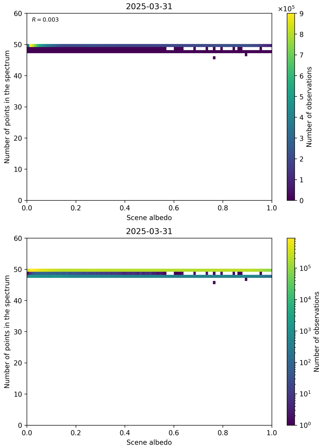
Figure 106: Scatter density plot of “Scene albedo” against “Number of points in the spectrum” for 2025-03-30 to 2025-04-01.
