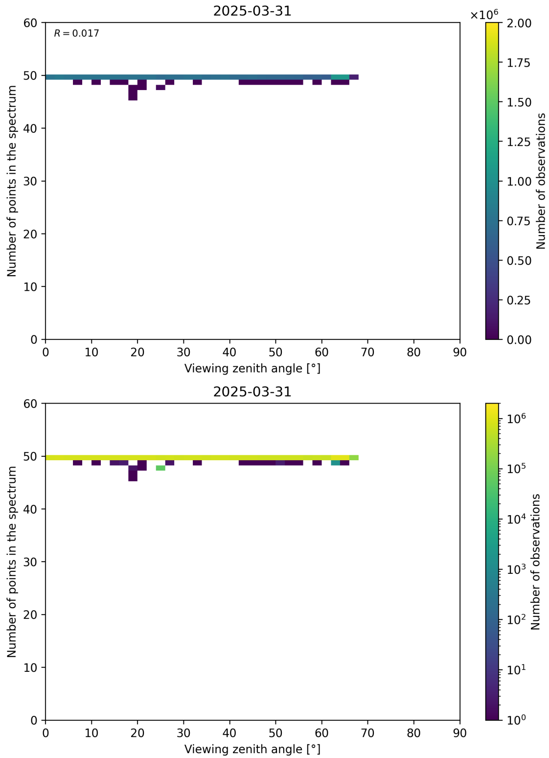
Figure 125: Scatter density plot of “Viewing zenith angle” against “Number of points in the spectrum” for 2025-03-30 to 2025-04-01.
