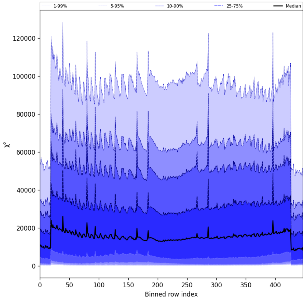
Figure 55: Along track statistics of “ \chi^2 ” for 2025-03-30 to 2025-04-01
