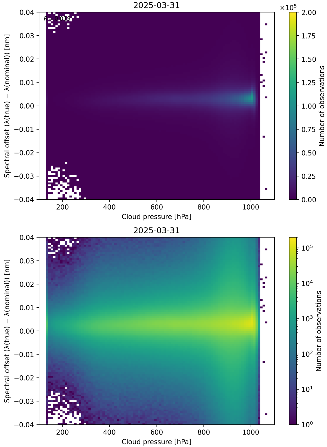
Figure 84: Scatter density plot of “Cloud pressure” against “Spectral offset ( \lambda_{\text{true}} - \lambda_{\text{nominal}} )” for 2025-03-30 to 2025-04-01.
