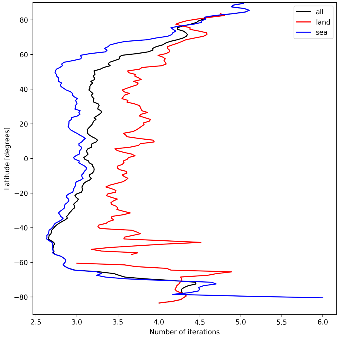
Figure 22: Zonal average of “Number of iterations” for 2025-03-30 to 2025-04-01.
