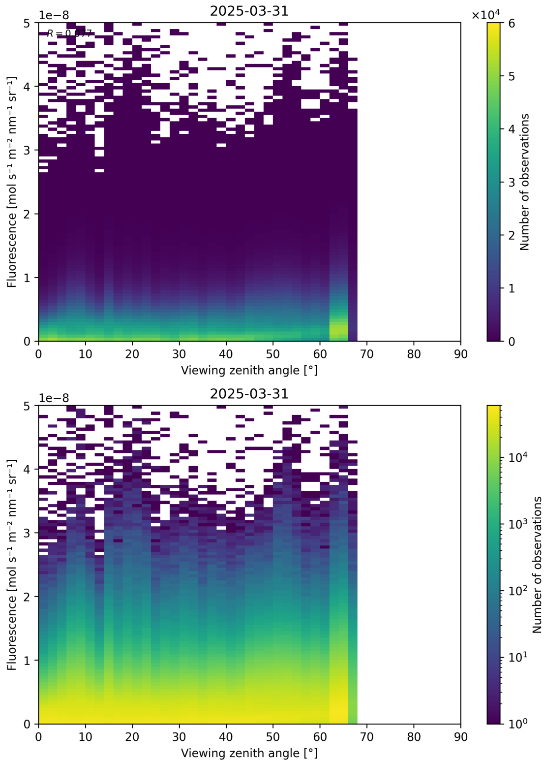
Figure 122: Scatter density plot of “Viewing zenith angle” against “Fluorescence” for 2025-03-30 to 2025-04-01.
