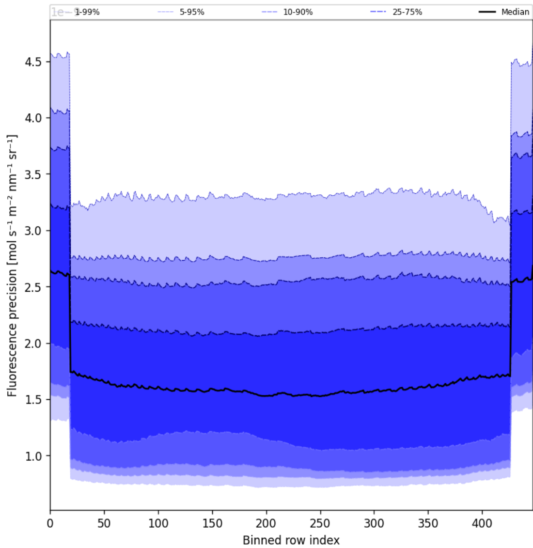
Figure 58: Along track statistics of “Fluorescence precision” for 2025-03-30 to 2025-04-01
