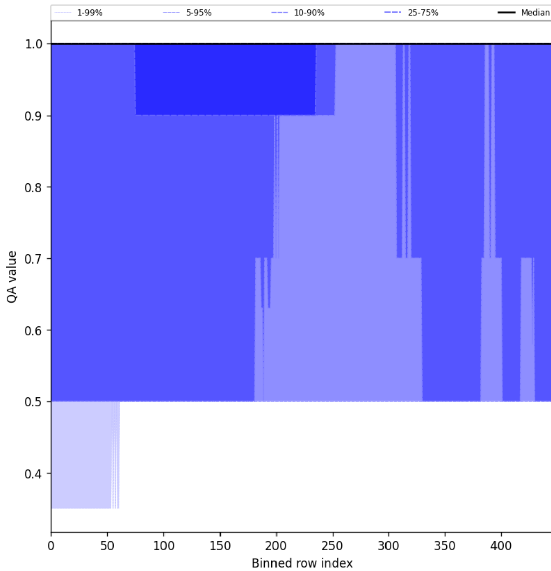
Figure 46: Along track statistics of “QA value” for 2025-03-30 to 2025-04-01
