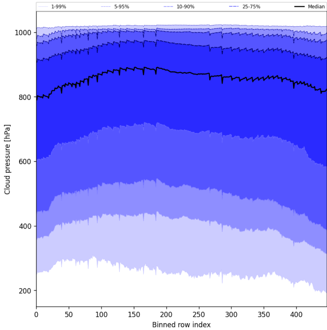
Figure 47: Along track statistics of “Cloud pressure” for 2025-03-30 to 2025-04-01
