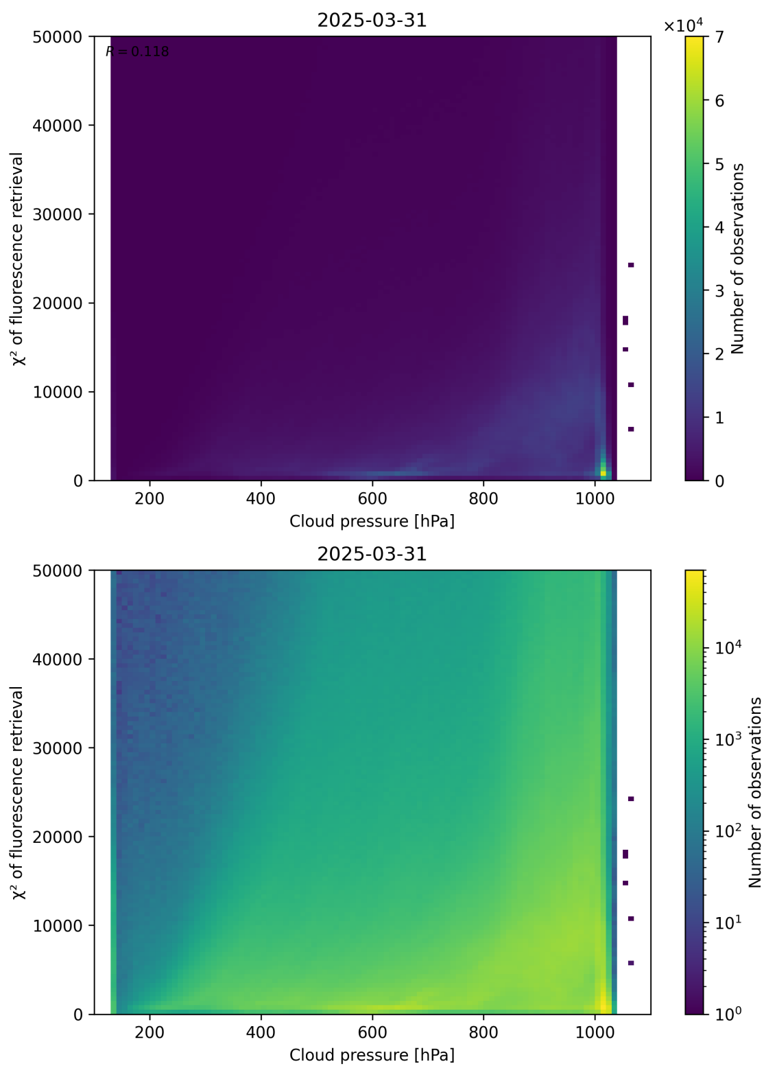
Figure 78: Scatter density plot of “Cloud pressure” against “ \chi^2 of fluorescence retrieval” for 2025-03-30 to 2025-04-01.
