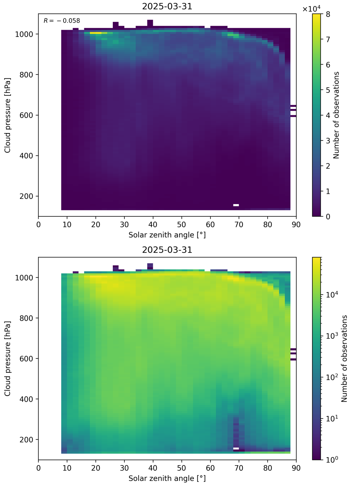
Figure 111: Scatter density plot of “Solar zenith angle” against “Cloud pressure” for 2025-03-30 to 2025-04-01.
