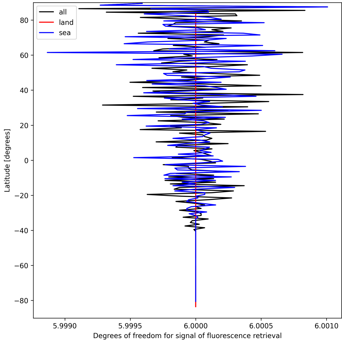
Figure 26: Zonal average of “Degrees of freedom for signal of fluorescence retrieval” for 2025-03-30 to 2025-04-01.
