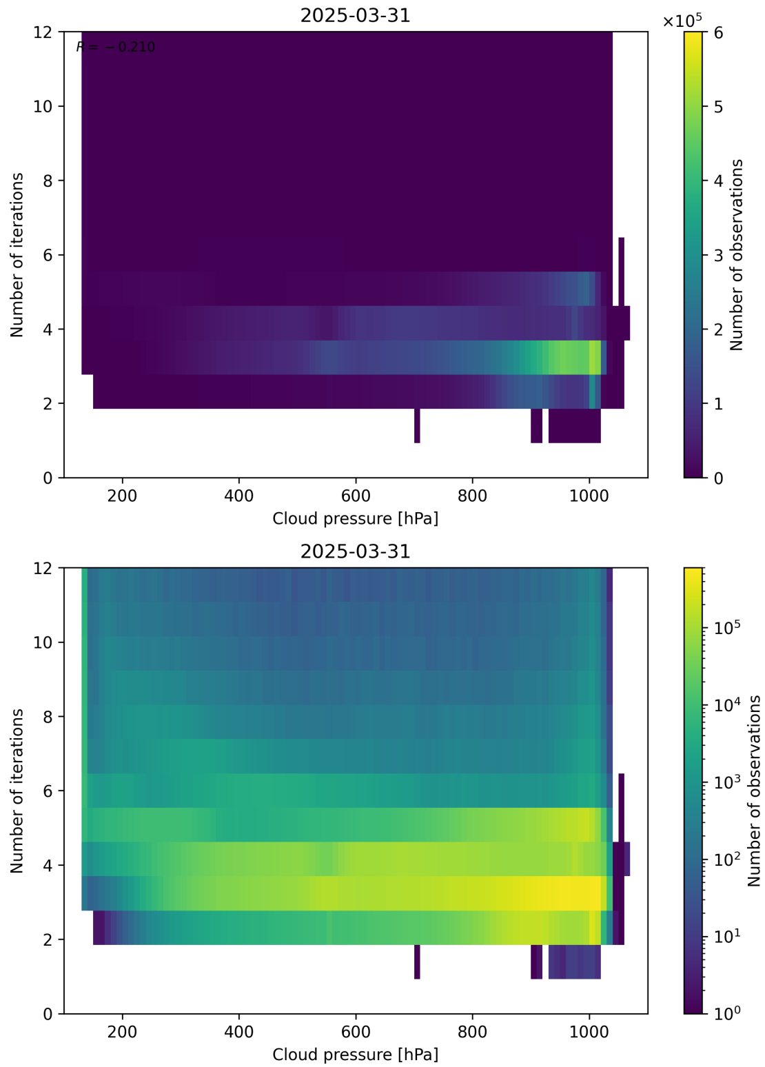
Figure 81: Scatter density plot of “Cloud pressure” against “Number of iterations” for 2025-03-30 to 2025-04-01.
