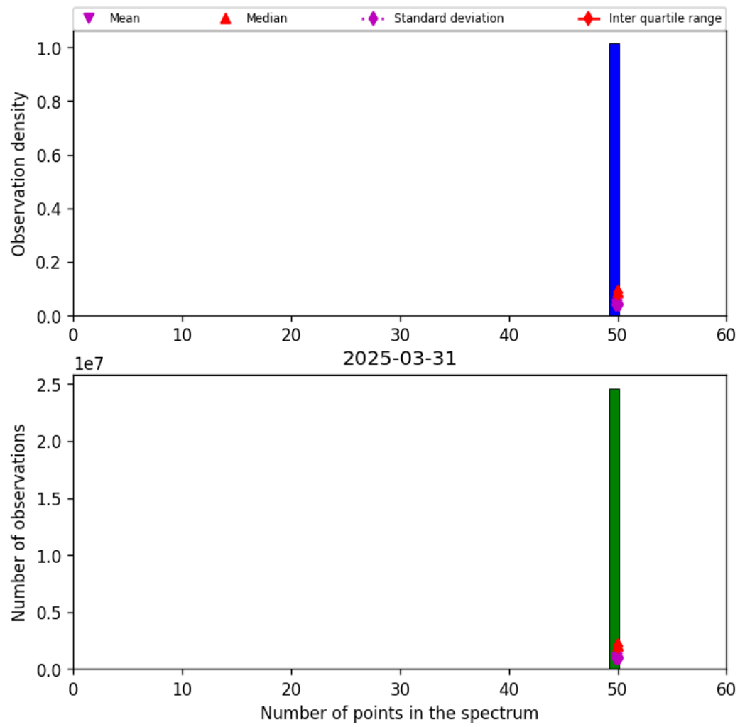
Figure 44: Histogram of “Number of points in the spectrum” for 2025-03-30 to 2025-04-01
