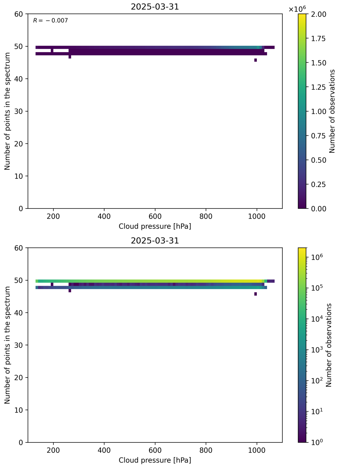
Figure 82: Scatter density plot of “Cloud pressure” against “Number of points in the spectrum” for 2025-03-30 to 2025-04-01.
