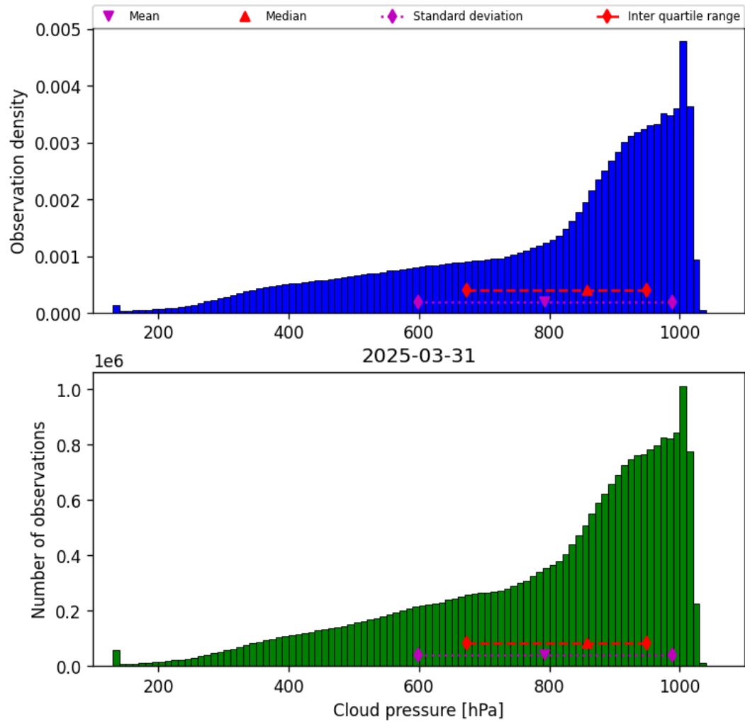
Figure 30: Histogram of “Cloud pressure” for 2025-03-30 to 2025-04-01
