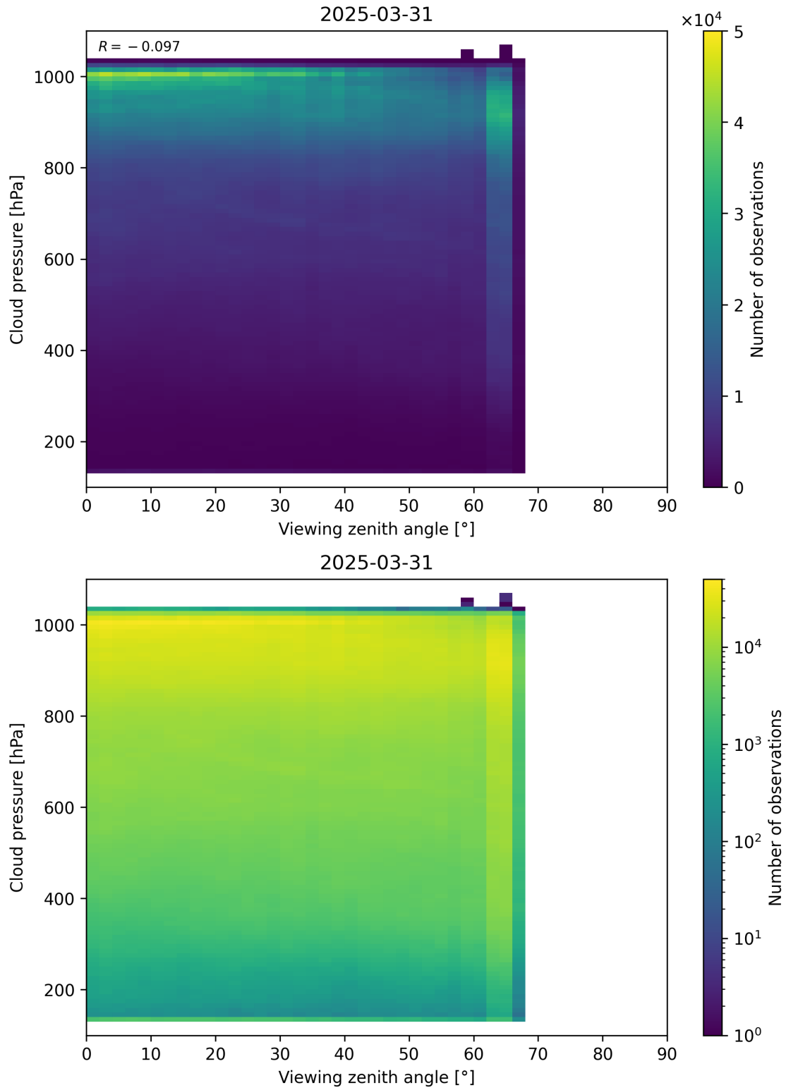
Figure 121: Scatter density plot of “Viewing zenith angle” against “Cloud pressure” for 2025-03-30 to 2025-04-01.
