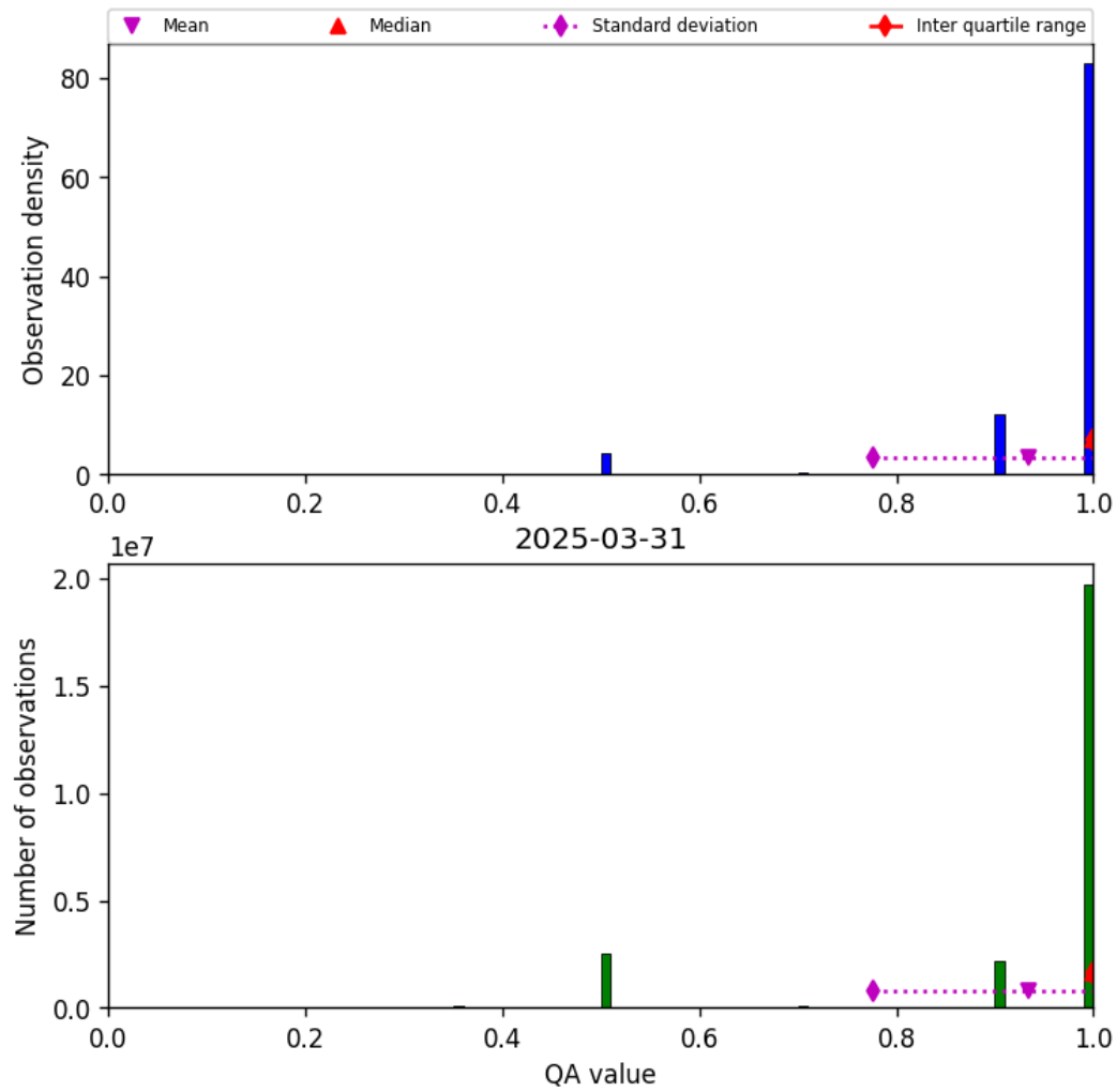
Figure 29: Histogram of “QA value” for 2025-03-30 to 2025-04-01
