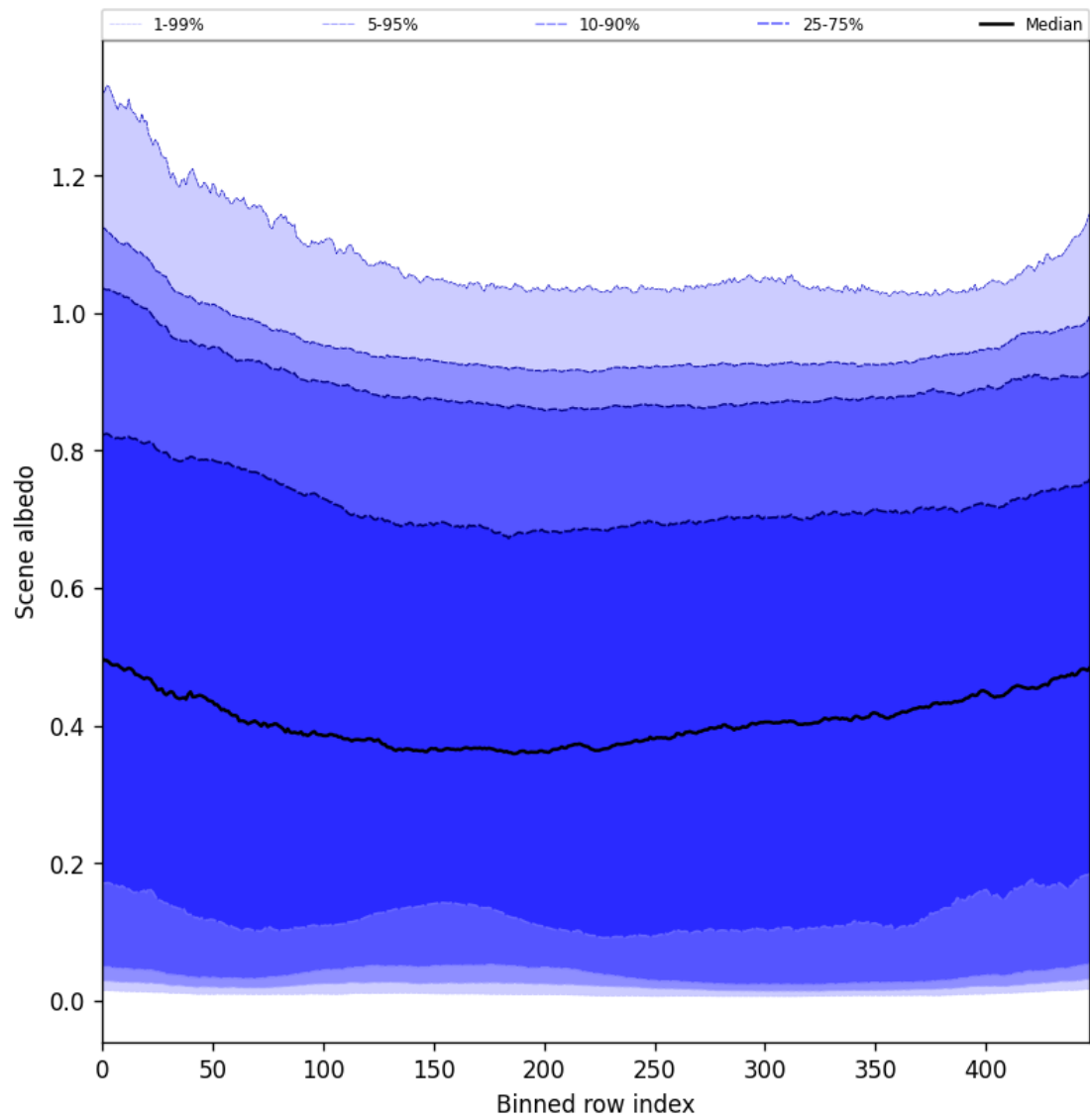
Figure 51: Along track statistics of “Scene albedo” for 2025-03-30 to 2025-04-01
