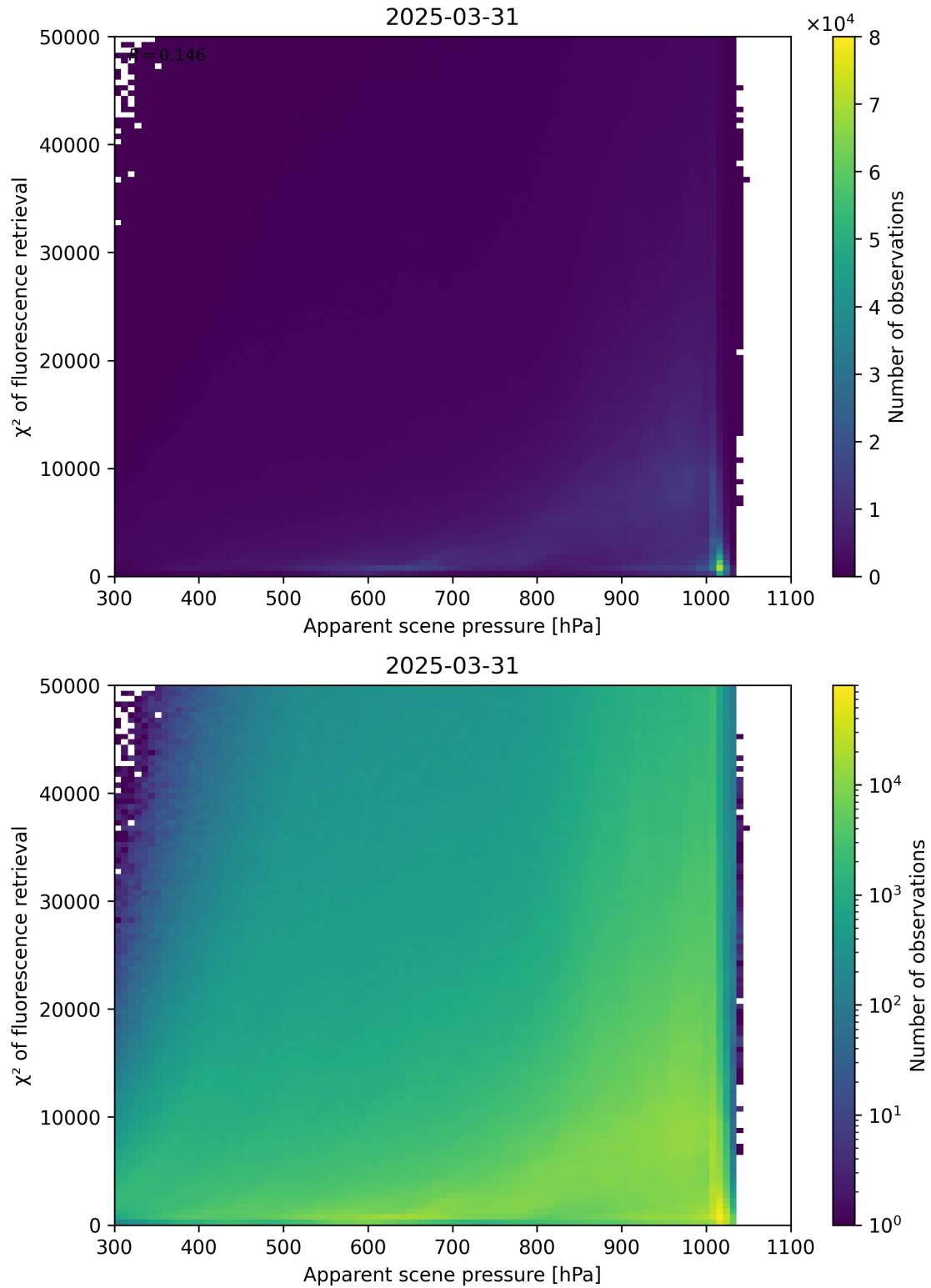
Figure 63: Scatter density plot of “Apparent scene pressure” against “ \chi^2 of fluorescence retrieval” for 2025-03-30 to 2025-04-01.
