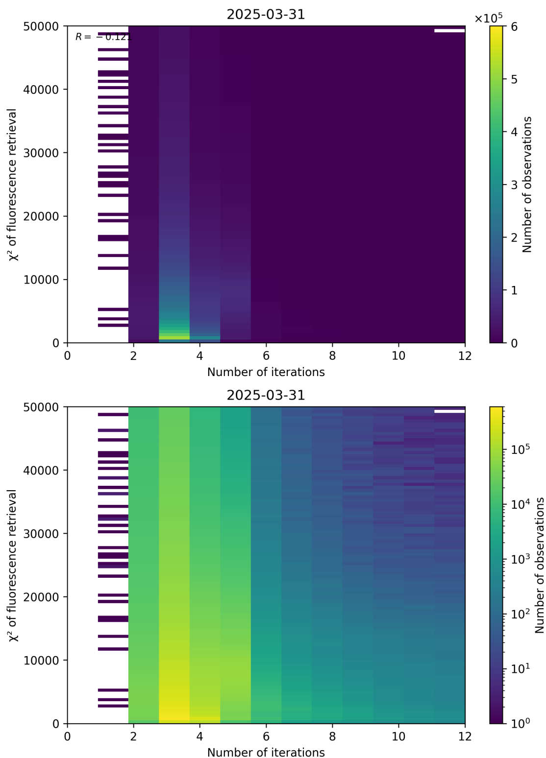
Figure 97: Scatter density plot of “Number of iterations” against “ \chi^2 of fluorescence retrieval” for 2025-03-30 to 2025-04-01.
