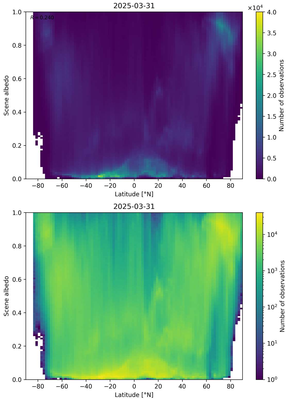
Figure 95: Scatter density plot of “Latitude” against “Scene albedo” for 2025-03-30 to 2025-04-01.
