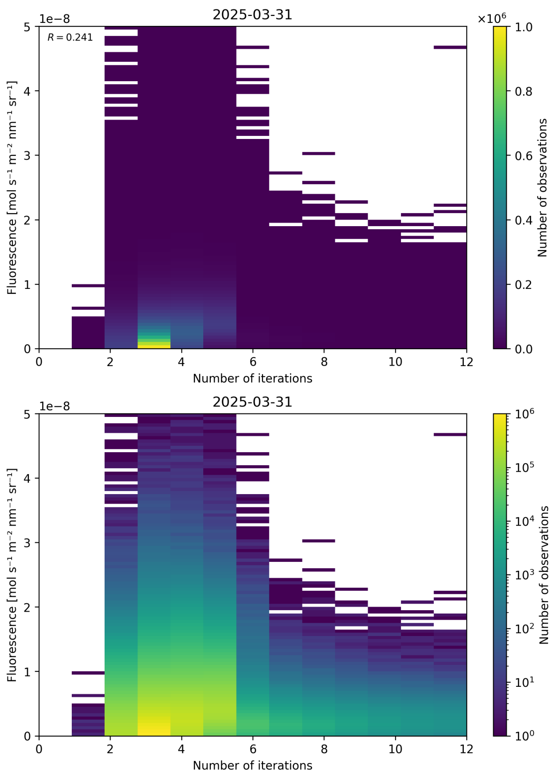
Figure 98: Scatter density plot of “Number of iterations” against “Fluorescence” for 2025-03-30 to 2025-04-01.
