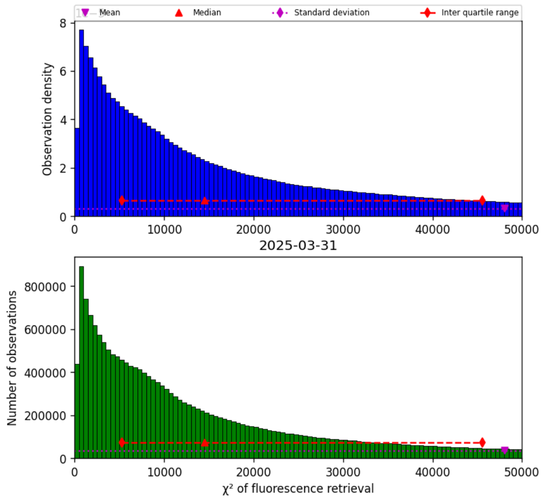
Figure 42: Histogram of “ \chi^2 of fluorescence retrieval” for 2025-03-30 to 2025-04-01
