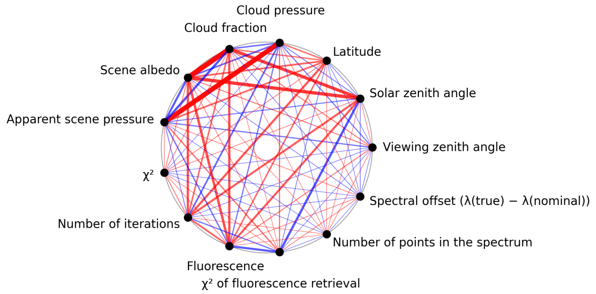
Figure 1: Map of correlation graph for 2025-03-30 to 2025-04-01.
