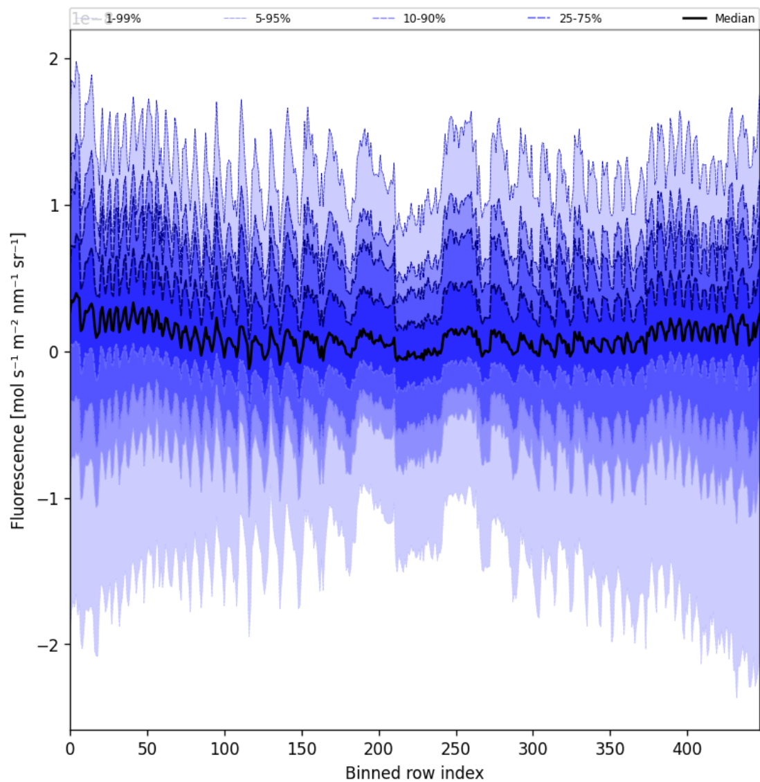
Figure 57: Along track statistics of “Fluorescence” for 2025-03-30 to 2025-04-01
