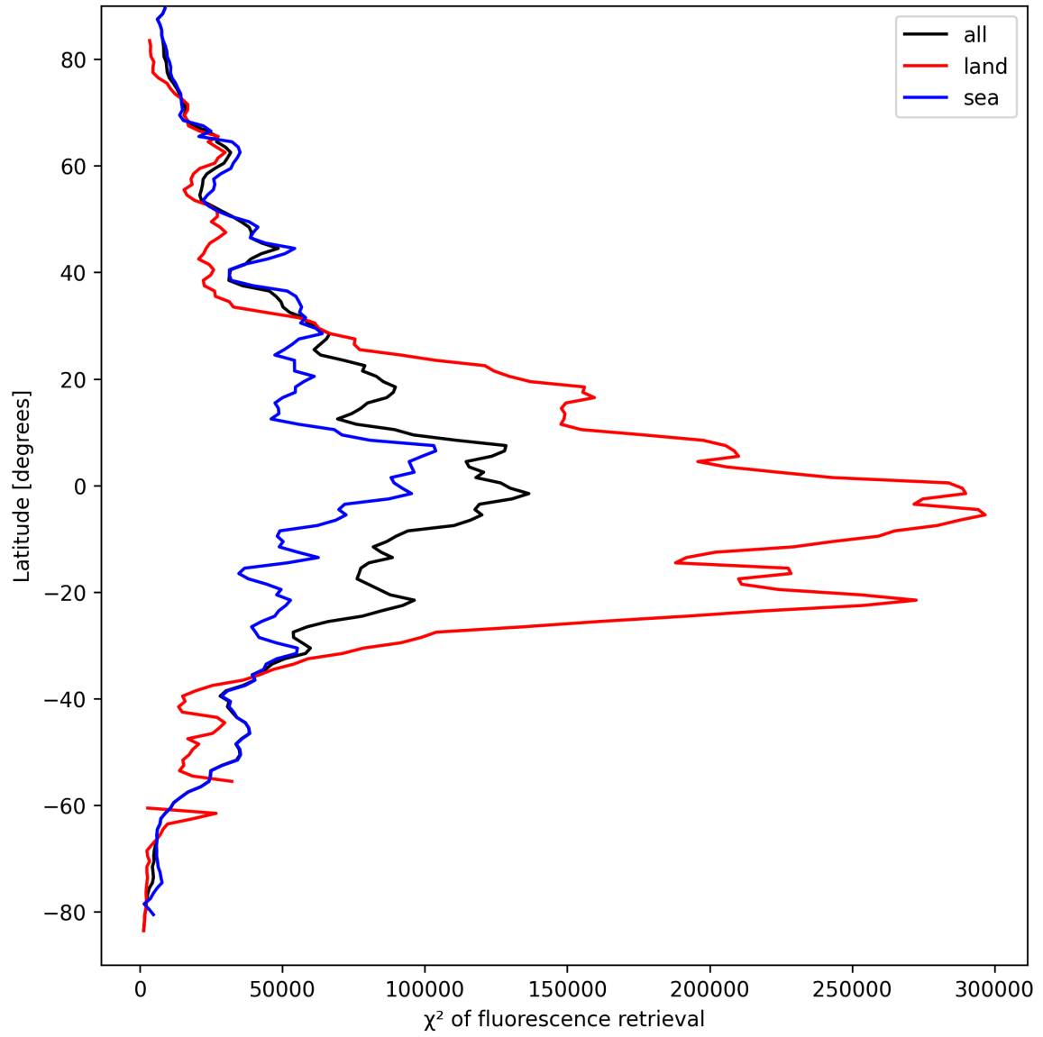
Figure 25: Zonal average of “ \chi^2 of fluorescence retrieval” for 2025-03-30 to 2025-04-01.
