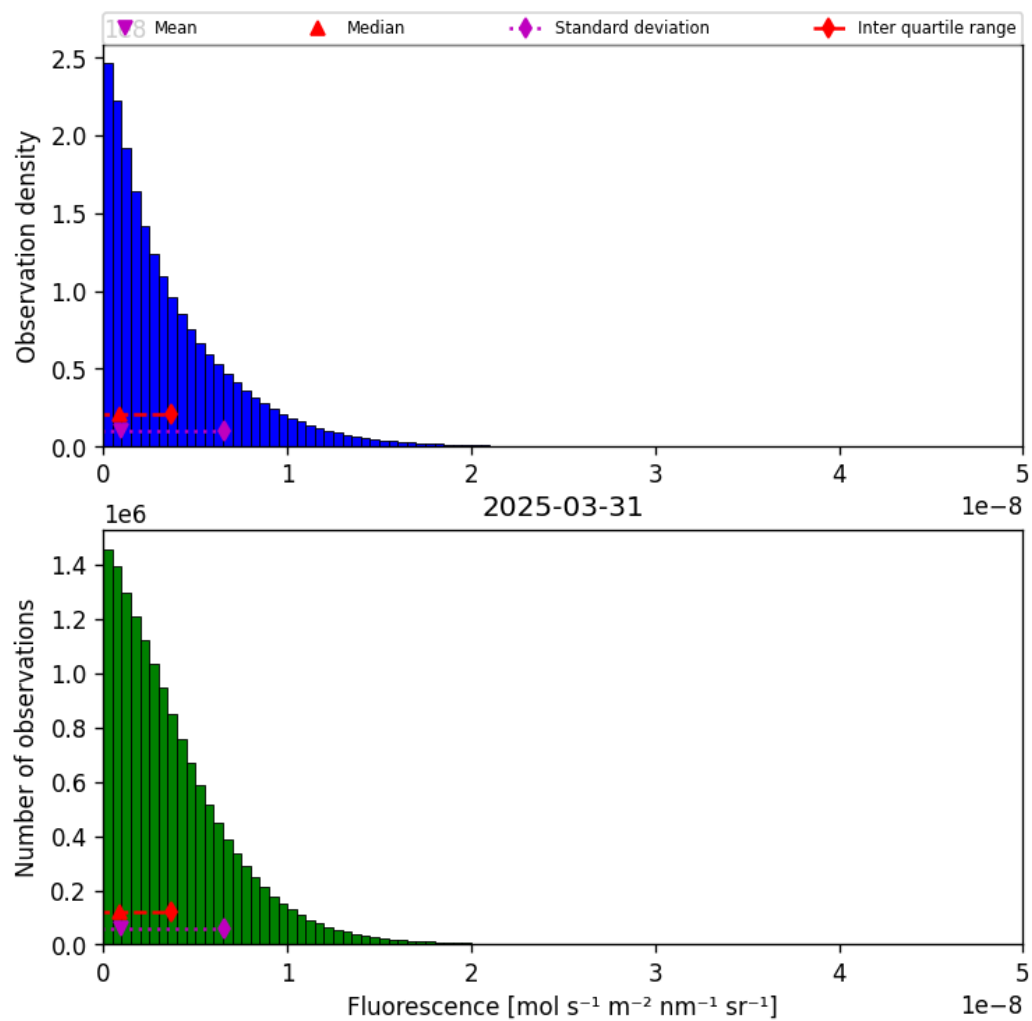
Figure 40: Histogram of “Fluorescence” for 2025-03-30 to 2025-04-01
