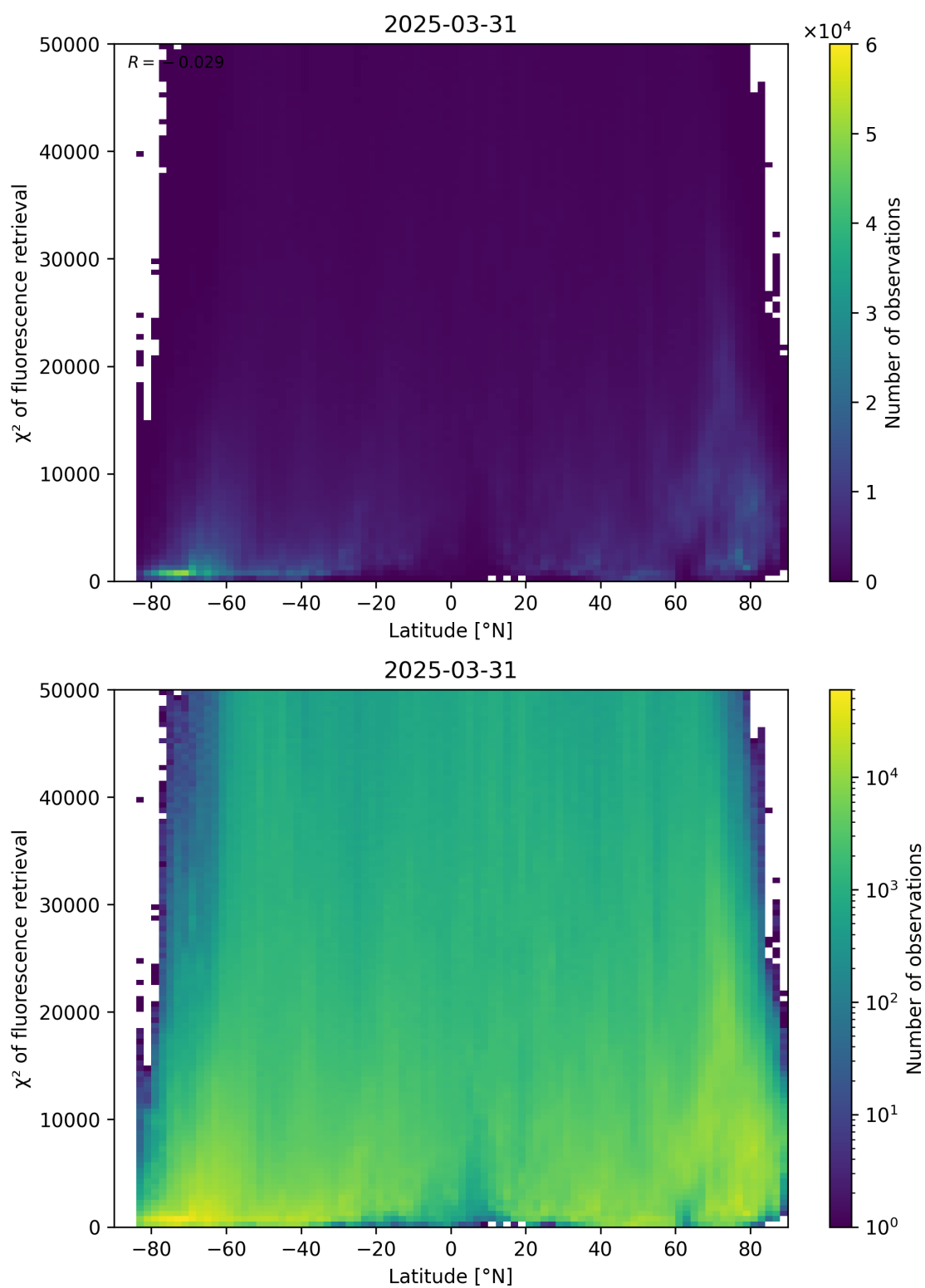
Figure 89: Scatter density plot of “Latitude” against “ \chi^2 of fluorescence retrieval” for 2025-03-30 to 2025-04-01.
