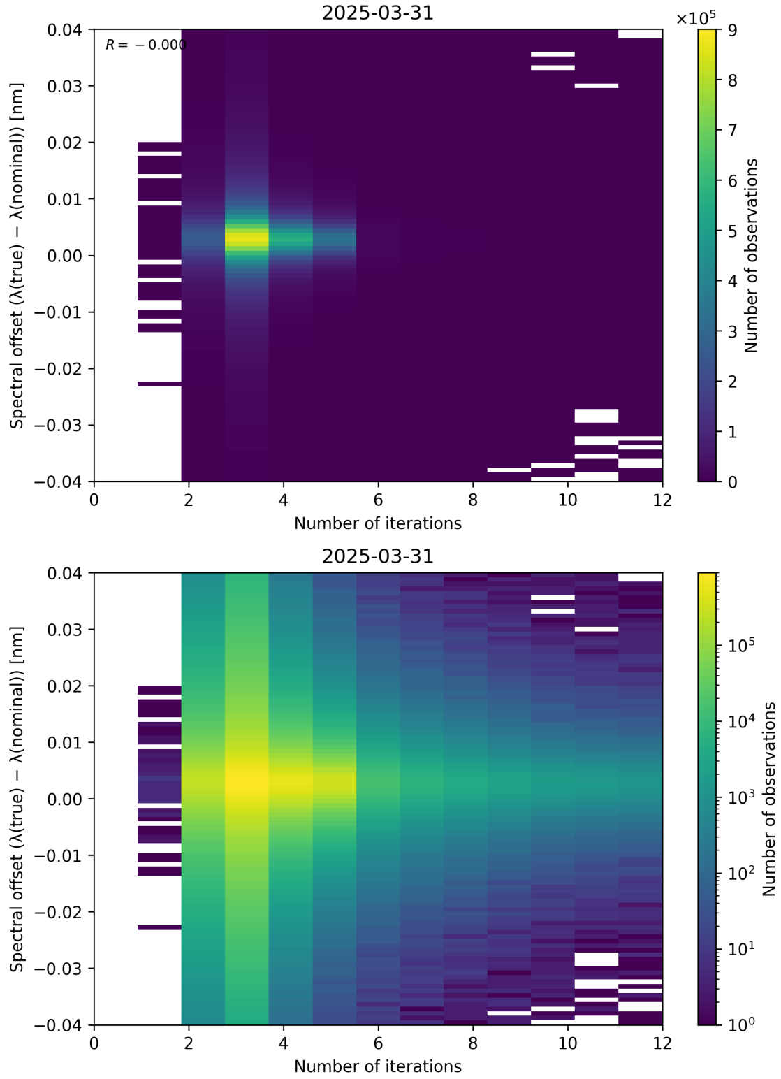
Figure 100: Scatter density plot of “Number of iterations” against “Spectral offset ( \lambda_{\text{true}} - \lambda_{\text{nominal}} )” for 2025-03-30 to 2025-04-01.
