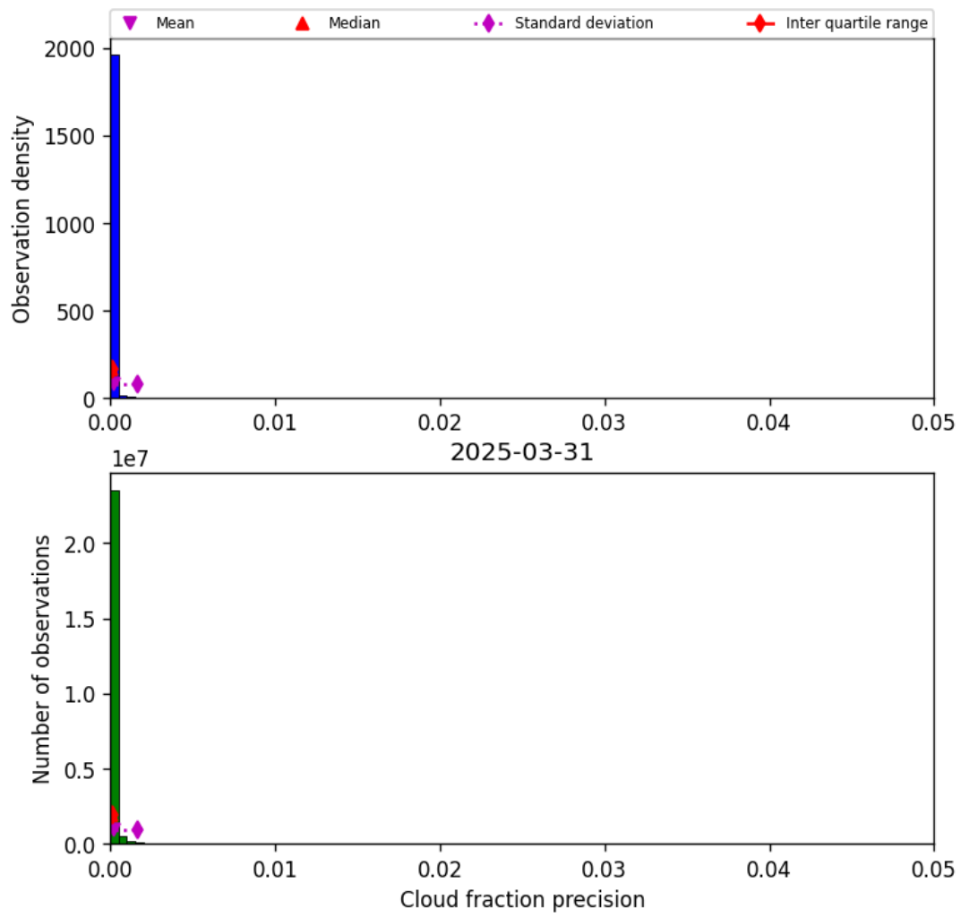
Figure 33: Histogram of “Cloud fraction precision” for 2025-03-30 to 2025-04-01
