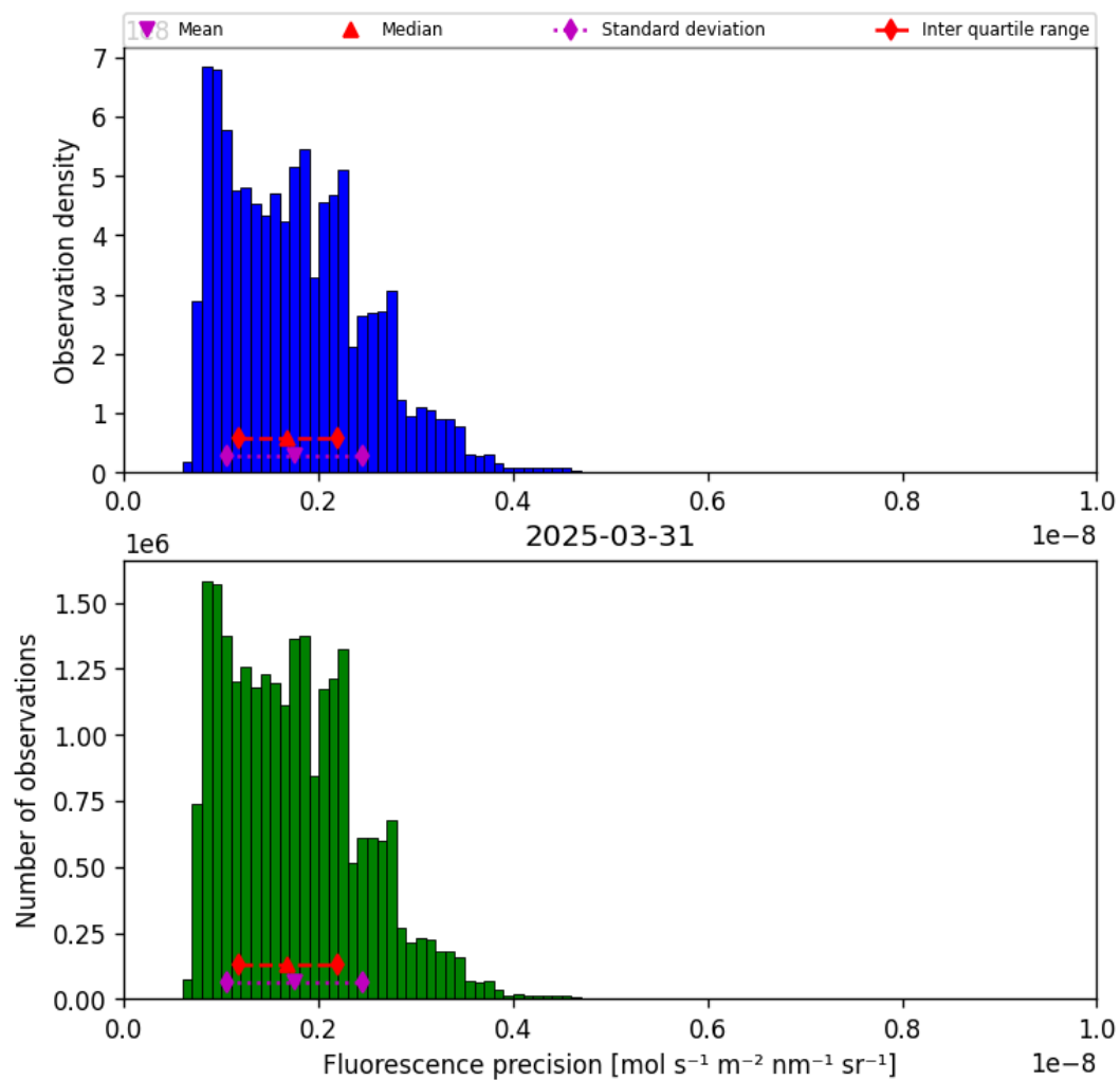
Figure 41: Histogram of “Fluorescence precision” for 2025-03-30 to 2025-04-01
