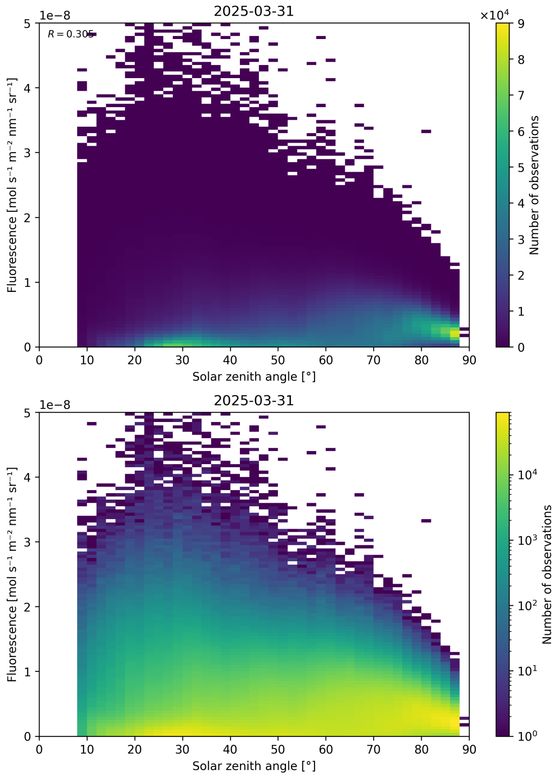
Figure 112: Scatter density plot of “Solar zenith angle” against “Fluorescence” for 2025-03-30 to 2025-04-01.
