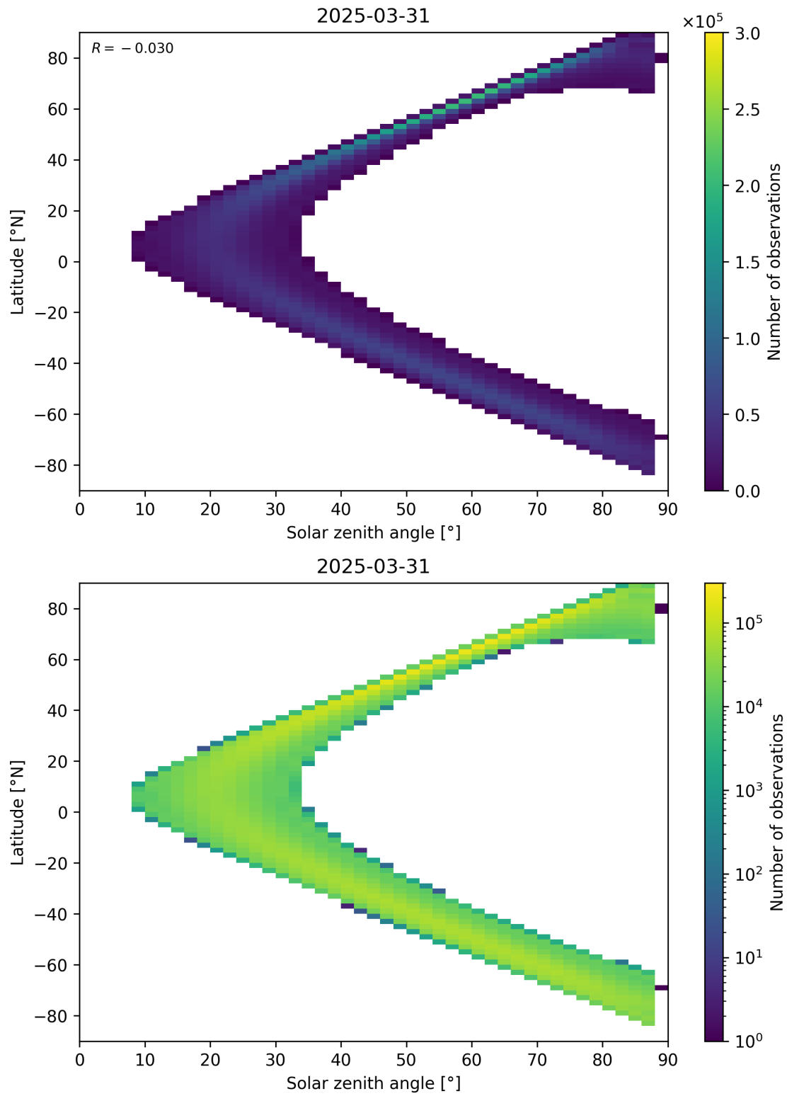
Figure 113: Scatter density plot of “Solar zenith angle” against “Latitude” for 2025-03-30 to 2025-04-01.
