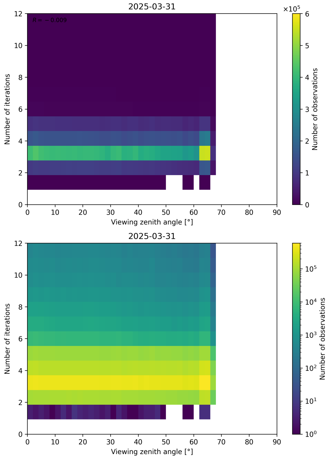
Figure 124: Scatter density plot of “Viewing zenith angle” against “Number of iterations” for 2025-03-30 to 2025-04-01.
