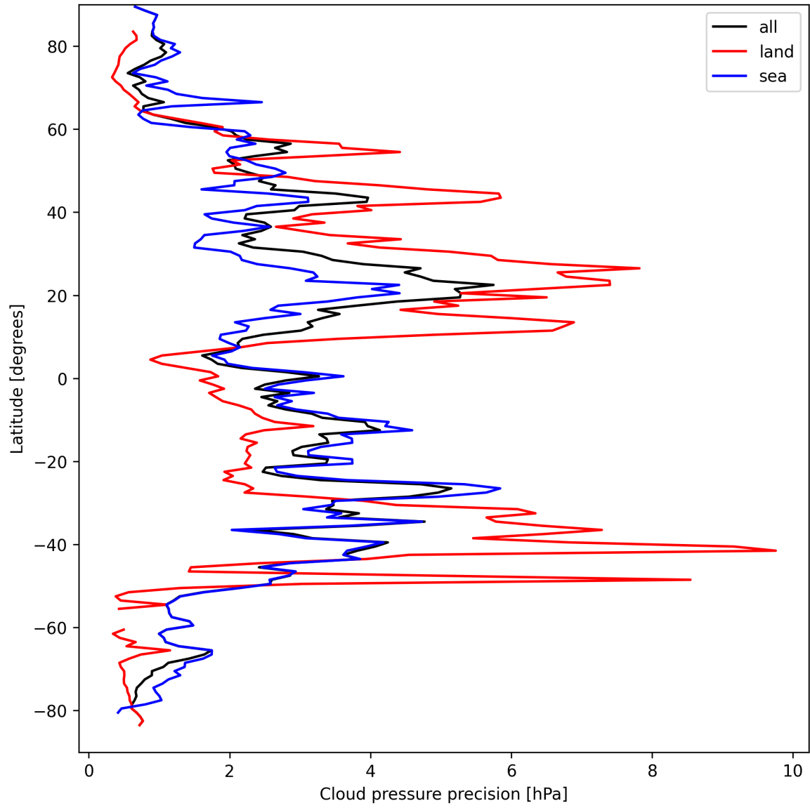
Figure 14: Zonal average of "Cloud pressure precision" for 2025-03-30 to 2025-04-01.
