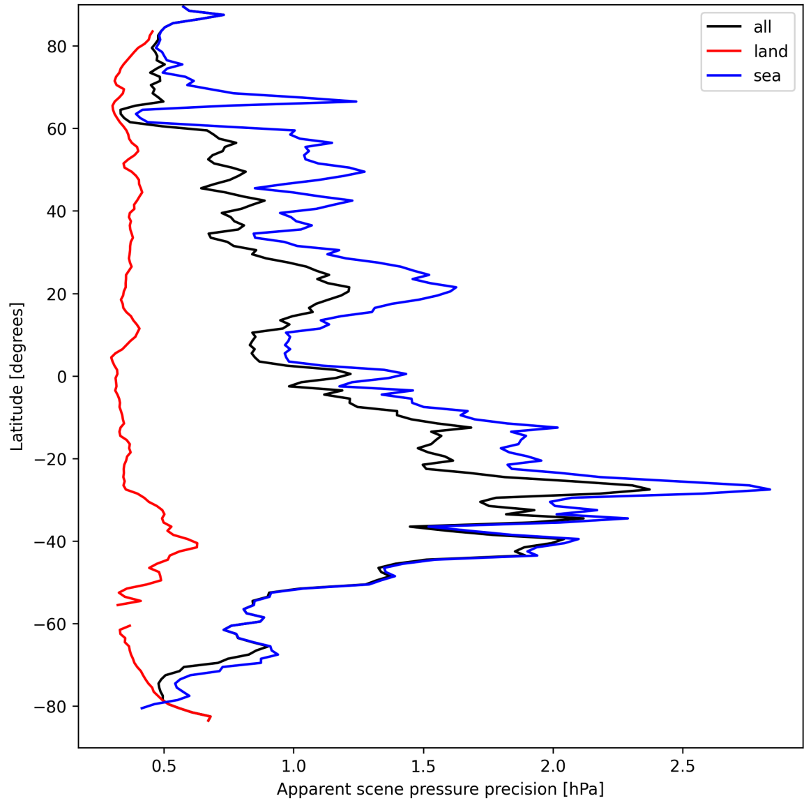
Figure 20: Zonal average of “Apparent scene pressure precision” for 2025-03-30 to 2025-04-01.
