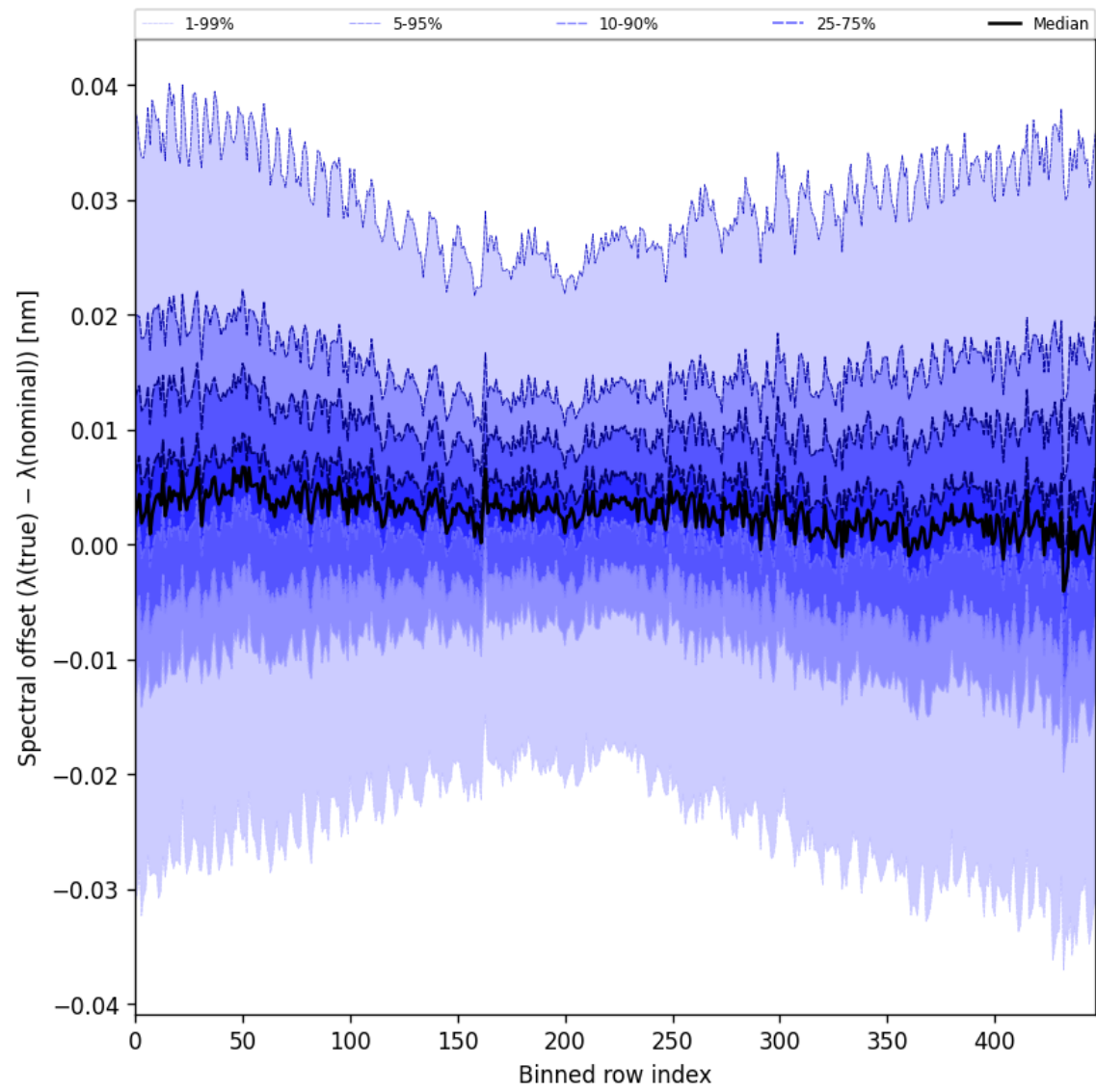
Figure 62: Along track statistics of “Spectral offset ( \lambda_{\text{true}} - \lambda_{\text{nominal}} )” for 2025-03-30 to 2025-04-01
