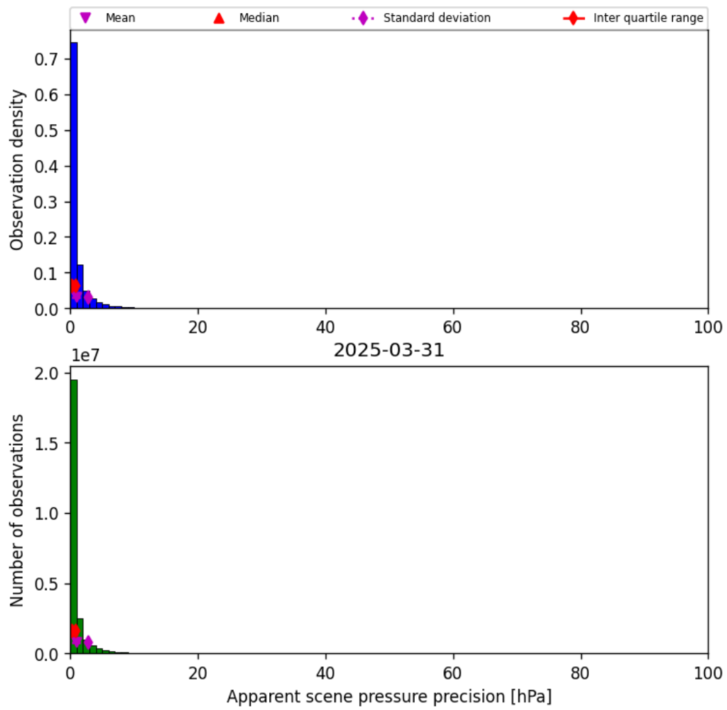
Figure 37: Histogram of “Apparent scene pressure precision” for 2025-03-30 to 2025-04-01
