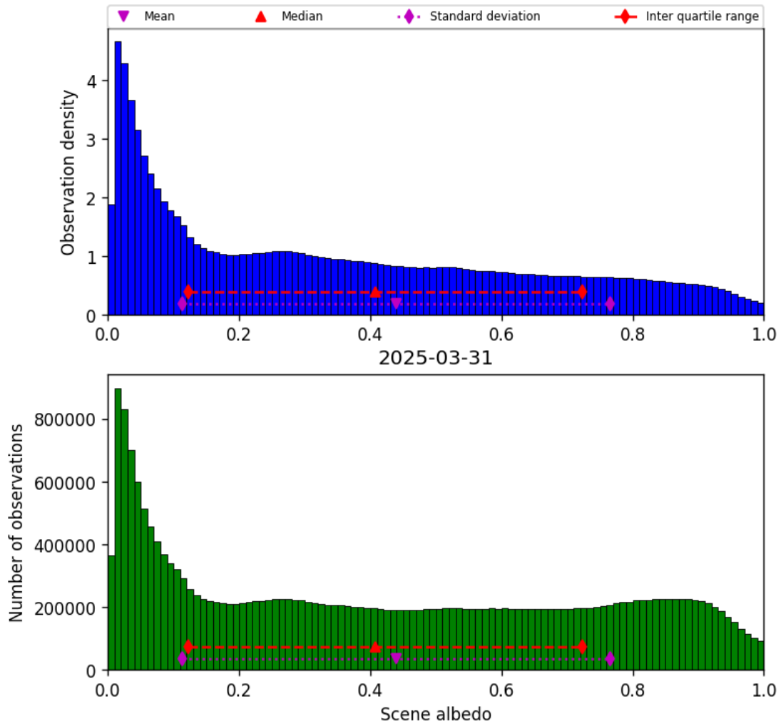
Figure 34: Histogram of “Scene albedo” for 2025-03-30 to 2025-04-01
