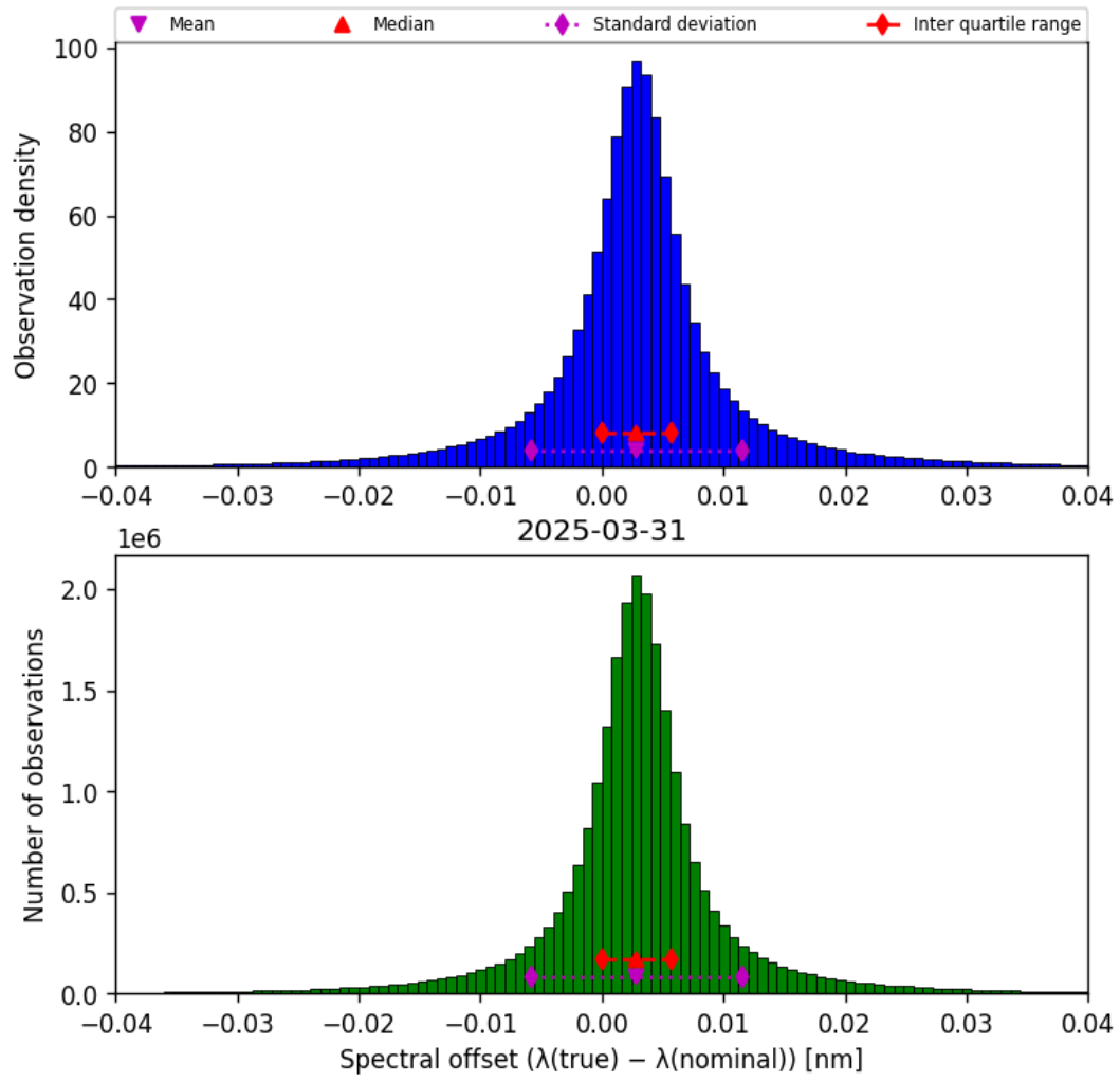
Figure 45: Histogram of “Spectral offset ( \lambda_{\text{true}} - \lambda_{\text{nominal}} )” for 2025-03-30 to 2025-04-01
