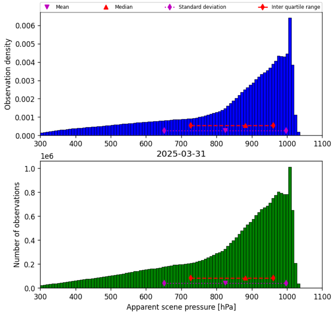
Figure 36: Histogram of “Apparent scene pressure” for 2025-03-30 to 2025-04-01
