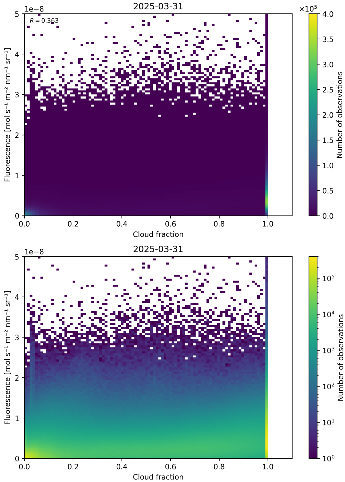
Figure 72: Scatter density plot of “Cloud fraction” against “Fluorescence” for 2025-03-30 to 2025-04-01.
