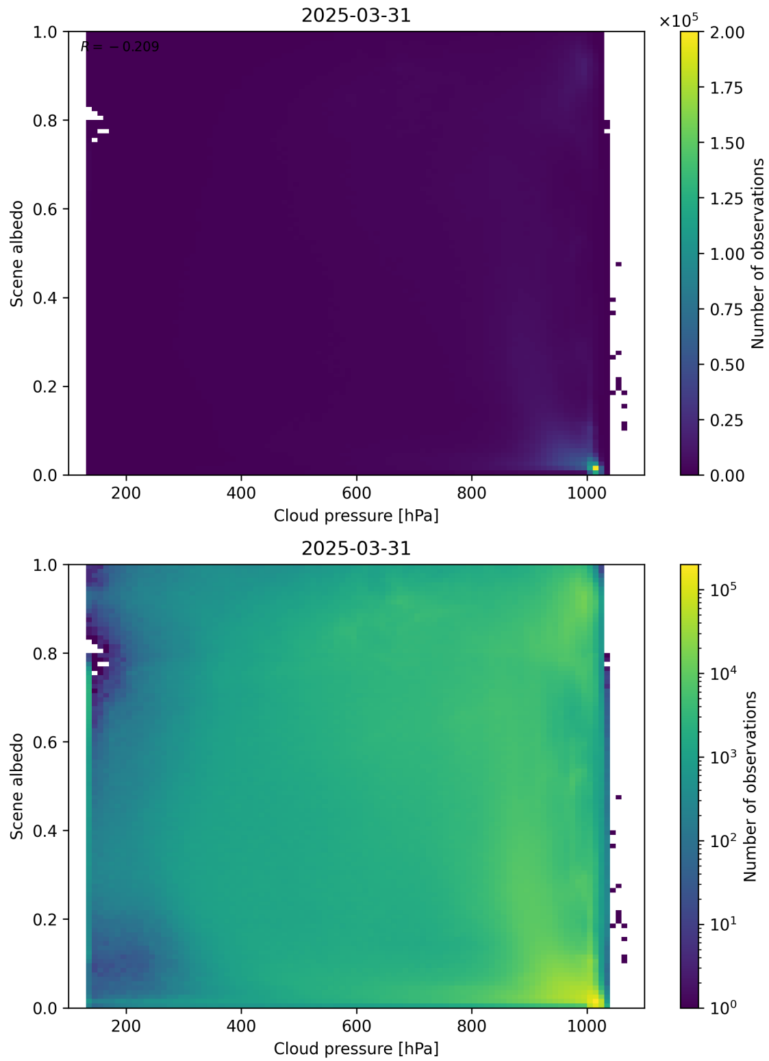
Figure 83: Scatter density plot of “Cloud pressure” against “Scene albedo” for 2025-03-30 to 2025-04-01.
