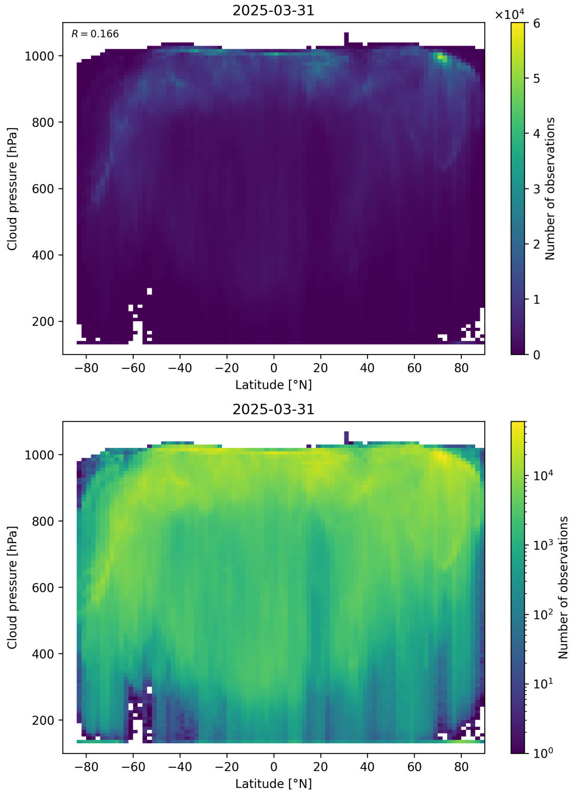
Figure 91: Scatter density plot of “Latitude” against “Cloud pressure” for 2025-03-30 to 2025-04-01.
