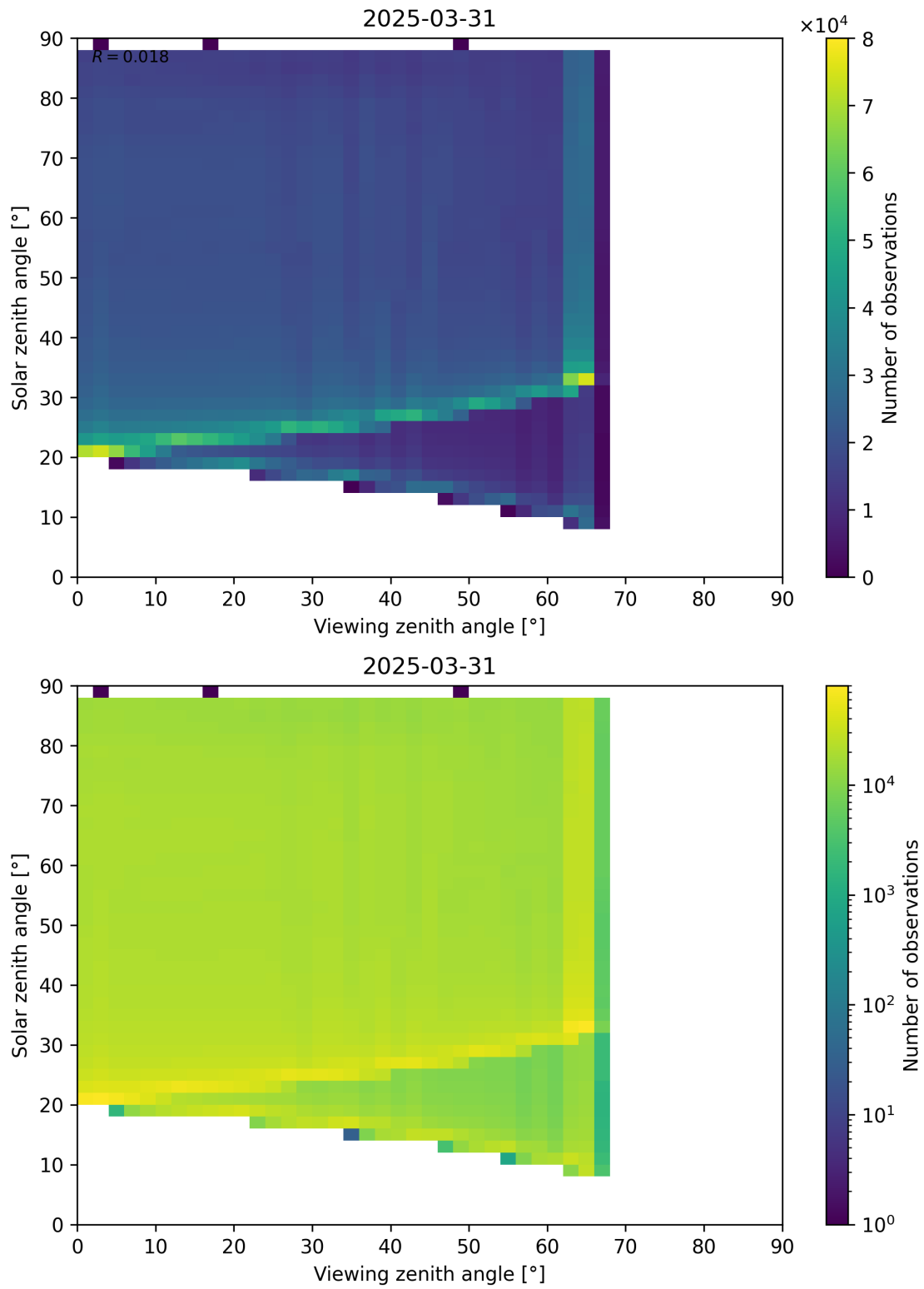
Figure 127: Scatter density plot of “Viewing zenith angle” against “Solar zenith angle” for 2025-03-30 to 2025-04-01.
