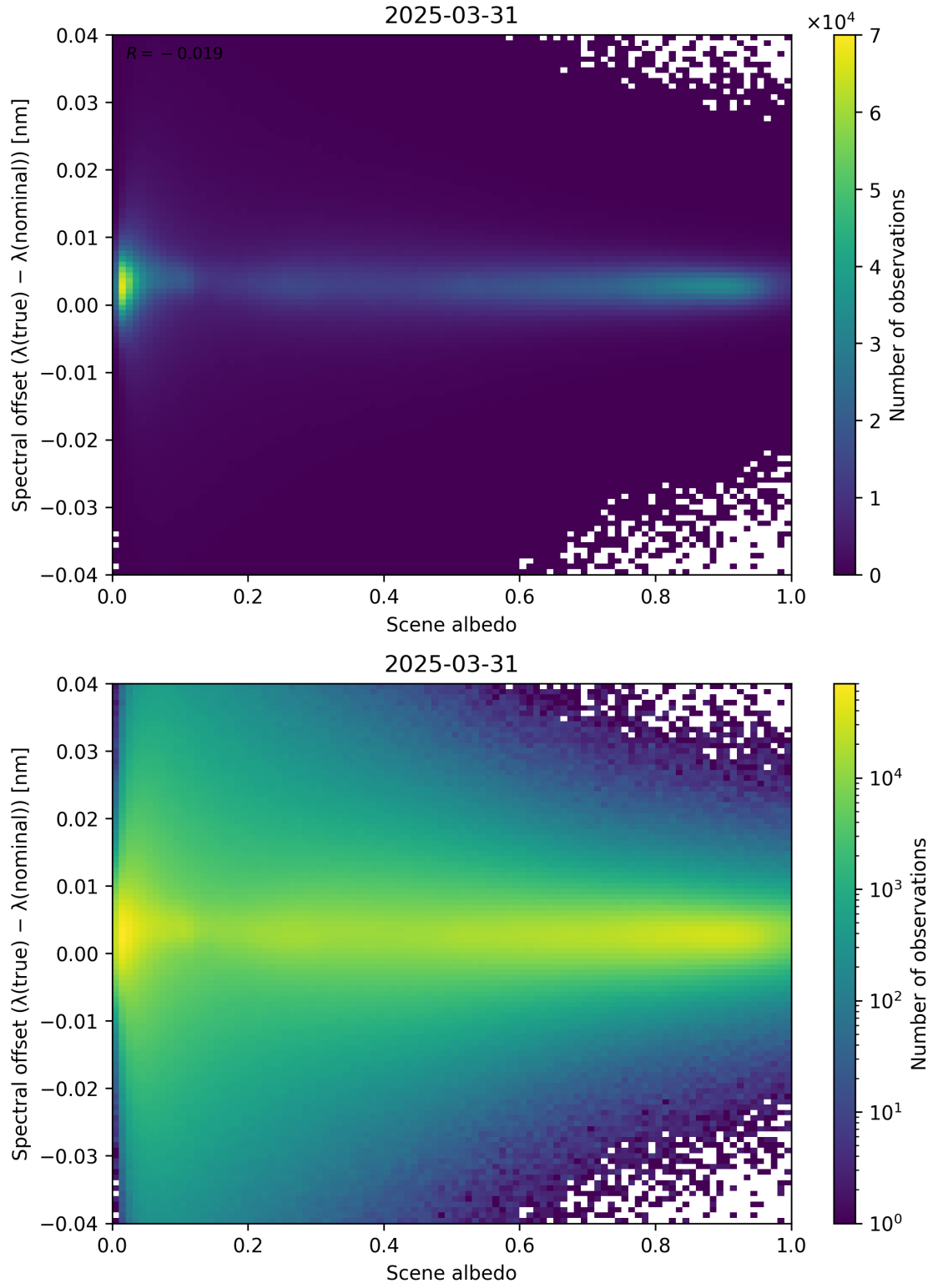
Figure 107: Scatter density plot of “Scene albedo” against “Spectral offset ( \lambda_{\text{true}} - \lambda_{\text{nominal}} )” for 2025-03-30 to 2025-04-01.
