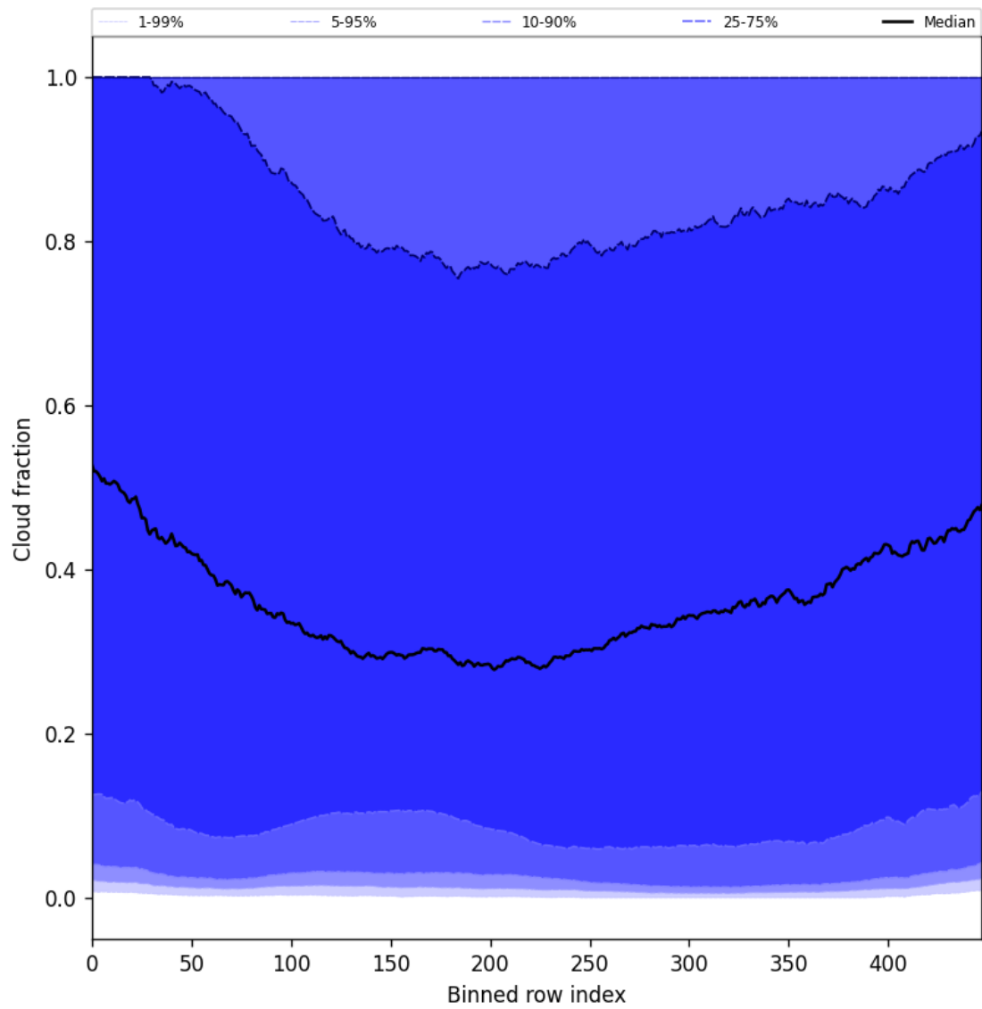
Figure 49: Along track statistics of “Cloud fraction” for 2025-03-30 to 2025-04-01
