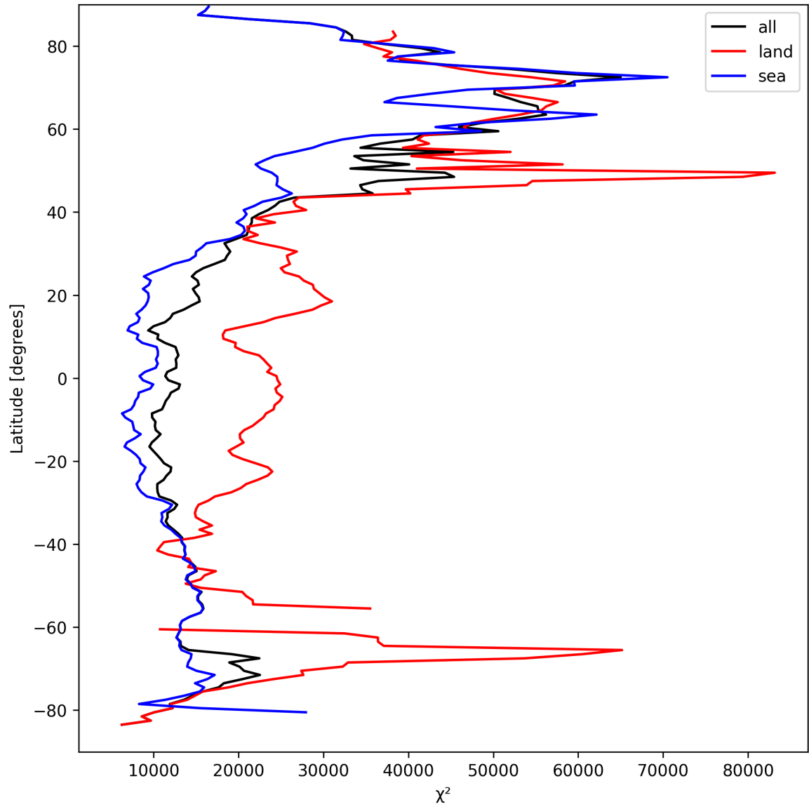
Figure 21: Zonal average of “ \chi^2 ” for 2025-03-30 to 2025-04-01.
