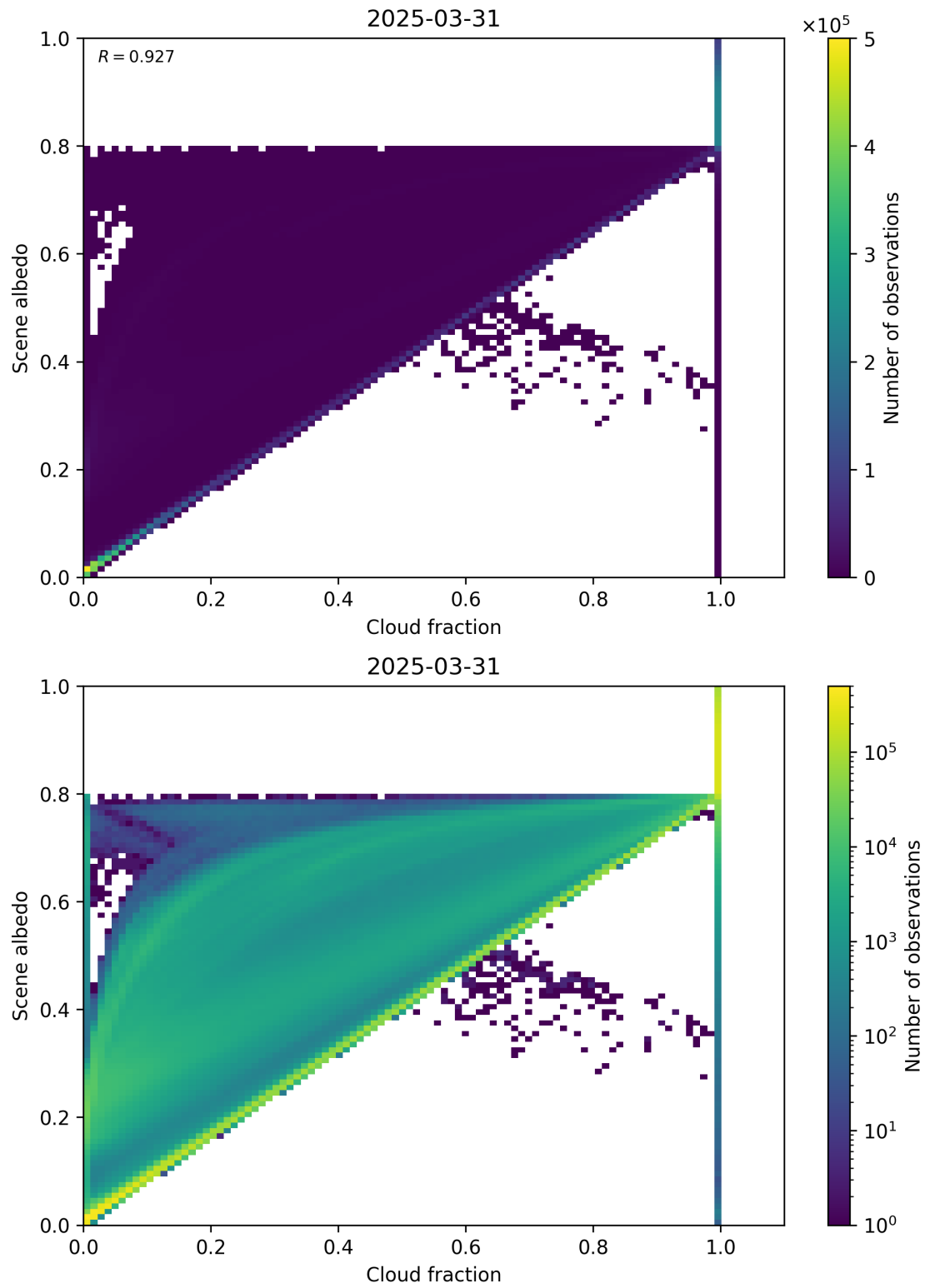
Figure 75: Scatter density plot of “Cloud fraction” against “Scene albedo” for 2025-03-30 to 2025-04-01.
