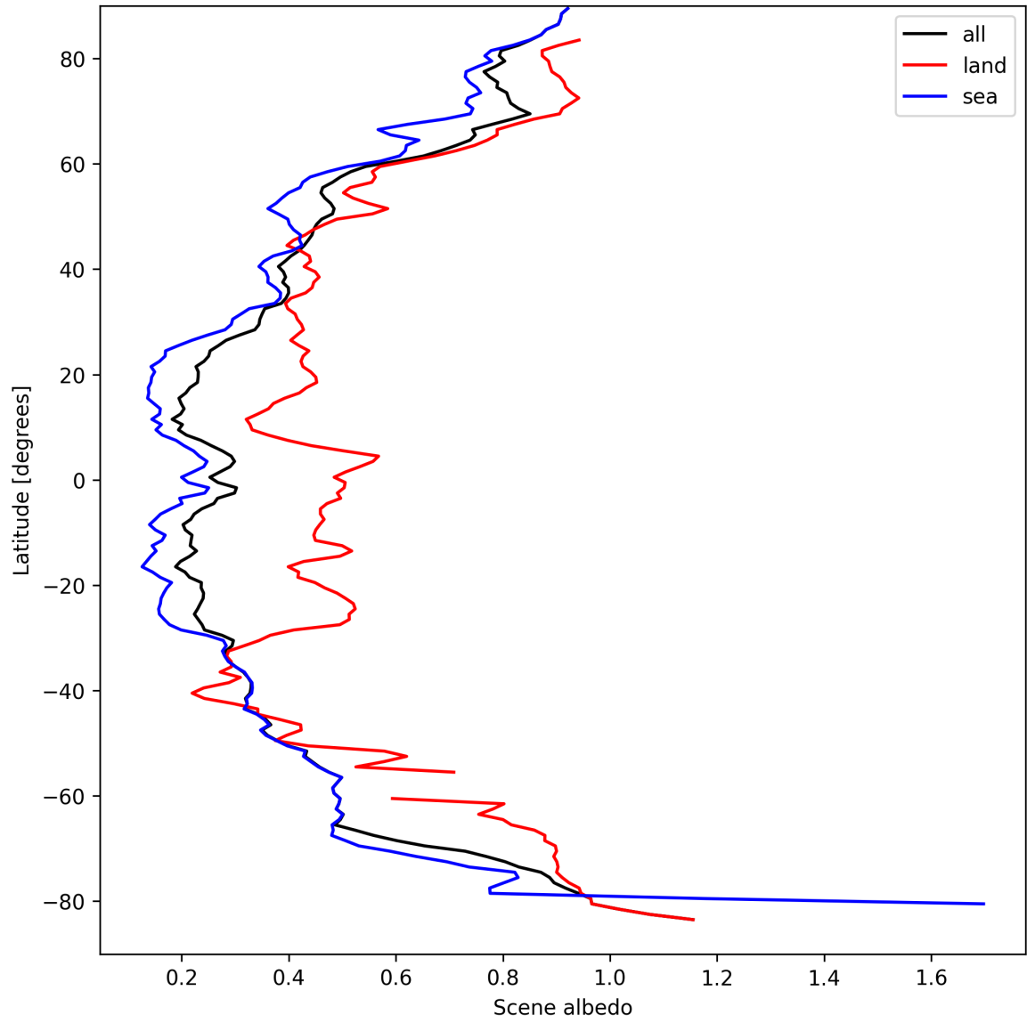
Figure 17: Zonal average of “Scene albedo” for 2025-03-30 to 2025-04-01.
