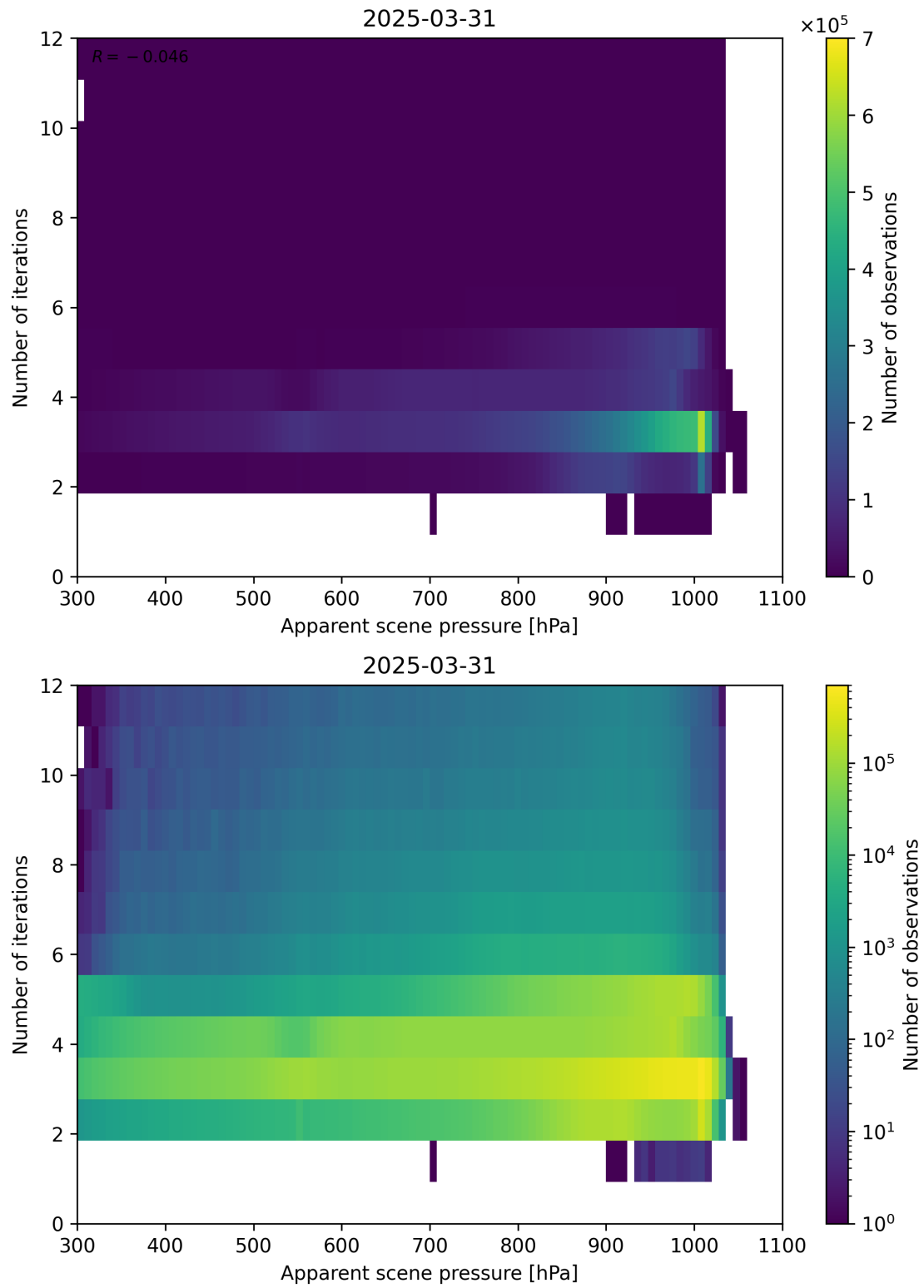
Figure 65: Scatter density plot of “Apparent scene pressure” against “Number of iterations” for 2025-03-30 to 2025-04-01.
