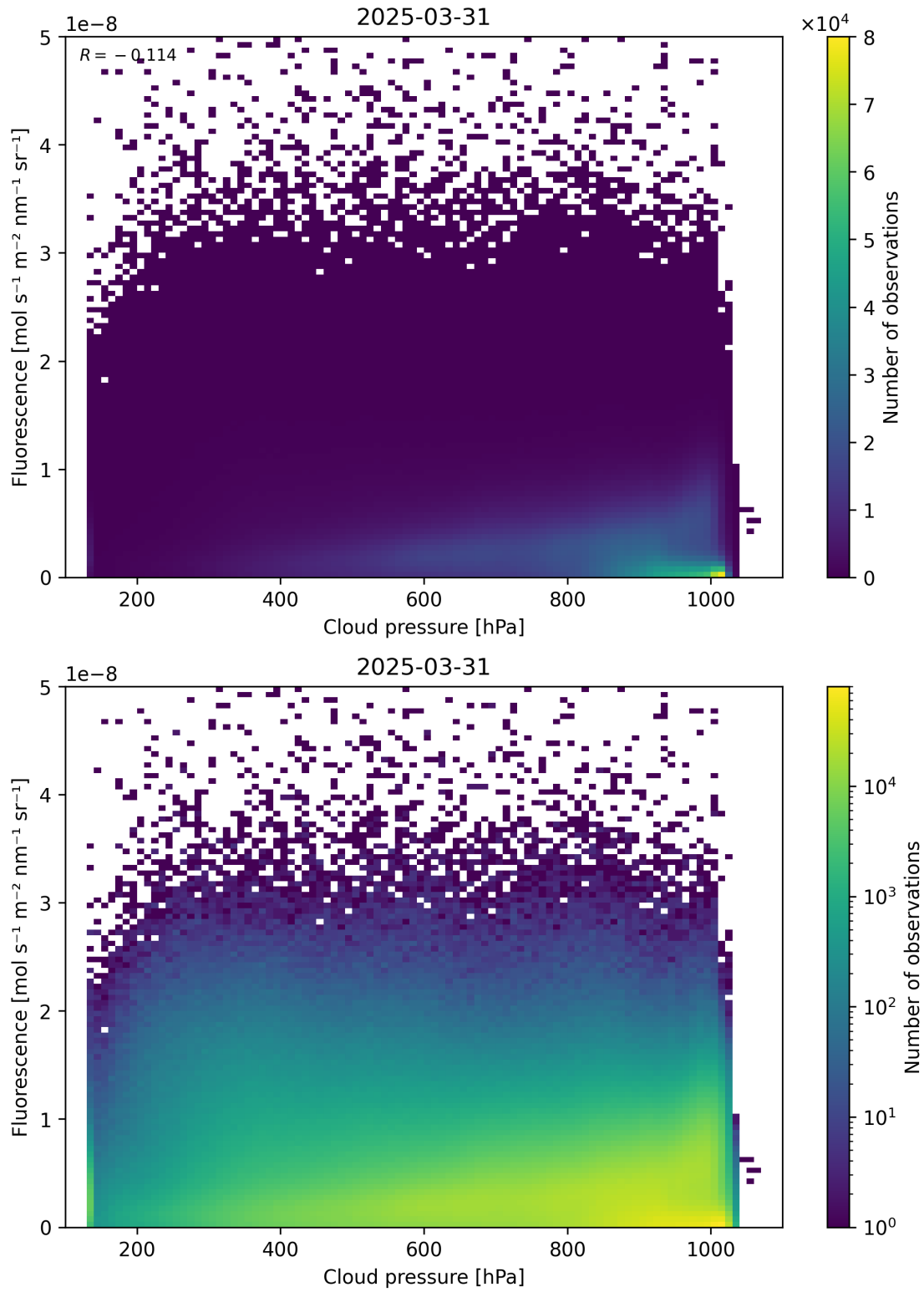
Figure 80: Scatter density plot of “Cloud pressure” against “Fluorescence” for 2025-03-30 to 2025-04-01.
