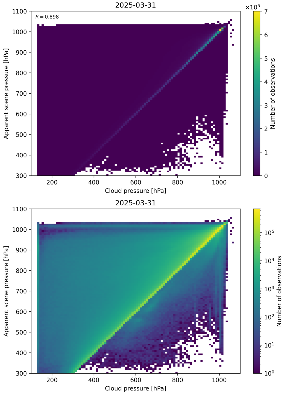
Figure 77: Scatter density plot of “Cloud pressure” against “Apparent scene pressure” for 2025-03-30 to 2025-04-01.
