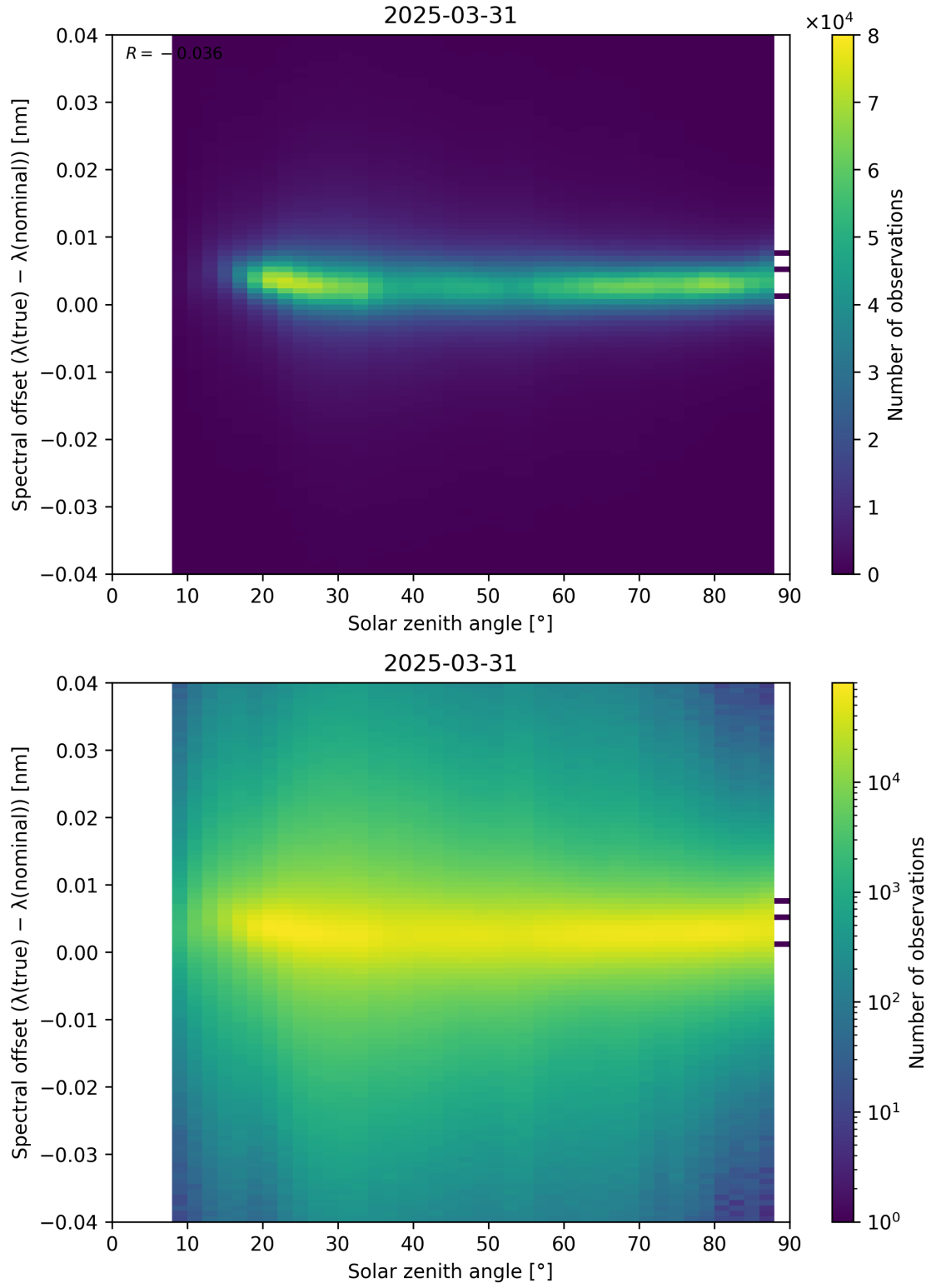
Figure 117: Scatter density plot of “Solar zenith angle” against “Spectral offset ( \lambda_{\text{true}} - \lambda_{\text{nominal}} )” for 2025-03-30 to 2025-04-01.
