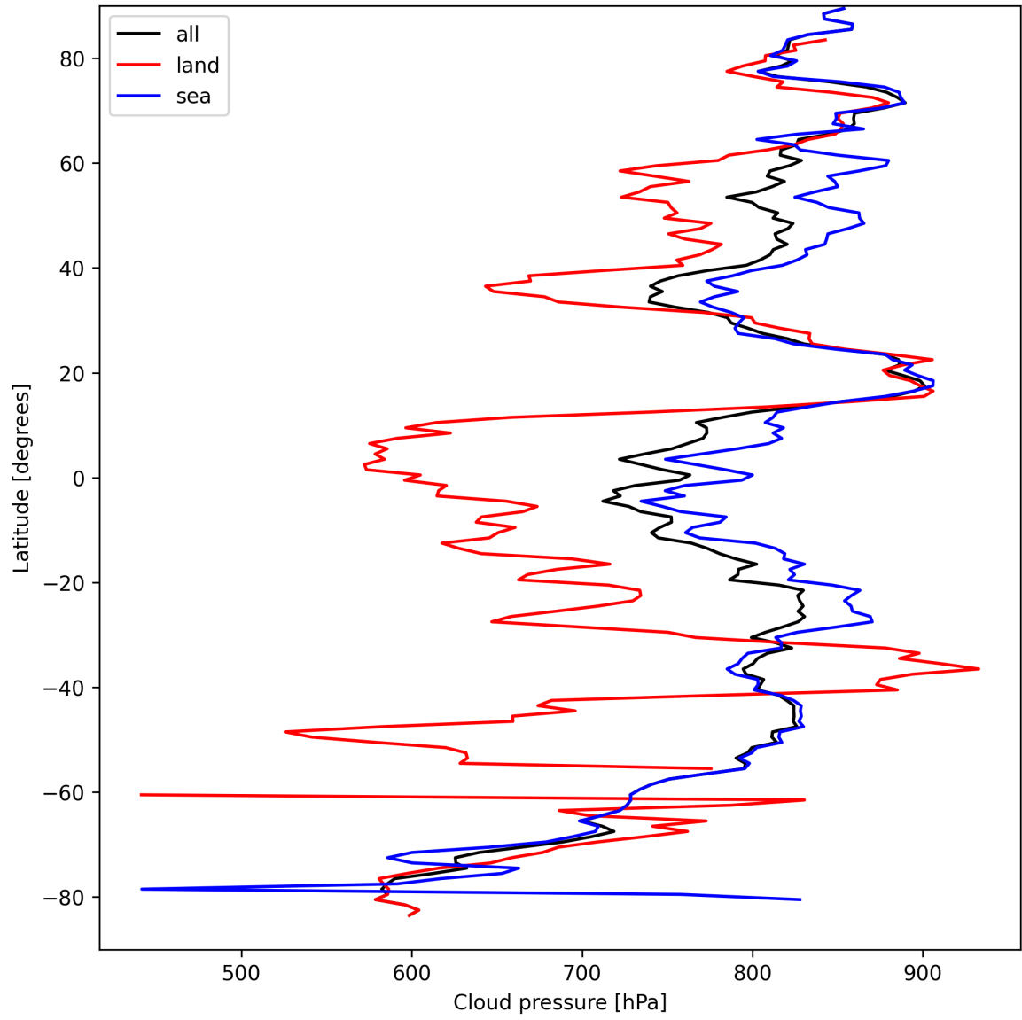
Figure 13: Zonal average of “Cloud pressure” for 2025-03-30 to 2025-04-01.
