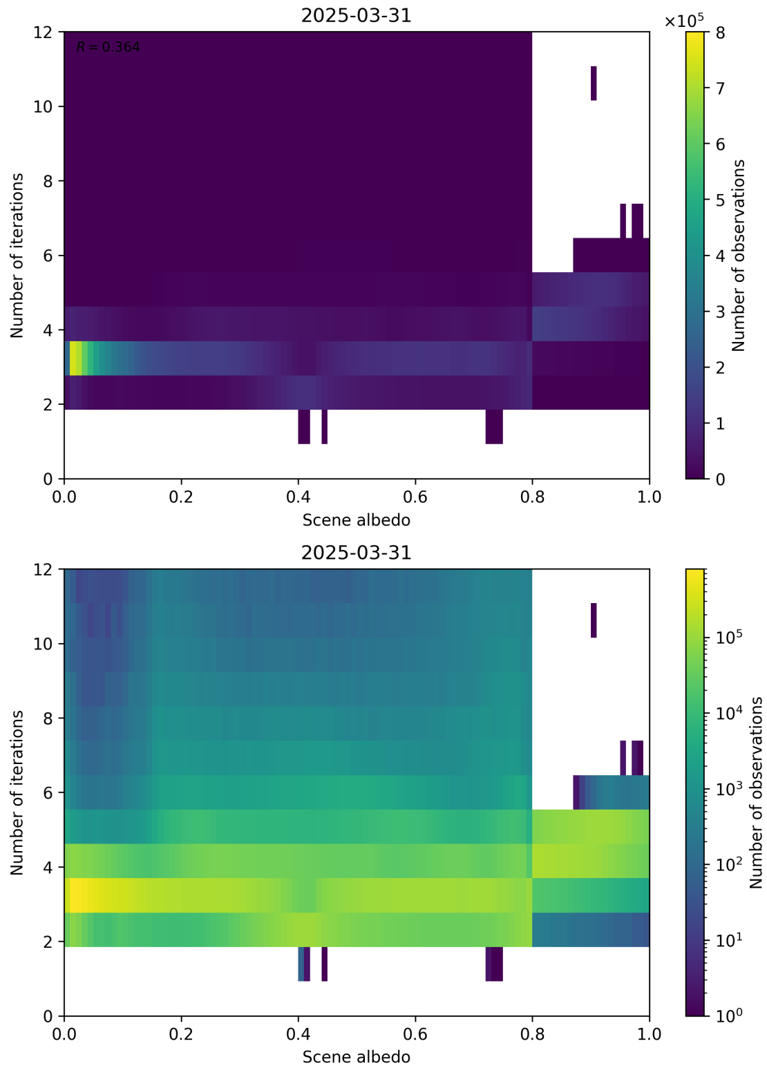
Figure 105: Scatter density plot of “Scene albedo” against “Number of iterations” for 2025-03-30 to 2025-04-01.
