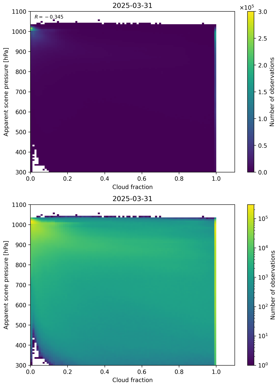
Figure 70: Scatter density plot of “Cloud fraction” against “Apparent scene pressure” for 2025-03-30 to 2025-04-01.
