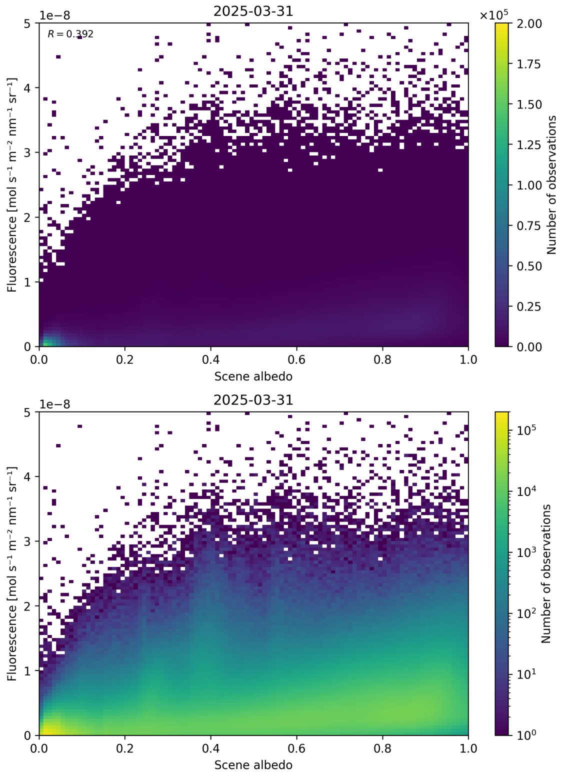
Figure 104: Scatter density plot of “Scene albedo” against “Fluorescence” for 2025-03-30 to 2025-04-01.
