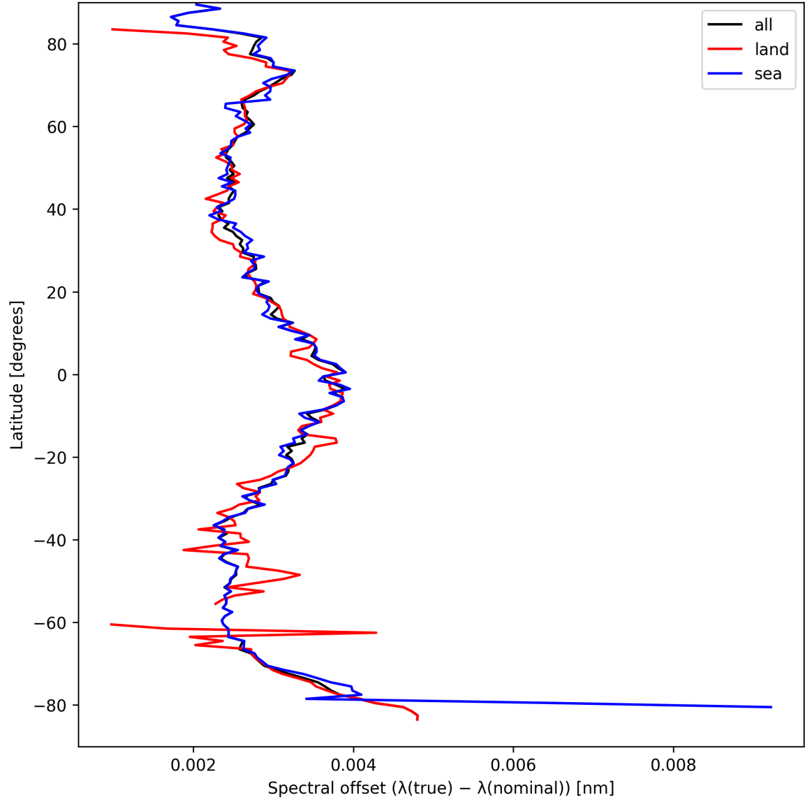
Figure 28: Zonal average of “Spectral offset ( \lambda_{\text{true}} - \lambda_{\text{nominal}} )” for 2025-03-30 to 2025-04-01.
