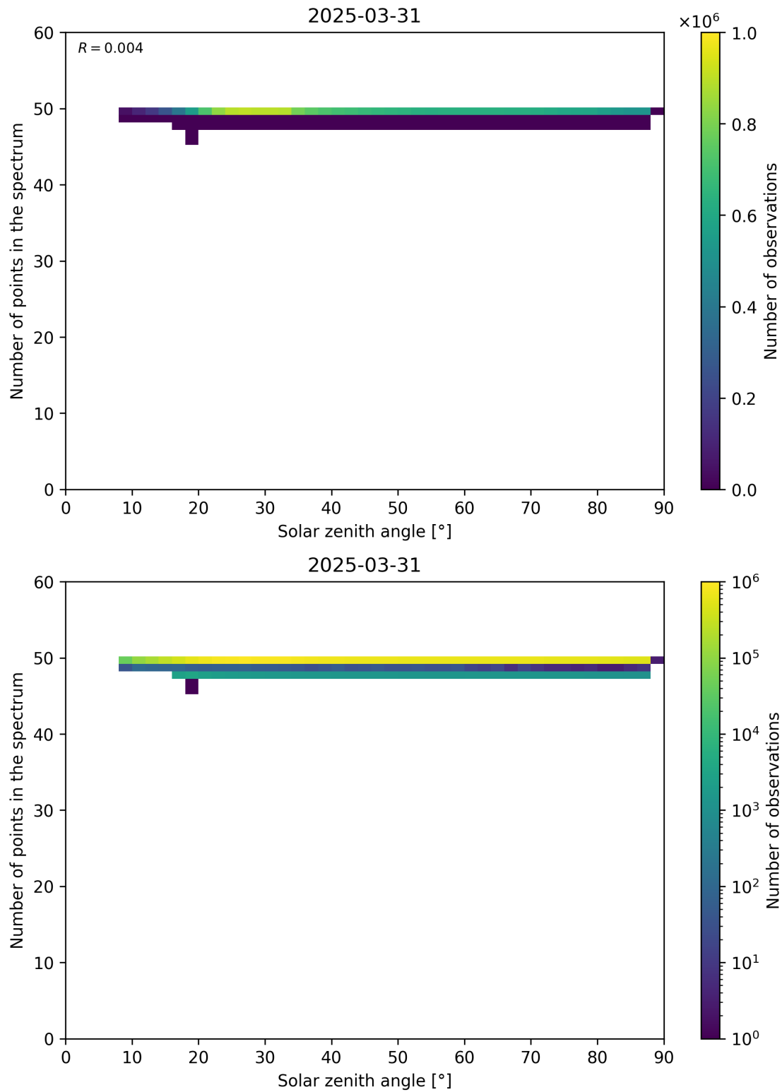
Figure 115: Scatter density plot of “Solar zenith angle” against “Number of points in the spectrum” for 2025-03-30 to 2025-04-01.
