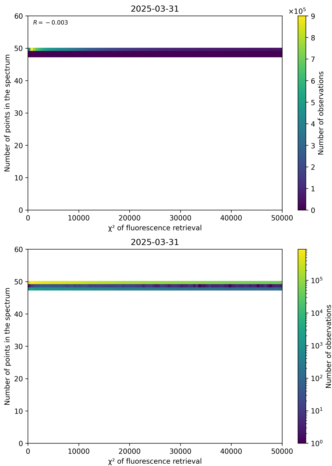
Figure 68: Scatter density plot of “ \chi^2 of fluorescence retrieval” against “Number of points in the spectrum” for 2025-03-30 to 2025-04-01.
