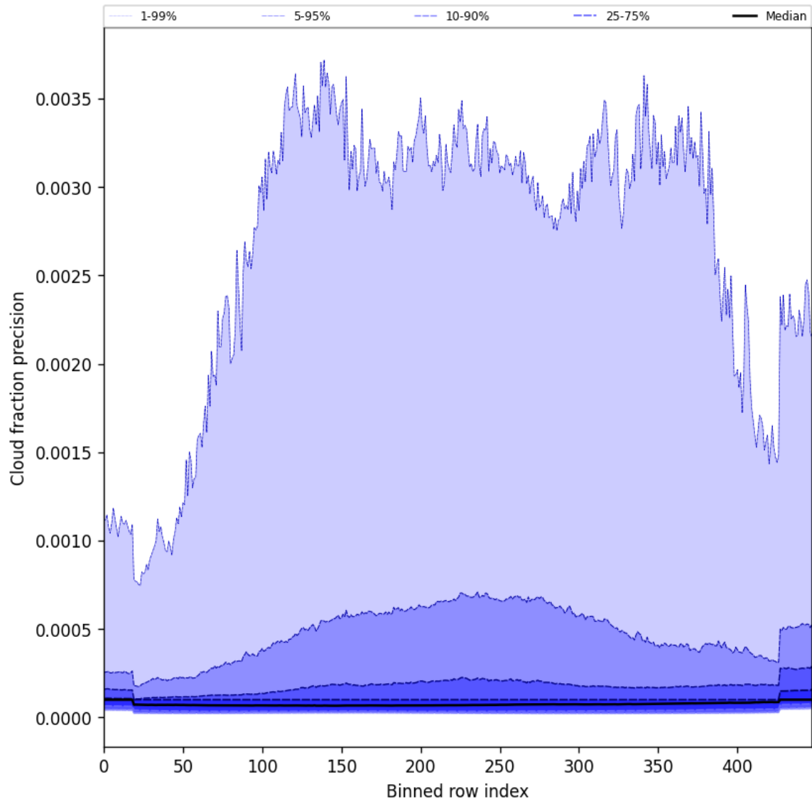
Figure 50: Along track statistics of “Cloud fraction precision” for 2025-03-30 to 2025-04-01
