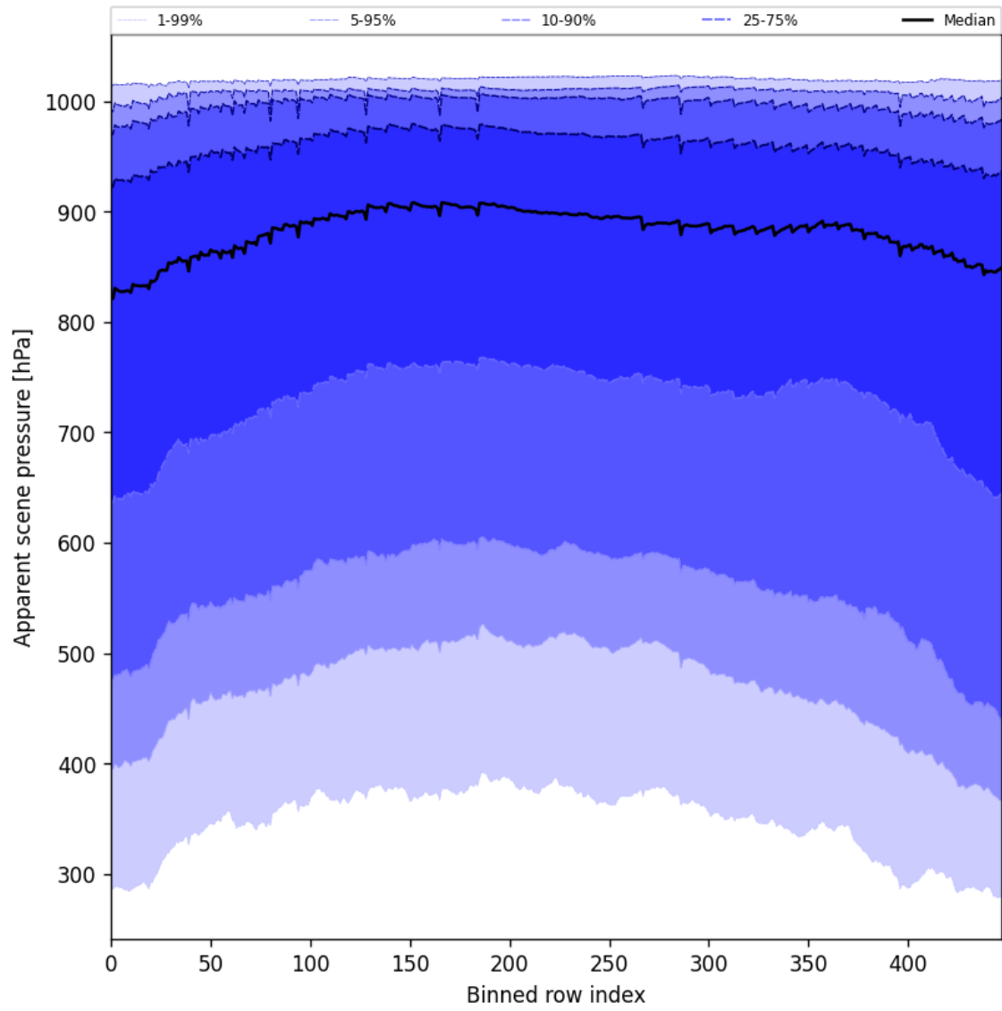
Figure 53: Along track statistics of “Apparent scene pressure” for 2025-03-30 to 2025-04-01
