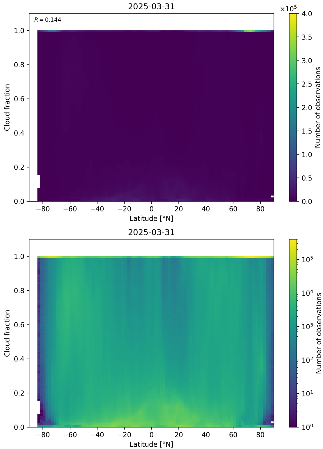
Figure 90: Scatter density plot of “Latitude” against “Cloud fraction” for 2025-03-30 to 2025-04-01.
