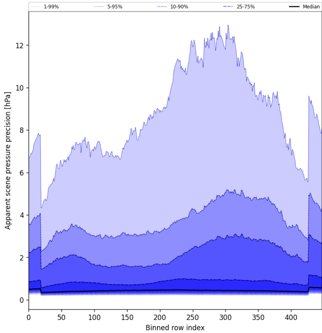
Figure 54: Along track statistics of “Apparent scene pressure precision” for 2025-03-30 to 2025-04-01
