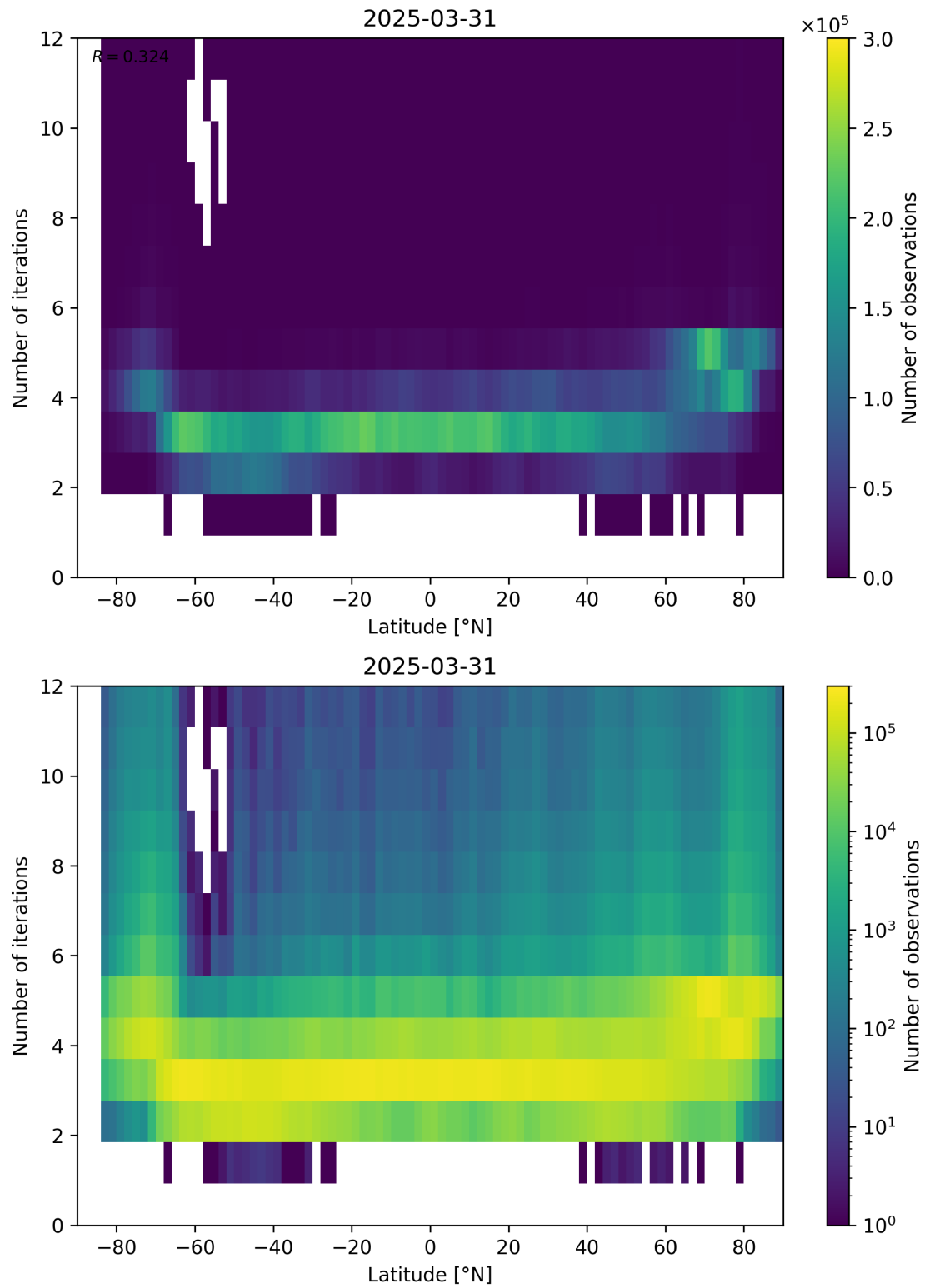
Figure 93: Scatter density plot of “Latitude” against “Number of iterations” for 2025-03-30 to 2025-04-01.
