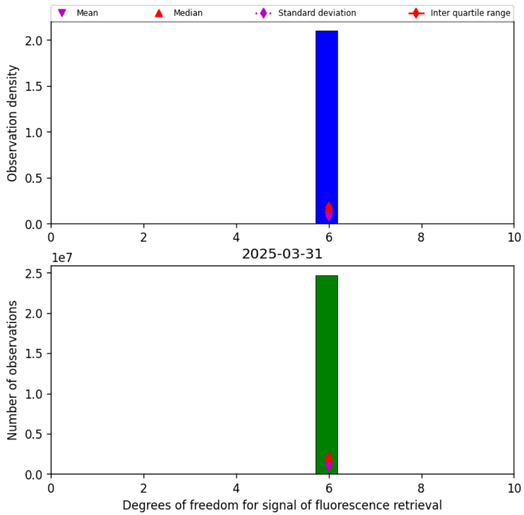
Figure 43: Histogram of “Degrees of freedom for signal of fluorescence retrieval” for 2025-03-30 to 2025-04-01
