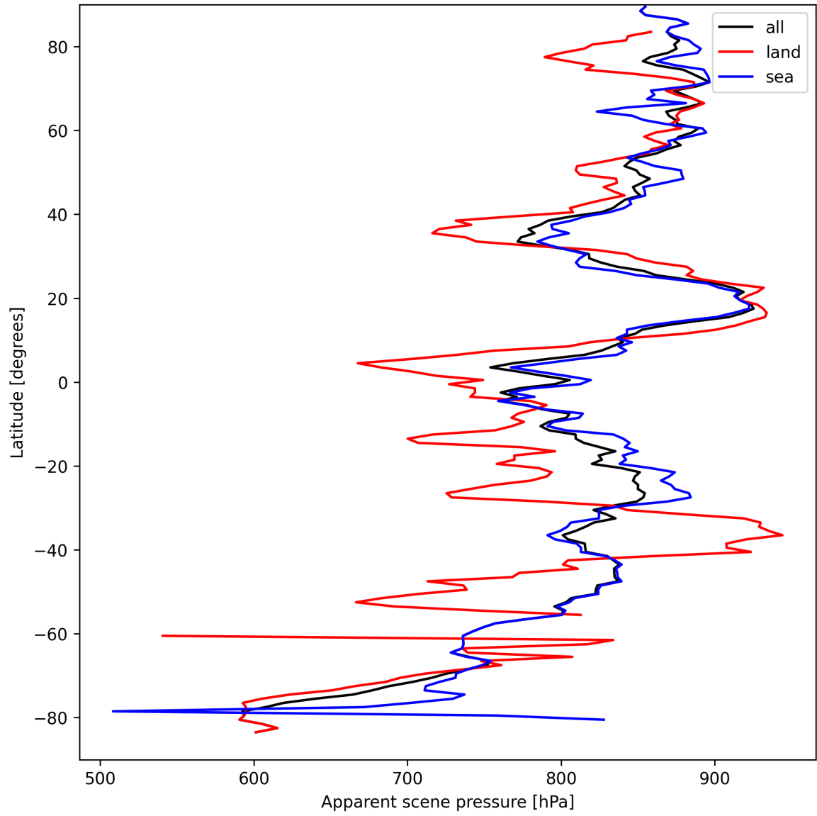
Figure 19: Zonal average of “Apparent scene pressure” for 2025-03-30 to 2025-04-01.
