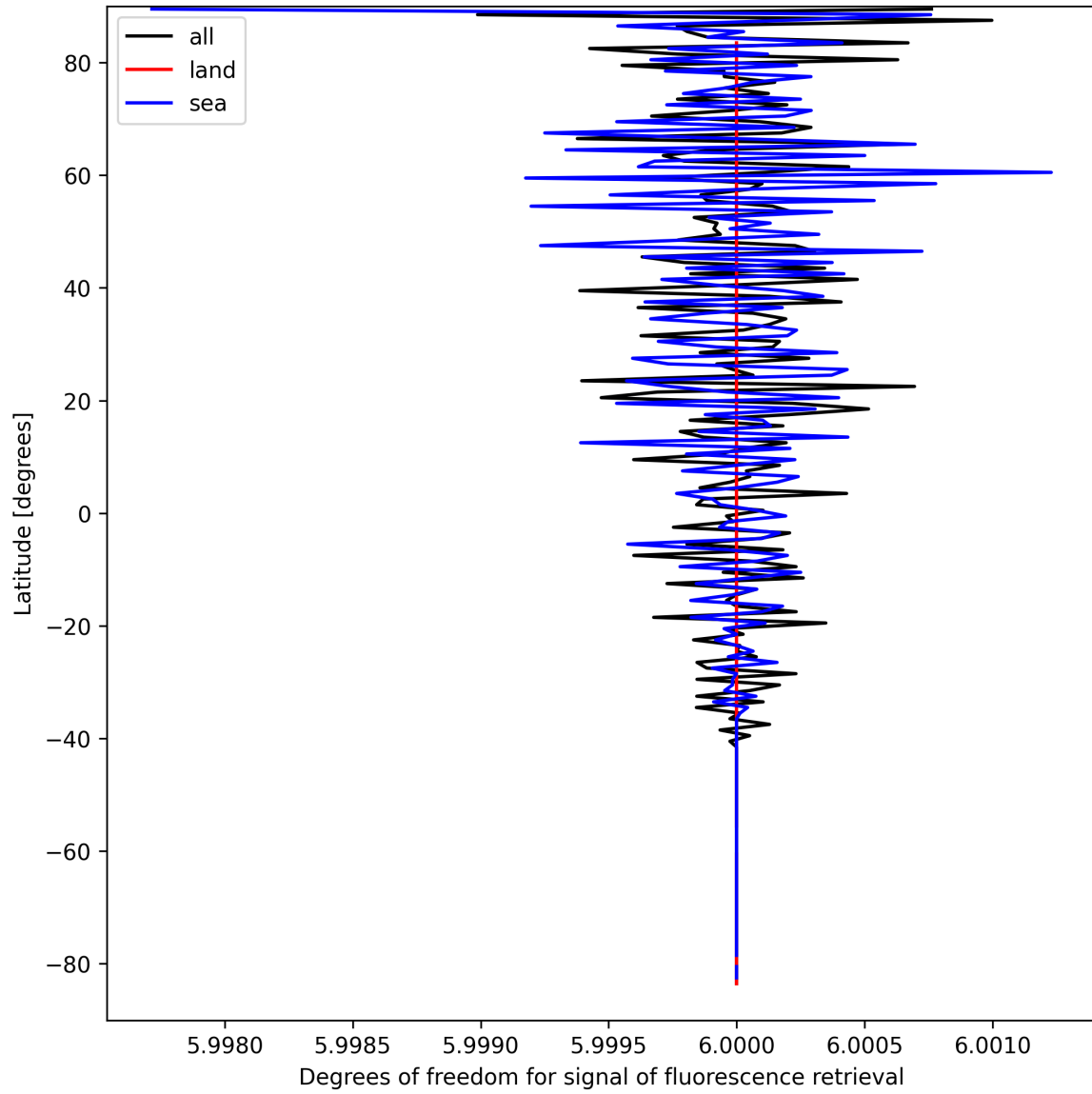
Figure 26: Zonal average of “Degrees of freedom for signal of fluorescence retrieval” for 2025-03-31 to 2025-04-02.
