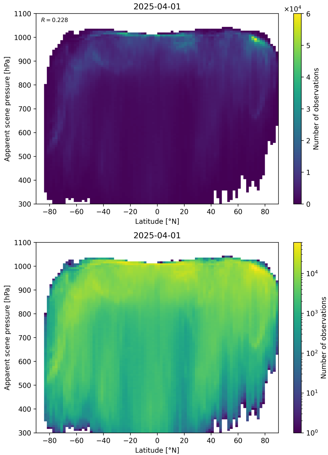
Figure 88: Scatter density plot of “Latitude” against “Apparent scene pressure” for 2025-03-31 to 2025-04-02.
