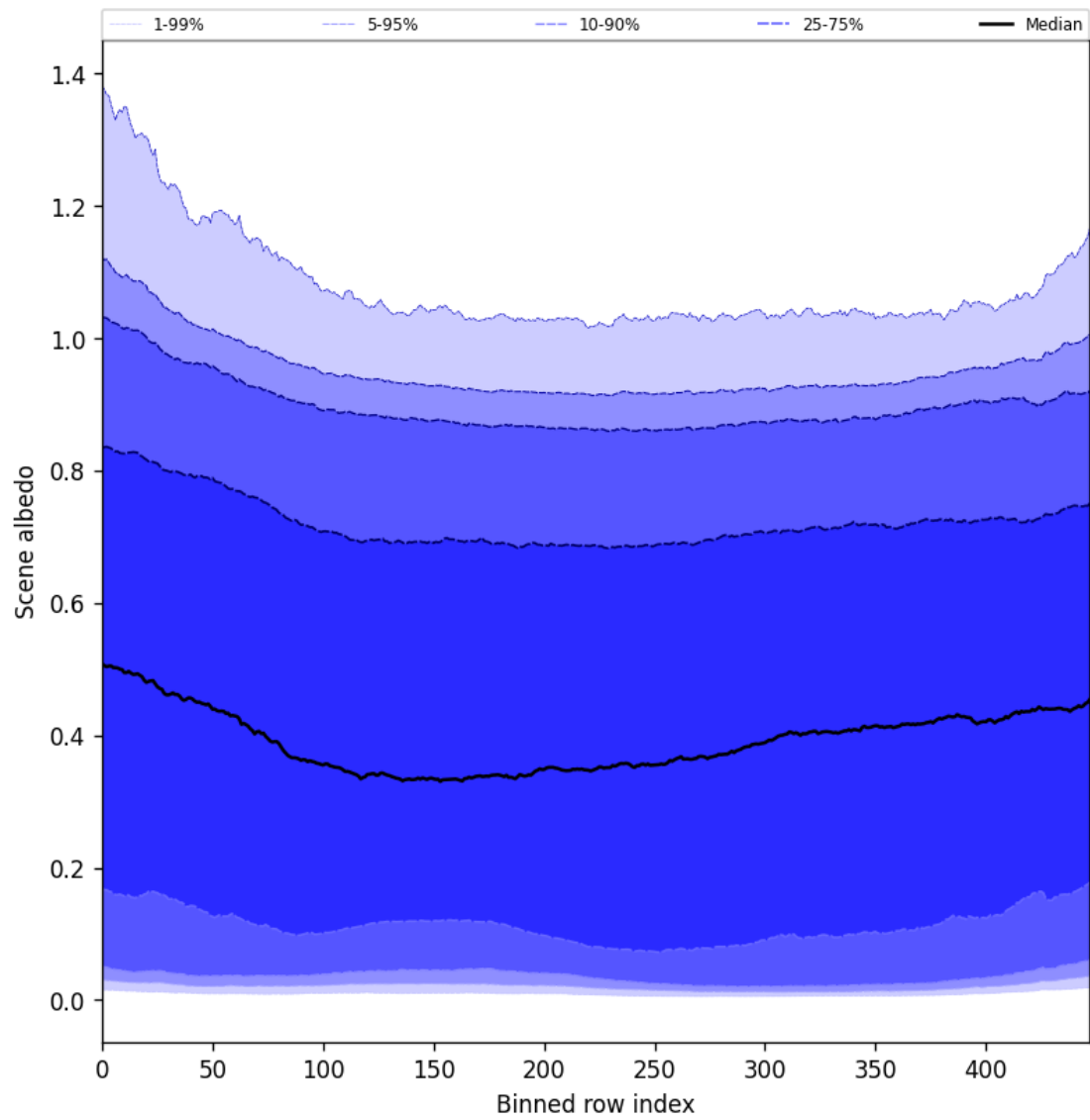
Figure 51: Along track statistics of “Scene albedo” for 2025-03-31 to 2025-04-02
