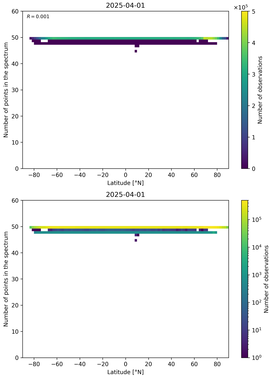
Figure 94: Scatter density plot of “Latitude” against “Number of points in the spectrum” for 2025-03-31 to 2025-04-02.
