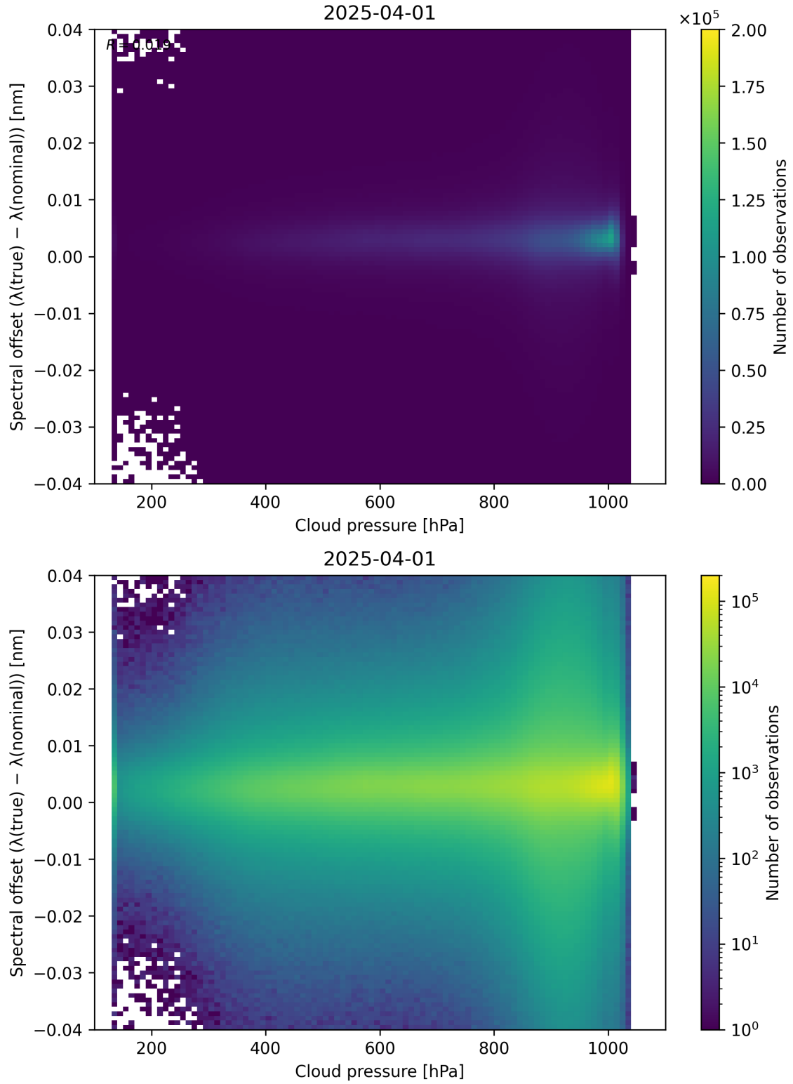
Figure 84: Scatter density plot of “Cloud pressure” against “Spectral offset ( \lambda_{\text{true}} - \lambda_{\text{nominal}} )” for 2025-03-31 to 2025-04-02.
