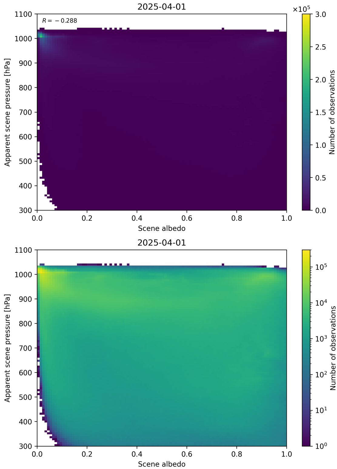
Figure 102: Scatter density plot of “Scene albedo” against “Apparent scene pressure” for 2025-03-31 to 2025-04-02.
