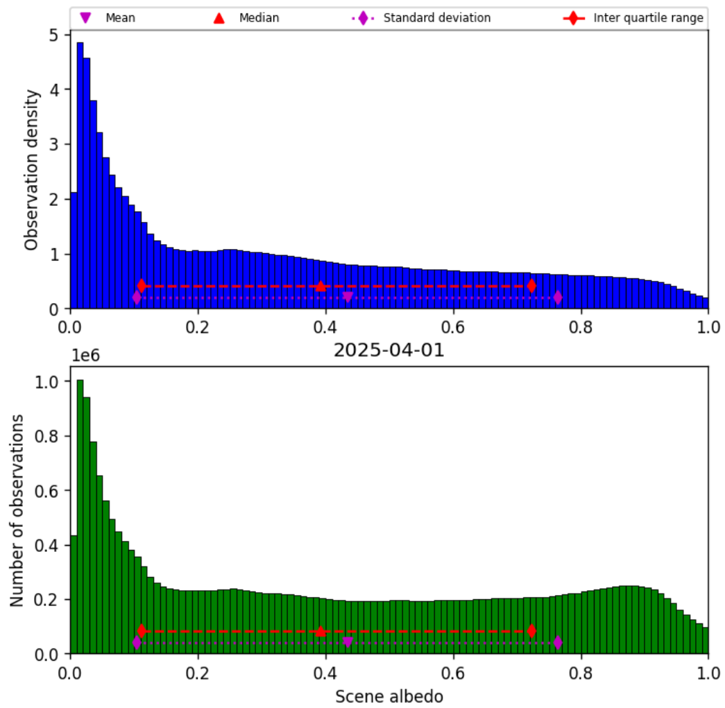
Figure 34: Histogram of “Scene albedo” for 2025-03-31 to 2025-04-02
