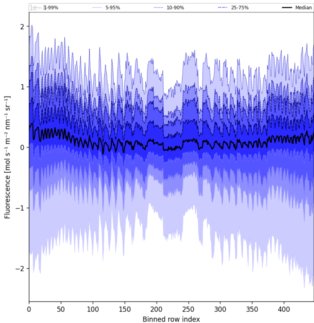
Figure 57: Along track statistics of “Fluorescence” for 2025-03-31 to 2025-04-02
