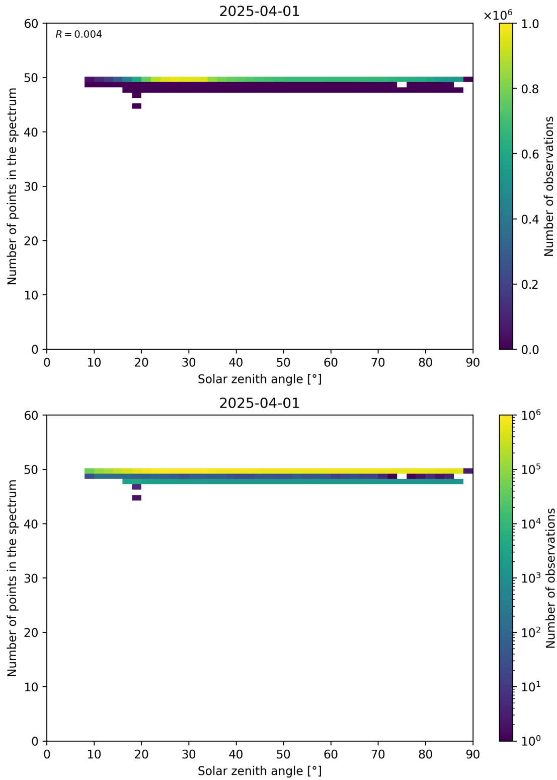
Figure 115: Scatter density plot of “Solar zenith angle” against “Number of points in the spectrum” for 2025-03-31 to 2025-04-02.
