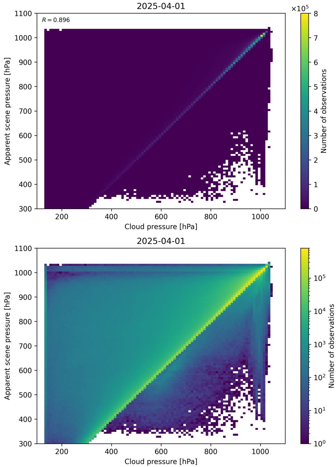
Figure 77: Scatter density plot of “Cloud pressure” against “Apparent scene pressure” for 2025-03-31 to 2025-04-02.
