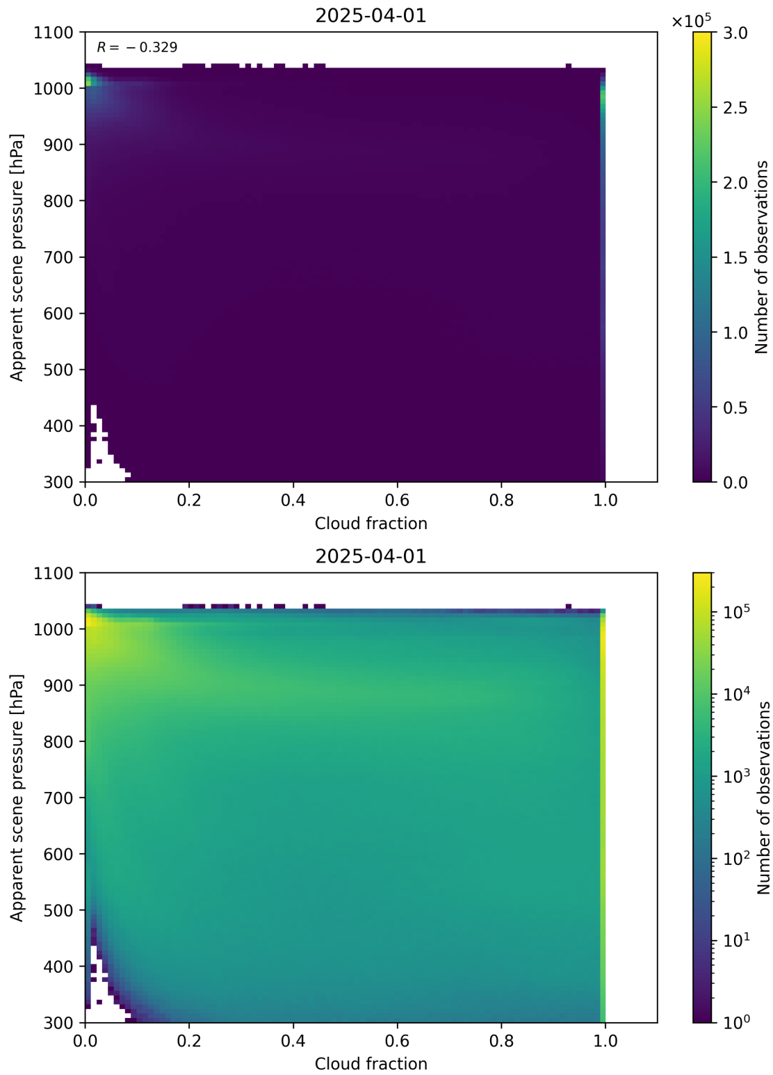
Figure 70: Scatter density plot of “Cloud fraction” against “Apparent scene pressure” for 2025-03-31 to 2025-04-02.
