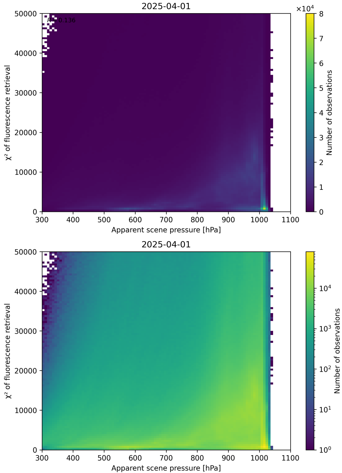
Figure 63: Scatter density plot of “Apparent scene pressure” against “ \chi^2 of fluorescence retrieval” for 2025-03-31 to 2025-04-02.
