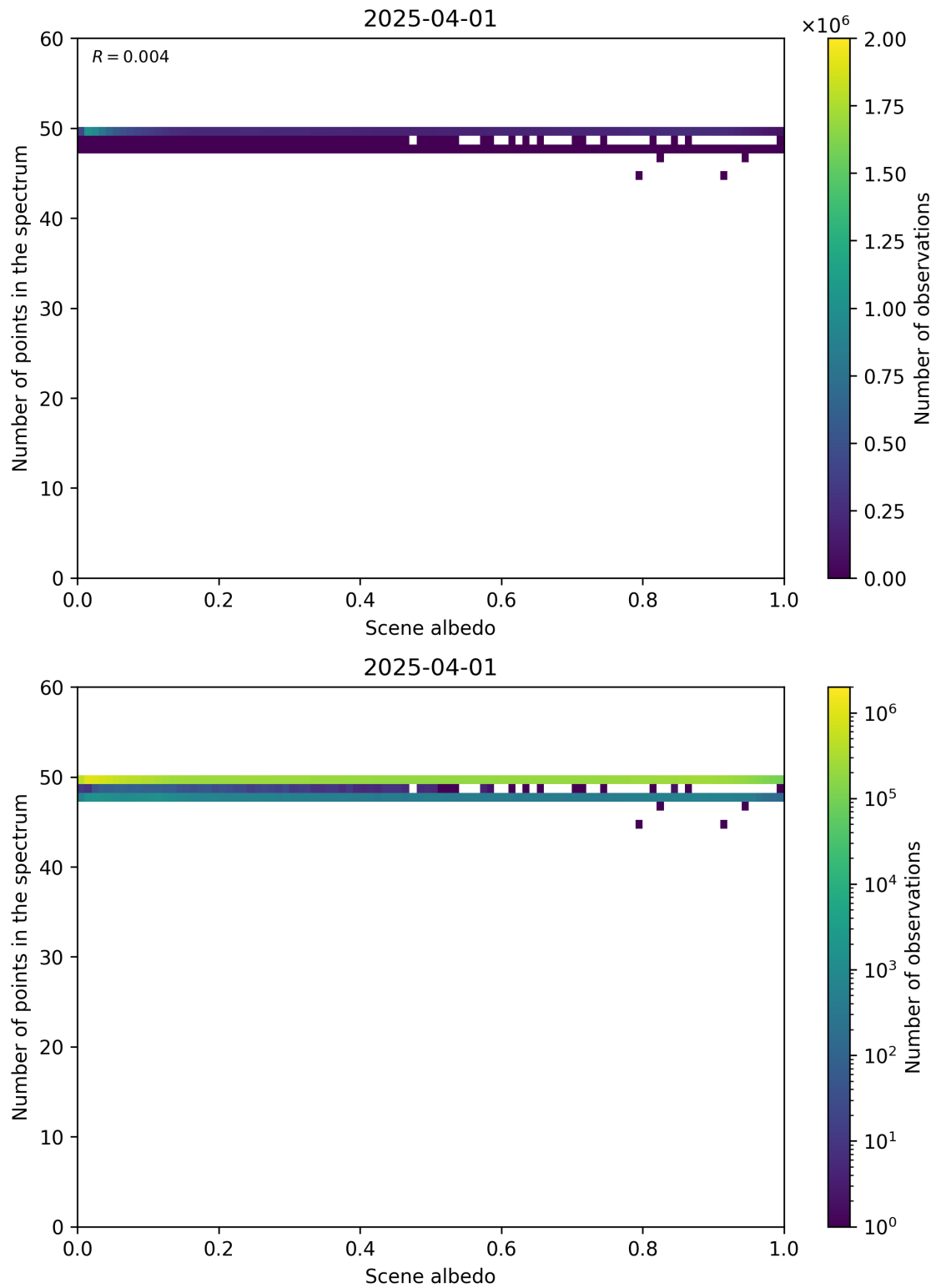
Figure 106: Scatter density plot of “Scene albedo” against “Number of points in the spectrum” for 2025-03-31 to 2025-04-02.
