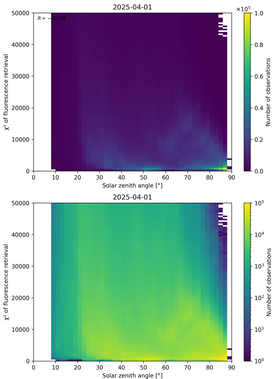
Figure 109: Scatter density plot of “Solar zenith angle” against “ \chi^2 of fluorescence retrieval” for 2025-03-31 to 2025-04-02.
