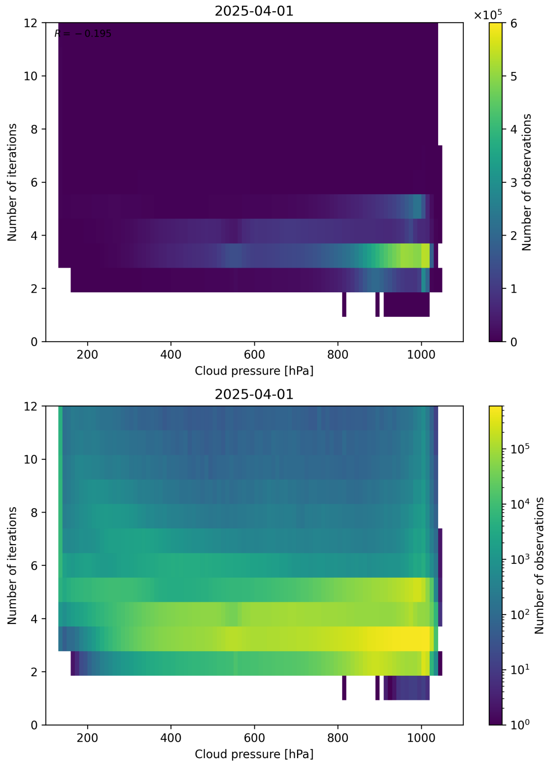
Figure 81: Scatter density plot of “Cloud pressure” against “Number of iterations” for 2025-03-31 to 2025-04-02.
