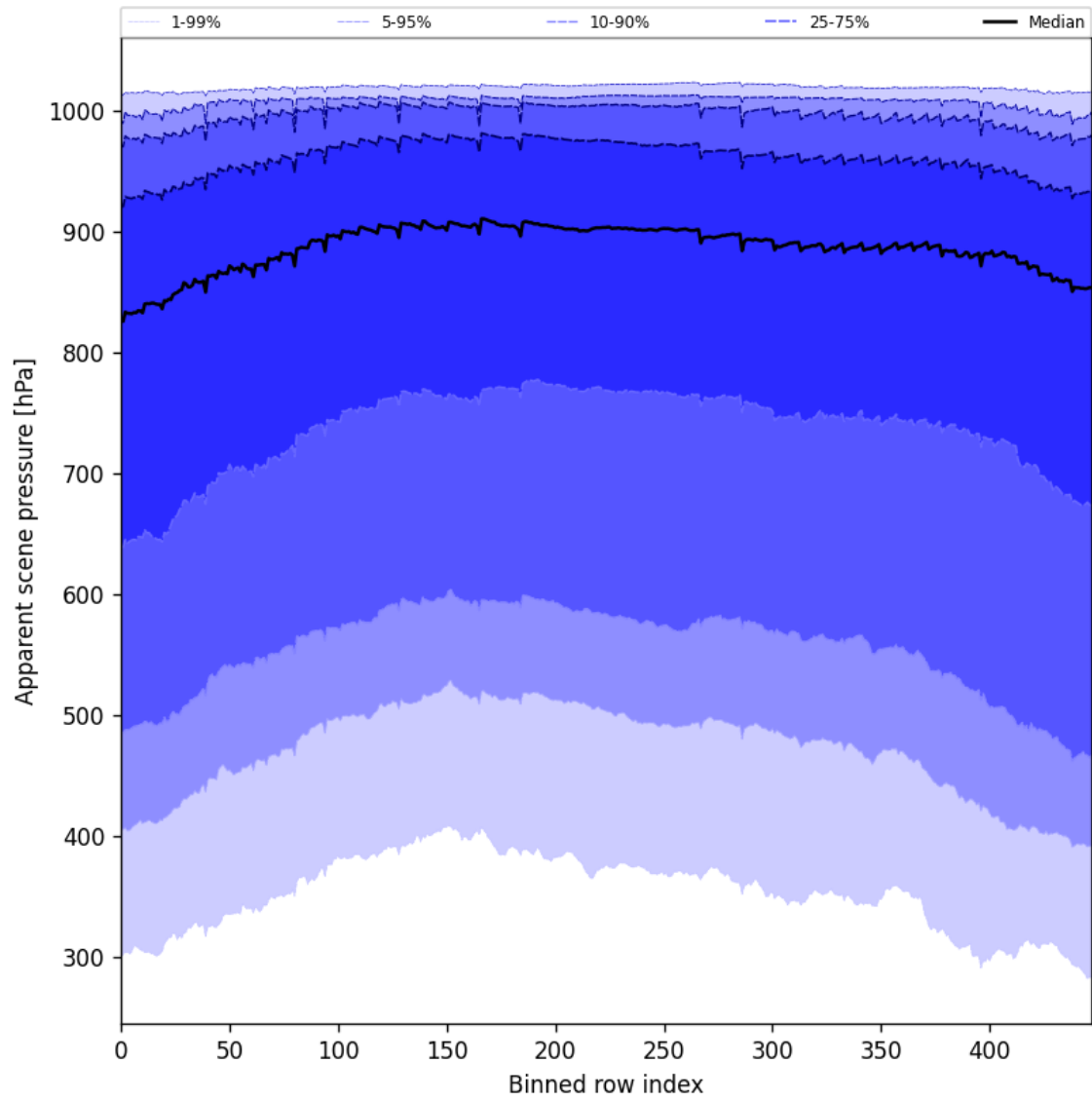
Figure 53: Along track statistics of “Apparent scene pressure” for 2025-03-31 to 2025-04-02
