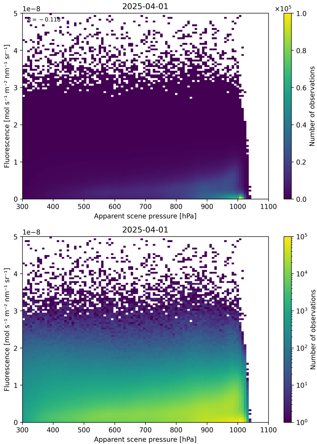
Figure 64: Scatter density plot of “Apparent scene pressure” against “Fluorescence” for 2025-03-31 to 2025-04-02.
