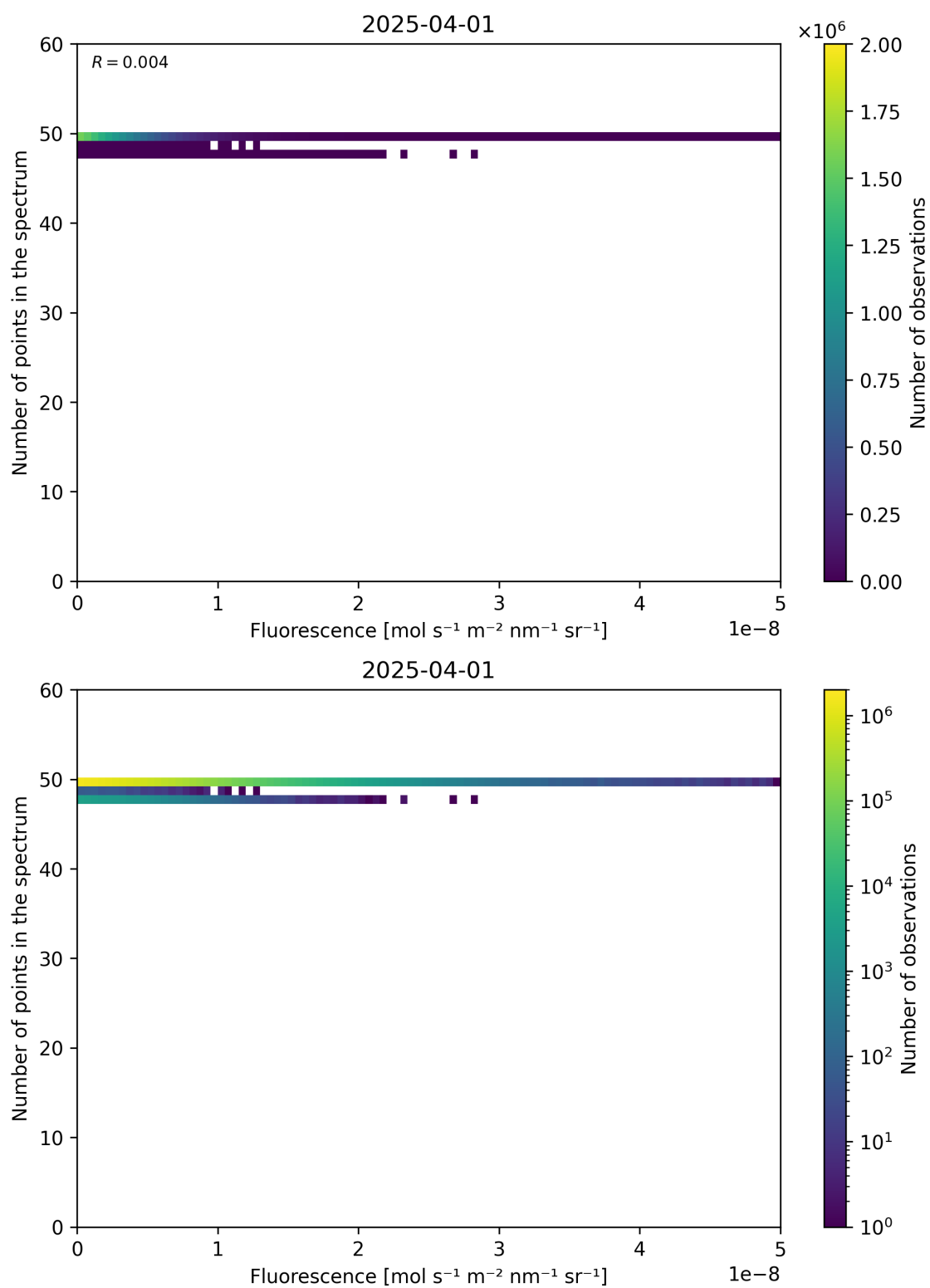
Figure 86: Scatter density plot of “Fluorescence” against “Number of points in the spectrum” for 2025-03-31 to 2025-04-02.
