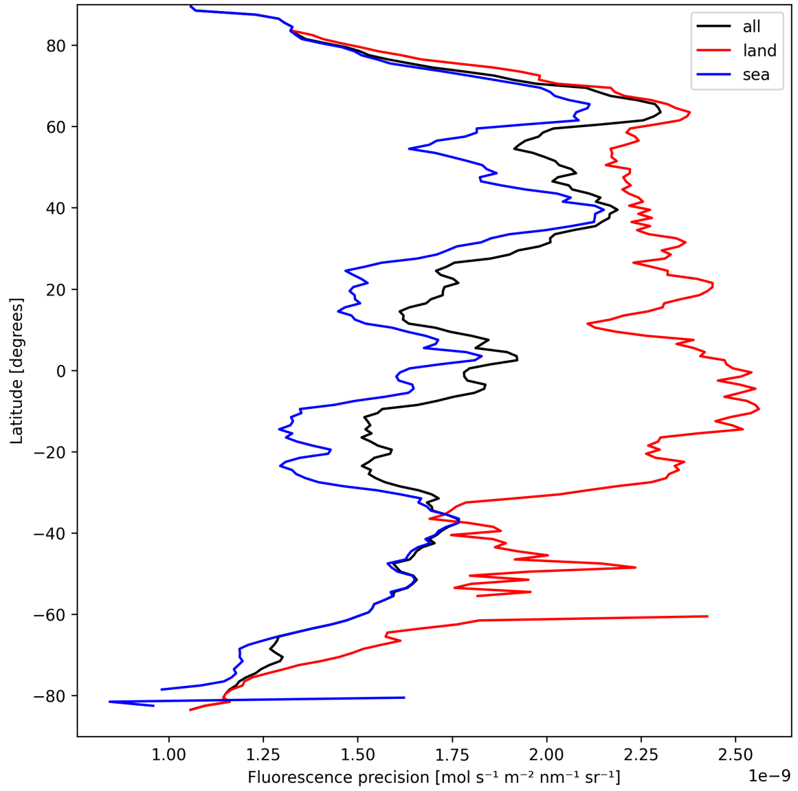
Figure 24: Zonal average of “Fluorescence precision” for 2025-03-31 to 2025-04-02.
