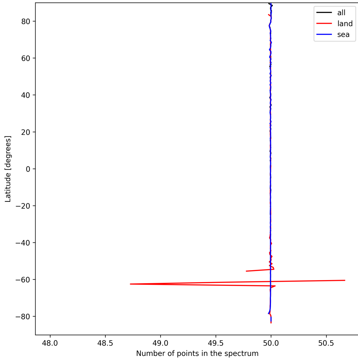
Figure 27: Zonal average of “Number of points in the spectrum” for 2025-03-31 to 2025-04-02.
