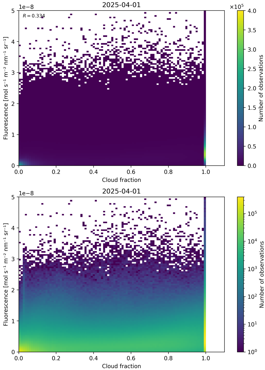
Figure 72: Scatter density plot of “Cloud fraction” against “Fluorescence” for 2025-03-31 to 2025-04-02.
