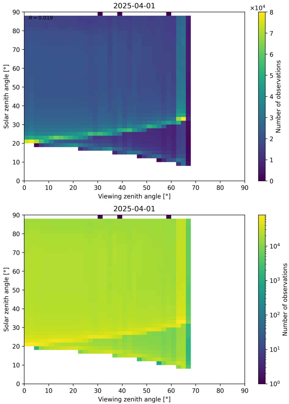
Figure 127: Scatter density plot of “Viewing zenith angle” against “Solar zenith angle” for 2025-03-31 to 2025-04-02.
