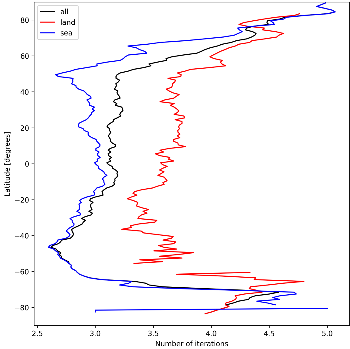
Figure 22: Zonal average of “Number of iterations” for 2025-03-31 to 2025-04-02.
