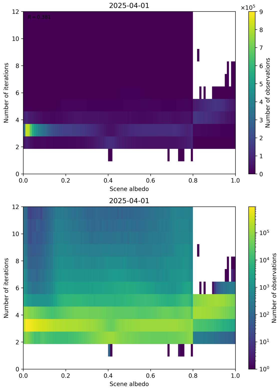
Figure 105: Scatter density plot of “Scene albedo” against “Number of iterations” for 2025-03-31 to 2025-04-02.
