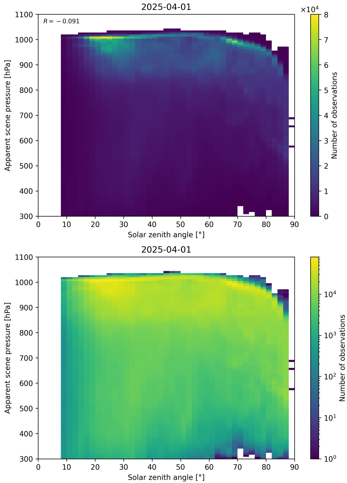
Figure 108: Scatter density plot of “Solar zenith angle” against “Apparent scene pressure” for 2025-03-31 to 2025-04-02.
