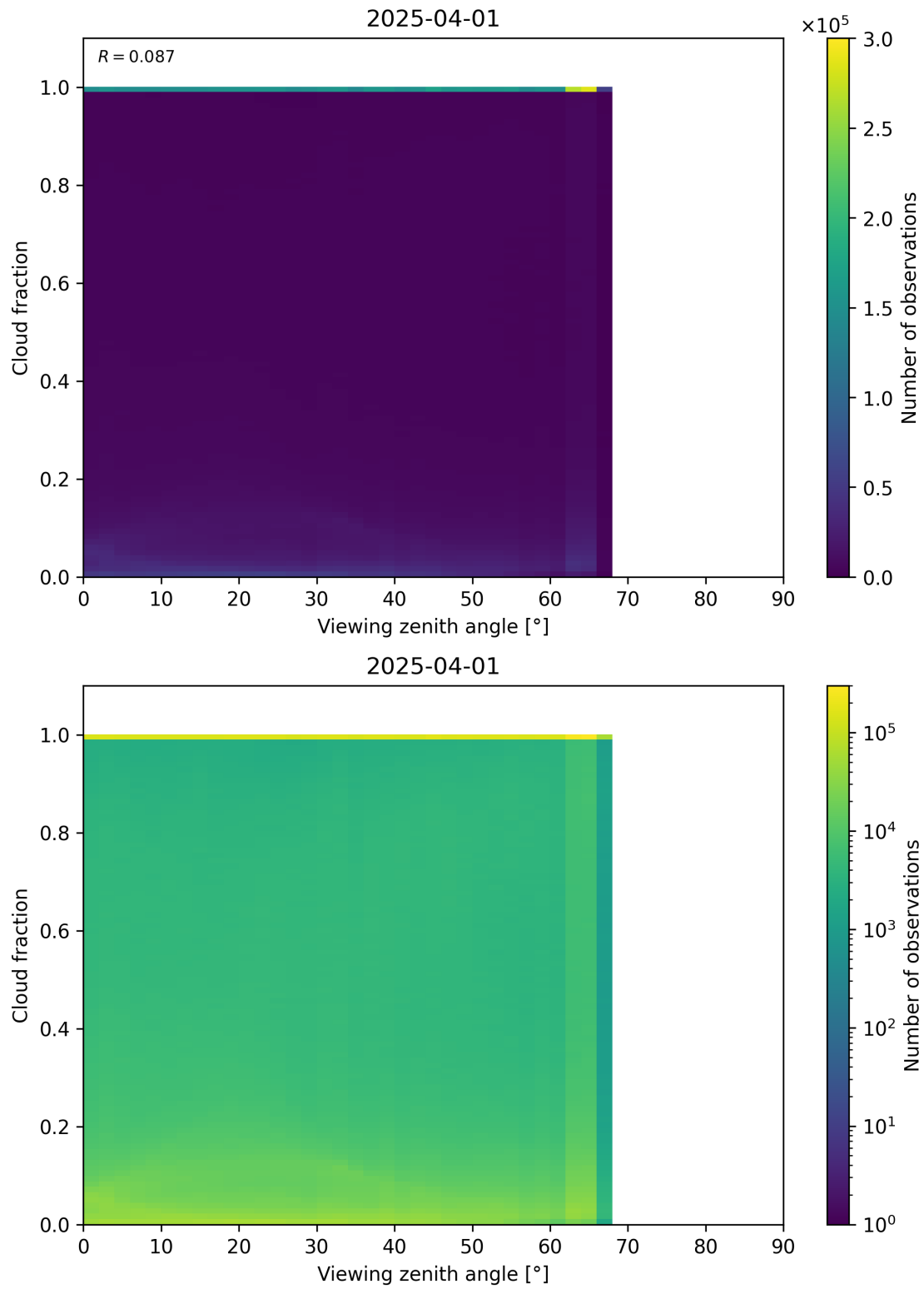
Figure 120: Scatter density plot of “Viewing zenith angle” against “Cloud fraction” for 2025-03-31 to 2025-04-02.
