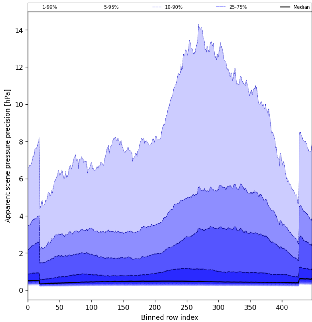
Figure 54: Along track statistics of “Apparent scene pressure precision” for 2025-03-31 to 2025-04-02
