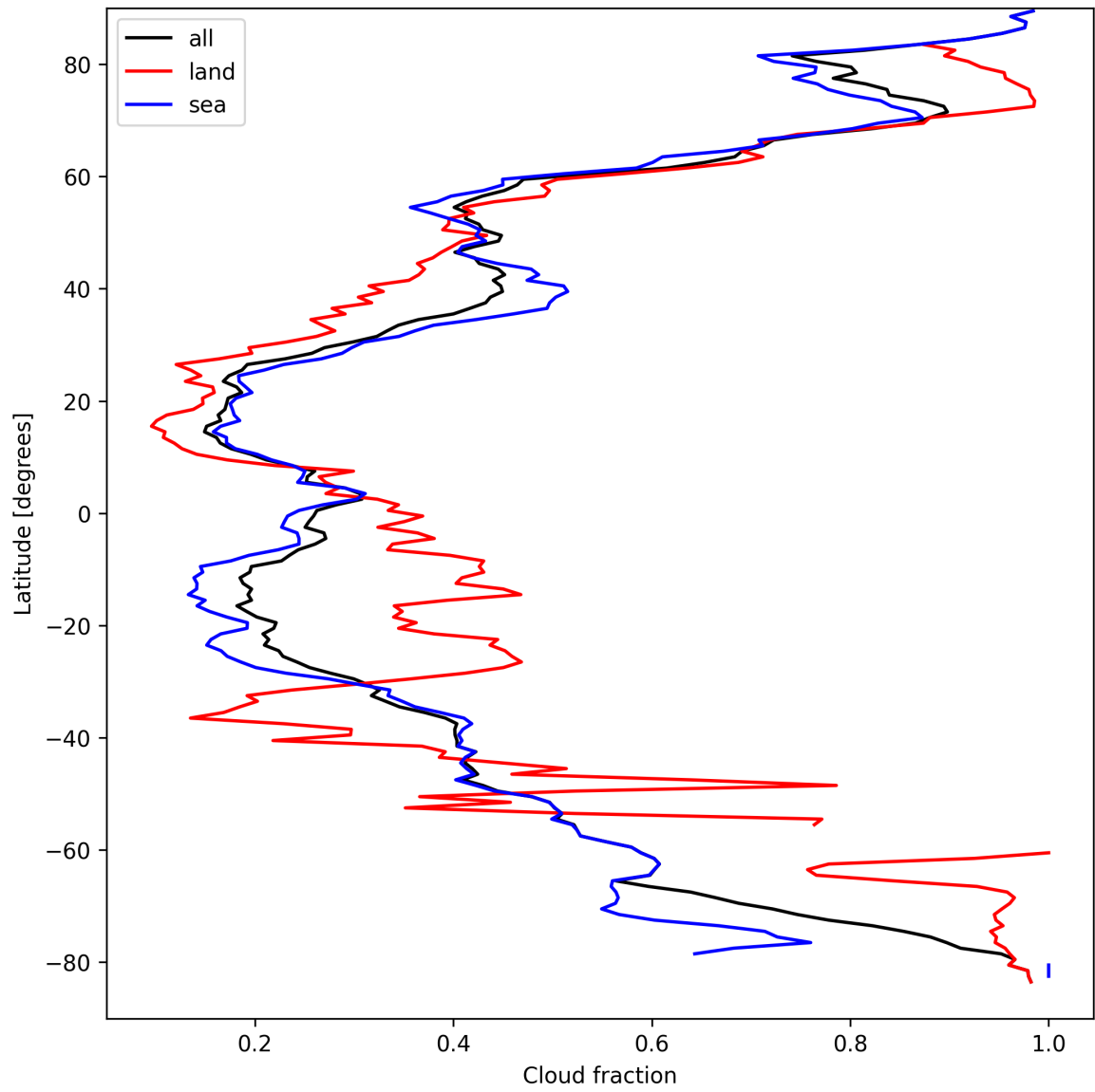
Figure 15: Zonal average of “Cloud fraction” for 2025-03-31 to 2025-04-02.
