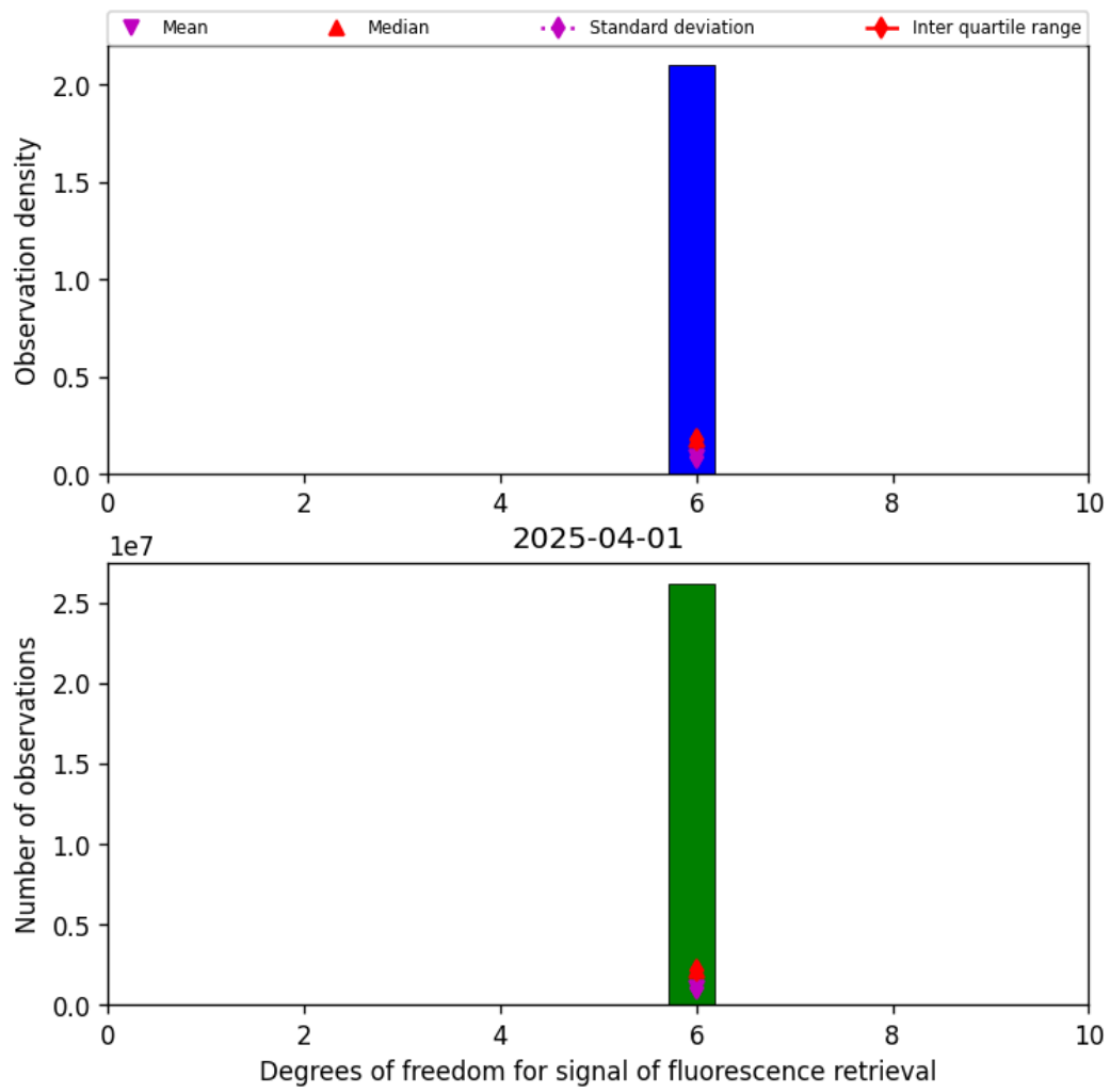
Figure 43: Histogram of "Degrees of freedom for signal of fluorescence retrieval" for 2025-03-31 to 2025-04-02
