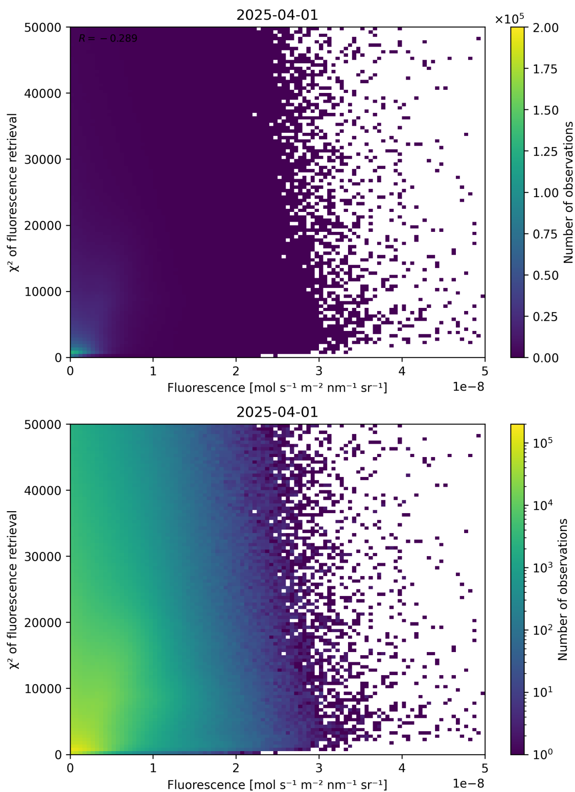
Figure 85: Scatter density plot of “Fluorescence” against “ \chi^2 of fluorescence retrieval” for 2025-03-31 to 2025-04-02.
