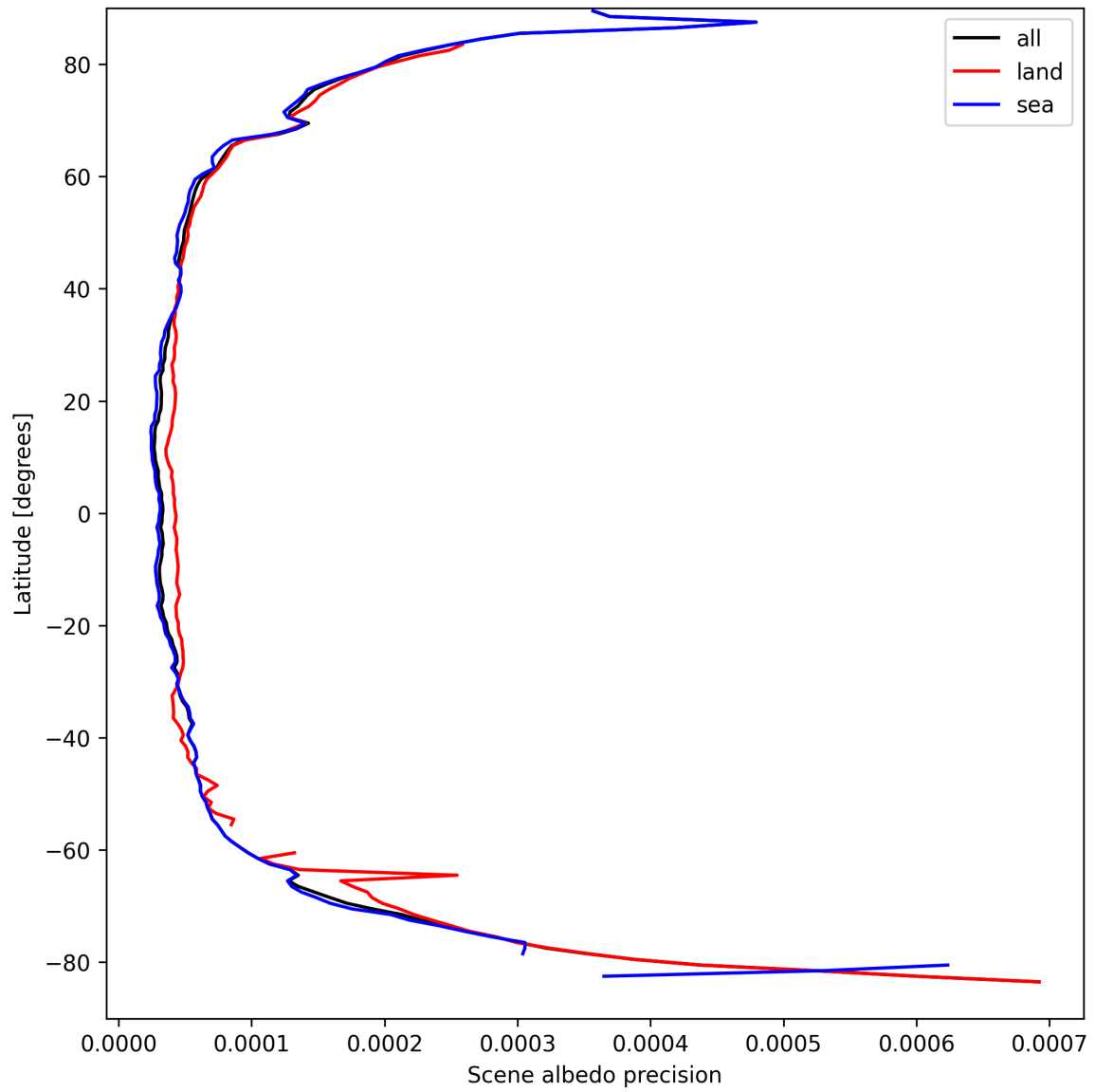
Figure 18: Zonal average of “Scene albedo precision” for 2025-03-31 to 2025-04-02.
