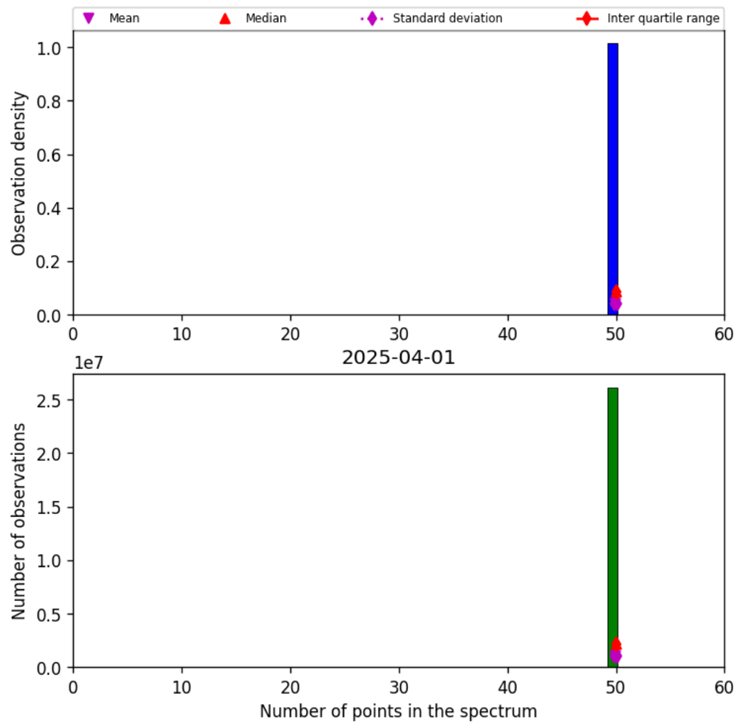
Figure 44: Histogram of “Number of points in the spectrum” for 2025-03-31 to 2025-04-02
