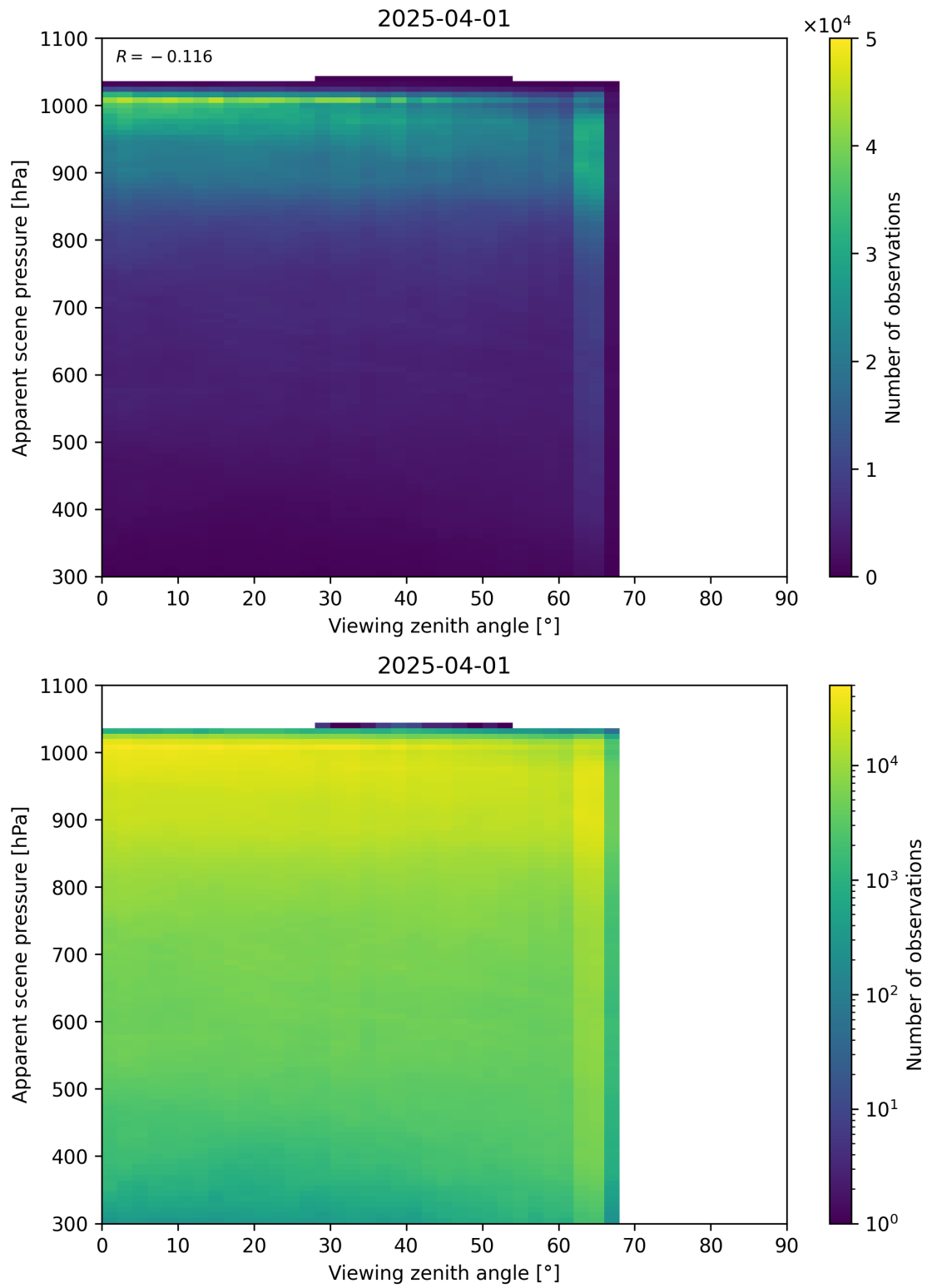
Figure 118: Scatter density plot of “Viewing zenith angle” against “Apparent scene pressure” for 2025-03-31 to 2025-04-02.
