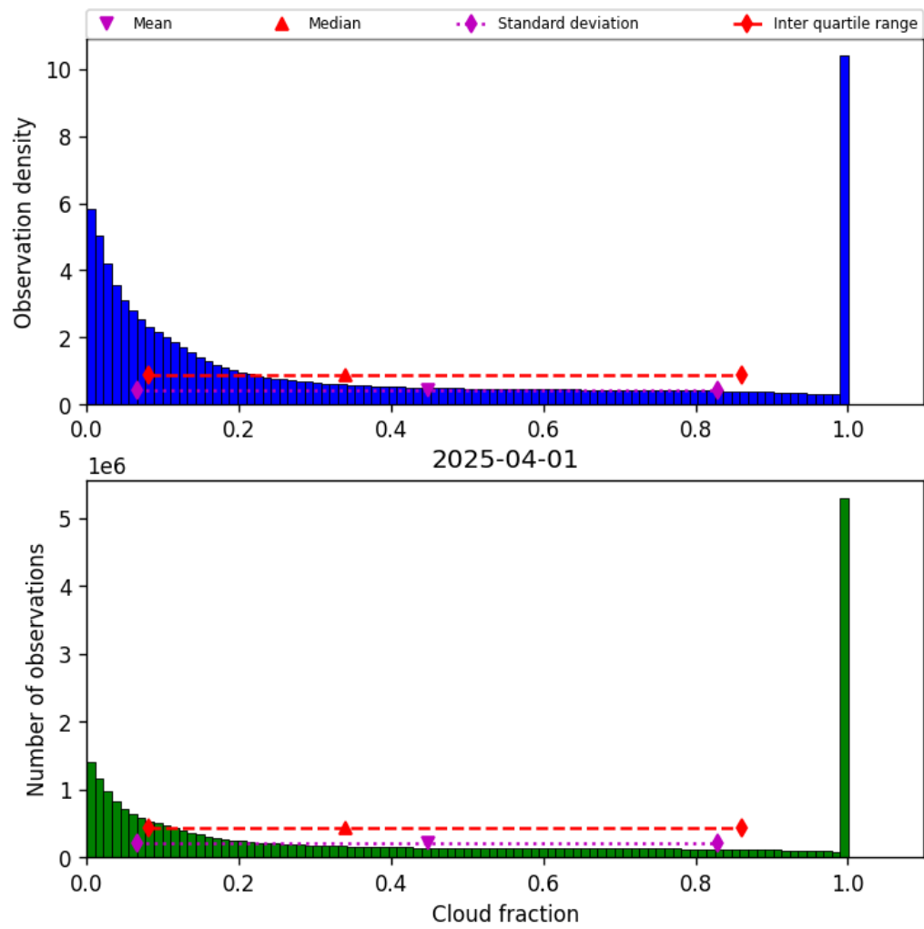
Figure 32: Histogram of “Cloud fraction” for 2025-03-31 to 2025-04-02
