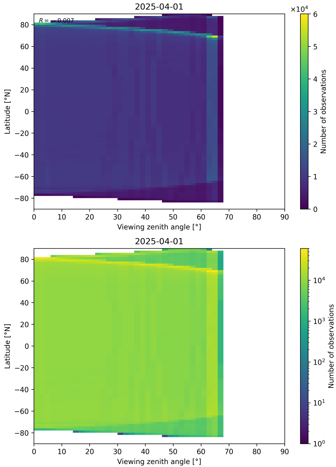
Figure 123: Scatter density plot of “Viewing zenith angle” against “Latitude” for 2025-03-31 to 2025-04-02.
