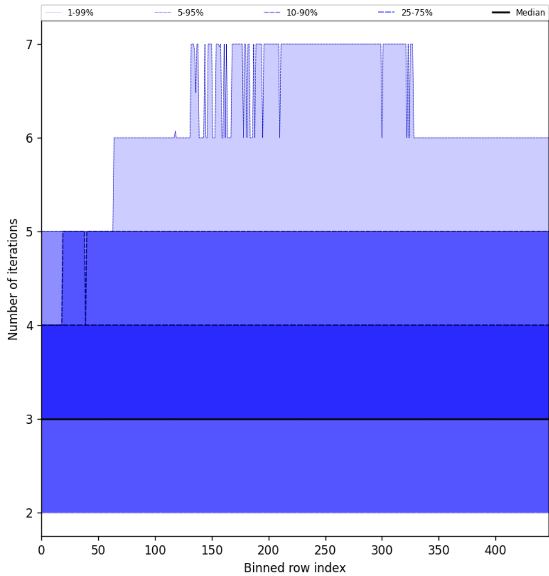
Figure 56: Along track statistics of “Number of iterations” for 2025-03-31 to 2025-04-02
