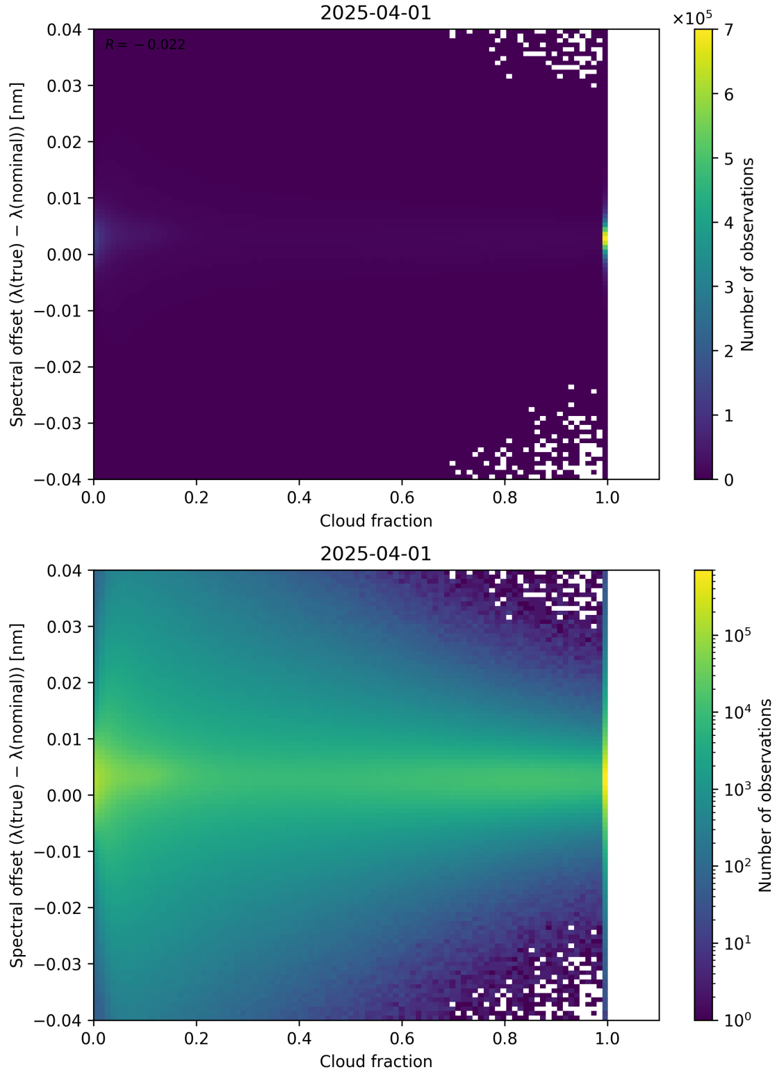
Figure 76: Scatter density plot of “Cloud fraction” against “Spectral offset ( \lambda_{\text{true}} - \lambda_{\text{nominal}} )” for 2025-03-31 to 2025-04-02.
