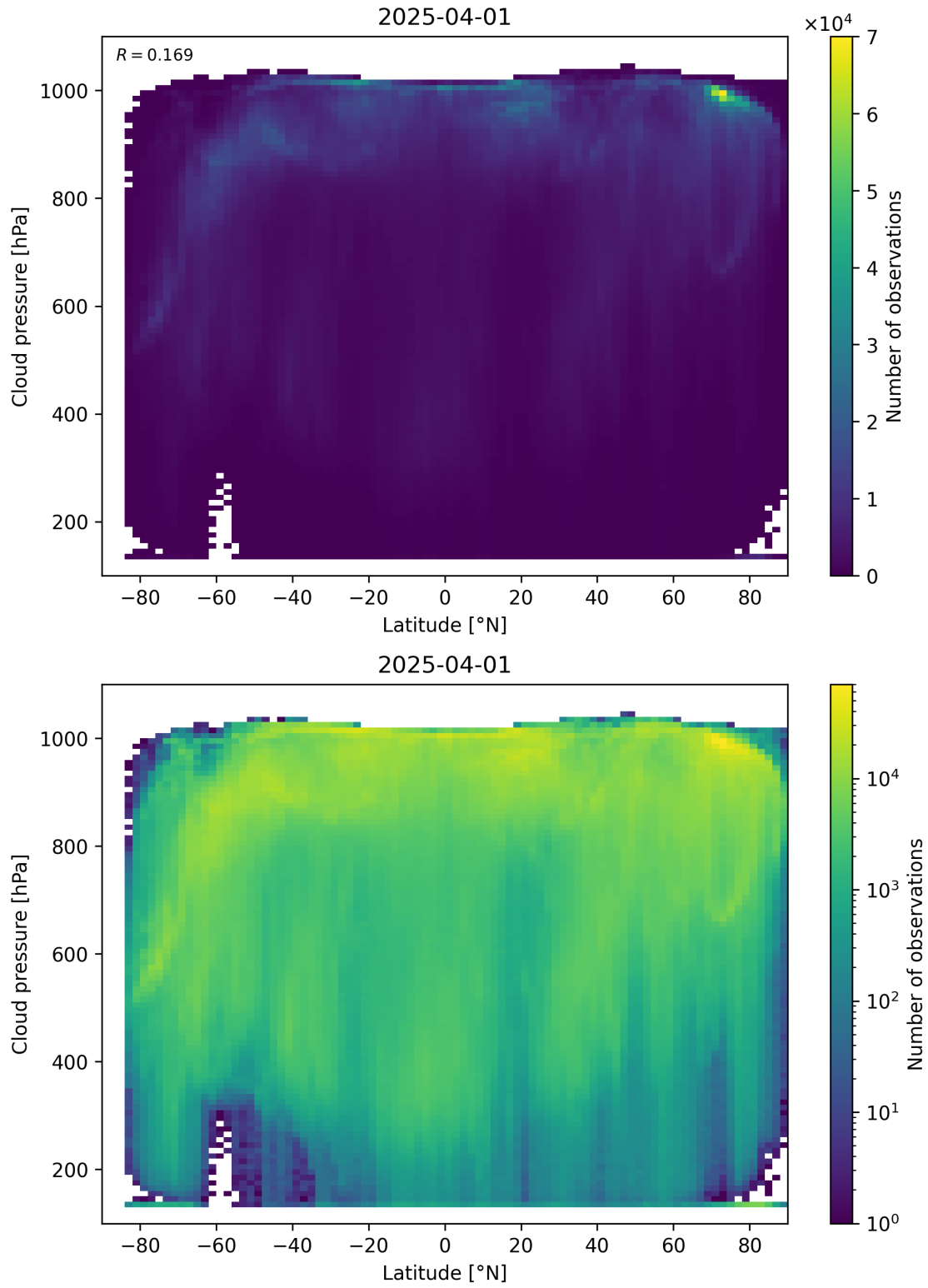
Figure 91: Scatter density plot of “Latitude” against “Cloud pressure” for 2025-03-31 to 2025-04-02.
