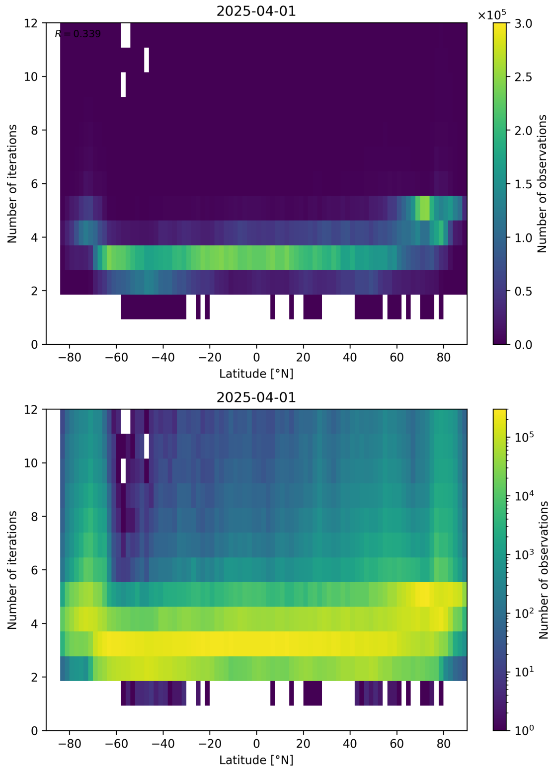
Figure 93: Scatter density plot of “Latitude” against “Number of iterations” for 2025-03-31 to 2025-04-02.
