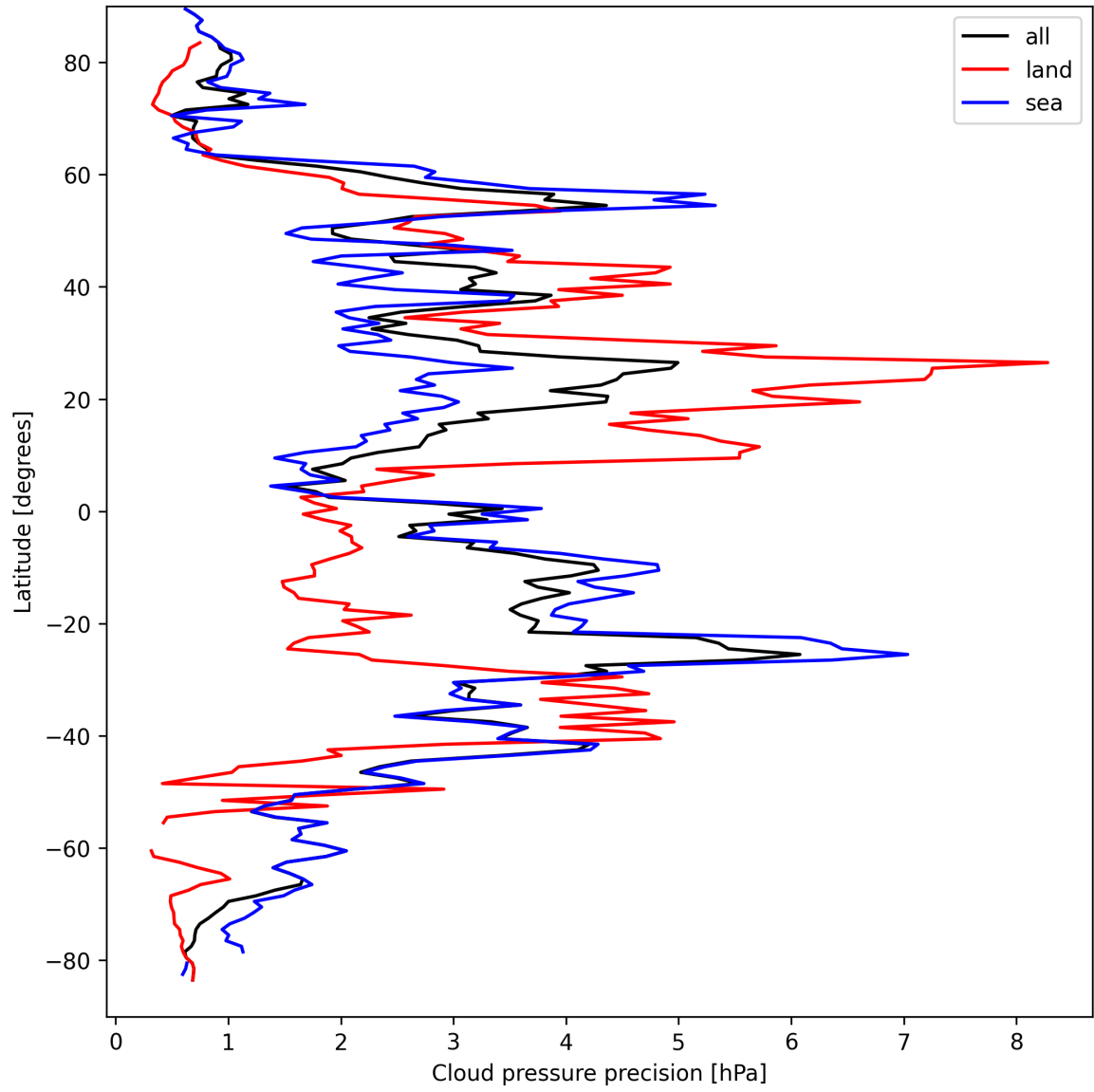
Figure 14: Zonal average of “Cloud pressure precision” for 2025-03-31 to 2025-04-02.
