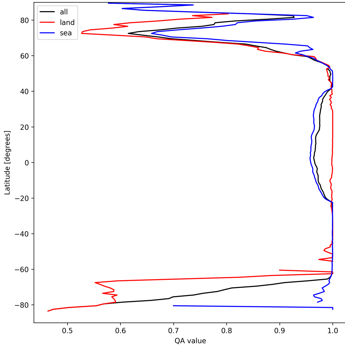
Figure 12: Zonal average of “QA value” for 2025-03-31 to 2025-04-02.
