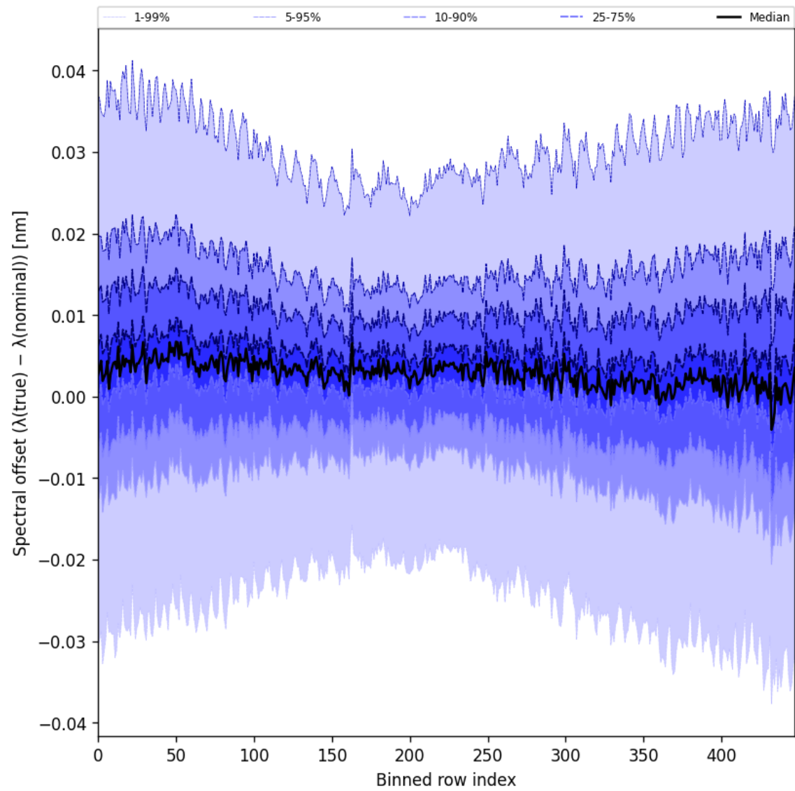
Figure 62: Along track statistics of “Spectral offset ( \lambda_{\text{true}} - \lambda_{\text{nominal}} )” for 2025-03-31 to 2025-04-02
