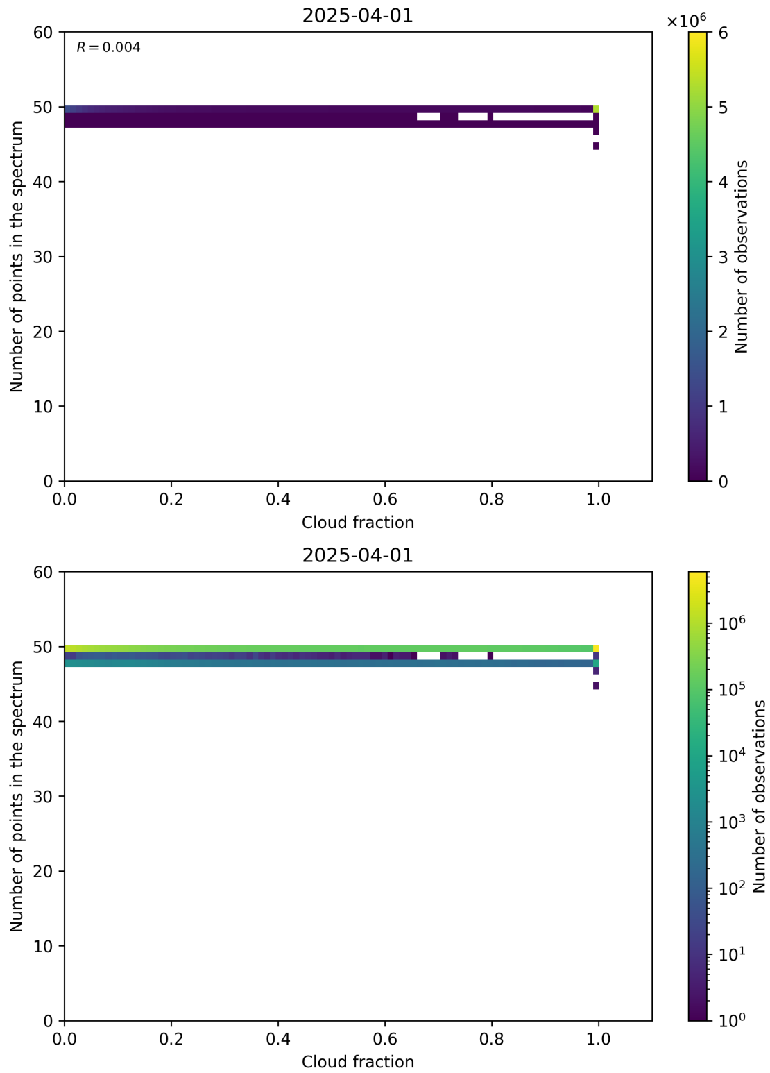
Figure 74: Scatter density plot of “Cloud fraction” against “Number of points in the spectrum” for 2025-03-31 to 2025-04-02.
