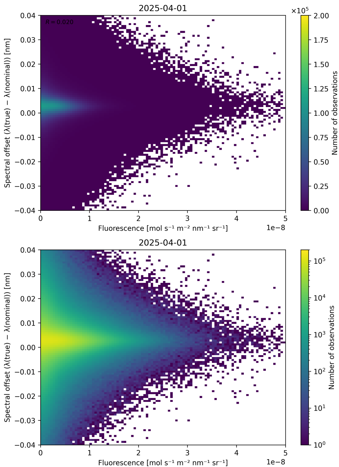
Figure 87: Scatter density plot of “Fluorescence” against “Spectral offset ( \lambda_{\text{true}} - \lambda_{\text{nominal}} )” for 2025-03-31 to 2025-04-02.
