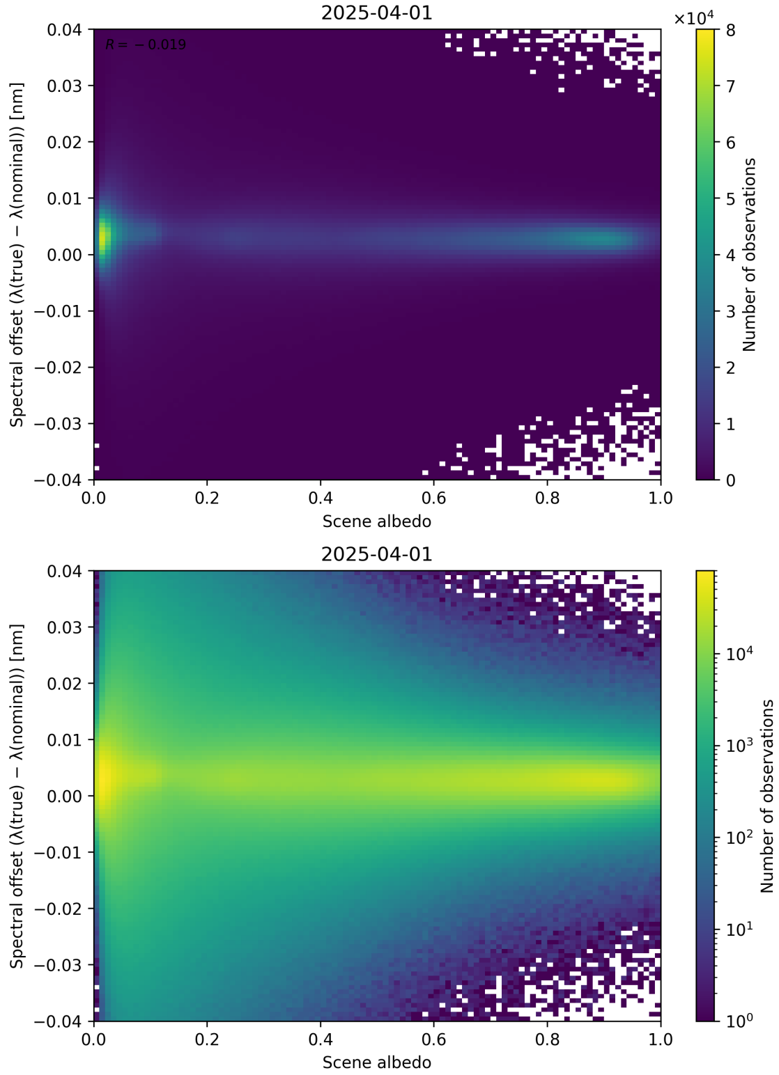
Figure 107: Scatter density plot of “Scene albedo” against “Spectral offset ( \lambda_{\text{true}} - \lambda_{\text{nominal}} )” for 2025-03-31 to 2025-04-02.
