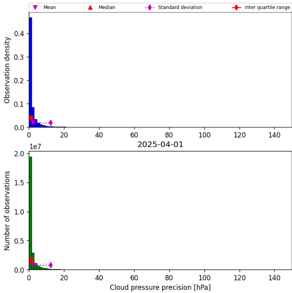
Figure 31: Histogram of “Cloud pressure precision” for 2025-03-31 to 2025-04-02
