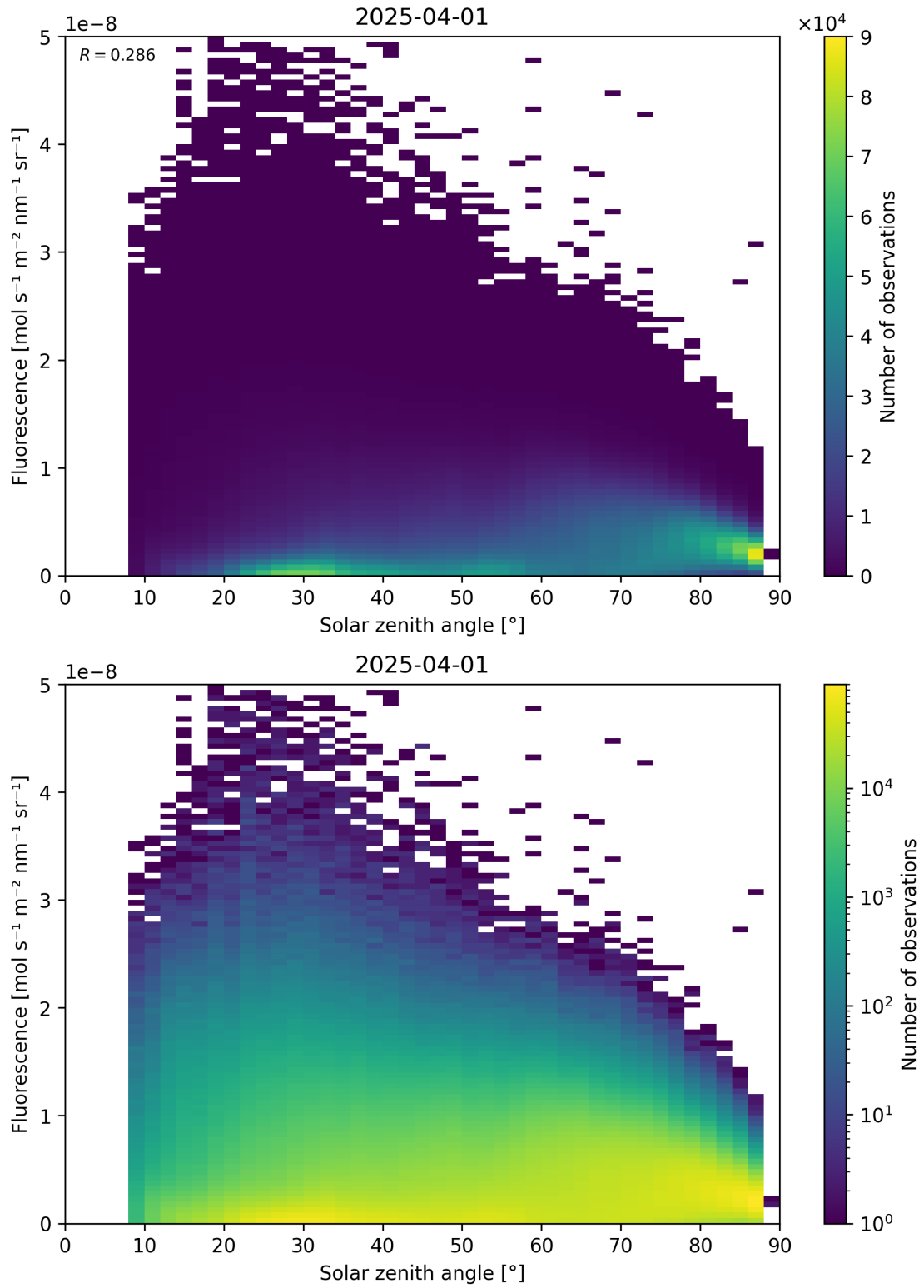
Figure 112: Scatter density plot of “Solar zenith angle” against “Fluorescence” for 2025-03-31 to 2025-04-02.
