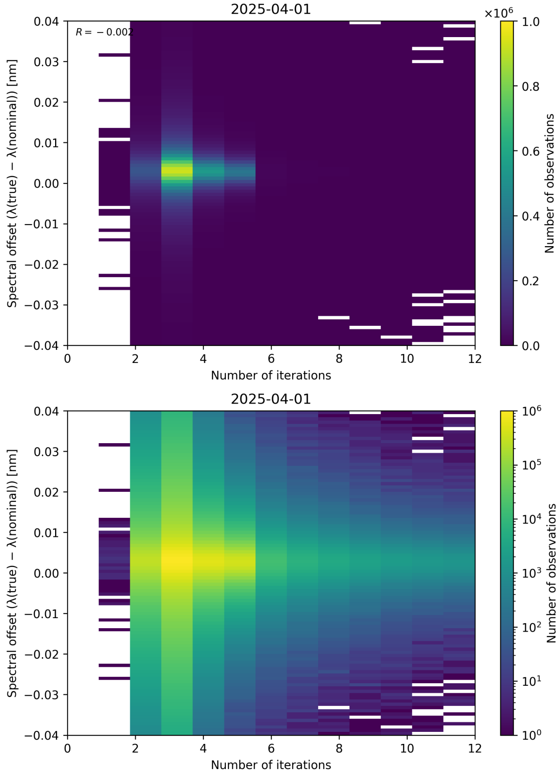
Figure 100: Scatter density plot of “Number of iterations” against “Spectral offset ( \lambda_{\text{true}} - \lambda_{\text{nominal}} )” for 2025-03-31 to 2025-04-02.
