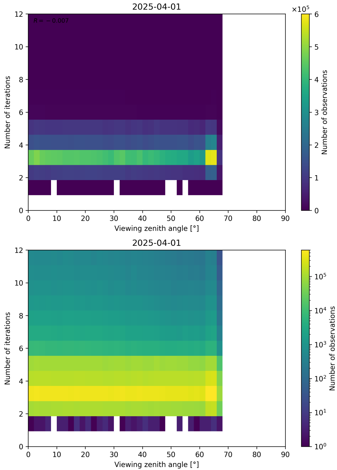
Figure 124: Scatter density plot of “Viewing zenith angle” against “Number of iterations” for 2025-03-31 to 2025-04-02.
