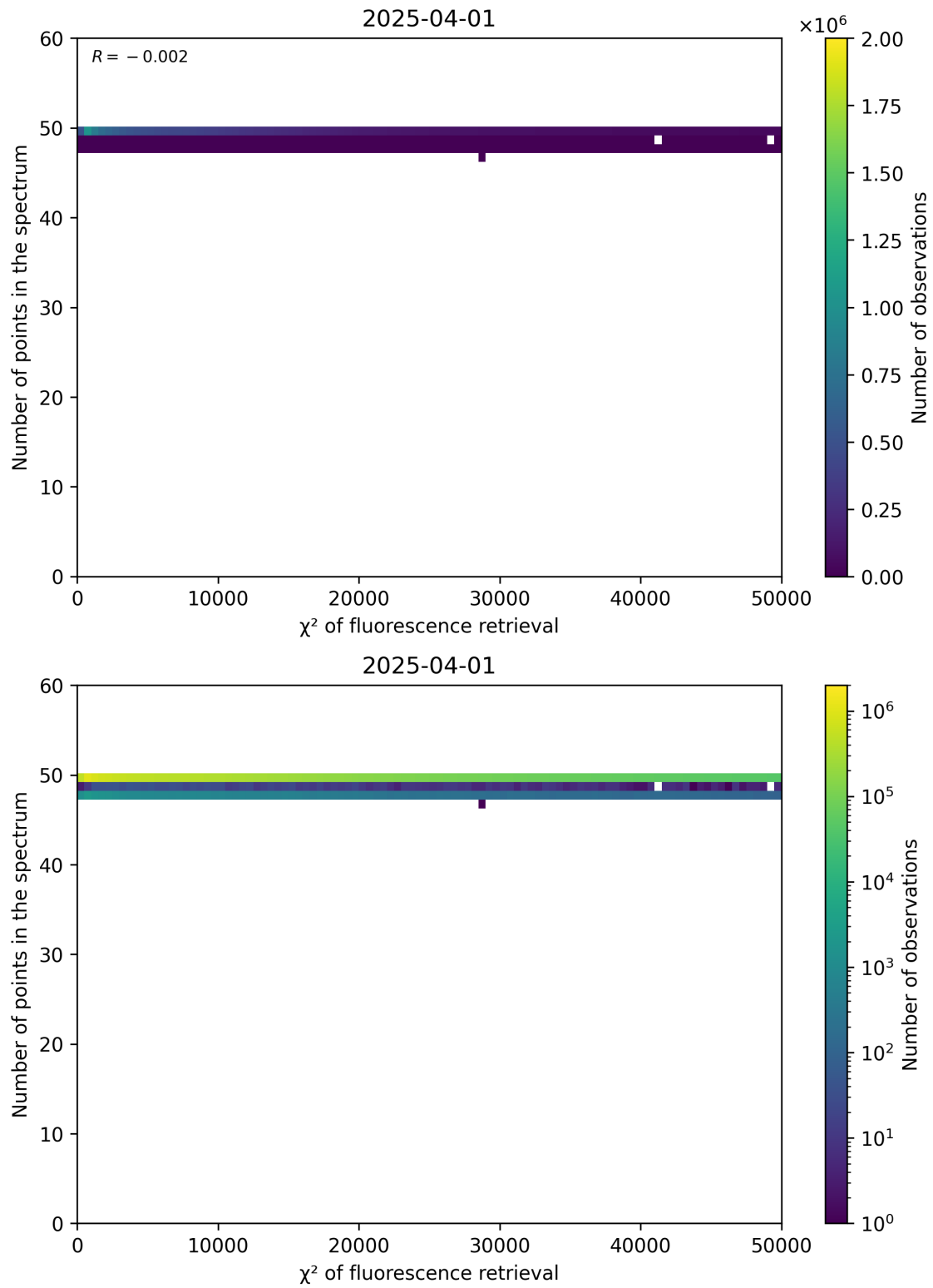
Figure 68: Scatter density plot of " \chi^2 of fluorescence retrieval" against "Number of points in the spectrum" for 2025-03-31 to 2025-04-02.
