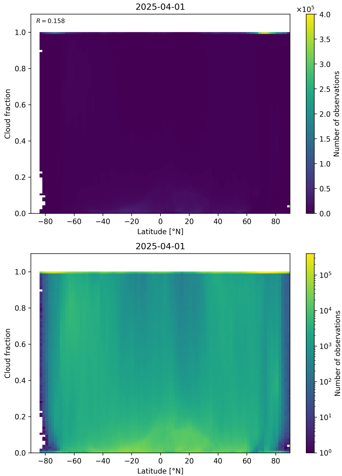
Figure 90: Scatter density plot of “Latitude” against “Cloud fraction” for 2025-03-31 to 2025-04-02.
