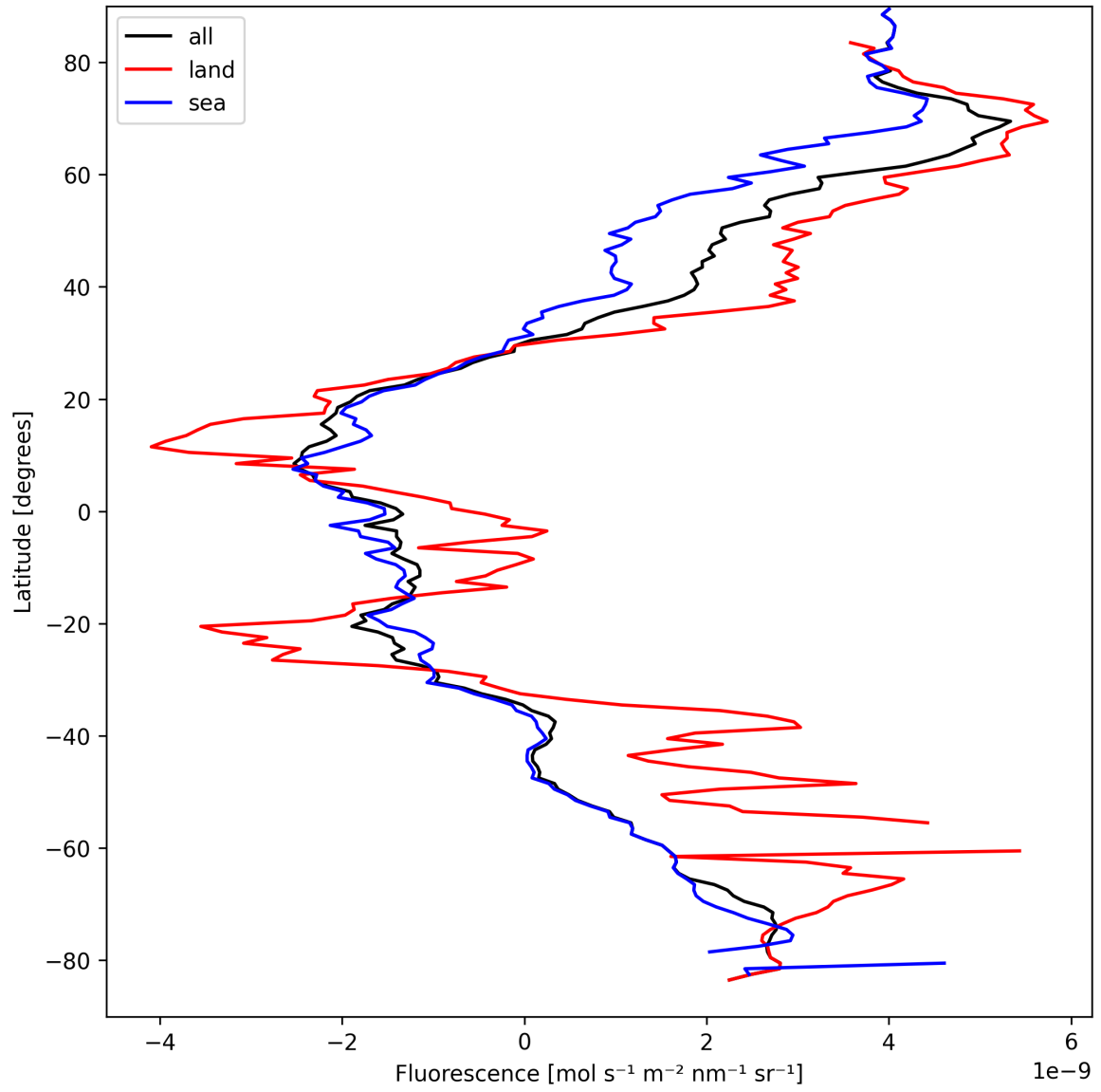
Figure 23: Zonal average of “Fluorescence” for 2025-03-31 to 2025-04-02.
