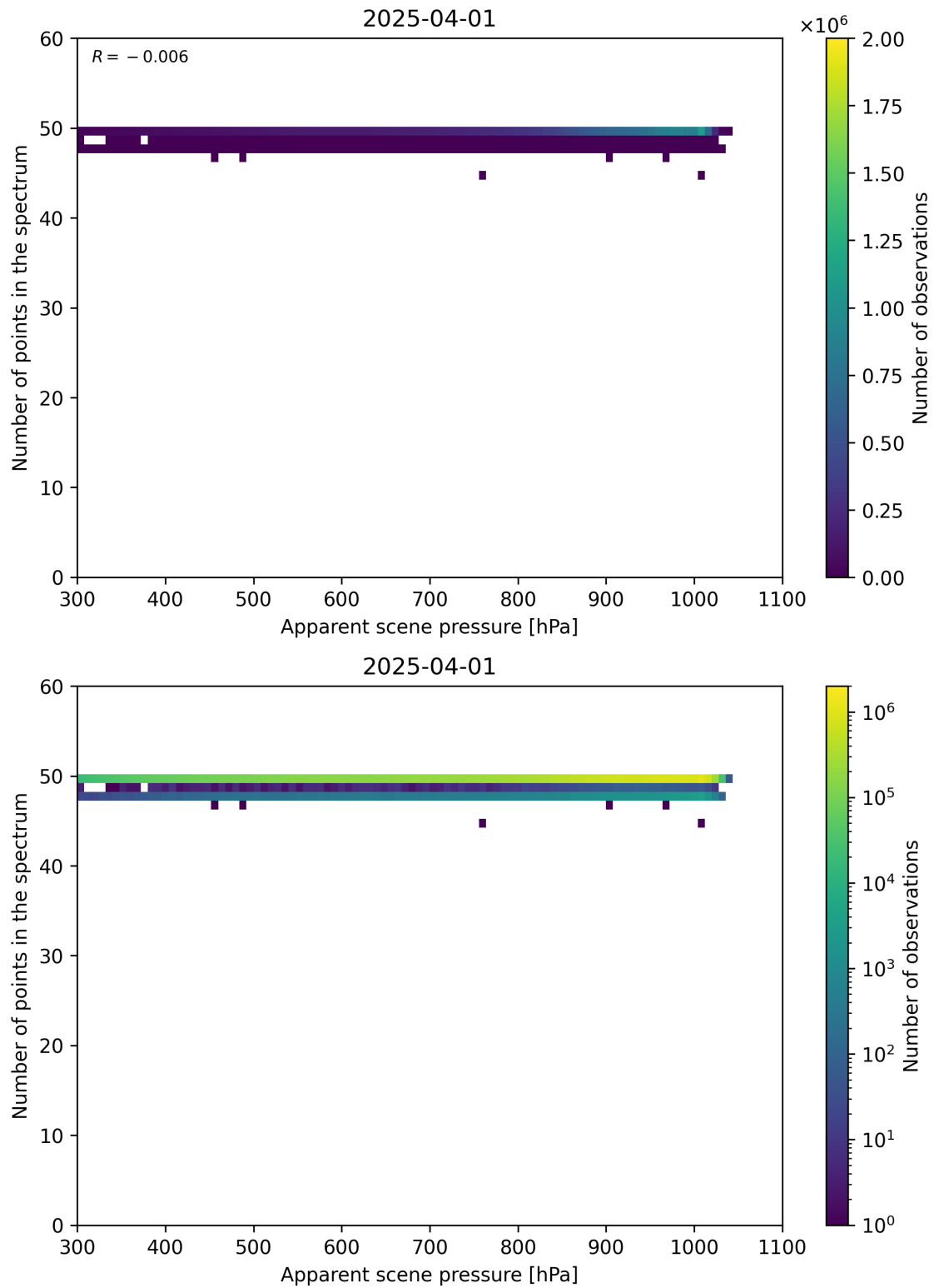
Figure 66: Scatter density plot of “Apparent scene pressure” against “Number of points in the spectrum” for 2025-03-31 to 2025-04-02.
