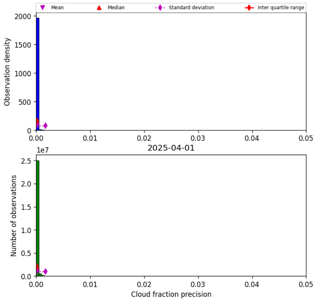
Figure 33: Histogram of “Cloud fraction precision” for 2025-03-31 to 2025-04-02
