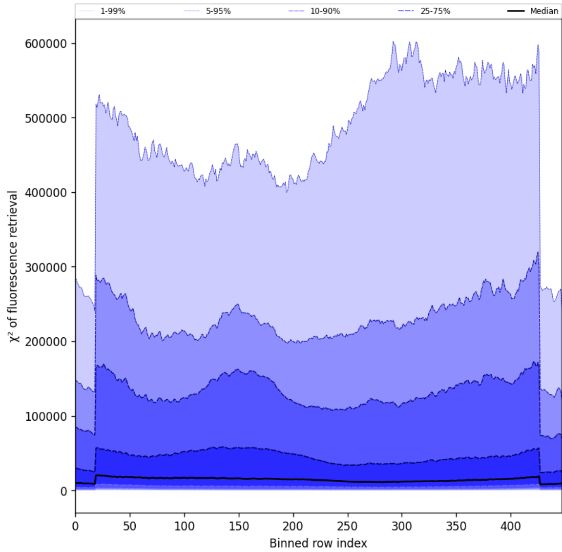
Figure 59: Along track statistics of " \chi^2 of fluorescence retrieval" for 2025-03-31 to 2025-04-02
