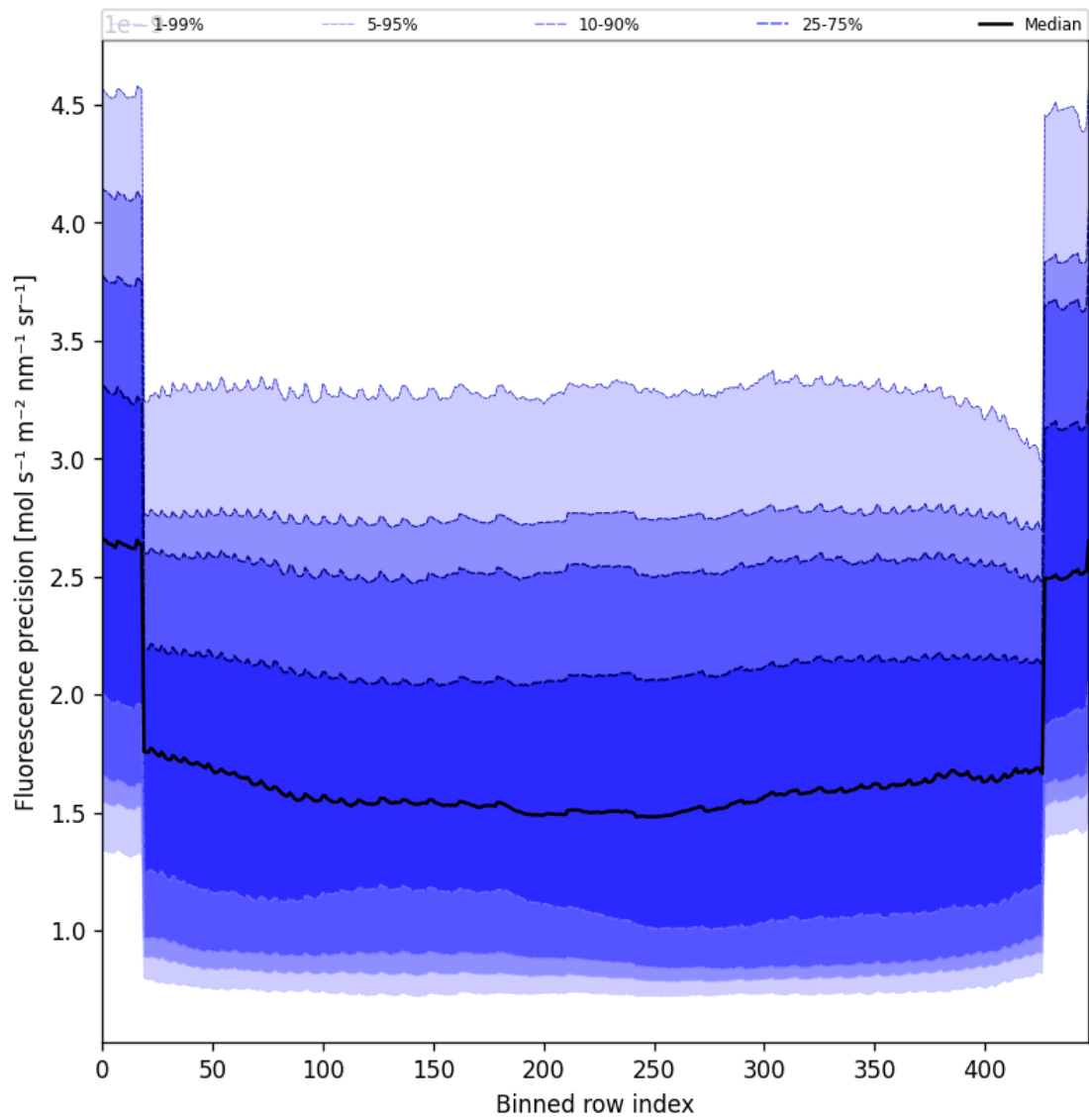
Figure 58: Along track statistics of “Fluorescence precision” for 2025-03-31 to 2025-04-02
