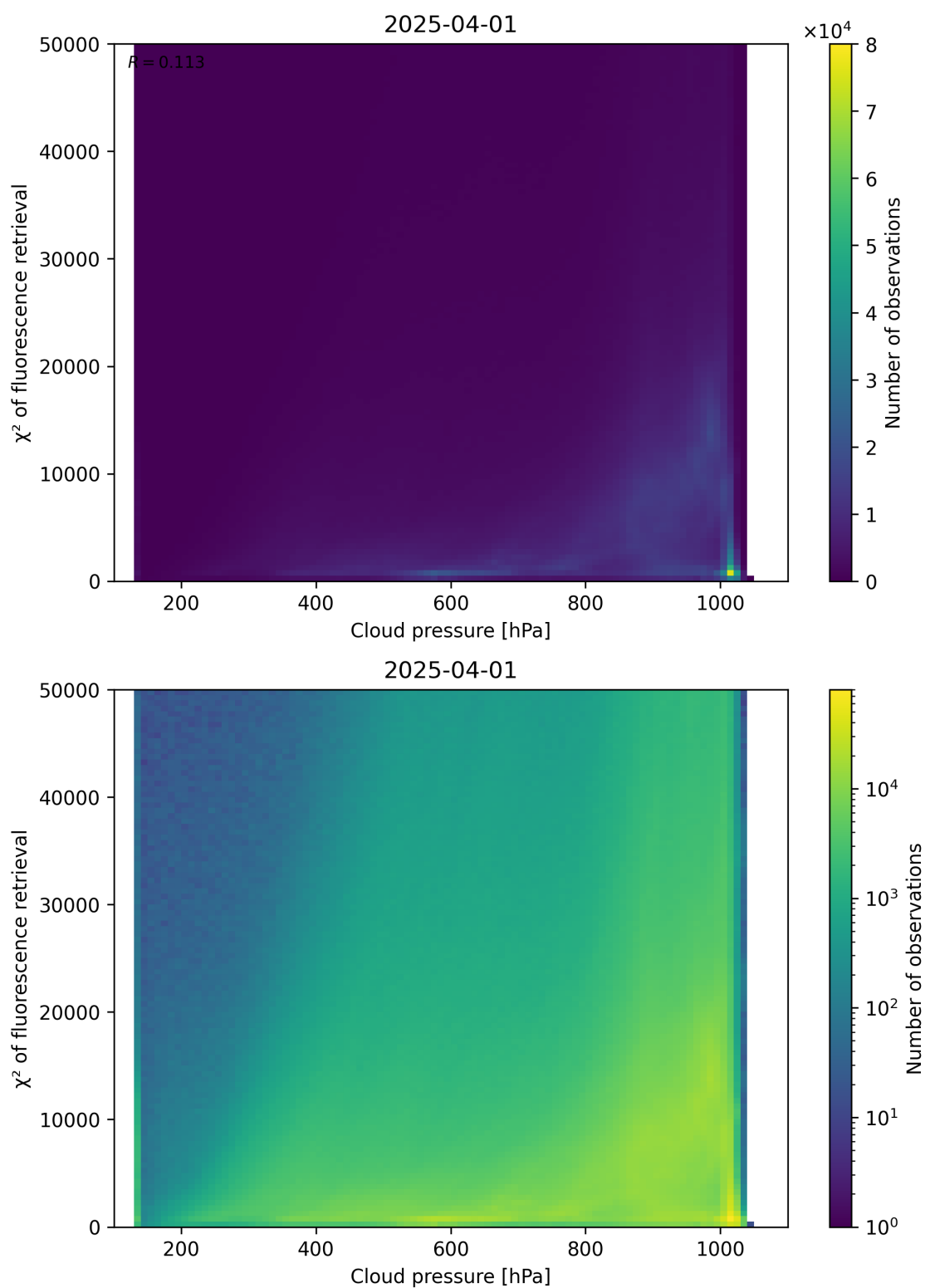
Figure 78: Scatter density plot of “Cloud pressure” against “ \chi^2 of fluorescence retrieval” for 2025-03-31 to 2025-04-02.
