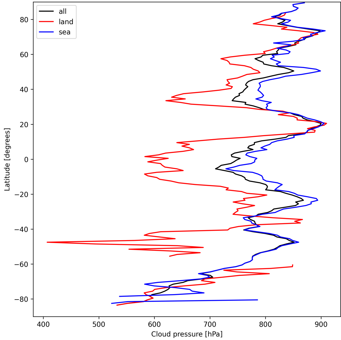
Figure 13: Zonal average of “Cloud pressure” for 2025-03-31 to 2025-04-02.
