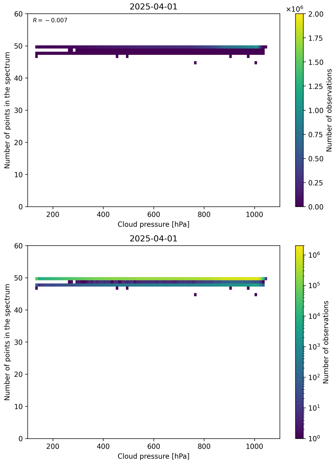
Figure 82: Scatter density plot of “Cloud pressure” against “Number of points in the spectrum” for 2025-03-31 to 2025-04-02.
