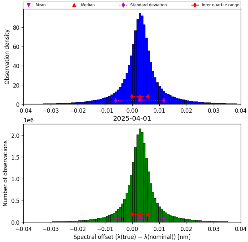
Figure 45: Histogram of “Spectral offset ( \lambda_{\text{true}} - \lambda_{\text{nominal}} )” for 2025-03-31 to 2025-04-02
