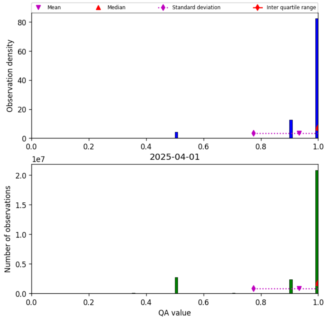
Figure 29: Histogram of “QA value” for 2025-03-31 to 2025-04-02
