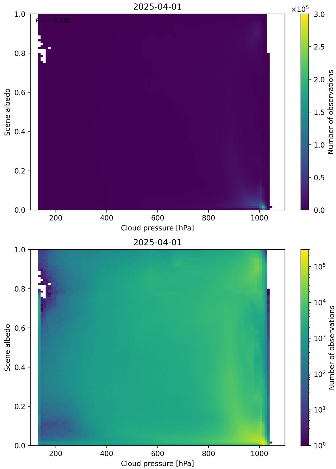
Figure 83: Scatter density plot of “Cloud pressure” against “Scene albedo” for 2025-03-31 to 2025-04-02.
