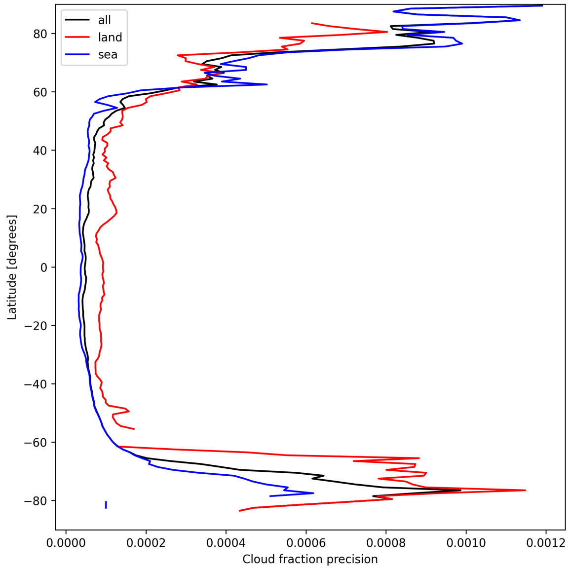
Figure 16: Zonal average of “Cloud fraction precision” for 2025-03-31 to 2025-04-02.
