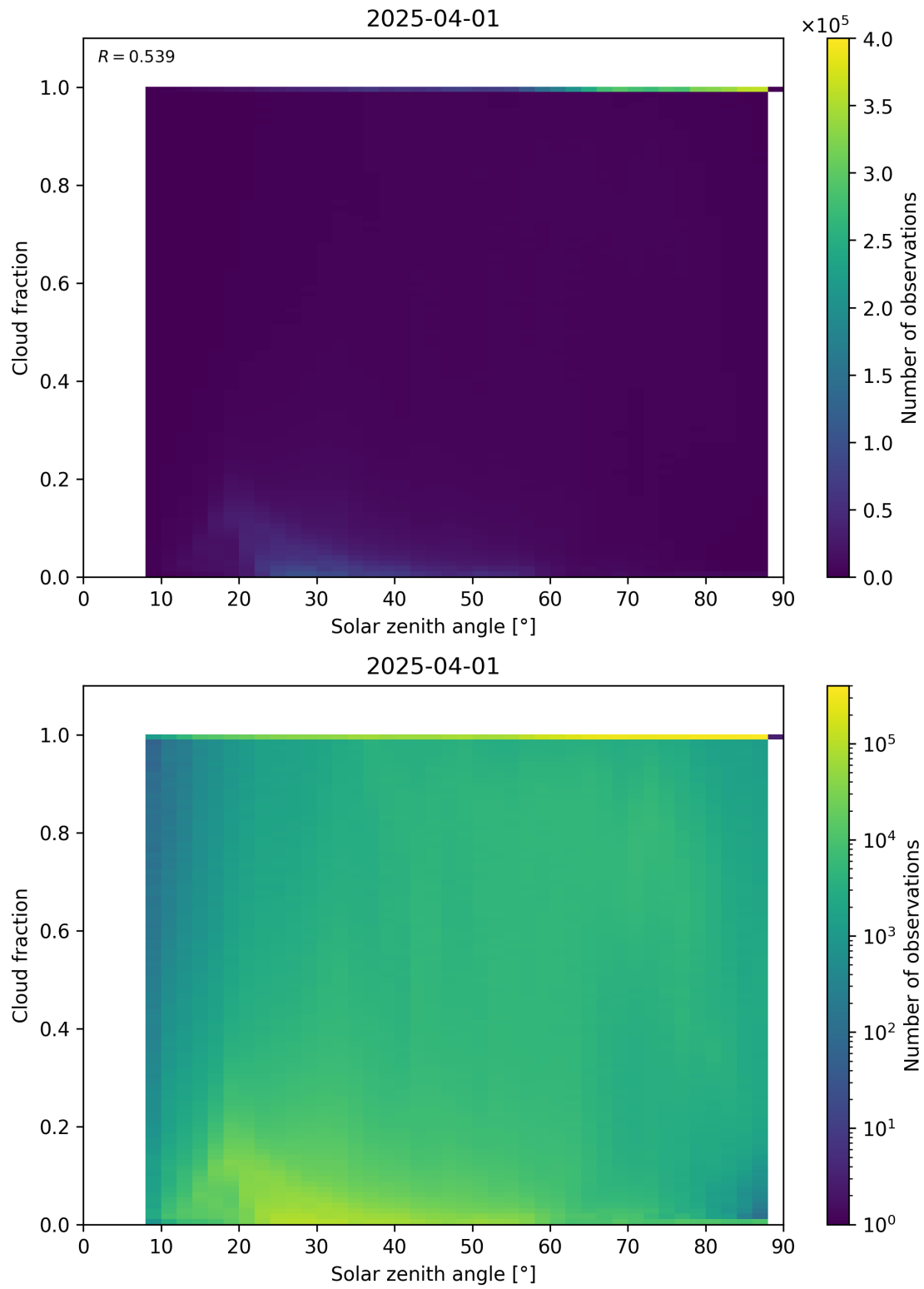
Figure 110: Scatter density plot of “Solar zenith angle” against “Cloud fraction” for 2025-03-31 to 2025-04-02.
