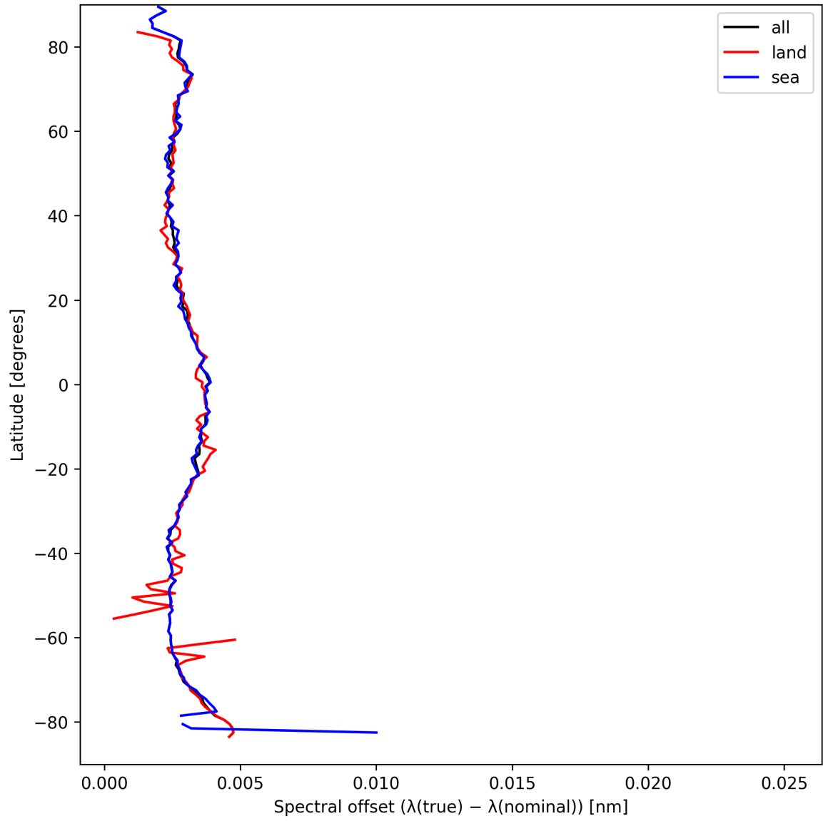
Figure 28: Zonal average of “Spectral offset ( \lambda_{\text{true}} - \lambda_{\text{nominal}} )” for 2025-03-31 to 2025-04-02.
