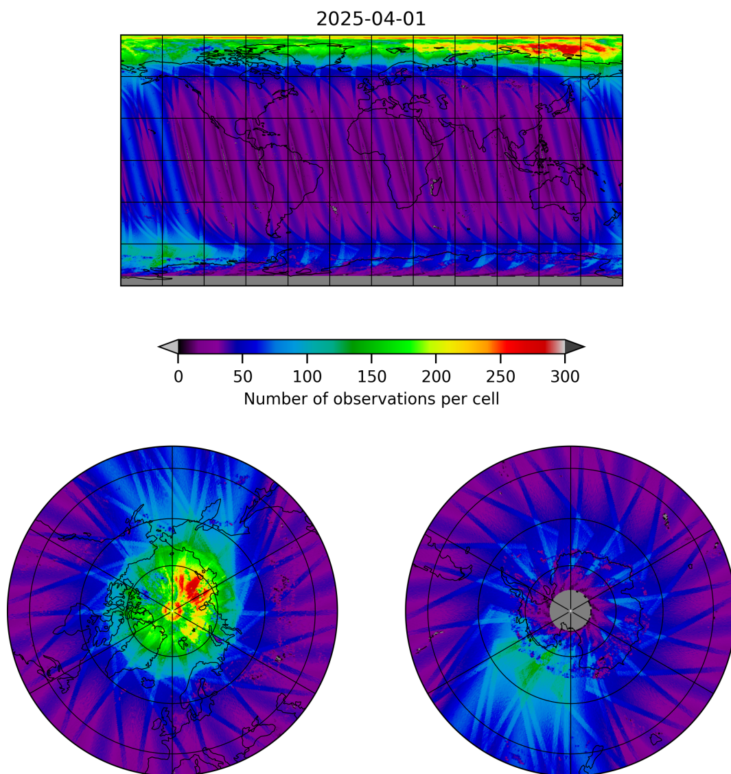
Figure 11: Map of the number of observations for 2025-03-31 to 2025-04-02
