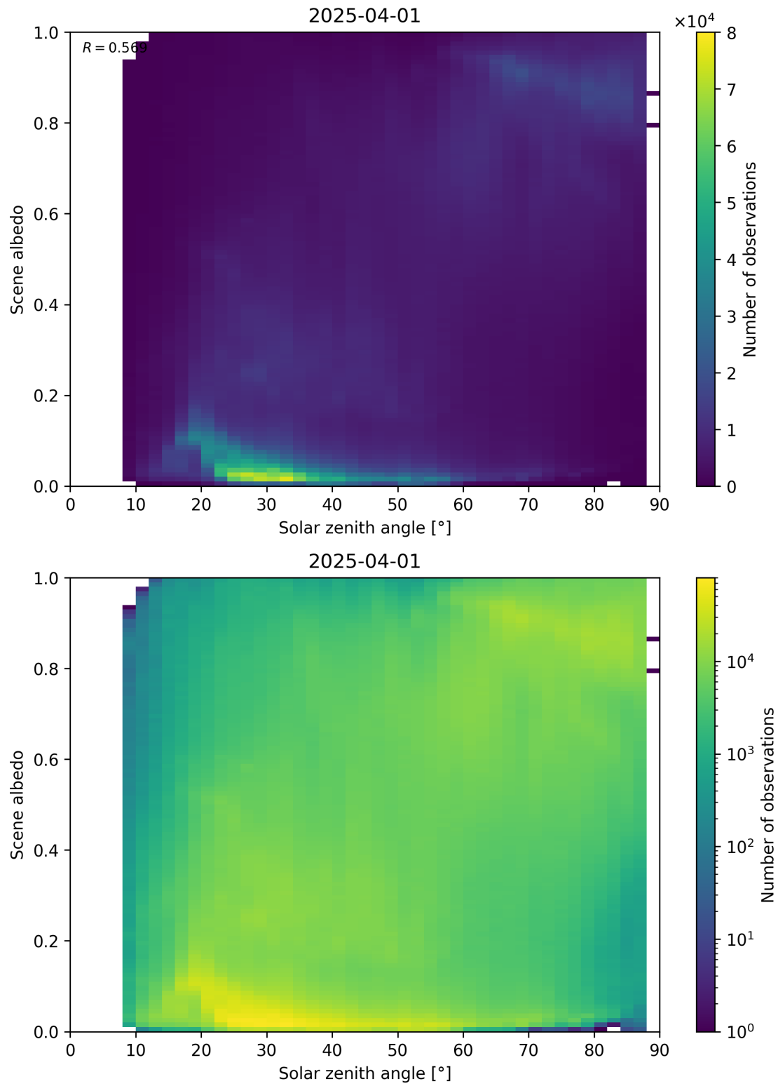
Figure 116: Scatter density plot of “Solar zenith angle” against “Scene albedo” for 2025-03-31 to 2025-04-02.
