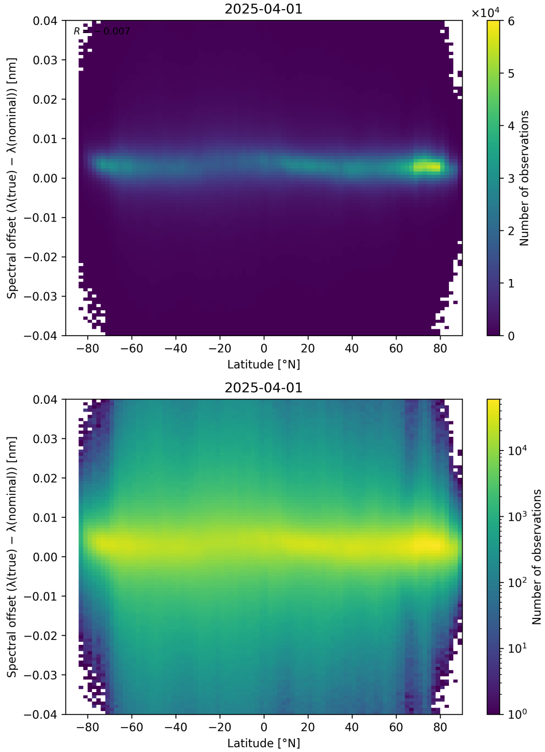
Figure 96: Scatter density plot of “Latitude” against “Spectral offset ( \lambda_{\text{true}} - \lambda_{\text{nominal}} )” for 2025-03-31 to 2025-04-02.
