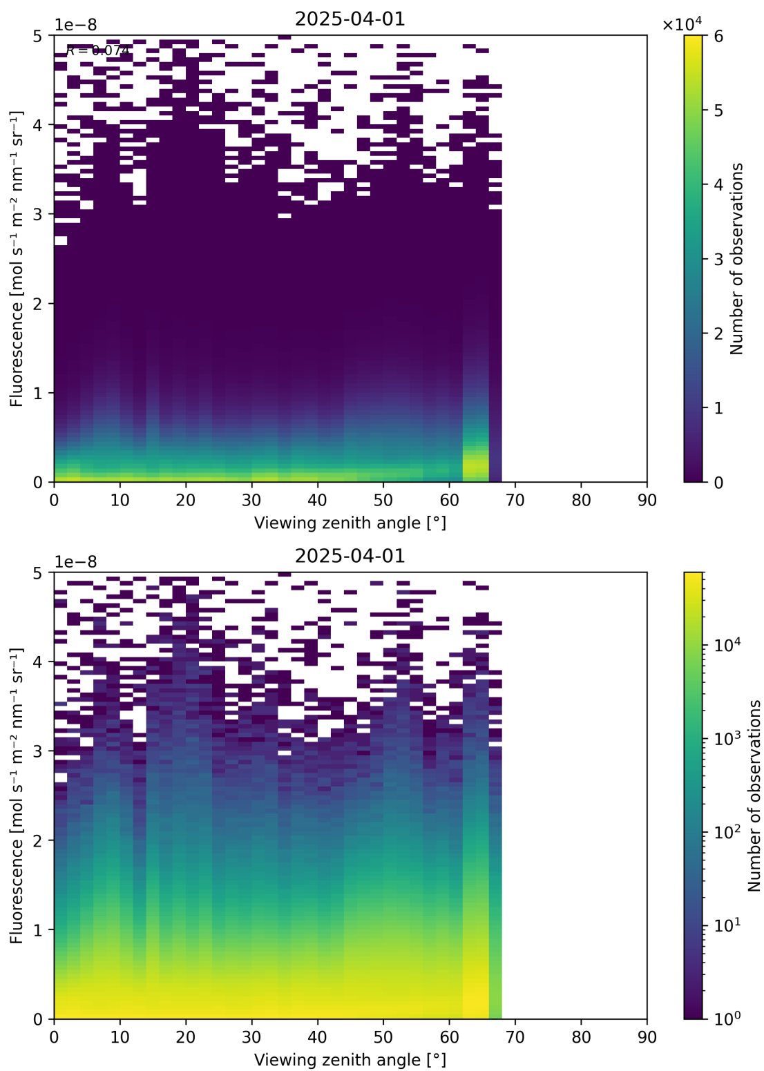
Figure 122: Scatter density plot of “Viewing zenith angle” against “Fluorescence” for 2025-03-31 to 2025-04-02.
