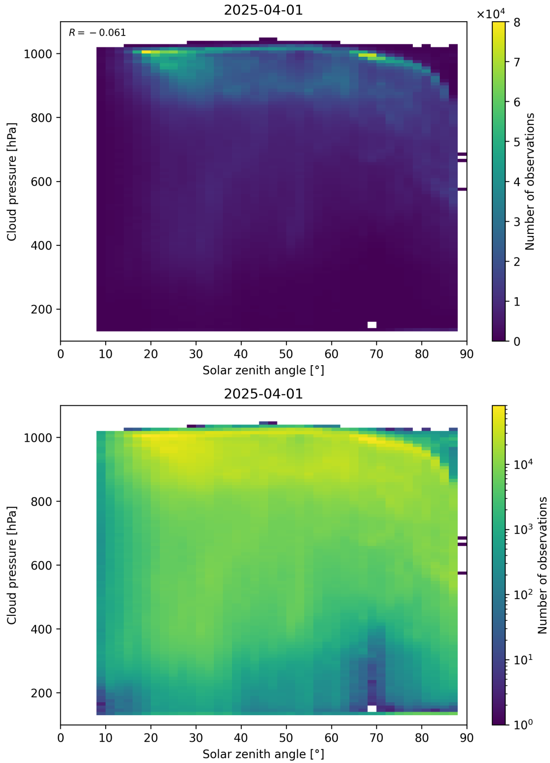
Figure 111: Scatter density plot of “Solar zenith angle” against “Cloud pressure” for 2025-03-31 to 2025-04-02.
