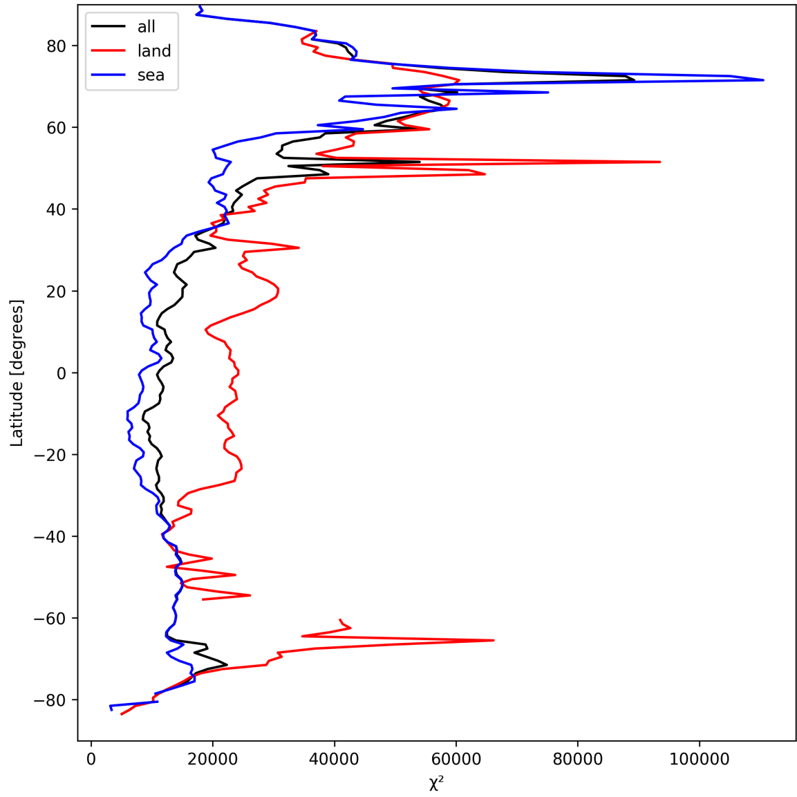
Figure 21: Zonal average of “ \chi^2 ” for 2025-03-31 to 2025-04-02.
