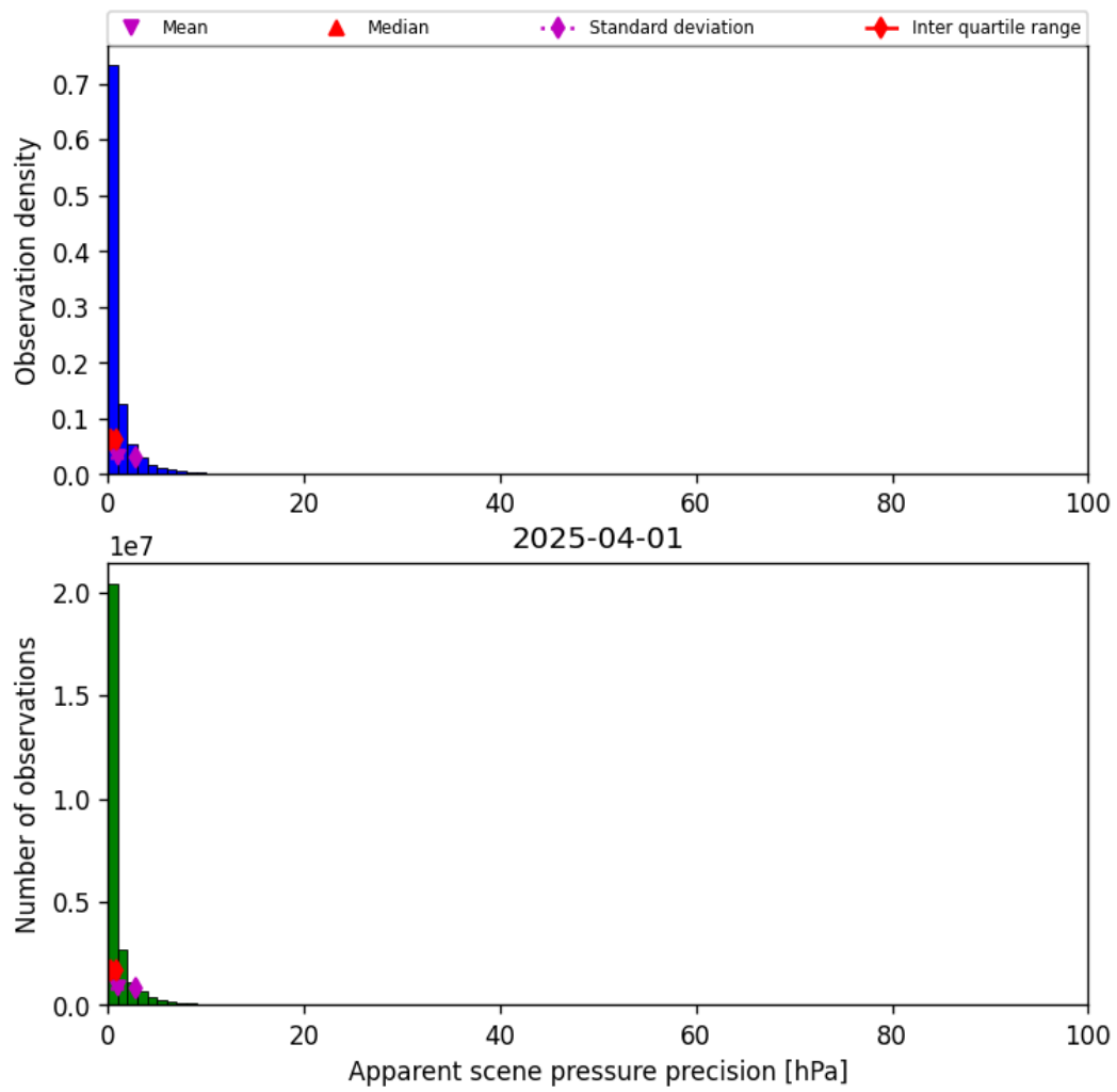
Figure 37: Histogram of “Apparent scene pressure precision” for 2025-03-31 to 2025-04-02
