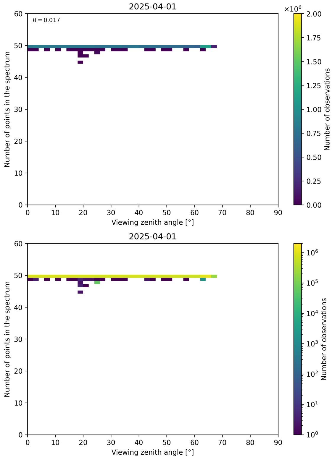
Figure 125: Scatter density plot of “Viewing zenith angle” against “Number of points in the spectrum” for 2025-03-31 to 2025-04-02.
