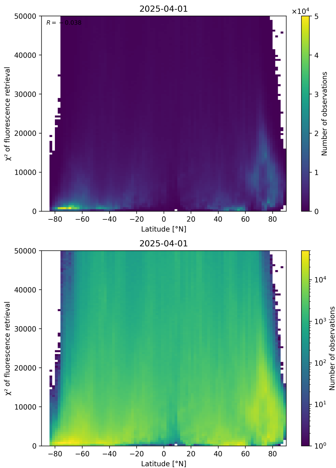
Figure 89: Scatter density plot of “Latitude” against “ \chi^2 of fluorescence retrieval” for 2025-03-31 to 2025-04-02.
