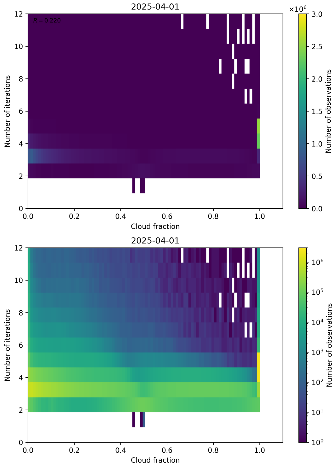
Figure 73: Scatter density plot of “Cloud fraction” against “Number of iterations” for 2025-03-31 to 2025-04-02.
