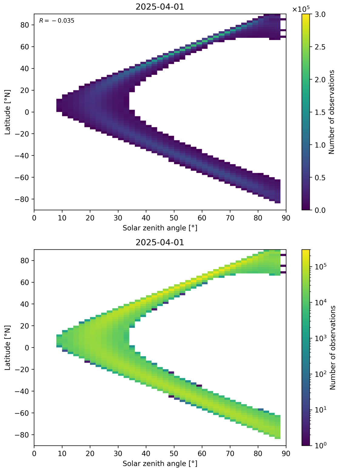
Figure 113: Scatter density plot of “Solar zenith angle” against “Latitude” for 2025-03-31 to 2025-04-02.
