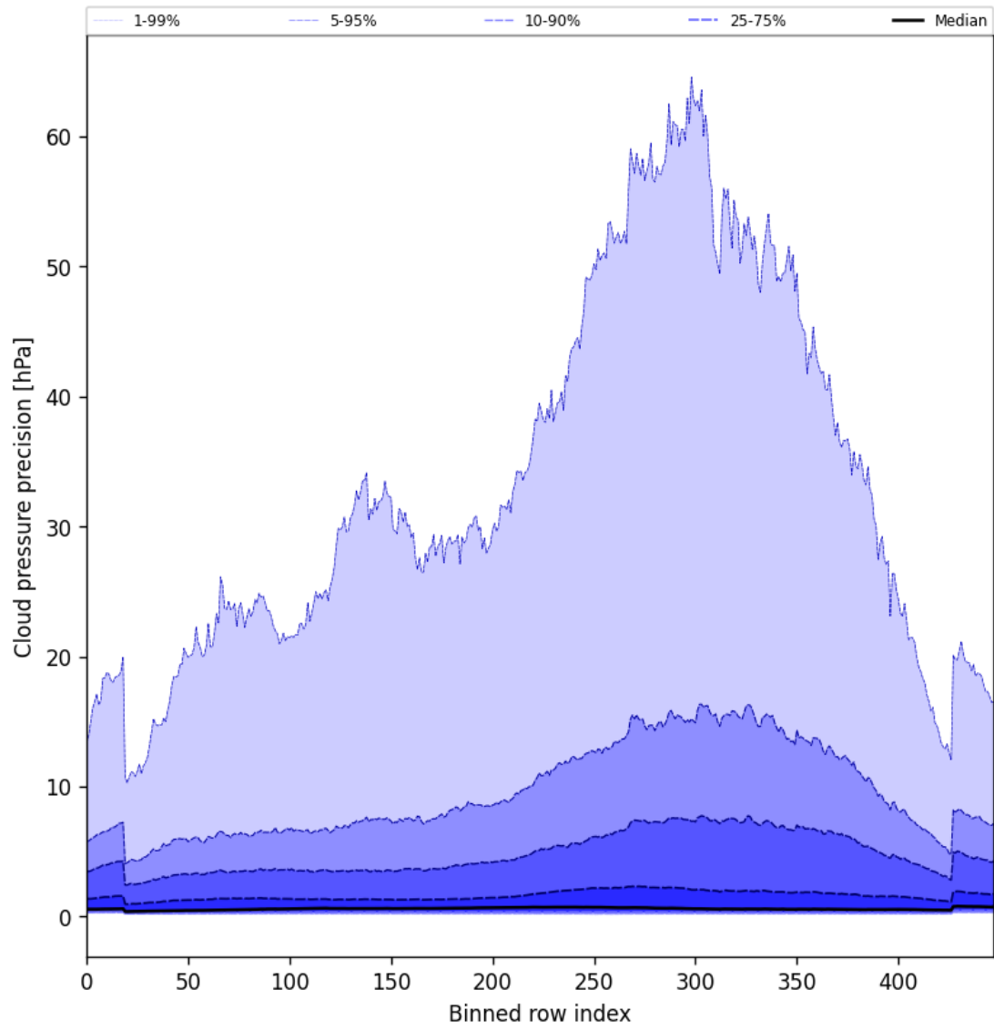
Figure 48: Along track statistics of “Cloud pressure precision” for 2025-03-31 to 2025-04-02
