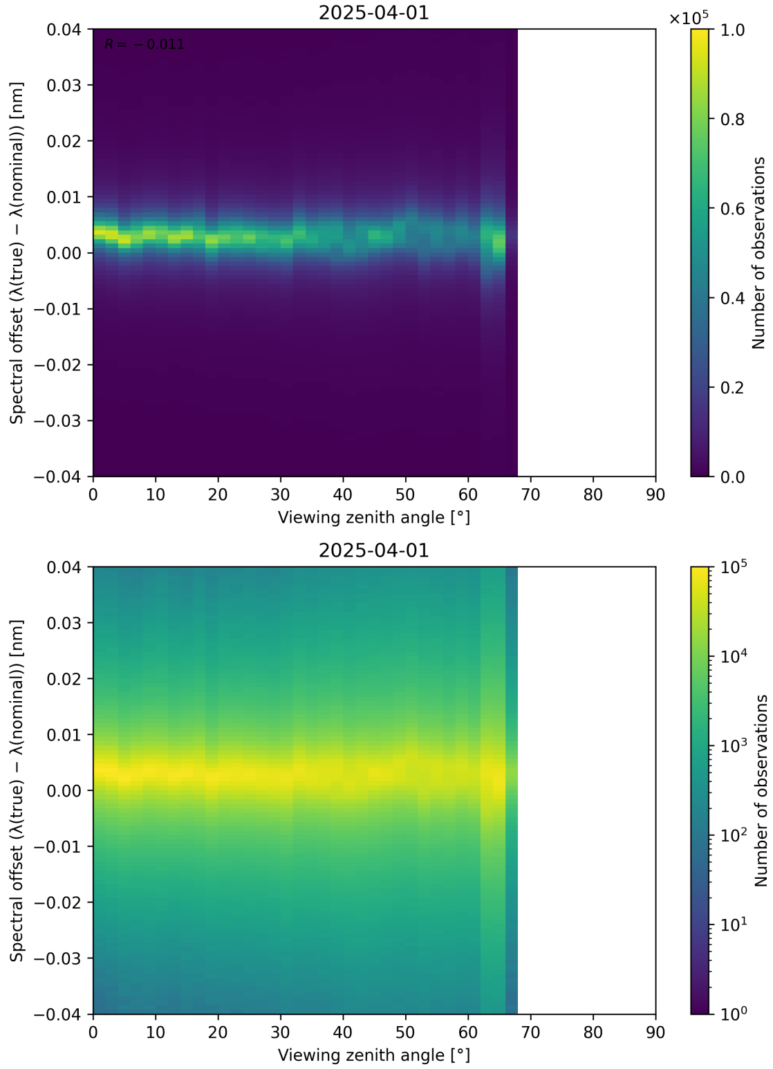
Figure 128: Scatter density plot of “Viewing zenith angle” against “Spectral offset ( \lambda_{\text{true}} - \lambda_{\text{nominal}} )” for 2025-03-31 to 2025-04-02.
