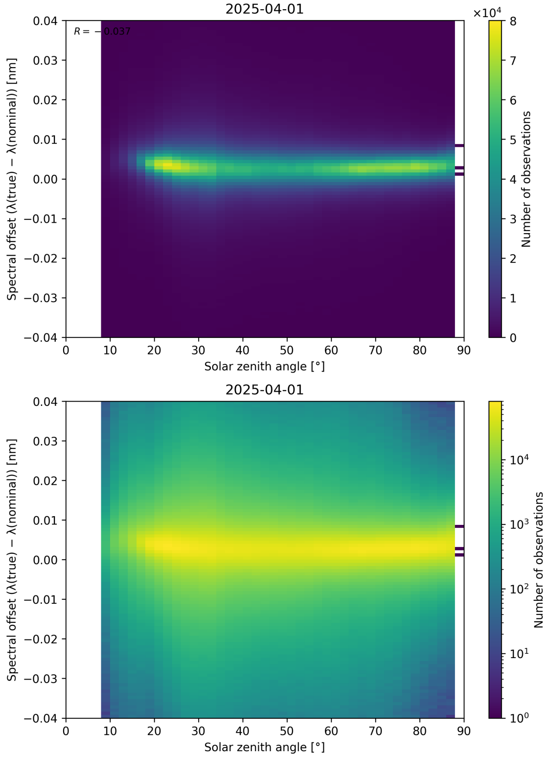
Figure 117: Scatter density plot of “Solar zenith angle” against “Spectral offset ( \lambda_{\text{true}} - \lambda_{\text{nominal}} )” for 2025-03-31 to 2025-04-02.
