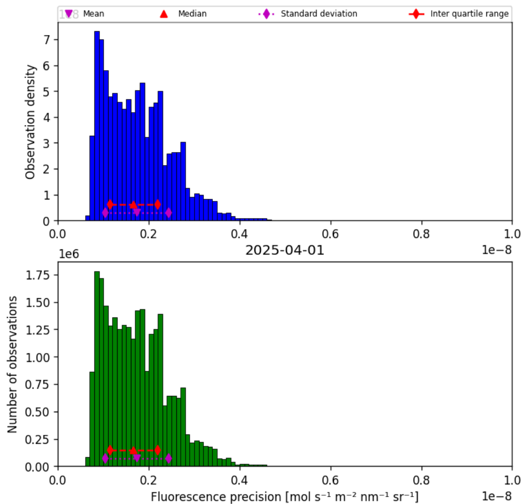
Figure 41: Histogram of “Fluorescence precision” for 2025-03-31 to 2025-04-02
