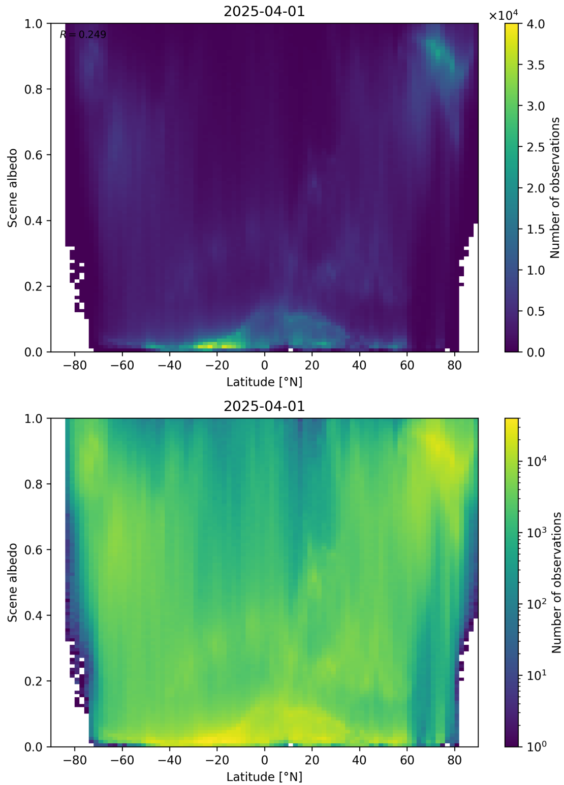
Figure 95: Scatter density plot of “Latitude” against “Scene albedo” for 2025-03-31 to 2025-04-02.
