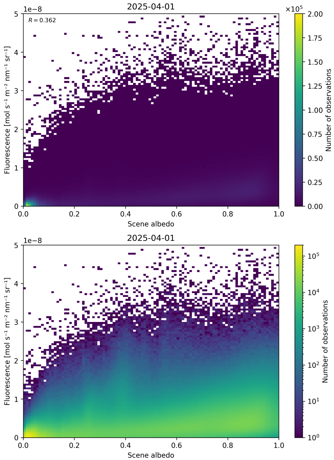
Figure 104: Scatter density plot of “Scene albedo” against “Fluorescence” for 2025-03-31 to 2025-04-02.
