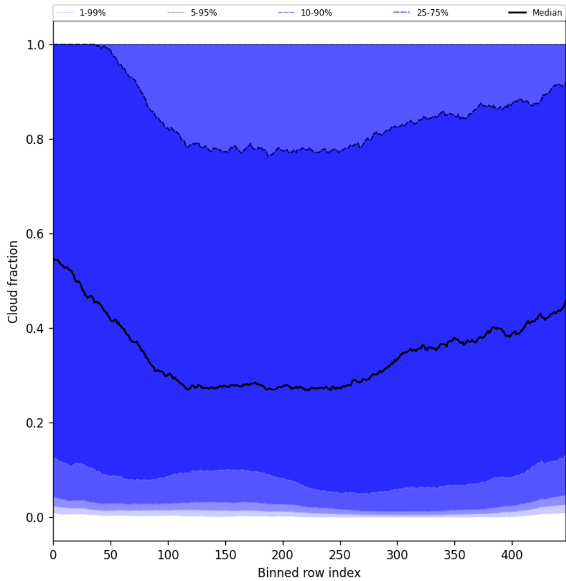
Figure 49: Along track statistics of “Cloud fraction” for 2025-03-31 to 2025-04-02
