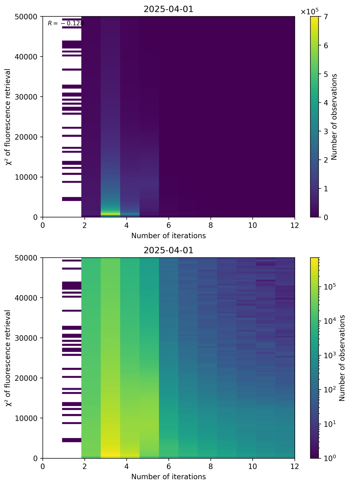
Figure 97: Scatter density plot of “Number of iterations” against “ \chi^2 of fluorescence retrieval” for 2025-03-31 to 2025-04-02.
