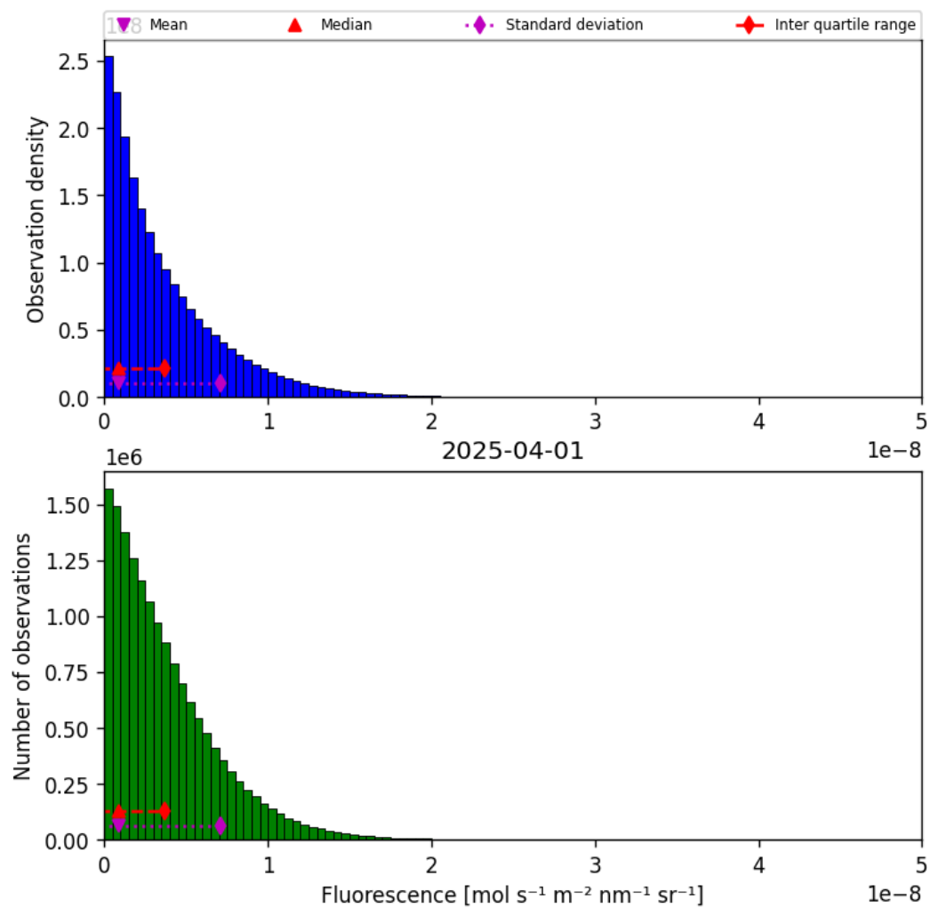
Figure 40: Histogram of “Fluorescence” for 2025-03-31 to 2025-04-02
