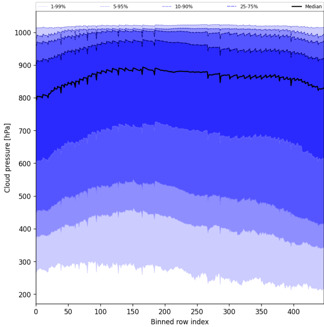
Figure 47: Along track statistics of “Cloud pressure” for 2025-03-31 to 2025-04-02
