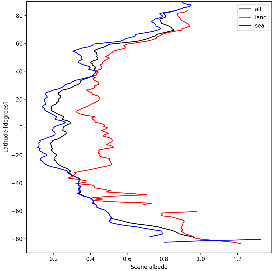
Figure 17: Zonal average of “Scene albedo” for 2025-03-31 to 2025-04-02.
