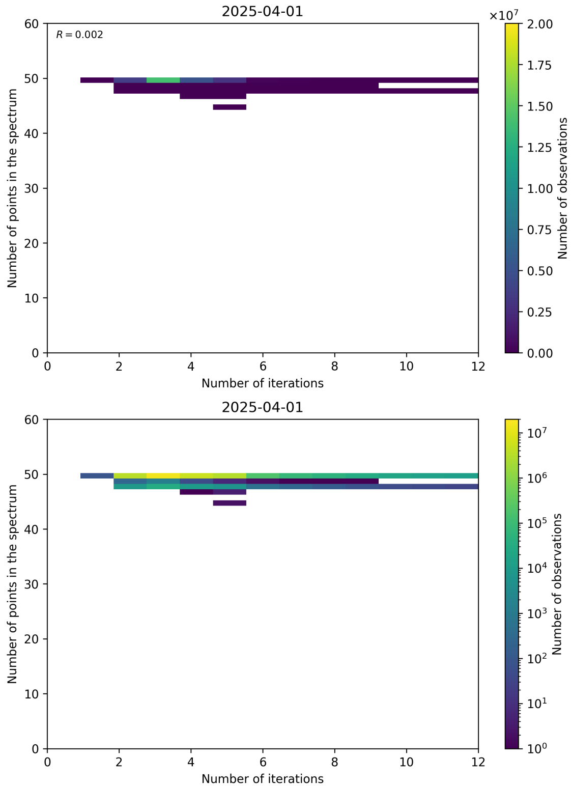
Figure 99: Scatter density plot of “Number of iterations” against “Number of points in the spectrum” for 2025-03-31 to 2025-04-02.
