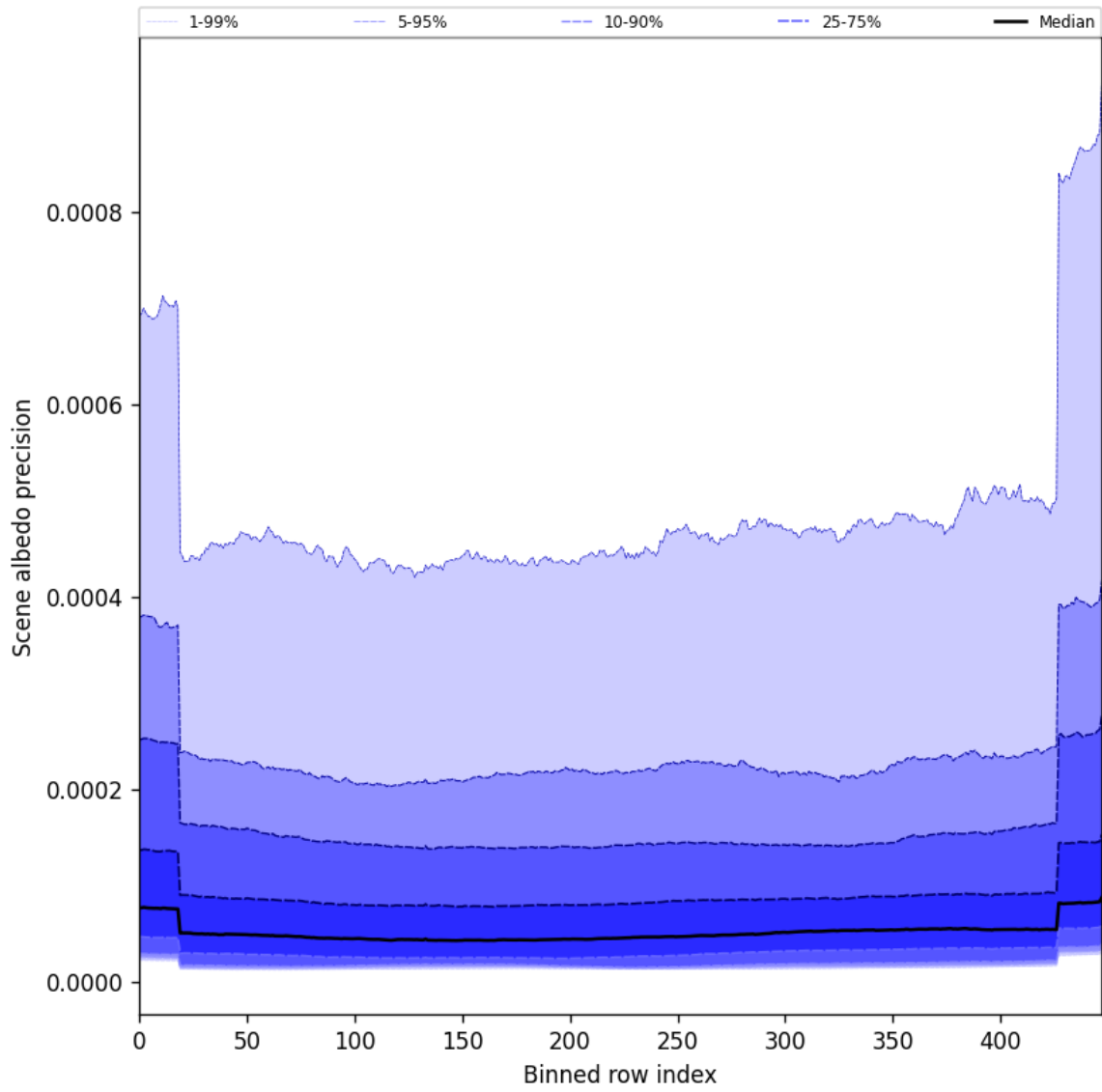
Figure 52: Along track statistics of “Scene albedo precision” for 2025-03-31 to 2025-04-02
