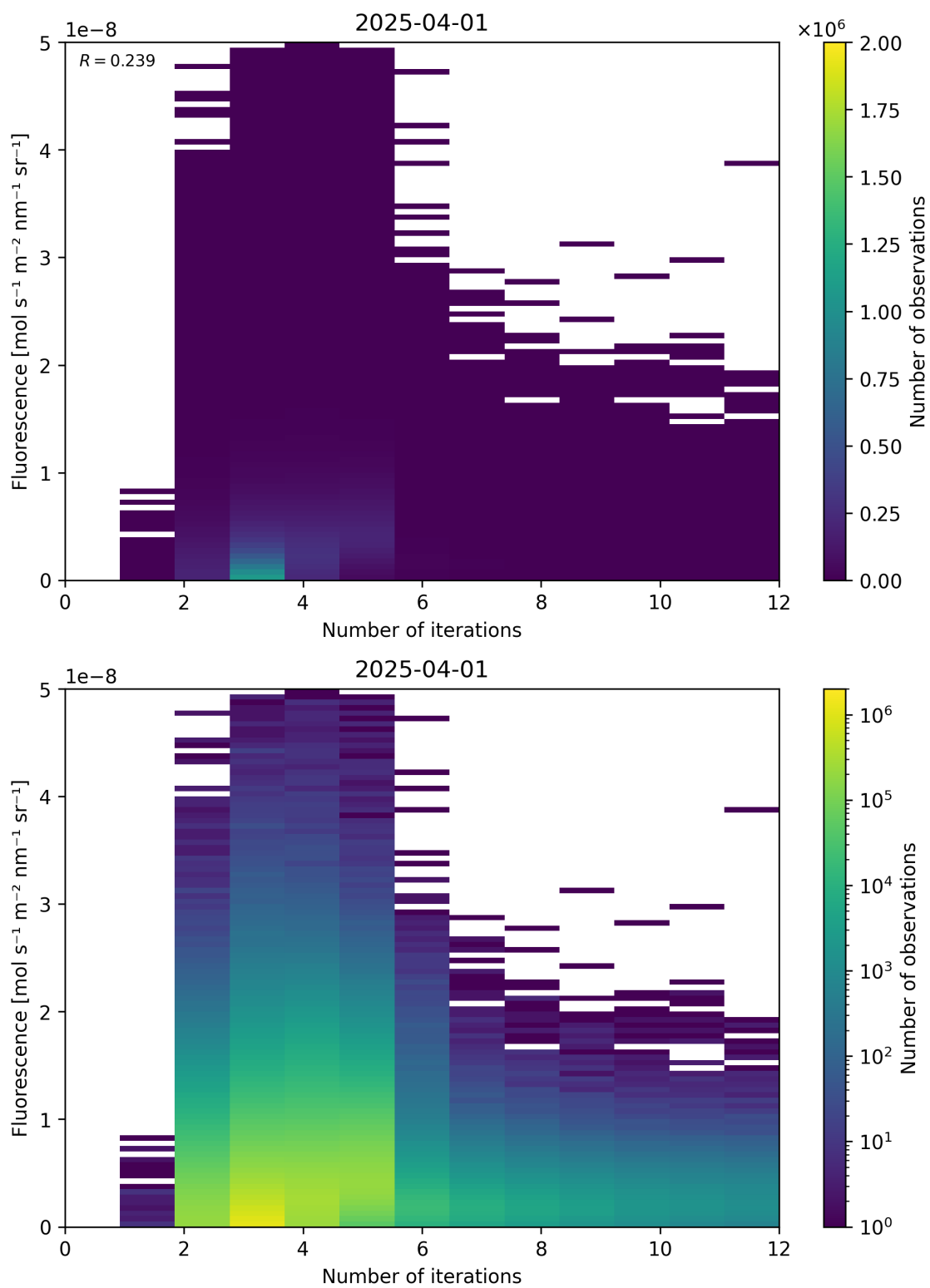
Figure 98: Scatter density plot of “Number of iterations” against “Fluorescence” for 2025-03-31 to 2025-04-02.
