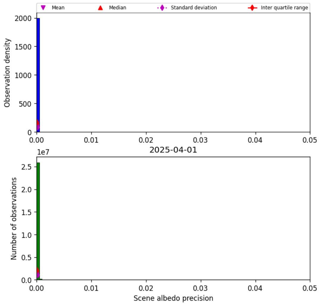
Figure 35: Histogram of “Scene albedo precision” for 2025-03-31 to 2025-04-02
