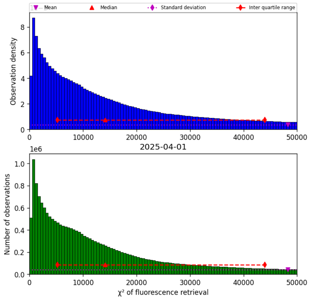
Figure 42: Histogram of “ \chi^2 of fluorescence retrieval” for 2025-03-31 to 2025-04-02
