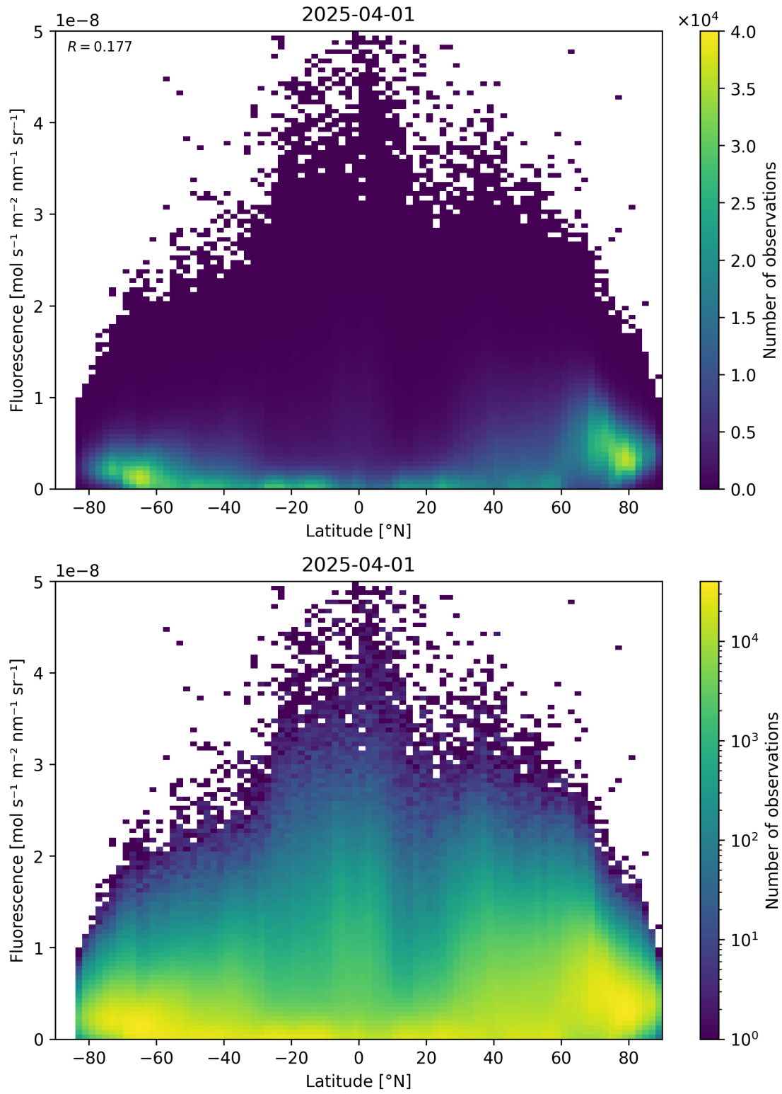
Figure 92: Scatter density plot of “Latitude” against “Fluorescence” for 2025-03-31 to 2025-04-02.
