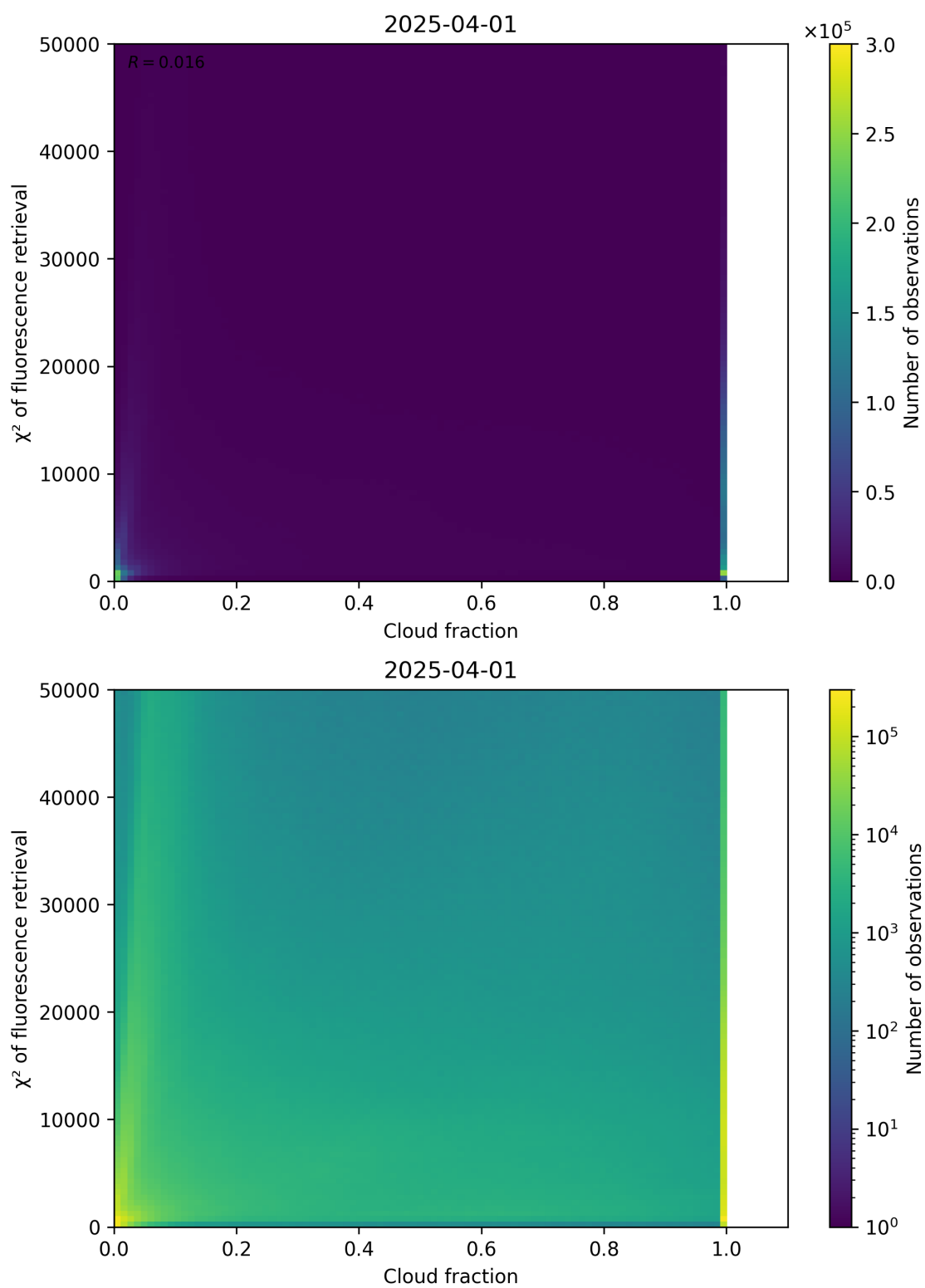
Figure 71: Scatter density plot of “Cloud fraction” against “ \chi^2 of fluorescence retrieval” for 2025-03-31 to 2025-04-02.
