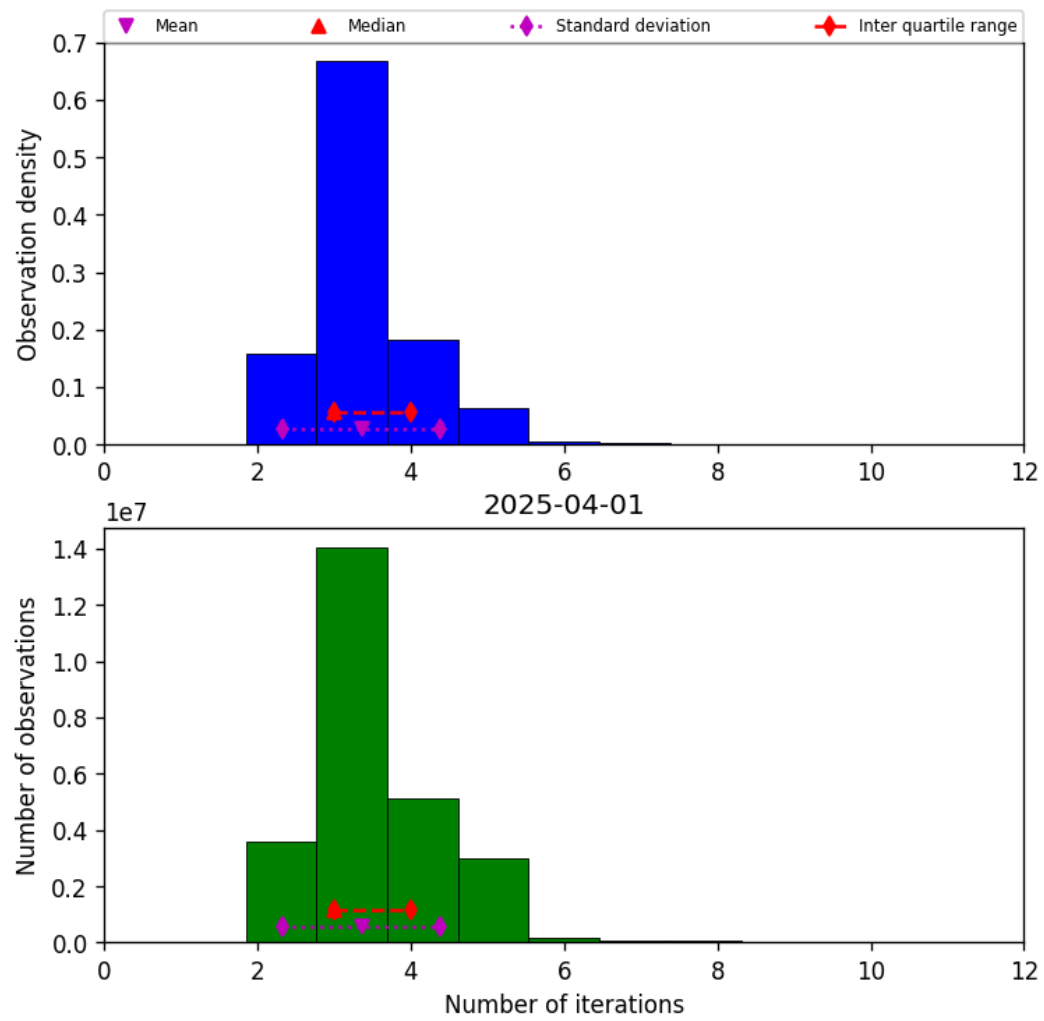
Figure 39: Histogram of “Number of iterations” for 2025-03-31 to 2025-04-02
