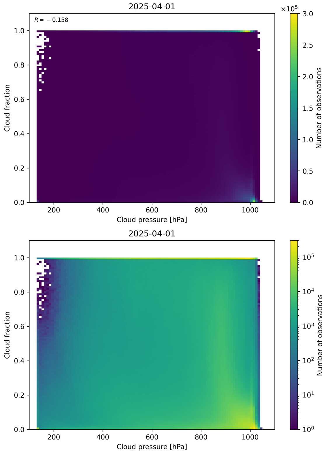
Figure 79: Scatter density plot of “Cloud pressure” against “Cloud fraction” for 2025-03-31 to 2025-04-02.
