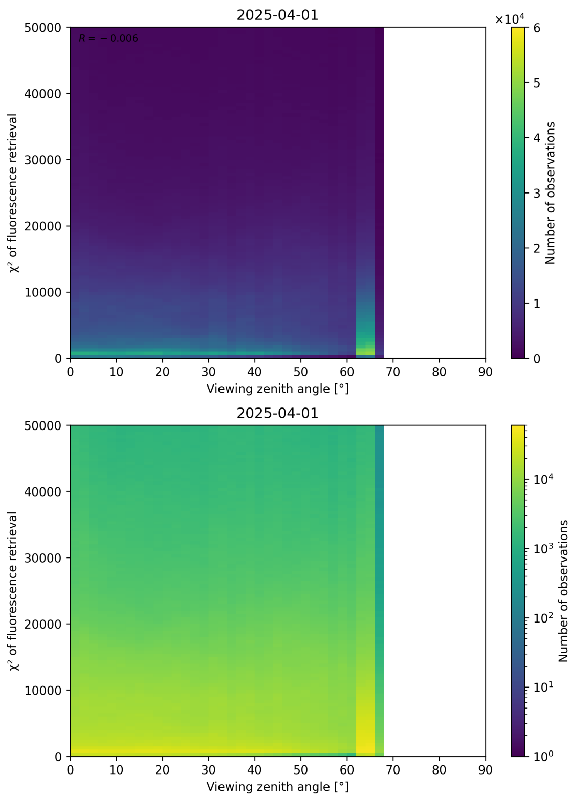
Figure 119: Scatter density plot of “Viewing zenith angle” against “ \chi^2 of fluorescence retrieval” for 2025-03-31 to 2025-04-02.
