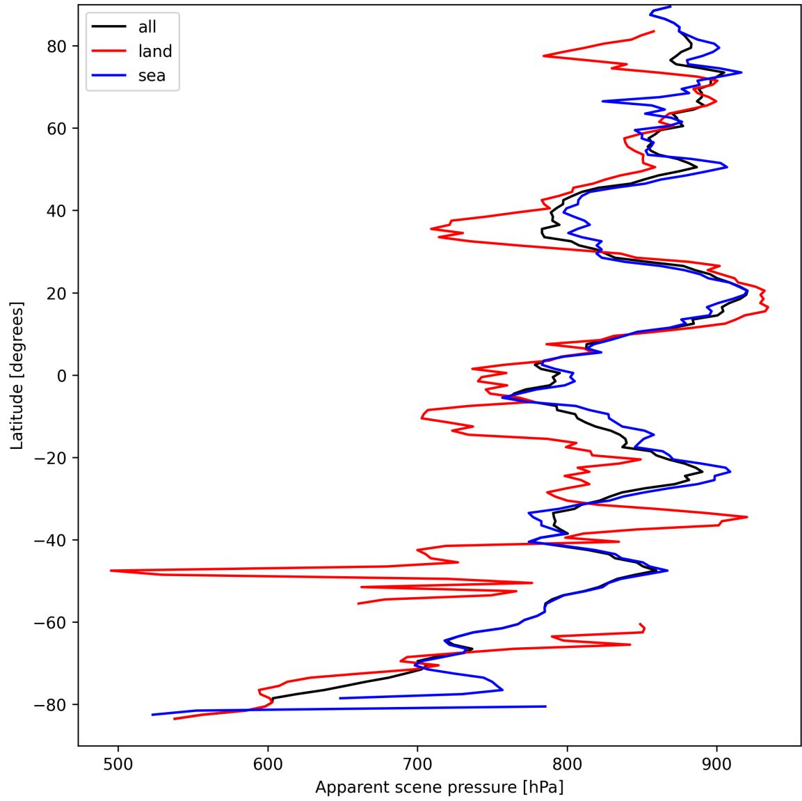
Figure 19: Zonal average of “Apparent scene pressure” for 2025-03-31 to 2025-04-02.
