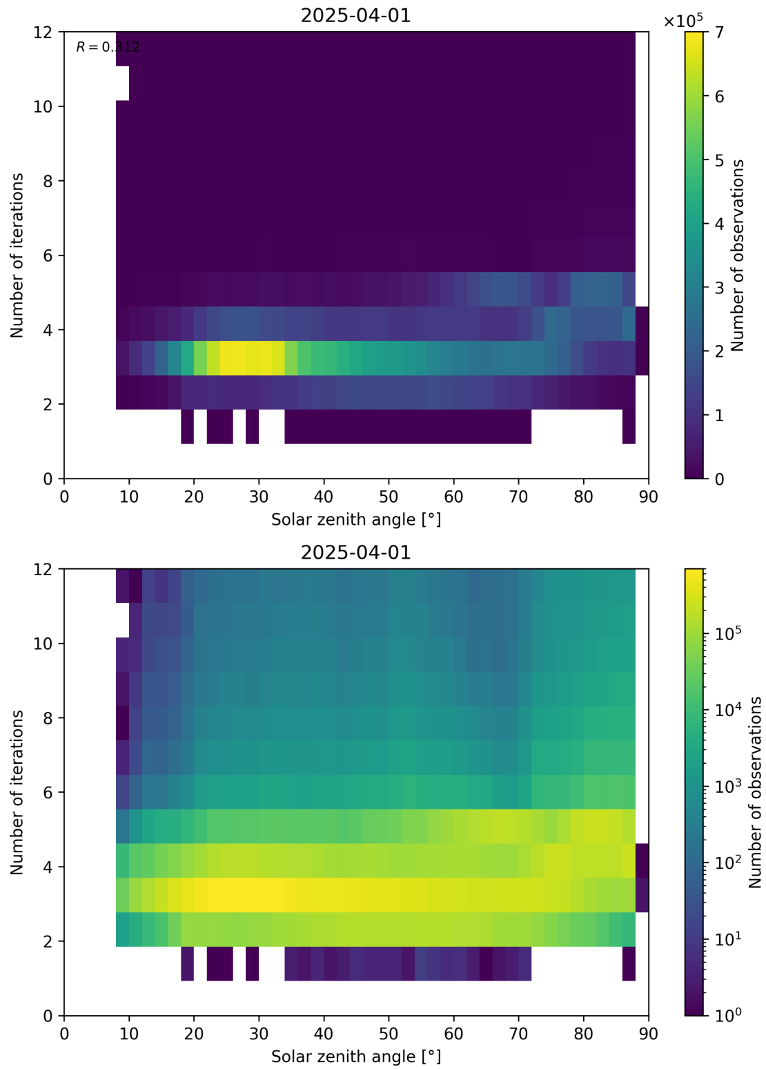
Figure 114: Scatter density plot of “Solar zenith angle” against “Number of iterations” for 2025-03-31 to 2025-04-02.
