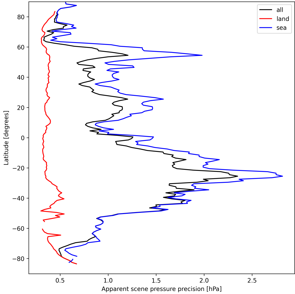
Figure 20: Zonal average of “Apparent scene pressure precision” for 2025-03-31 to 2025-04-02.
