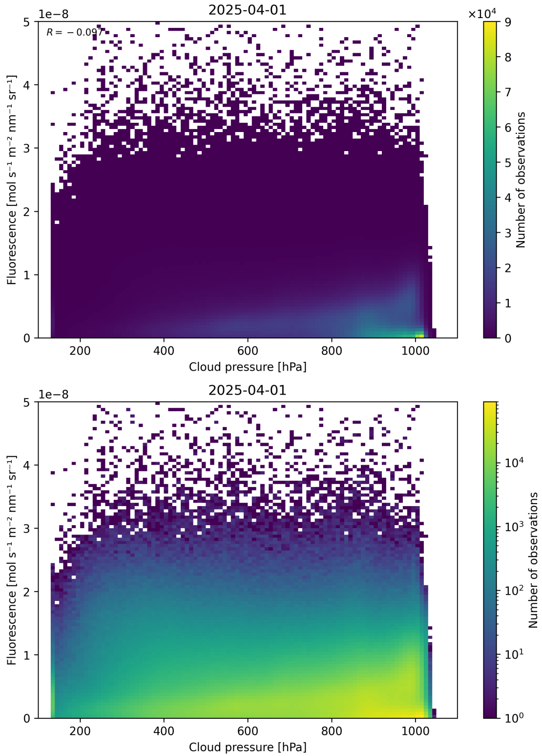
Figure 80: Scatter density plot of “Cloud pressure” against “Fluorescence” for 2025-03-31 to 2025-04-02.
