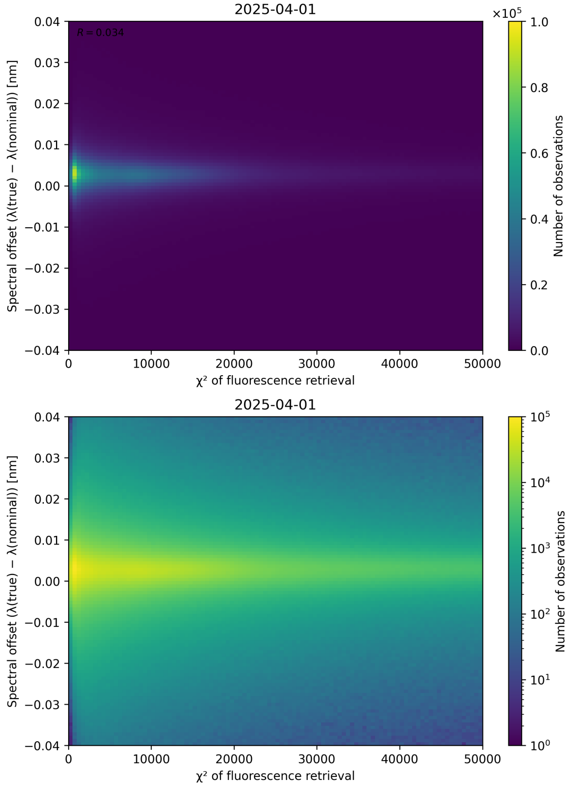
Figure 69: Scatter density plot of “ \chi^2 of fluorescence retrieval” against “Spectral offset ( \lambda_{\text{true}} - \lambda_{\text{nominal}} )” for 2025-03-31 to 2025-04-02.
