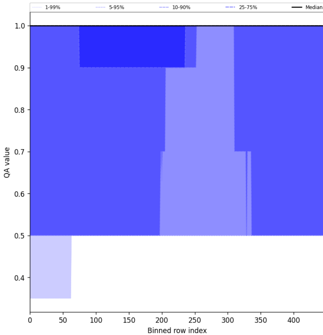
Figure 46: Along track statistics of “QA value” for 2025-03-31 to 2025-04-02
