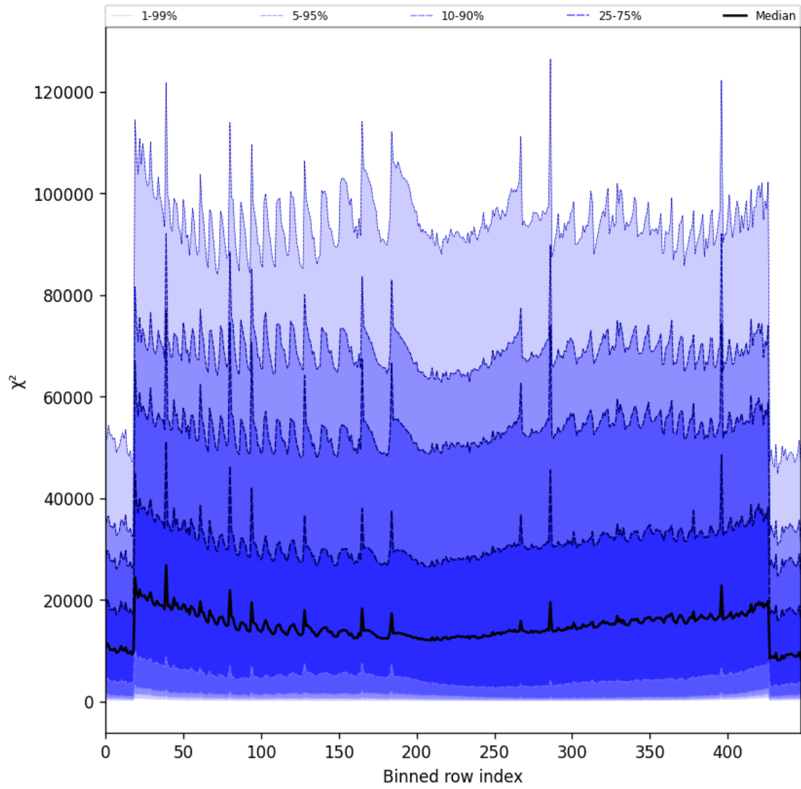
Figure 55: Along track statistics of “ \chi^2 ” for 2025-03-31 to 2025-04-02
