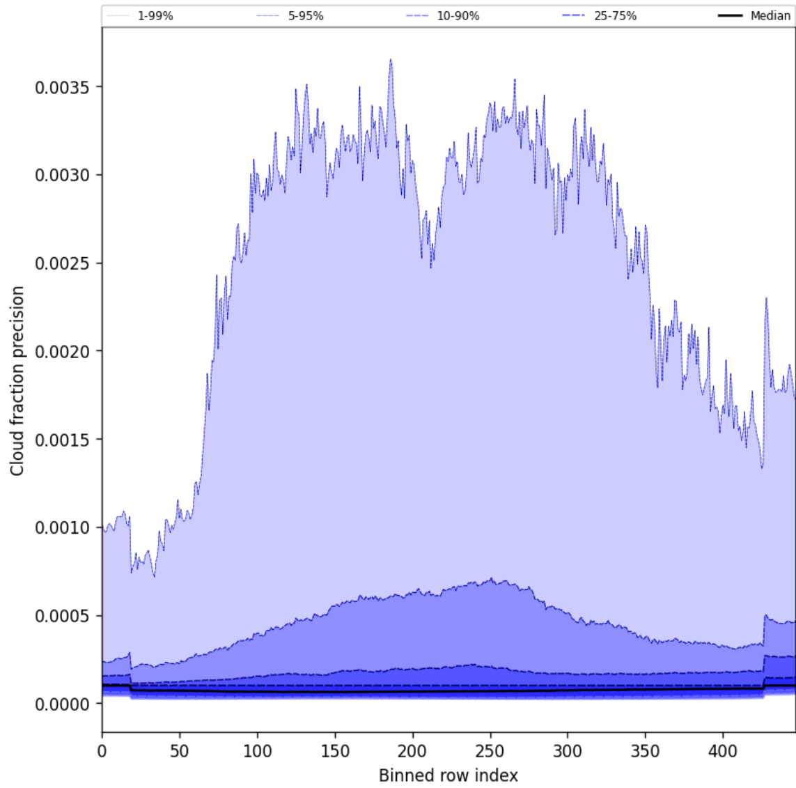
Figure 50: Along track statistics of “Cloud fraction precision” for 2025-03-31 to 2025-04-02
