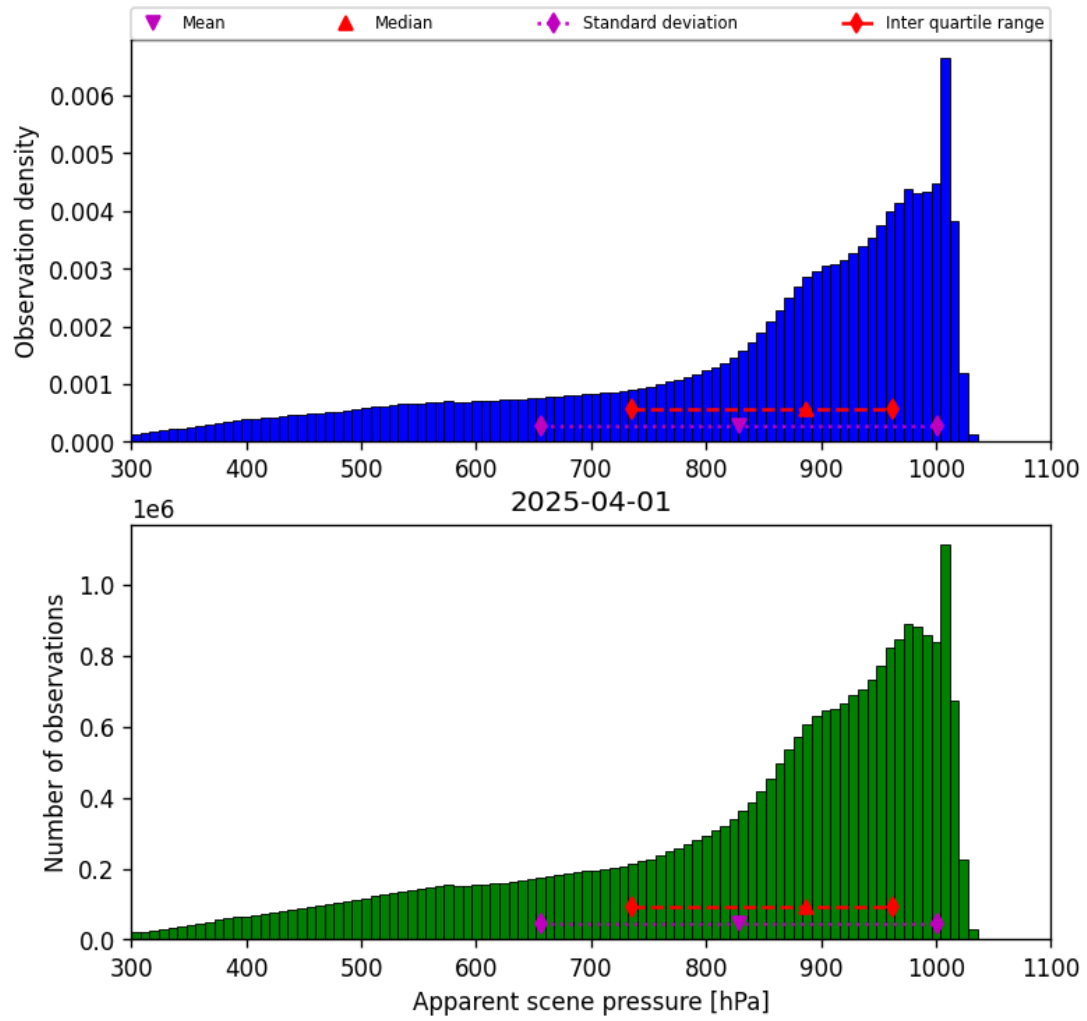
Figure 36: Histogram of “Apparent scene pressure” for 2025-03-31 to 2025-04-02
