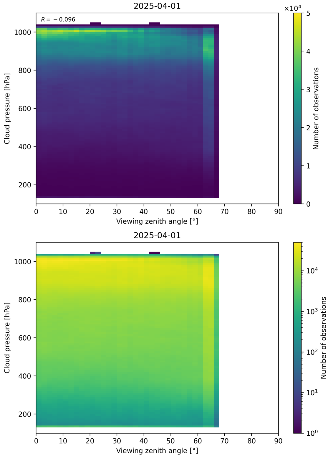
Figure 121: Scatter density plot of “Viewing zenith angle” against “Cloud pressure” for 2025-03-31 to 2025-04-02.
