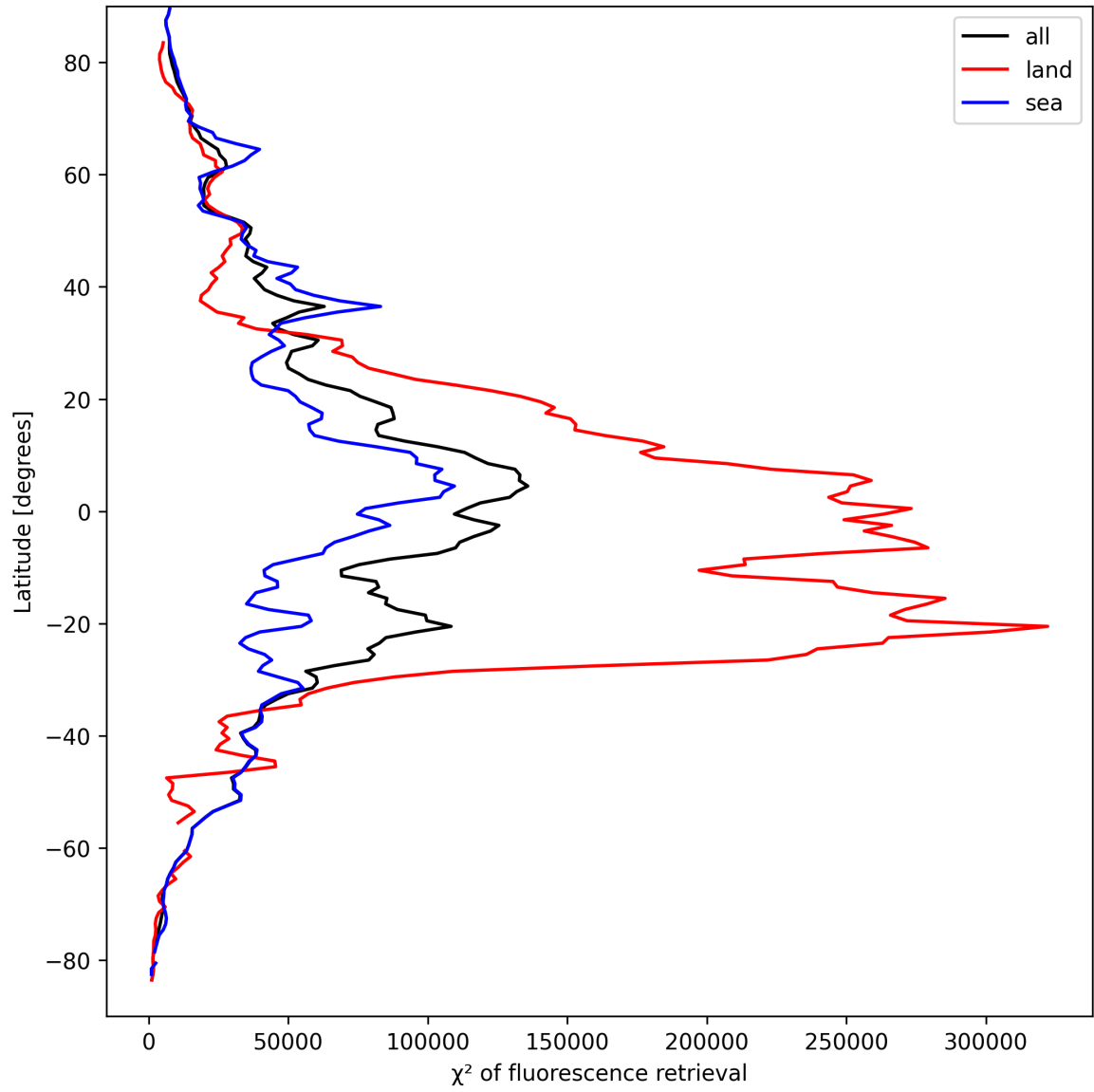
Figure 25: Zonal average of “ \chi^2 of fluorescence retrieval” for 2025-03-31 to 2025-04-02.
