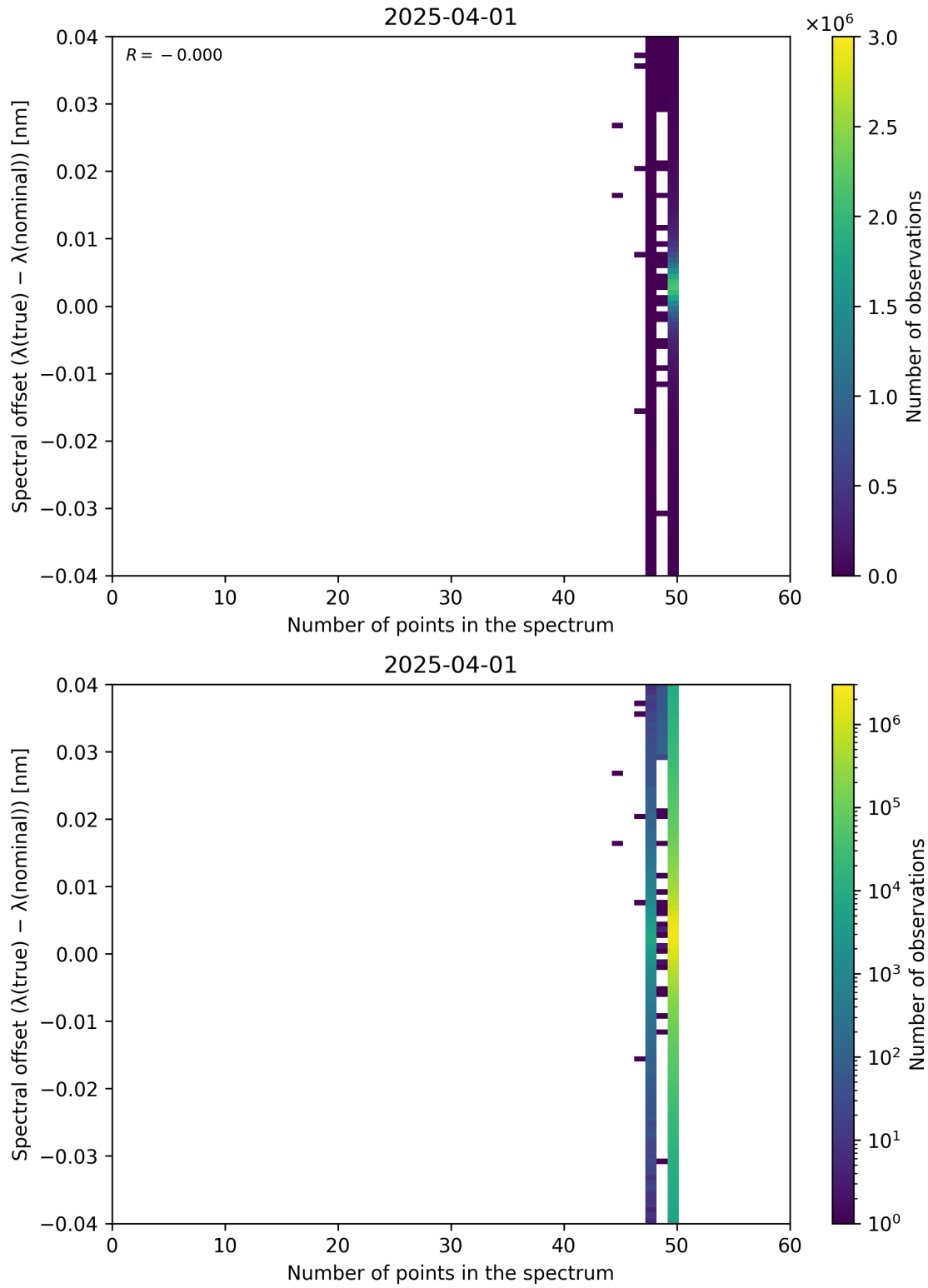
Figure 101: Scatter density plot of “Number of points in the spectrum” against “Spectral offset ( \lambda_{\text{true}} - \lambda_{\text{nominal}} )” for 2025-03-31 to 2025-04-02.
