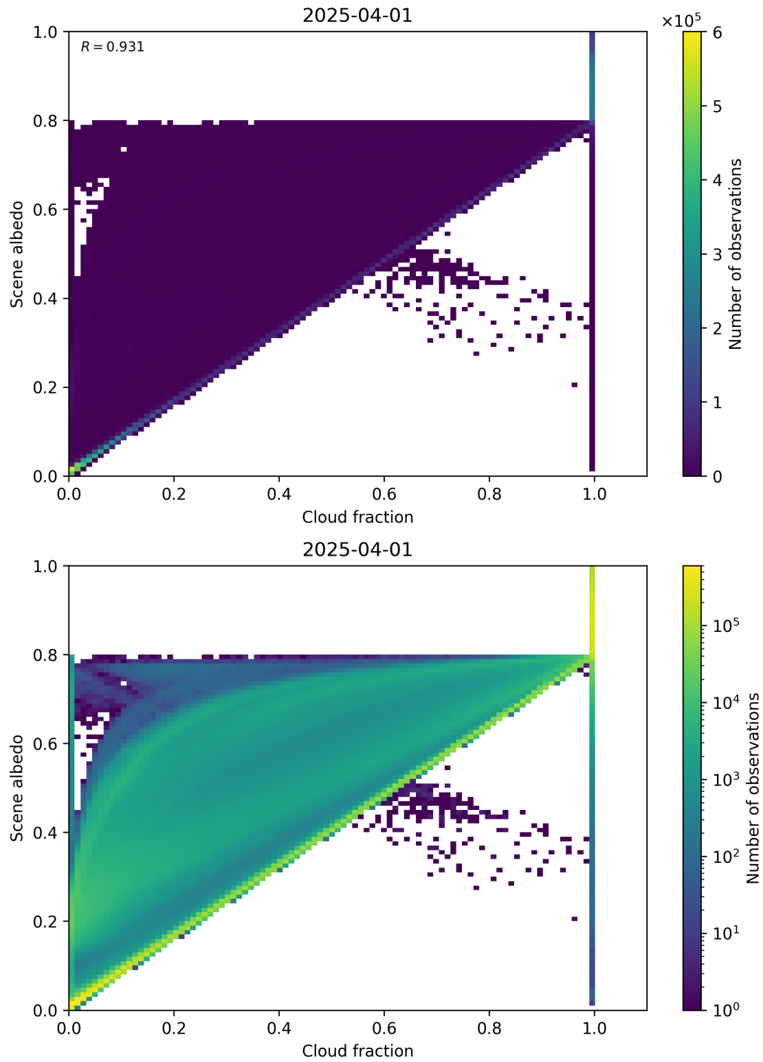
Figure 75: Scatter density plot of “Cloud fraction” against “Scene albedo” for 2025-03-31 to 2025-04-02.
