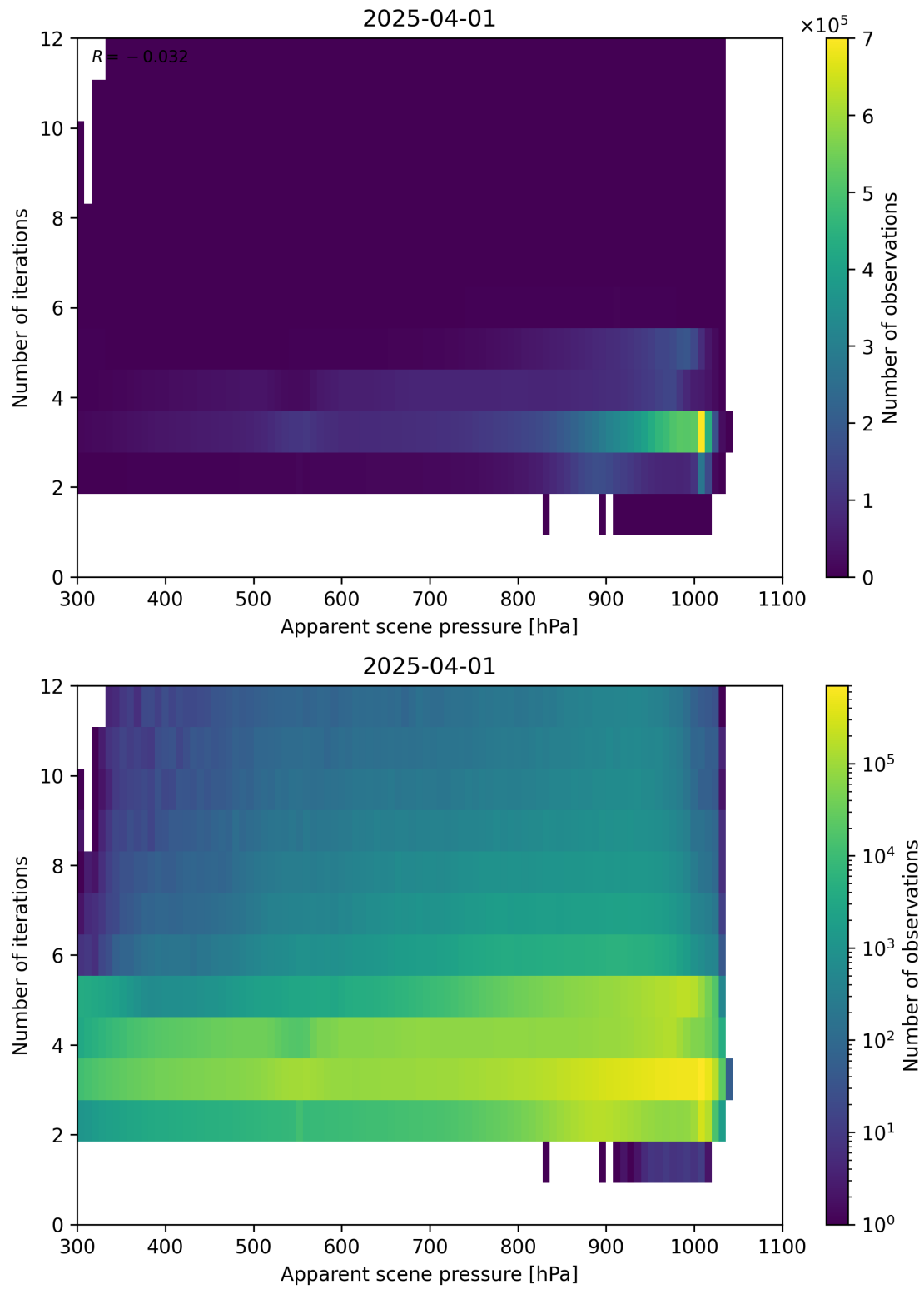
Figure 65: Scatter density plot of “Apparent scene pressure” against “Number of iterations” for 2025-03-31 to 2025-04-02.
