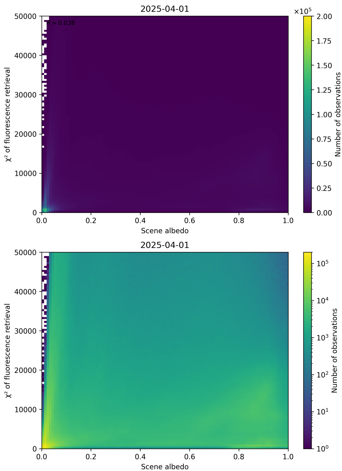
Figure 103: Scatter density plot of “Scene albedo” against “ \chi^2 of fluorescence retrieval” for 2025-03-31 to 2025-04-02.
