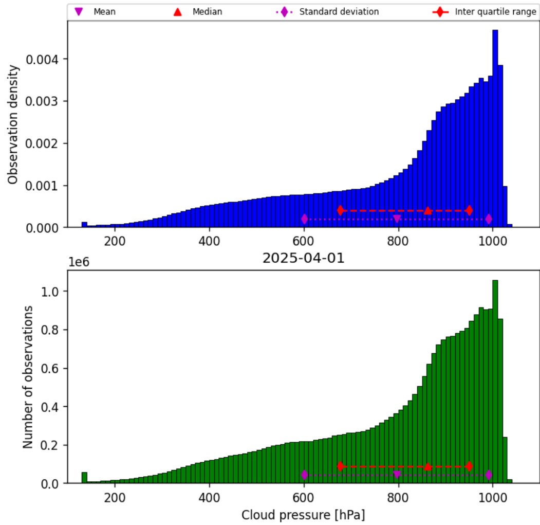
Figure 30: Histogram of “Cloud pressure” for 2025-03-31 to 2025-04-02
