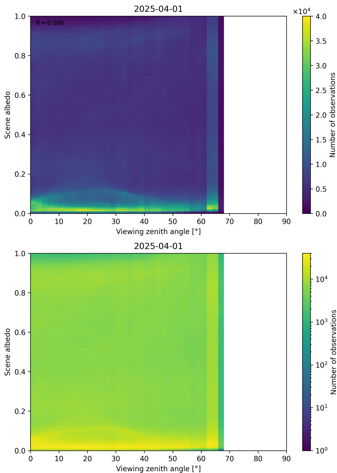
Figure 126: Scatter density plot of “Viewing zenith angle” against “Scene albedo” for 2025-03-31 to 2025-04-02.
