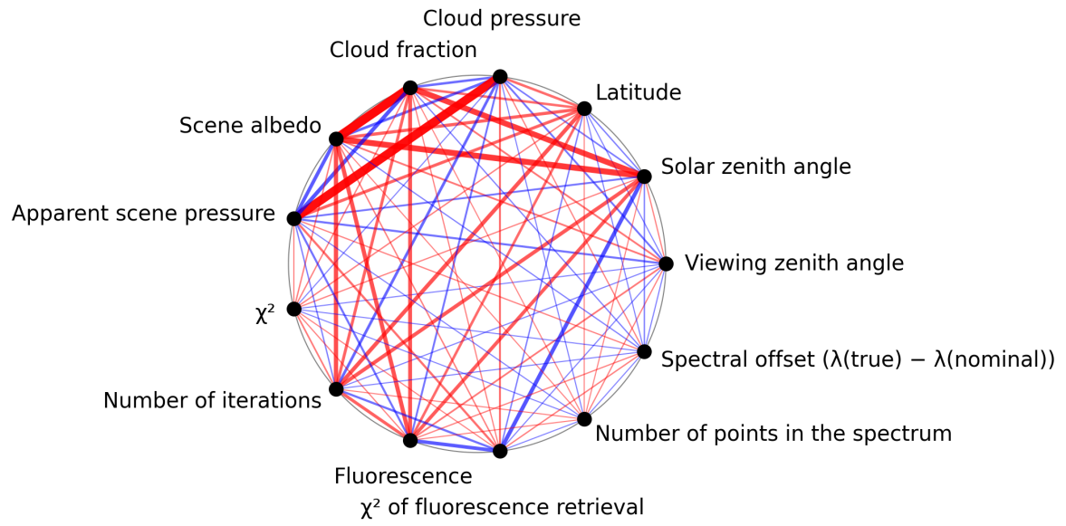
Figure 1: Map of correlation graph for 2025-03-31 to 2025-04-02.
