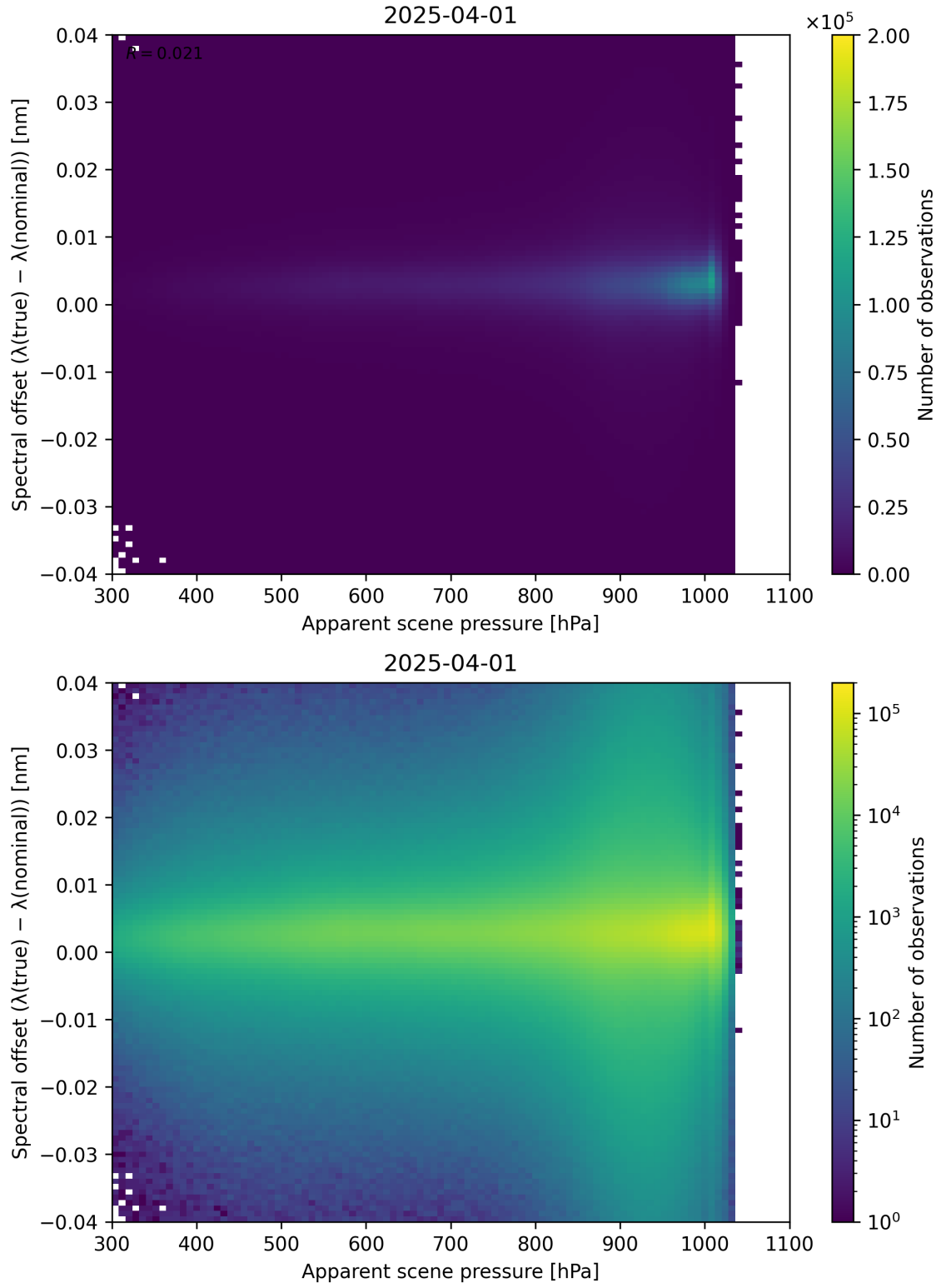
Figure 67: Scatter density plot of “Apparent scene pressure” against “Spectral offset ( \lambda_{\text{true}} - \lambda_{\text{nominal}} )” for 2025-03-31 to 2025-04-02.
