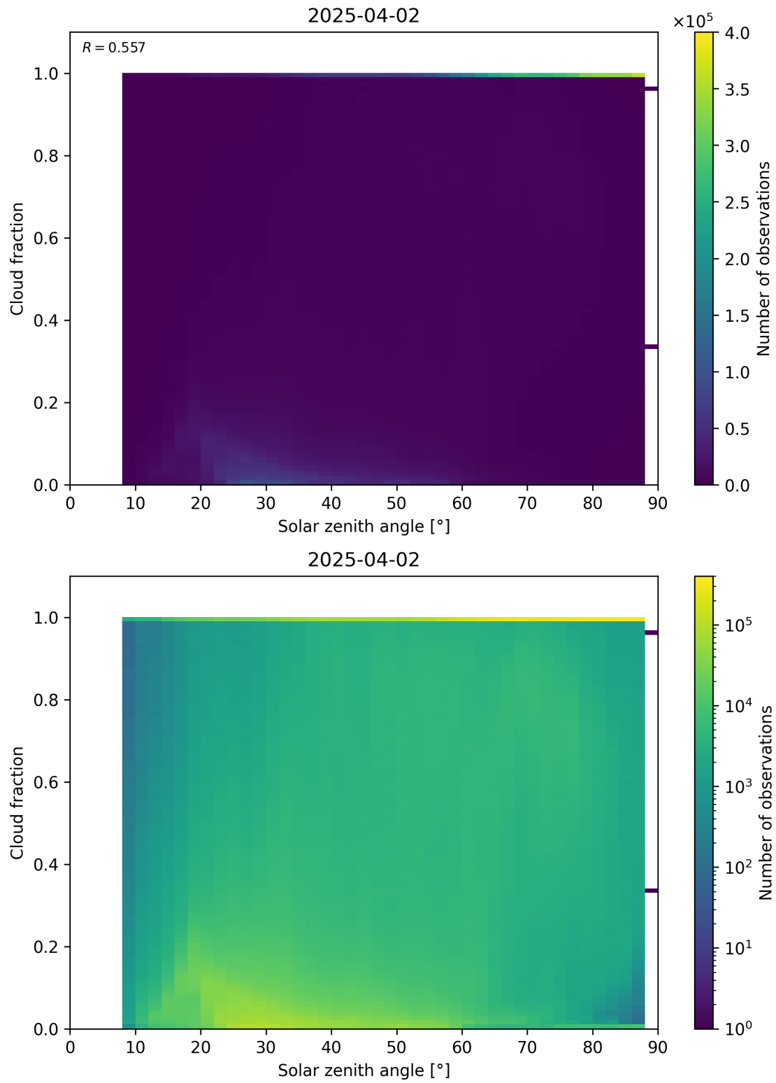
Figure 110: Scatter density plot of “Solar zenith angle” against “Cloud fraction” for 2025-04-02 to 2025-04-03.
