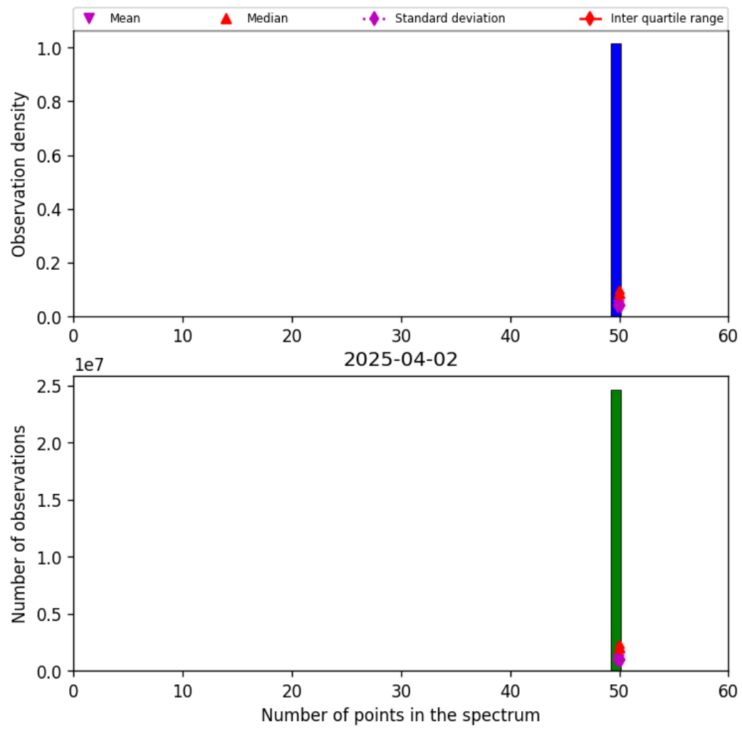
Figure 44: Histogram of “Number of points in the spectrum” for 2025-04-02 to 2025-04-03
