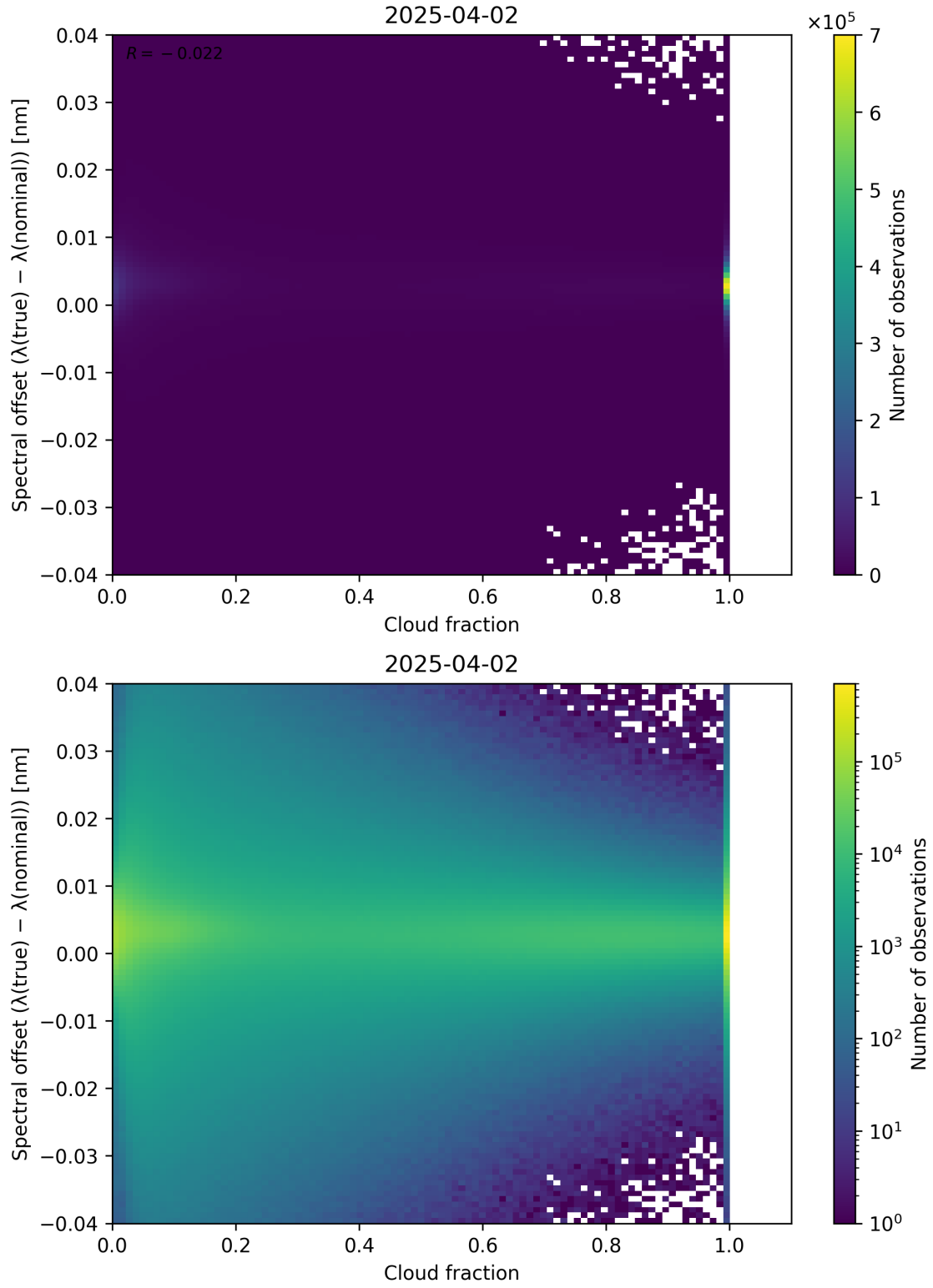
Figure 76: Scatter density plot of “Cloud fraction” against “Spectral offset ( \lambda_{\text{true}} - \lambda_{\text{nominal}} )” for 2025-04-02 to 2025-04-03.
