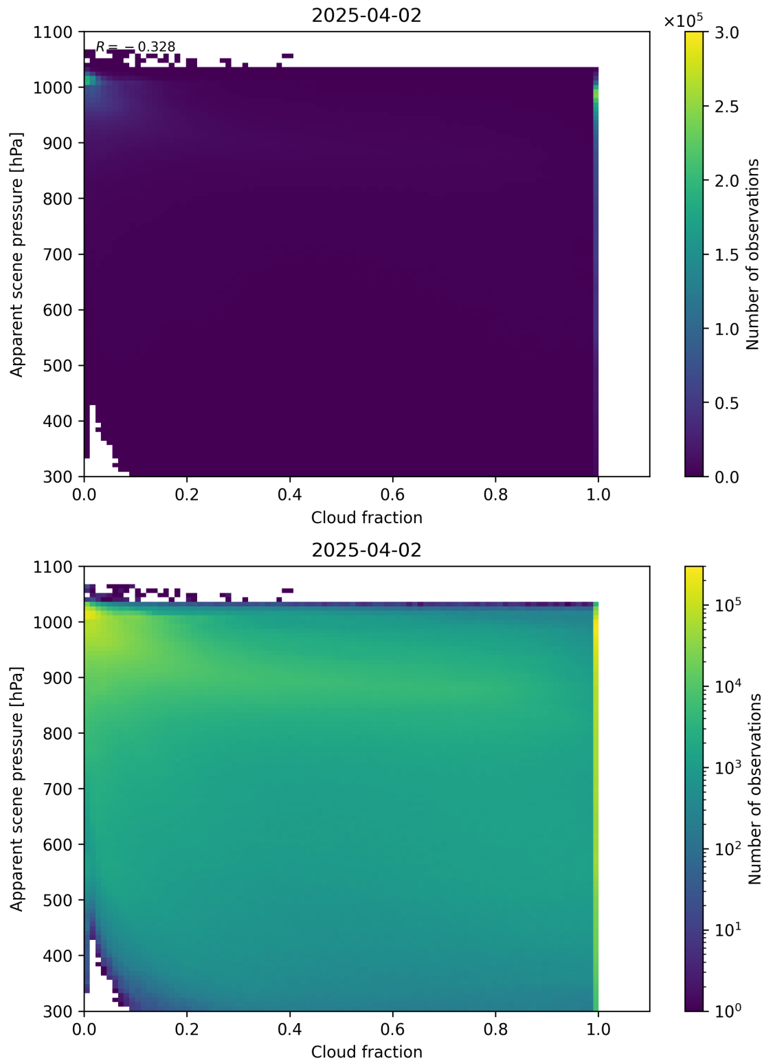
Figure 70: Scatter density plot of “Cloud fraction” against “Apparent scene pressure” for 2025-04-02 to 2025-04-03.
