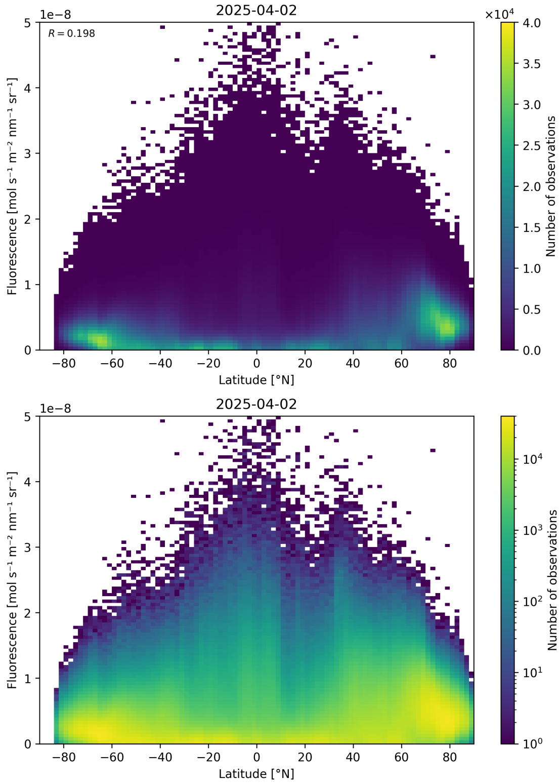
Figure 92: Scatter density plot of “Latitude” against “Fluorescence” for 2025-04-02 to 2025-04-03.
