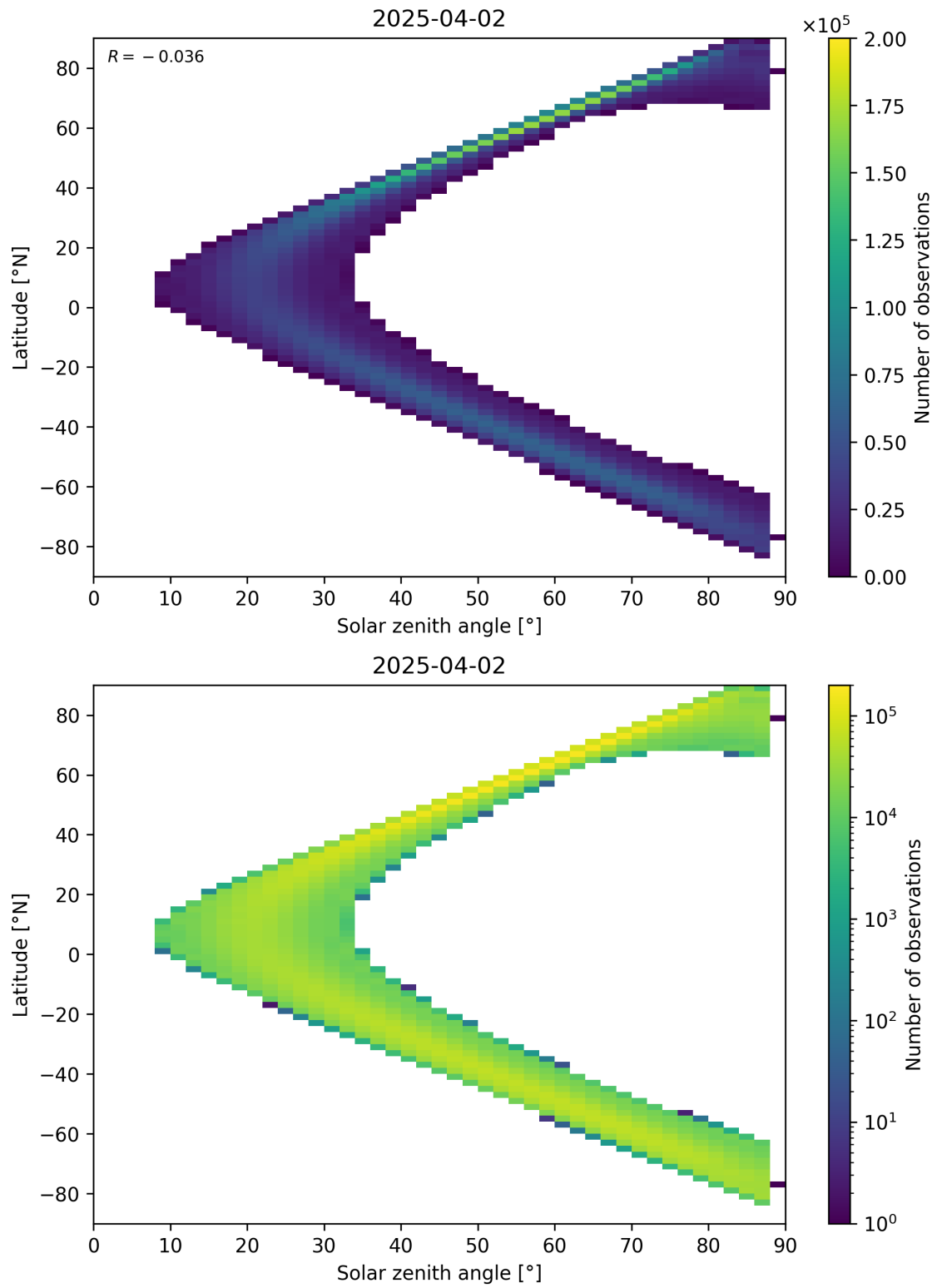
Figure 113: Scatter density plot of “Solar zenith angle” against “Latitude” for 2025-04-02 to 2025-04-03.
