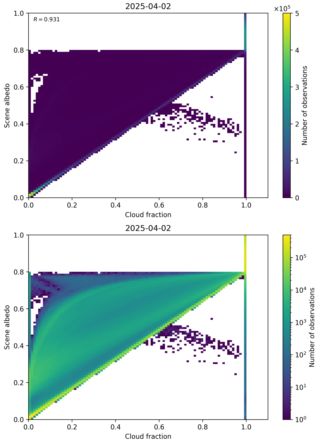
Figure 75: Scatter density plot of “Cloud fraction” against “Scene albedo” for 2025-04-02 to 2025-04-03.
