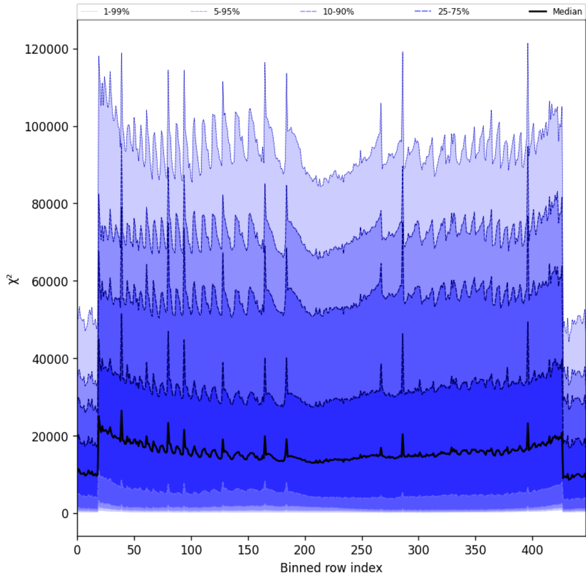
Figure 55: Along track statistics of “ \chi^2 ” for 2025-04-02 to 2025-04-03
