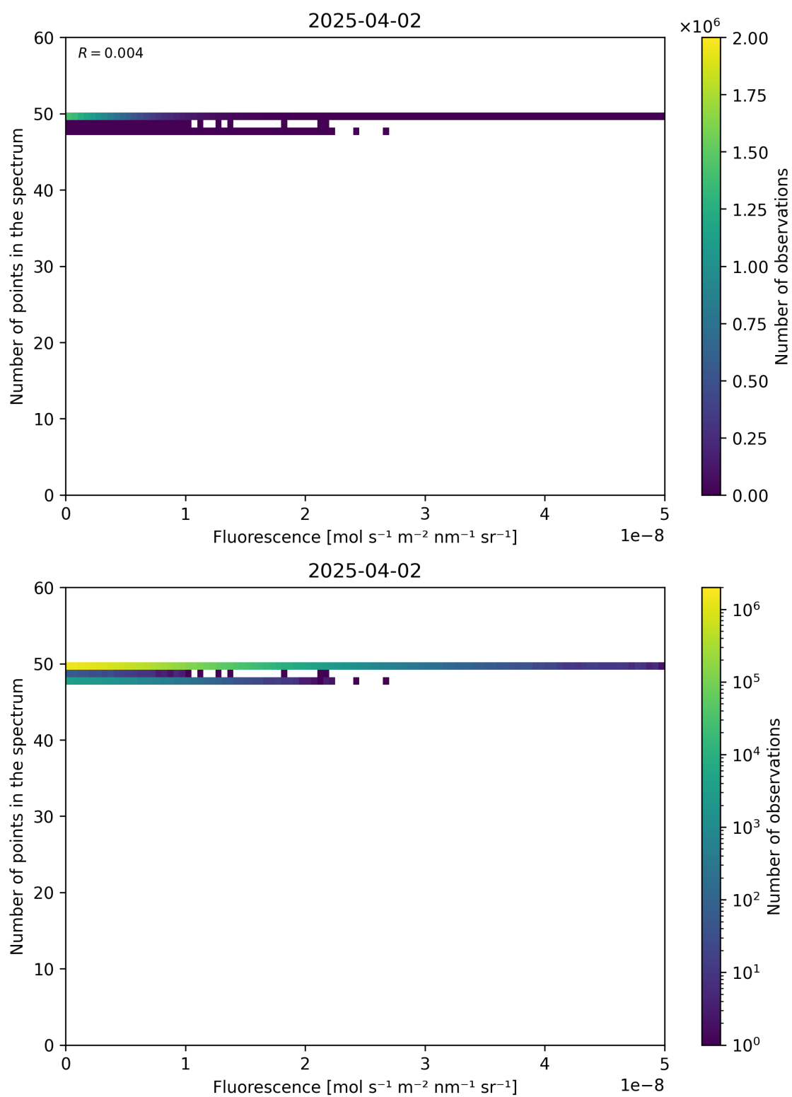
Figure 86: Scatter density plot of “Fluorescence” against “Number of points in the spectrum” for 2025-04-02 to 2025-04-03.
