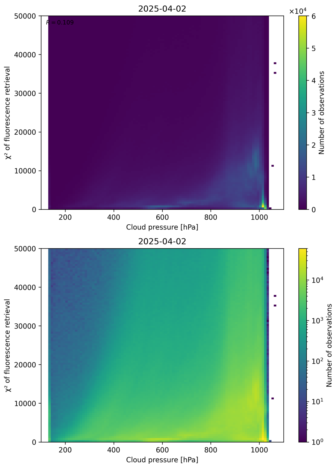
Figure 78: Scatter density plot of “Cloud pressure” against “ \chi^2 of fluorescence retrieval” for 2025-04-02 to 2025-04-03.
