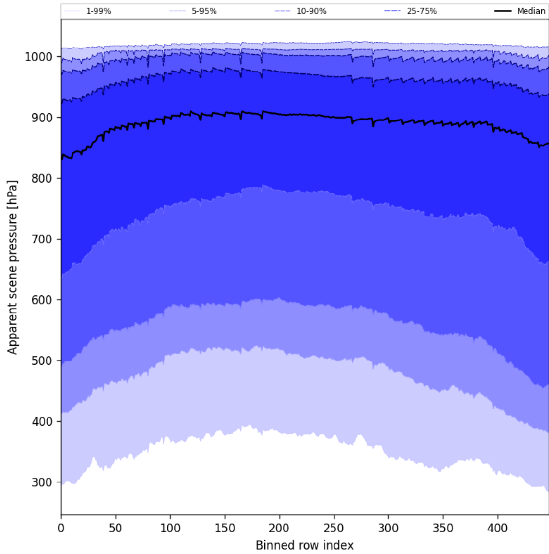
Figure 53: Along track statistics of “Apparent scene pressure” for 2025-04-02 to 2025-04-03
