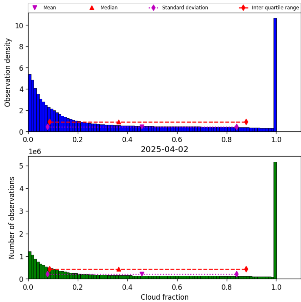
Figure 32: Histogram of “Cloud fraction” for 2025-04-02 to 2025-04-03
