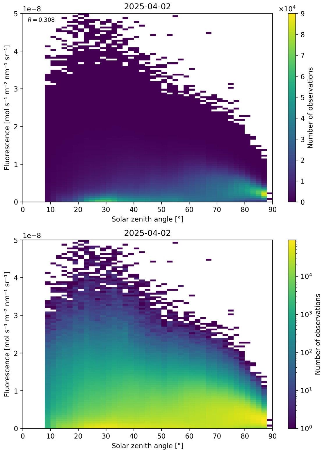
Figure 112: Scatter density plot of “Solar zenith angle” against “Fluorescence” for 2025-04-02 to 2025-04-03.
