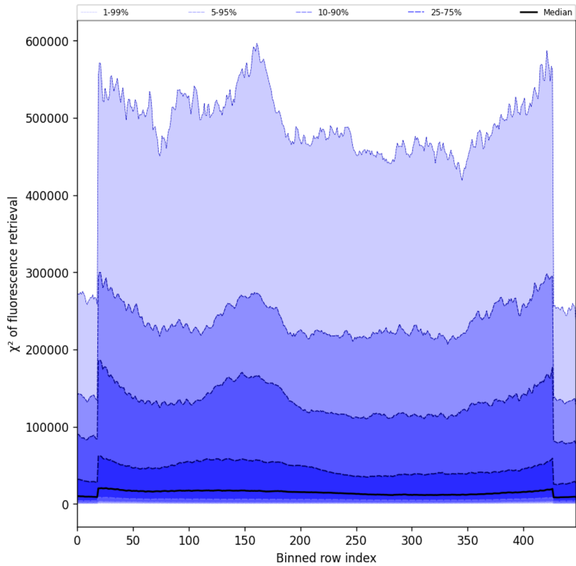
Figure 59: Along track statistics of “ \chi^2 of fluorescence retrieval” for 2025-04-02 to 2025-04-03
