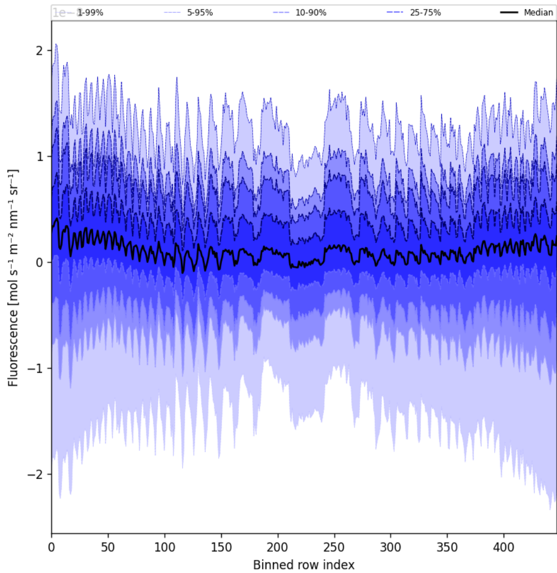
Figure 57: Along track statistics of “Fluorescence” for 2025-04-02 to 2025-04-03
