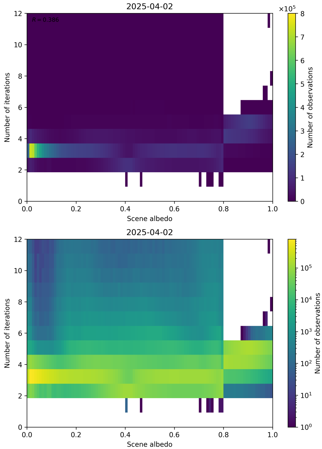
Figure 105: Scatter density plot of “Scene albedo” against “Number of iterations” for 2025-04-02 to 2025-04-03.
