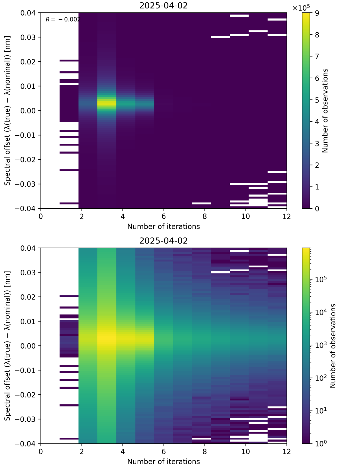
Figure 100: Scatter density plot of “Number of iterations” against “Spectral offset ( \lambda_{\text{true}} - \lambda_{\text{nominal}} )” for 2025-04-02 to 2025-04-03.
