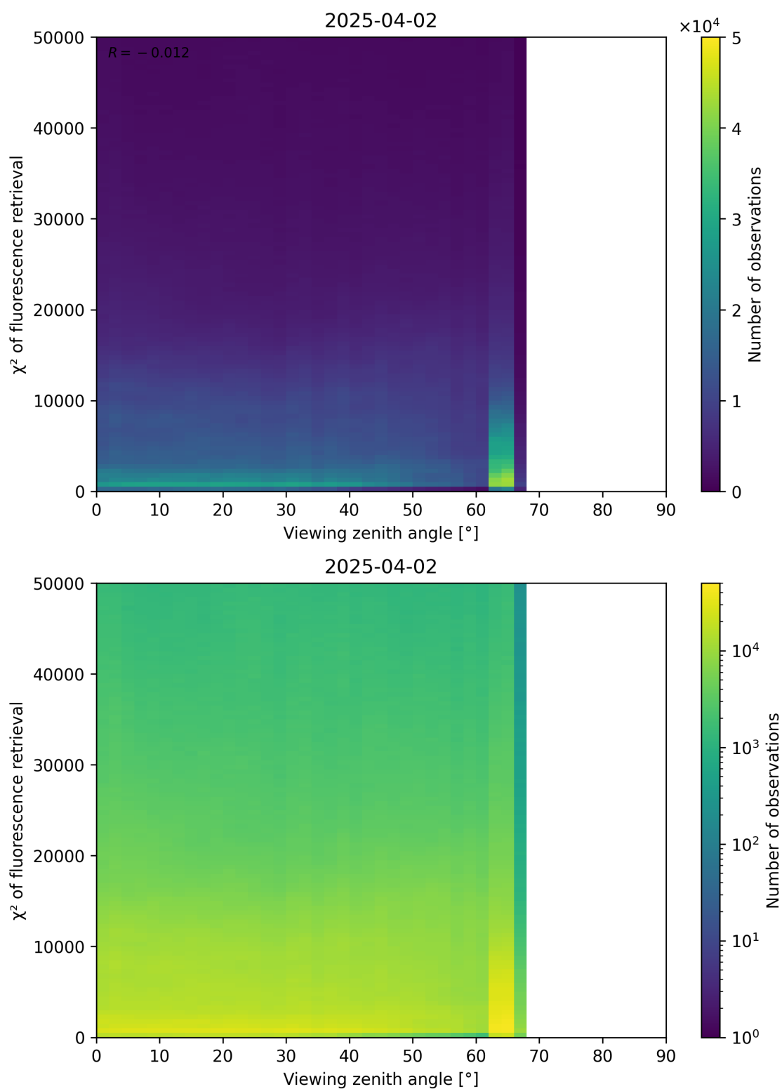
Figure 119: Scatter density plot of “Viewing zenith angle” against “ \chi^2 of fluorescence retrieval” for 2025-04-02 to 2025-04-03.
