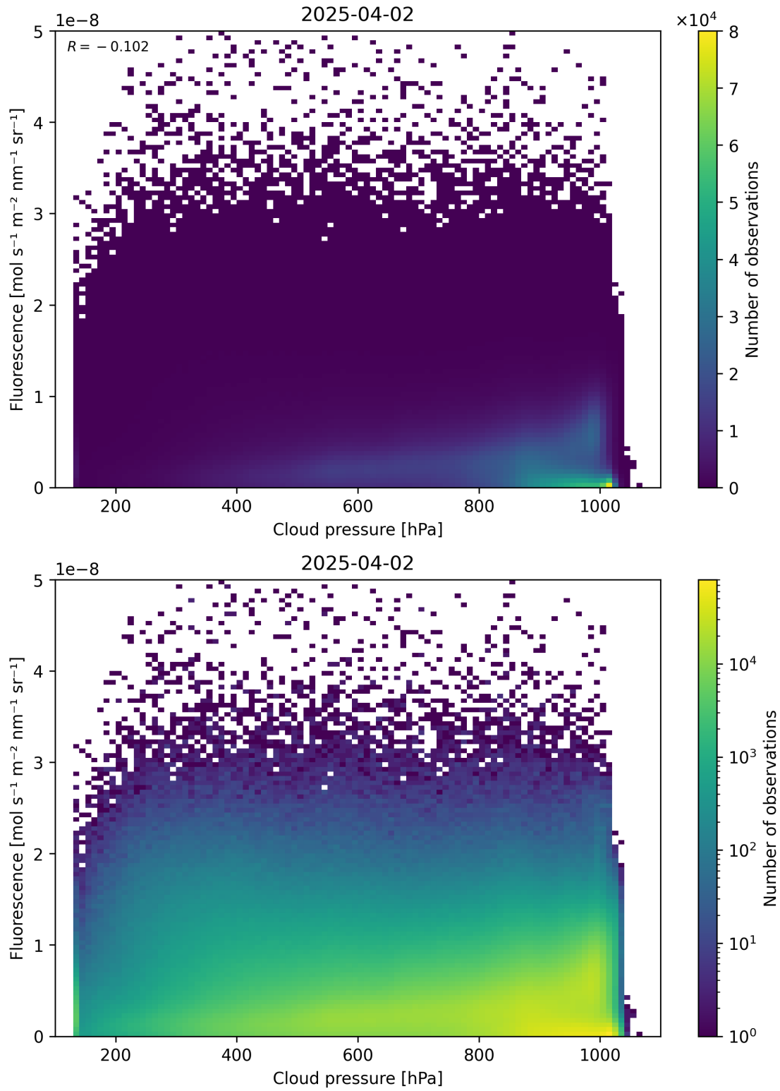
Figure 80: Scatter density plot of “Cloud pressure” against “Fluorescence” for 2025-04-02 to 2025-04-03.
