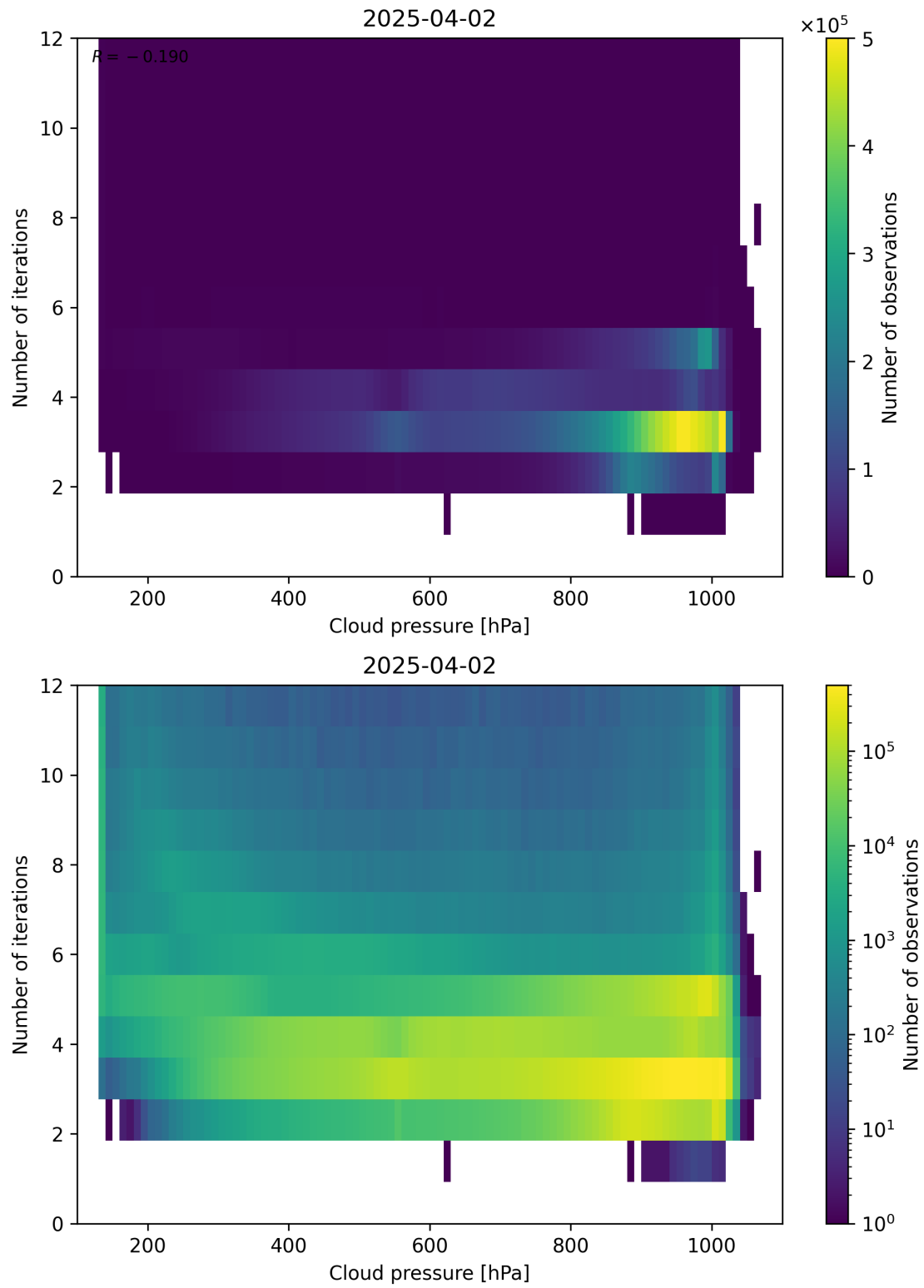
Figure 81: Scatter density plot of “Cloud pressure” against “Number of iterations” for 2025-04-02 to 2025-04-03.
