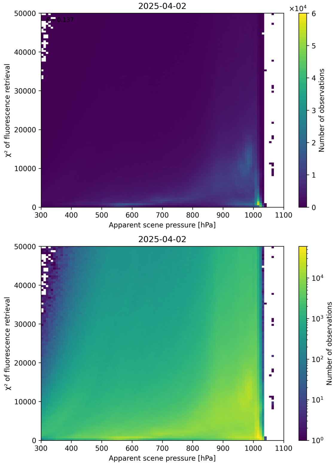
Figure 63: Scatter density plot of “Apparent scene pressure” against “ \chi^2 of fluorescence retrieval” for 2025-04-02 to 2025-04-03.
