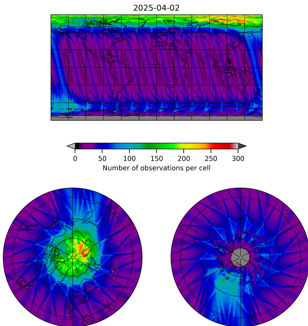
Figure 11: Map of the number of observations for 2025-04-02 to 2025-04-03
