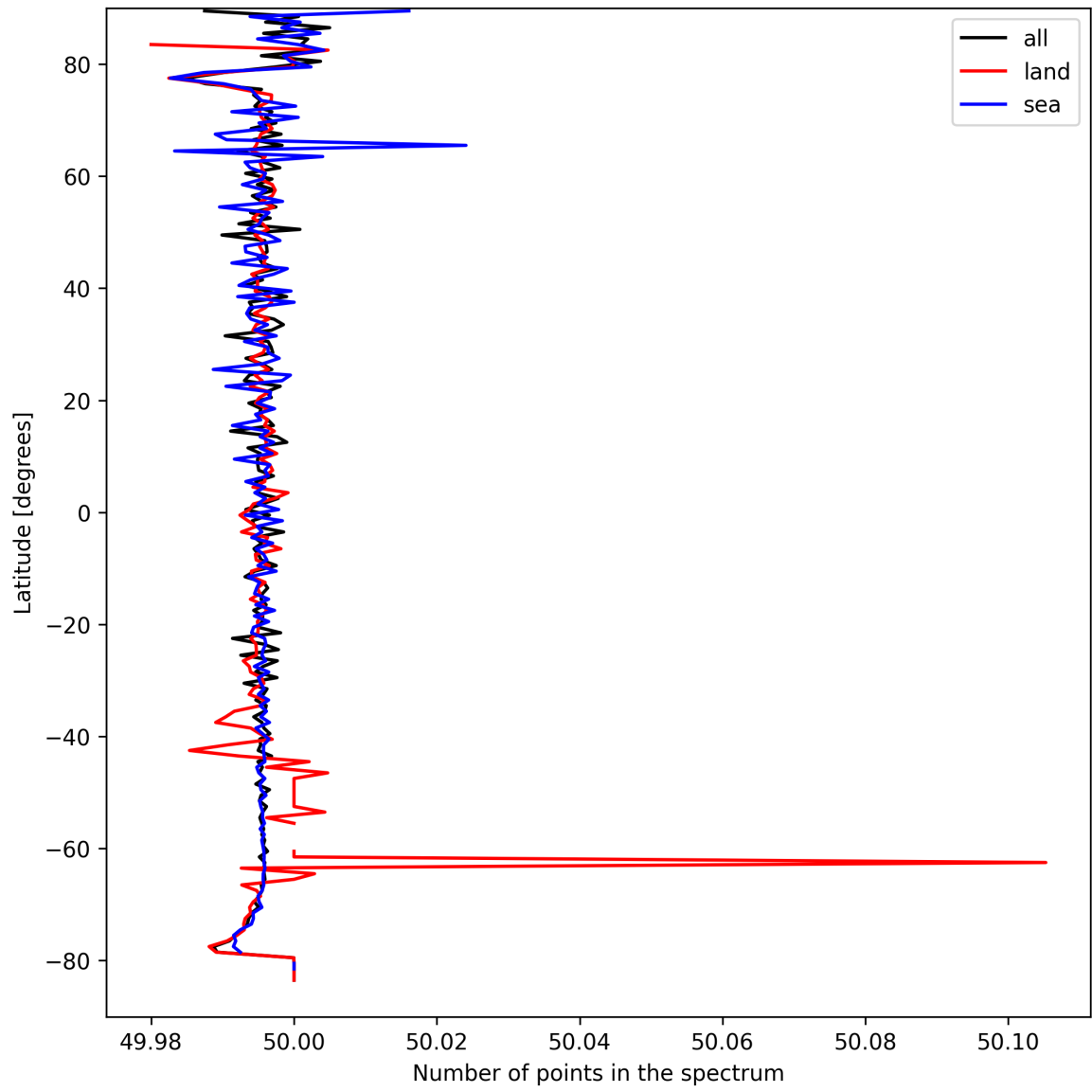
Figure 27: Zonal average of “Number of points in the spectrum” for 2025-04-02 to 2025-04-03.
