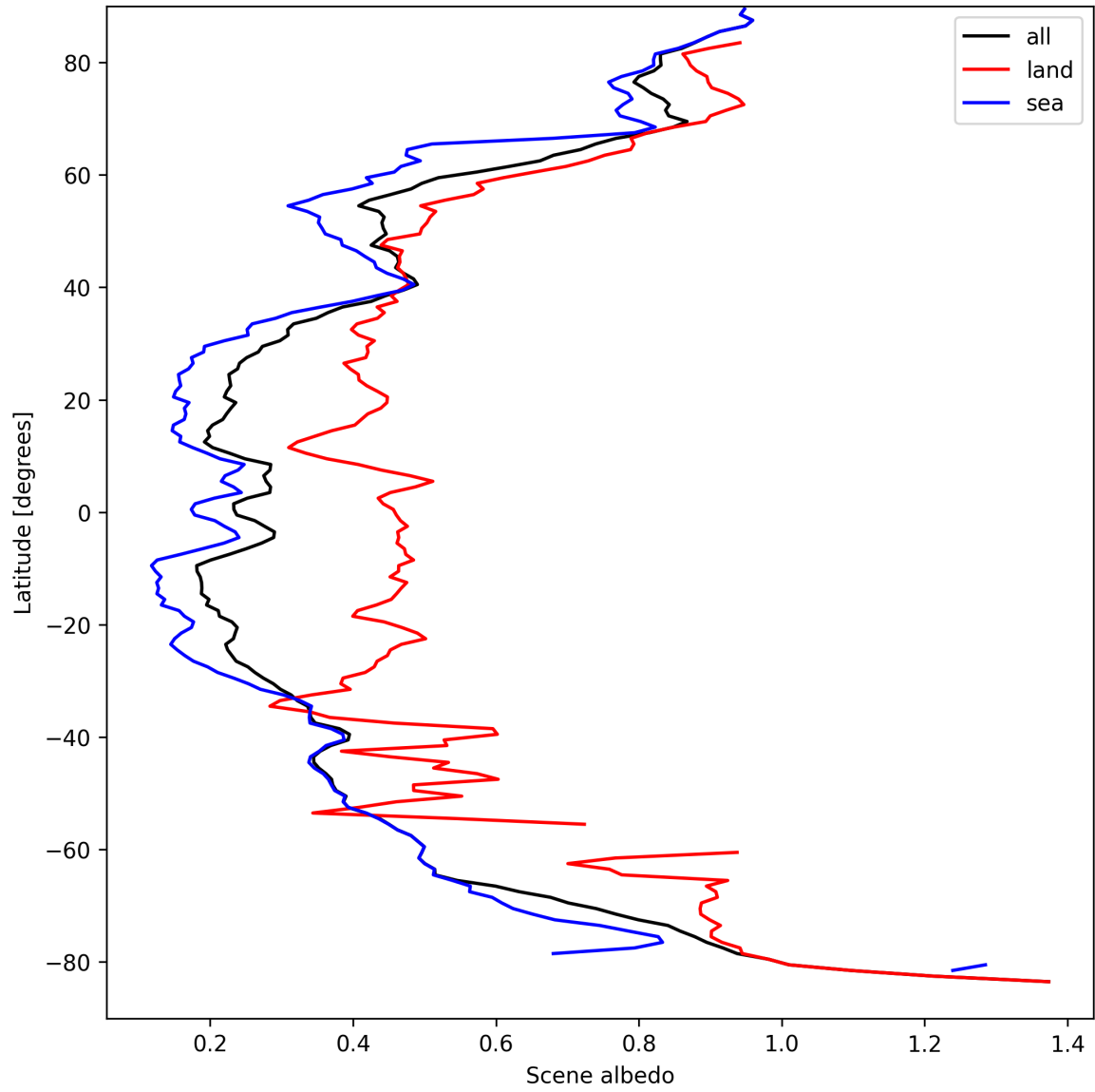
Figure 17: Zonal average of “Scene albedo” for 2025-04-02 to 2025-04-03.
