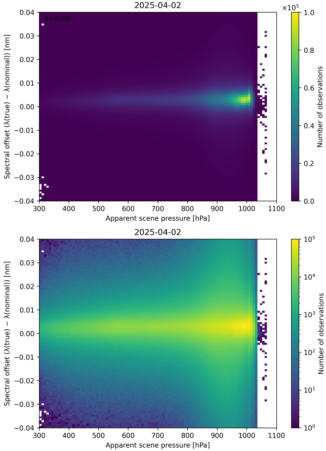
Figure 67: Scatter density plot of “Apparent scene pressure” against “Spectral offset ( \lambda_{\text{true}} - \lambda_{\text{nominal}} )” for 2025-04-02 to 2025-04-03.
