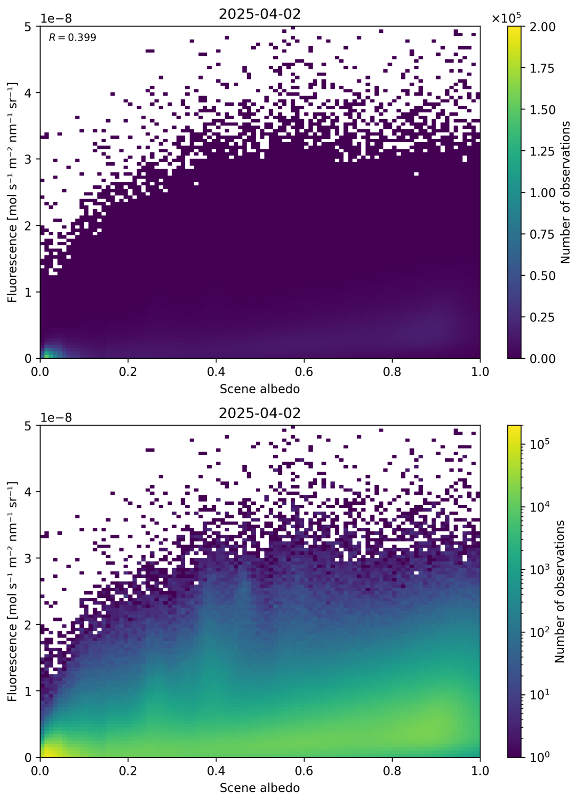
Figure 104: Scatter density plot of “Scene albedo” against “Fluorescence” for 2025-04-02 to 2025-04-03.
