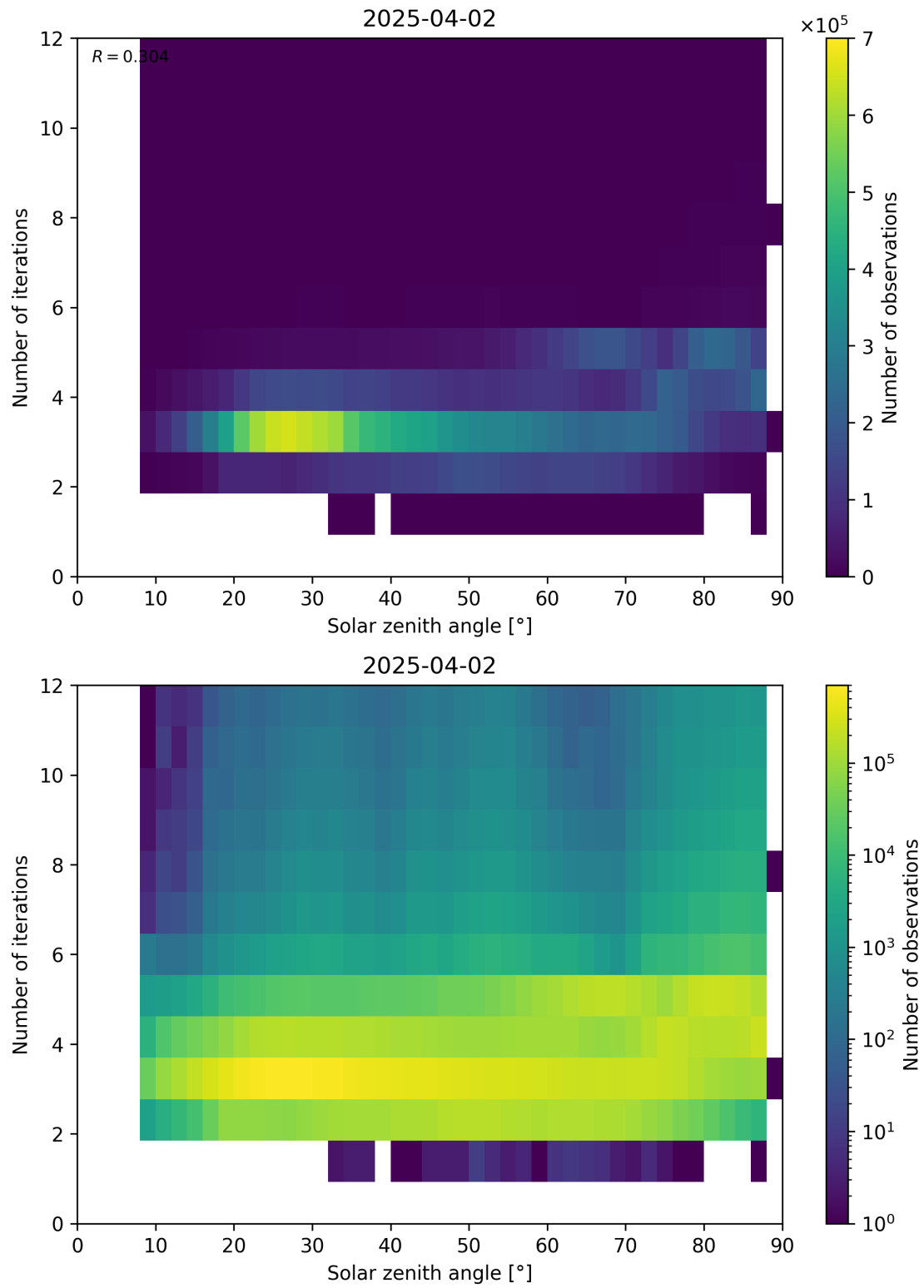
Figure 114: Scatter density plot of “Solar zenith angle” against “Number of iterations” for 2025-04-02 to 2025-04-03.
