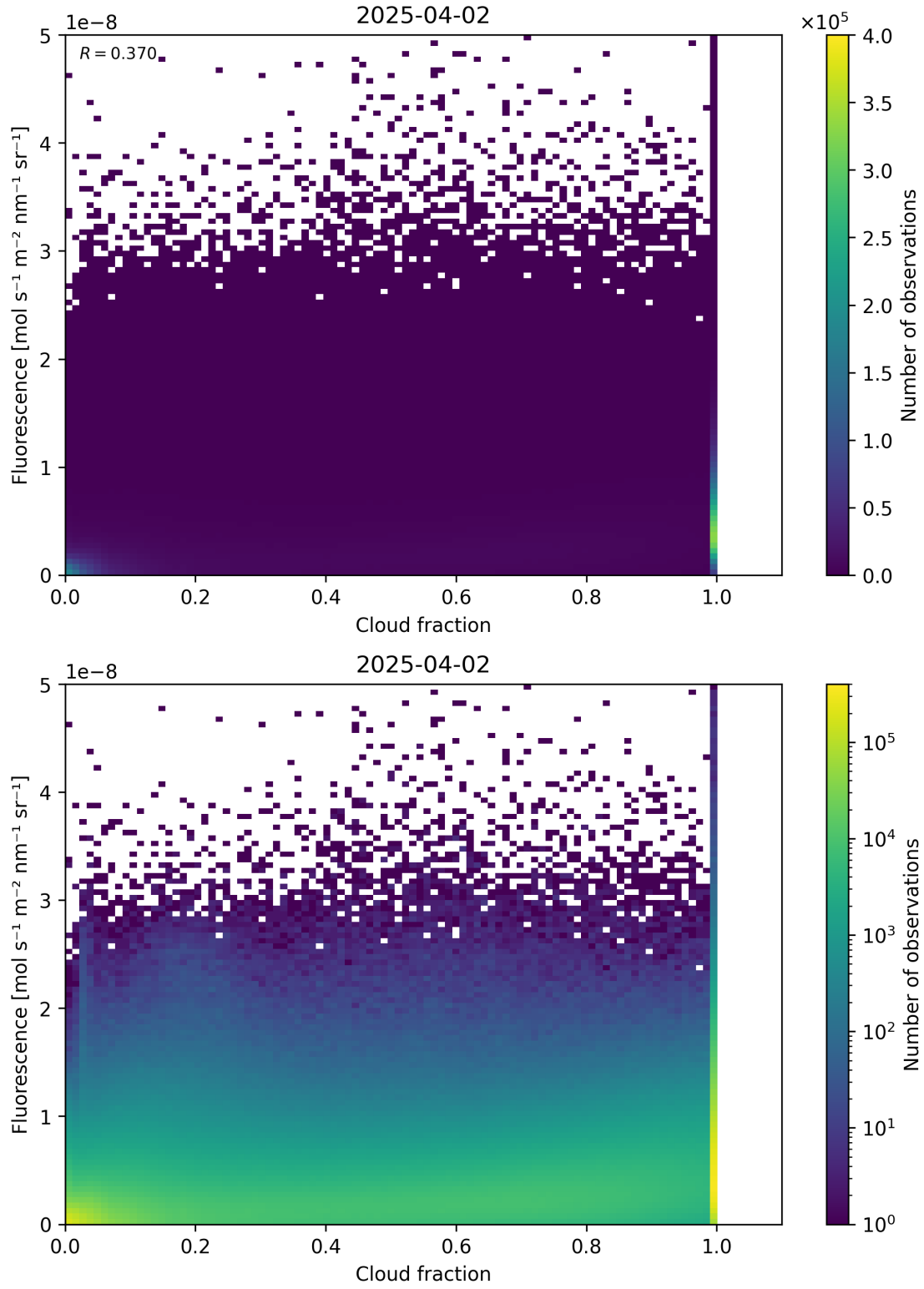
Figure 72: Scatter density plot of “Cloud fraction” against “Fluorescence” for 2025-04-02 to 2025-04-03.
