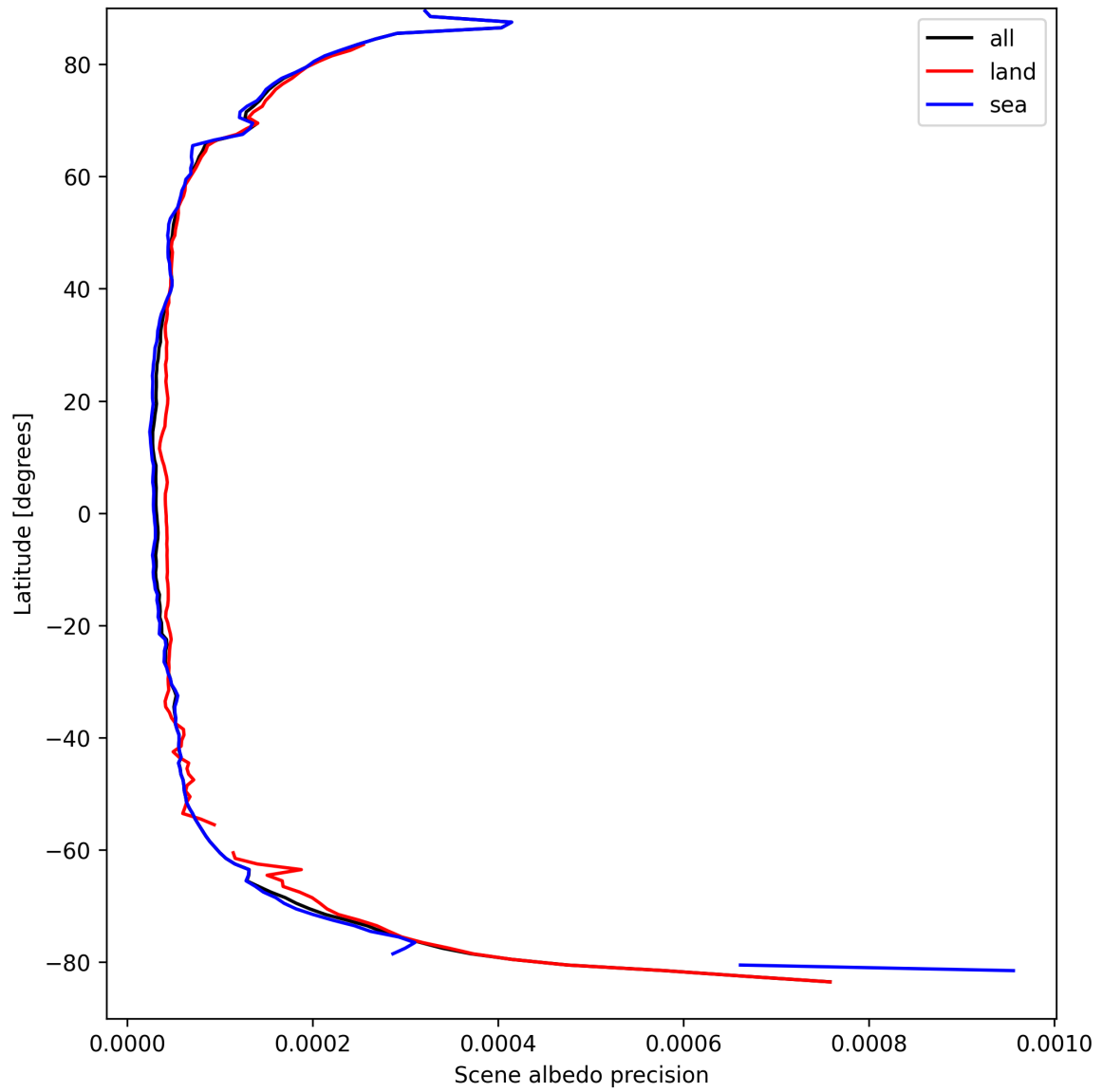
Figure 18: Zonal average of “Scene albedo precision” for 2025-04-02 to 2025-04-03.
