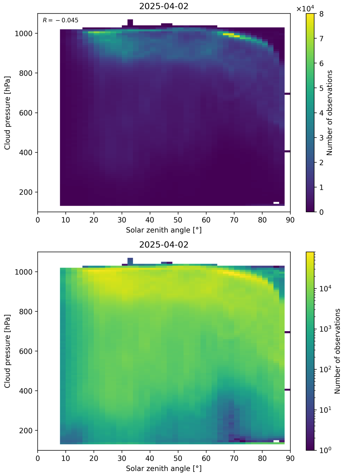
Figure 111: Scatter density plot of “Solar zenith angle” against “Cloud pressure” for 2025-04-02 to 2025-04-03.
