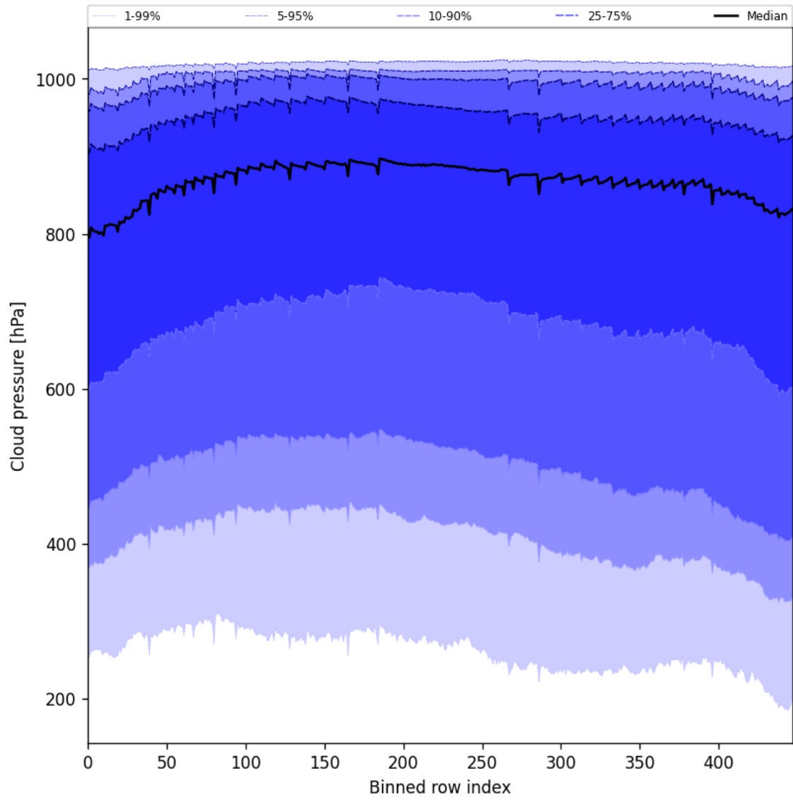
Figure 47: Along track statistics of “Cloud pressure” for 2025-04-02 to 2025-04-03
