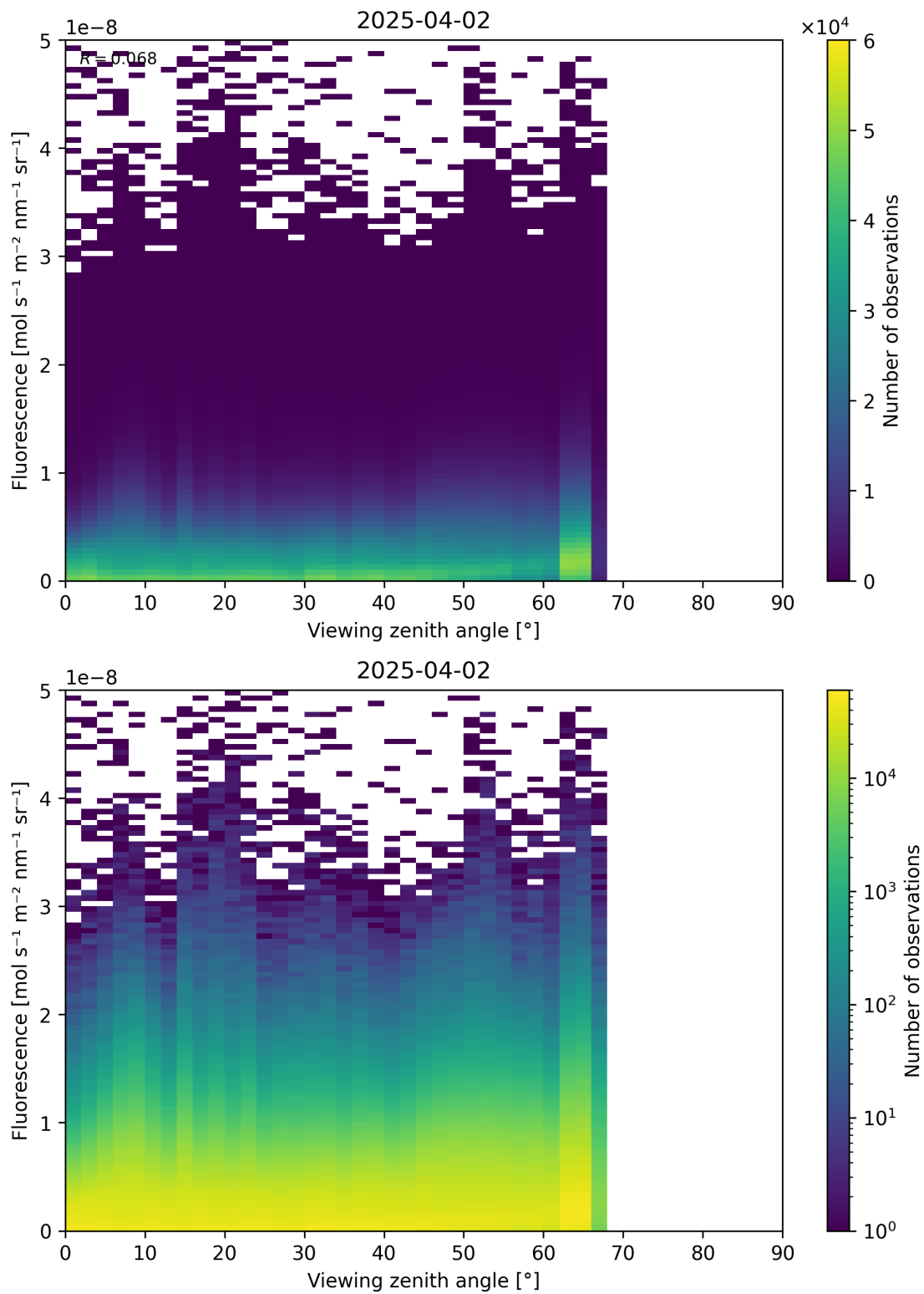
Figure 122: Scatter density plot of "Viewing zenith angle" against "Fluorescence" for 2025-04-02 to 2025-04-03.
