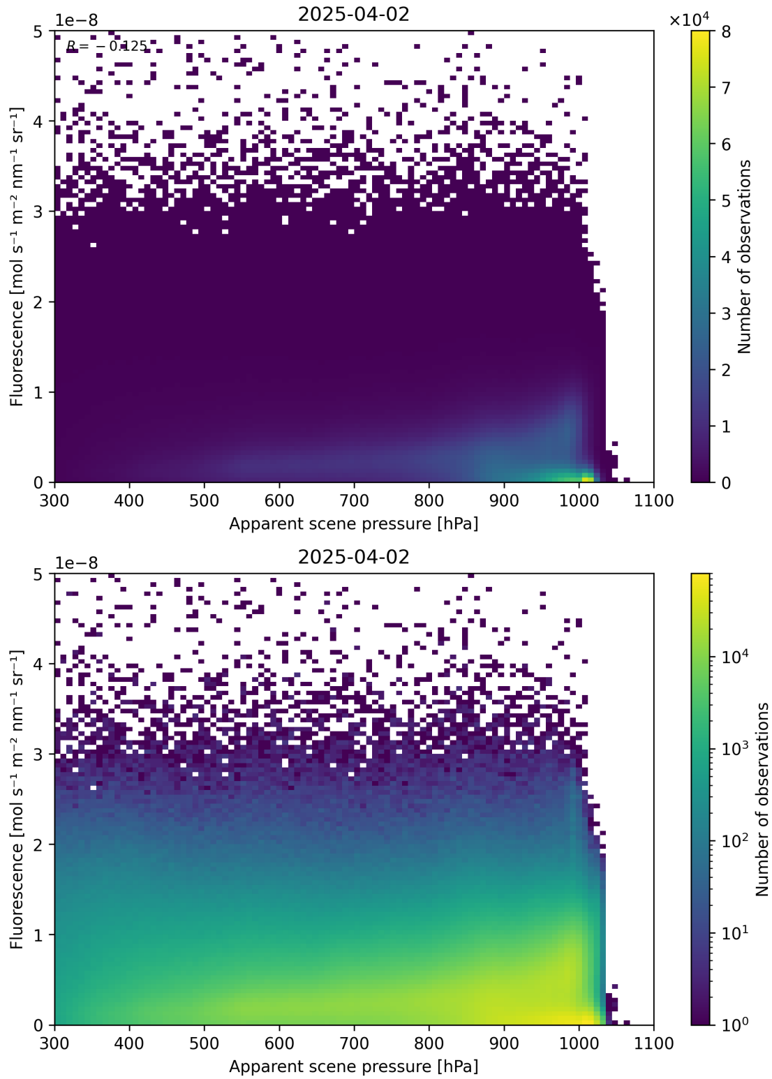
Figure 64: Scatter density plot of “Apparent scene pressure” against “Fluorescence” for 2025-04-02 to 2025-04-03.
