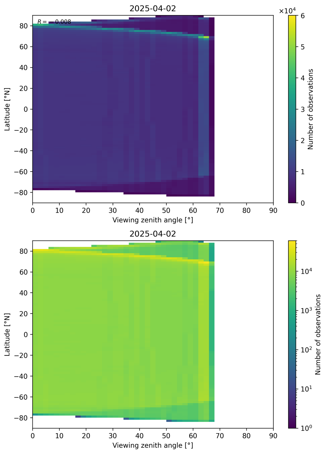
Figure 123: Scatter density plot of “Viewing zenith angle” against “Latitude” for 2025-04-02 to 2025-04-03.
