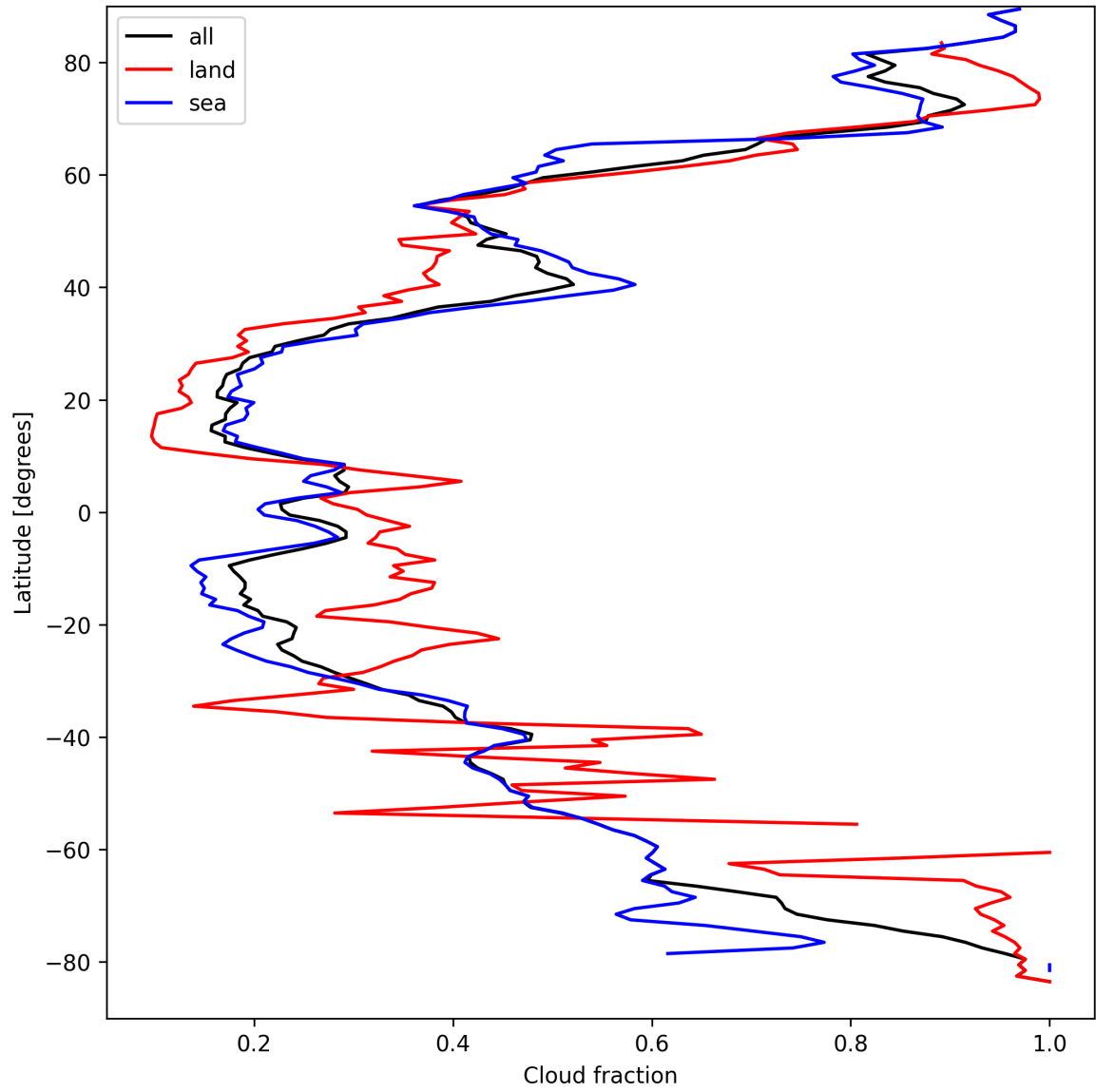
Figure 15: Zonal average of “Cloud fraction” for 2025-04-02 to 2025-04-03.
