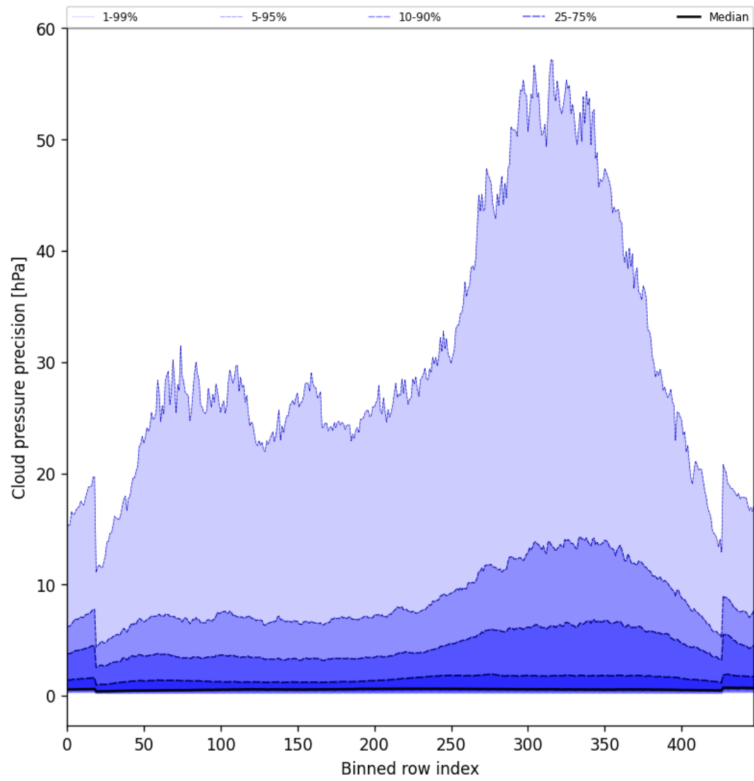
Figure 48: Along track statistics of “Cloud pressure precision” for 2025-04-02 to 2025-04-03
