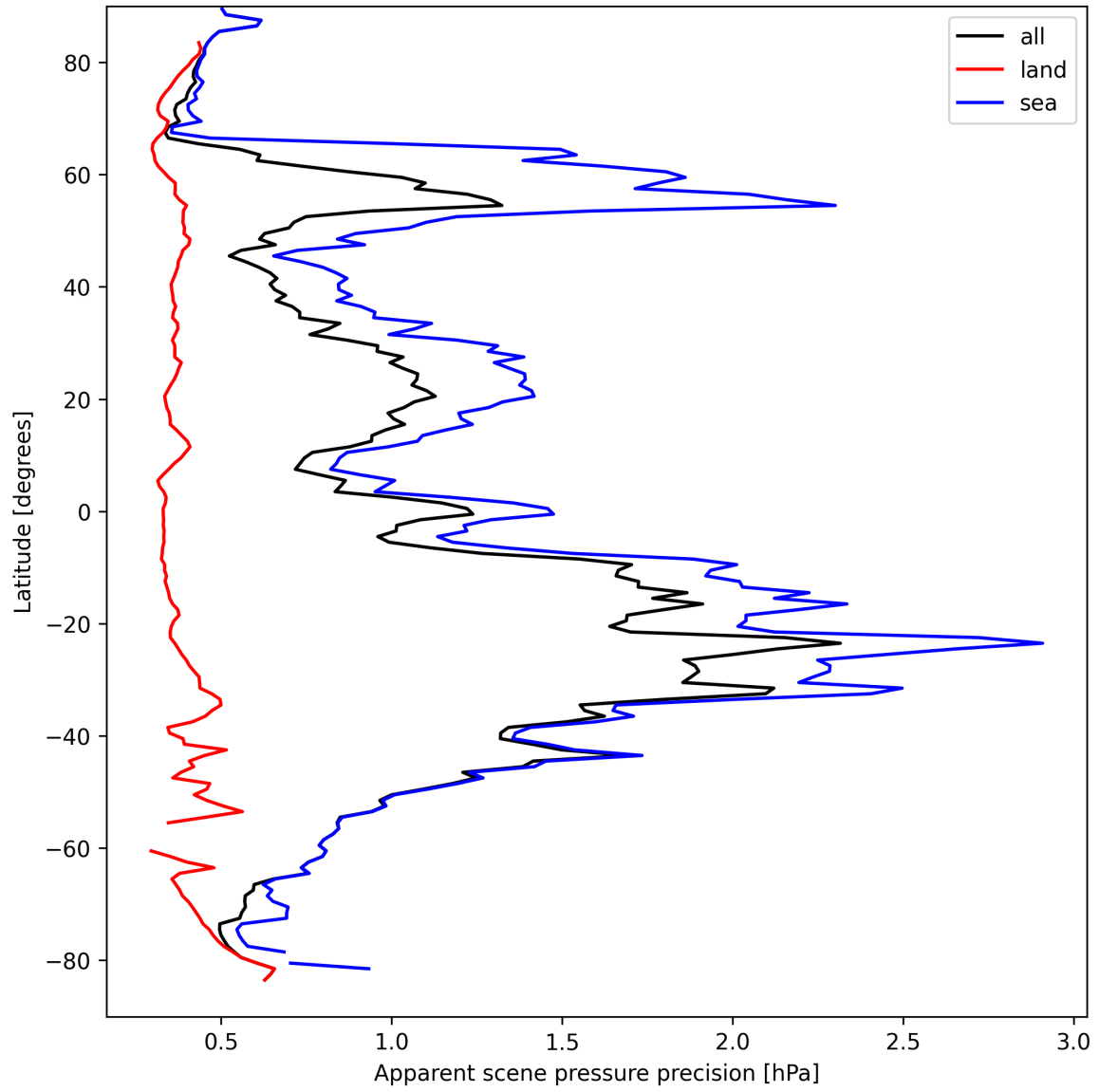
Figure 20: Zonal average of “Apparent scene pressure precision” for 2025-04-02 to 2025-04-03.
