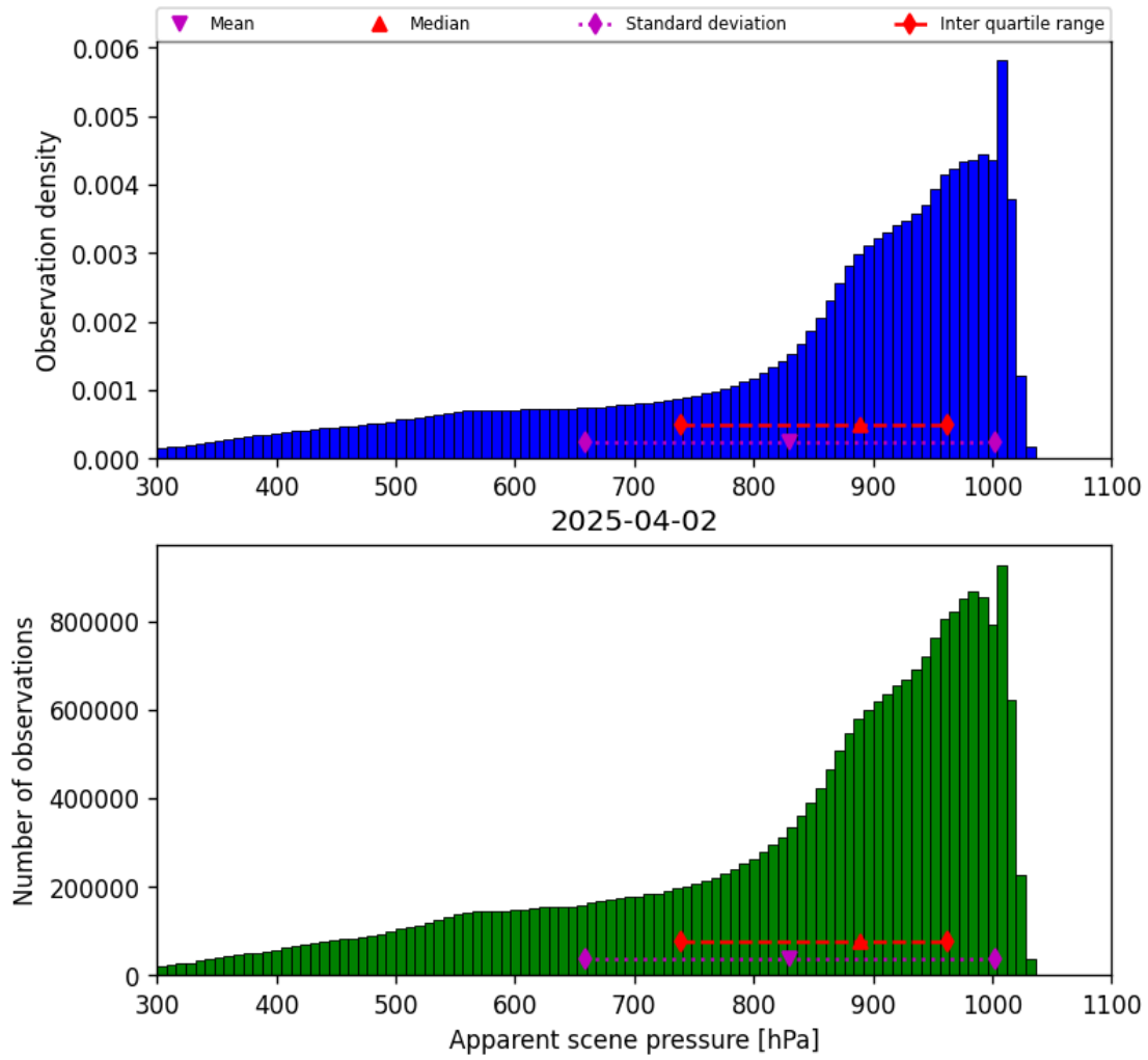
Figure 36: Histogram of “Apparent scene pressure” for 2025-04-02 to 2025-04-03
