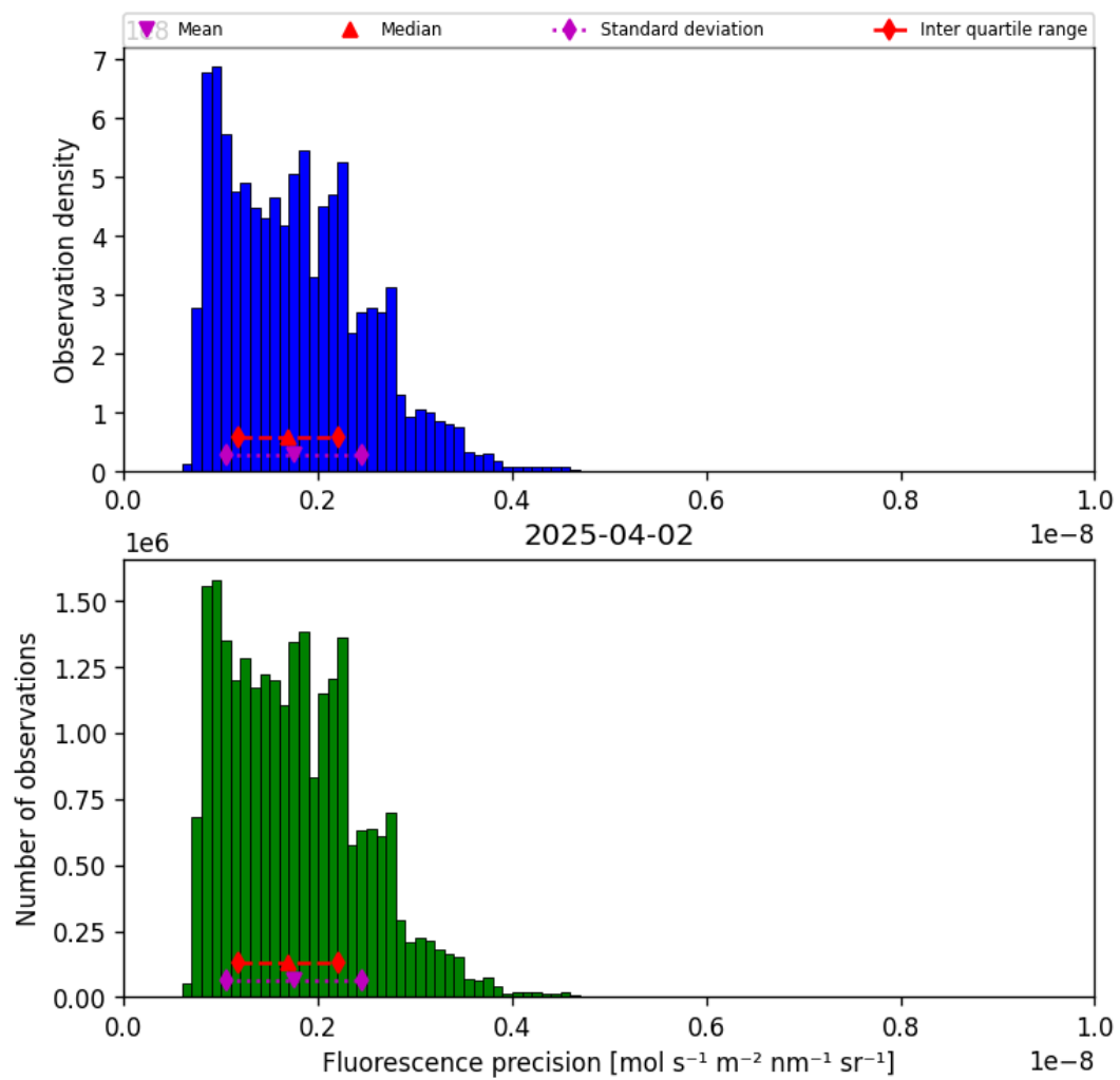
Figure 41: Histogram of “Fluorescence precision” for 2025-04-02 to 2025-04-03
