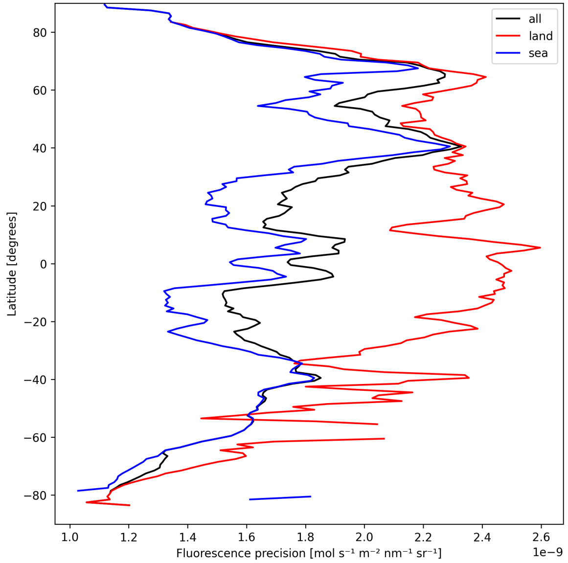
Figure 24: Zonal average of “Fluorescence precision” for 2025-04-02 to 2025-04-03.
