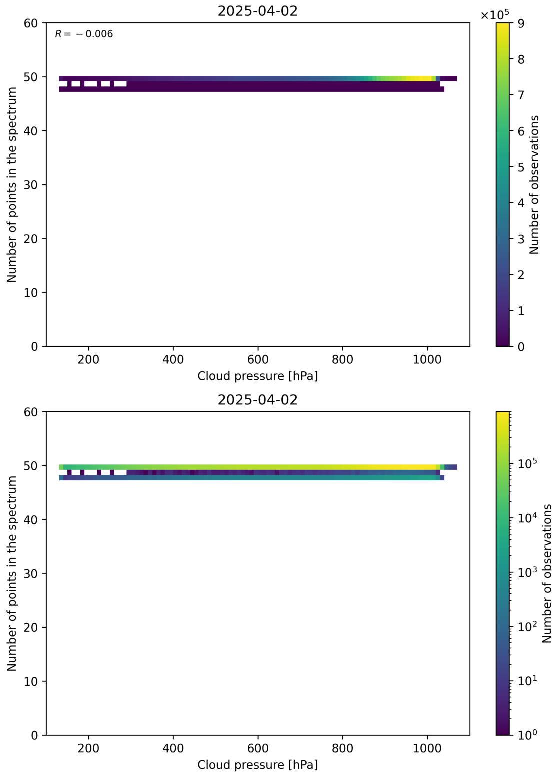
Figure 82: Scatter density plot of “Cloud pressure” against “Number of points in the spectrum” for 2025-04-02 to 2025-04-03.
