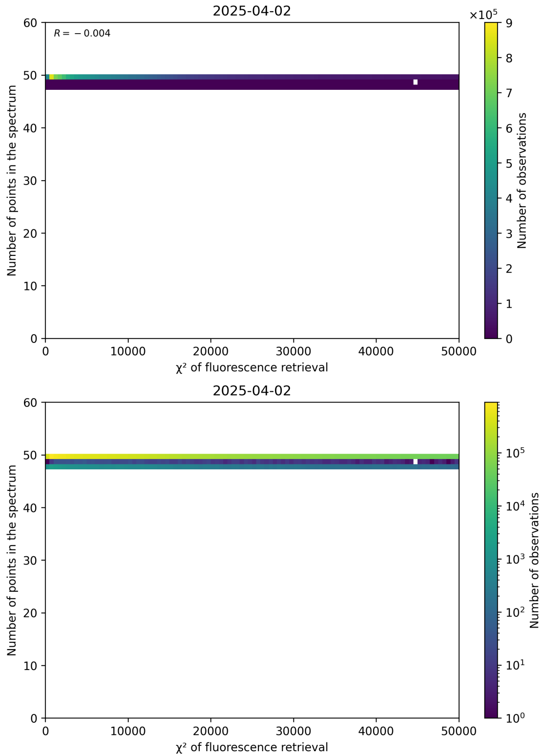
Figure 68: Scatter density plot of “ \chi^2 of fluorescence retrieval” against “Number of points in the spectrum” for 2025-04-02 to 2025-04-03.
