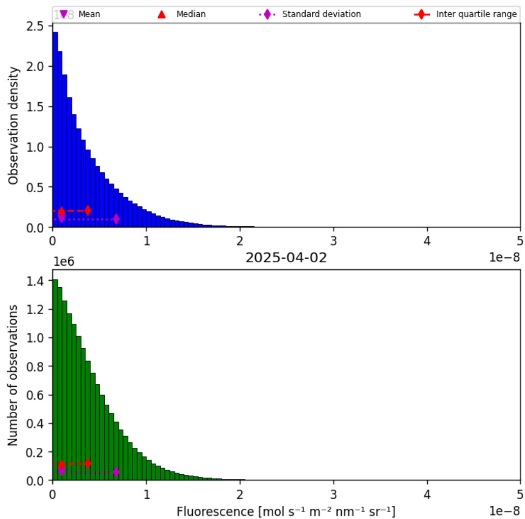
Figure 40: Histogram of “Fluorescence” for 2025-04-02 to 2025-04-03
