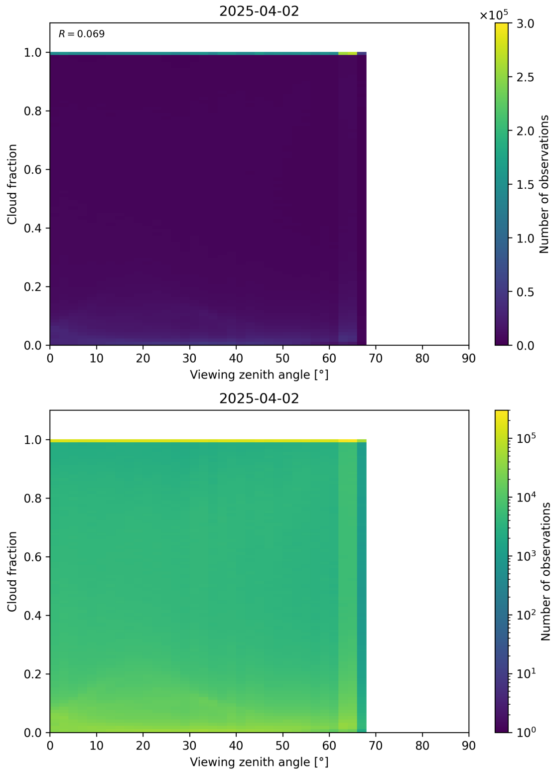
Figure 120: Scatter density plot of “Viewing zenith angle” against “Cloud fraction” for 2025-04-02 to 2025-04-03.
