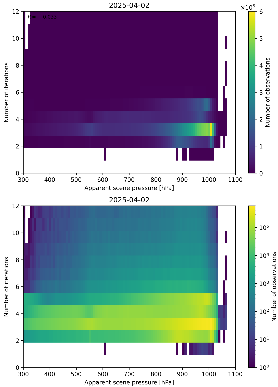
Figure 65: Scatter density plot of “Apparent scene pressure” against “Number of iterations” for 2025-04-02 to 2025-04-03.
