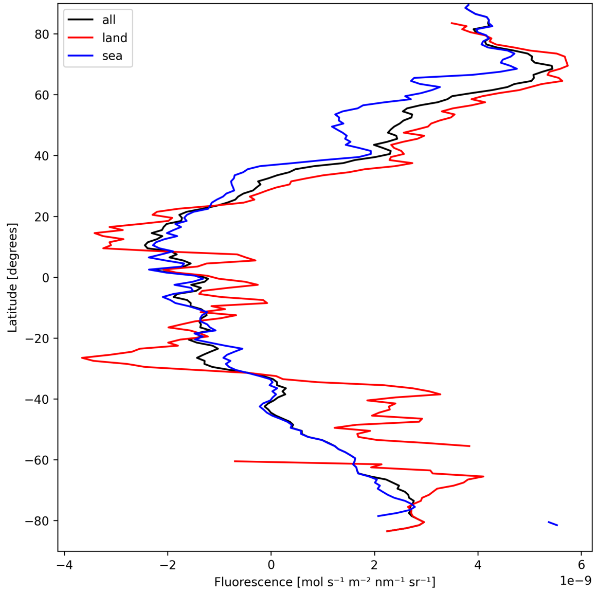
Figure 23: Zonal average of “Fluorescence” for 2025-04-02 to 2025-04-03.
