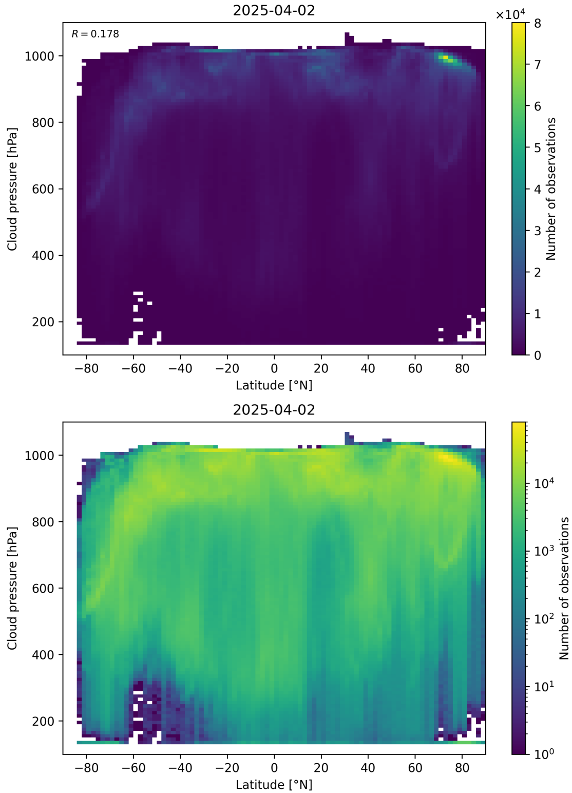
Figure 91: Scatter density plot of “Latitude” against “Cloud pressure” for 2025-04-02 to 2025-04-03.
