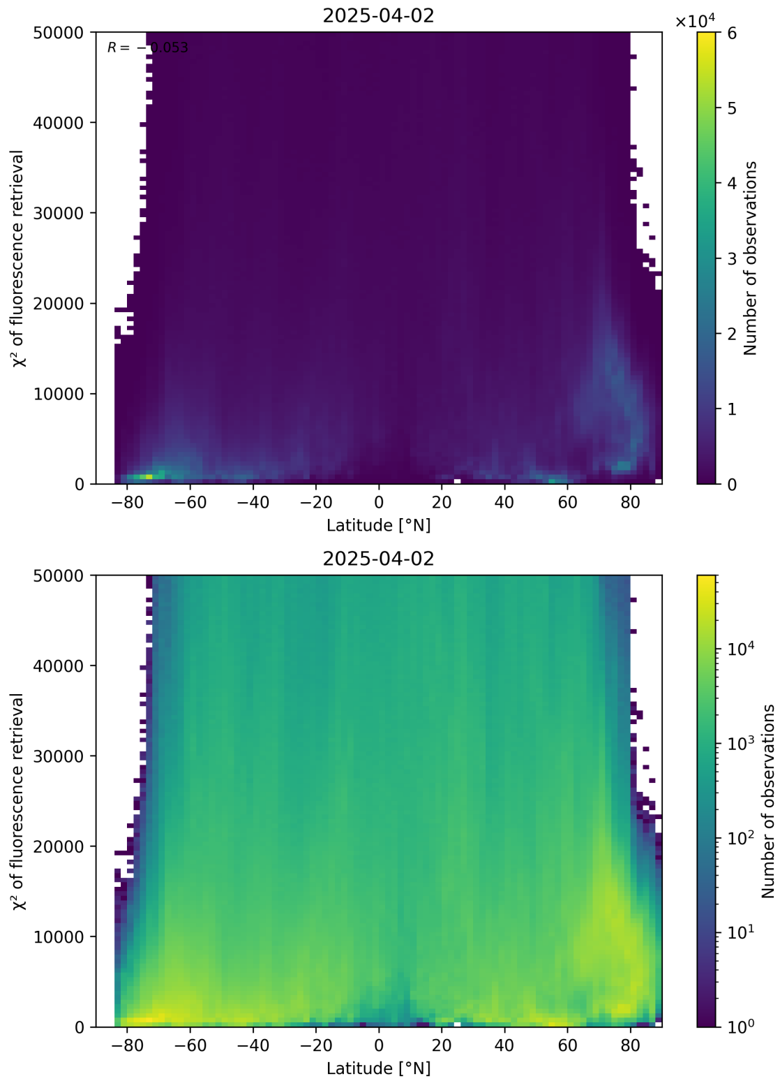
Figure 89: Scatter density plot of “Latitude” against “ \chi^2 of fluorescence retrieval” for 2025-04-02 to 2025-04-03.
