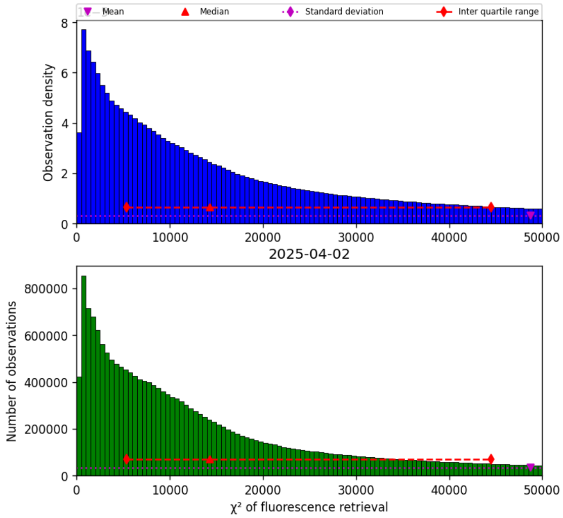
Figure 42: Histogram of “ \chi^2 of fluorescence retrieval” for 2025-04-02 to 2025-04-03
