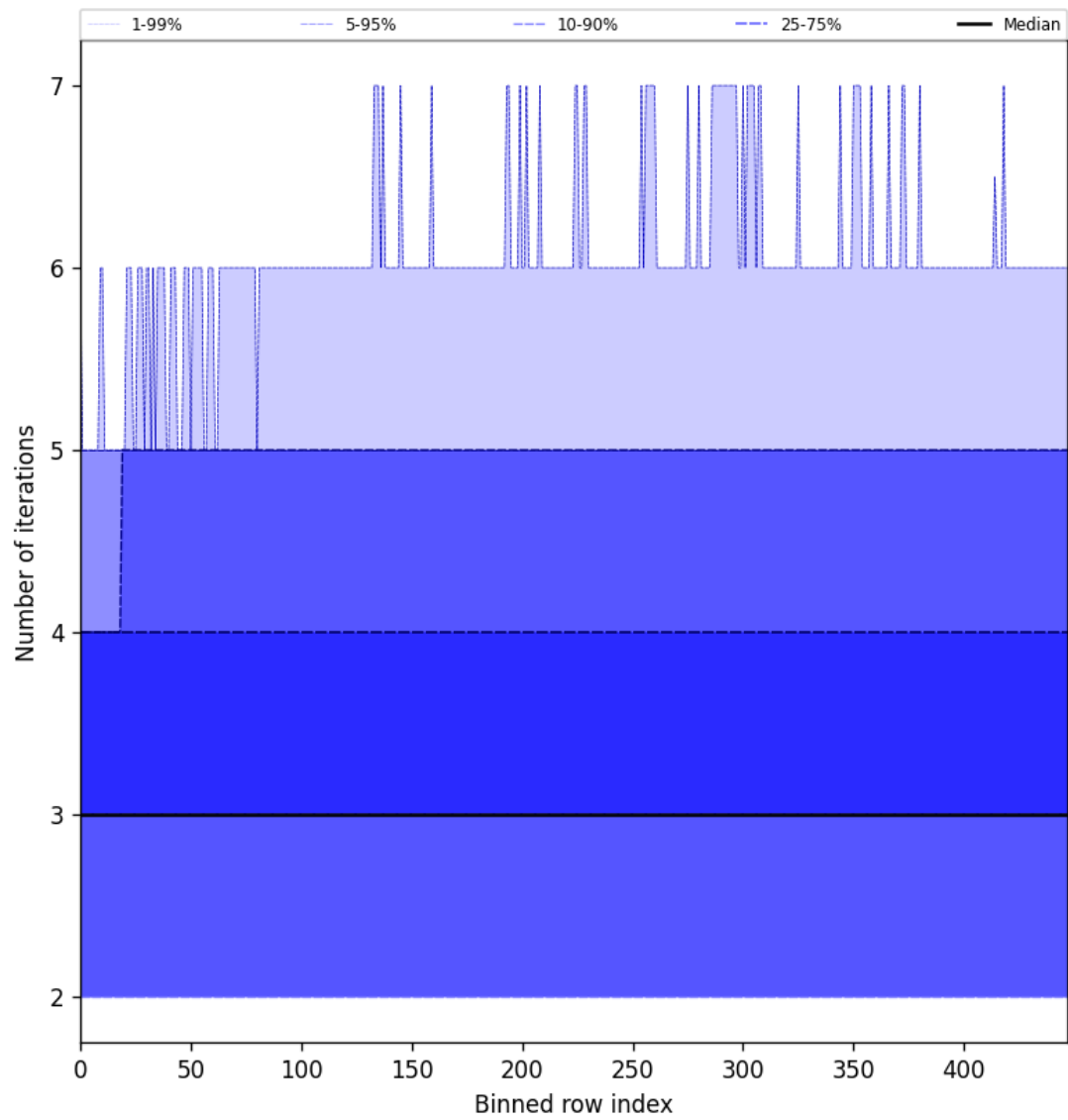
Figure 56: Along track statistics of “Number of iterations” for 2025-04-02 to 2025-04-03
