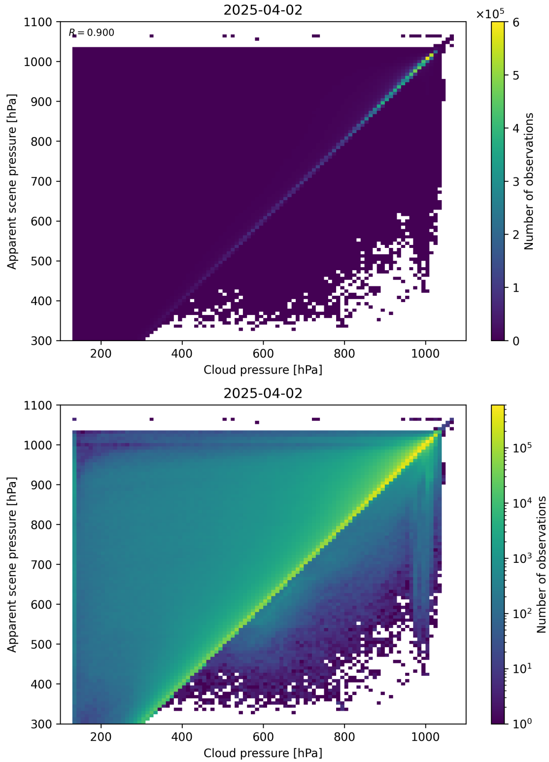
Figure 77: Scatter density plot of “Cloud pressure” against “Apparent scene pressure” for 2025-04-02 to 2025-04-03.
