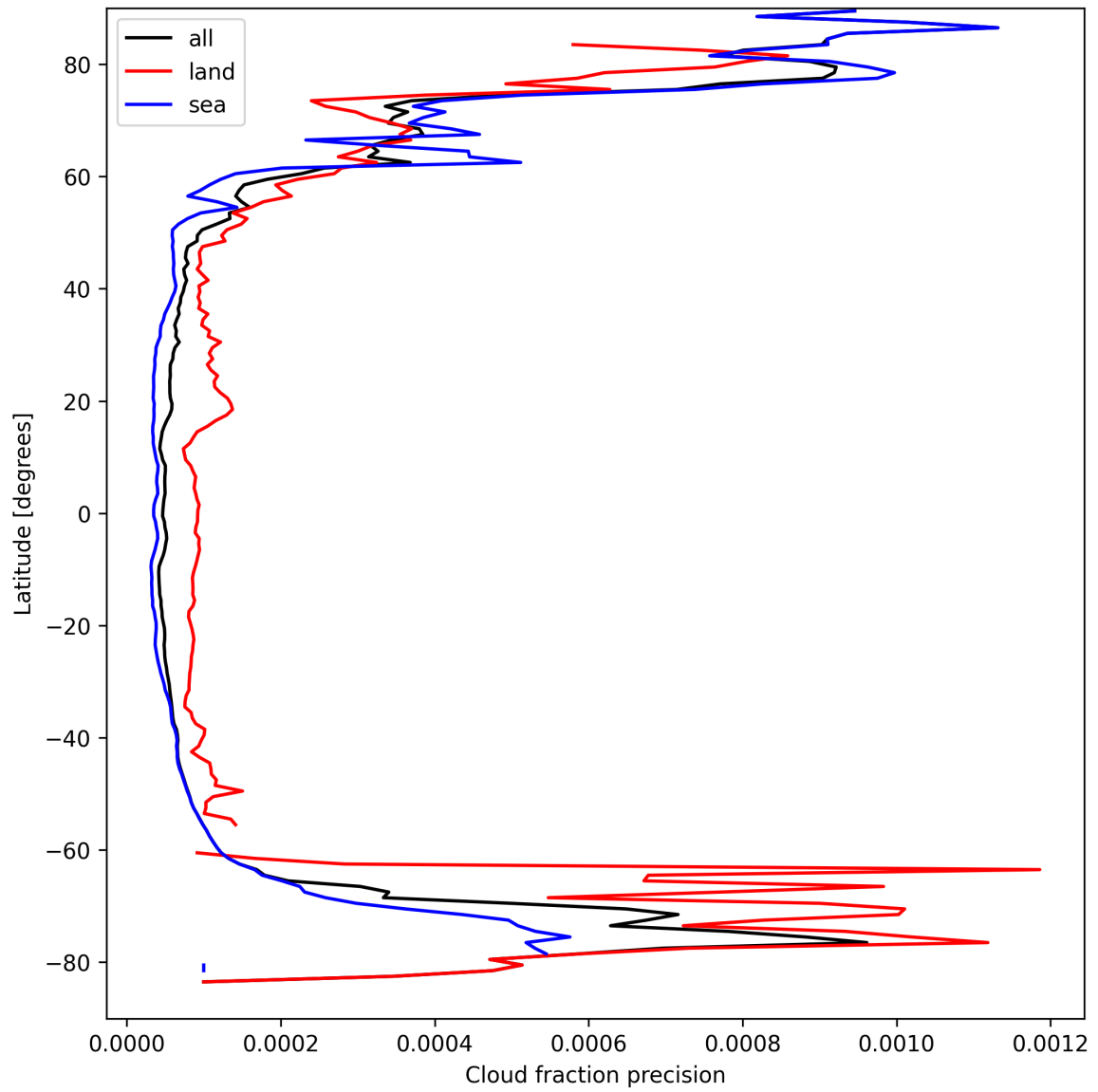
Figure 16: Zonal average of “Cloud fraction precision” for 2025-04-02 to 2025-04-03.
