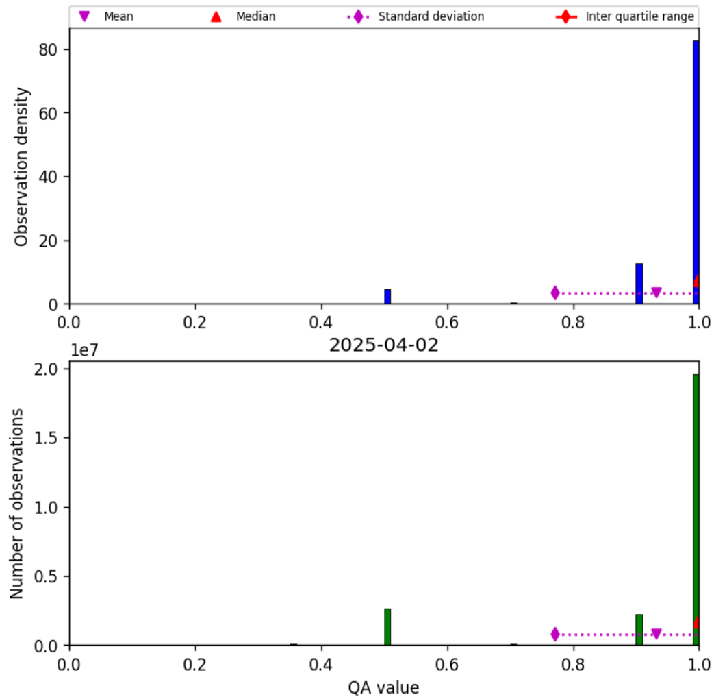
Figure 29: Histogram of “QA value” for 2025-04-02 to 2025-04-03
