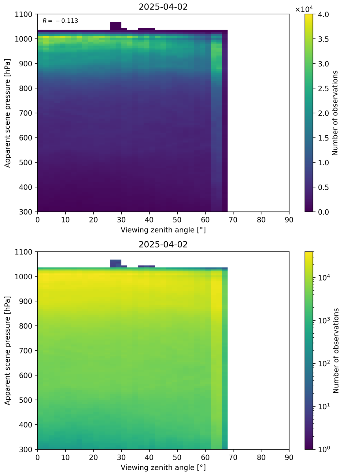
Figure 118: Scatter density plot of “Viewing zenith angle” against “Apparent scene pressure” for 2025-04-02 to 2025-04-03.
