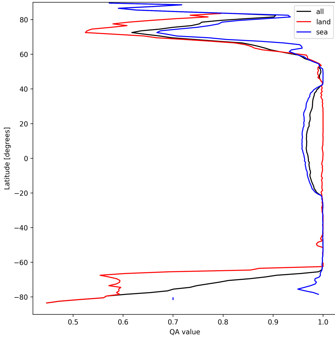
Figure 12: Zonal average of “QA value” for 2025-04-02 to 2025-04-03.
