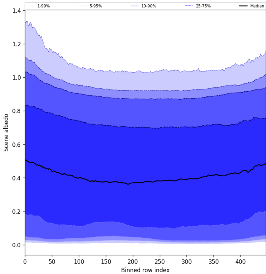
Figure 51: Along track statistics of “Scene albedo” for 2025-04-02 to 2025-04-03
