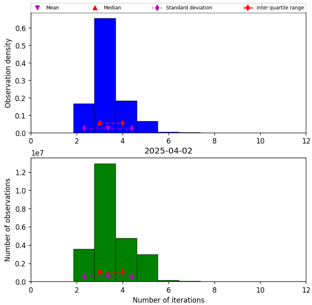
Figure 39: Histogram of “Number of iterations” for 2025-04-02 to 2025-04-03
