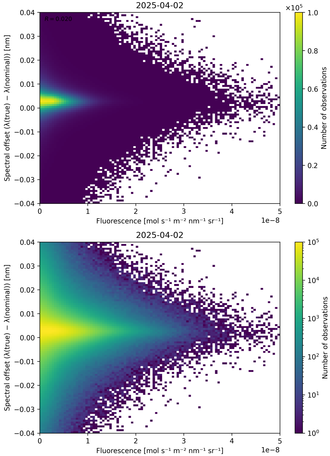
Figure 87: Scatter density plot of “Fluorescence” against “Spectral offset ( \lambda_{\text{true}} - \lambda_{\text{nominal}} )” for 2025-04-02 to 2025-04-03.
