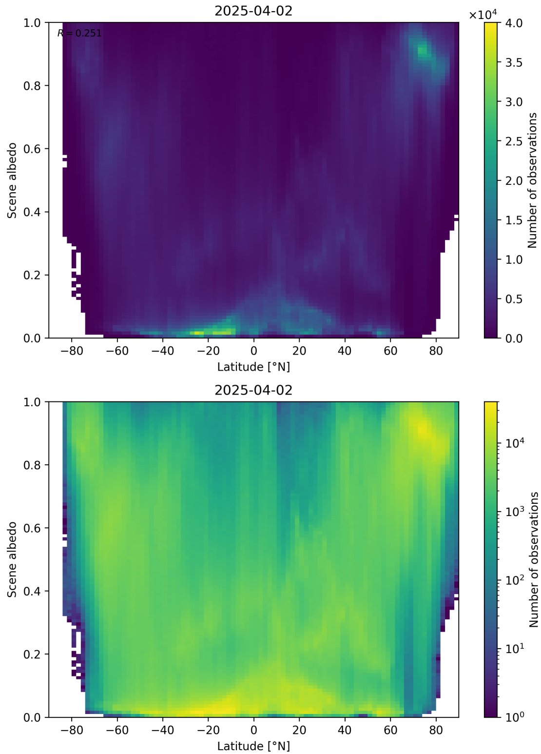
Figure 95: Scatter density plot of “Latitude” against “Scene albedo” for 2025-04-02 to 2025-04-03.
