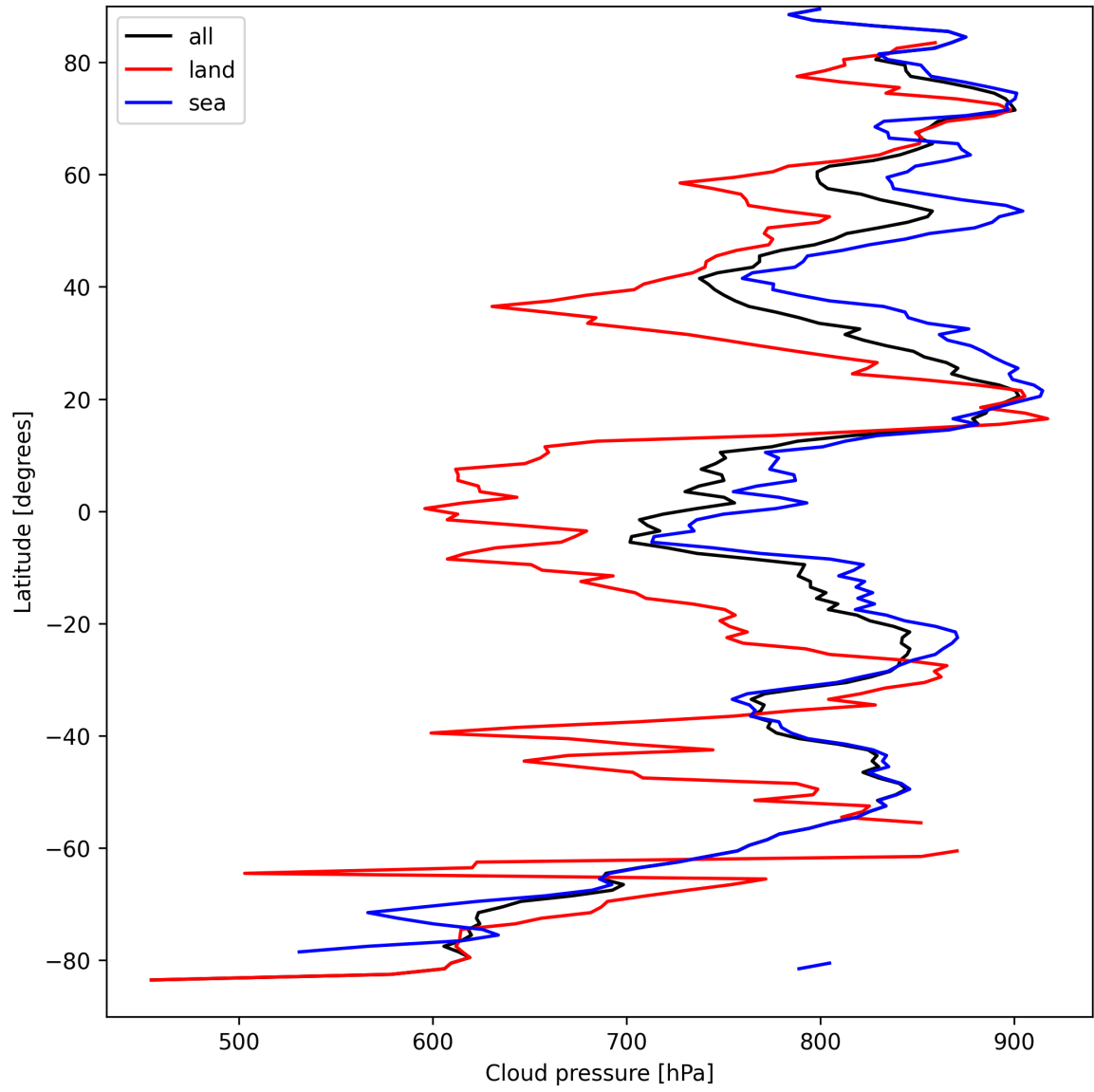
Figure 13: Zonal average of “Cloud pressure” for 2025-04-02 to 2025-04-03.
