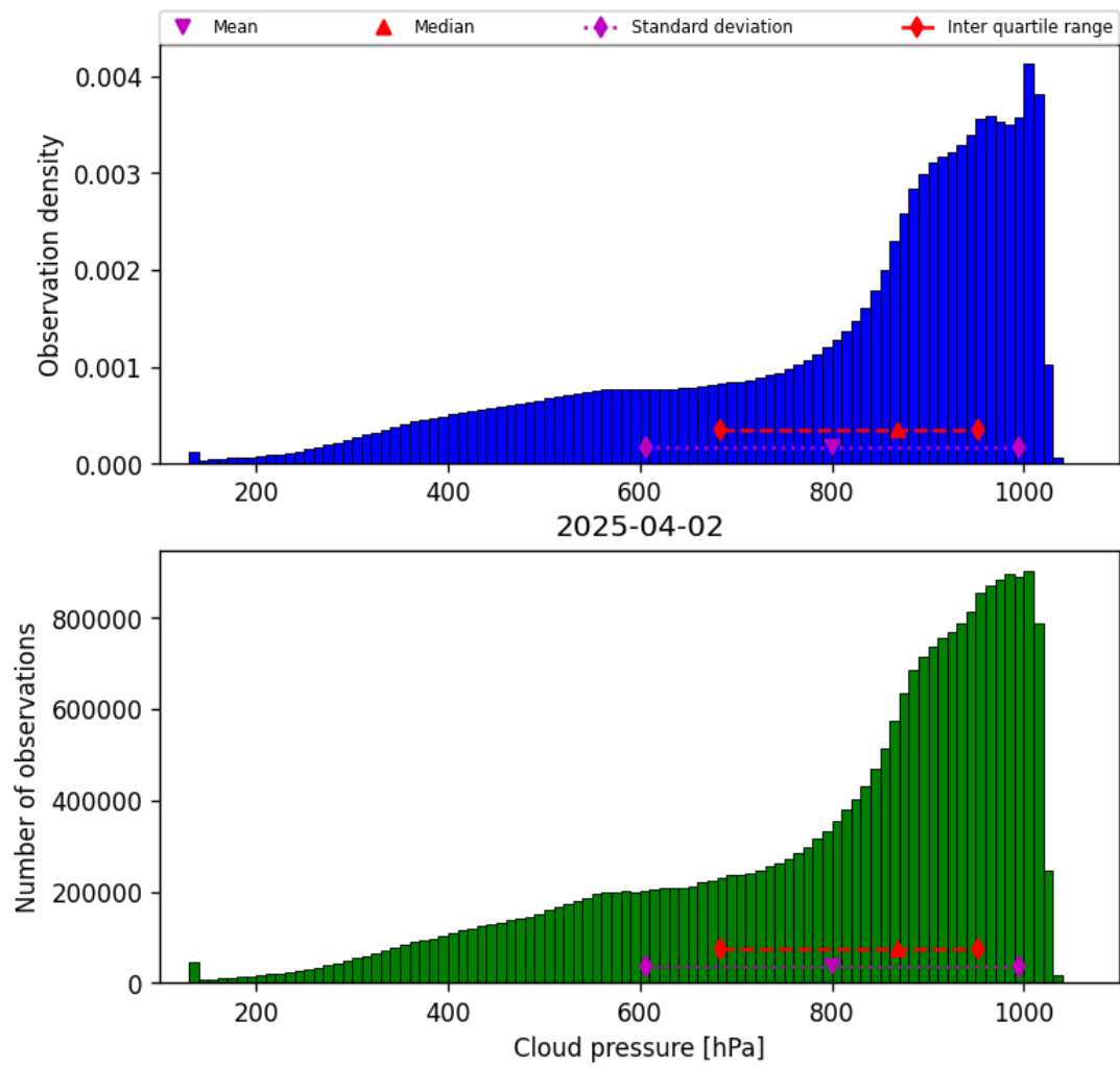
Figure 30: Histogram of “Cloud pressure” for 2025-04-02 to 2025-04-03
