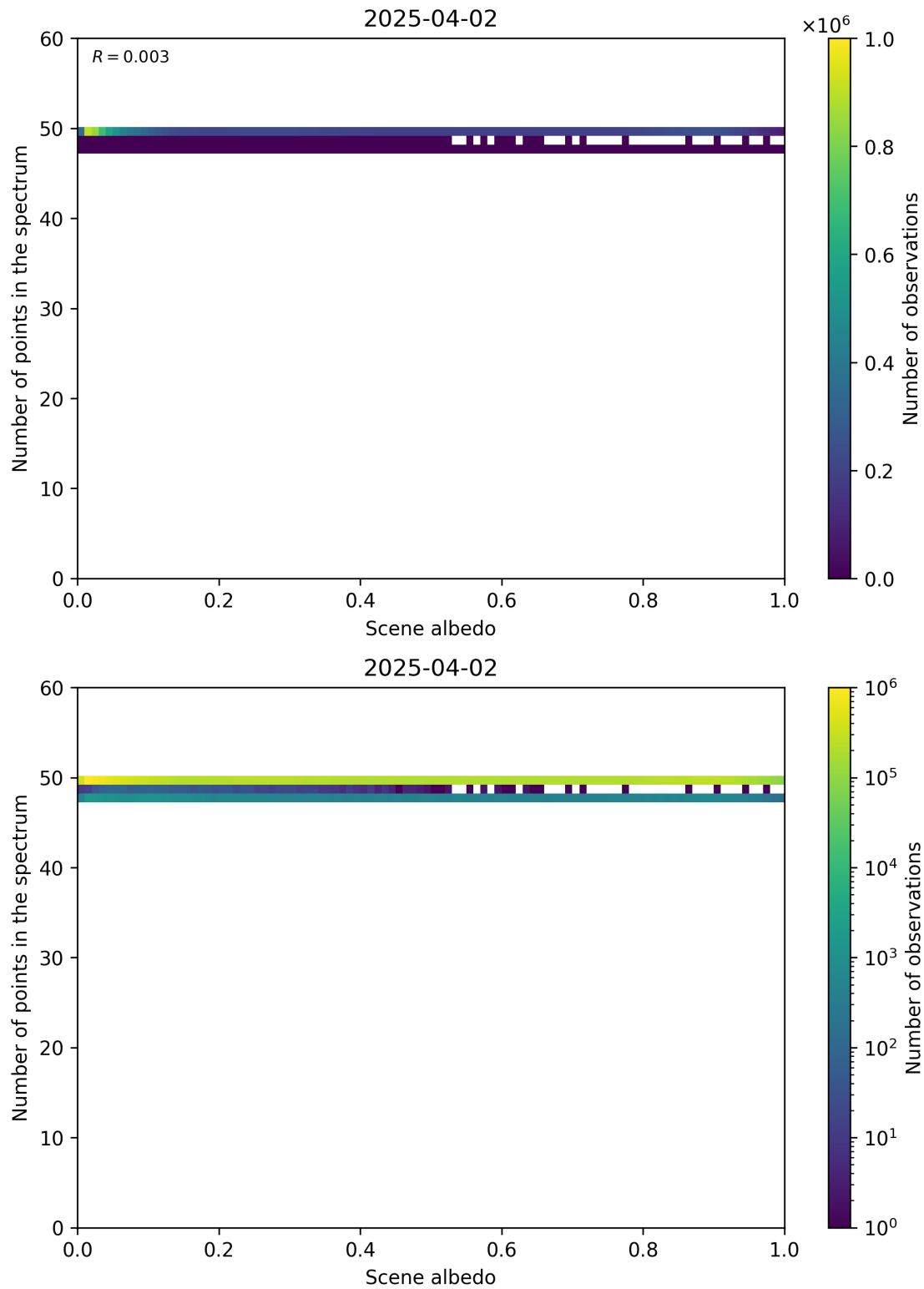
Figure 106: Scatter density plot of “Scene albedo” against “Number of points in the spectrum” for 2025-04-02 to 2025-04-03.
