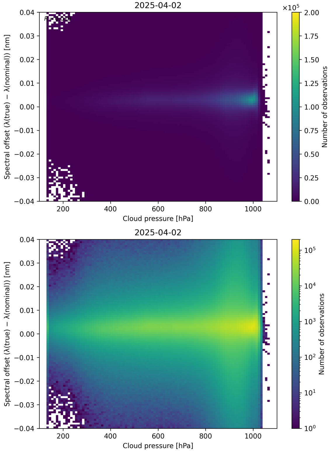
Figure 84: Scatter density plot of “Cloud pressure” against “Spectral offset ( \lambda_{\text{true}} - \lambda_{\text{nominal}} )” for 2025-04-02 to 2025-04-03.
