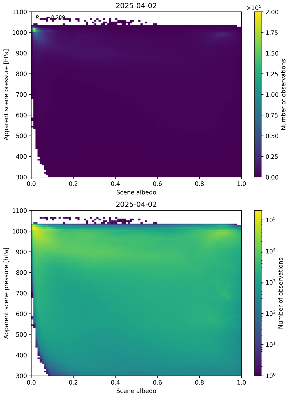
Figure 102: Scatter density plot of “Scene albedo” against “Apparent scene pressure” for 2025-04-02 to 2025-04-03.
