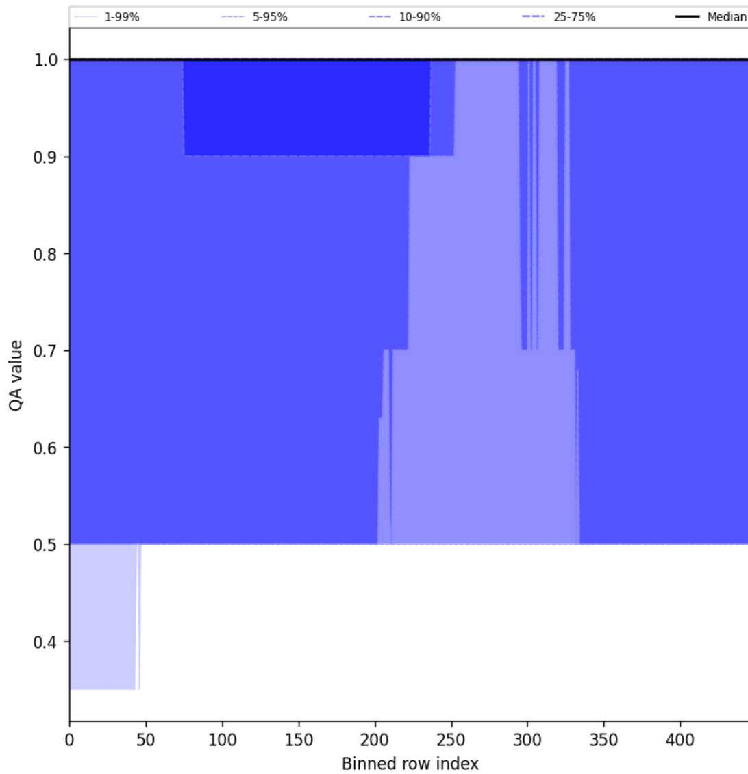
Figure 46: Along track statistics of “QA value” for 2025-04-02 to 2025-04-03
