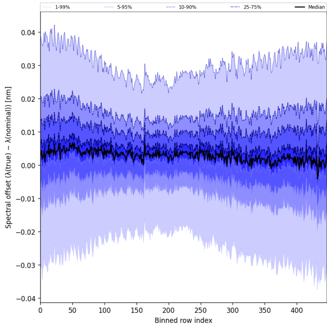
Figure 62: Along track statistics of “Spectral offset ( \lambda_{\text{true}} - \lambda_{\text{nominal}} )” for 2025-04-02 to 2025-04-03
