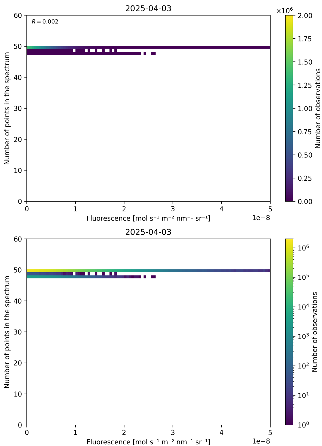
Figure 86: Scatter density plot of “Fluorescence” against “Number of points in the spectrum” for 2025-04-03 to 2025-04-04.
