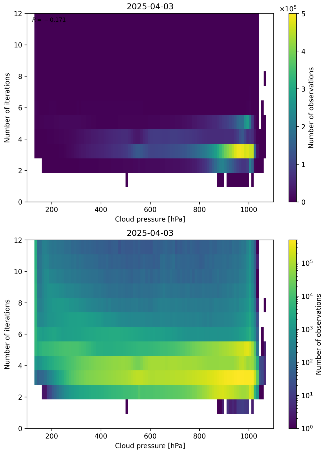
Figure 81: Scatter density plot of “Cloud pressure” against “Number of iterations” for 2025-04-03 to 2025-04-04.
