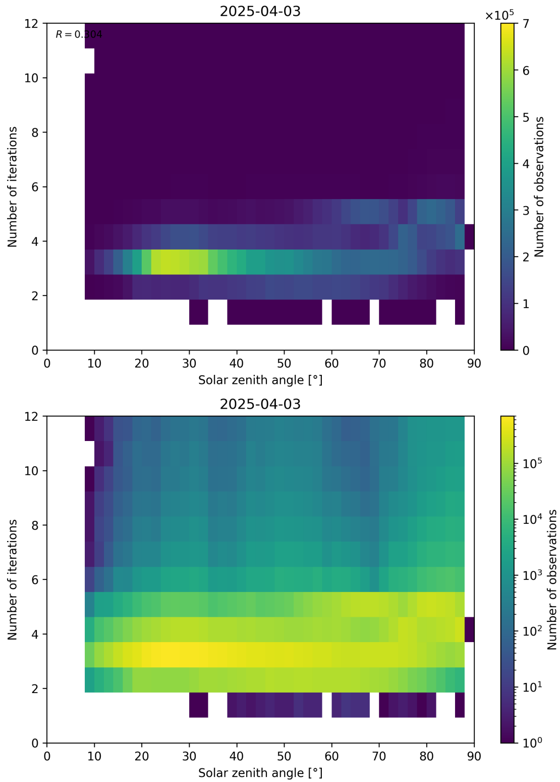
Figure 114: Scatter density plot of “Solar zenith angle” against “Number of iterations” for 2025-04-03 to 2025-04-04.
