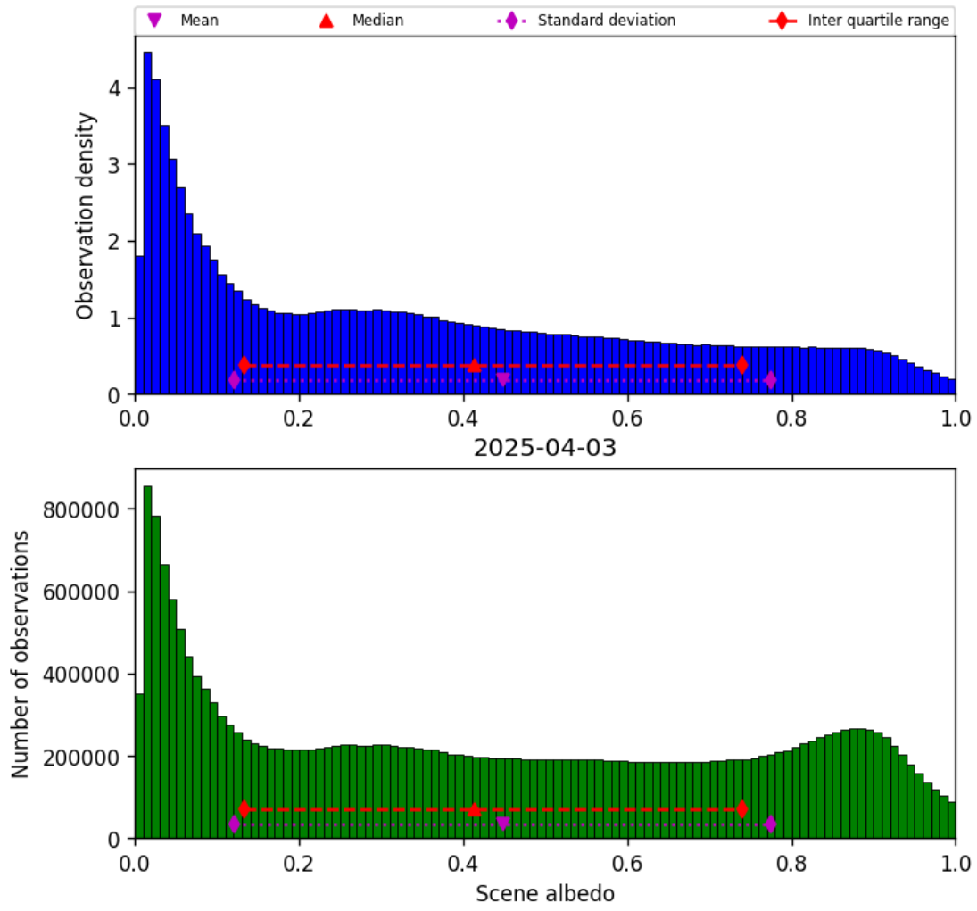
Figure 34: Histogram of “Scene albedo” for 2025-04-03 to 2025-04-04
