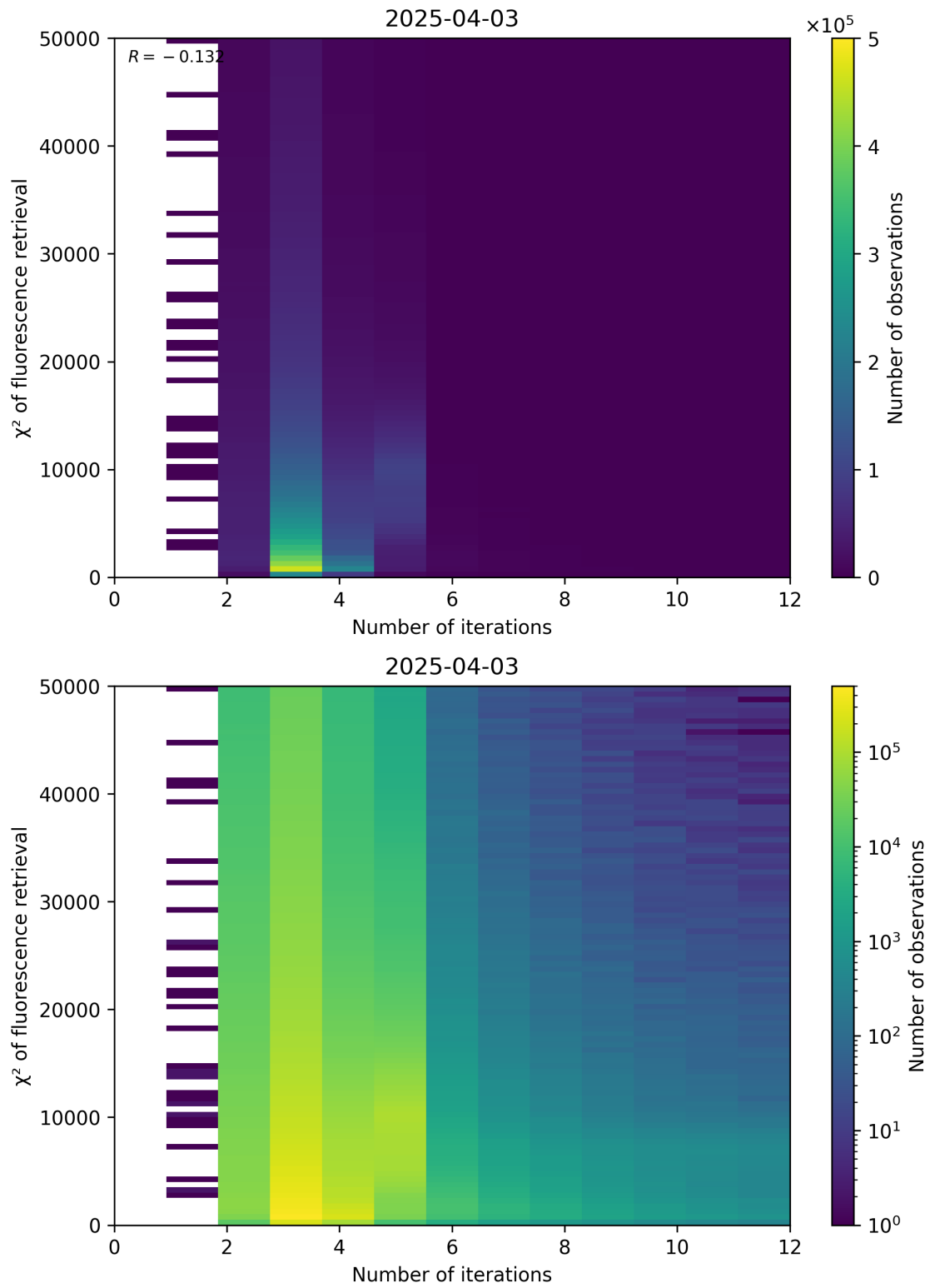
Figure 97: Scatter density plot of “Number of iterations” against “ \chi^2 of fluorescence retrieval” for 2025-04-03 to 2025-04-04.
