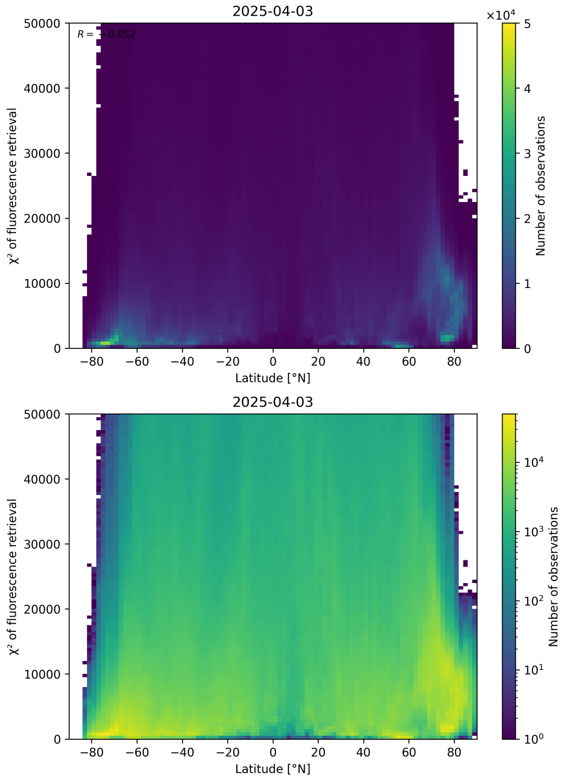
Figure 89: Scatter density plot of “Latitude” against “ \chi^2 of fluorescence retrieval” for 2025-04-03 to 2025-04-04.
