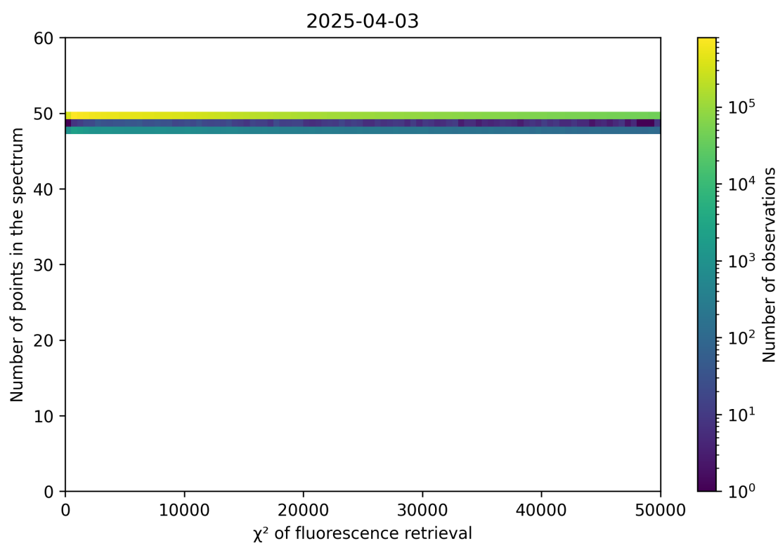
Figure 68: Scatter density plot of “ \chi^2 of fluorescence retrieval” against “Number of points in the spectrum” for 2025-04-03 to 2025-04-04.
