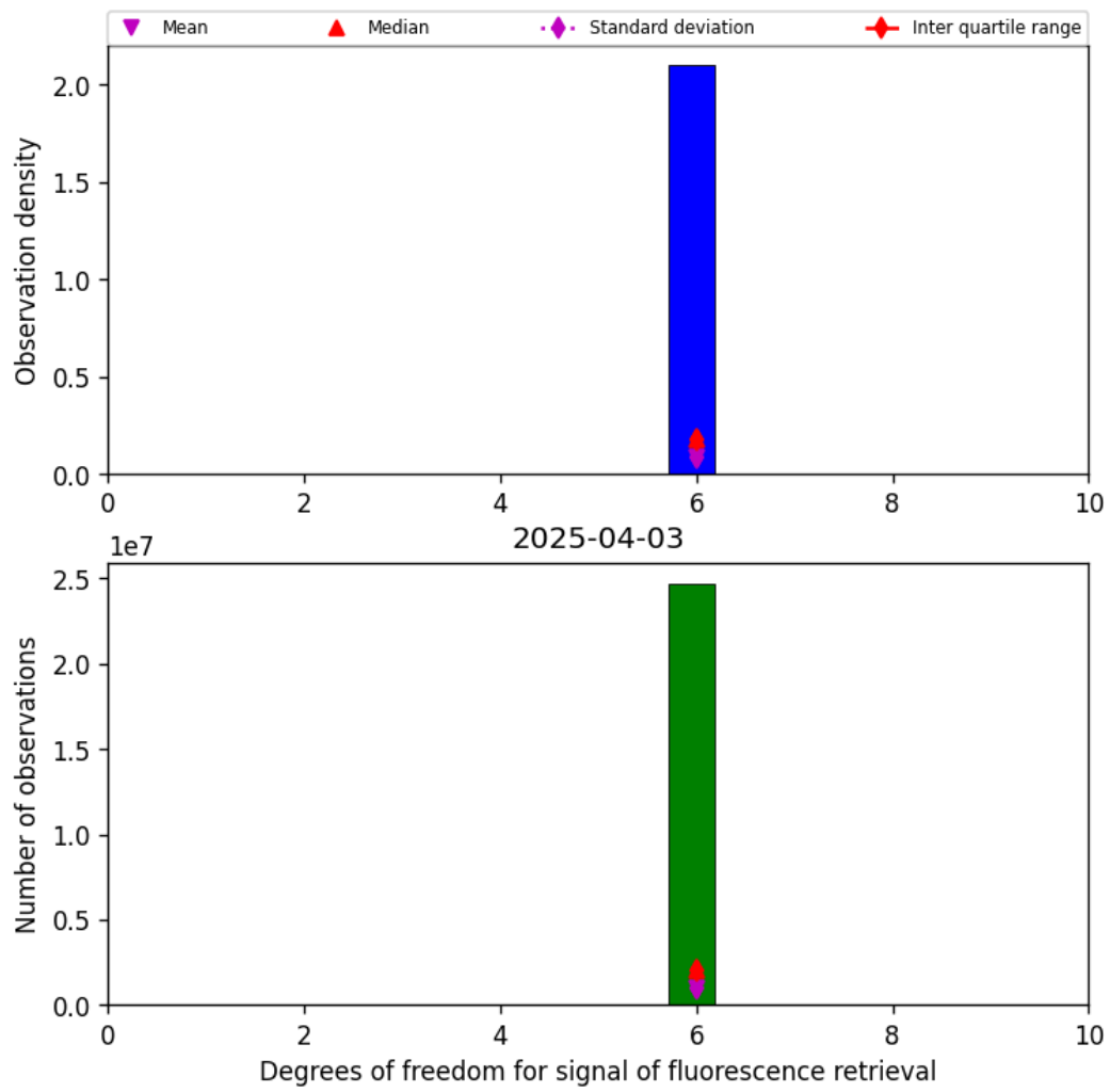
Figure 43: Histogram of “Degrees of freedom for signal of fluorescence retrieval” for 2025-04-03 to 2025-04-04
