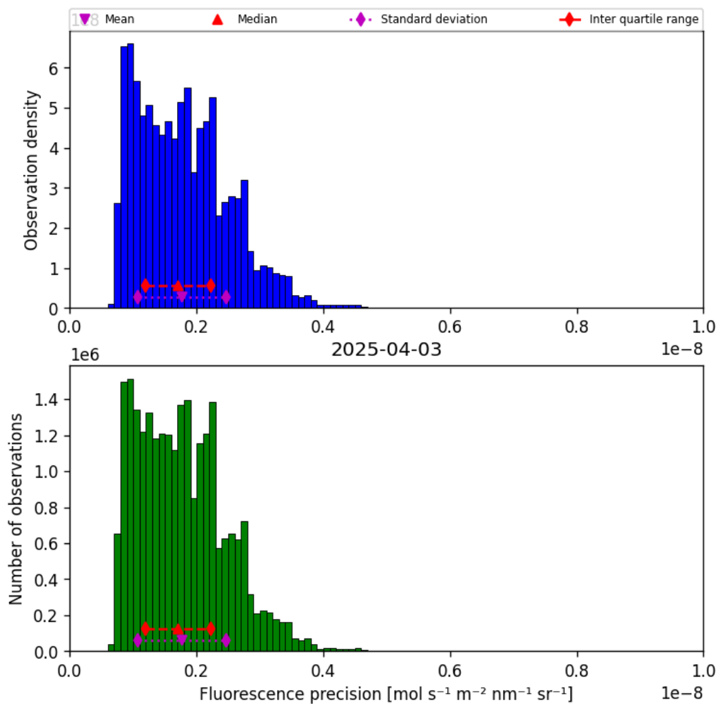
Figure 41: Histogram of “Fluorescence precision” for 2025-04-03 to 2025-04-04
