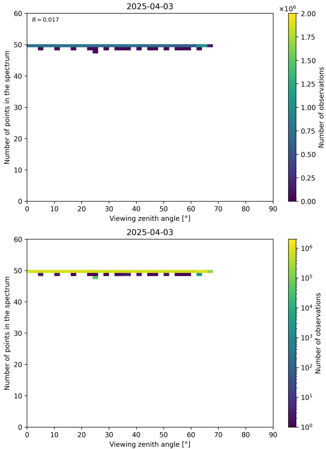
Figure 125: Scatter density plot of “Viewing zenith angle” against “Number of points in the spectrum” for 2025-04-03 to 2025-04-04.
