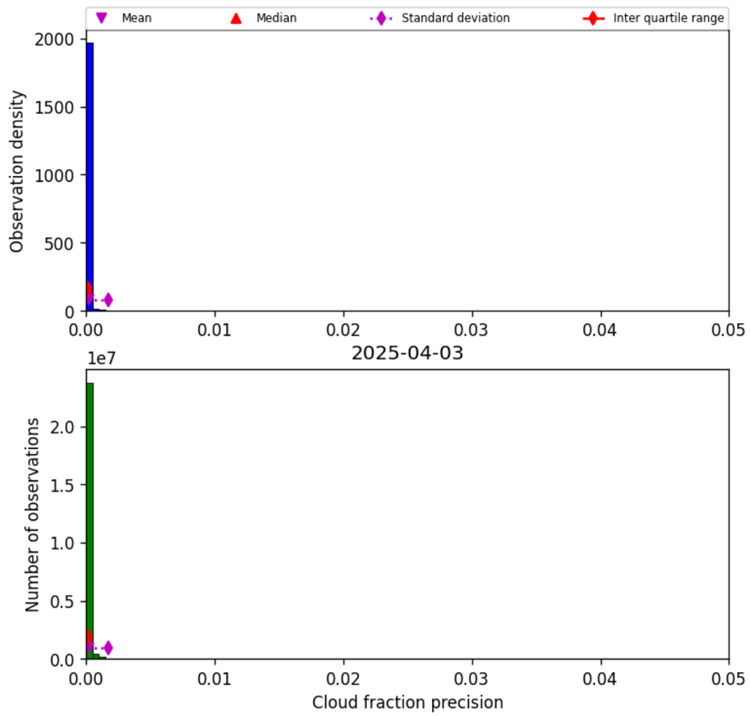
Figure 33: Histogram of “Cloud fraction precision” for 2025-04-03 to 2025-04-04
