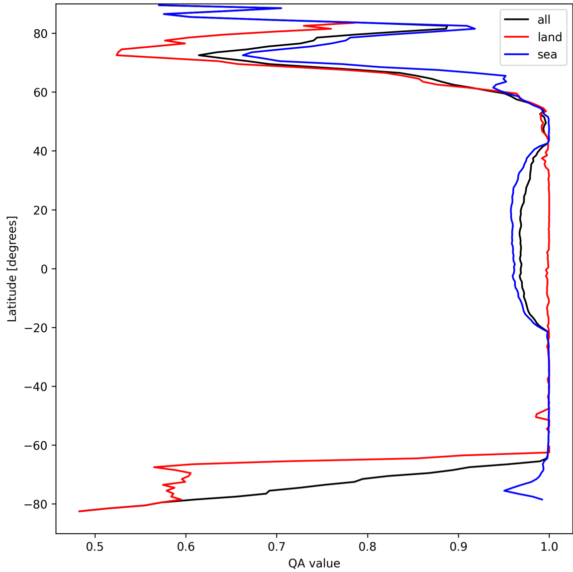
Figure 12: Zonal average of “QA value” for 2025-04-03 to 2025-04-04.
