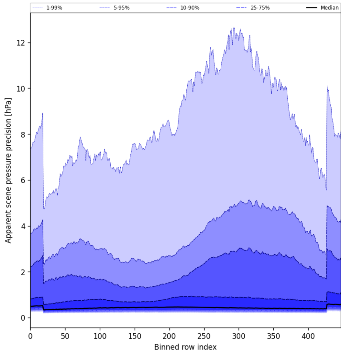
Figure 54: Along track statistics of “Apparent scene pressure precision” for 2025-04-03 to 2025-04-04
