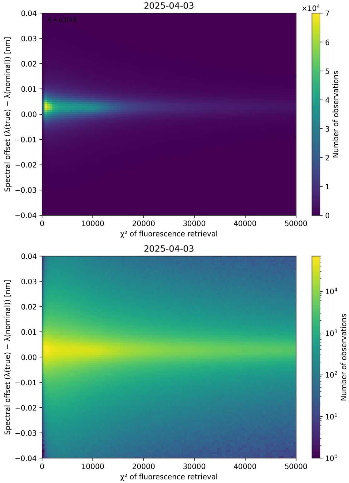
Figure 69: Scatter density plot of “ \chi^2 of fluorescence retrieval” against “Spectral offset ( \lambda_{\text{true}} - \lambda_{\text{nominal}} )” for 2025-04-03 to 2025-04-04.
