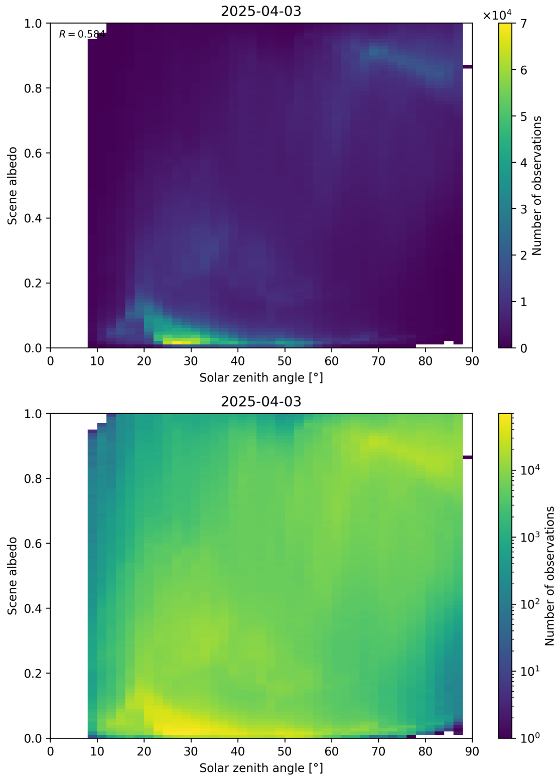
Figure 116: Scatter density plot of “Solar zenith angle” against “Scene albedo” for 2025-04-03 to 2025-04-04.
