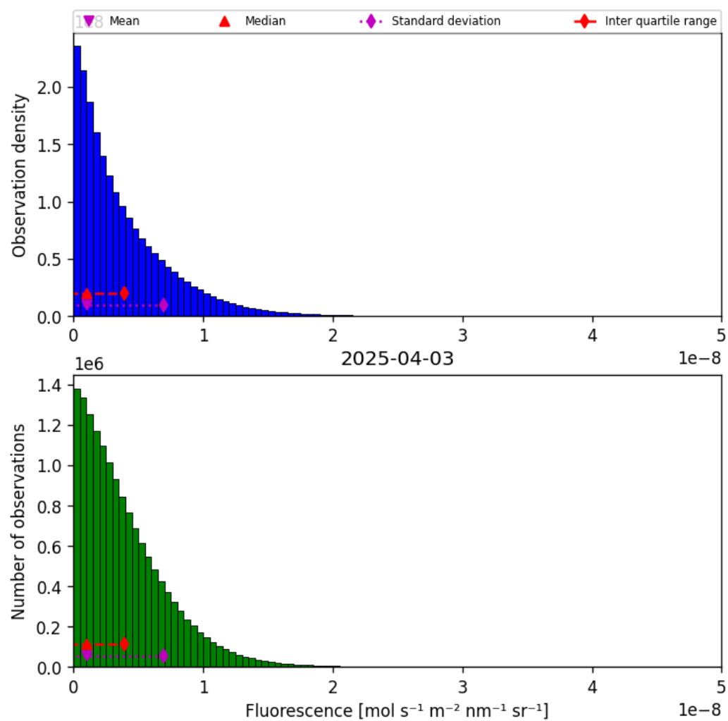
Figure 40: Histogram of “Fluorescence” for 2025-04-03 to 2025-04-04
