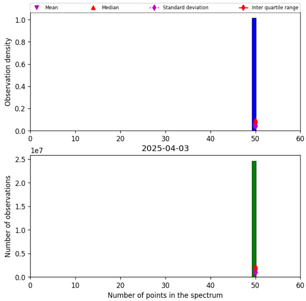
Figure 44: Histogram of “Number of points in the spectrum” for 2025-04-03 to 2025-04-04
