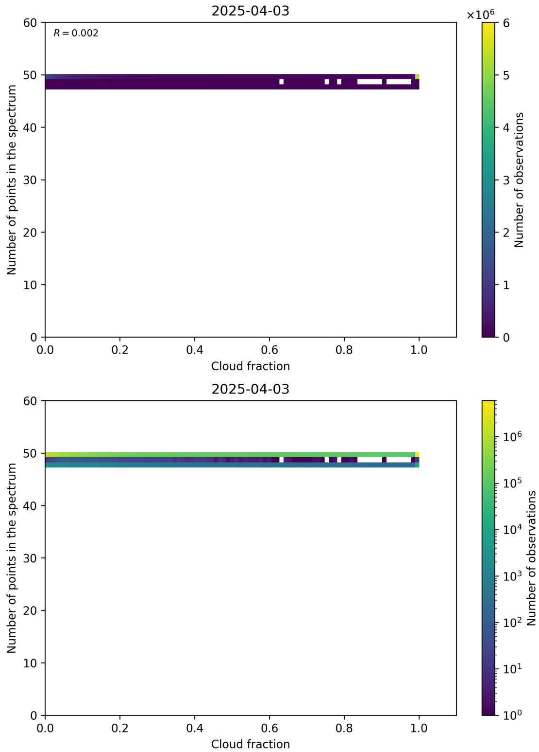
Figure 74: Scatter density plot of “Cloud fraction” against “Number of points in the spectrum” for 2025-04-03 to 2025-04-04.
