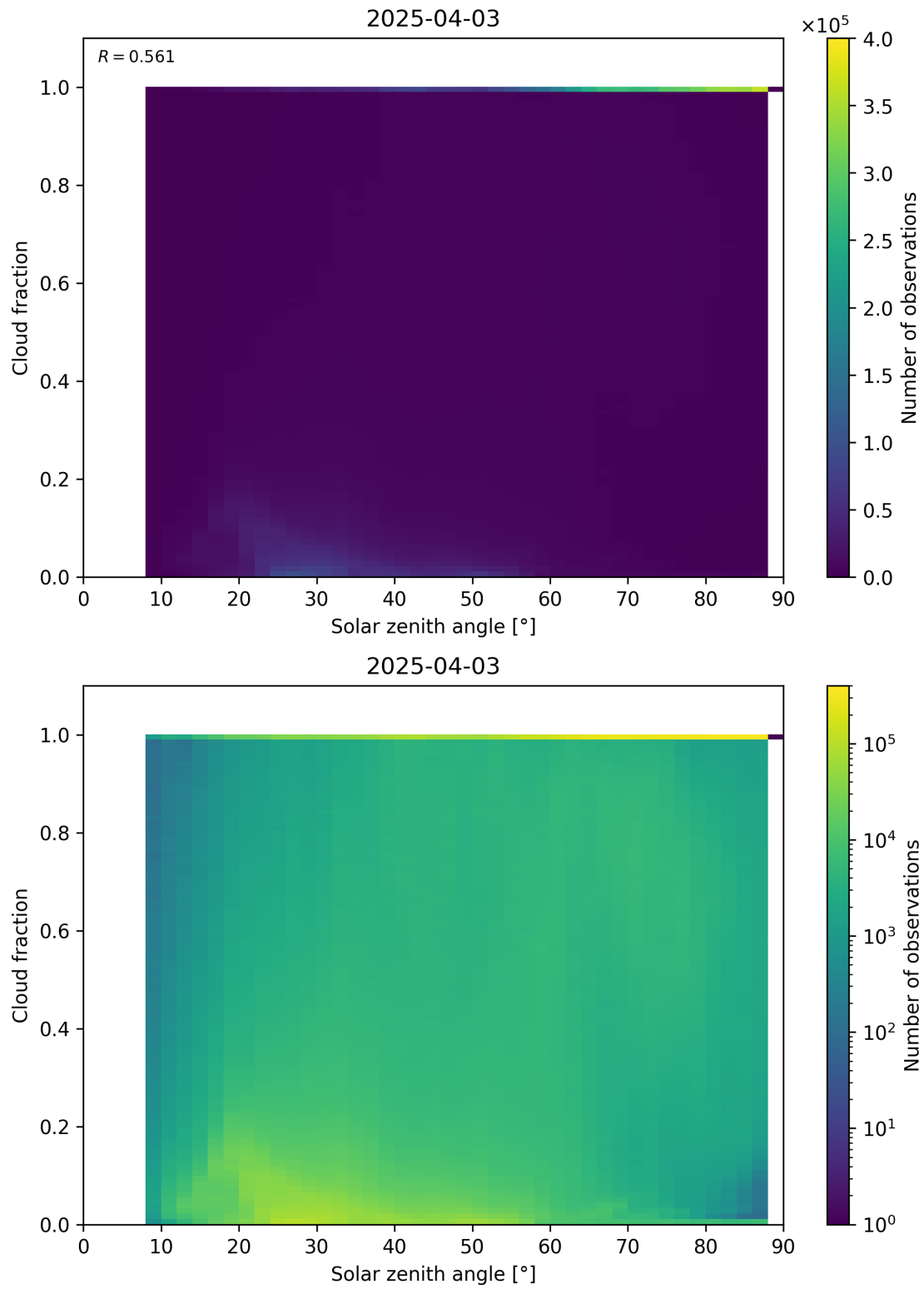
Figure 110: Scatter density plot of “Solar zenith angle” against “Cloud fraction” for 2025-04-03 to 2025-04-04.
