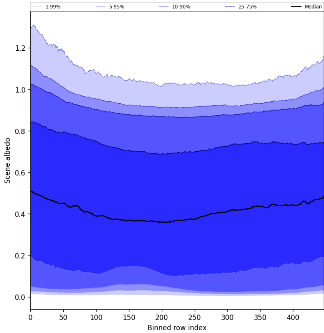
Figure 51: Along track statistics of “Scene albedo” for 2025-04-03 to 2025-04-04
