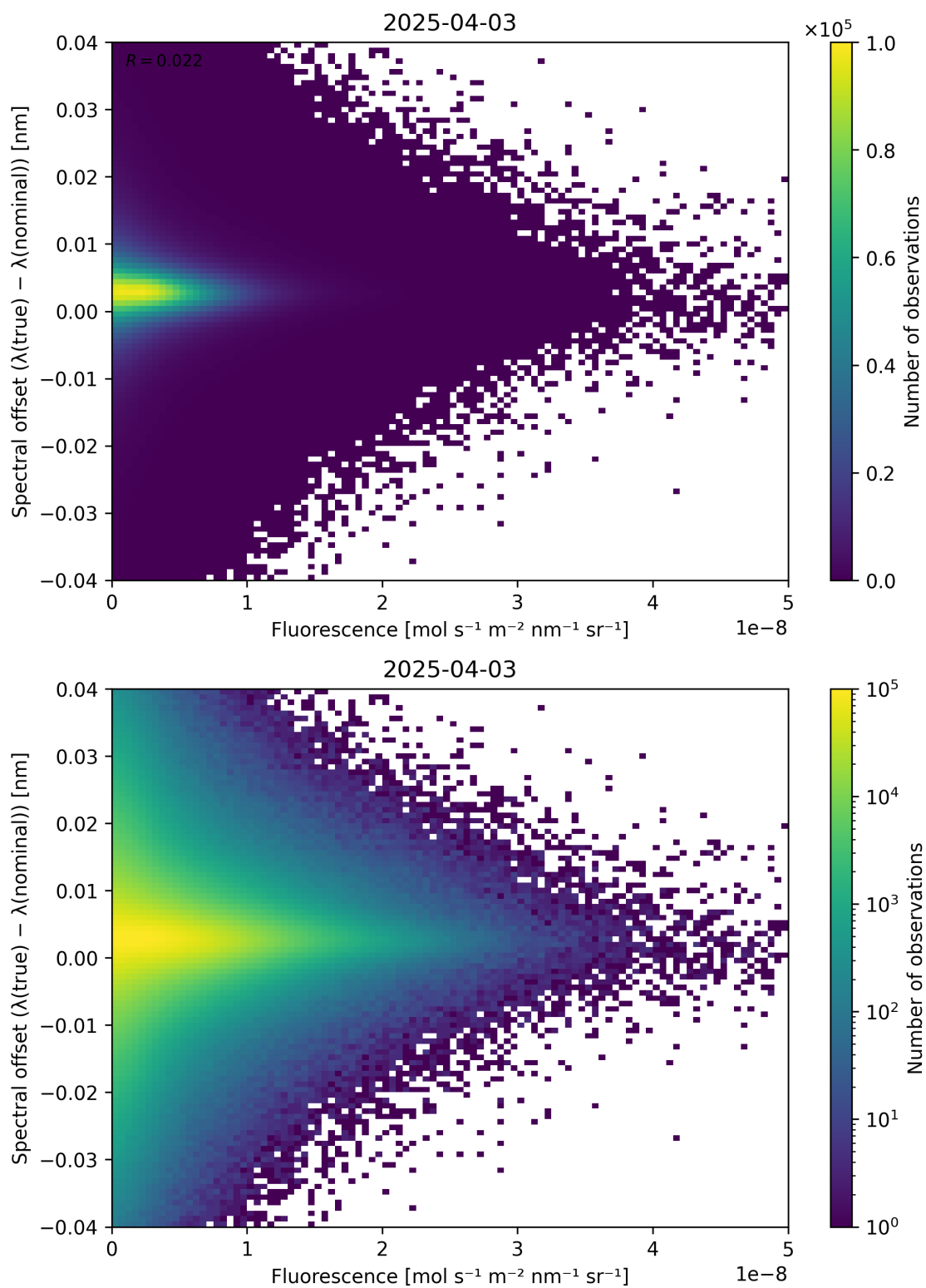
Figure 87: Scatter density plot of “Fluorescence” against “Spectral offset ( \lambda_{\text{true}} - \lambda_{\text{nominal}} )” for 2025-04-03 to 2025-04-04.
