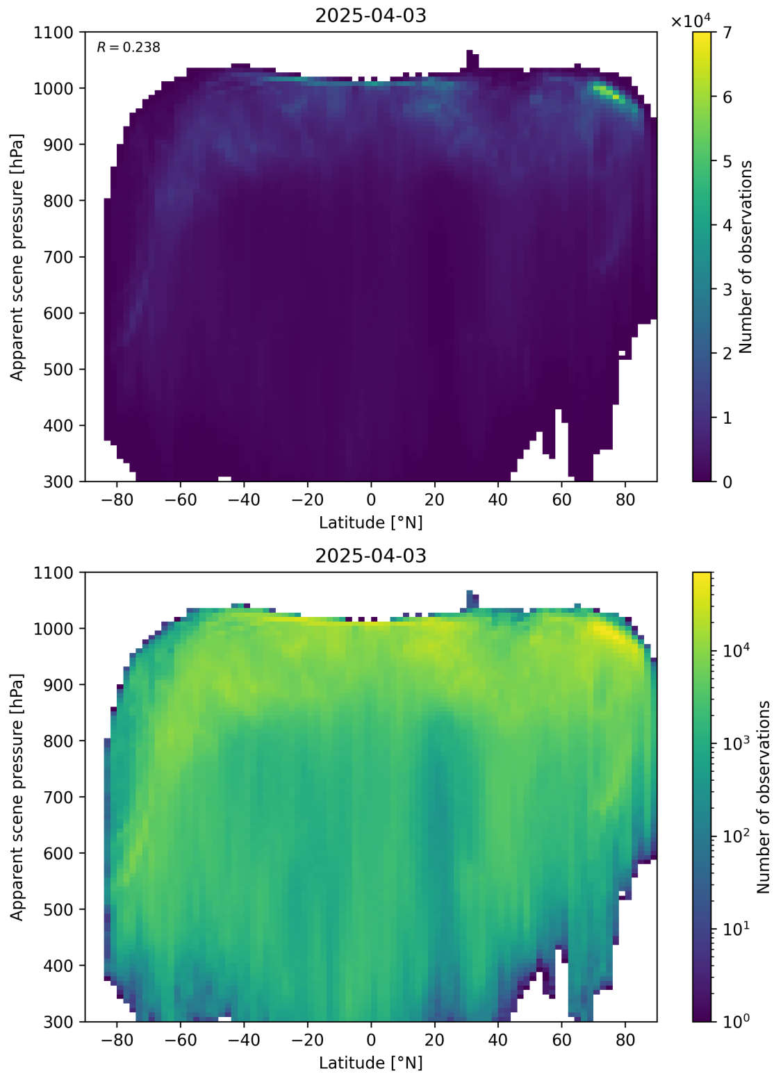
Figure 88: Scatter density plot of “Latitude” against “Apparent scene pressure” for 2025-04-03 to 2025-04-04.
