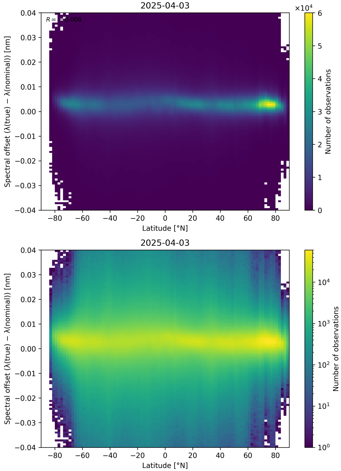
Figure 96: Scatter density plot of “Latitude” against “Spectral offset ( \lambda_{\text{true}} - \lambda_{\text{nominal}} )” for 2025-04-03 to 2025-04-04.
