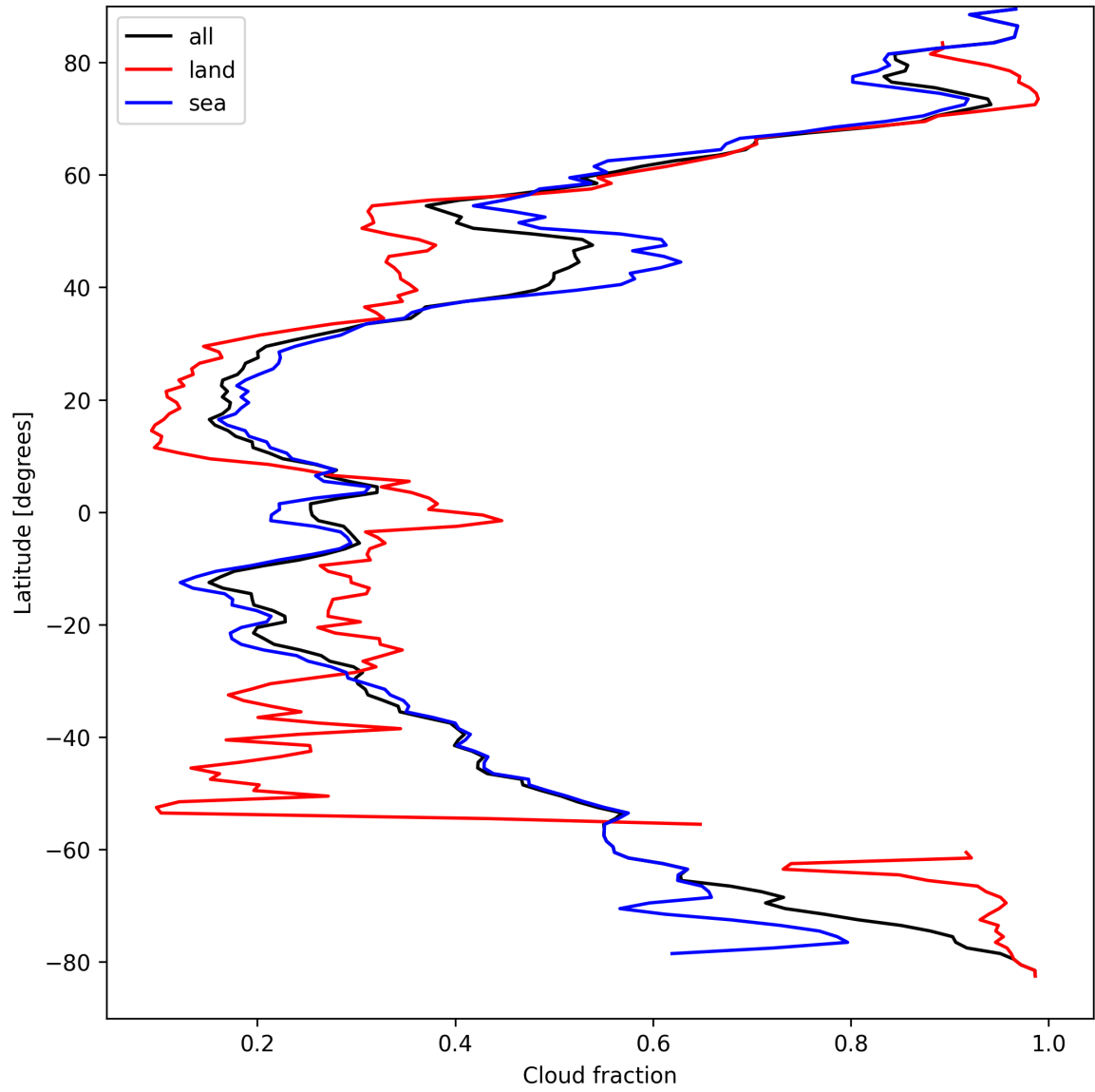
Figure 15: Zonal average of “Cloud fraction” for 2025-04-03 to 2025-04-04.
