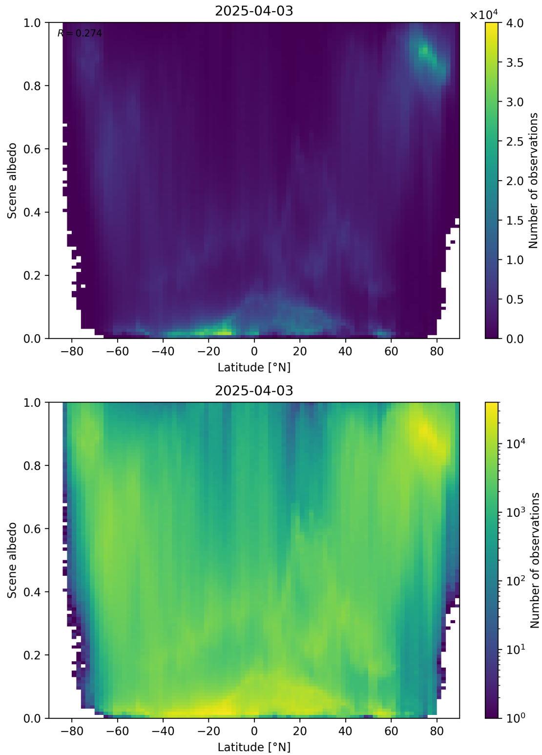
Figure 95: Scatter density plot of “Latitude” against “Scene albedo” for 2025-04-03 to 2025-04-04.
