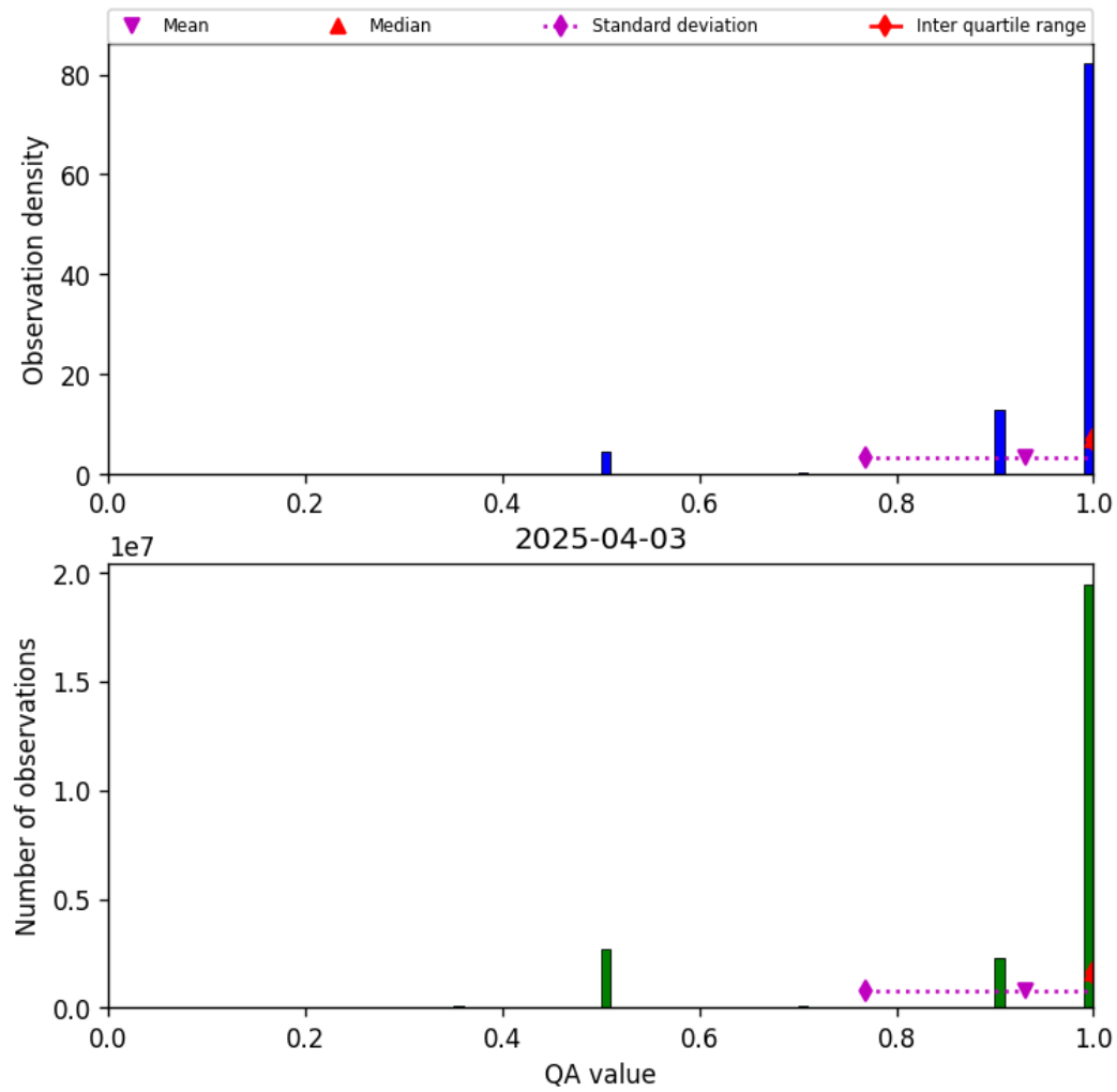
Figure 29: Histogram of “QA value” for 2025-04-03 to 2025-04-04
