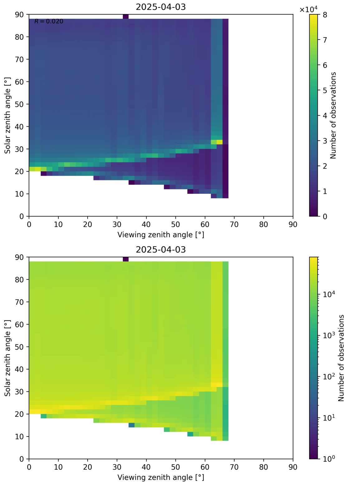
Figure 127: Scatter density plot of “Viewing zenith angle” against “Solar zenith angle” for 2025-04-03 to 2025-04-04.
