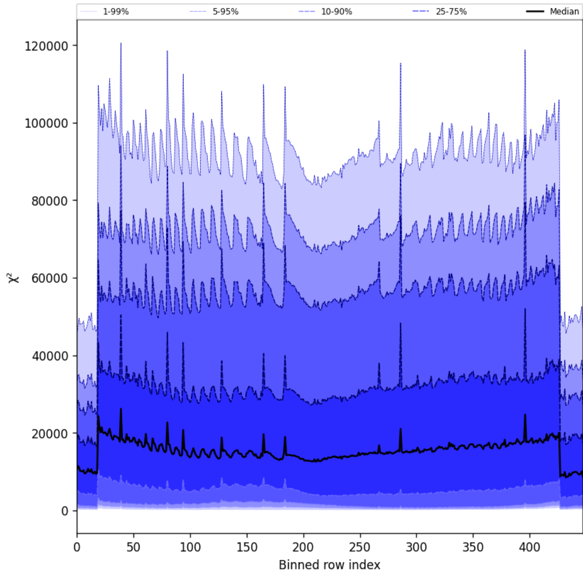
Figure 55: Along track statistics of “ \chi^2 ” for 2025-04-03 to 2025-04-04
