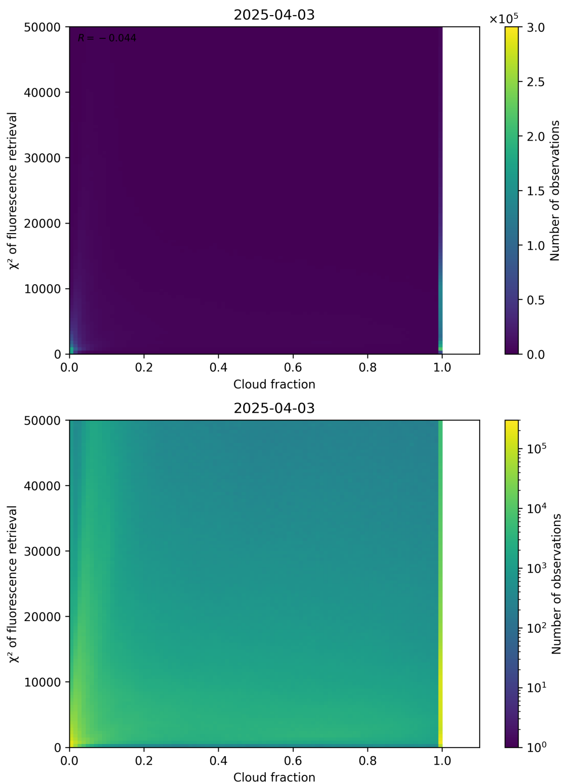
Figure 71: Scatter density plot of “Cloud fraction” against “ \chi^2 of fluorescence retrieval” for 2025-04-03 to 2025-04-04.
