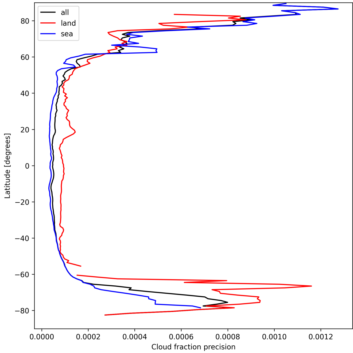
Figure 16: Zonal average of “Cloud fraction precision” for 2025-04-03 to 2025-04-04.
