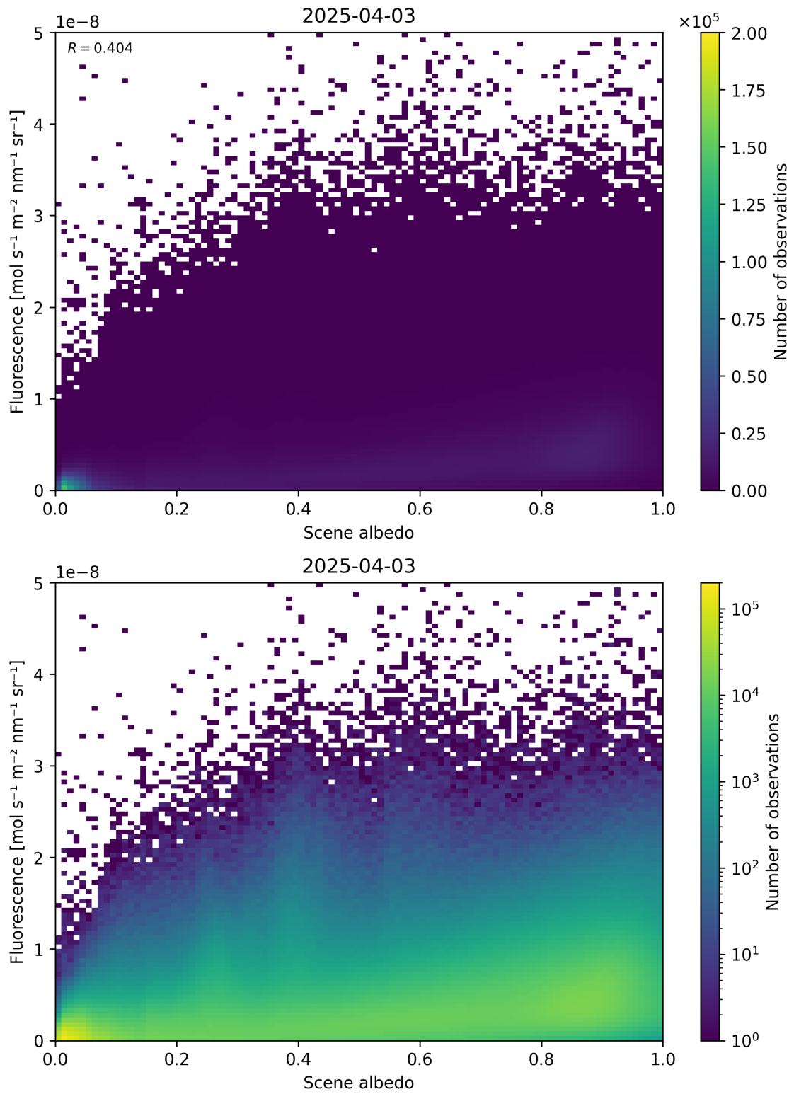
Figure 104: Scatter density plot of “Scene albedo” against “Fluorescence” for 2025-04-03 to 2025-04-04.
