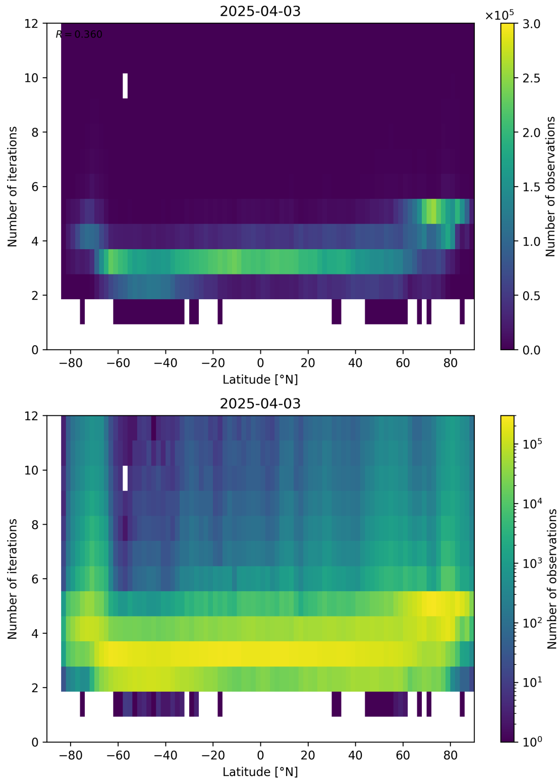
Figure 93: Scatter density plot of “Latitude” against “Number of iterations” for 2025-04-03 to 2025-04-04.
