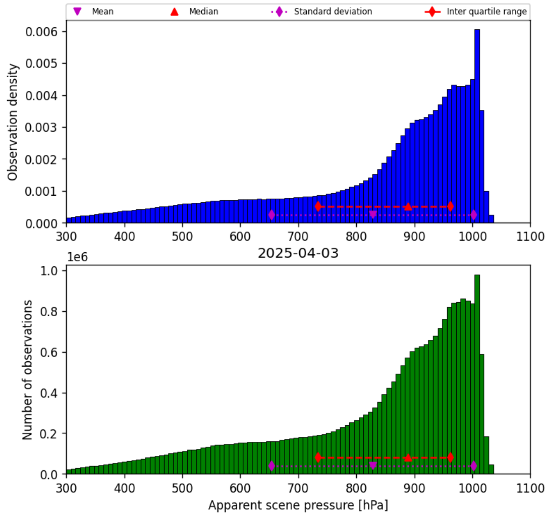
Figure 36: Histogram of “Apparent scene pressure” for 2025-04-03 to 2025-04-04
