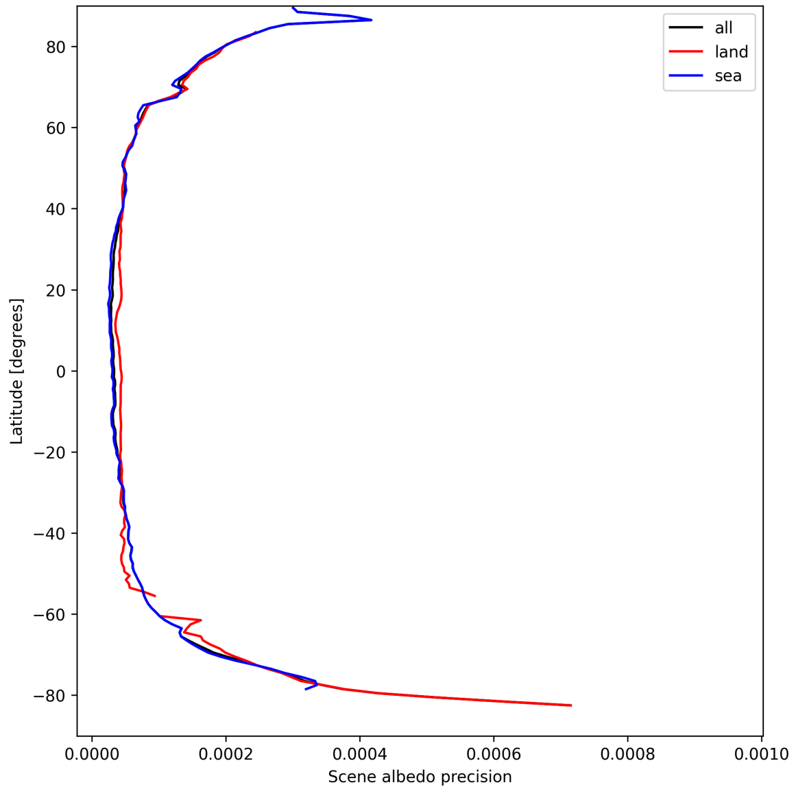
Figure 18: Zonal average of “Scene albedo precision” for 2025-04-03 to 2025-04-04.
