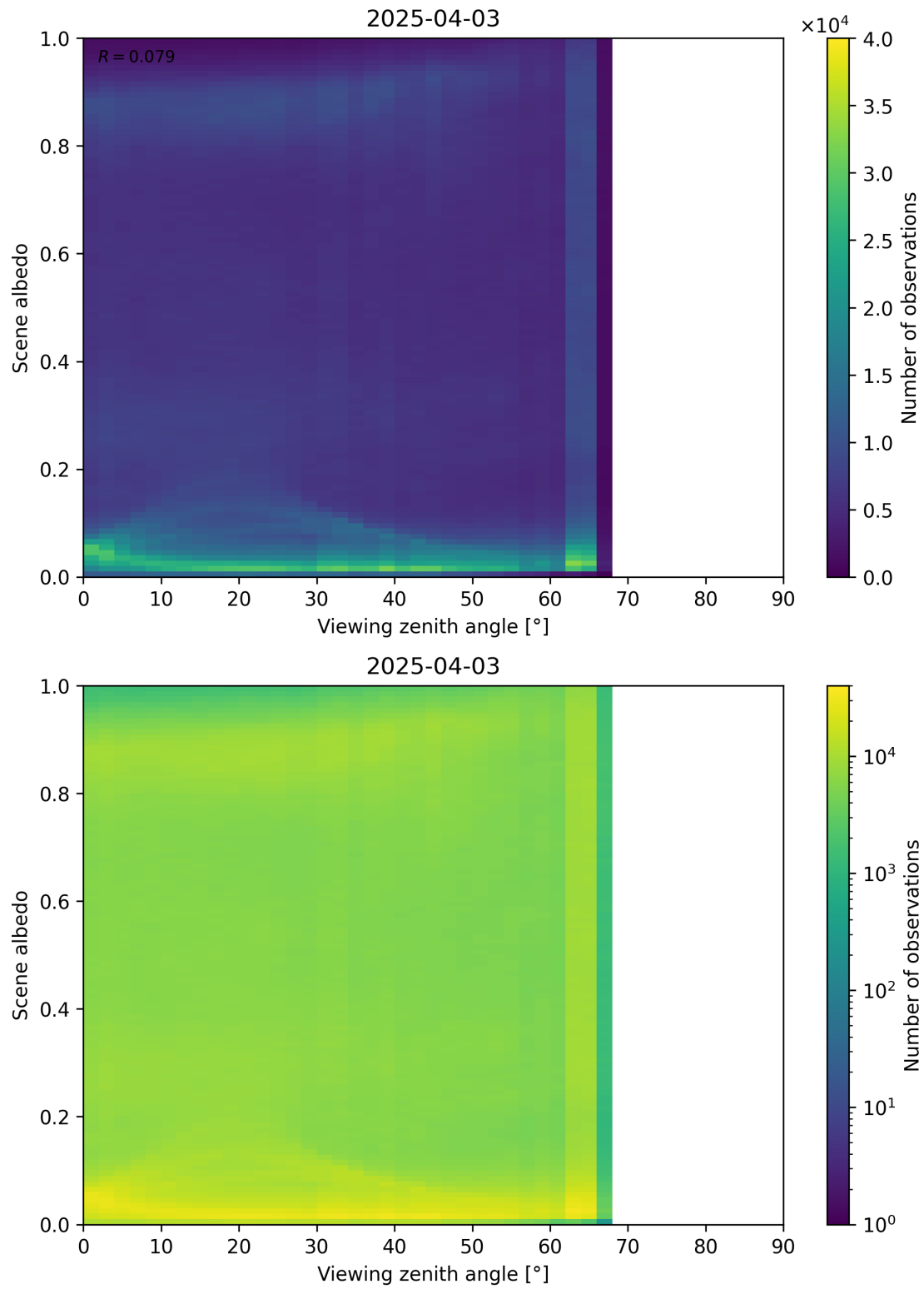
Figure 126: Scatter density plot of “Viewing zenith angle” against “Scene albedo” for 2025-04-03 to 2025-04-04.
