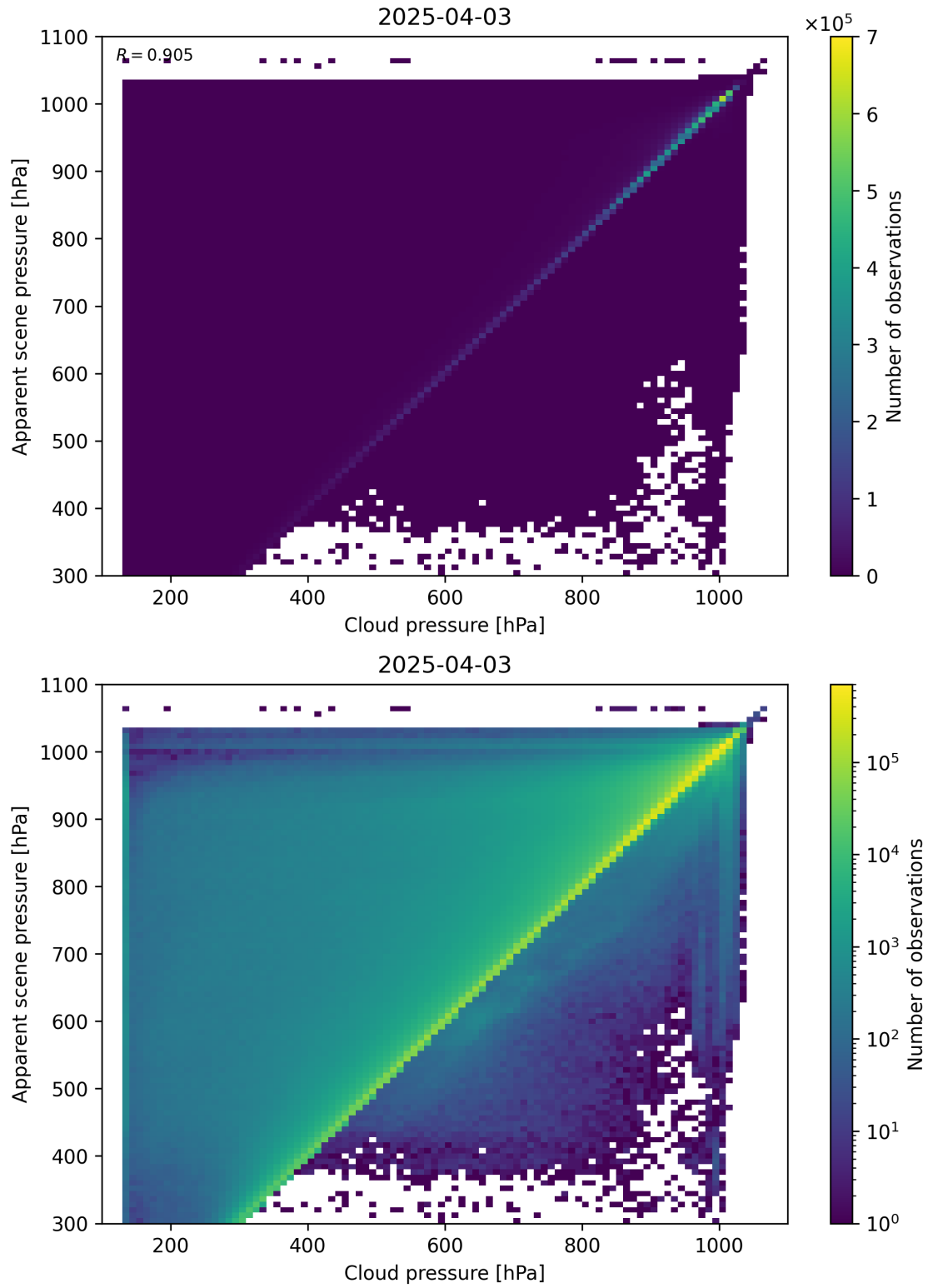
Figure 77: Scatter density plot of “Cloud pressure” against “Apparent scene pressure” for 2025-04-03 to 2025-04-04.
