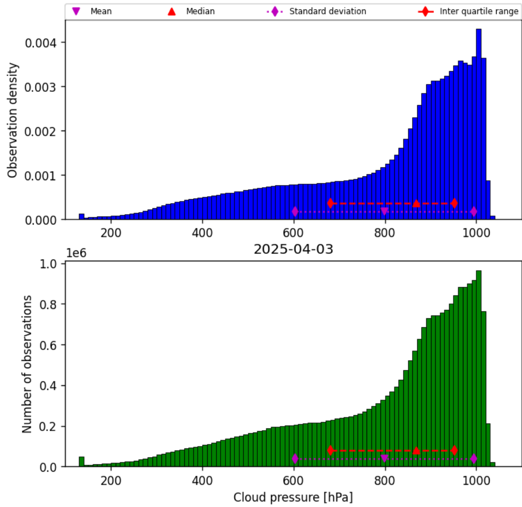
Figure 30: Histogram of “Cloud pressure” for 2025-04-03 to 2025-04-04
