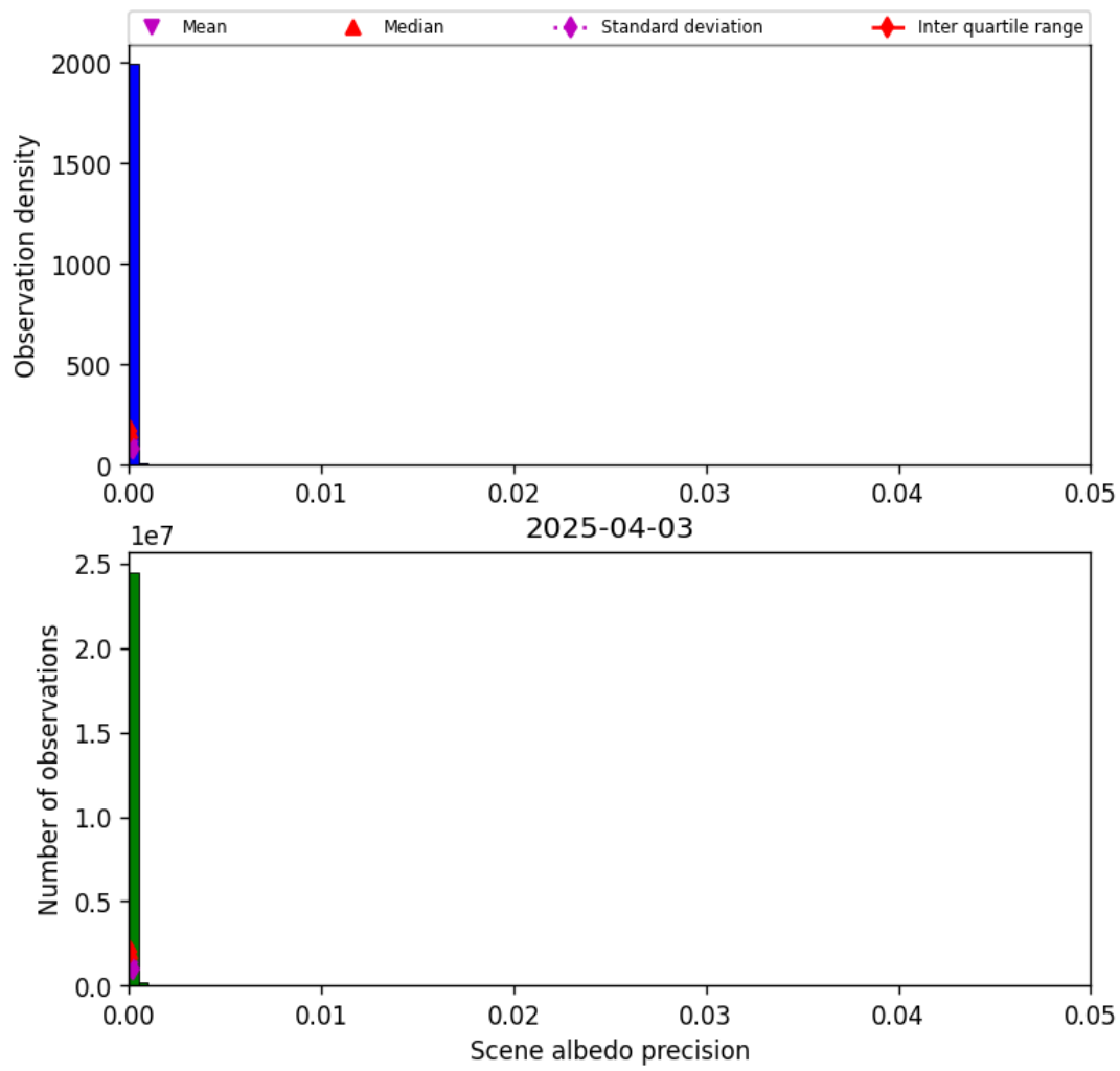
Figure 35: Histogram of “Scene albedo precision” for 2025-04-03 to 2025-04-04
