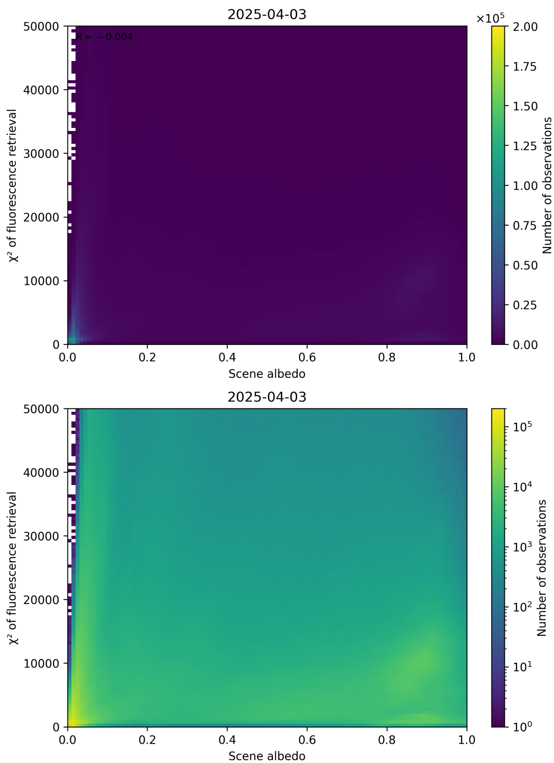
Figure 103: Scatter density plot of “Scene albedo” against “ \chi^2 of fluorescence retrieval” for 2025-04-03 to 2025-04-04.
