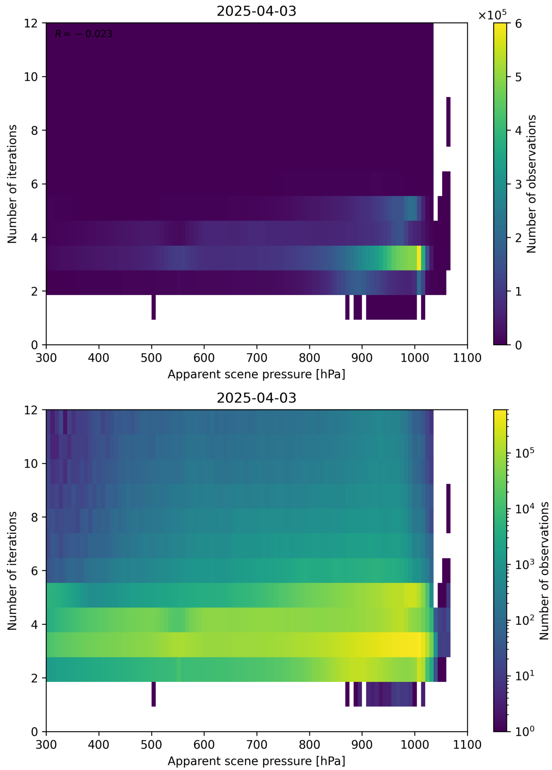
Figure 65: Scatter density plot of “Apparent scene pressure” against “Number of iterations” for 2025-04-03 to 2025-04-04.
