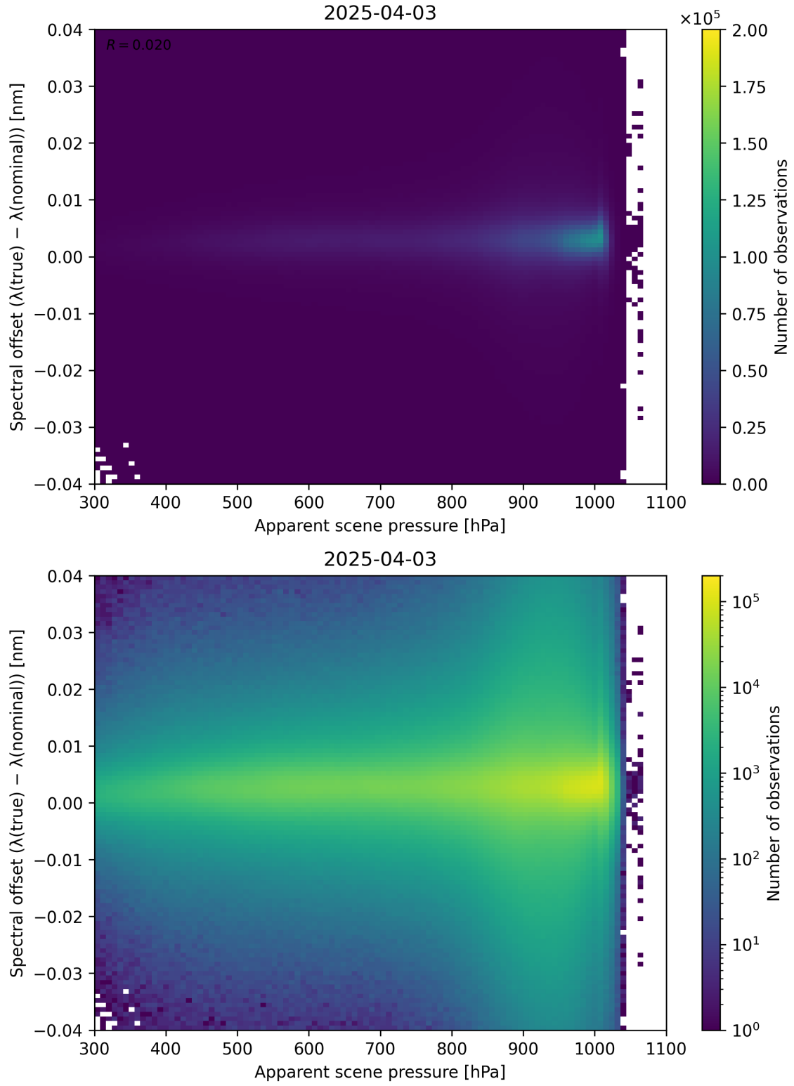
Figure 67: Scatter density plot of “Apparent scene pressure” against “Spectral offset ( \lambda_{\text{true}} - \lambda_{\text{nominal}} )” for 2025-04-03 to 2025-04-04.
