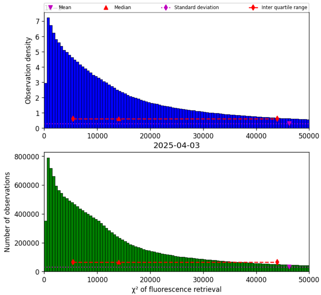
Figure 42: Histogram of “ \chi^2 of fluorescence retrieval” for 2025-04-03 to 2025-04-04
