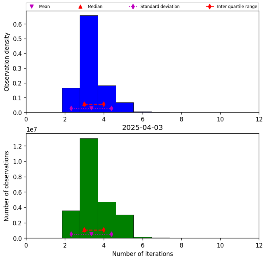
Figure 39: Histogram of “Number of iterations” for 2025-04-03 to 2025-04-04
