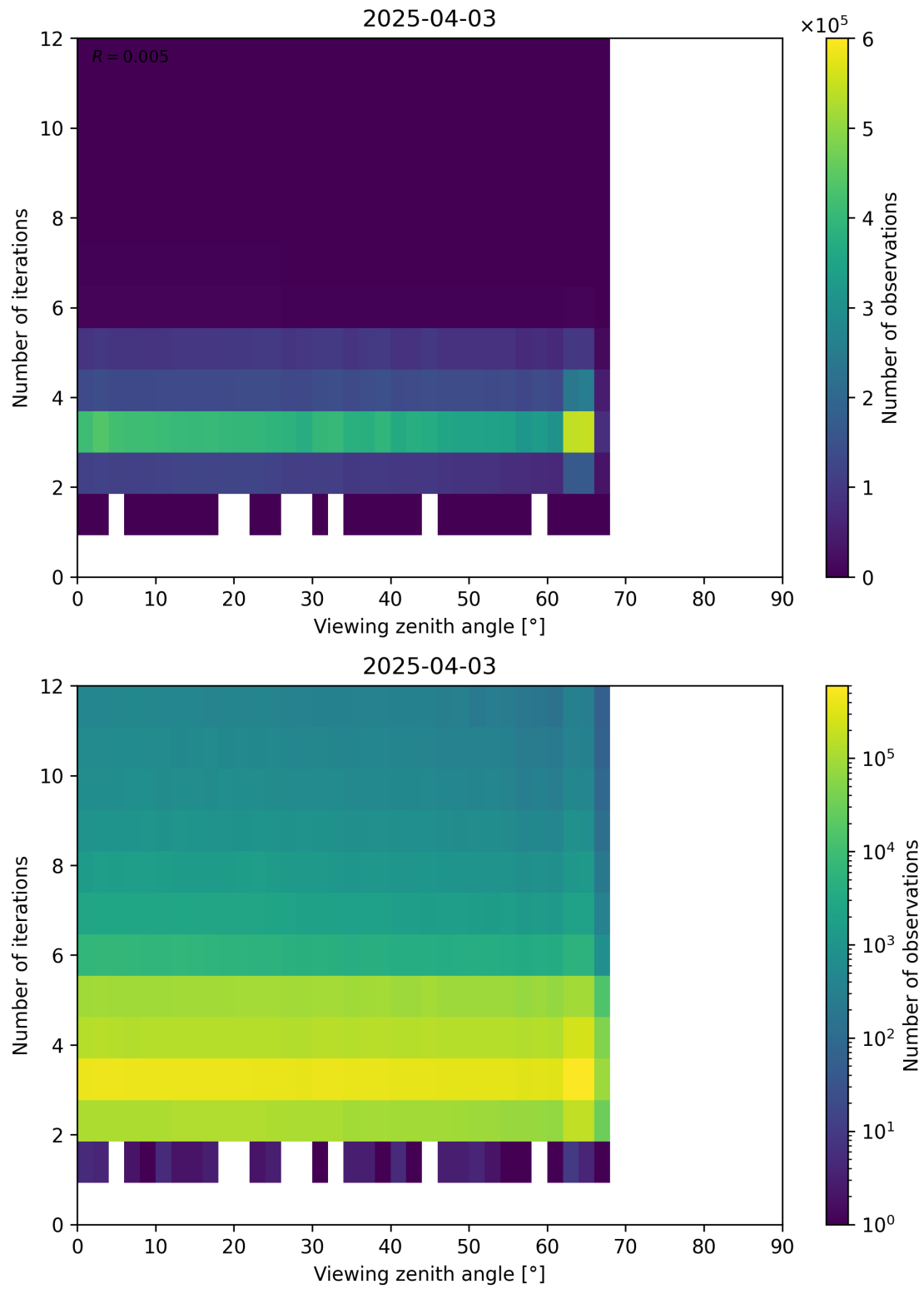
Figure 124: Scatter density plot of “Viewing zenith angle” against “Number of iterations” for 2025-04-03 to 2025-04-04.
