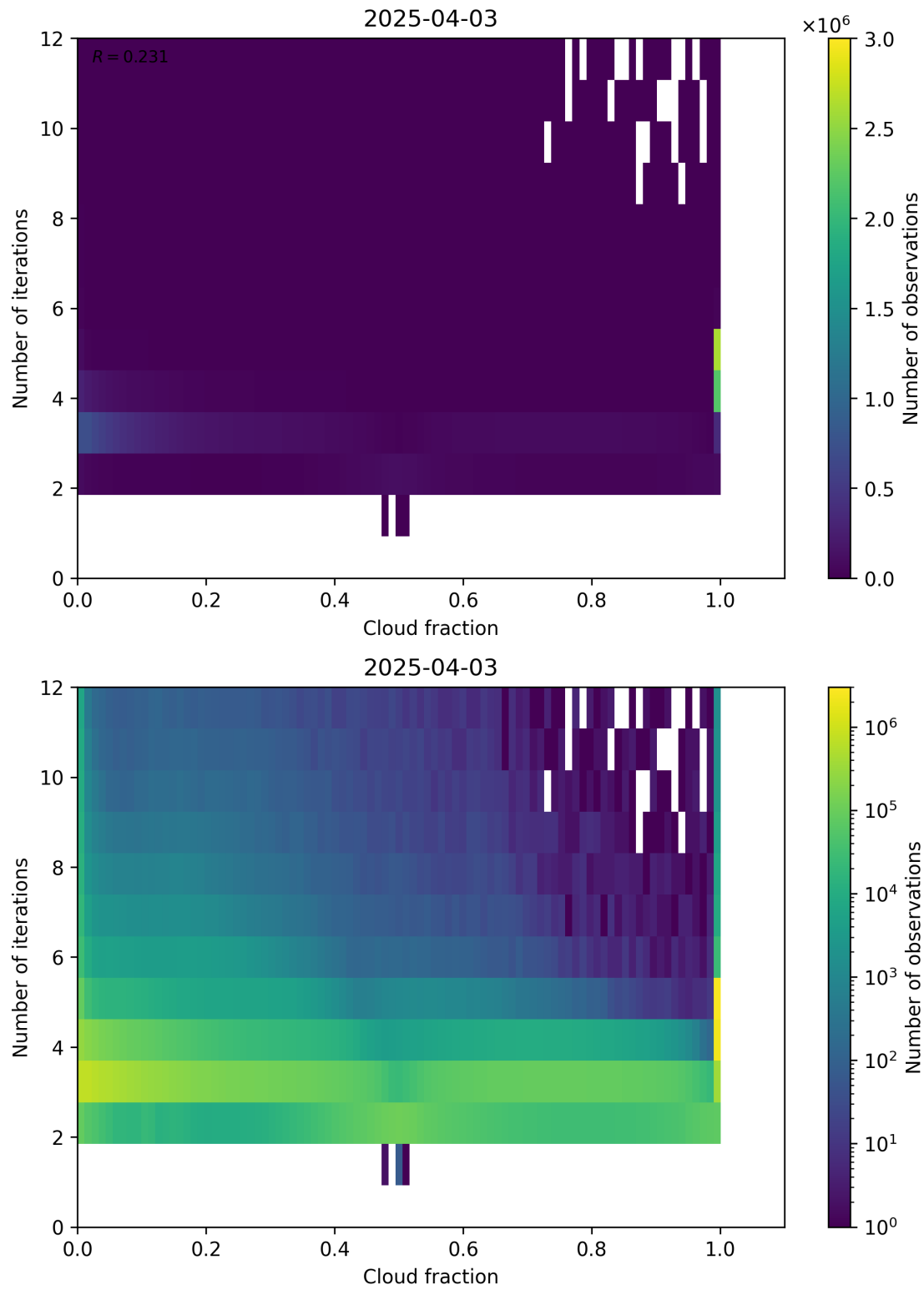
Figure 73: Scatter density plot of “Cloud fraction” against “Number of iterations” for 2025-04-03 to 2025-04-04.
