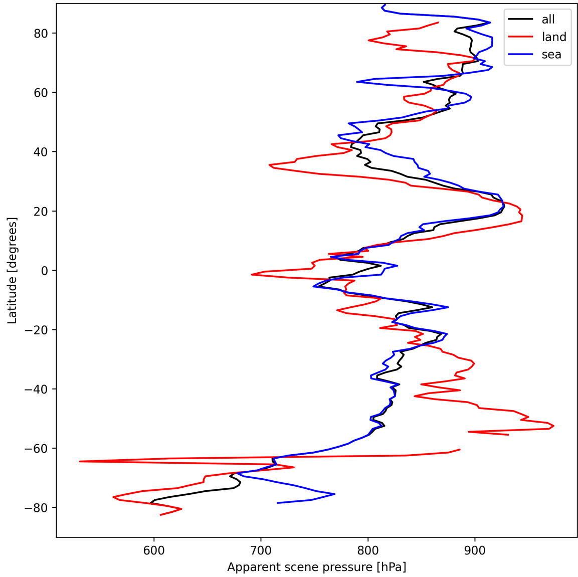
Figure 19: Zonal average of “Apparent scene pressure” for 2025-04-03 to 2025-04-04.
