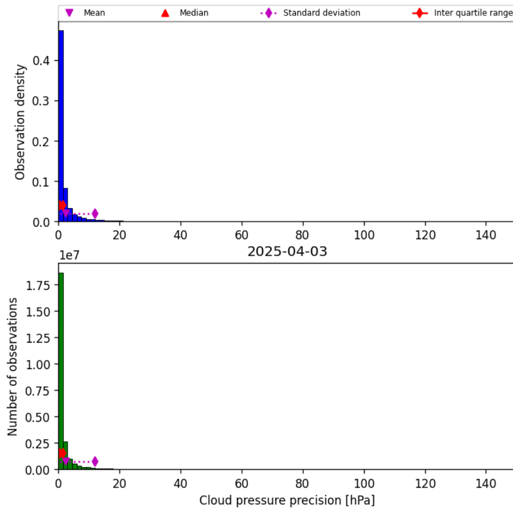
Figure 31: Histogram of “Cloud pressure precision” for 2025-04-03 to 2025-04-04
