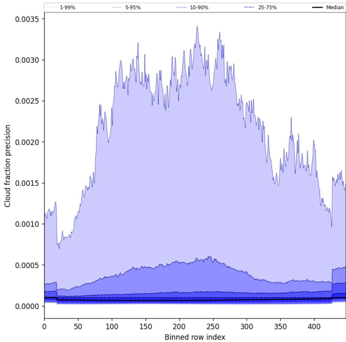
Figure 50: Along track statistics of “Cloud fraction precision” for 2025-04-03 to 2025-04-04
