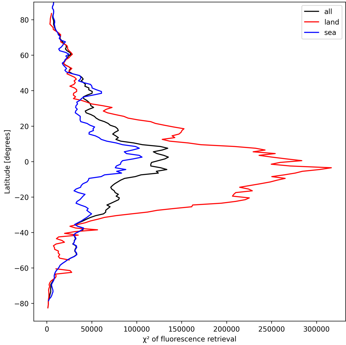
Figure 25: Zonal average of “ \chi^2 of fluorescence retrieval” for 2025-04-03 to 2025-04-04.
