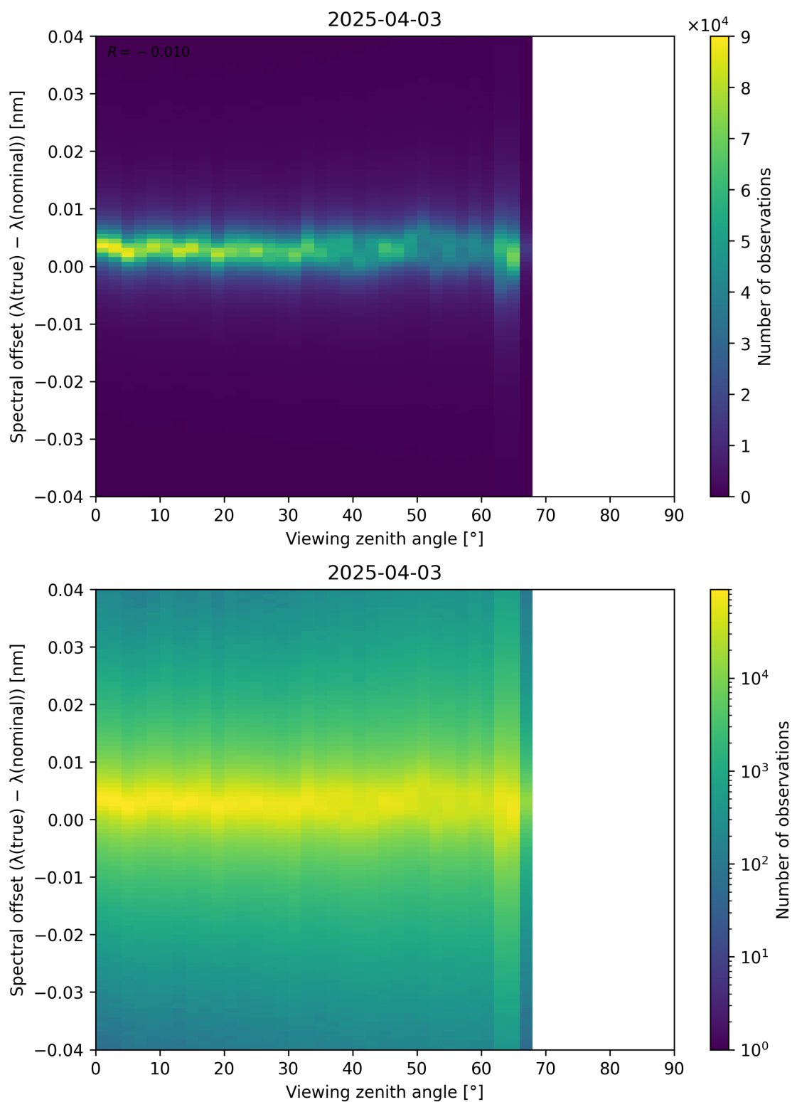
Figure 128: Scatter density plot of “Viewing zenith angle” against “Spectral offset ( \lambda_{\text{true}} - \lambda_{\text{nominal}} )” for 2025-04-03 to 2025-04-04.
