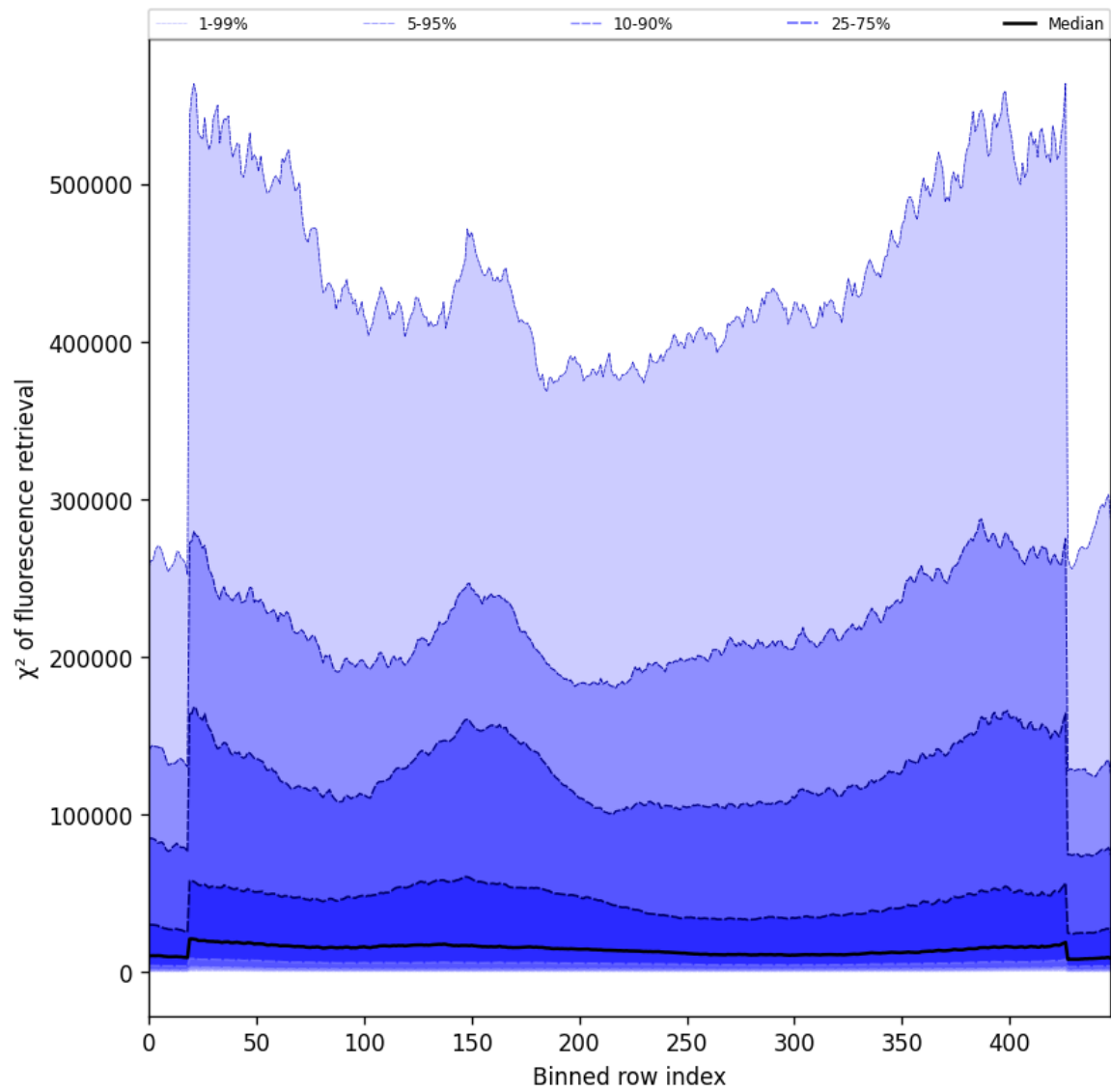
Figure 59: Along track statistics of “ \chi^2 of fluorescence retrieval” for 2025-04-03 to 2025-04-04
