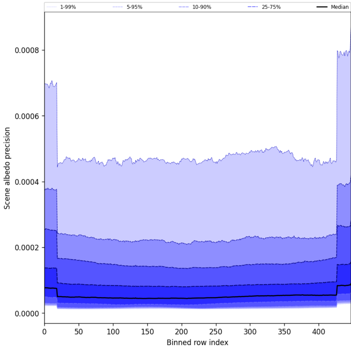
Figure 52: Along track statistics of “Scene albedo precision” for 2025-04-03 to 2025-04-04
