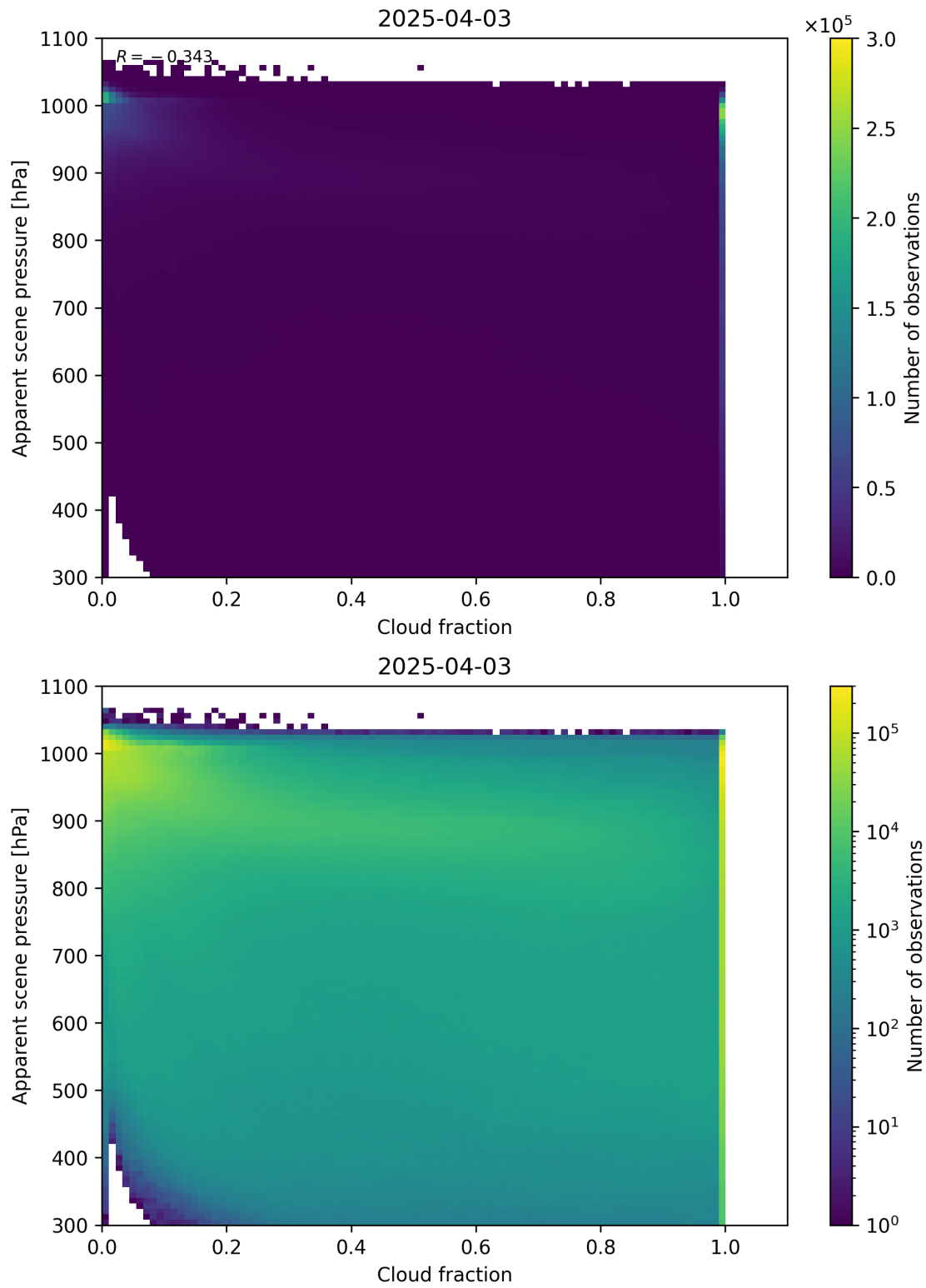
Figure 70: Scatter density plot of “Cloud fraction” against “Apparent scene pressure” for 2025-04-03 to 2025-04-04.
