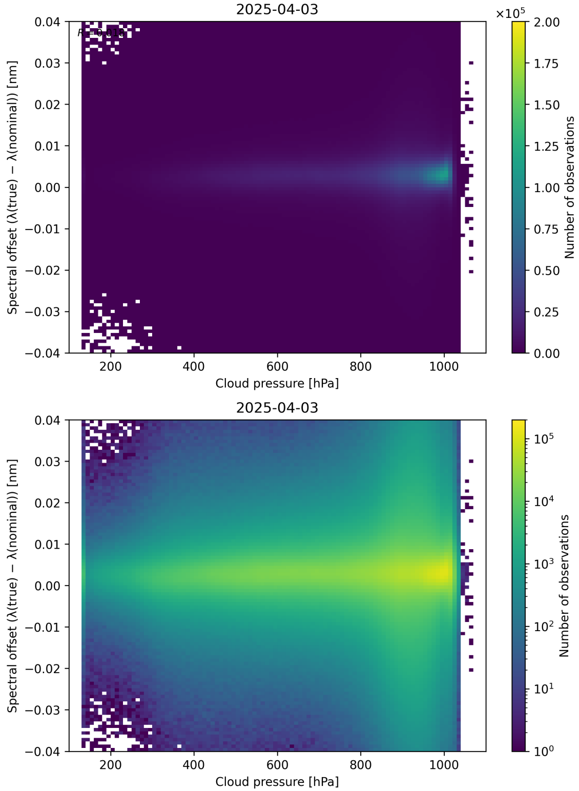
Figure 84: Scatter density plot of “Cloud pressure” against “Spectral offset ( \lambda_{\text{true}} - \lambda_{\text{nominal}} )” for 2025-04-03 to 2025-04-04.
