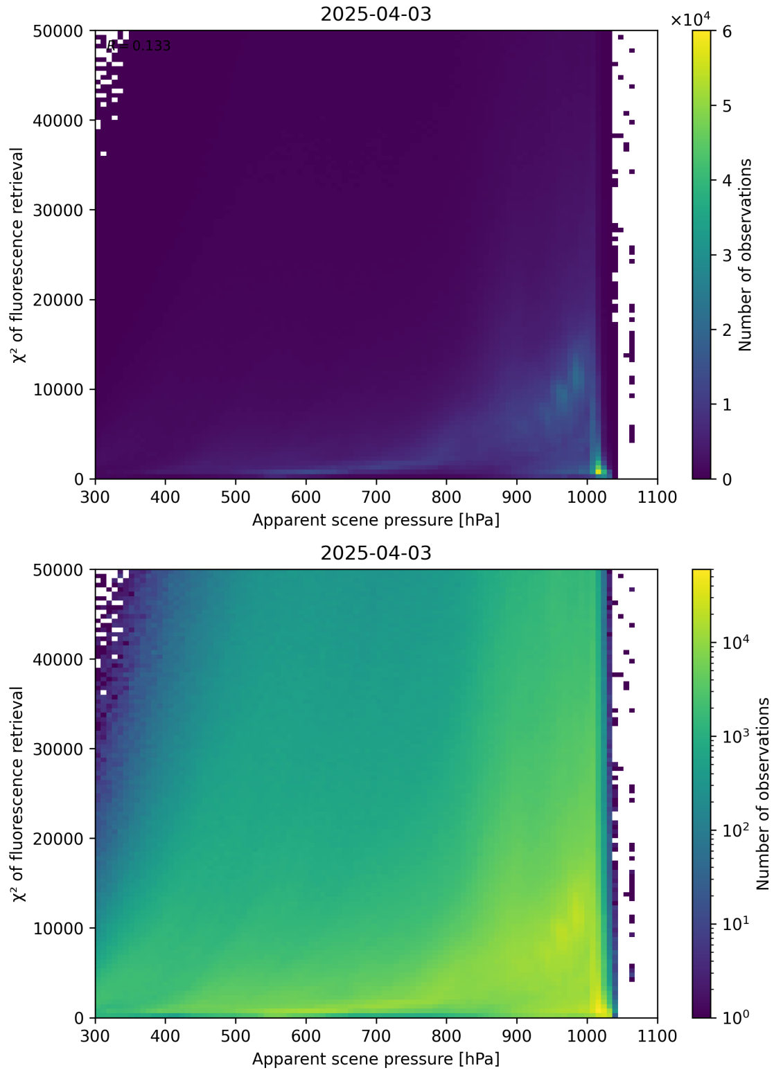
Figure 63: Scatter density plot of “Apparent scene pressure” against “ \chi^2 of fluorescence retrieval” for 2025-04-03 to 2025-04-04.
