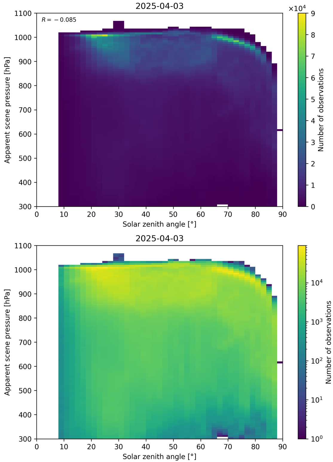
Figure 108: Scatter density plot of “Solar zenith angle” against “Apparent scene pressure” for 2025-04-03 to 2025-04-04.
