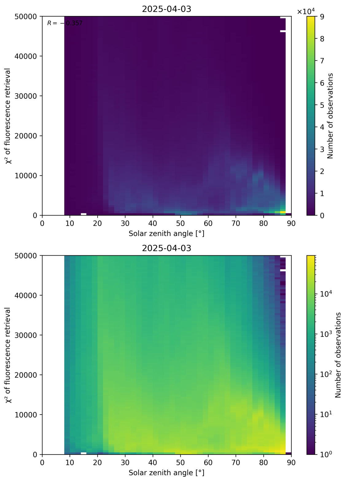
Figure 109: Scatter density plot of “Solar zenith angle” against “ \chi^2 of fluorescence retrieval” for 2025-04-03 to 2025-04-04.
