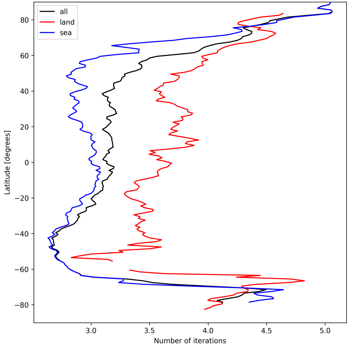
Figure 22: Zonal average of “Number of iterations” for 2025-04-03 to 2025-04-04.
