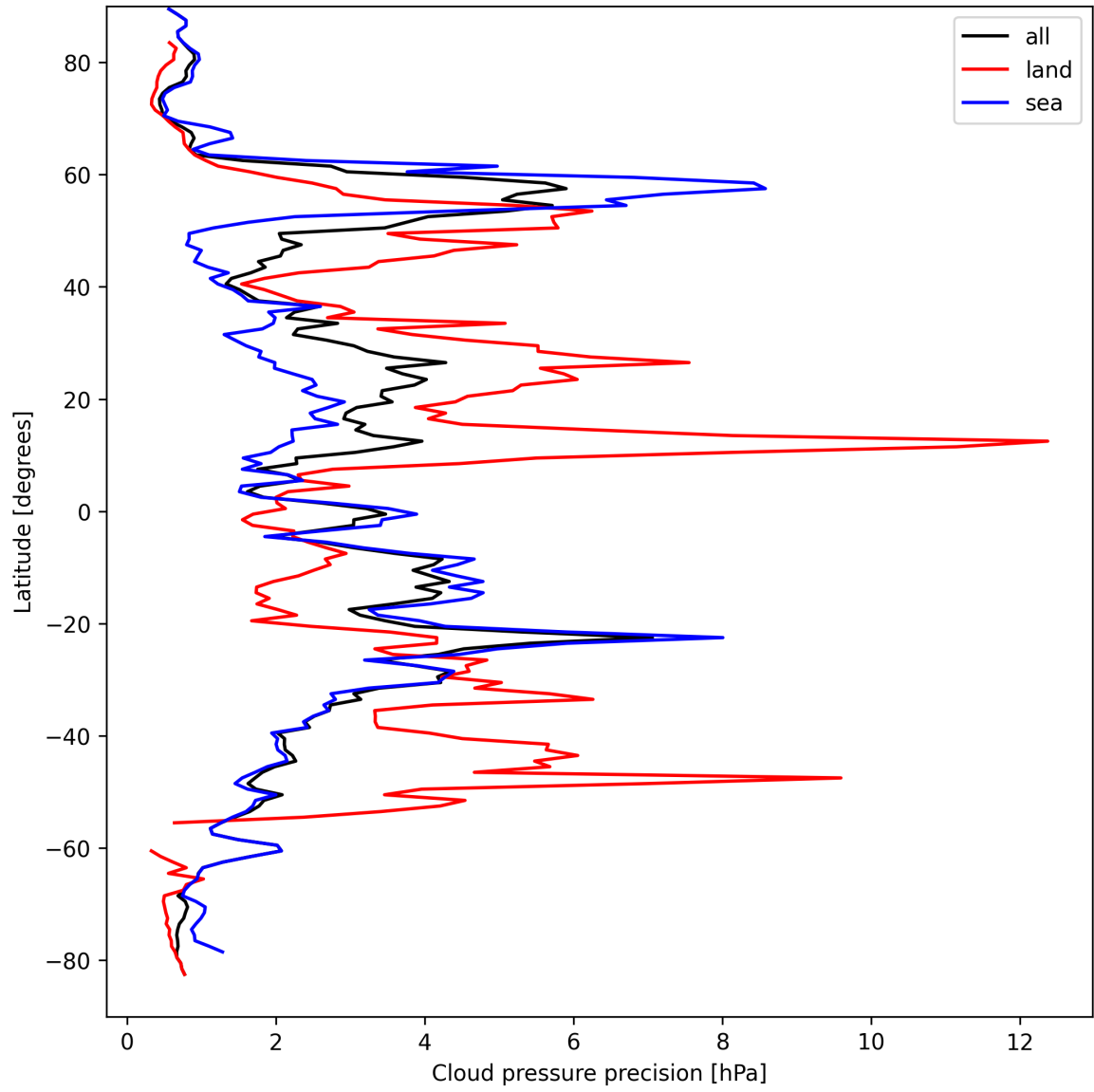
Figure 14: Zonal average of “Cloud pressure precision” for 2025-04-03 to 2025-04-04.
