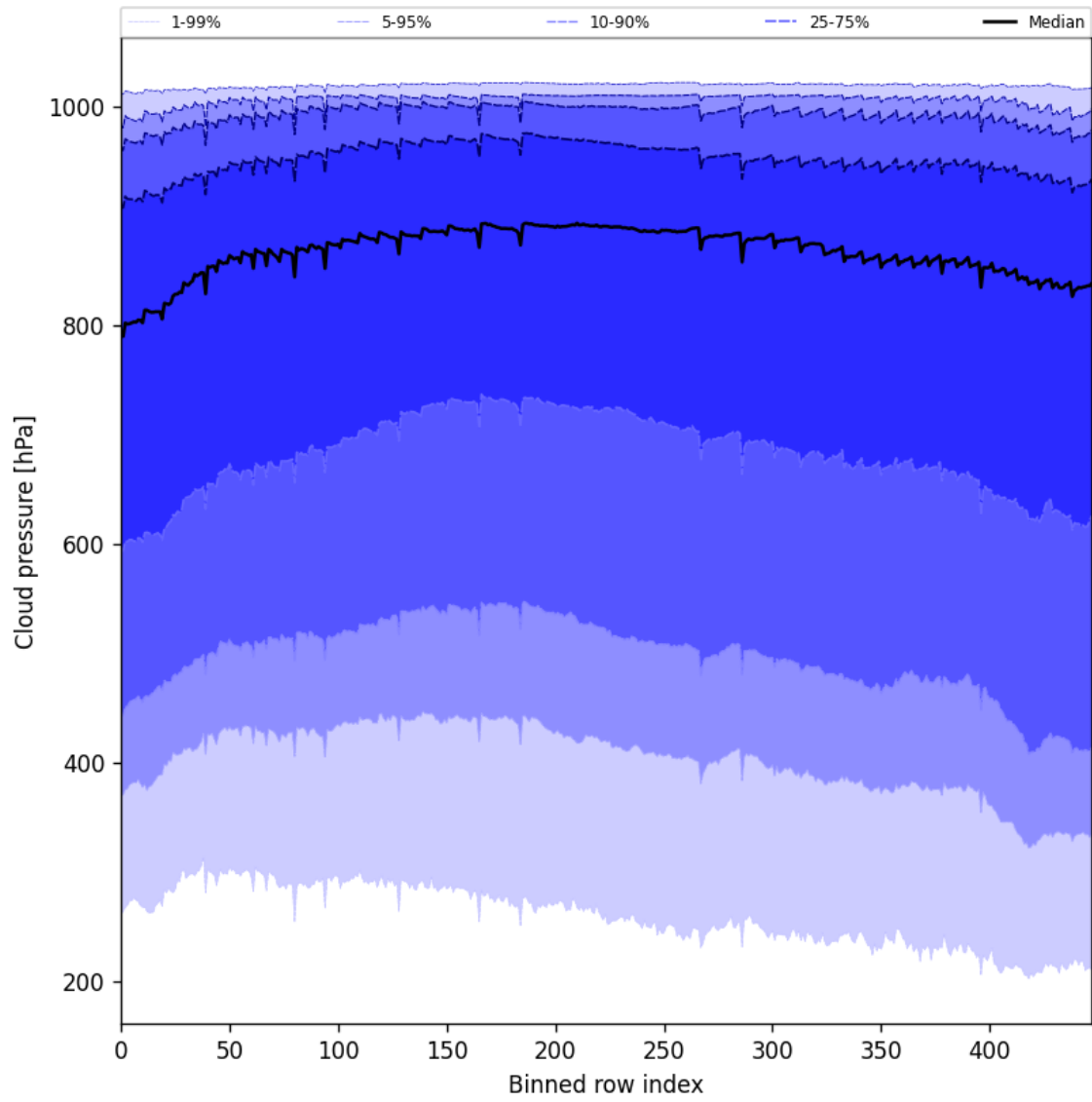
Figure 47: Along track statistics of “Cloud pressure” for 2025-04-03 to 2025-04-04
