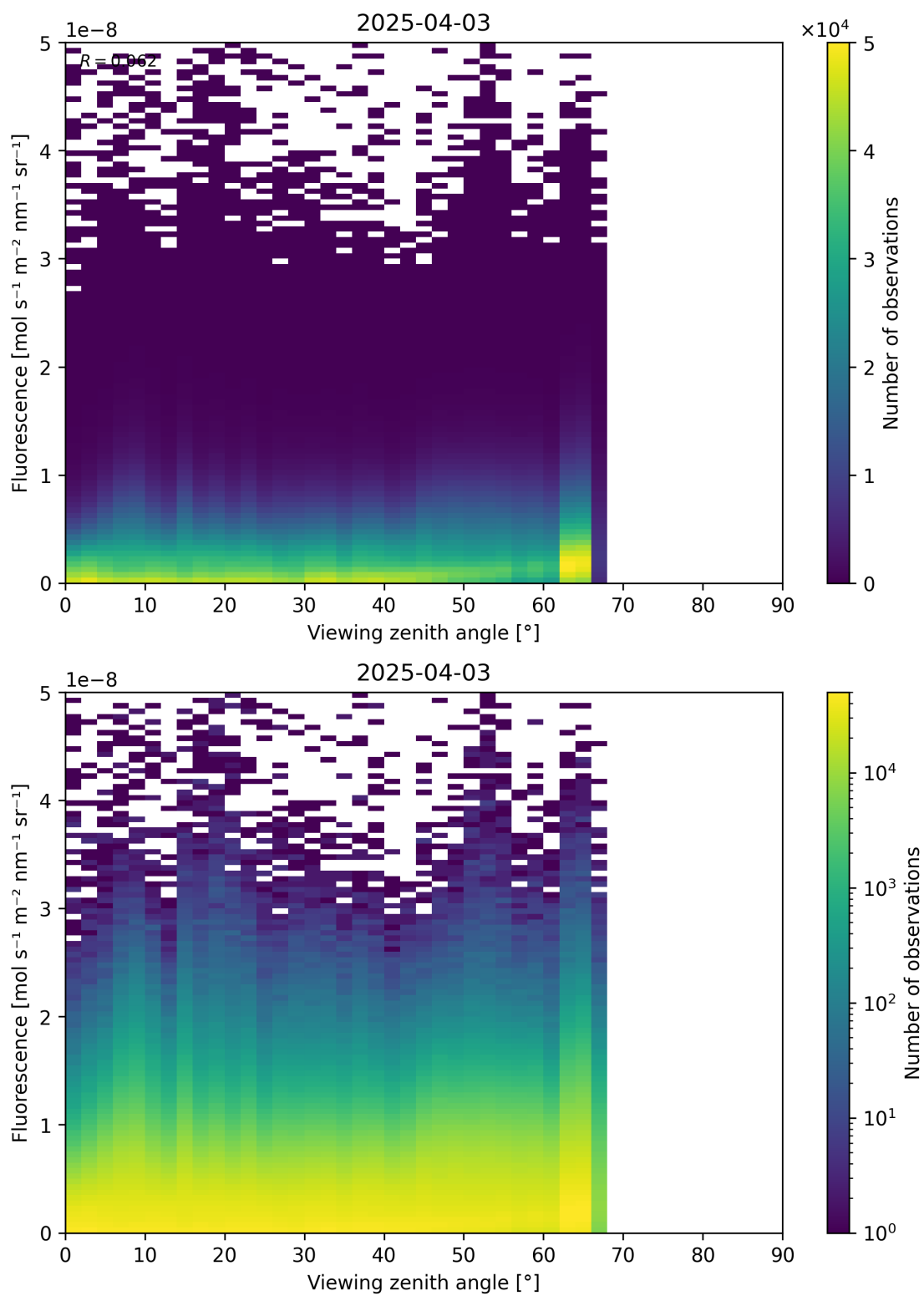
Figure 122: Scatter density plot of “Viewing zenith angle” against “Fluorescence” for 2025-04-03 to 2025-04-04.
