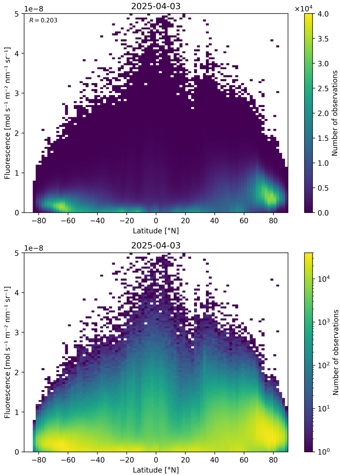
Figure 92: Scatter density plot of “Latitude” against “Fluorescence” for 2025-04-03 to 2025-04-04.
