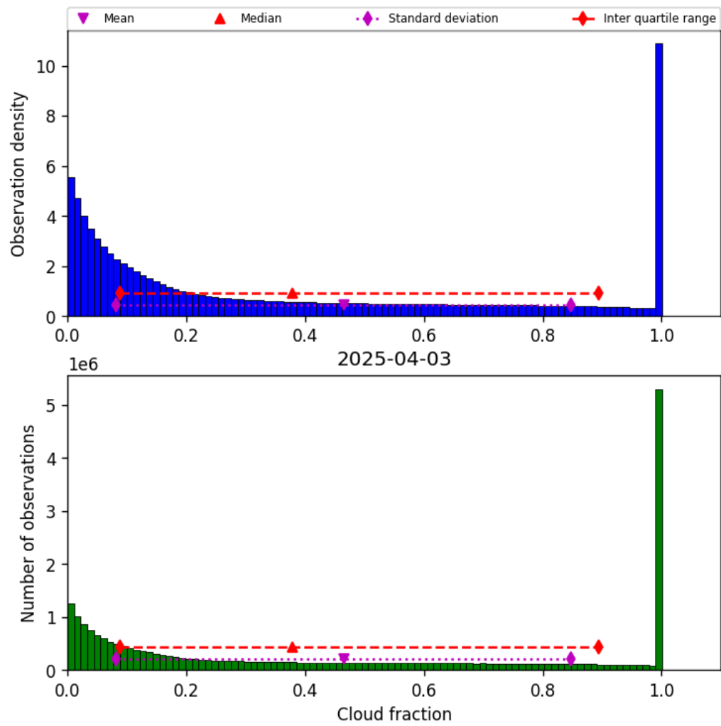
Figure 32: Histogram of “Cloud fraction” for 2025-04-03 to 2025-04-04
