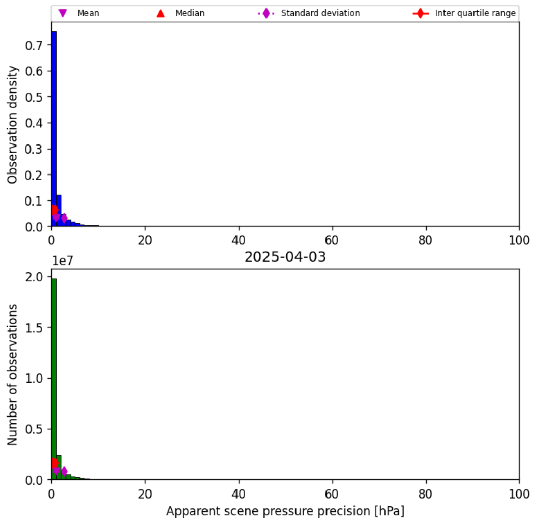
Figure 37: Histogram of “Apparent scene pressure precision” for 2025-04-03 to 2025-04-04
