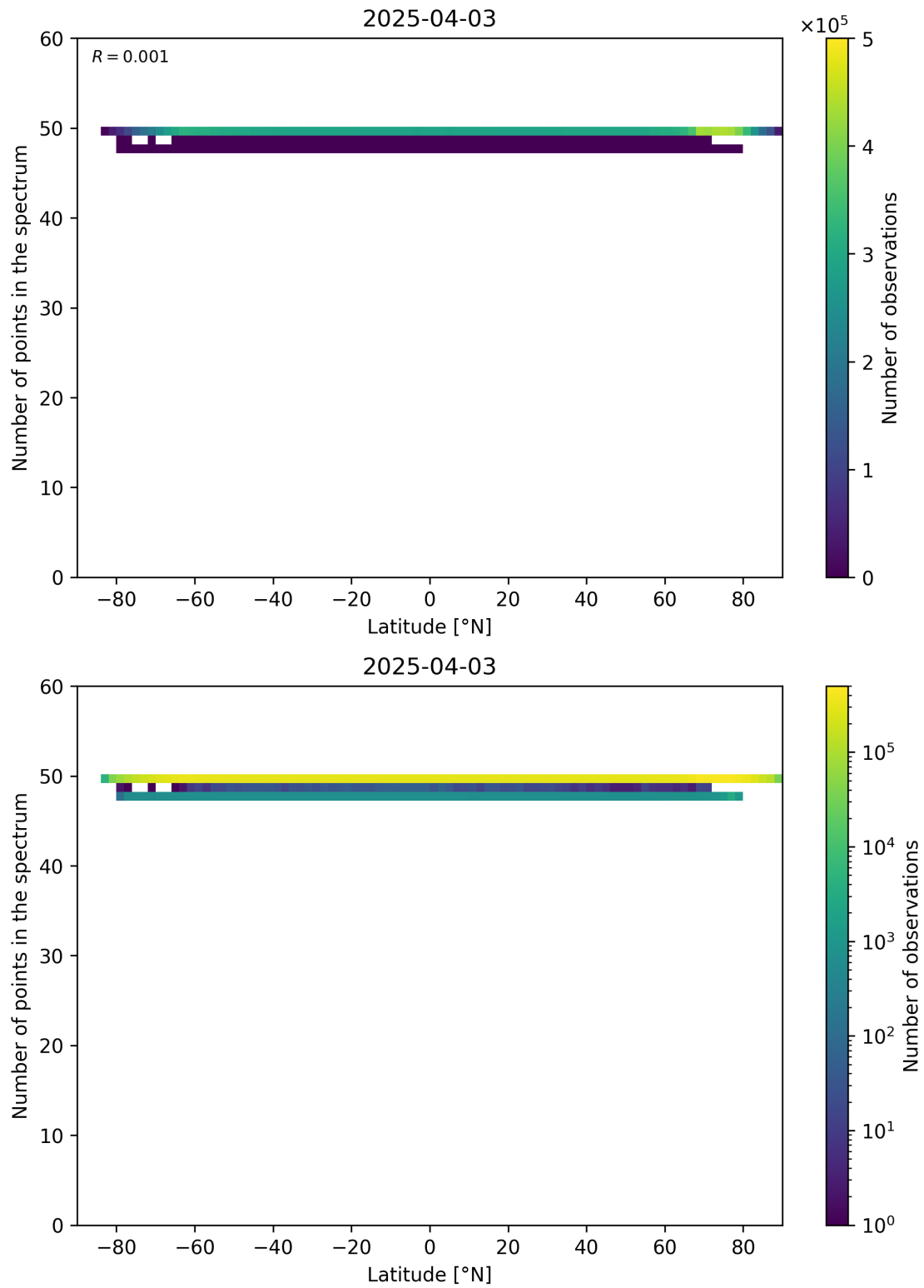
Figure 94: Scatter density plot of “Latitude” against “Number of points in the spectrum” for 2025-04-03 to 2025-04-04.
