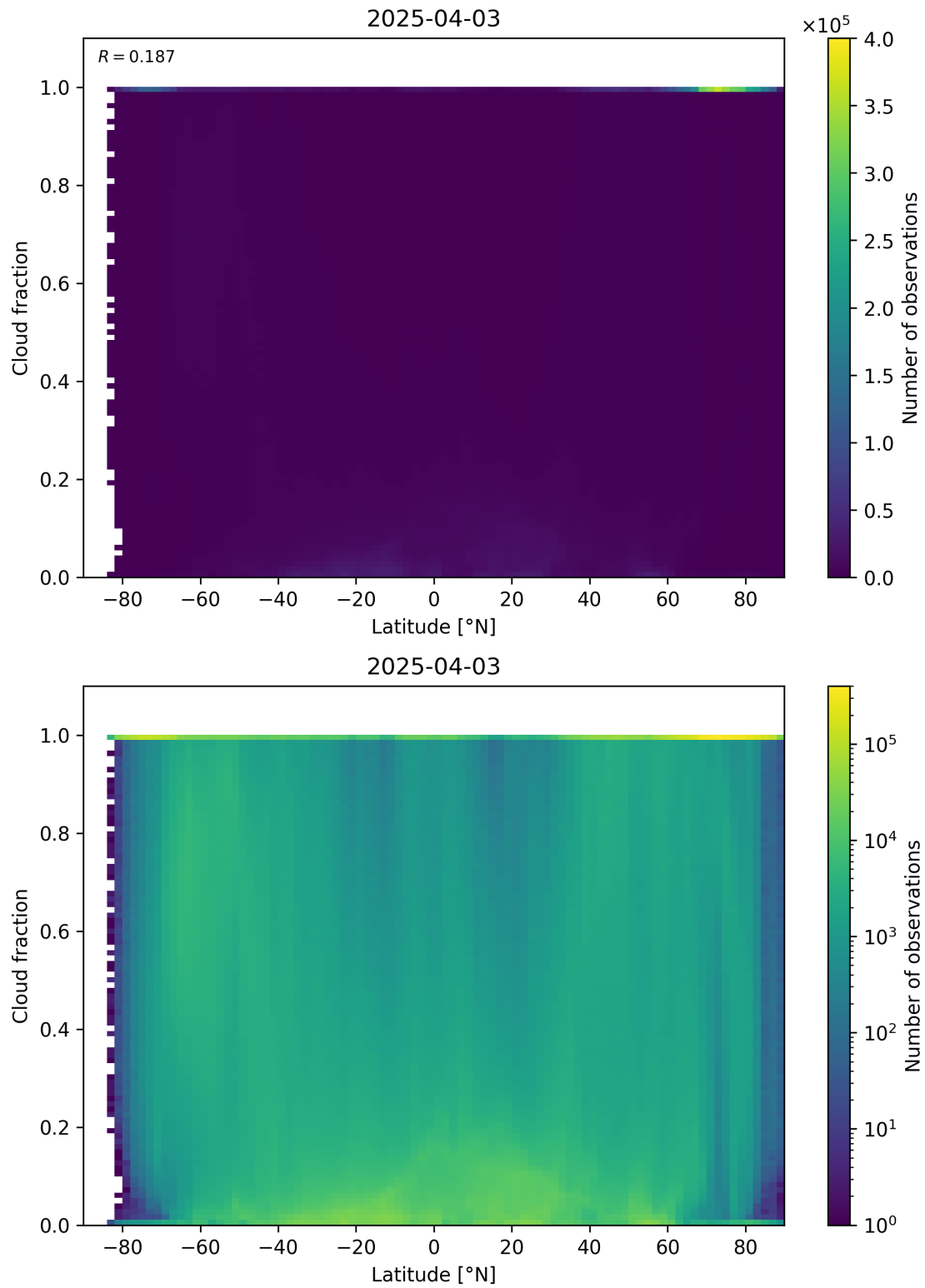
Figure 90: Scatter density plot of “Latitude” against “Cloud fraction” for 2025-04-03 to 2025-04-04.
