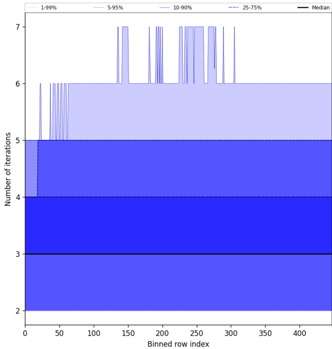
Figure 56: Along track statistics of “Number of iterations” for 2025-04-03 to 2025-04-04
