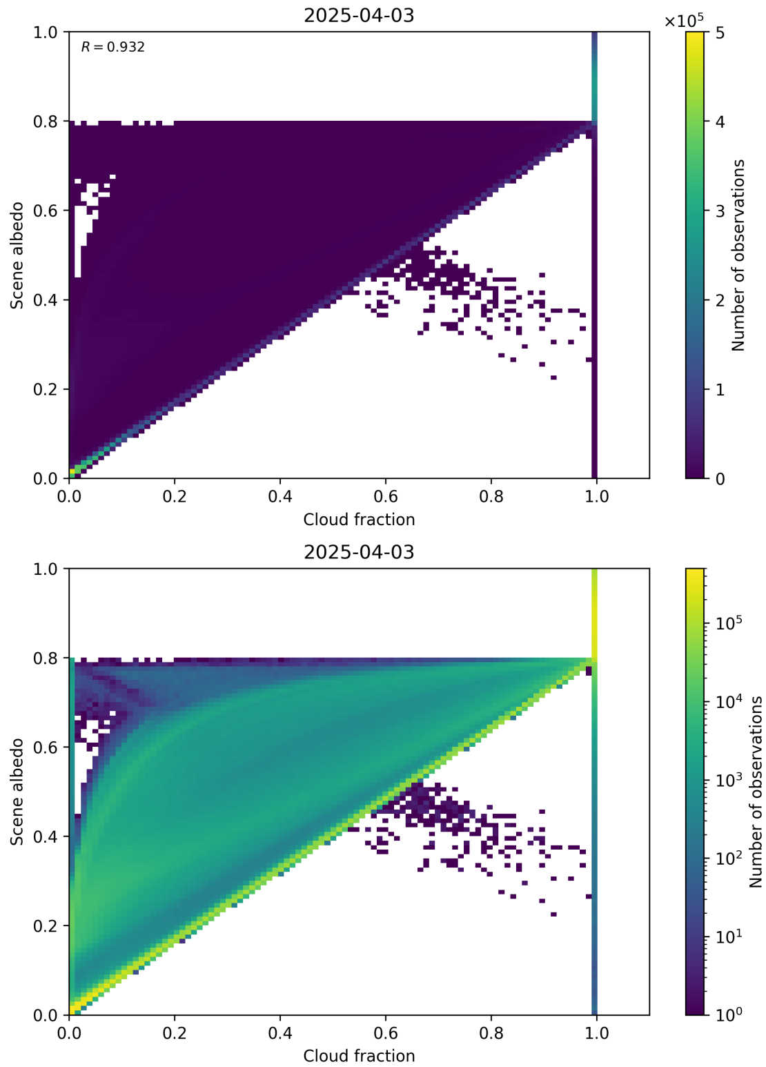
Figure 75: Scatter density plot of “Cloud fraction” against “Scene albedo” for 2025-04-03 to 2025-04-04.
