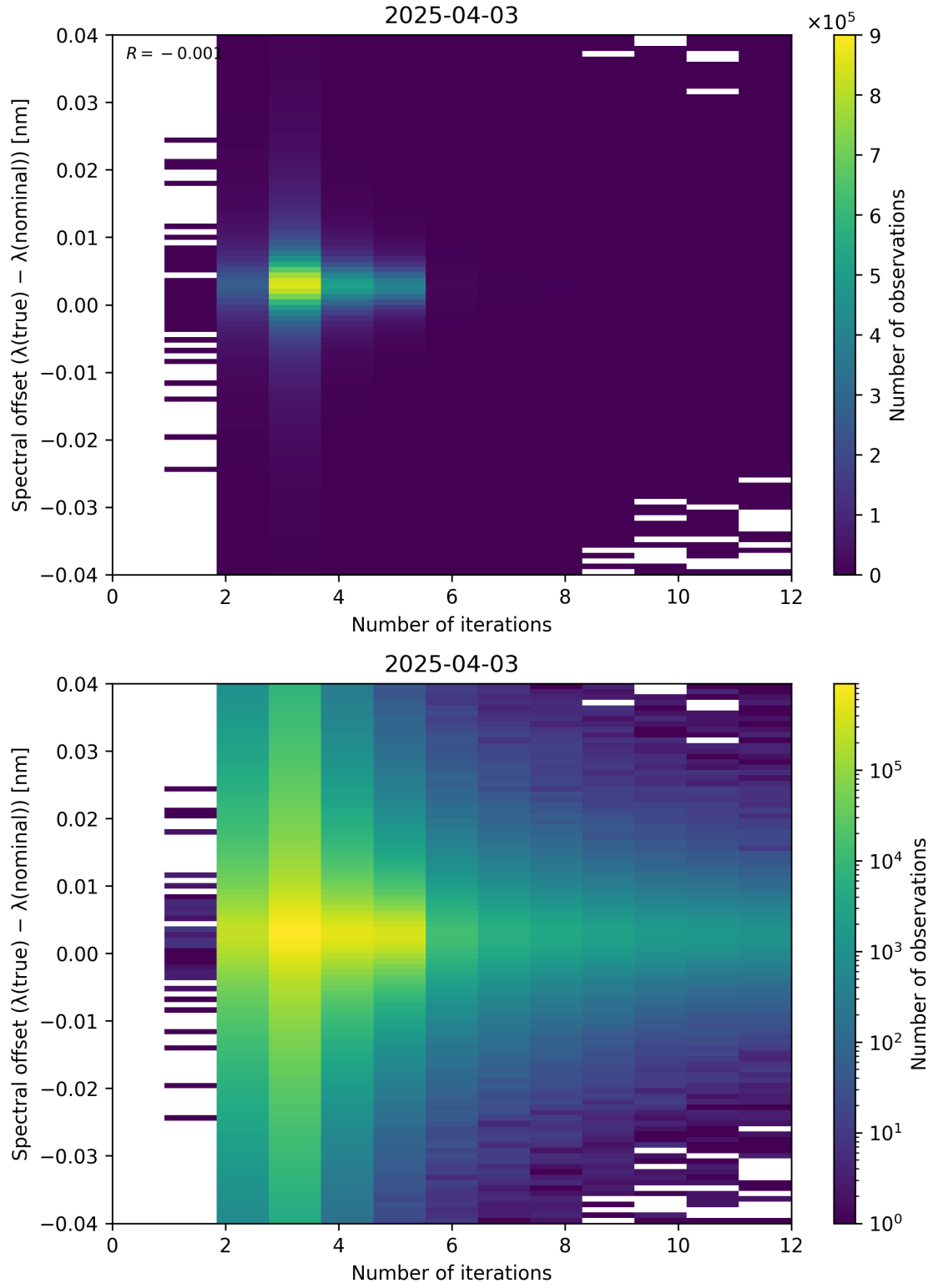
Figure 100: Scatter density plot of “Number of iterations” against “Spectral offset ( \lambda_{\text{true}} - \lambda_{\text{nominal}} )” for 2025-04-03 to 2025-04-04.
