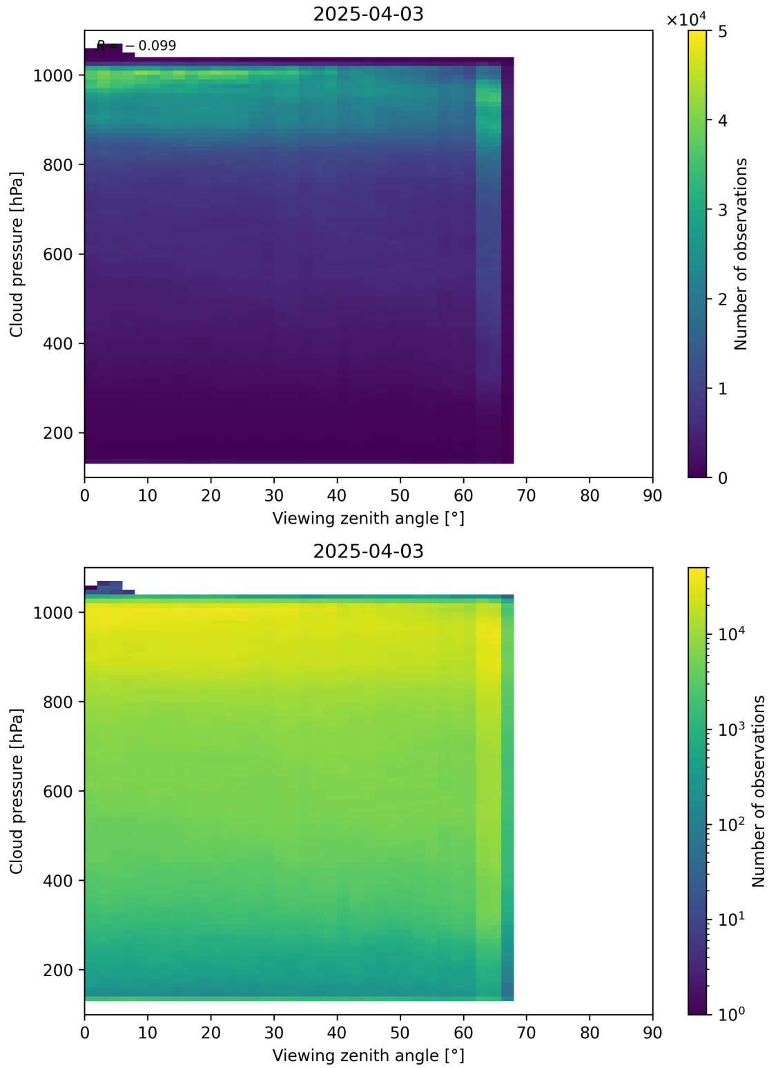
Figure 121: Scatter density plot of “Viewing zenith angle” against “Cloud pressure” for 2025-04-03 to 2025-04-04.
