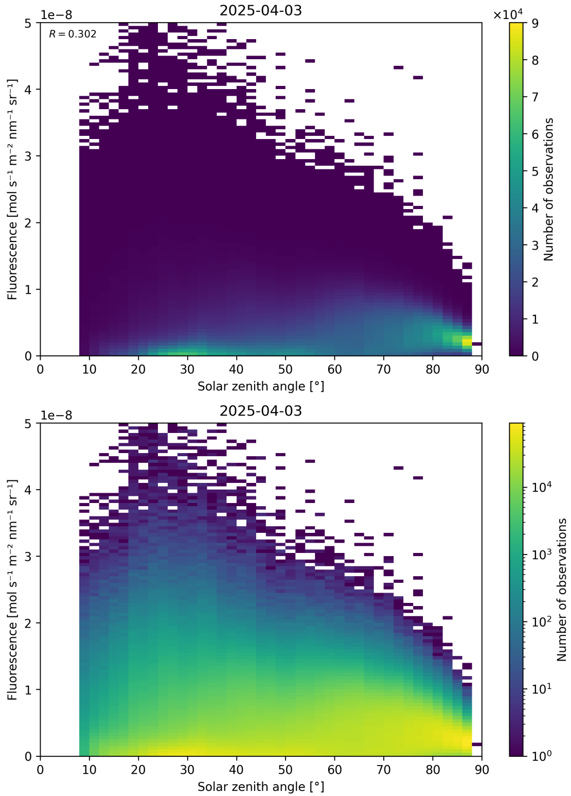
Figure 112: Scatter density plot of “Solar zenith angle” against “Fluorescence” for 2025-04-03 to 2025-04-04.
