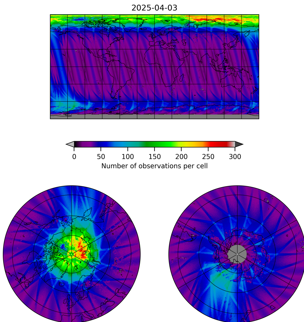
Figure 11: Map of the number of observations for 2025-04-03 to 2025-04-04
