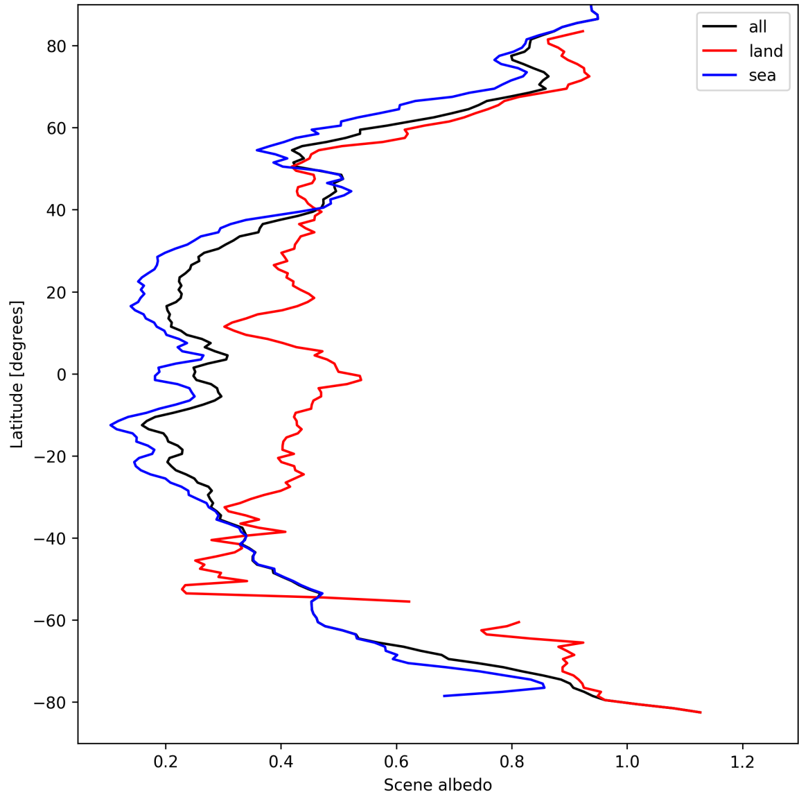
Figure 17: Zonal average of “Scene albedo” for 2025-04-03 to 2025-04-04.
