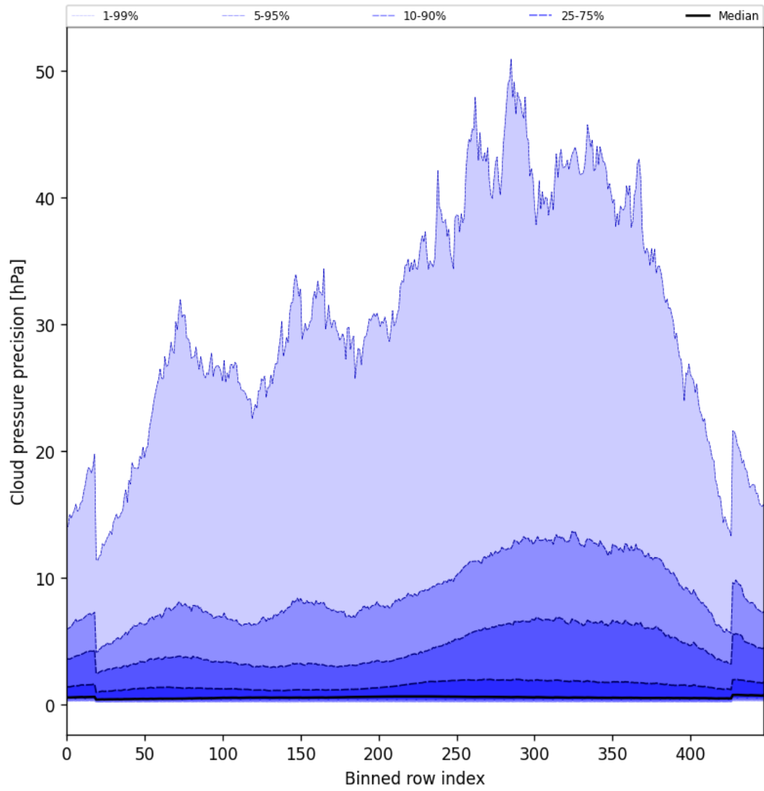
Figure 48: Along track statistics of “Cloud pressure precision” for 2025-04-03 to 2025-04-04
