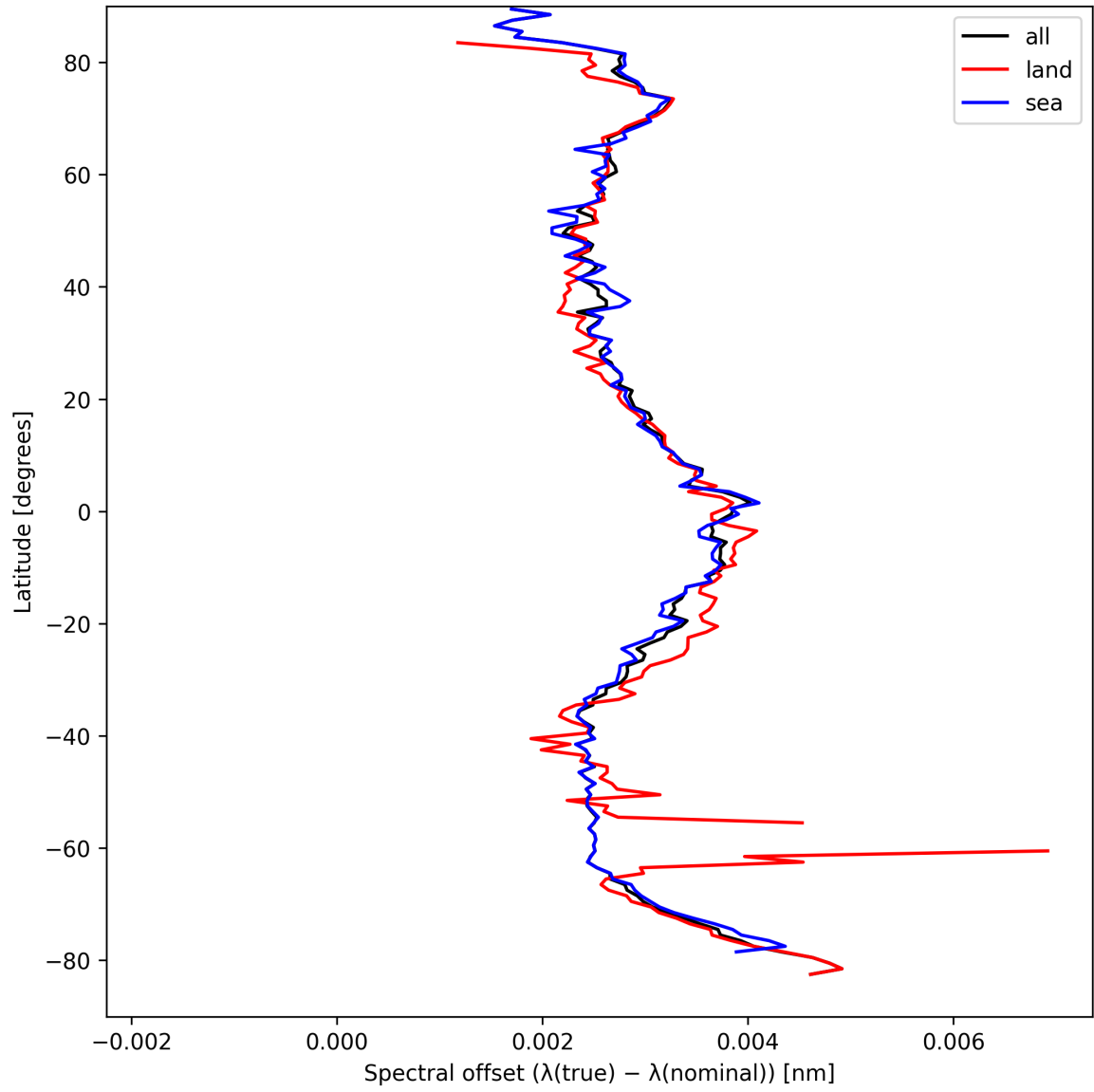
Figure 28: Zonal average of “Spectral offset ( \lambda_{\text{true}} - \lambda_{\text{nominal}} )” for 2025-04-03 to 2025-04-04.
