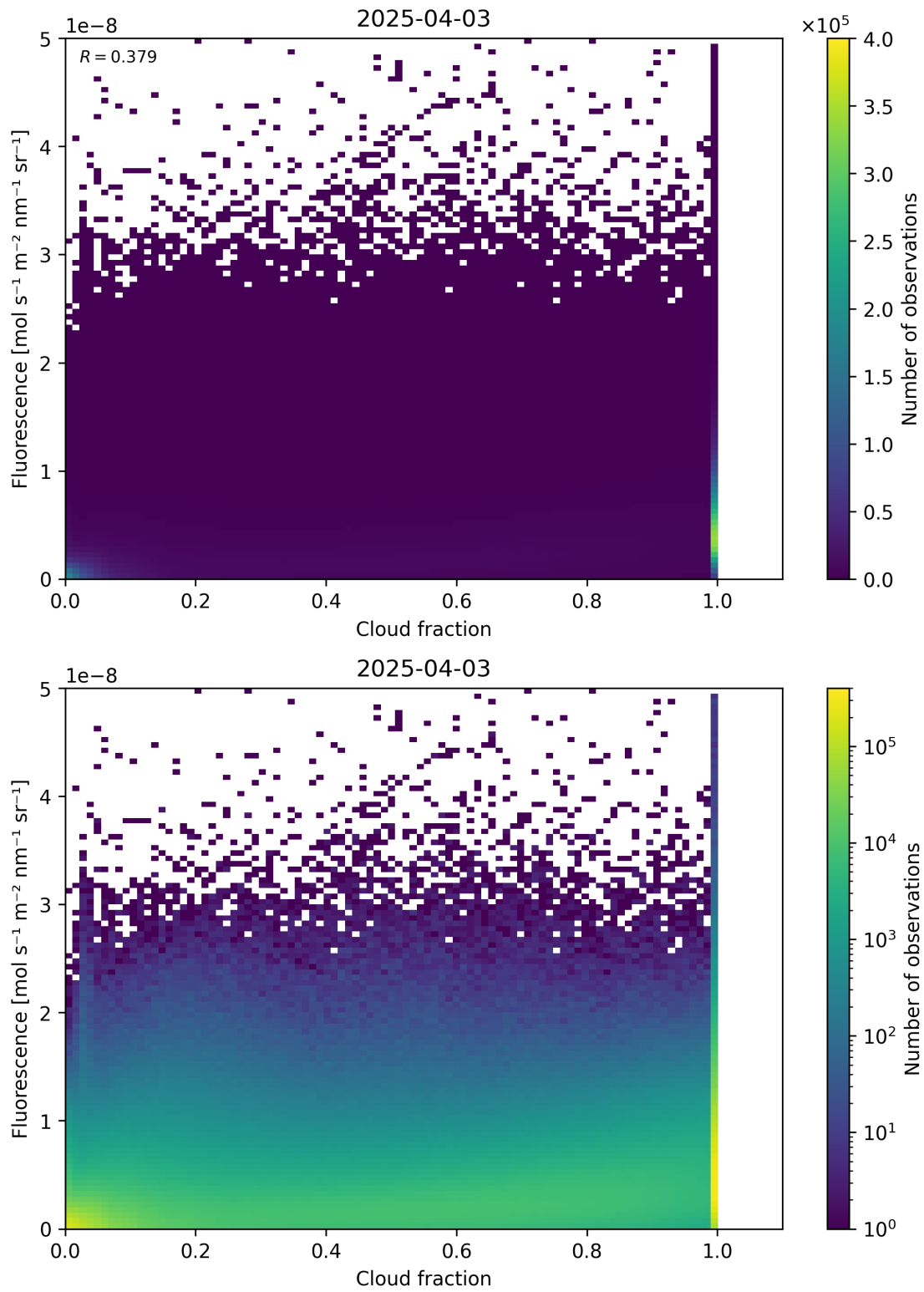
Figure 72: Scatter density plot of “Cloud fraction” against “Fluorescence” for 2025-04-03 to 2025-04-04.
