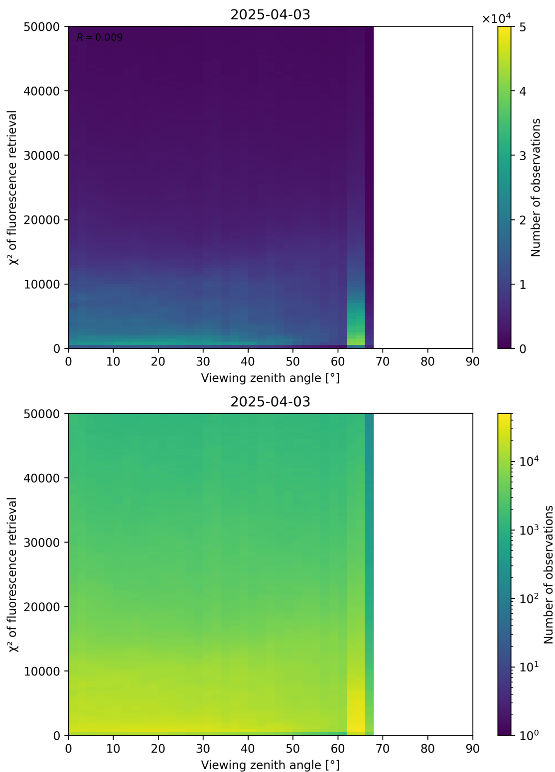
Figure 119: Scatter density plot of “Viewing zenith angle” against “ \chi^2 of fluorescence retrieval” for 2025-04-03 to 2025-04-04.
