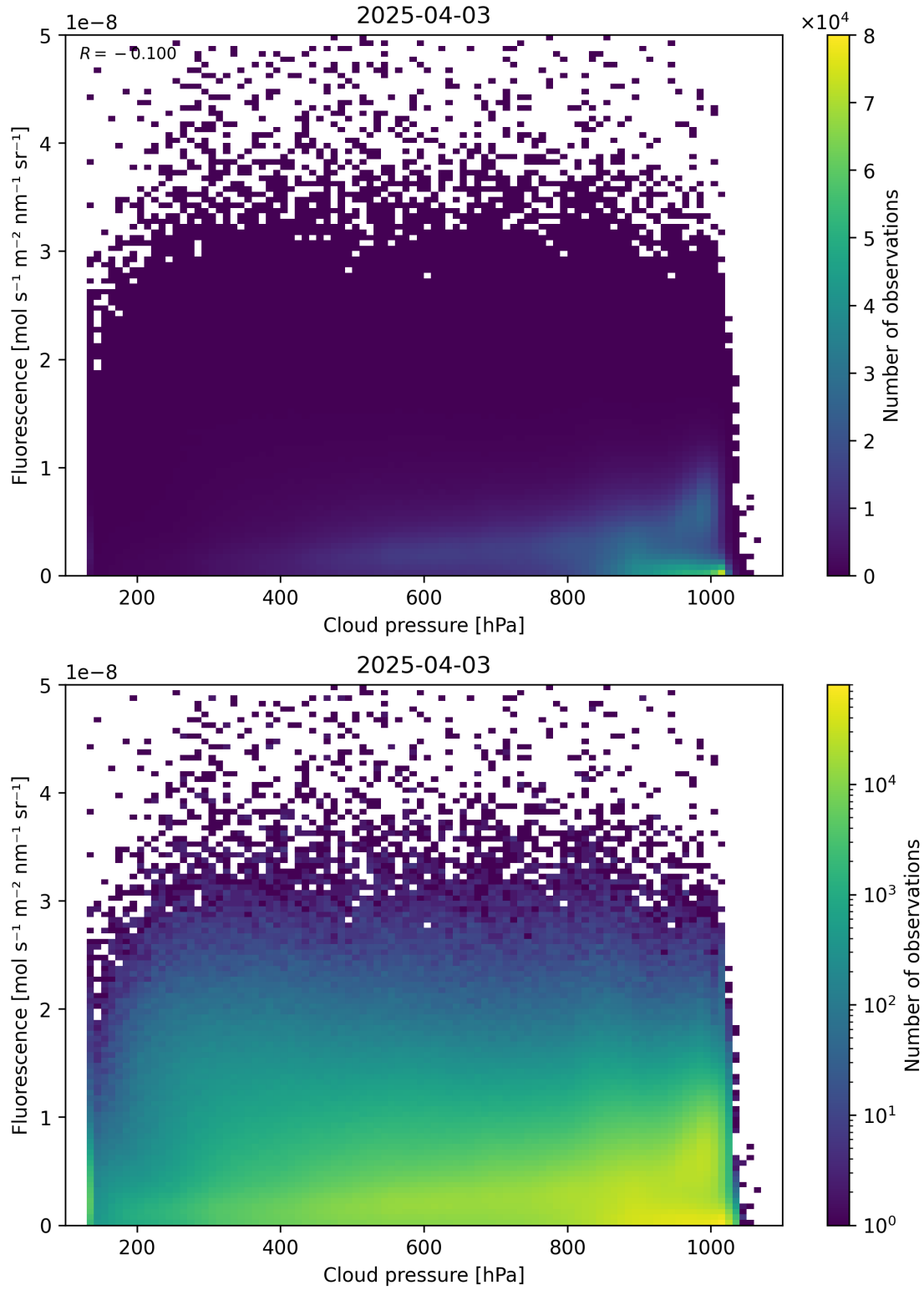
Figure 80: Scatter density plot of “Cloud pressure” against “Fluorescence” for 2025-04-03 to 2025-04-04.
