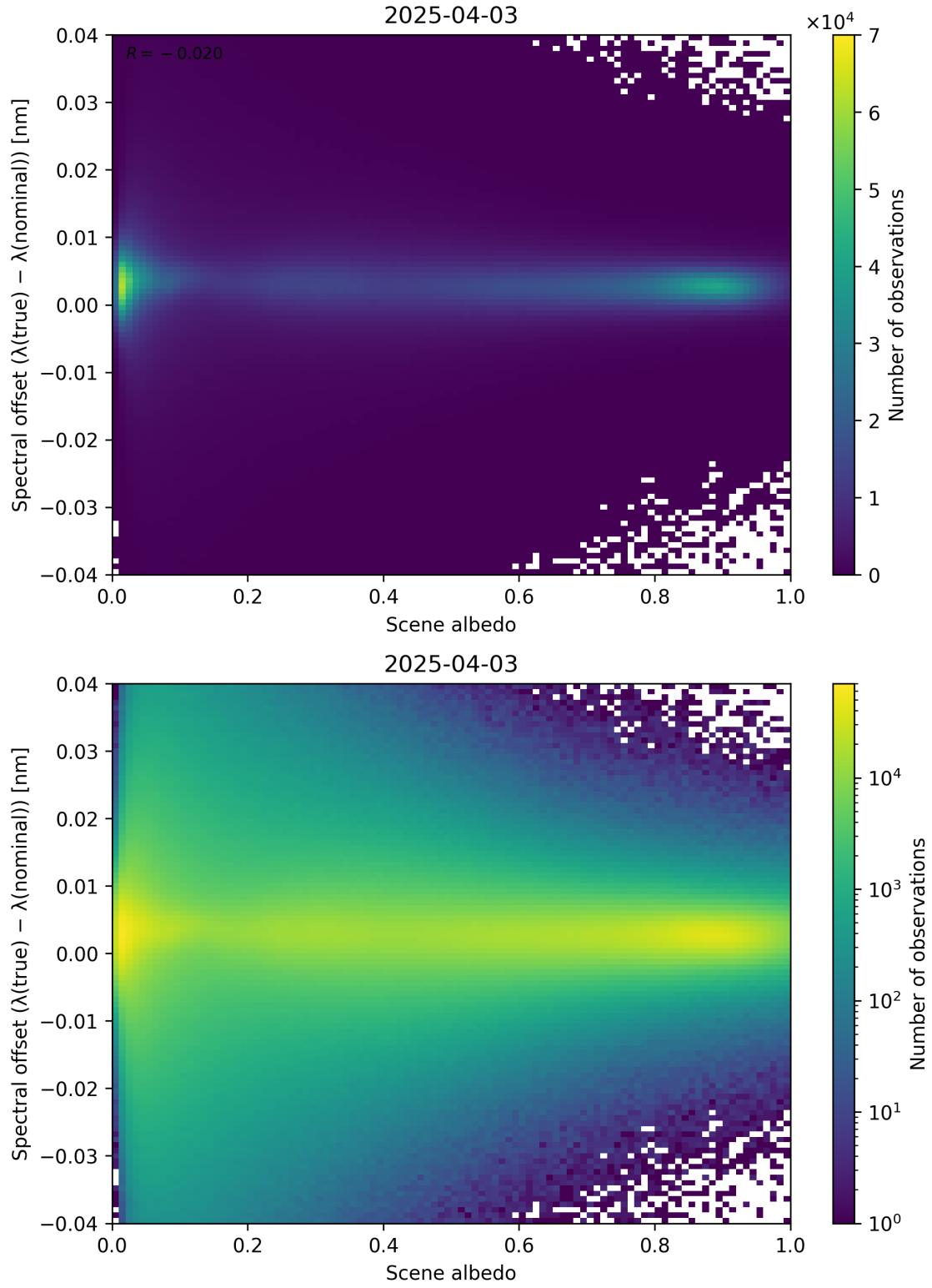
Figure 107: Scatter density plot of “Scene albedo” against “Spectral offset ( \lambda_{\text{true}} - \lambda_{\text{nominal}} )” for 2025-04-03 to 2025-04-04.
