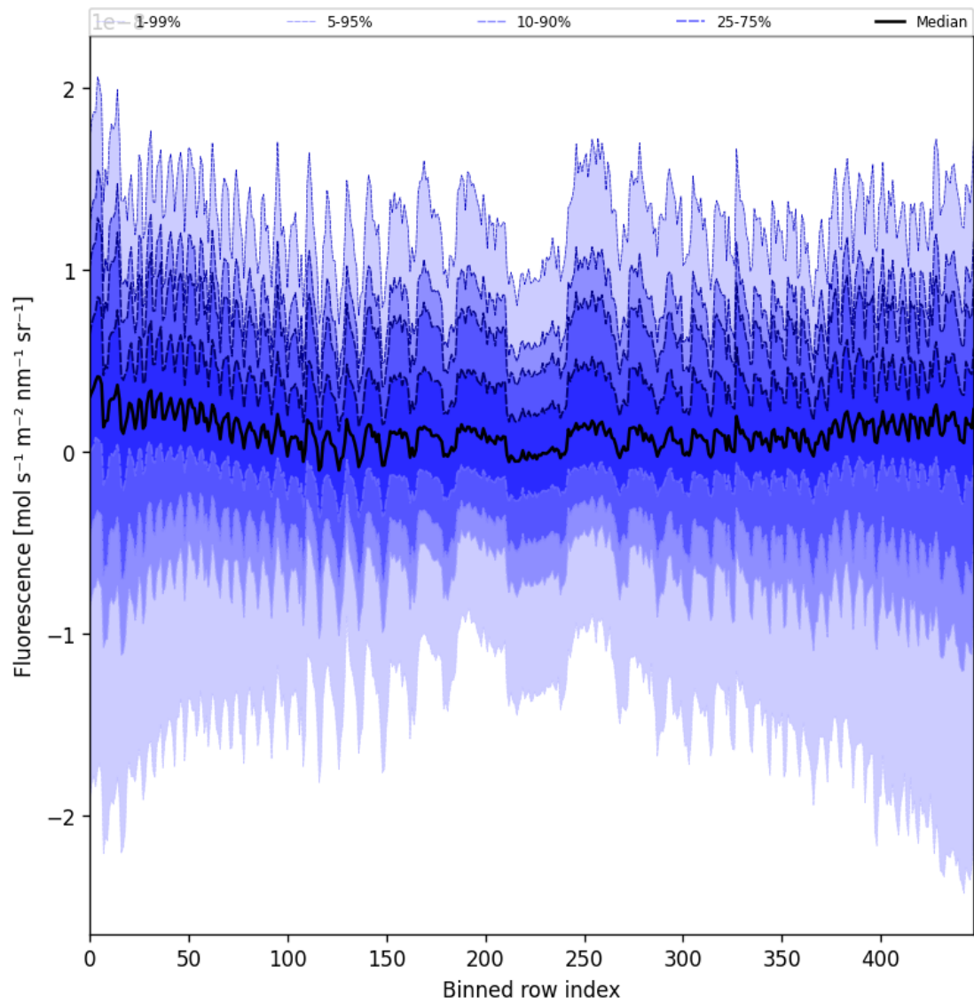
Figure 57: Along track statistics of “Fluorescence” for 2025-04-03 to 2025-04-04
