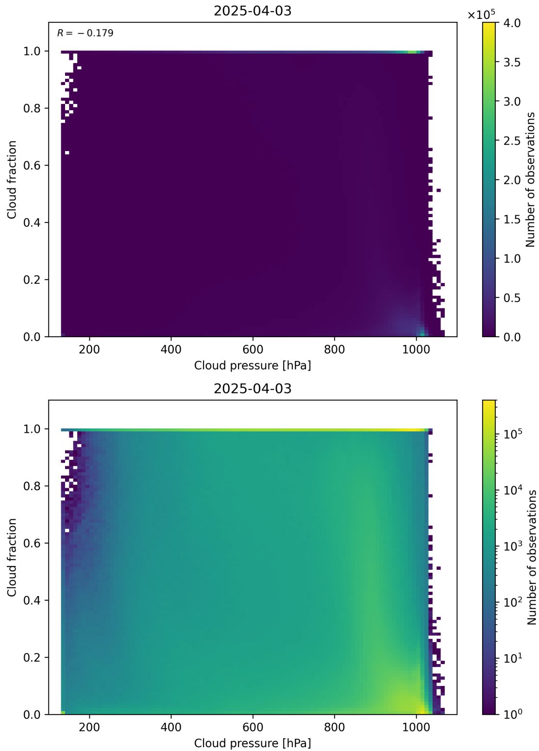
Figure 79: Scatter density plot of “Cloud pressure” against “Cloud fraction” for 2025-04-03 to 2025-04-04.
