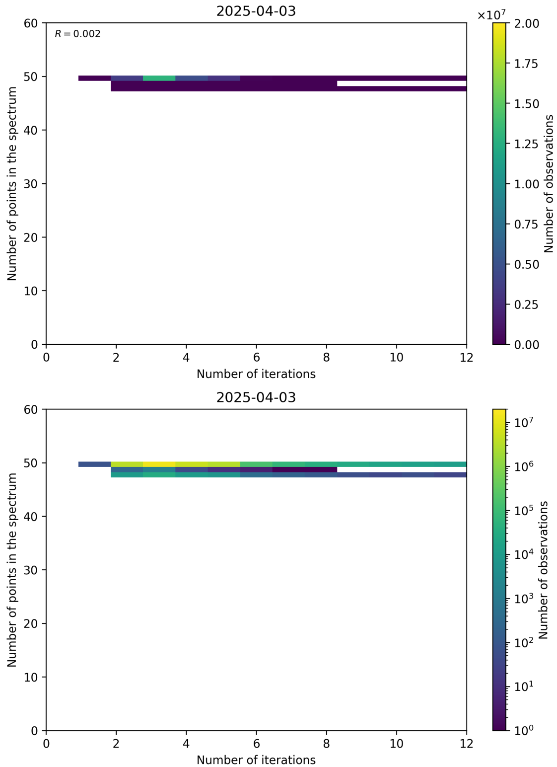
Figure 99: Scatter density plot of “Number of iterations” against “Number of points in the spectrum” for 2025-04-03 to 2025-04-04.
