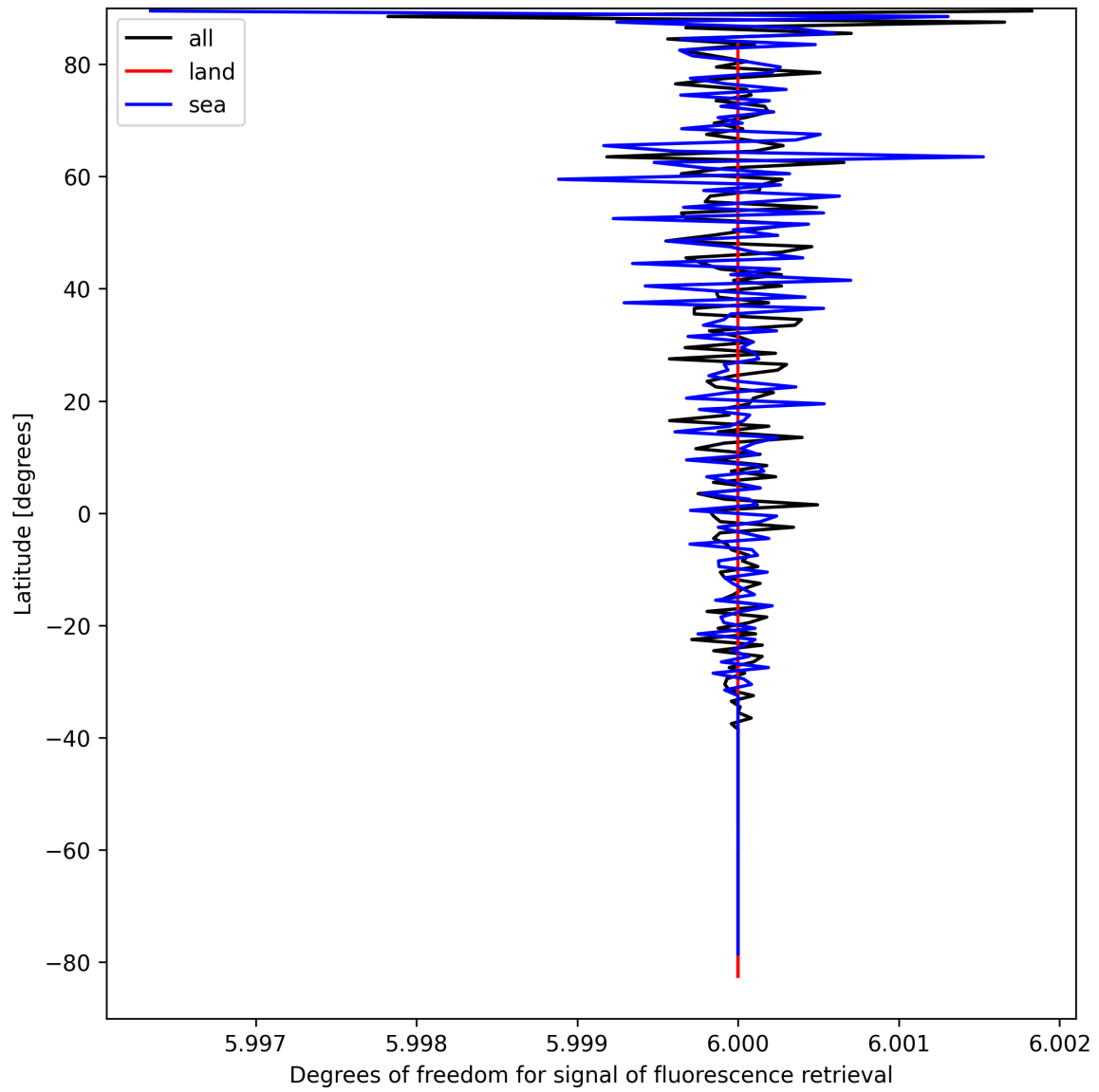
Figure 26: Zonal average of “Degrees of freedom for signal of fluorescence retrieval” for 2025-04-03 to 2025-04-04.
