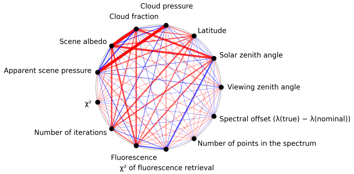
Figure 1: Map of correlation graph for 2025-04-03 to 2025-04-04.
