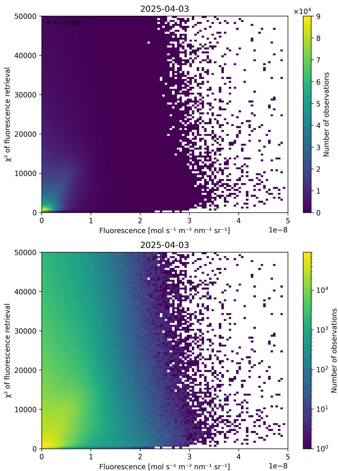
Figure 85: Scatter density plot of “Fluorescence” against “ \chi^2 of fluorescence retrieval” for 2025-04-03 to 2025-04-04.
