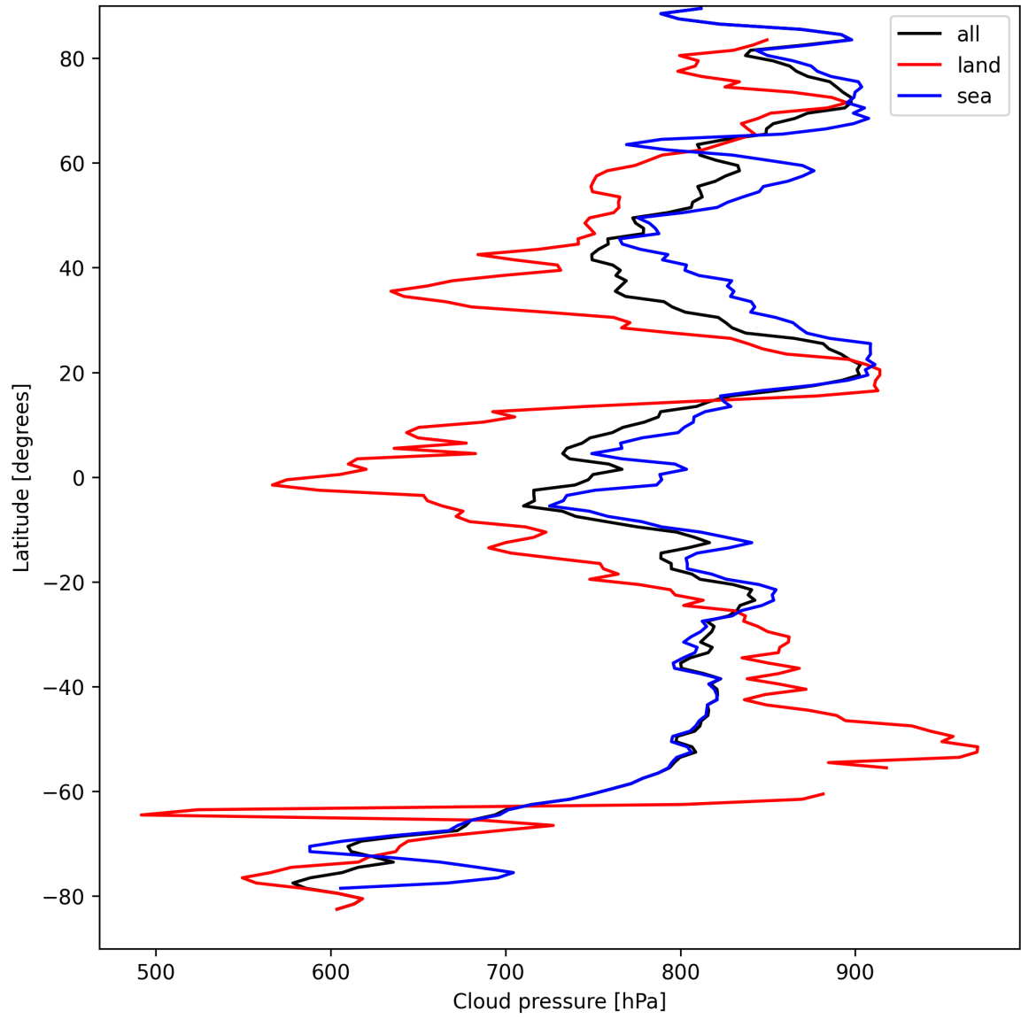
Figure 13: Zonal average of “Cloud pressure” for 2025-04-03 to 2025-04-04.
