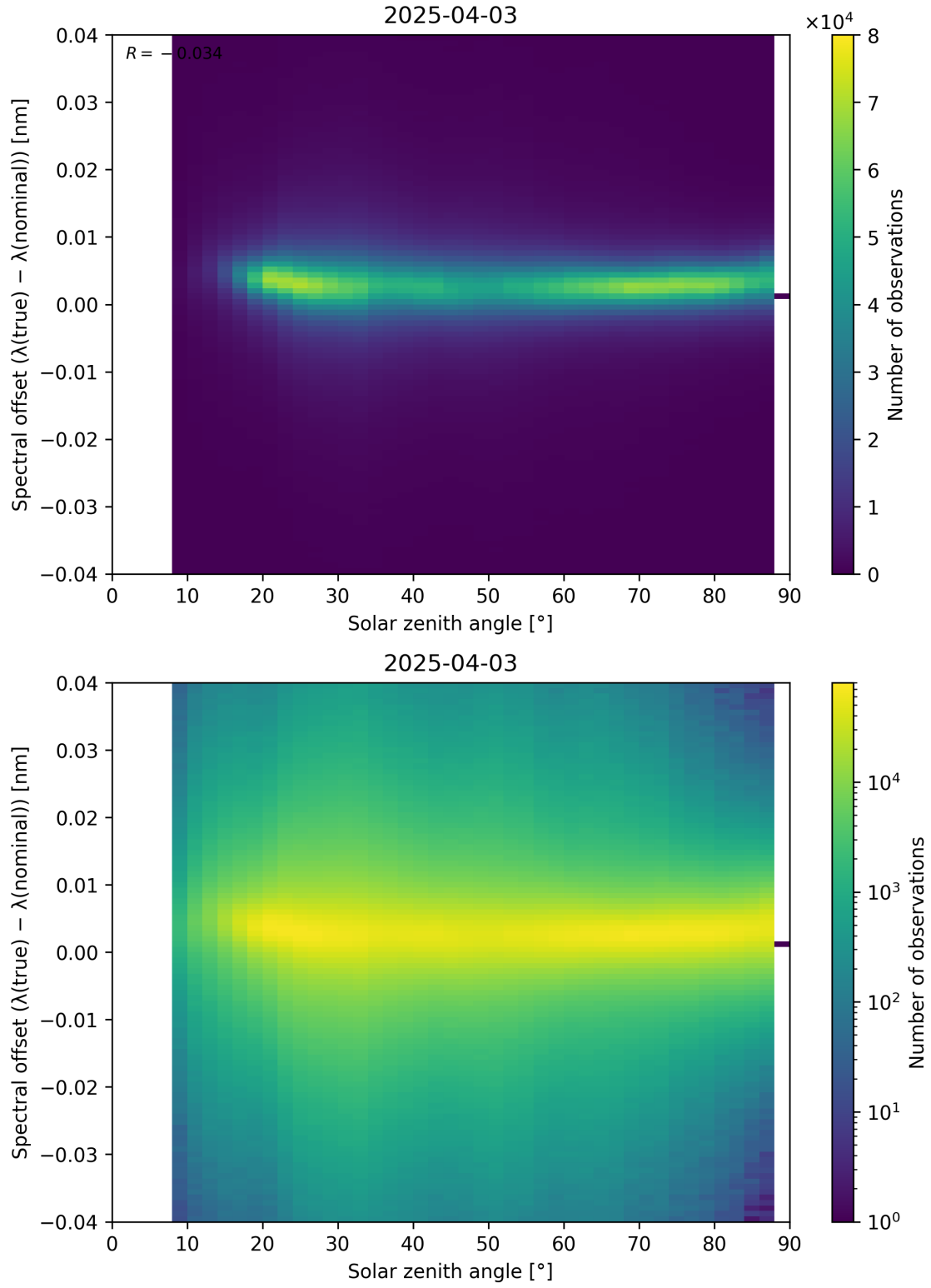
Figure 117: Scatter density plot of “Solar zenith angle” against “Spectral offset ( \lambda_{\text{true}} - \lambda_{\text{nominal}} )” for 2025-04-03 to 2025-04-04.
