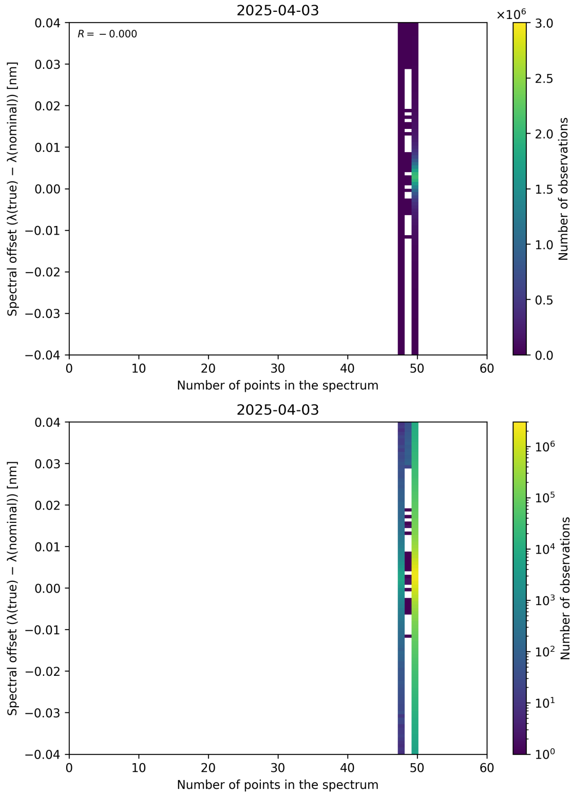
Figure 101: Scatter density plot of “Number of points in the spectrum” against “Spectral offset ( \lambda_{\text{true}} - \lambda_{\text{nominal}} )” for 2025-04-03 to 2025-04-04.
