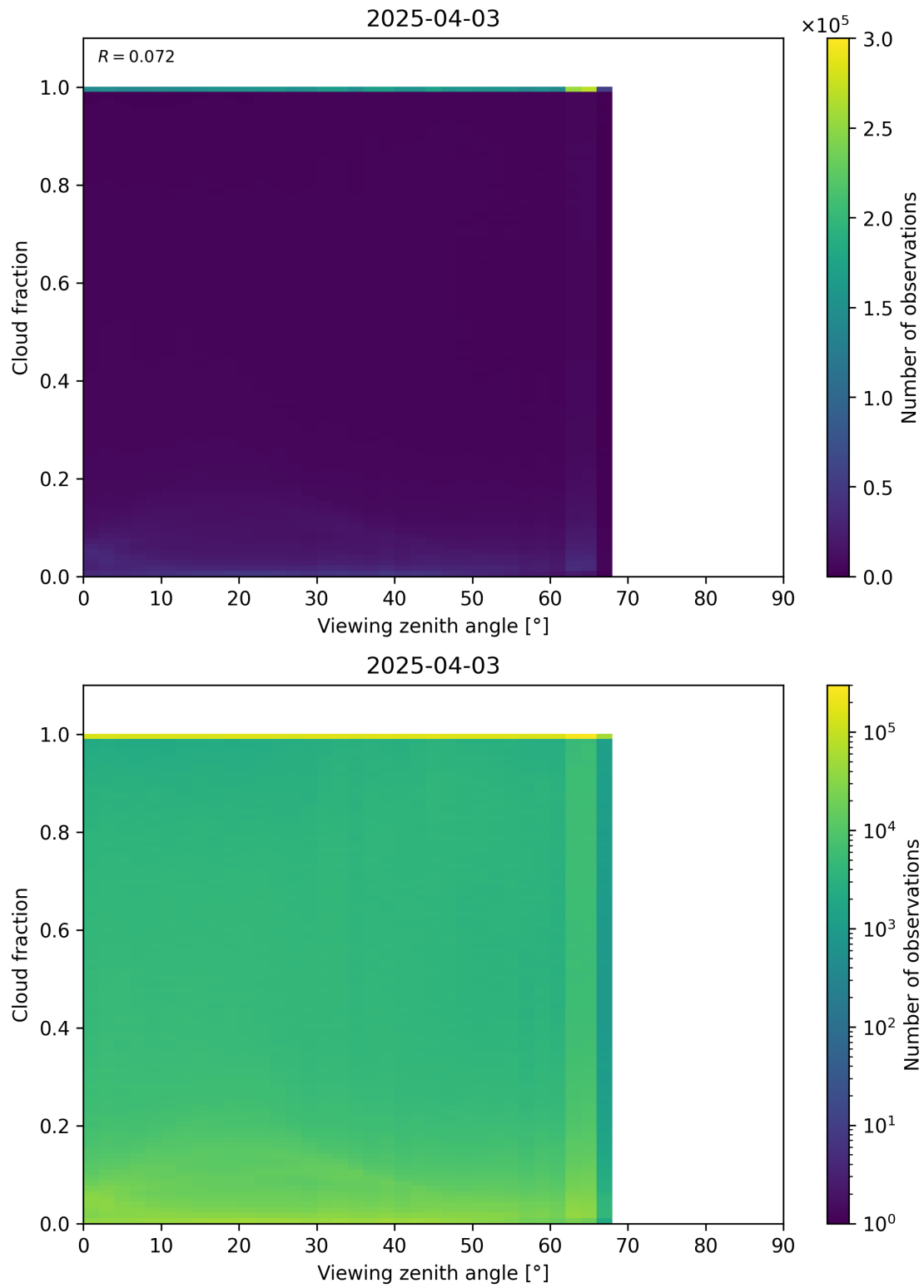
Figure 120: Scatter density plot of “Viewing zenith angle” against “Cloud fraction” for 2025-04-03 to 2025-04-04.
