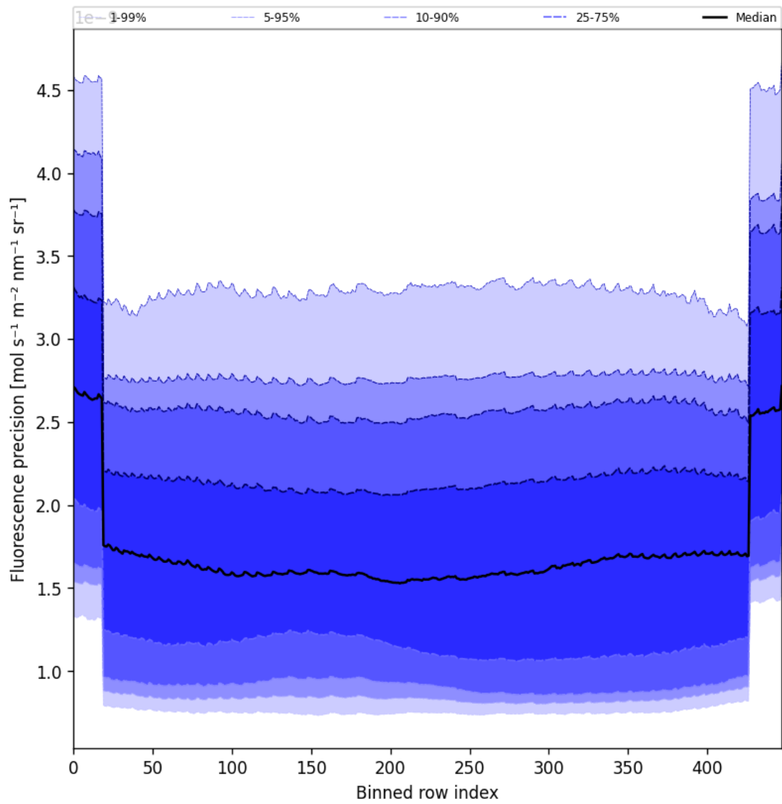
Figure 58: Along track statistics of “Fluorescence precision” for 2025-04-03 to 2025-04-04
