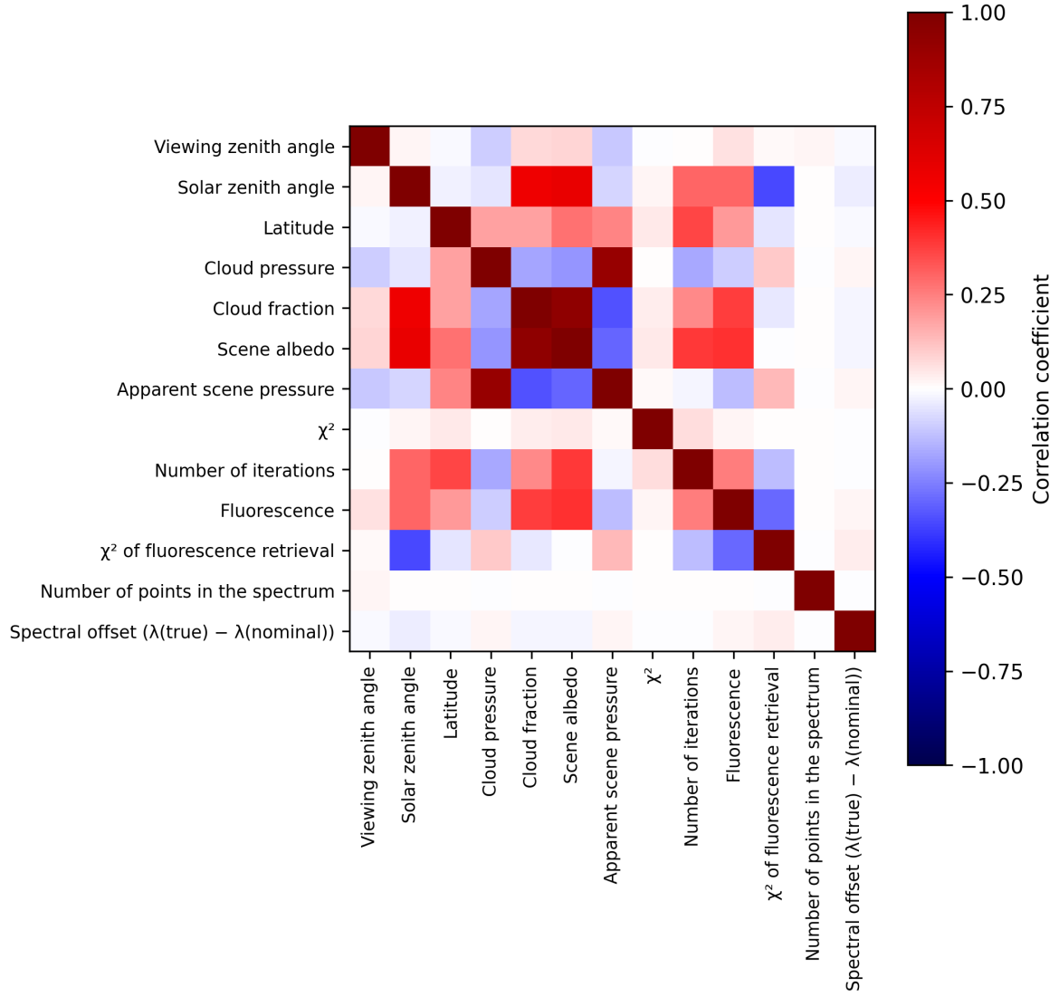
Figure 2: Map of correlation matrix for 2025-04-03 to 2025-04-04.
