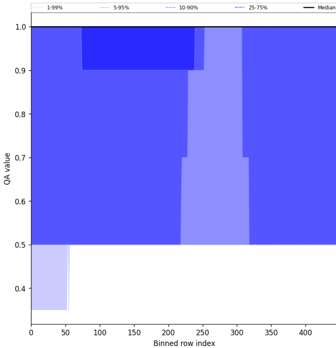
Figure 46: Along track statistics of “QA value” for 2025-04-03 to 2025-04-04
