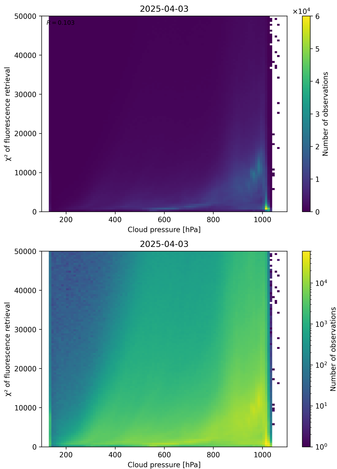
Figure 78: Scatter density plot of “Cloud pressure” against “ \chi^2 of fluorescence retrieval” for 2025-04-03 to 2025-04-04.
