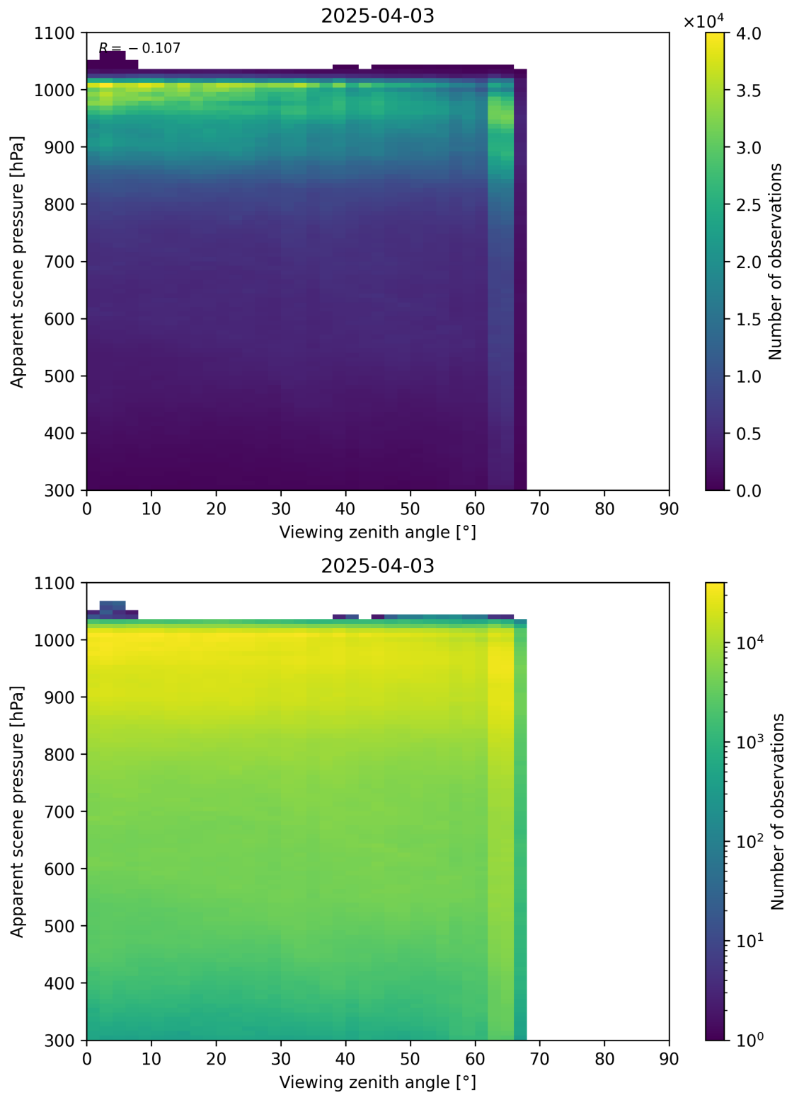
Figure 118: Scatter density plot of “Viewing zenith angle” against “Apparent scene pressure” for 2025-04-03 to 2025-04-04.
