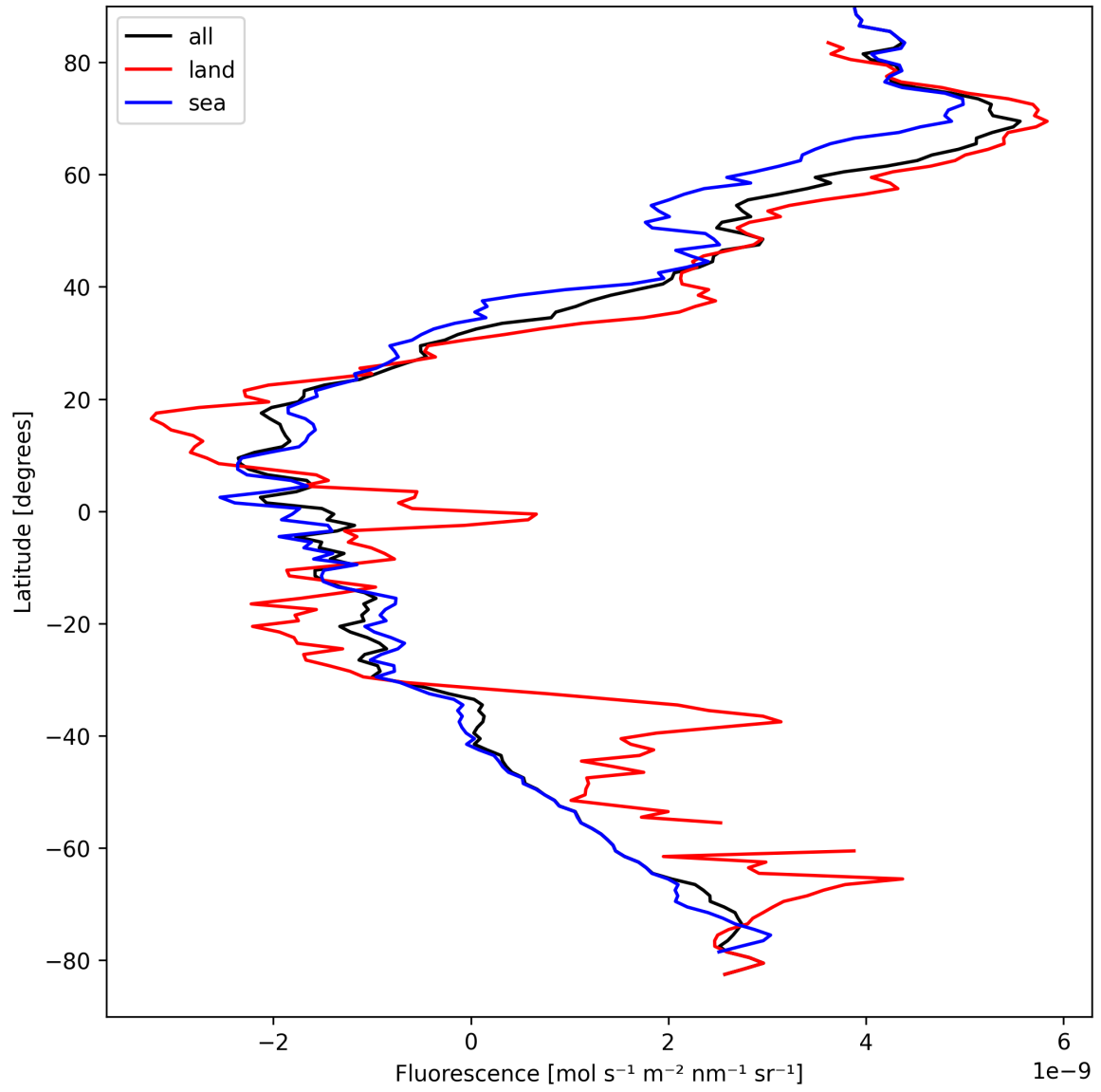
Figure 23: Zonal average of “Fluorescence” for 2025-04-03 to 2025-04-04.
