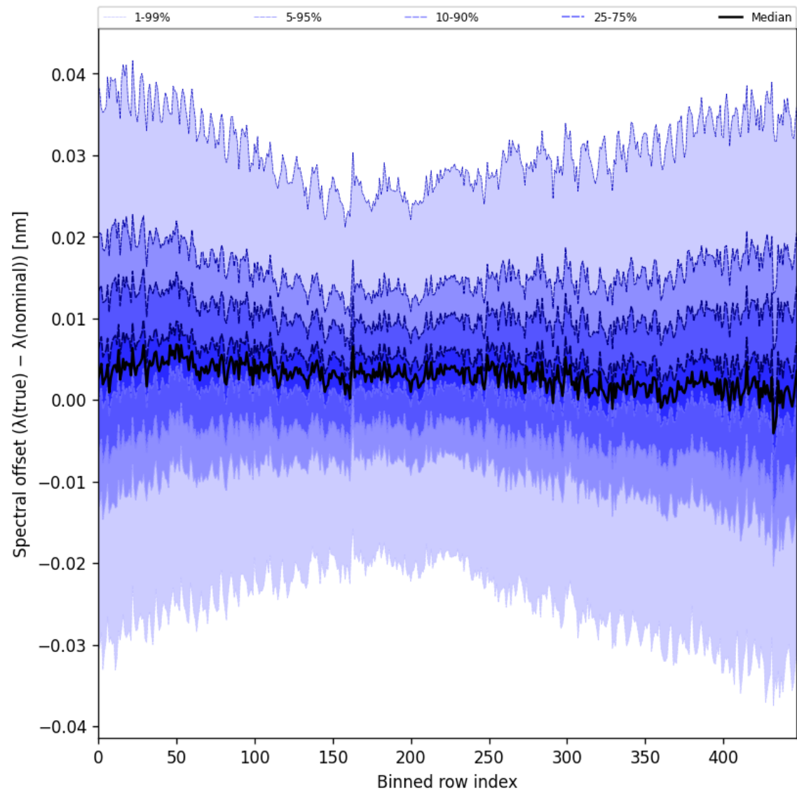
Figure 62: Along track statistics of “Spectral offset ( \lambda_{\text{true}} - \lambda_{\text{nominal}} )” for 2025-04-03 to 2025-04-04
