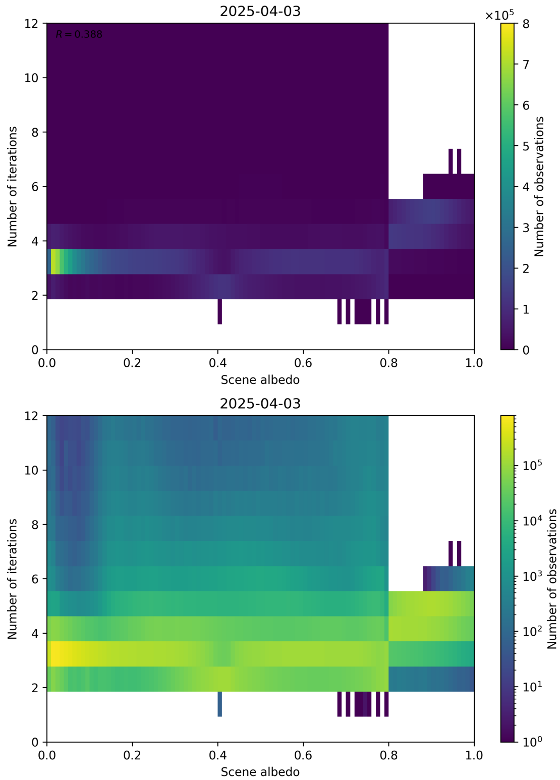
Figure 105: Scatter density plot of “Scene albedo” against “Number of iterations” for 2025-04-03 to 2025-04-04.
