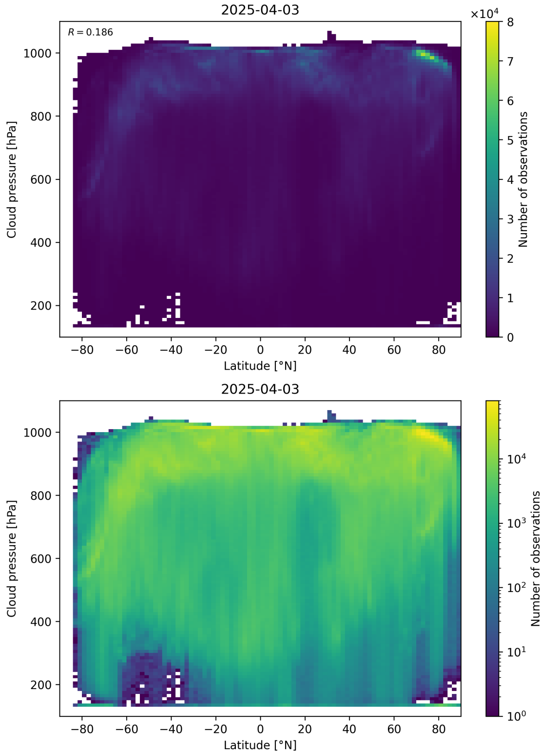
Figure 91: Scatter density plot of “Latitude” against “Cloud pressure” for 2025-04-03 to 2025-04-04.
