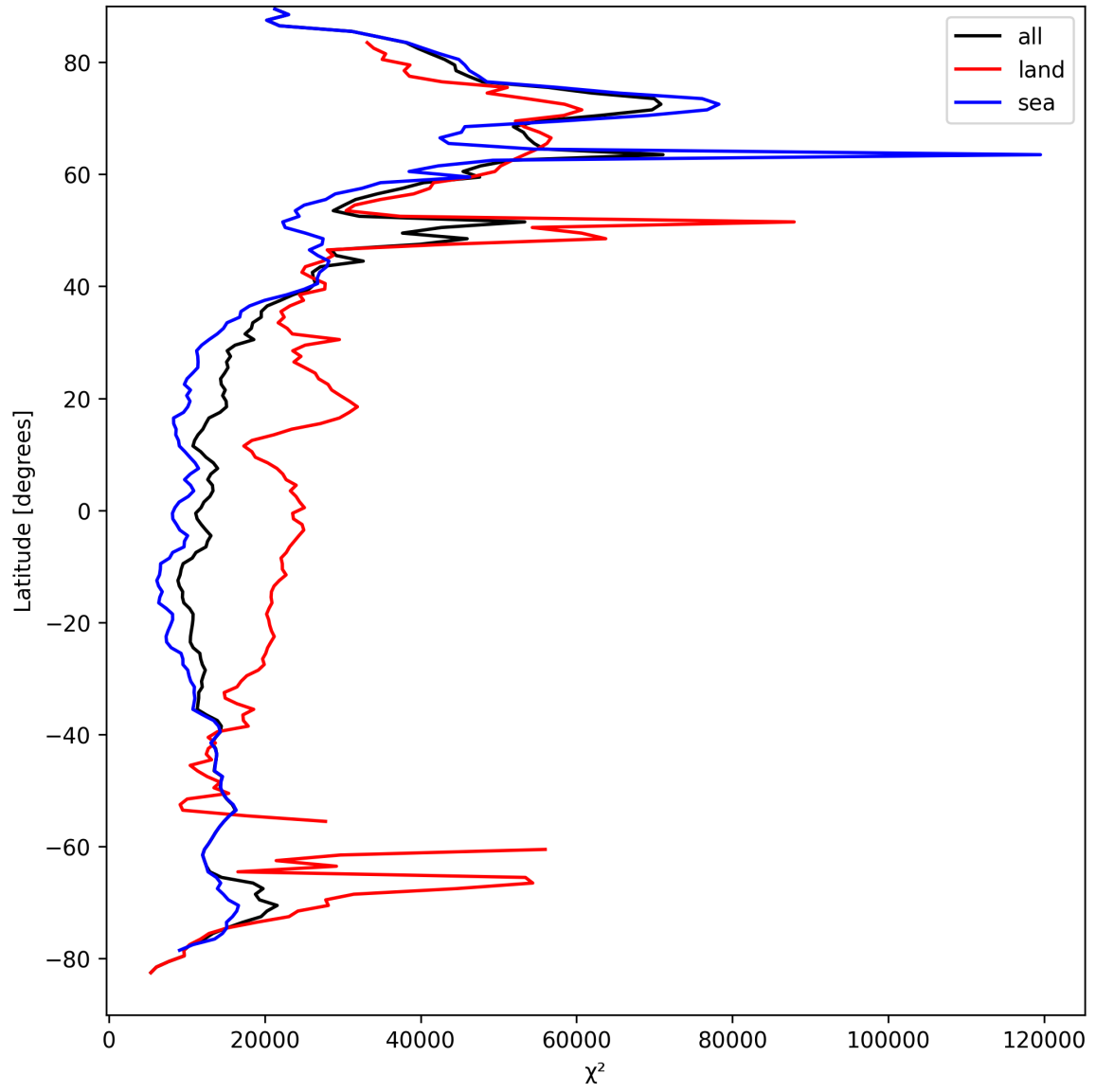
Figure 21: Zonal average of “ \chi^2 ” for 2025-04-03 to 2025-04-04.
