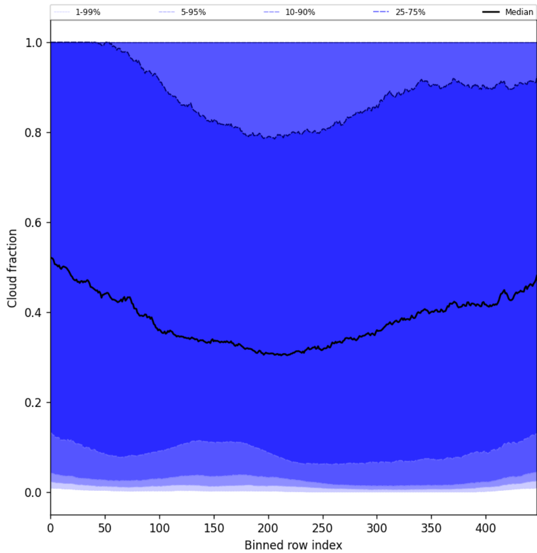
Figure 49: Along track statistics of “Cloud fraction” for 2025-04-03 to 2025-04-04
