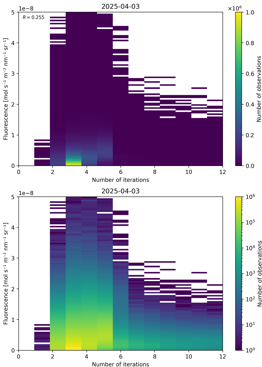
Figure 98: Scatter density plot of “Number of iterations” against “Fluorescence” for 2025-04-03 to 2025-04-04.
