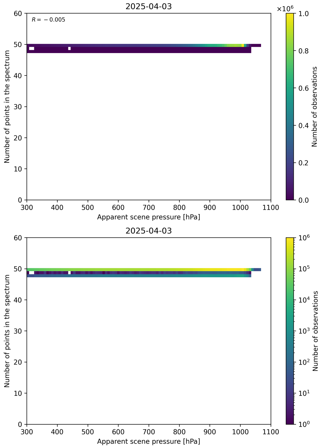
Figure 66: Scatter density plot of “Apparent scene pressure” against “Number of points in the spectrum” for 2025-04-03 to 2025-04-04.
