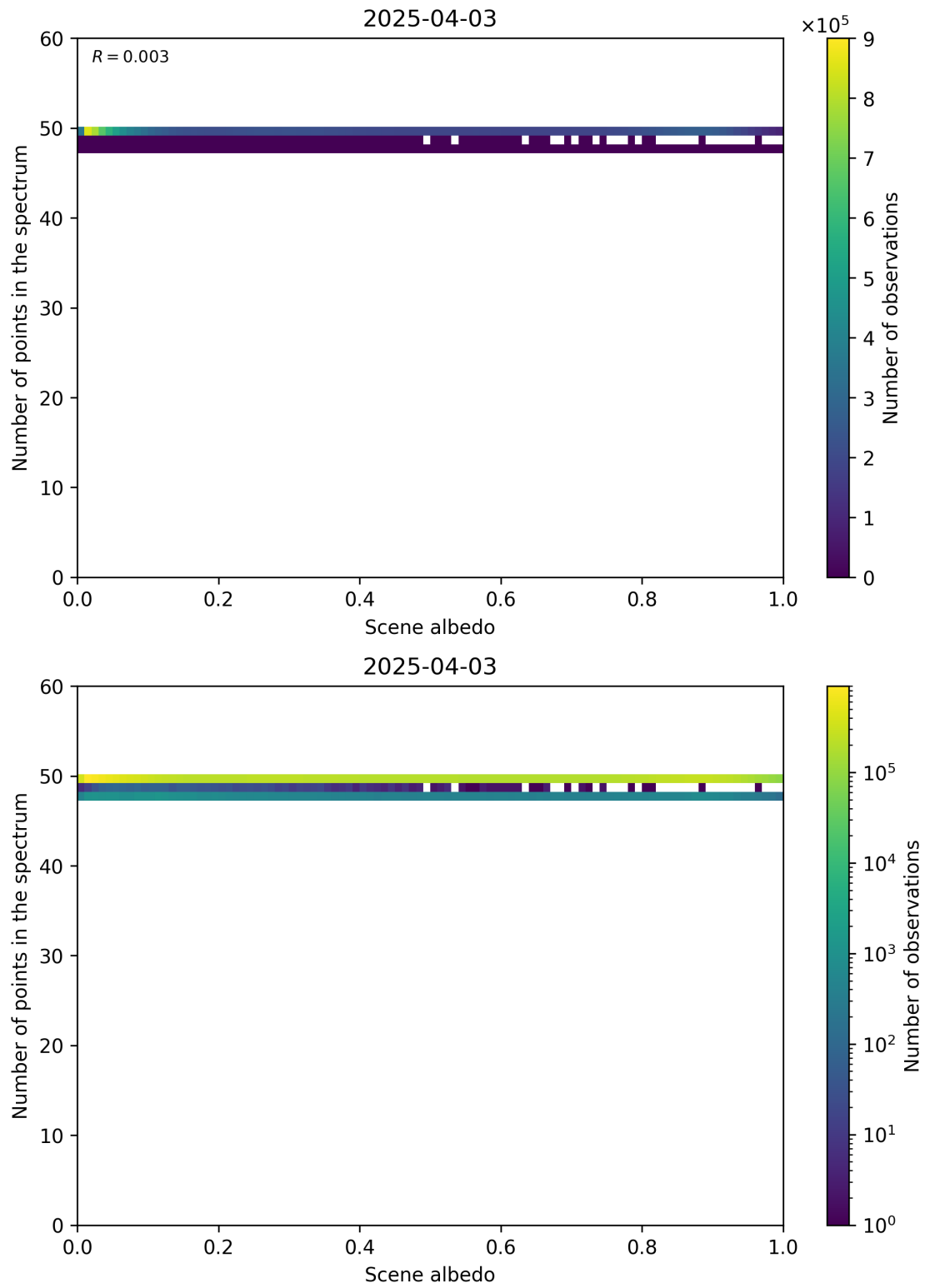
Figure 106: Scatter density plot of “Scene albedo” against “Number of points in the spectrum” for 2025-04-03 to 2025-04-04.
