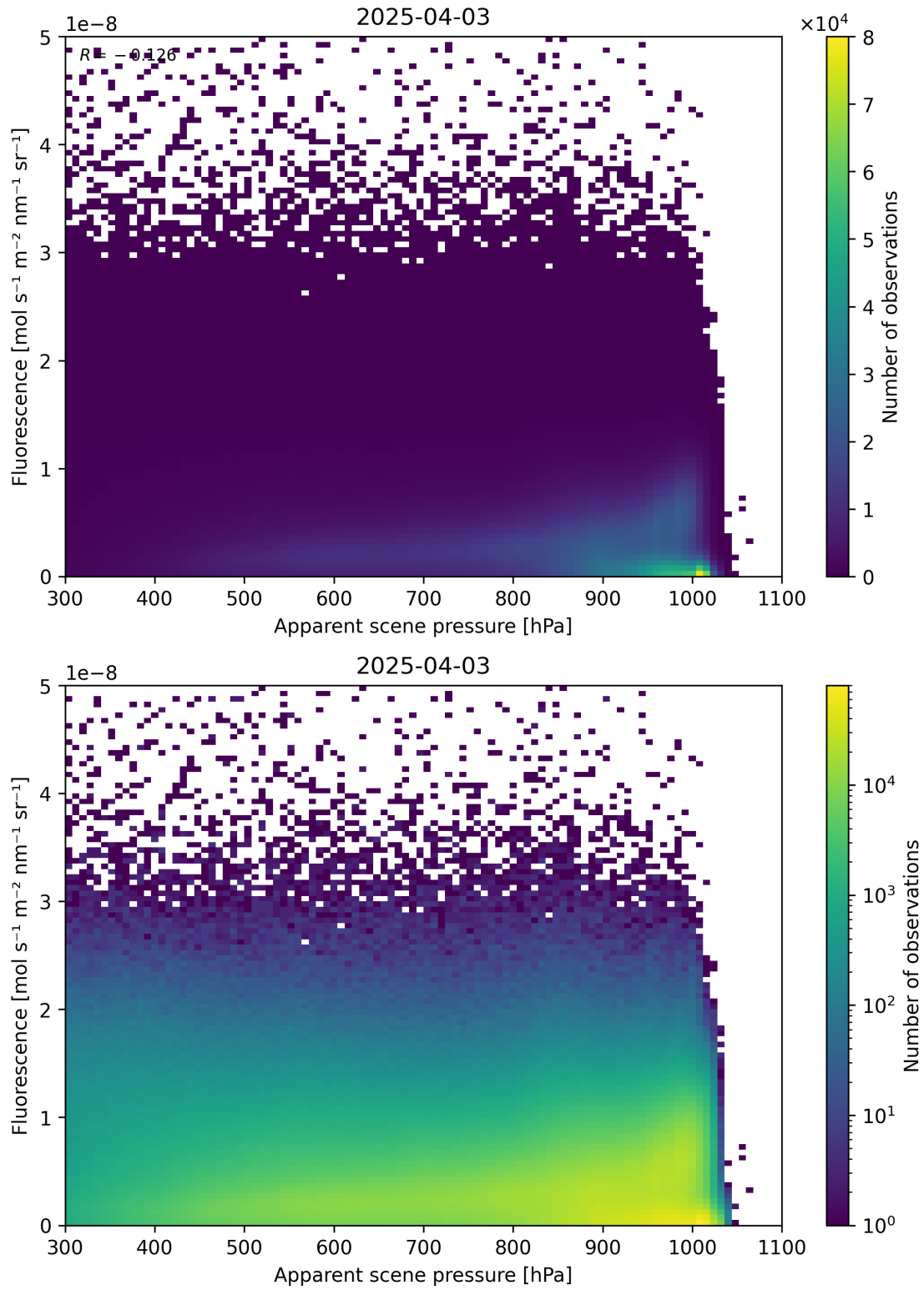
Figure 64: Scatter density plot of “Apparent scene pressure” against “Fluorescence” for 2025-04-03 to 2025-04-04.
