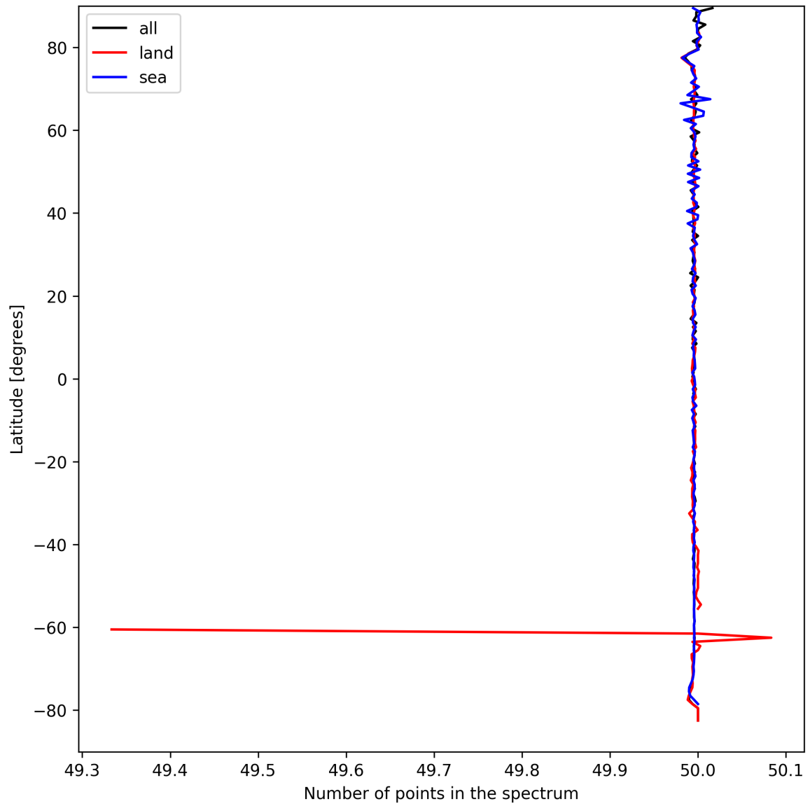
Figure 27: Zonal average of “Number of points in the spectrum” for 2025-04-03 to 2025-04-04.
