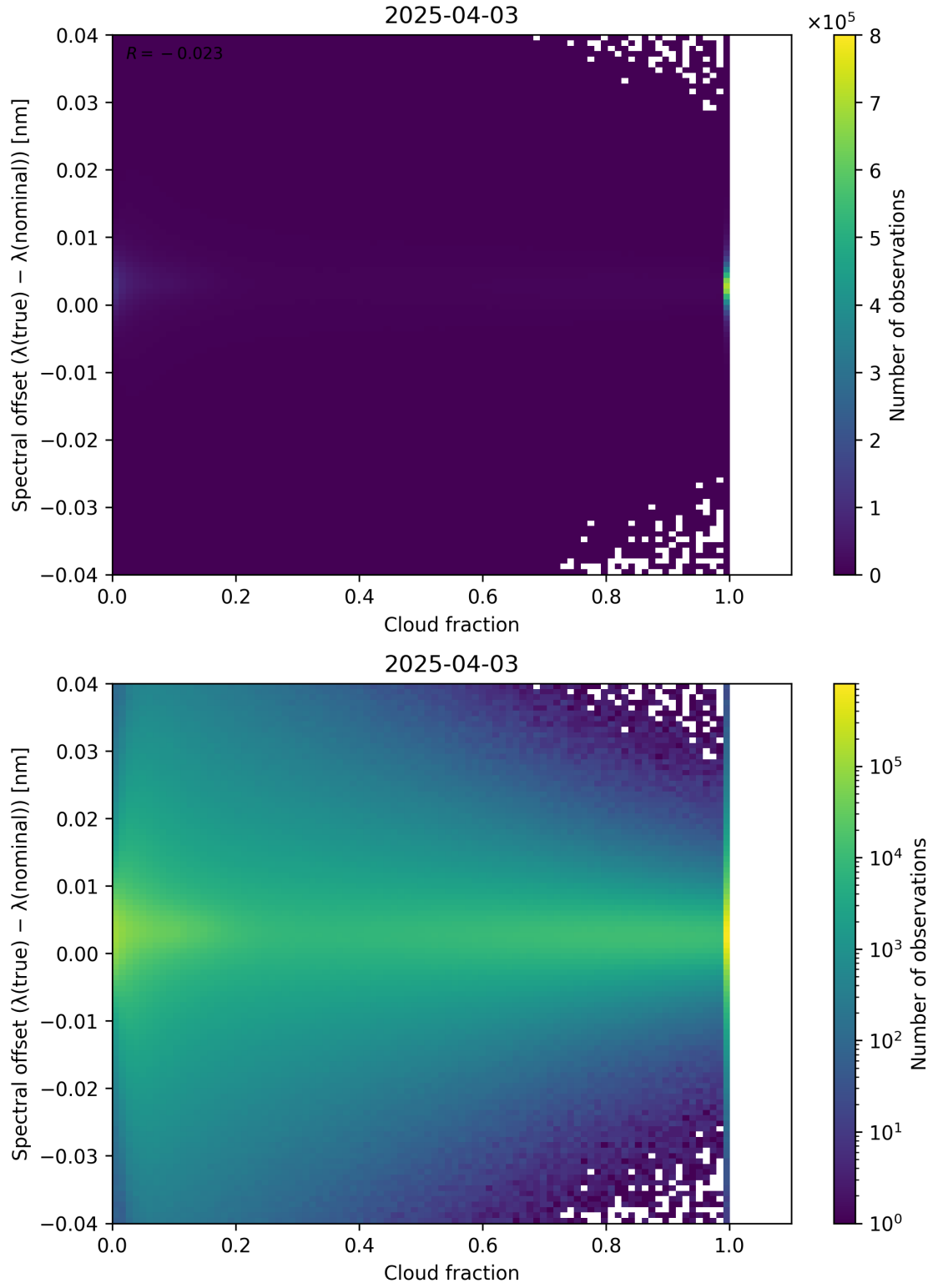
Figure 76: Scatter density plot of “Cloud fraction” against “Spectral offset ( \lambda_{\text{true}} - \lambda_{\text{nominal}} )” for 2025-04-03 to 2025-04-04.
