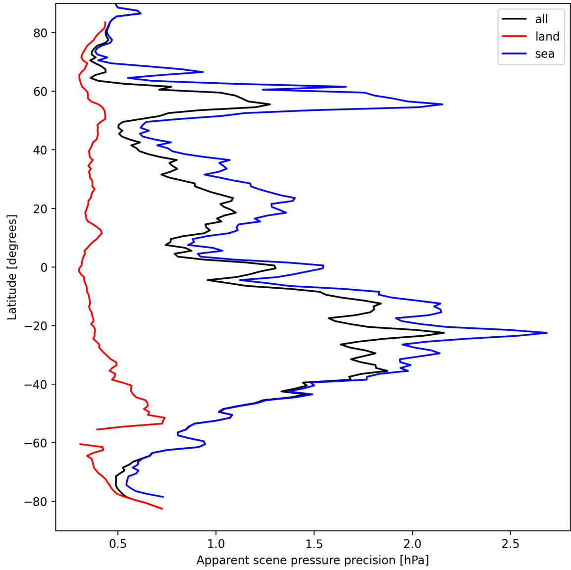
Figure 20: Zonal average of “Apparent scene pressure precision” for 2025-04-03 to 2025-04-04.
