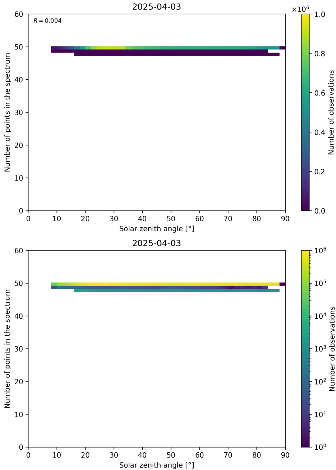
Figure 115: Scatter density plot of “Solar zenith angle” against “Number of points in the spectrum” for 2025-04-03 to 2025-04-04.
