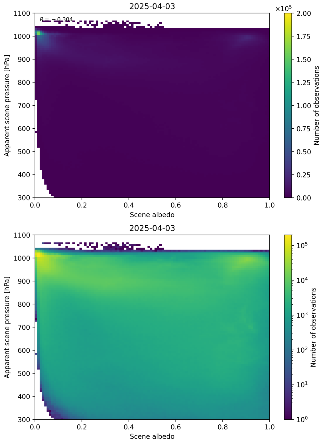
Figure 102: Scatter density plot of “Scene albedo” against “Apparent scene pressure” for 2025-04-03 to 2025-04-04.
