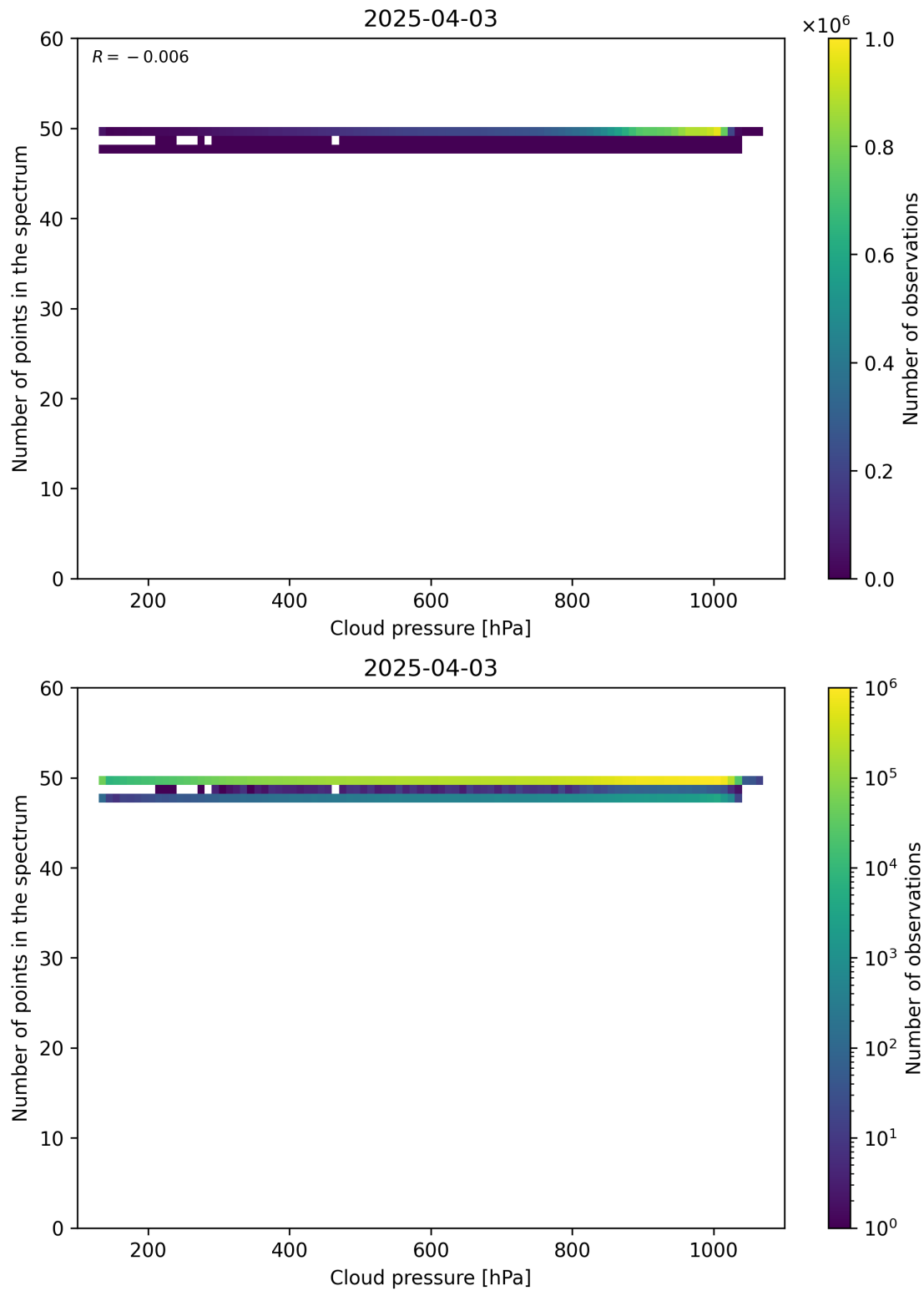
Figure 82: Scatter density plot of “Cloud pressure” against “Number of points in the spectrum” for 2025-04-03 to 2025-04-04.
