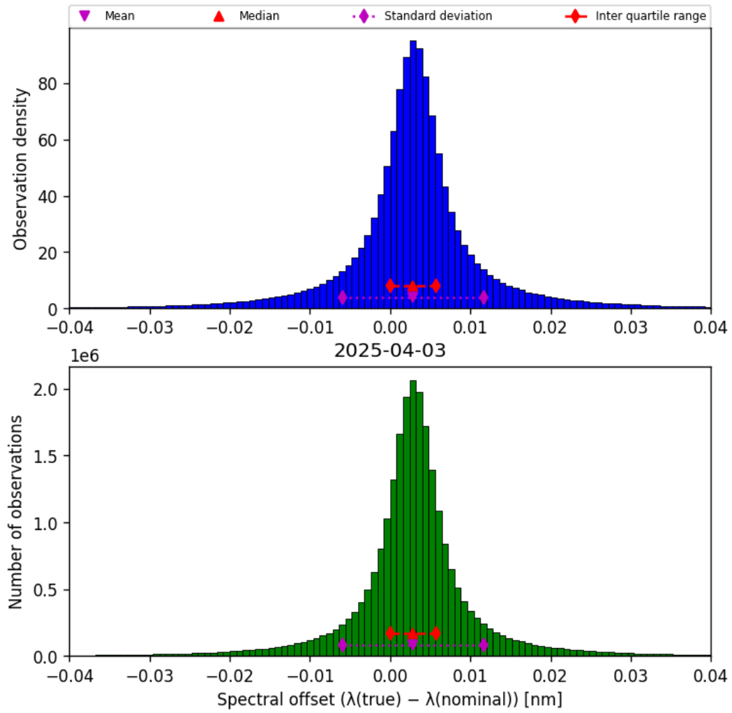
Figure 45: Histogram of “Spectral offset ( \lambda_{\text{true}} - \lambda_{\text{nominal}} )” for 2025-04-03 to 2025-04-04
