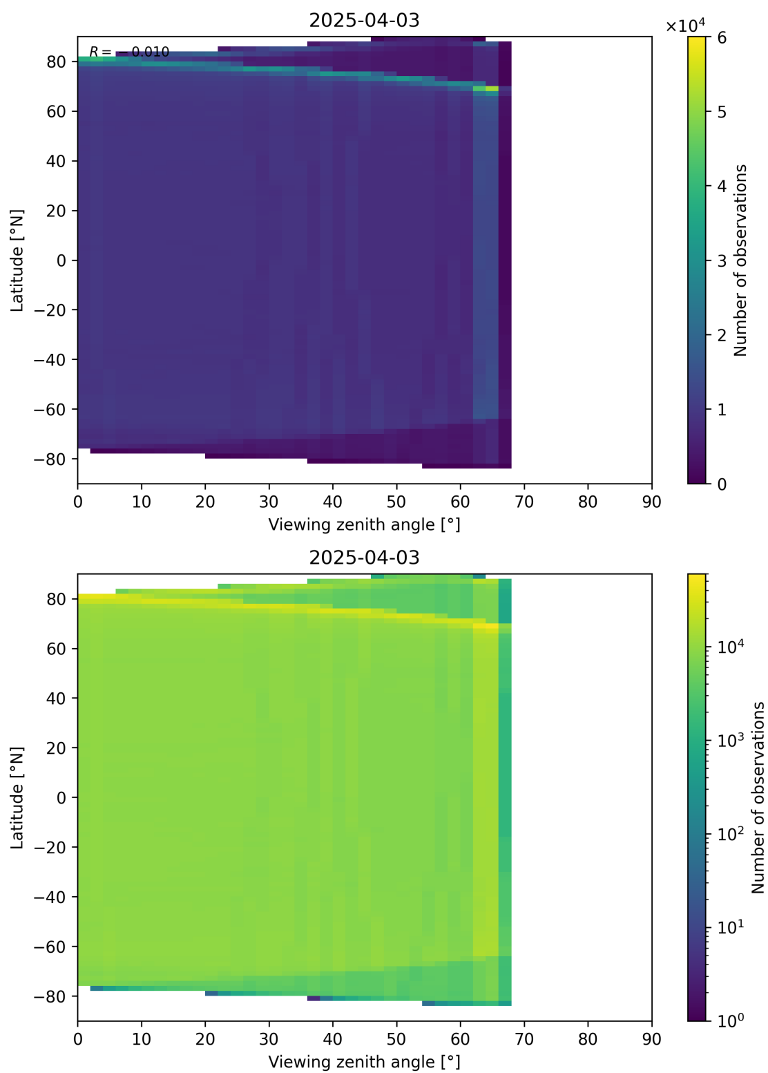
Figure 123: Scatter density plot of “Viewing zenith angle” against “Latitude” for 2025-04-03 to 2025-04-04.
