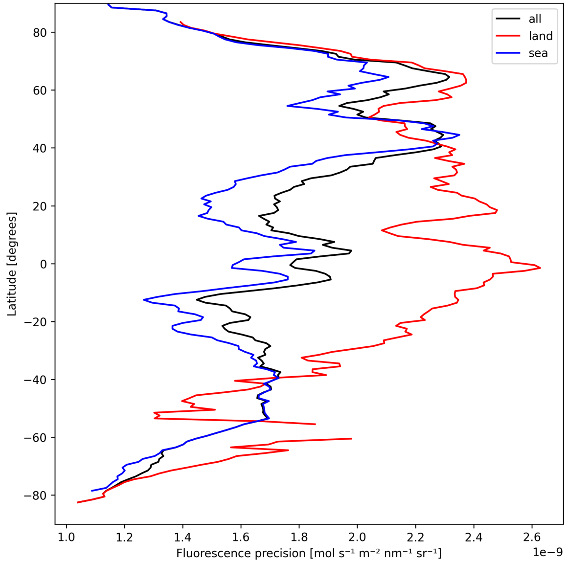
Figure 24: Zonal average of “Fluorescence precision” for 2025-04-03 to 2025-04-04.
