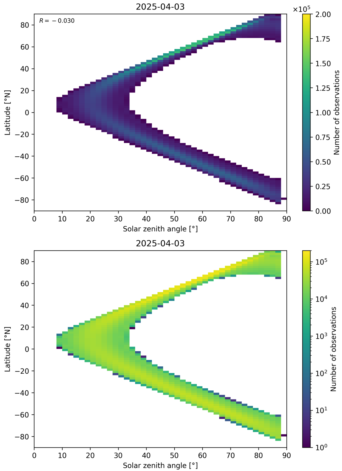
Figure 113: Scatter density plot of “Solar zenith angle” against “Latitude” for 2025-04-03 to 2025-04-04.
