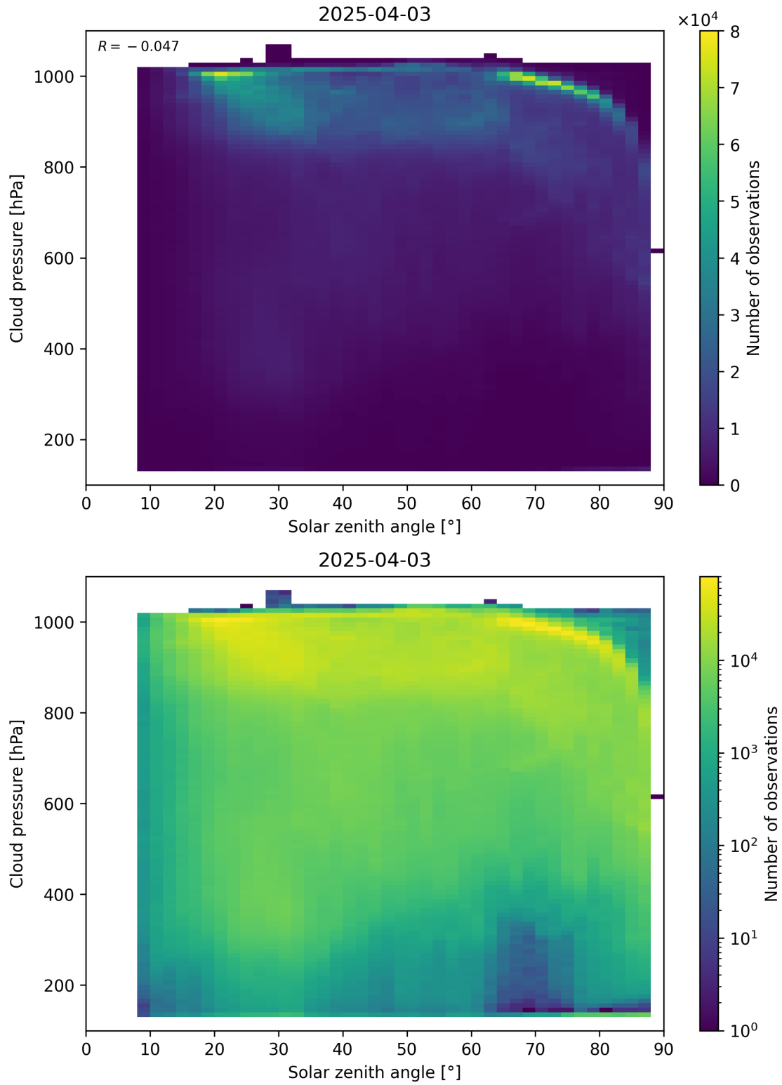
Figure 111: Scatter density plot of “Solar zenith angle” against “Cloud pressure” for 2025-04-03 to 2025-04-04.
