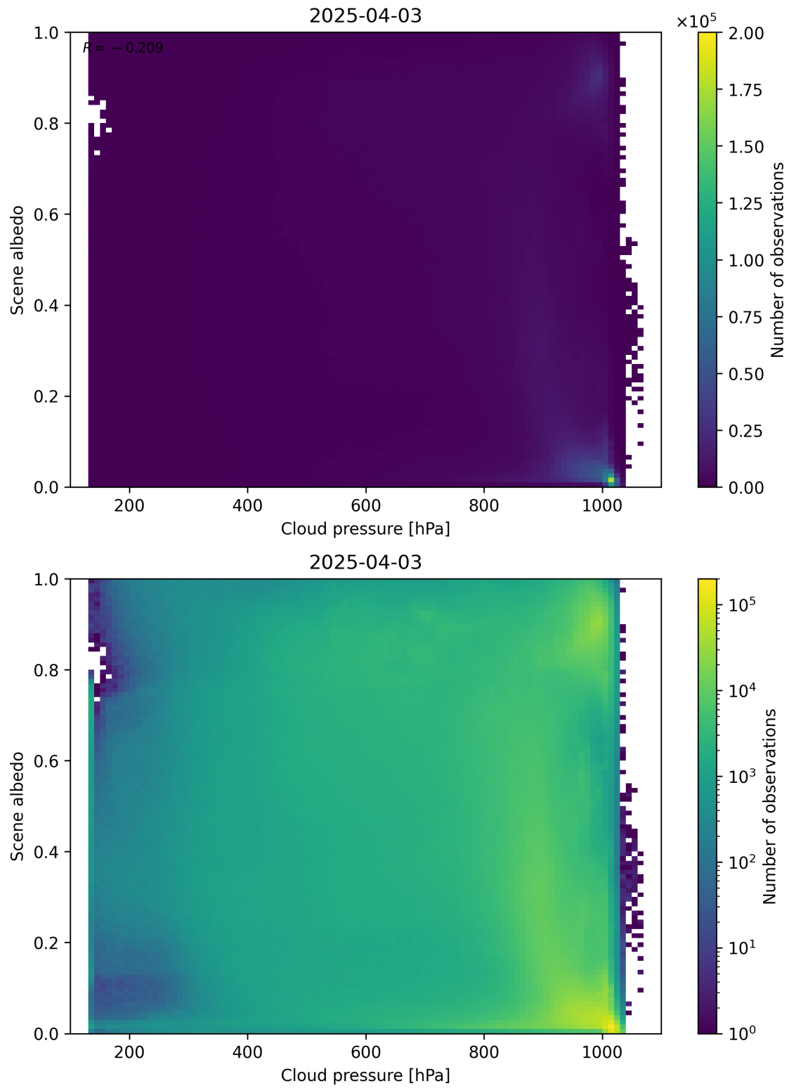
Figure 83: Scatter density plot of “Cloud pressure” against “Scene albedo” for 2025-04-03 to 2025-04-04.
