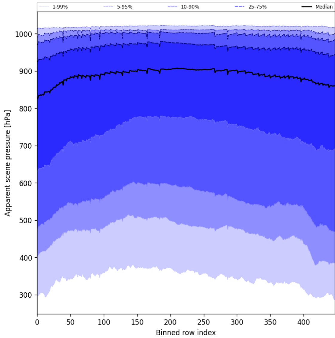
Figure 53: Along track statistics of “Apparent scene pressure” for 2025-04-03 to 2025-04-04
