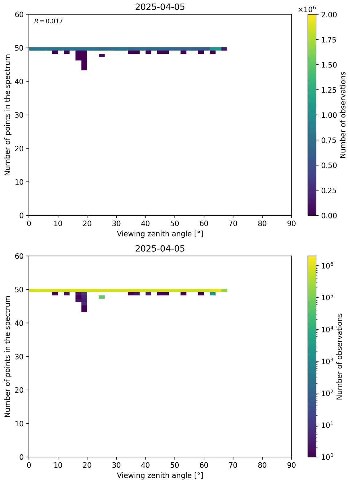
Figure 125: Scatter density plot of “Viewing zenith angle” against “Number of points in the spectrum” for 2025-04-04 to 2025-04-06.
