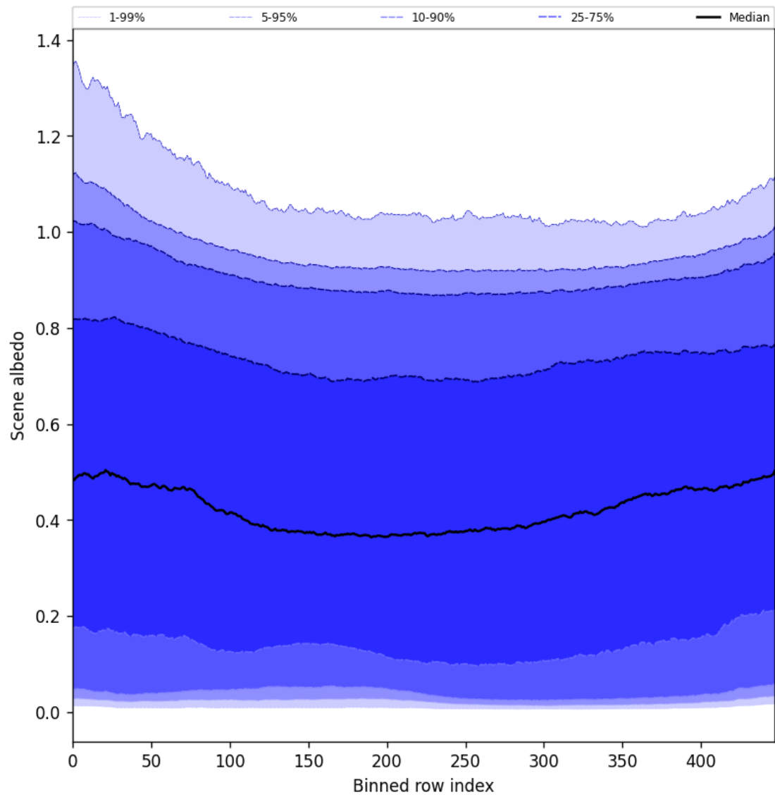
Figure 51: Along track statistics of “Scene albedo” for 2025-04-04 to 2025-04-06
