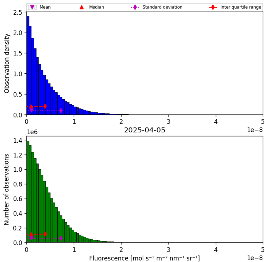
Figure 40: Histogram of “Fluorescence” for 2025-04-04 to 2025-04-06
