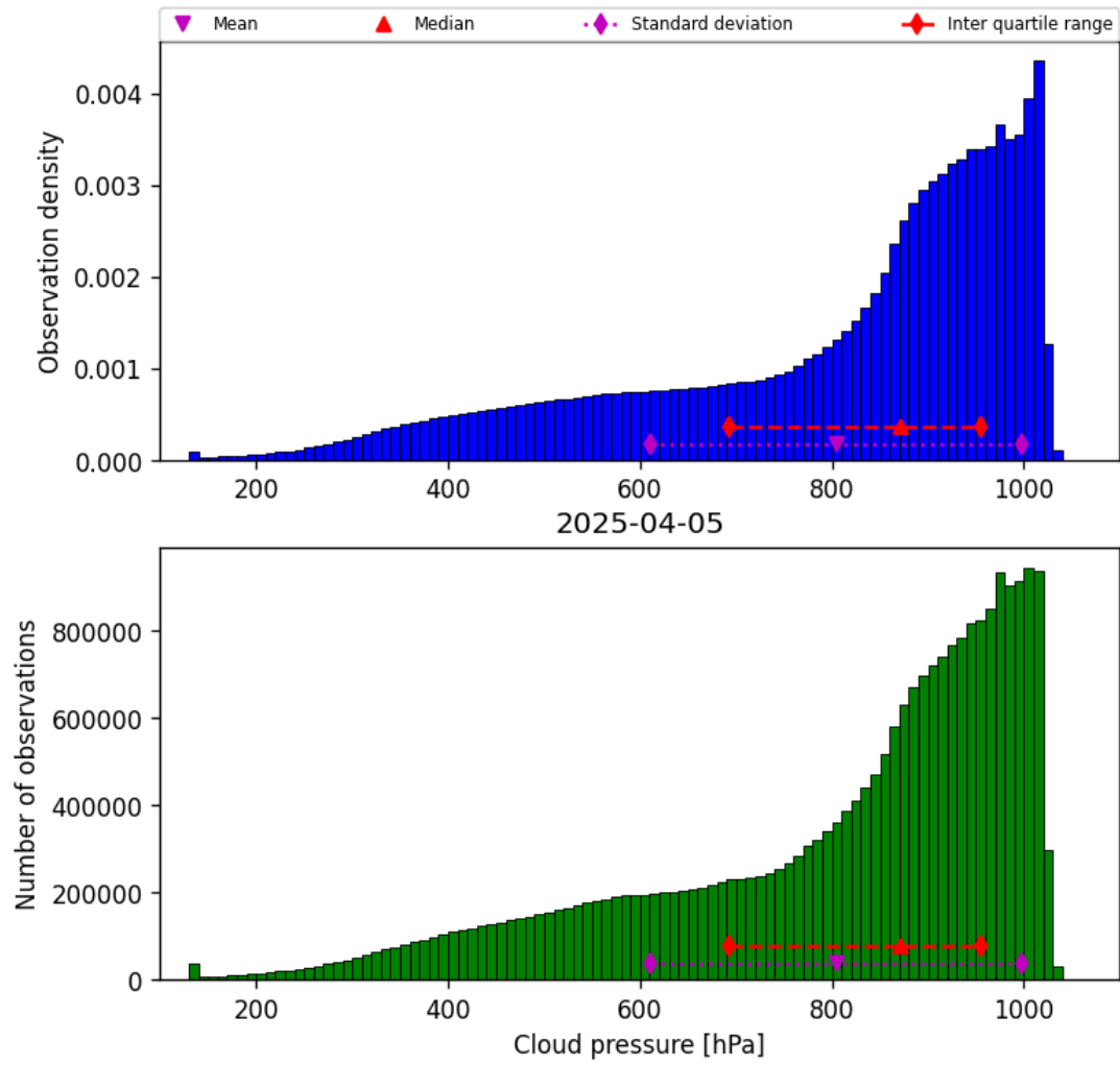
Figure 30: Histogram of “Cloud pressure” for 2025-04-04 to 2025-04-06
