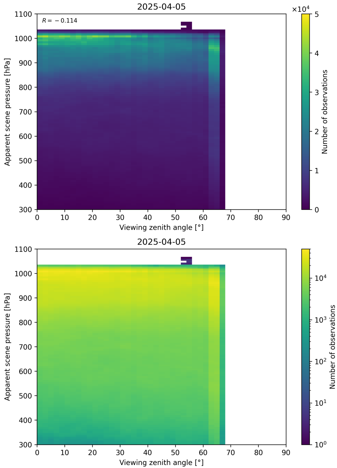
Figure 118: Scatter density plot of “Viewing zenith angle” against “Apparent scene pressure” for 2025-04-04 to 2025-04-06.
