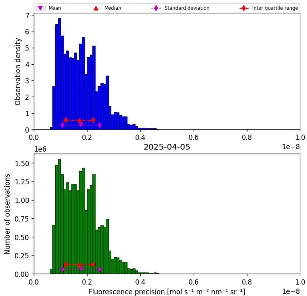
Figure 41: Histogram of “Fluorescence precision” for 2025-04-04 to 2025-04-06
