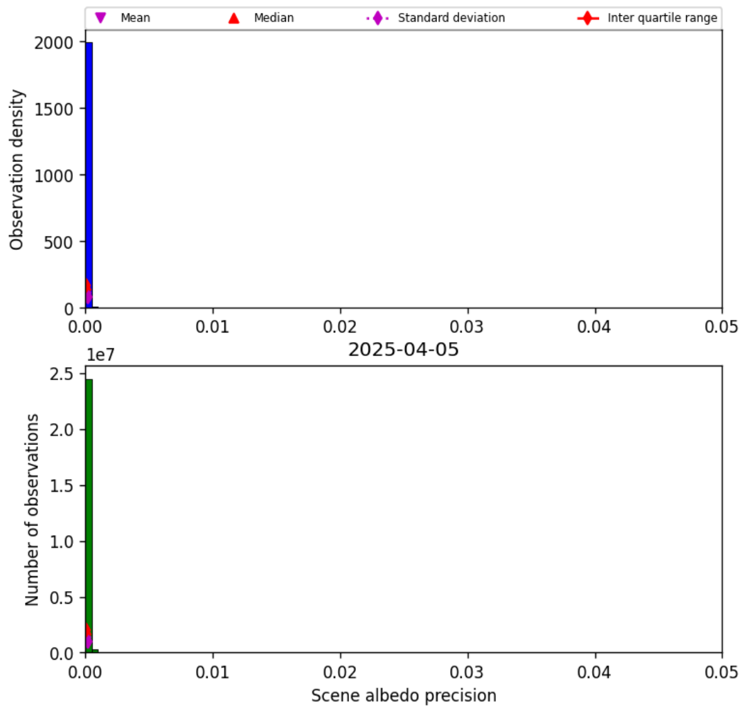
Figure 35: Histogram of “Scene albedo precision” for 2025-04-04 to 2025-04-06
