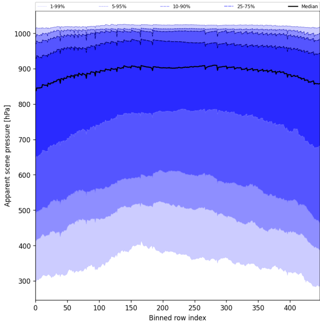
Figure 53: Along track statistics of “Apparent scene pressure” for 2025-04-04 to 2025-04-06
