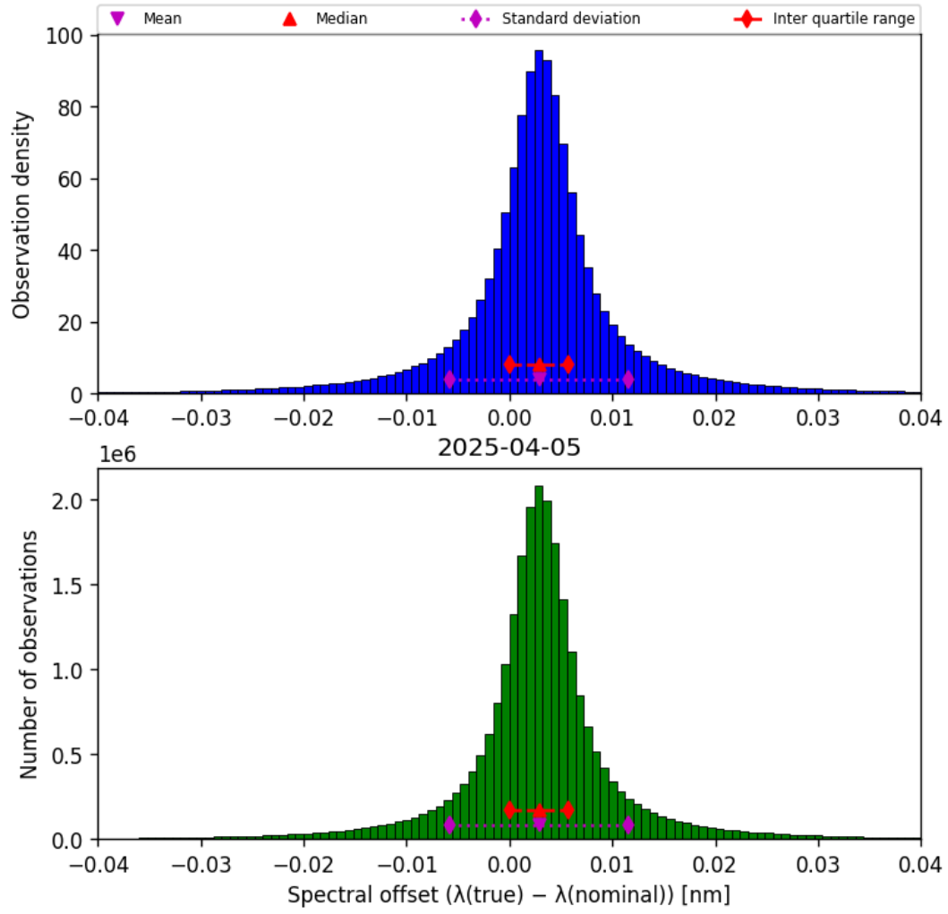
Figure 45: Histogram of “Spectral offset ( \lambda_{\text{true}} - \lambda_{\text{nominal}} )” for 2025-04-04 to 2025-04-06
