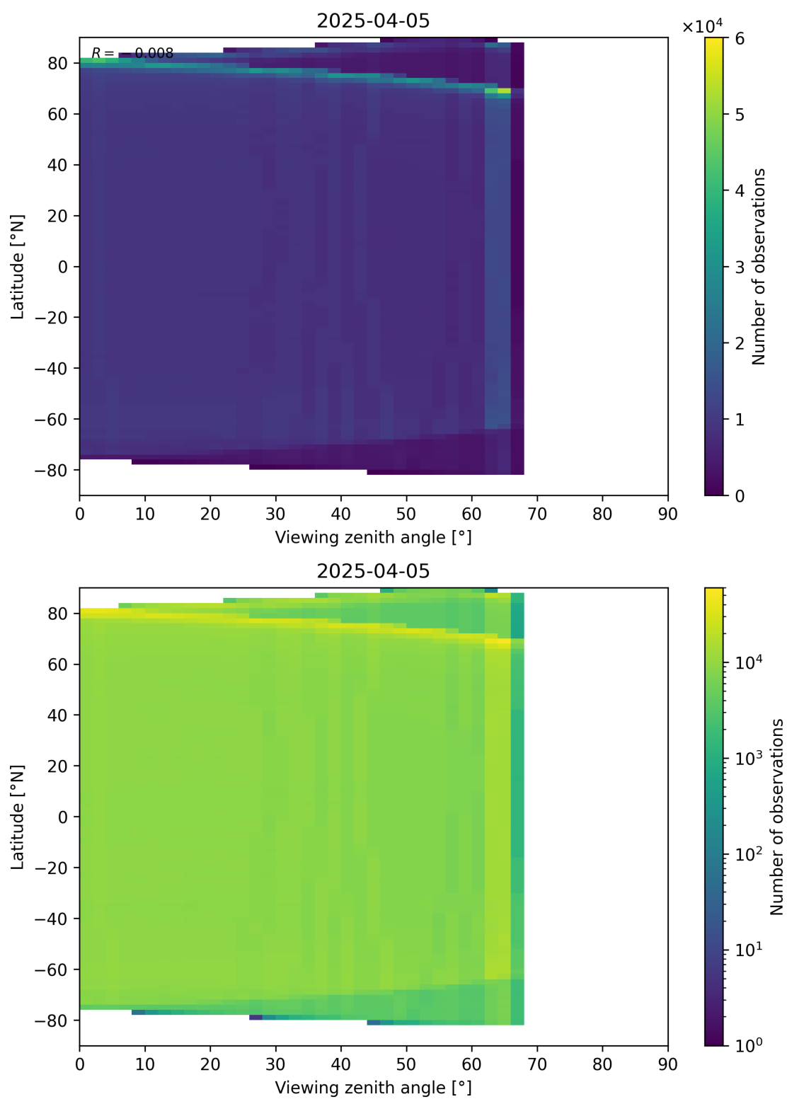
Figure 123: Scatter density plot of “Viewing zenith angle” against “Latitude” for 2025-04-04 to 2025-04-06.
