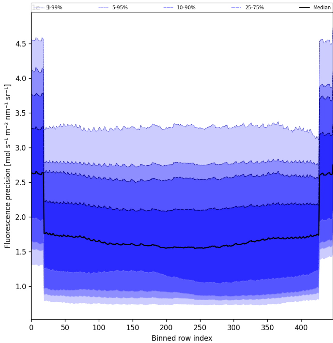
Figure 58: Along track statistics of “Fluorescence precision” for 2025-04-04 to 2025-04-06
