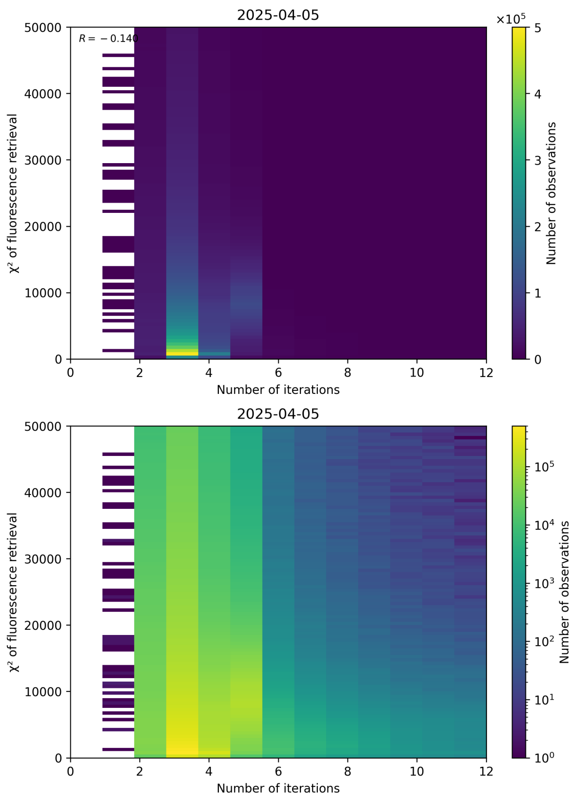
Figure 97: Scatter density plot of “Number of iterations” against “ \chi^2 of fluorescence retrieval” for 2025-04-04 to 2025-04-06.
