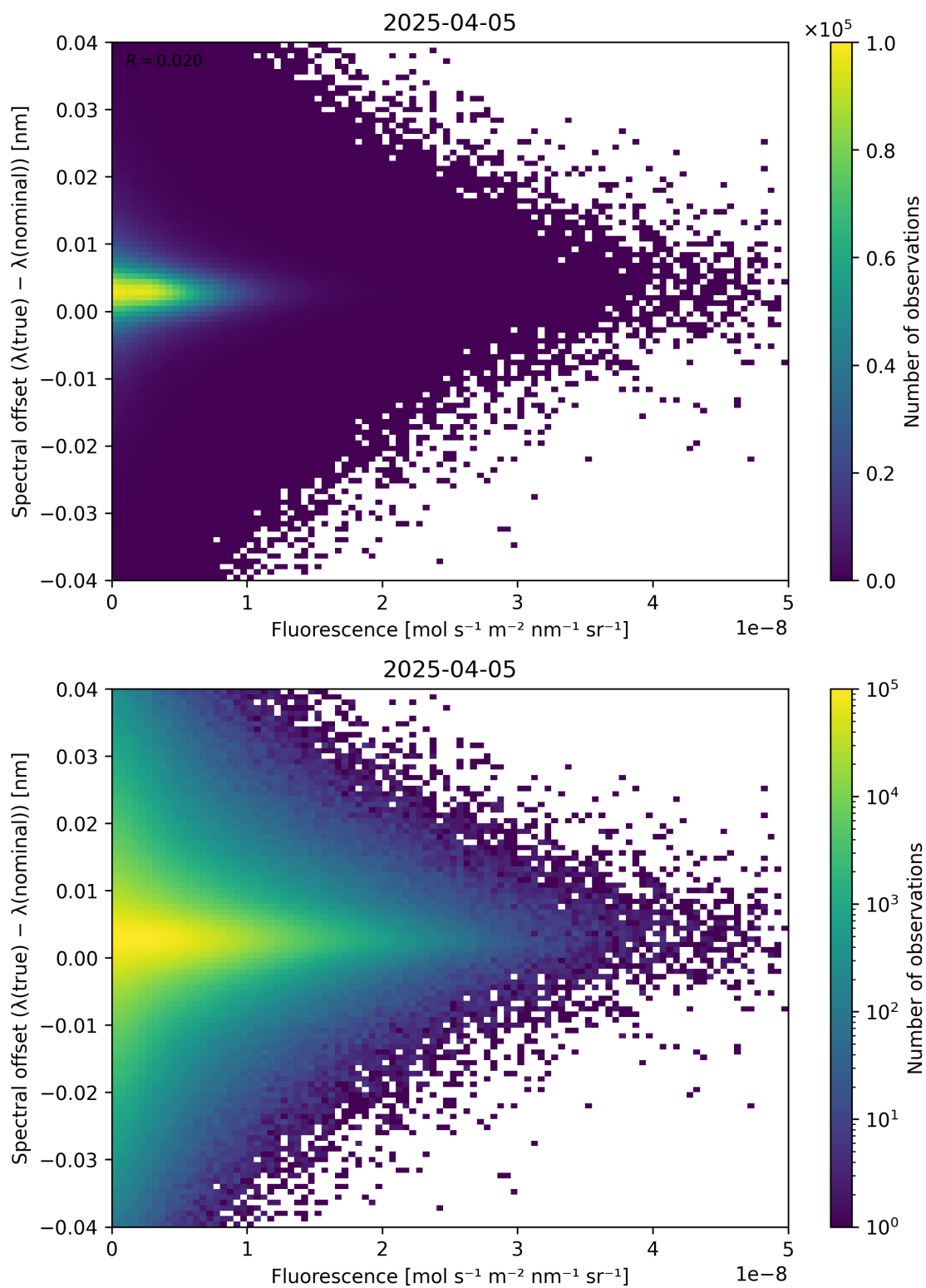
Figure 87: Scatter density plot of “Fluorescence” against “Spectral offset ( \lambda_{\text{true}} - \lambda_{\text{nominal}} )” for 2025-04-04 to 2025-04-06.
