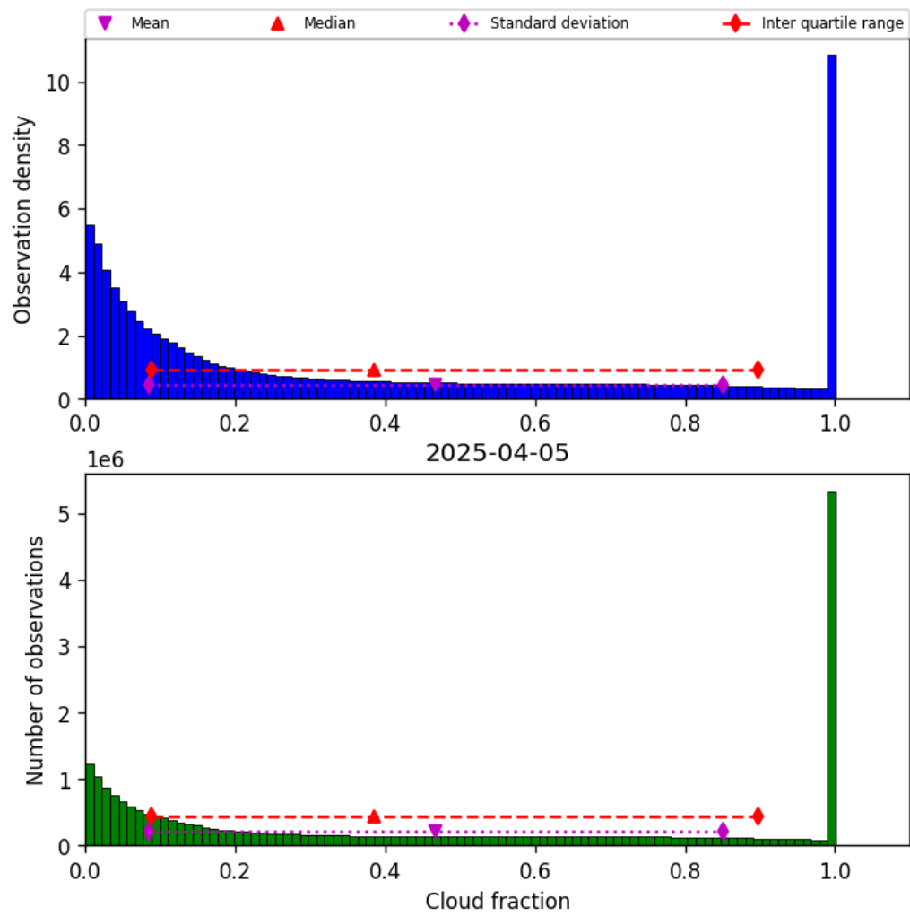
Figure 32: Histogram of “Cloud fraction” for 2025-04-04 to 2025-04-06
