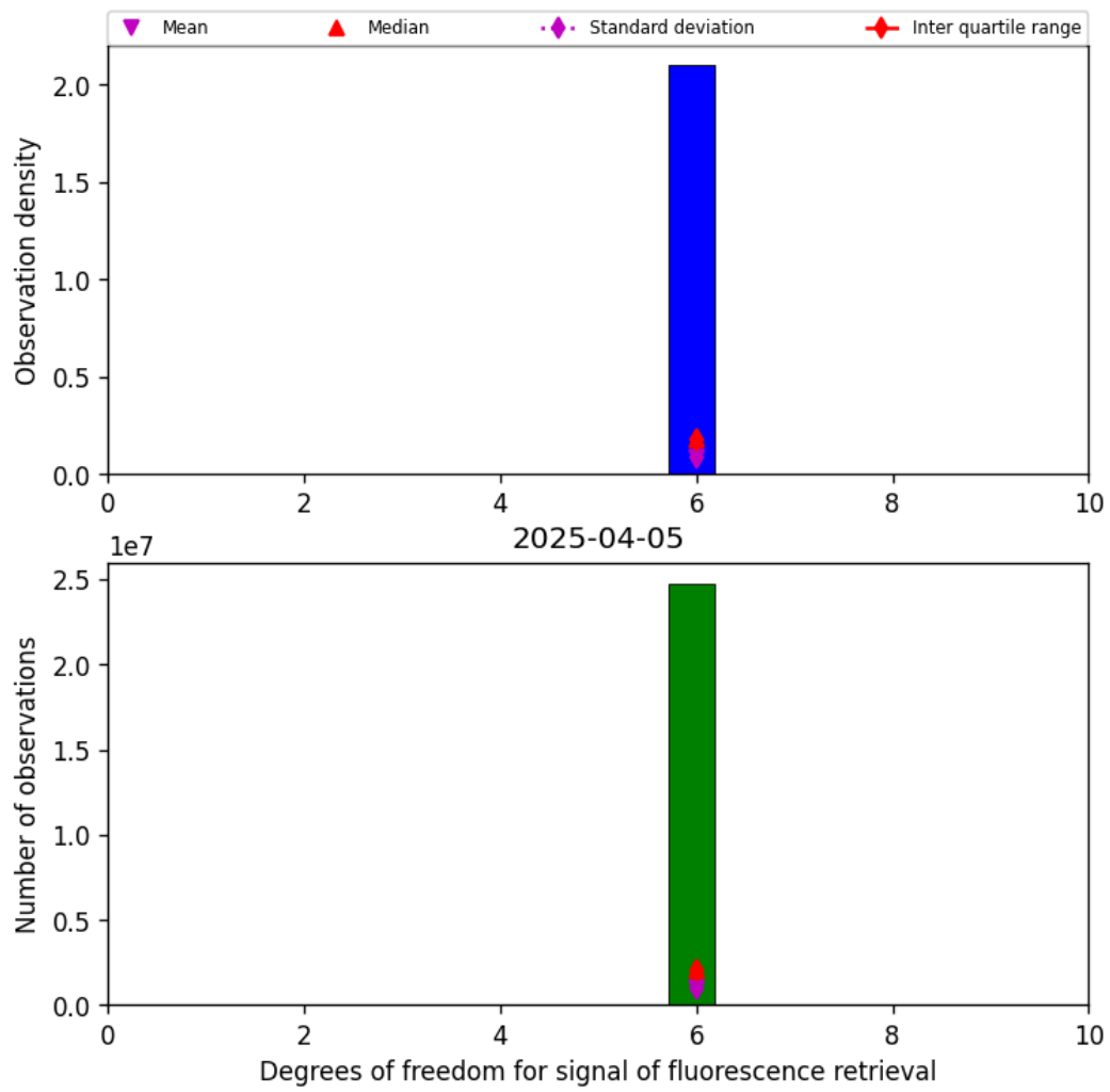
Figure 43: Histogram of "Degrees of freedom for signal of fluorescence retrieval" for 2025-04-04 to 2025-04-06
