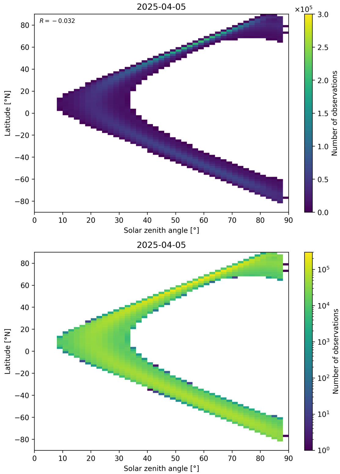
Figure 113: Scatter density plot of “Solar zenith angle” against “Latitude” for 2025-04-04 to 2025-04-06.
