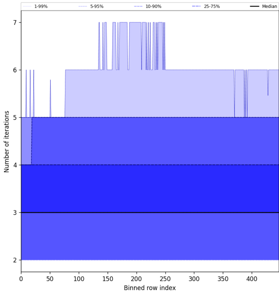
Figure 56: Along track statistics of “Number of iterations” for 2025-04-04 to 2025-04-06
