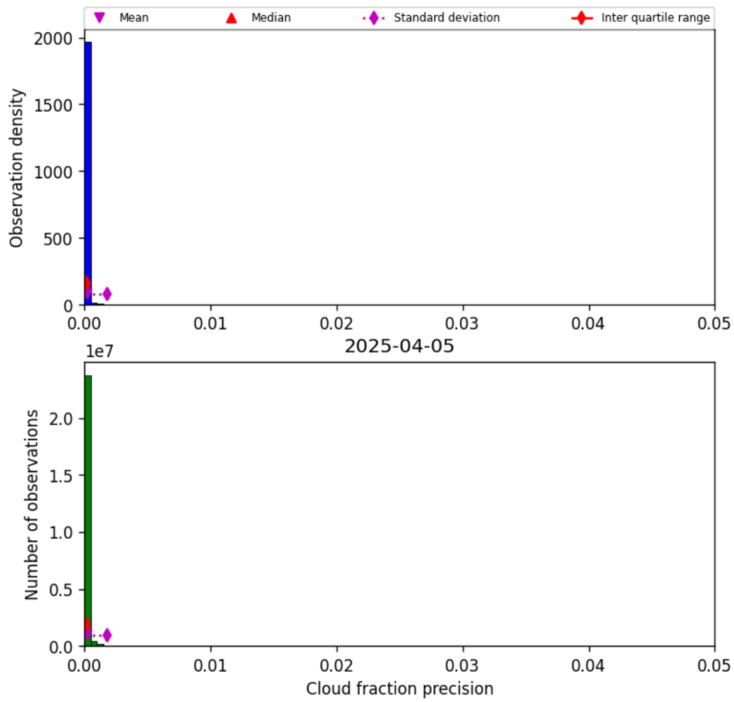
Figure 33: Histogram of “Cloud fraction precision” for 2025-04-04 to 2025-04-06
