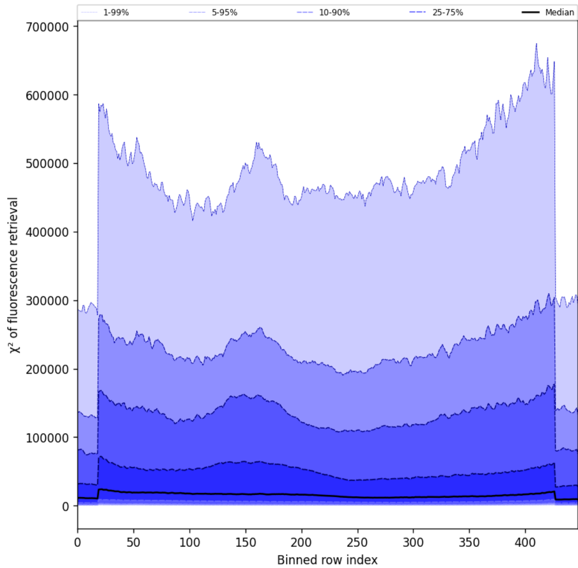
Figure 59: Along track statistics of “ \chi^2 of fluorescence retrieval” for 2025-04-04 to 2025-04-06
