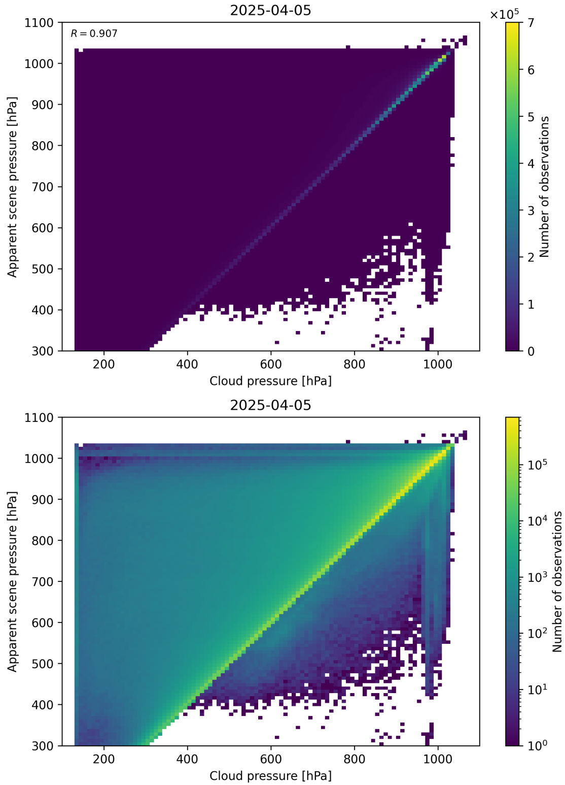
Figure 77: Scatter density plot of “Cloud pressure” against “Apparent scene pressure” for 2025-04-04 to 2025-04-06.
