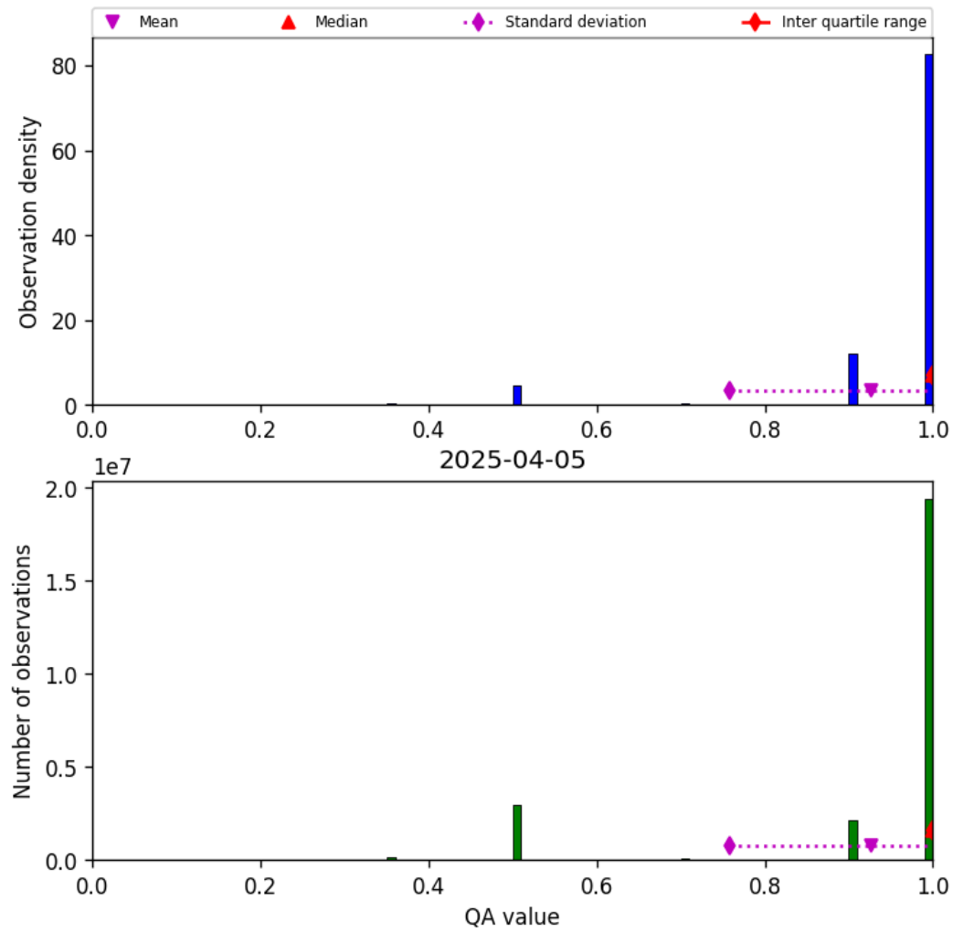
Figure 29: Histogram of “QA value” for 2025-04-04 to 2025-04-06
