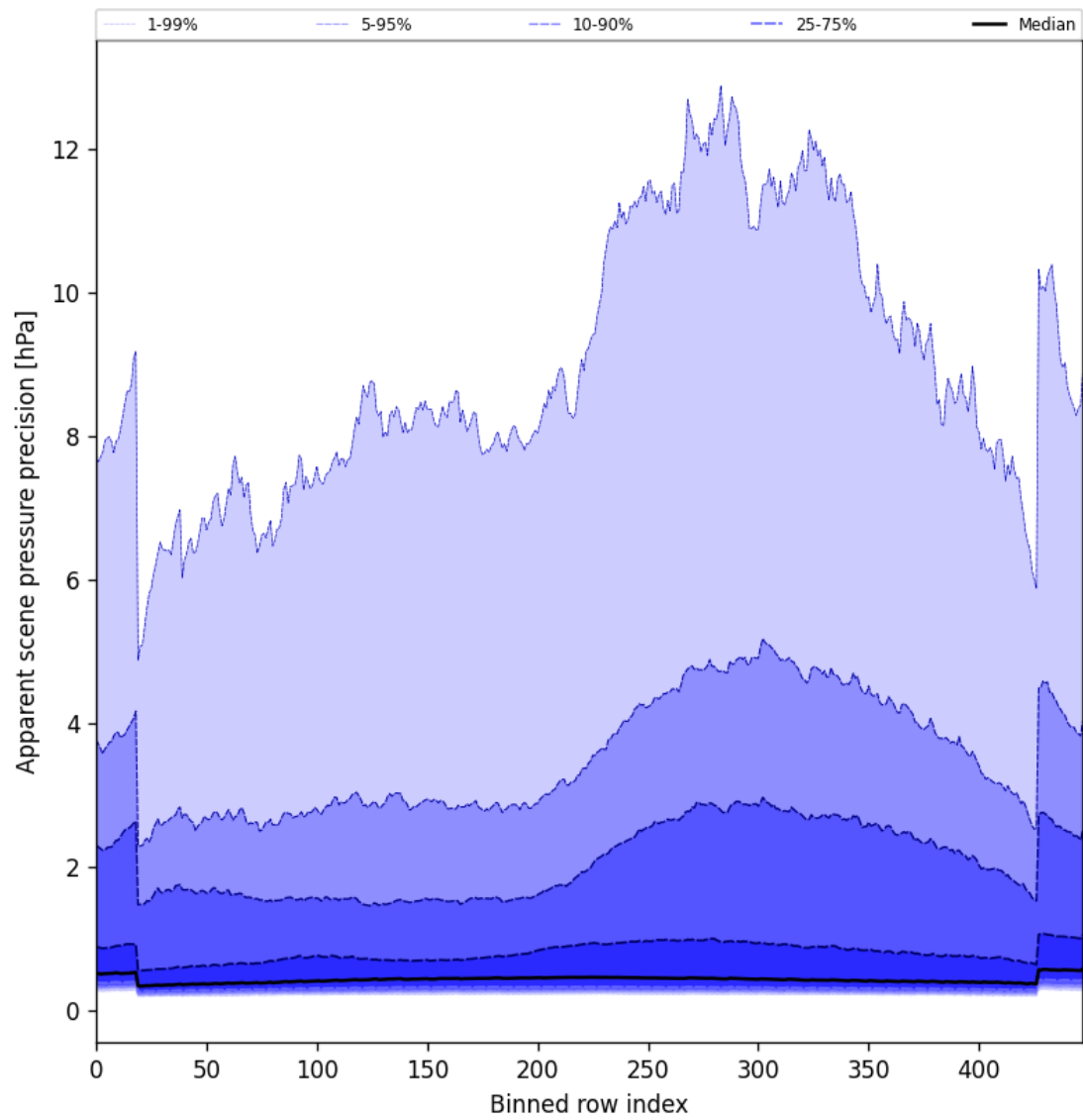
Figure 54: Along track statistics of “Apparent scene pressure precision” for 2025-04-04 to 2025-04-06
