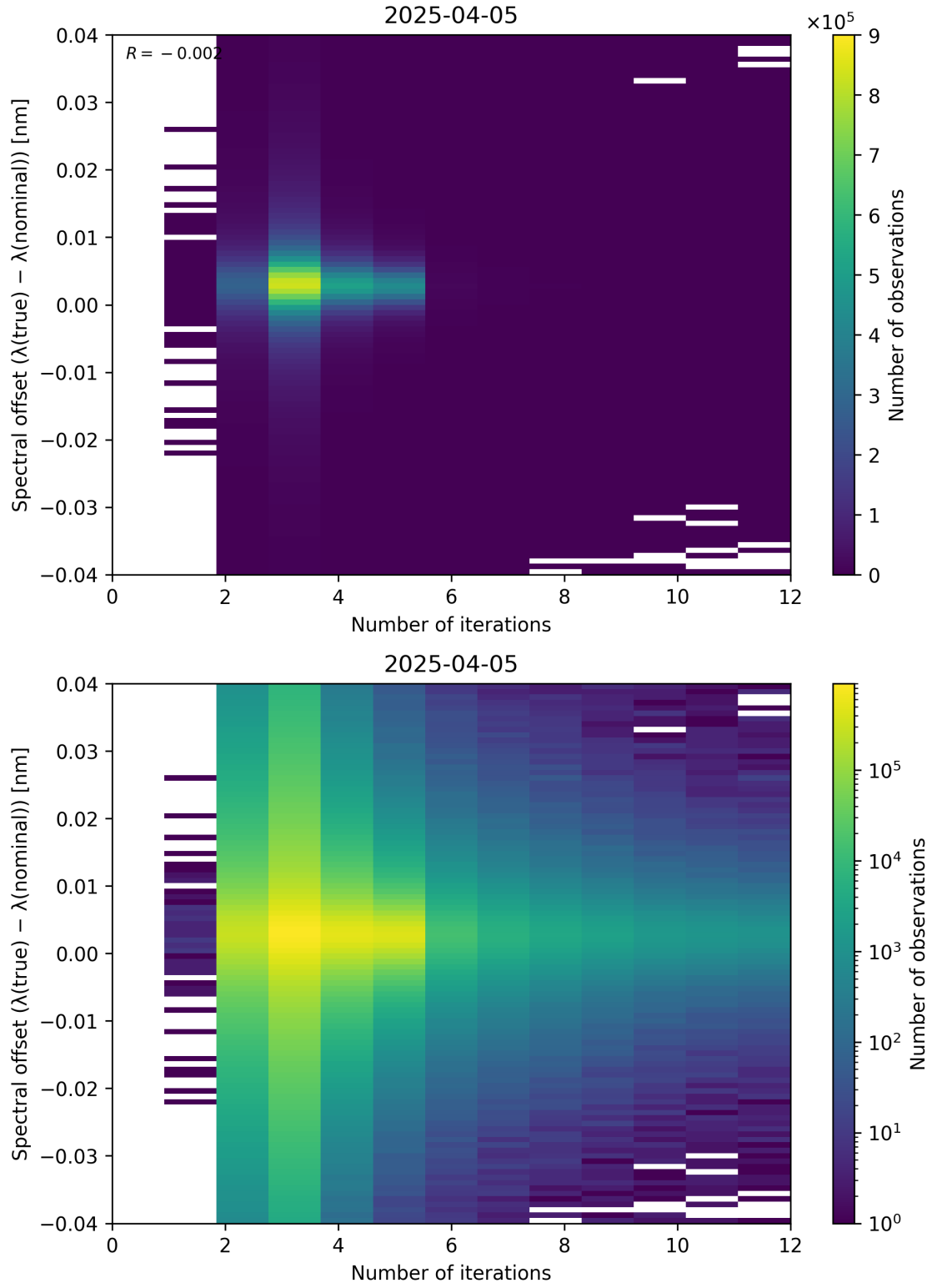
Figure 100: Scatter density plot of “Number of iterations” against “Spectral offset ( \lambda_{\text{true}} - \lambda_{\text{nominal}} )” for 2025-04-04 to 2025-04-06.
