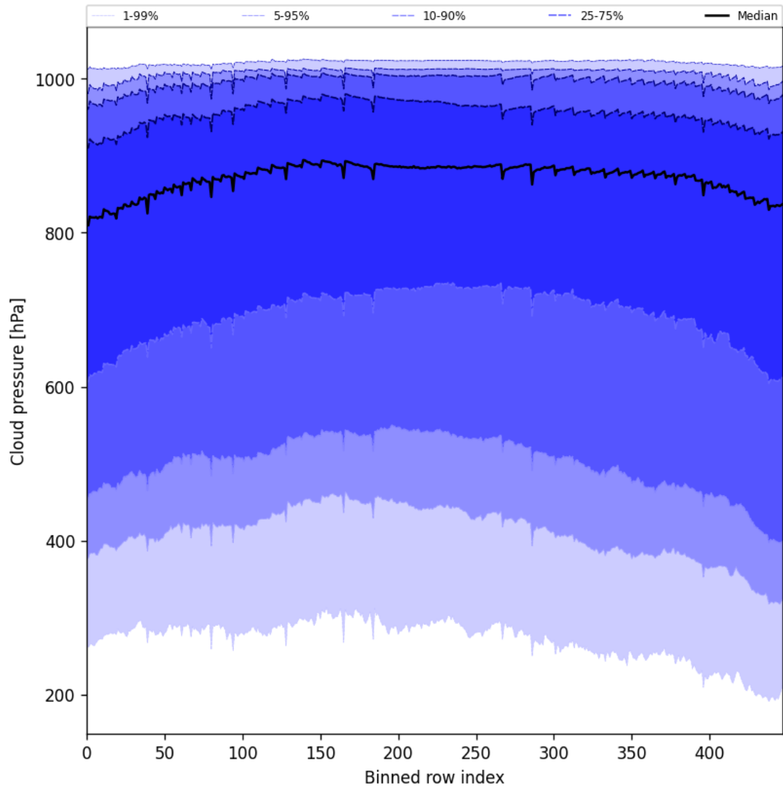
Figure 47: Along track statistics of “Cloud pressure” for 2025-04-04 to 2025-04-06
