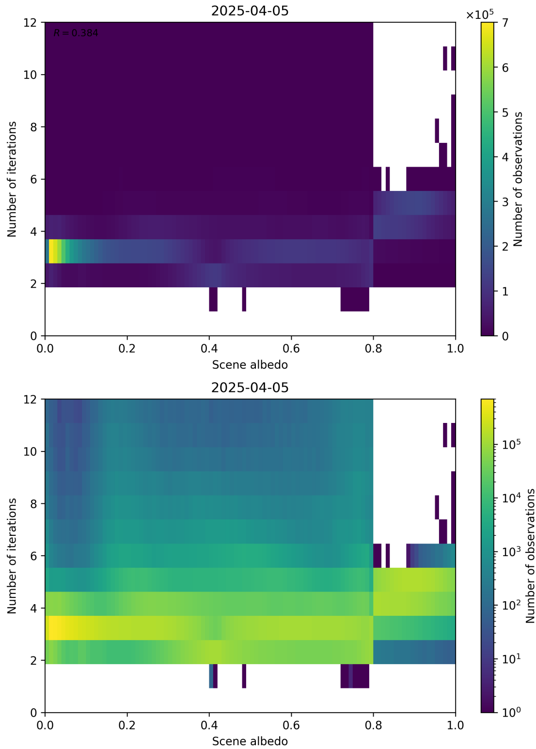
Figure 105: Scatter density plot of “Scene albedo” against “Number of iterations” for 2025-04-04 to 2025-04-06.
