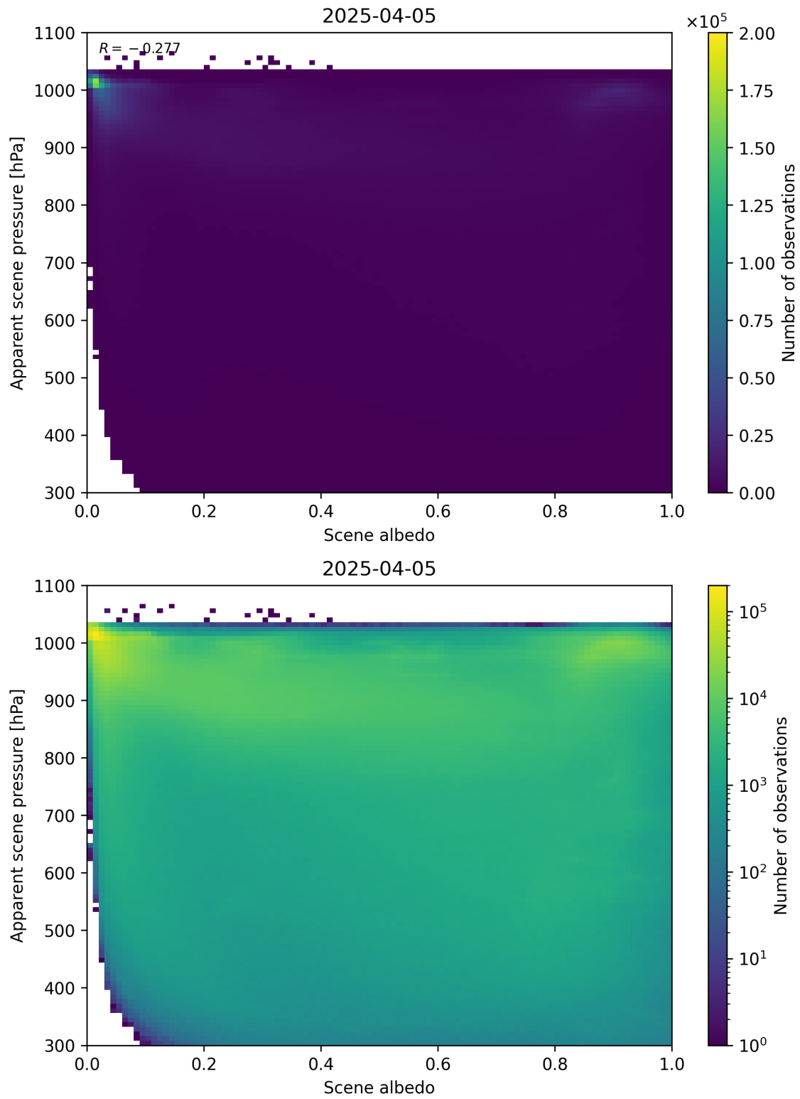
Figure 102: Scatter density plot of “Scene albedo” against “Apparent scene pressure” for 2025-04-04 to 2025-04-06.
