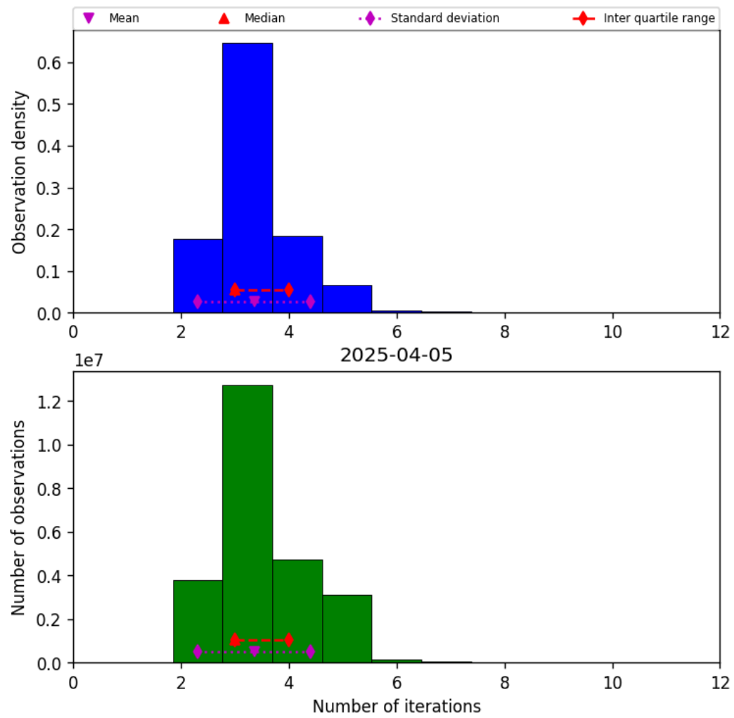
Figure 39: Histogram of “Number of iterations” for 2025-04-04 to 2025-04-06
