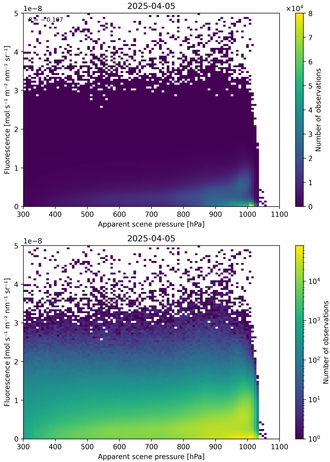
Figure 64: Scatter density plot of “Apparent scene pressure” against “Fluorescence” for 2025-04-04 to 2025-04-06.
