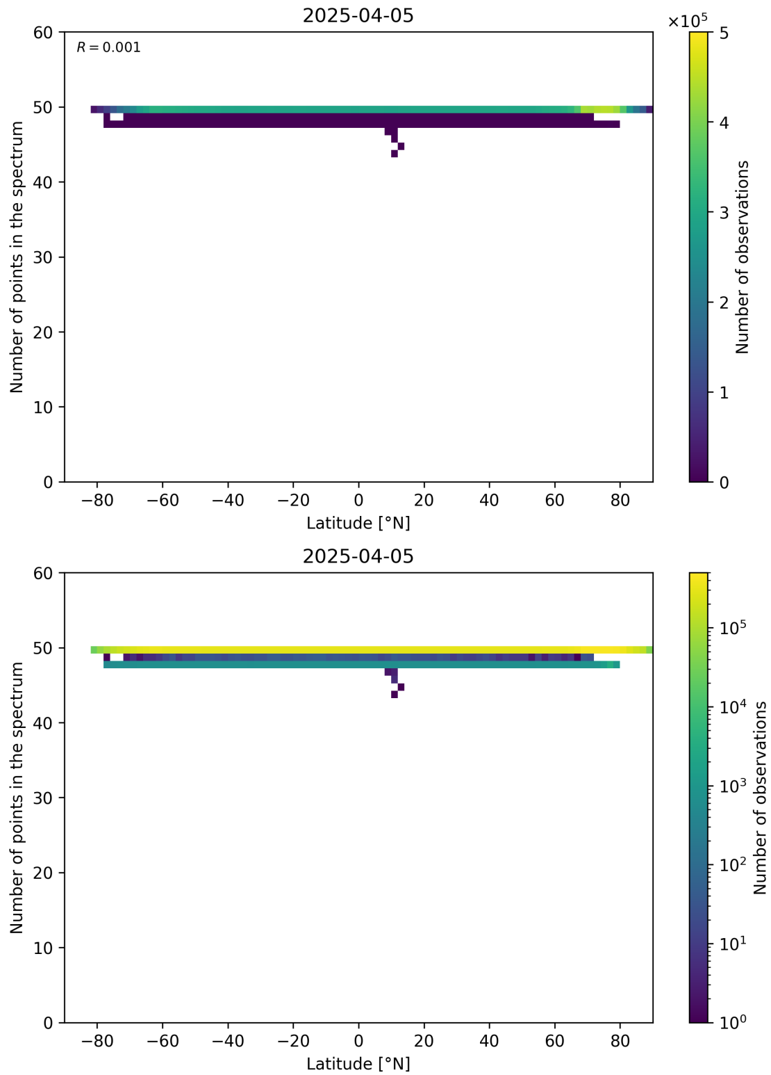
Figure 94: Scatter density plot of “Latitude” against “Number of points in the spectrum” for 2025-04-04 to 2025-04-06.
