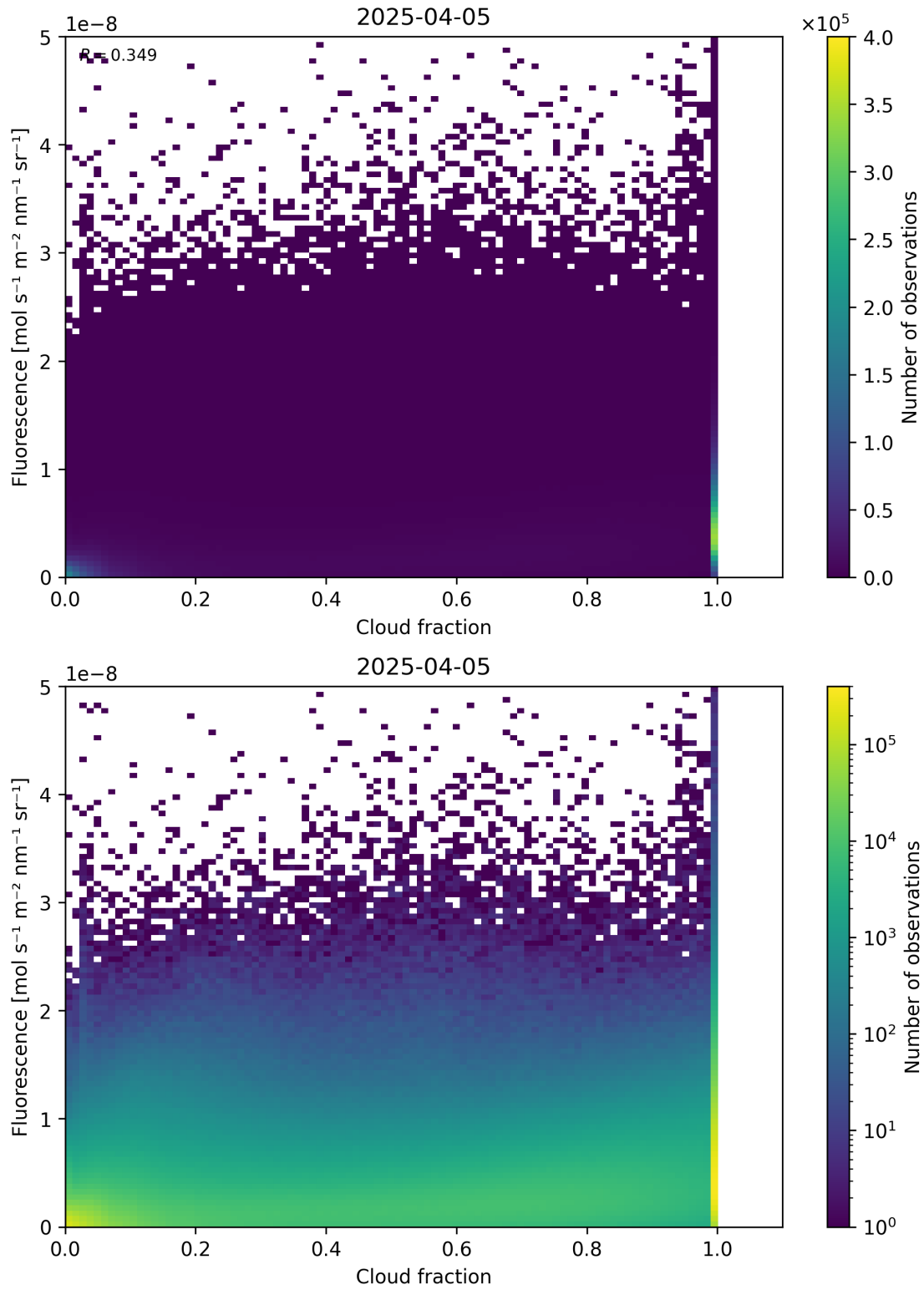
Figure 72: Scatter density plot of “Cloud fraction” against “Fluorescence” for 2025-04-04 to 2025-04-06.
