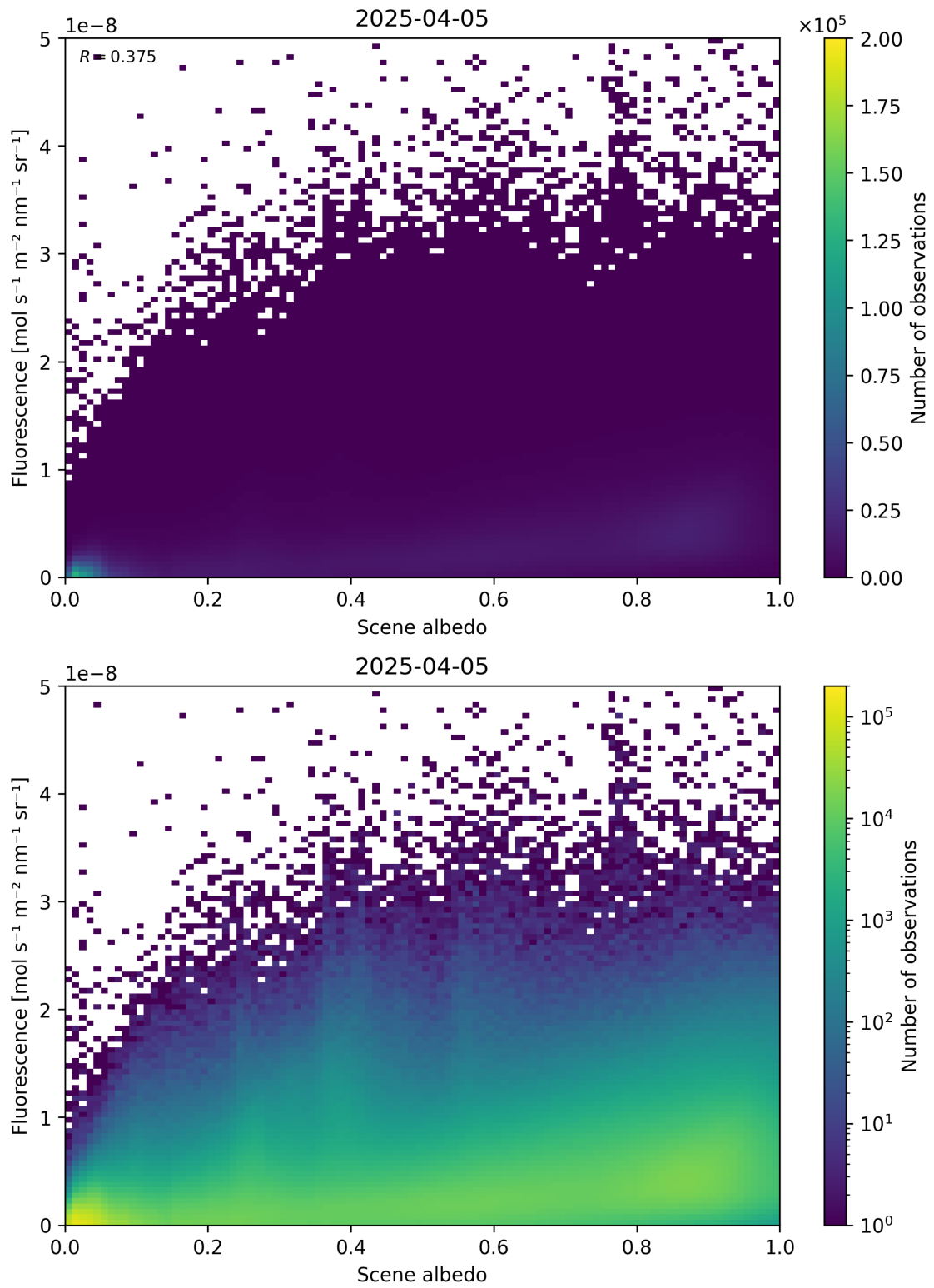
Figure 104: Scatter density plot of "Scene albedo" against "Fluorescence" for 2025-04-04 to 2025-04-06.
