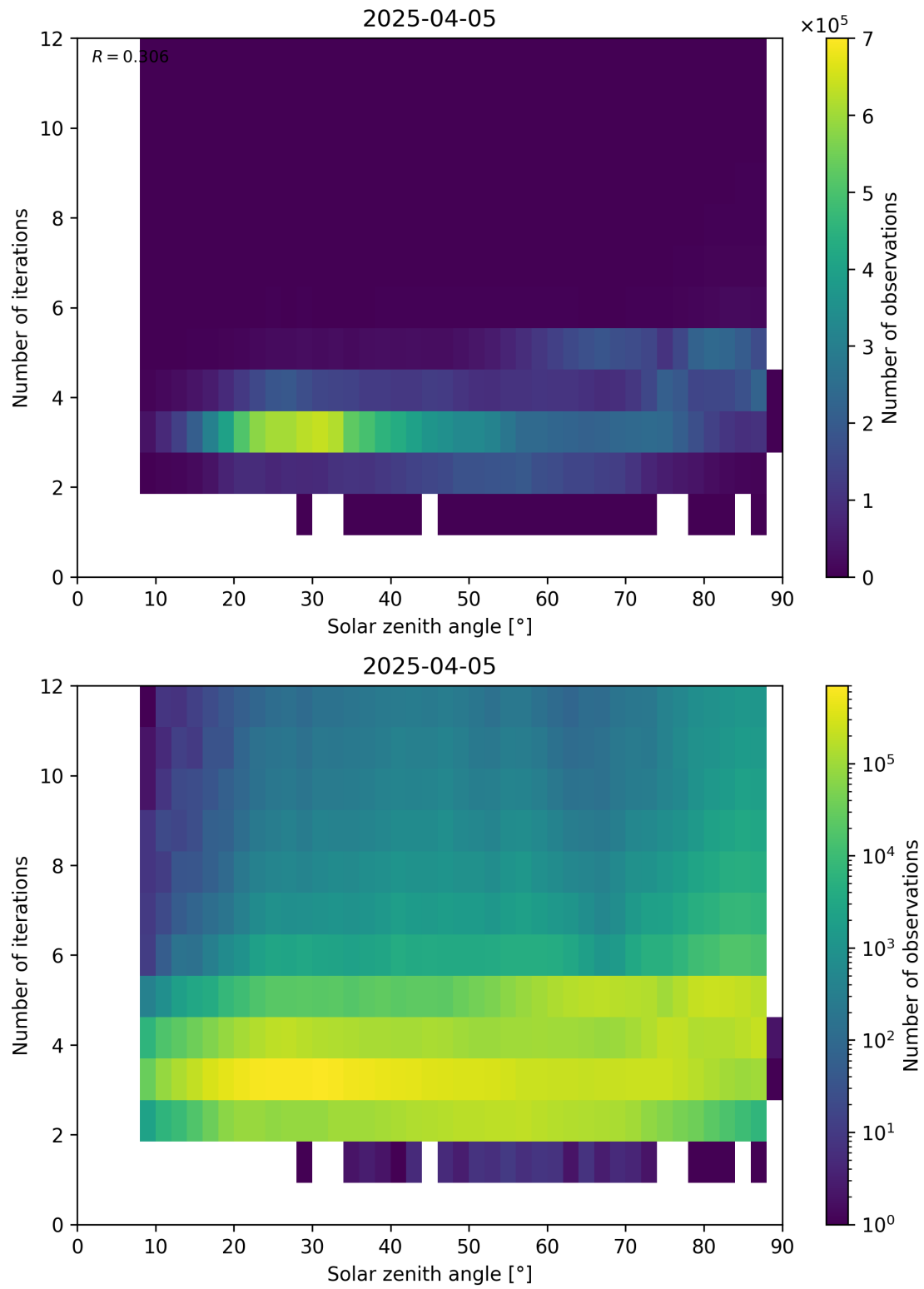
Figure 114: Scatter density plot of “Solar zenith angle” against “Number of iterations” for 2025-04-04 to 2025-04-06.
