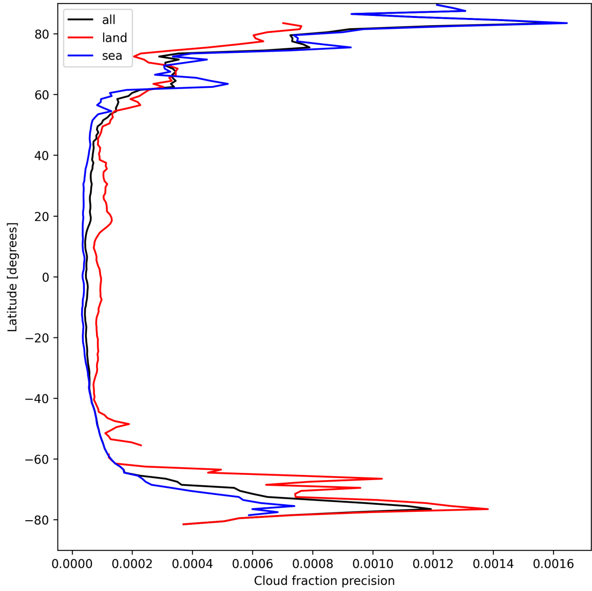
Figure 16: Zonal average of “Cloud fraction precision” for 2025-04-04 to 2025-04-06.
