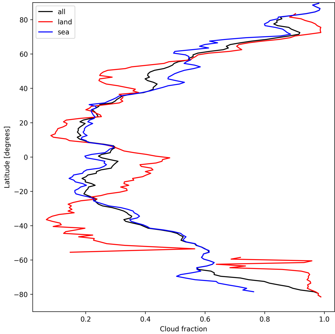
Figure 15: Zonal average of “Cloud fraction” for 2025-04-04 to 2025-04-06.
