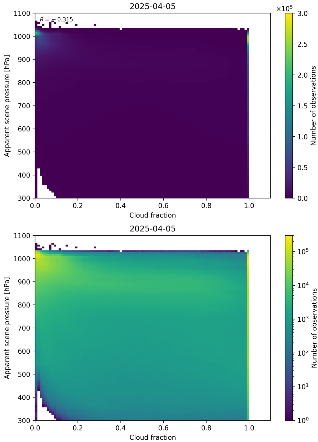
Figure 70: Scatter density plot of “Cloud fraction” against “Apparent scene pressure” for 2025-04-04 to 2025-04-06.
