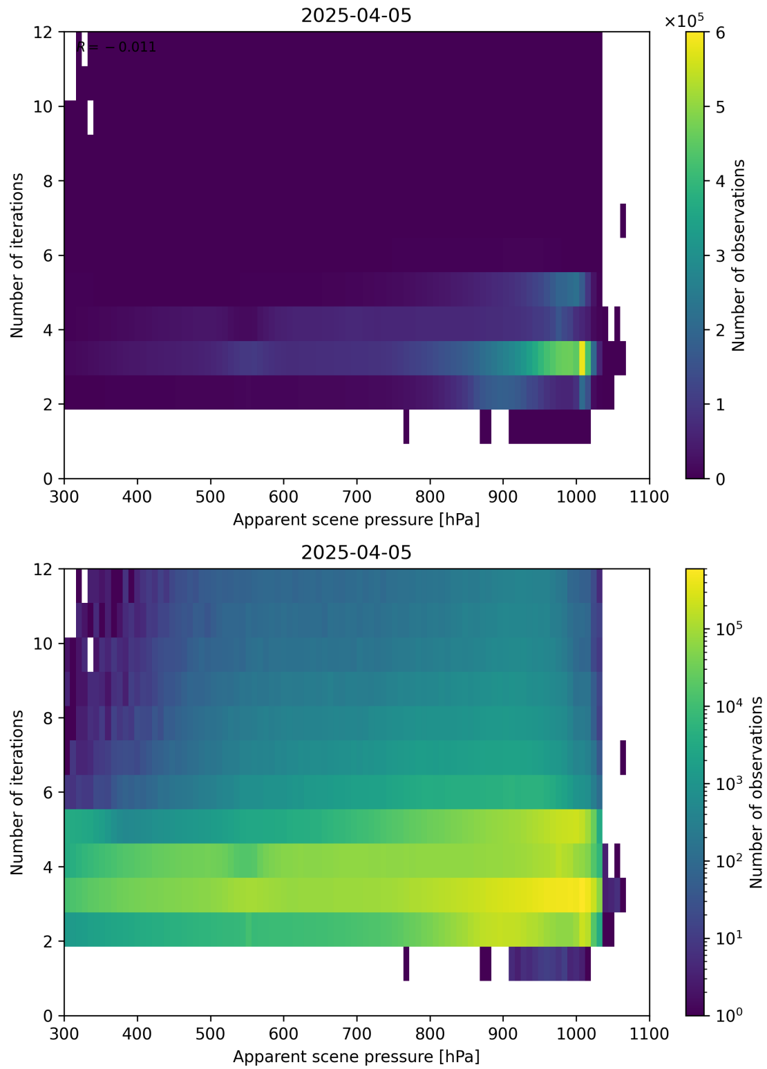
Figure 65: Scatter density plot of “Apparent scene pressure” against “Number of iterations” for 2025-04-04 to 2025-04-06.
