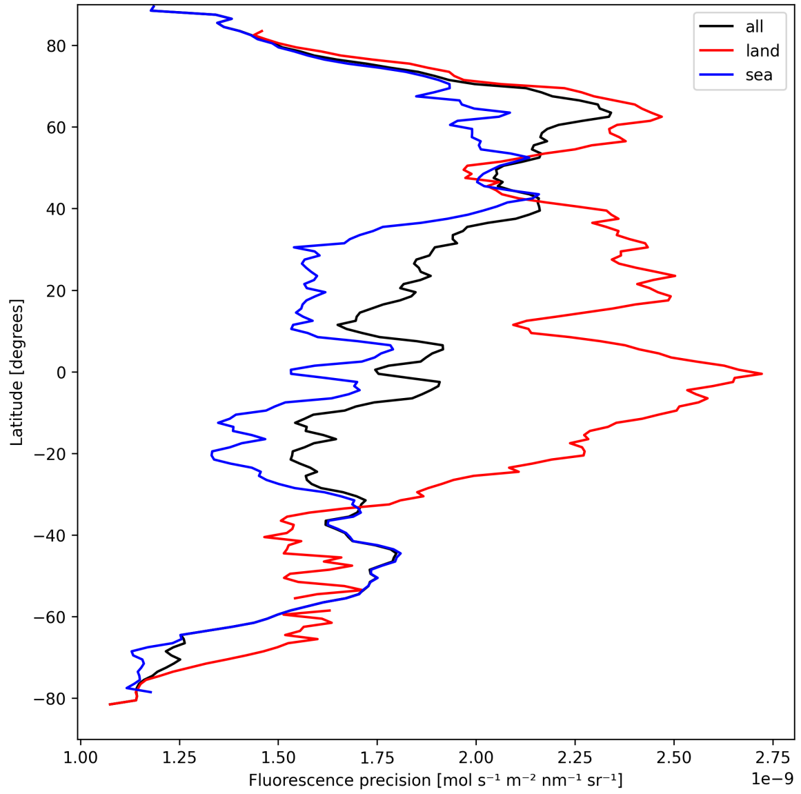
Figure 24: Zonal average of “Fluorescence precision” for 2025-04-04 to 2025-04-06.
