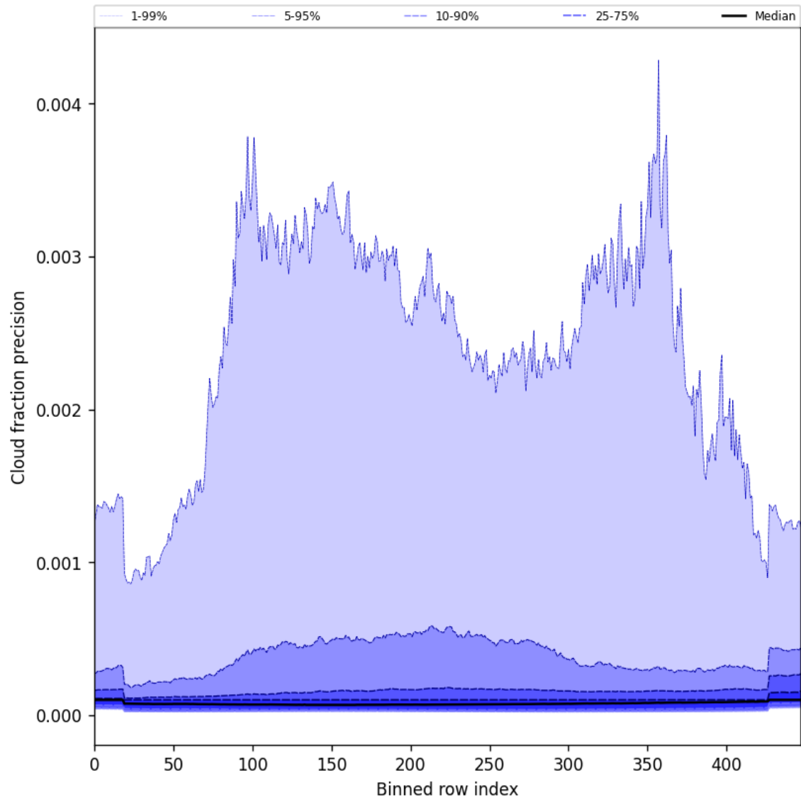
Figure 50: Along track statistics of “Cloud fraction precision” for 2025-04-04 to 2025-04-06
