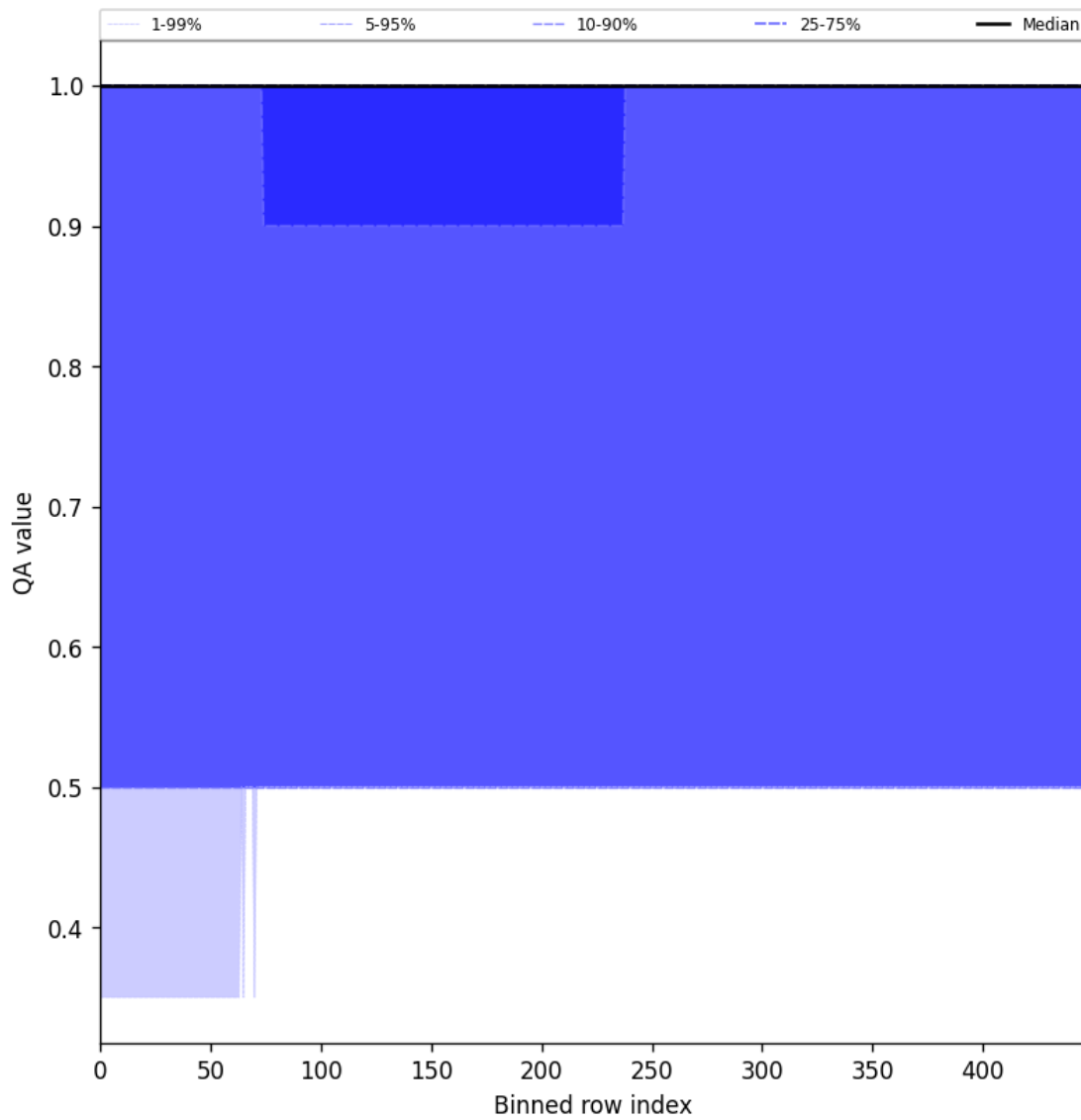
Figure 46: Along track statistics of “QA value” for 2025-04-04 to 2025-04-06
