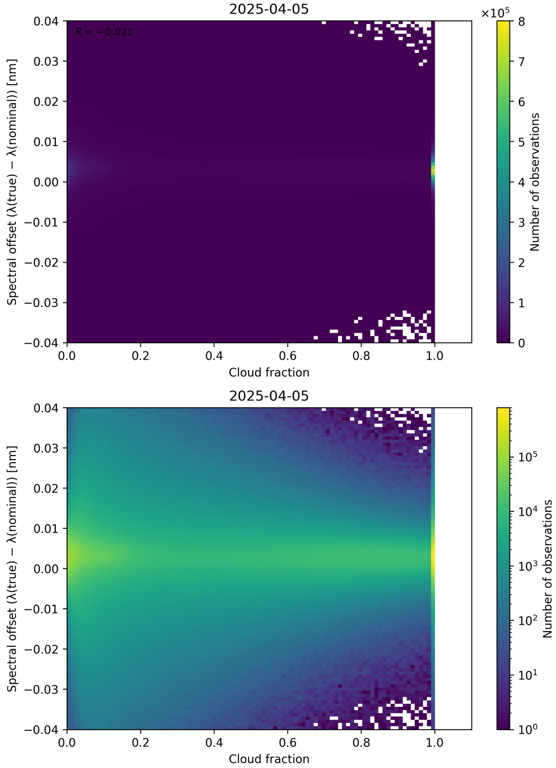
Figure 76: Scatter density plot of “Cloud fraction” against “Spectral offset ( \lambda_{\text{true}} - \lambda_{\text{nominal}} )” for 2025-04-04 to 2025-04-06.
