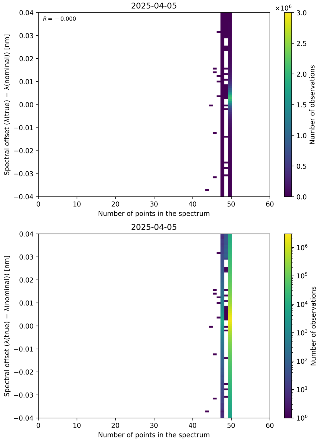
Figure 101: Scatter density plot of “Number of points in the spectrum” against “Spectral offset ( \lambda_{\text{true}} - \lambda_{\text{nominal}} )” for 2025-04-04 to 2025-04-06.
