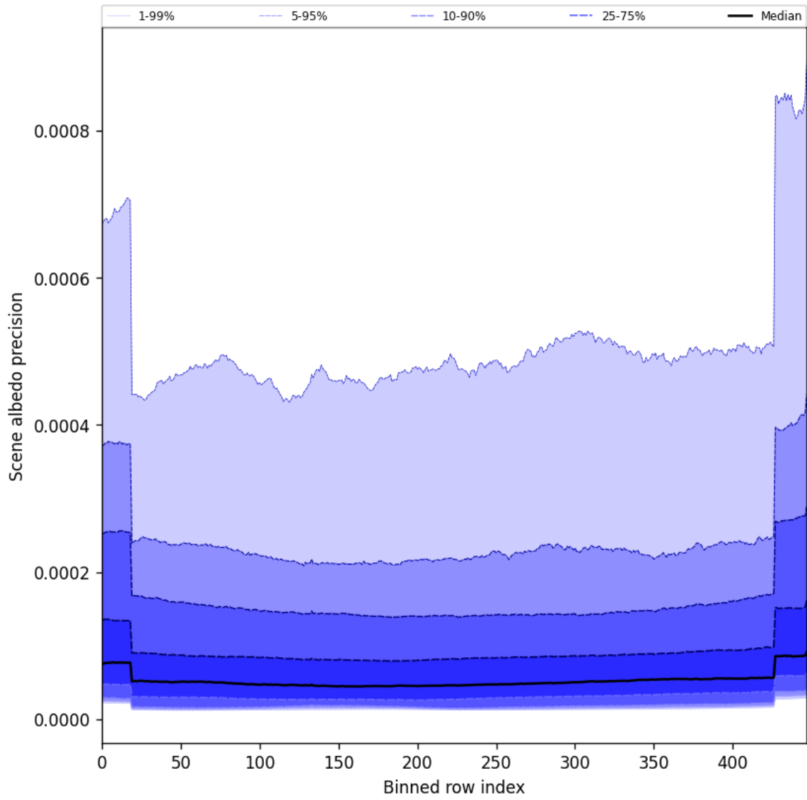
Figure 52: Along track statistics of “Scene albedo precision” for 2025-04-04 to 2025-04-06
