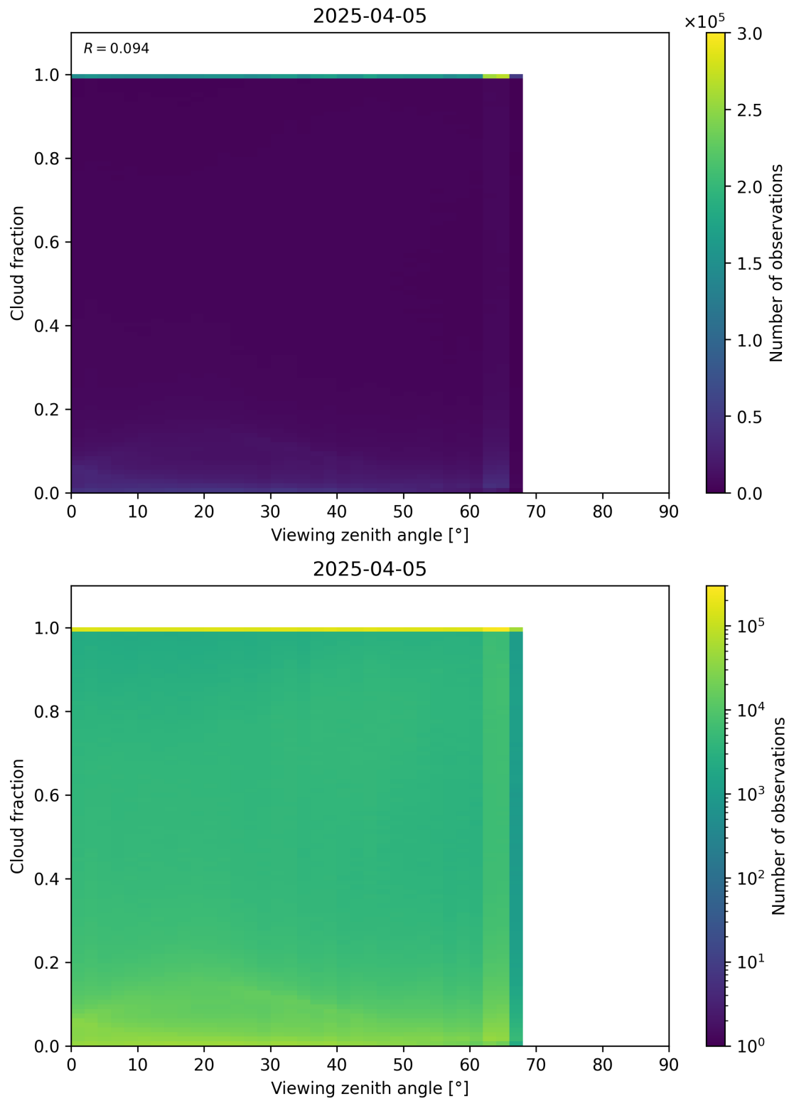
Figure 120: Scatter density plot of “Viewing zenith angle” against “Cloud fraction” for 2025-04-04 to 2025-04-06.
