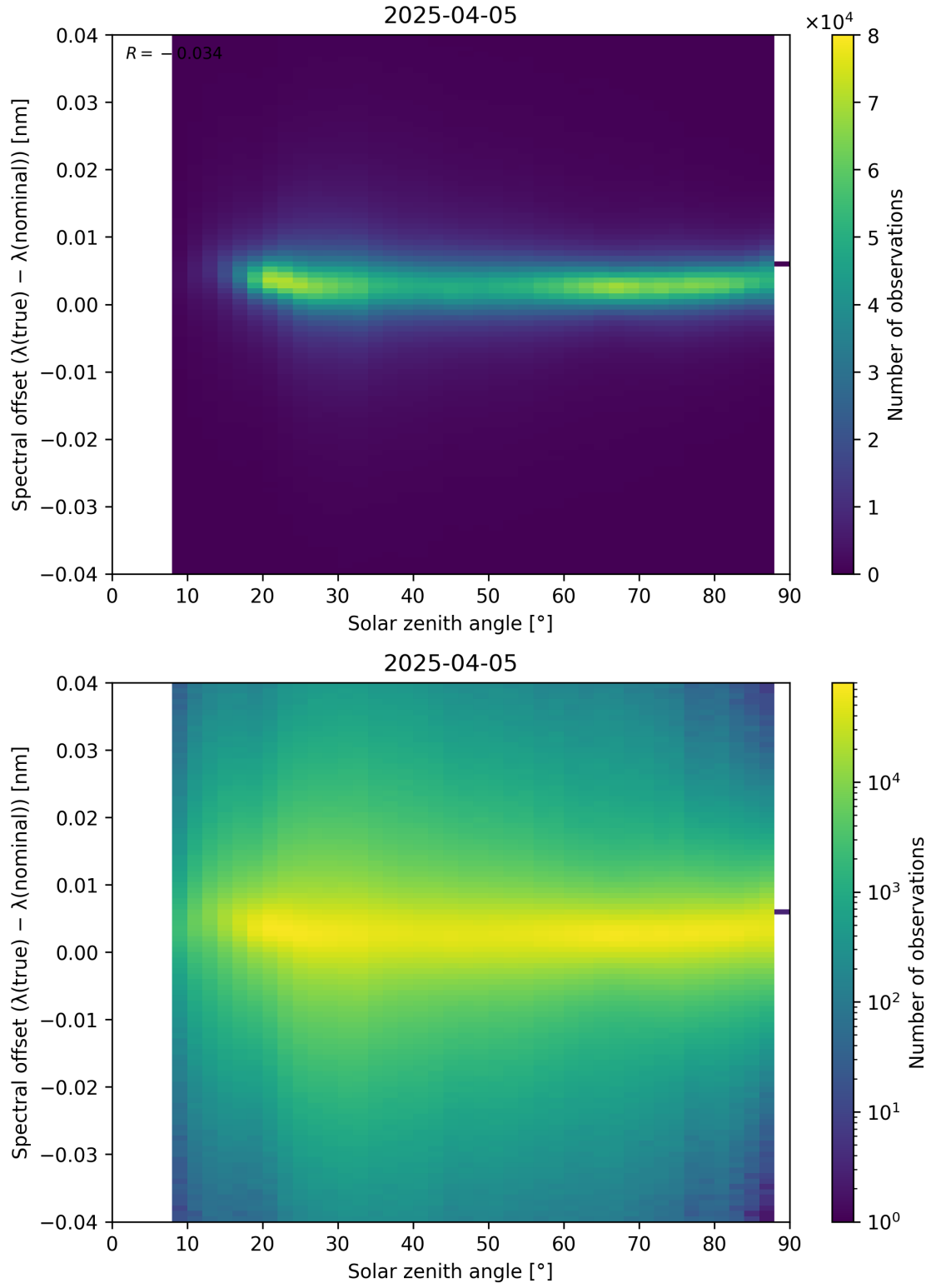
Figure 117: Scatter density plot of “Solar zenith angle” against “Spectral offset ( \lambda_{\text{true}} - \lambda_{\text{nominal}} )” for 2025-04-04 to 2025-04-06.
