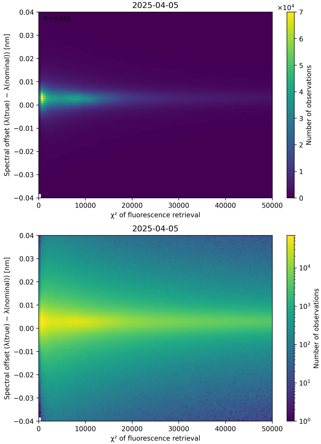
Figure 69: Scatter density plot of “ \chi^2 of fluorescence retrieval” against “Spectral offset ( \lambda_{\text{true}} - \lambda_{\text{nominal}} )” for 2025-04-04 to 2025-04-06.
