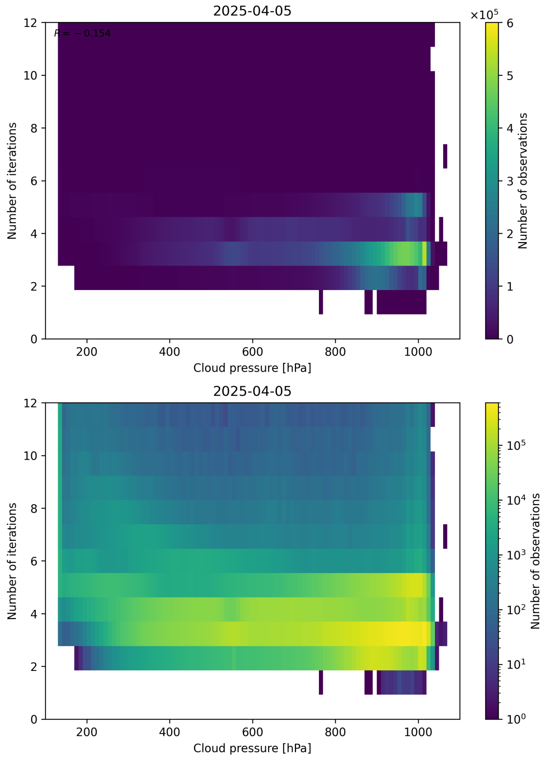
Figure 81: Scatter density plot of “Cloud pressure” against “Number of iterations” for 2025-04-04 to 2025-04-06.
