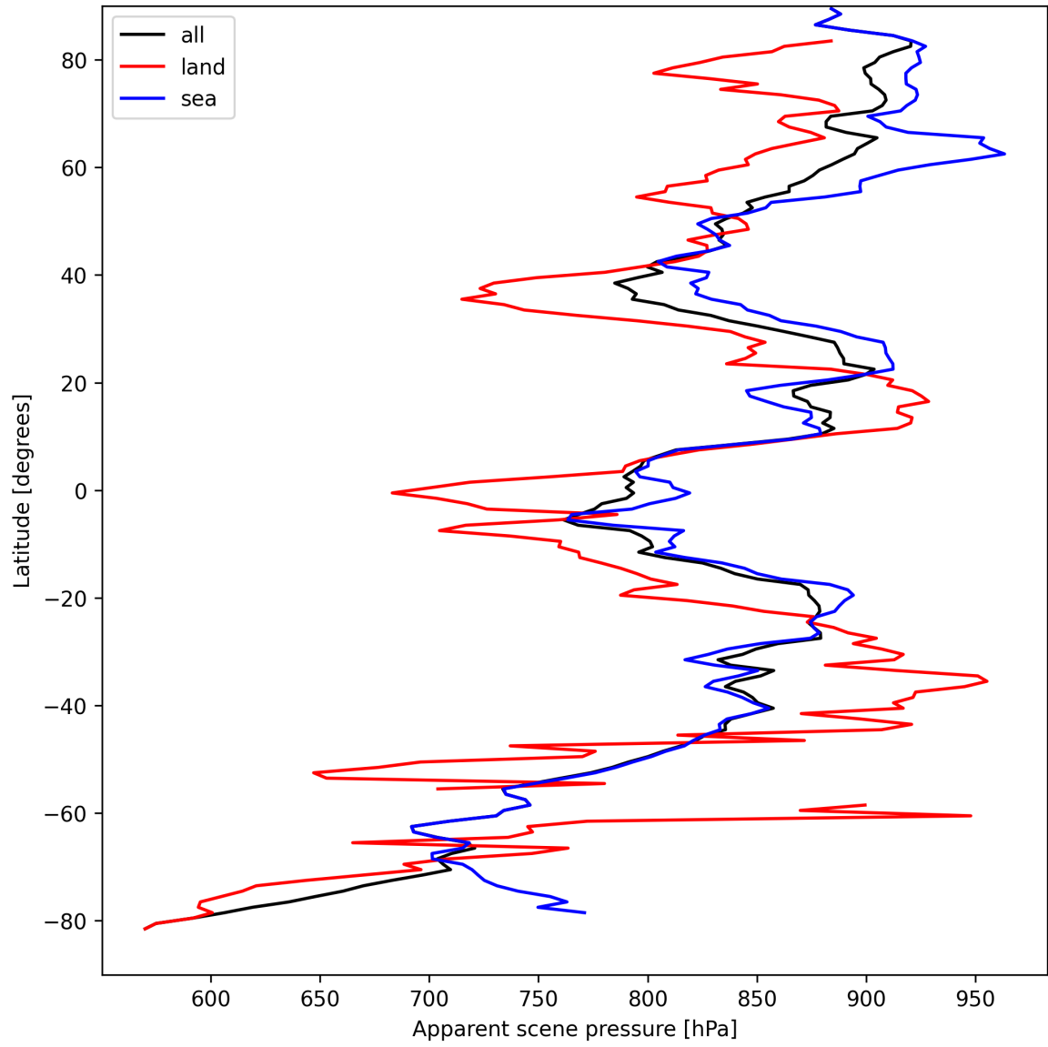
Figure 19: Zonal average of “Apparent scene pressure” for 2025-04-04 to 2025-04-06.
