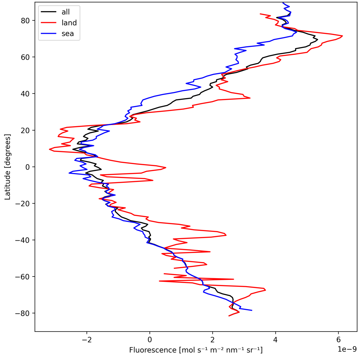
Figure 23: Zonal average of “Fluorescence” for 2025-04-04 to 2025-04-06.
