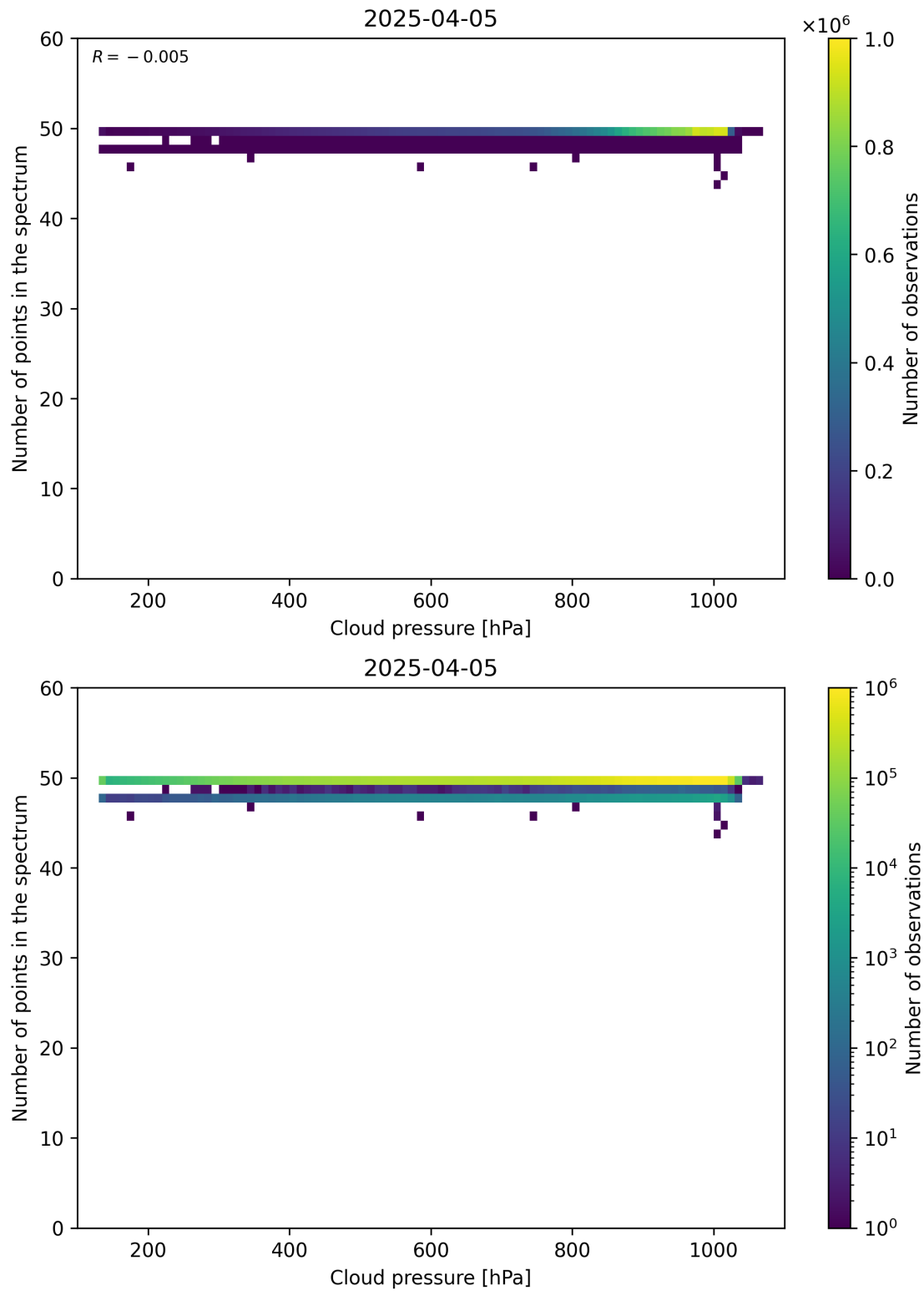
Figure 82: Scatter density plot of “Cloud pressure” against “Number of points in the spectrum” for 2025-04-04 to 2025-04-06.
