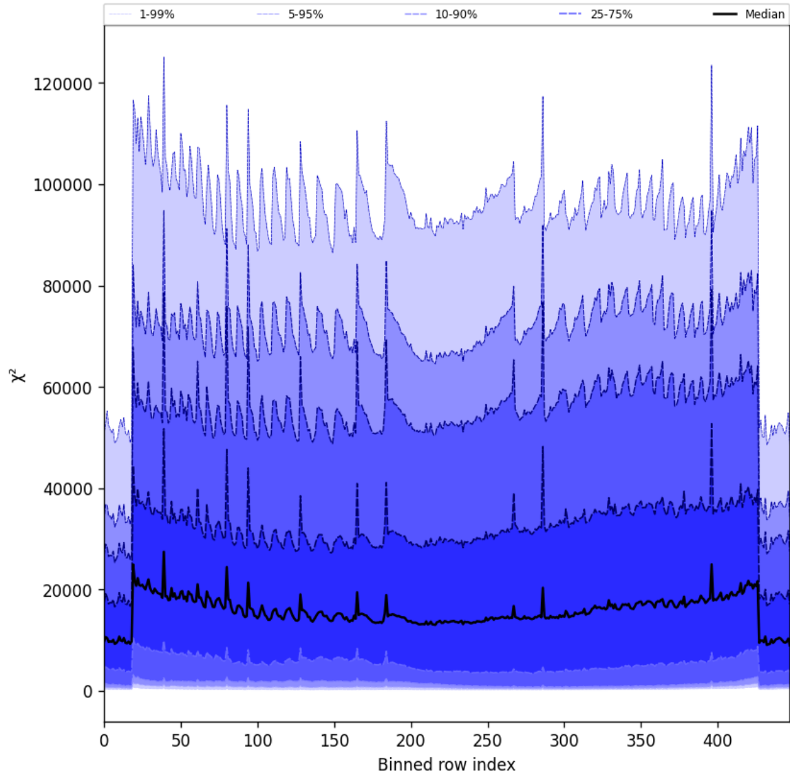
Figure 55: Along track statistics of “ \chi^2 ” for 2025-04-04 to 2025-04-06
