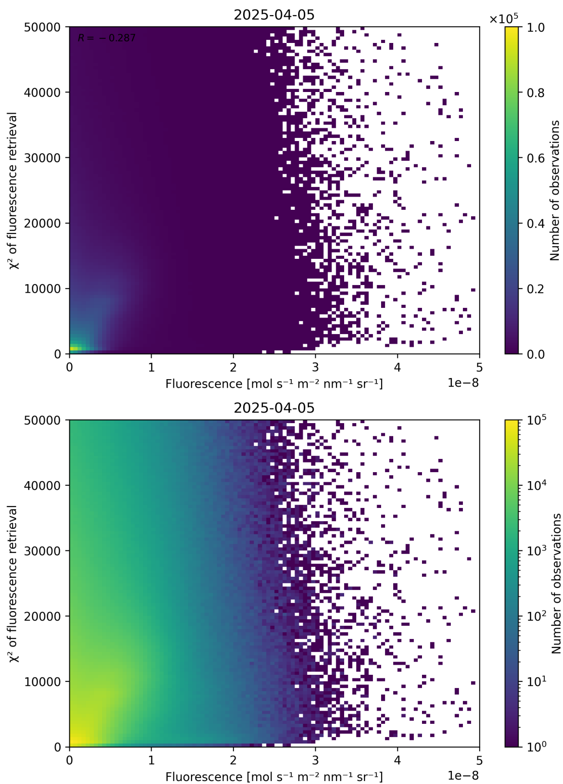
Figure 85: Scatter density plot of “Fluorescence” against “ \chi^2 of fluorescence retrieval” for 2025-04-04 to 2025-04-06.
