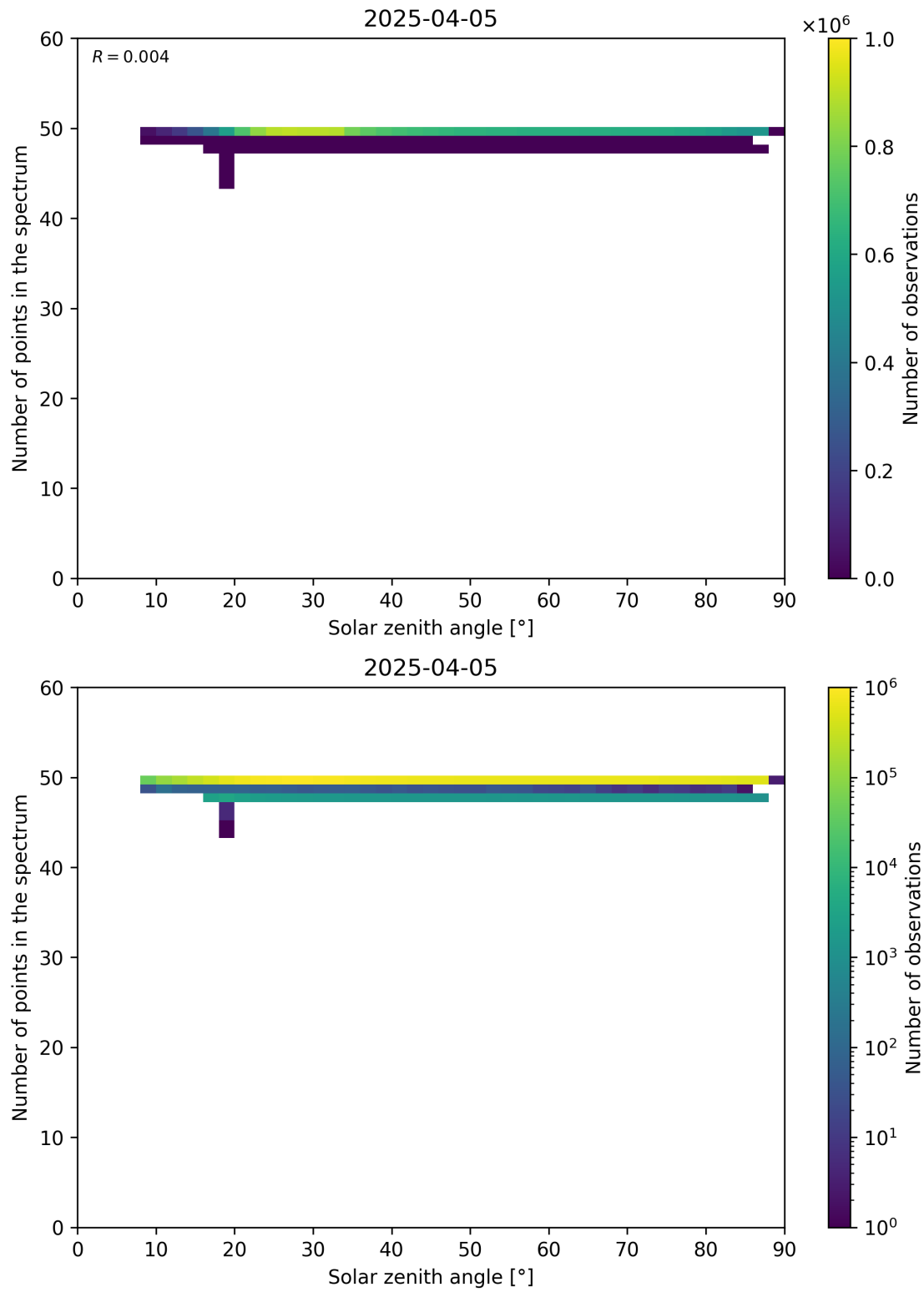
Figure 115: Scatter density plot of “Solar zenith angle” against “Number of points in the spectrum” for 2025-04-04 to 2025-04-06.
