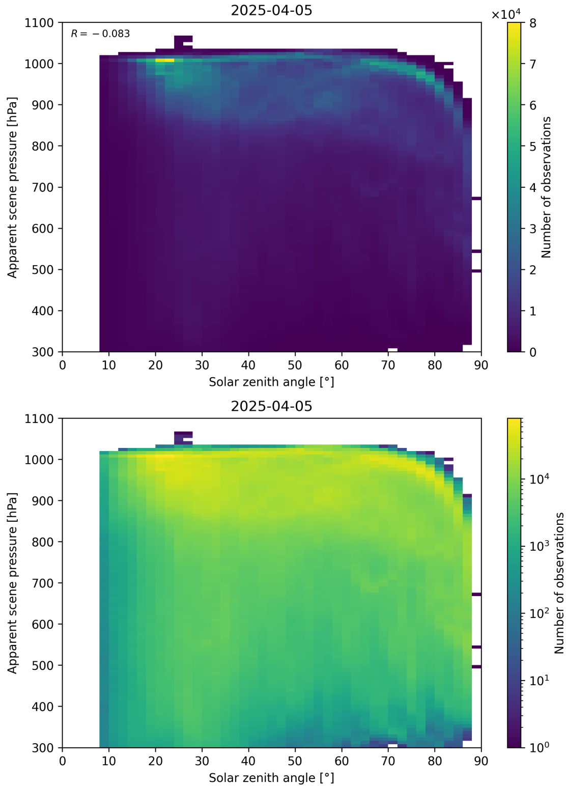
Figure 108: Scatter density plot of “Solar zenith angle” against “Apparent scene pressure” for 2025-04-04 to 2025-04-06.
