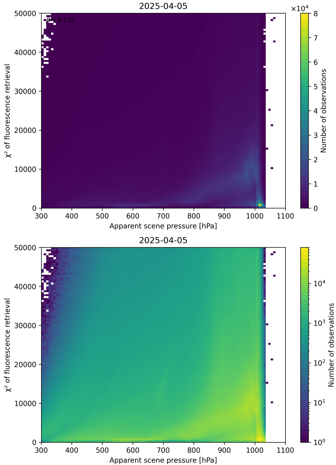
Figure 63: Scatter density plot of “Apparent scene pressure” against “ \chi^2 of fluorescence retrieval” for 2025-04-04 to 2025-04-06.
