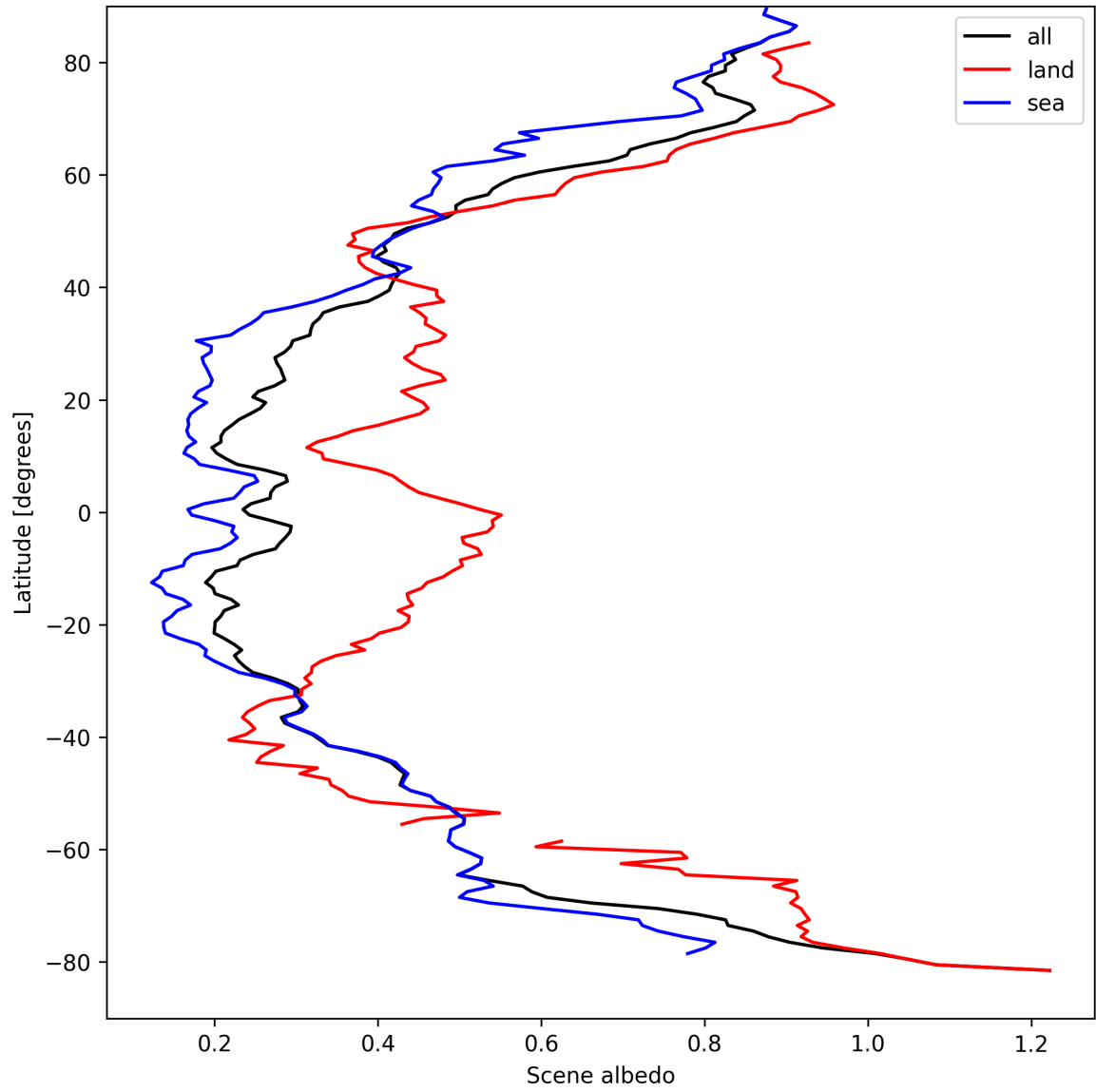
Figure 17: Zonal average of "Scene albedo" for 2025-04-04 to 2025-04-06.
