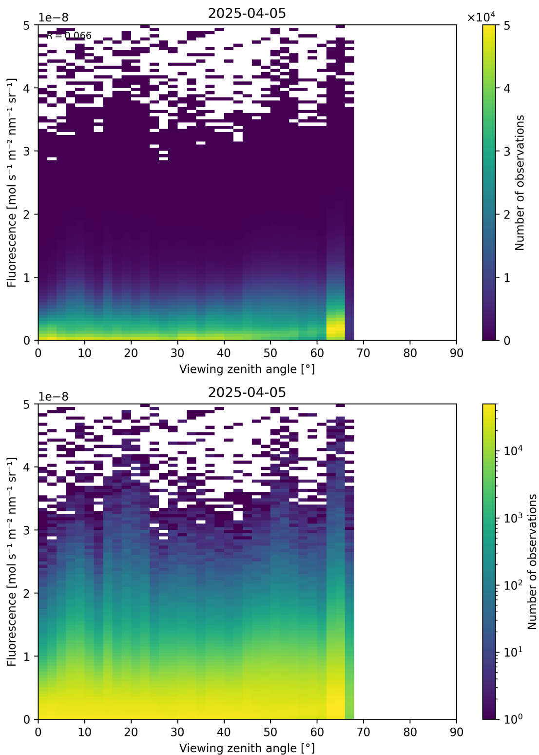
Figure 122: Scatter density plot of “Viewing zenith angle” against “Fluorescence” for 2025-04-04 to 2025-04-06.
