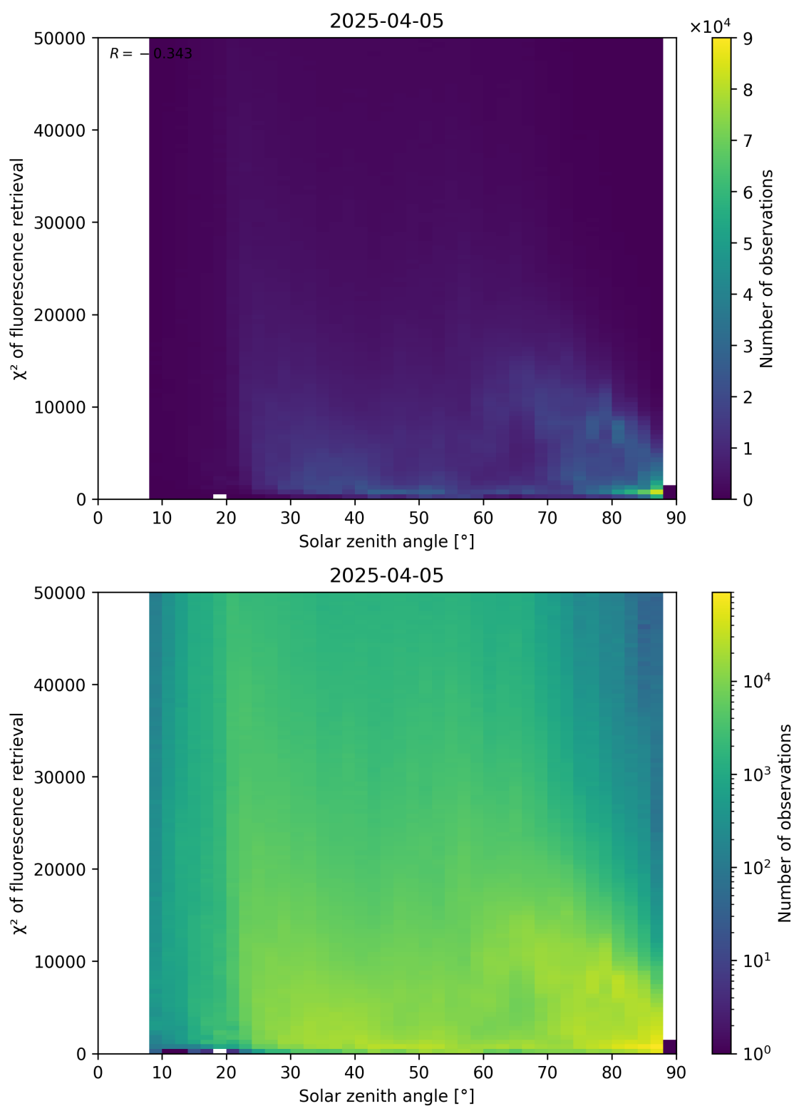
Figure 109: Scatter density plot of “Solar zenith angle” against “ \chi^2 of fluorescence retrieval” for 2025-04-04 to 2025-04-06.
