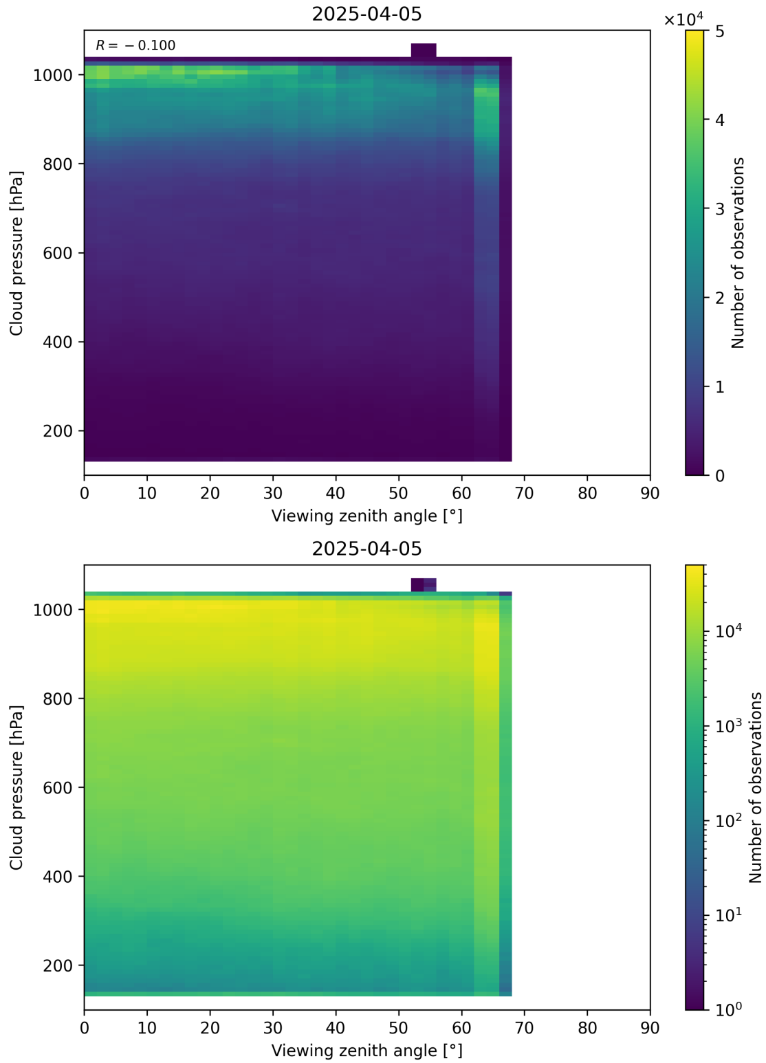
Figure 121: Scatter density plot of “Viewing zenith angle” against “Cloud pressure” for 2025-04-04 to 2025-04-06.
