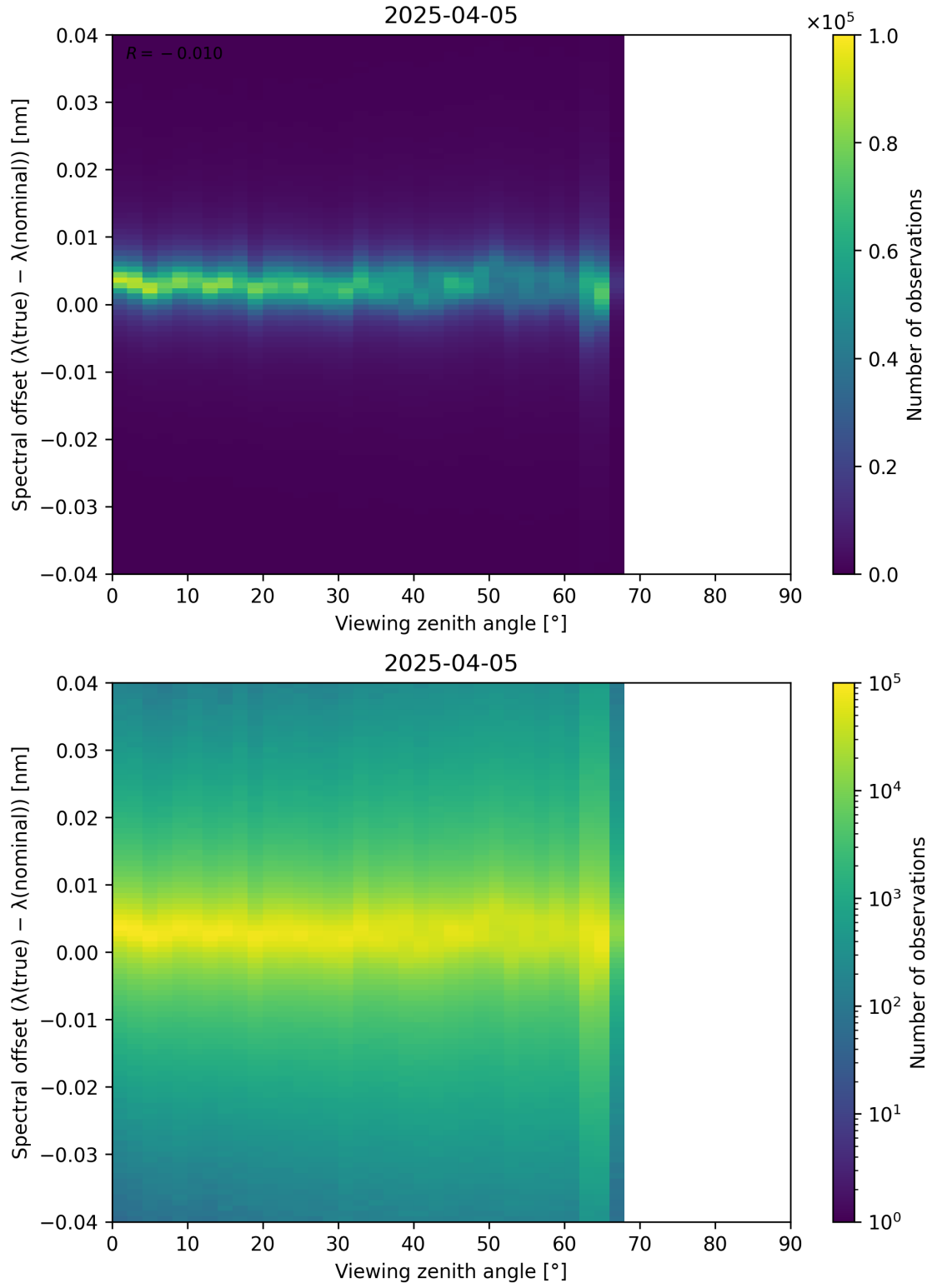
Figure 128: Scatter density plot of “Viewing zenith angle” against “Spectral offset ( \lambda_{\text{true}} - \lambda_{\text{nominal}} )” for 2025-04-04 to 2025-04-06.
