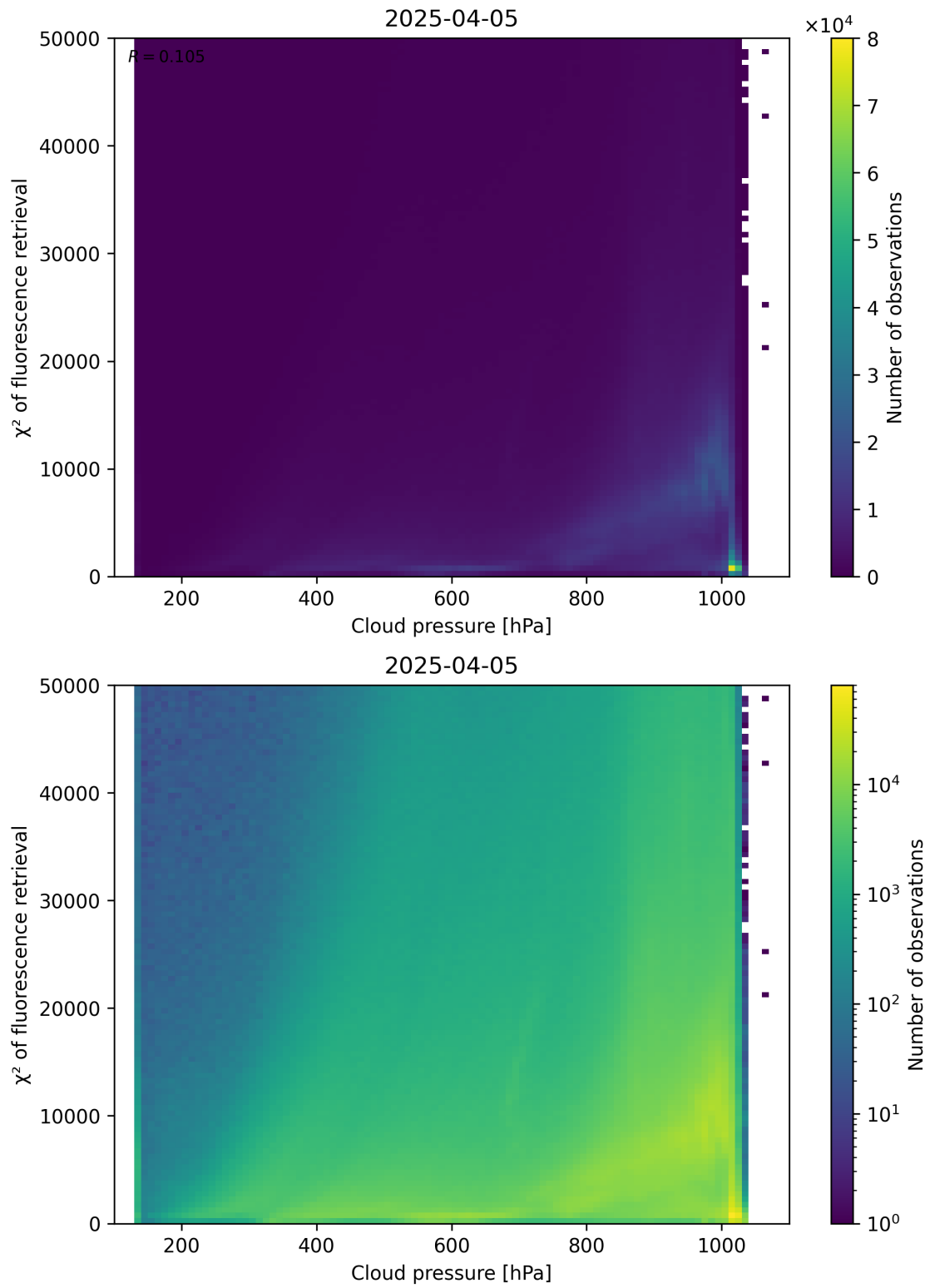
Figure 78: Scatter density plot of “Cloud pressure” against “ \chi^2 of fluorescence retrieval” for 2025-04-04 to 2025-04-06.
