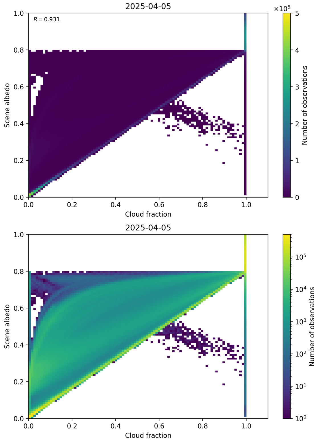
Figure 75: Scatter density plot of “Cloud fraction” against “Scene albedo” for 2025-04-04 to 2025-04-06.
