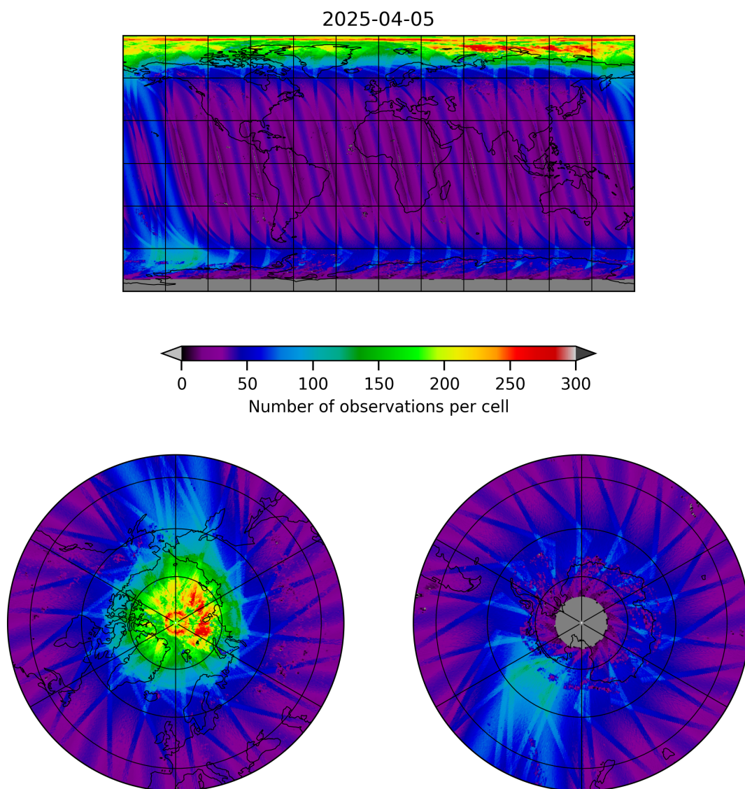
Figure 11: Map of the number of observations for 2025-04-04 to 2025-04-06
