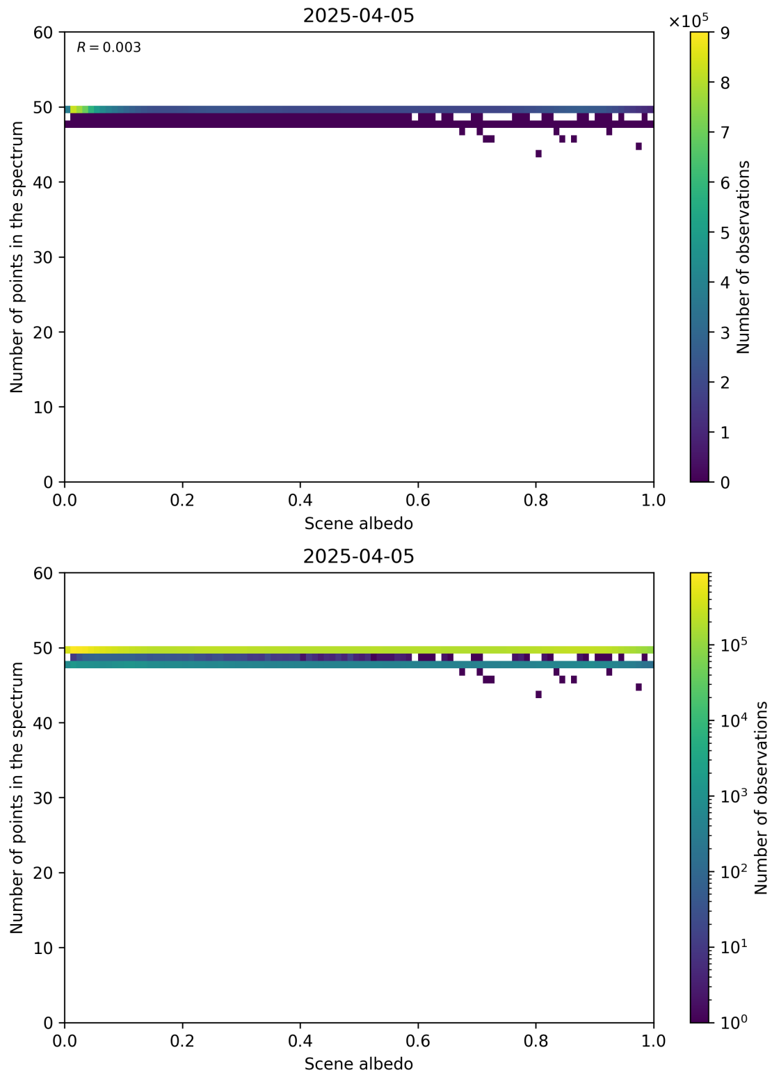
Figure 106: Scatter density plot of “Scene albedo” against “Number of points in the spectrum” for 2025-04-04 to 2025-04-06.
