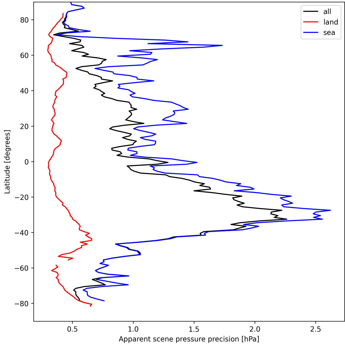
Figure 20: Zonal average of “Apparent scene pressure precision” for 2025-04-04 to 2025-04-06.
