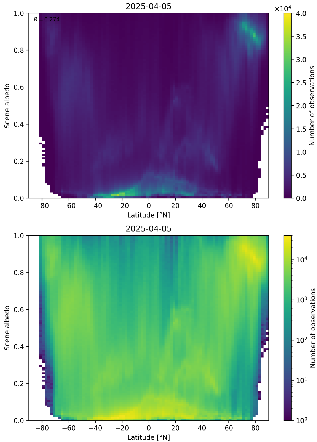
Figure 95: Scatter density plot of “Latitude” against “Scene albedo” for 2025-04-04 to 2025-04-06.
