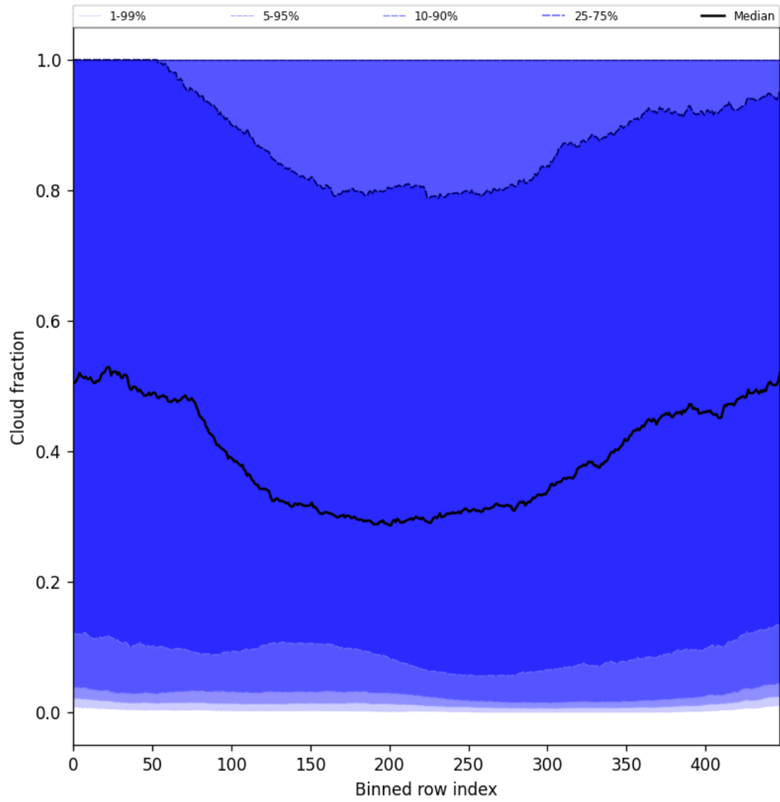
Figure 49: Along track statistics of “Cloud fraction” for 2025-04-04 to 2025-04-06
