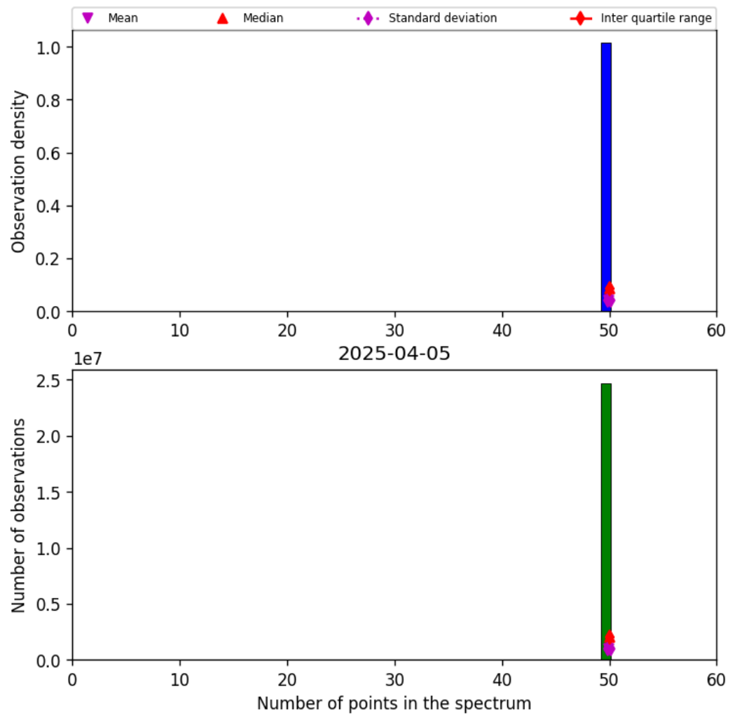
Figure 44: Histogram of “Number of points in the spectrum” for 2025-04-04 to 2025-04-06
