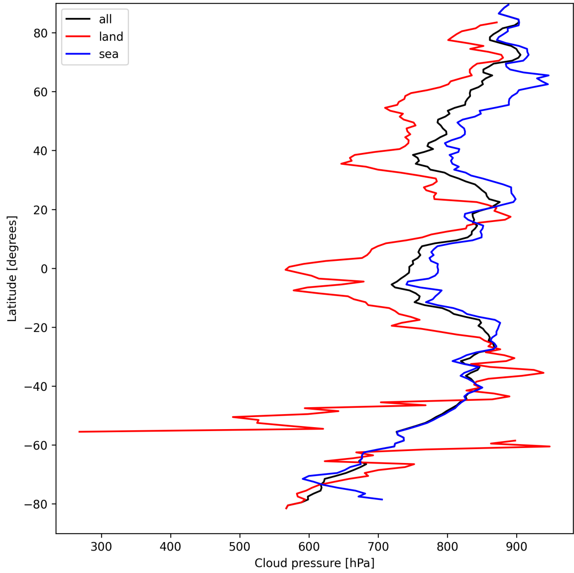
Figure 13: Zonal average of “Cloud pressure” for 2025-04-04 to 2025-04-06.
