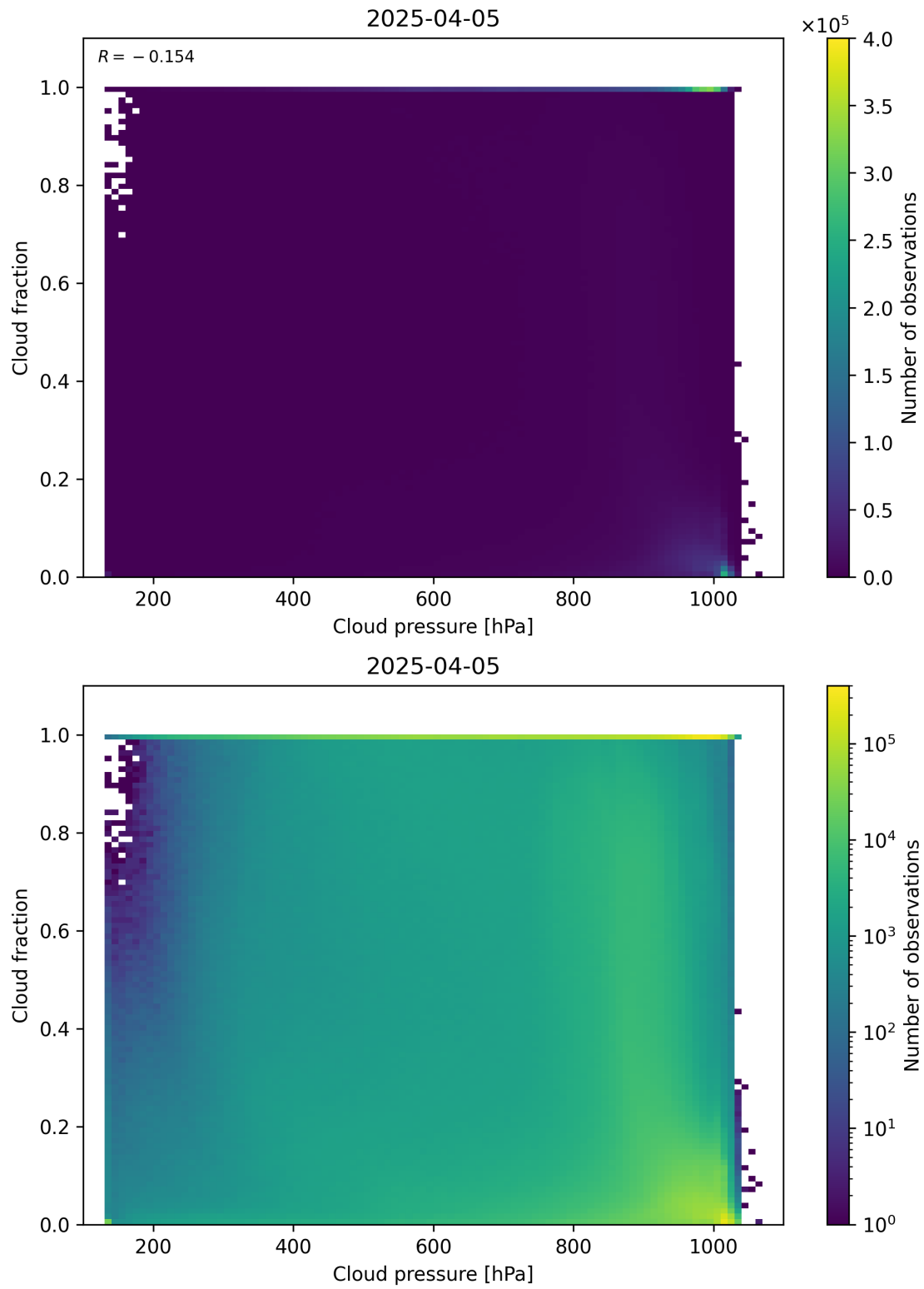
Figure 79: Scatter density plot of “Cloud pressure” against “Cloud fraction” for 2025-04-04 to 2025-04-06.
