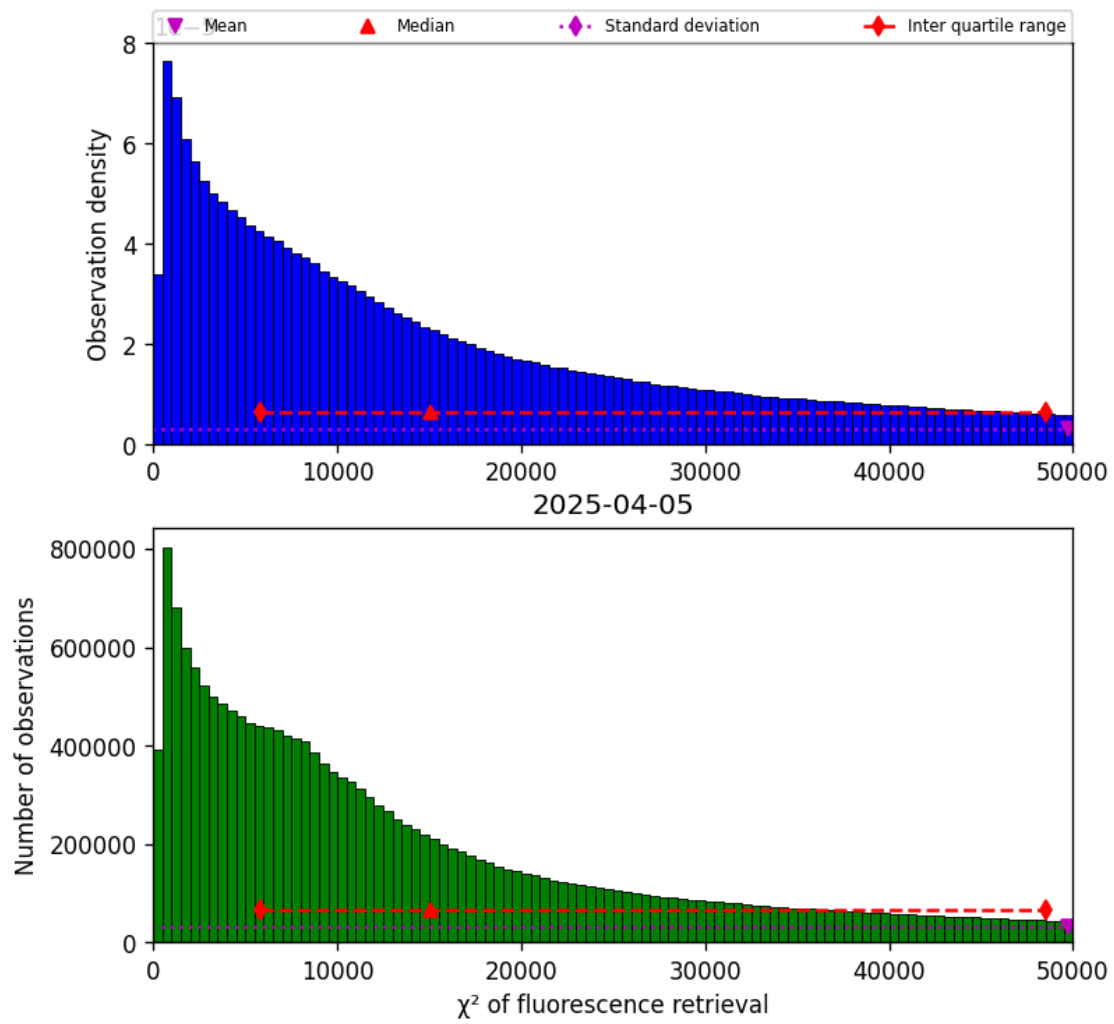
Figure 42: Histogram of “ \chi^2 of fluorescence retrieval” for 2025-04-04 to 2025-04-06
