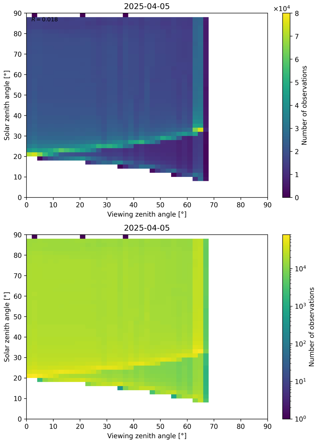
Figure 127: Scatter density plot of “Viewing zenith angle” against “Solar zenith angle” for 2025-04-04 to 2025-04-06.
