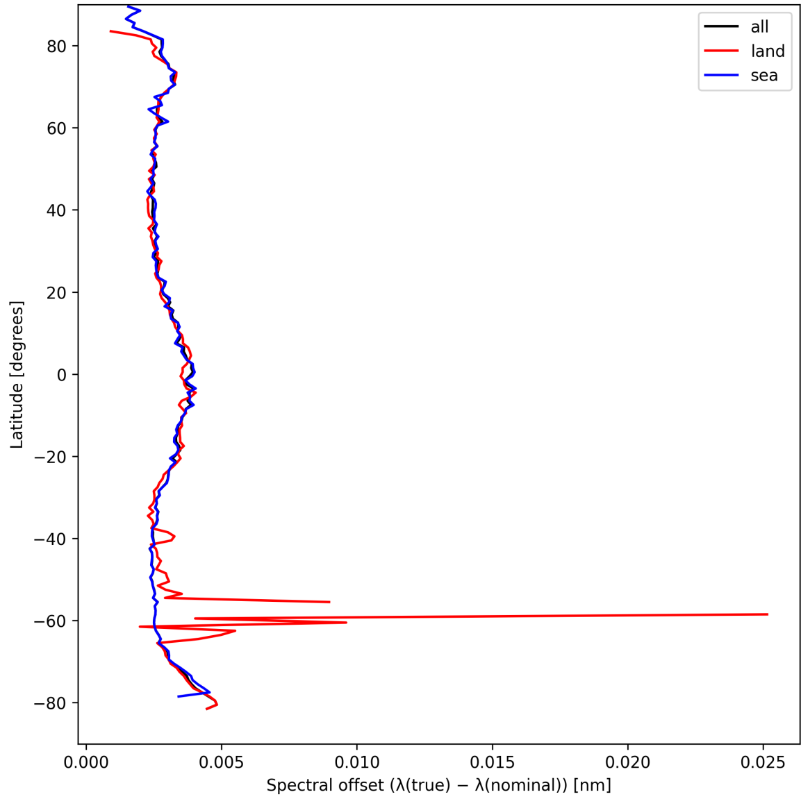
Figure 28: Zonal average of “Spectral offset ( \lambda_{\text{true}} - \lambda_{\text{nominal}} )” for 2025-04-04 to 2025-04-06.
