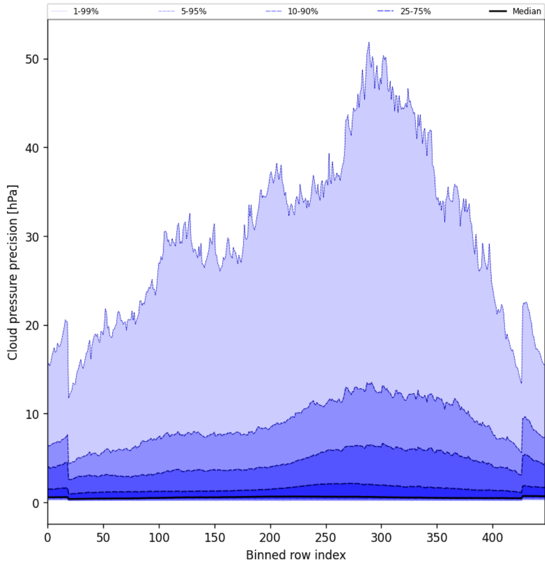
Figure 48: Along track statistics of “Cloud pressure precision” for 2025-04-04 to 2025-04-06
