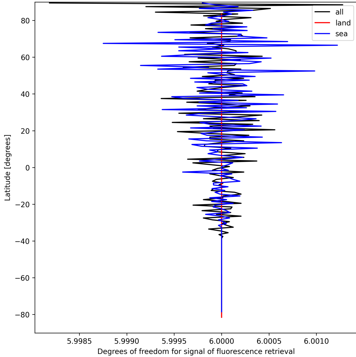
Figure 26: Zonal average of “Degrees of freedom for signal of fluorescence retrieval” for 2025-04-04 to 2025-04-06.
