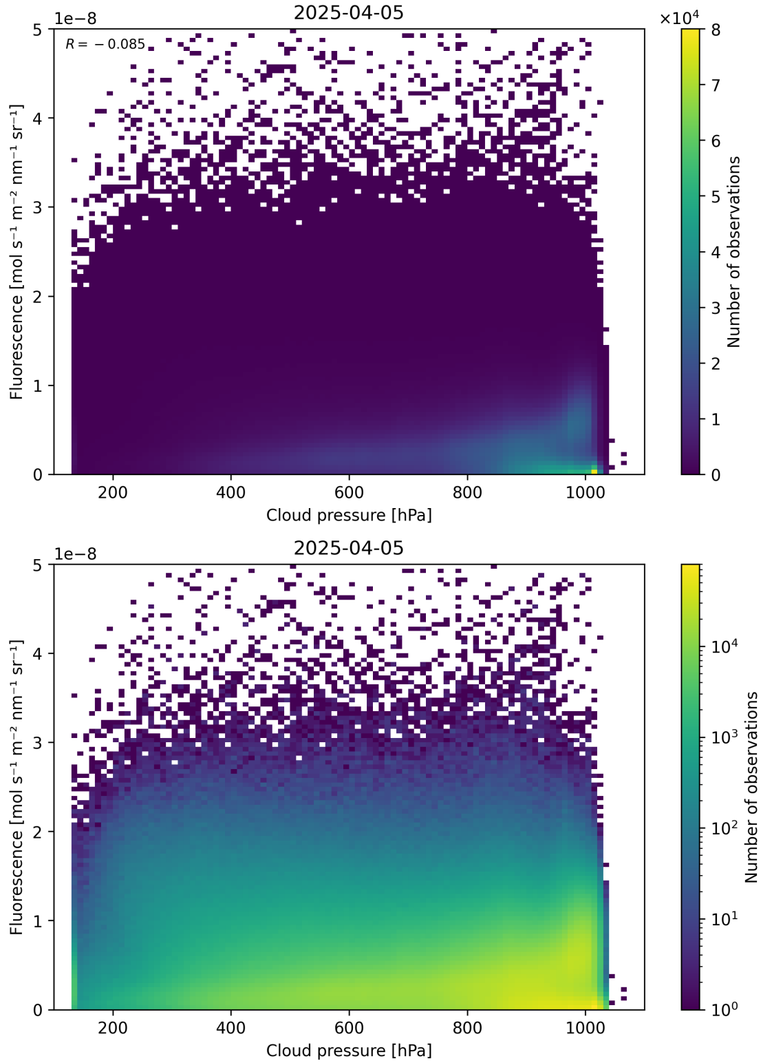
Figure 80: Scatter density plot of “Cloud pressure” against “Fluorescence” for 2025-04-04 to 2025-04-06.
