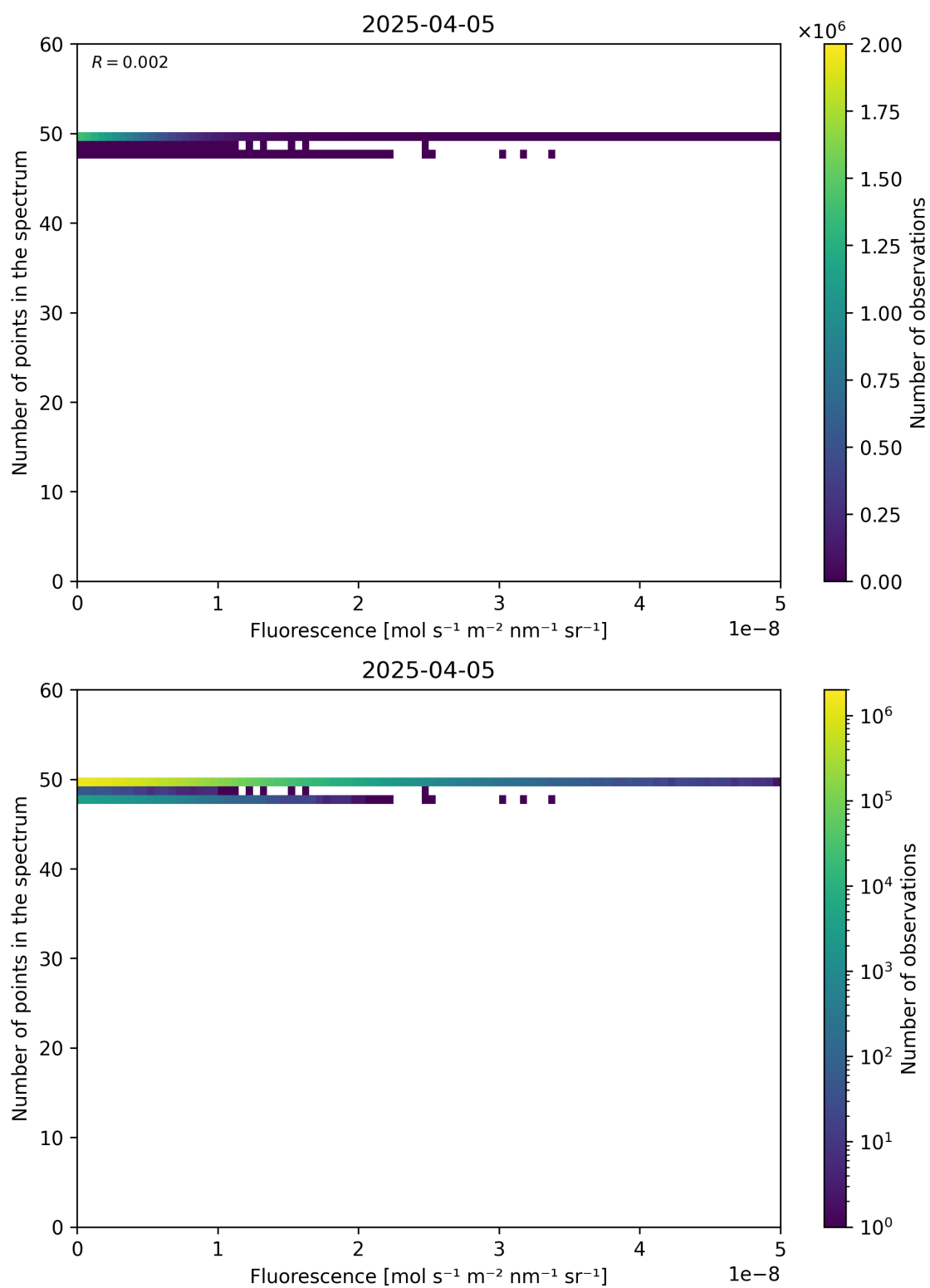
Figure 86: Scatter density plot of “Fluorescence” against “Number of points in the spectrum” for 2025-04-04 to 2025-04-06.
