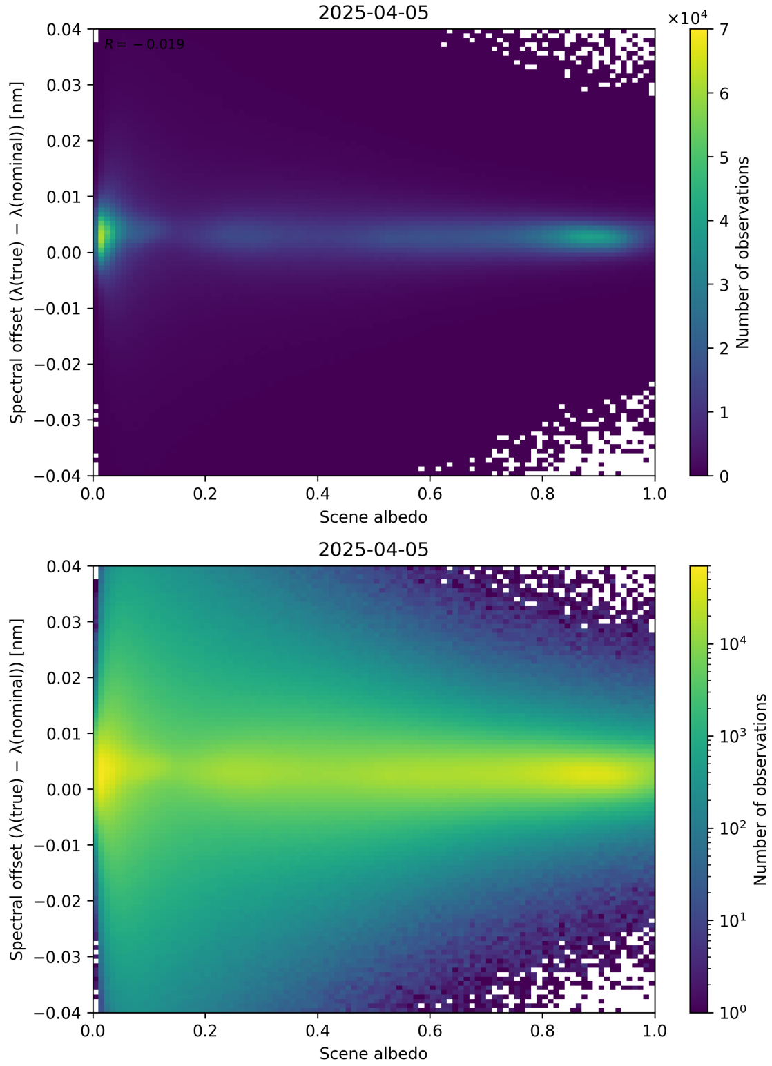
Figure 107: Scatter density plot of “Scene albedo” against “Spectral offset ( \lambda_{\text{true}} - \lambda_{\text{nominal}} )” for 2025-04-04 to 2025-04-06.
