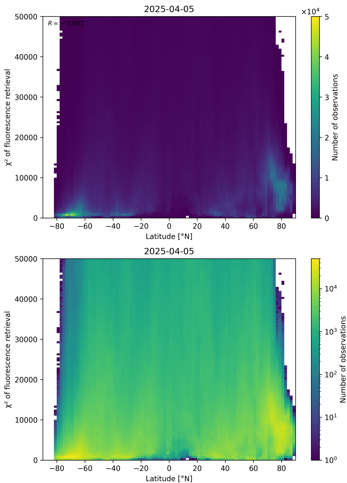
Figure 89: Scatter density plot of “Latitude” against “ \chi^2 of fluorescence retrieval” for 2025-04-04 to 2025-04-06.
