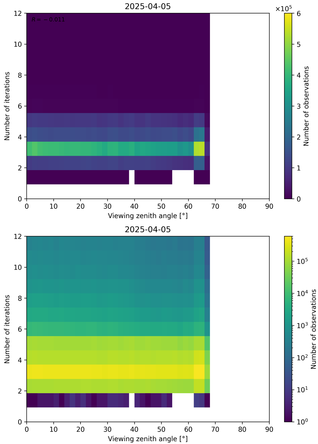
Figure 124: Scatter density plot of “Viewing zenith angle” against “Number of iterations” for 2025-04-04 to 2025-04-06.
