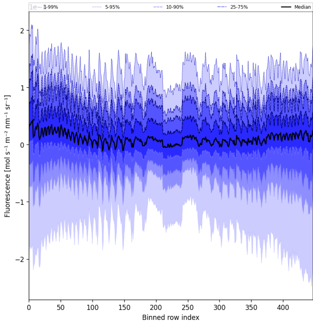
Figure 57: Along track statistics of “Fluorescence” for 2025-04-04 to 2025-04-06
