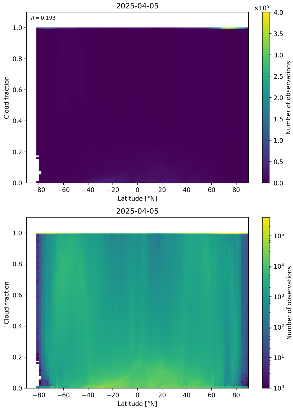
Figure 90: Scatter density plot of “Latitude” against “Cloud fraction” for 2025-04-04 to 2025-04-06.
