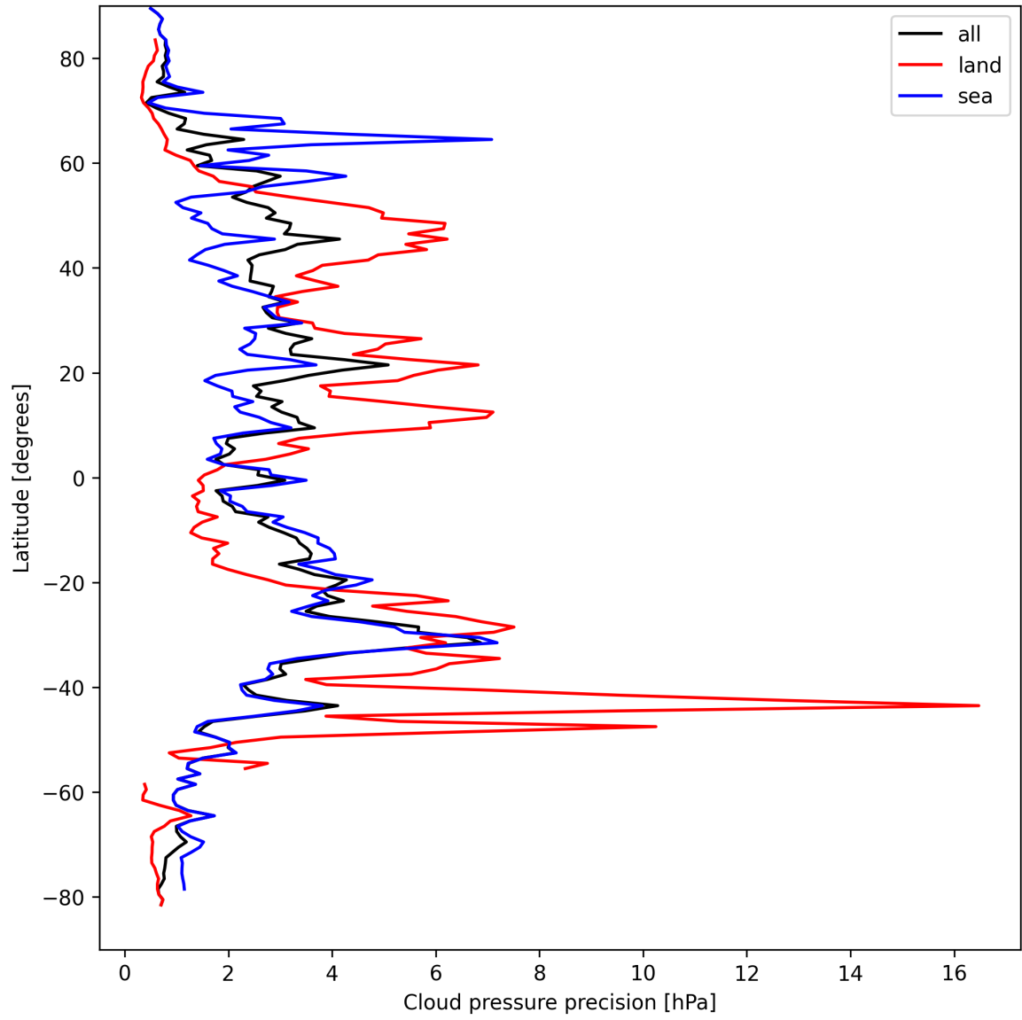
Figure 14: Zonal average of “Cloud pressure precision” for 2025-04-04 to 2025-04-06.
