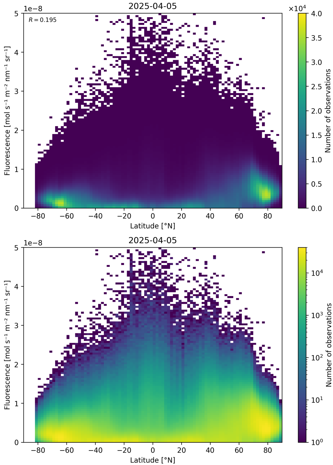
Figure 92: Scatter density plot of “Latitude” against “Fluorescence” for 2025-04-04 to 2025-04-06.
