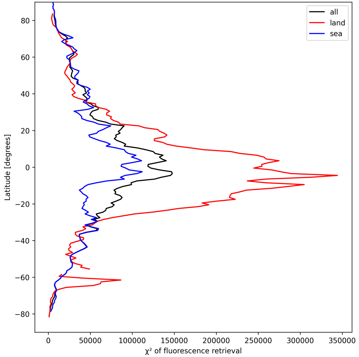
Figure 25: Zonal average of “ \chi^2 of fluorescence retrieval” for 2025-04-04 to 2025-04-06.
