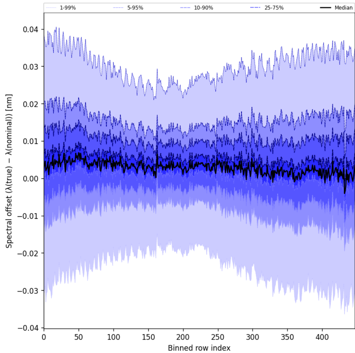
Figure 62: Along track statistics of “Spectral offset ( \lambda_{\text{true}} - \lambda_{\text{nominal}} )” for 2025-04-04 to 2025-04-06
