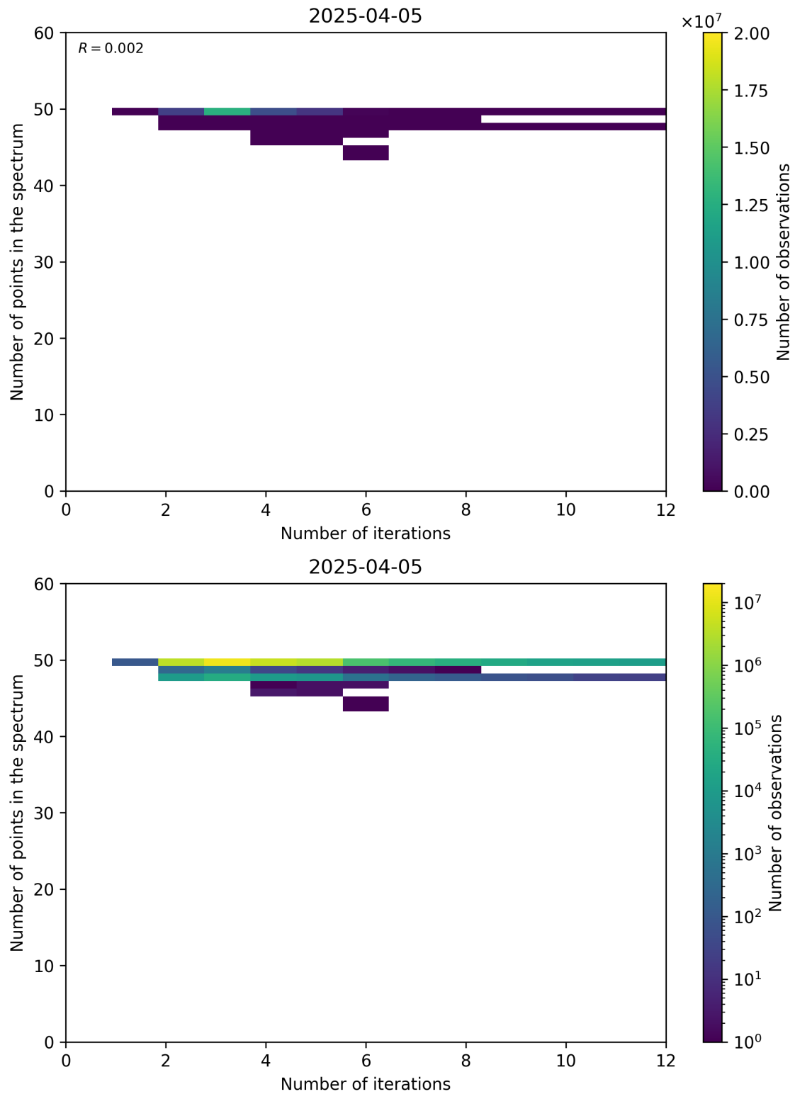
Figure 99: Scatter density plot of “Number of iterations” against “Number of points in the spectrum” for 2025-04-04 to 2025-04-06.
