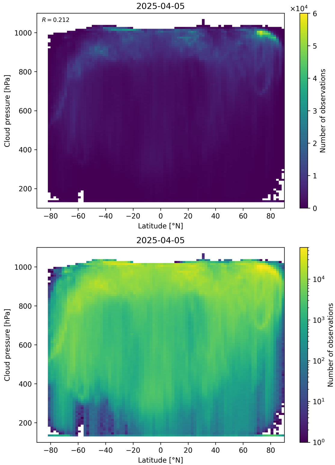
Figure 91: Scatter density plot of “Latitude” against “Cloud pressure” for 2025-04-04 to 2025-04-06.
