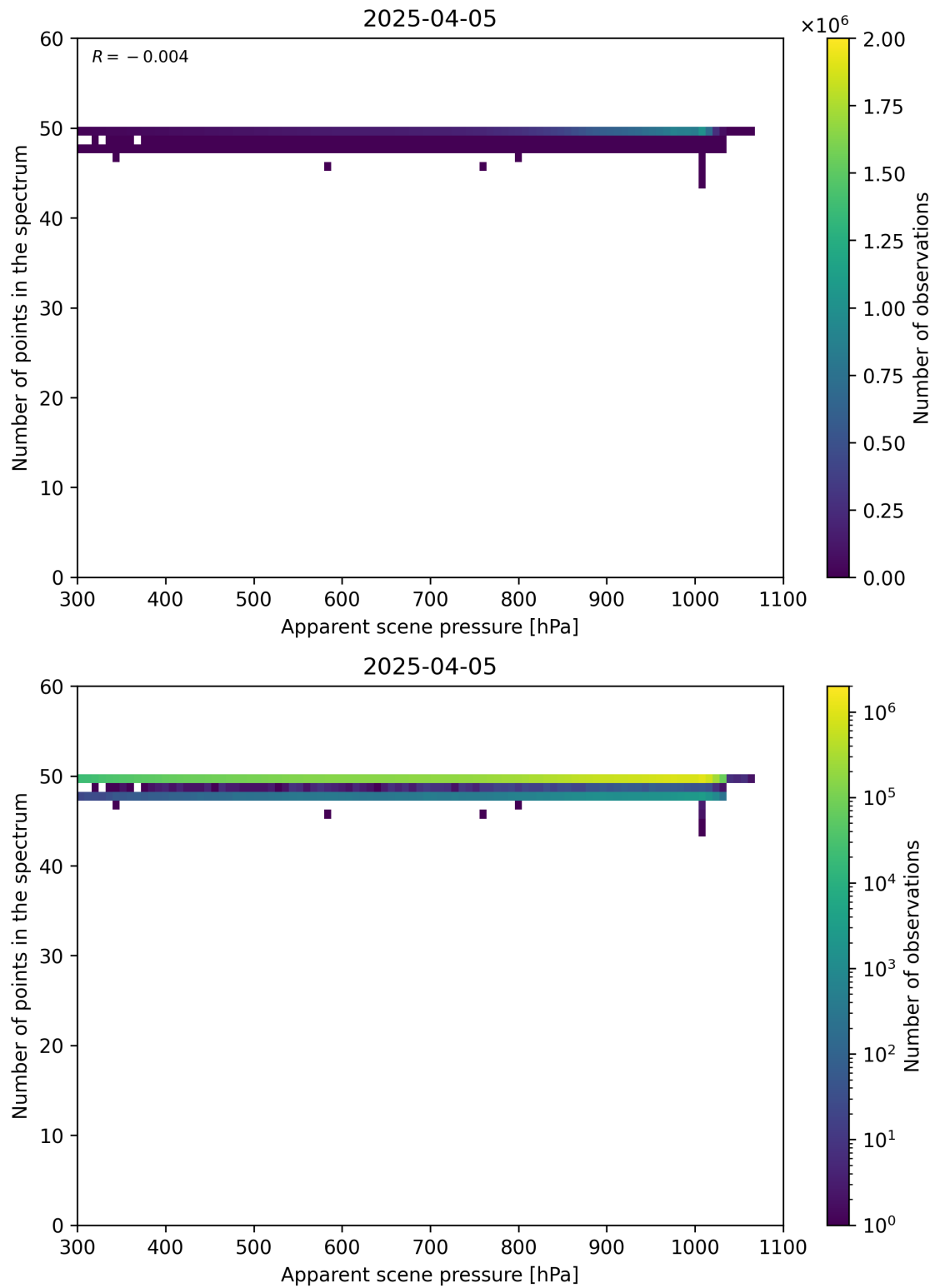
Figure 66: Scatter density plot of “Apparent scene pressure” against “Number of points in the spectrum” for 2025-04-04 to 2025-04-06.
