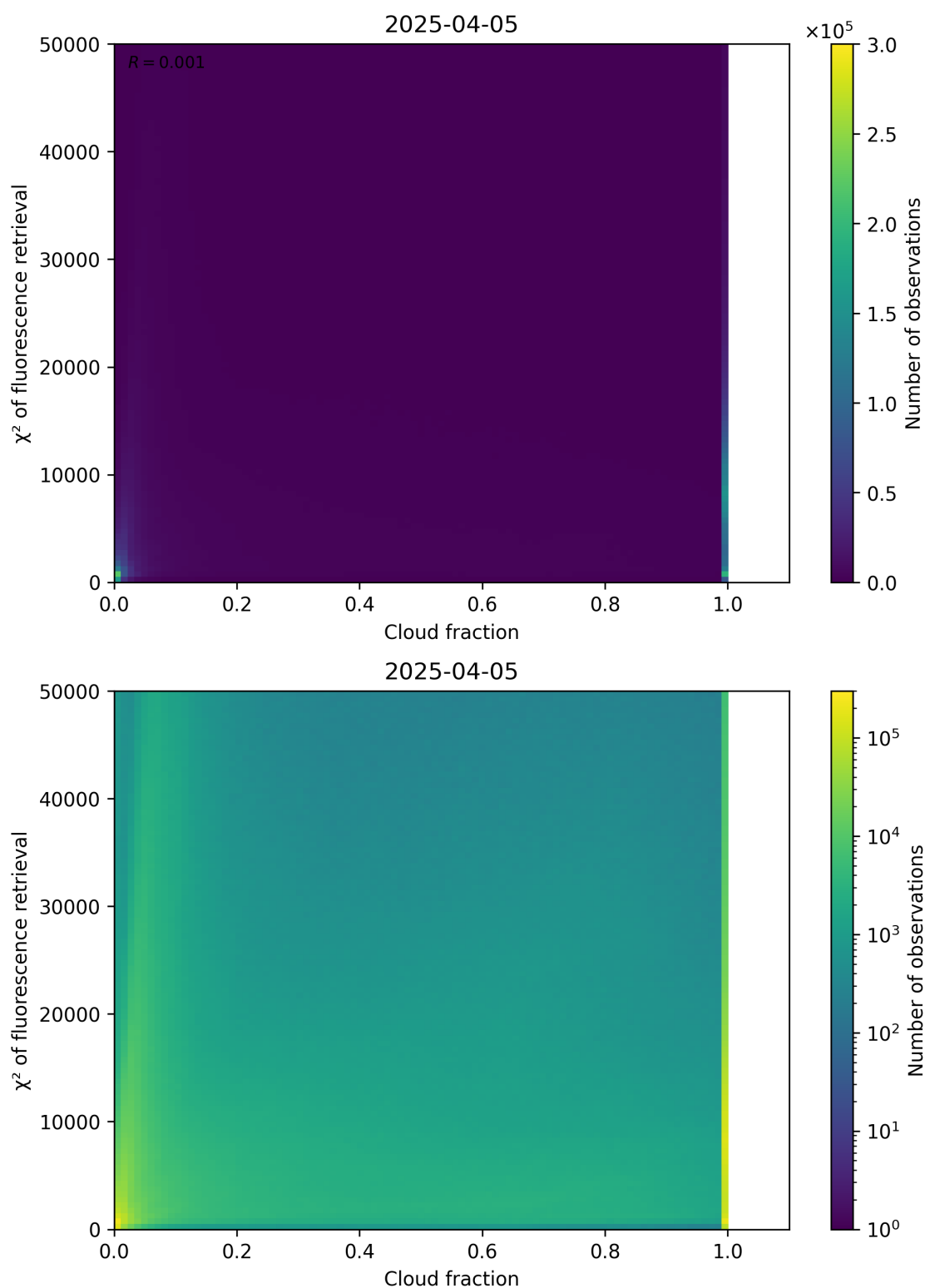
Figure 71: Scatter density plot of “Cloud fraction” against “ \chi^2 of fluorescence retrieval” for 2025-04-04 to 2025-04-06.
