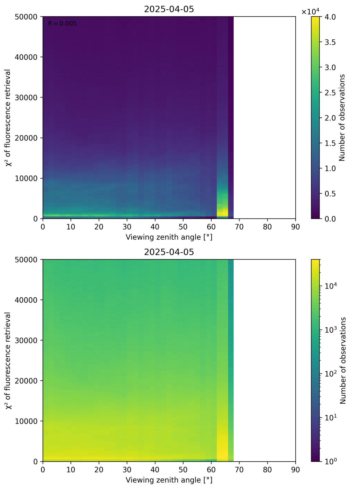
Figure 119: Scatter density plot of “Viewing zenith angle” against “ \chi^2 of fluorescence retrieval” for 2025-04-04 to 2025-04-06.
