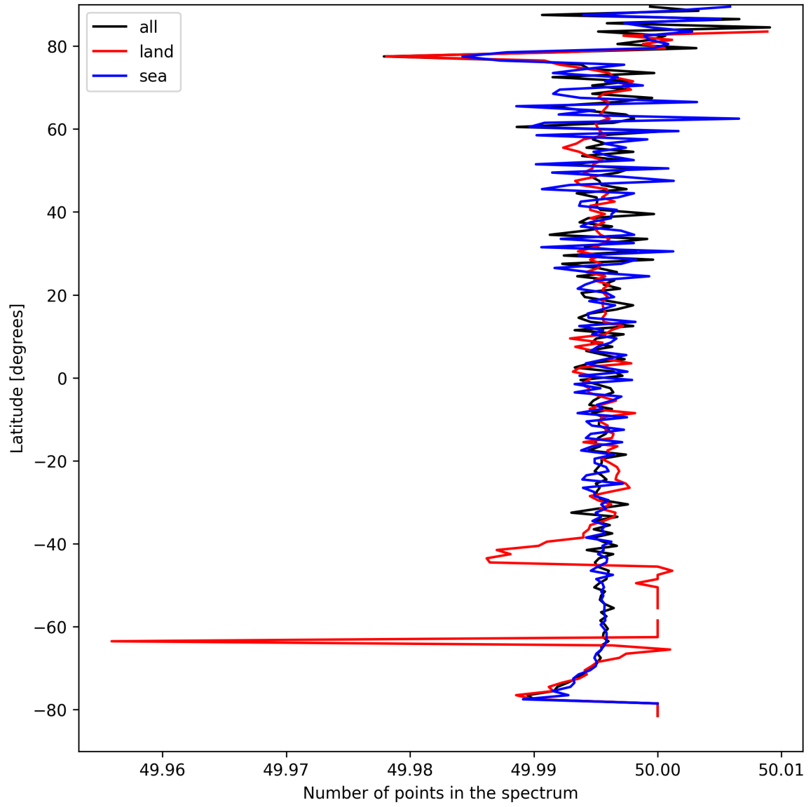
Figure 27: Zonal average of “Number of points in the spectrum” for 2025-04-04 to 2025-04-06.
