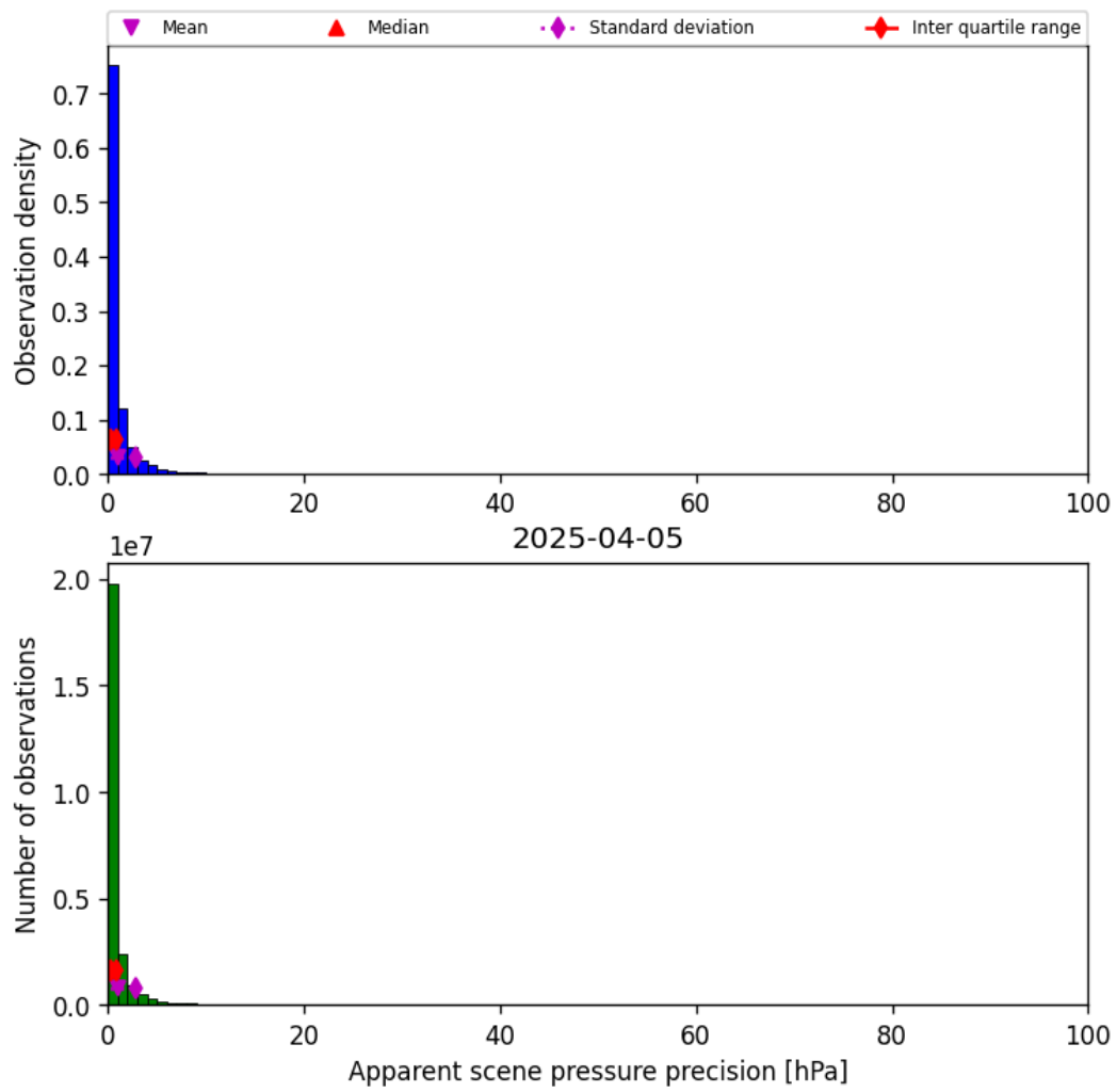
Figure 37: Histogram of “Apparent scene pressure precision” for 2025-04-04 to 2025-04-06
