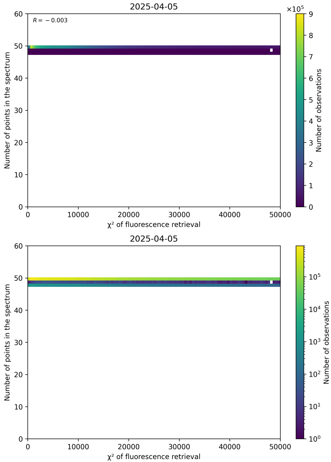
Figure 68: Scatter density plot of “ \chi^2 of fluorescence retrieval” against “Number of points in the spectrum” for 2025-04-04 to 2025-04-06.
