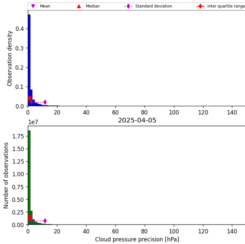
Figure 31: Histogram of “Cloud pressure precision” for 2025-04-04 to 2025-04-06
