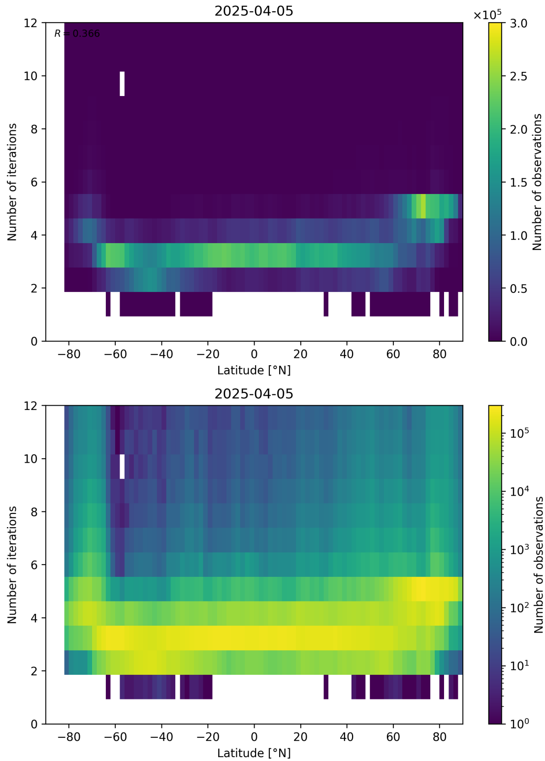
Figure 93: Scatter density plot of “Latitude” against “Number of iterations” for 2025-04-04 to 2025-04-06.
