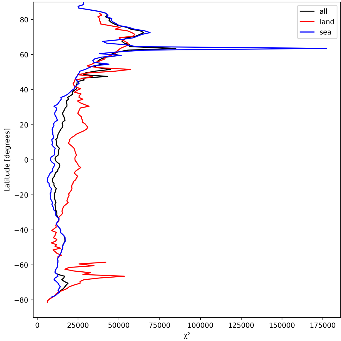
Figure 21: Zonal average of “ \chi^2 ” for 2025-04-04 to 2025-04-06.
