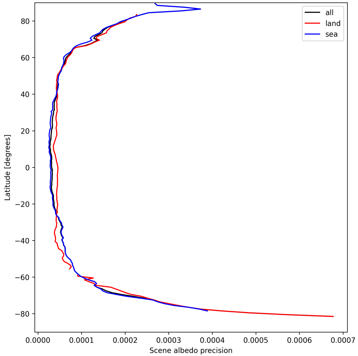
Figure 18: Zonal average of “Scene albedo precision” for 2025-04-04 to 2025-04-06.
