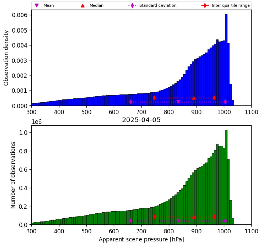
Figure 36: Histogram of “Apparent scene pressure” for 2025-04-04 to 2025-04-06
