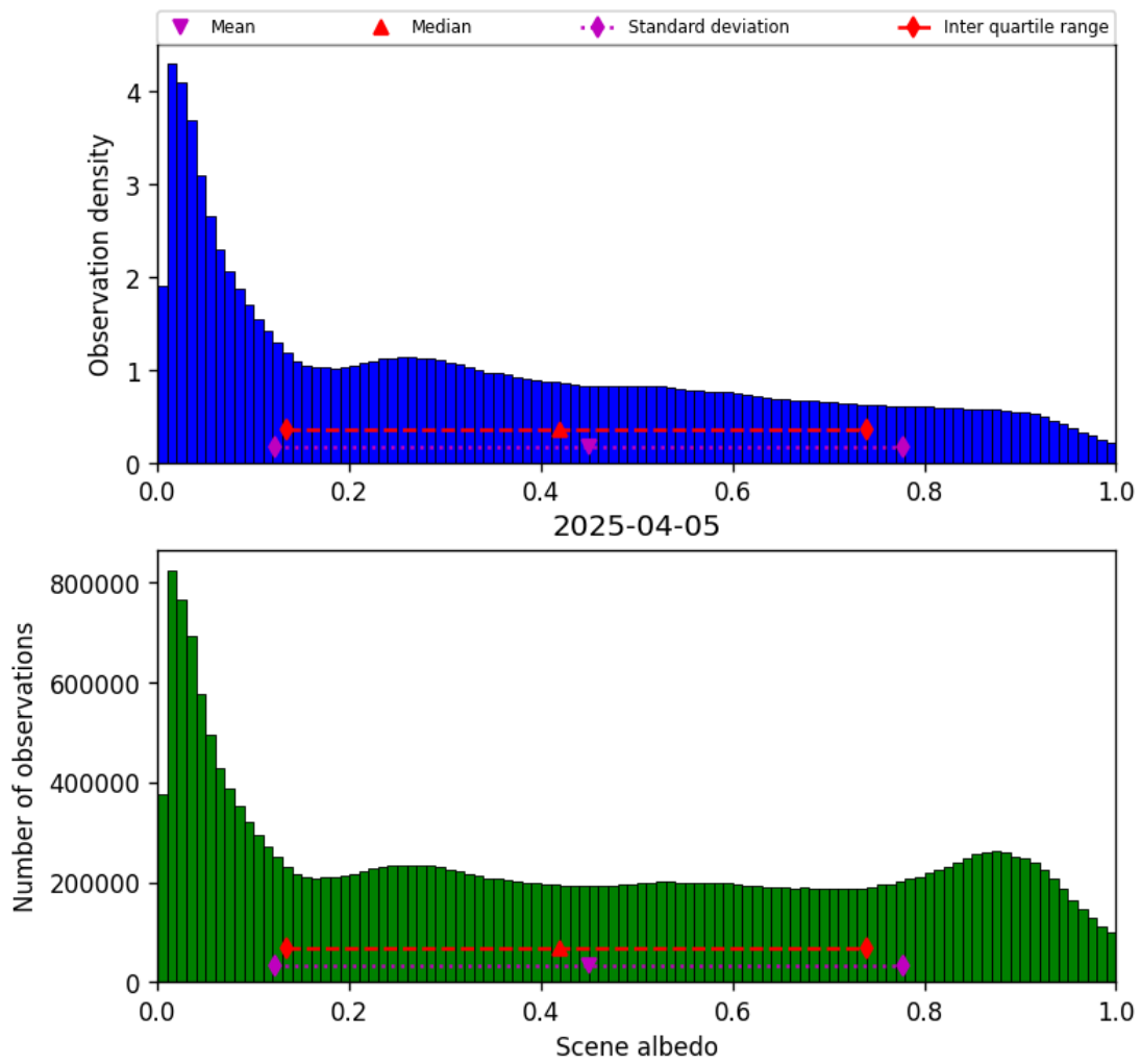
Figure 34: Histogram of “Scene albedo” for 2025-04-04 to 2025-04-06
