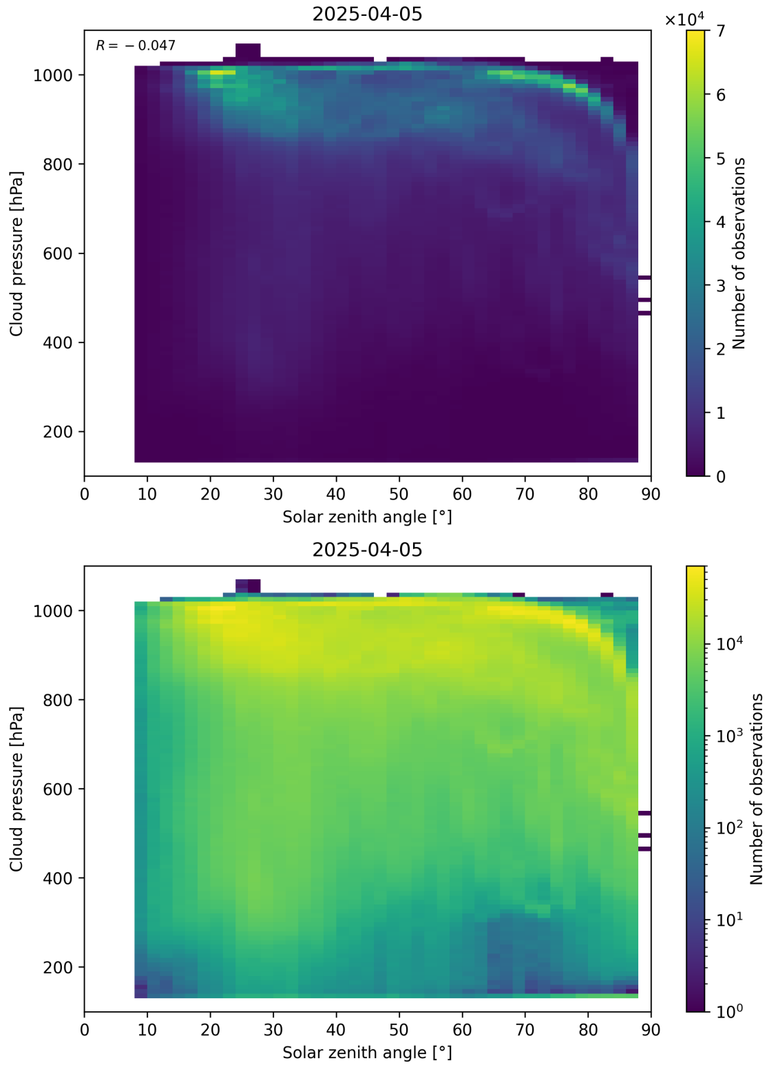
Figure 111: Scatter density plot of “Solar zenith angle” against “Cloud pressure” for 2025-04-04 to 2025-04-06.
