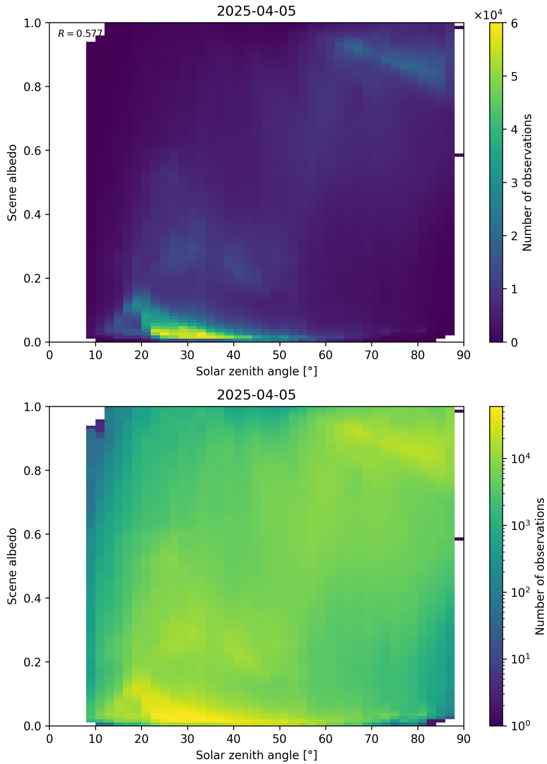
Figure 116: Scatter density plot of “Solar zenith angle” against “Scene albedo” for 2025-04-04 to 2025-04-06.
