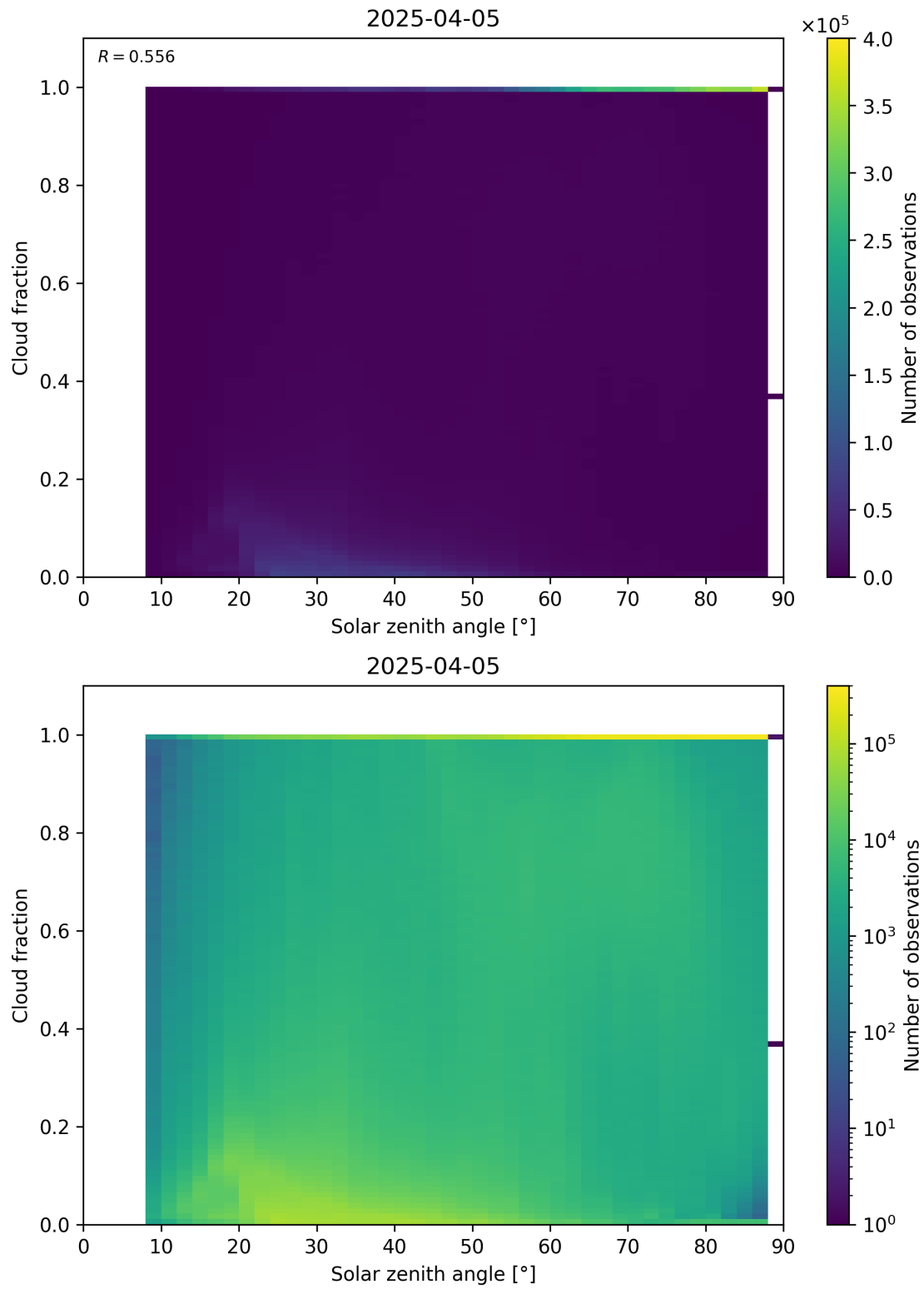
Figure 110: Scatter density plot of “Solar zenith angle” against “Cloud fraction” for 2025-04-04 to 2025-04-06.
