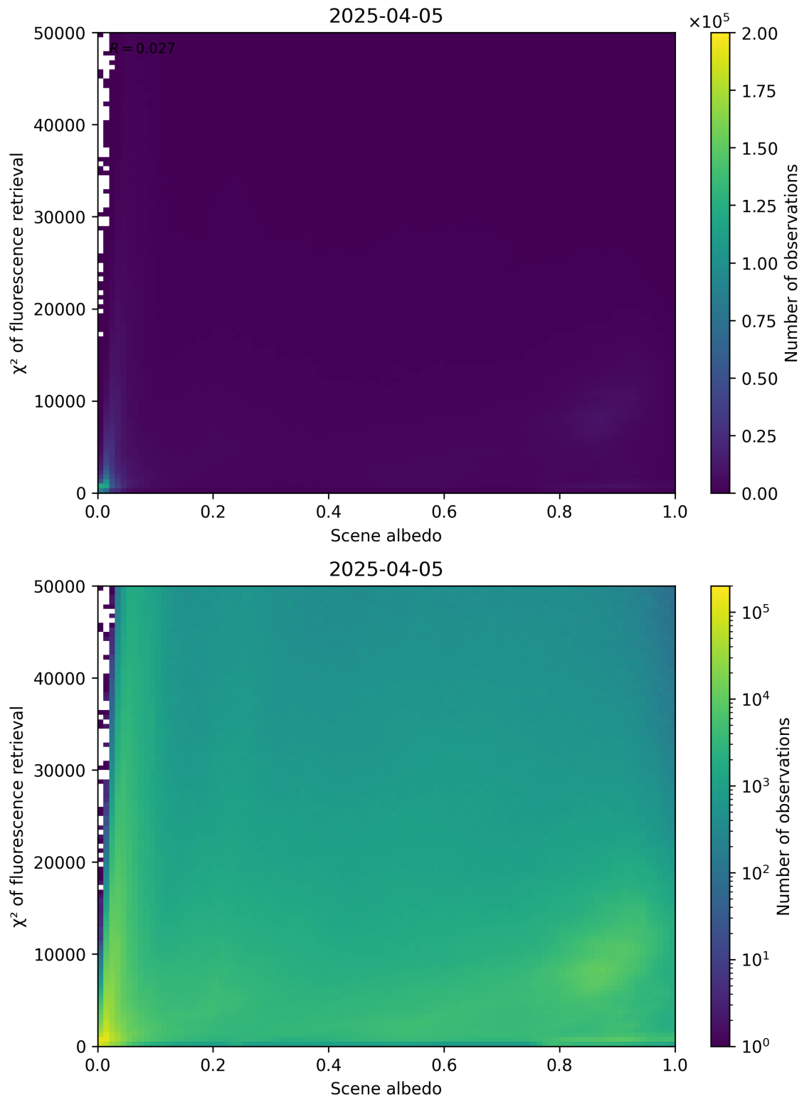
Figure 103: Scatter density plot of “Scene albedo” against “ \chi^2 of fluorescence retrieval” for 2025-04-04 to 2025-04-06.
