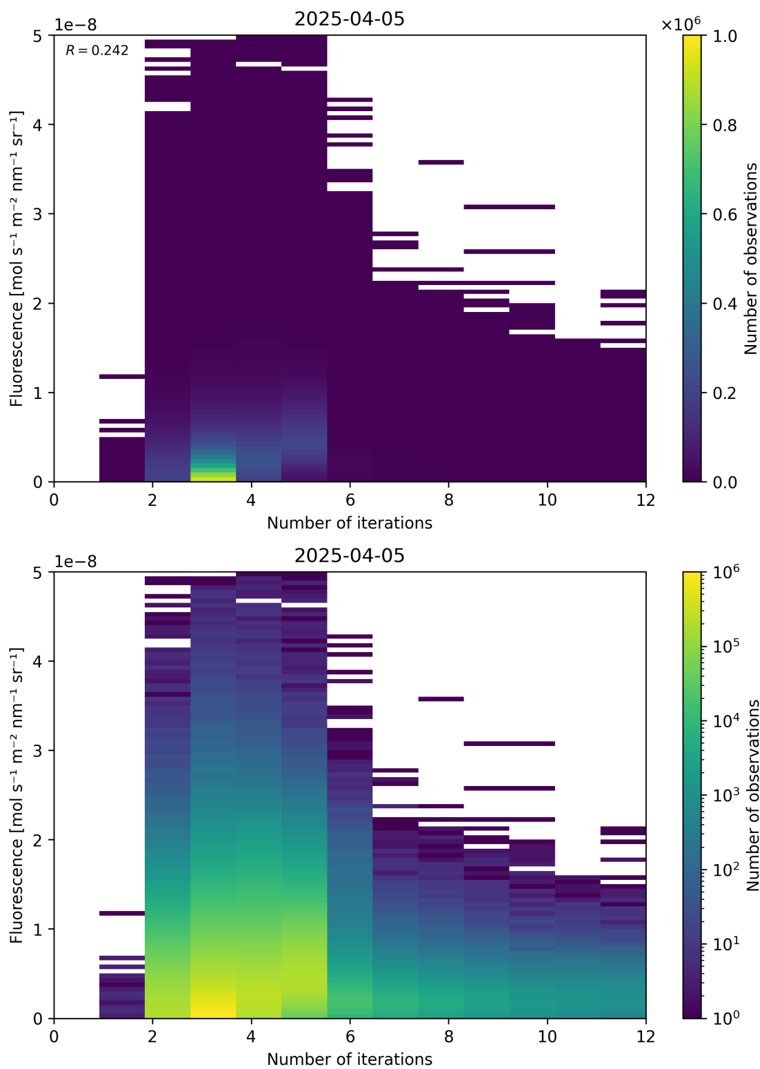
Figure 98: Scatter density plot of “Number of iterations” against “Fluorescence” for 2025-04-04 to 2025-04-06.
