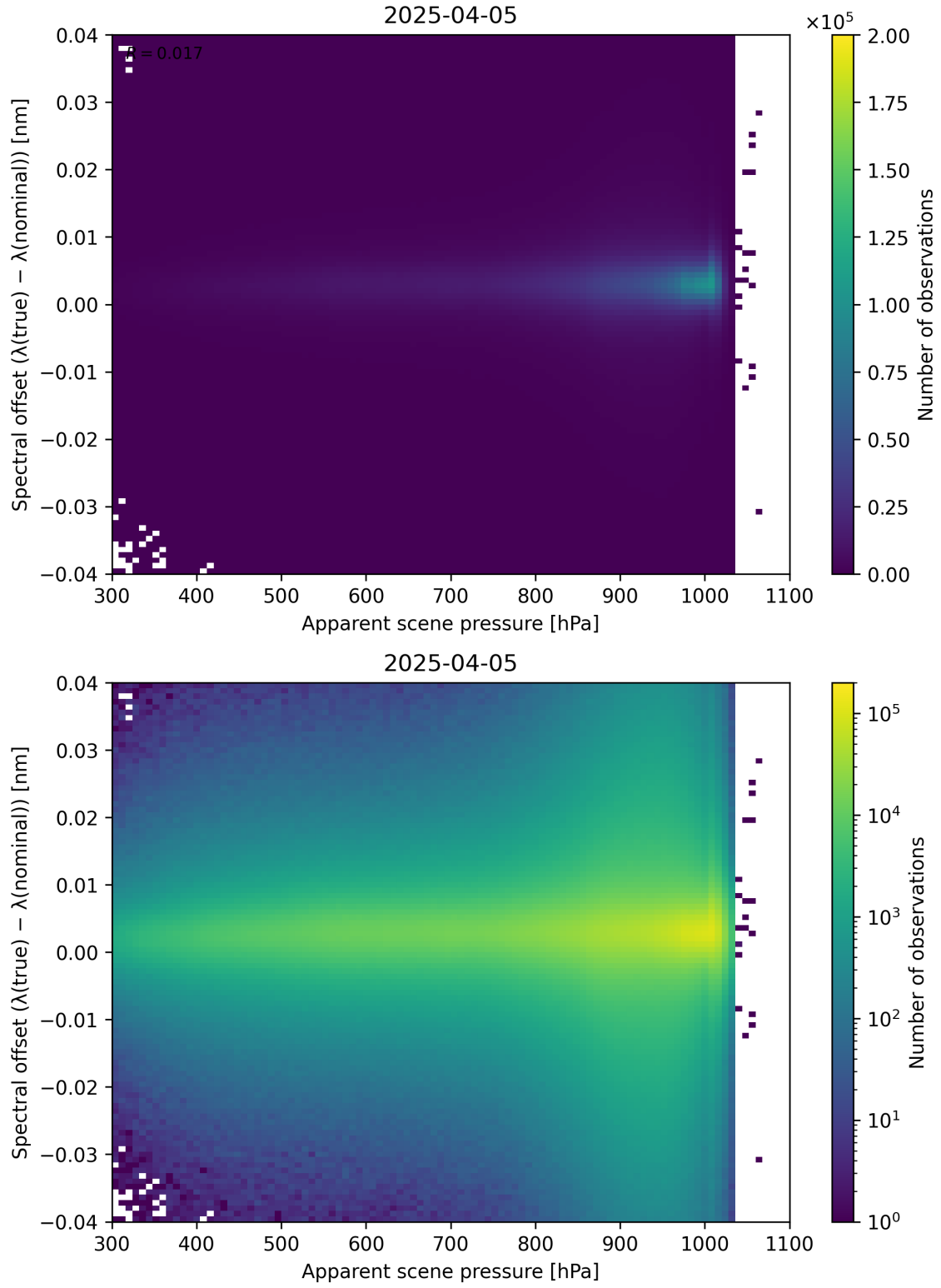
Figure 67: Scatter density plot of “Apparent scene pressure” against “Spectral offset ( \lambda_{\text{true}} - \lambda_{\text{nominal}} )” for 2025-04-04 to 2025-04-06.
