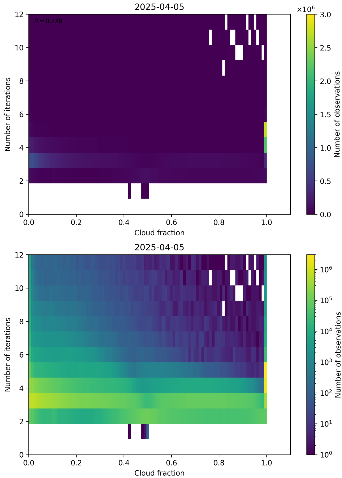
Figure 73: Scatter density plot of “Cloud fraction” against “Number of iterations” for 2025-04-04 to 2025-04-06.
