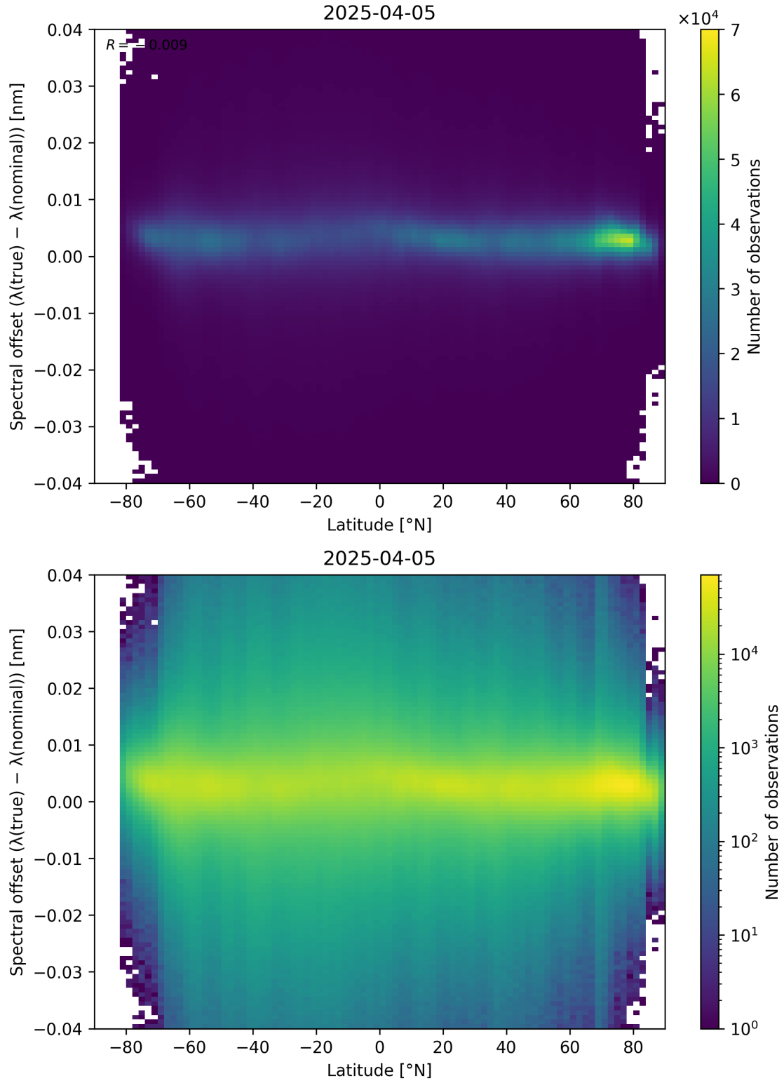
Figure 96: Scatter density plot of “Latitude” against “Spectral offset ( \lambda_{\text{true}} - \lambda_{\text{nominal}} )” for 2025-04-04 to 2025-04-06.
