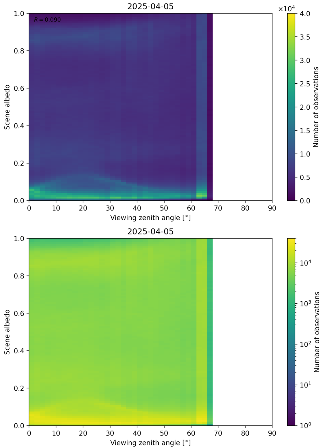
Figure 126: Scatter density plot of “Viewing zenith angle” against “Scene albedo” for 2025-04-04 to 2025-04-06.
