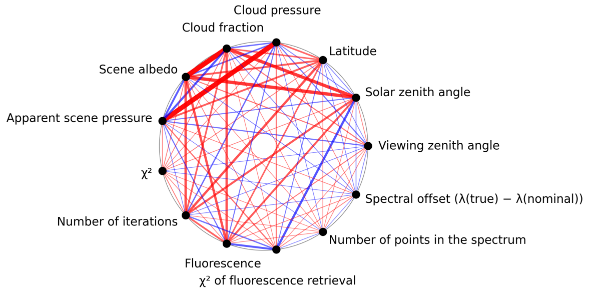
Figure 1: Map of correlation graph for 2025-04-04 to 2025-04-06.
