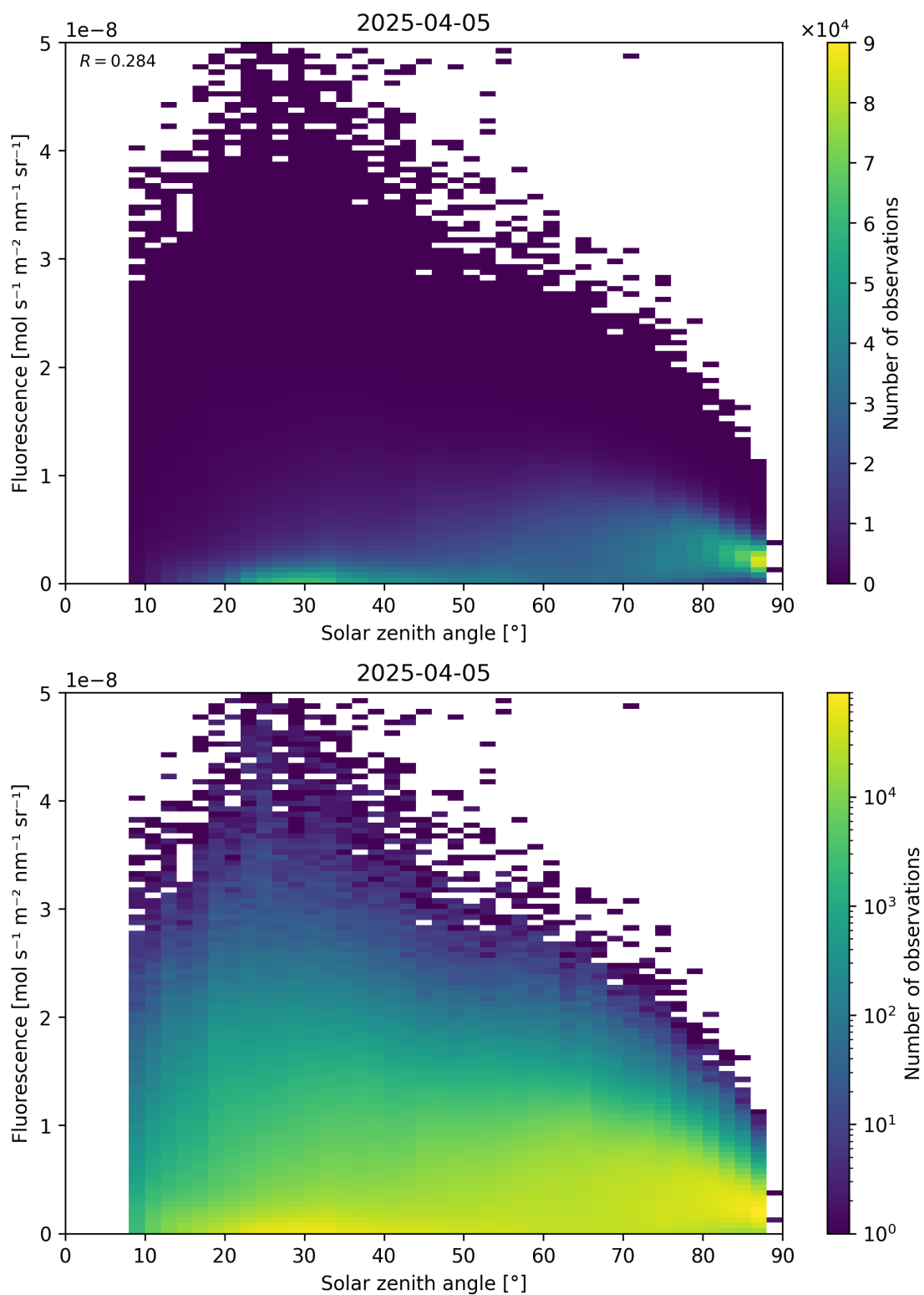
Figure 112: Scatter density plot of “Solar zenith angle” against “Fluorescence” for 2025-04-04 to 2025-04-06.
