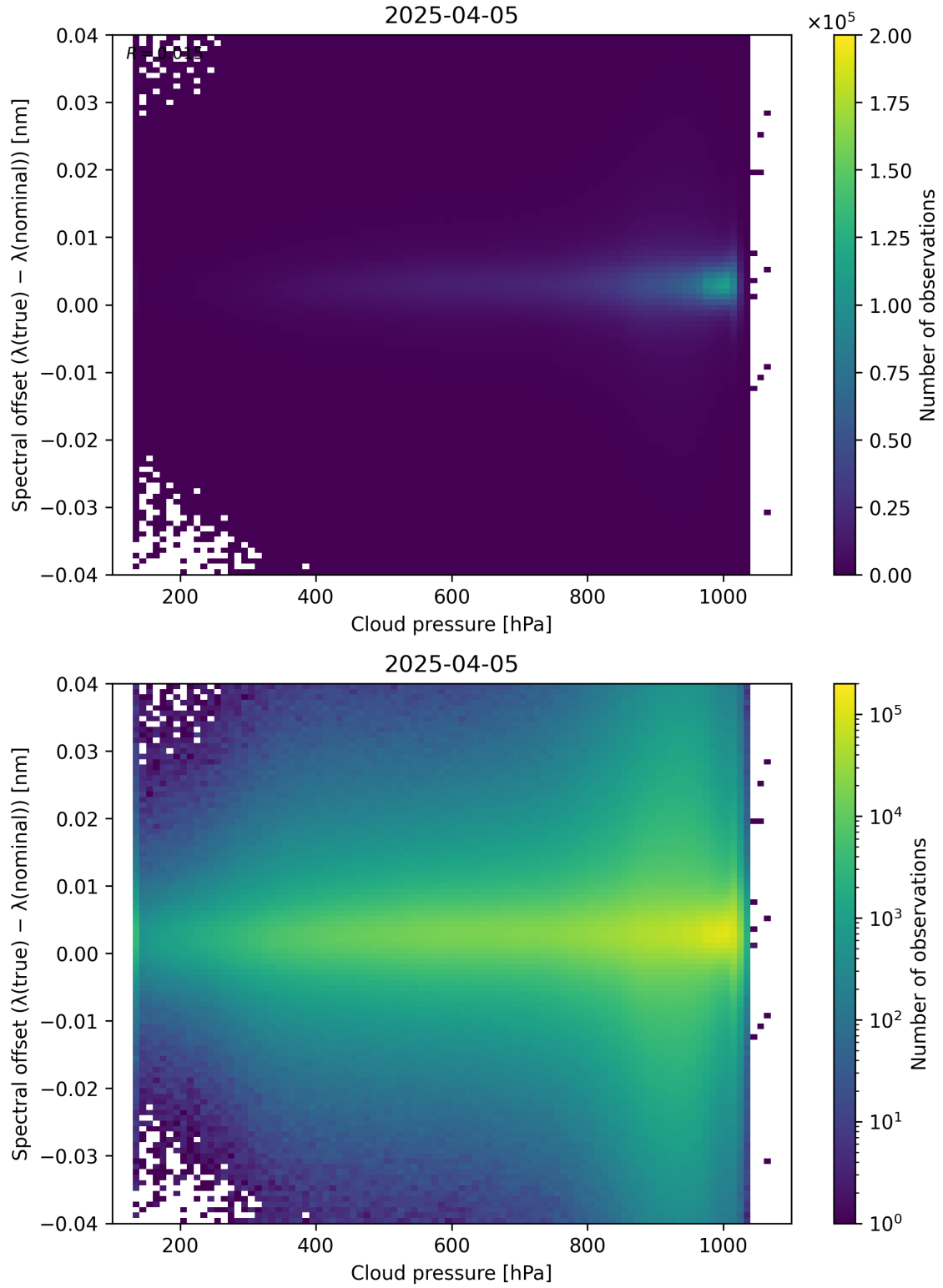
Figure 84: Scatter density plot of “Cloud pressure” against “Spectral offset ( \lambda_{\text{true}} - \lambda_{\text{nominal}} )” for 2025-04-04 to 2025-04-06.
