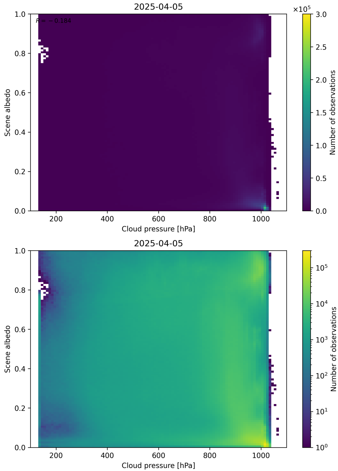
Figure 83: Scatter density plot of “Cloud pressure” against “Scene albedo” for 2025-04-04 to 2025-04-06.
