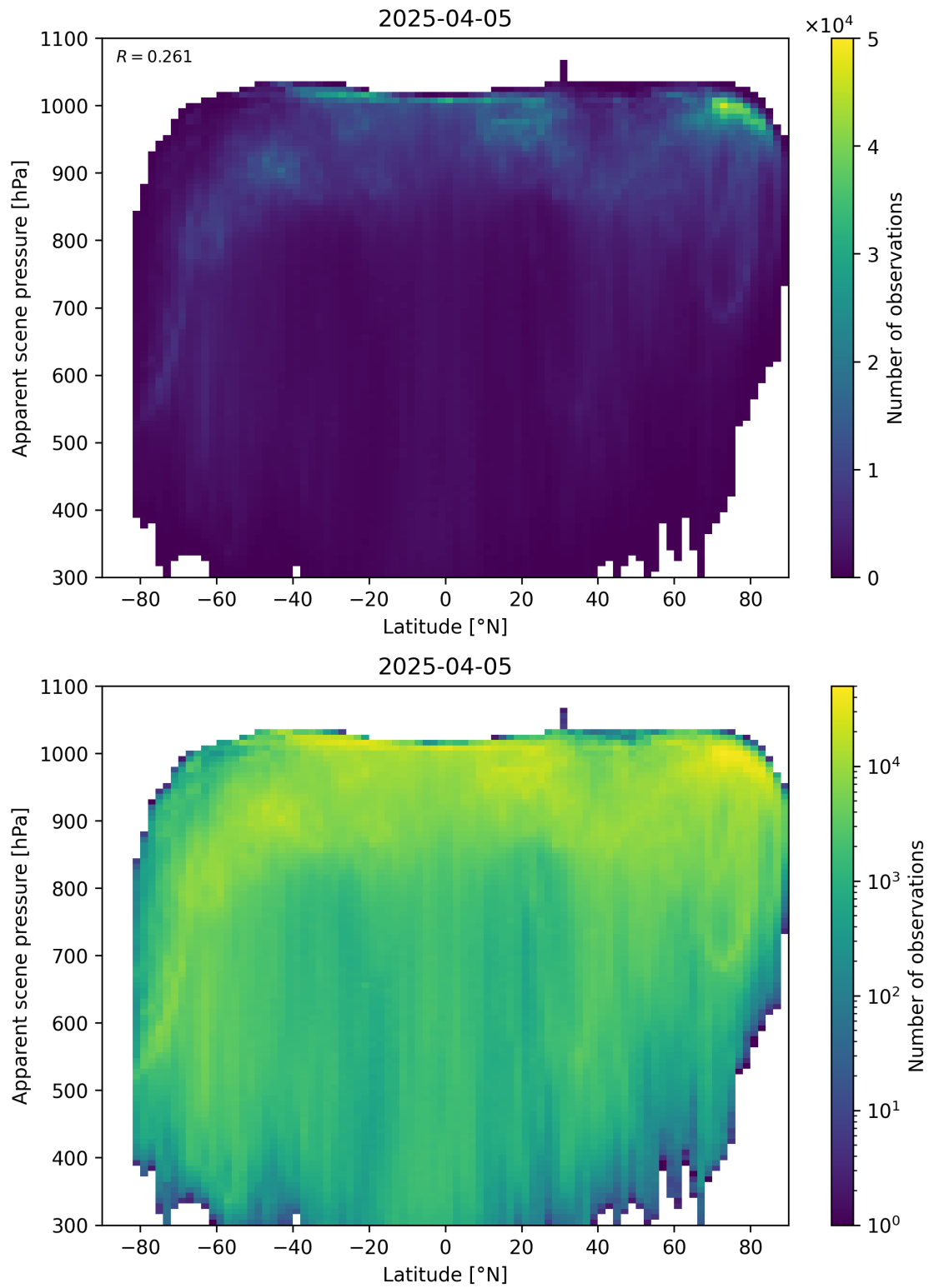
Figure 88: Scatter density plot of “Latitude” against “Apparent scene pressure” for 2025-04-04 to 2025-04-06.
