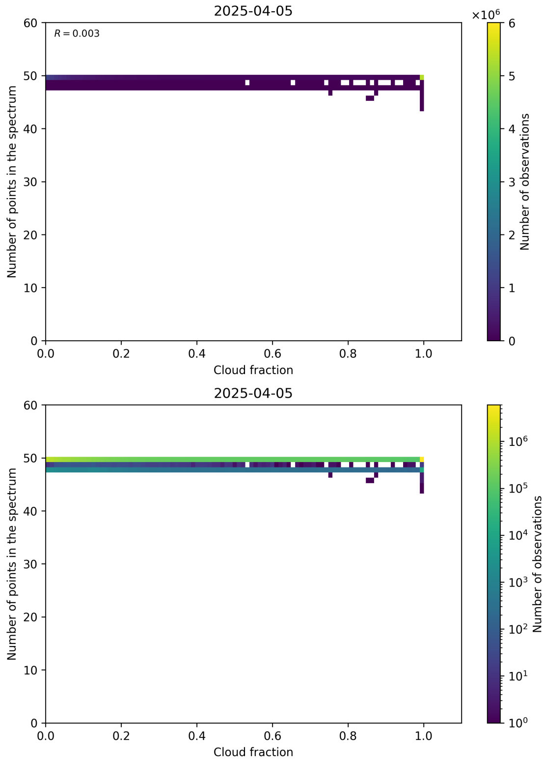
Figure 74: Scatter density plot of “Cloud fraction” against “Number of points in the spectrum” for 2025-04-04 to 2025-04-06.
