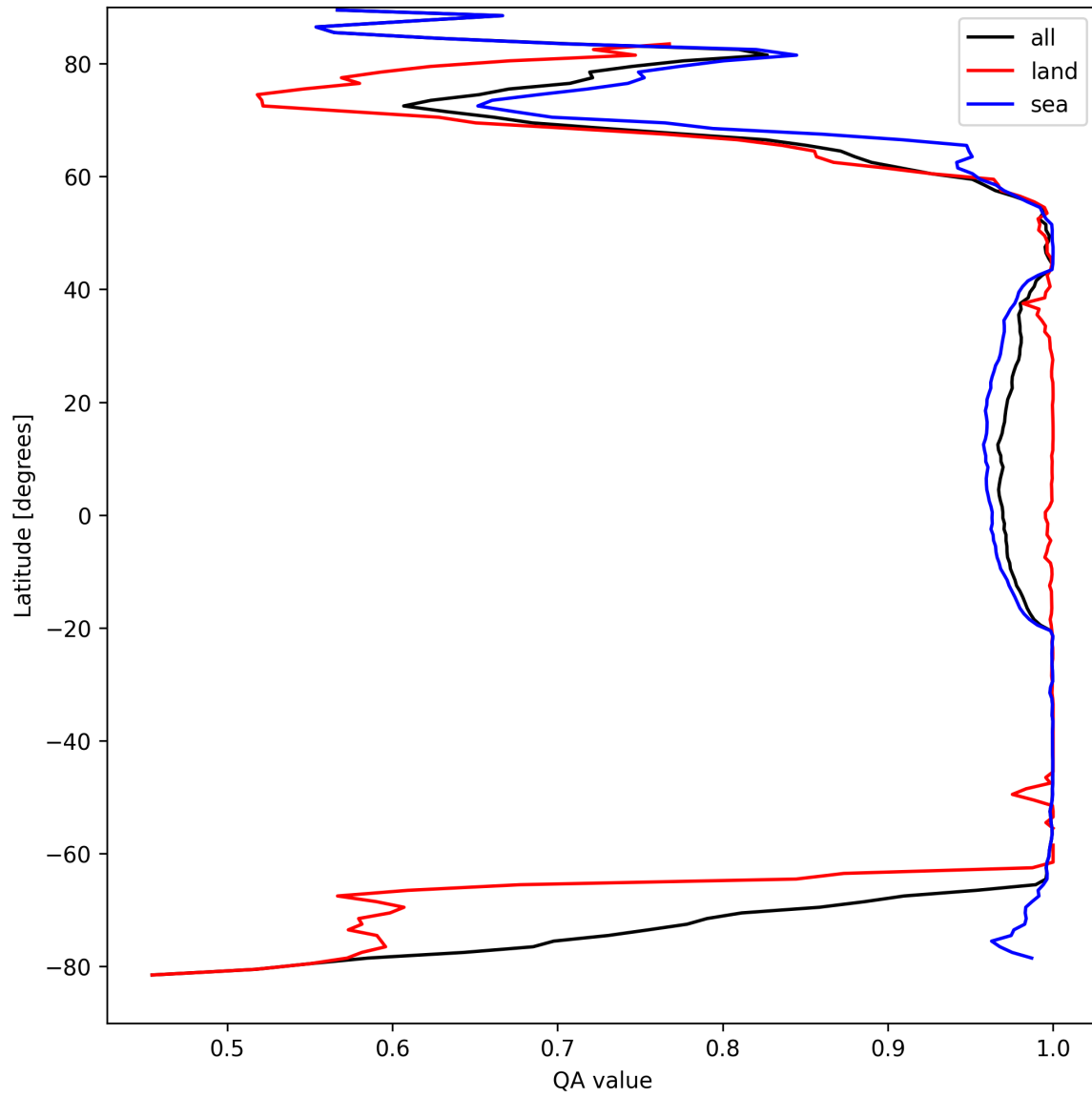
Figure 12: Zonal average of “QA value” for 2025-04-04 to 2025-04-06.
