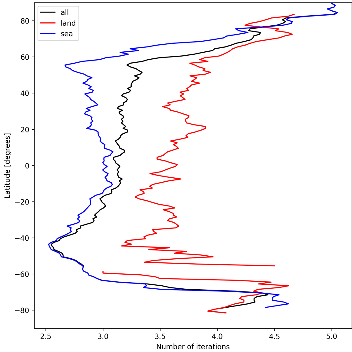
Figure 22: Zonal average of “Number of iterations” for 2025-04-04 to 2025-04-06.
