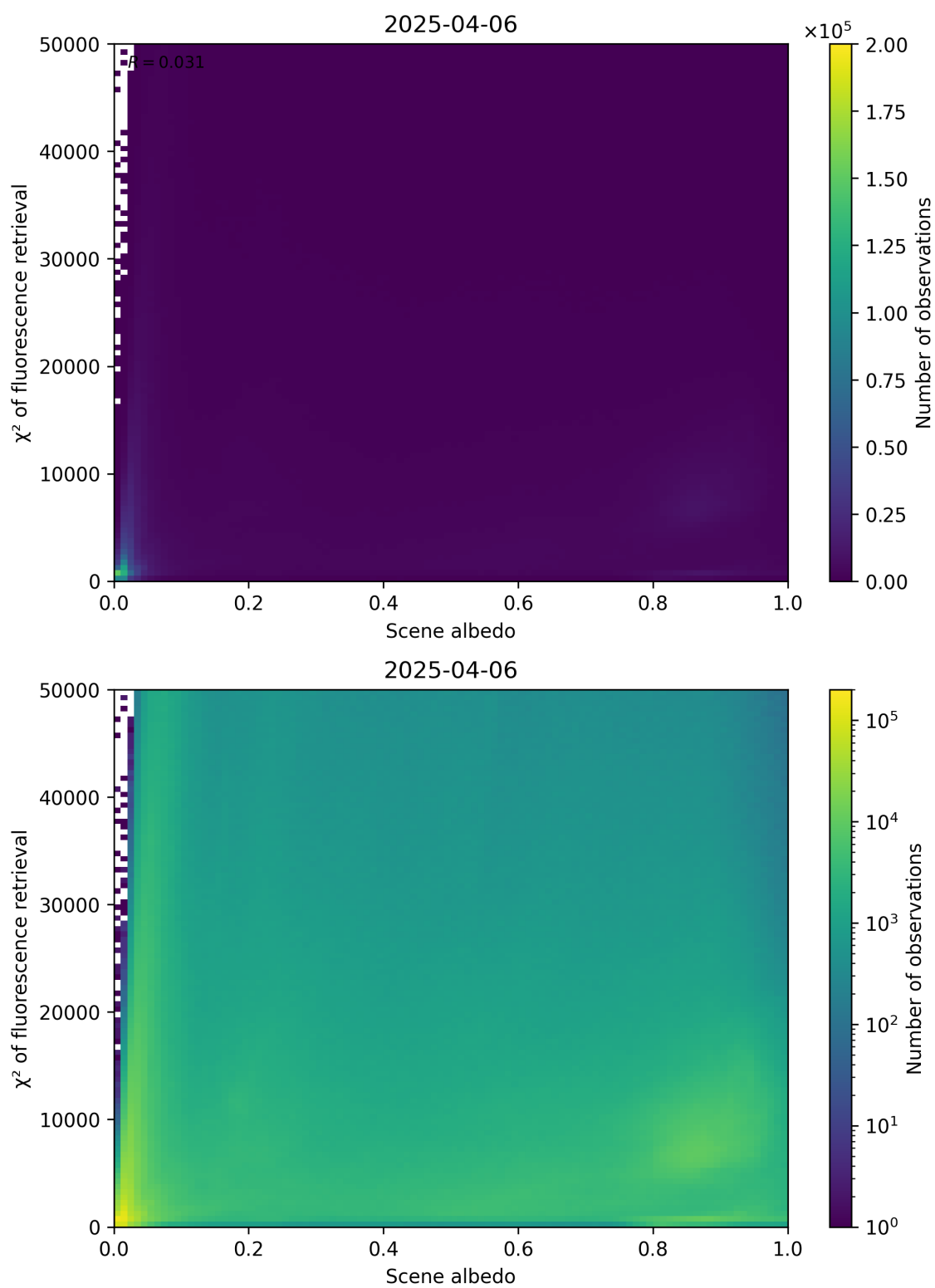
Figure 103: Scatter density plot of “Scene albedo” against “ \chi^2 of fluorescence retrieval” for 2025-04-05 to 2025-04-07.
