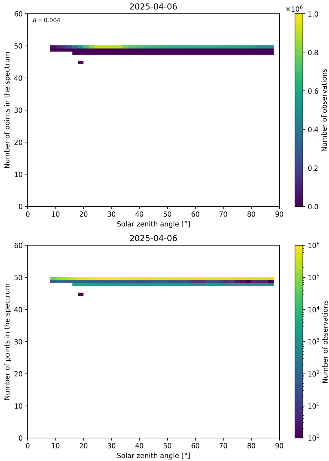
Figure 115: Scatter density plot of “Solar zenith angle” against “Number of points in the spectrum” for 2025-04-05 to 2025-04-07.
