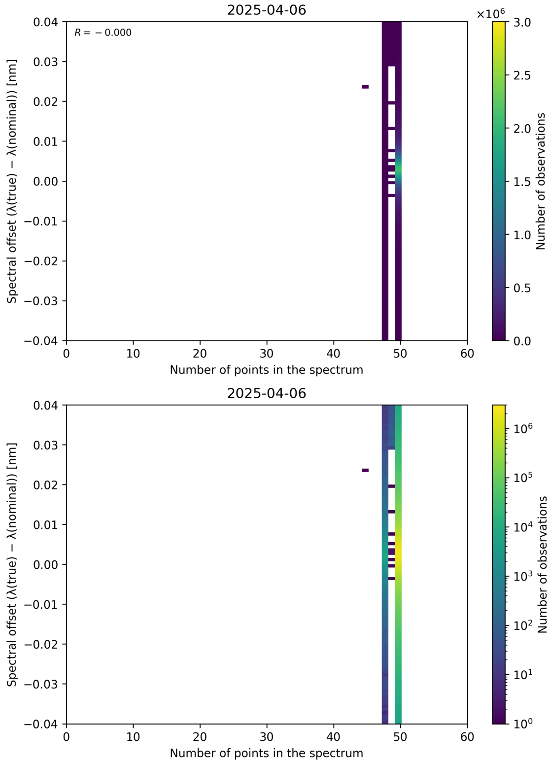
Figure 101: Scatter density plot of “Number of points in the spectrum” against “Spectral offset ( \lambda_{\text{true}} - \lambda_{\text{nominal}} )” for 2025-04-05 to 2025-04-07.
