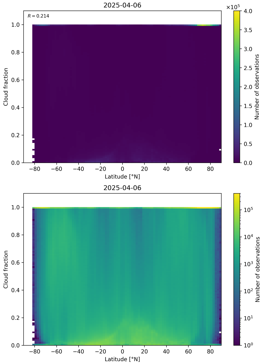
Figure 90: Scatter density plot of “Latitude” against “Cloud fraction” for 2025-04-05 to 2025-04-07.
