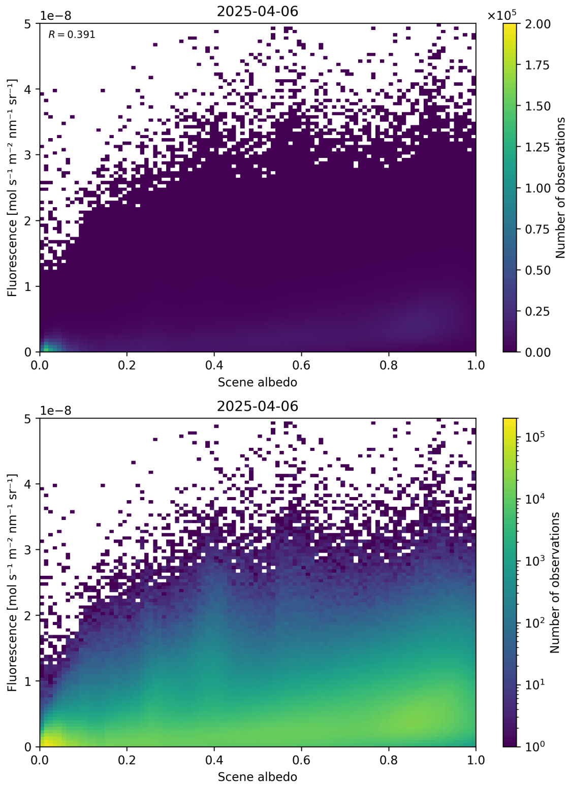
Figure 104: Scatter density plot of “Scene albedo” against “Fluorescence” for 2025-04-05 to 2025-04-07.
