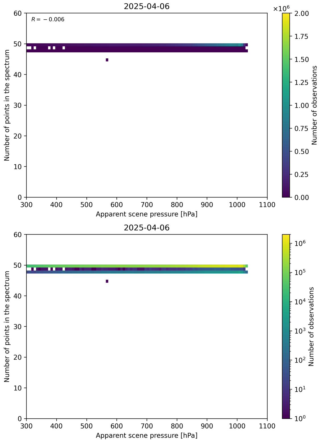
Figure 66: Scatter density plot of “Apparent scene pressure” against “Number of points in the spectrum” for 2025-04-05 to 2025-04-07.
