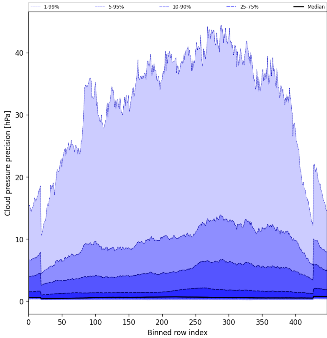
Figure 48: Along track statistics of “Cloud pressure precision” for 2025-04-05 to 2025-04-07
