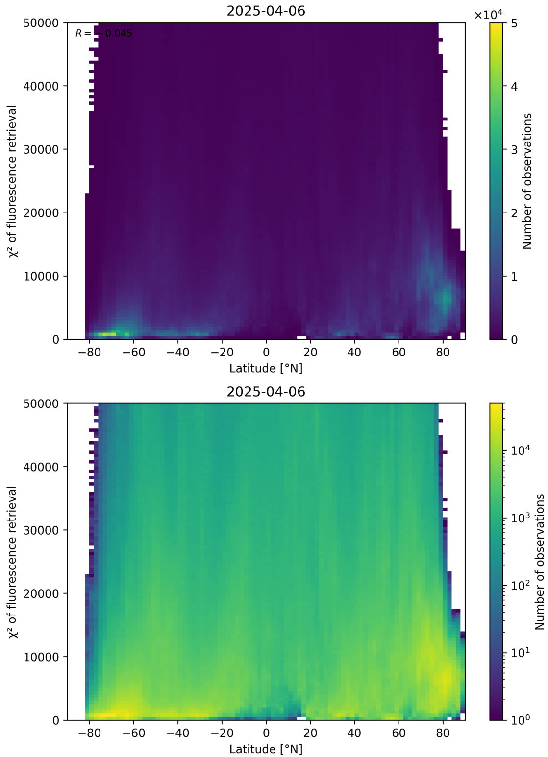
Figure 89: Scatter density plot of “Latitude” against “ \chi^2 of fluorescence retrieval” for 2025-04-05 to 2025-04-07.
