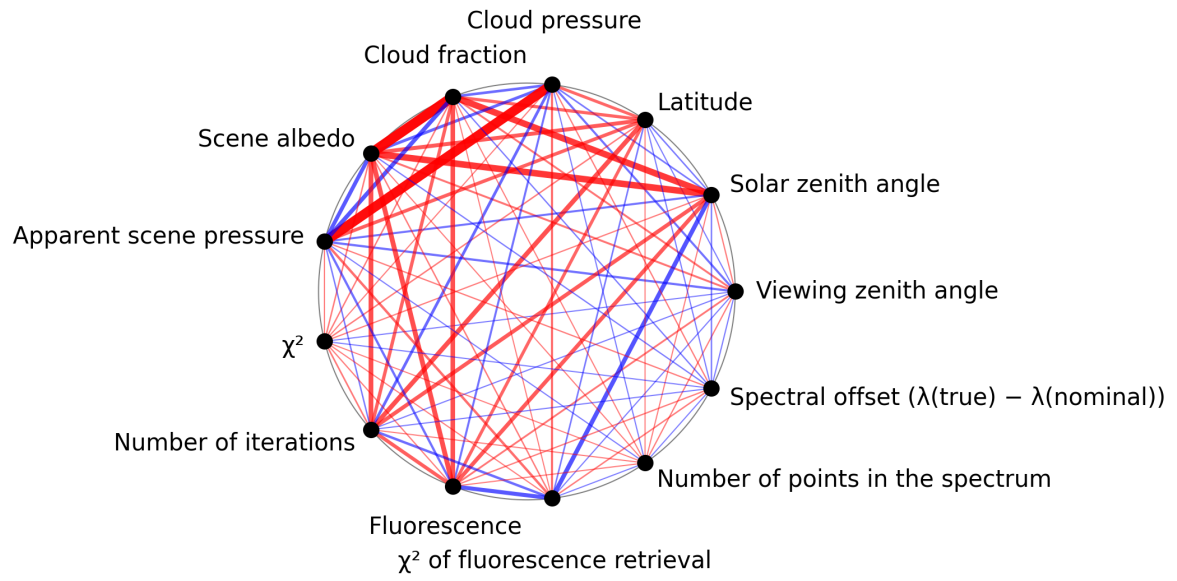
Figure 1: Map of correlation graph for 2025-04-05 to 2025-04-07.
