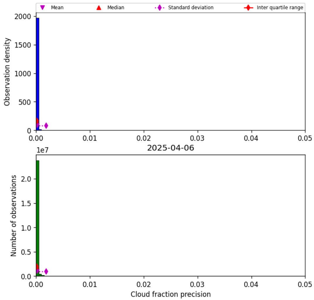
Figure 33: Histogram of “Cloud fraction precision” for 2025-04-05 to 2025-04-07
