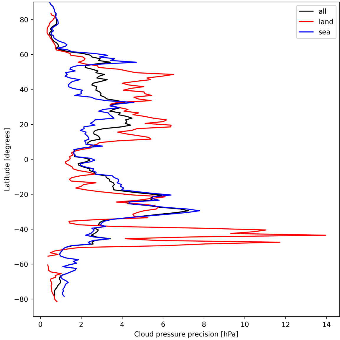
Figure 14: Zonal average of “Cloud pressure precision” for 2025-04-05 to 2025-04-07.
