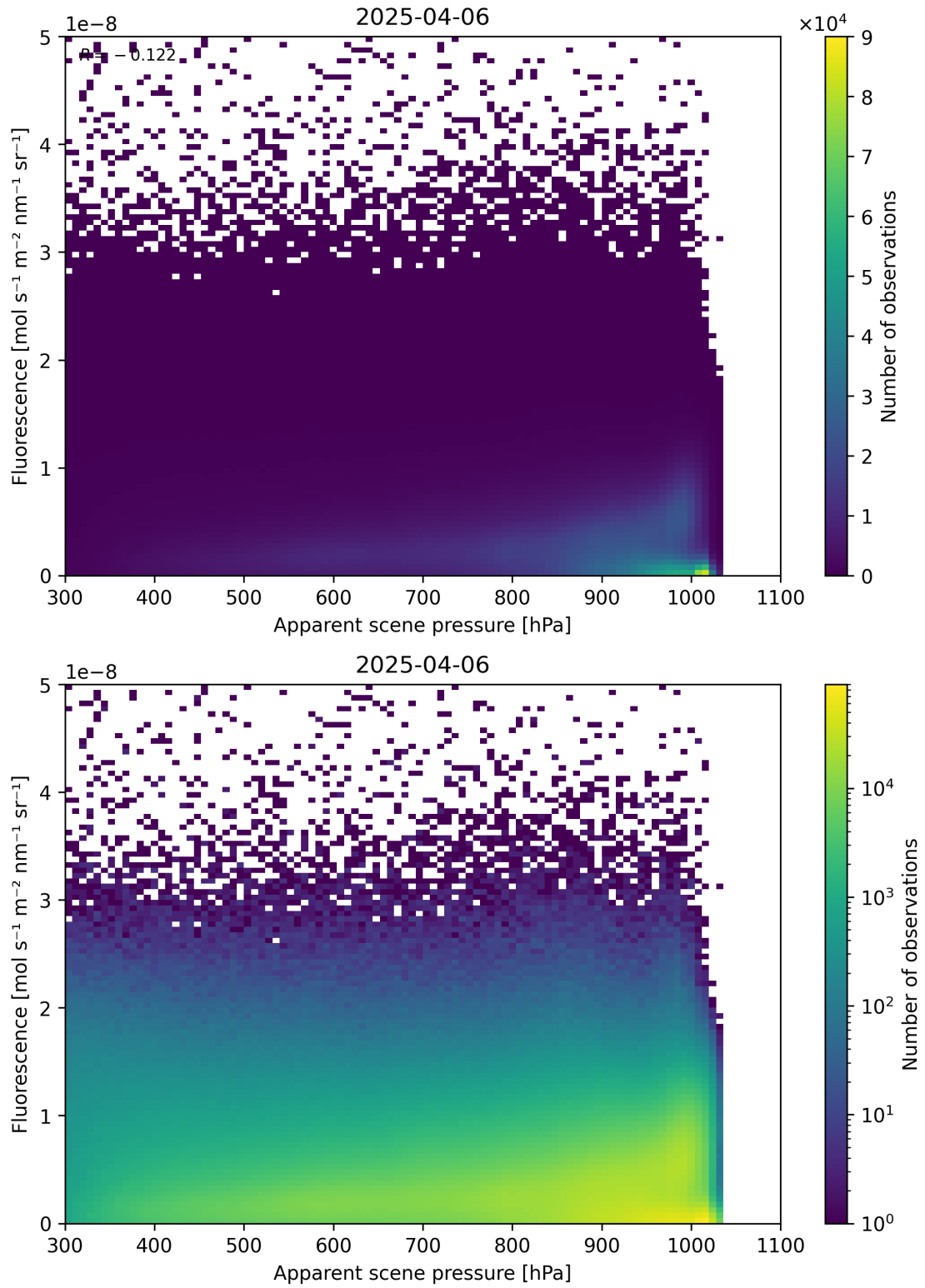
Figure 64: Scatter density plot of “Apparent scene pressure” against “Fluorescence” for 2025-04-05 to 2025-04-07.
