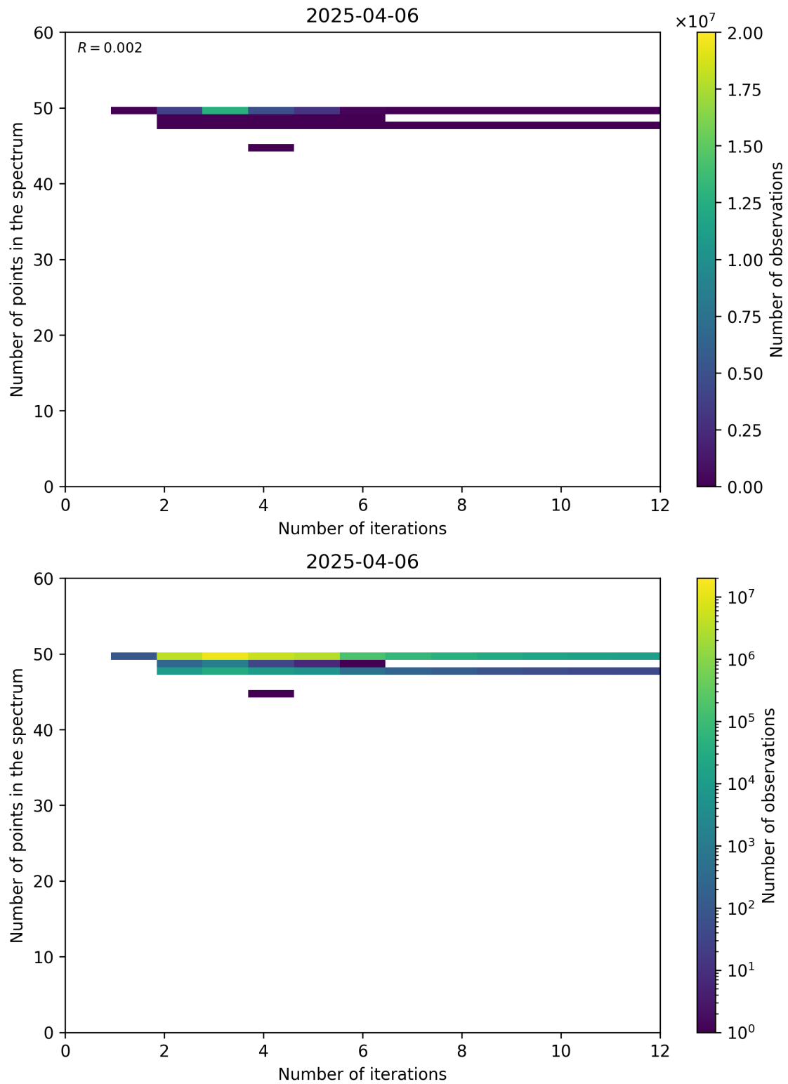
Figure 99: Scatter density plot of “Number of iterations” against “Number of points in the spectrum” for 2025-04-05 to 2025-04-07.
