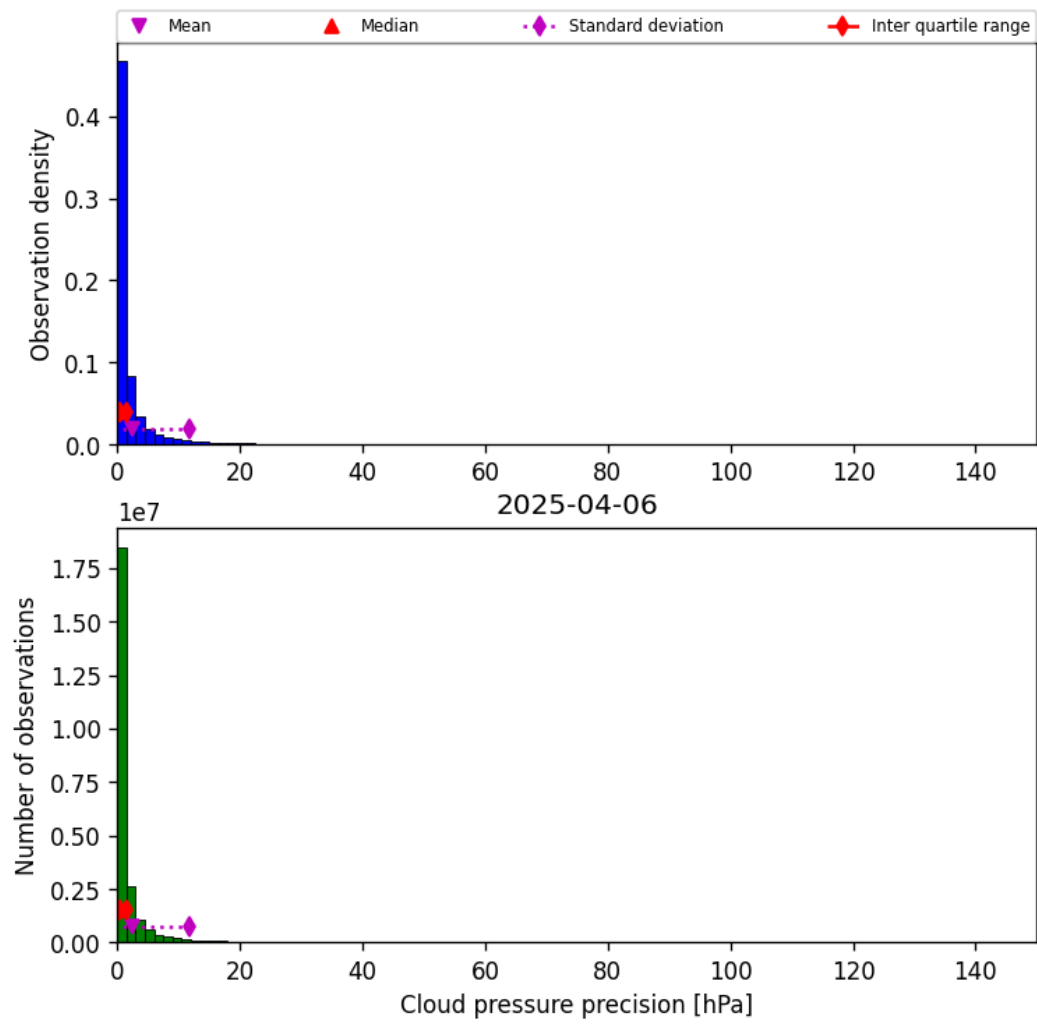
Figure 31: Histogram of “Cloud pressure precision” for 2025-04-05 to 2025-04-07
