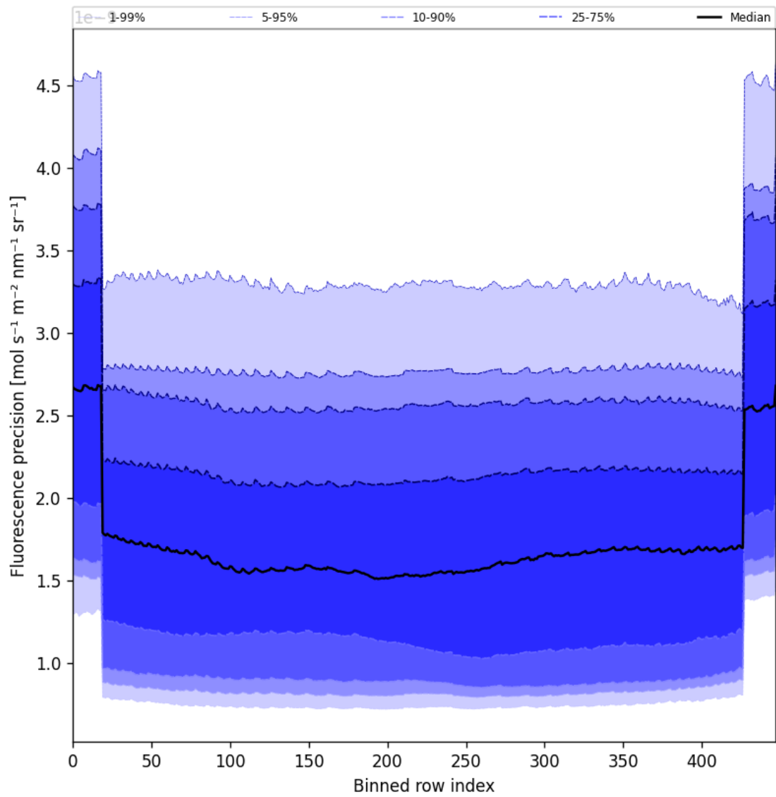
Figure 58: Along track statistics of “Fluorescence precision” for 2025-04-05 to 2025-04-07
