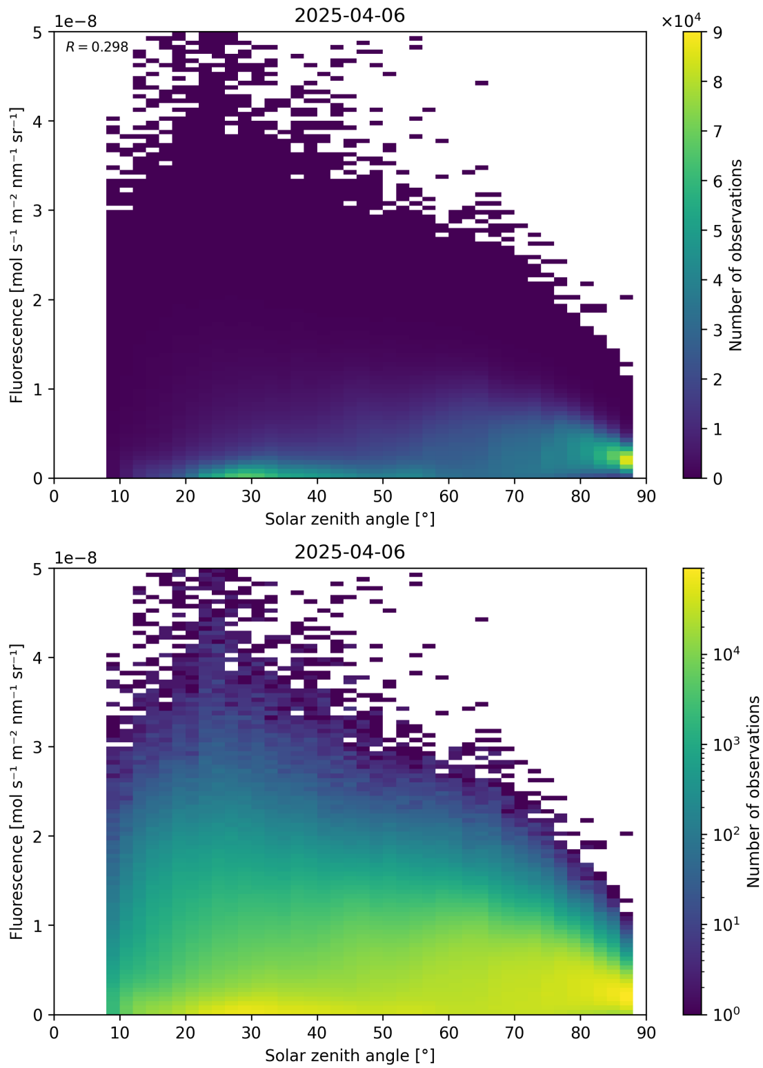
Figure 112: Scatter density plot of “Solar zenith angle” against “Fluorescence” for 2025-04-05 to 2025-04-07.
