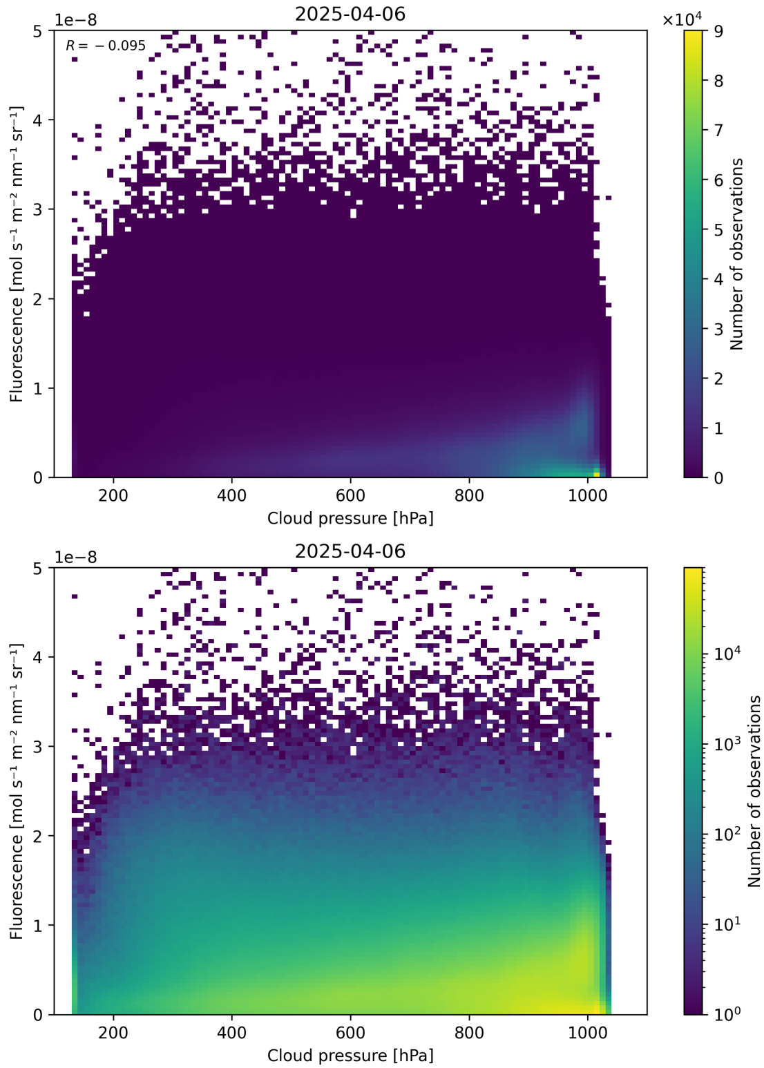
Figure 80: Scatter density plot of “Cloud pressure” against “Fluorescence” for 2025-04-05 to 2025-04-07.
