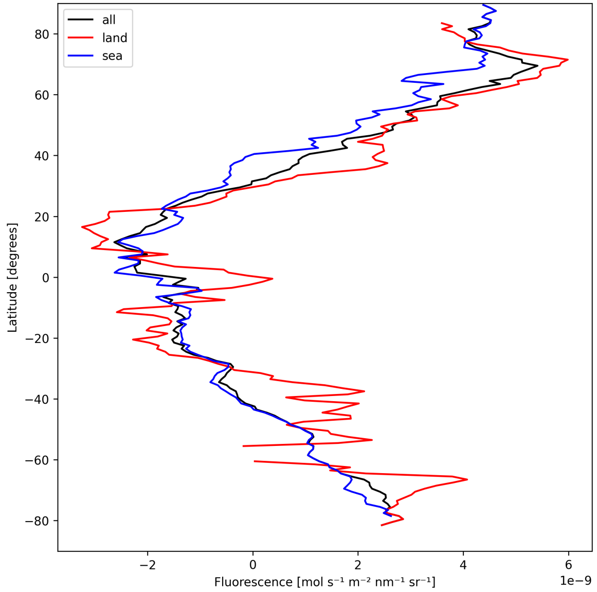
Figure 23: Zonal average of “Fluorescence” for 2025-04-05 to 2025-04-07.
