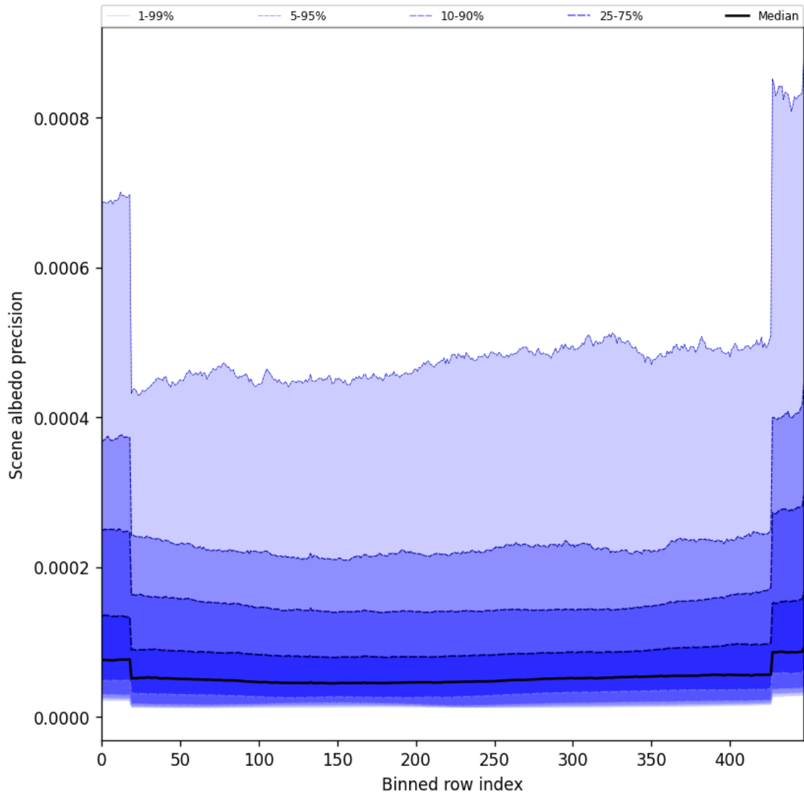
Figure 52: Along track statistics of “Scene albedo precision” for 2025-04-05 to 2025-04-07
