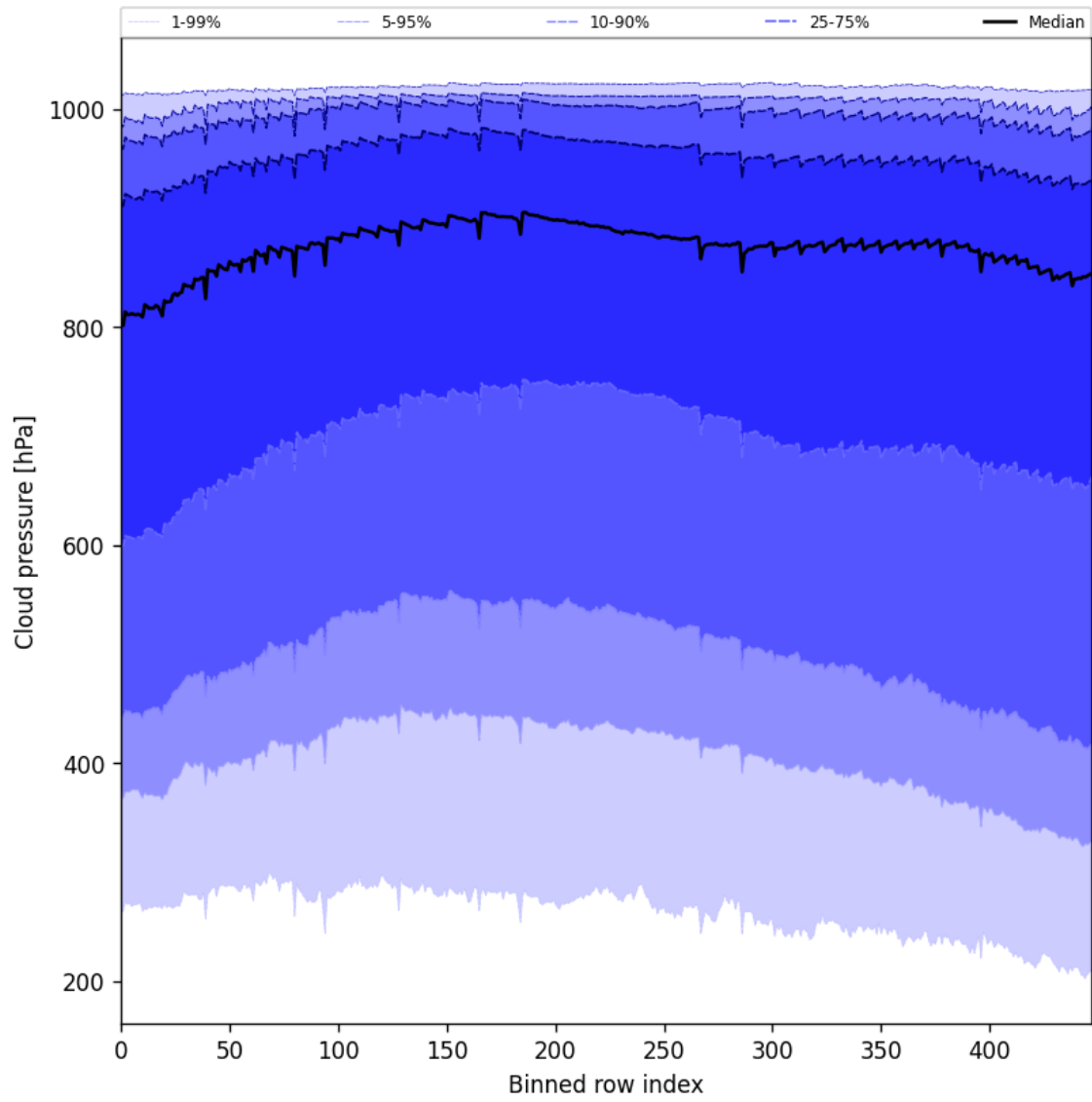
Figure 47: Along track statistics of “Cloud pressure” for 2025-04-05 to 2025-04-07
