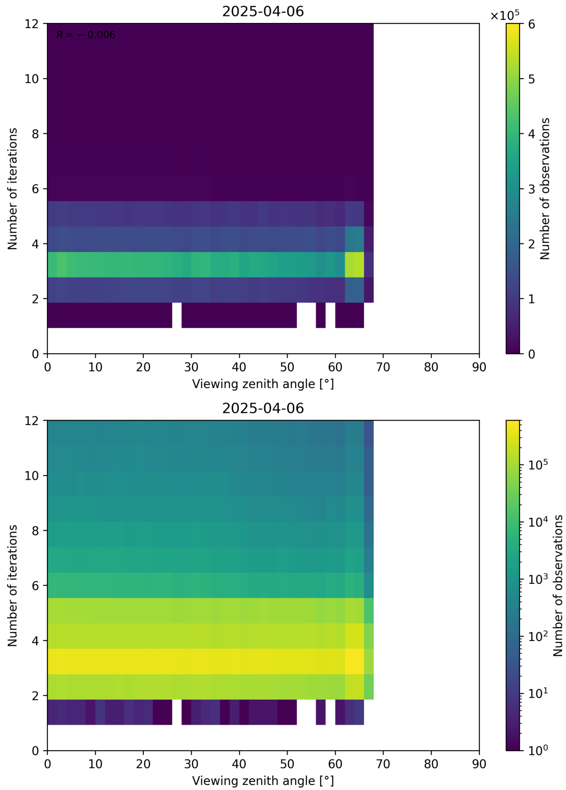
Figure 124: Scatter density plot of “Viewing zenith angle” against “Number of iterations” for 2025-04-05 to 2025-04-07.
