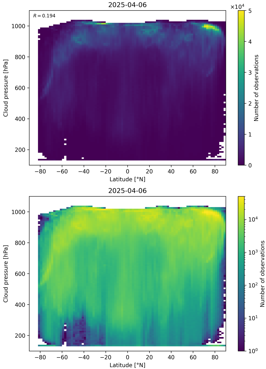
Figure 91: Scatter density plot of “Latitude” against “Cloud pressure” for 2025-04-05 to 2025-04-07.
