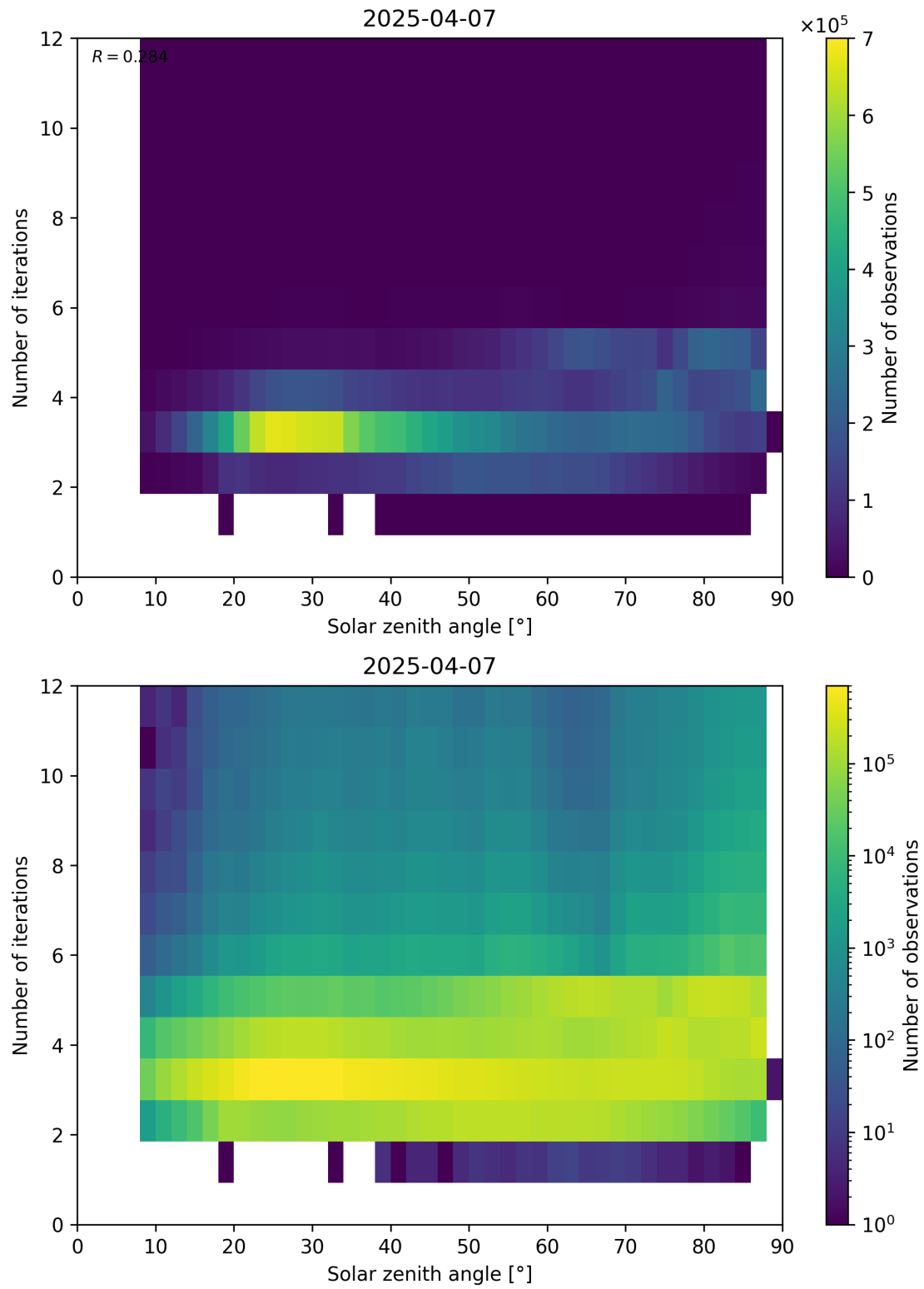
Figure 114: Scatter density plot of “Solar zenith angle” against “Number of iterations” for 2025-04-06 to 2025-04-08.
