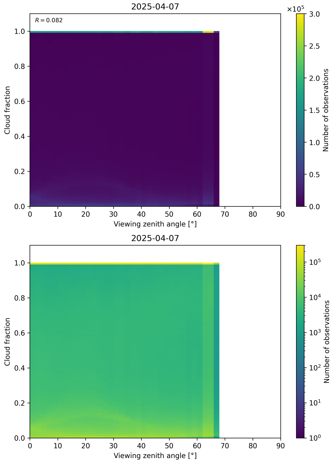
Figure 120: Scatter density plot of “Viewing zenith angle” against “Cloud fraction” for 2025-04-06 to 2025-04-08.
