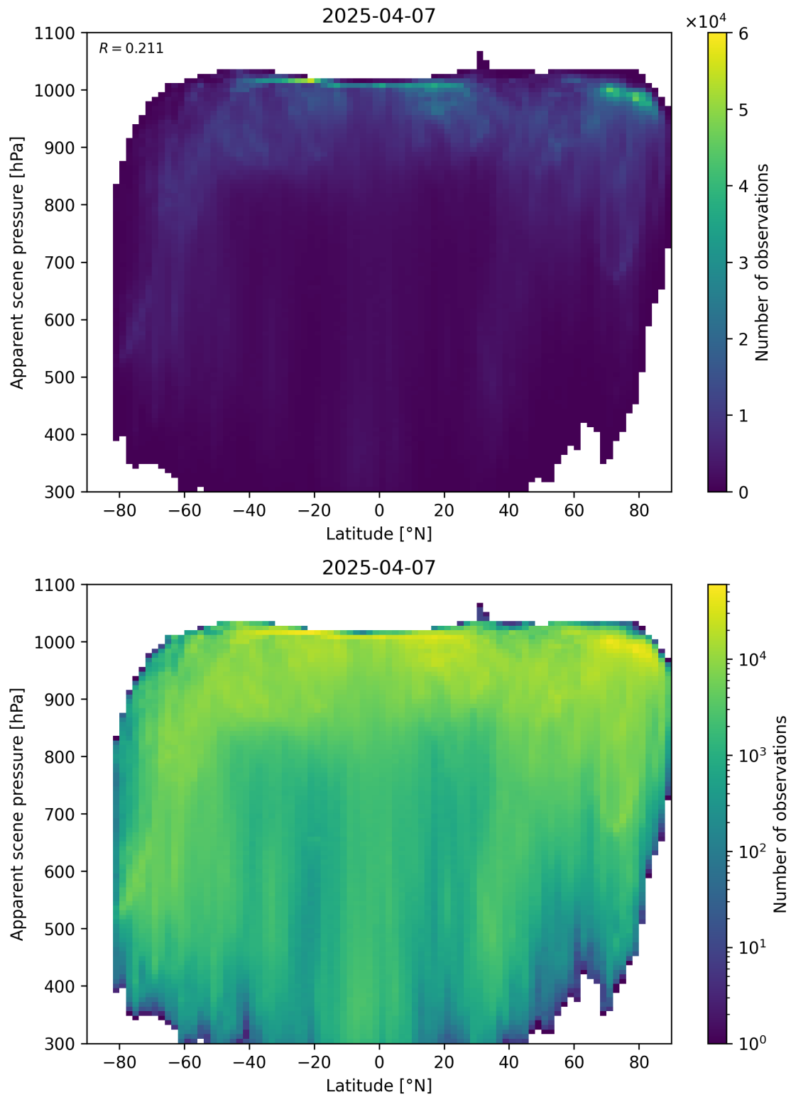
Figure 88: Scatter density plot of “Latitude” against “Apparent scene pressure” for 2025-04-06 to 2025-04-08.
