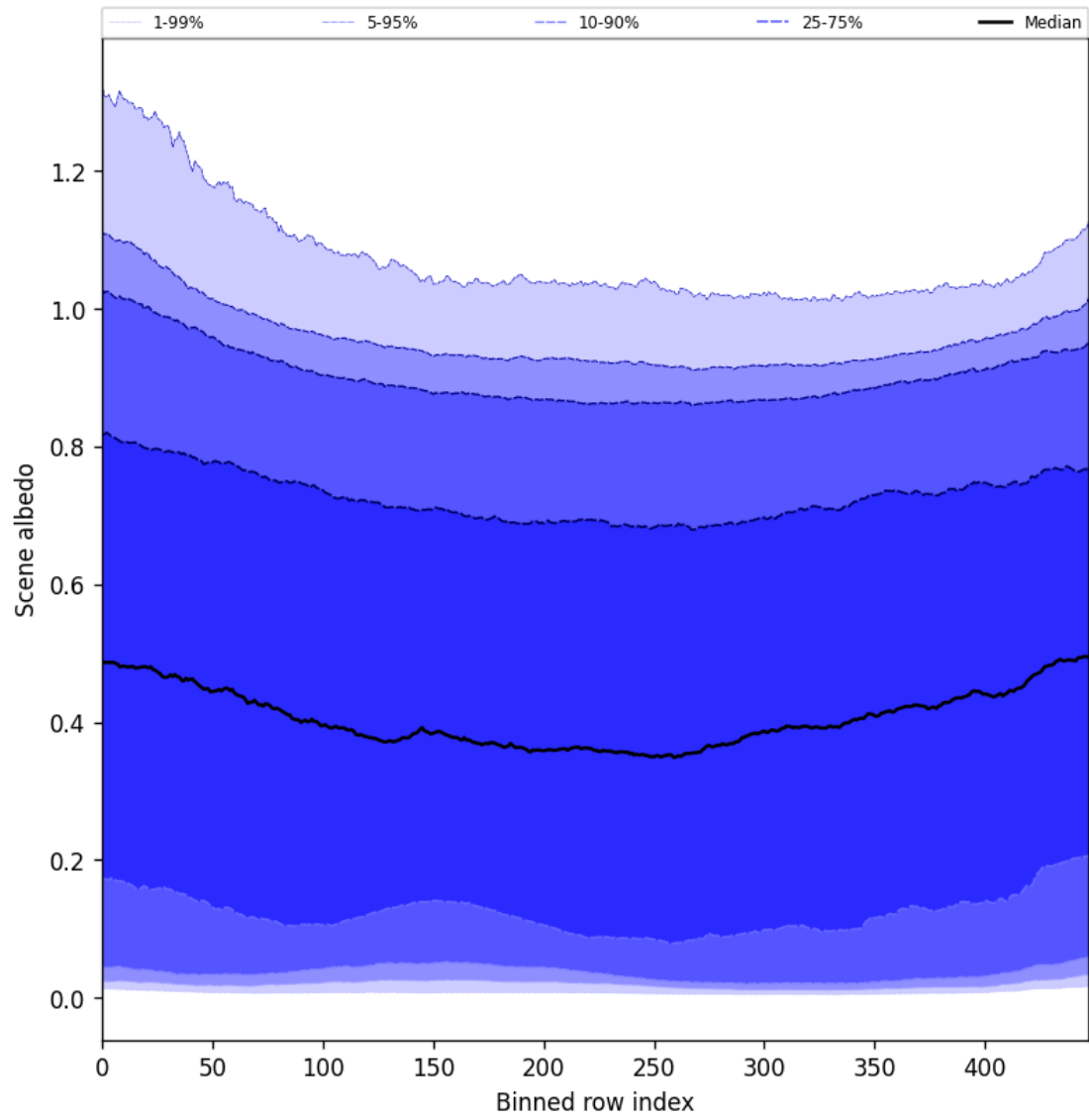
Figure 51: Along track statistics of “Scene albedo” for 2025-04-06 to 2025-04-08
