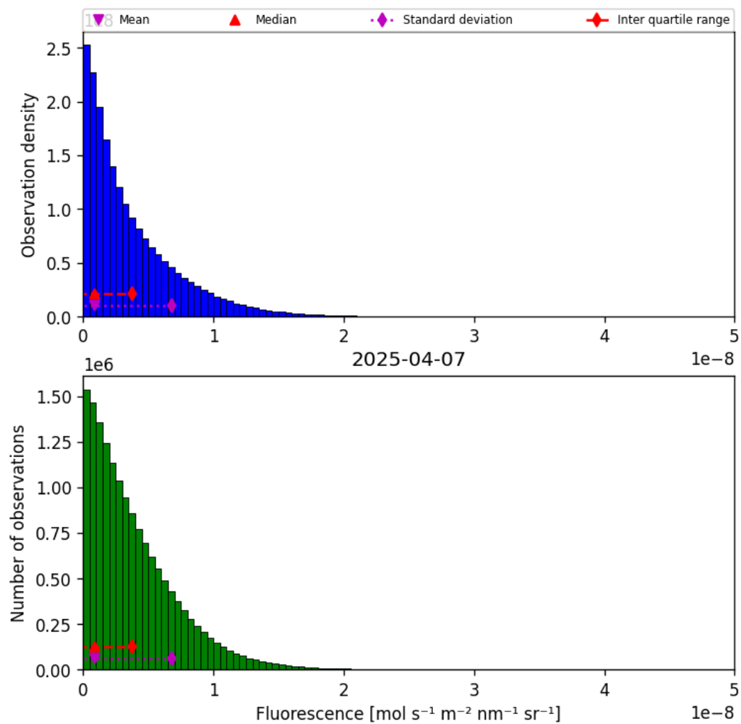
Figure 40: Histogram of “Fluorescence” for 2025-04-06 to 2025-04-08
