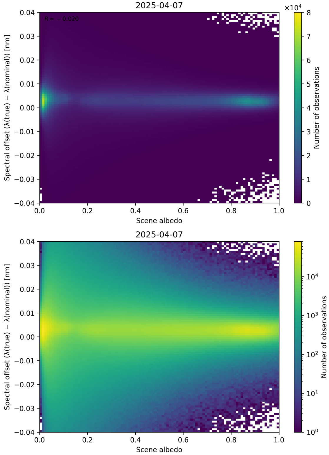
Figure 107: Scatter density plot of “Scene albedo” against “Spectral offset ( \lambda_{\text{true}} - \lambda_{\text{nominal}} )” for 2025-04-06 to 2025-04-08.
