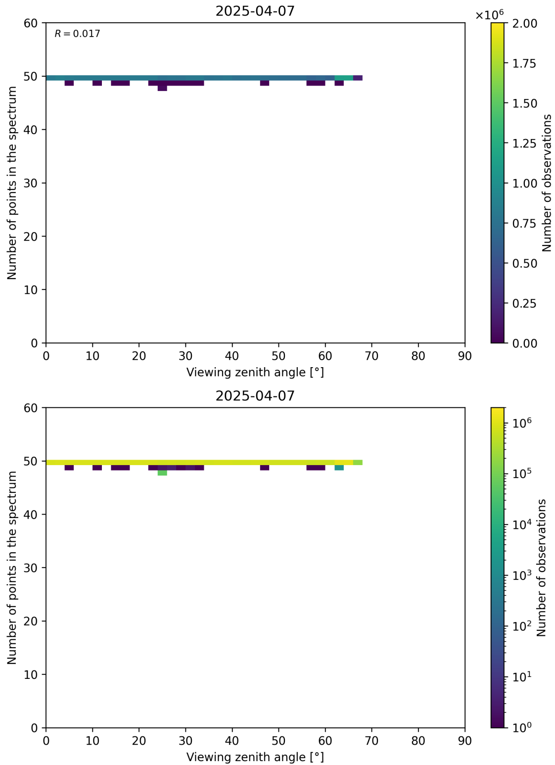
Figure 125: Scatter density plot of “Viewing zenith angle” against “Number of points in the spectrum” for 2025-04-06 to 2025-04-08.
