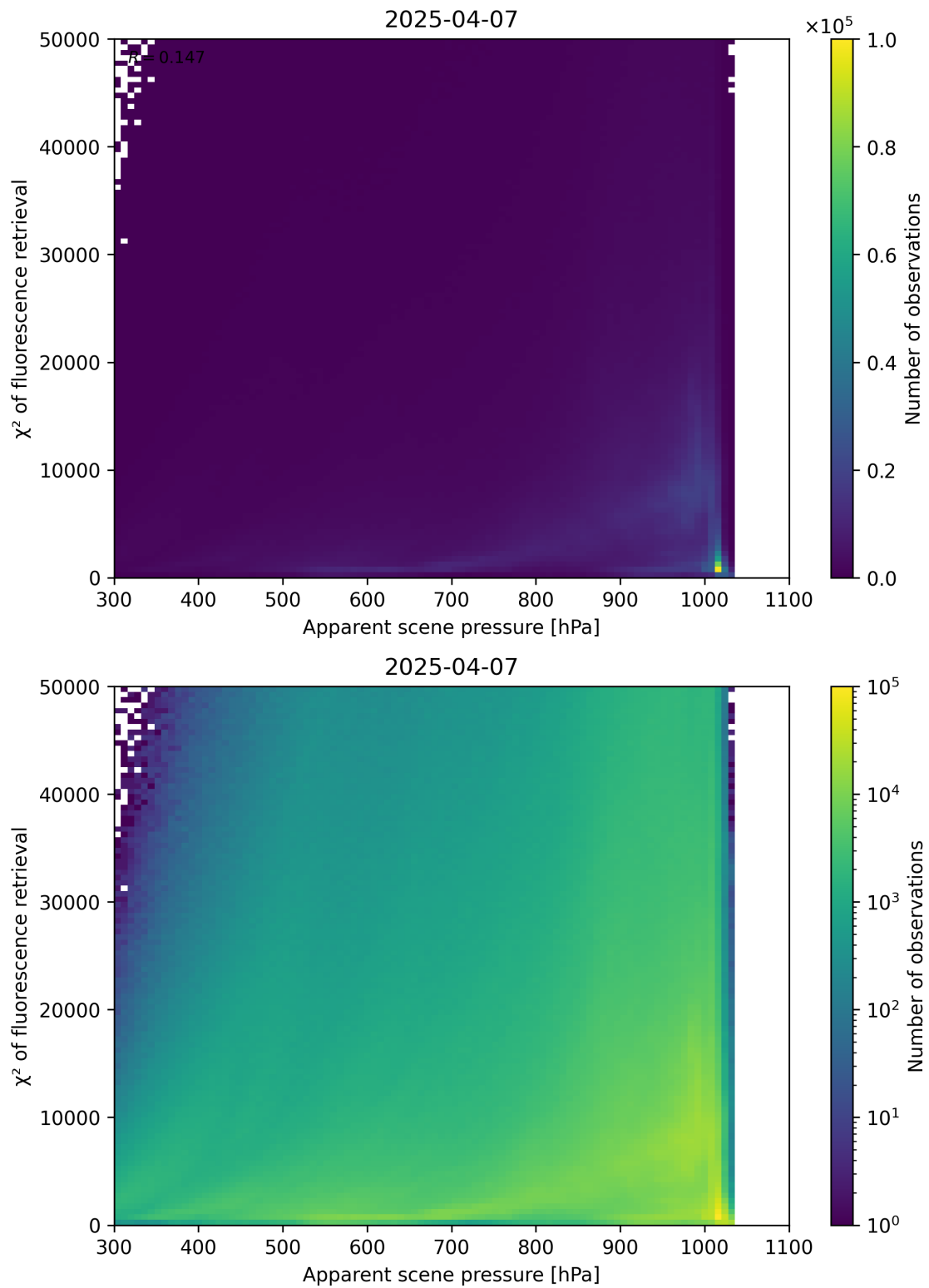
Figure 63: Scatter density plot of “Apparent scene pressure” against “ \chi^2 of fluorescence retrieval” for 2025-04-06 to 2025-04-08.
