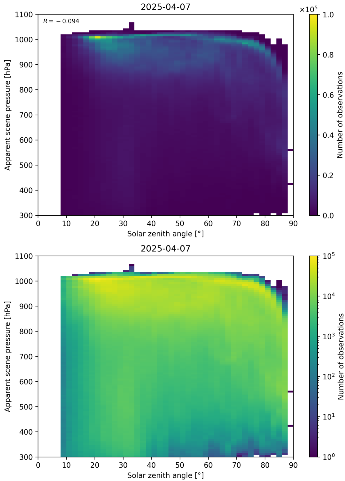
Figure 108: Scatter density plot of “Solar zenith angle” against “Apparent scene pressure” for 2025-04-06 to 2025-04-08.
