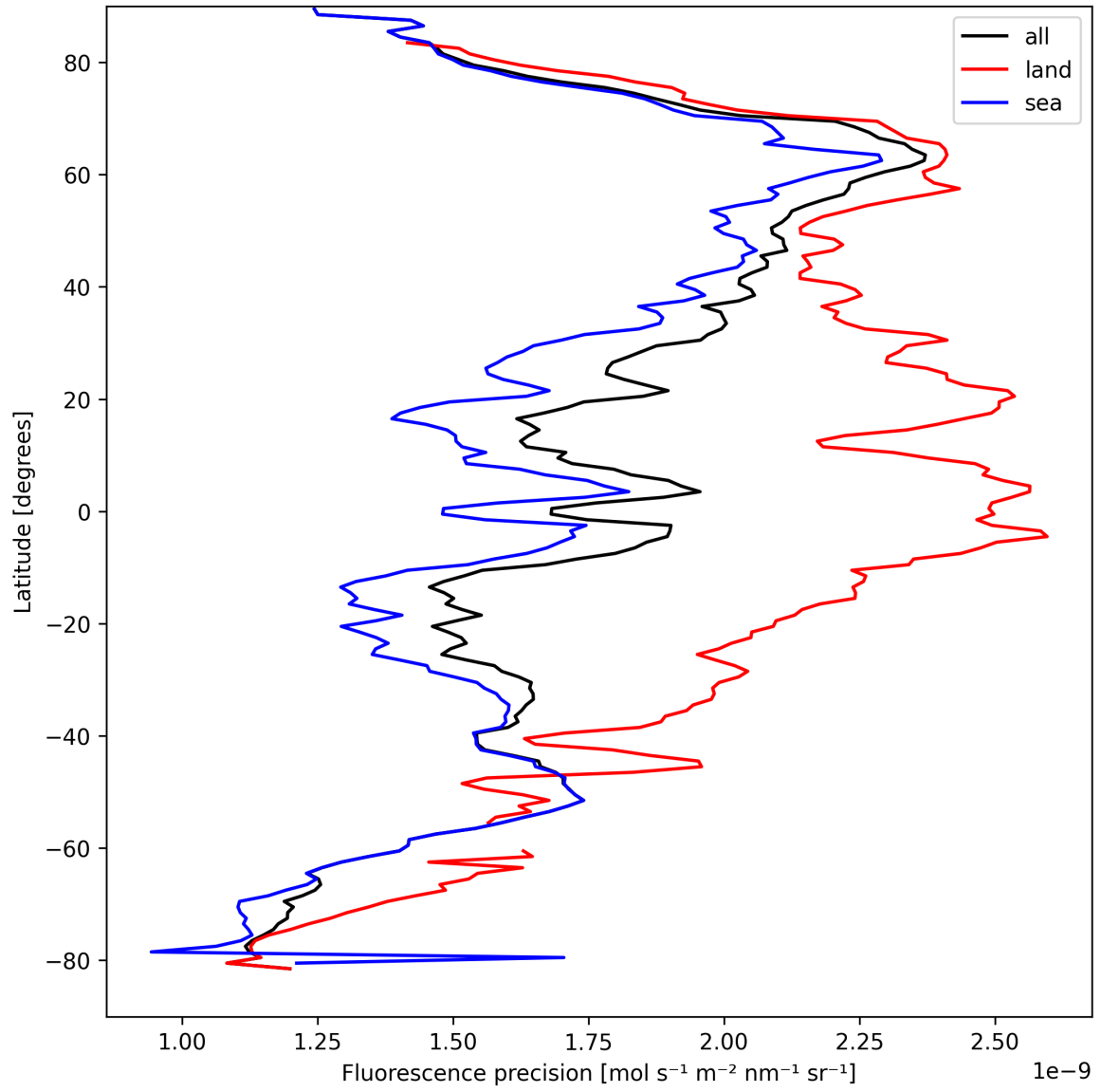
Figure 24: Zonal average of “Fluorescence precision” for 2025-04-06 to 2025-04-08.
