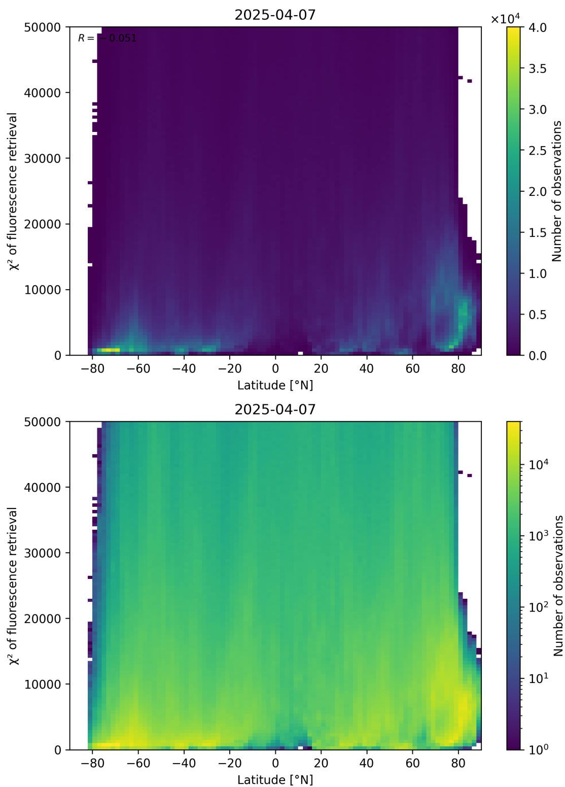
Figure 89: Scatter density plot of “Latitude” against “ \chi^2 of fluorescence retrieval” for 2025-04-06 to 2025-04-08.
