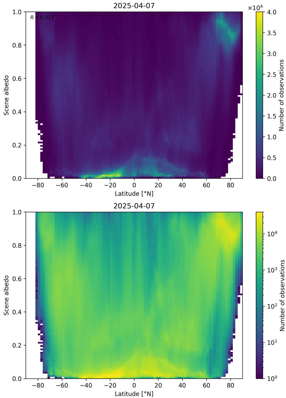
Figure 95: Scatter density plot of “Latitude” against “Scene albedo” for 2025-04-06 to 2025-04-08.
