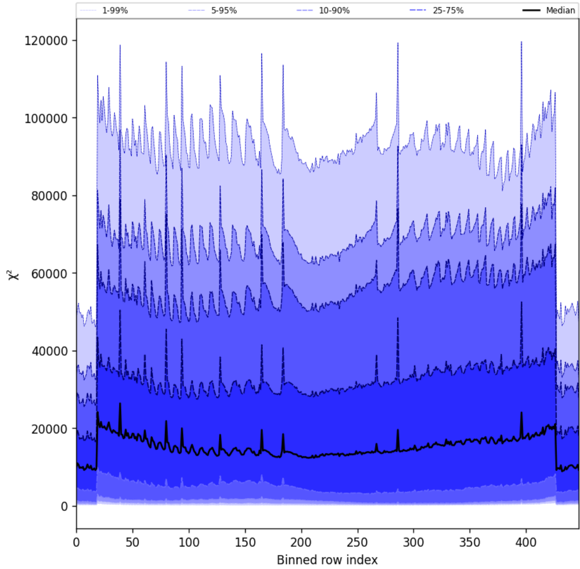
Figure 55: Along track statistics of “ \chi^2 ” for 2025-04-06 to 2025-04-08
