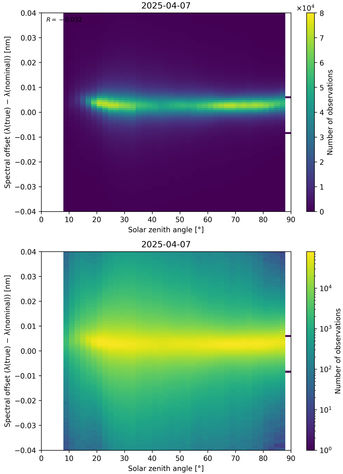
Figure 117: Scatter density plot of “Solar zenith angle” against “Spectral offset ( \lambda_{\text{true}} - \lambda_{\text{nominal}} )” for 2025-04-06 to 2025-04-08.
