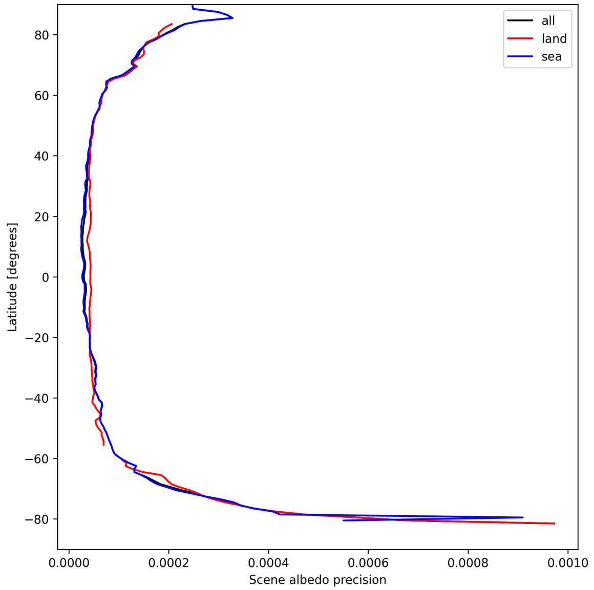
Figure 18: Zonal average of “Scene albedo precision” for 2025-04-06 to 2025-04-08.
