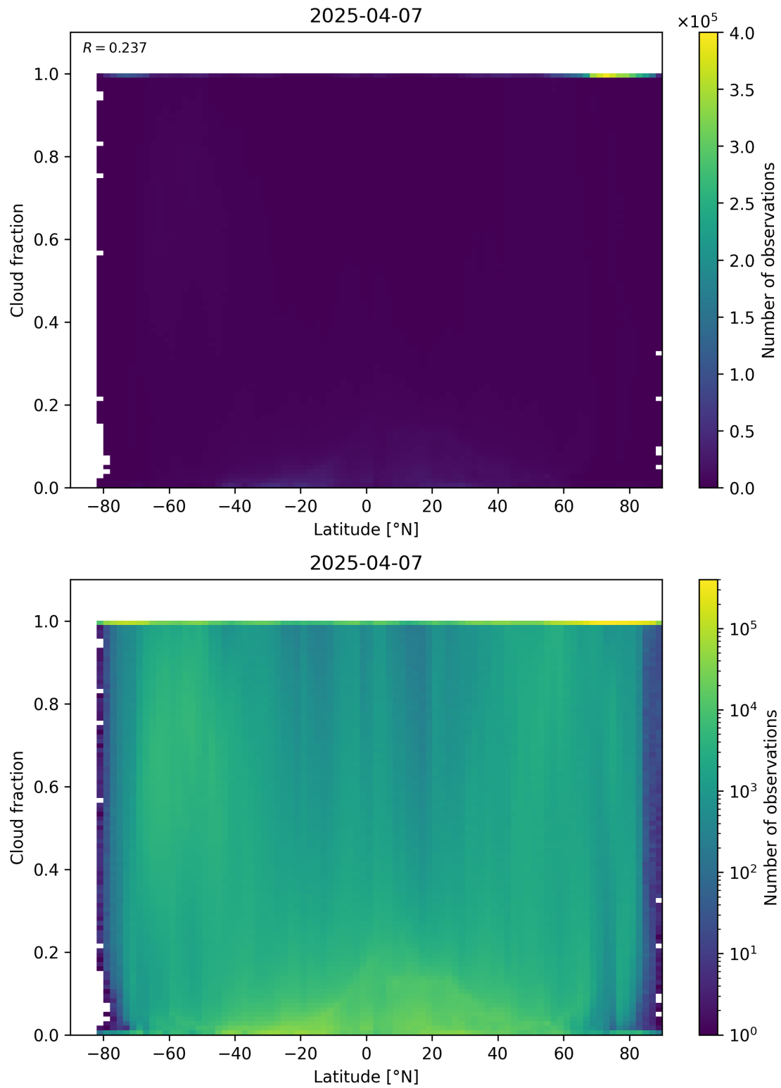
Figure 90: Scatter density plot of “Latitude” against “Cloud fraction” for 2025-04-06 to 2025-04-08.
