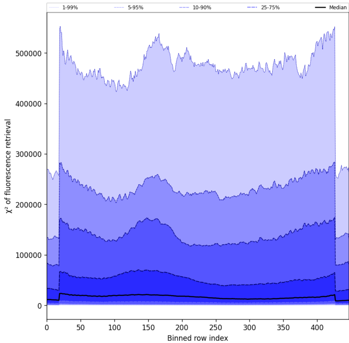
Figure 59: Along track statistics of “ \chi^2 of fluorescence retrieval” for 2025-04-06 to 2025-04-08
