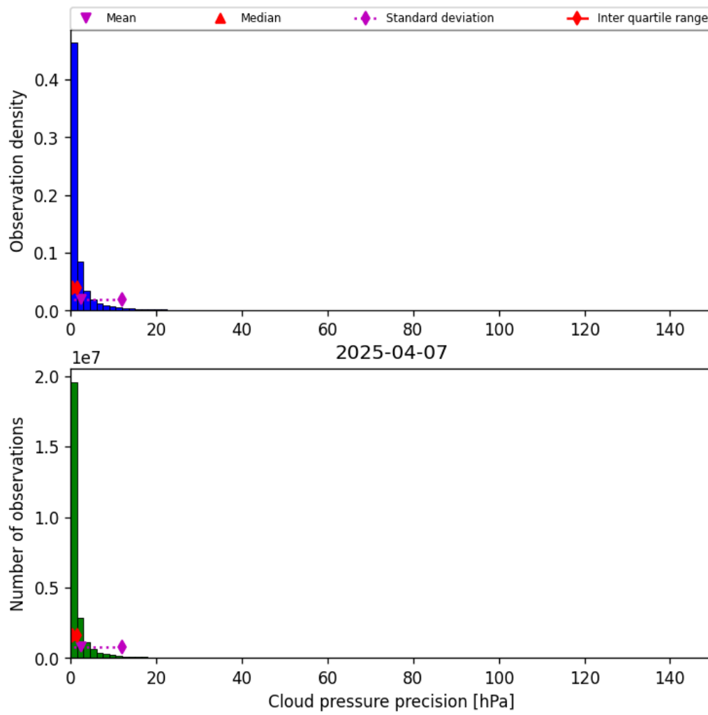
Figure 31: Histogram of “Cloud pressure precision” for 2025-04-06 to 2025-04-08
