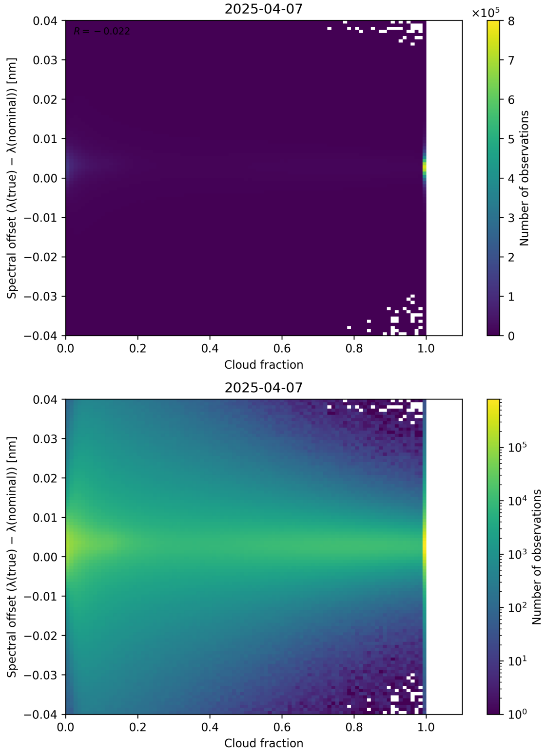
Figure 76: Scatter density plot of “Cloud fraction” against “Spectral offset ( \lambda_{\text{true}} - \lambda_{\text{nominal}} )” for 2025-04-06 to 2025-04-08.
