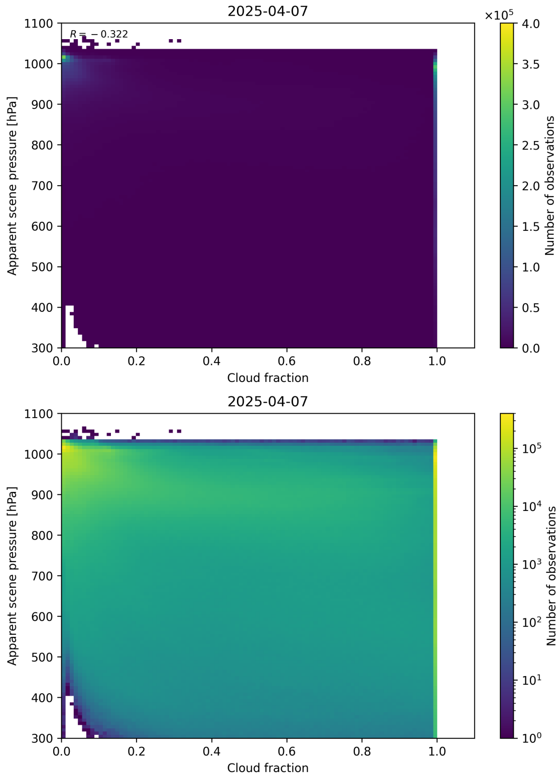
Figure 70: Scatter density plot of “Cloud fraction” against “Apparent scene pressure” for 2025-04-06 to 2025-04-08.
