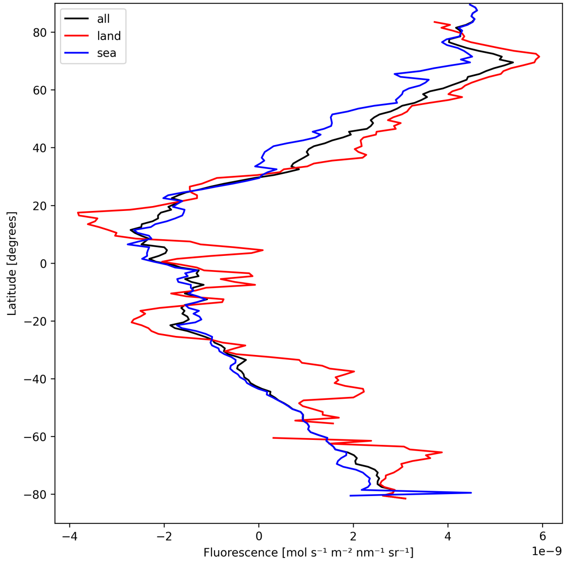
Figure 23: Zonal average of “Fluorescence” for 2025-04-06 to 2025-04-08.
