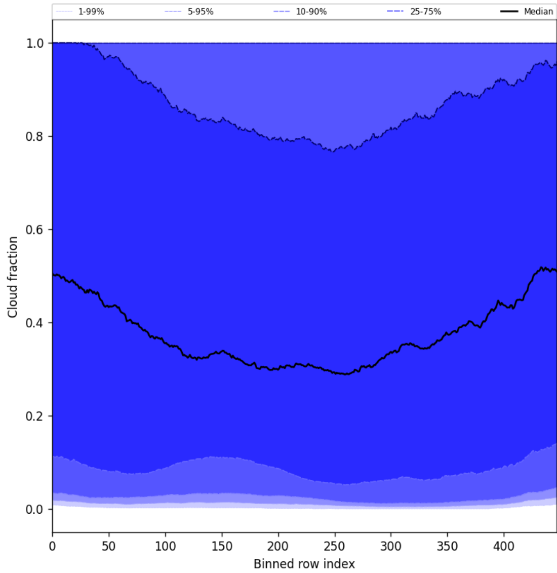
Figure 49: Along track statistics of “Cloud fraction” for 2025-04-06 to 2025-04-08
