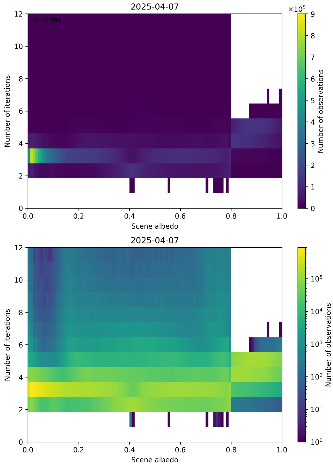
Figure 105: Scatter density plot of “Scene albedo” against “Number of iterations” for 2025-04-06 to 2025-04-08.
