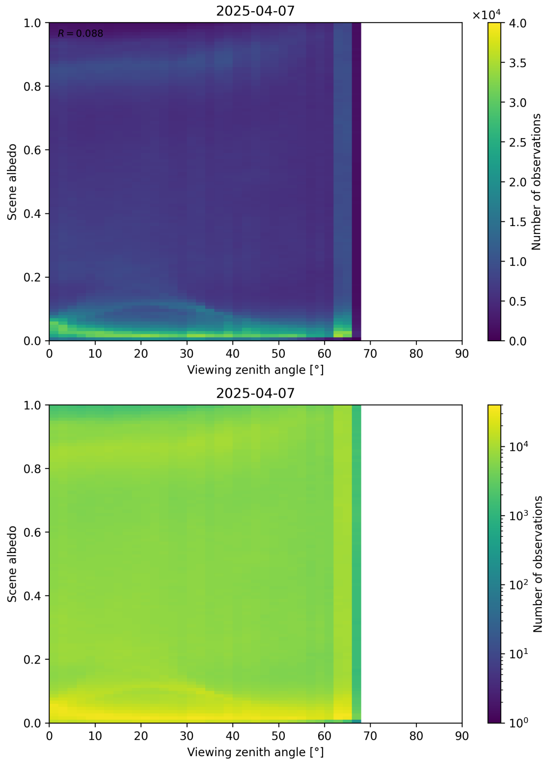
Figure 126: Scatter density plot of “Viewing zenith angle” against “Scene albedo” for 2025-04-06 to 2025-04-08.
