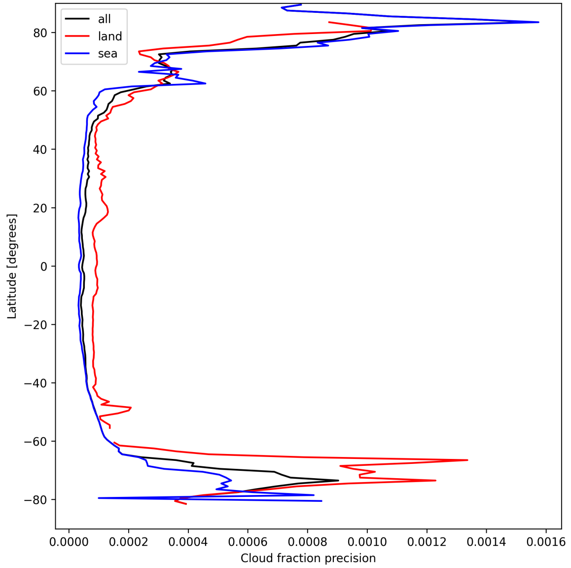
Figure 16: Zonal average of “Cloud fraction precision” for 2025-04-06 to 2025-04-08.
