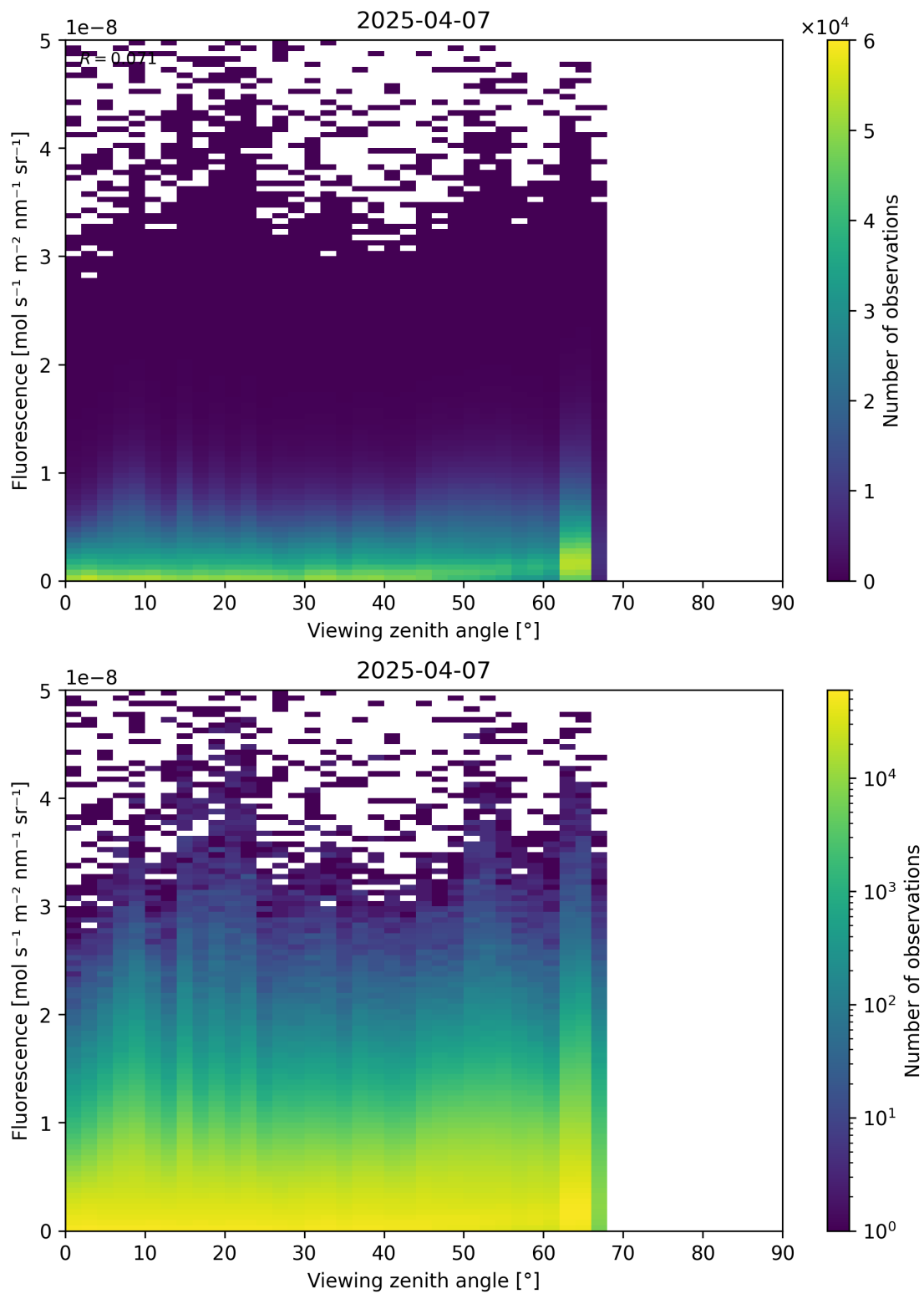
Figure 122: Scatter density plot of "Viewing zenith angle" against "Fluorescence" for 2025-04-06 to 2025-04-08.
