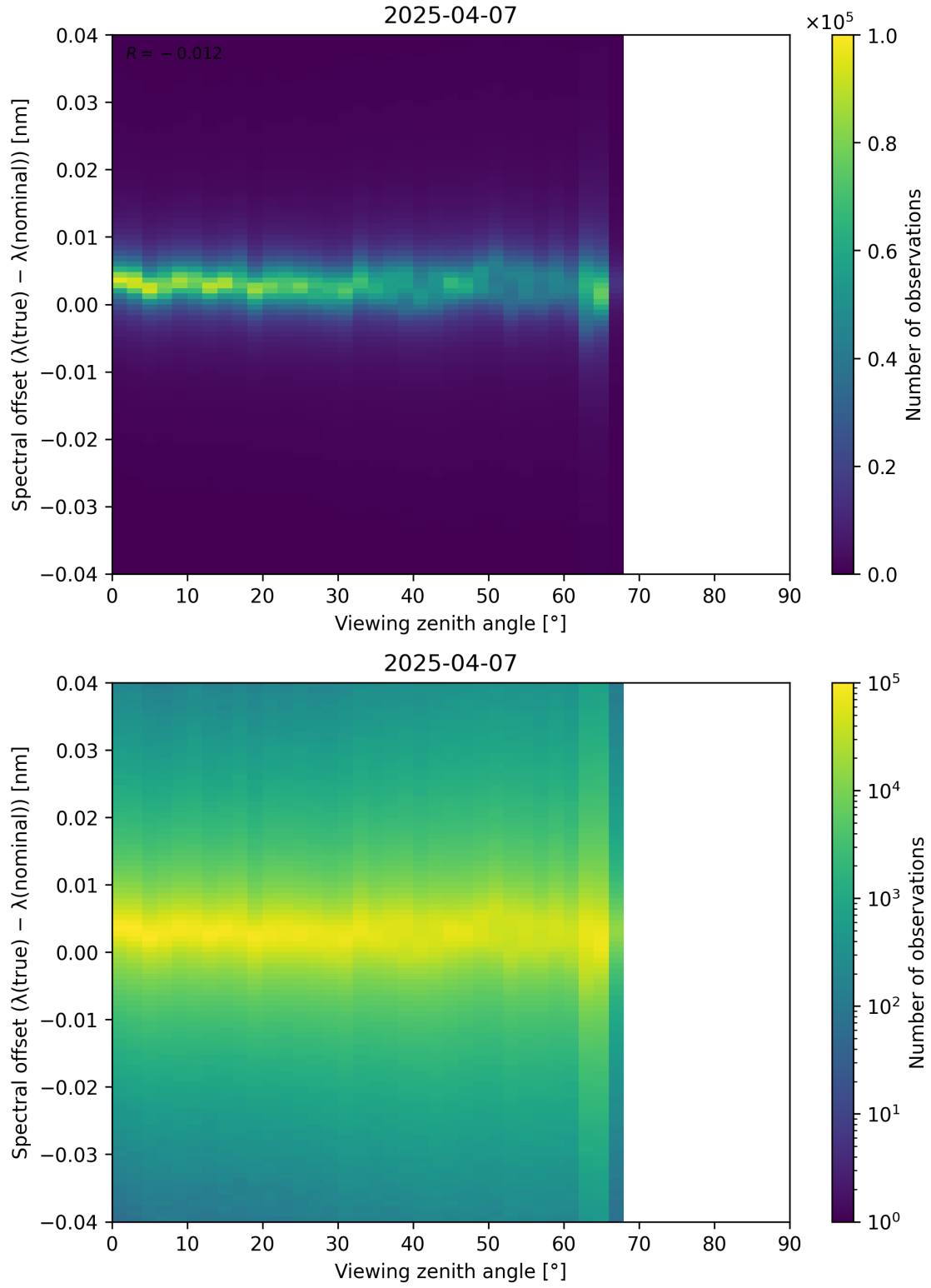
Figure 128: Scatter density plot of “Viewing zenith angle” against “Spectral offset ( \lambda_{\text{true}} - \lambda_{\text{nominal}} )” for 2025-04-06 to 2025-04-08.
