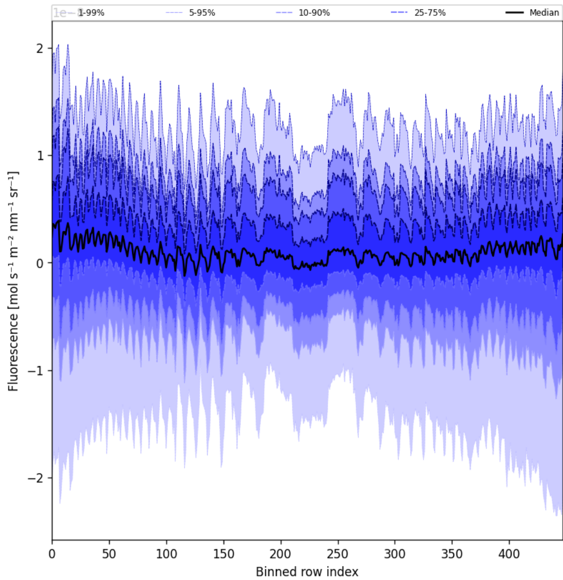
Figure 57: Along track statistics of “Fluorescence” for 2025-04-06 to 2025-04-08
