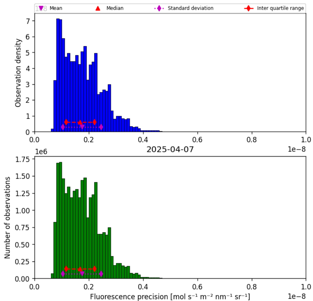
Figure 41: Histogram of “Fluorescence precision” for 2025-04-06 to 2025-04-08
