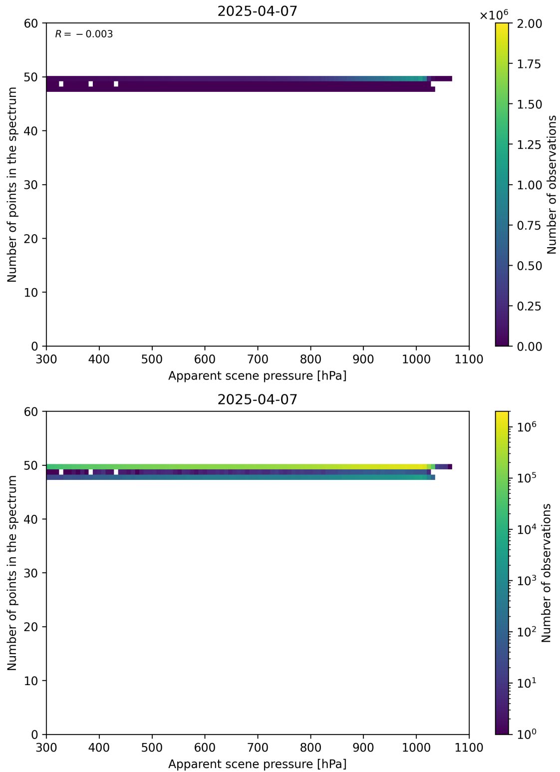
Figure 66: Scatter density plot of “Apparent scene pressure” against “Number of points in the spectrum” for 2025-04-06 to 2025-04-08.
