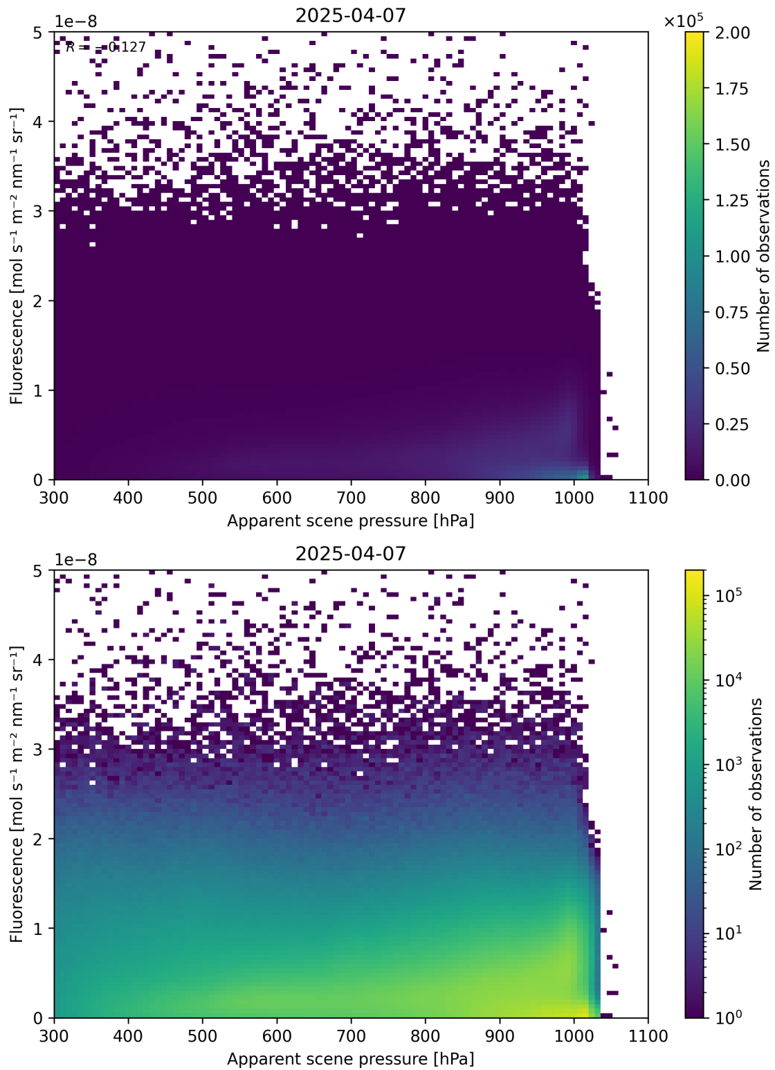
Figure 64: Scatter density plot of “Apparent scene pressure” against “Fluorescence” for 2025-04-06 to 2025-04-08.
