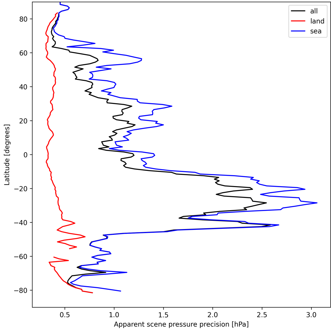
Figure 20: Zonal average of “Apparent scene pressure precision” for 2025-04-06 to 2025-04-08.
