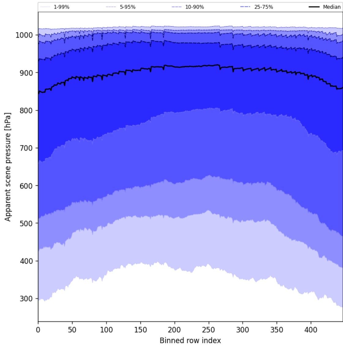
Figure 53: Along track statistics of “Apparent scene pressure” for 2025-04-06 to 2025-04-08
