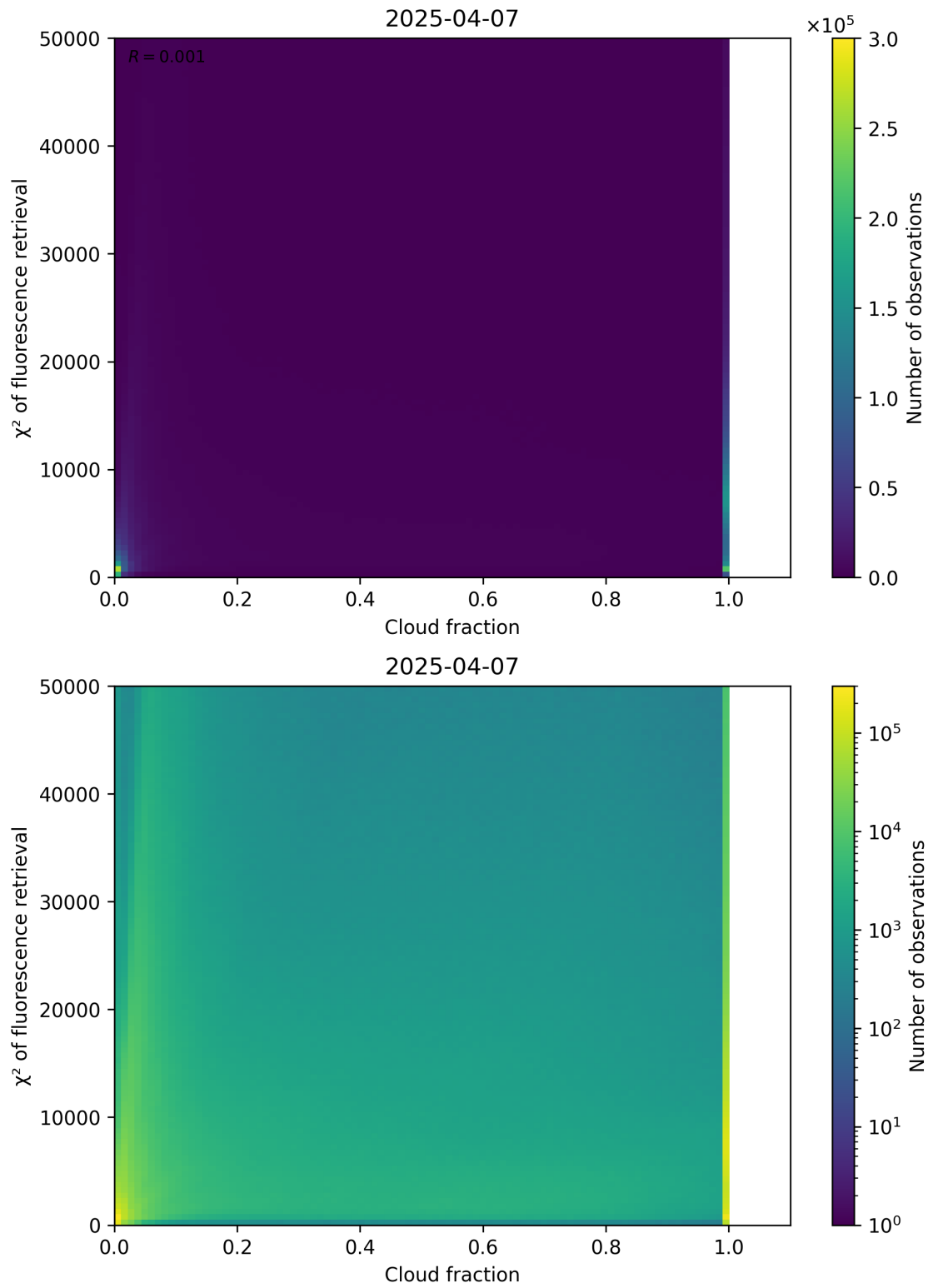
Figure 71: Scatter density plot of “Cloud fraction” against “ \chi^2 of fluorescence retrieval” for 2025-04-06 to 2025-04-08.
