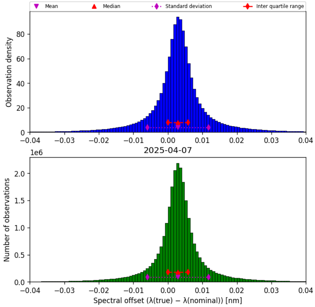
Figure 45: Histogram of “Spectral offset ( \lambda_{\text{true}} - \lambda_{\text{nominal}} )” for 2025-04-06 to 2025-04-08
