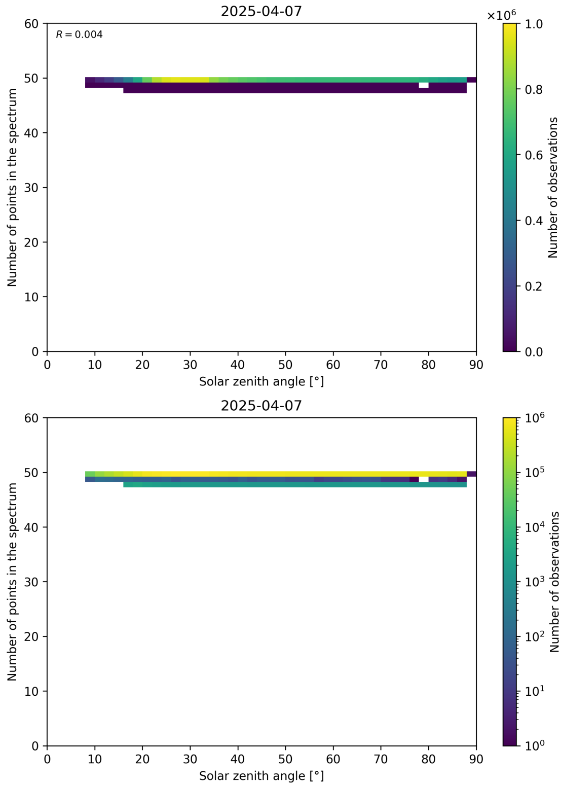
Figure 115: Scatter density plot of “Solar zenith angle” against “Number of points in the spectrum” for 2025-04-06 to 2025-04-08.
