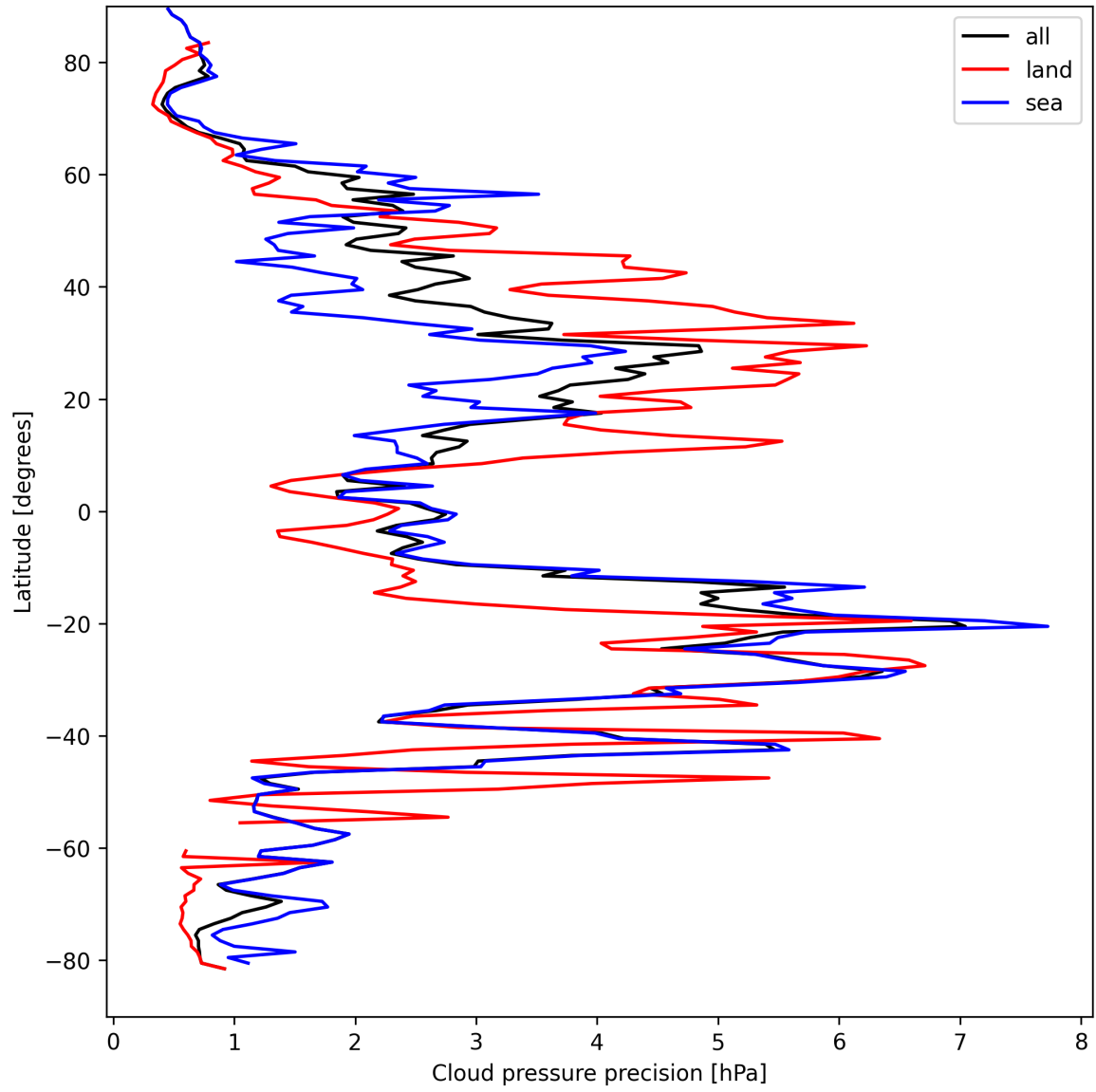
Figure 14: Zonal average of "Cloud pressure precision" for 2025-04-06 to 2025-04-08.
