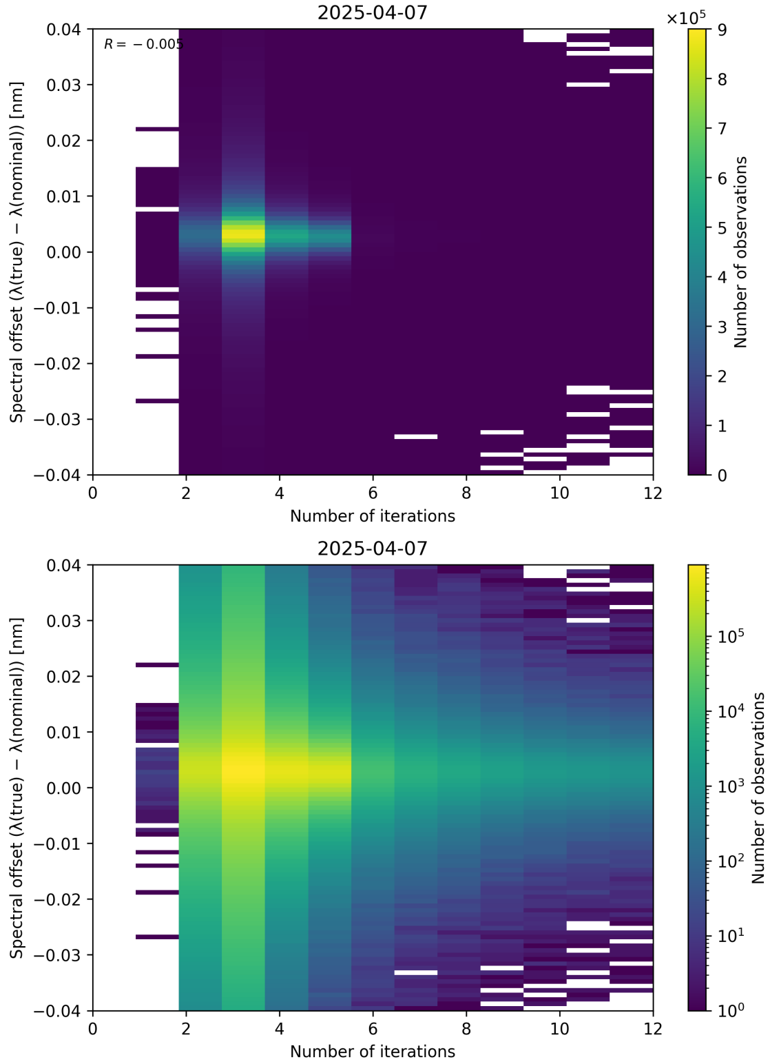
Figure 100: Scatter density plot of “Number of iterations” against “Spectral offset ( \lambda_{\text{true}} - \lambda_{\text{nominal}} )” for 2025-04-06 to 2025-04-08.
