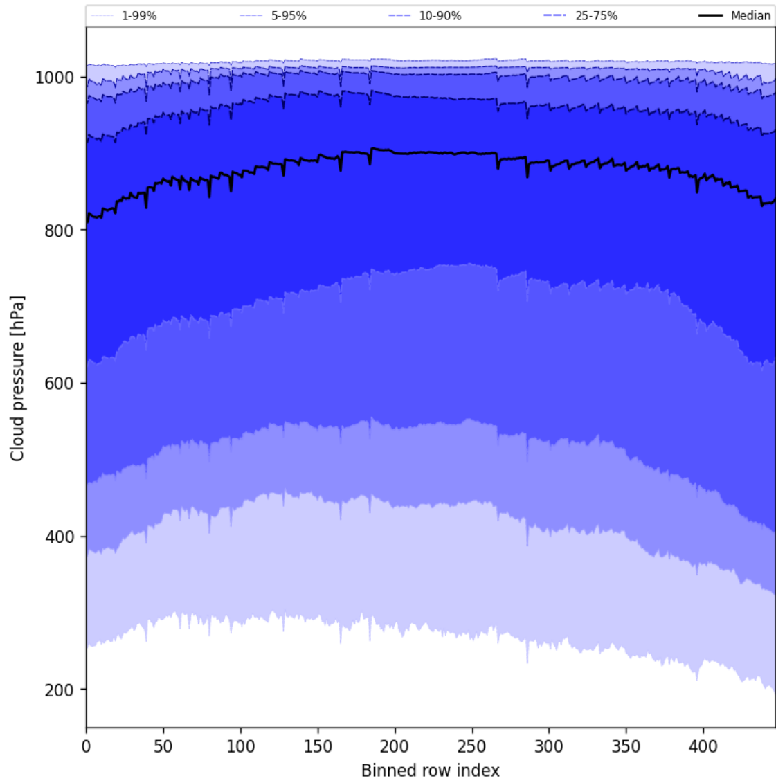
Figure 47: Along track statistics of “Cloud pressure” for 2025-04-06 to 2025-04-08
