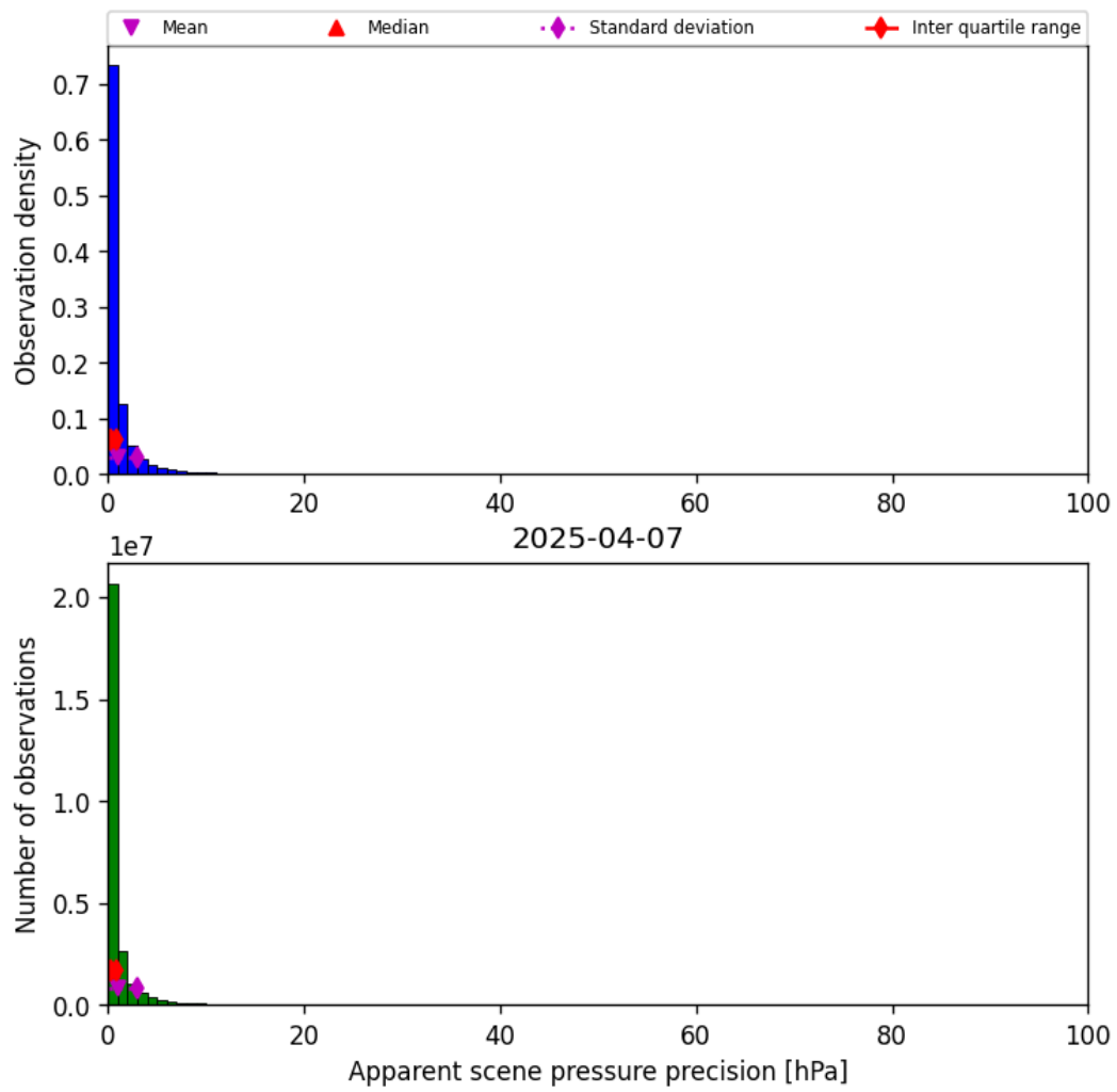
Figure 37: Histogram of “Apparent scene pressure precision” for 2025-04-06 to 2025-04-08
