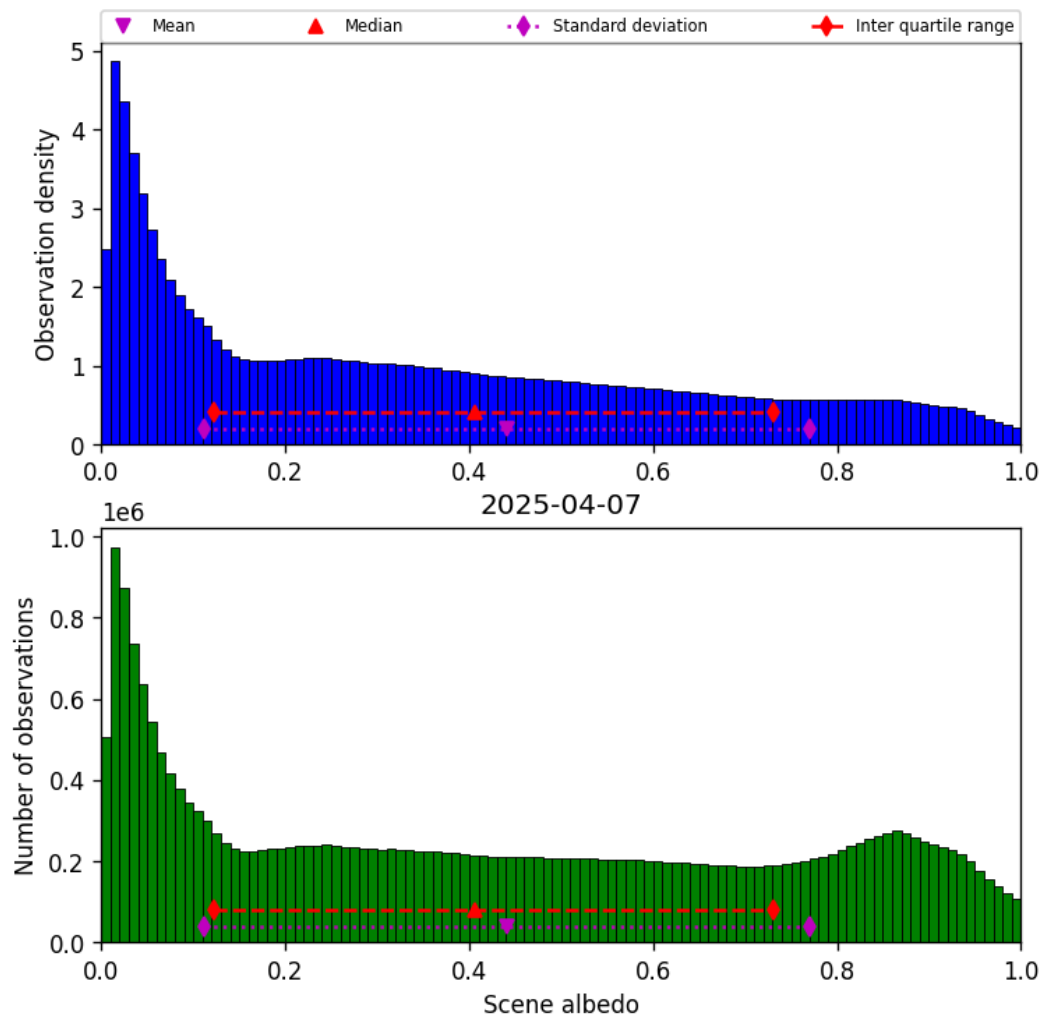
Figure 34: Histogram of “Scene albedo” for 2025-04-06 to 2025-04-08
