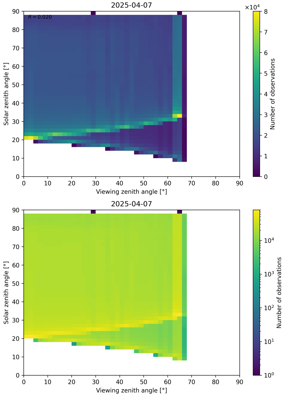
Figure 127: Scatter density plot of “Viewing zenith angle” against “Solar zenith angle” for 2025-04-06 to 2025-04-08.
