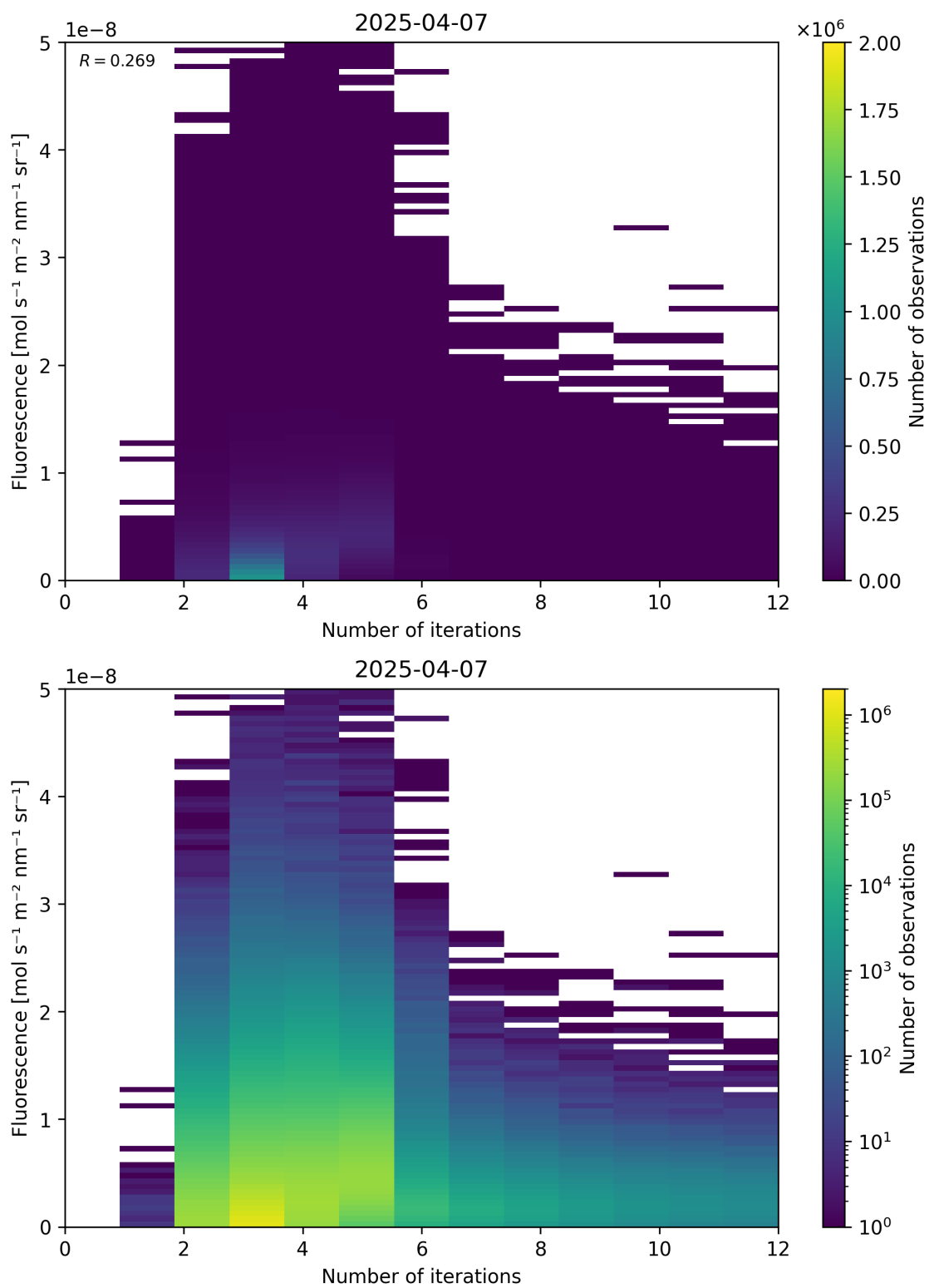
Figure 98: Scatter density plot of “Number of iterations” against “Fluorescence” for 2025-04-06 to 2025-04-08.
