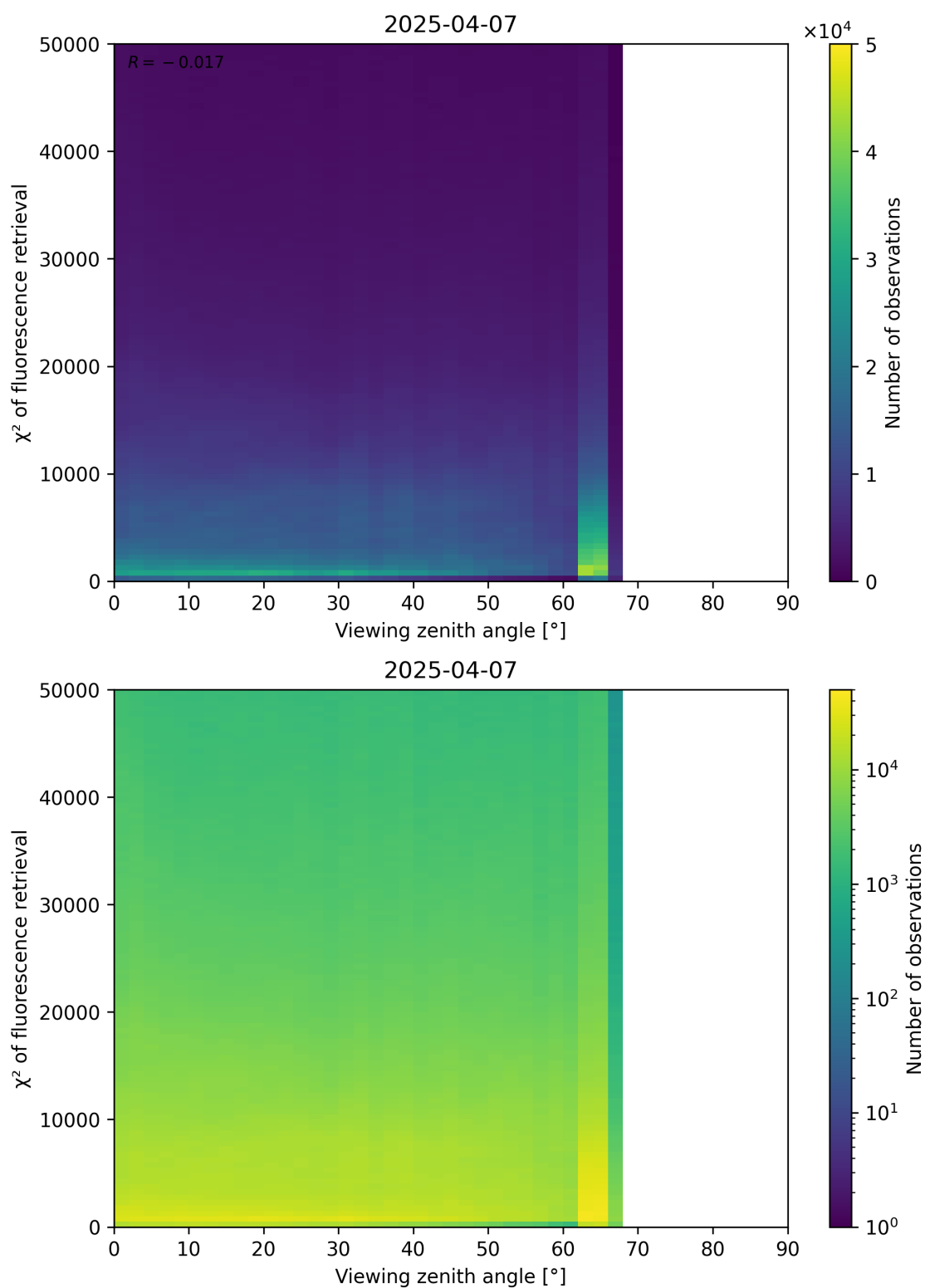
Figure 119: Scatter density plot of “Viewing zenith angle” against “ \chi^2 of fluorescence retrieval” for 2025-04-06 to 2025-04-08.
