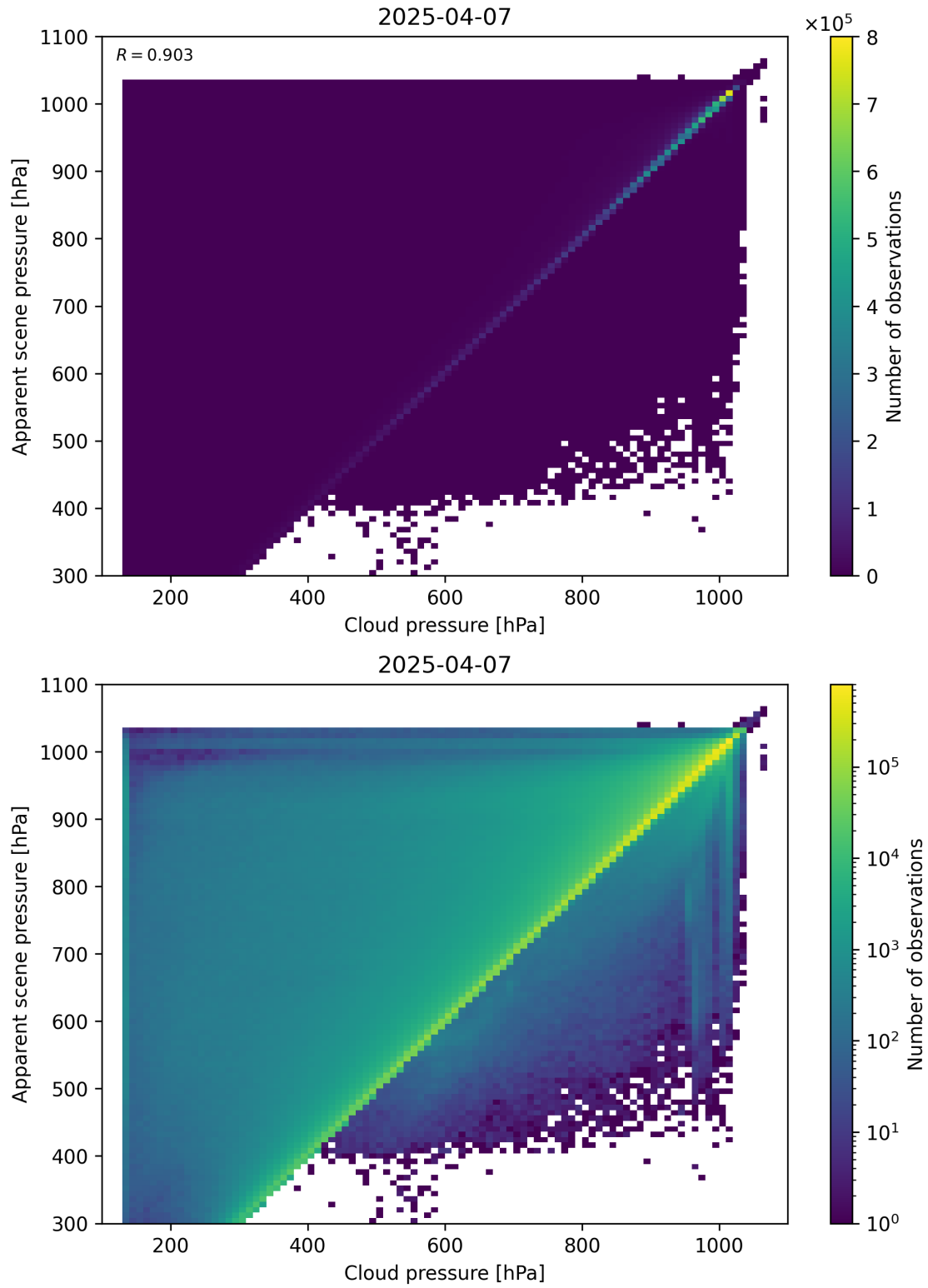
Figure 77: Scatter density plot of “Cloud pressure” against “Apparent scene pressure” for 2025-04-06 to 2025-04-08.
