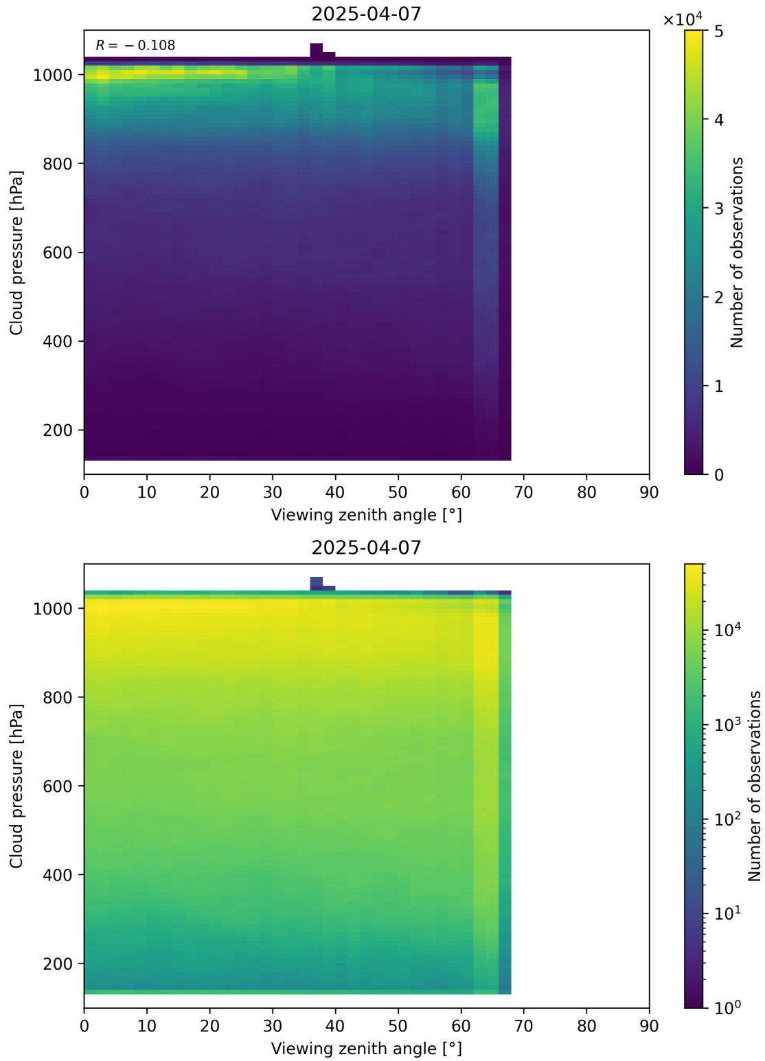
Figure 121: Scatter density plot of “Viewing zenith angle” against “Cloud pressure” for 2025-04-06 to 2025-04-08.
