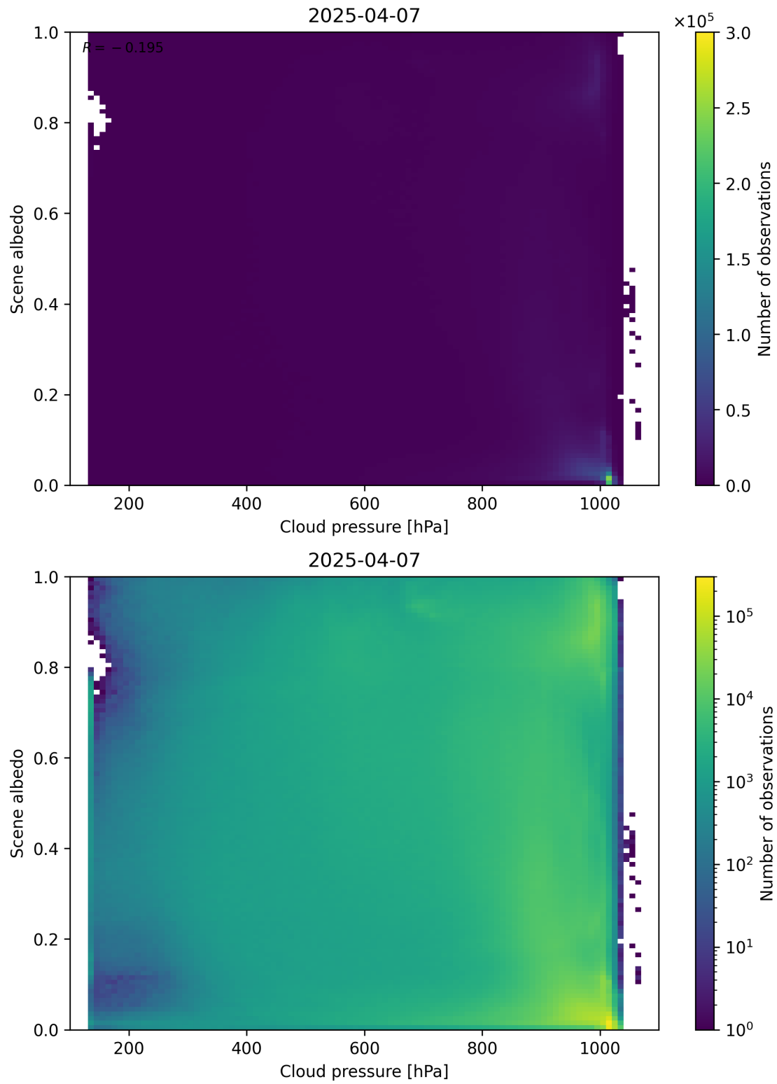
Figure 83: Scatter density plot of “Cloud pressure” against “Scene albedo” for 2025-04-06 to 2025-04-08.
