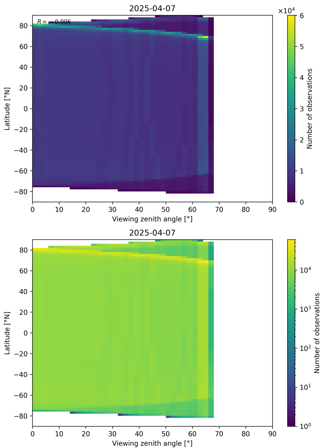
Figure 123: Scatter density plot of “Viewing zenith angle” against “Latitude” for 2025-04-06 to 2025-04-08.
