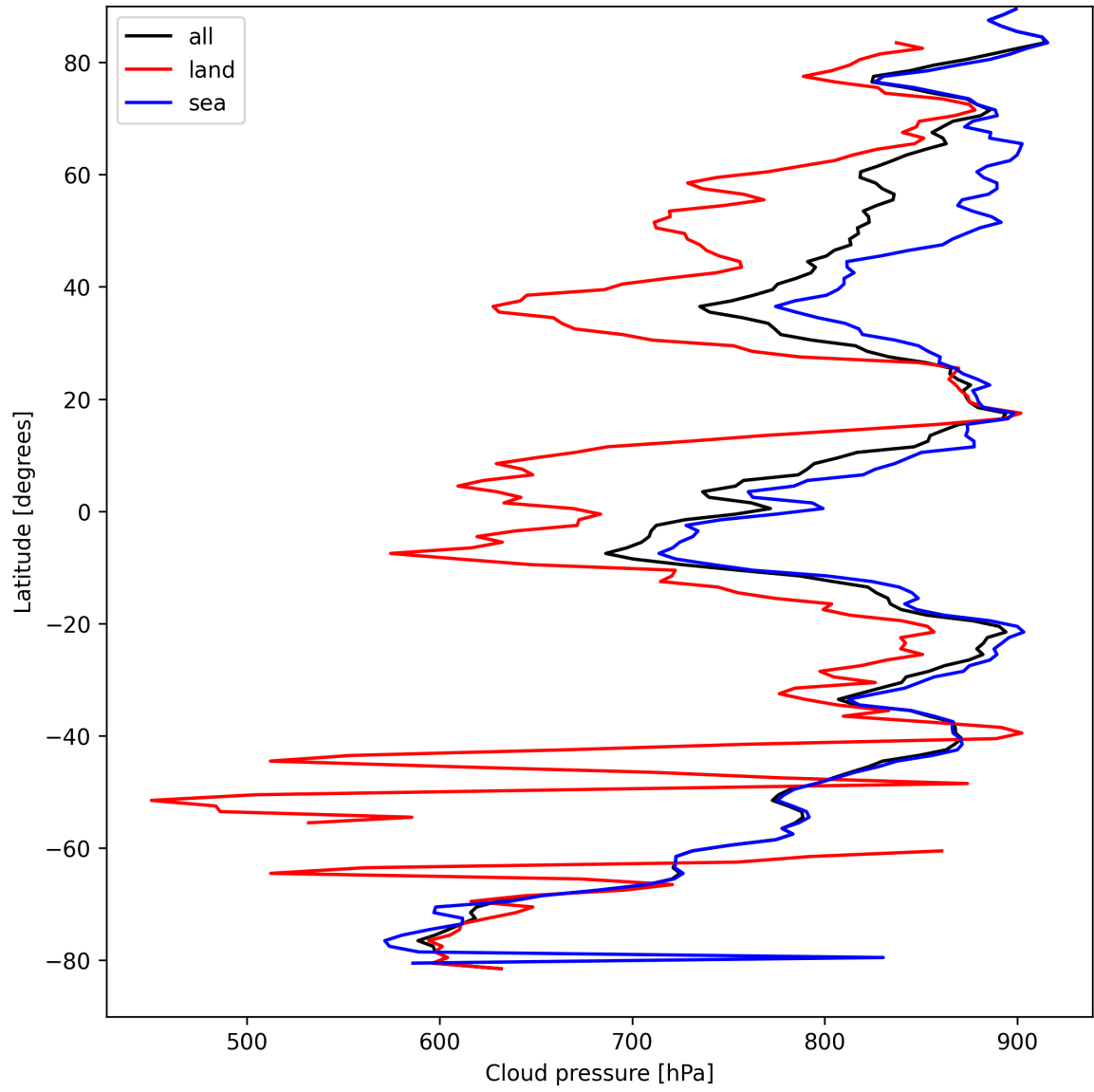
Figure 13: Zonal average of “Cloud pressure” for 2025-04-06 to 2025-04-08.
