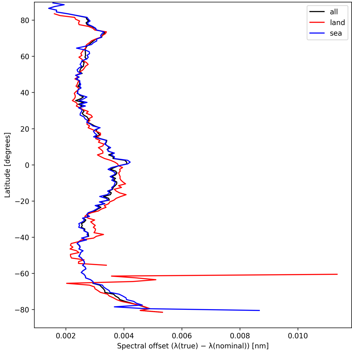
Figure 28: Zonal average of “Spectral offset ( \lambda_{\text{true}} - \lambda_{\text{nominal}} )” for 2025-04-06 to 2025-04-08.
