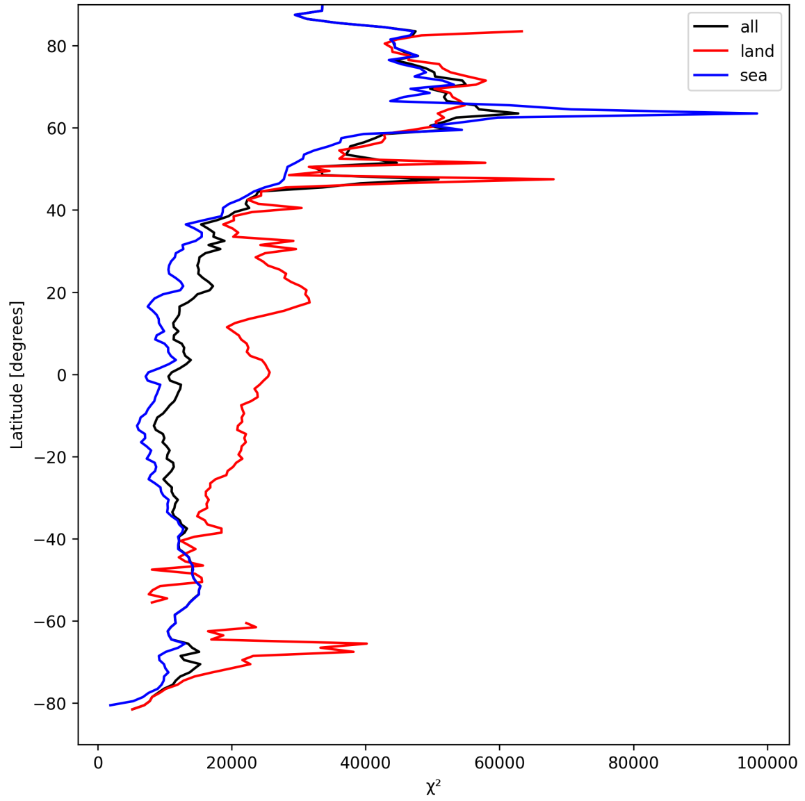
Figure 21: Zonal average of “ \chi^2 ” for 2025-04-06 to 2025-04-08.
