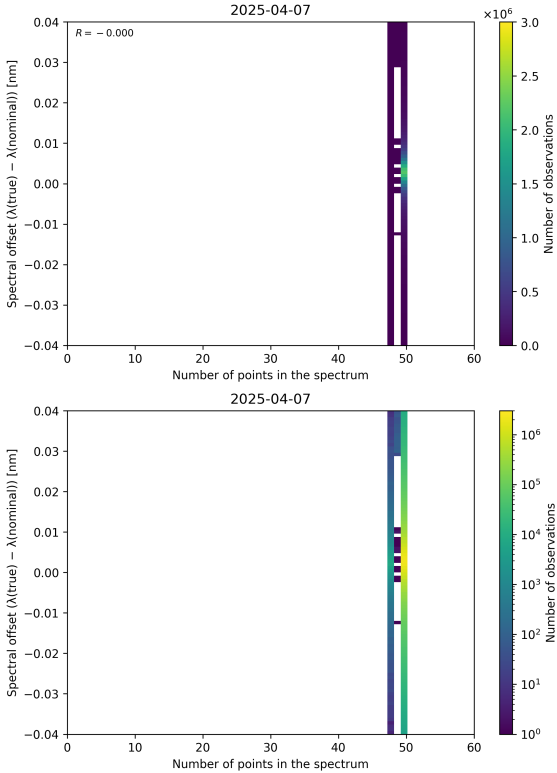
Figure 101: Scatter density plot of “Number of points in the spectrum” against “Spectral offset ( \lambda_{\text{true}} - \lambda_{\text{nominal}} )” for 2025-04-06 to 2025-04-08.
