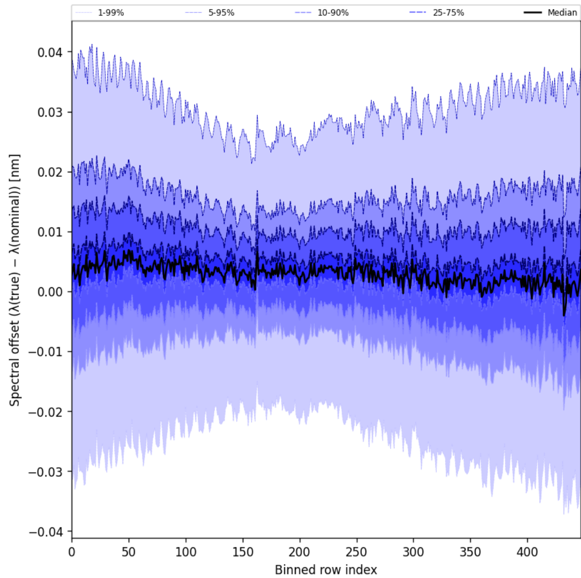
Figure 62: Along track statistics of “Spectral offset ( \lambda_{\text{true}} - \lambda_{\text{nominal}} )” for 2025-04-06 to 2025-04-08
