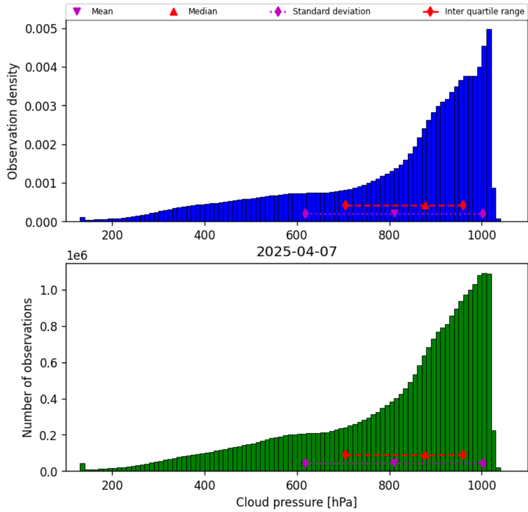
Figure 30: Histogram of “Cloud pressure” for 2025-04-06 to 2025-04-08
