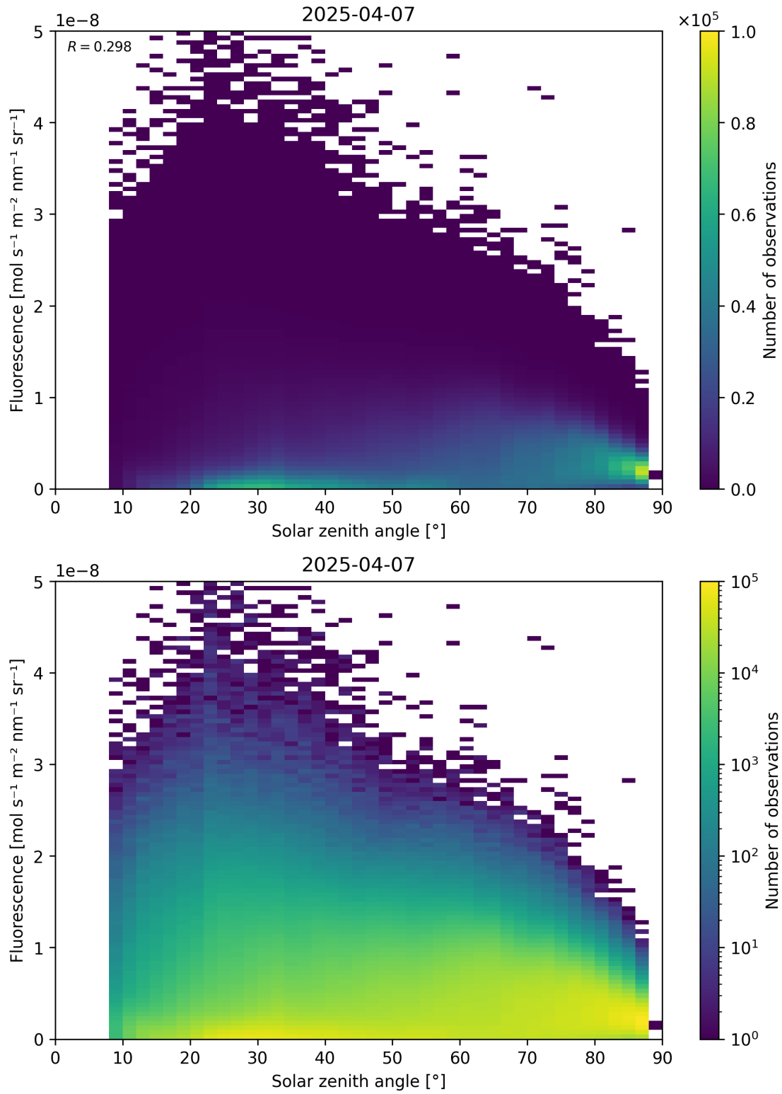
Figure 112: Scatter density plot of “Solar zenith angle” against “Fluorescence” for 2025-04-06 to 2025-04-08.
