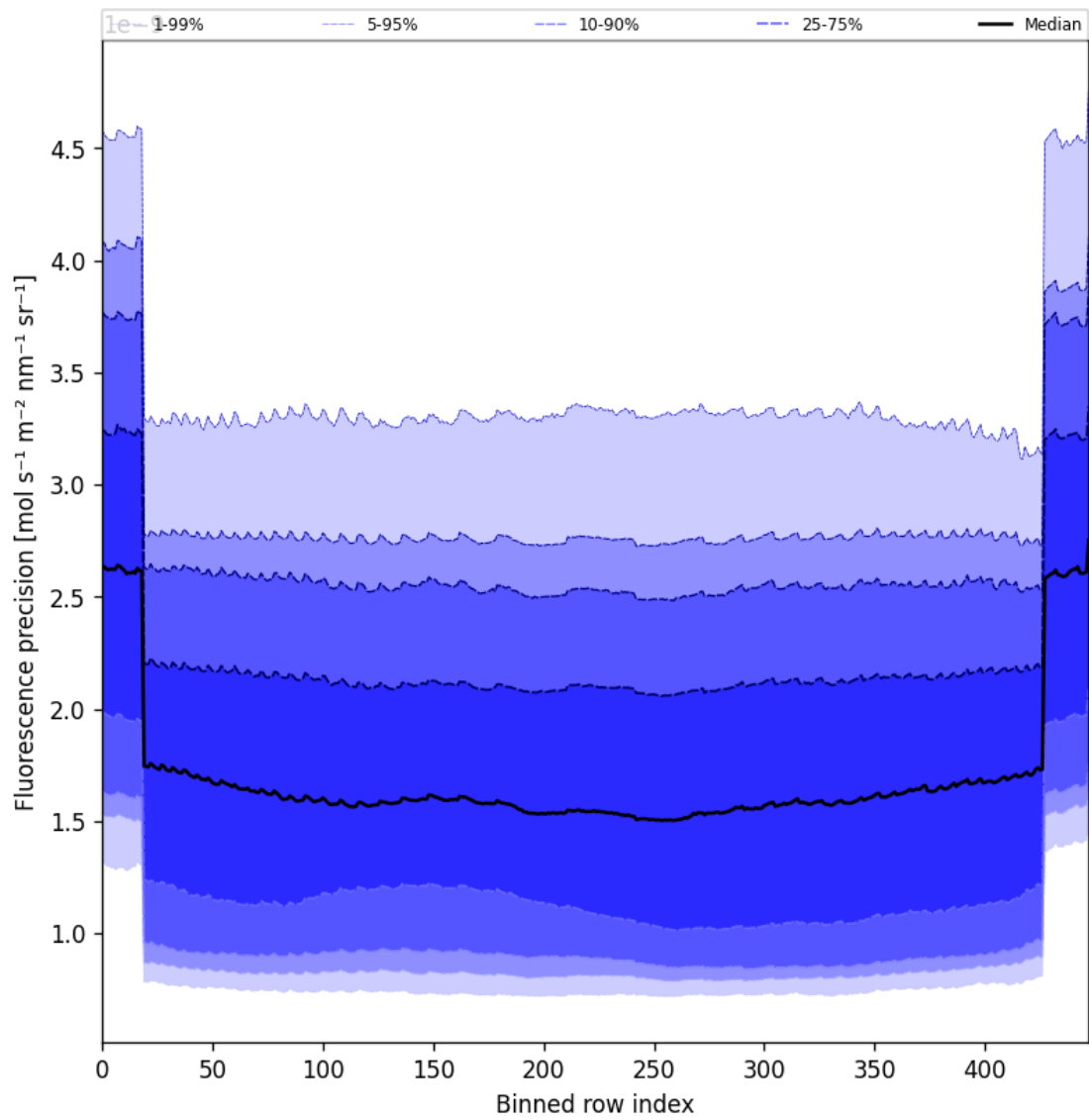
Figure 58: Along track statistics of “Fluorescence precision” for 2025-04-06 to 2025-04-08
