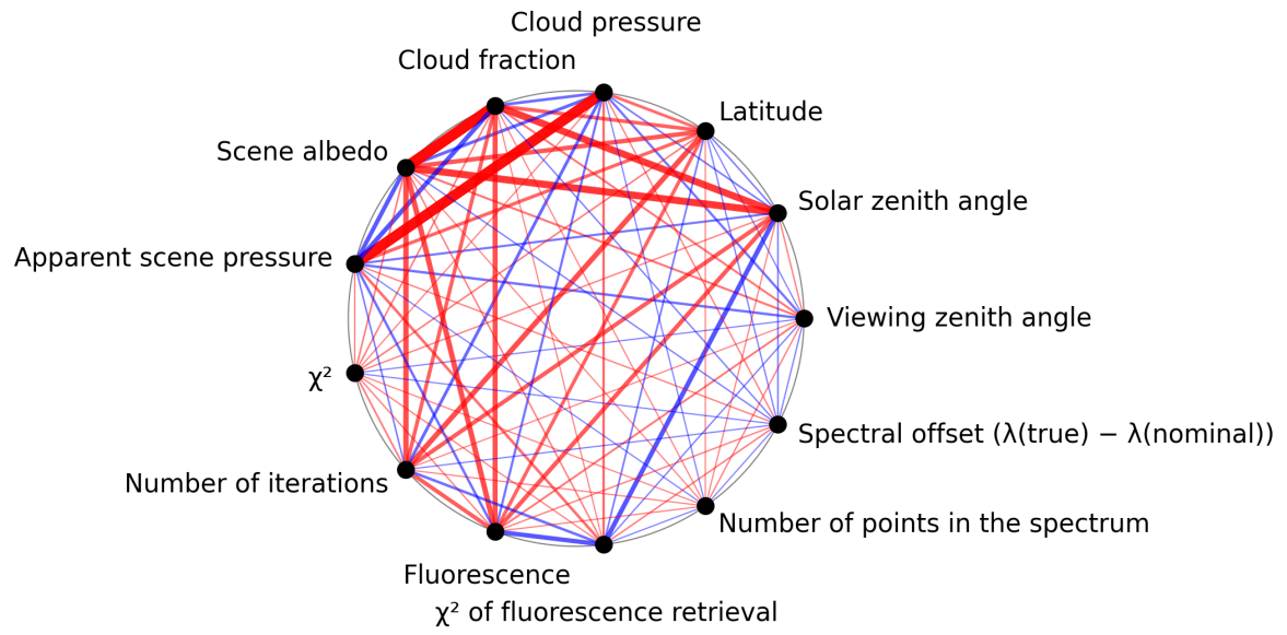
Figure 1: Map of correlation graph for 2025-04-06 to 2025-04-08.
