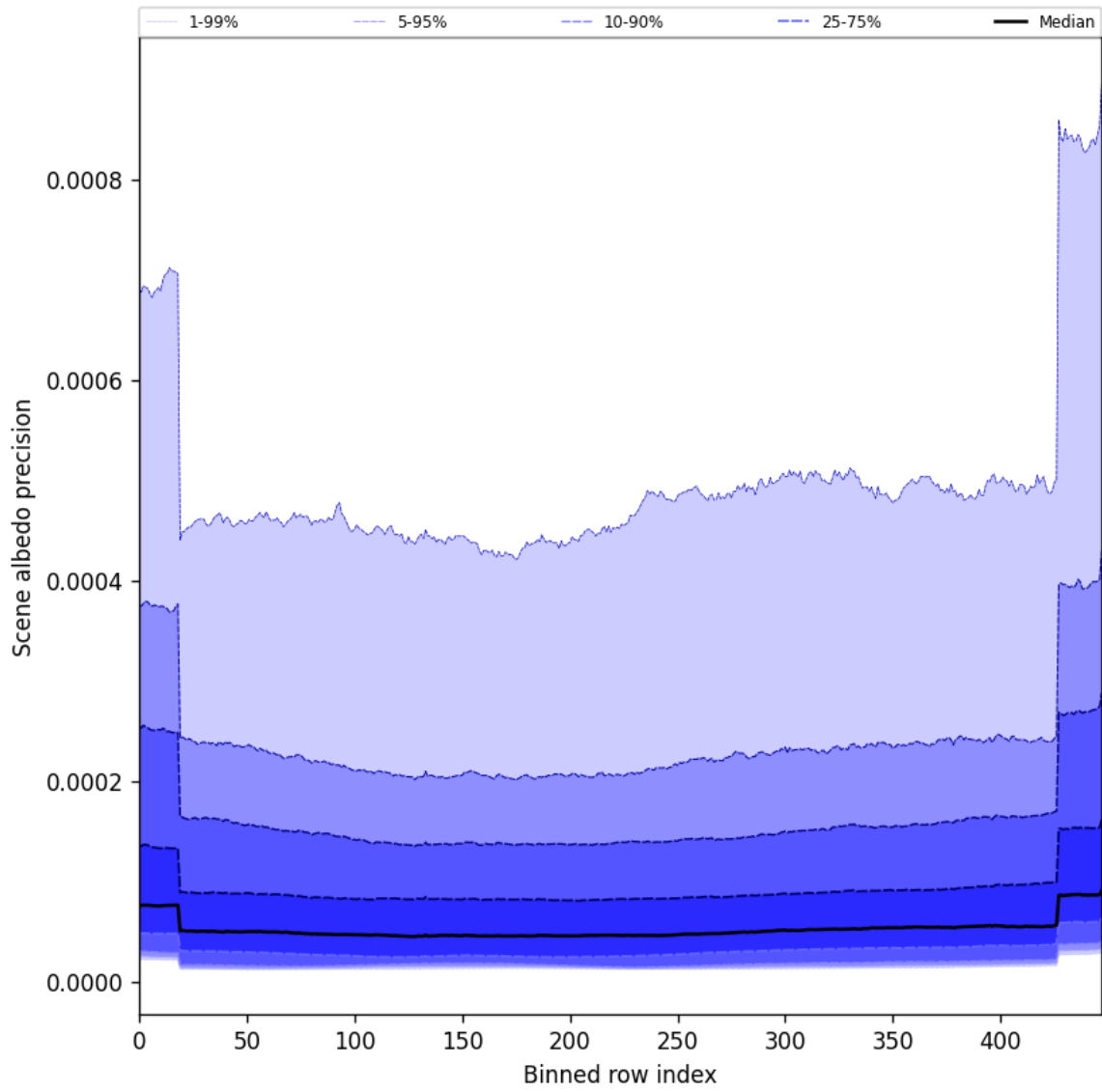
Figure 52: Along track statistics of “Scene albedo precision” for 2025-04-06 to 2025-04-08
