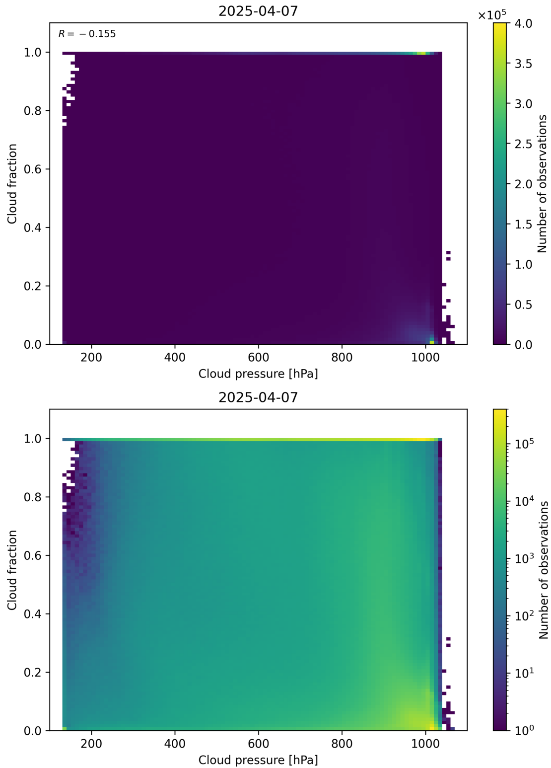
Figure 79: Scatter density plot of “Cloud pressure” against “Cloud fraction” for 2025-04-06 to 2025-04-08.
