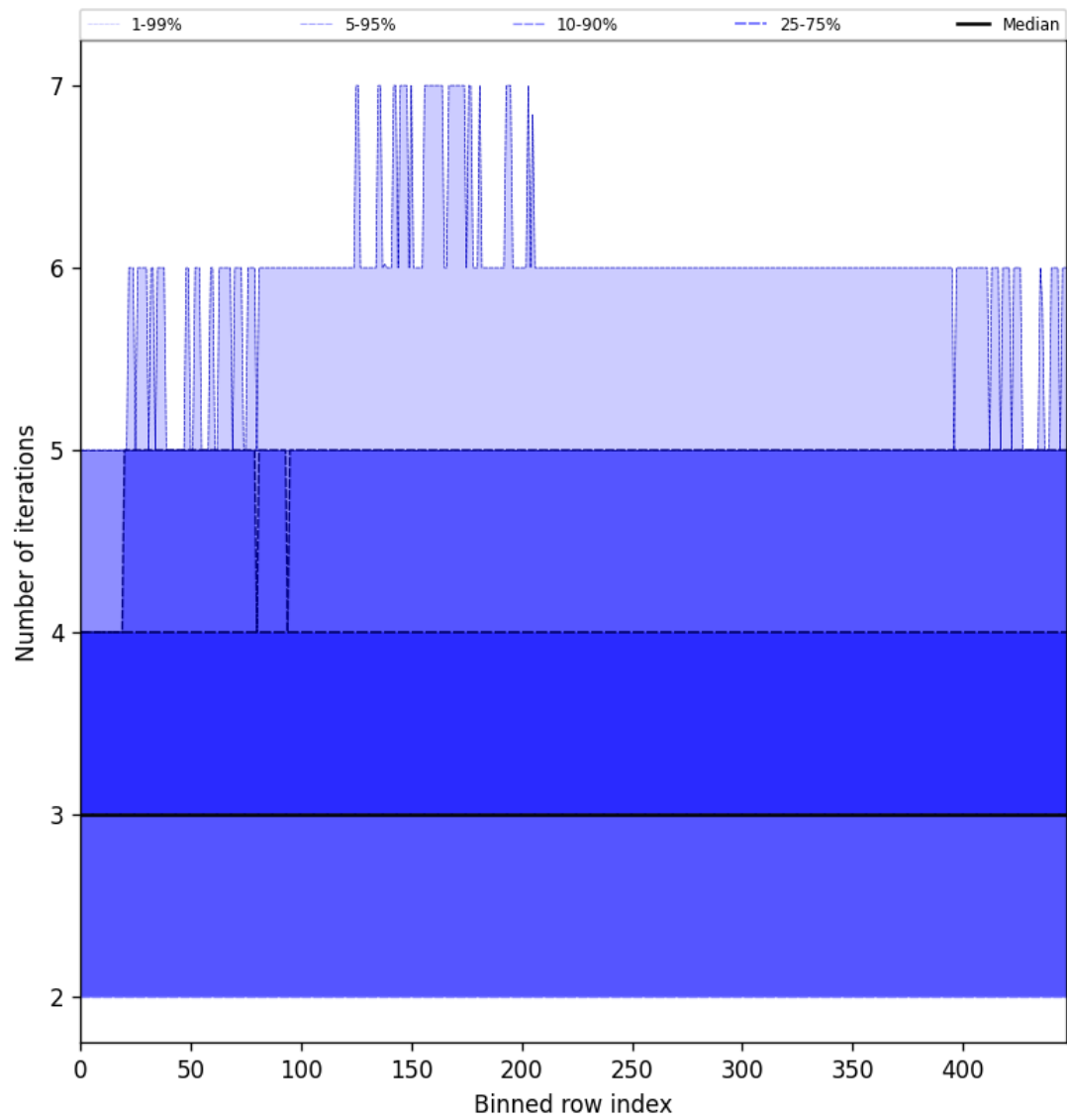
Figure 56: Along track statistics of “Number of iterations” for 2025-04-06 to 2025-04-08
