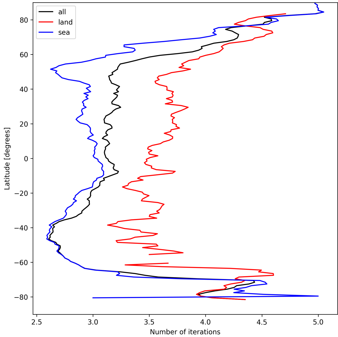
Figure 22: Zonal average of “Number of iterations” for 2025-04-06 to 2025-04-08.
