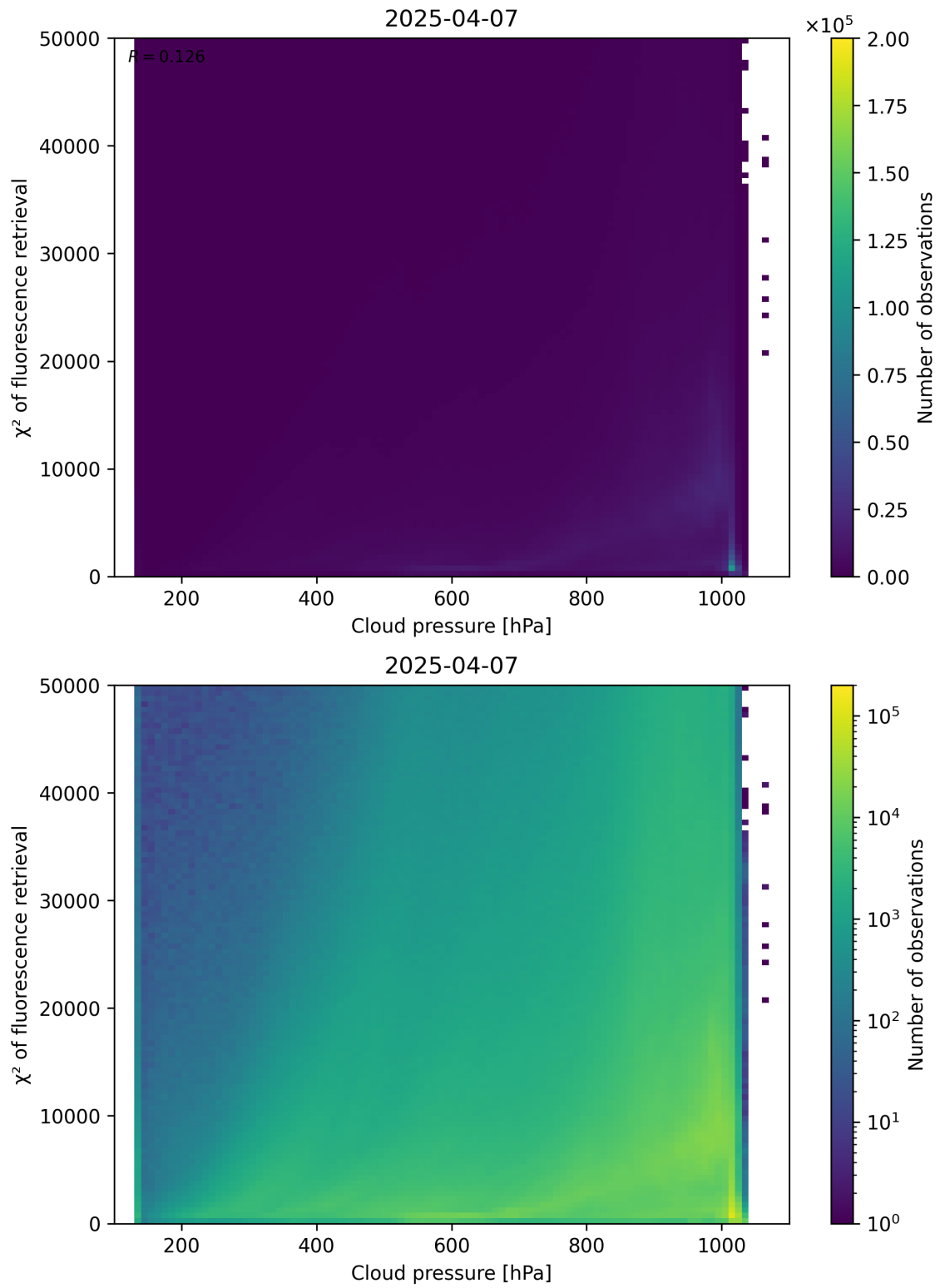
Figure 78: Scatter density plot of “Cloud pressure” against “ \chi^2 of fluorescence retrieval” for 2025-04-06 to 2025-04-08.
