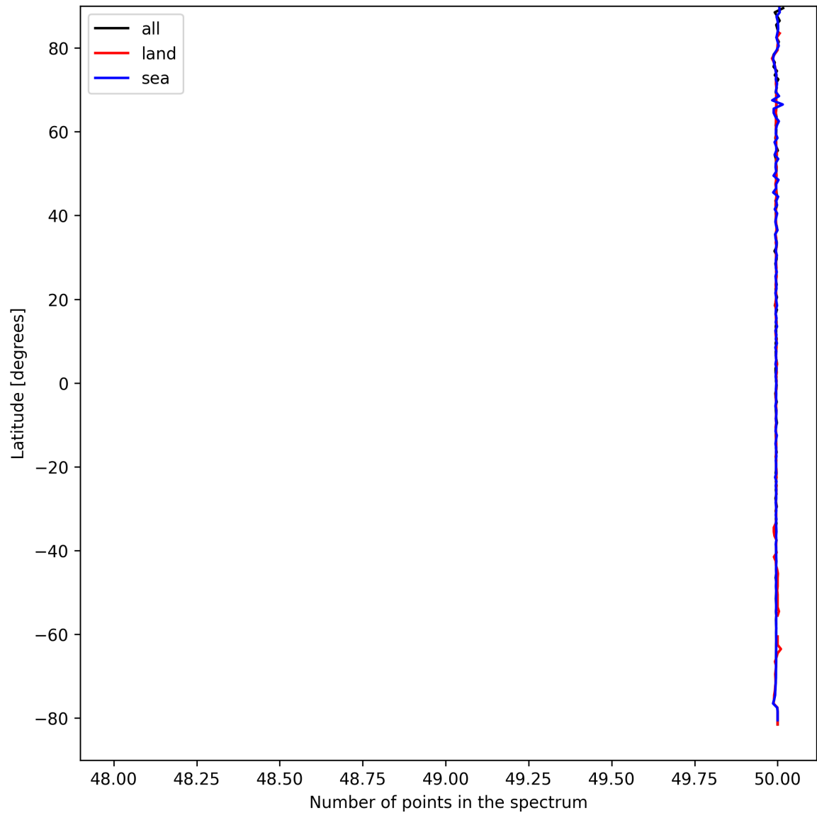
Figure 27: Zonal average of “Number of points in the spectrum” for 2025-04-06 to 2025-04-08.
