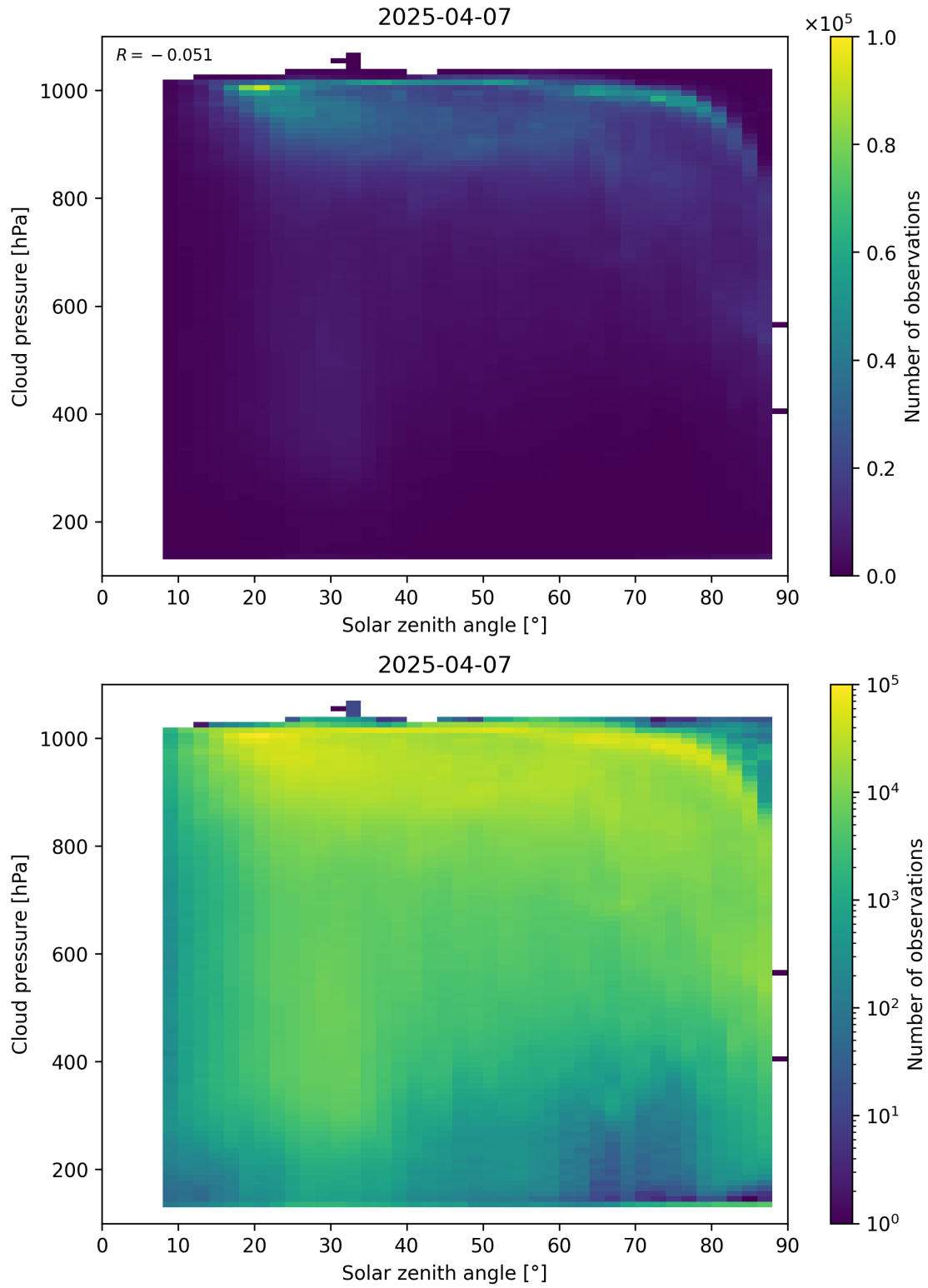
Figure 111: Scatter density plot of “Solar zenith angle” against “Cloud pressure” for 2025-04-06 to 2025-04-08.
