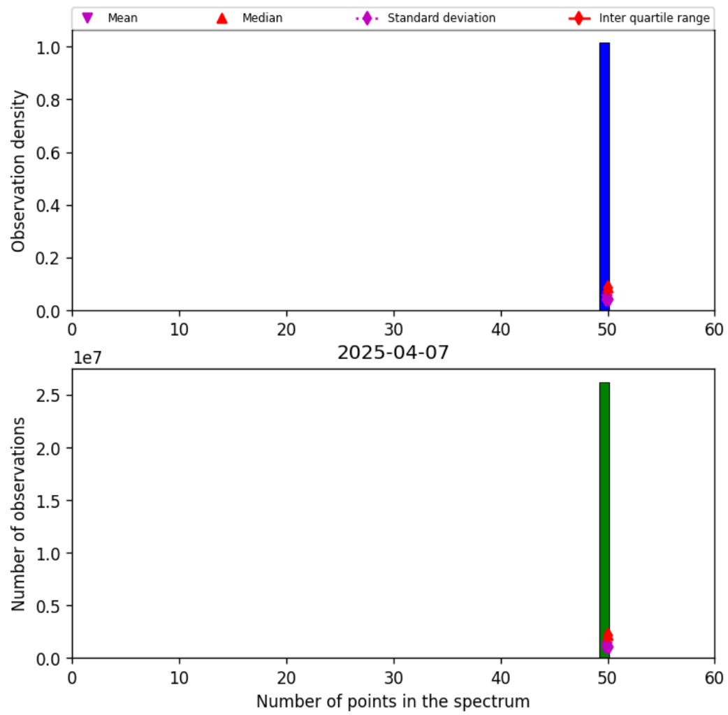
Figure 44: Histogram of “Number of points in the spectrum” for 2025-04-06 to 2025-04-08
