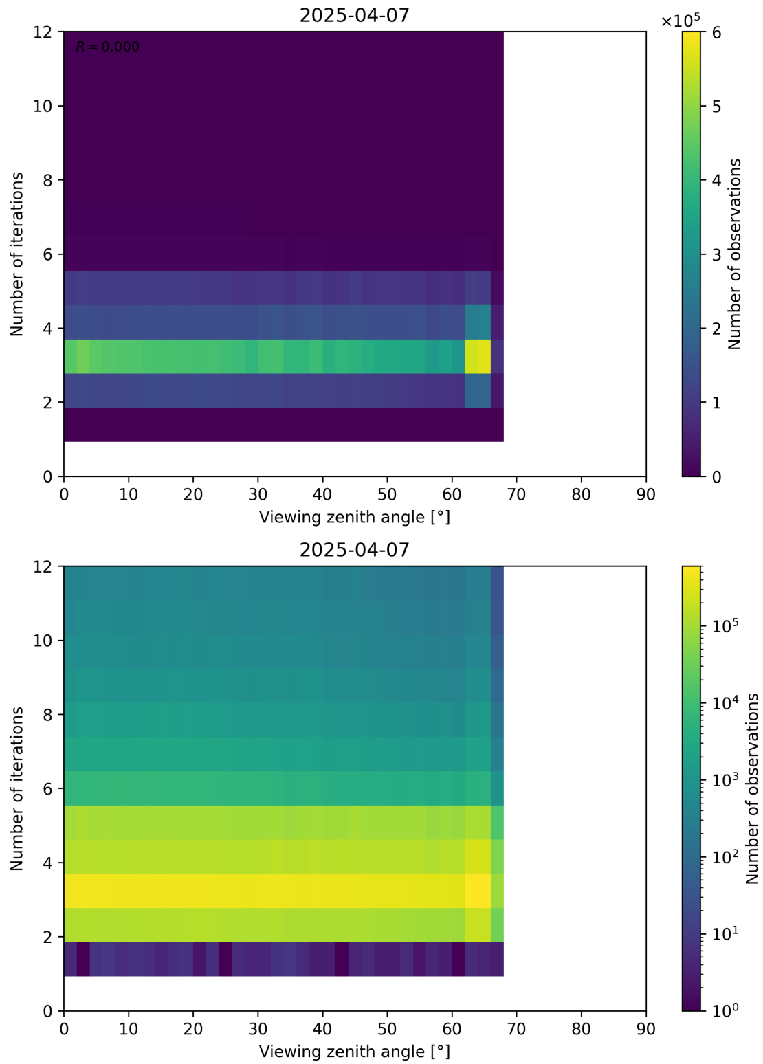
Figure 124: Scatter density plot of “Viewing zenith angle” against “Number of iterations” for 2025-04-06 to 2025-04-08.
