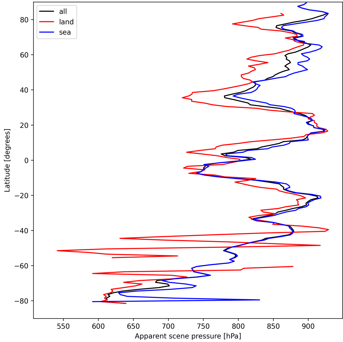
Figure 19: Zonal average of “Apparent scene pressure” for 2025-04-06 to 2025-04-08.
