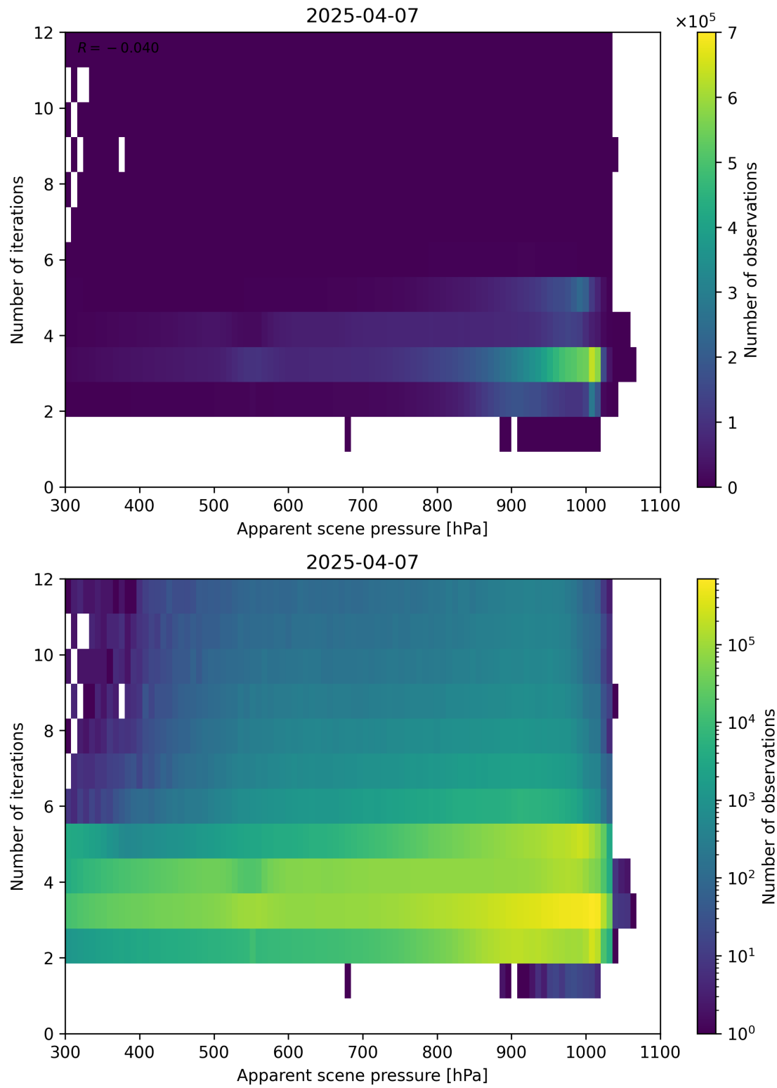
Figure 65: Scatter density plot of “Apparent scene pressure” against “Number of iterations” for 2025-04-06 to 2025-04-08.
