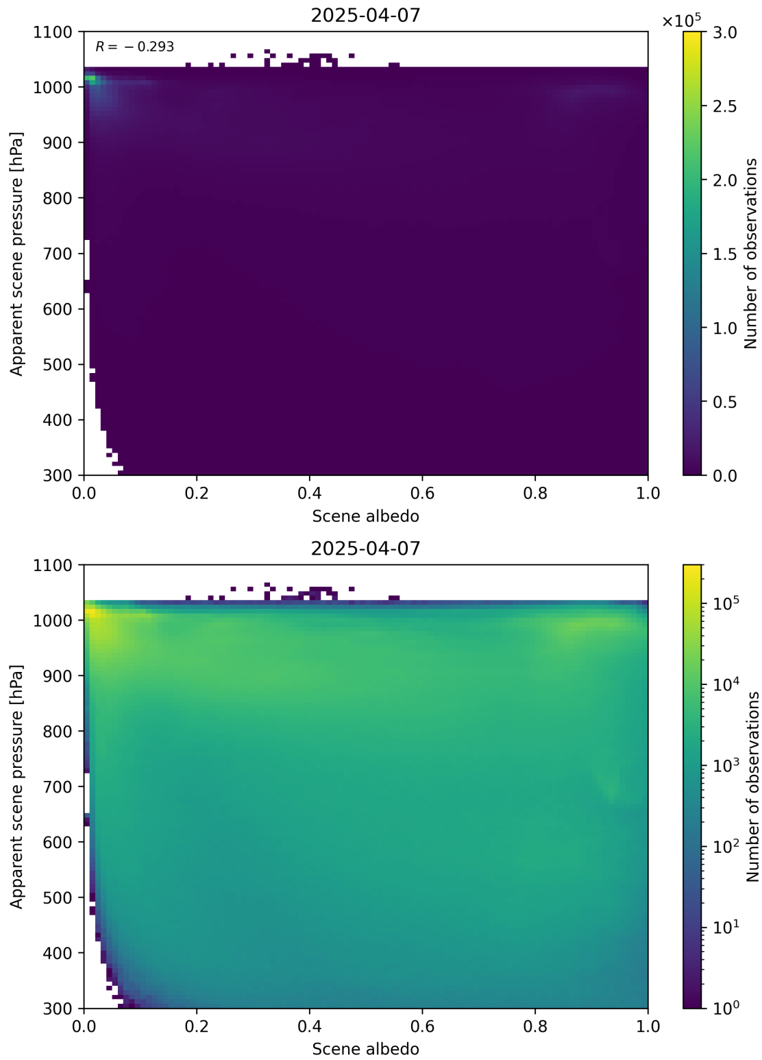
Figure 102: Scatter density plot of “Scene albedo” against “Apparent scene pressure” for 2025-04-06 to 2025-04-08.
