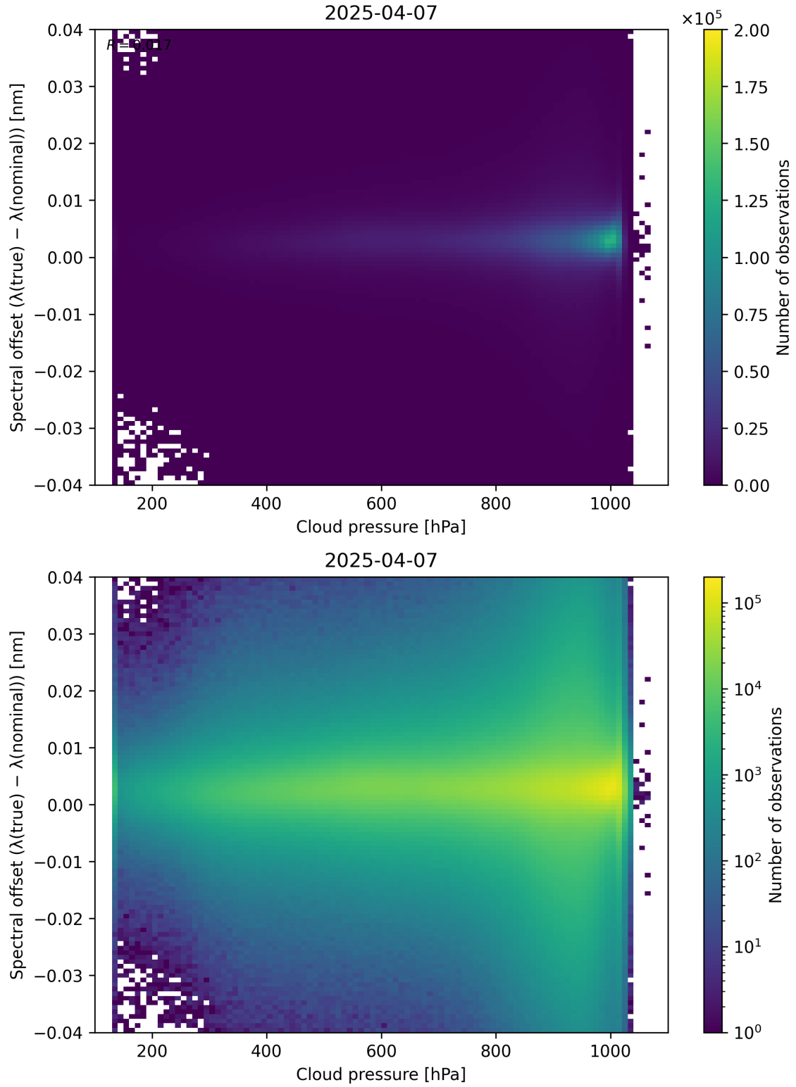
Figure 84: Scatter density plot of “Cloud pressure” against “Spectral offset ( \lambda_{\text{true}} - \lambda_{\text{nominal}} )” for 2025-04-06 to 2025-04-08.
