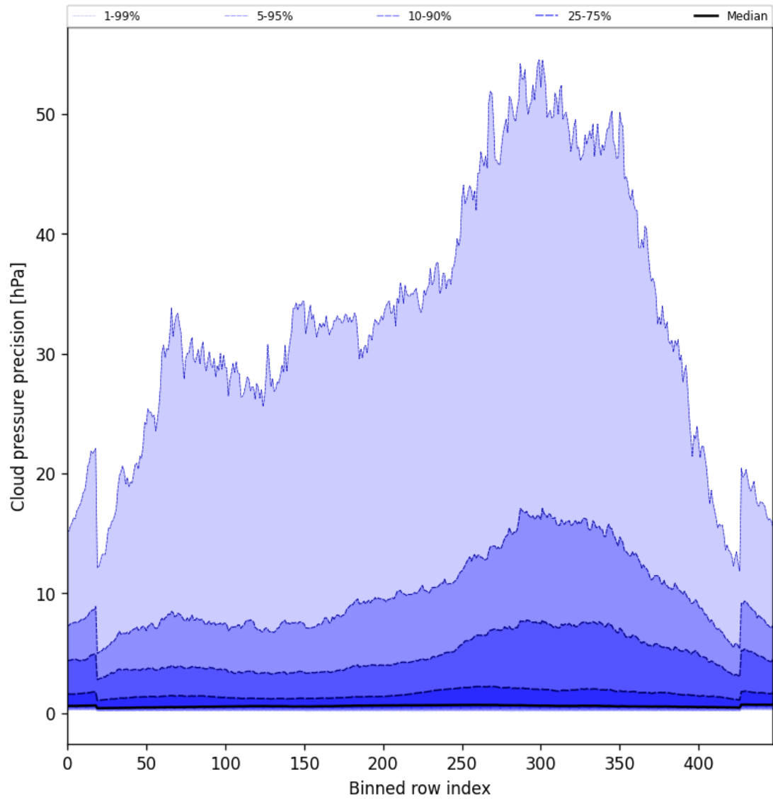
Figure 48: Along track statistics of “Cloud pressure precision” for 2025-04-06 to 2025-04-08
