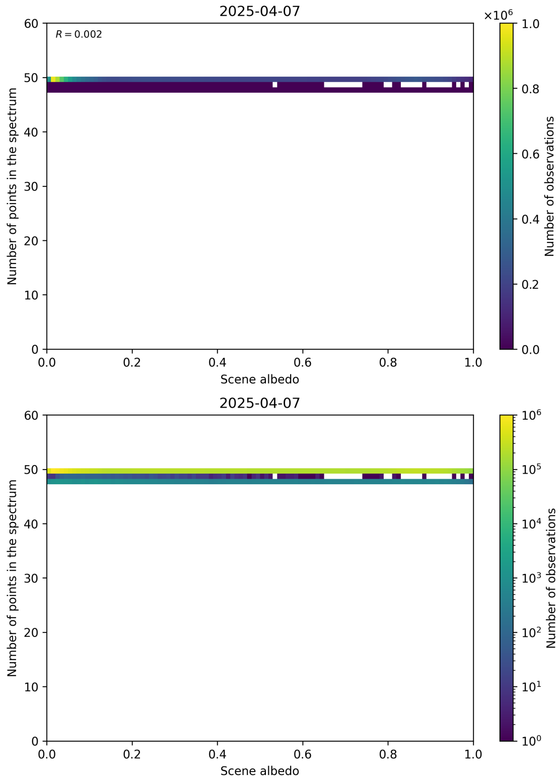
Figure 106: Scatter density plot of “Scene albedo” against “Number of points in the spectrum” for 2025-04-06 to 2025-04-08.
