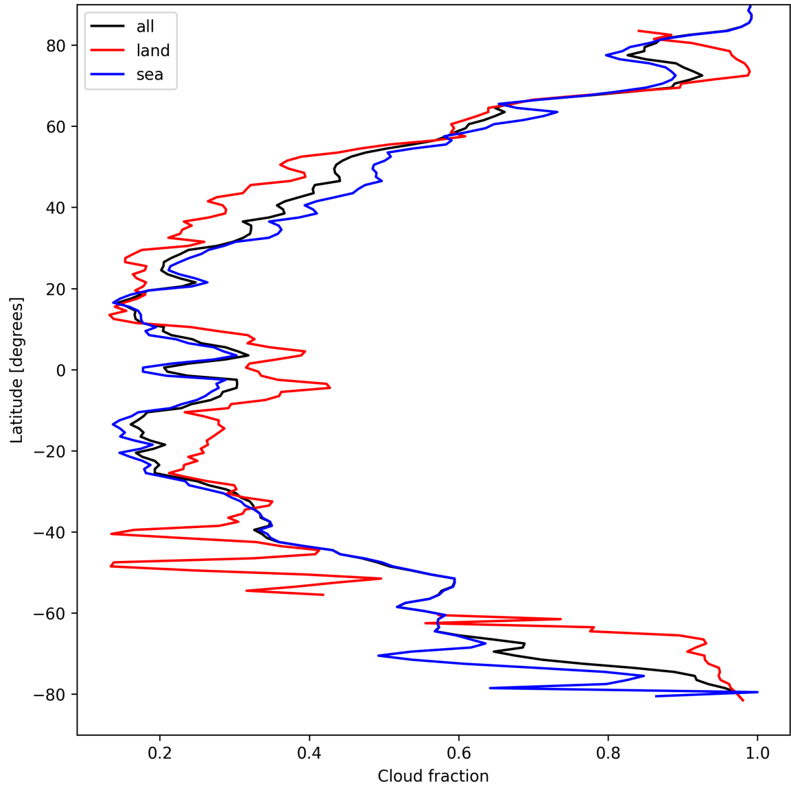
Figure 15: Zonal average of “Cloud fraction” for 2025-04-06 to 2025-04-08.
