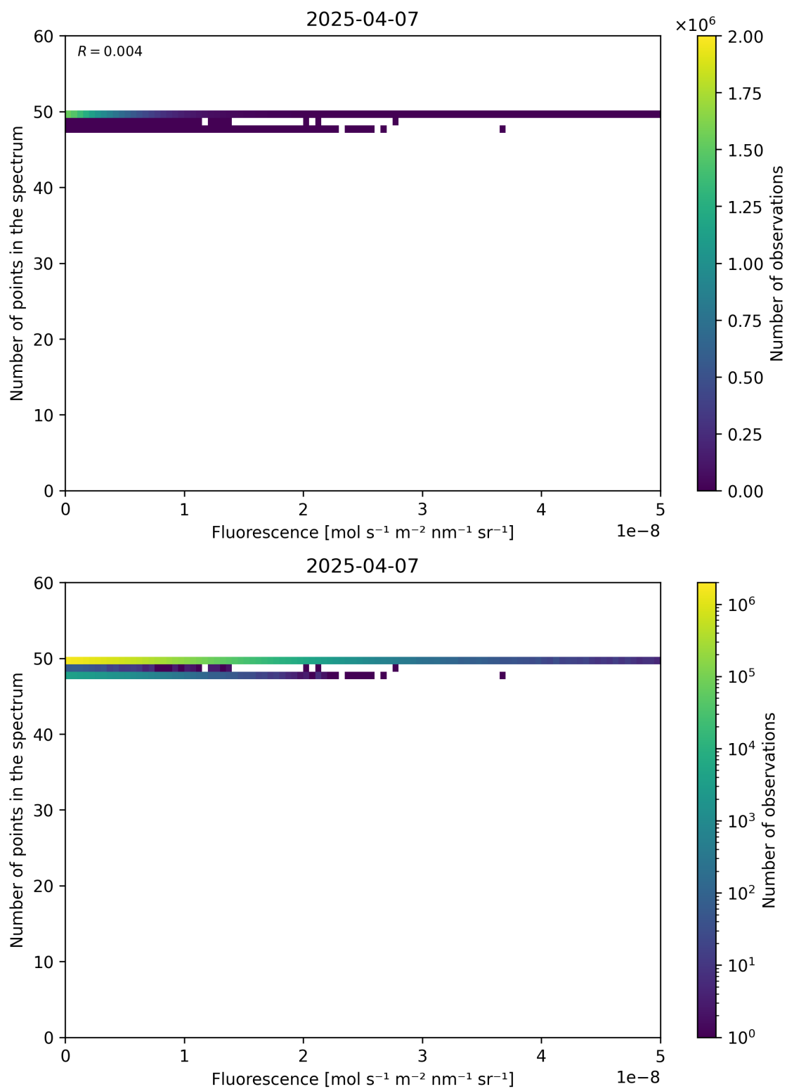
Figure 86: Scatter density plot of “Fluorescence” against “Number of points in the spectrum” for 2025-04-06 to 2025-04-08.
