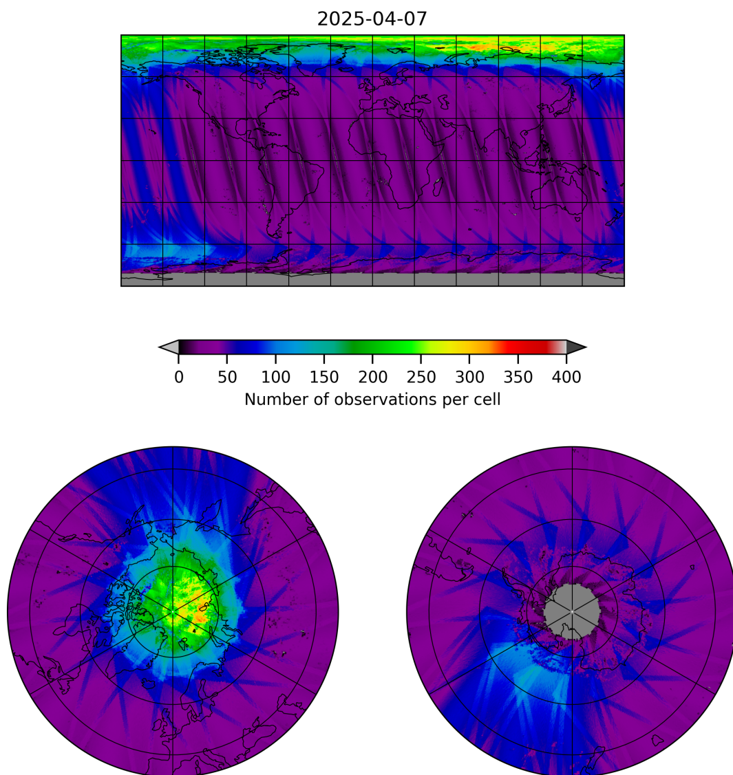
Figure 11: Map of the number of observations for 2025-04-06 to 2025-04-08
