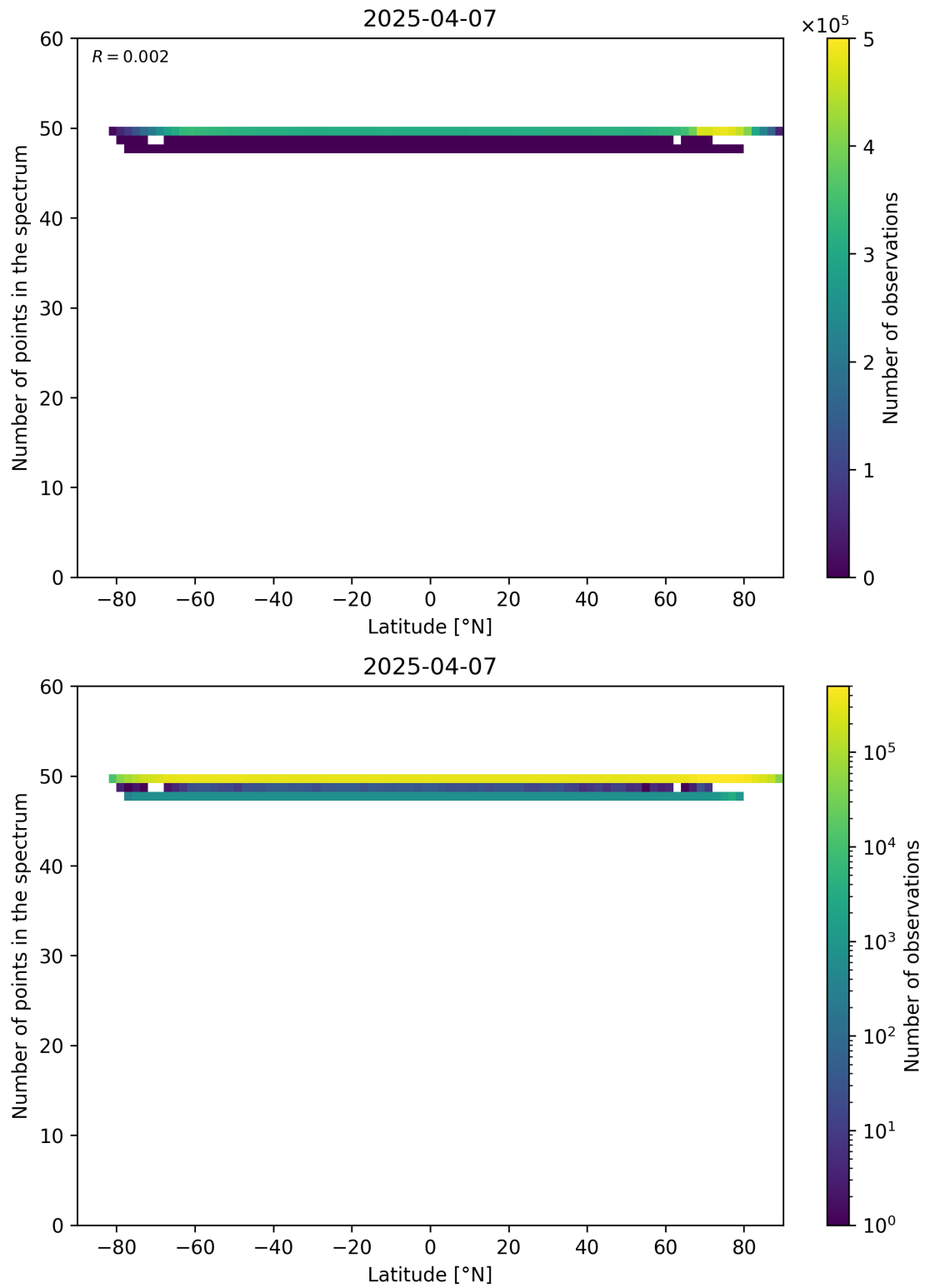
Figure 94: Scatter density plot of “Latitude” against “Number of points in the spectrum” for 2025-04-06 to 2025-04-08.
