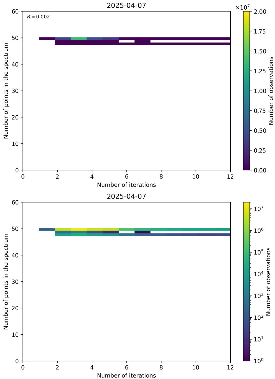
Figure 99: Scatter density plot of “Number of iterations” against “Number of points in the spectrum” for 2025-04-06 to 2025-04-08.
