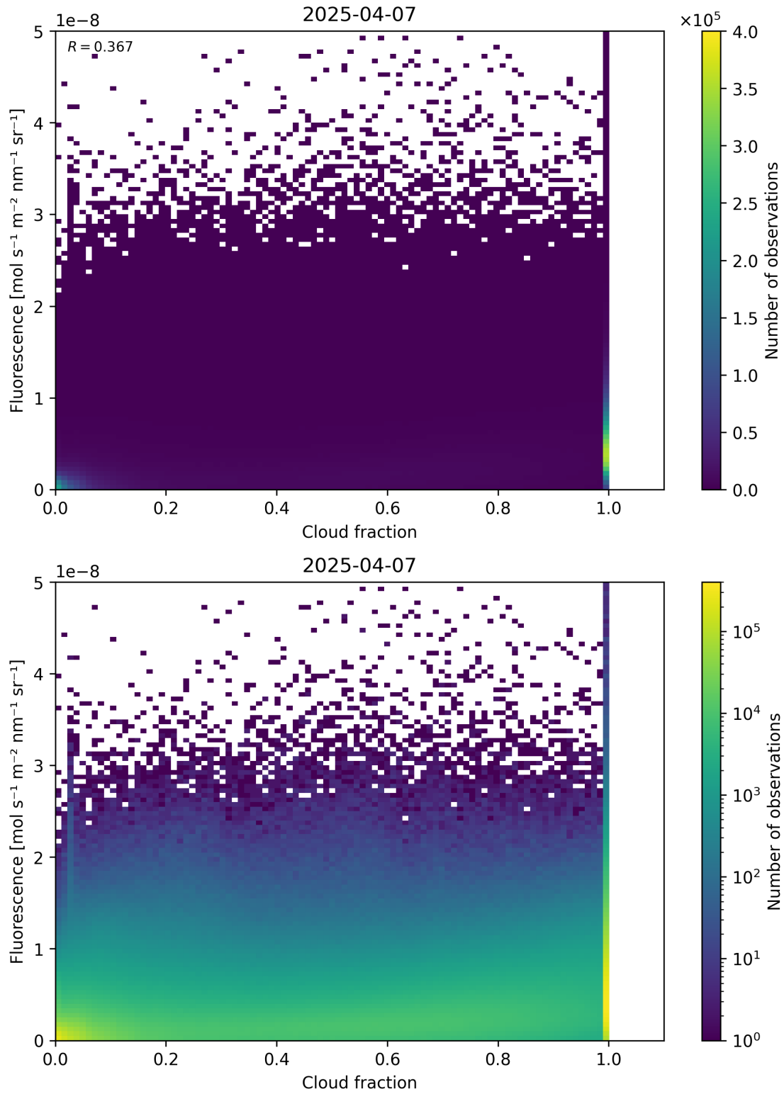
Figure 72: Scatter density plot of “Cloud fraction” against “Fluorescence” for 2025-04-06 to 2025-04-08.
