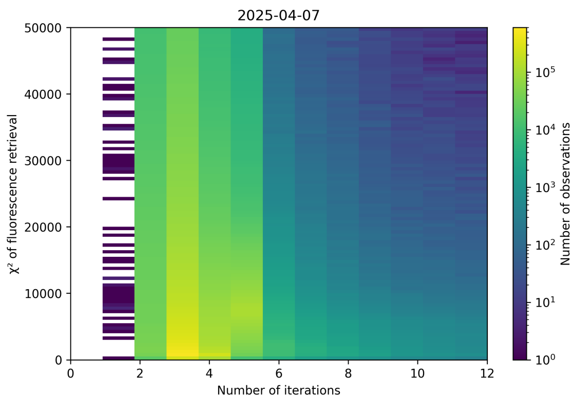
Figure 97: Scatter density plot of “Number of iterations” against “ \chi^2 of fluorescence retrieval” for 2025-04-06 to 2025-04-08.
