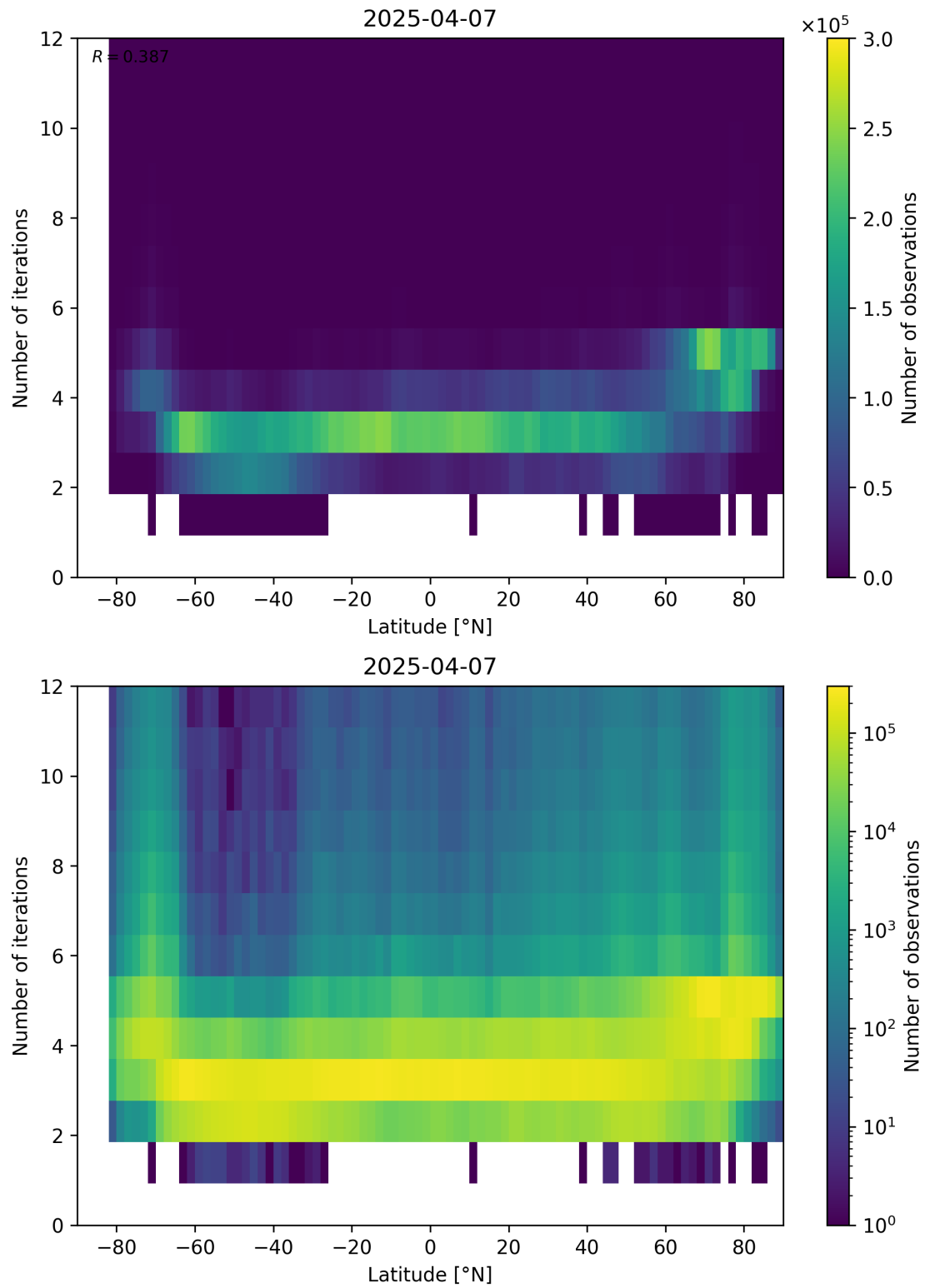
Figure 93: Scatter density plot of “Latitude” against “Number of iterations” for 2025-04-06 to 2025-04-08.
