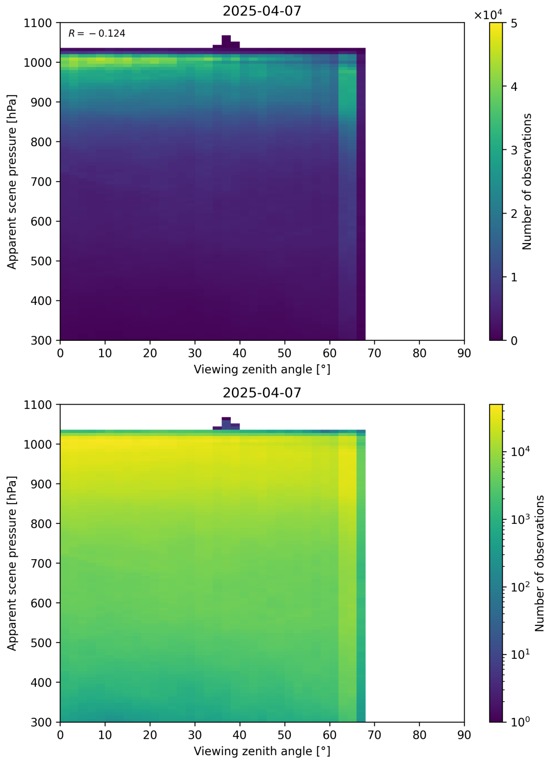
Figure 118: Scatter density plot of “Viewing zenith angle” against “Apparent scene pressure” for 2025-04-06 to 2025-04-08.
