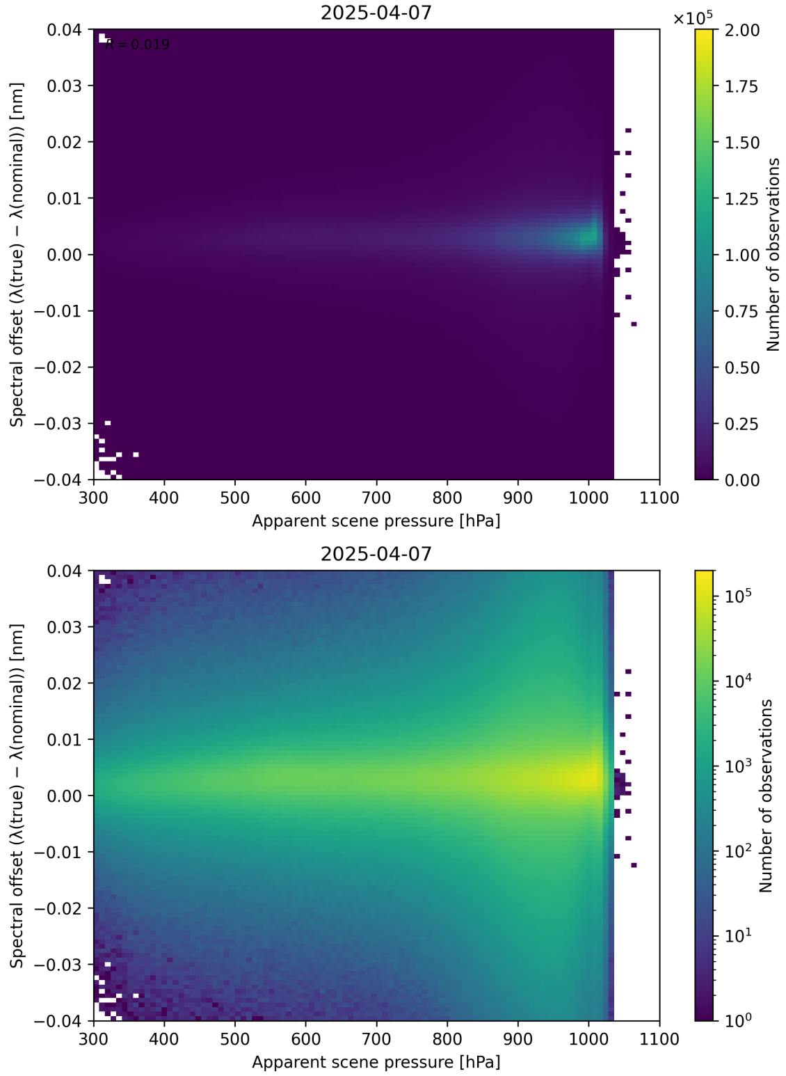
Figure 67: Scatter density plot of “Apparent scene pressure” against “Spectral offset ( \lambda_{\text{true}} - \lambda_{\text{nominal}} )” for 2025-04-06 to 2025-04-08.
