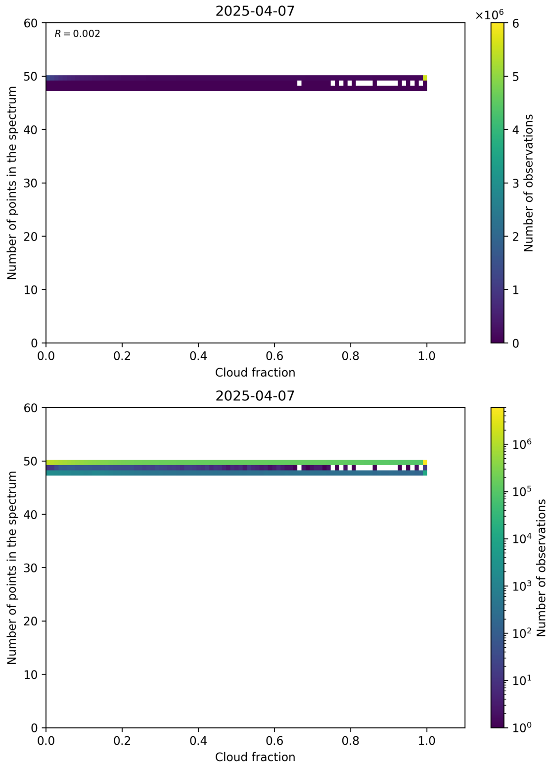
Figure 74: Scatter density plot of “Cloud fraction” against “Number of points in the spectrum” for 2025-04-06 to 2025-04-08.
