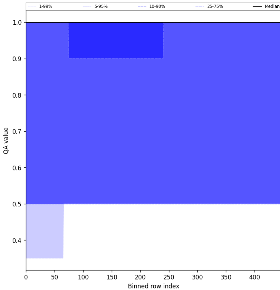
Figure 46: Along track statistics of “QA value” for 2025-04-06 to 2025-04-08
