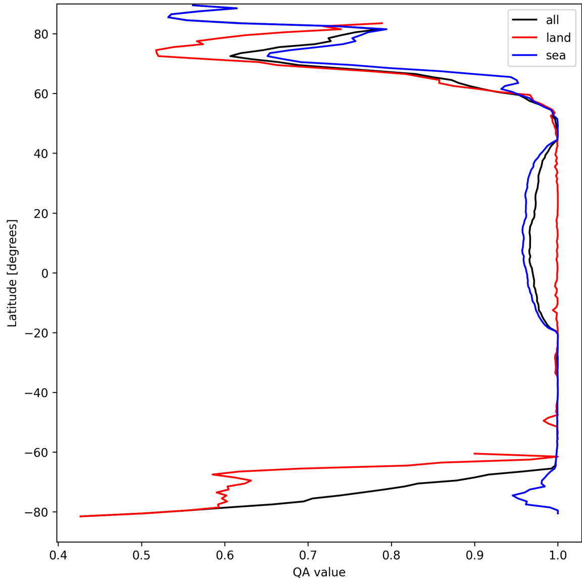
Figure 12: Zonal average of “QA value” for 2025-04-06 to 2025-04-08.
