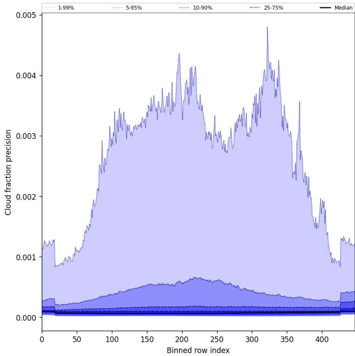
Figure 50: Along track statistics of “Cloud fraction precision” for 2025-04-06 to 2025-04-08
