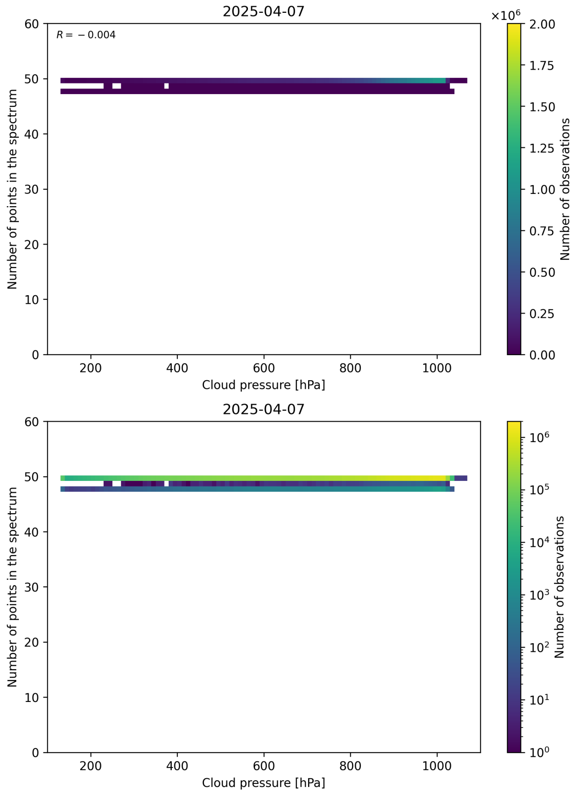
Figure 82: Scatter density plot of “Cloud pressure” against “Number of points in the spectrum” for 2025-04-06 to 2025-04-08.
