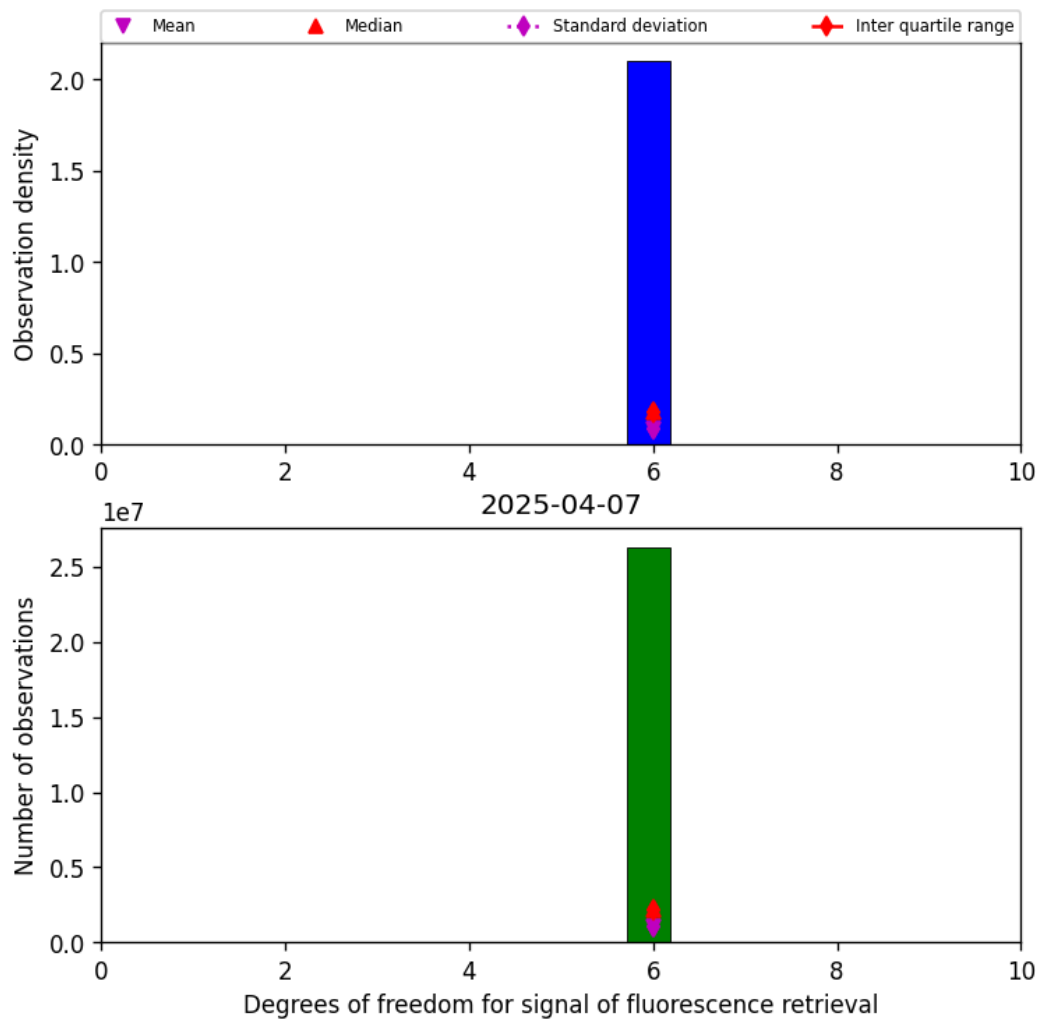
Figure 43: Histogram of "Degrees of freedom for signal of fluorescence retrieval" for 2025-04-06 to 2025-04-08
