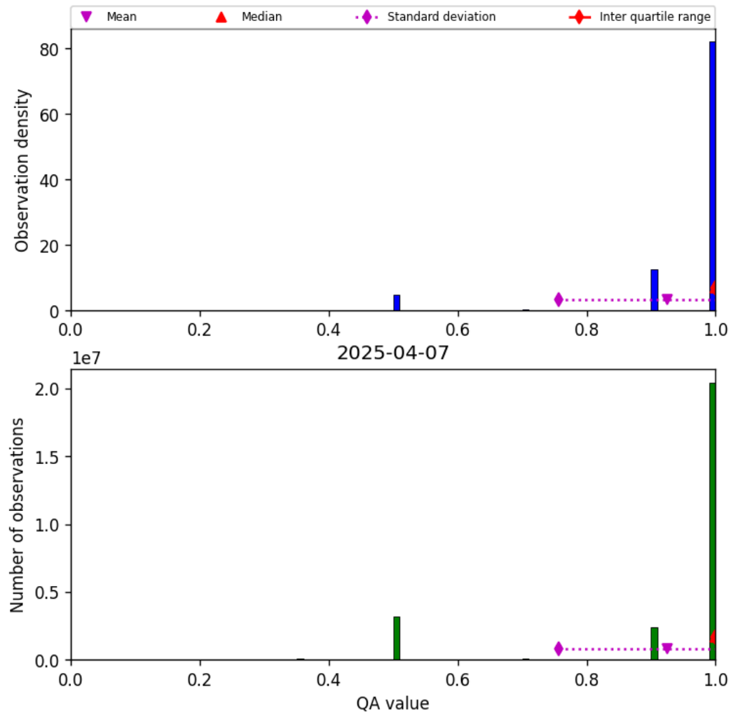
Figure 29: Histogram of “QA value” for 2025-04-06 to 2025-04-08
