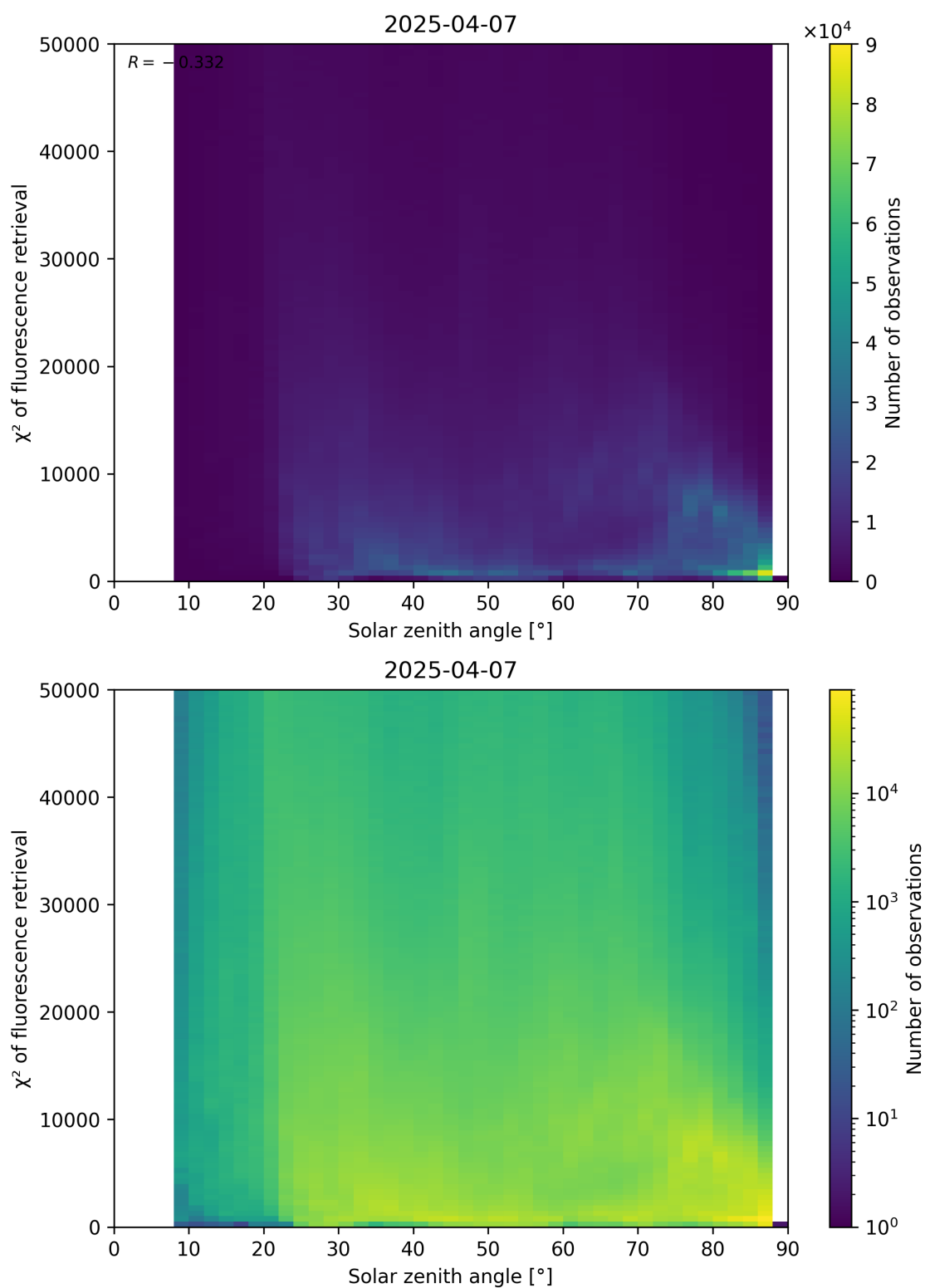
Figure 109: Scatter density plot of “Solar zenith angle” against “ \chi^2 of fluorescence retrieval” for 2025-04-06 to 2025-04-08.
