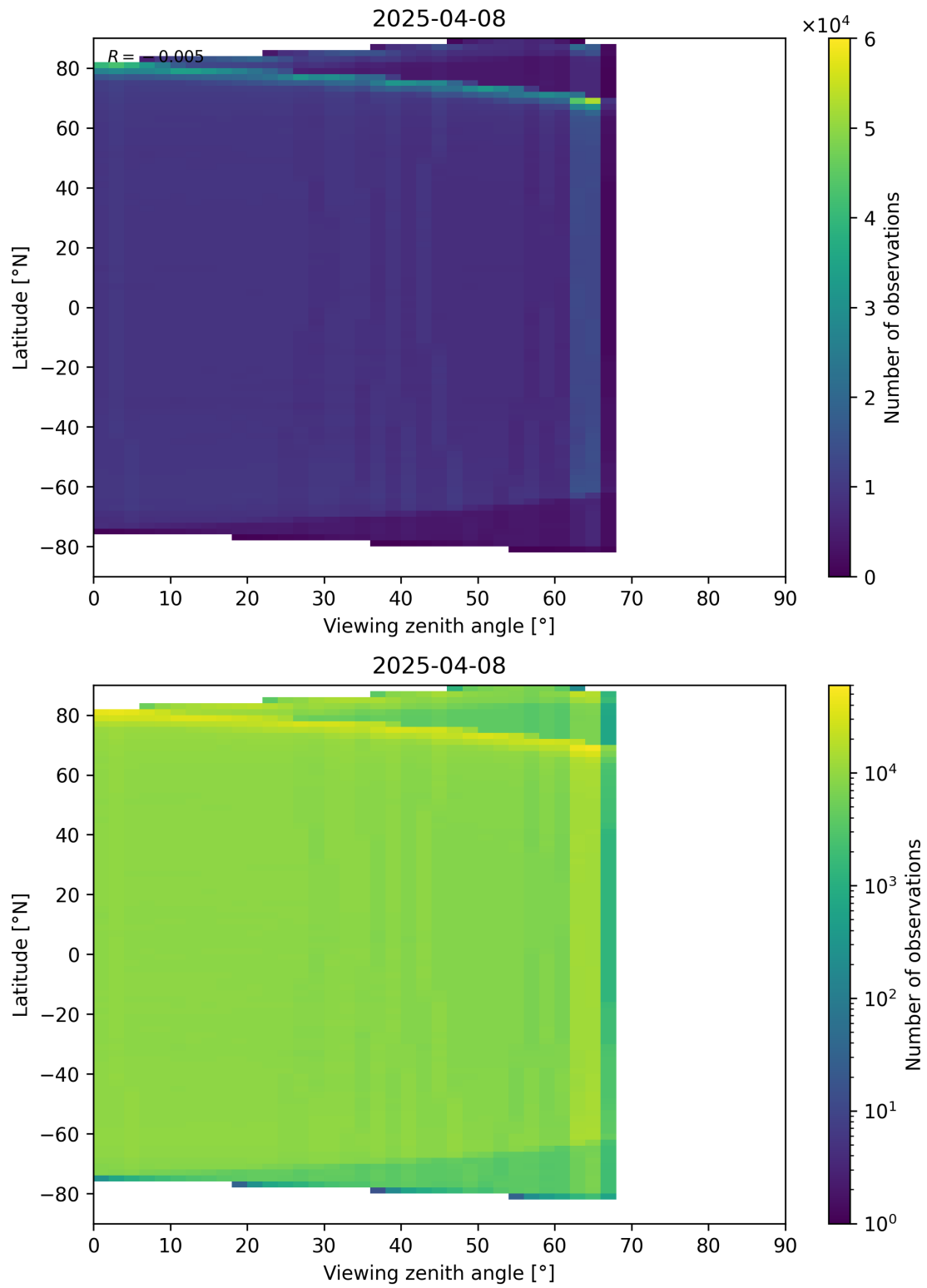
Figure 123: Scatter density plot of “Viewing zenith angle” against “Latitude” for 2025-04-08 to 2025-04-09.
