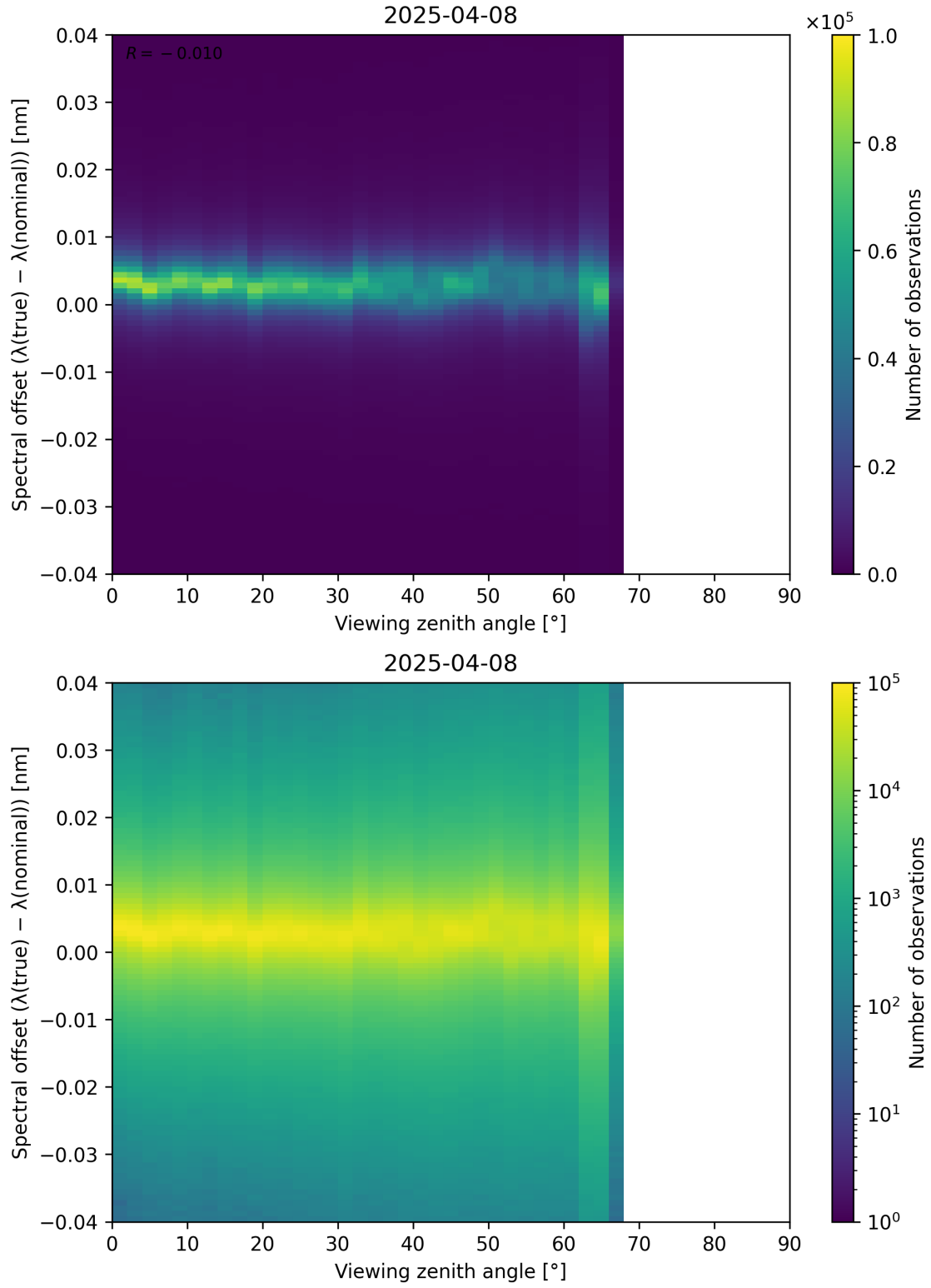
Figure 128: Scatter density plot of “Viewing zenith angle” against “Spectral offset ( \lambda_{\text{true}} - \lambda_{\text{nominal}} )” for 2025-04-08 to 2025-04-09.
