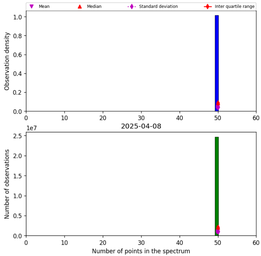
Figure 44: Histogram of “Number of points in the spectrum” for 2025-04-08 to 2025-04-09
