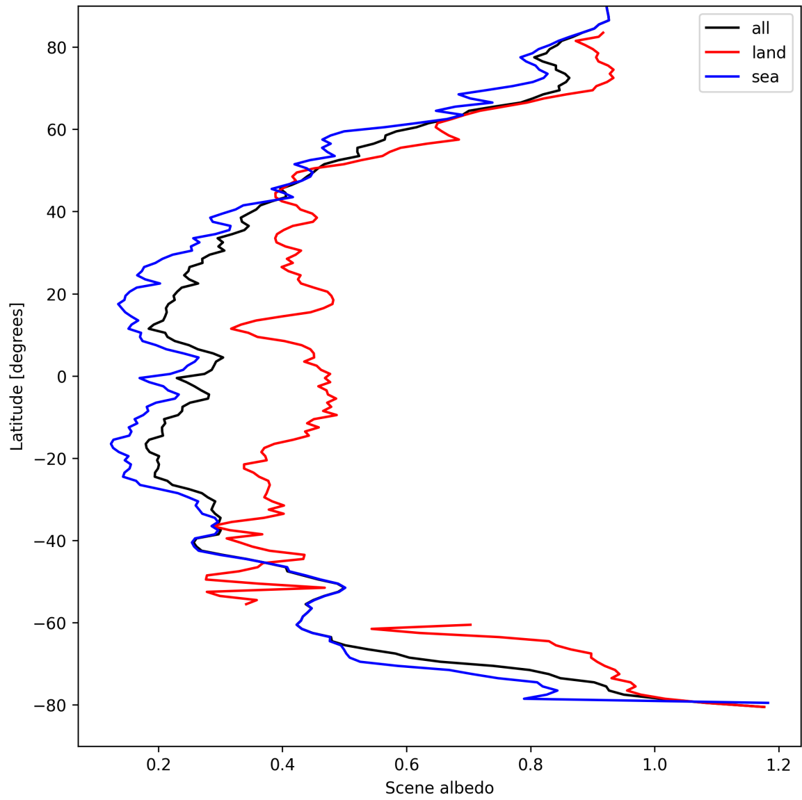
Figure 17: Zonal average of “Scene albedo” for 2025-04-08 to 2025-04-09.
