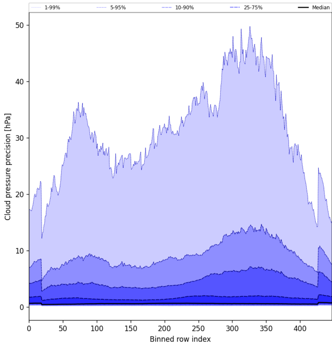
Figure 48: Along track statistics of “Cloud pressure precision” for 2025-04-08 to 2025-04-09
