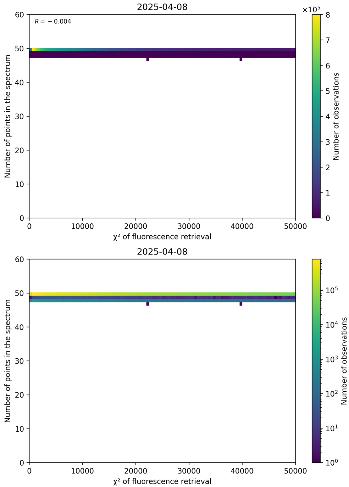
Figure 68: Scatter density plot of “ \chi^2 of fluorescence retrieval” against “Number of points in the spectrum” for 2025-04-08 to 2025-04-09.
