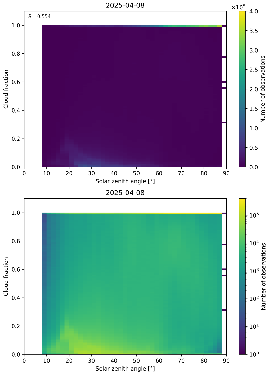
Figure 110: Scatter density plot of “Solar zenith angle” against “Cloud fraction” for 2025-04-08 to 2025-04-09.
