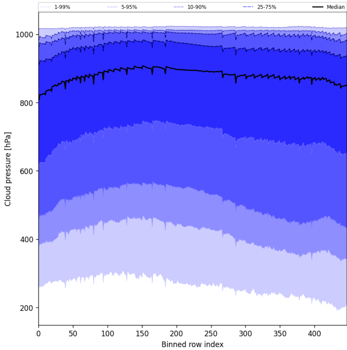
Figure 47: Along track statistics of “Cloud pressure” for 2025-04-08 to 2025-04-09
