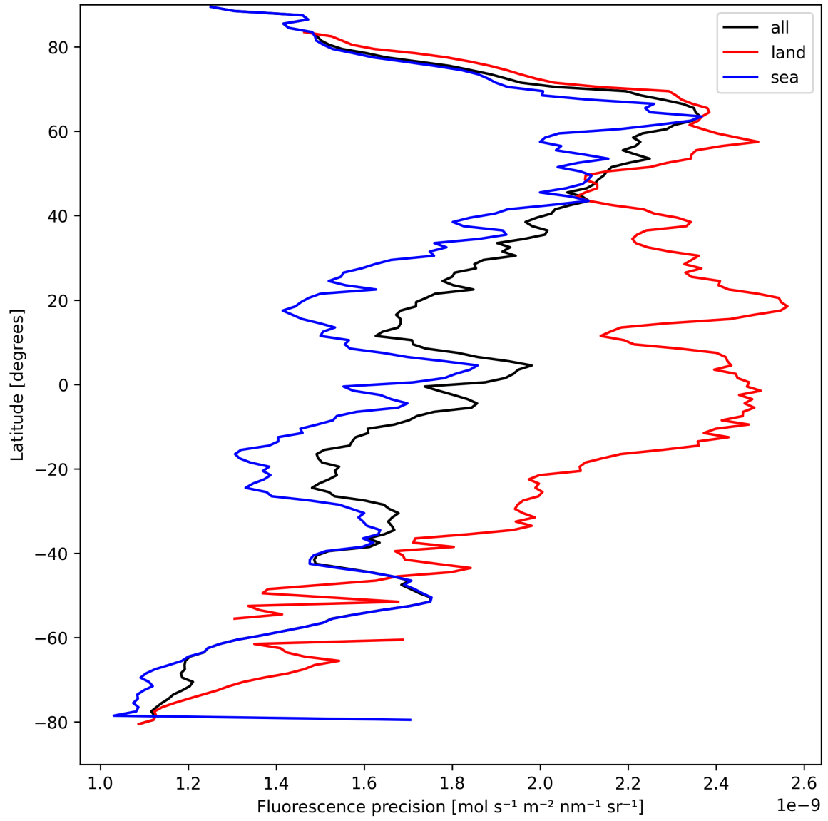
Figure 24: Zonal average of “Fluorescence precision” for 2025-04-08 to 2025-04-09.
