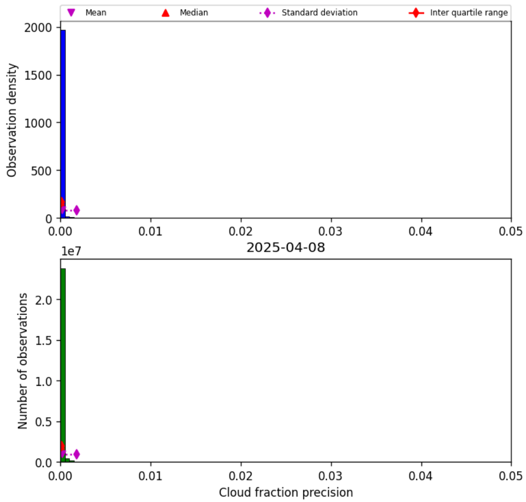
Figure 33: Histogram of “Cloud fraction precision” for 2025-04-08 to 2025-04-09
