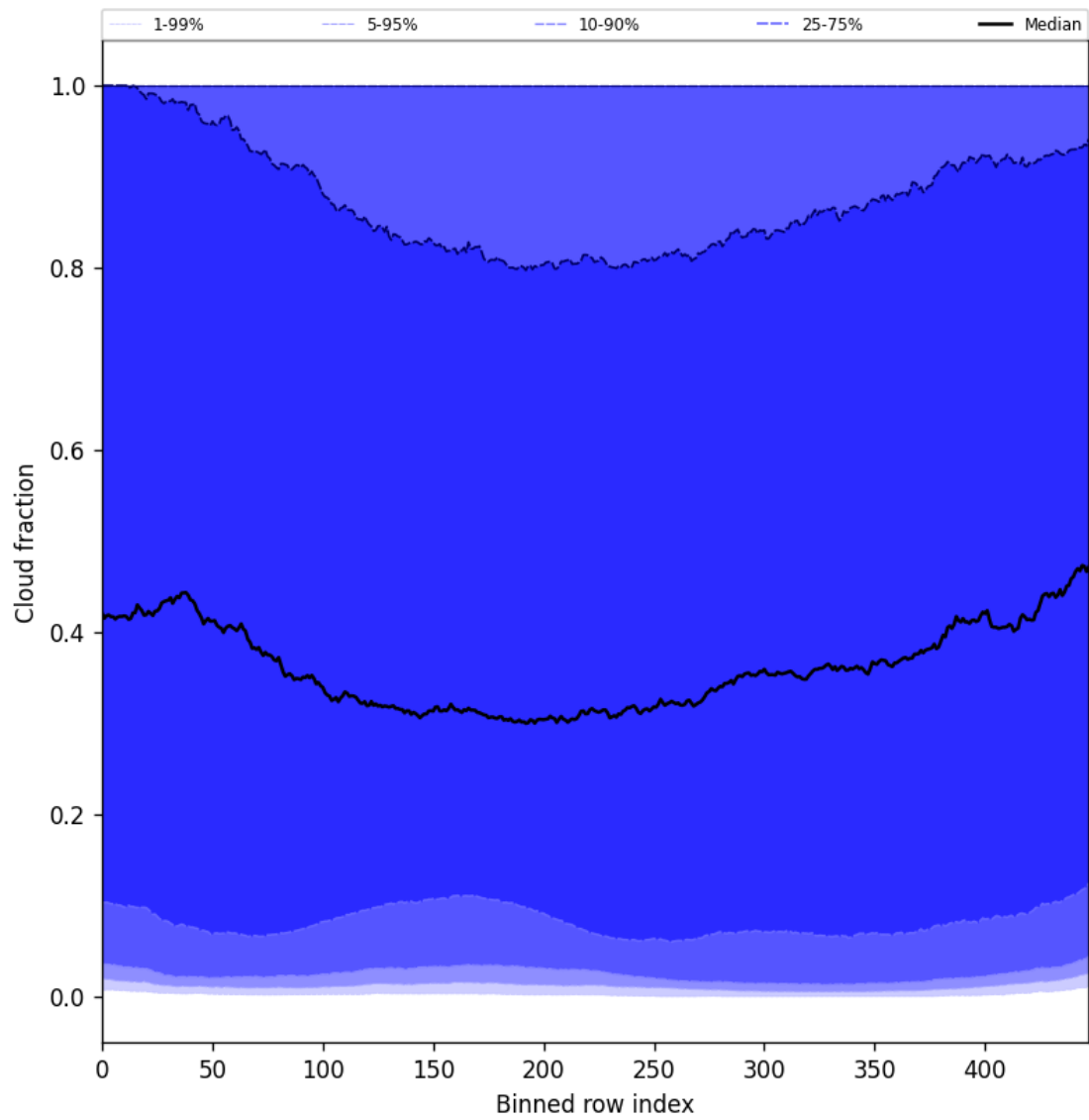
Figure 49: Along track statistics of “Cloud fraction” for 2025-04-08 to 2025-04-09
