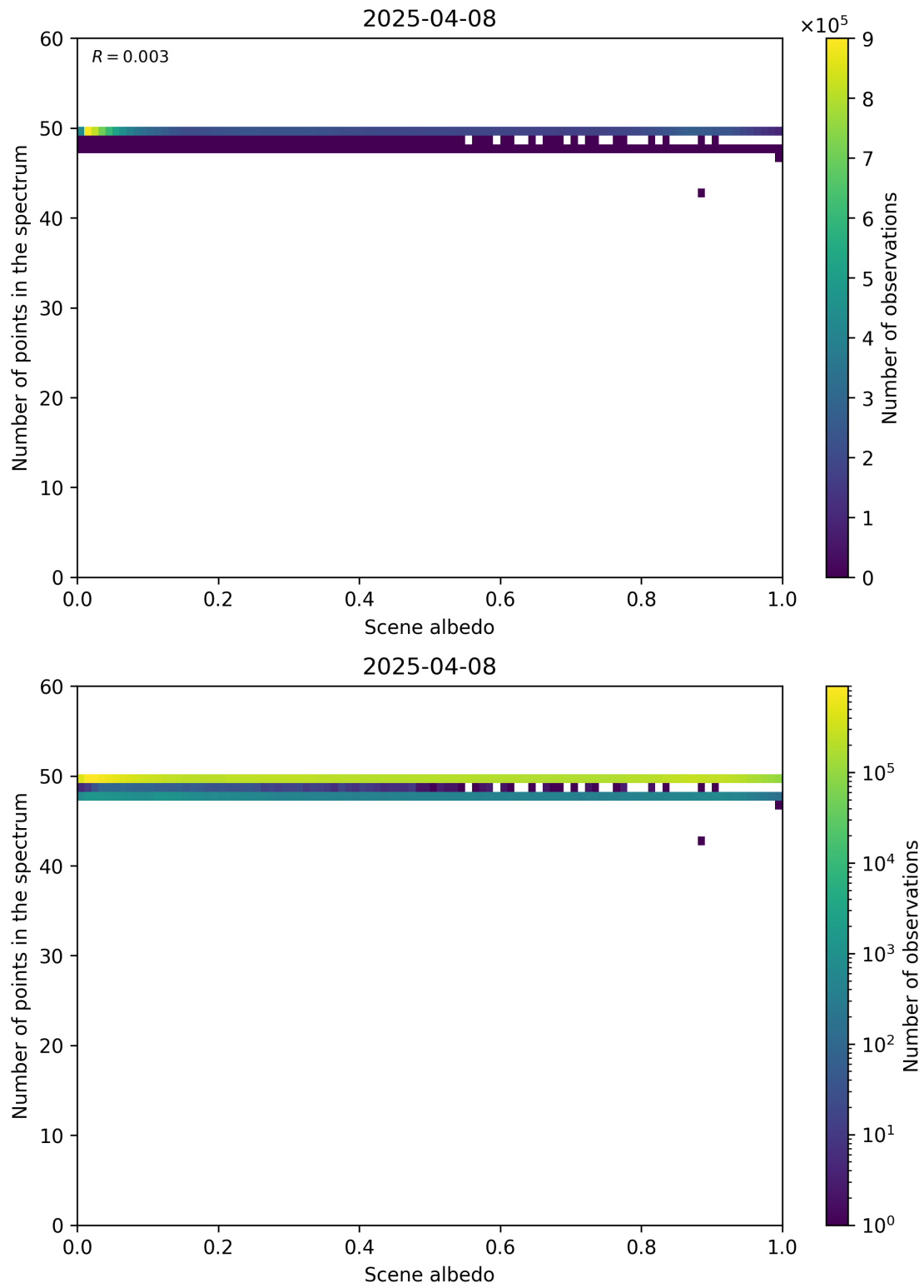
Figure 106: Scatter density plot of “Scene albedo” against “Number of points in the spectrum” for 2025-04-08 to 2025-04-09.
