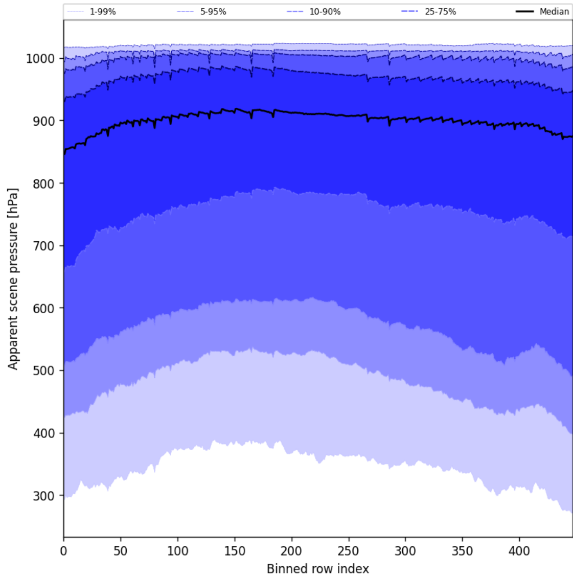
Figure 53: Along track statistics of “Apparent scene pressure” for 2025-04-08 to 2025-04-09
