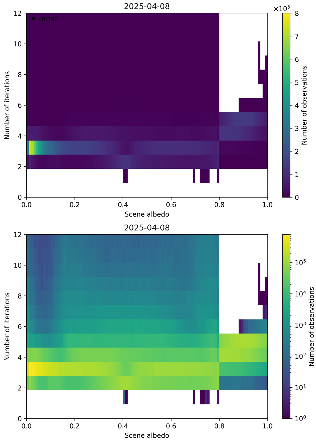
Figure 105: Scatter density plot of “Scene albedo” against “Number of iterations” for 2025-04-08 to 2025-04-09.
