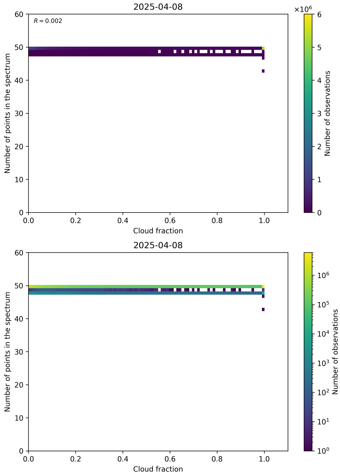
Figure 74: Scatter density plot of “Cloud fraction” against “Number of points in the spectrum” for 2025-04-08 to 2025-04-09.
