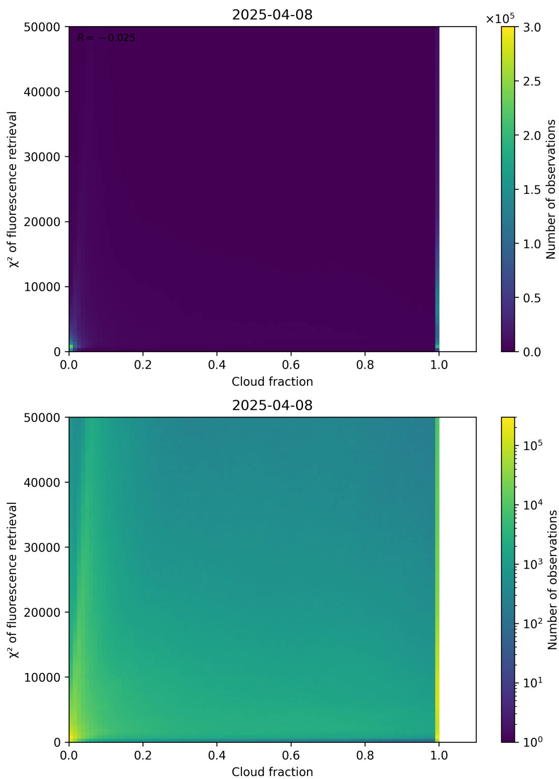
Figure 71: Scatter density plot of “Cloud fraction” against “ \chi^2 of fluorescence retrieval” for 2025-04-08 to 2025-04-09.
