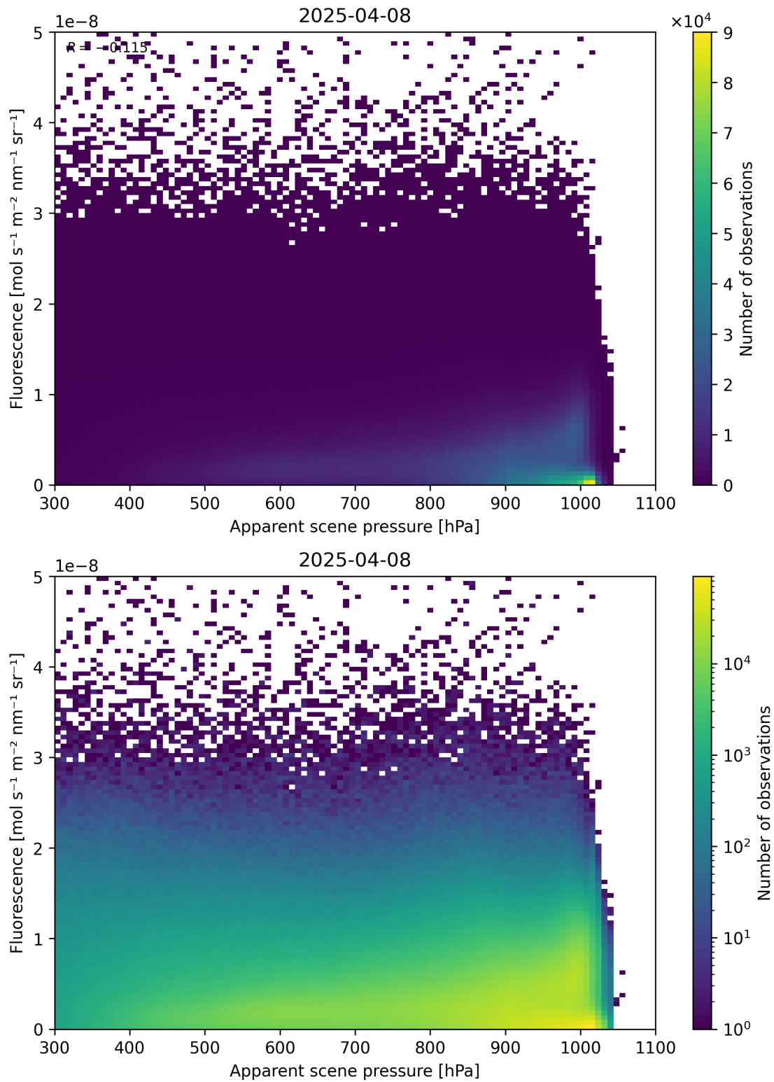
Figure 64: Scatter density plot of “Apparent scene pressure” against “Fluorescence” for 2025-04-08 to 2025-04-09.
