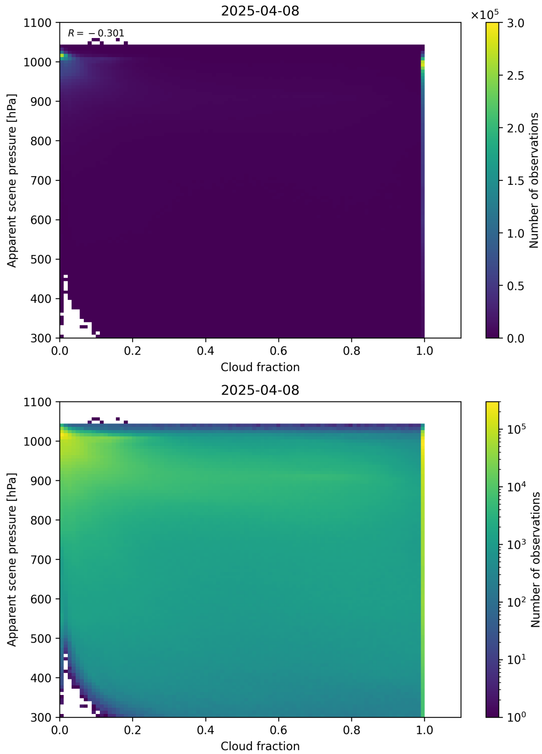
Figure 70: Scatter density plot of “Cloud fraction” against “Apparent scene pressure” for 2025-04-08 to 2025-04-09.
