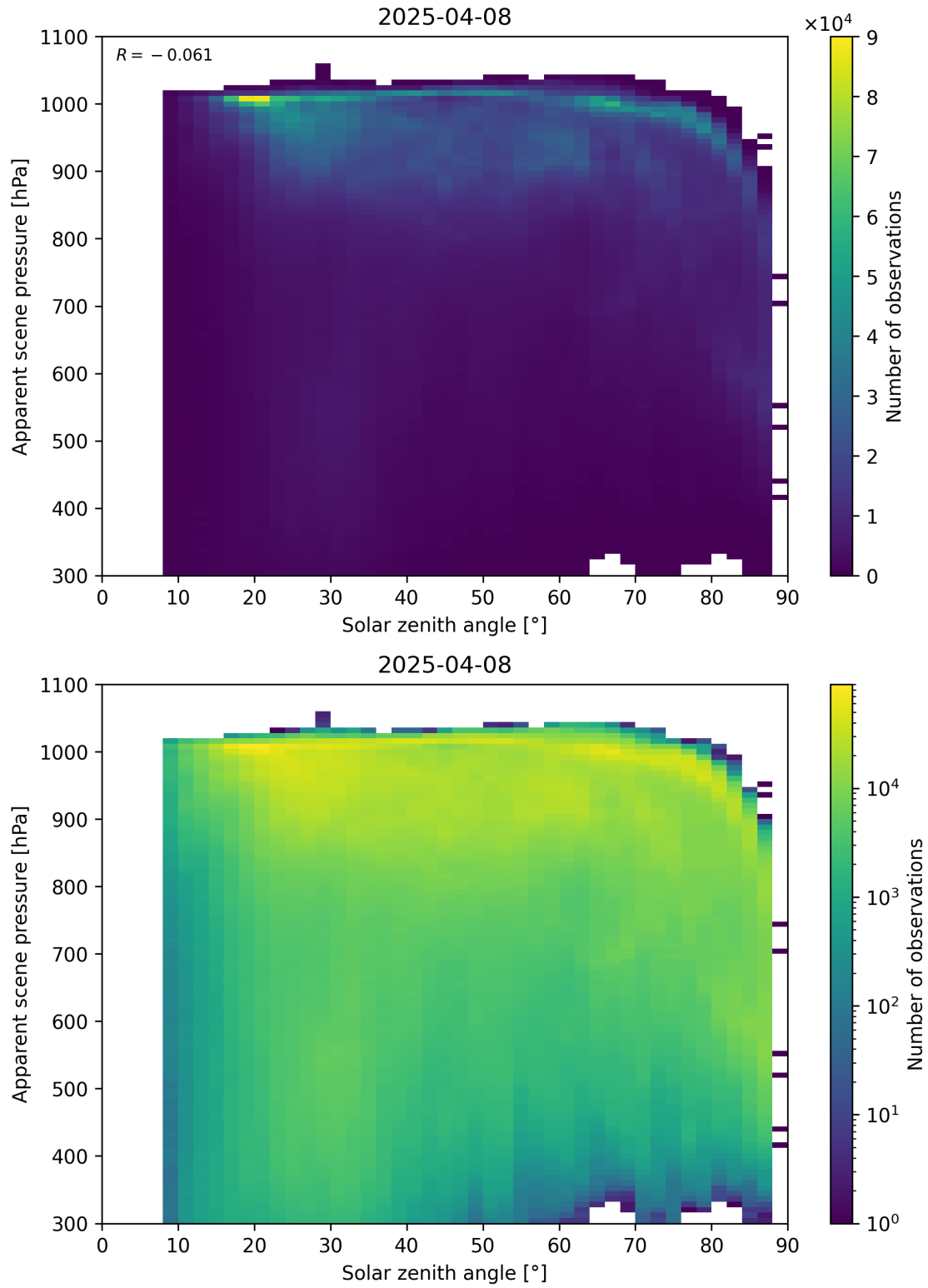
Figure 108: Scatter density plot of “Solar zenith angle” against “Apparent scene pressure” for 2025-04-08 to 2025-04-09.
