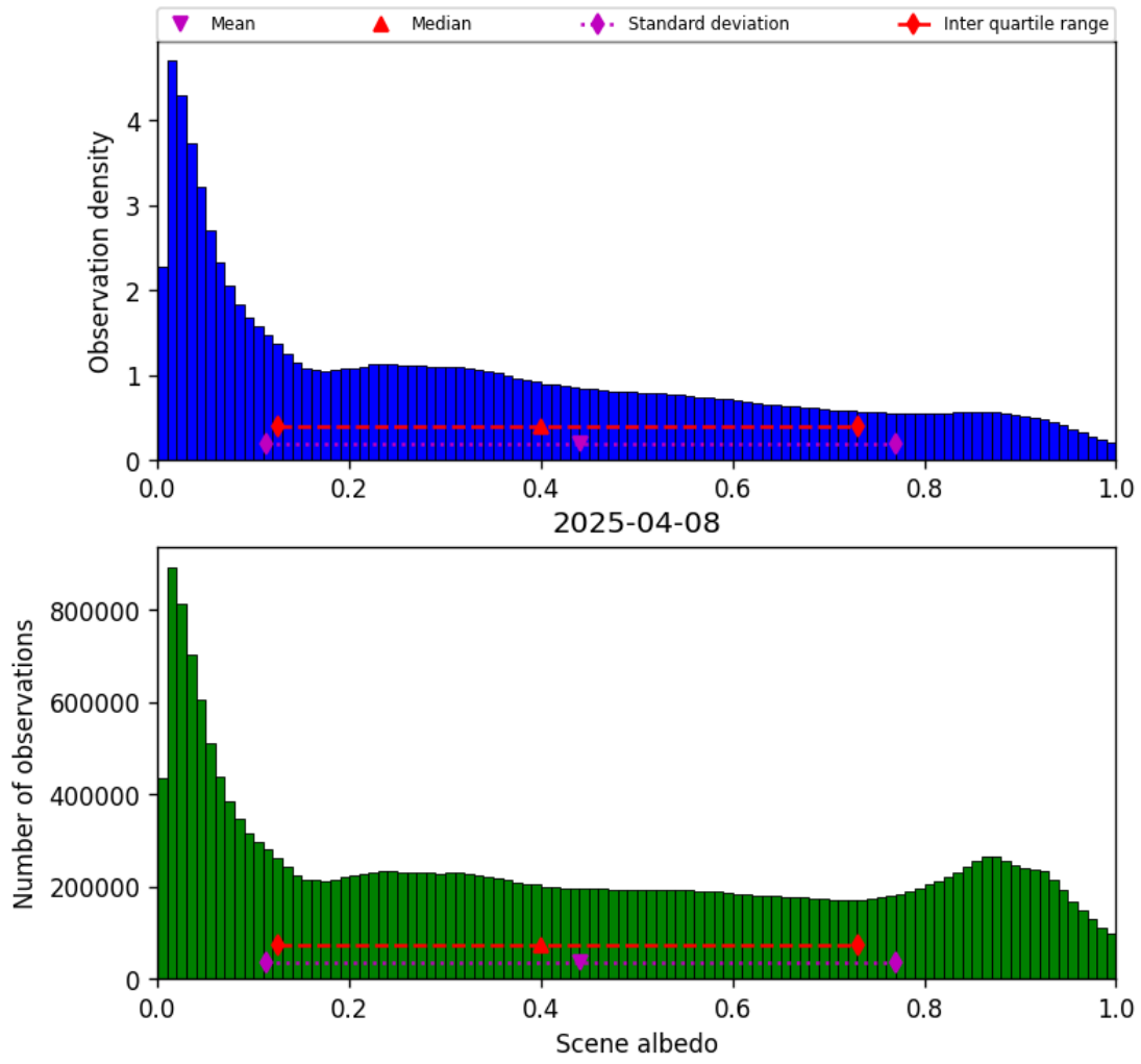
Figure 34: Histogram of “Scene albedo” for 2025-04-08 to 2025-04-09
