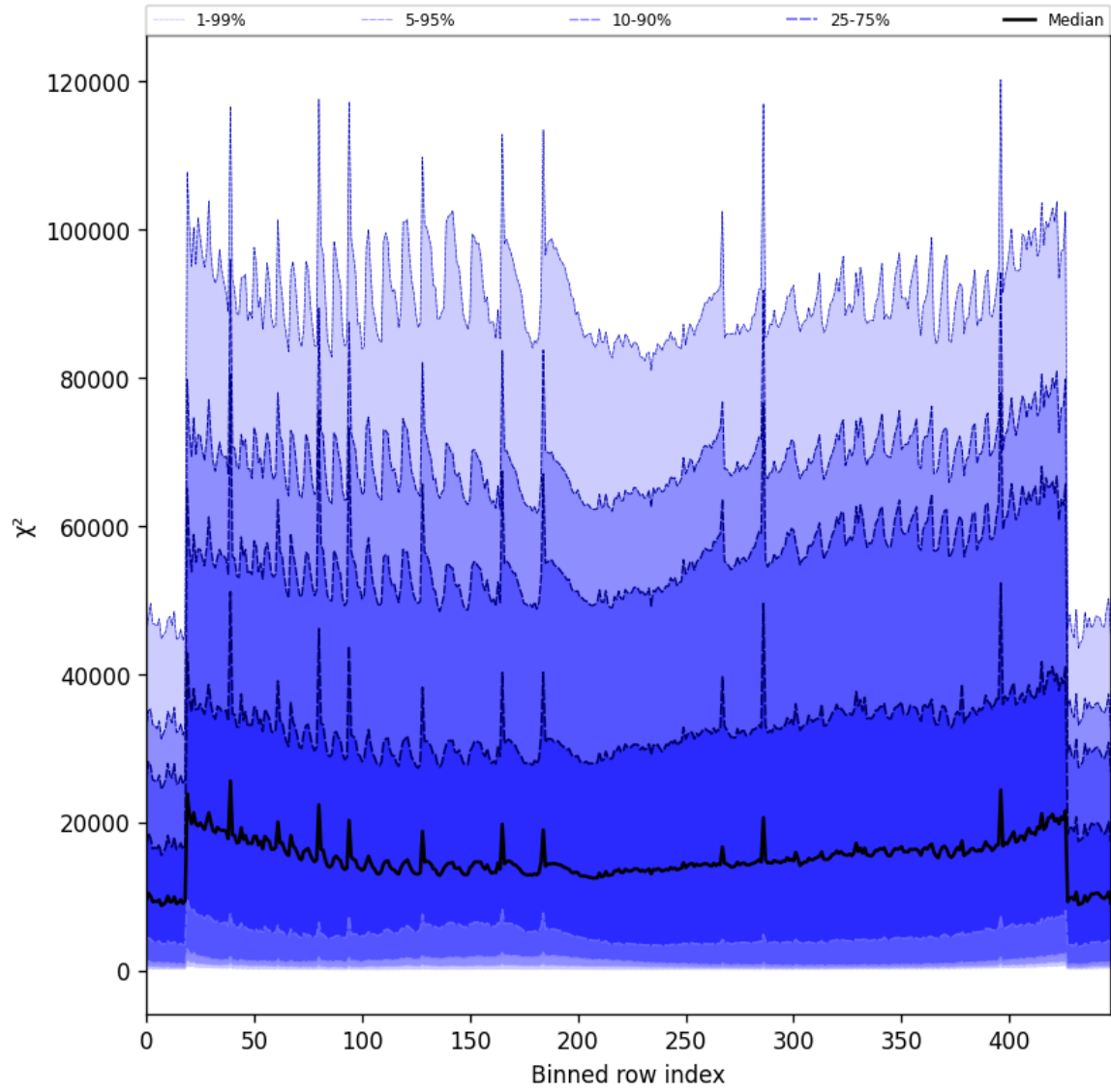
Figure 55: Along track statistics of “ \chi^2 ” for 2025-04-08 to 2025-04-09
