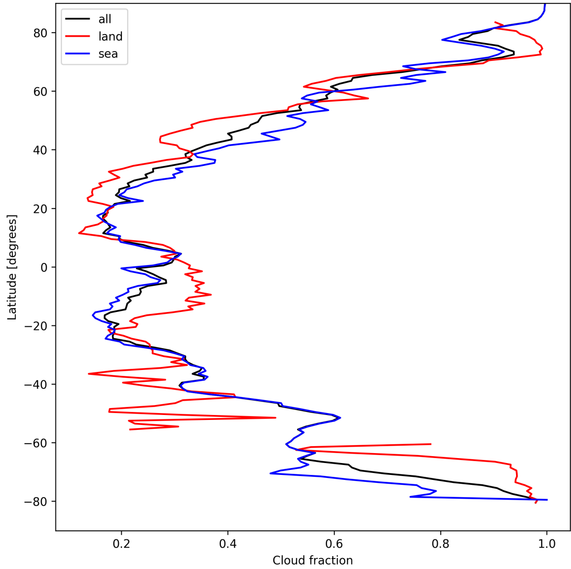
Figure 15: Zonal average of “Cloud fraction” for 2025-04-08 to 2025-04-09.
