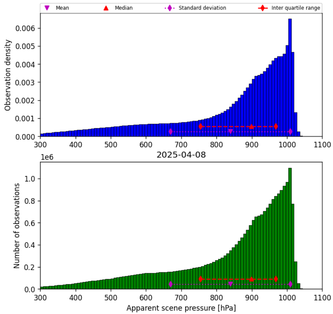
Figure 36: Histogram of “Apparent scene pressure” for 2025-04-08 to 2025-04-09
