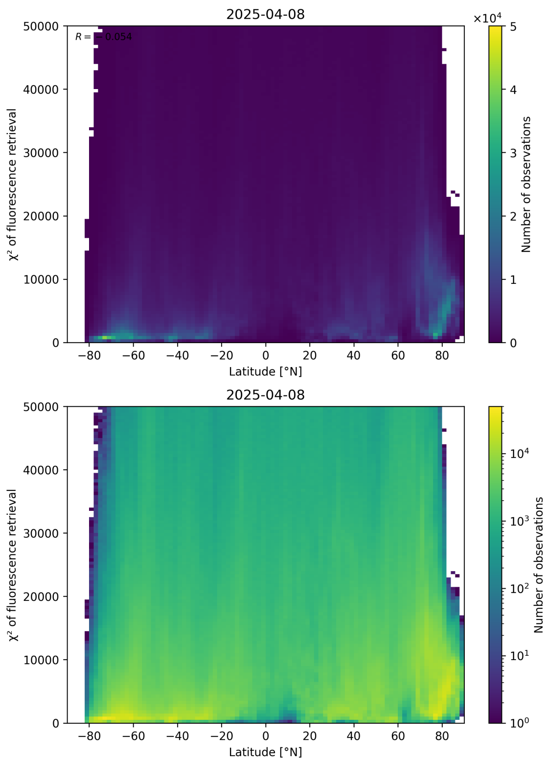
Figure 89: Scatter density plot of “Latitude” against “ \chi^2 of fluorescence retrieval” for 2025-04-08 to 2025-04-09.
