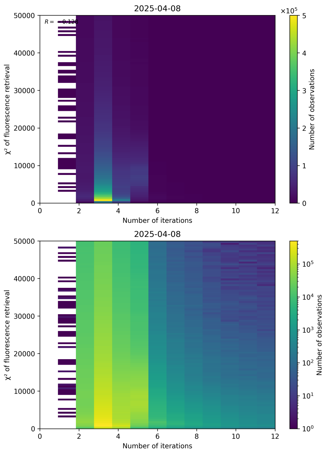
Figure 97: Scatter density plot of “Number of iterations” against “ \chi^2 of fluorescence retrieval” for 2025-04-08 to 2025-04-09.
