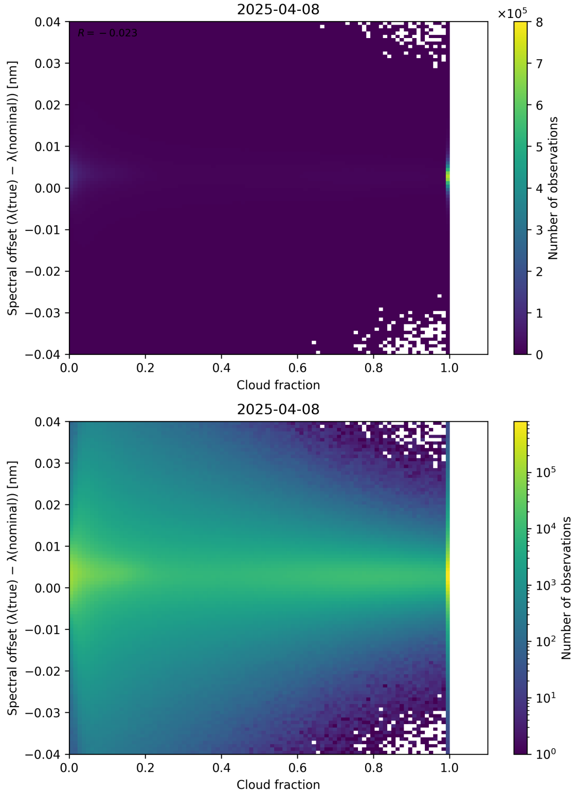
Figure 76: Scatter density plot of “Cloud fraction” against “Spectral offset ( \lambda_{\text{true}} - \lambda_{\text{nominal}} )” for 2025-04-08 to 2025-04-09.
