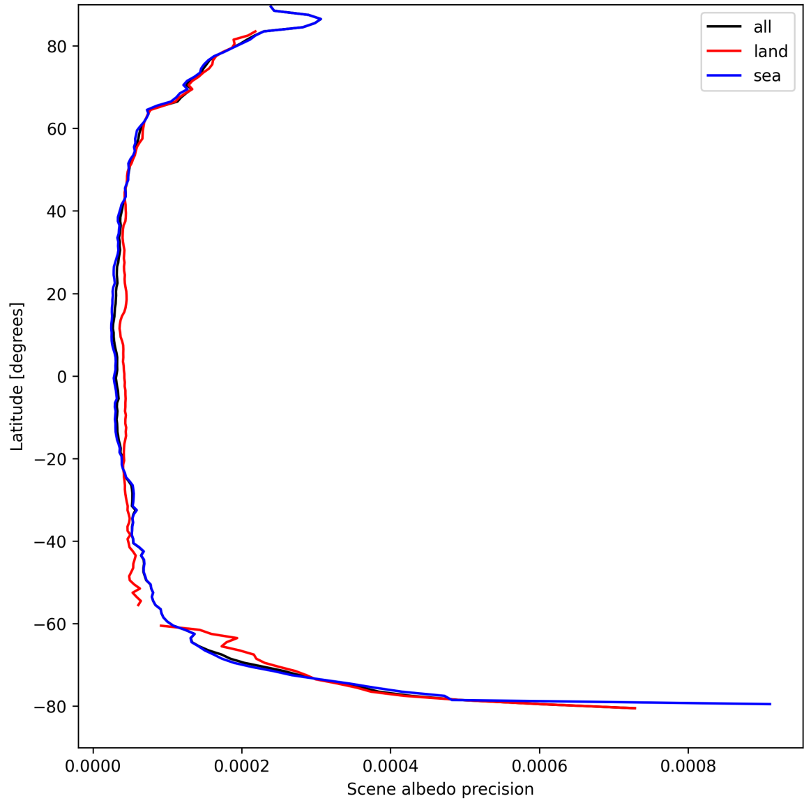
Figure 18: Zonal average of “Scene albedo precision” for 2025-04-08 to 2025-04-09.
