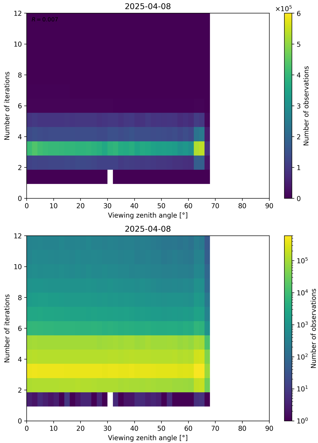
Figure 124: Scatter density plot of “Viewing zenith angle” against “Number of iterations” for 2025-04-08 to 2025-04-09.
