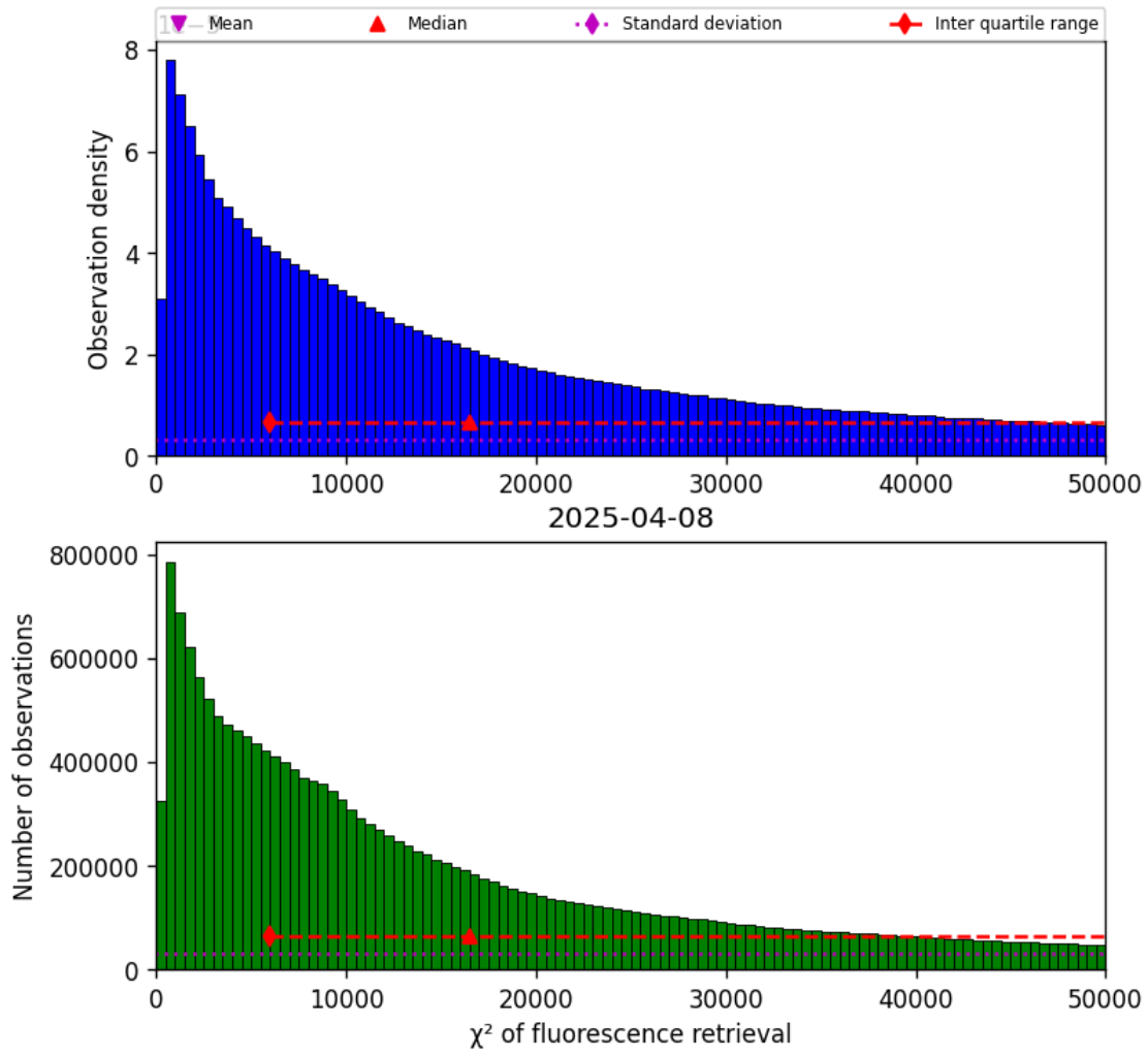
Figure 42: Histogram of “ \chi^2 of fluorescence retrieval” for 2025-04-08 to 2025-04-09
