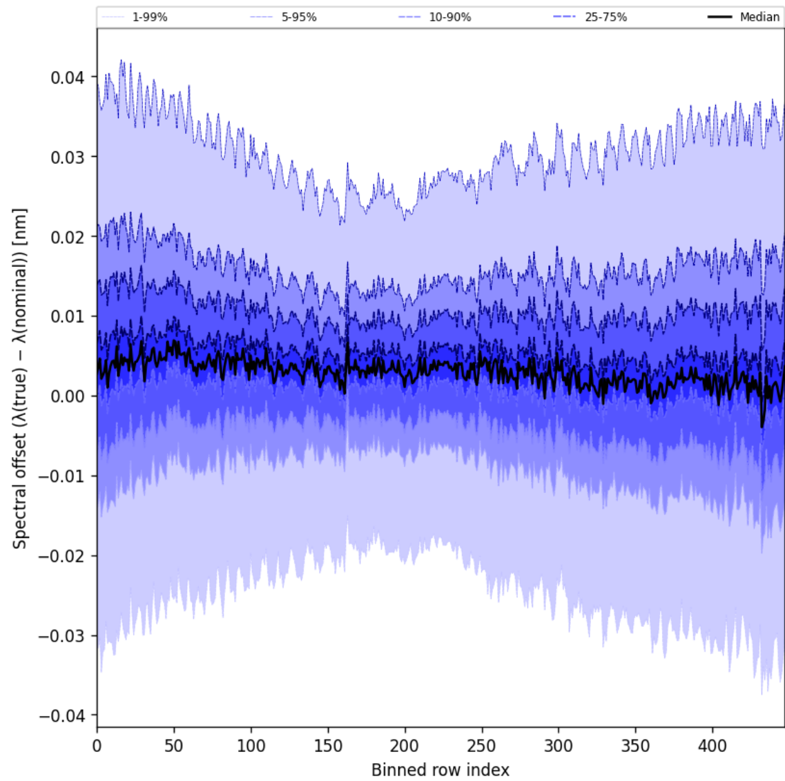
Figure 62: Along track statistics of “Spectral offset ( \lambda_{\text{true}} - \lambda_{\text{nominal}} )” for 2025-04-08 to 2025-04-09
