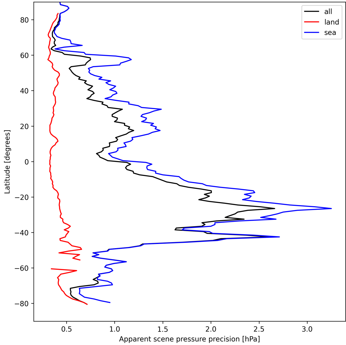
Figure 20: Zonal average of “Apparent scene pressure precision” for 2025-04-08 to 2025-04-09.
