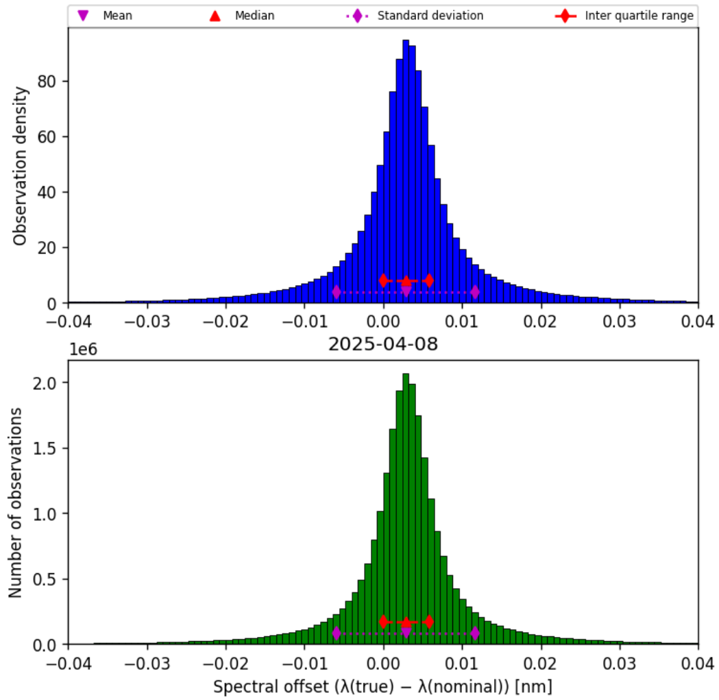
Figure 45: Histogram of “Spectral offset ( \lambda_{\text{true}} - \lambda_{\text{nominal}} )” for 2025-04-08 to 2025-04-09
