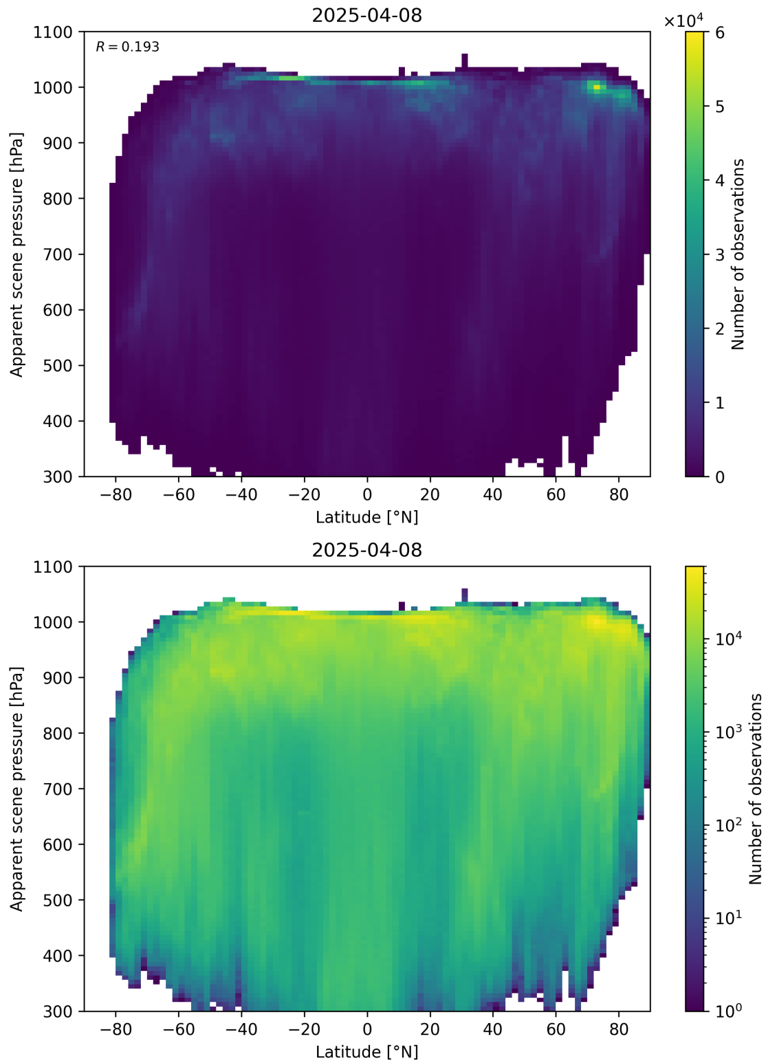
Figure 88: Scatter density plot of “Latitude” against “Apparent scene pressure” for 2025-04-08 to 2025-04-09.
