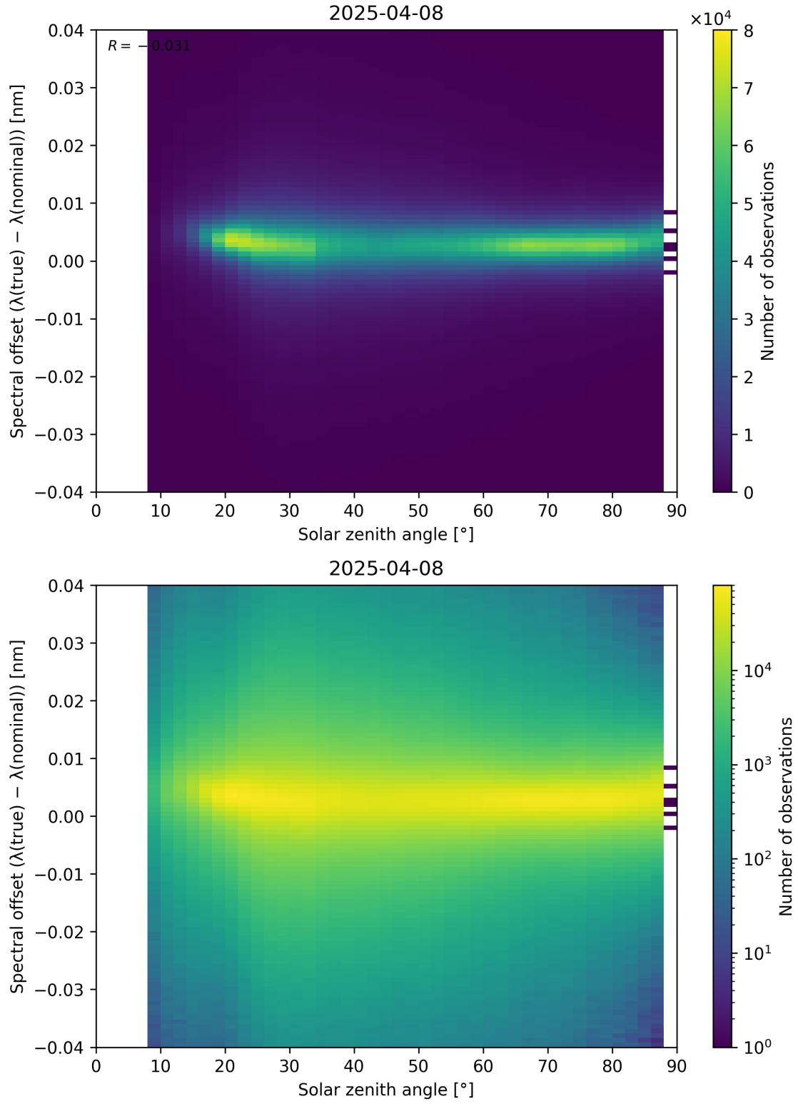
Figure 117: Scatter density plot of “Solar zenith angle” against “Spectral offset ( \lambda_{\text{true}} - \lambda_{\text{nominal}} )” for 2025-04-08 to 2025-04-09.
