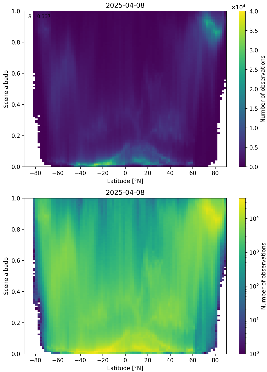
Figure 95: Scatter density plot of “Latitude” against “Scene albedo” for 2025-04-08 to 2025-04-09.
