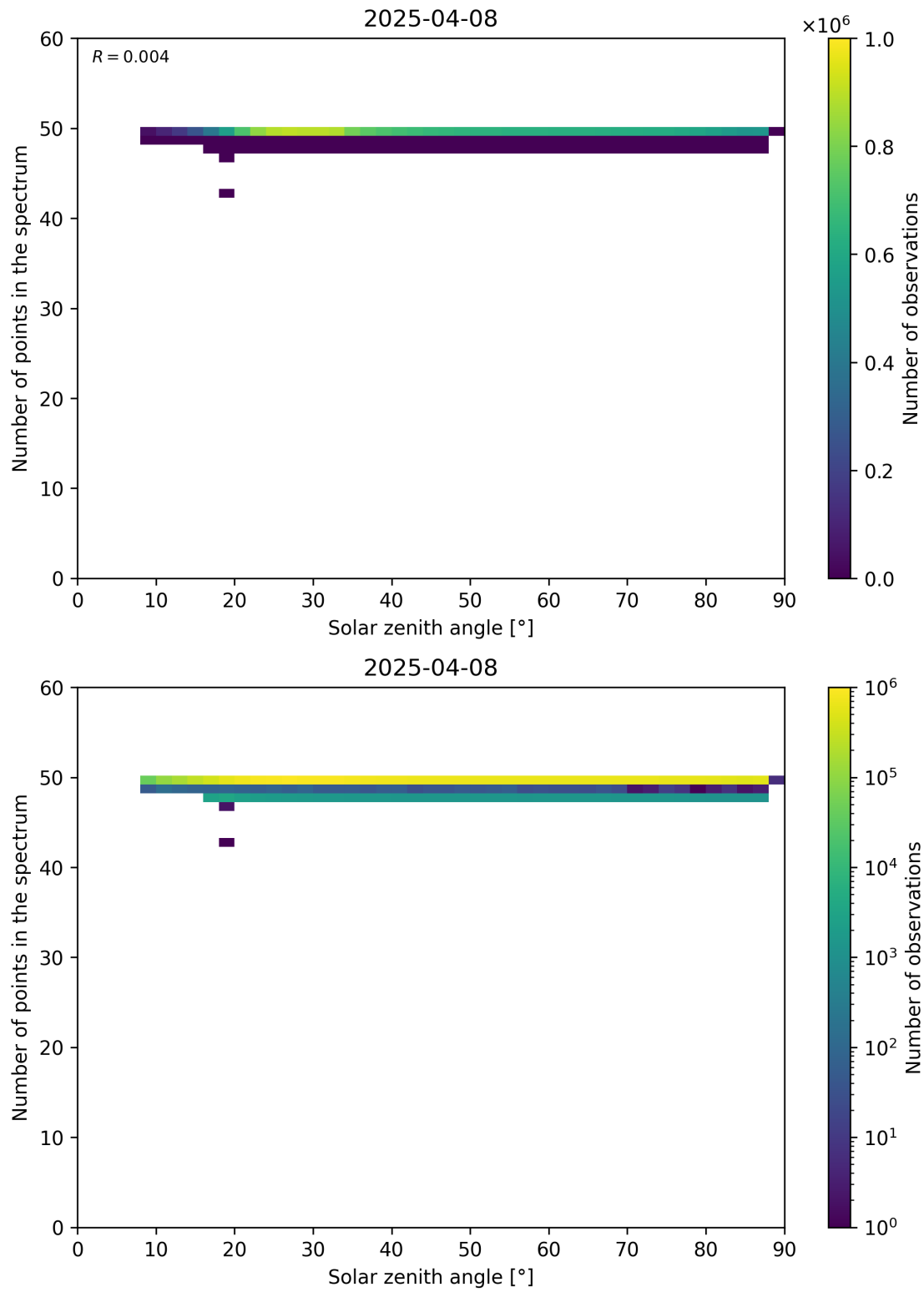
Figure 115: Scatter density plot of “Solar zenith angle” against “Number of points in the spectrum” for 2025-04-08 to 2025-04-09.
