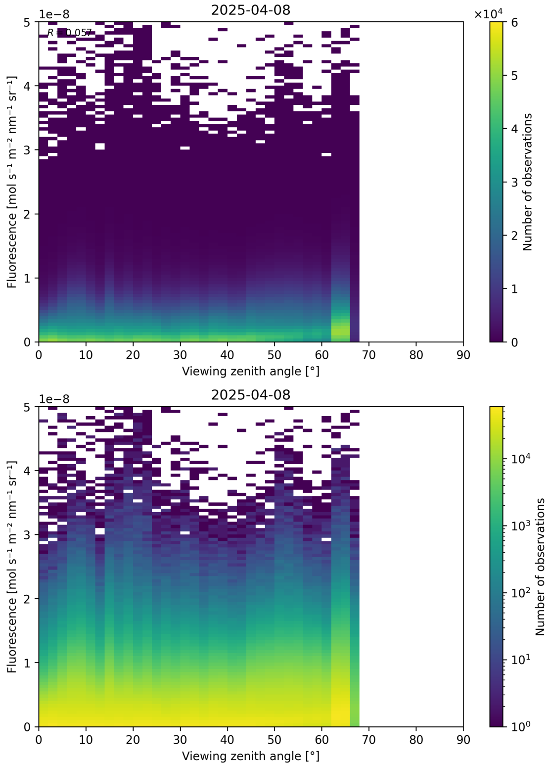
Figure 122: Scatter density plot of “Viewing zenith angle” against “Fluorescence” for 2025-04-08 to 2025-04-09.
