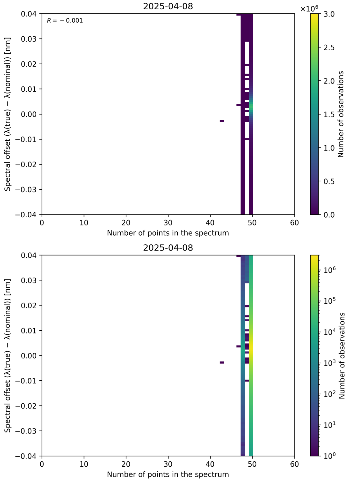
Figure 101: Scatter density plot of “Number of points in the spectrum” against “Spectral offset ( \lambda_{\text{true}} - \lambda_{\text{nominal}} )” for 2025-04-08 to 2025-04-09.
