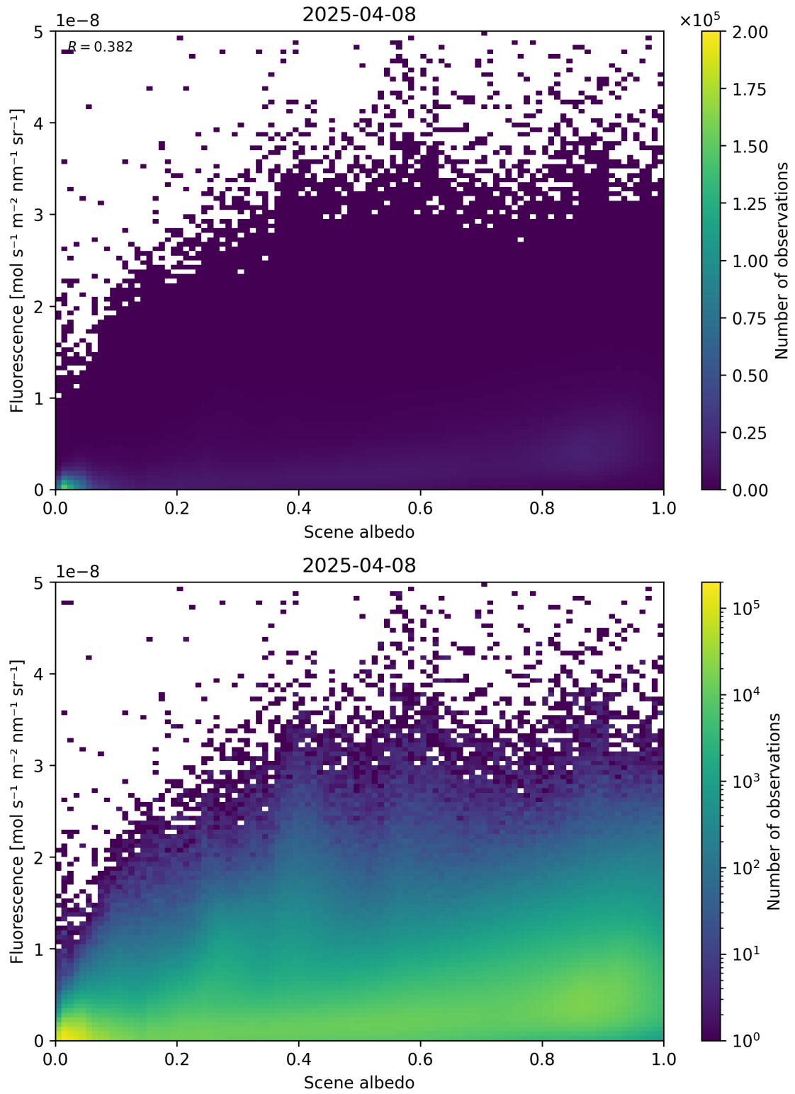
Figure 104: Scatter density plot of “Scene albedo” against “Fluorescence” for 2025-04-08 to 2025-04-09.
