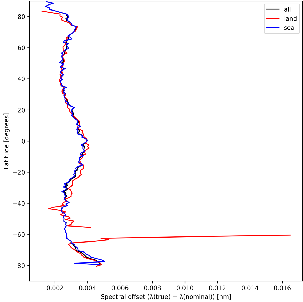
Figure 28: Zonal average of “Spectral offset ( \lambda_{\text{true}} - \lambda_{\text{nominal}} )” for 2025-04-08 to 2025-04-09.
