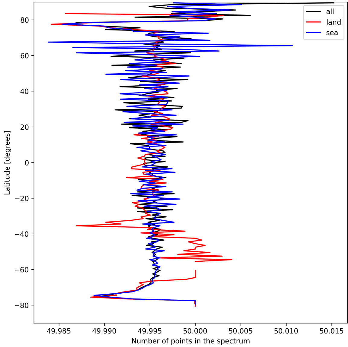
Figure 27: Zonal average of “Number of points in the spectrum” for 2025-04-08 to 2025-04-09.
