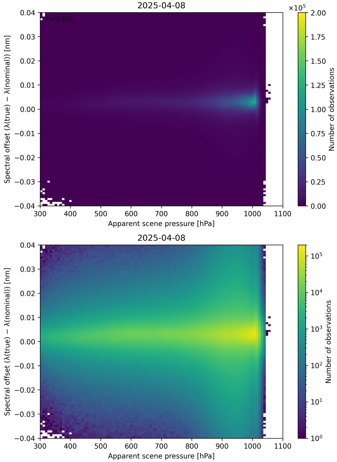
Figure 67: Scatter density plot of “Apparent scene pressure” against “Spectral offset ( \lambda_{\text{true}} - \lambda_{\text{nominal}} )” for 2025-04-08 to 2025-04-09.
