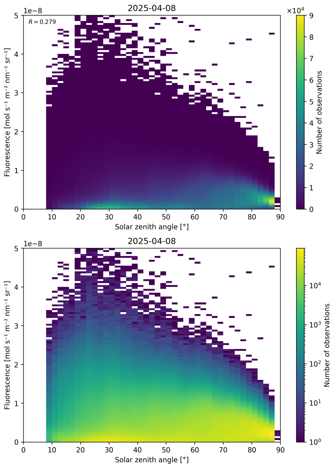
Figure 112: Scatter density plot of “Solar zenith angle” against “Fluorescence” for 2025-04-08 to 2025-04-09.
