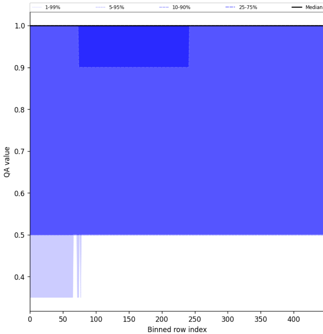
Figure 46: Along track statistics of “QA value” for 2025-04-08 to 2025-04-09
