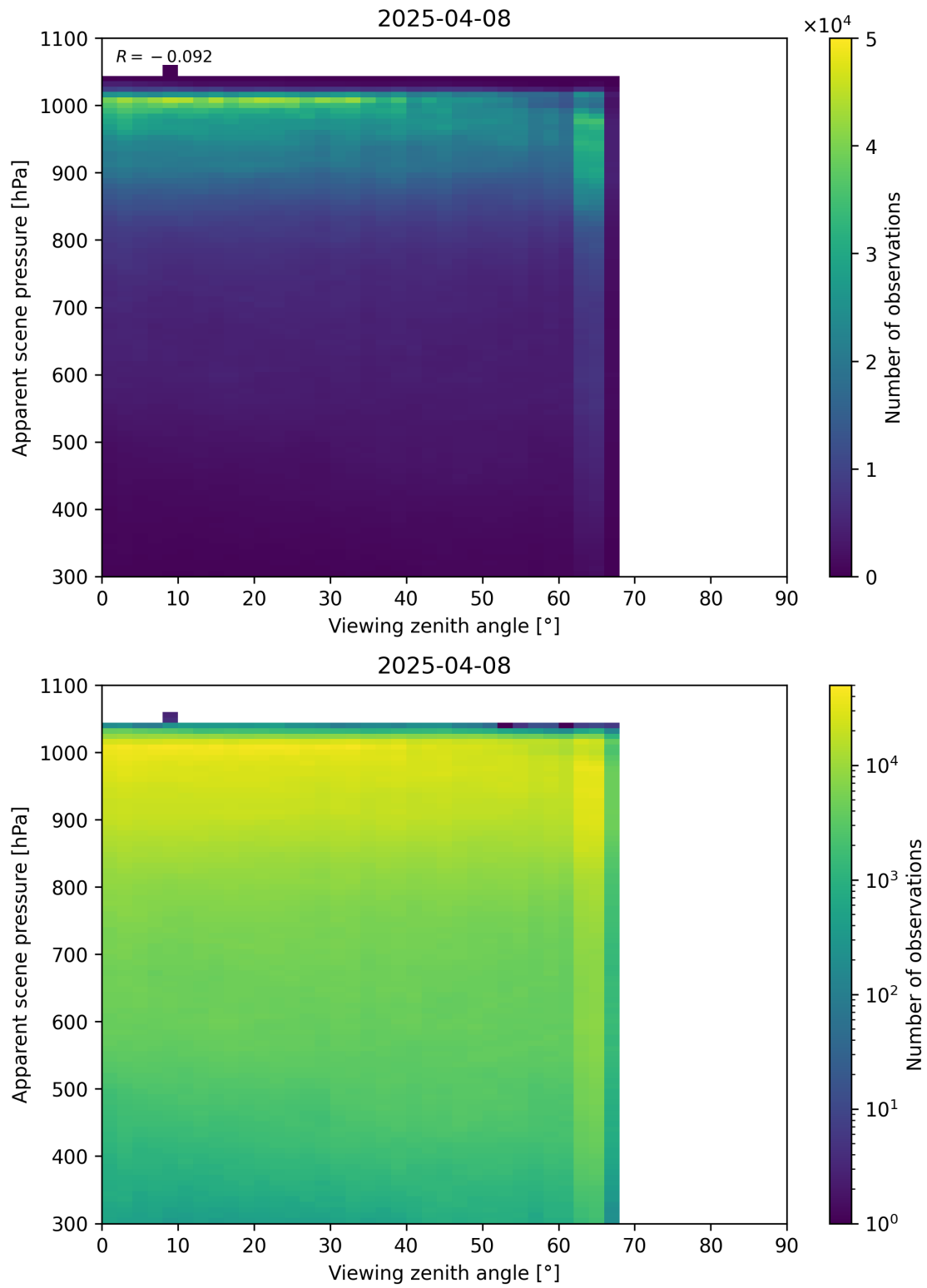
Figure 118: Scatter density plot of “Viewing zenith angle” against “Apparent scene pressure” for 2025-04-08 to 2025-04-09.
