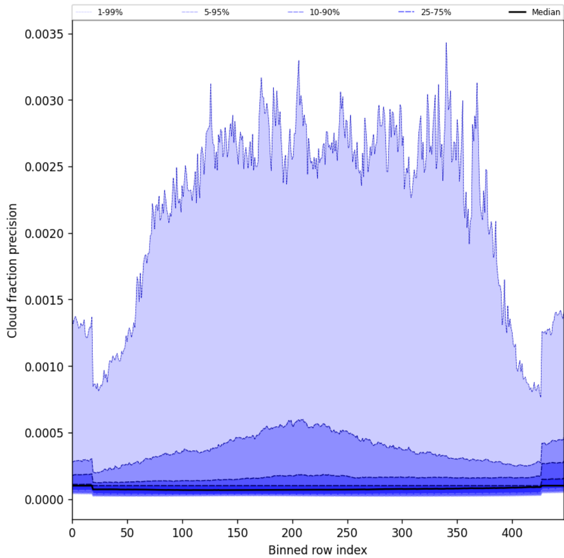
Figure 50: Along track statistics of “Cloud fraction precision” for 2025-04-08 to 2025-04-09
