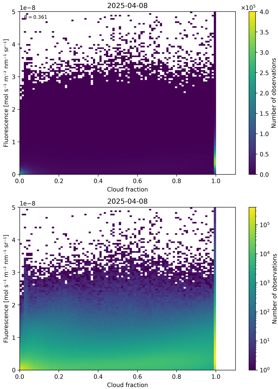
Figure 72: Scatter density plot of “Cloud fraction” against “Fluorescence” for 2025-04-08 to 2025-04-09.
