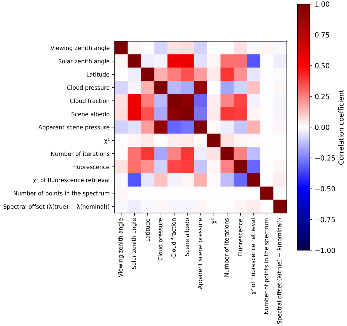
Figure 2: Map of correlation matrix for 2025-04-08 to 2025-04-09.
