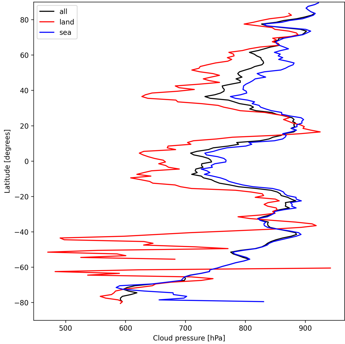
Figure 13: Zonal average of “Cloud pressure” for 2025-04-08 to 2025-04-09.
