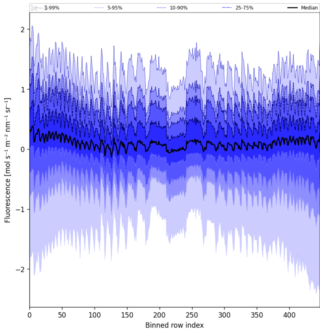
Figure 57: Along track statistics of “Fluorescence” for 2025-04-08 to 2025-04-09
