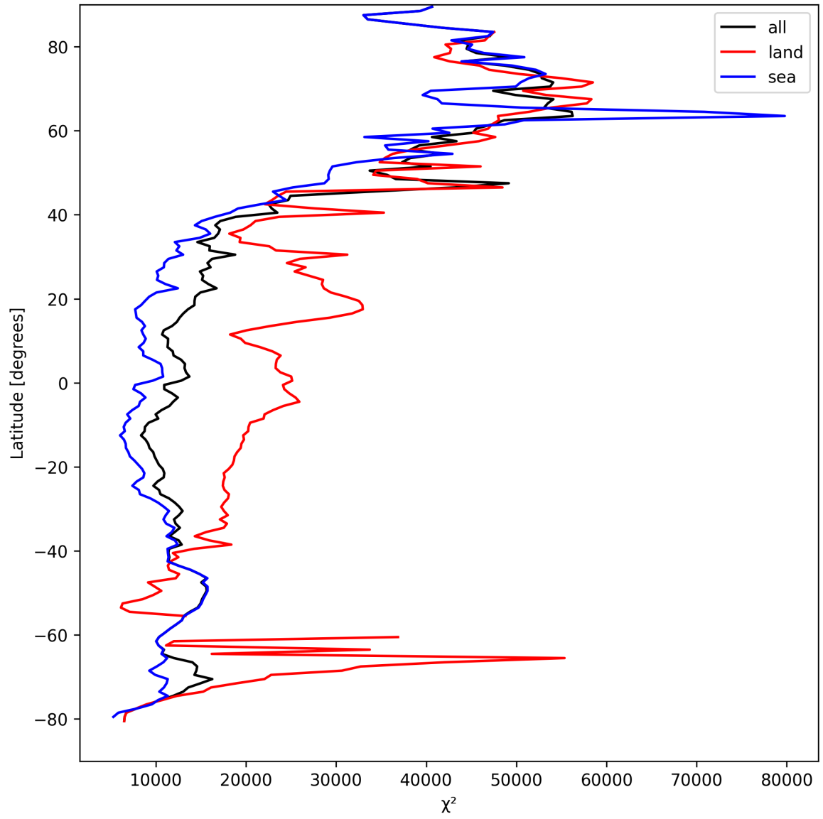
Figure 21: Zonal average of “ \chi^2 ” for 2025-04-08 to 2025-04-09.
