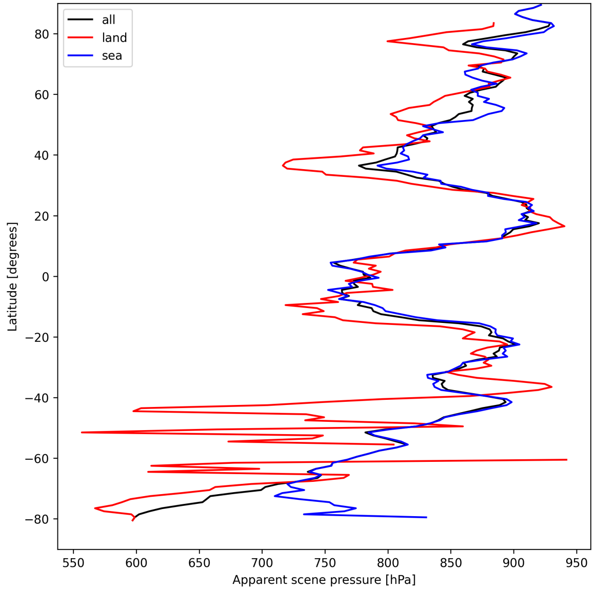
Figure 19: Zonal average of “Apparent scene pressure” for 2025-04-08 to 2025-04-09.
