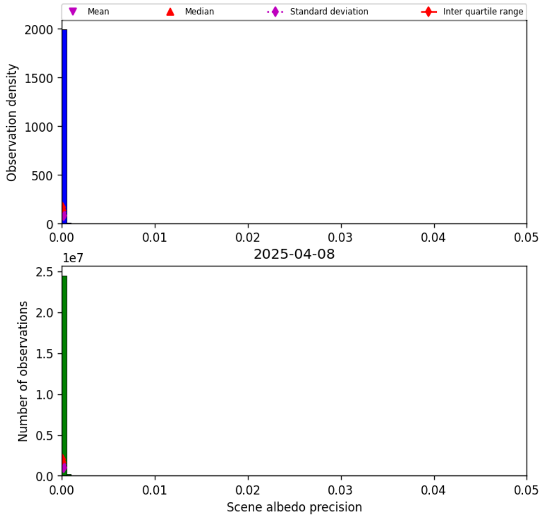
Figure 35: Histogram of “Scene albedo precision” for 2025-04-08 to 2025-04-09
