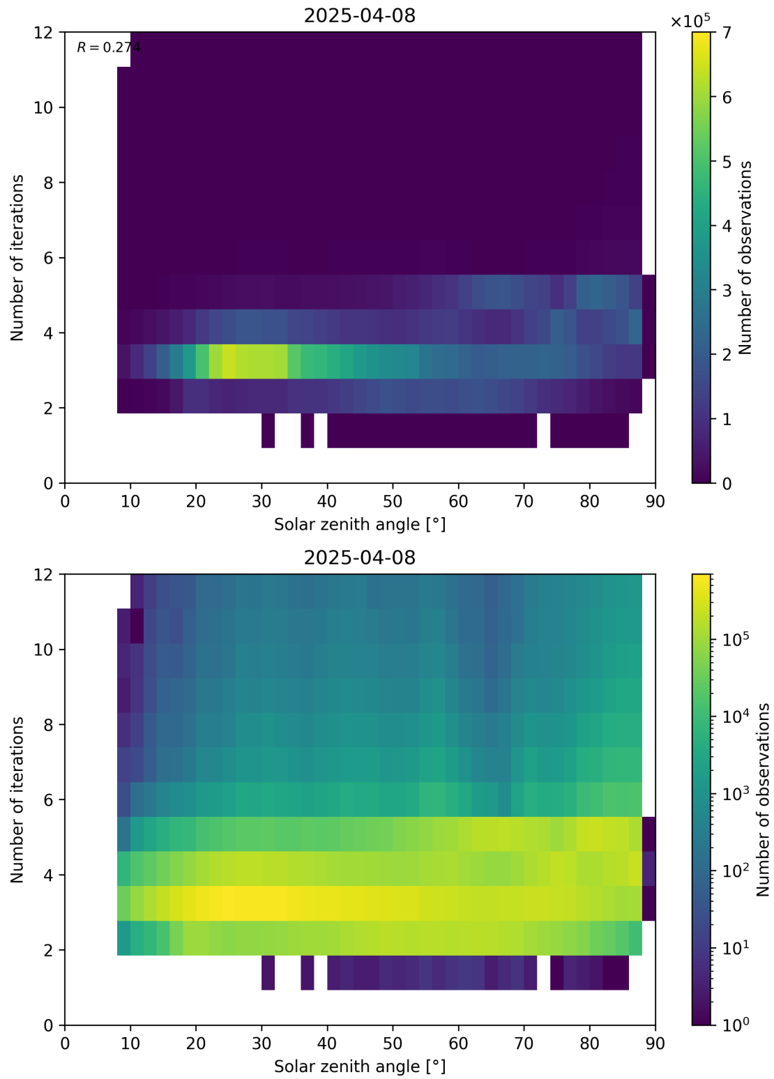
Figure 114: Scatter density plot of “Solar zenith angle” against “Number of iterations” for 2025-04-08 to 2025-04-09.
