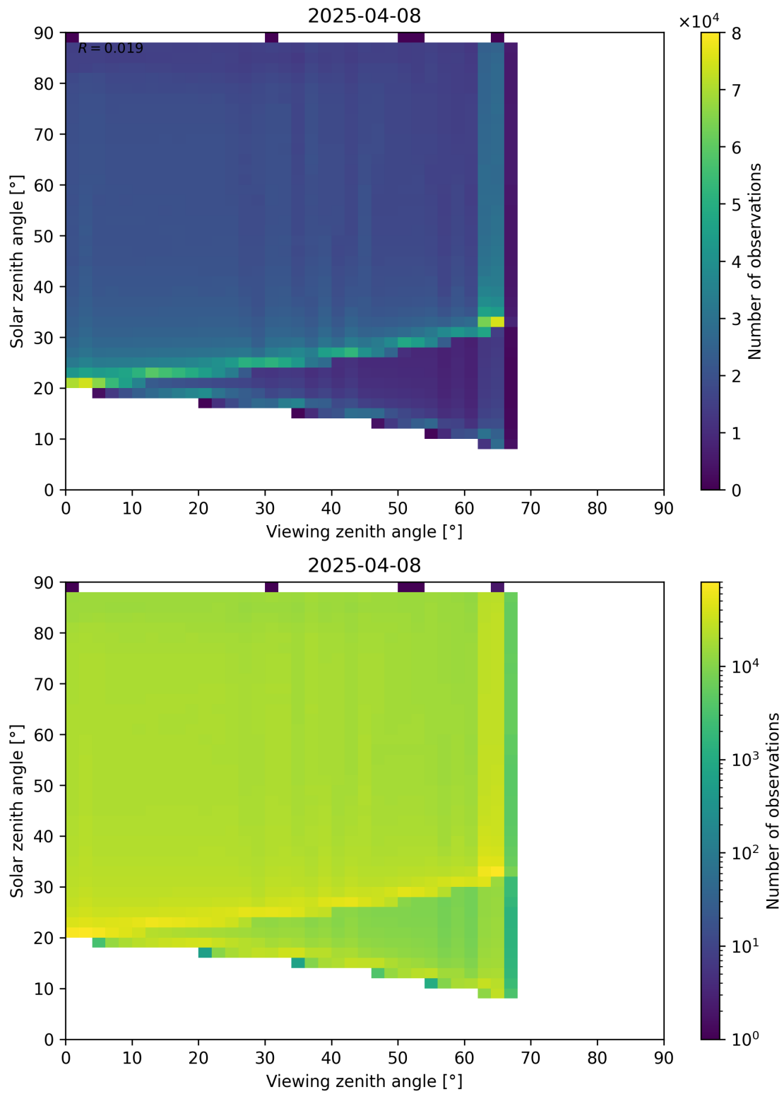
Figure 127: Scatter density plot of “Viewing zenith angle” against “Solar zenith angle” for 2025-04-08 to 2025-04-09.
