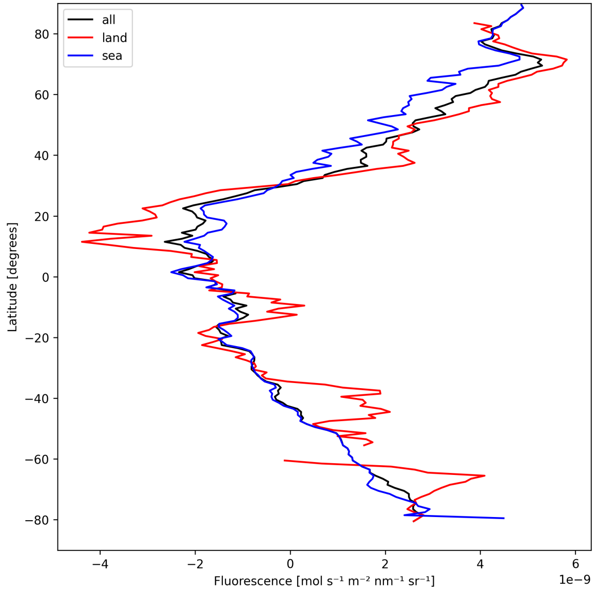
Figure 23: Zonal average of “Fluorescence” for 2025-04-08 to 2025-04-09.
