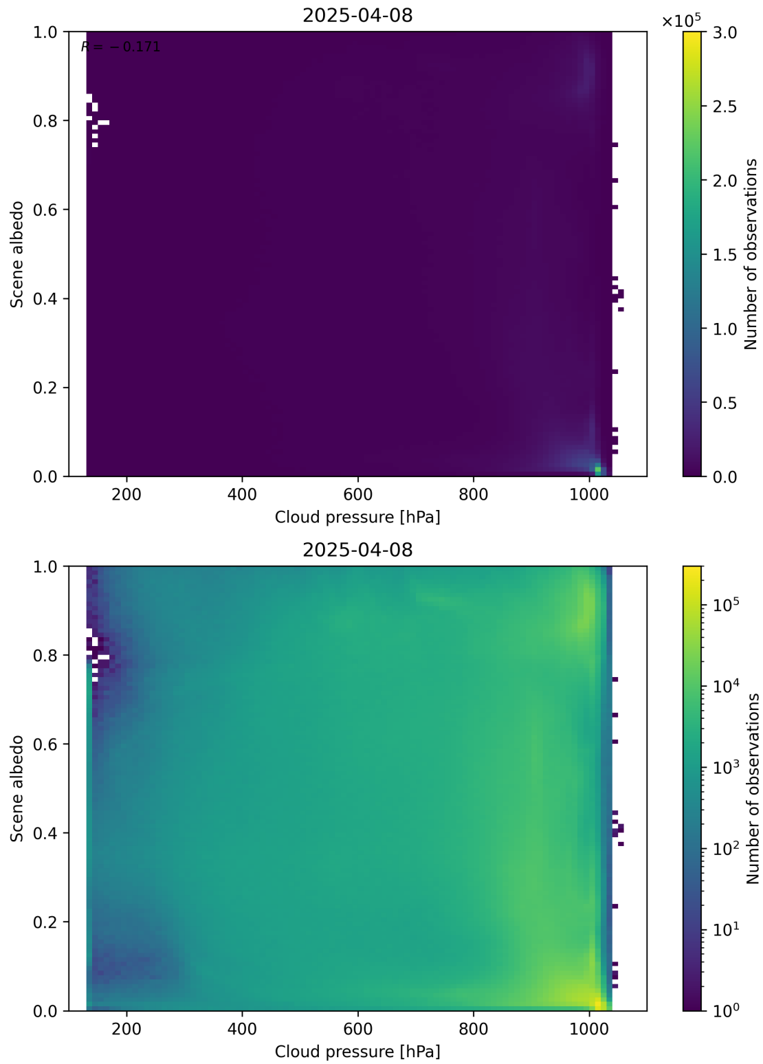
Figure 83: Scatter density plot of “Cloud pressure” against “Scene albedo” for 2025-04-08 to 2025-04-09.
