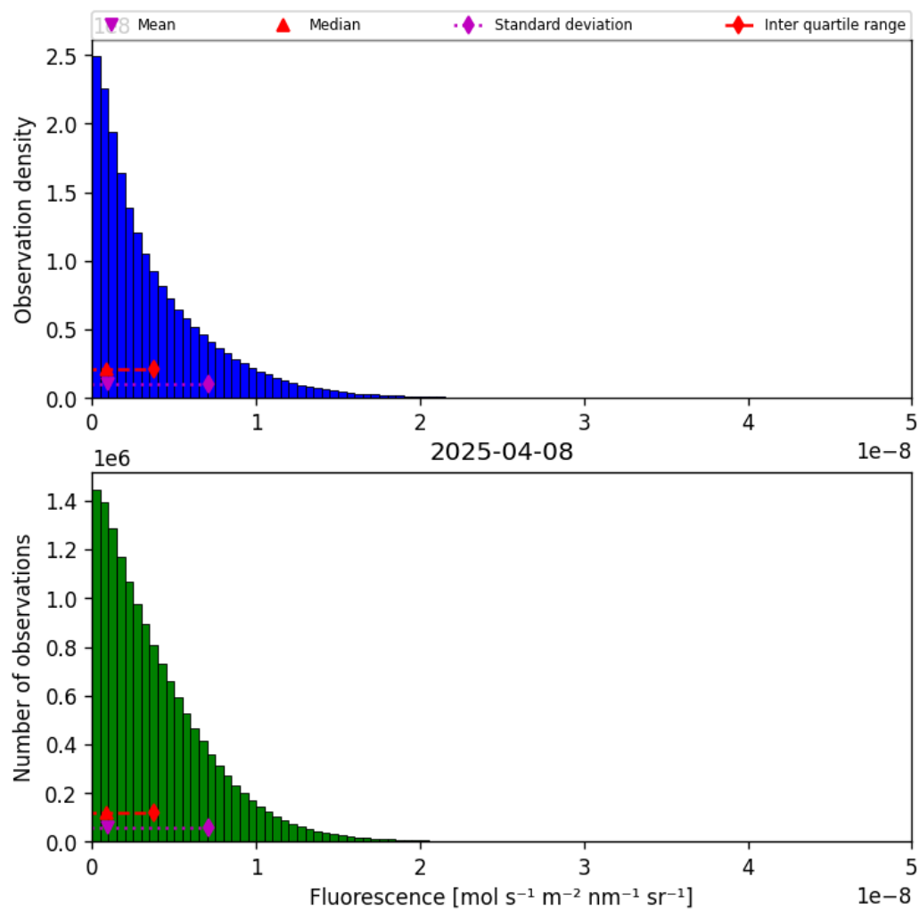
Figure 40: Histogram of “Fluorescence” for 2025-04-08 to 2025-04-09
