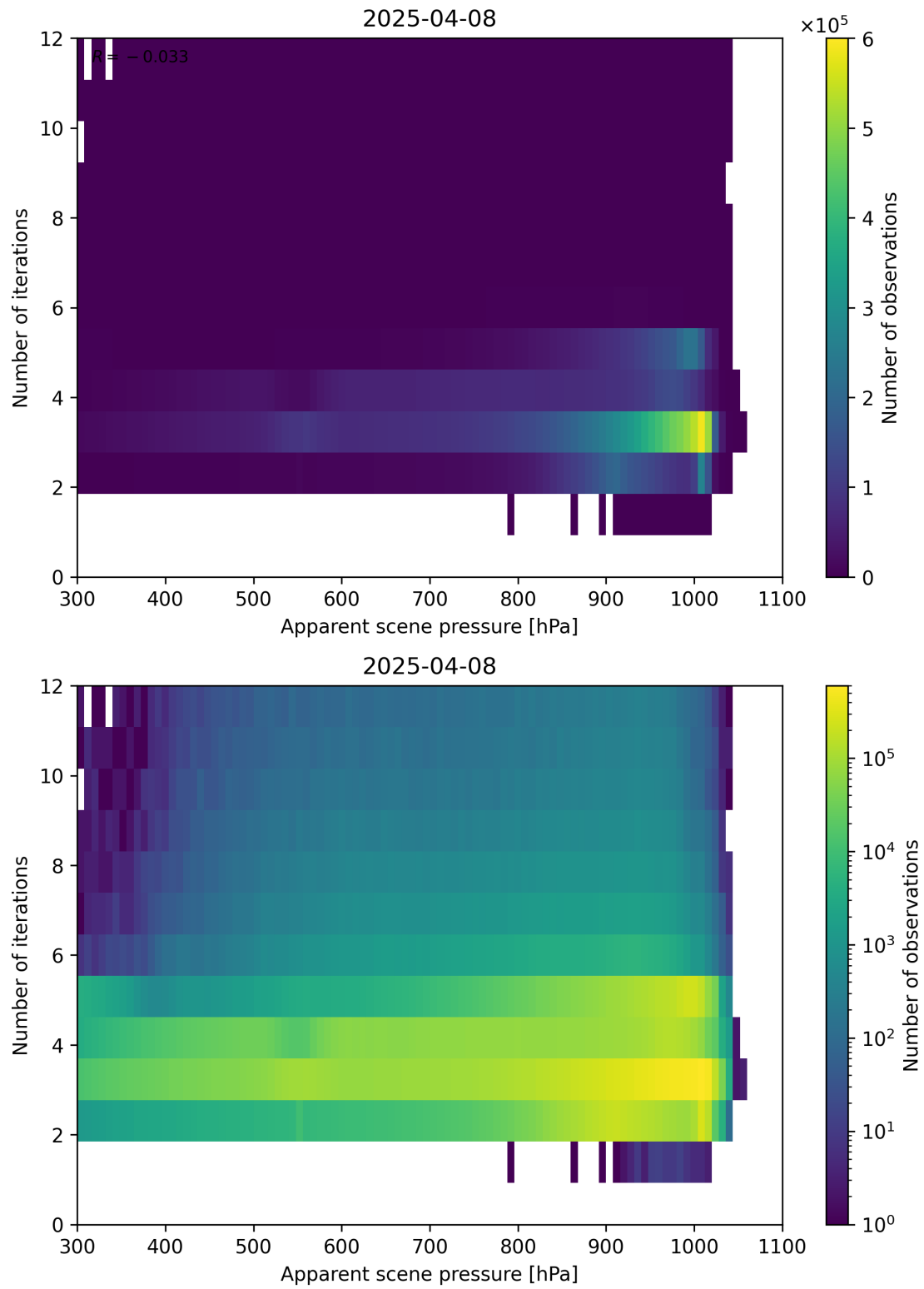
Figure 65: Scatter density plot of “Apparent scene pressure” against “Number of iterations” for 2025-04-08 to 2025-04-09.
