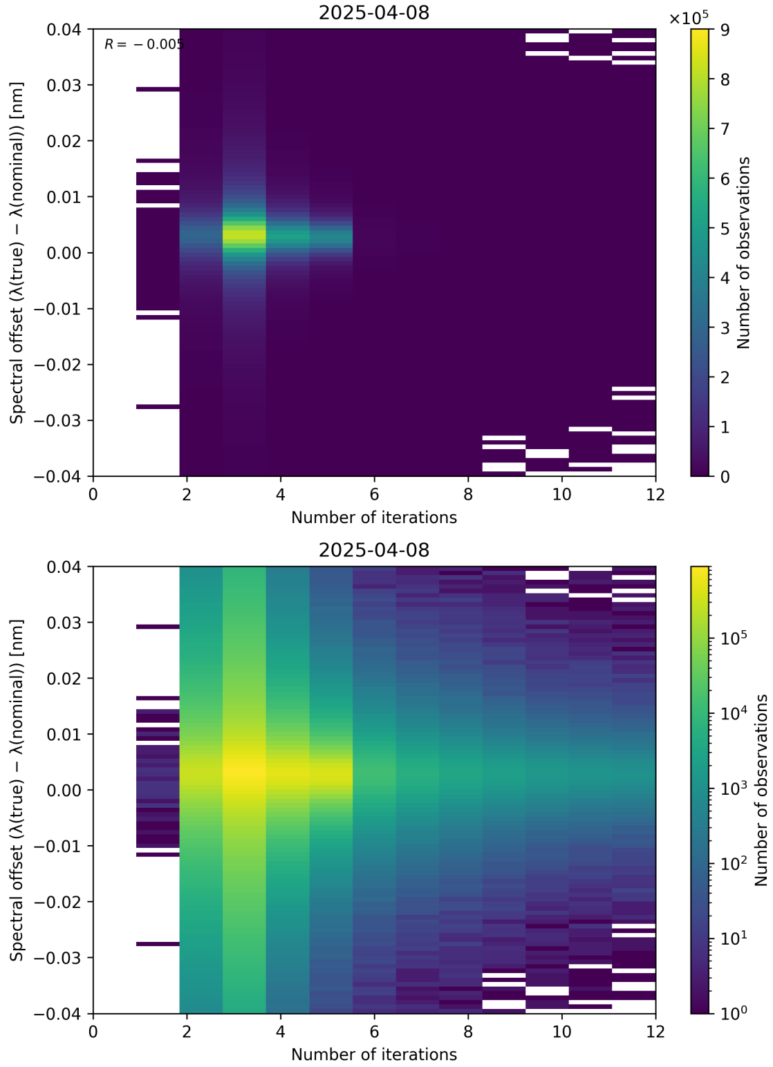
Figure 100: Scatter density plot of “Number of iterations” against “Spectral offset ( \lambda_{\text{true}} - \lambda_{\text{nominal}} )” for 2025-04-08 to 2025-04-09.
