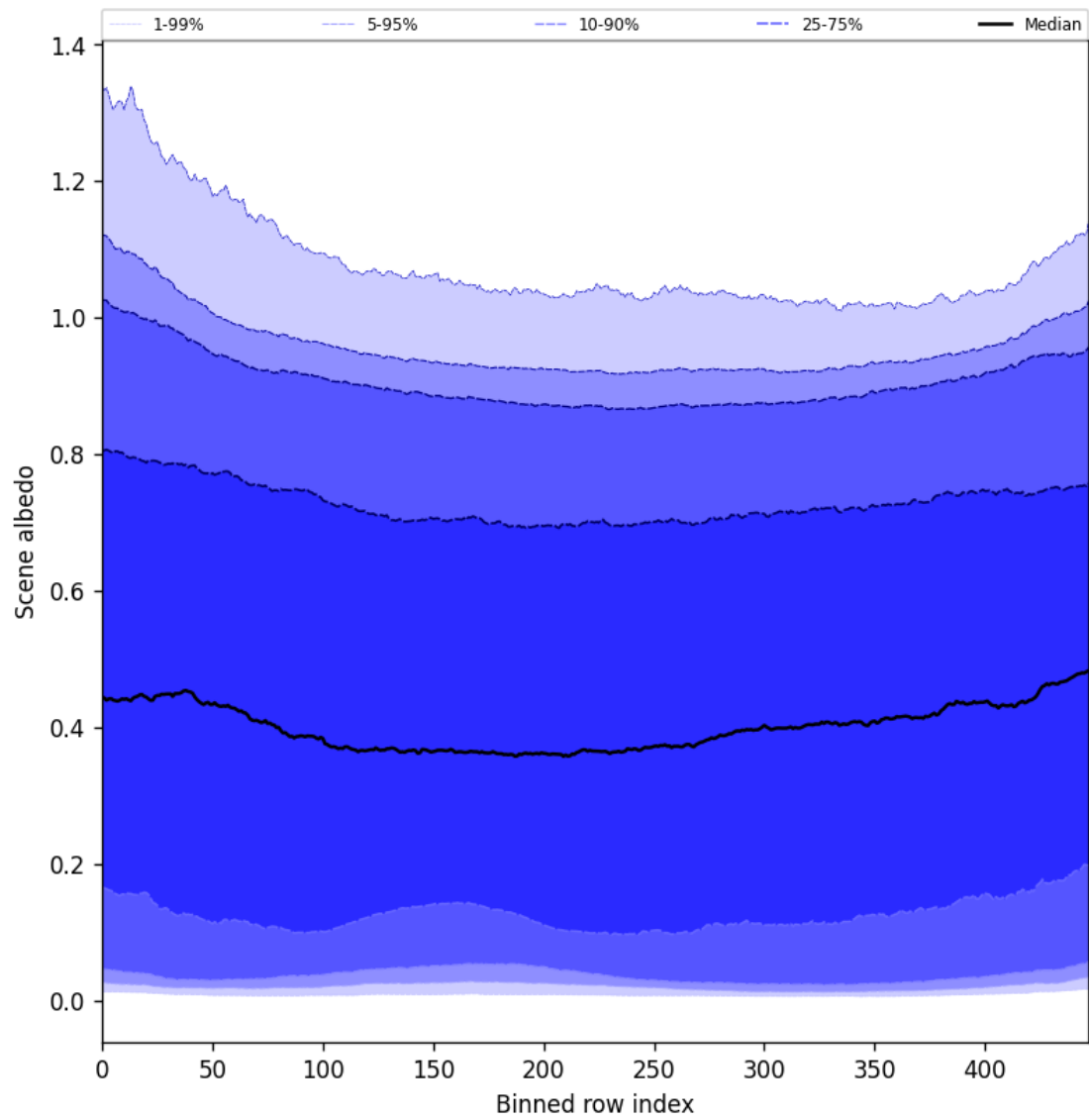
Figure 51: Along track statistics of “Scene albedo” for 2025-04-08 to 2025-04-09
