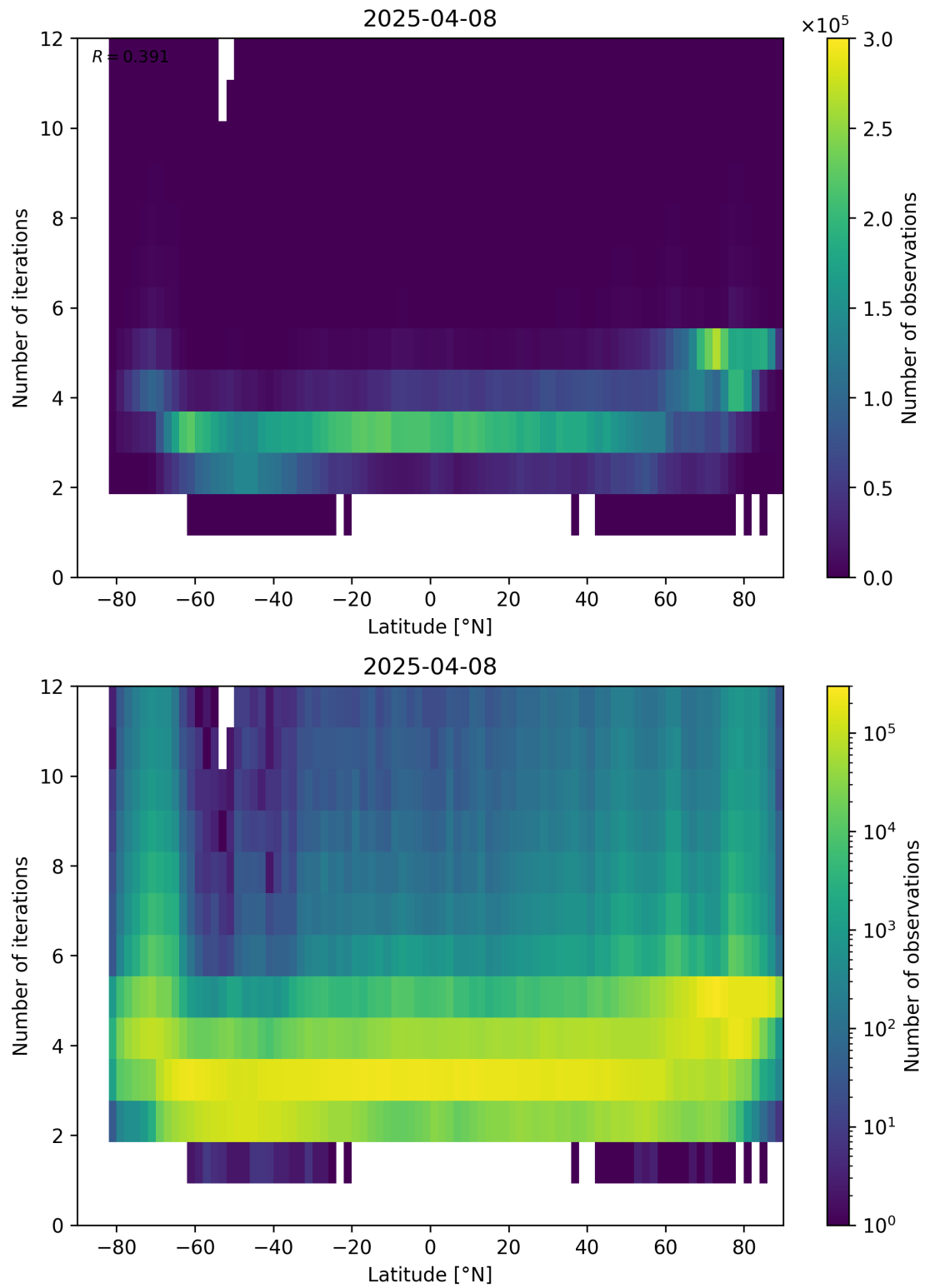
Figure 93: Scatter density plot of “Latitude” against “Number of iterations” for 2025-04-08 to 2025-04-09.
