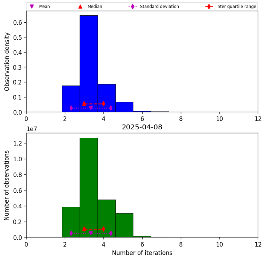
Figure 39: Histogram of “Number of iterations” for 2025-04-08 to 2025-04-09
