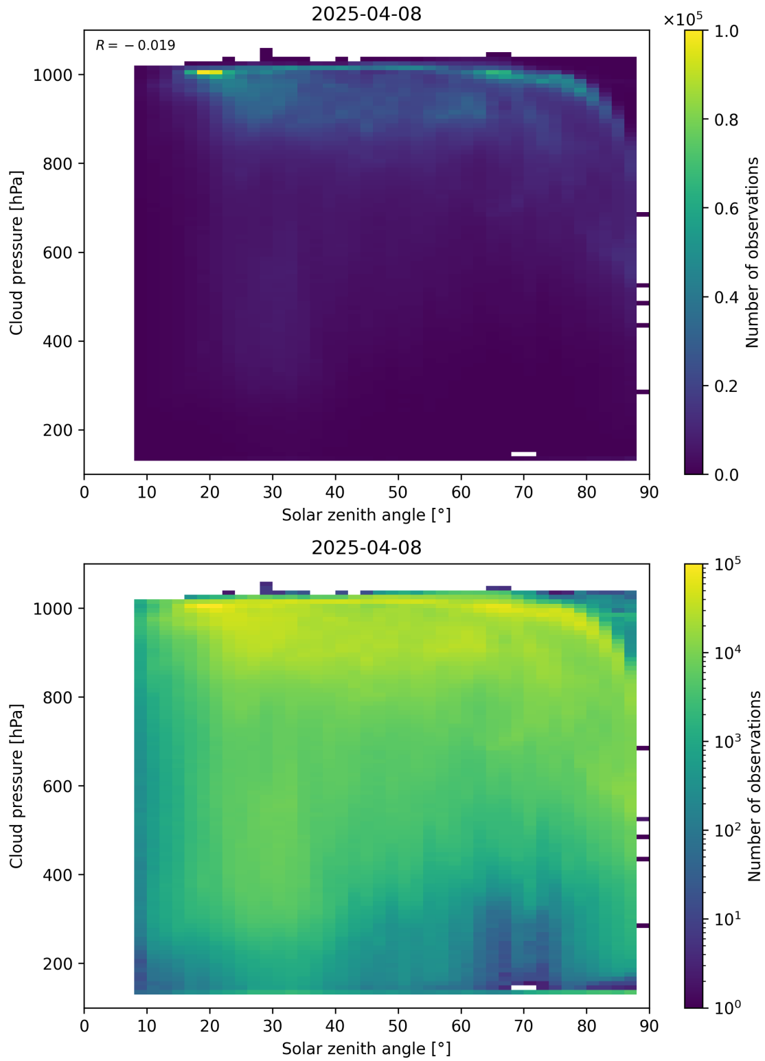
Figure 111: Scatter density plot of “Solar zenith angle” against “Cloud pressure” for 2025-04-08 to 2025-04-09.
