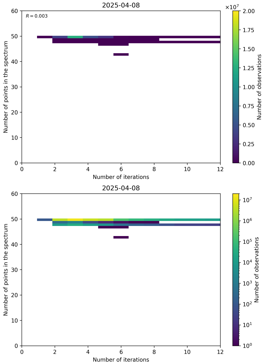
Figure 99: Scatter density plot of “Number of iterations” against “Number of points in the spectrum” for 2025-04-08 to 2025-04-09.
