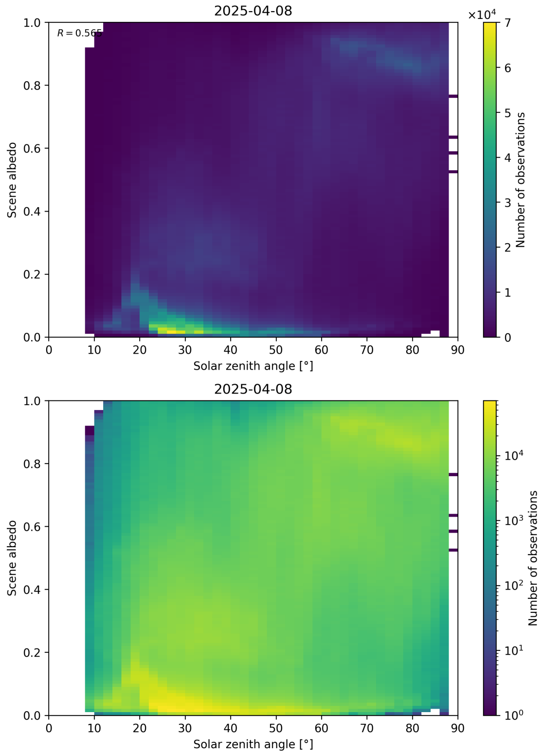
Figure 116: Scatter density plot of “Solar zenith angle” against “Scene albedo” for 2025-04-08 to 2025-04-09.
