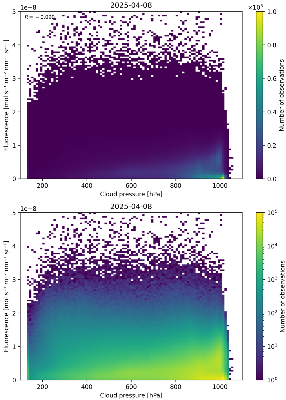
Figure 80: Scatter density plot of “Cloud pressure” against “Fluorescence” for 2025-04-08 to 2025-04-09.
