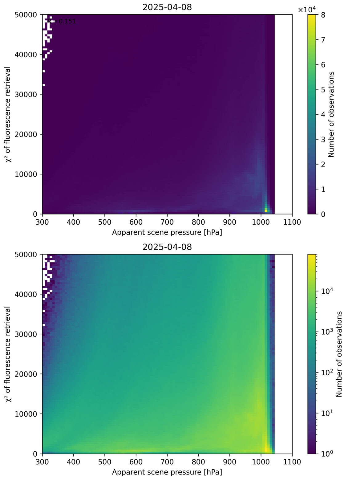
Figure 63: Scatter density plot of “Apparent scene pressure” against “ \chi^2 of fluorescence retrieval” for 2025-04-08 to 2025-04-09.
