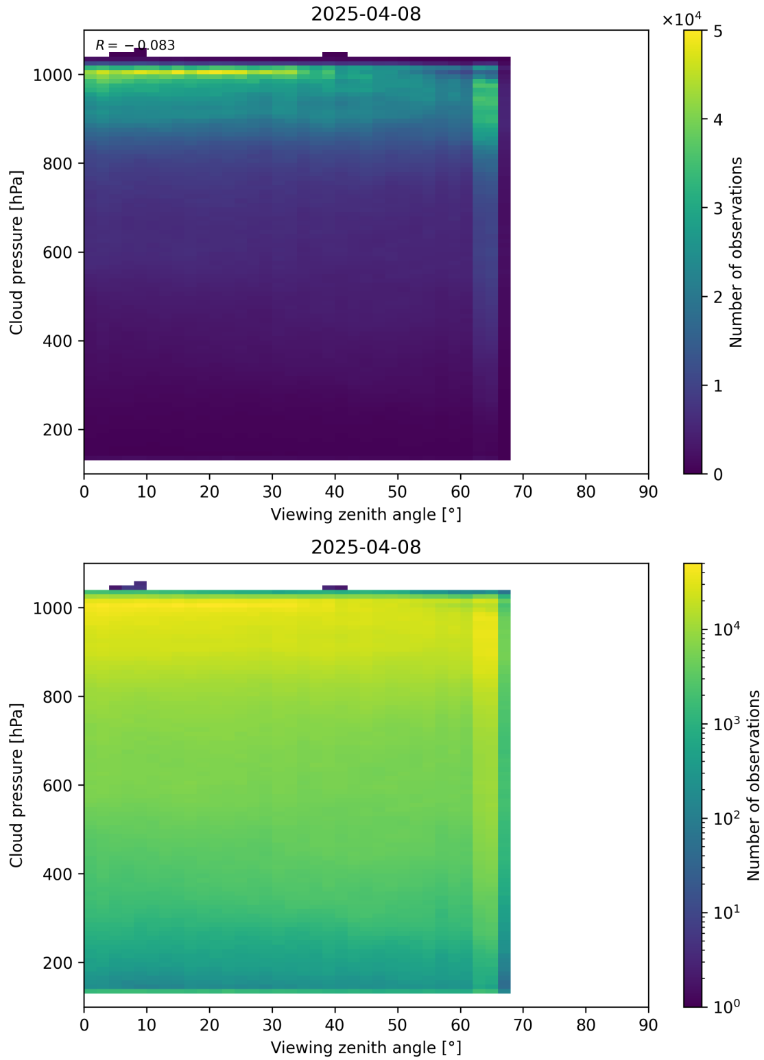
Figure 121: Scatter density plot of “Viewing zenith angle” against “Cloud pressure” for 2025-04-08 to 2025-04-09.
