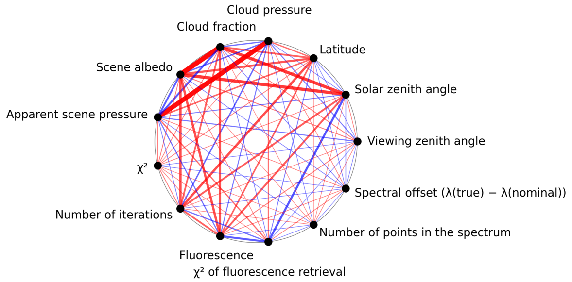
Figure 1: Map of correlation graph for 2025-04-08 to 2025-04-09.
