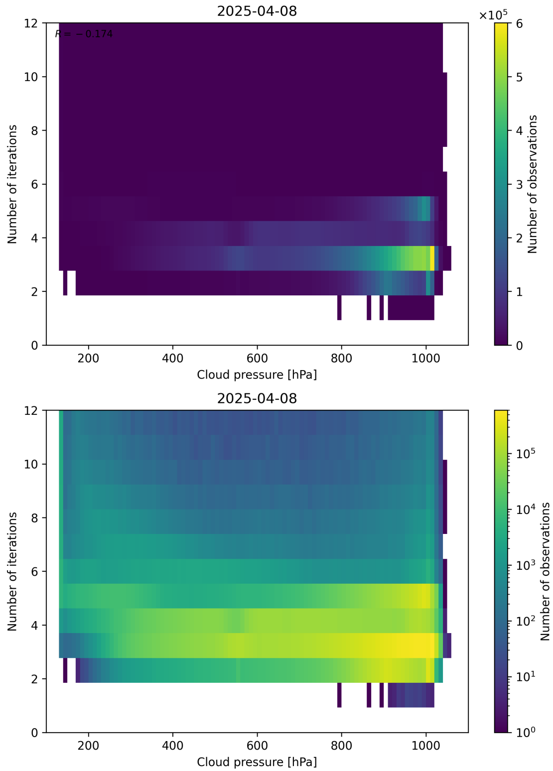
Figure 81: Scatter density plot of “Cloud pressure” against “Number of iterations” for 2025-04-08 to 2025-04-09.
