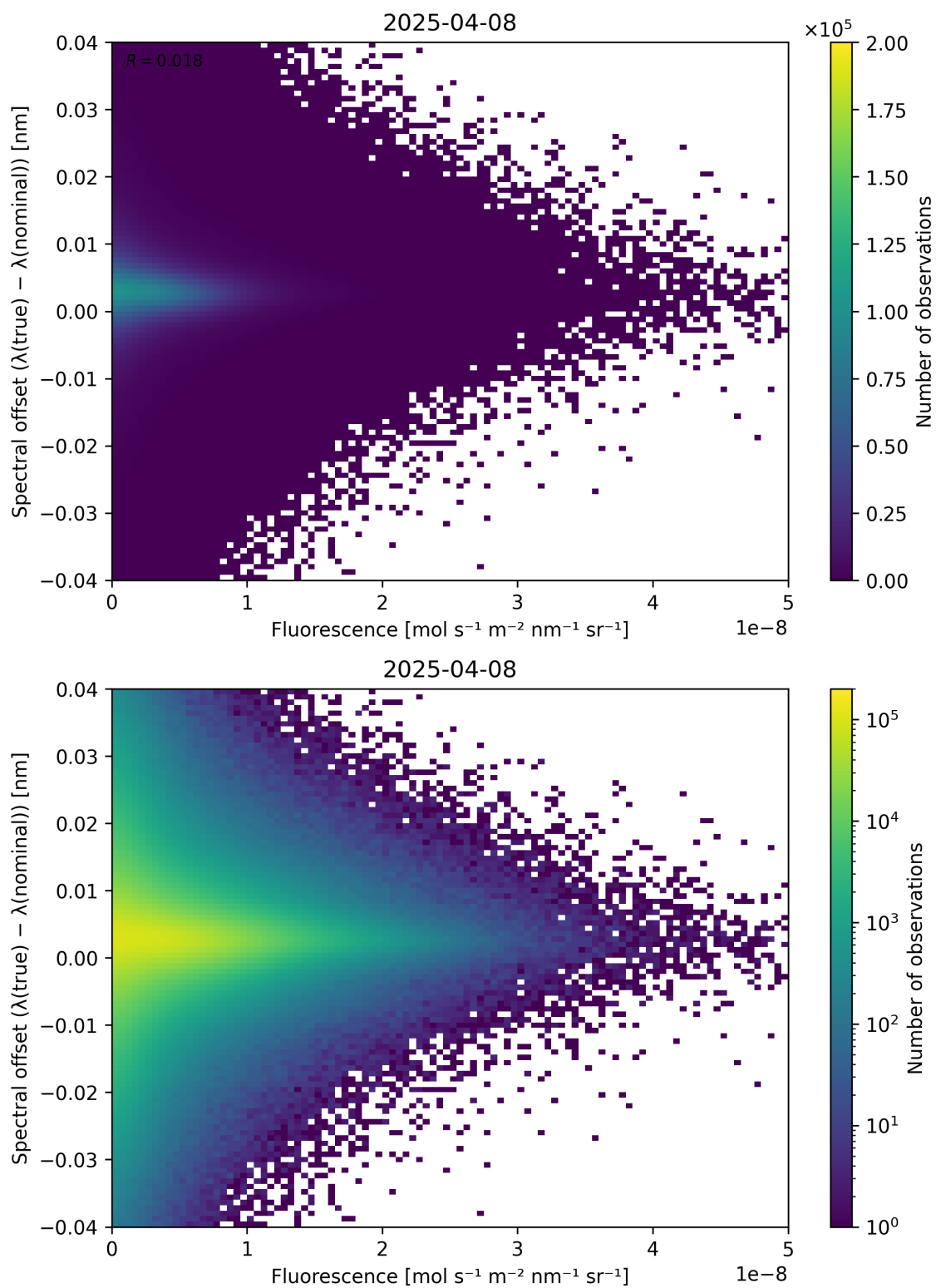
Figure 87: Scatter density plot of “Fluorescence” against “Spectral offset ( \lambda_{\text{true}} - \lambda_{\text{nominal}} )” for 2025-04-08 to 2025-04-09.
