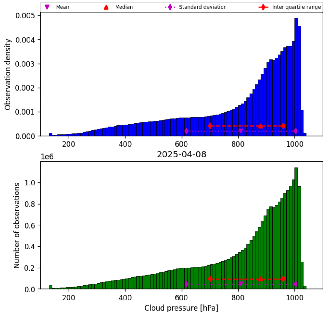
Figure 30: Histogram of “Cloud pressure” for 2025-04-08 to 2025-04-09
