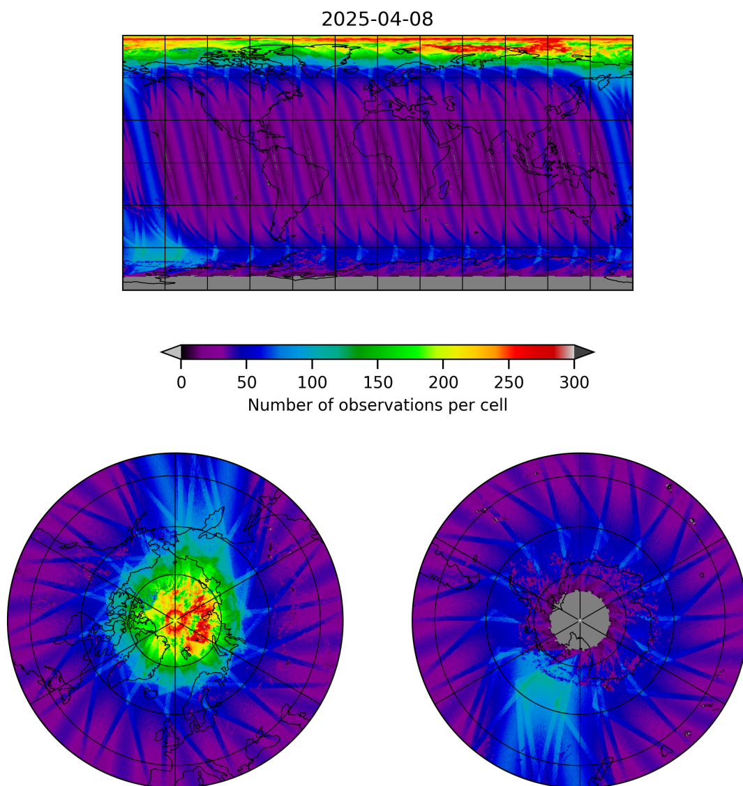
Figure 11: Map of the number of observations for 2025-04-08 to 2025-04-09
