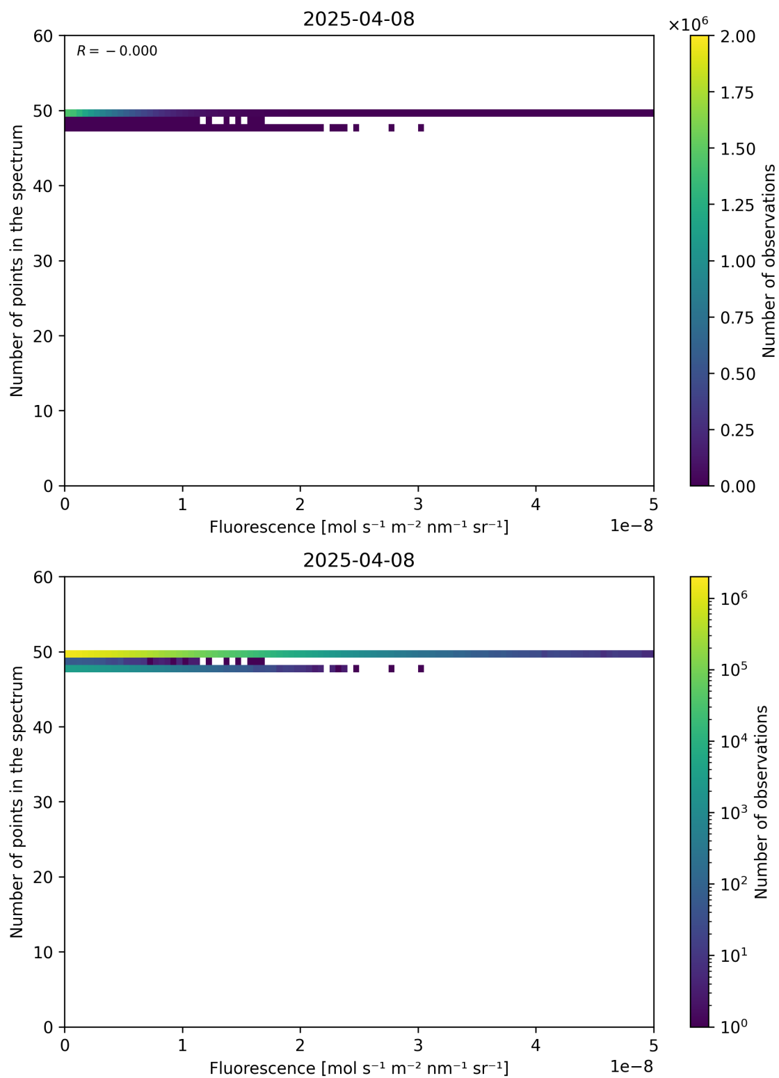
Figure 86: Scatter density plot of “Fluorescence” against “Number of points in the spectrum” for 2025-04-08 to 2025-04-09.
