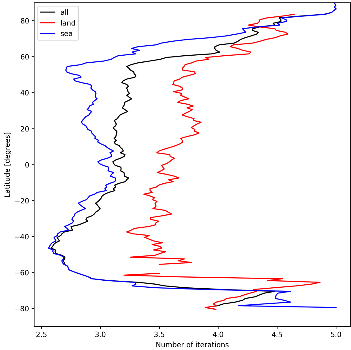
Figure 22: Zonal average of “Number of iterations” for 2025-04-08 to 2025-04-09.
