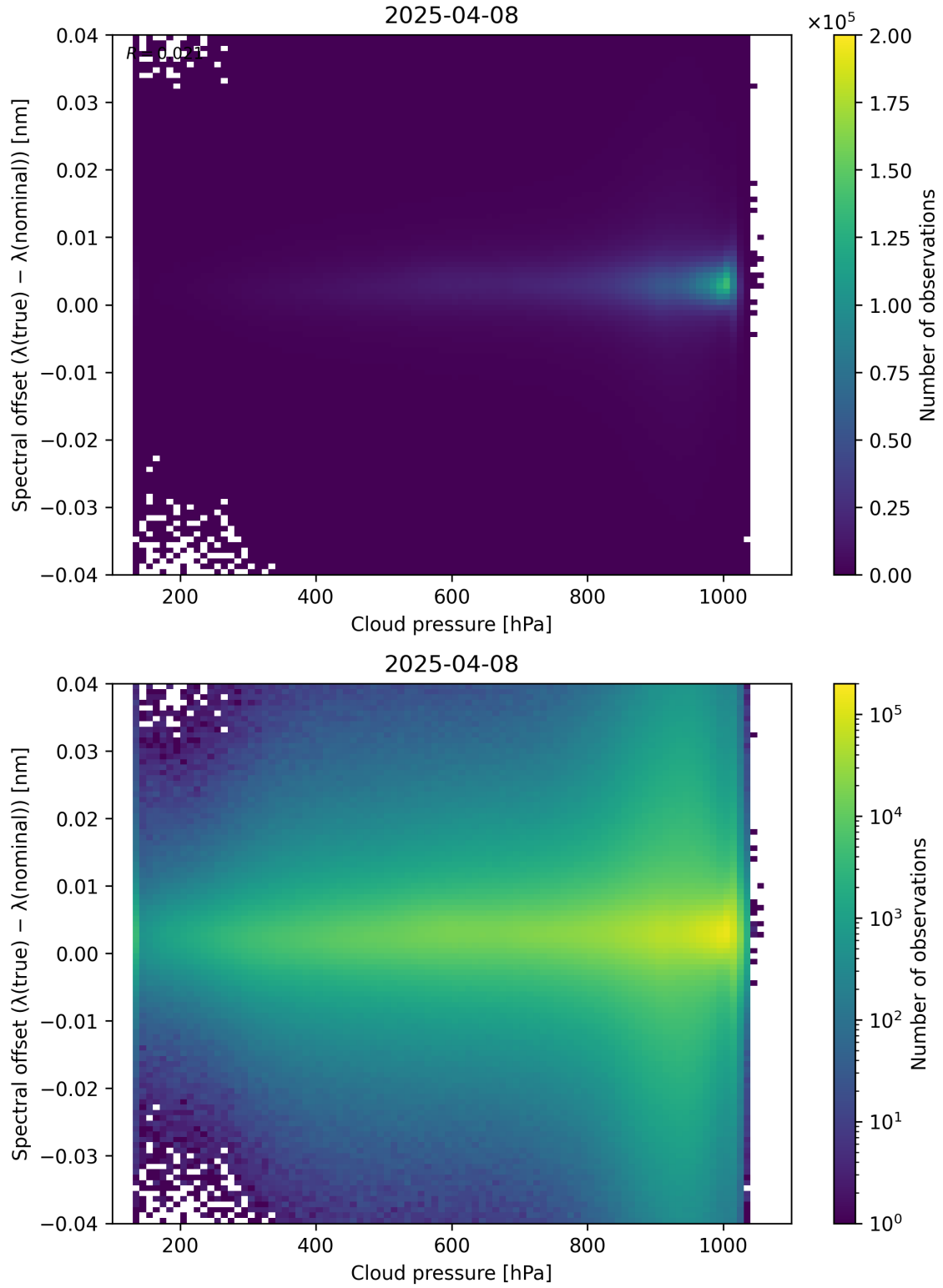
Figure 84: Scatter density plot of “Cloud pressure” against “Spectral offset ( \lambda_{\text{true}} - \lambda_{\text{nominal}} )” for 2025-04-08 to 2025-04-09.
