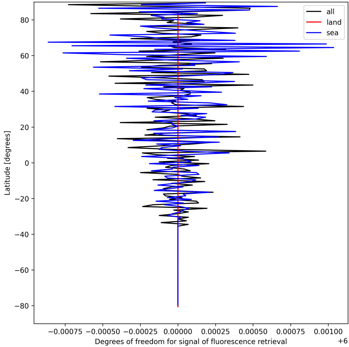
Figure 26: Zonal average of “Degrees of freedom for signal of fluorescence retrieval” for 2025-04-08 to 2025-04-09.
