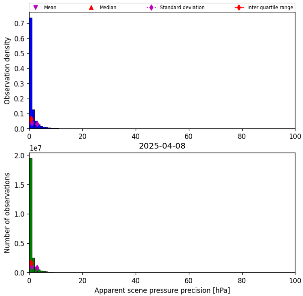
Figure 37: Histogram of “Apparent scene pressure precision” for 2025-04-08 to 2025-04-09
