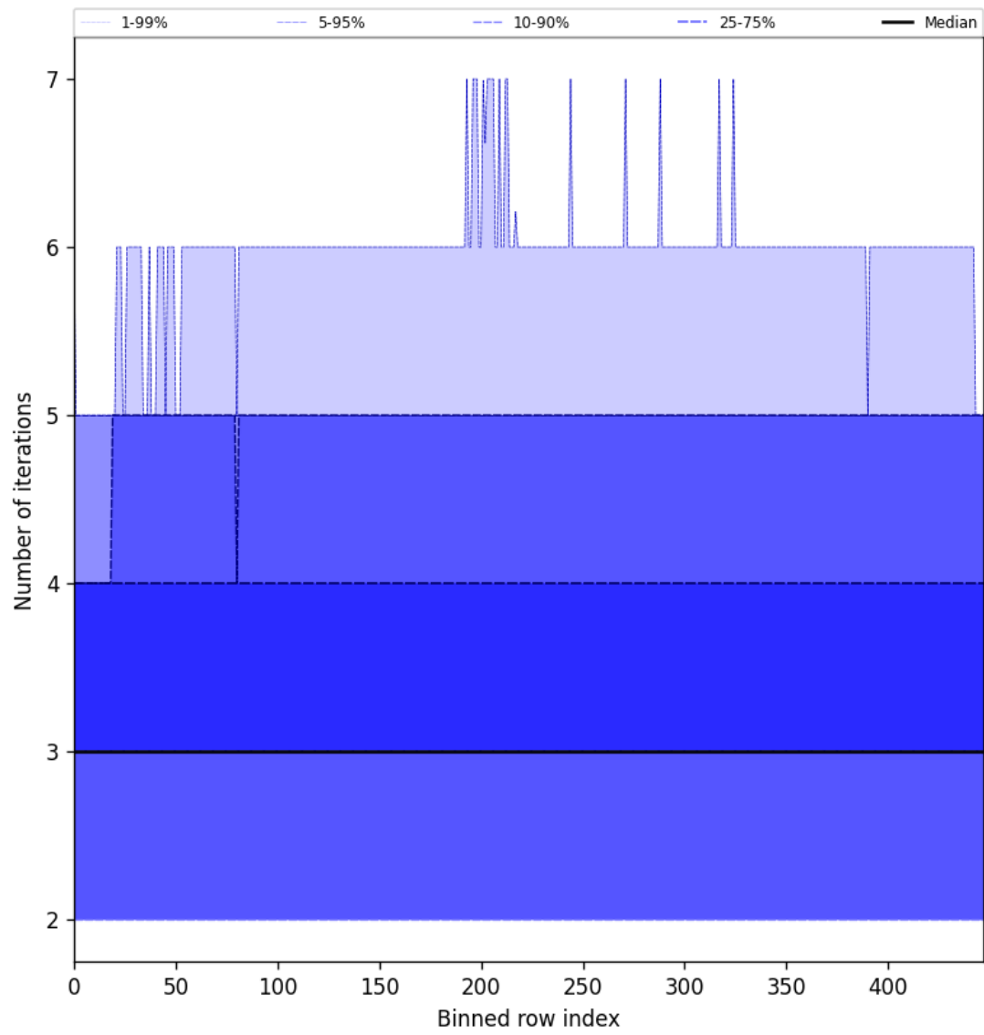
Figure 56: Along track statistics of “Number of iterations” for 2025-04-08 to 2025-04-09
