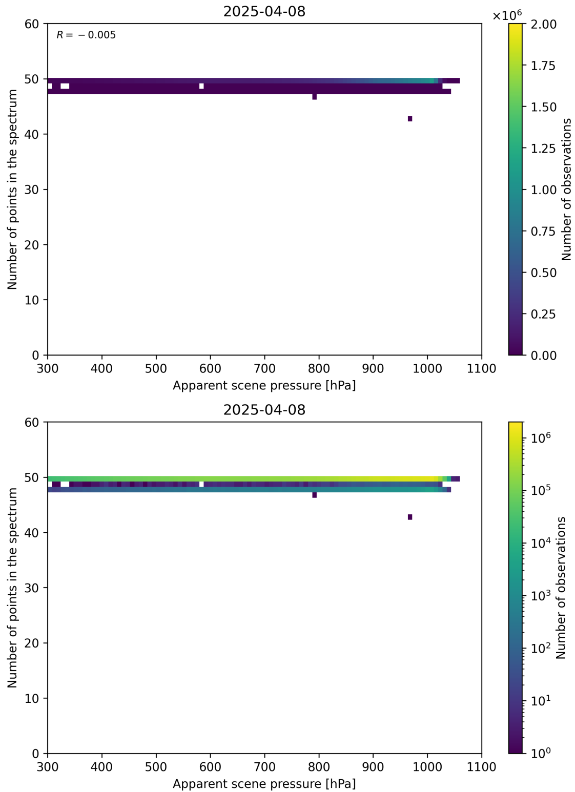
Figure 66: Scatter density plot of “Apparent scene pressure” against “Number of points in the spectrum” for 2025-04-08 to 2025-04-09.
