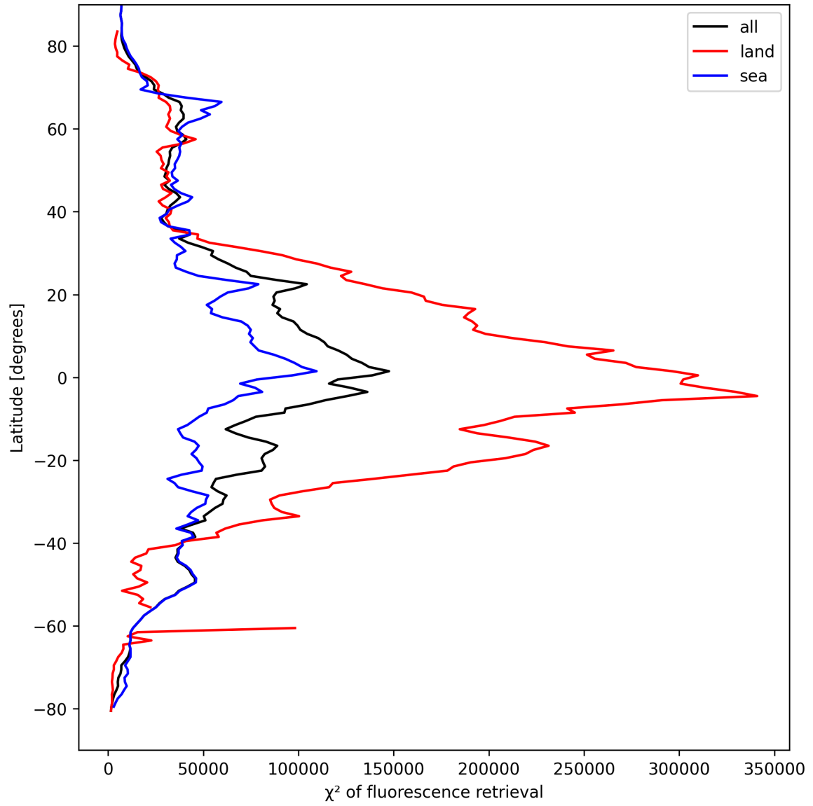
Figure 25: Zonal average of “ \chi^2 of fluorescence retrieval” for 2025-04-08 to 2025-04-09.
