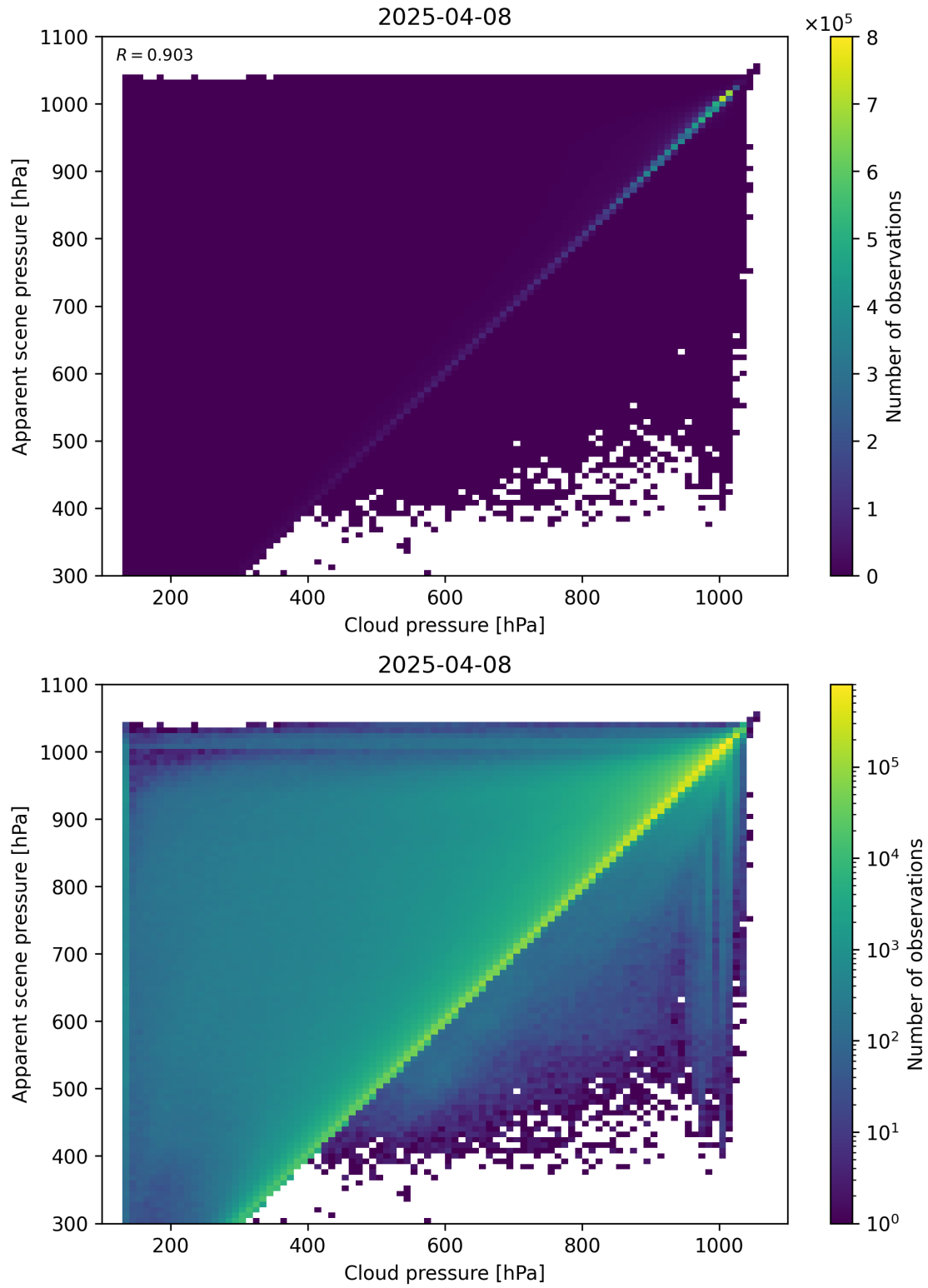
Figure 77: Scatter density plot of “Cloud pressure” against “Apparent scene pressure” for 2025-04-08 to 2025-04-09.
