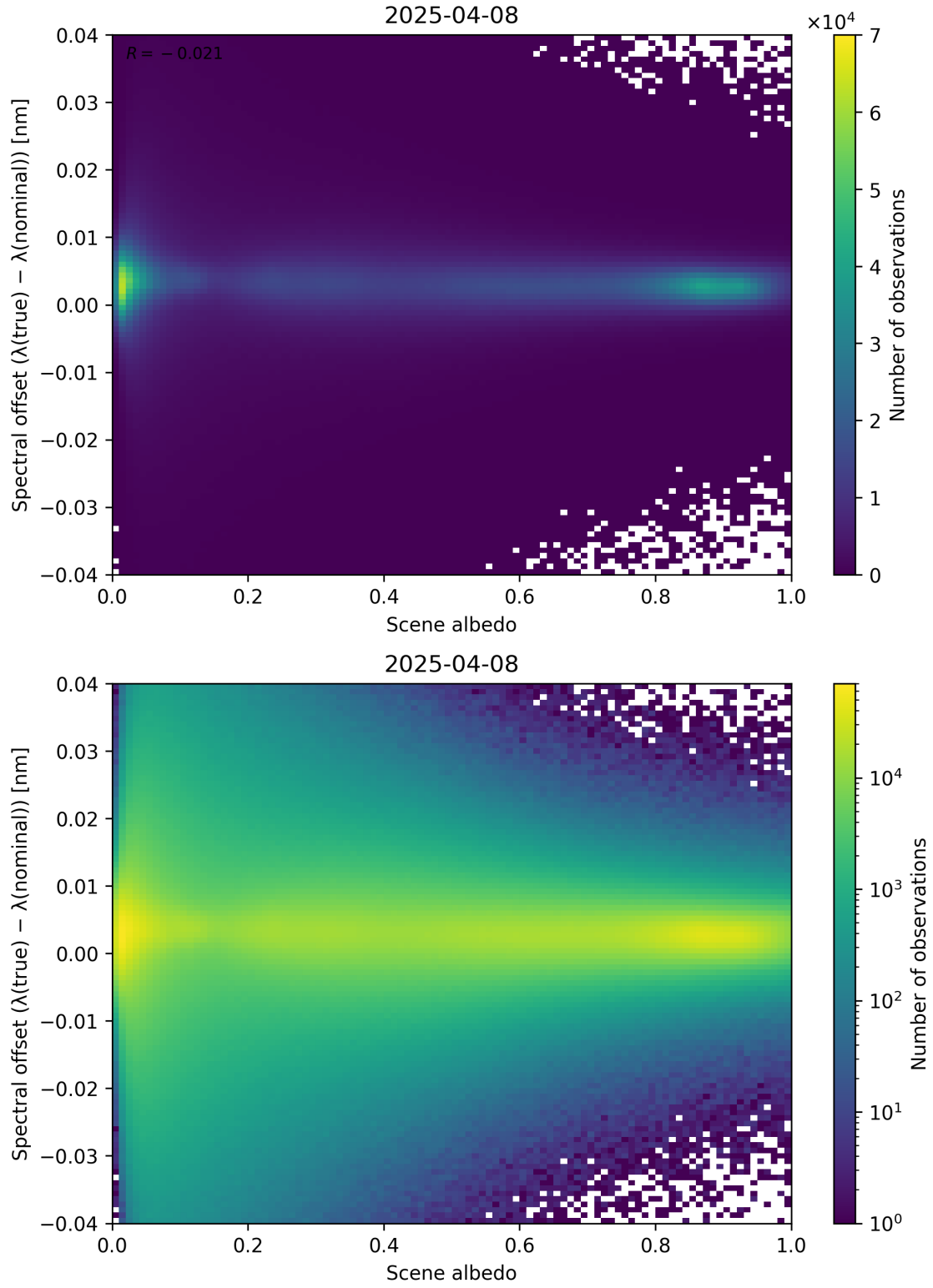
Figure 107: Scatter density plot of “Scene albedo” against “Spectral offset ( \lambda_{\text{true}} - \lambda_{\text{nominal}} )” for 2025-04-08 to 2025-04-09.
