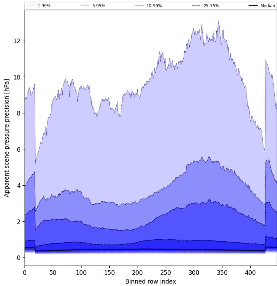
Figure 54: Along track statistics of “Apparent scene pressure precision” for 2025-04-08 to 2025-04-09
