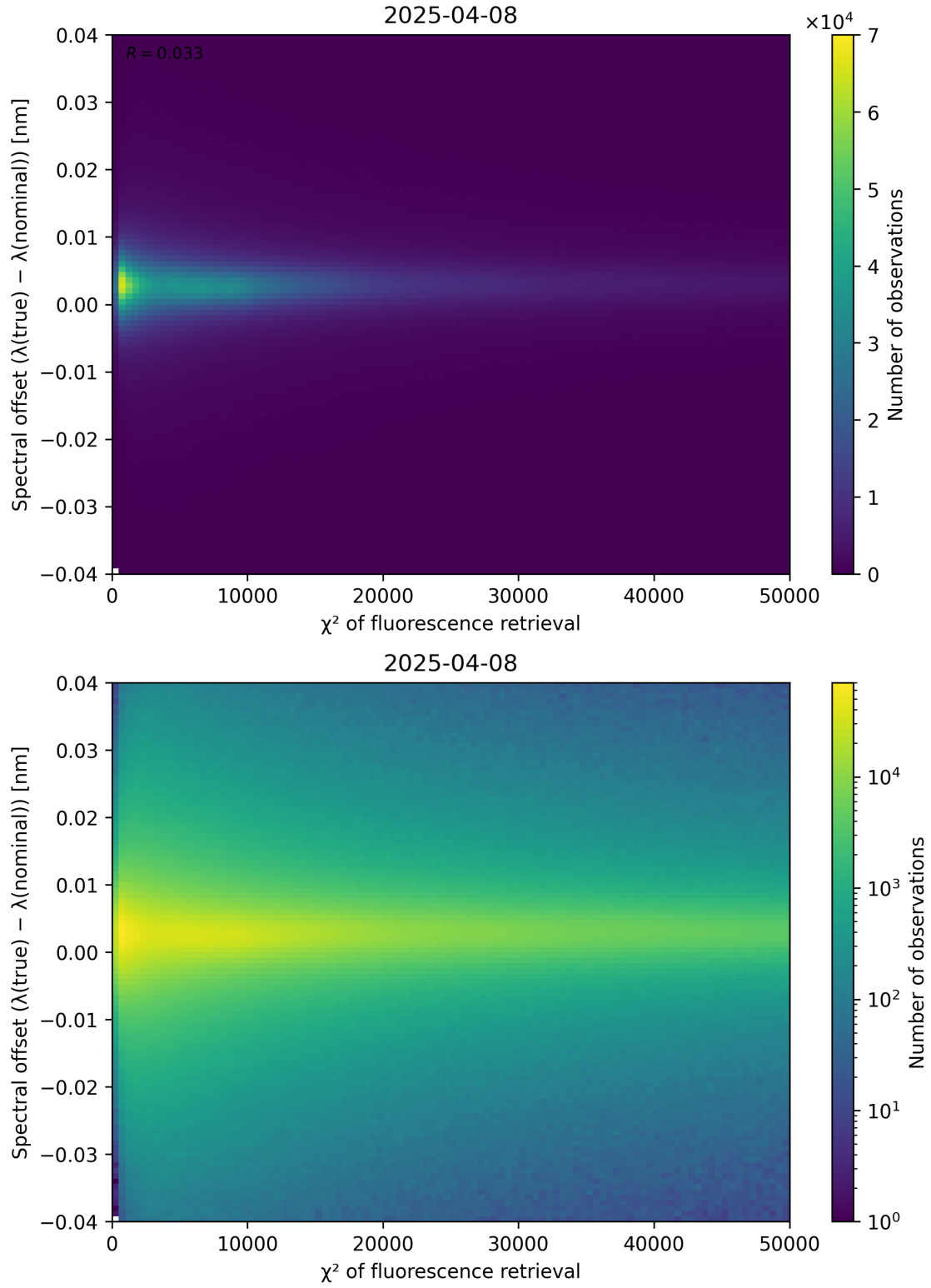
Figure 69: Scatter density plot of “ \chi^2 of fluorescence retrieval” against “Spectral offset ( \lambda_{\text{true}} - \lambda_{\text{nominal}} )” for 2025-04-08 to 2025-04-09.
