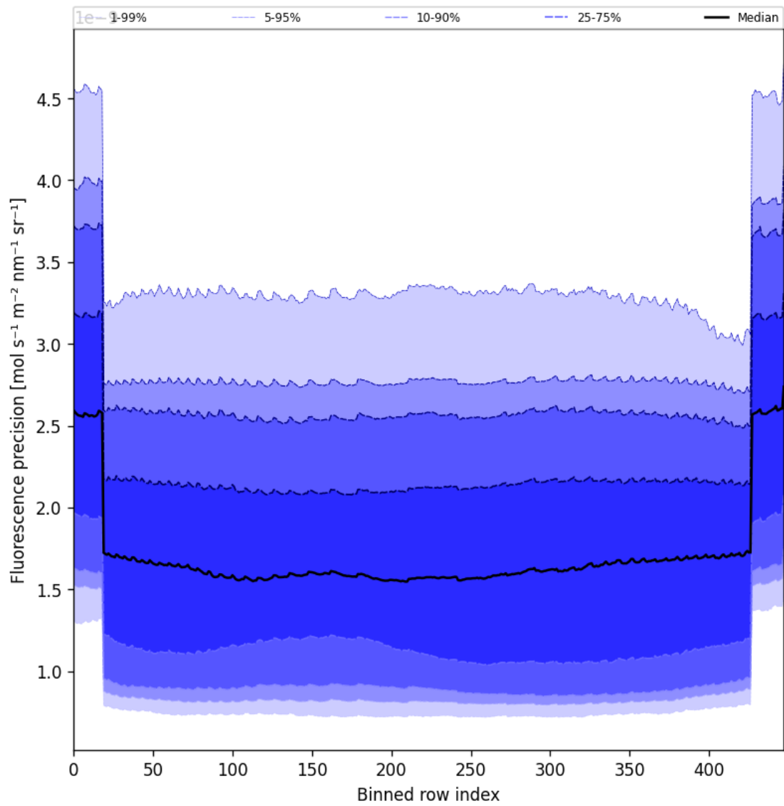
Figure 58: Along track statistics of “Fluorescence precision” for 2025-04-08 to 2025-04-09
