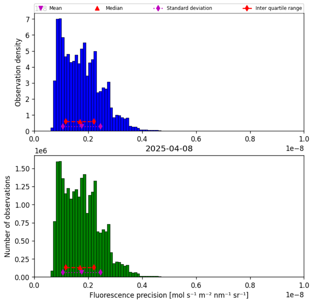
Figure 41: Histogram of “Fluorescence precision” for 2025-04-08 to 2025-04-09
