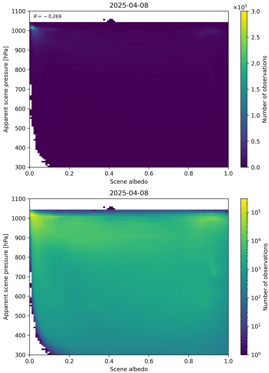
Figure 102: Scatter density plot of “Scene albedo” against “Apparent scene pressure” for 2025-04-08 to 2025-04-09.
