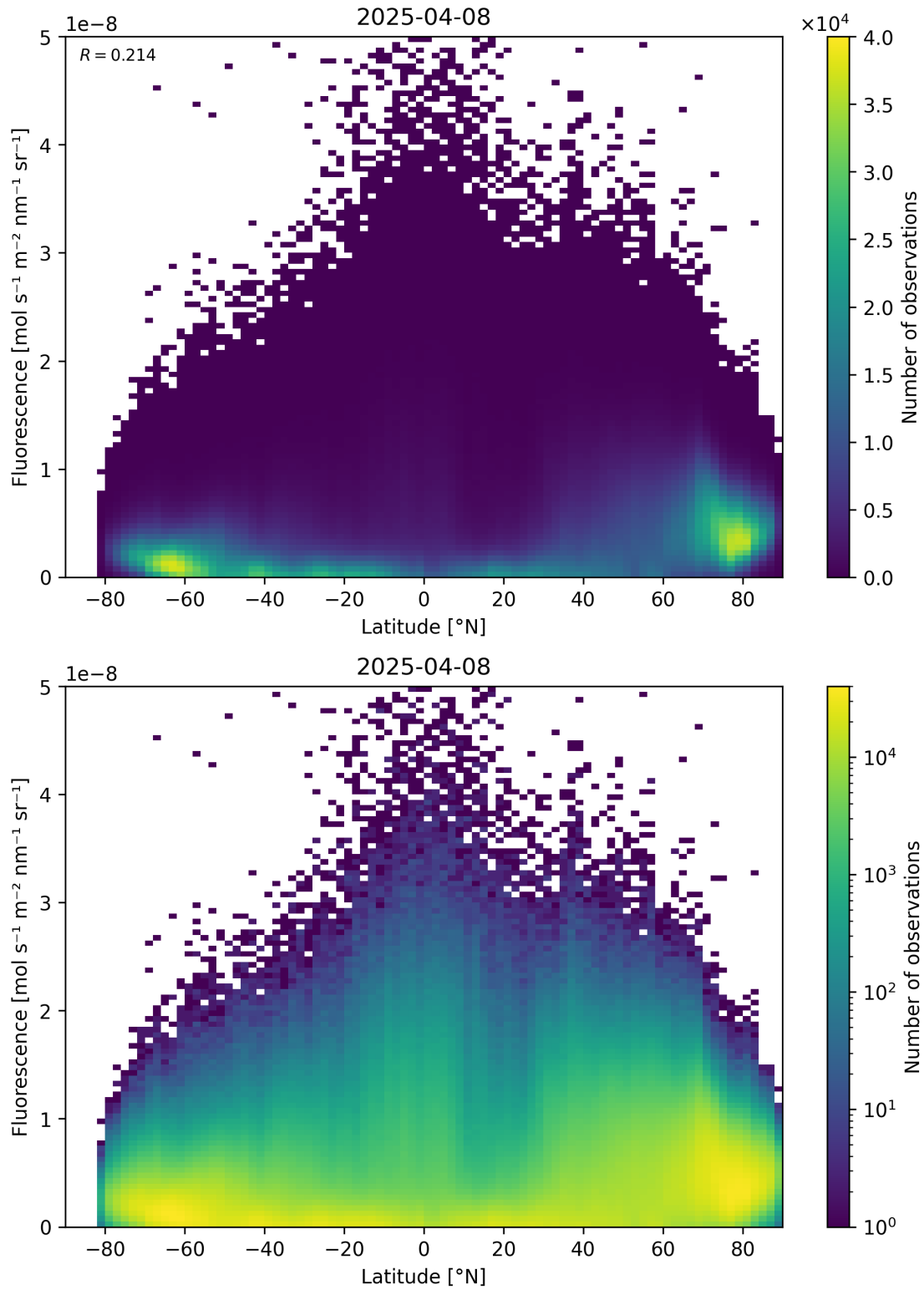
Figure 92: Scatter density plot of “Latitude” against “Fluorescence” for 2025-04-08 to 2025-04-09.
