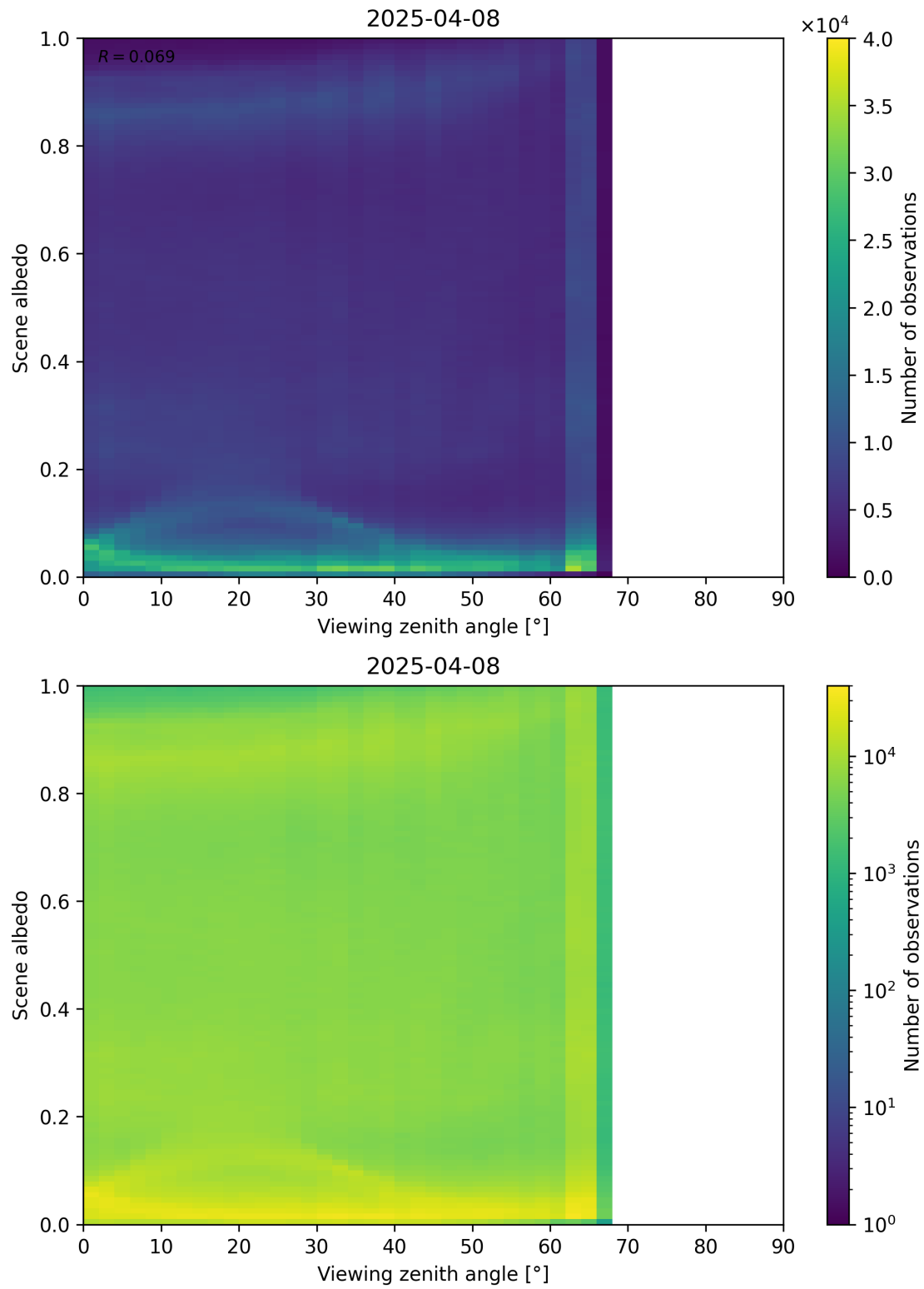
Figure 126: Scatter density plot of “Viewing zenith angle” against “Scene albedo” for 2025-04-08 to 2025-04-09.
