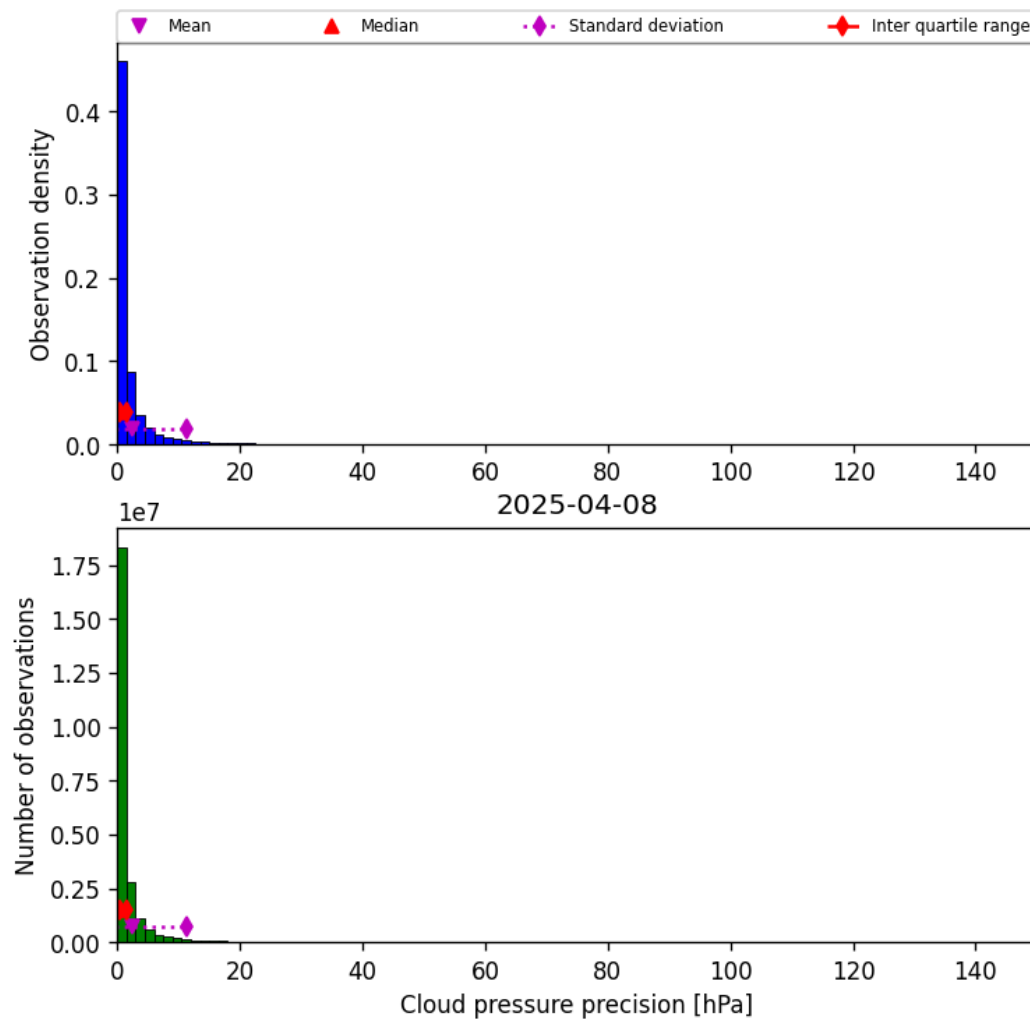
Figure 31: Histogram of “Cloud pressure precision” for 2025-04-08 to 2025-04-09
