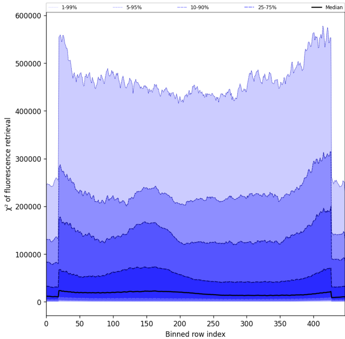
Figure 59: Along track statistics of “ \chi^2 of fluorescence retrieval” for 2025-04-08 to 2025-04-09
