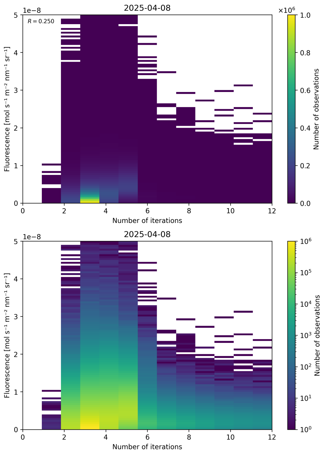
Figure 98: Scatter density plot of “Number of iterations” against “Fluorescence” for 2025-04-08 to 2025-04-09.
