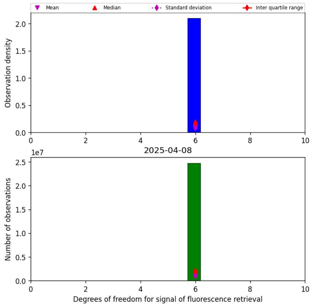
Figure 43: Histogram of “Degrees of freedom for signal of fluorescence retrieval” for 2025-04-08 to 2025-04-09
