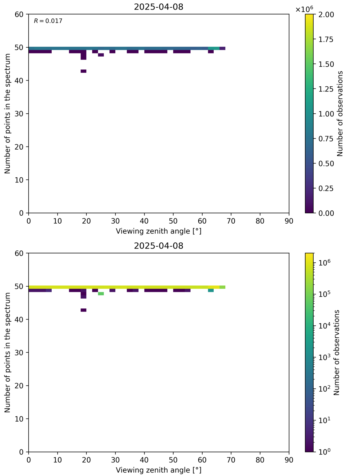
Figure 125: Scatter density plot of “Viewing zenith angle” against “Number of points in the spectrum” for 2025-04-08 to 2025-04-09.
