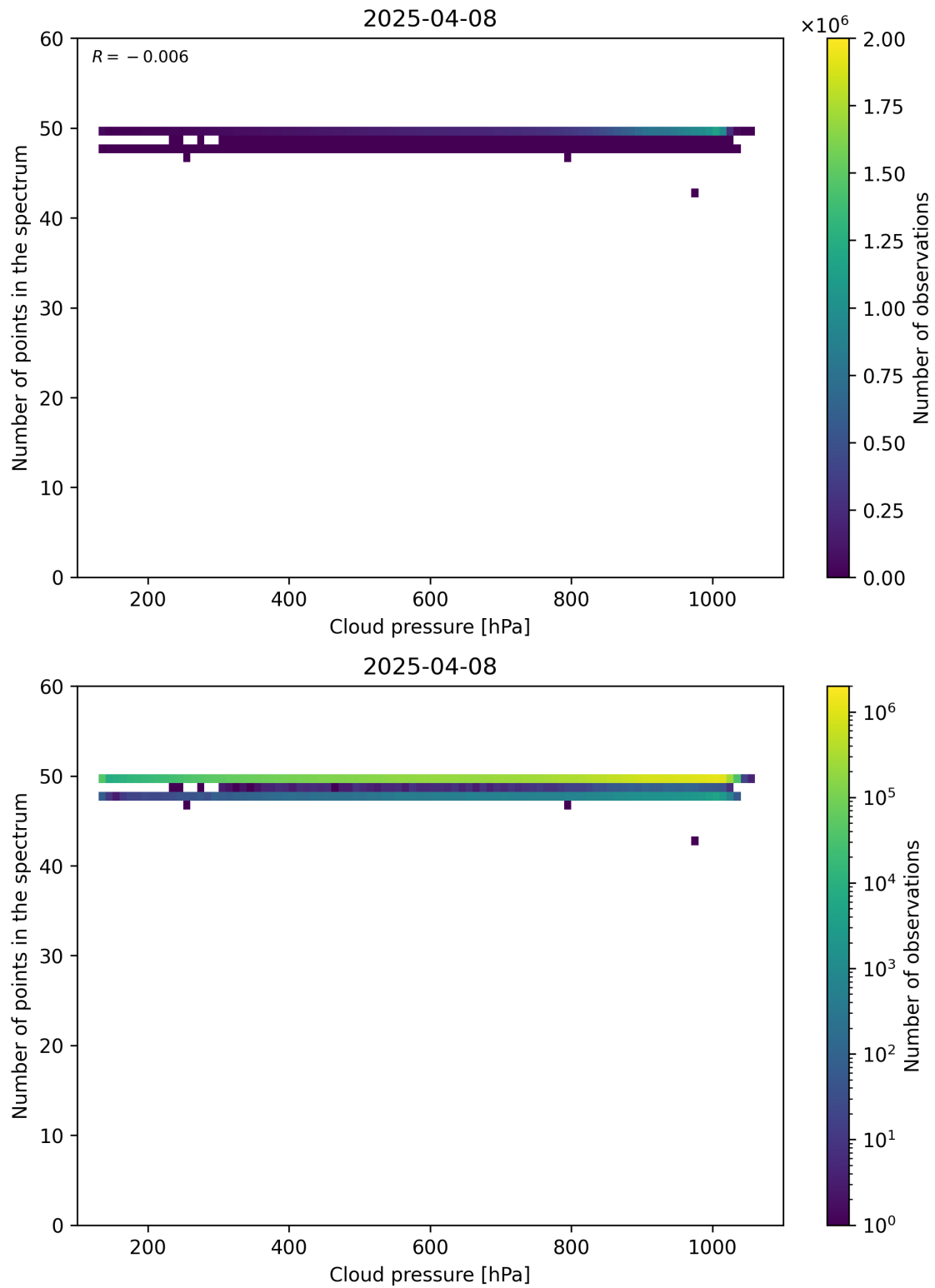
Figure 82: Scatter density plot of “Cloud pressure” against “Number of points in the spectrum” for 2025-04-08 to 2025-04-09.
