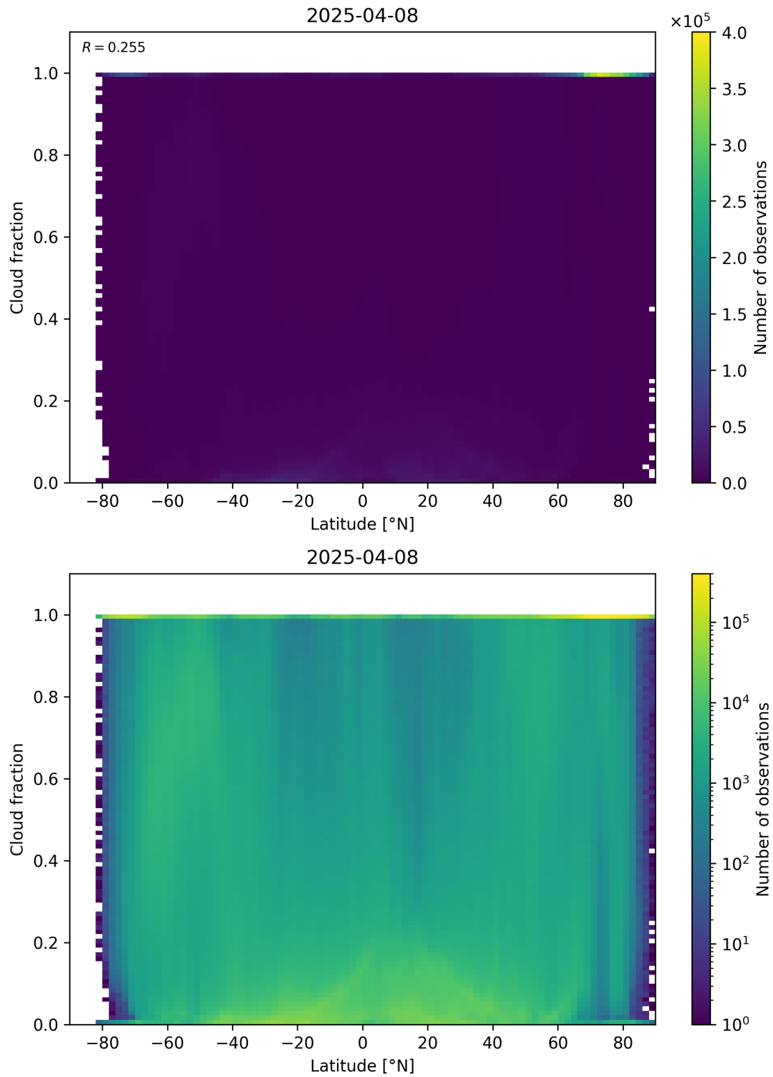
Figure 90: Scatter density plot of “Latitude” against “Cloud fraction” for 2025-04-08 to 2025-04-09.
