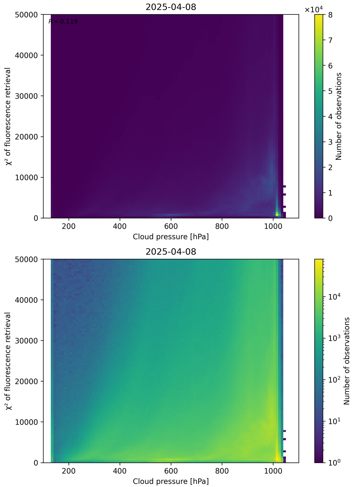
Figure 78: Scatter density plot of “Cloud pressure” against “ \chi^2 of fluorescence retrieval” for 2025-04-08 to 2025-04-09.
