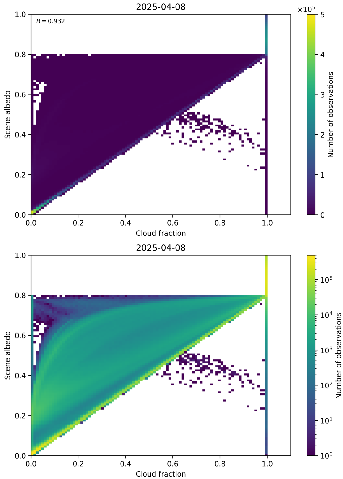
Figure 75: Scatter density plot of “Cloud fraction” against “Scene albedo” for 2025-04-08 to 2025-04-09.
