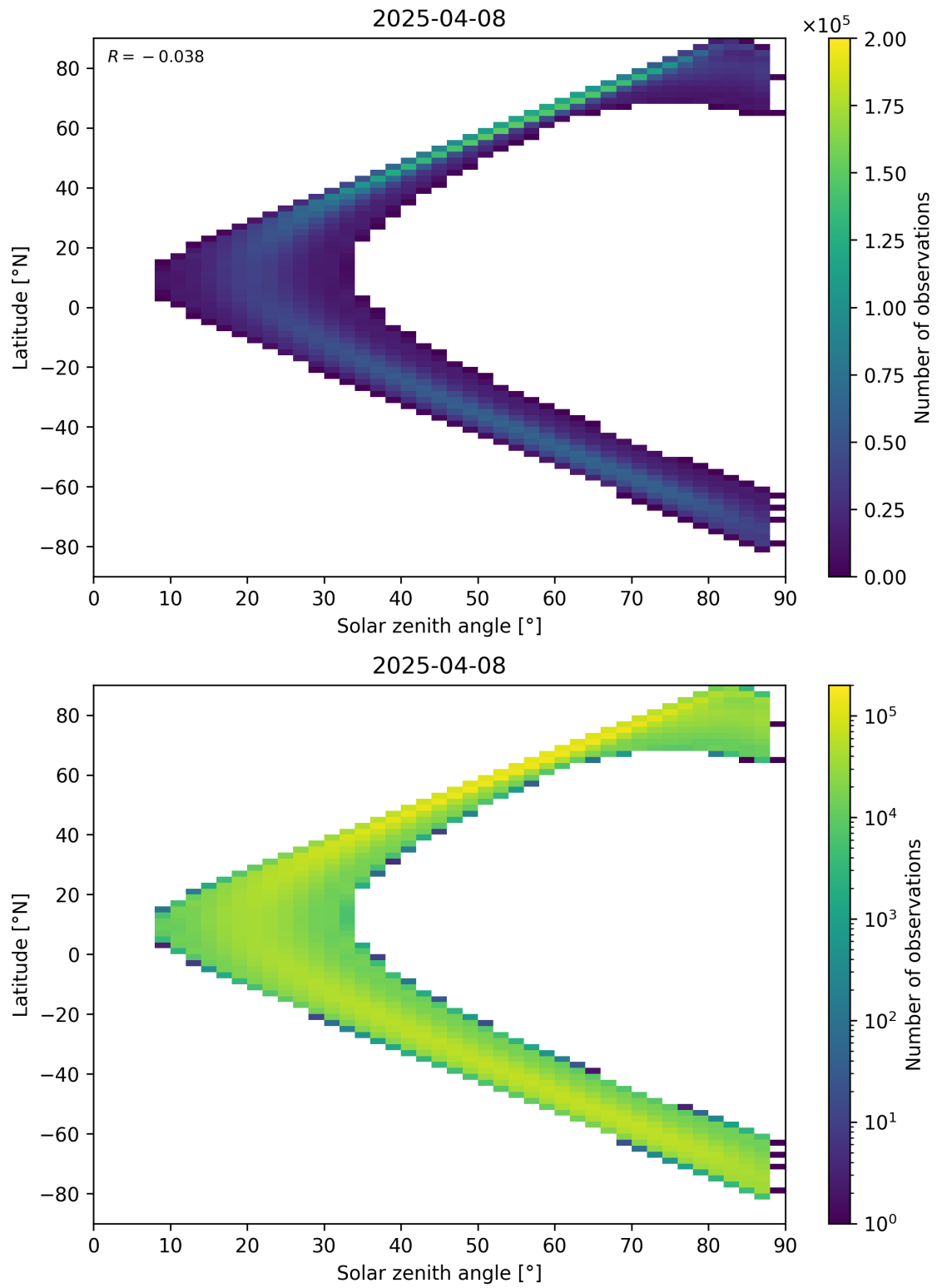
Figure 113: Scatter density plot of “Solar zenith angle” against “Latitude” for 2025-04-08 to 2025-04-09.
