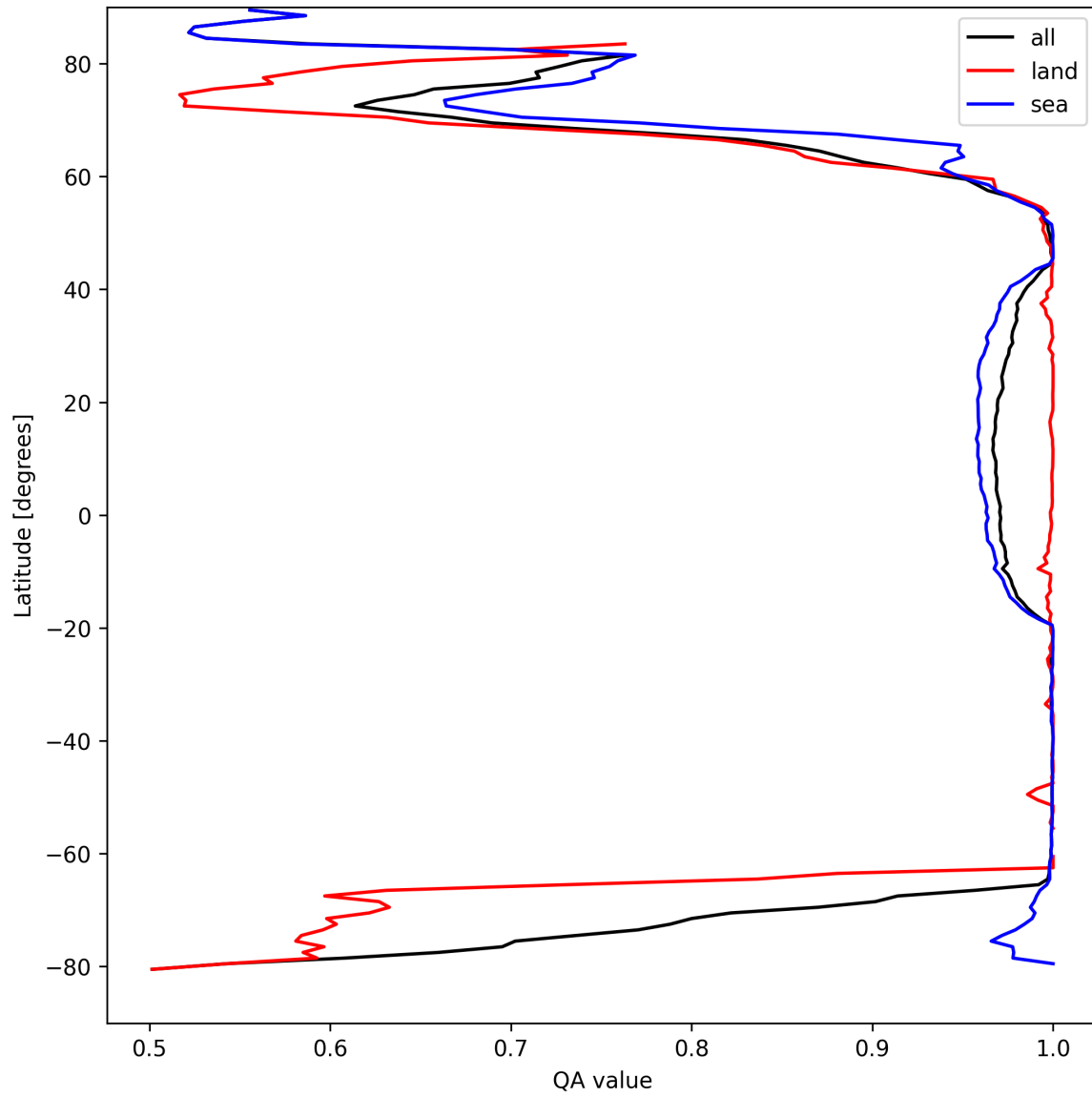
Figure 12: Zonal average of “QA value” for 2025-04-08 to 2025-04-09.
