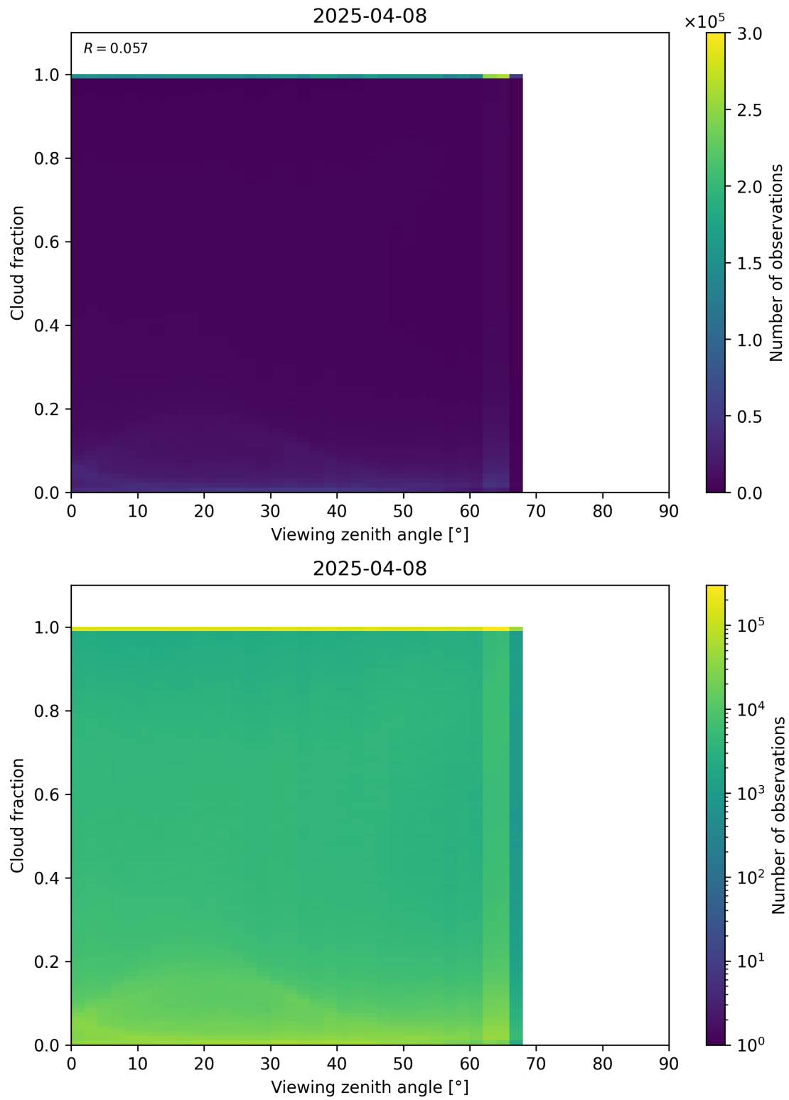
Figure 120: Scatter density plot of “Viewing zenith angle” against “Cloud fraction” for 2025-04-08 to 2025-04-09.
