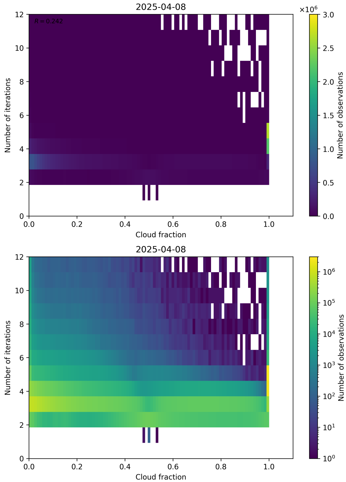
Figure 73: Scatter density plot of “Cloud fraction” against “Number of iterations” for 2025-04-08 to 2025-04-09.
