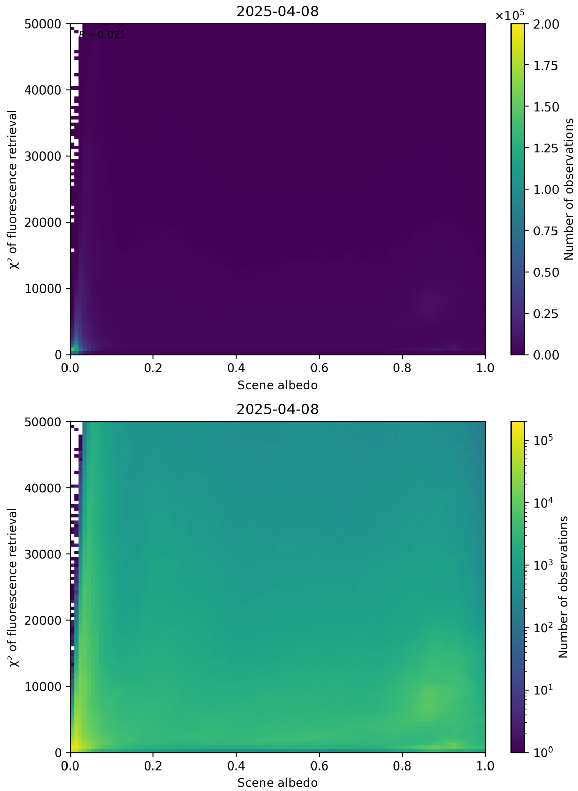
Figure 103: Scatter density plot of “Scene albedo” against “ \chi^2 of fluorescence retrieval” for 2025-04-08 to 2025-04-09.
