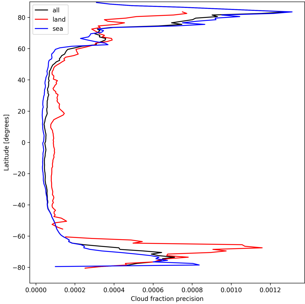
Figure 16: Zonal average of “Cloud fraction precision” for 2025-04-08 to 2025-04-09.
