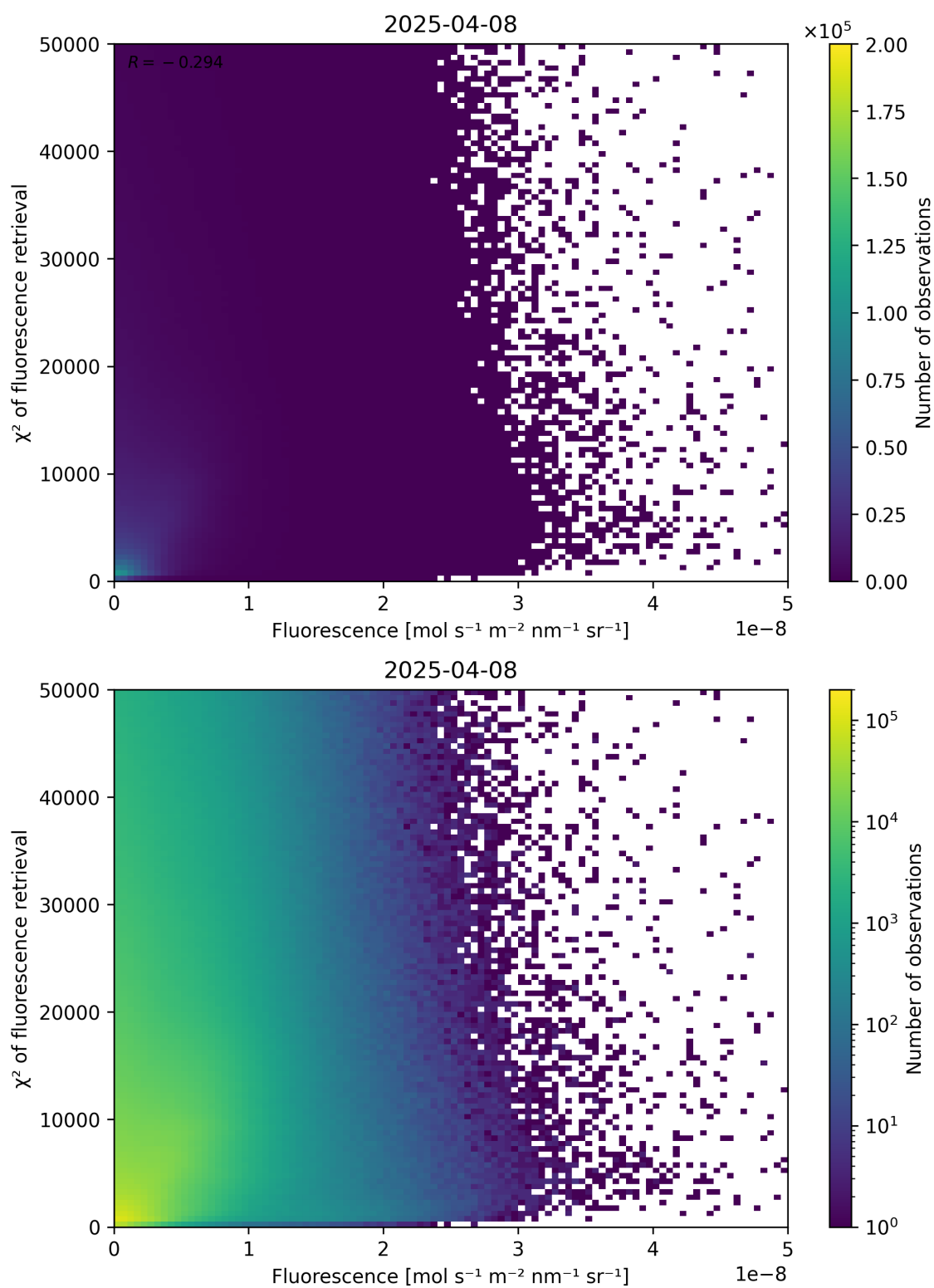
Figure 85: Scatter density plot of “Fluorescence” against “ \chi^2 of fluorescence retrieval” for 2025-04-08 to 2025-04-09.
