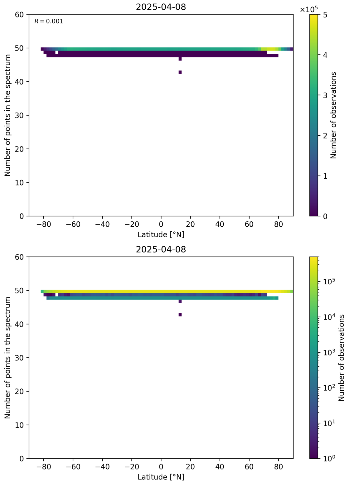
Figure 94: Scatter density plot of “Latitude” against “Number of points in the spectrum” for 2025-04-08 to 2025-04-09.
