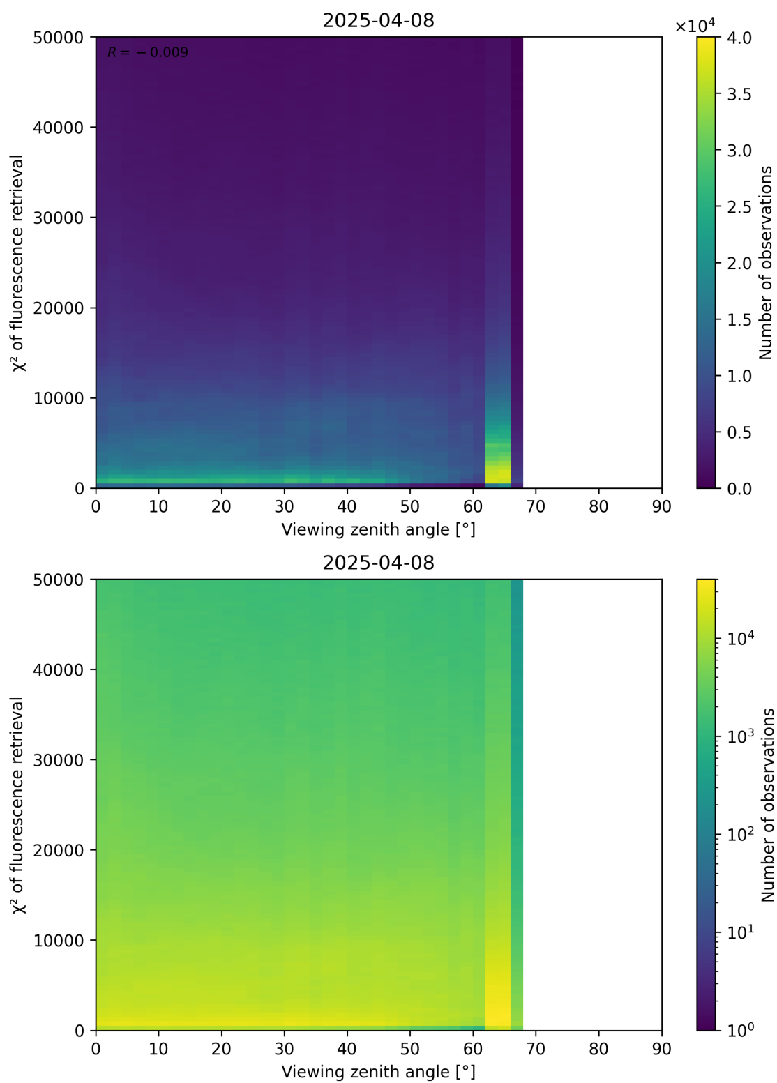
Figure 119: Scatter density plot of “Viewing zenith angle” against “ \chi^2 of fluorescence retrieval” for 2025-04-08 to 2025-04-09.
