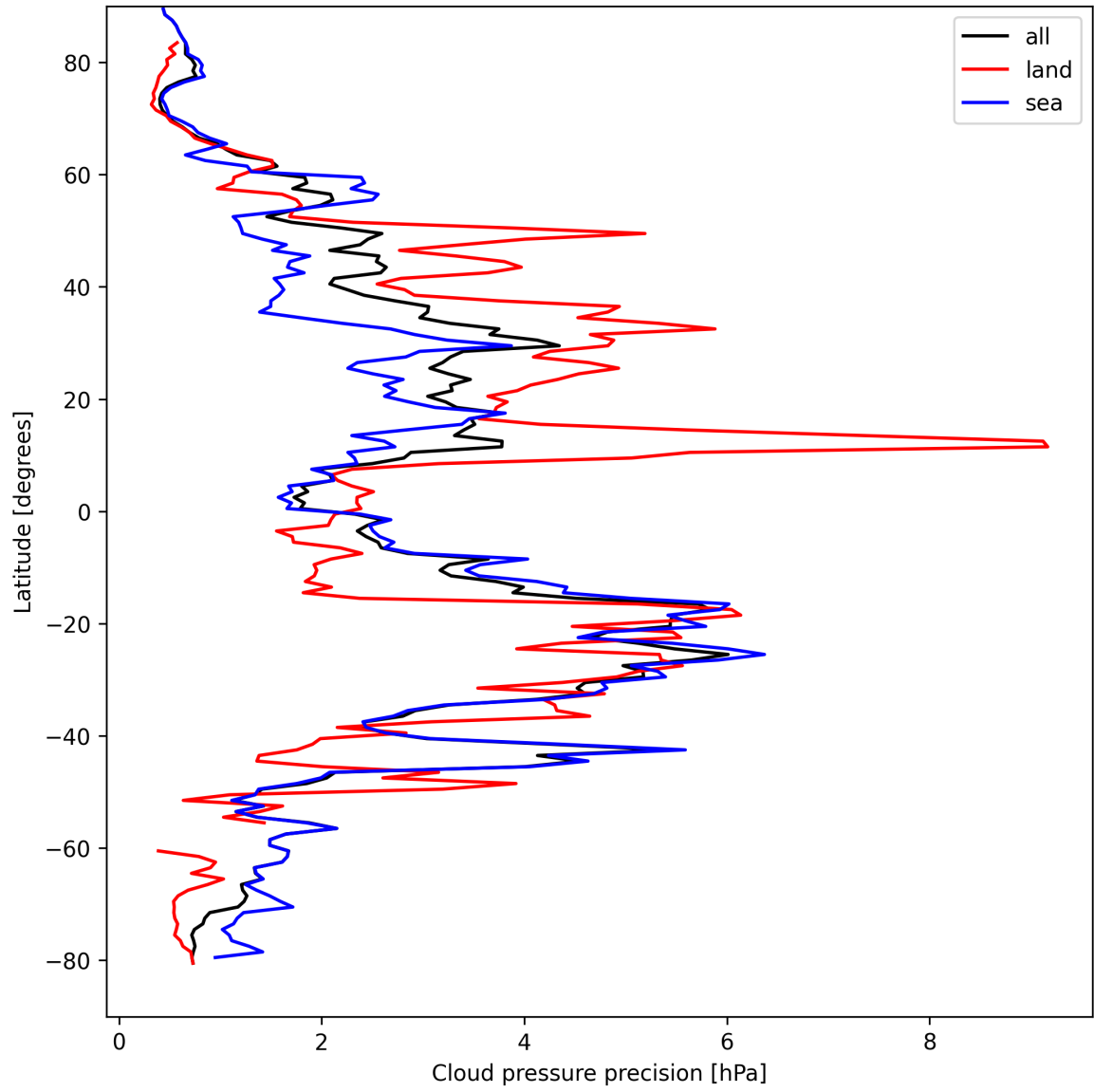
Figure 14: Zonal average of “Cloud pressure precision” for 2025-04-08 to 2025-04-09.
