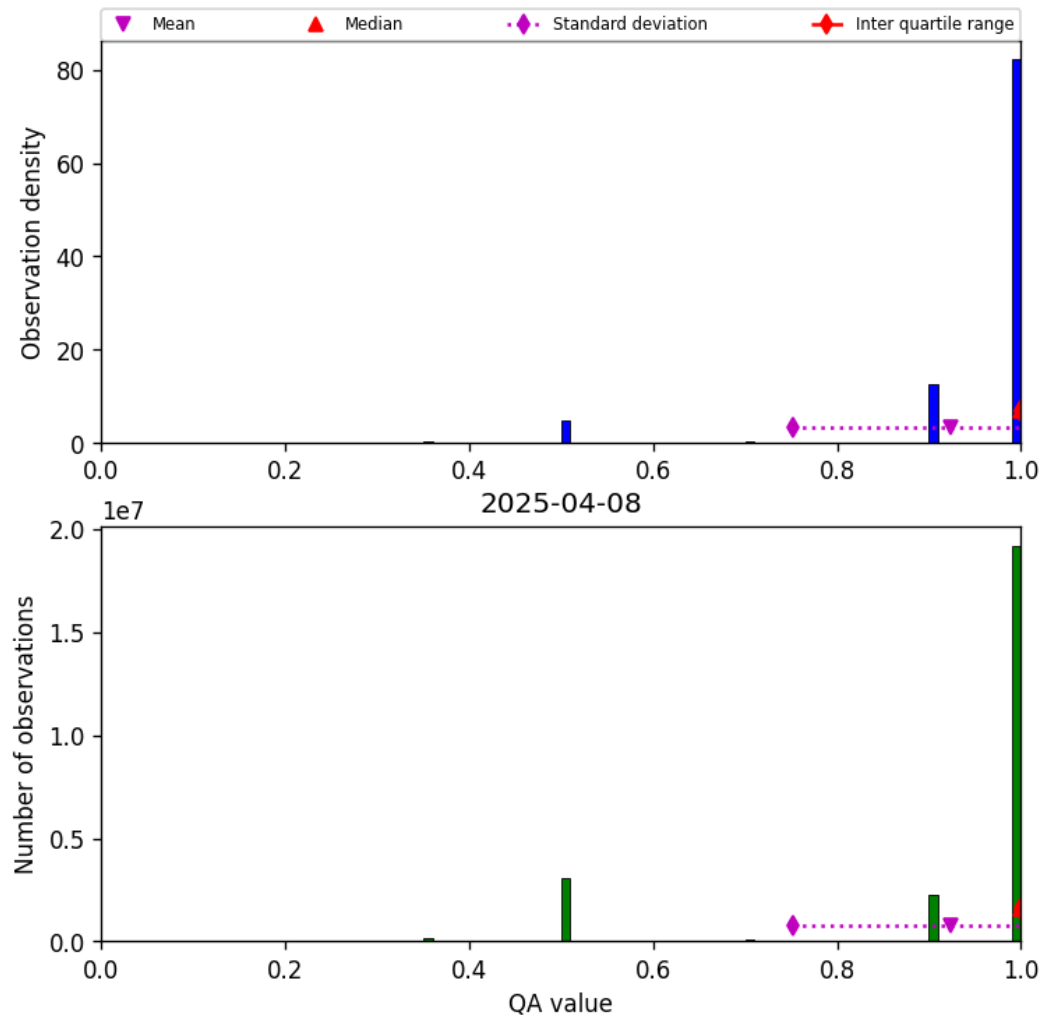
Figure 29: Histogram of “QA value” for 2025-04-08 to 2025-04-09
