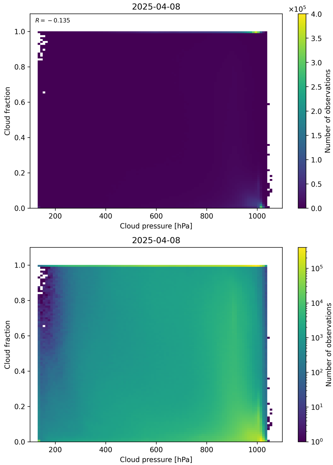
Figure 79: Scatter density plot of “Cloud pressure” against “Cloud fraction” for 2025-04-08 to 2025-04-09.
