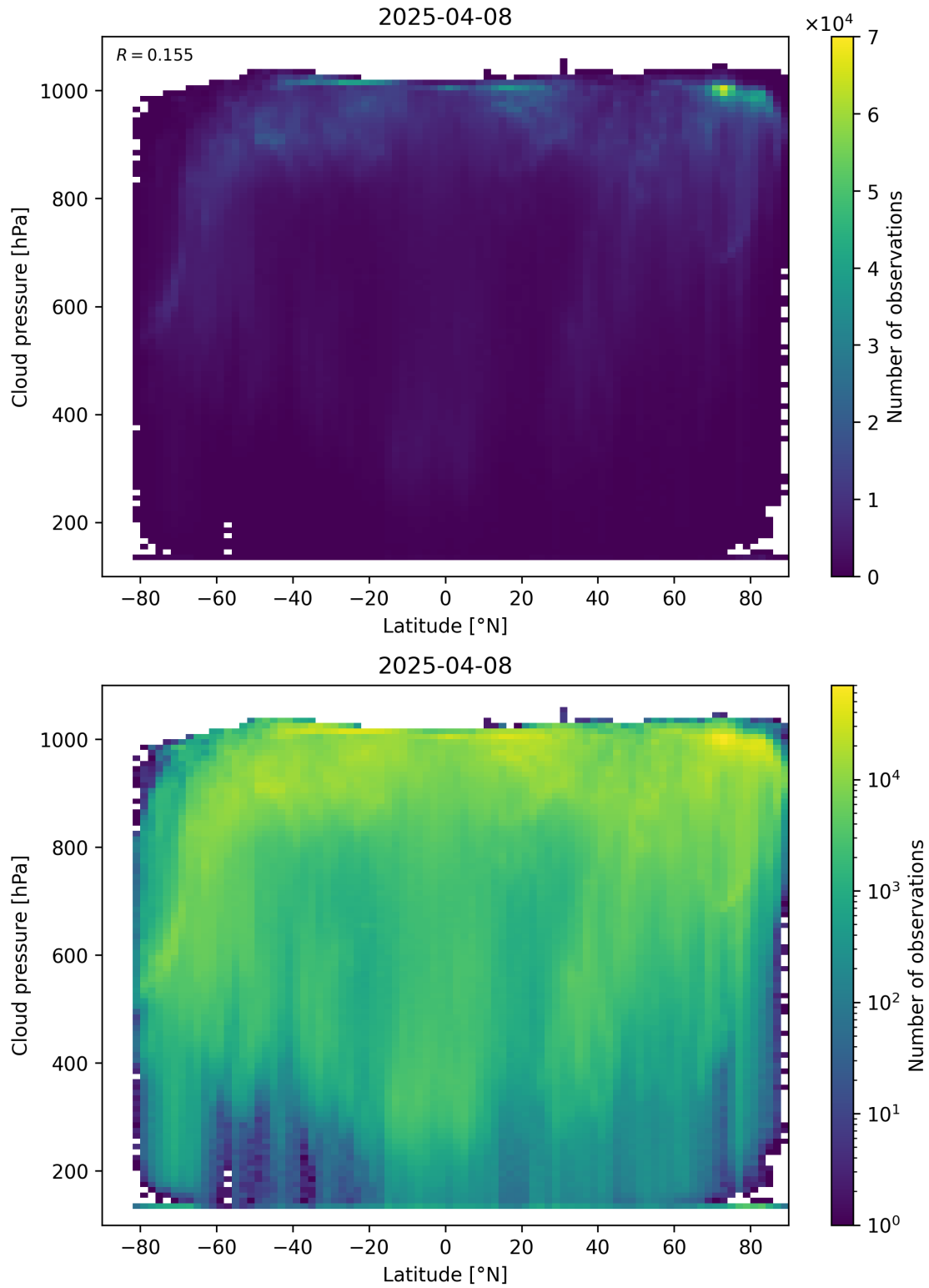
Figure 91: Scatter density plot of “Latitude” against “Cloud pressure” for 2025-04-08 to 2025-04-09.
