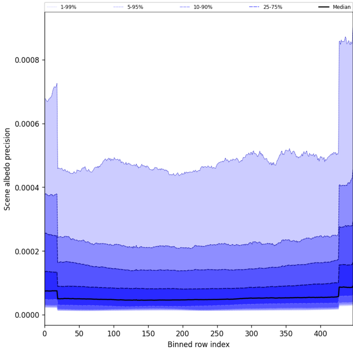
Figure 52: Along track statistics of “Scene albedo precision” for 2025-04-08 to 2025-04-09
