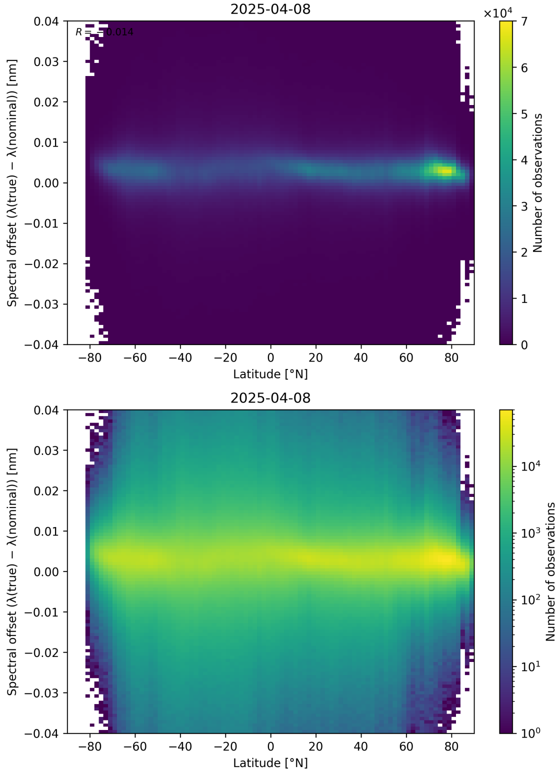
Figure 96: Scatter density plot of “Latitude” against “Spectral offset ( \lambda_{\text{true}} - \lambda_{\text{nominal}} )” for 2025-04-08 to 2025-04-09.
