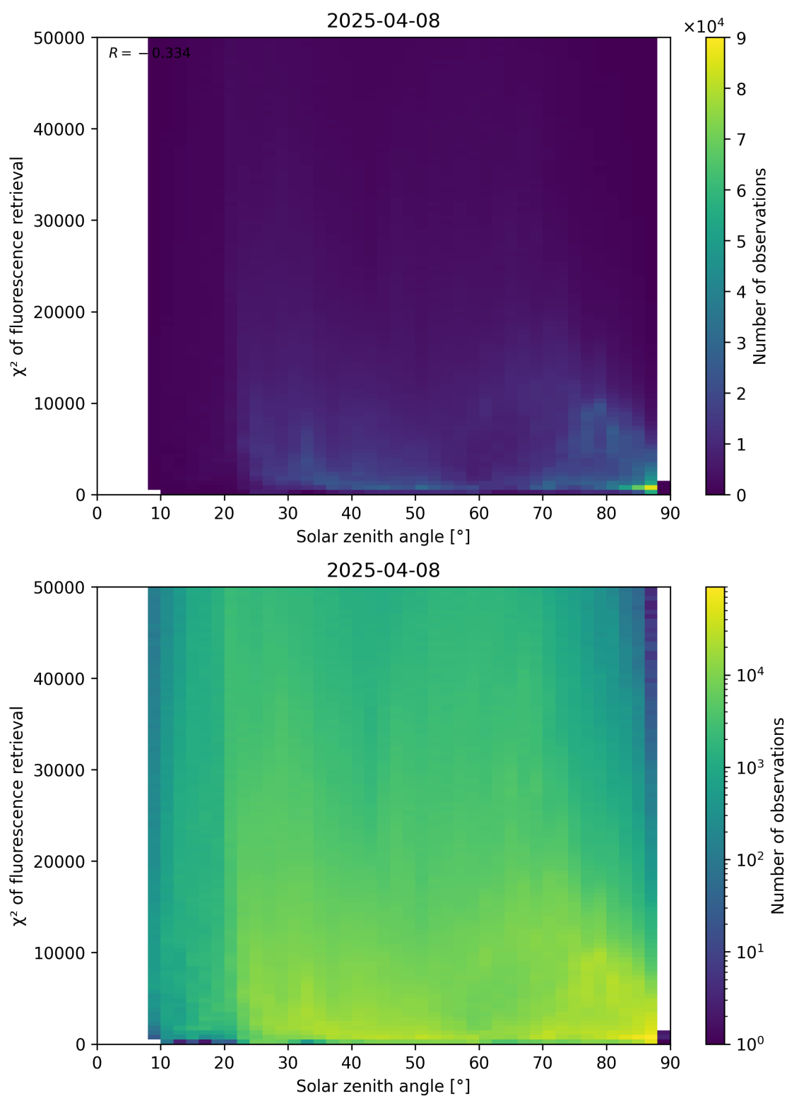
Figure 109: Scatter density plot of “Solar zenith angle” against “ \chi^2 of fluorescence retrieval” for 2025-04-08 to 2025-04-09.
