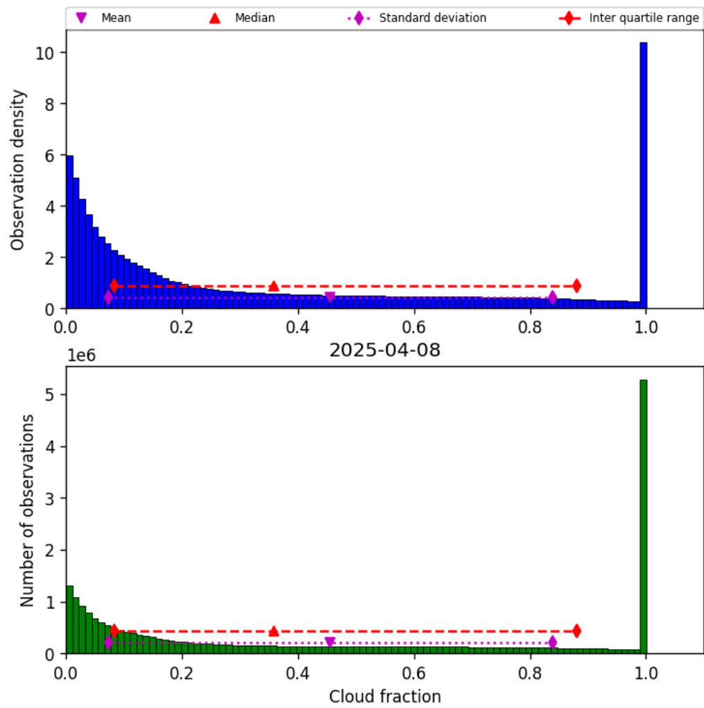
Figure 32: Histogram of “Cloud fraction” for 2025-04-08 to 2025-04-09
