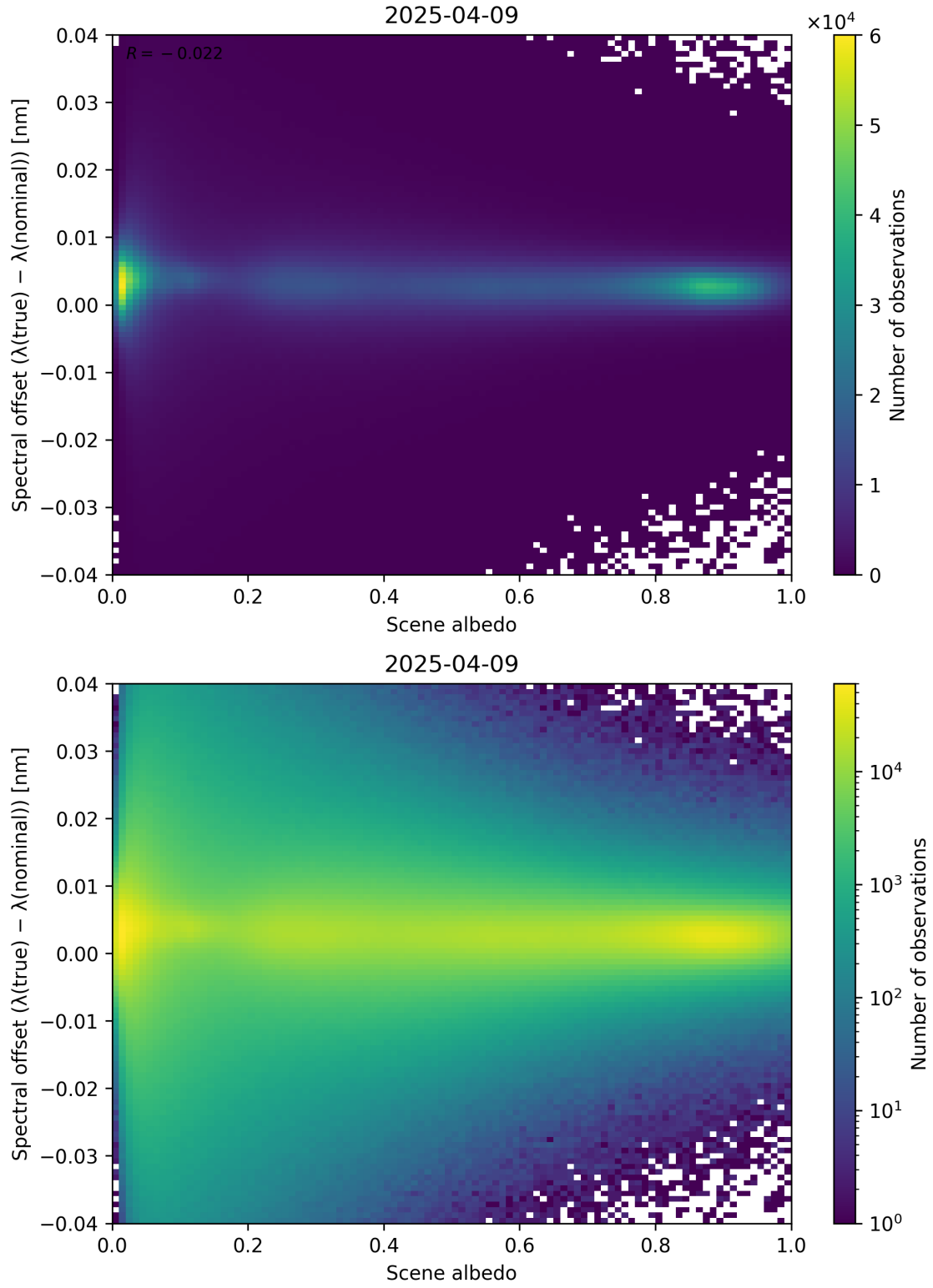
Figure 107: Scatter density plot of “Scene albedo” against “Spectral offset ( \lambda_{\text{true}} - \lambda_{\text{nominal}} )” for 2025-04-08 to 2025-04-10.
