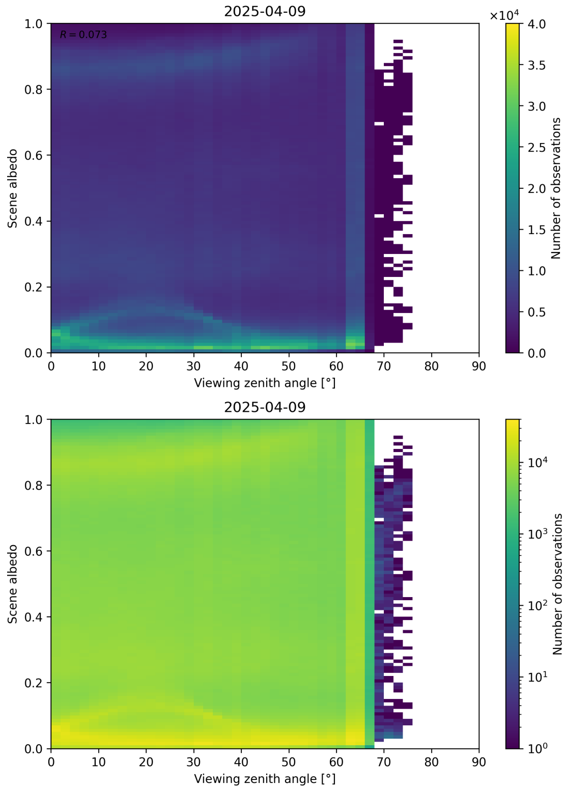
Figure 126: Scatter density plot of “Viewing zenith angle” against “Scene albedo” for 2025-04-08 to 2025-04-10.
