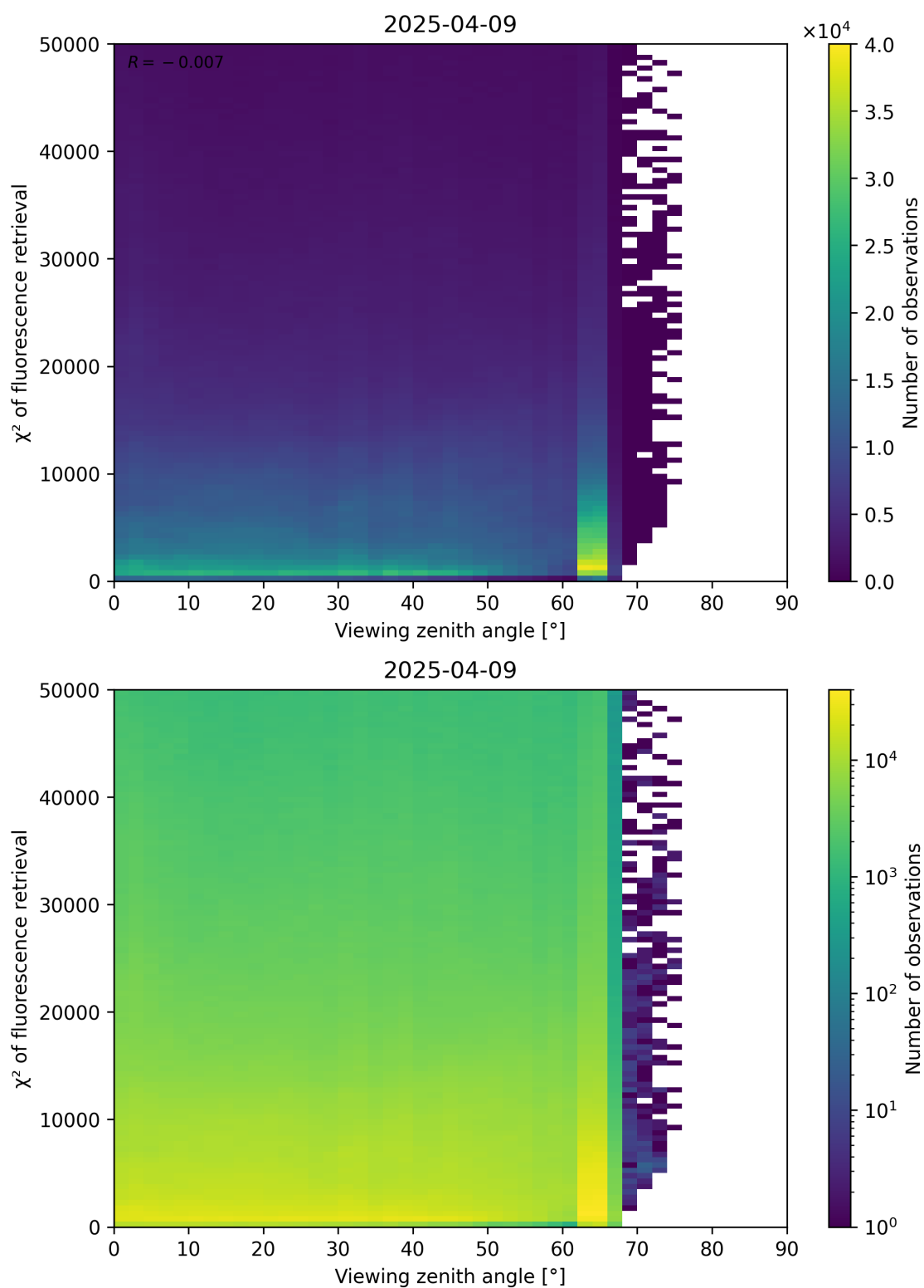
Figure 119: Scatter density plot of “Viewing zenith angle” against “ \chi^2 of fluorescence retrieval” for 2025-04-08 to 2025-04-10.
