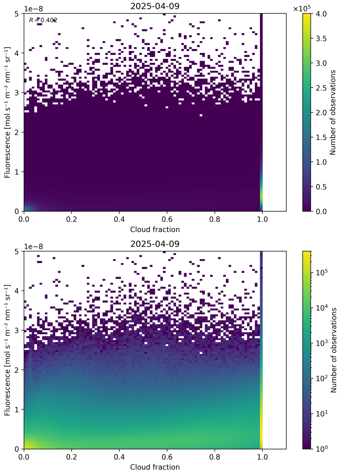
Figure 72: Scatter density plot of “Cloud fraction” against “Fluorescence” for 2025-04-08 to 2025-04-10.
