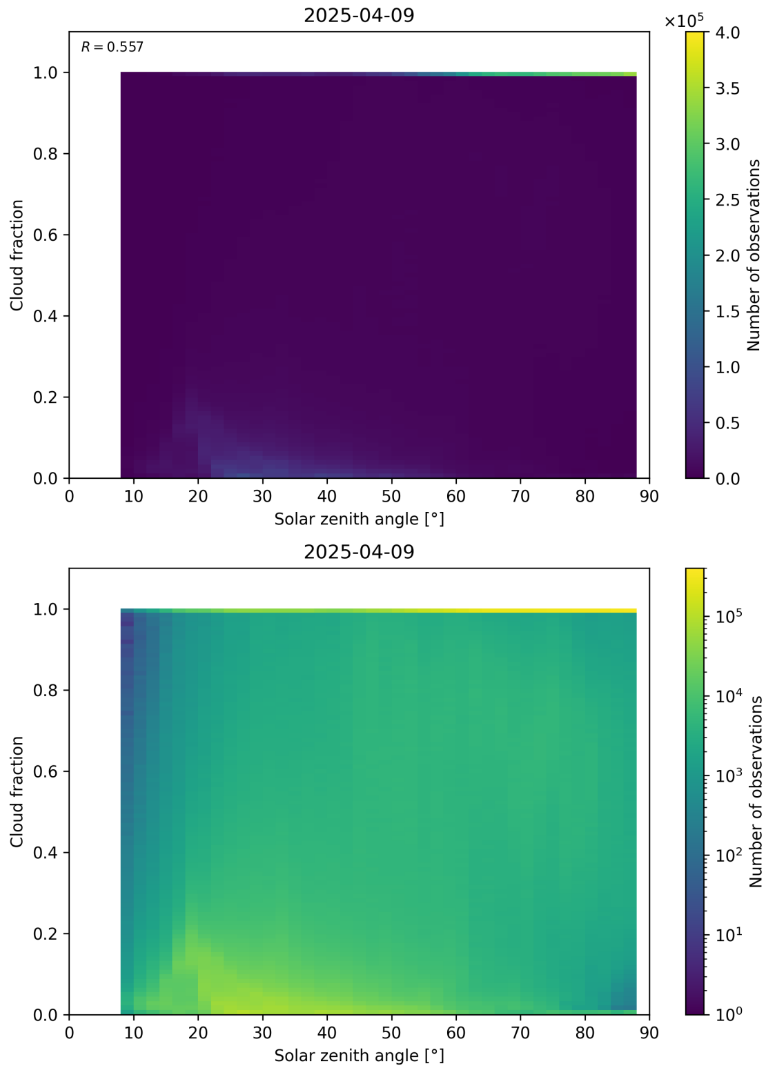
Figure 110: Scatter density plot of “Solar zenith angle” against “Cloud fraction” for 2025-04-08 to 2025-04-10.
