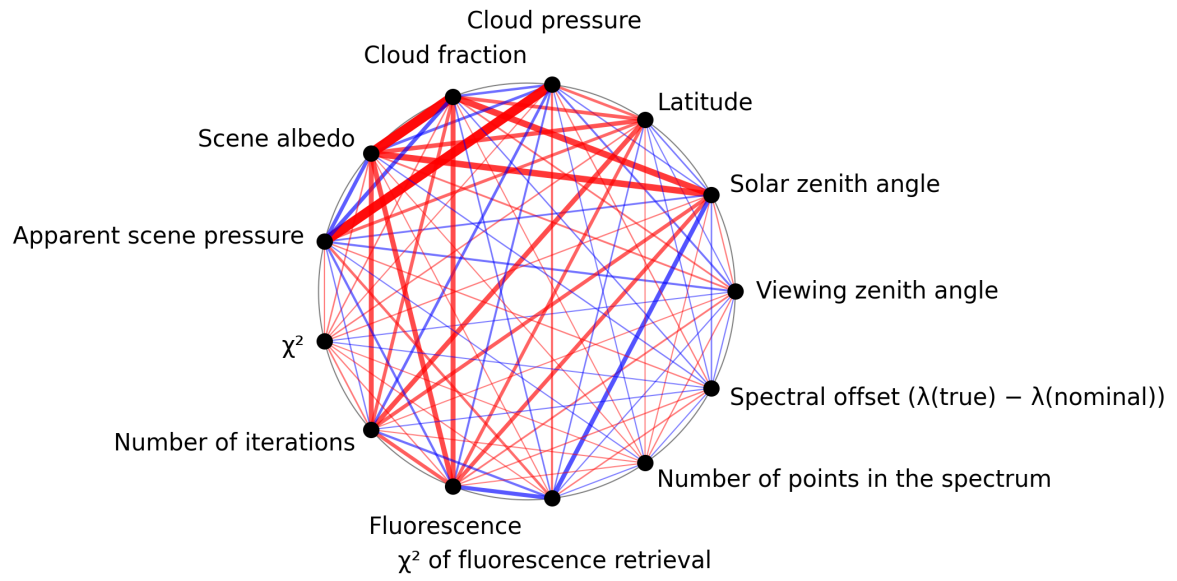
Figure 1: Map of correlation graph for 2025-04-08 to 2025-04-10.
