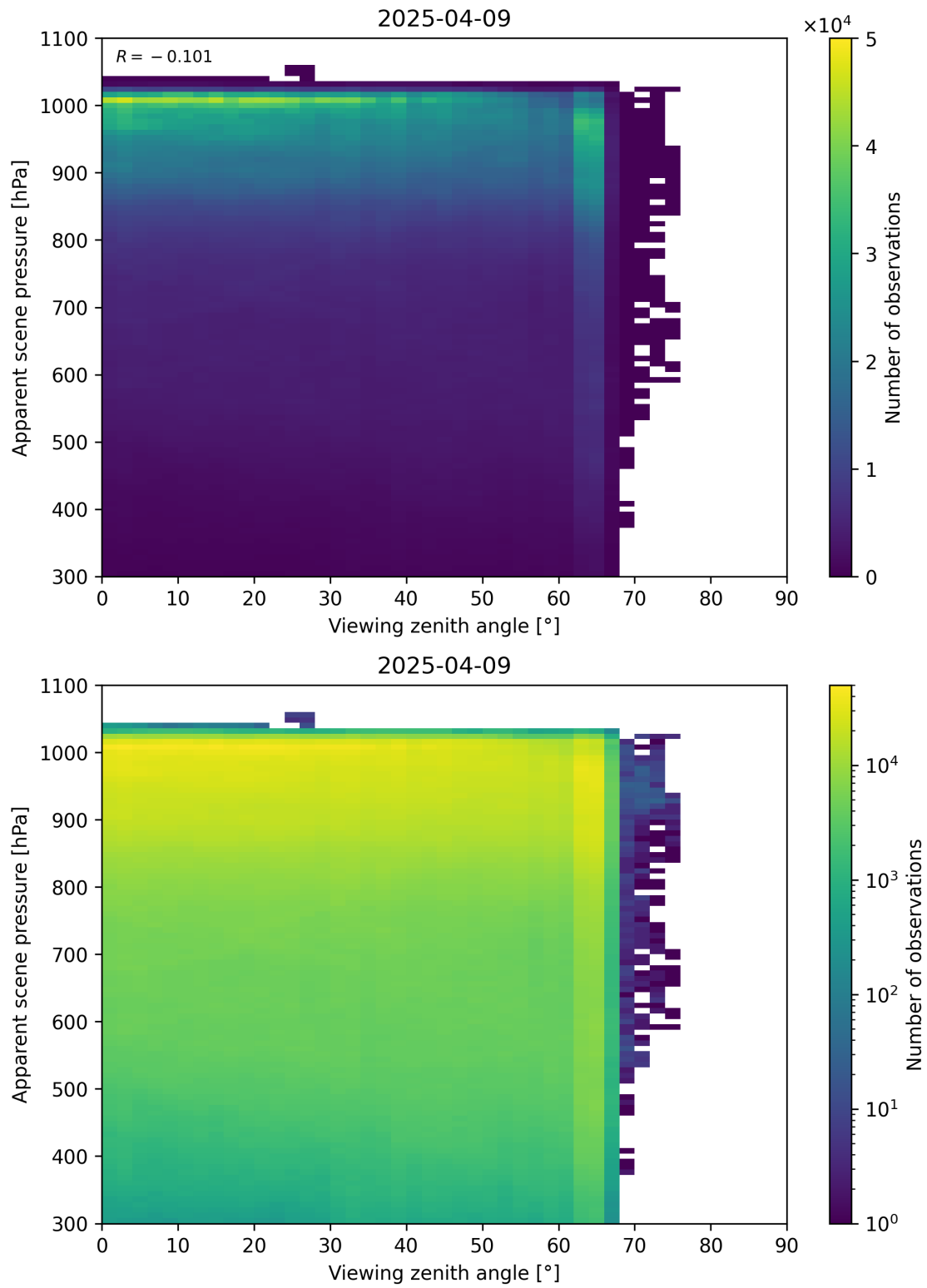
Figure 118: Scatter density plot of “Viewing zenith angle” against “Apparent scene pressure” for 2025-04-08 to 2025-04-10.
