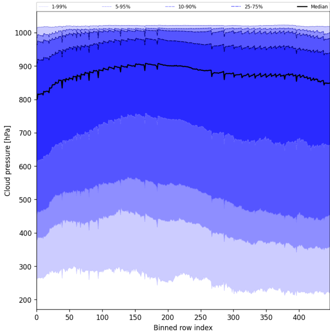
Figure 47: Along track statistics of “Cloud pressure” for 2025-04-08 to 2025-04-10
