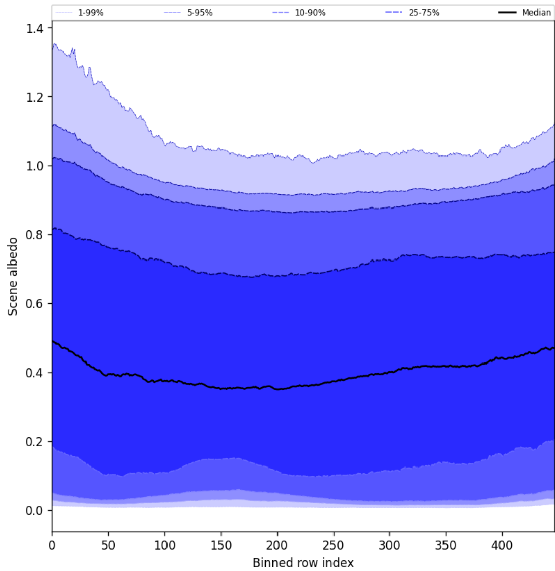
Figure 51: Along track statistics of “Scene albedo” for 2025-04-08 to 2025-04-10
