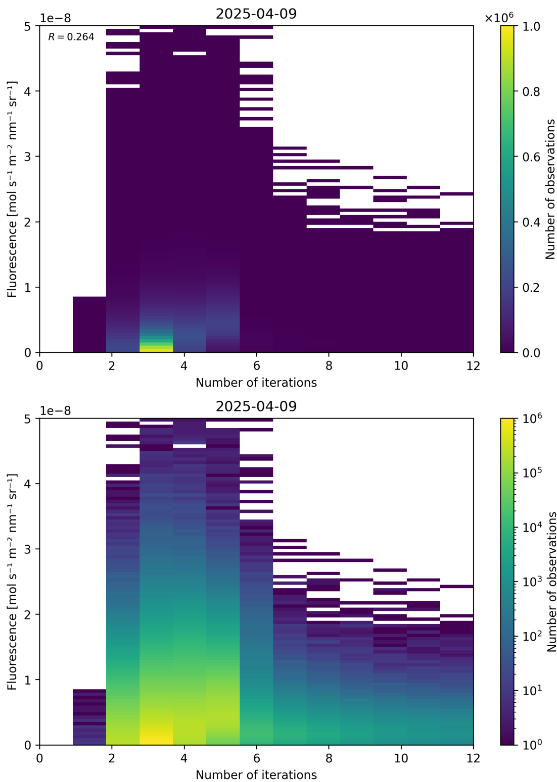
Figure 98: Scatter density plot of “Number of iterations” against “Fluorescence” for 2025-04-08 to 2025-04-10.
