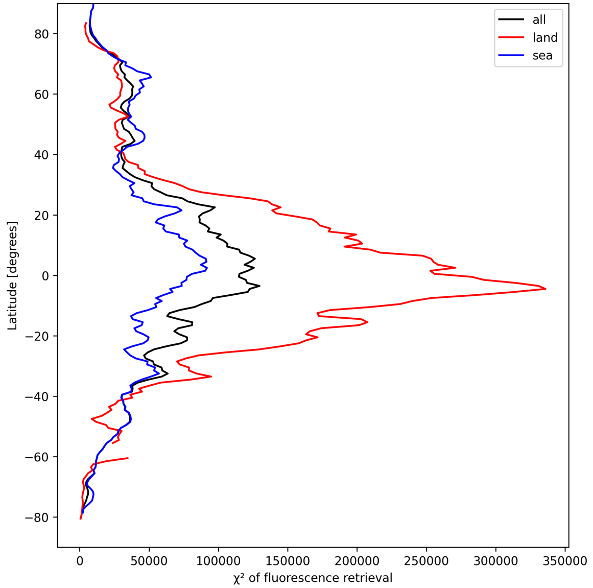
Figure 25: Zonal average of “ \chi^2 of fluorescence retrieval” for 2025-04-08 to 2025-04-10.
