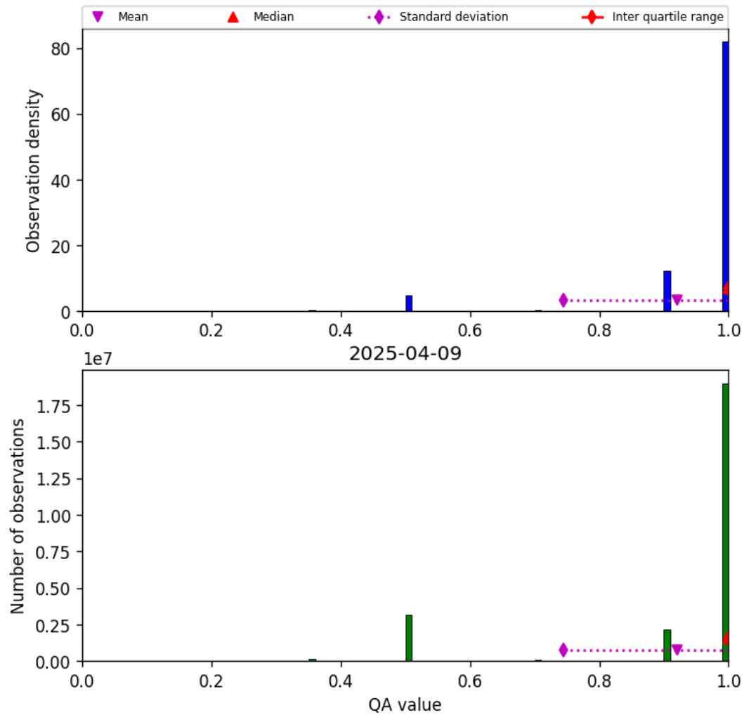
Figure 29: Histogram of “QA value” for 2025-04-08 to 2025-04-10
