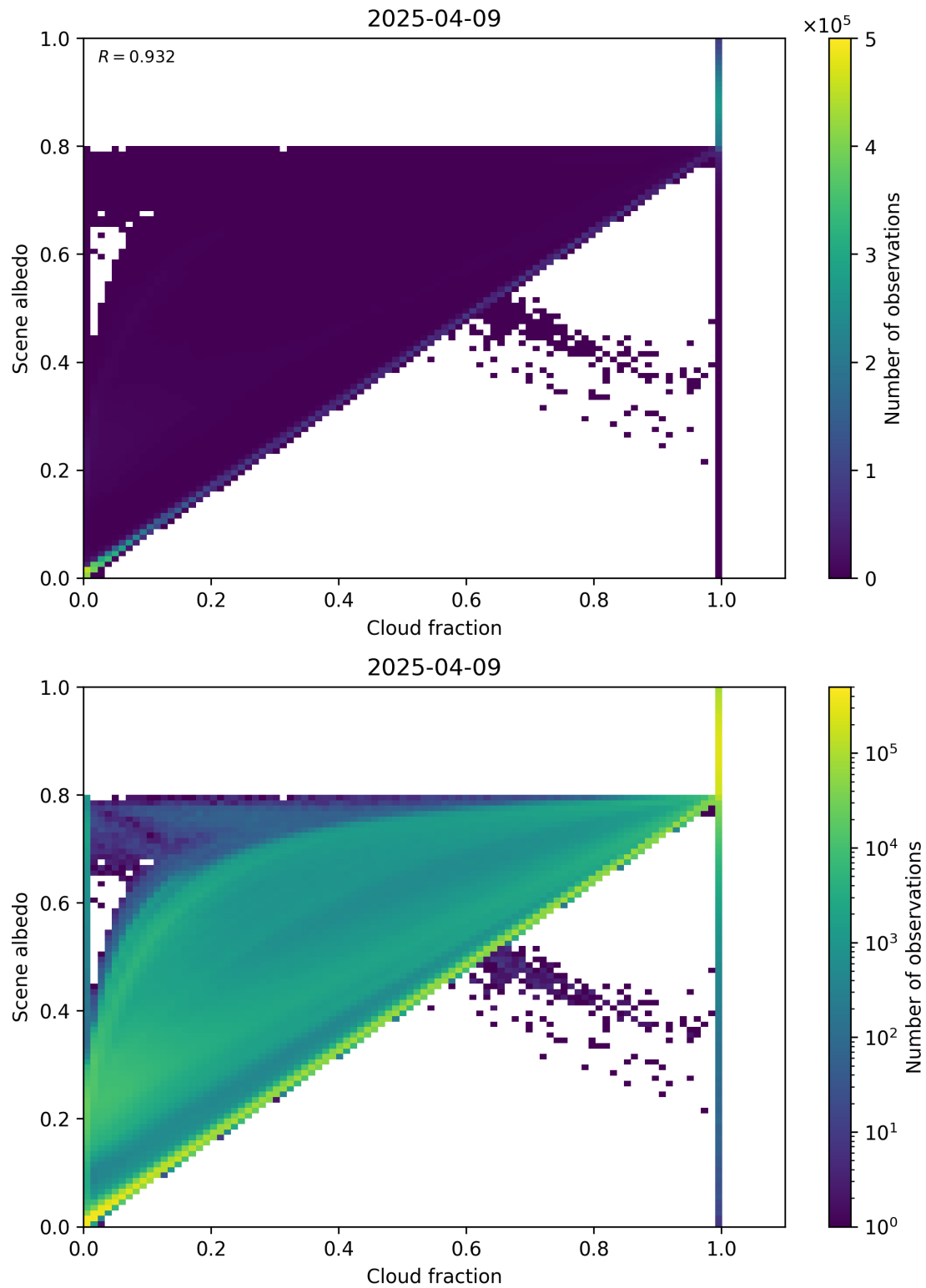
Figure 75: Scatter density plot of “Cloud fraction” against “Scene albedo” for 2025-04-08 to 2025-04-10.
