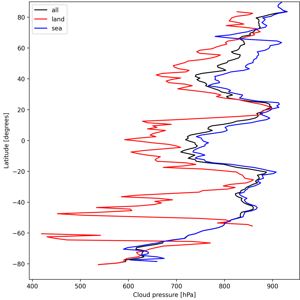
Figure 13: Zonal average of “Cloud pressure” for 2025-04-08 to 2025-04-10.
