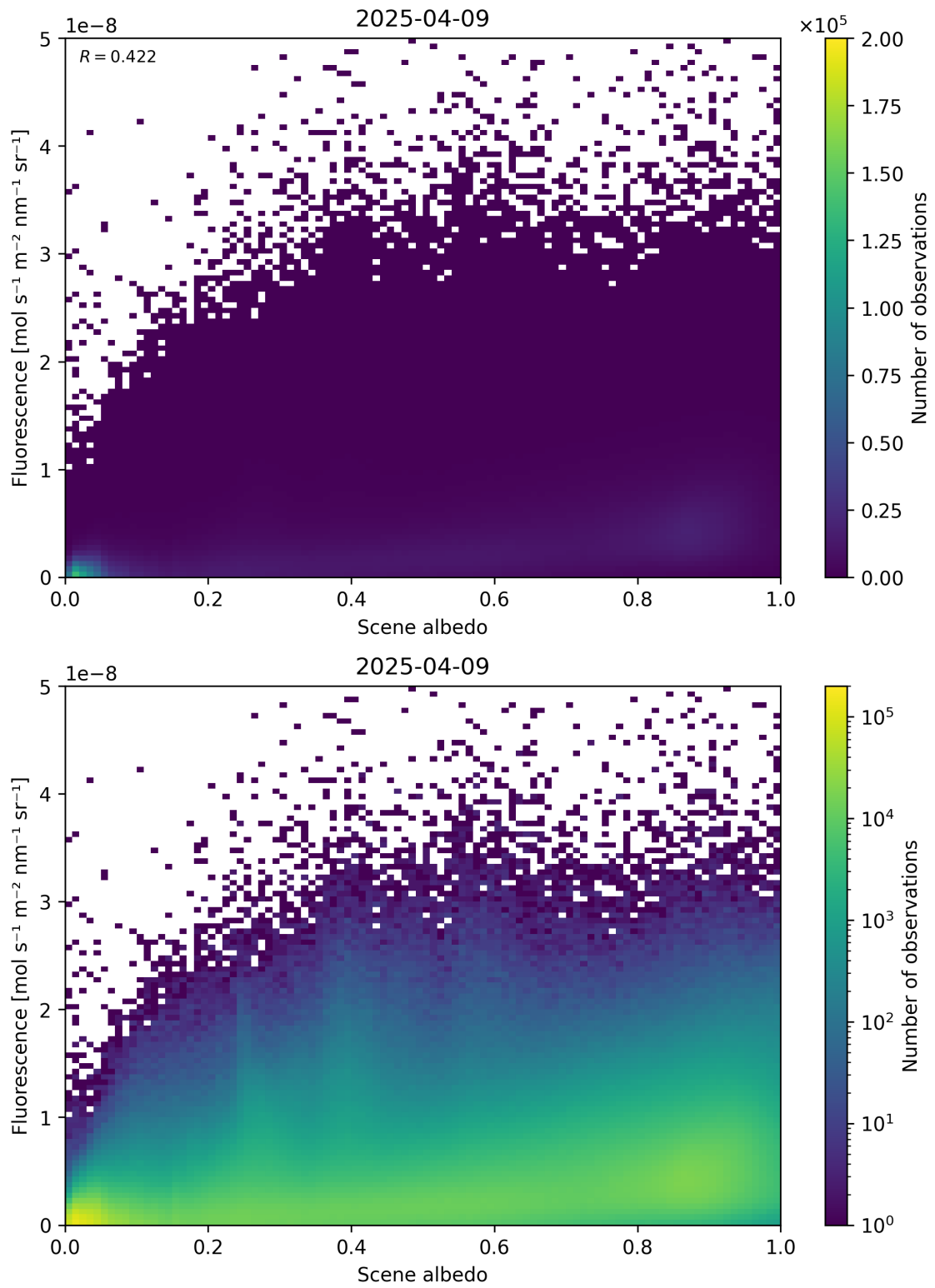
Figure 104: Scatter density plot of “Scene albedo” against “Fluorescence” for 2025-04-08 to 2025-04-10.
