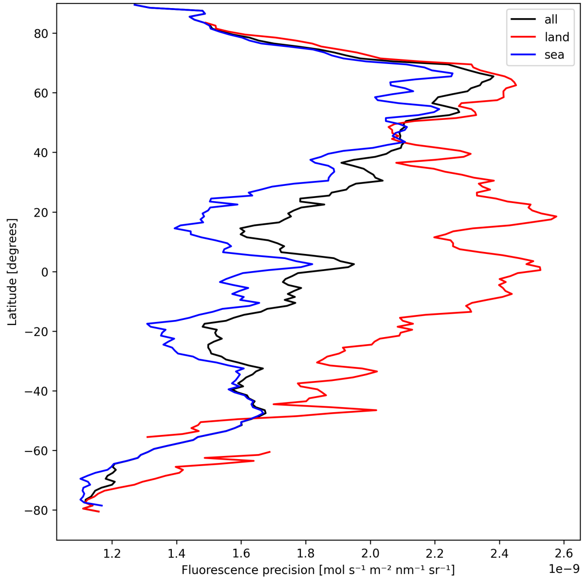
Figure 24: Zonal average of “Fluorescence precision” for 2025-04-08 to 2025-04-10.
