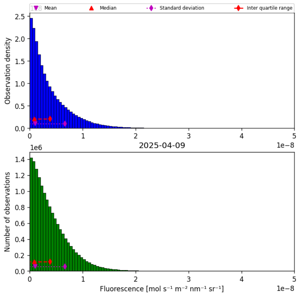
Figure 40: Histogram of “Fluorescence” for 2025-04-08 to 2025-04-10
