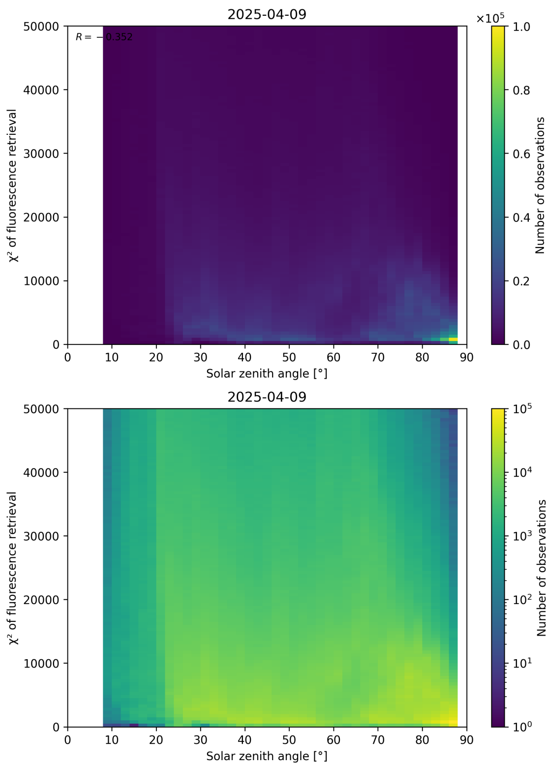
Figure 109: Scatter density plot of “Solar zenith angle” against “ \chi^2 of fluorescence retrieval” for 2025-04-08 to 2025-04-10.
