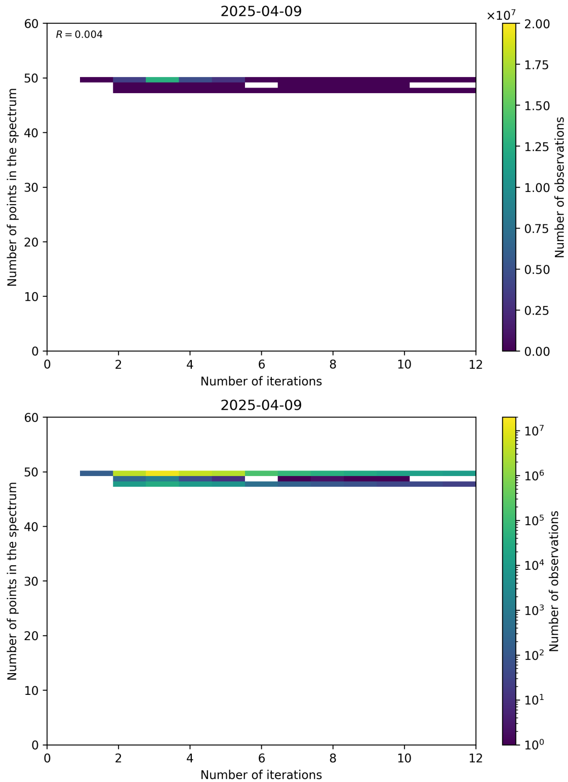
Figure 99: Scatter density plot of “Number of iterations” against “Number of points in the spectrum” for 2025-04-08 to 2025-04-10.
