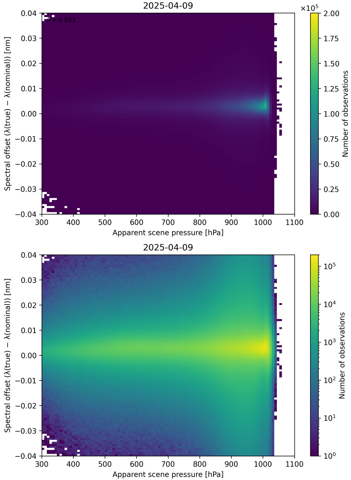
Figure 67: Scatter density plot of “Apparent scene pressure” against “Spectral offset ( \lambda_{\text{true}} - \lambda_{\text{nominal}} )” for 2025-04-08 to 2025-04-10.
