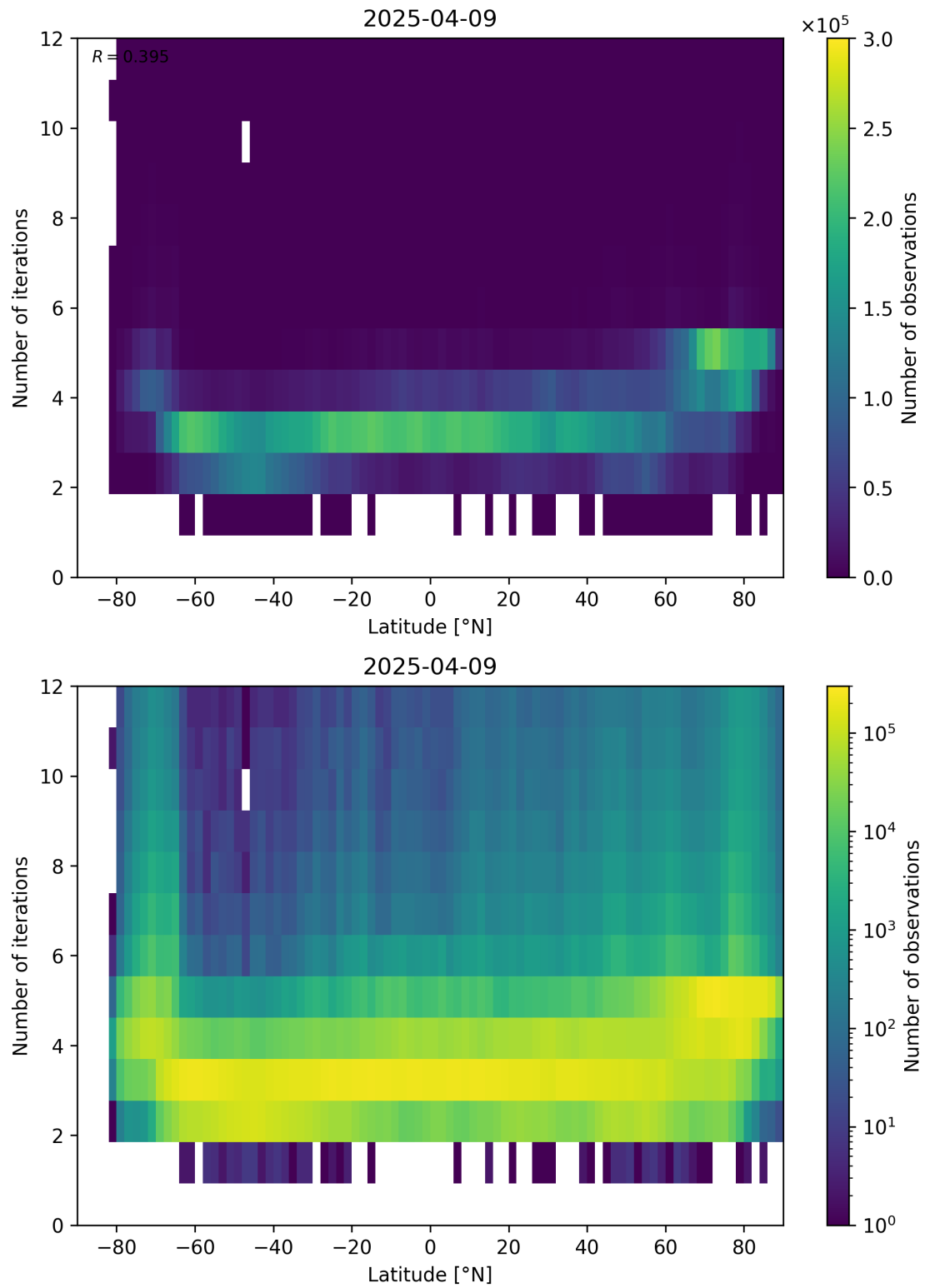
Figure 93: Scatter density plot of “Latitude” against “Number of iterations” for 2025-04-08 to 2025-04-10.
