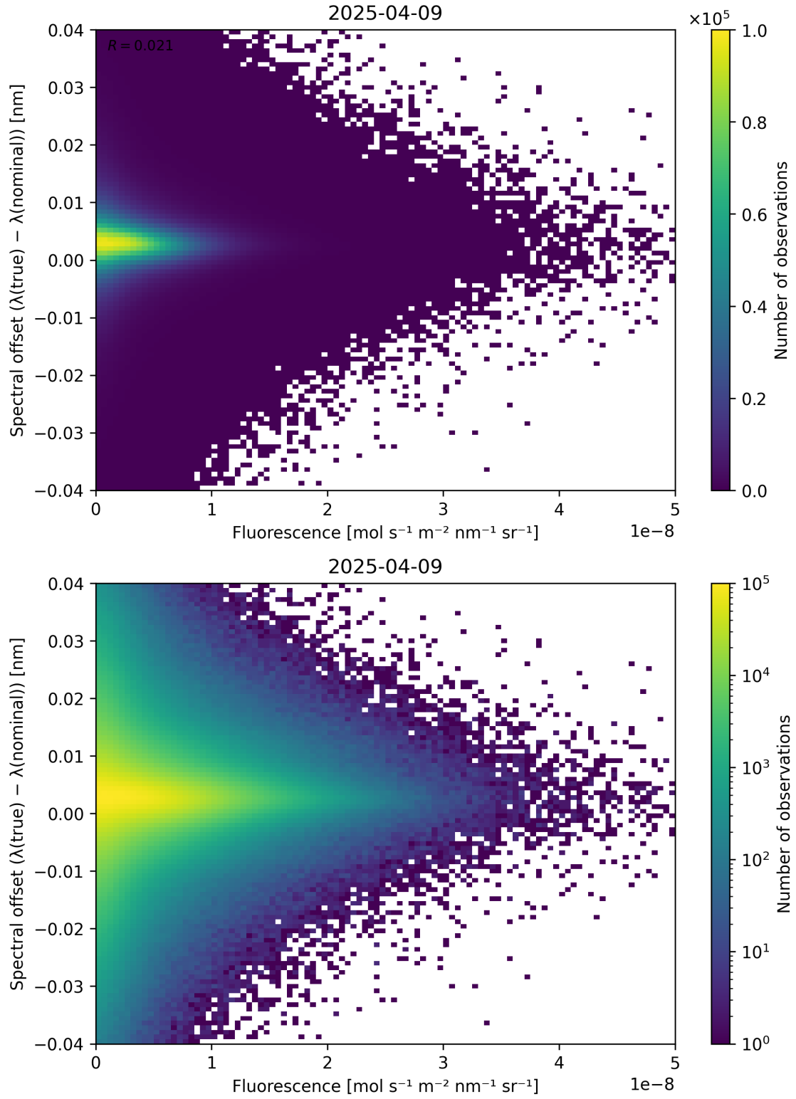
Figure 87: Scatter density plot of “Fluorescence” against “Spectral offset ( \lambda_{\text{true}} - \lambda_{\text{nominal}} )” for 2025-04-08 to 2025-04-10.
