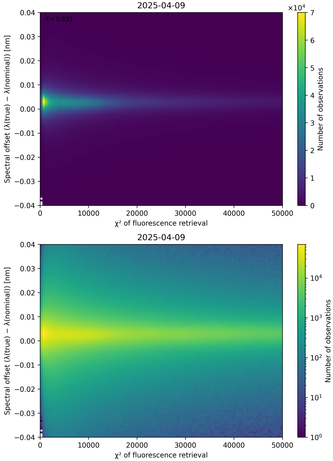
Figure 69: Scatter density plot of “ \chi^2 of fluorescence retrieval” against “Spectral offset ( \lambda_{\text{true}} - \lambda_{\text{nominal}} )” for 2025-04-08 to 2025-04-10.
