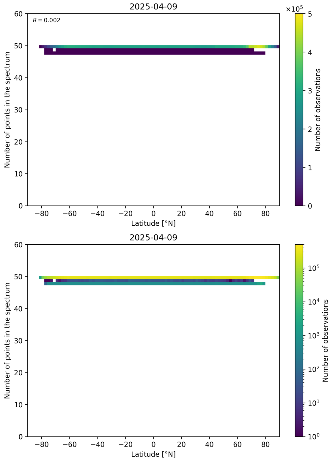
Figure 94: Scatter density plot of “Latitude” against “Number of points in the spectrum” for 2025-04-08 to 2025-04-10.
