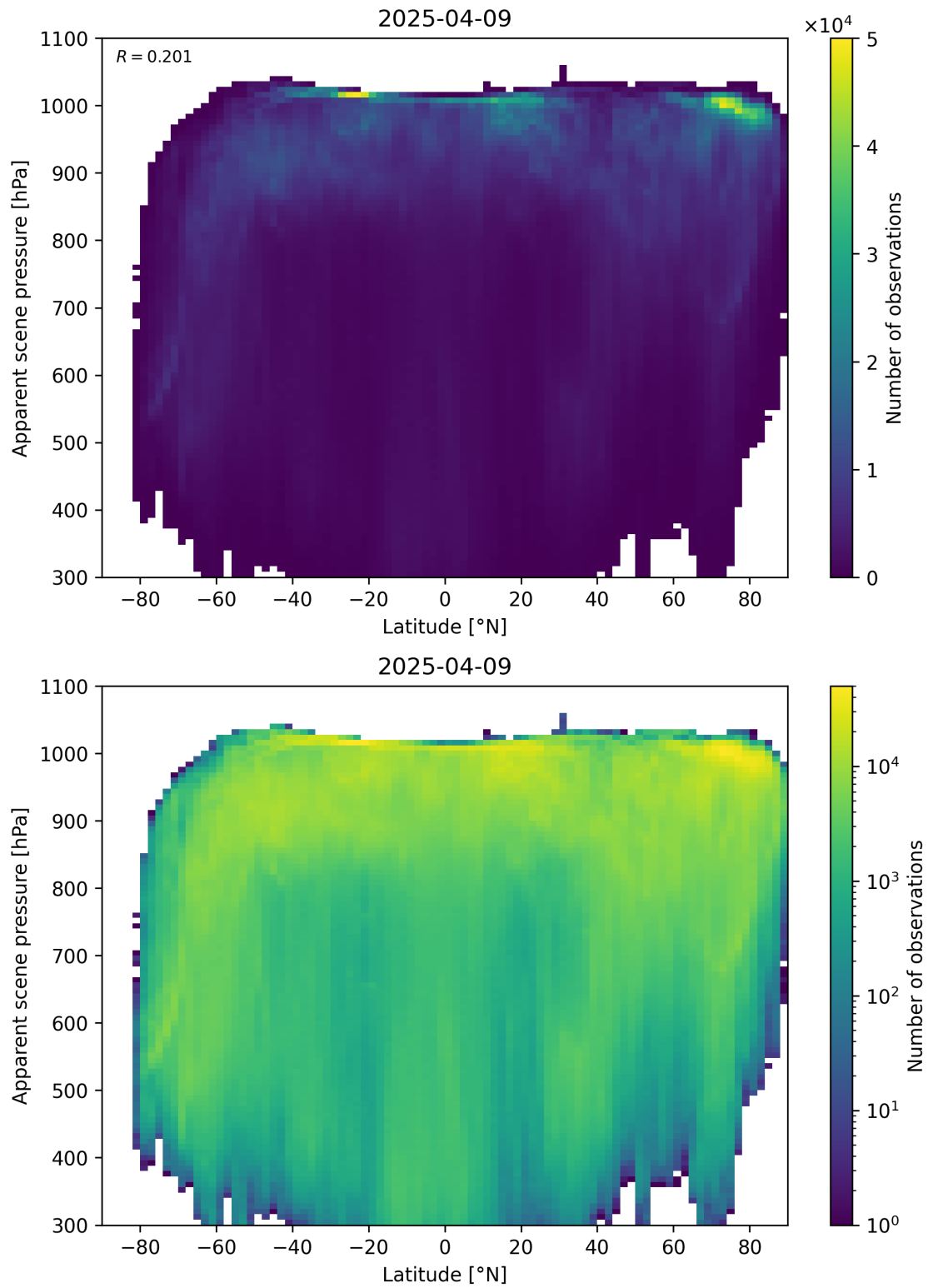
Figure 88: Scatter density plot of “Latitude” against “Apparent scene pressure” for 2025-04-08 to 2025-04-10.
