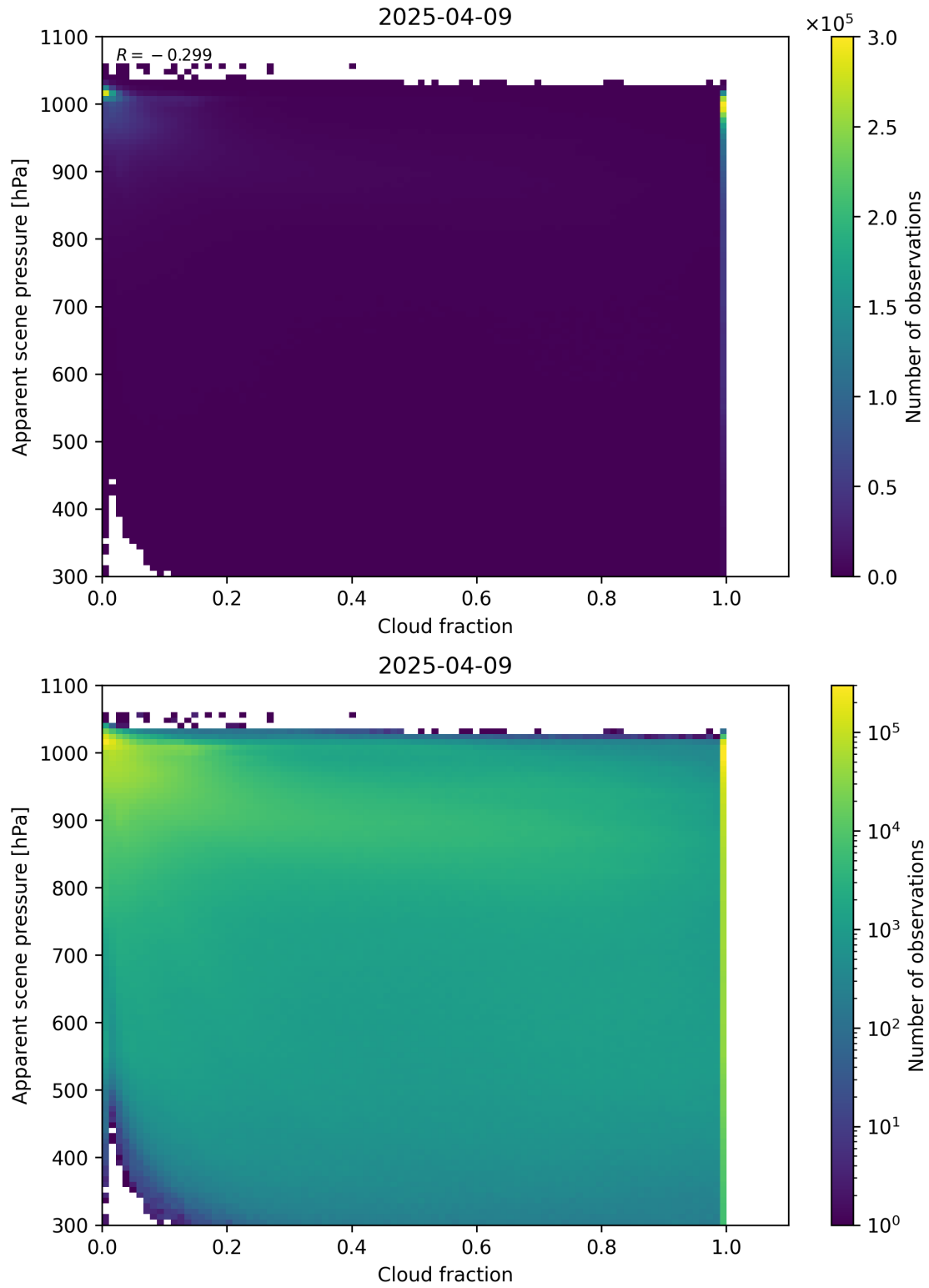
Figure 70: Scatter density plot of “Cloud fraction” against “Apparent scene pressure” for 2025-04-08 to 2025-04-10.
