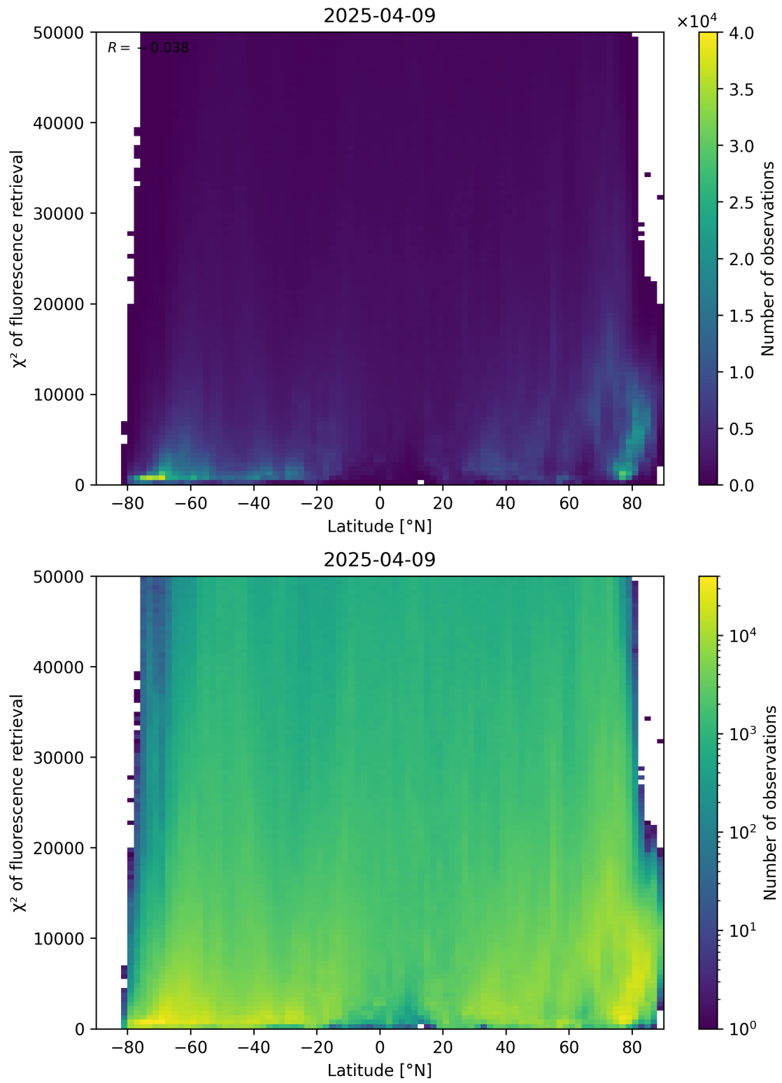
Figure 89: Scatter density plot of “Latitude” against “ \chi^2 of fluorescence retrieval” for 2025-04-08 to 2025-04-10.
