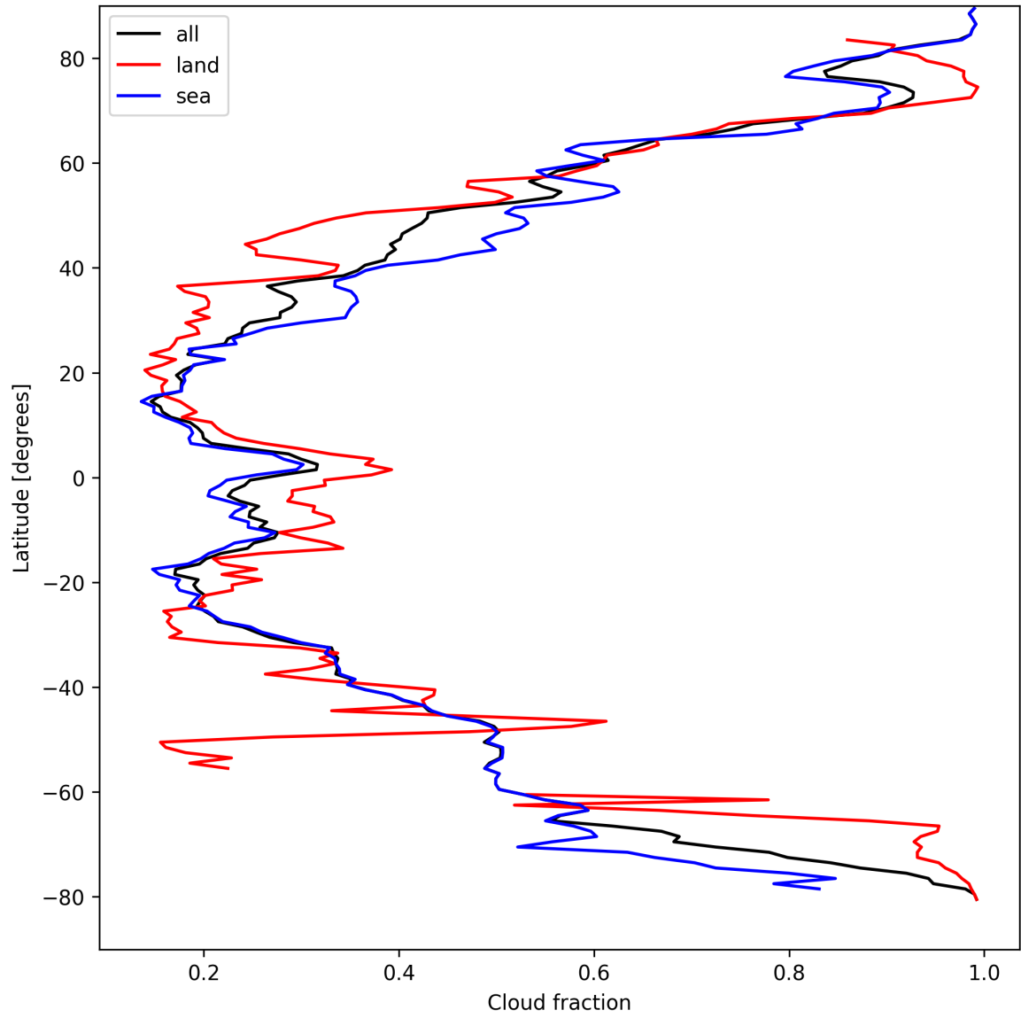
Figure 15: Zonal average of “Cloud fraction” for 2025-04-08 to 2025-04-10.
