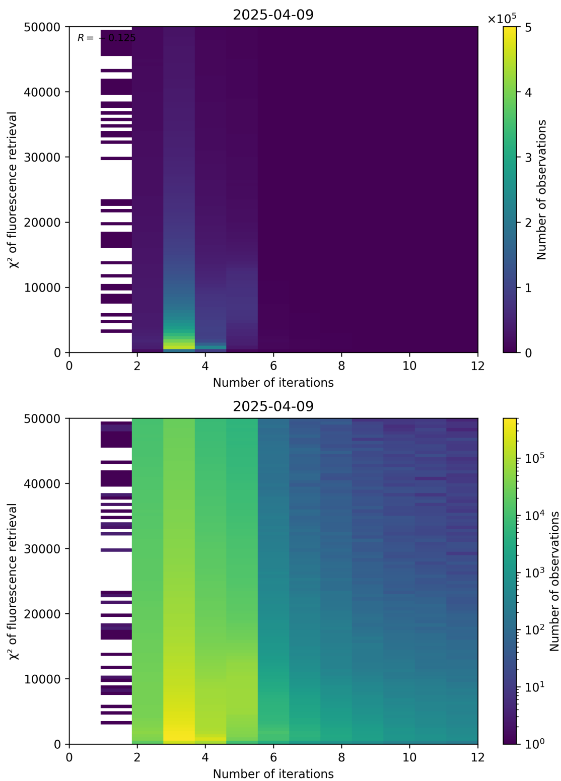
Figure 97: Scatter density plot of “Number of iterations” against “ \chi^2 of fluorescence retrieval” for 2025-04-08 to 2025-04-10.
