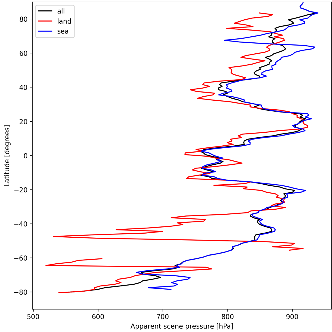
Figure 19: Zonal average of “Apparent scene pressure” for 2025-04-08 to 2025-04-10.
