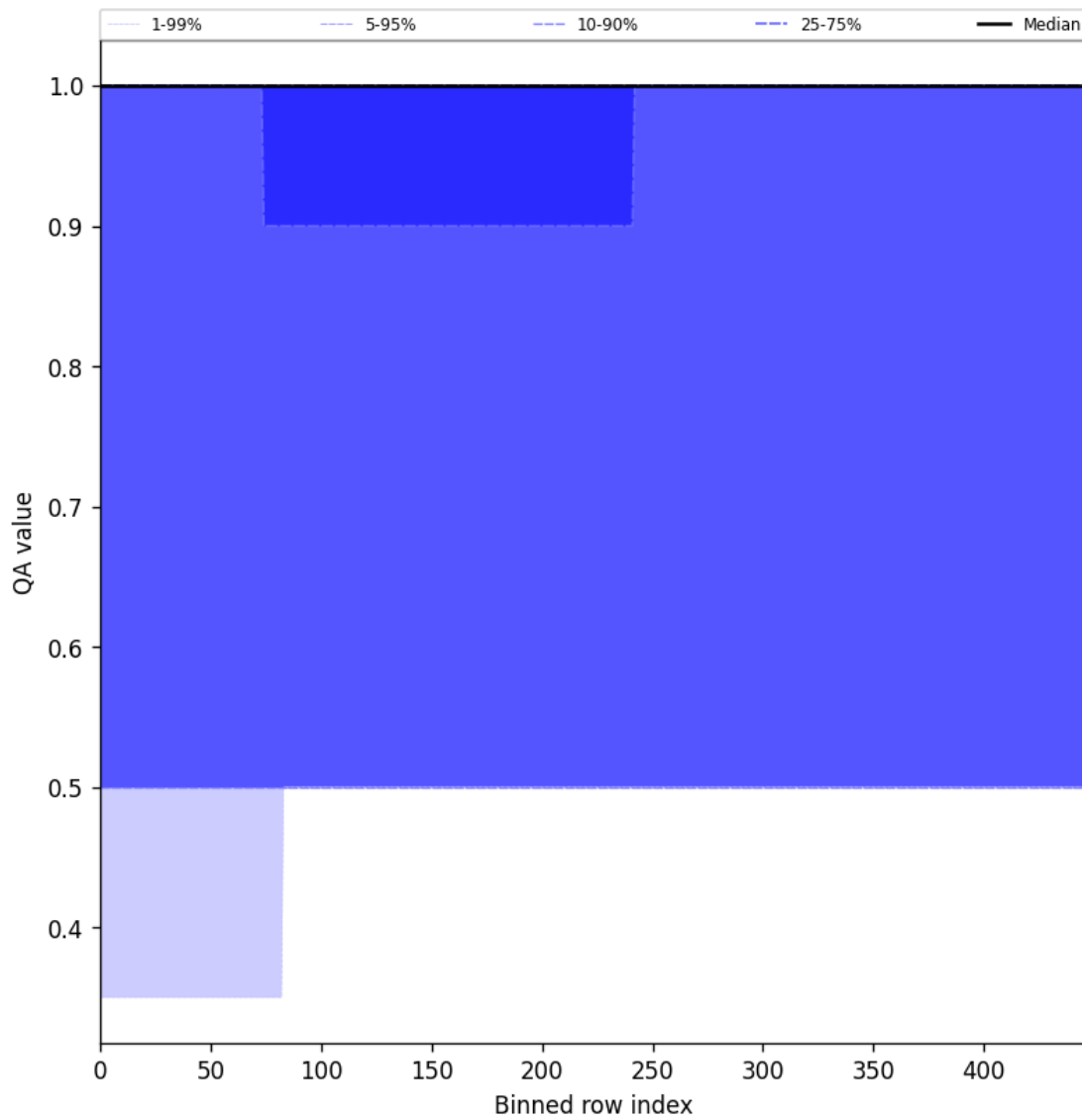
Figure 46: Along track statistics of “QA value” for 2025-04-08 to 2025-04-10
