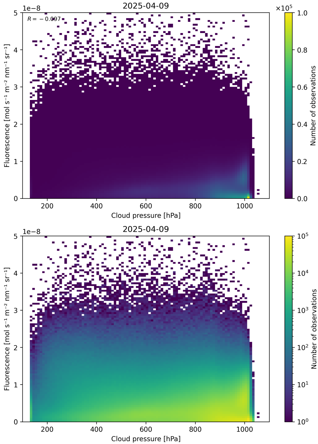
Figure 80: Scatter density plot of “Cloud pressure” against “Fluorescence” for 2025-04-08 to 2025-04-10.
