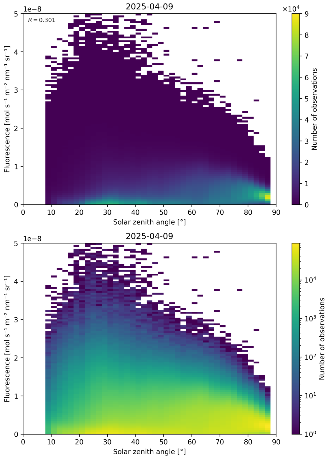
Figure 112: Scatter density plot of “Solar zenith angle” against “Fluorescence” for 2025-04-08 to 2025-04-10.
