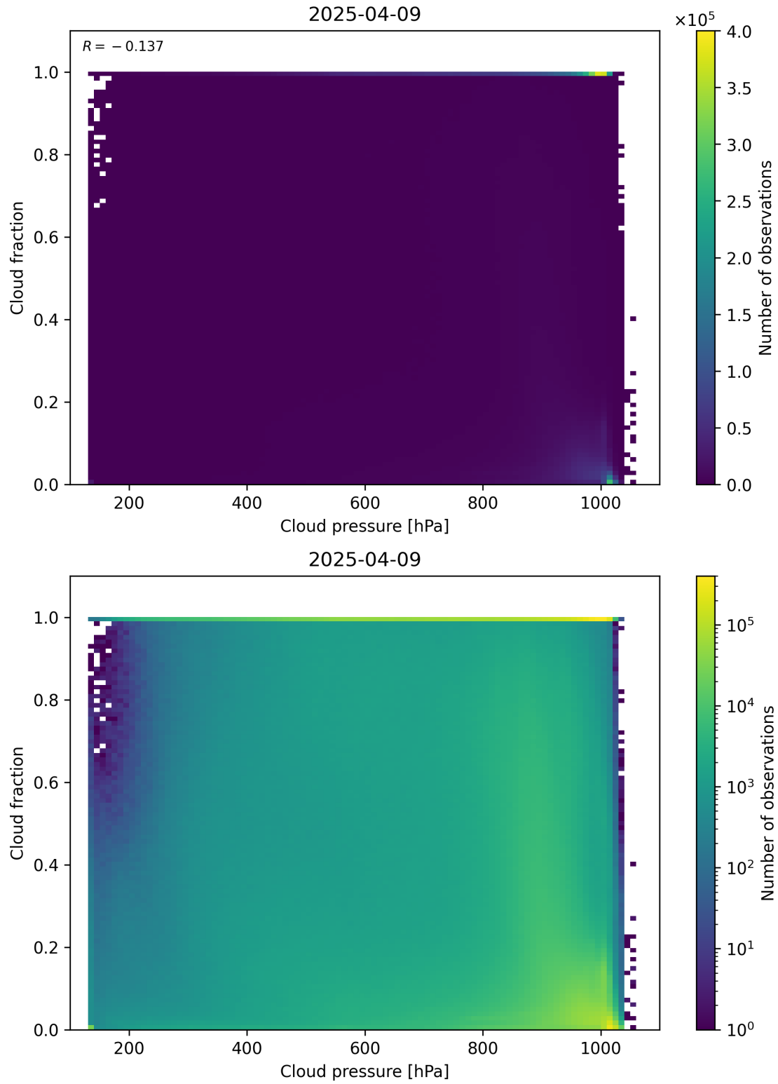
Figure 79: Scatter density plot of “Cloud pressure” against “Cloud fraction” for 2025-04-08 to 2025-04-10.
