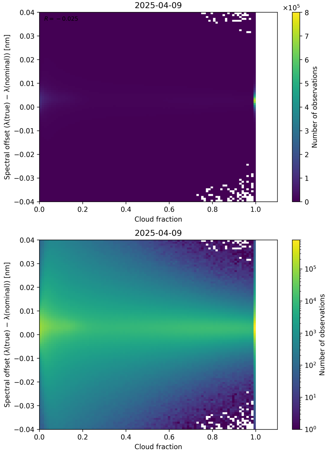
Figure 76: Scatter density plot of “Cloud fraction” against “Spectral offset ( \lambda_{\text{true}} - \lambda_{\text{nominal}} )” for 2025-04-08 to 2025-04-10.
