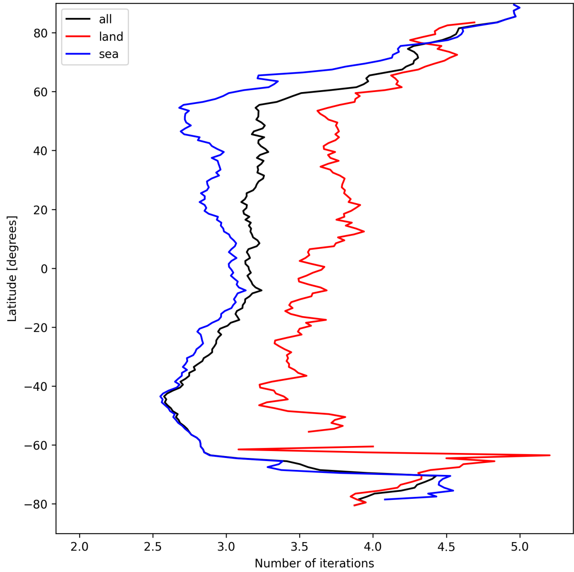
Figure 22: Zonal average of “Number of iterations” for 2025-04-08 to 2025-04-10.
