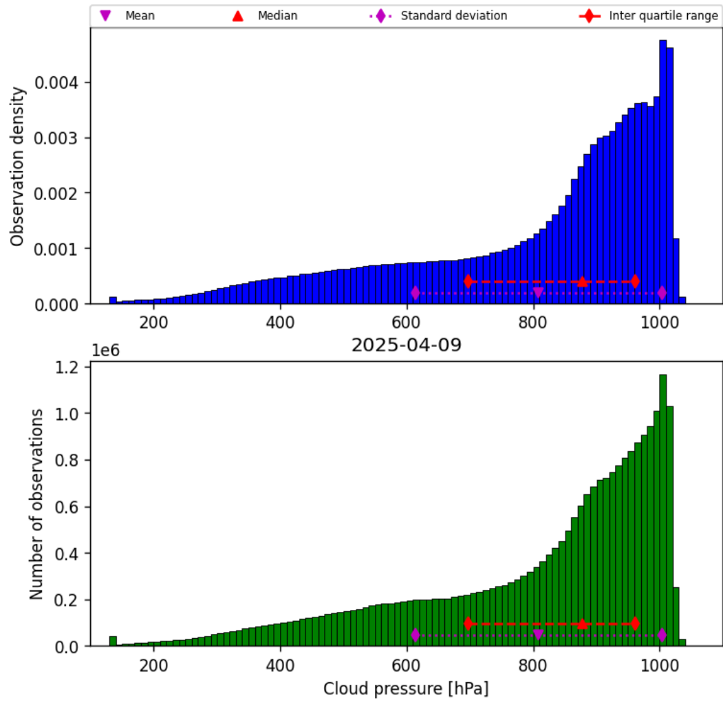
Figure 30: Histogram of “Cloud pressure” for 2025-04-08 to 2025-04-10
