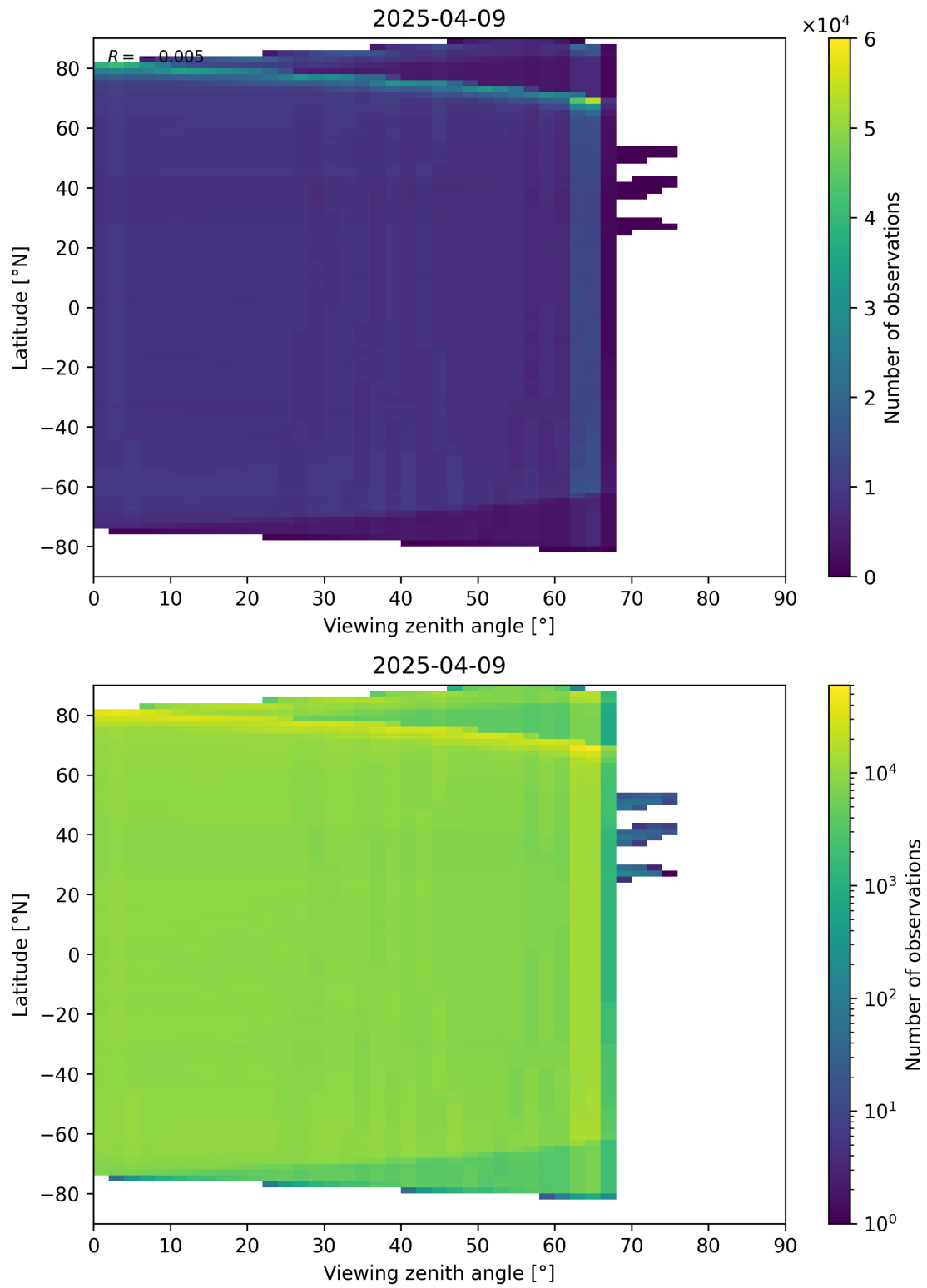
Figure 123: Scatter density plot of “Viewing zenith angle” against “Latitude” for 2025-04-08 to 2025-04-10.
