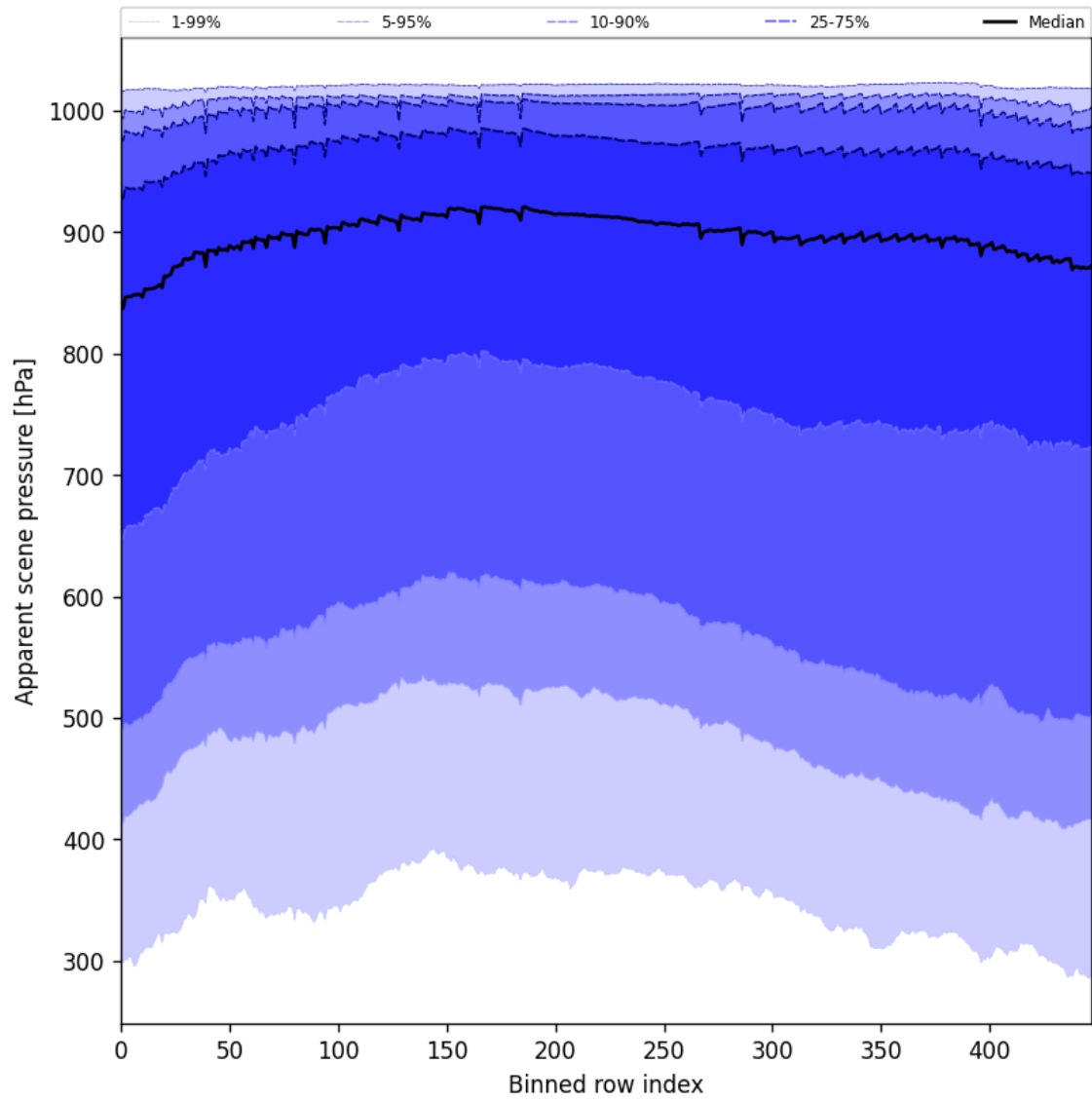
Figure 53: Along track statistics of “Apparent scene pressure” for 2025-04-08 to 2025-04-10
