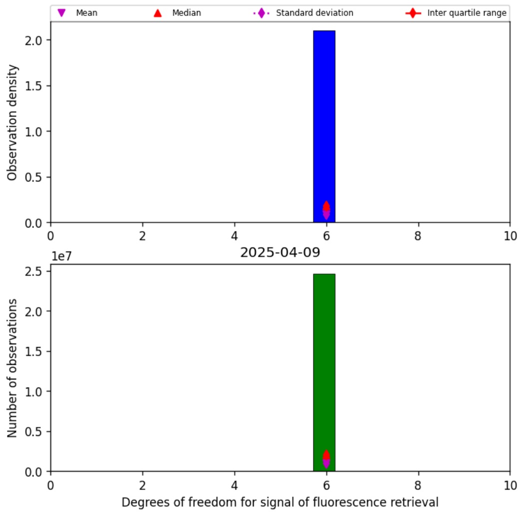
Figure 43: Histogram of "Degrees of freedom for signal of fluorescence retrieval" for 2025-04-08 to 2025-04-10
