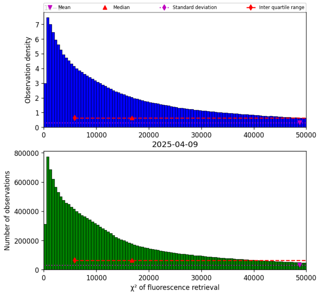
Figure 42: Histogram of “ \chi^2 of fluorescence retrieval” for 2025-04-08 to 2025-04-10
