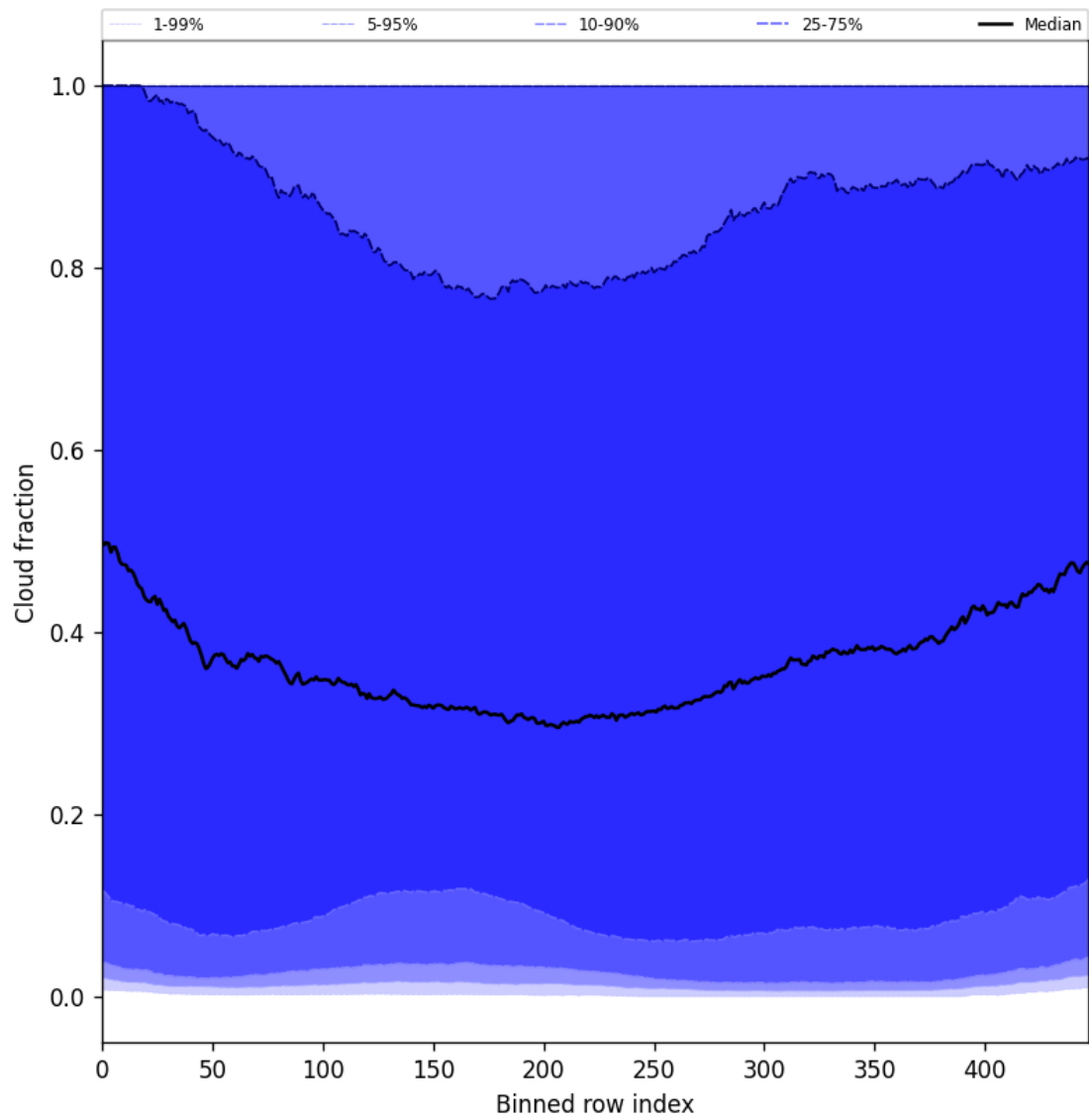
Figure 49: Along track statistics of “Cloud fraction” for 2025-04-08 to 2025-04-10
