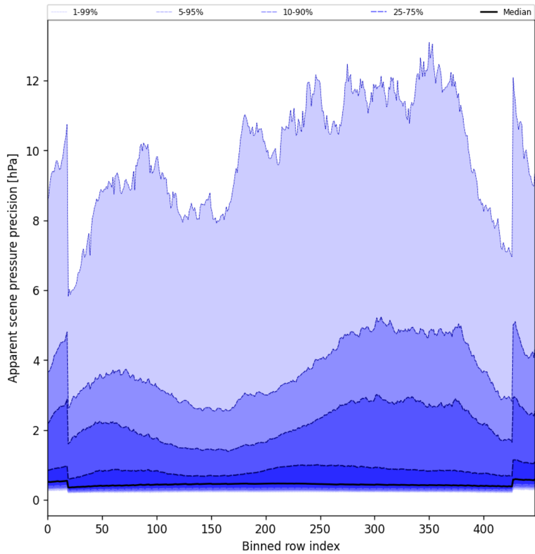
Figure 54: Along track statistics of “Apparent scene pressure precision” for 2025-04-08 to 2025-04-10
