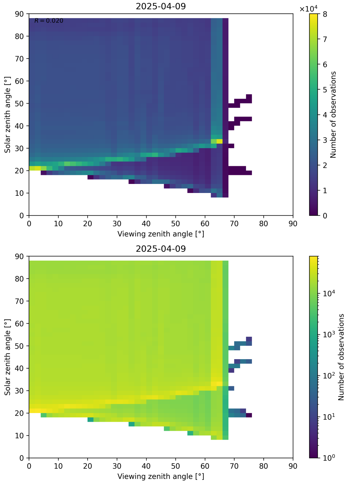
Figure 127: Scatter density plot of “Viewing zenith angle” against “Solar zenith angle” for 2025-04-08 to 2025-04-10.
