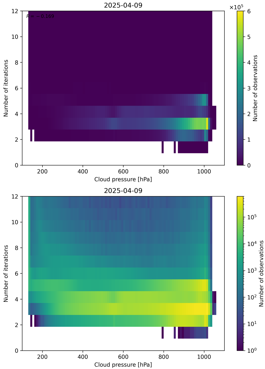
Figure 81: Scatter density plot of “Cloud pressure” against “Number of iterations” for 2025-04-08 to 2025-04-10.
