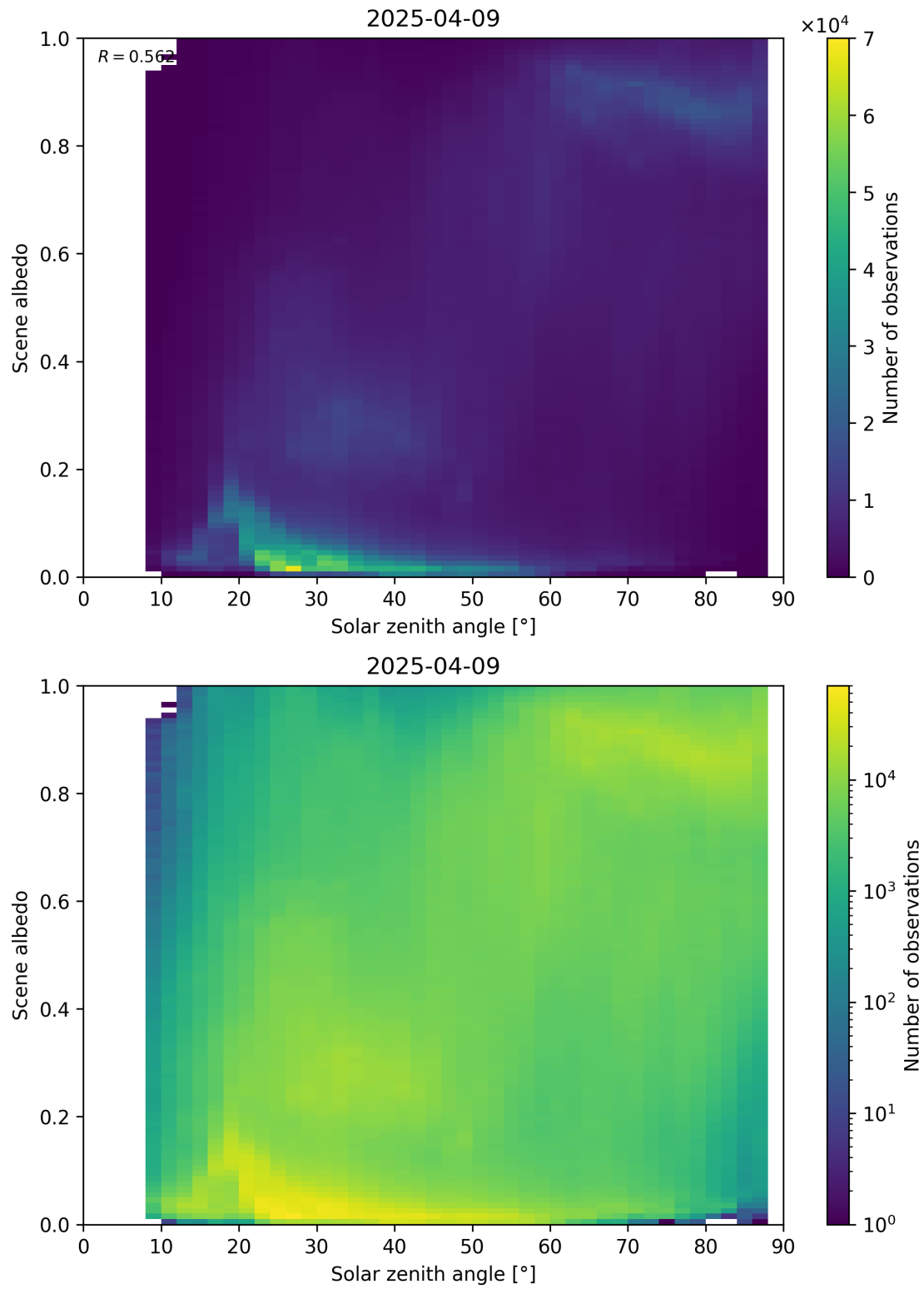
Figure 116: Scatter density plot of “Solar zenith angle” against “Scene albedo” for 2025-04-08 to 2025-04-10.
