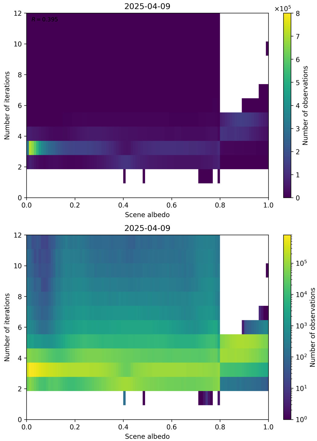
Figure 105: Scatter density plot of “Scene albedo” against “Number of iterations” for 2025-04-08 to 2025-04-10.
