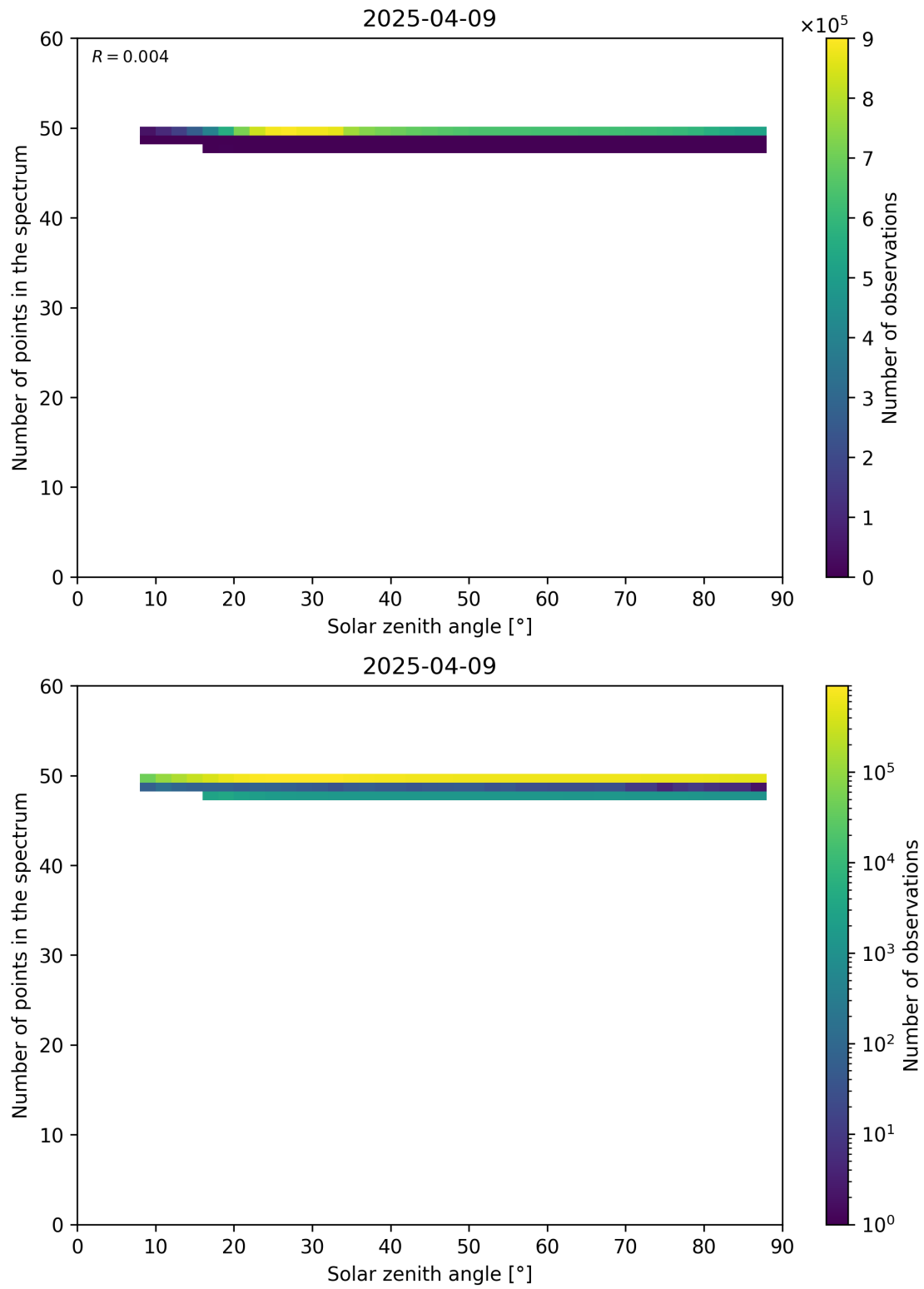
Figure 115: Scatter density plot of “Solar zenith angle” against “Number of points in the spectrum” for 2025-04-08 to 2025-04-10.
