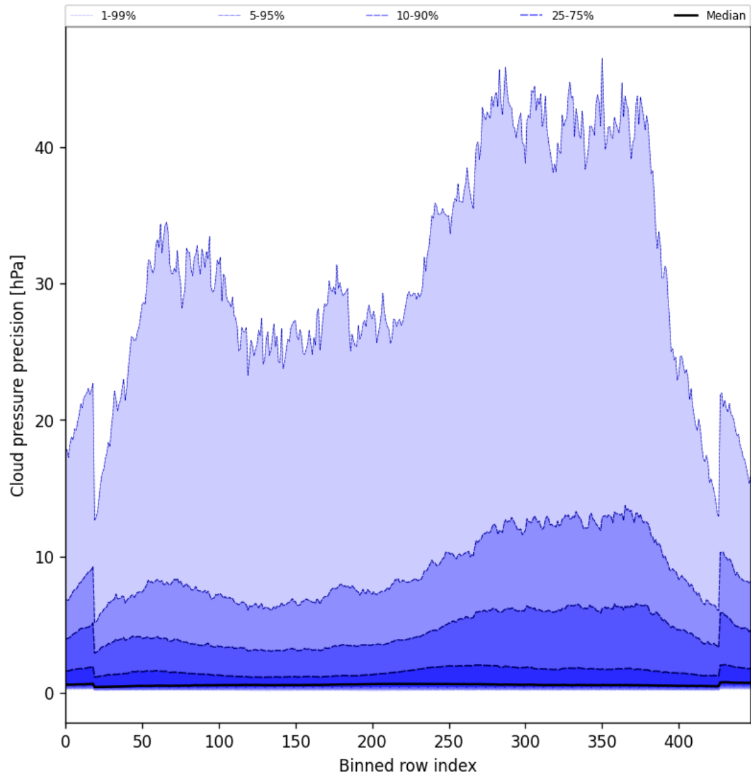
Figure 48: Along track statistics of “Cloud pressure precision” for 2025-04-08 to 2025-04-10
