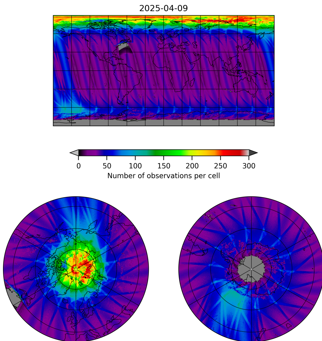
Figure 11: Map of the number of observations for 2025-04-08 to 2025-04-10
