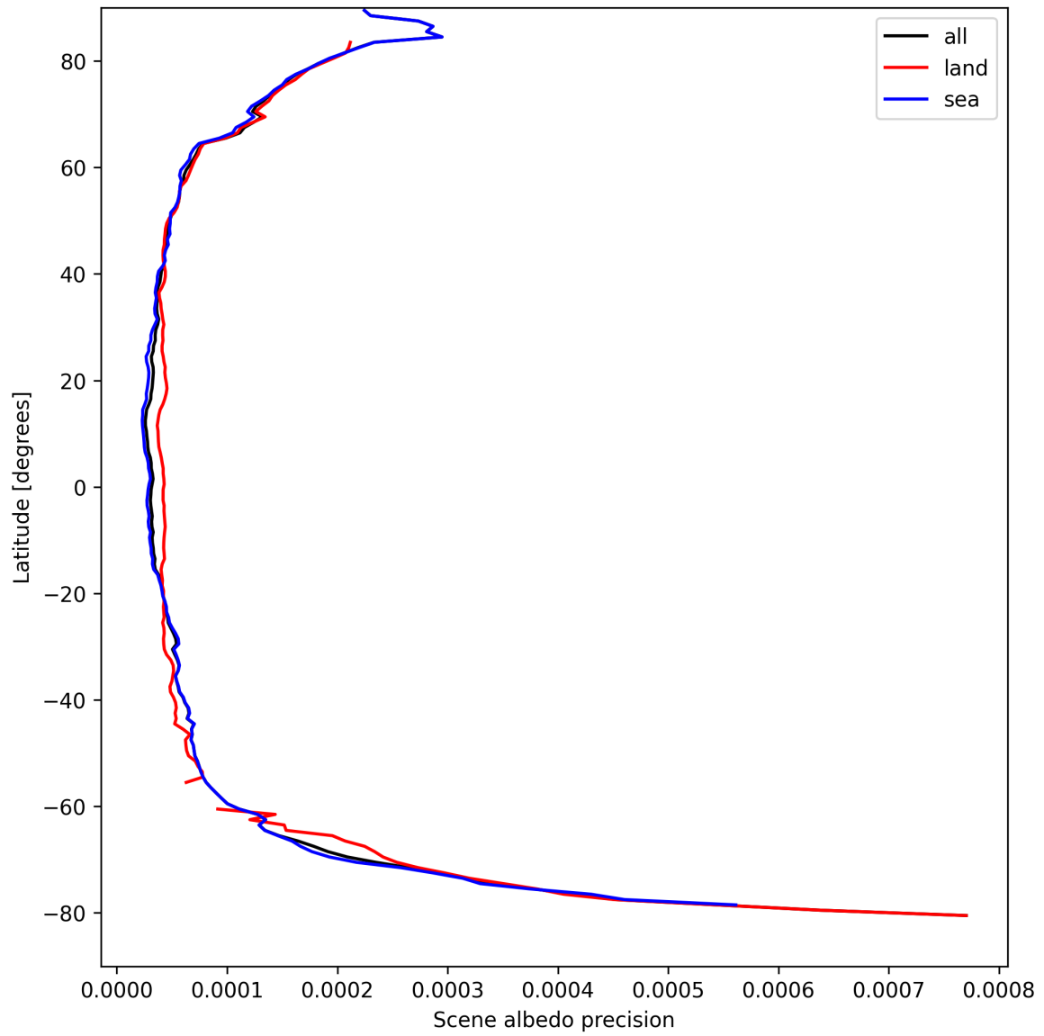
Figure 18: Zonal average of “Scene albedo precision” for 2025-04-08 to 2025-04-10.
