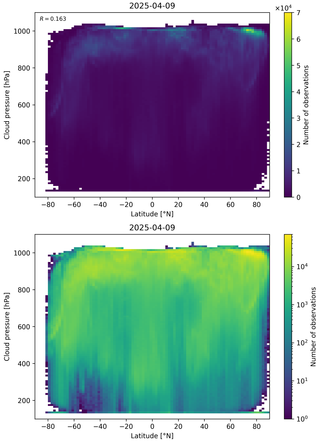
Figure 91: Scatter density plot of “Latitude” against “Cloud pressure” for 2025-04-08 to 2025-04-10.
