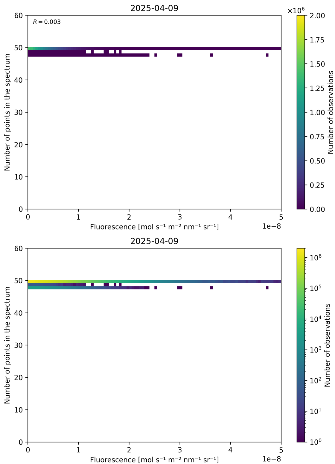
Figure 86: Scatter density plot of “Fluorescence” against “Number of points in the spectrum” for 2025-04-08 to 2025-04-10.
