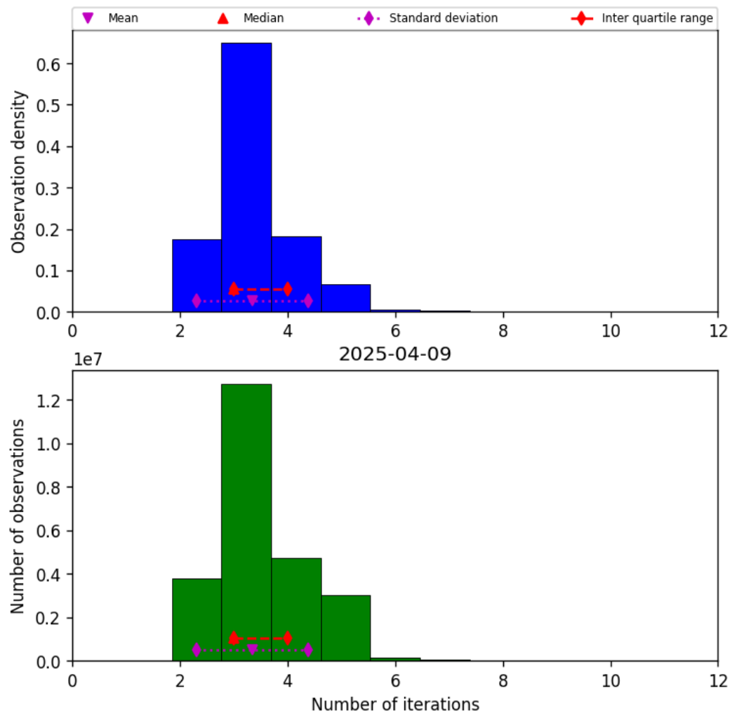
Figure 39: Histogram of “Number of iterations” for 2025-04-08 to 2025-04-10
