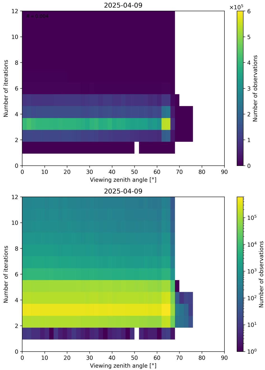
Figure 124: Scatter density plot of “Viewing zenith angle” against “Number of iterations” for 2025-04-08 to 2025-04-10.
