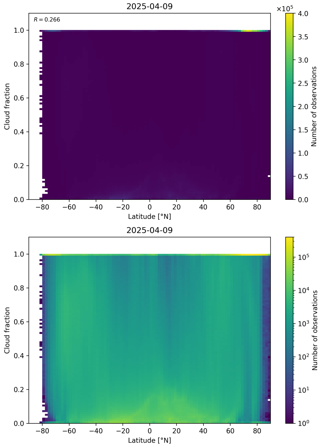
Figure 90: Scatter density plot of “Latitude” against “Cloud fraction” for 2025-04-08 to 2025-04-10.
