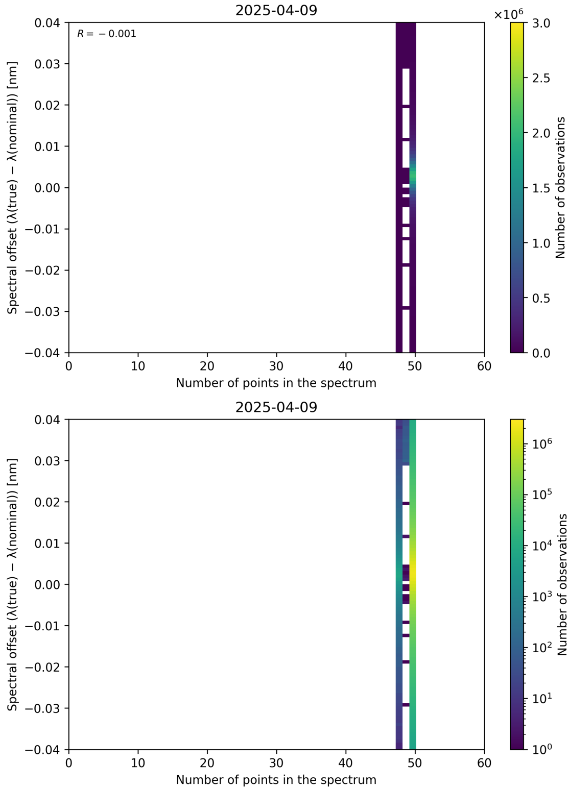
Figure 101: Scatter density plot of “Number of points in the spectrum” against “Spectral offset ( \lambda_{\text{true}} - \lambda_{\text{nominal}} )” for 2025-04-08 to 2025-04-10.
