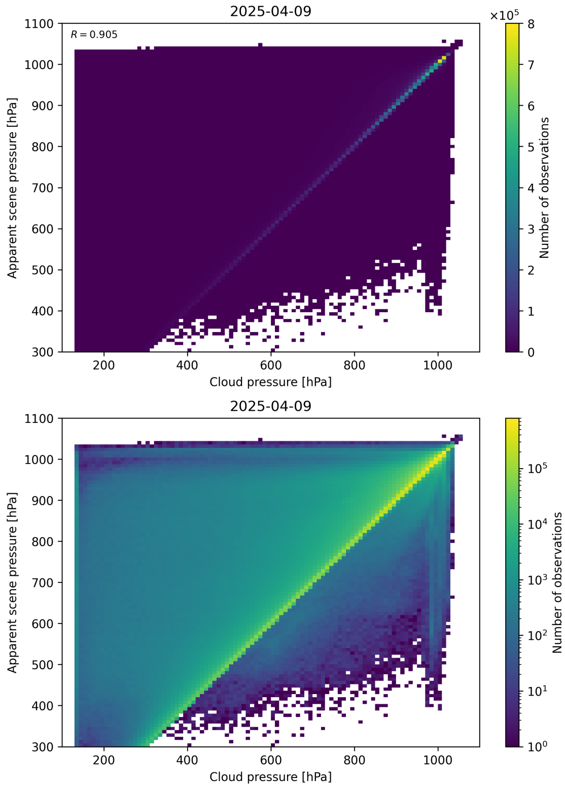
Figure 77: Scatter density plot of “Cloud pressure” against “Apparent scene pressure” for 2025-04-08 to 2025-04-10.
