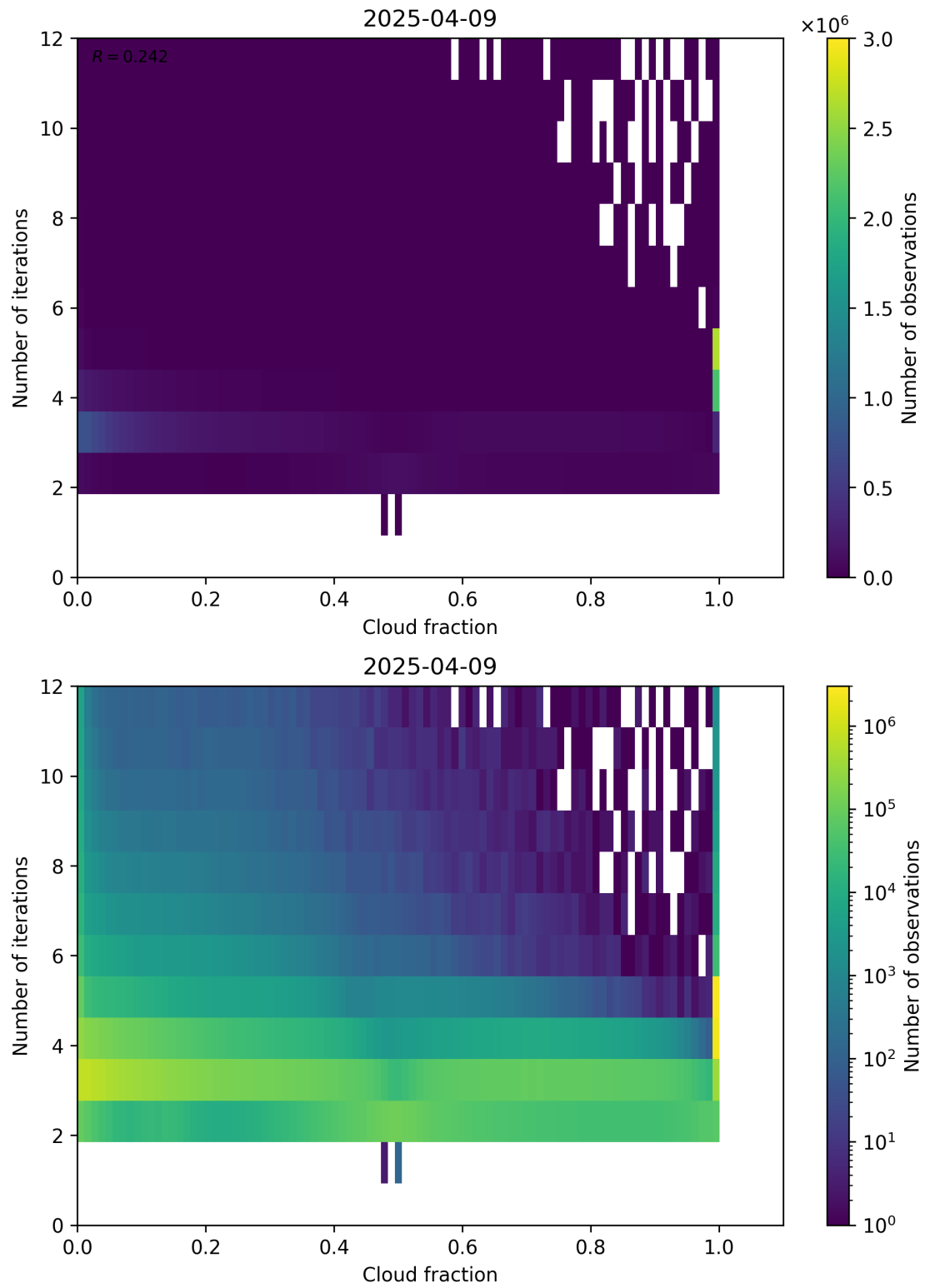
Figure 73: Scatter density plot of “Cloud fraction” against “Number of iterations” for 2025-04-08 to 2025-04-10.
