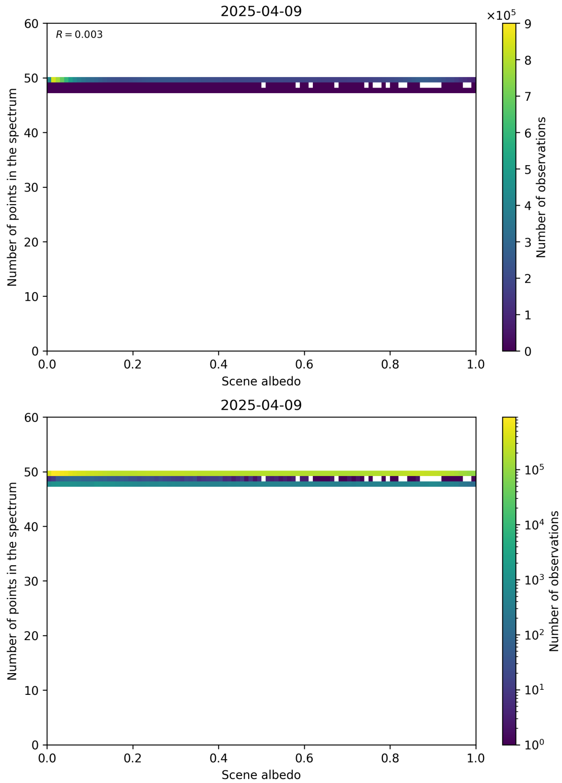
Figure 106: Scatter density plot of “Scene albedo” against “Number of points in the spectrum” for 2025-04-08 to 2025-04-10.
