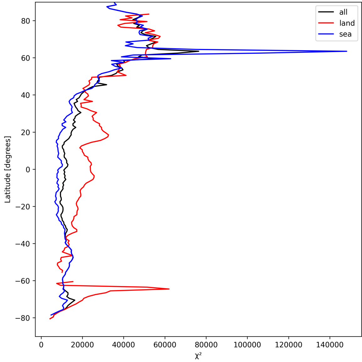
Figure 21: Zonal average of “ \chi^2 ” for 2025-04-08 to 2025-04-10.
