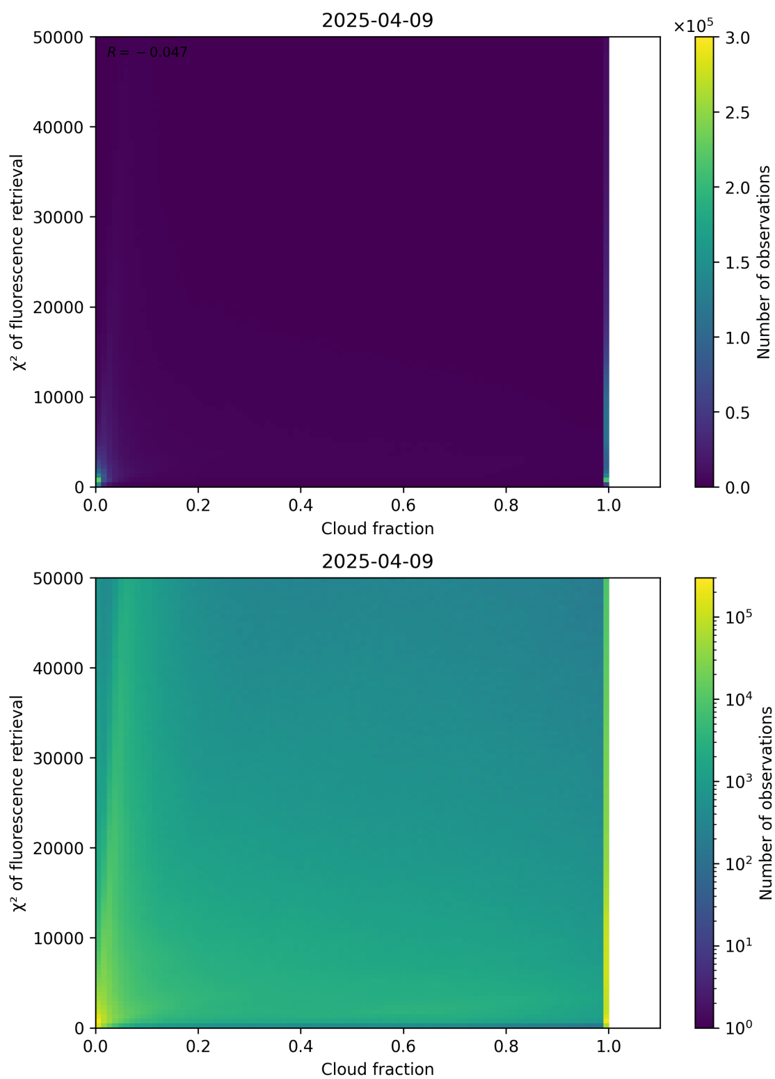
Figure 71: Scatter density plot of “Cloud fraction” against “ \chi^2 of fluorescence retrieval” for 2025-04-08 to 2025-04-10.
