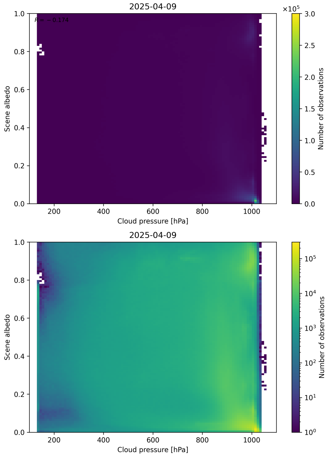
Figure 83: Scatter density plot of “Cloud pressure” against “Scene albedo” for 2025-04-08 to 2025-04-10.
