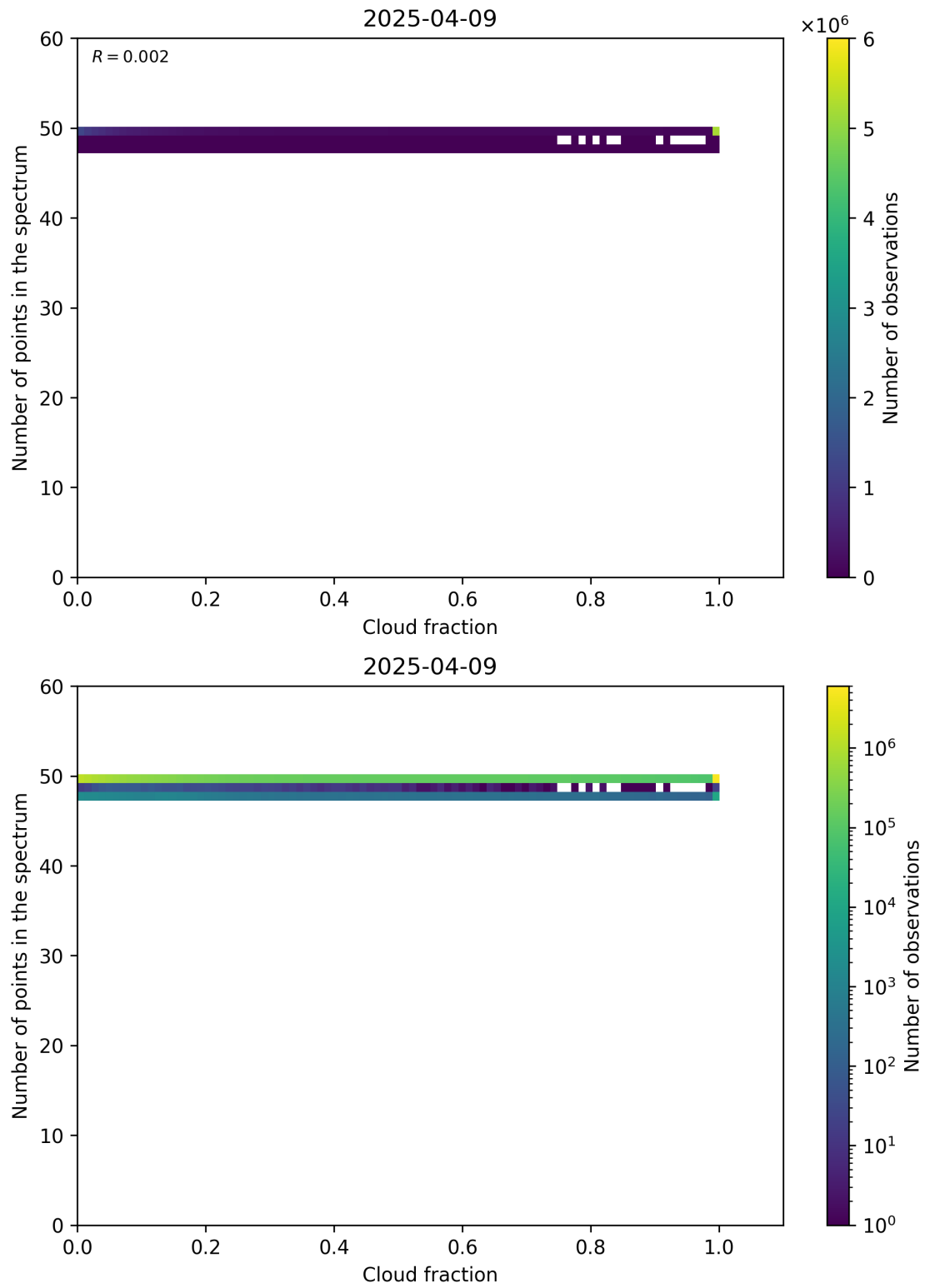
Figure 74: Scatter density plot of “Cloud fraction” against “Number of points in the spectrum” for 2025-04-08 to 2025-04-10.
