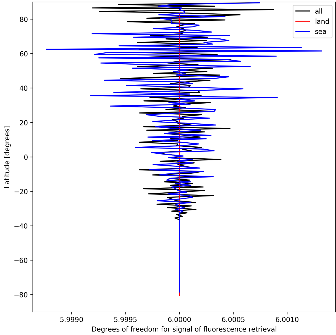
Figure 26: Zonal average of “Degrees of freedom for signal of fluorescence retrieval” for 2025-04-08 to 2025-04-10.
