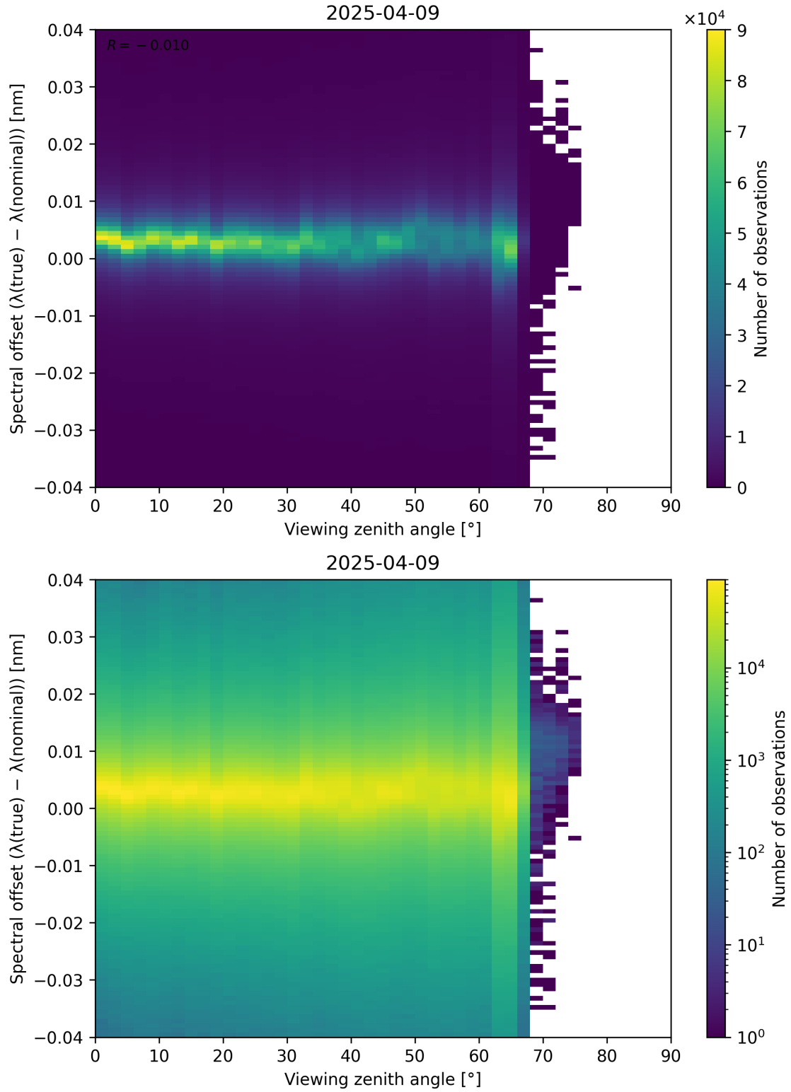
Figure 128: Scatter density plot of “Viewing zenith angle” against “Spectral offset ( \lambda_{\text{true}} - \lambda_{\text{nominal}} )” for 2025-04-08 to 2025-04-10.
