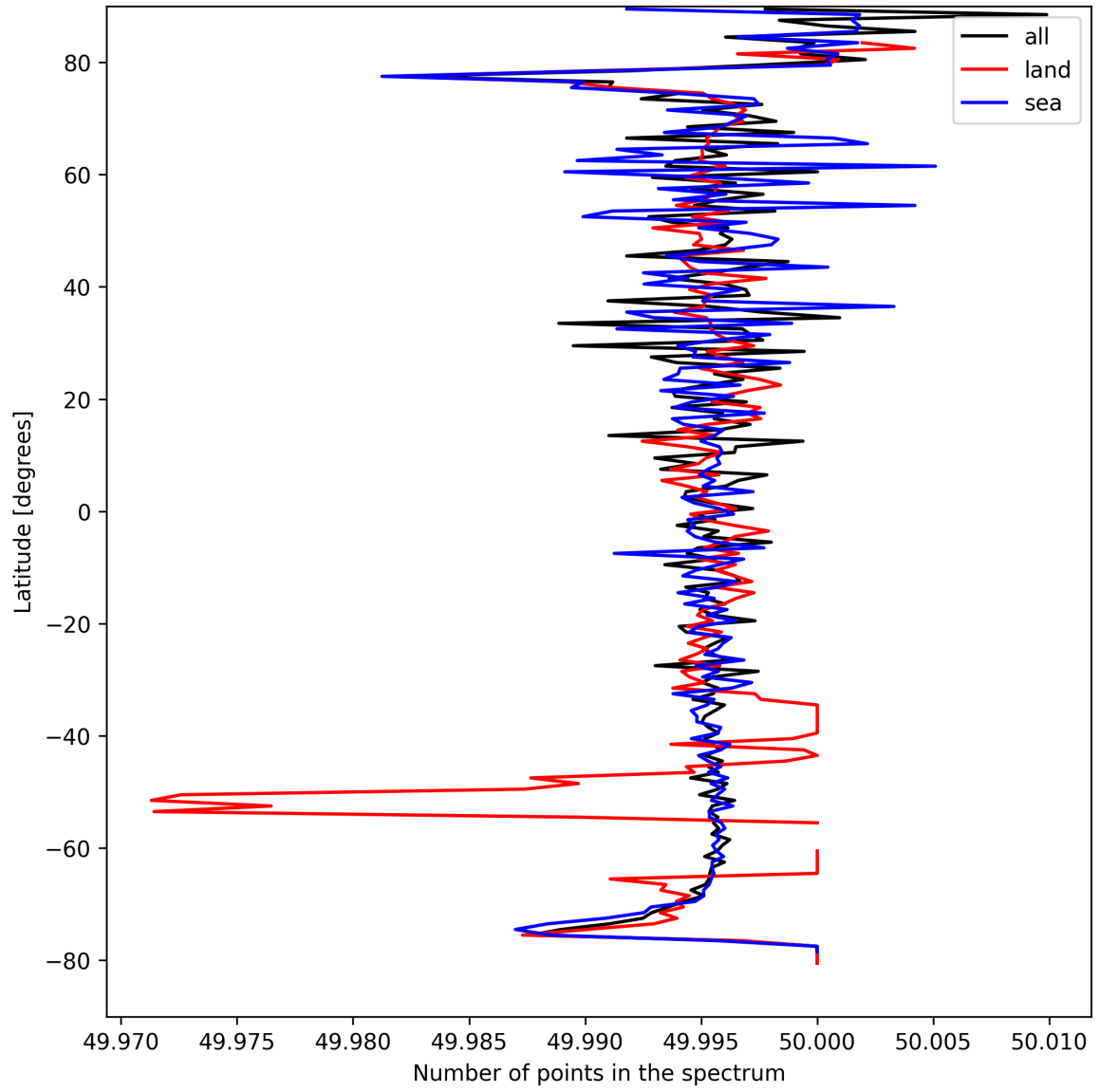
Figure 27: Zonal average of “Number of points in the spectrum” for 2025-04-08 to 2025-04-10.
