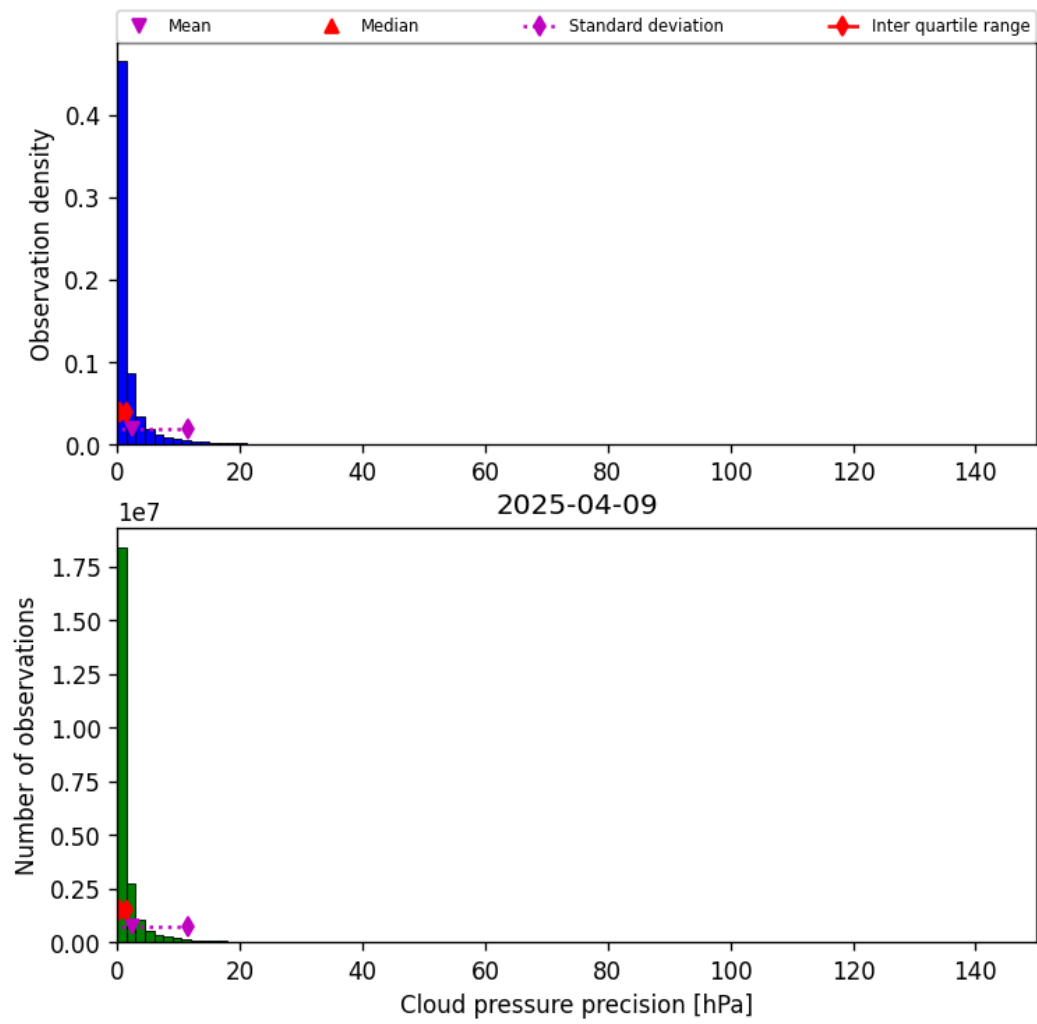
Figure 31: Histogram of “Cloud pressure precision” for 2025-04-08 to 2025-04-10
