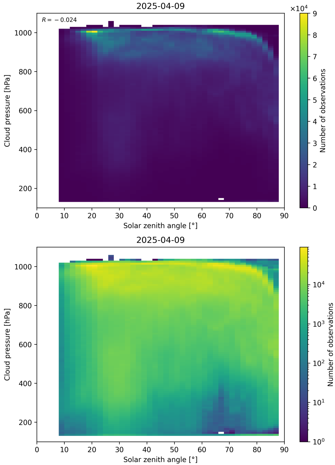
Figure 111: Scatter density plot of “Solar zenith angle” against “Cloud pressure” for 2025-04-08 to 2025-04-10.
