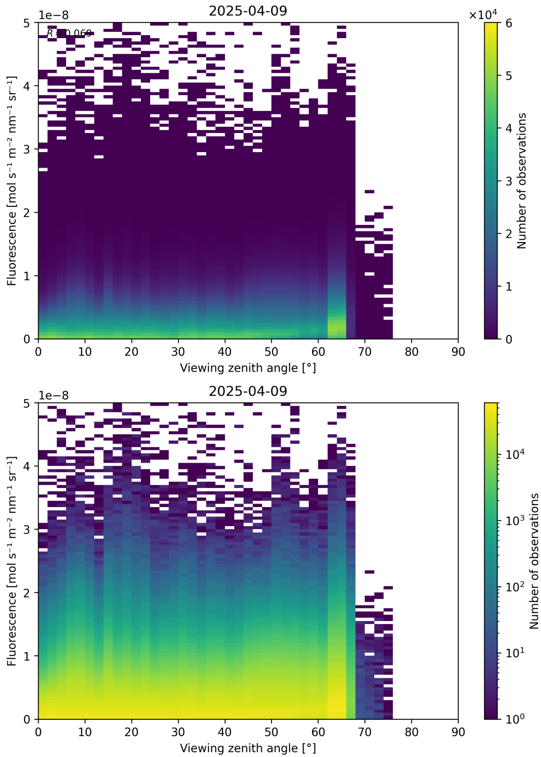
Figure 122: Scatter density plot of “Viewing zenith angle” against “Fluorescence” for 2025-04-08 to 2025-04-10.
