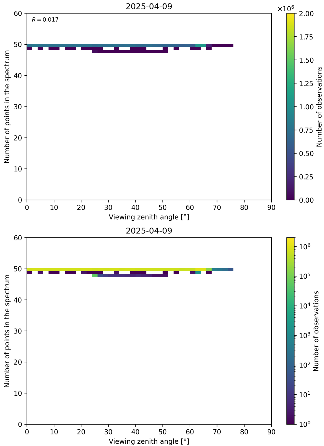
Figure 125: Scatter density plot of “Viewing zenith angle” against “Number of points in the spectrum” for 2025-04-08 to 2025-04-10.
