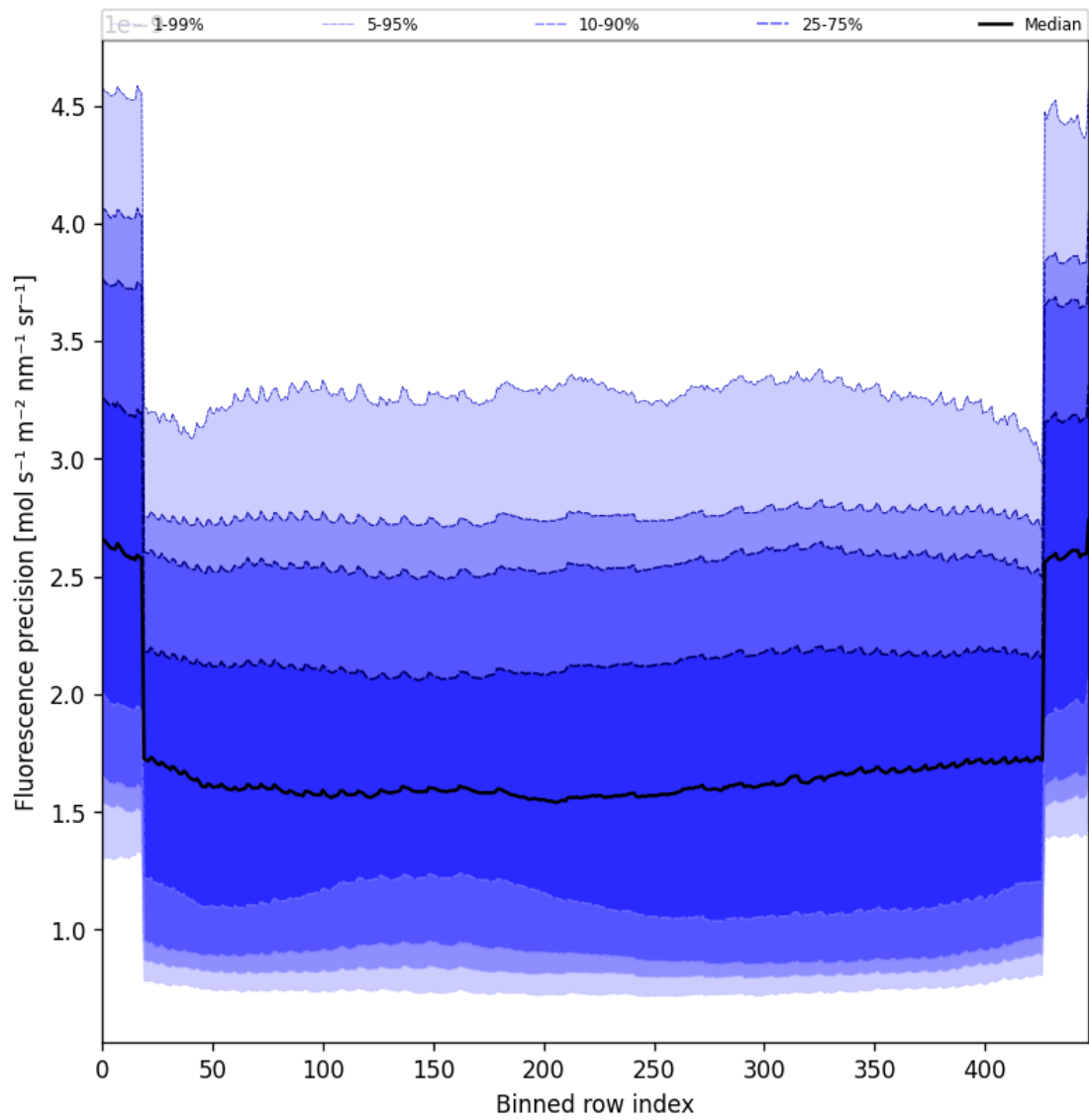
Figure 58: Along track statistics of “Fluorescence precision” for 2025-04-08 to 2025-04-10
