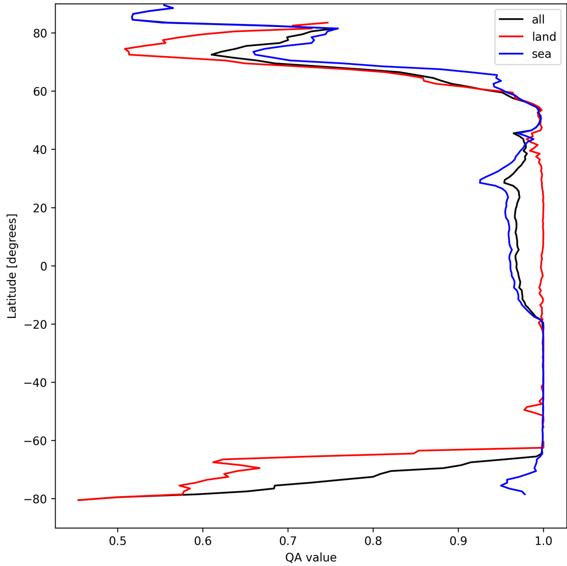
Figure 12: Zonal average of “QA value” for 2025-04-08 to 2025-04-10.
