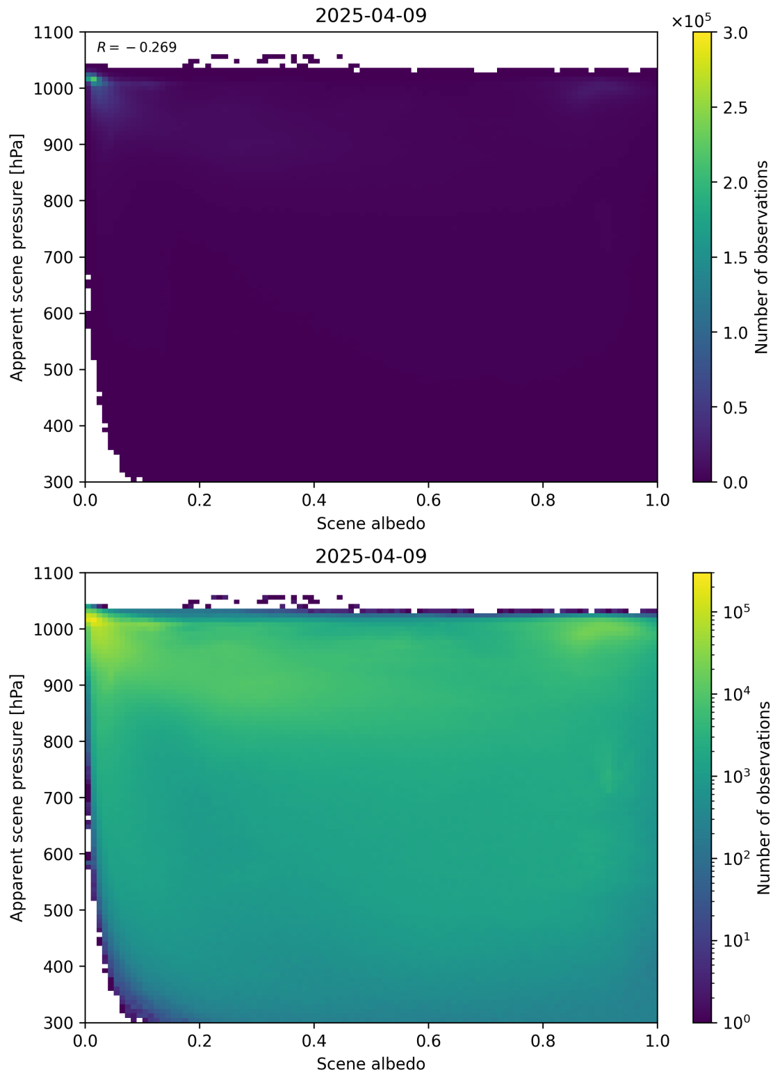
Figure 102: Scatter density plot of “Scene albedo” against “Apparent scene pressure” for 2025-04-08 to 2025-04-10.
