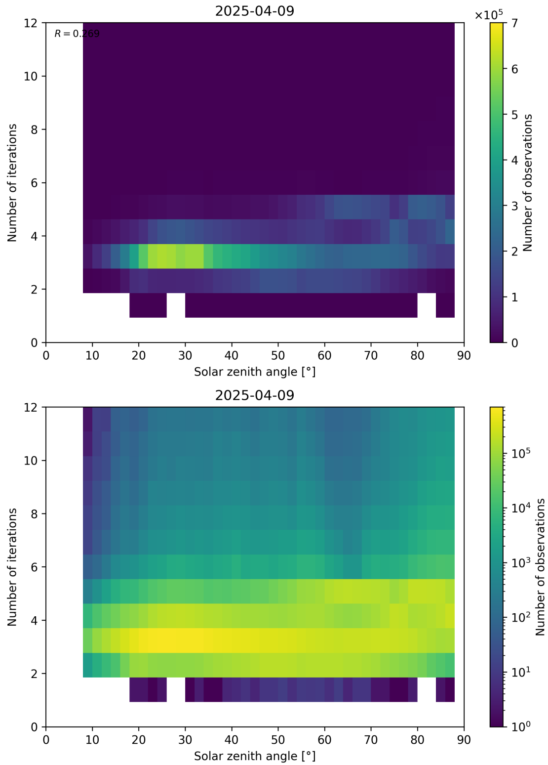
Figure 114: Scatter density plot of “Solar zenith angle” against “Number of iterations” for 2025-04-08 to 2025-04-10.
