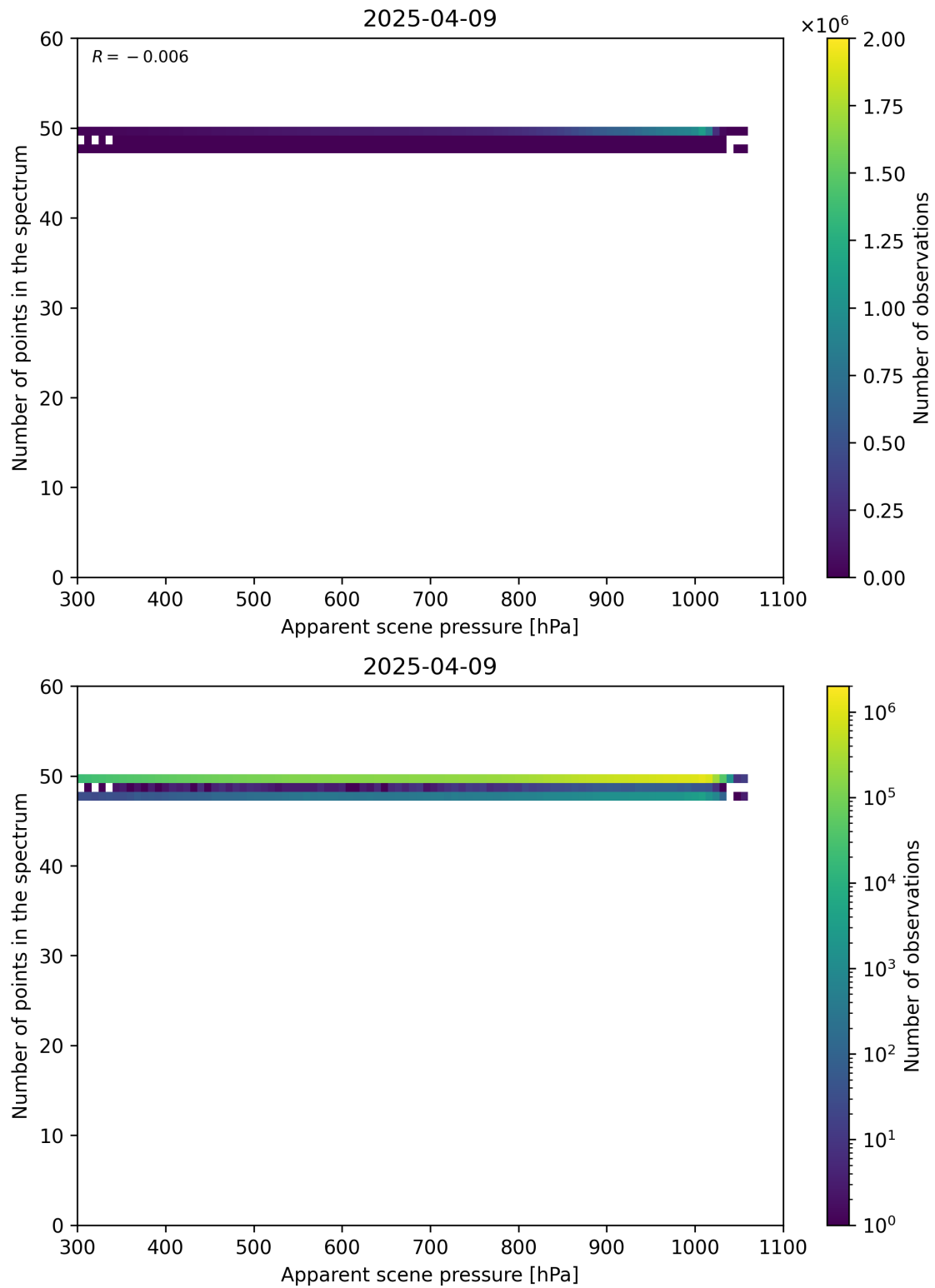
Figure 66: Scatter density plot of “Apparent scene pressure” against “Number of points in the spectrum” for 2025-04-08 to 2025-04-10.
