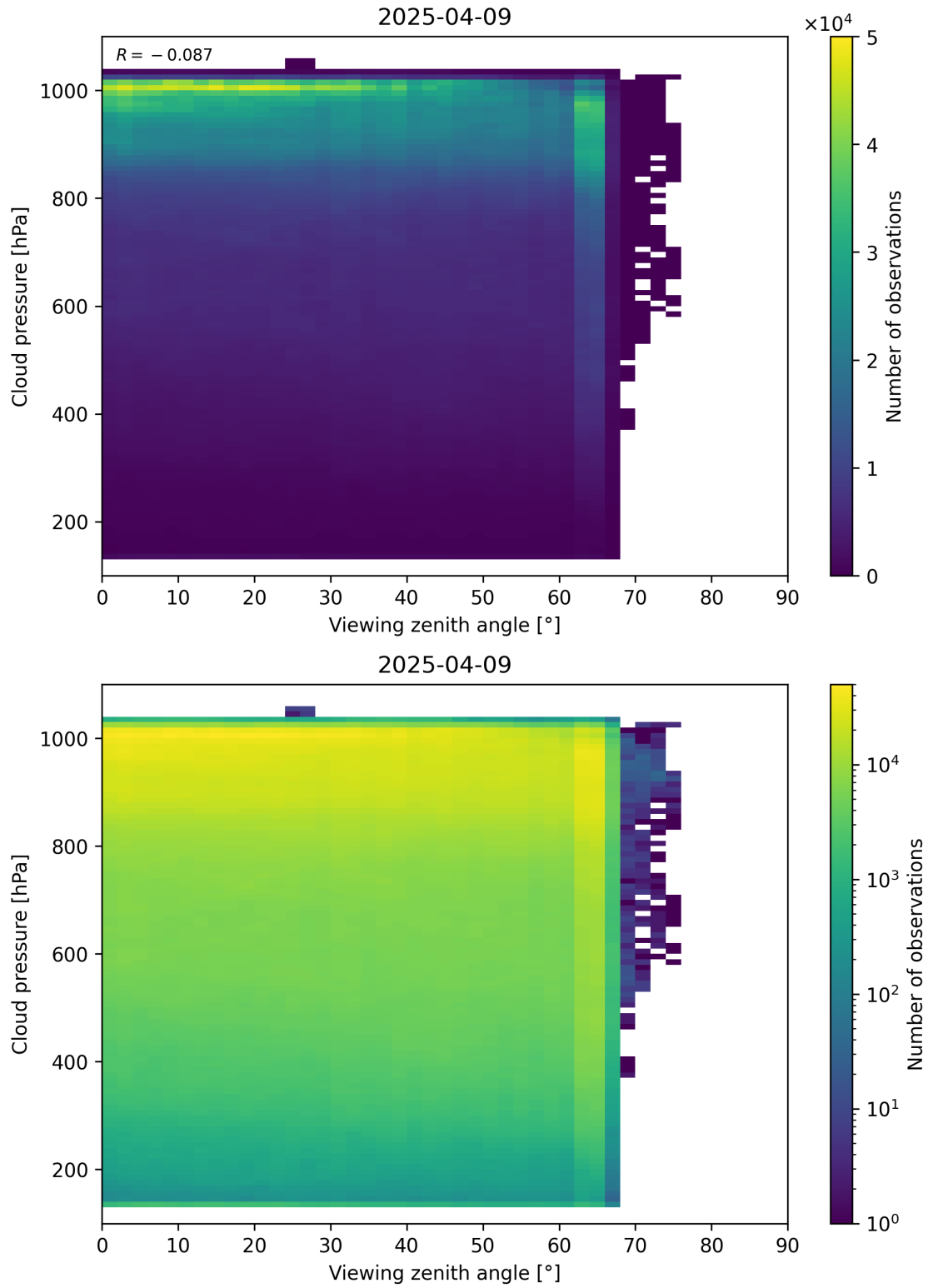
Figure 121: Scatter density plot of “Viewing zenith angle” against “Cloud pressure” for 2025-04-08 to 2025-04-10.
