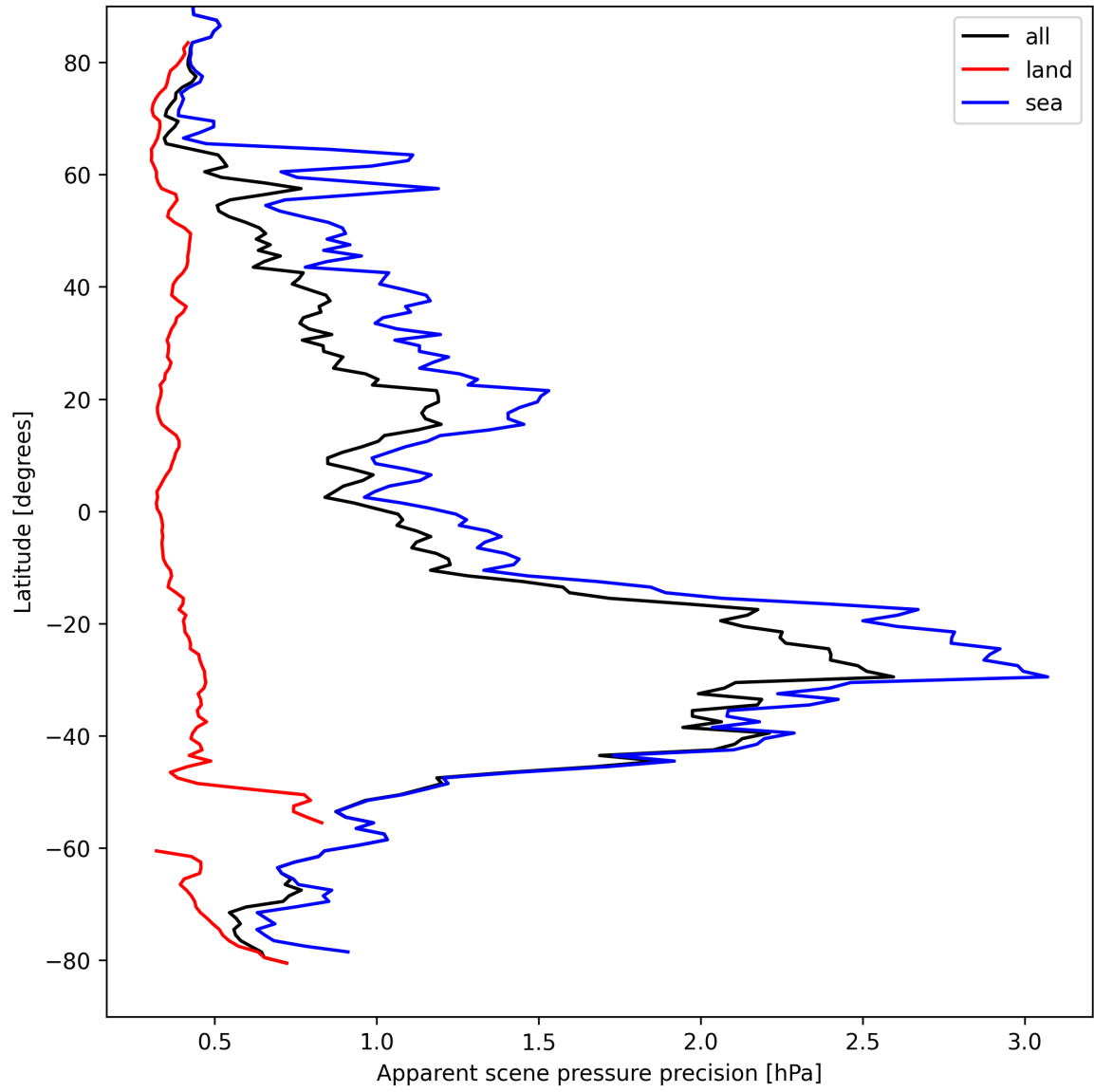
Figure 20: Zonal average of “Apparent scene pressure precision” for 2025-04-08 to 2025-04-10.
