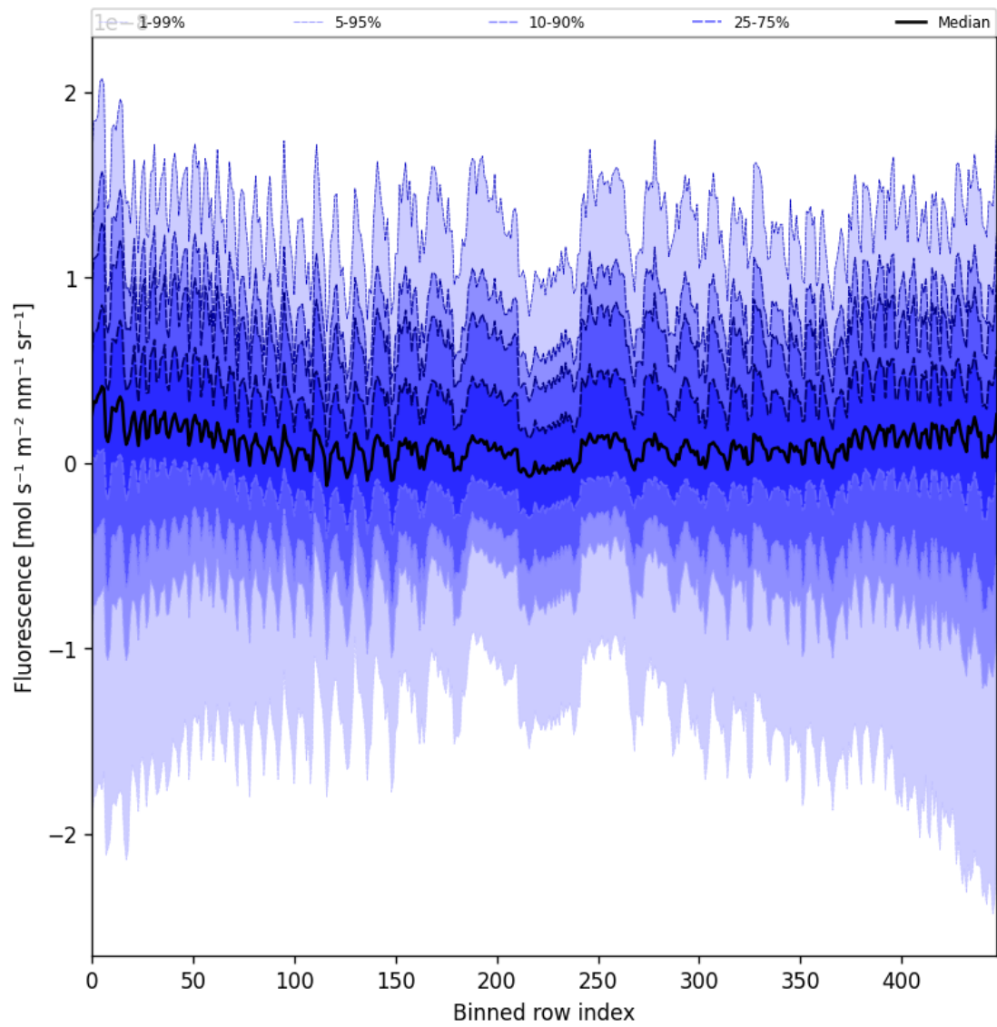
Figure 57: Along track statistics of “Fluorescence” for 2025-04-08 to 2025-04-10
