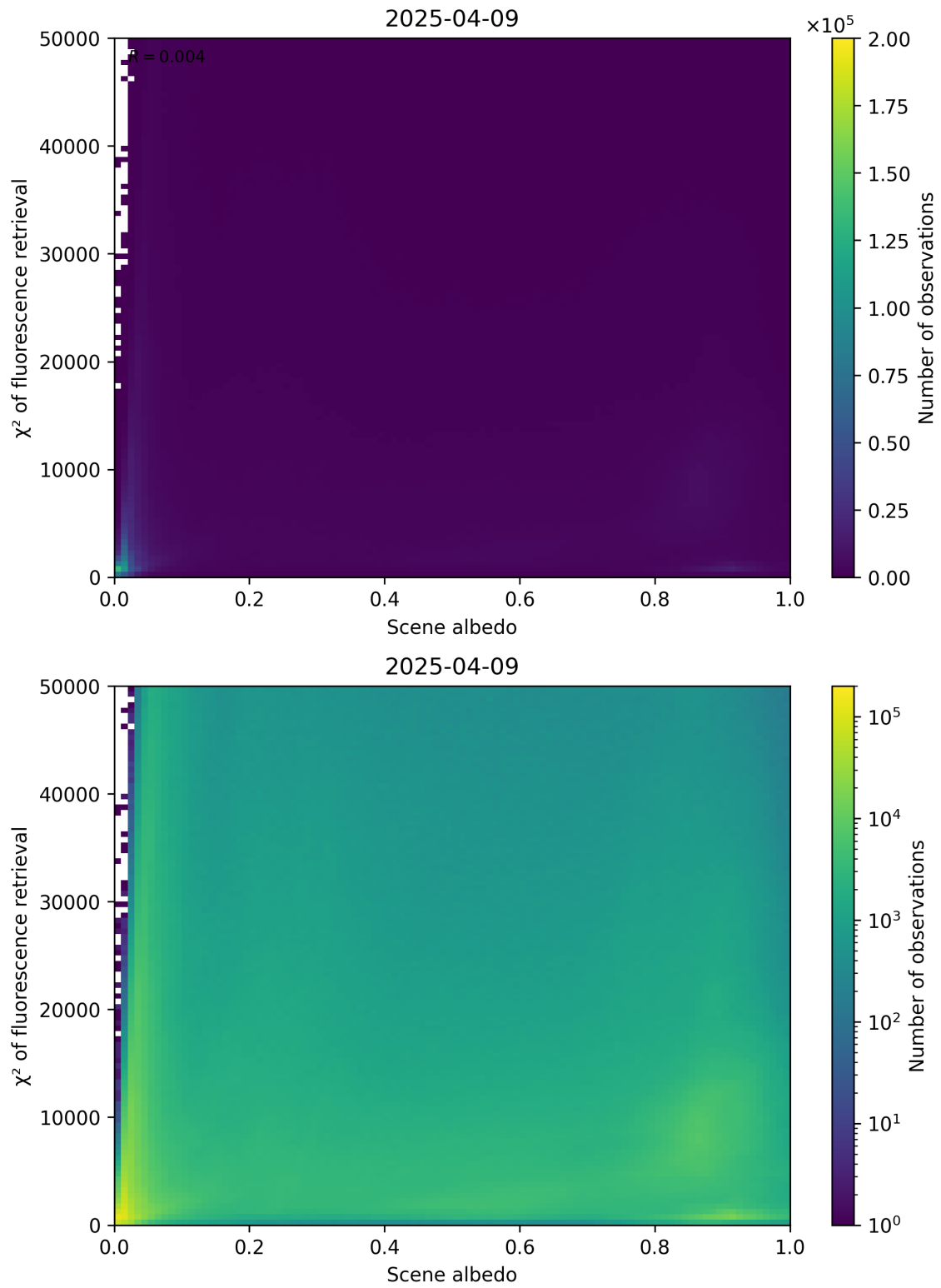
Figure 103: Scatter density plot of “Scene albedo” against “ \chi^2 of fluorescence retrieval” for 2025-04-08 to 2025-04-10.
