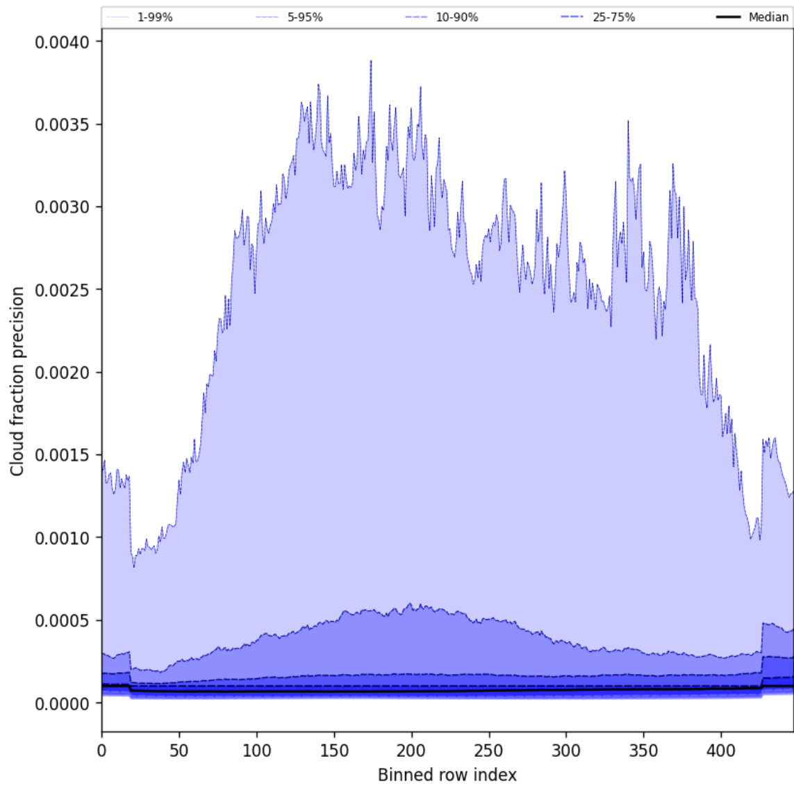
Figure 50: Along track statistics of “Cloud fraction precision” for 2025-04-08 to 2025-04-10
