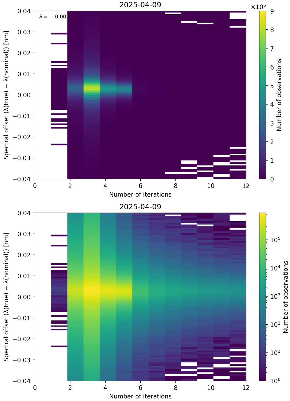
Figure 100: Scatter density plot of “Number of iterations” against “Spectral offset ( \lambda_{\text{true}} - \lambda_{\text{nominal}} )” for 2025-04-08 to 2025-04-10.
