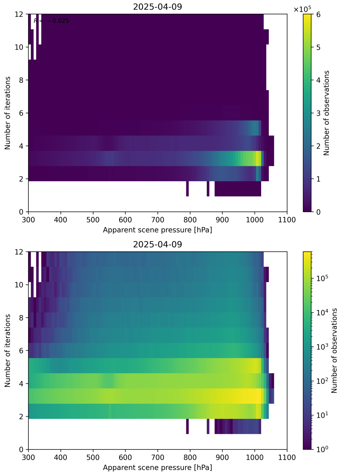
Figure 65: Scatter density plot of “Apparent scene pressure” against “Number of iterations” for 2025-04-08 to 2025-04-10.
