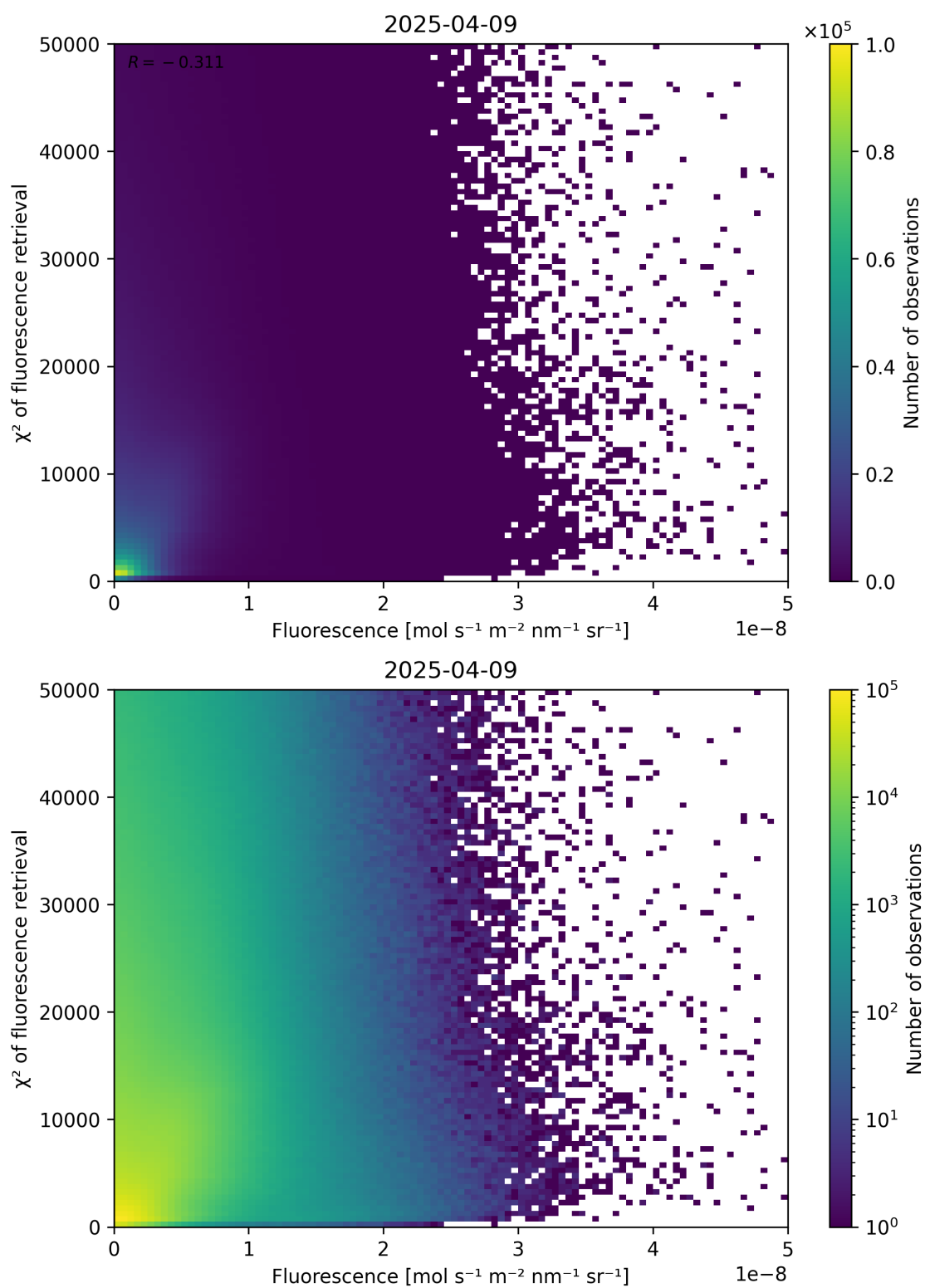
Figure 85: Scatter density plot of “Fluorescence” against “ \chi^2 of fluorescence retrieval” for 2025-04-08 to 2025-04-10.
