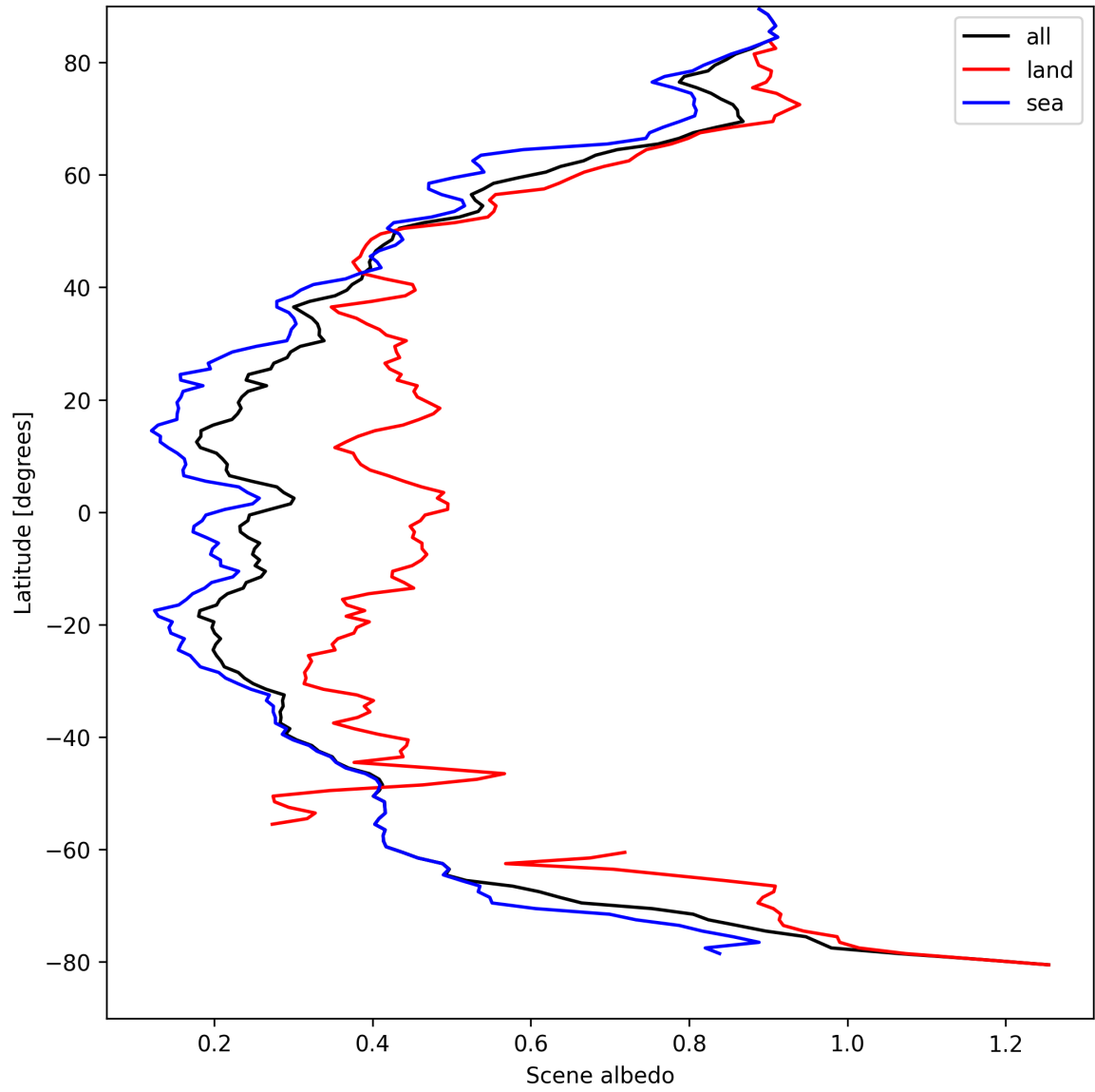
Figure 17: Zonal average of “Scene albedo” for 2025-04-08 to 2025-04-10.
