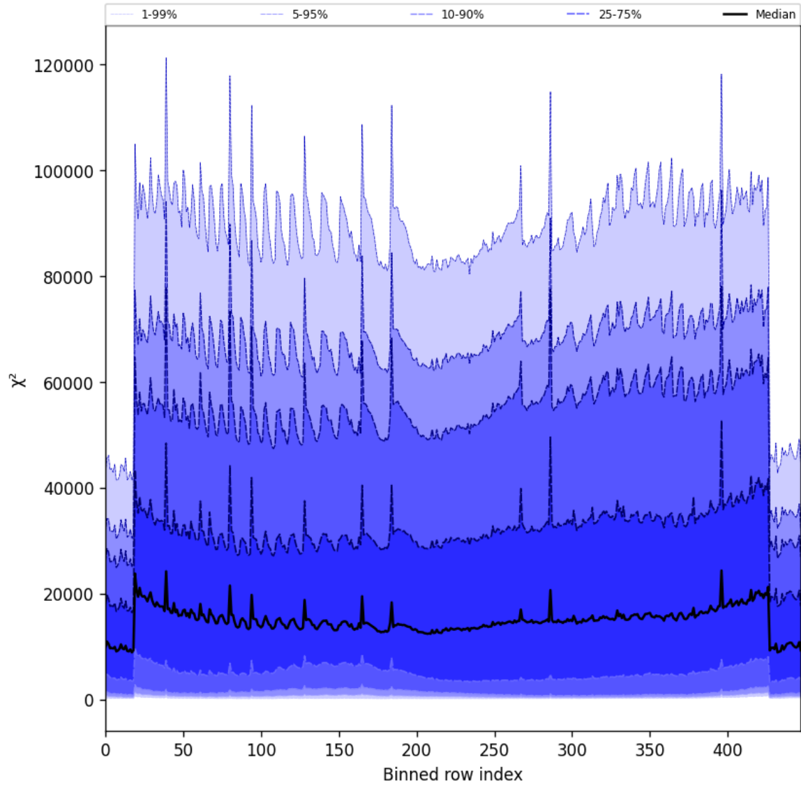
Figure 55: Along track statistics of “ \chi^2 ” for 2025-04-08 to 2025-04-10
