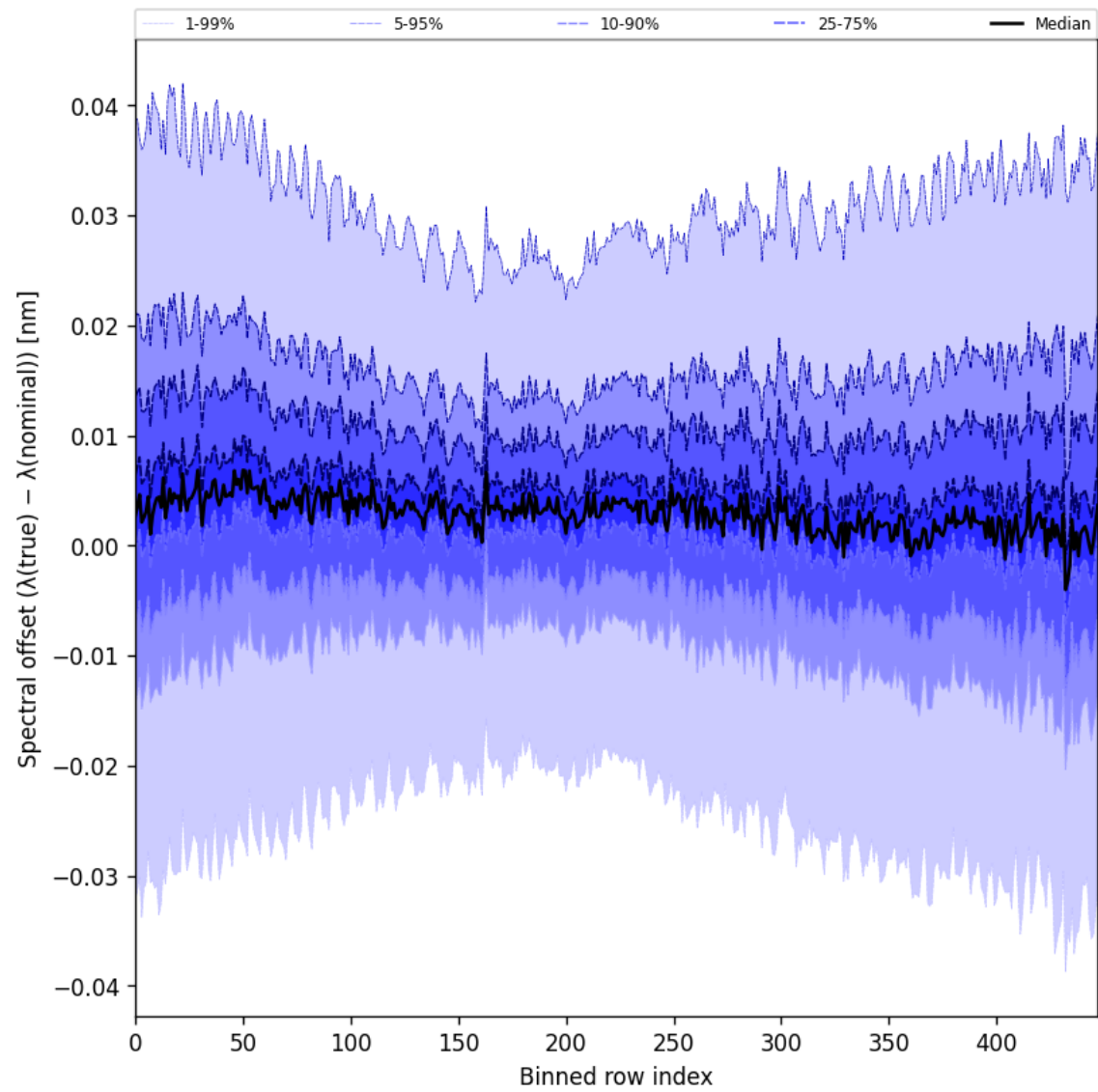
Figure 62: Along track statistics of “Spectral offset ( \lambda_{\text{true}} - \lambda_{\text{nominal}} )” for 2025-04-08 to 2025-04-10
