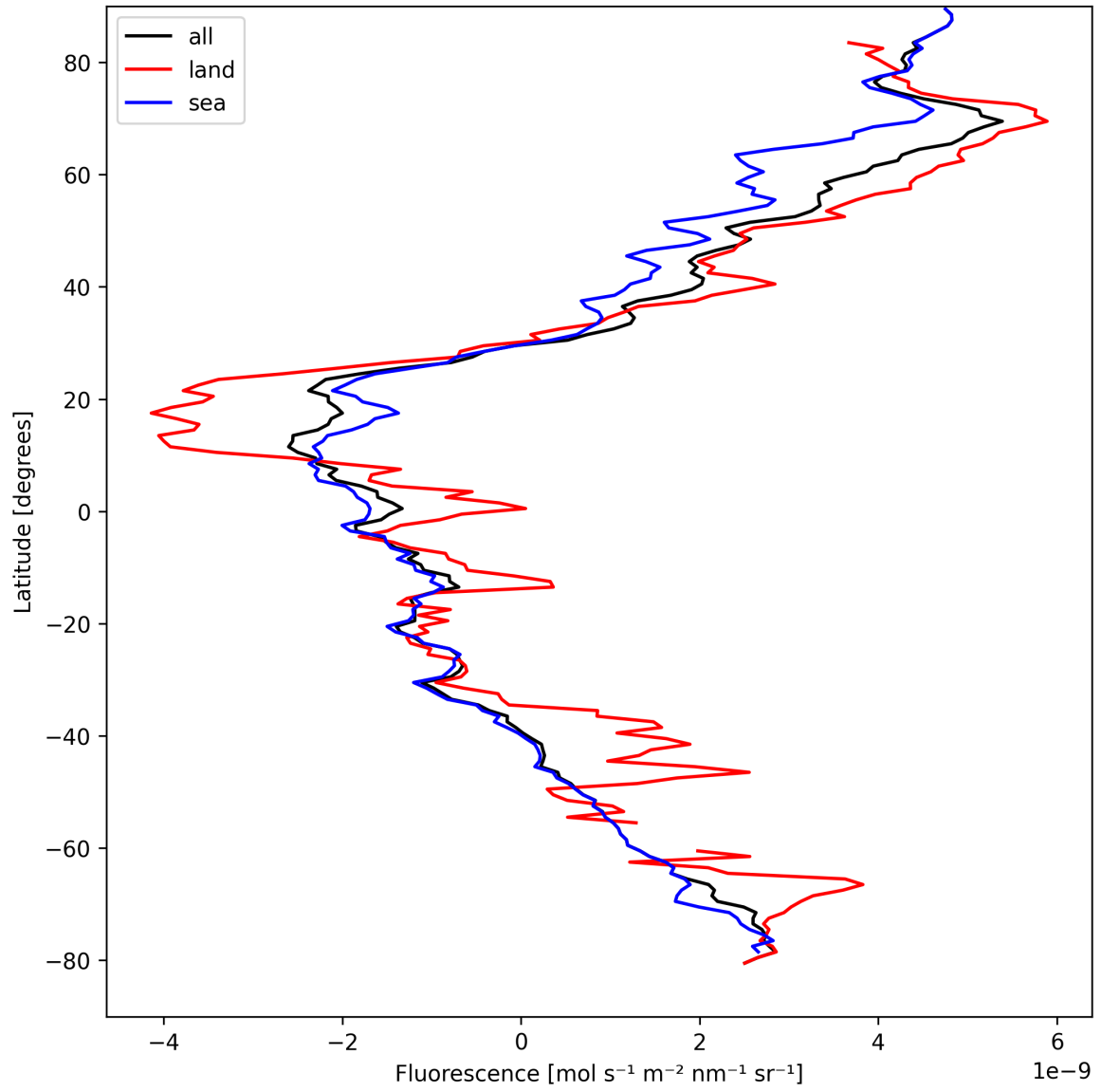
Figure 23: Zonal average of “Fluorescence” for 2025-04-08 to 2025-04-10.
