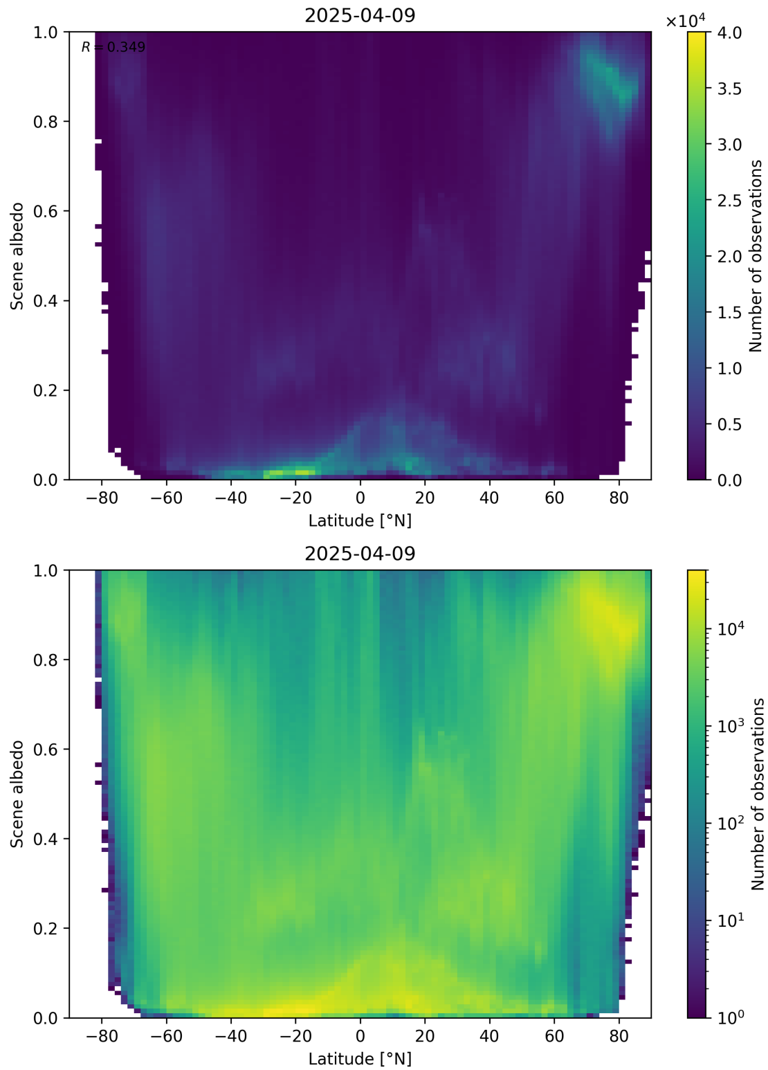
Figure 95: Scatter density plot of “Latitude” against “Scene albedo” for 2025-04-08 to 2025-04-10.
