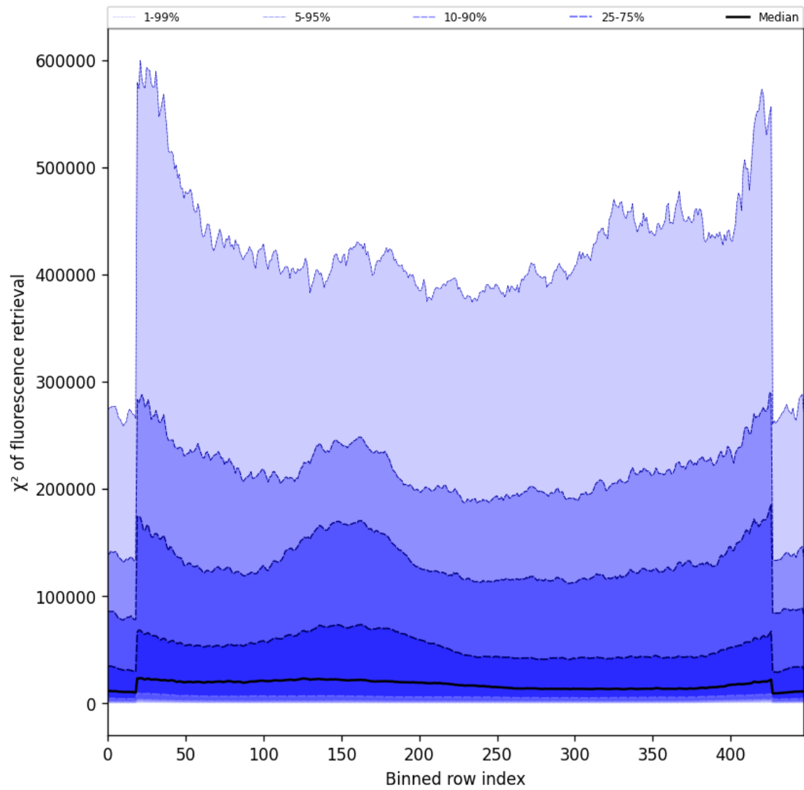
Figure 59: Along track statistics of “ \chi^2 of fluorescence retrieval” for 2025-04-08 to 2025-04-10
