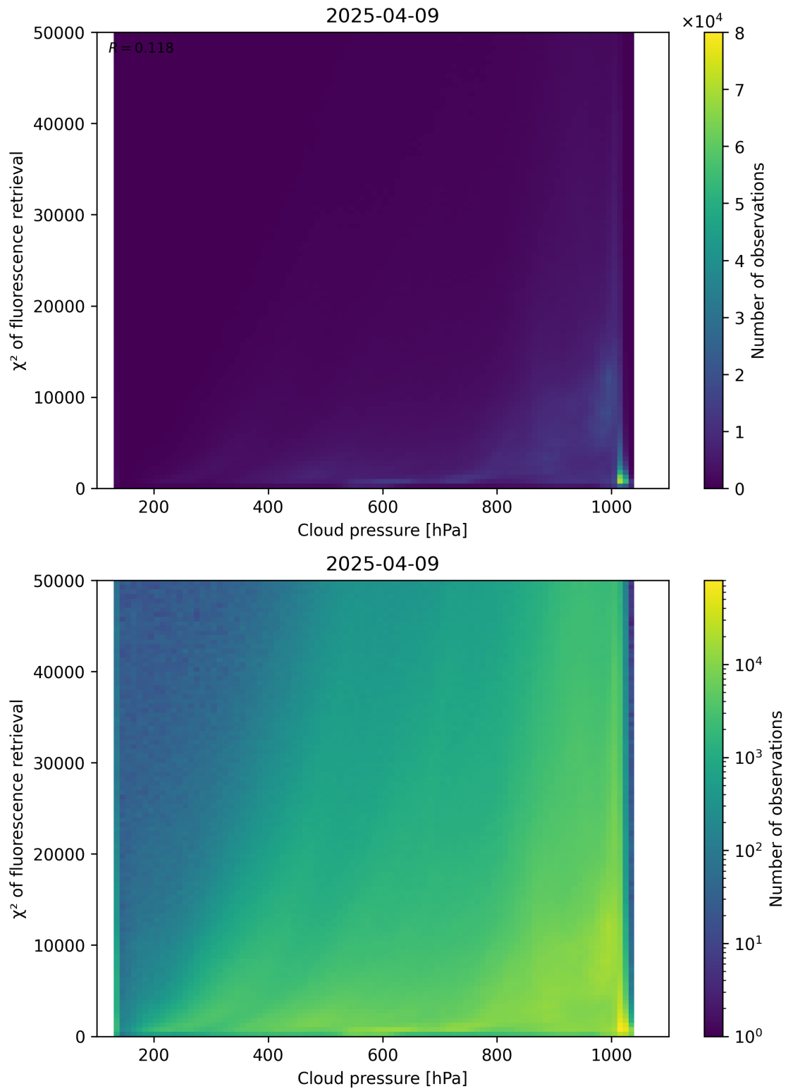
Figure 78: Scatter density plot of “Cloud pressure” against “ \chi^2 of fluorescence retrieval” for 2025-04-08 to 2025-04-10.
