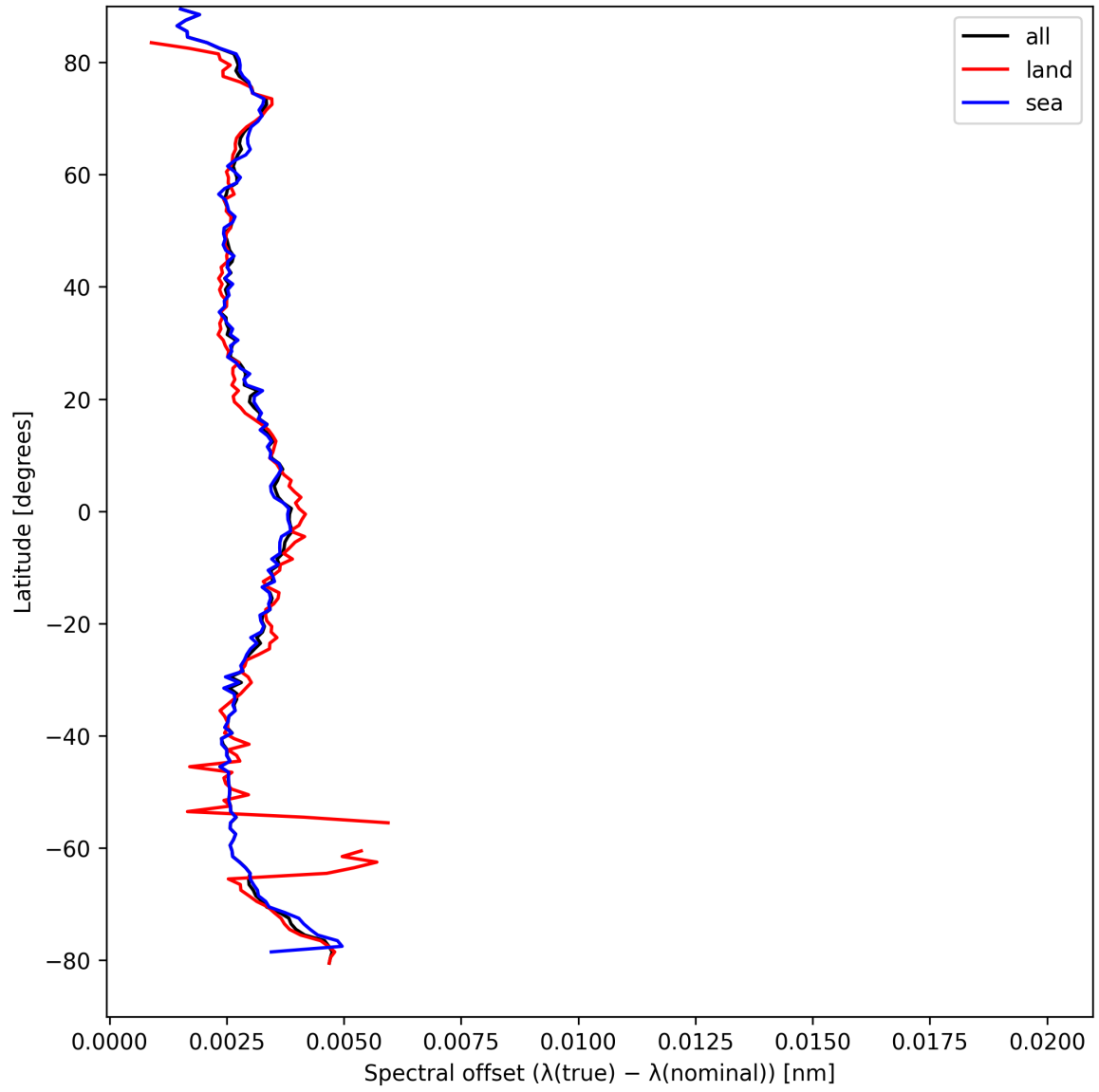
Figure 28: Zonal average of “Spectral offset ( \lambda_{\text{true}} - \lambda_{\text{nominal}} )” for 2025-04-08 to 2025-04-10.
