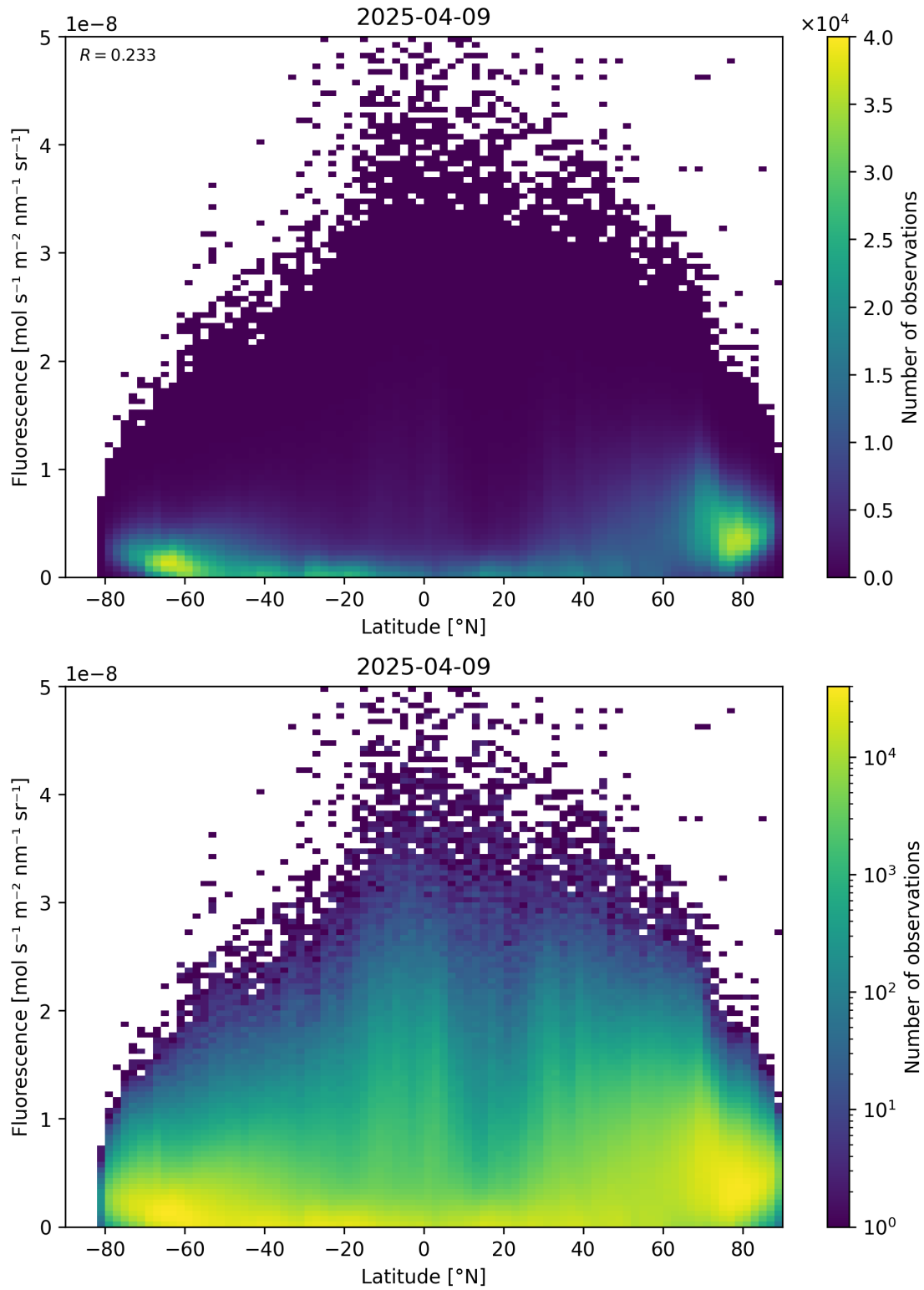
Figure 92: Scatter density plot of “Latitude” against “Fluorescence” for 2025-04-08 to 2025-04-10.
