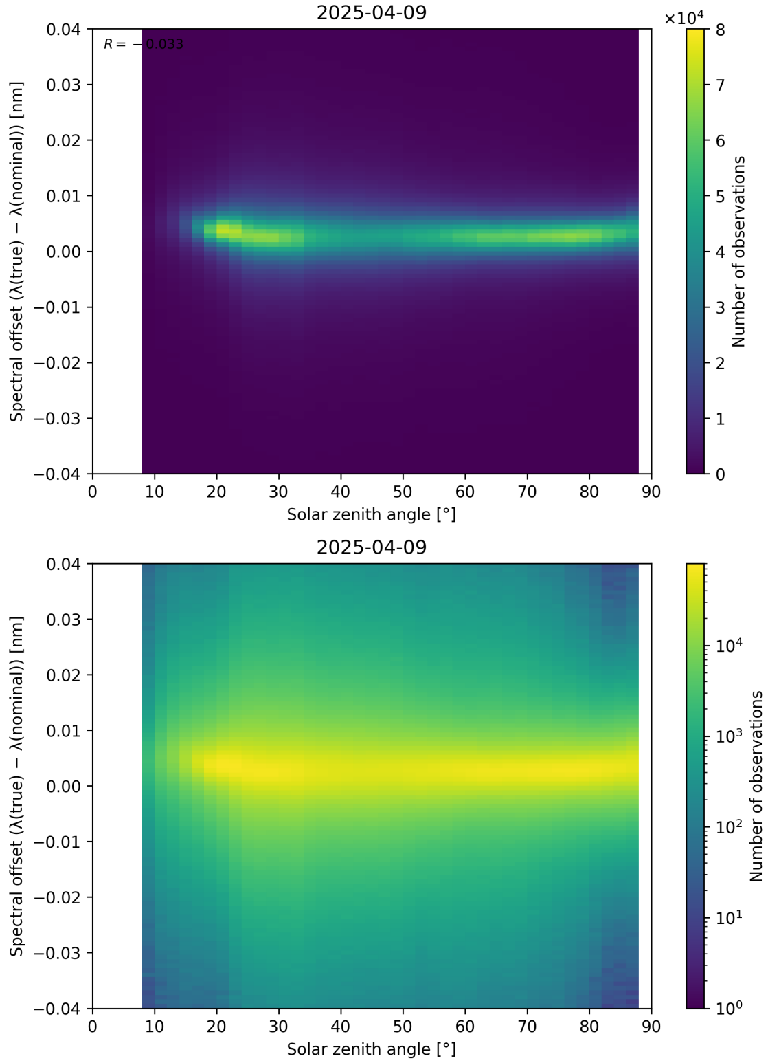
Figure 117: Scatter density plot of “Solar zenith angle” against “Spectral offset ( \lambda_{\text{true}} - \lambda_{\text{nominal}} )” for 2025-04-08 to 2025-04-10.
