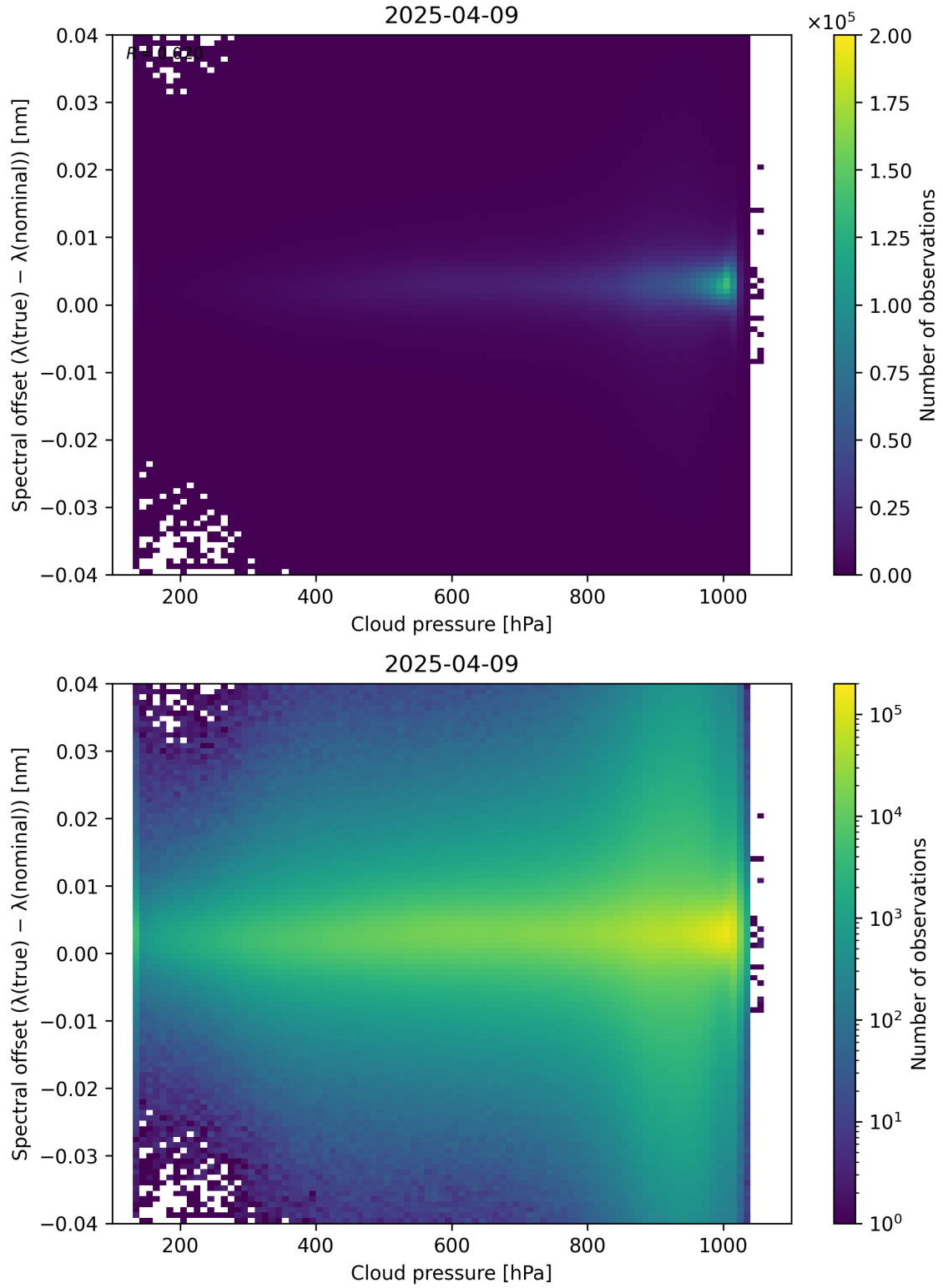
Figure 84: Scatter density plot of “Cloud pressure” against “Spectral offset ( \lambda_{\text{true}} - \lambda_{\text{nominal}} )” for 2025-04-08 to 2025-04-10.
