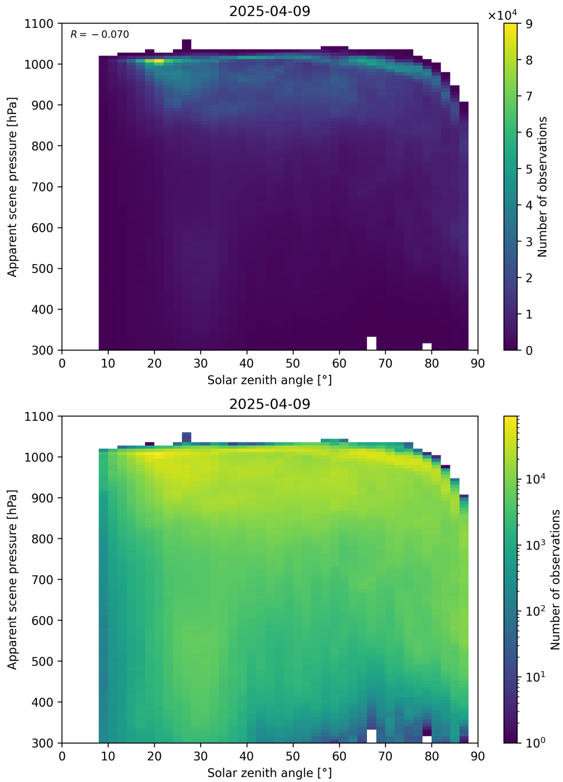
Figure 108: Scatter density plot of “Solar zenith angle” against “Apparent scene pressure” for 2025-04-08 to 2025-04-10.
