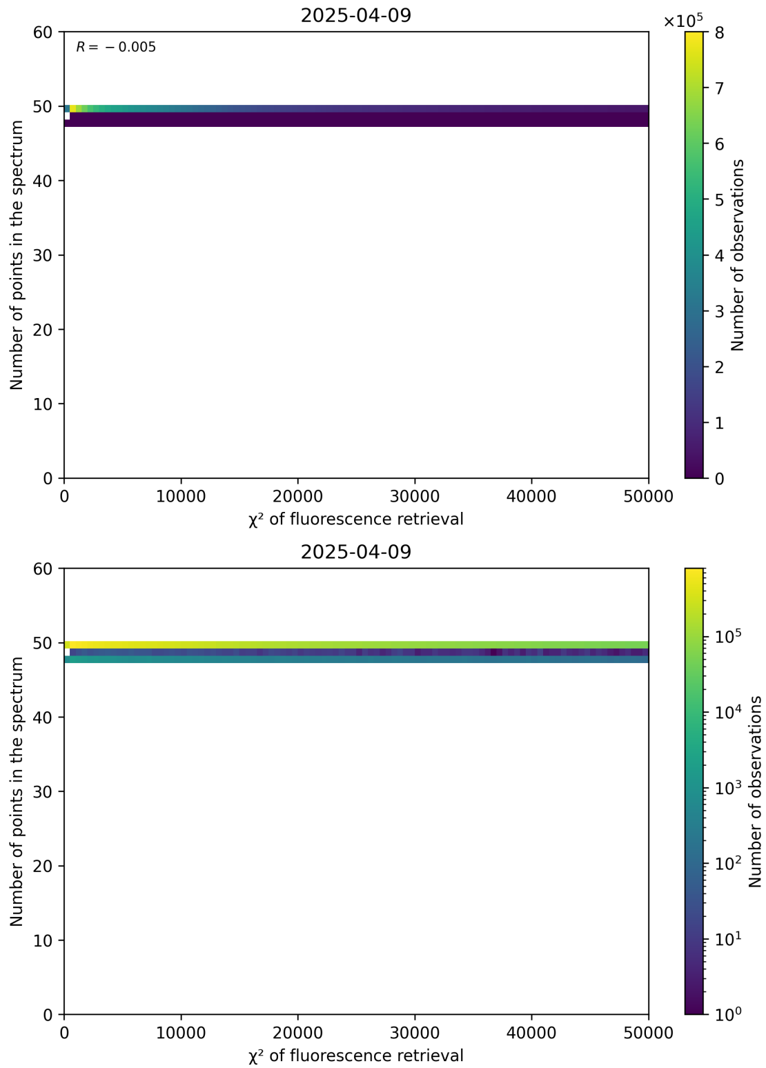
Figure 68: Scatter density plot of “ \chi^2 of fluorescence retrieval” against “Number of points in the spectrum” for 2025-04-08 to 2025-04-10.
