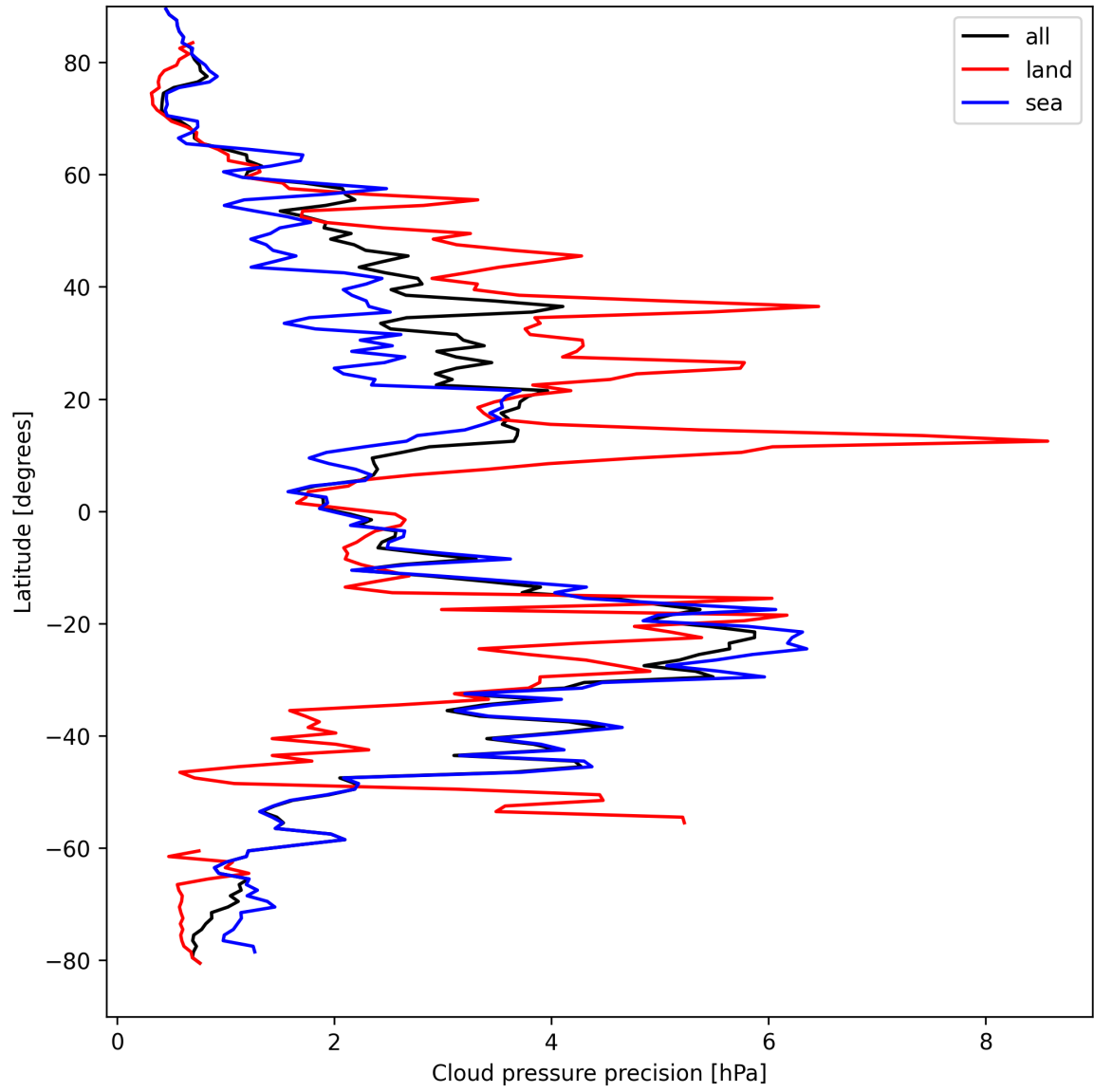
Figure 14: Zonal average of “Cloud pressure precision” for 2025-04-08 to 2025-04-10.
