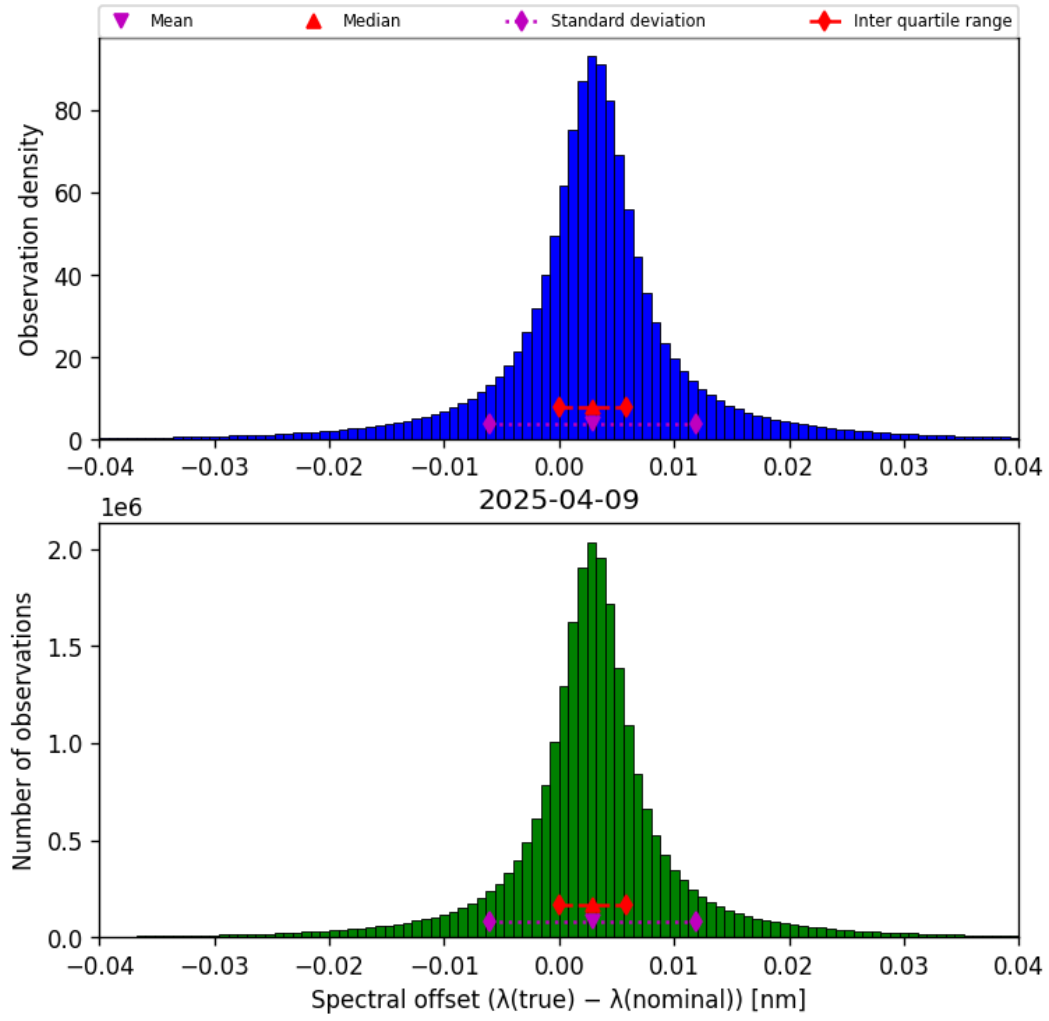
Figure 45: Histogram of “Spectral offset ( \lambda_{\text{true}} - \lambda_{\text{nominal}} )” for 2025-04-08 to 2025-04-10
