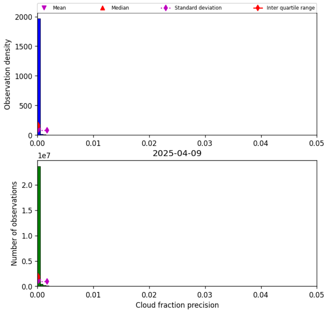
Figure 33: Histogram of “Cloud fraction precision” for 2025-04-08 to 2025-04-10
