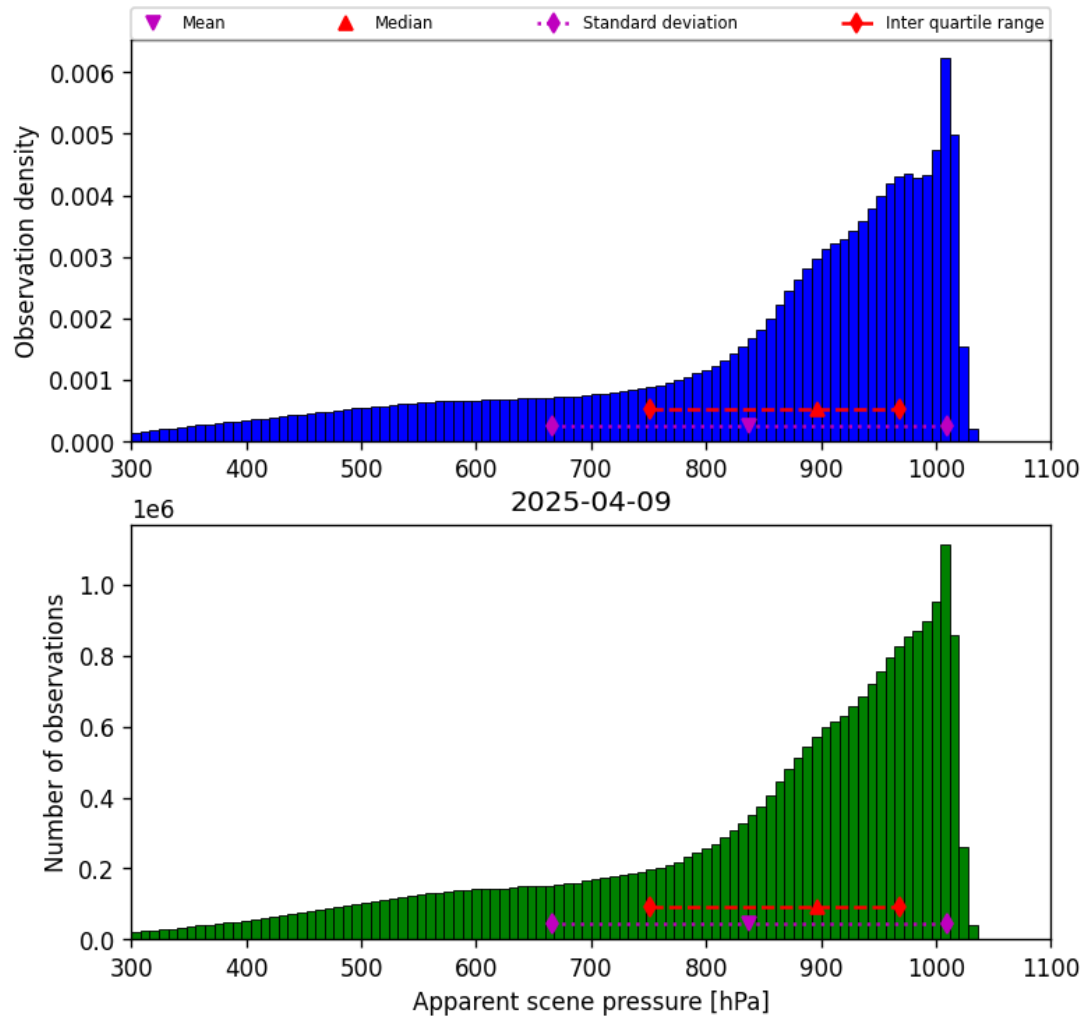
Figure 36: Histogram of “Apparent scene pressure” for 2025-04-08 to 2025-04-10
