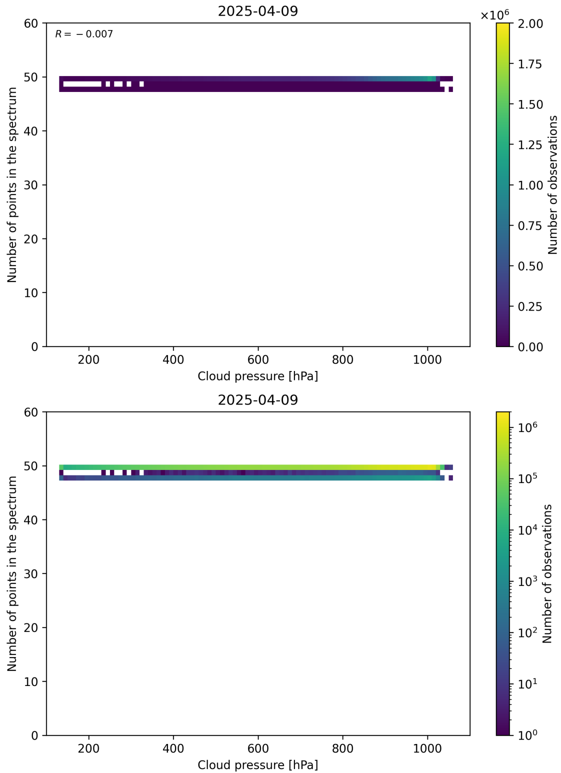
Figure 82: Scatter density plot of “Cloud pressure” against “Number of points in the spectrum” for 2025-04-08 to 2025-04-10.
