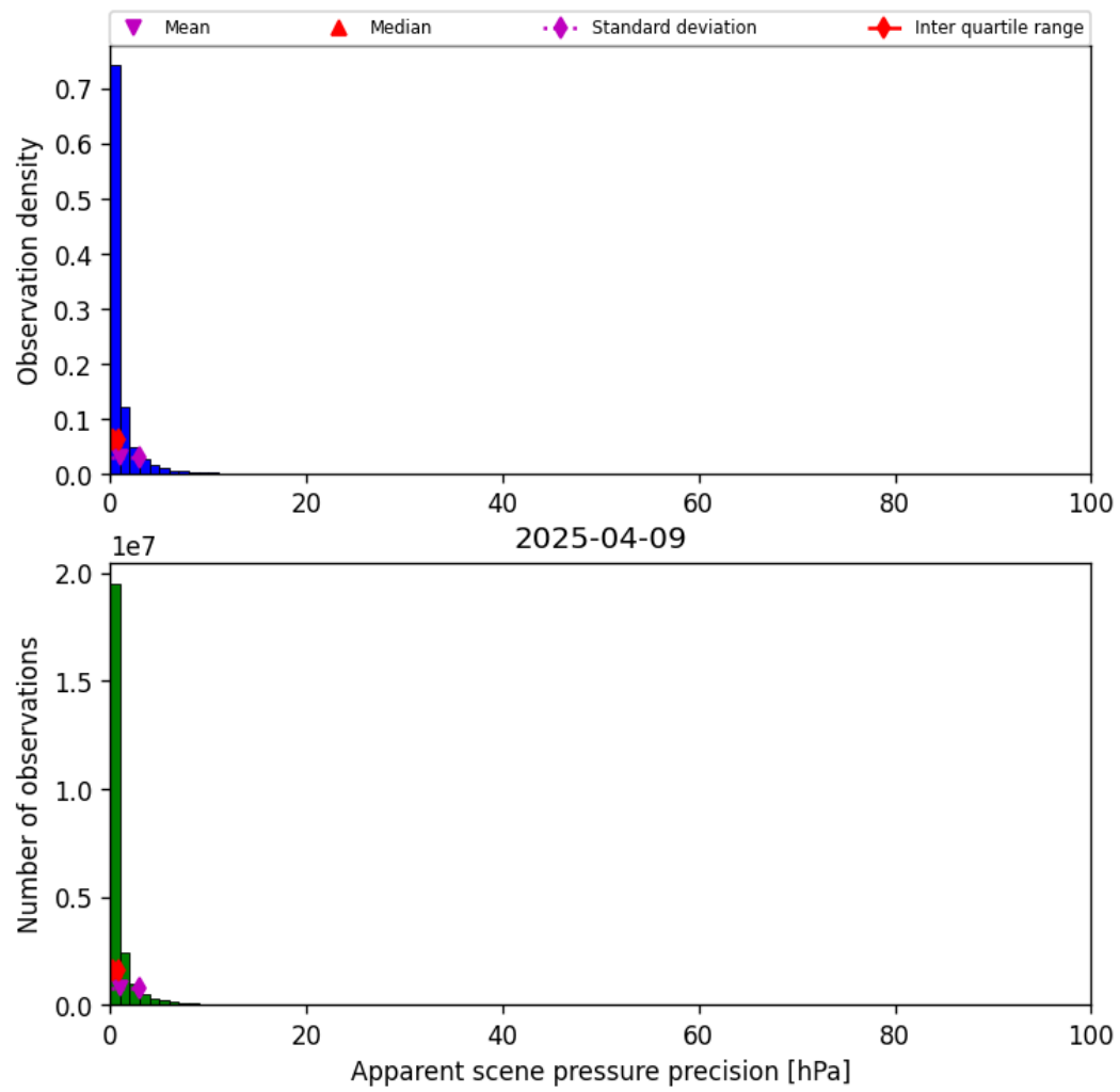
Figure 37: Histogram of “Apparent scene pressure precision” for 2025-04-08 to 2025-04-10
