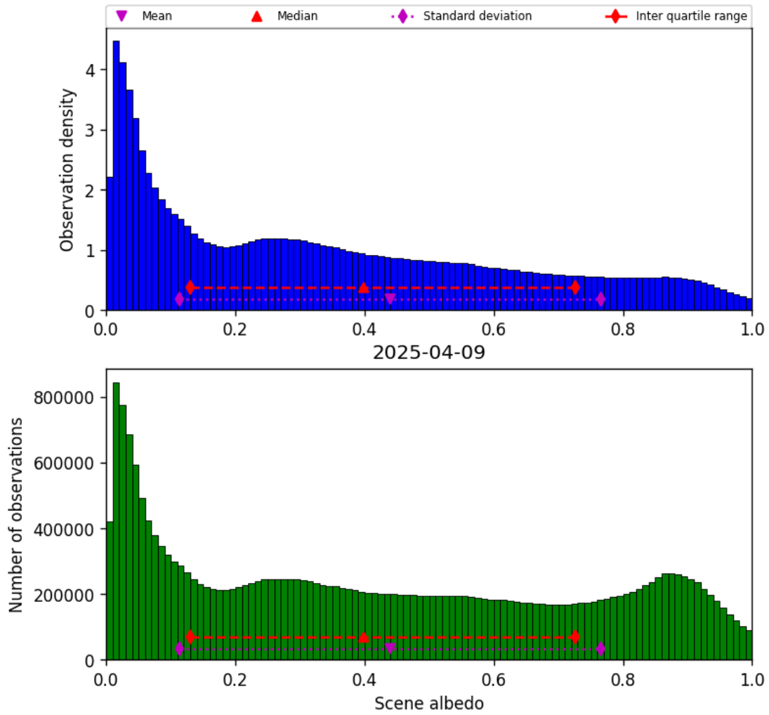
Figure 34: Histogram of “Scene albedo” for 2025-04-08 to 2025-04-10
