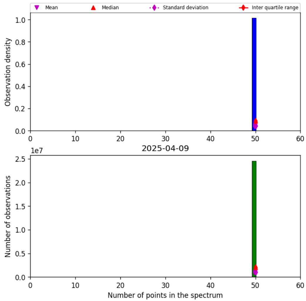
Figure 44: Histogram of “Number of points in the spectrum” for 2025-04-08 to 2025-04-10
