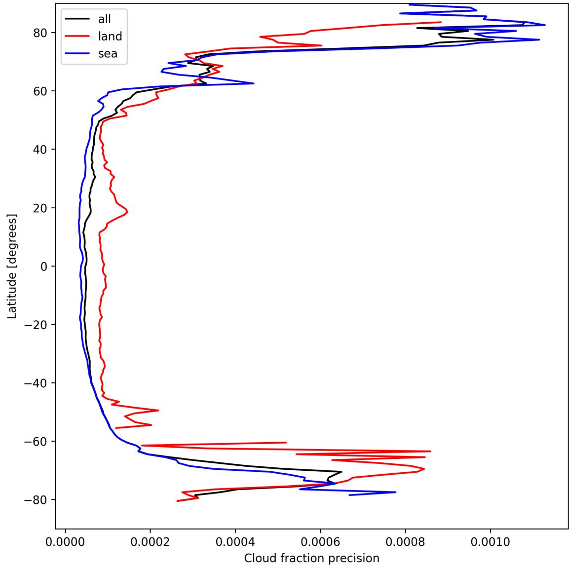
Figure 16: Zonal average of “Cloud fraction precision” for 2025-04-08 to 2025-04-10.
