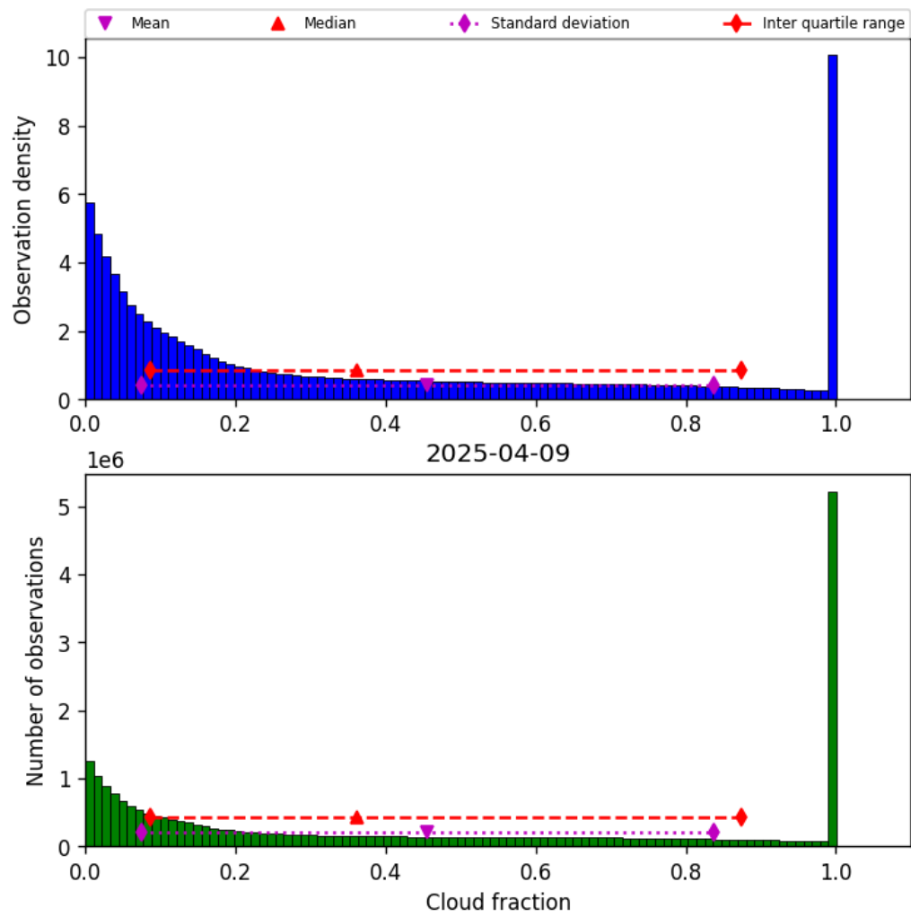
Figure 32: Histogram of “Cloud fraction” for 2025-04-08 to 2025-04-10
