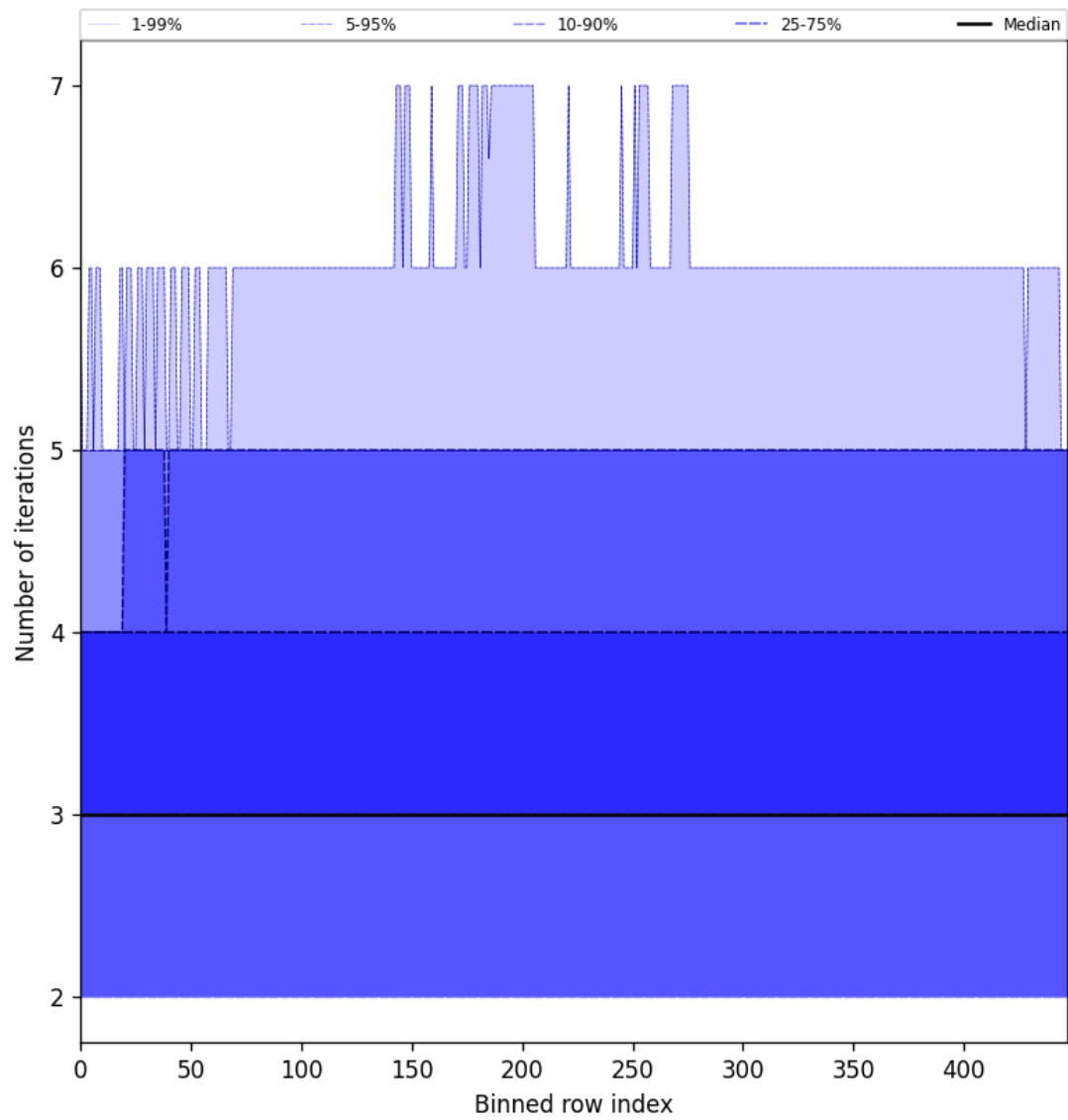
Figure 56: Along track statistics of “Number of iterations” for 2025-04-08 to 2025-04-10
