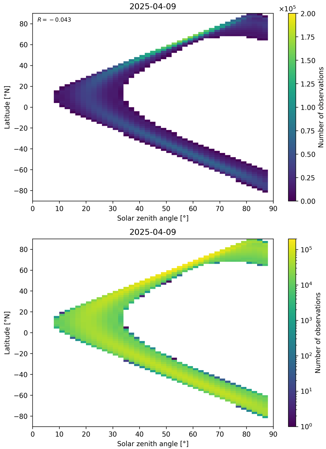
Figure 113: Scatter density plot of “Solar zenith angle” against “Latitude” for 2025-04-08 to 2025-04-10.
