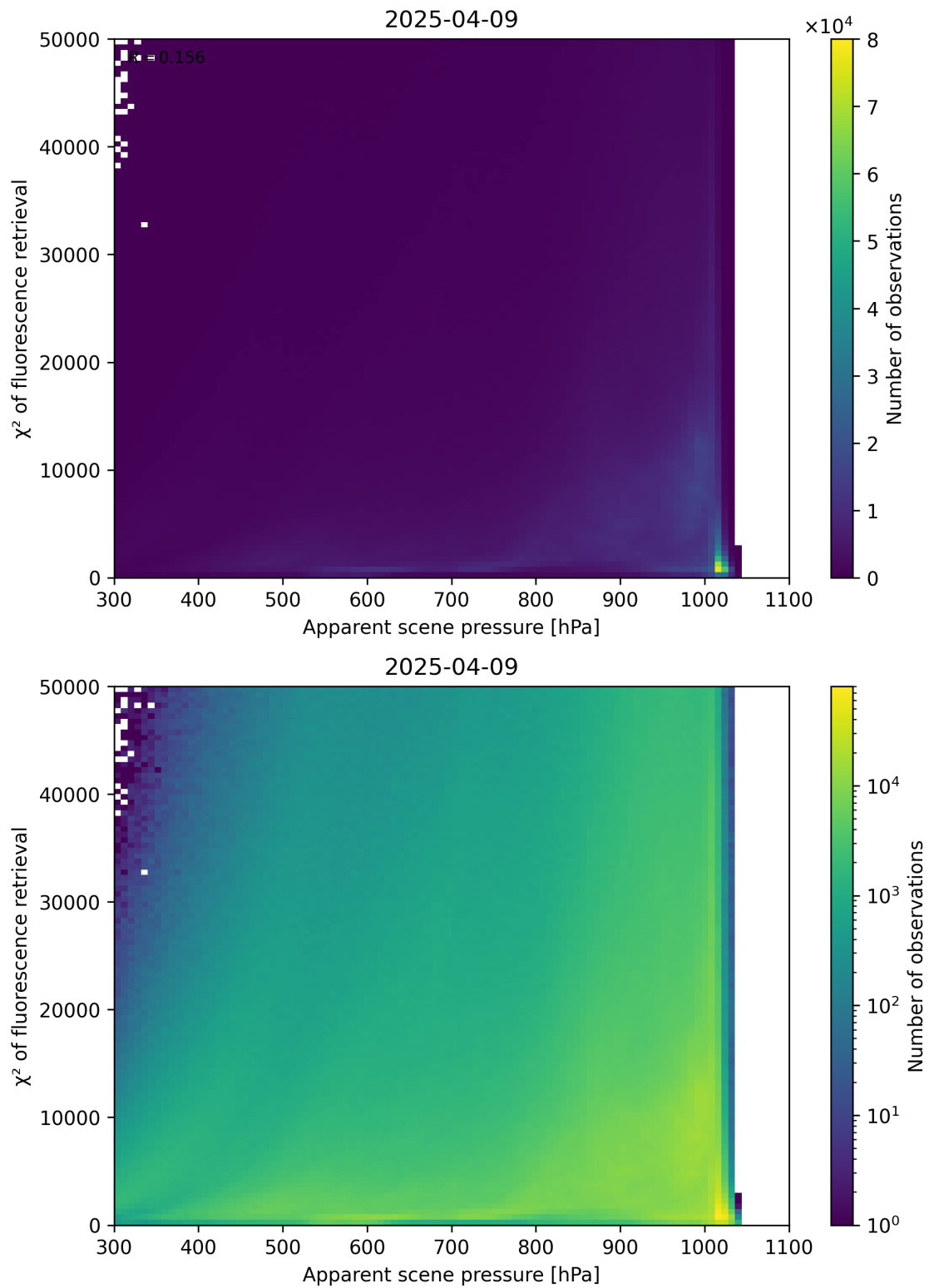
Figure 63: Scatter density plot of “Apparent scene pressure” against “ \chi^2 of fluorescence retrieval” for 2025-04-08 to 2025-04-10.
