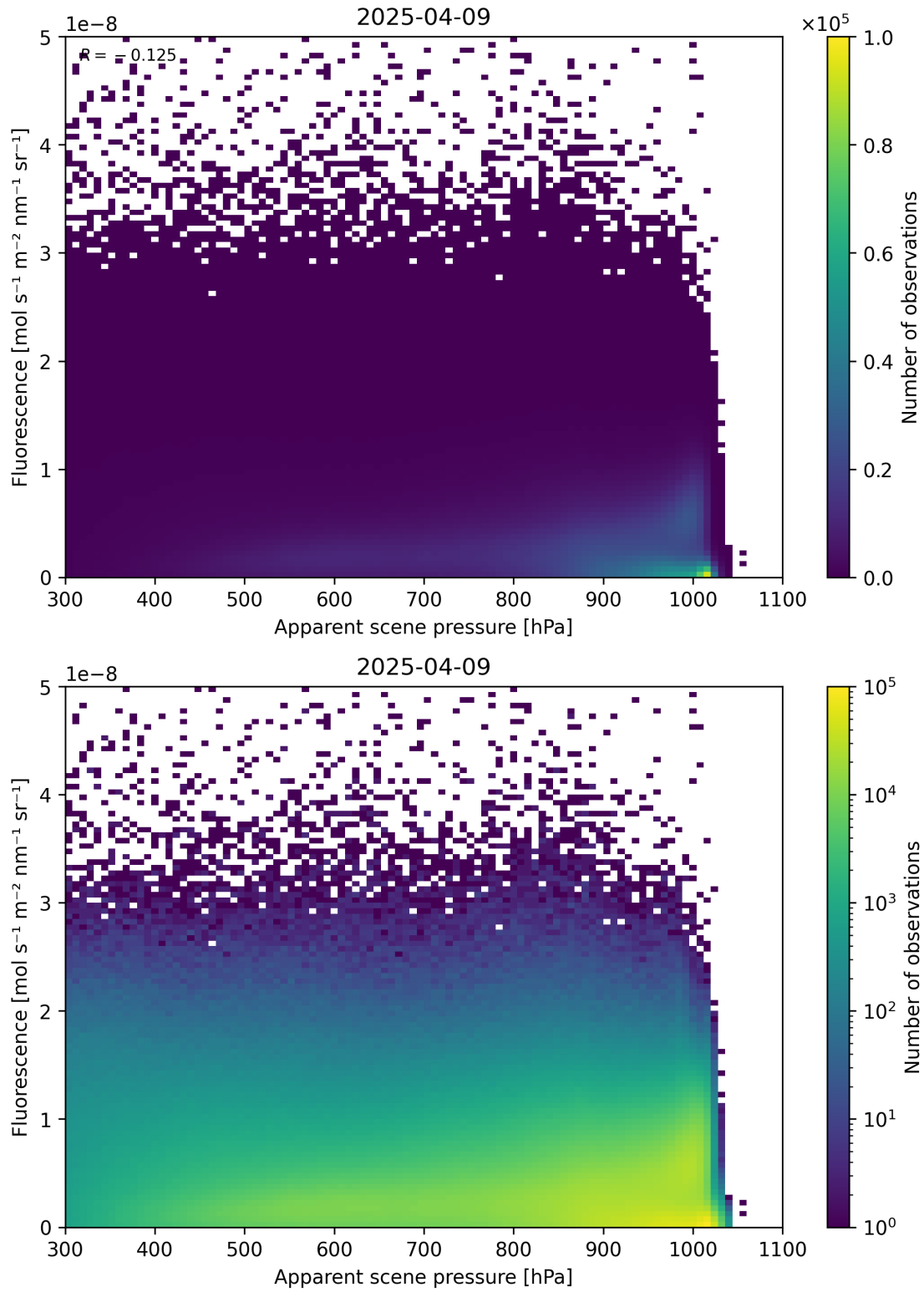
Figure 64: Scatter density plot of “Apparent scene pressure” against “Fluorescence” for 2025-04-08 to 2025-04-10.
