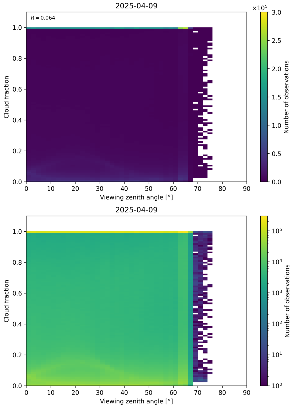
Figure 120: Scatter density plot of “Viewing zenith angle” against “Cloud fraction” for 2025-04-08 to 2025-04-10.
