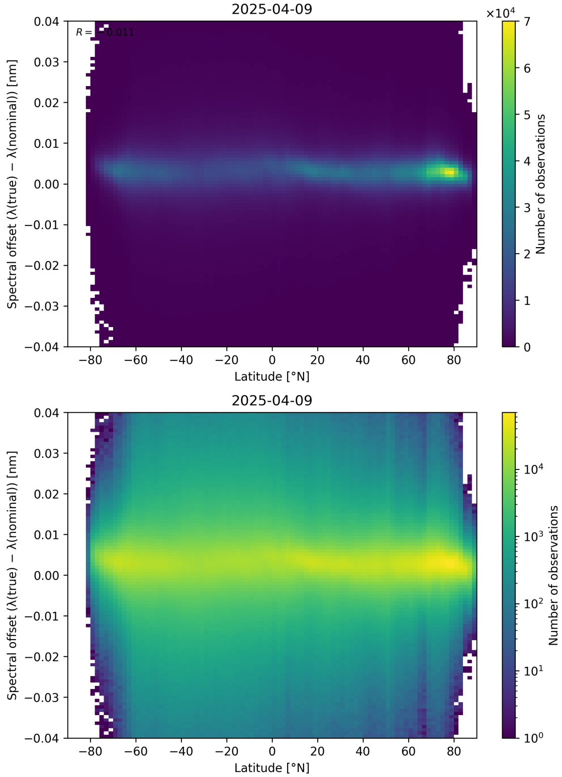
Figure 96: Scatter density plot of “Latitude” against “Spectral offset ( \lambda_{\text{true}} - \lambda_{\text{nominal}} )” for 2025-04-08 to 2025-04-10.
