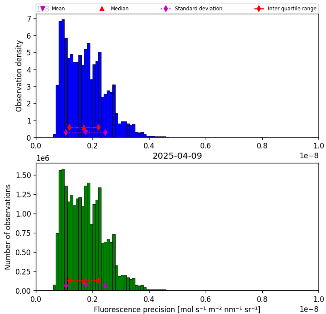
Figure 41: Histogram of “Fluorescence precision” for 2025-04-08 to 2025-04-10
