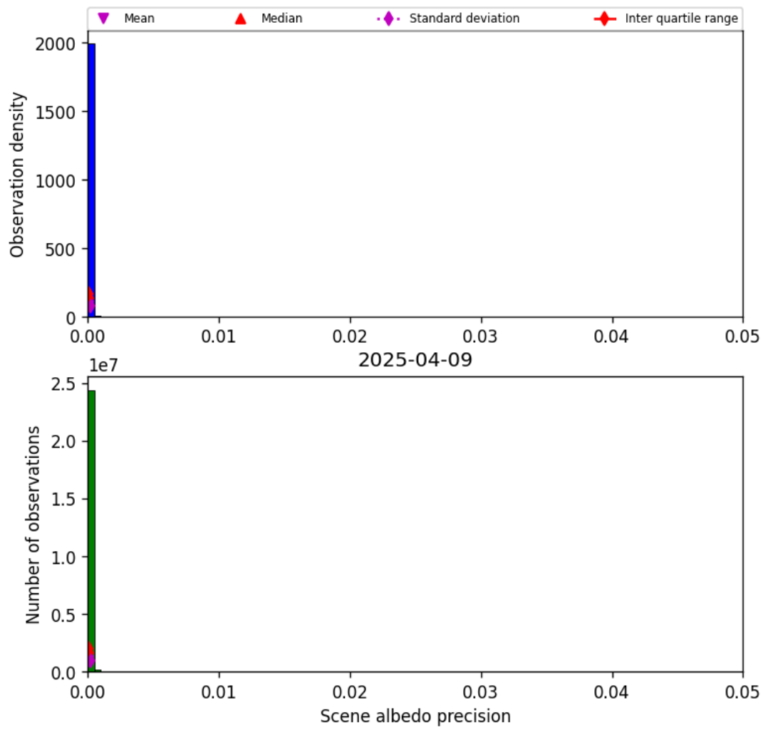
Figure 35: Histogram of “Scene albedo precision” for 2025-04-08 to 2025-04-10
