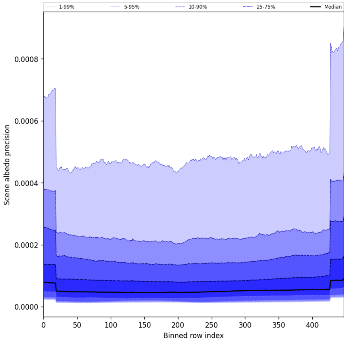
Figure 52: Along track statistics of “Scene albedo precision” for 2025-04-08 to 2025-04-10
