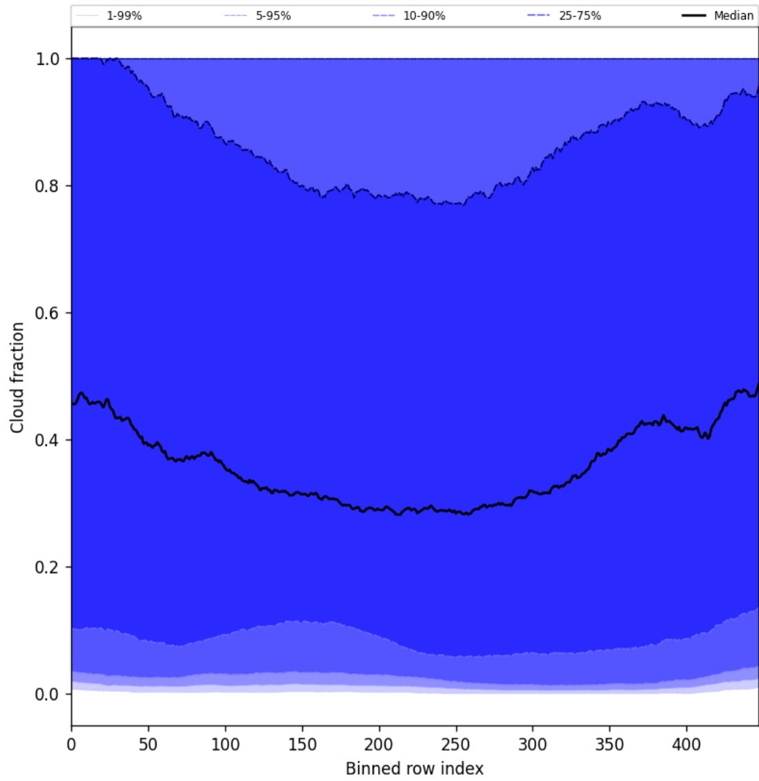
Figure 49: Along track statistics of “Cloud fraction” for 2025-04-09 to 2025-04-11
