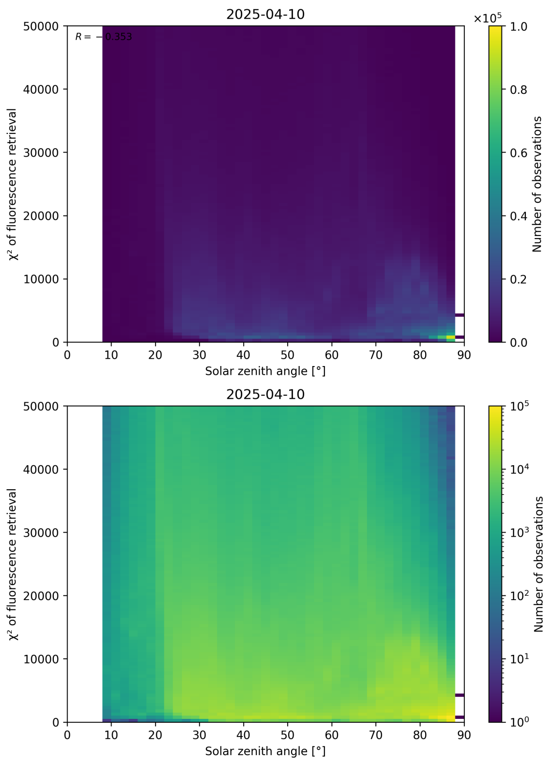
Figure 109: Scatter density plot of “Solar zenith angle” against “ \chi^2 of fluorescence retrieval” for 2025-04-09 to 2025-04-11.
