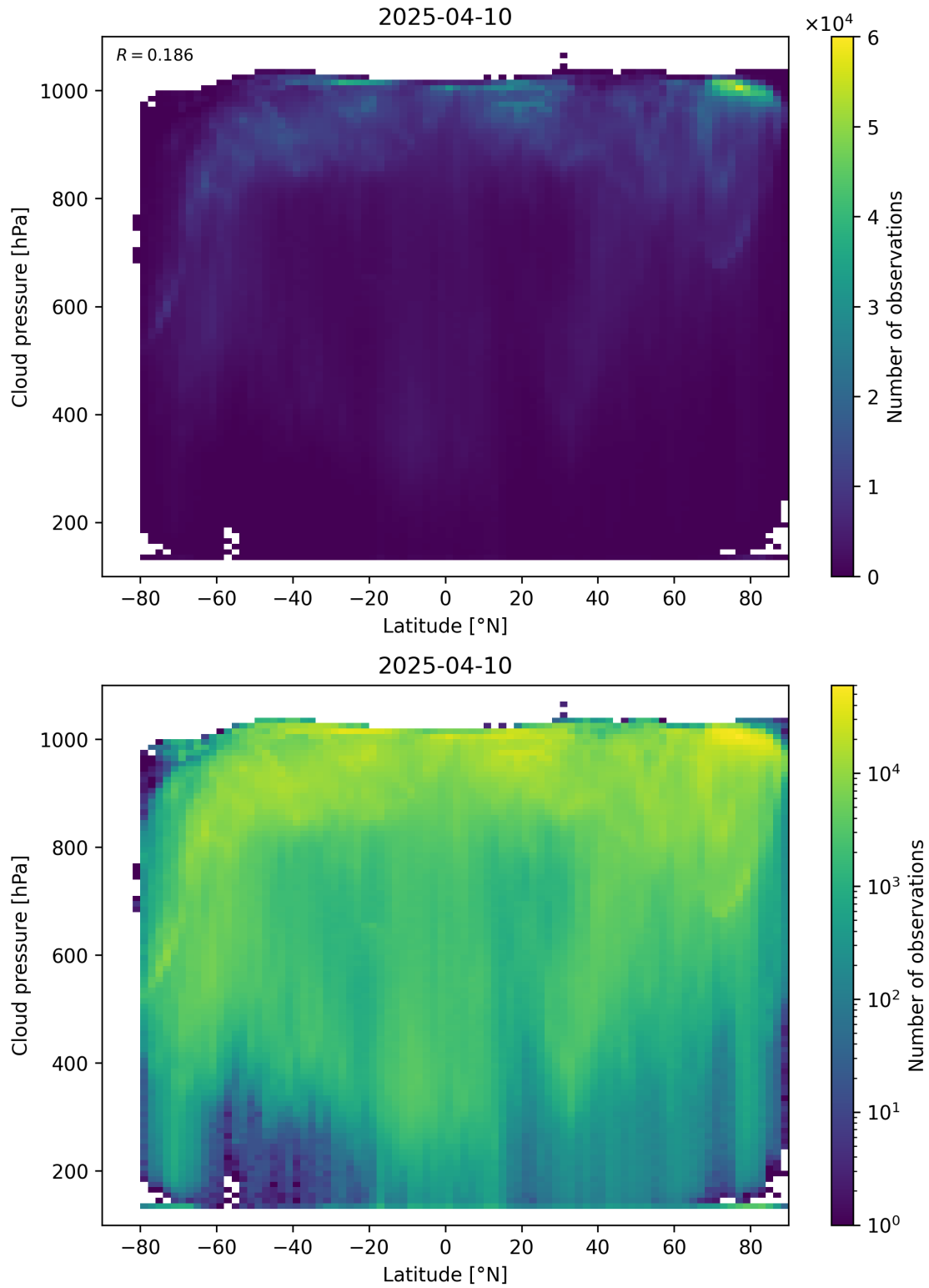
Figure 91: Scatter density plot of “Latitude” against “Cloud pressure” for 2025-04-09 to 2025-04-11.
