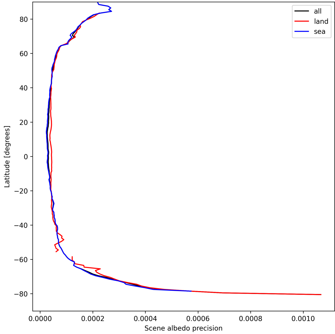
Figure 18: Zonal average of “Scene albedo precision” for 2025-04-09 to 2025-04-11.
