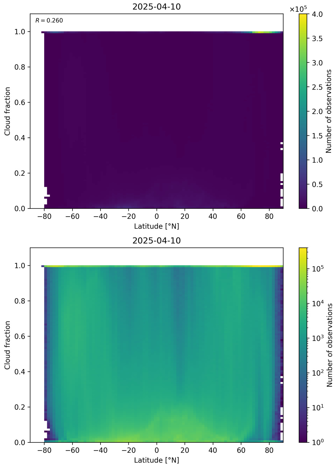
Figure 90: Scatter density plot of “Latitude” against “Cloud fraction” for 2025-04-09 to 2025-04-11.
