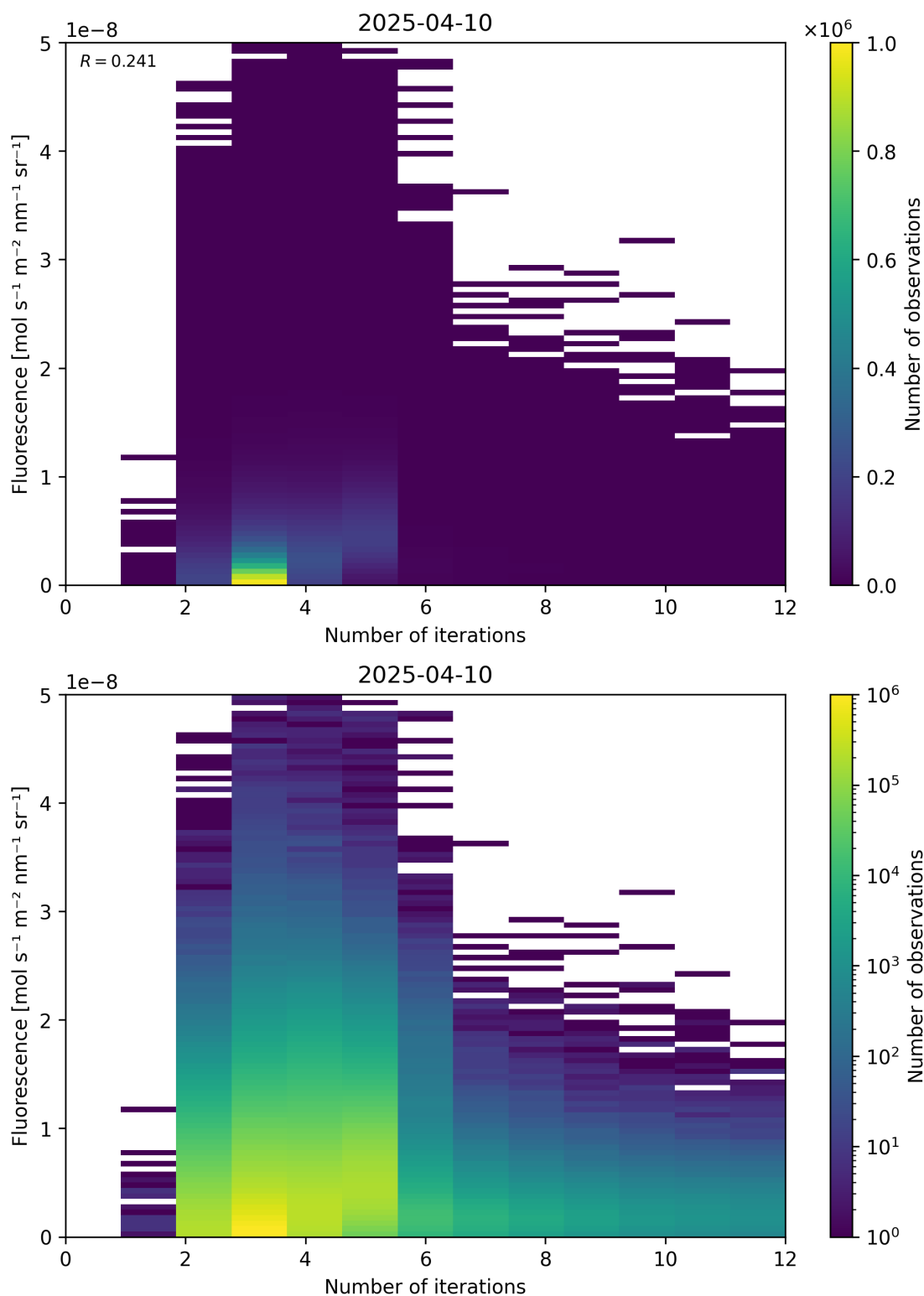
Figure 98: Scatter density plot of “Number of iterations” against “Fluorescence” for 2025-04-09 to 2025-04-11.
