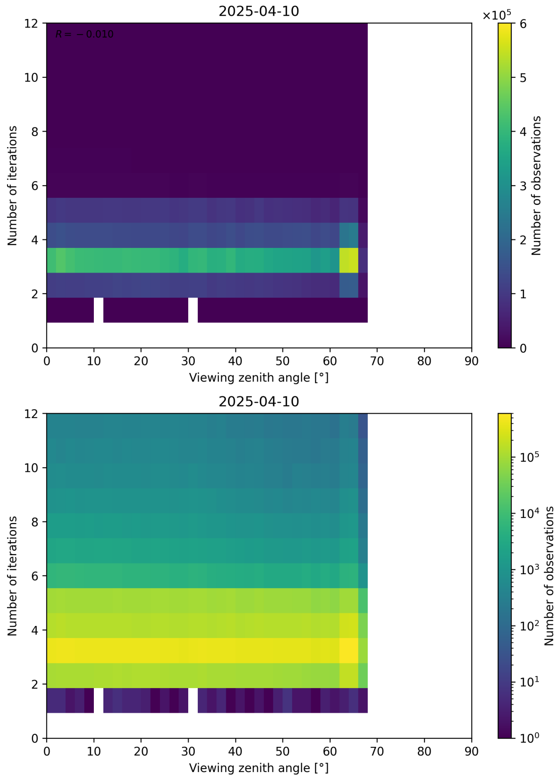
Figure 124: Scatter density plot of “Viewing zenith angle” against “Number of iterations” for 2025-04-09 to 2025-04-11.
