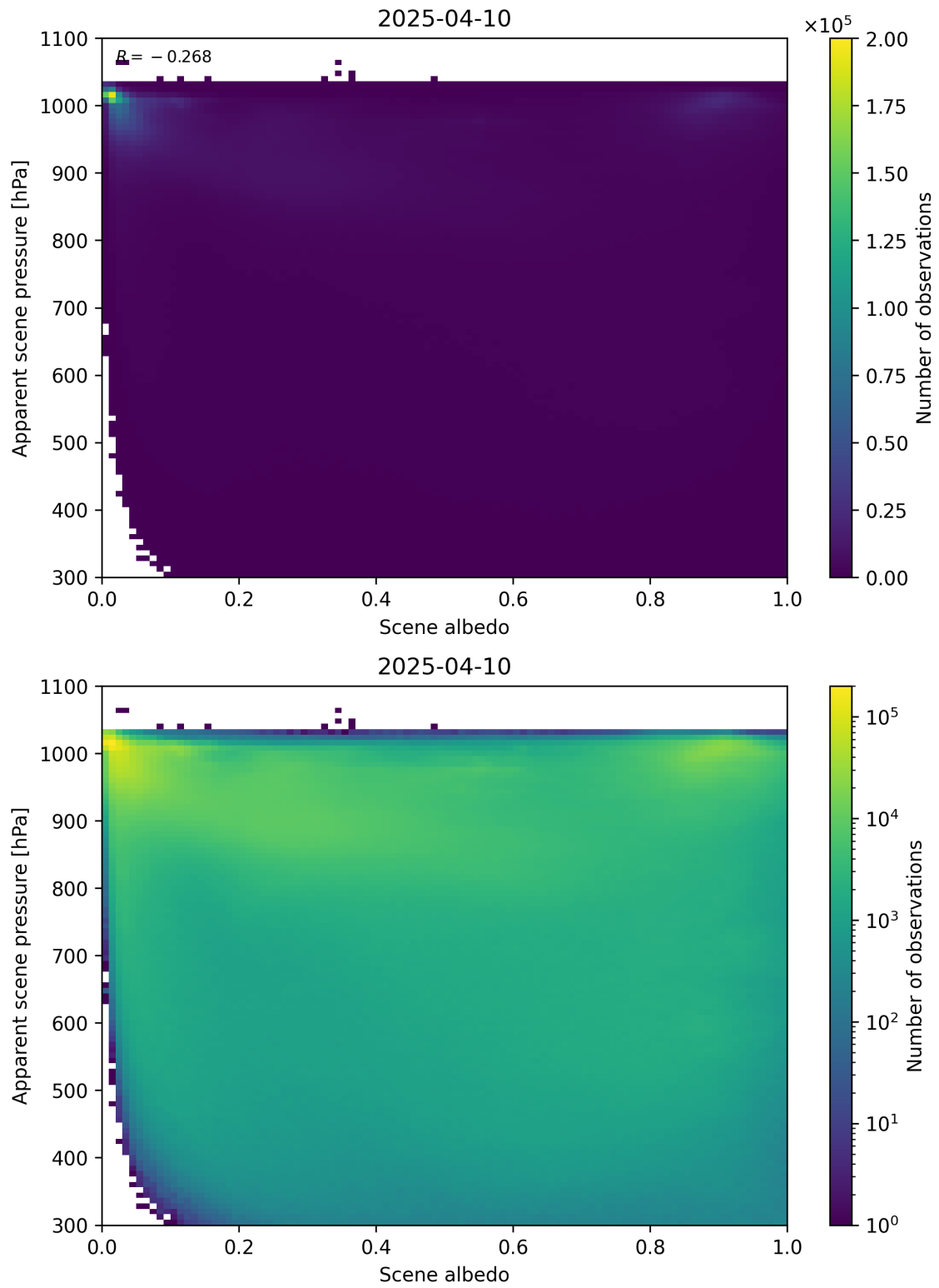
Figure 102: Scatter density plot of “Scene albedo” against “Apparent scene pressure” for 2025-04-09 to 2025-04-11.
