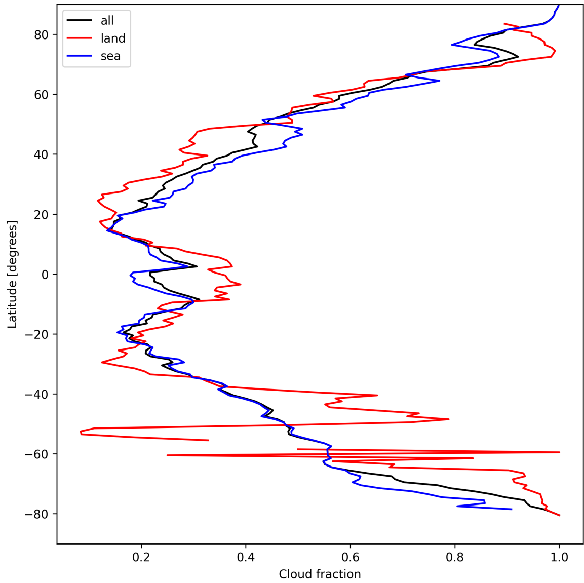
Figure 15: Zonal average of “Cloud fraction” for 2025-04-09 to 2025-04-11.
