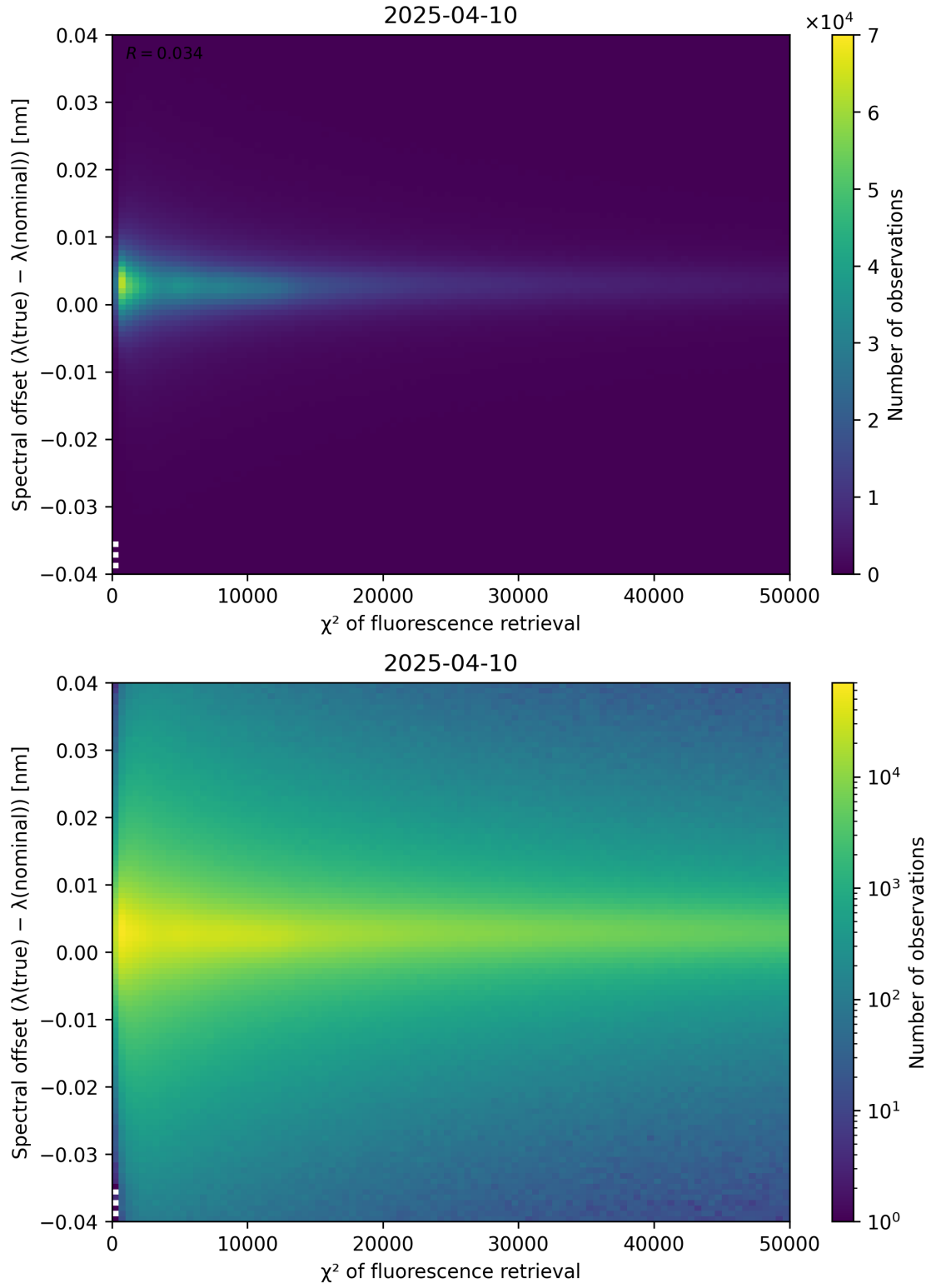
Figure 69: Scatter density plot of “ \chi^2 of fluorescence retrieval” against “Spectral offset ( \lambda_{\text{true}} - \lambda_{\text{nominal}} )” for 2025-04-09 to 2025-04-11.
