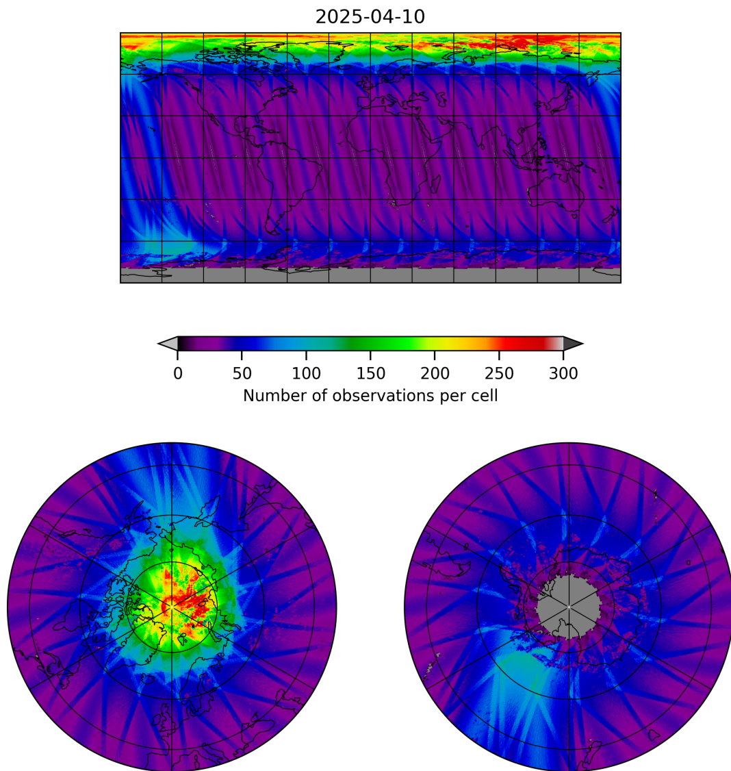
Figure 11: Map of the number of observations for 2025-04-09 to 2025-04-11
