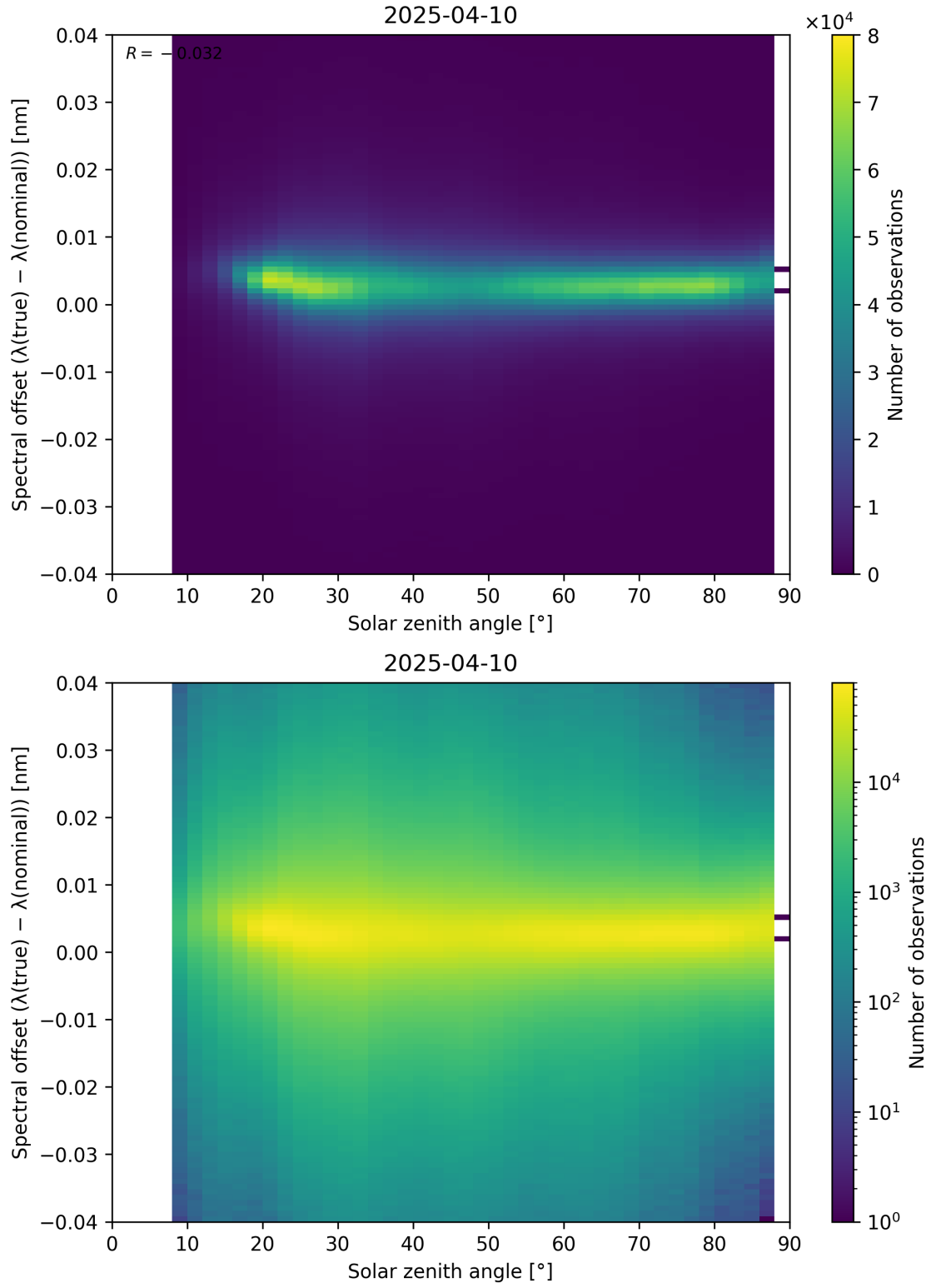
Figure 117: Scatter density plot of “Solar zenith angle” against “Spectral offset ( \lambda_{\text{true}} - \lambda_{\text{nominal}} )” for 2025-04-09 to 2025-04-11.
