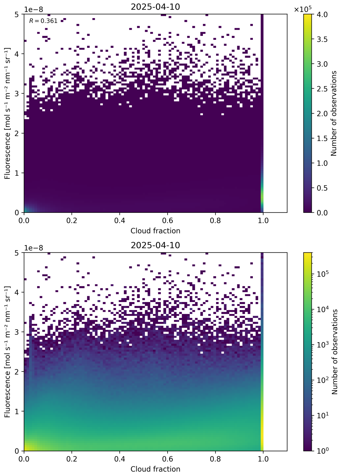
Figure 72: Scatter density plot of “Cloud fraction” against “Fluorescence” for 2025-04-09 to 2025-04-11.
