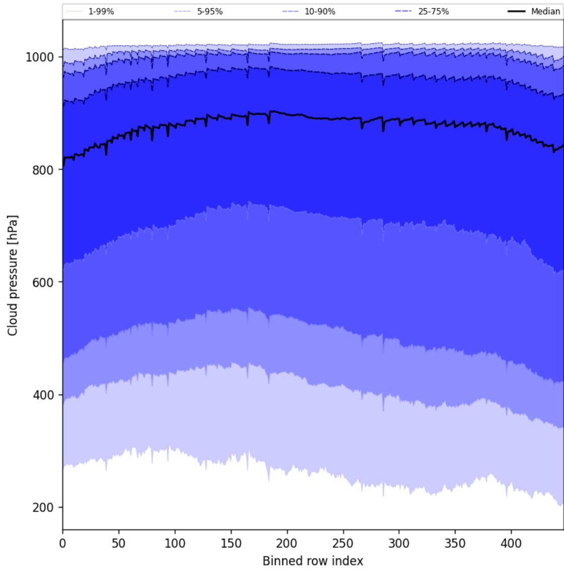
Figure 47: Along track statistics of "Cloud pressure" for 2025-04-09 to 2025-04-11
