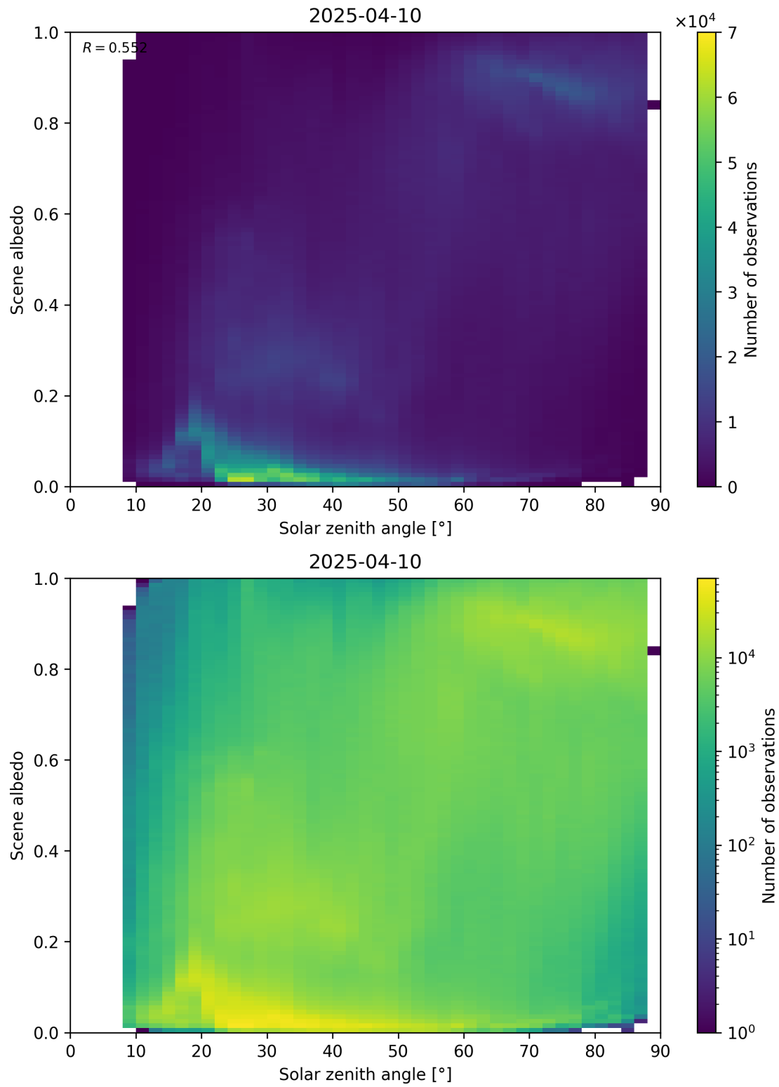
Figure 116: Scatter density plot of “Solar zenith angle” against “Scene albedo” for 2025-04-09 to 2025-04-11.
