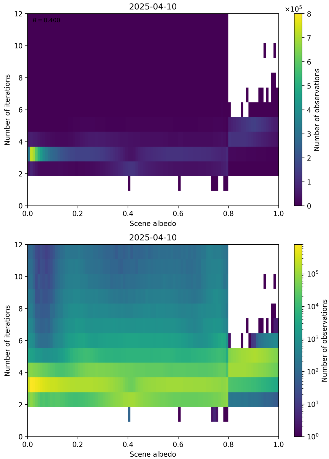
Figure 105: Scatter density plot of “Scene albedo” against “Number of iterations” for 2025-04-09 to 2025-04-11.
