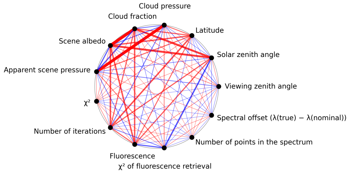
Figure 1: Map of correlation graph for 2025-04-09 to 2025-04-11.
