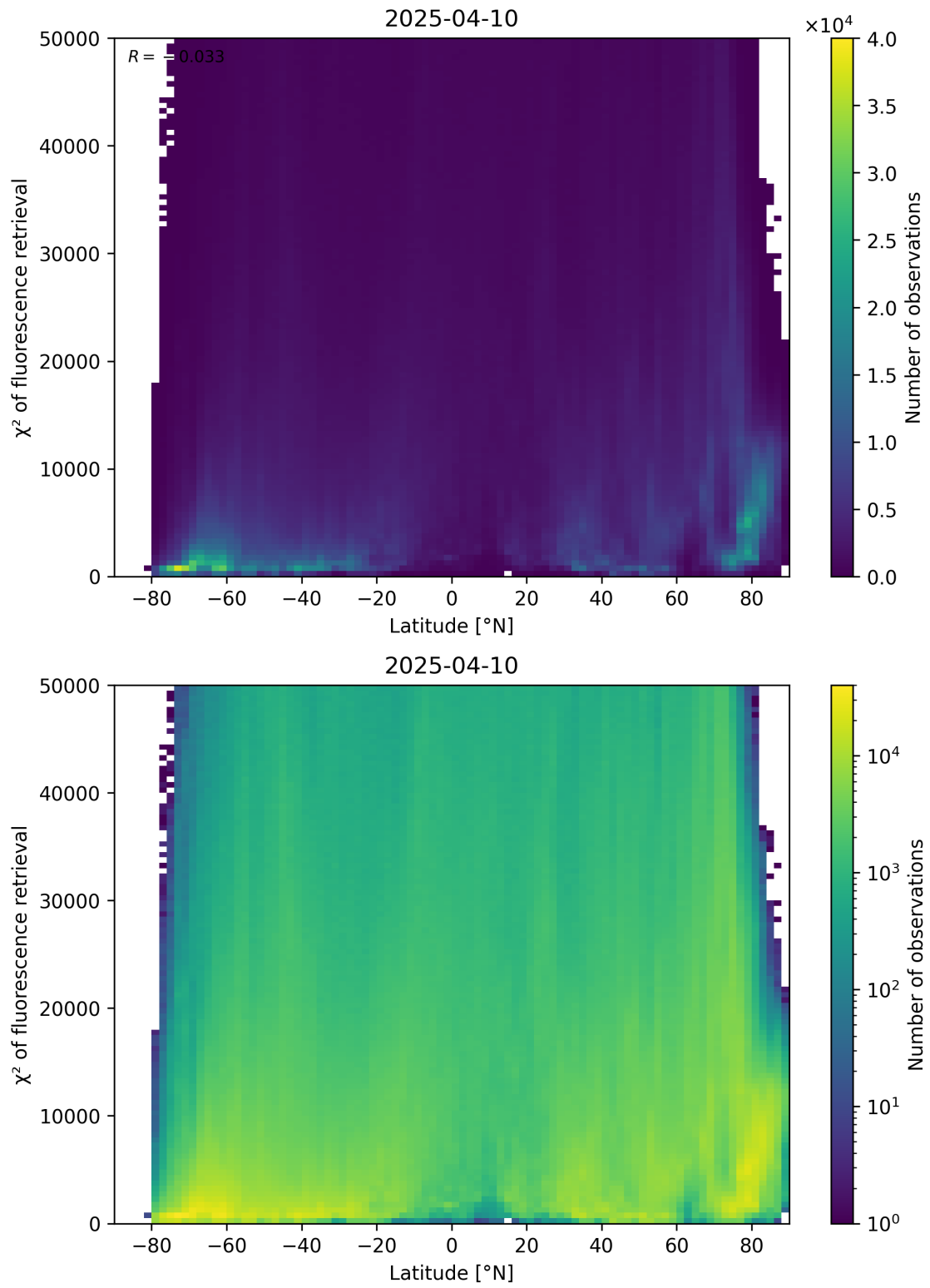
Figure 89: Scatter density plot of “Latitude” against “ \chi^2 of fluorescence retrieval” for 2025-04-09 to 2025-04-11.
