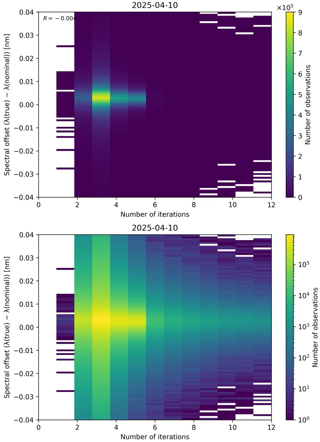
Figure 100: Scatter density plot of “Number of iterations” against “Spectral offset ( \lambda_{\text{true}} - \lambda_{\text{nominal}} )” for 2025-04-09 to 2025-04-11.
