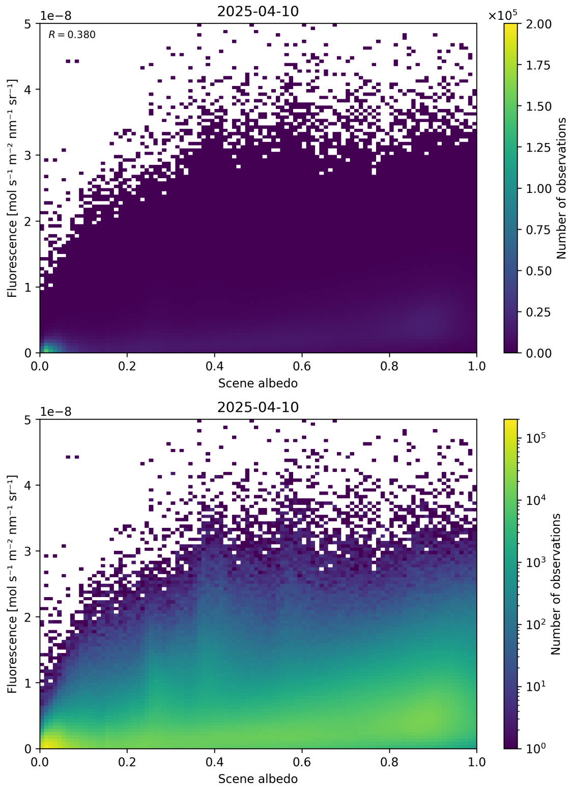
Figure 104: Scatter density plot of “Scene albedo” against “Fluorescence” for 2025-04-09 to 2025-04-11.
