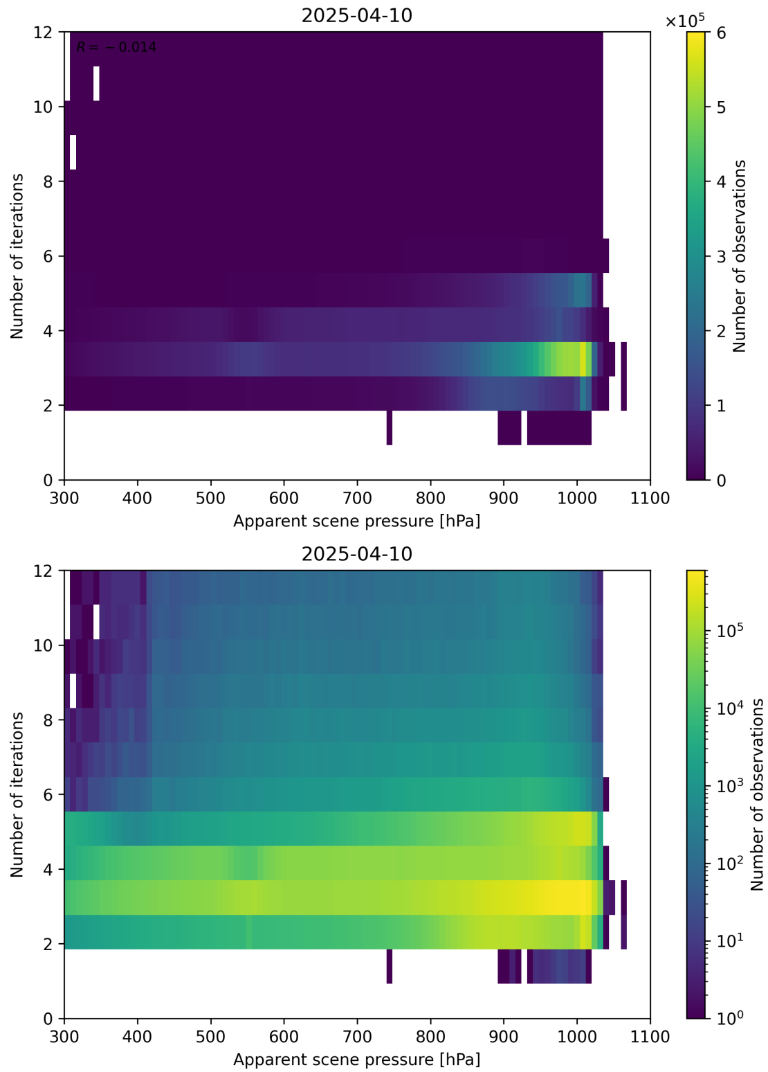
Figure 65: Scatter density plot of “Apparent scene pressure” against “Number of iterations” for 2025-04-09 to 2025-04-11.
