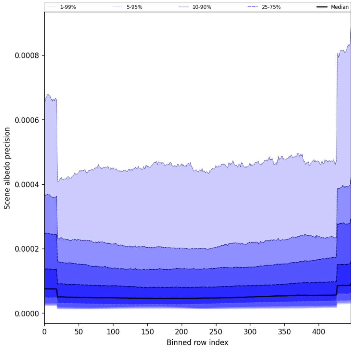
Figure 52: Along track statistics of “Scene albedo precision” for 2025-04-09 to 2025-04-11
