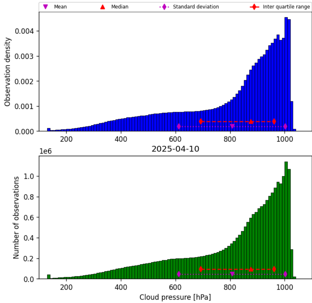
Figure 30: Histogram of “Cloud pressure” for 2025-04-09 to 2025-04-11
