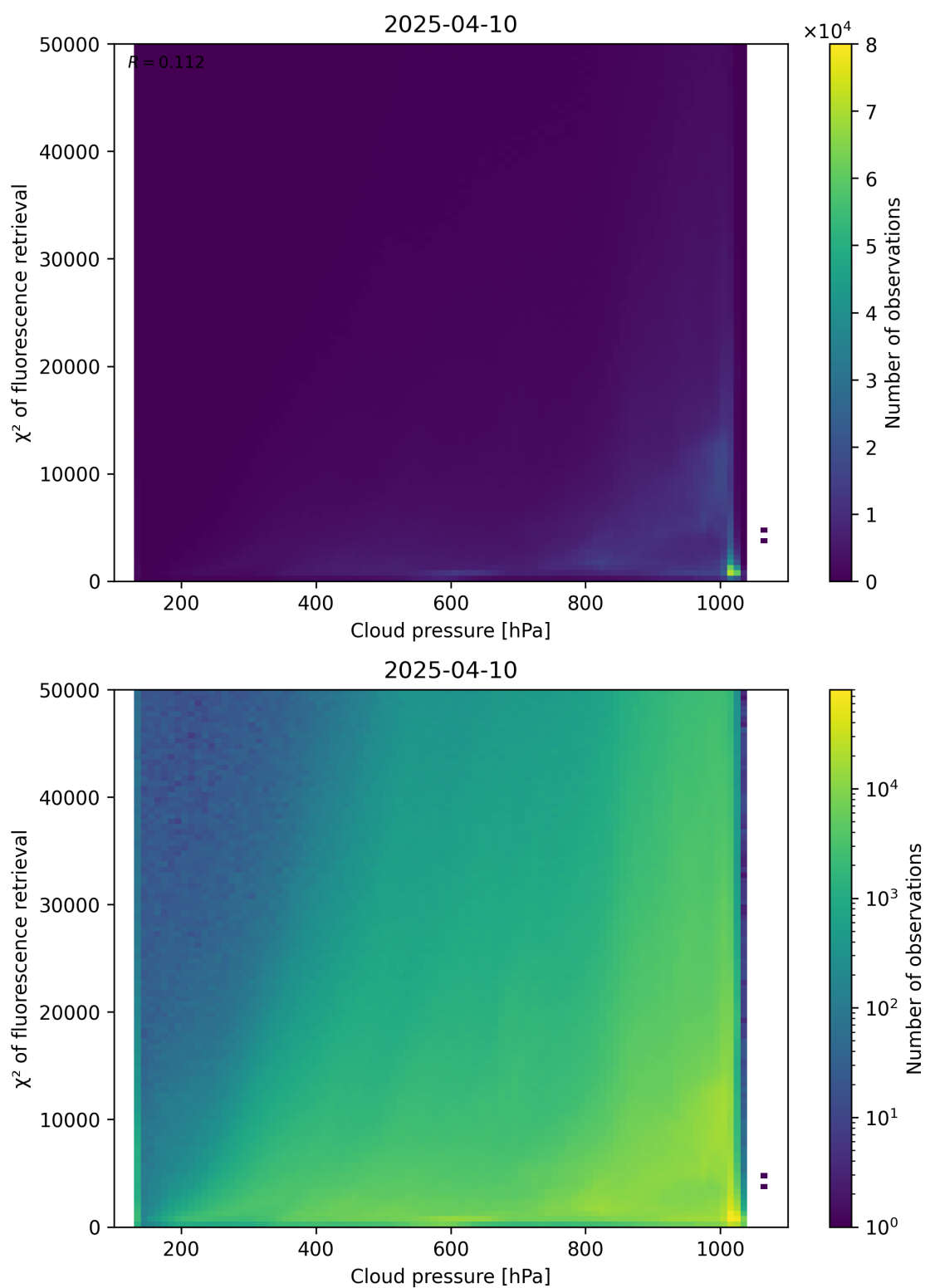
Figure 78: Scatter density plot of “Cloud pressure” against “ \chi^2 of fluorescence retrieval” for 2025-04-09 to 2025-04-11.
