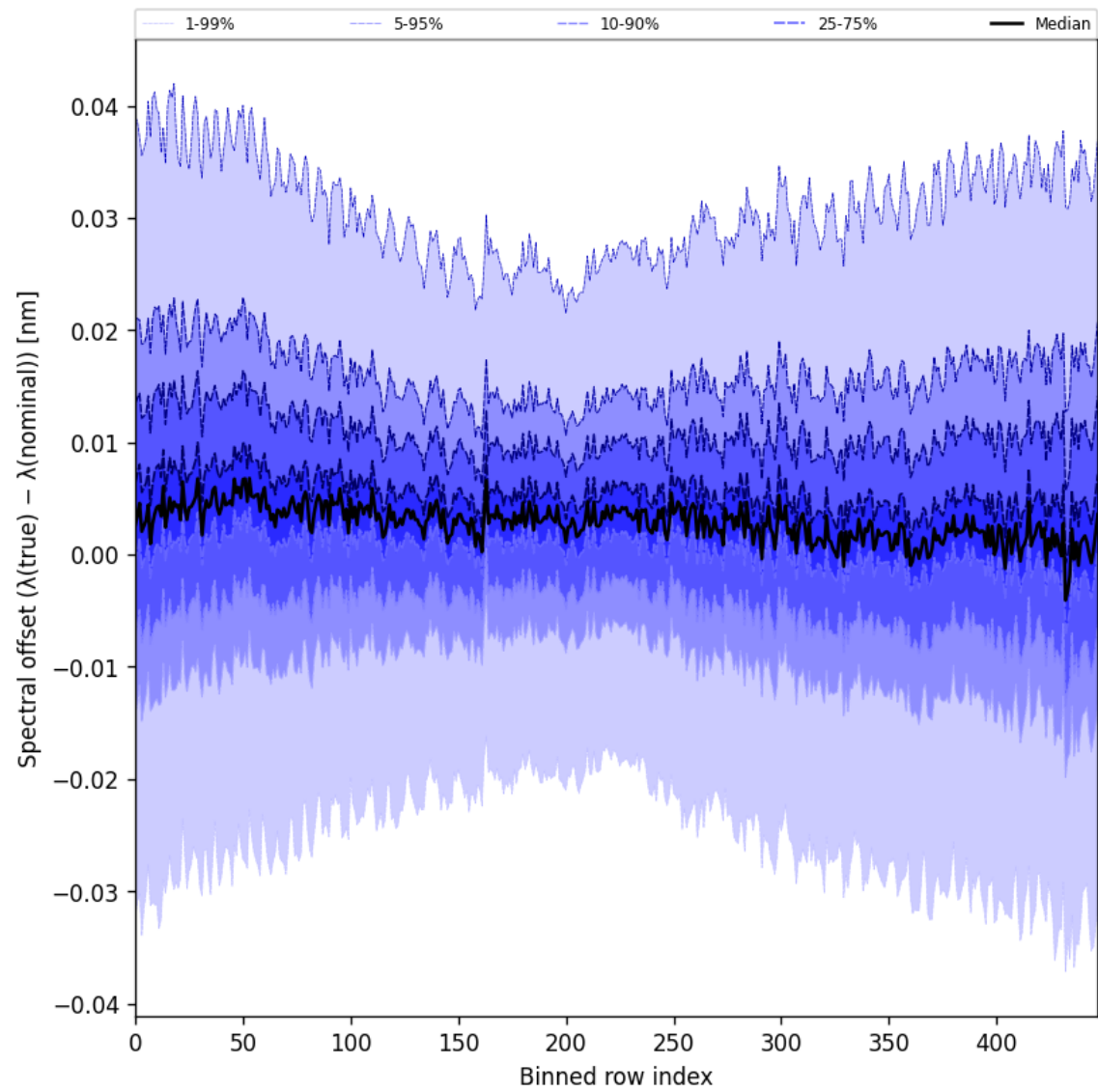
Figure 62: Along track statistics of “Spectral offset ( \lambda_{\text{true}} - \lambda_{\text{nominal}} )” for 2025-04-09 to 2025-04-11
