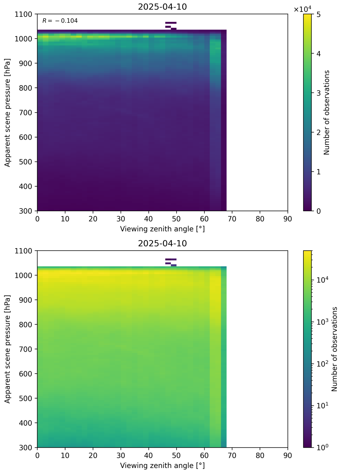
Figure 118: Scatter density plot of “Viewing zenith angle” against “Apparent scene pressure” for 2025-04-09 to 2025-04-11.
