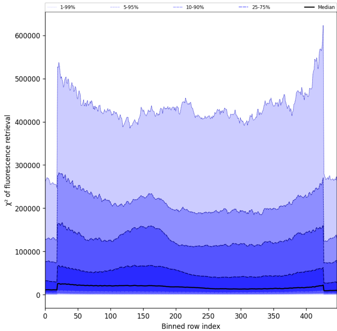
Figure 59: Along track statistics of “ \chi^2 of fluorescence retrieval” for 2025-04-09 to 2025-04-11
