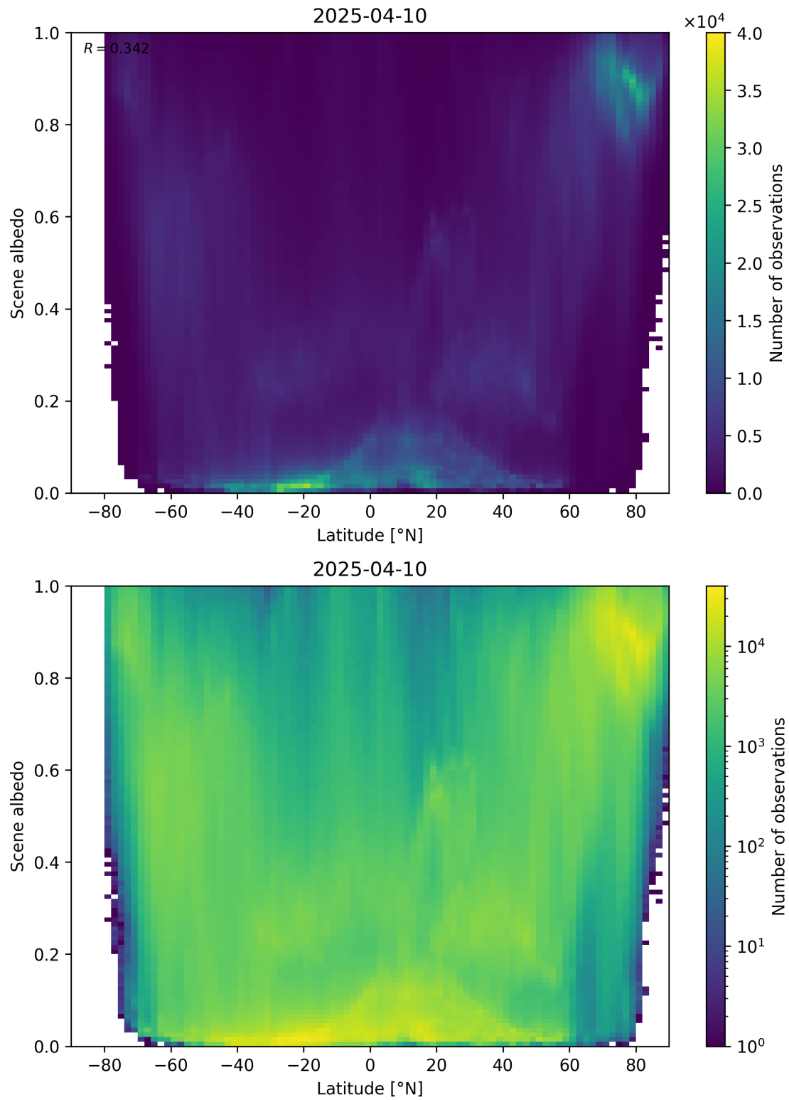
Figure 95: Scatter density plot of “Latitude” against “Scene albedo” for 2025-04-09 to 2025-04-11.
