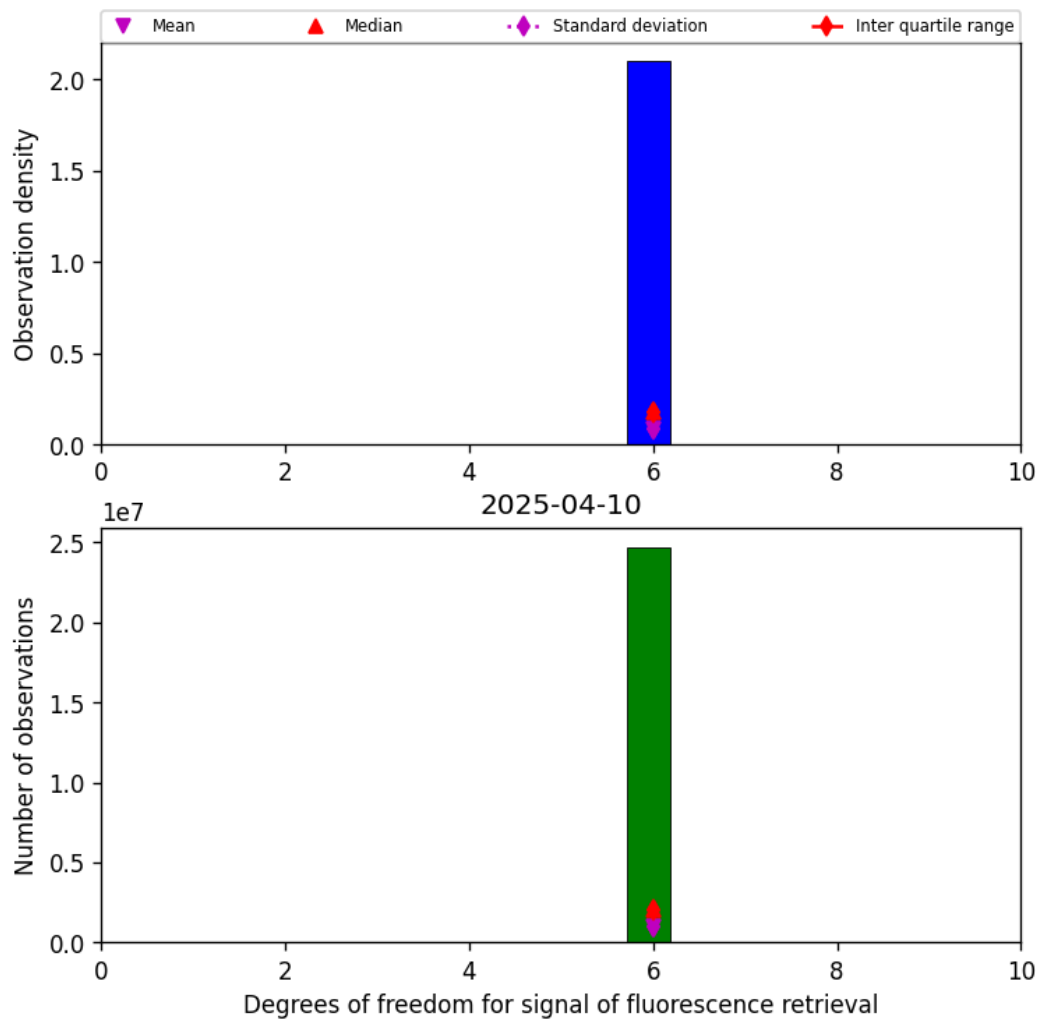
Figure 43: Histogram of “Degrees of freedom for signal of fluorescence retrieval” for 2025-04-09 to 2025-04-11
