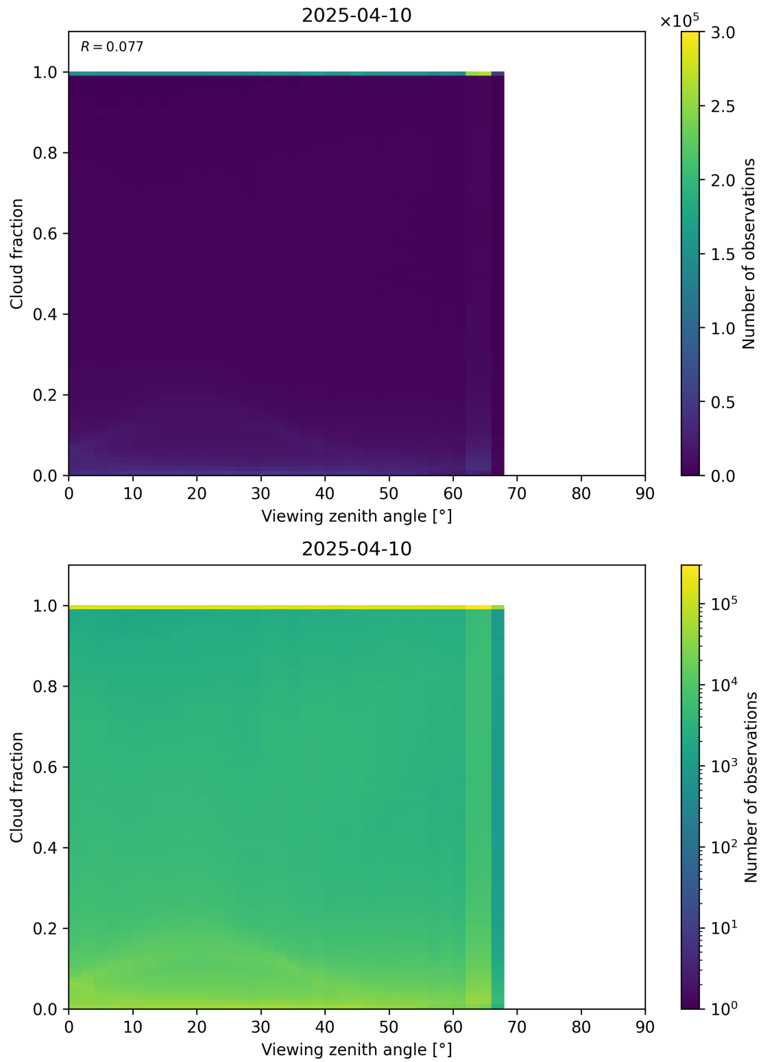
Figure 120: Scatter density plot of “Viewing zenith angle” against “Cloud fraction” for 2025-04-09 to 2025-04-11.
