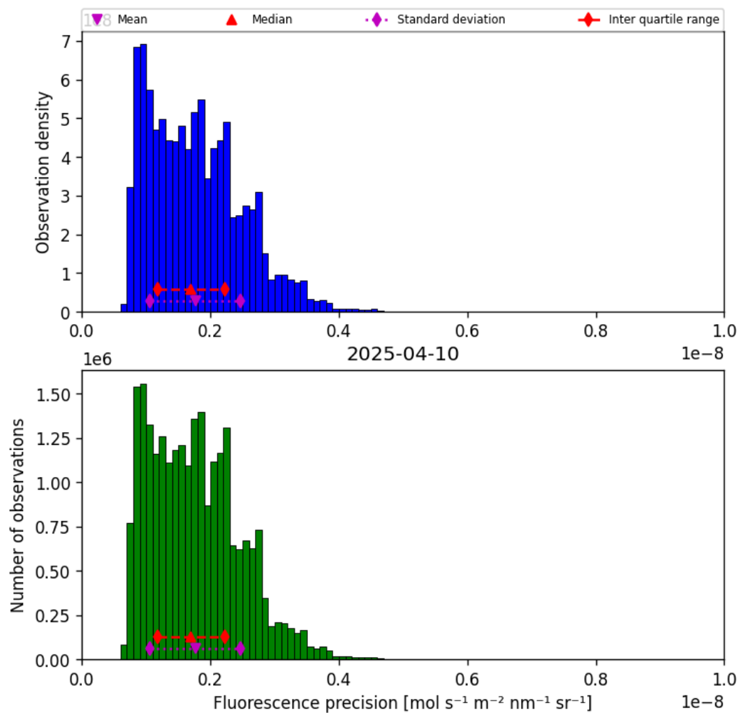
Figure 41: Histogram of “Fluorescence precision” for 2025-04-09 to 2025-04-11
