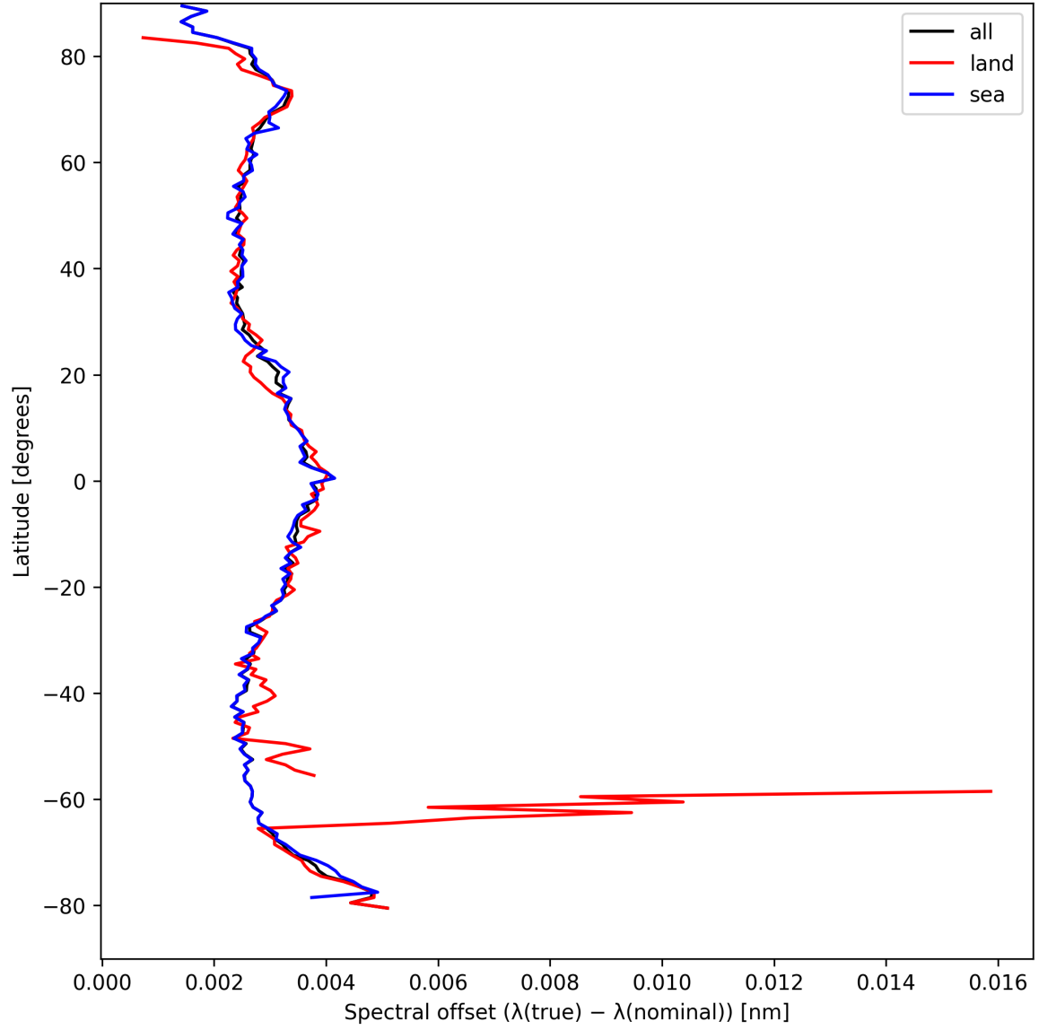
Figure 28: Zonal average of “Spectral offset ( \lambda_{\text{true}} - \lambda_{\text{nominal}} )” for 2025-04-09 to 2025-04-11.
