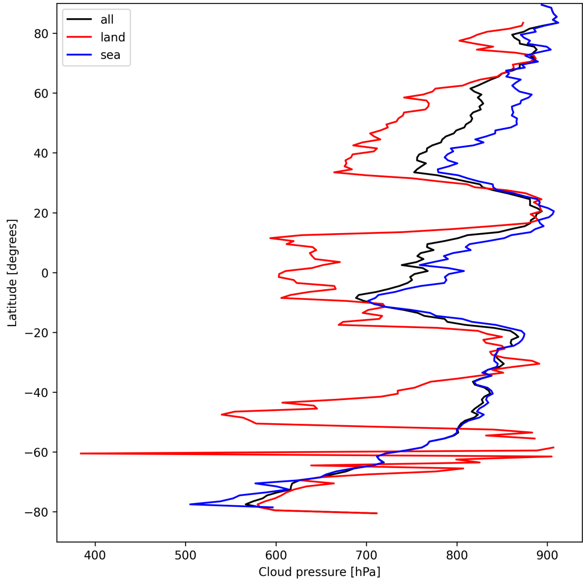
Figure 13: Zonal average of “Cloud pressure” for 2025-04-09 to 2025-04-11.
