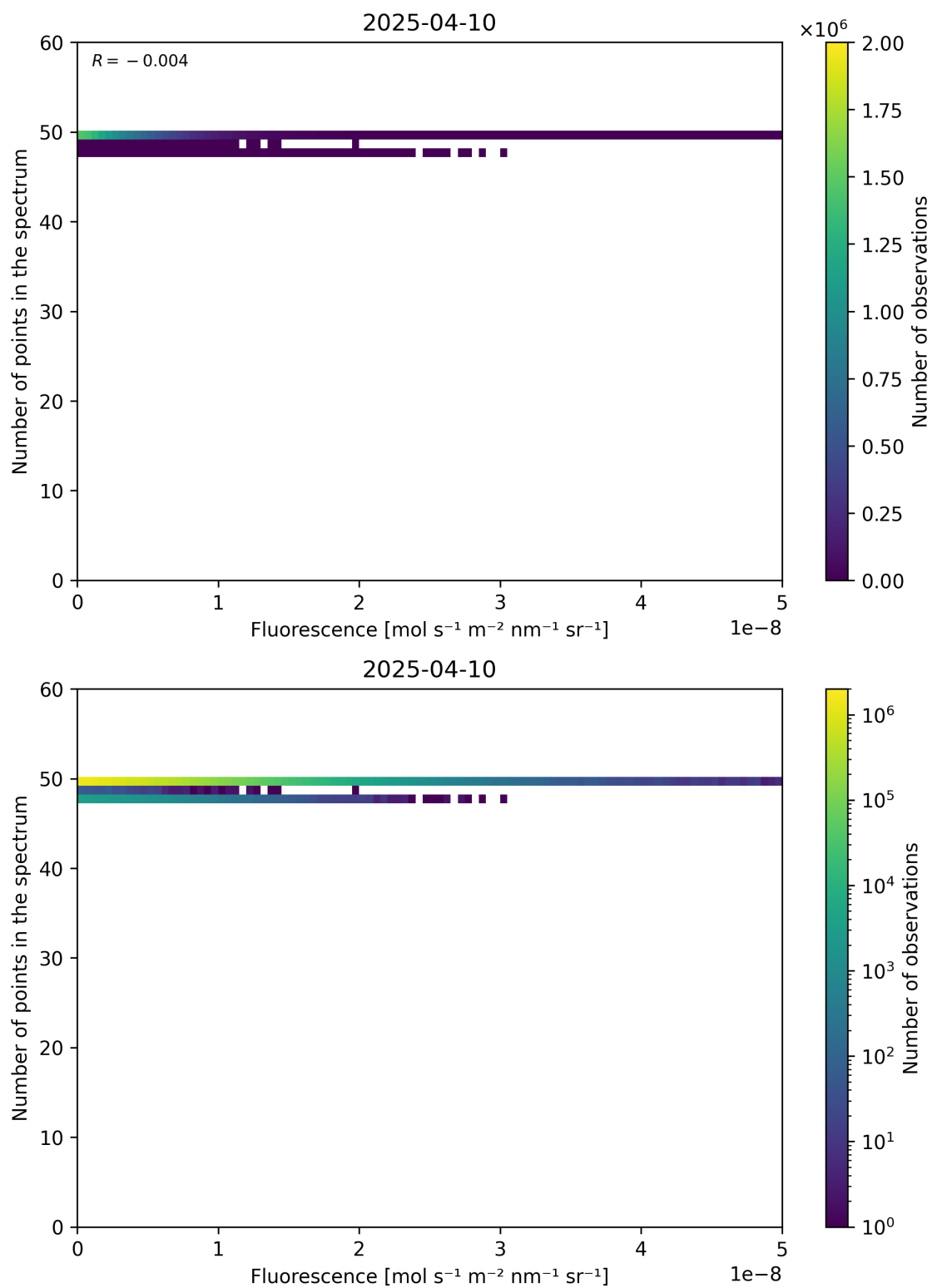
Figure 86: Scatter density plot of “Fluorescence” against “Number of points in the spectrum” for 2025-04-09 to 2025-04-11.
