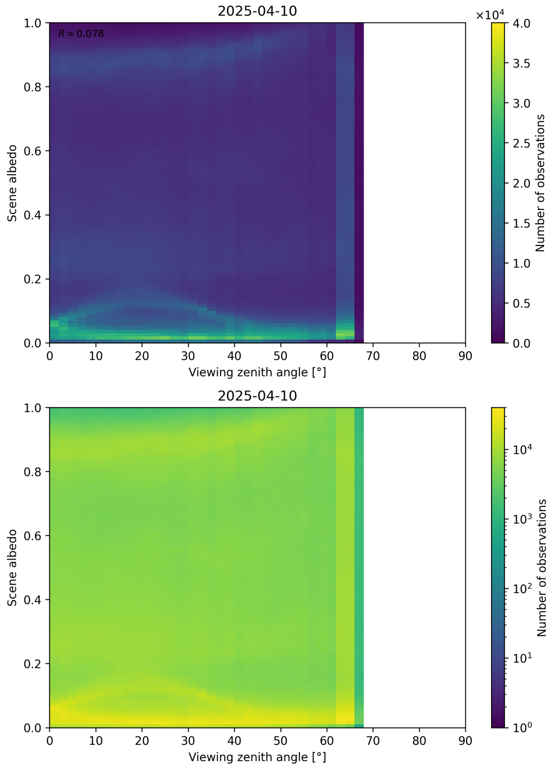
Figure 126: Scatter density plot of “Viewing zenith angle” against “Scene albedo” for 2025-04-09 to 2025-04-11.
