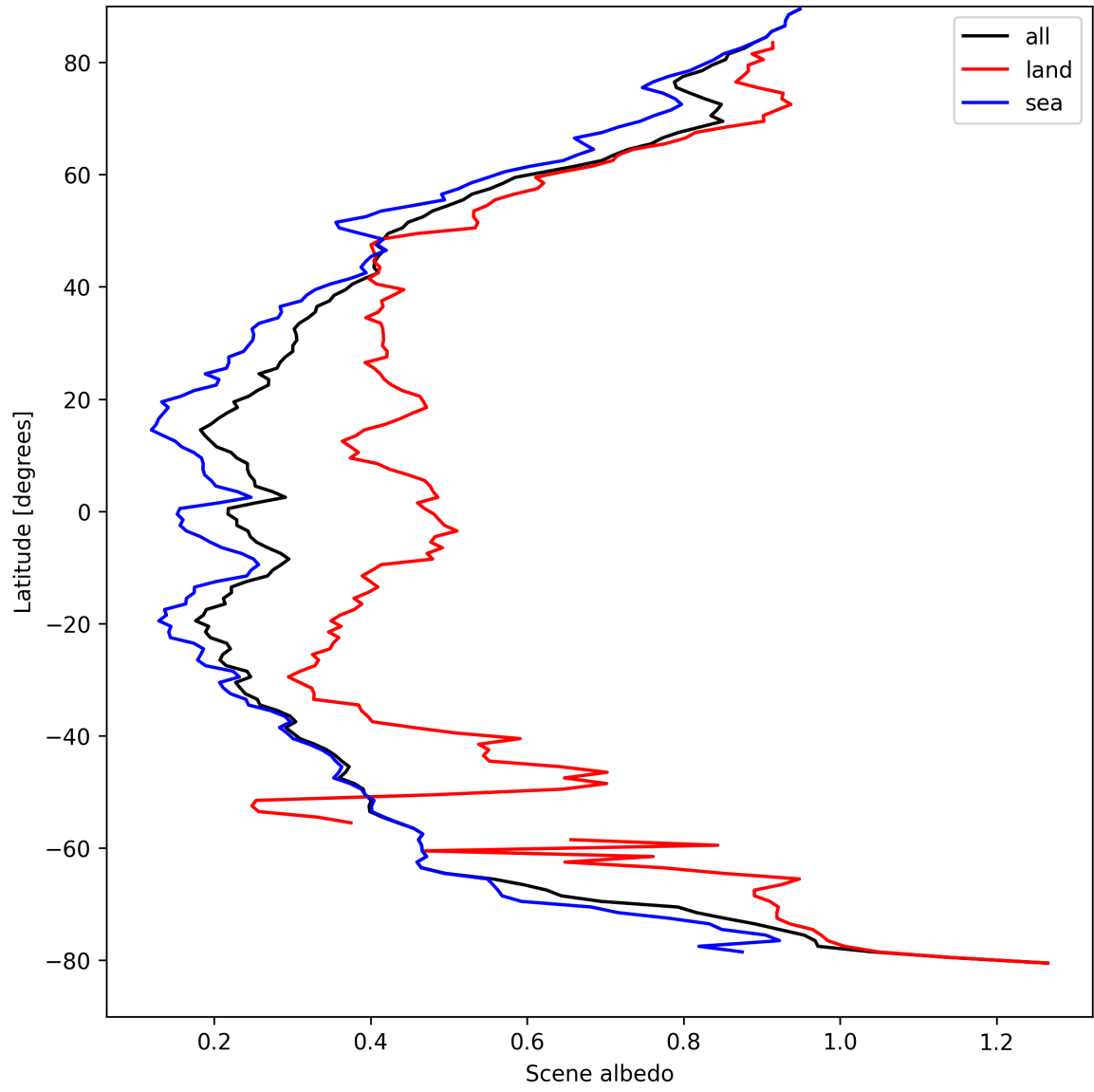
Figure 17: Zonal average of “Scene albedo” for 2025-04-09 to 2025-04-11.
