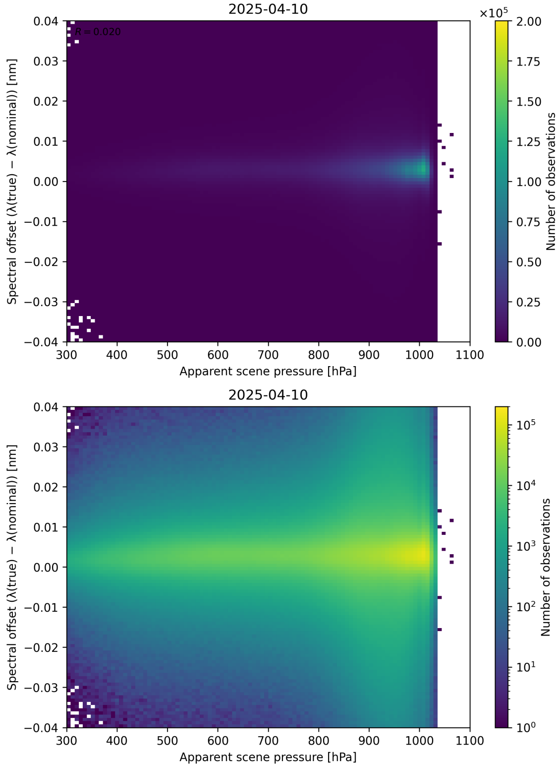
Figure 67: Scatter density plot of “Apparent scene pressure” against “Spectral offset ( \lambda_{\text{true}} - \lambda_{\text{nominal}} )” for 2025-04-09 to 2025-04-11.
