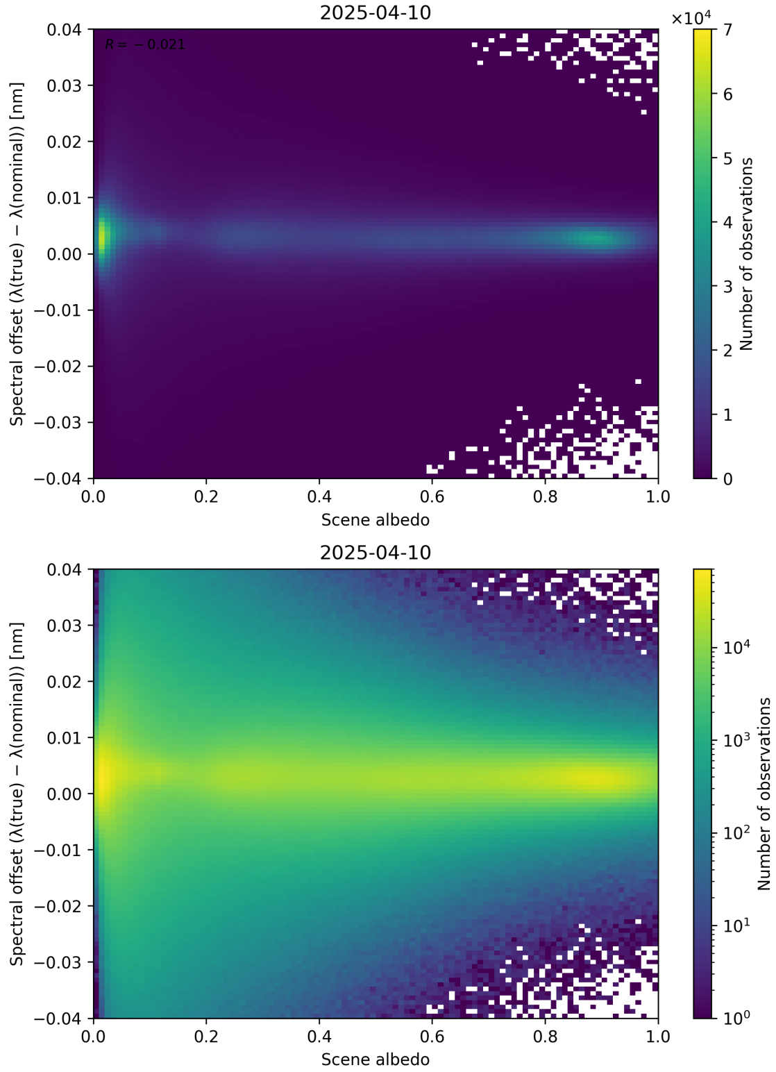
Figure 107: Scatter density plot of “Scene albedo” against “Spectral offset ( \lambda_{\text{true}} - \lambda_{\text{nominal}} )” for 2025-04-09 to 2025-04-11.
