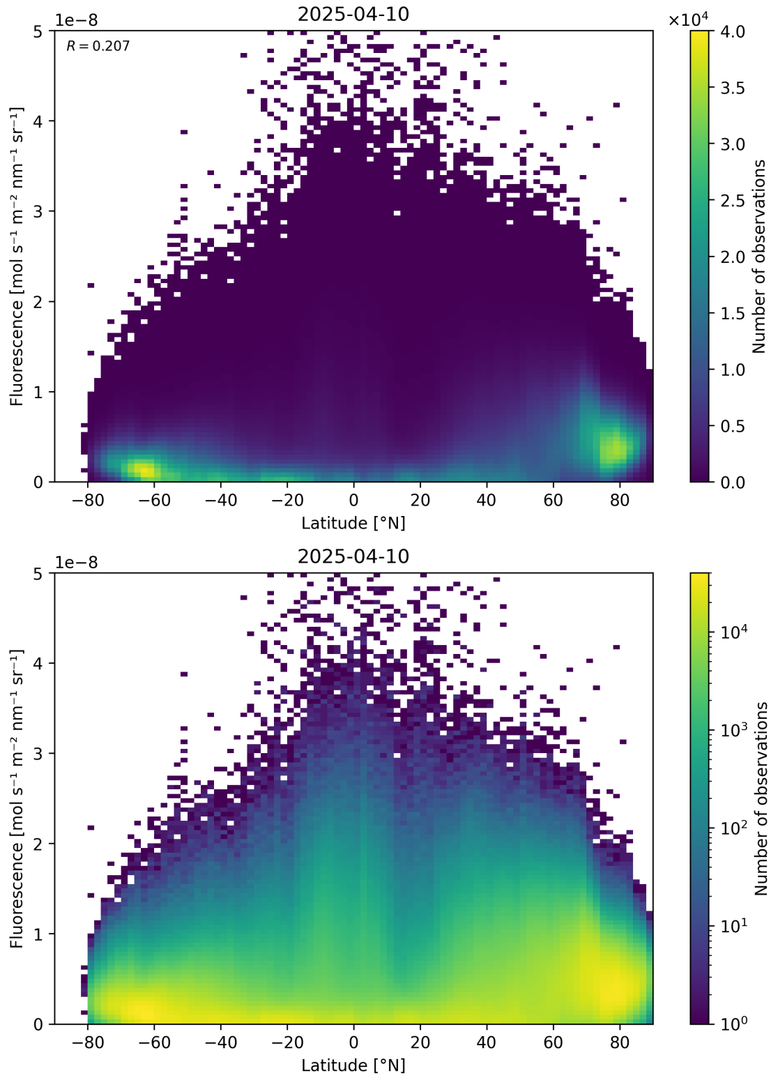
Figure 92: Scatter density plot of “Latitude” against “Fluorescence” for 2025-04-09 to 2025-04-11.
