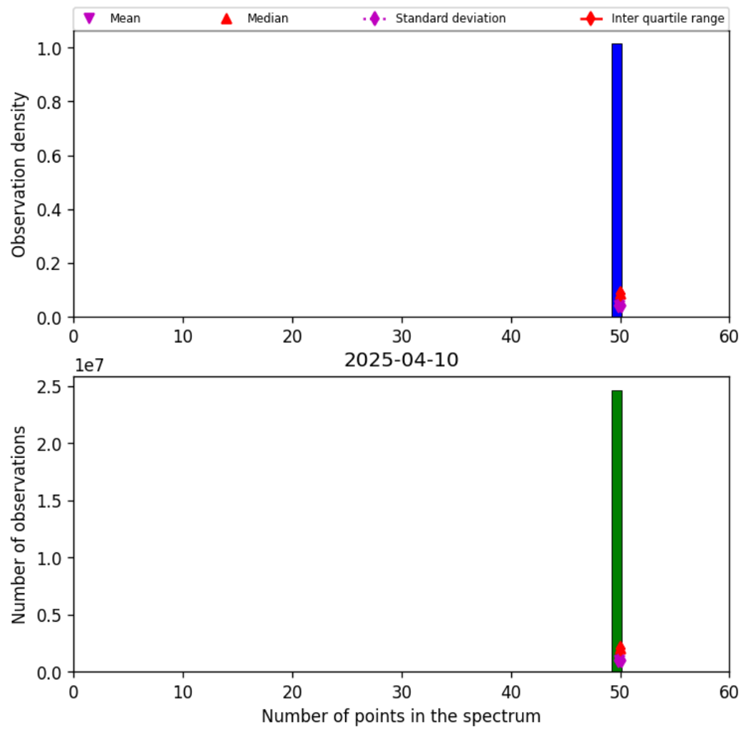
Figure 44: Histogram of "Number of points in the spectrum" for 2025-04-09 to 2025-04-11
