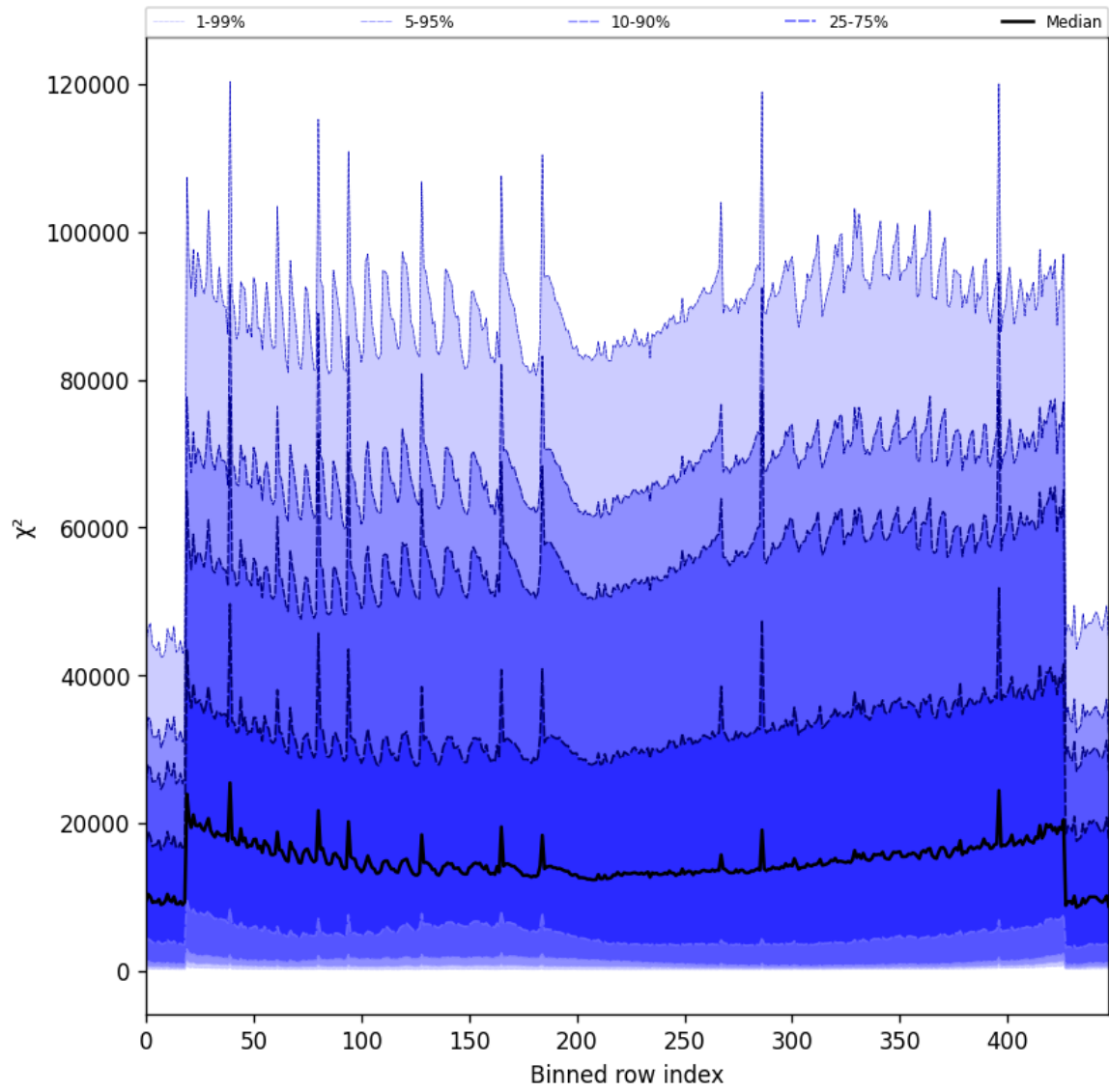
Figure 55: Along track statistics of “ \chi^2 ” for 2025-04-09 to 2025-04-11
