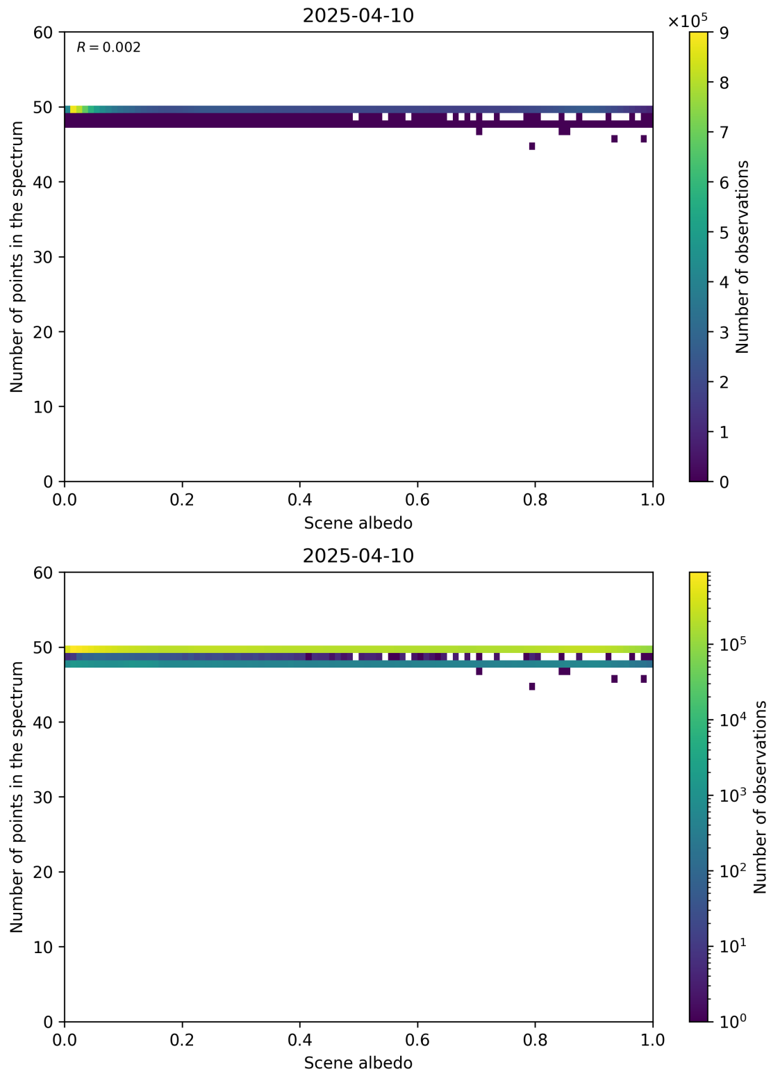
Figure 106: Scatter density plot of “Scene albedo” against “Number of points in the spectrum” for 2025-04-09 to 2025-04-11.
