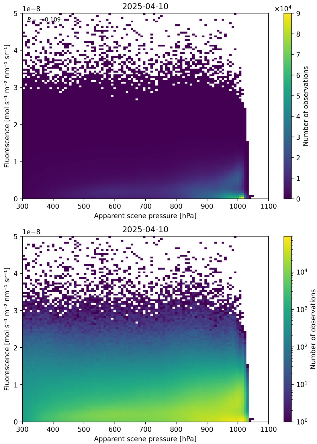
Figure 64: Scatter density plot of “Apparent scene pressure” against “Fluorescence” for 2025-04-09 to 2025-04-11.
