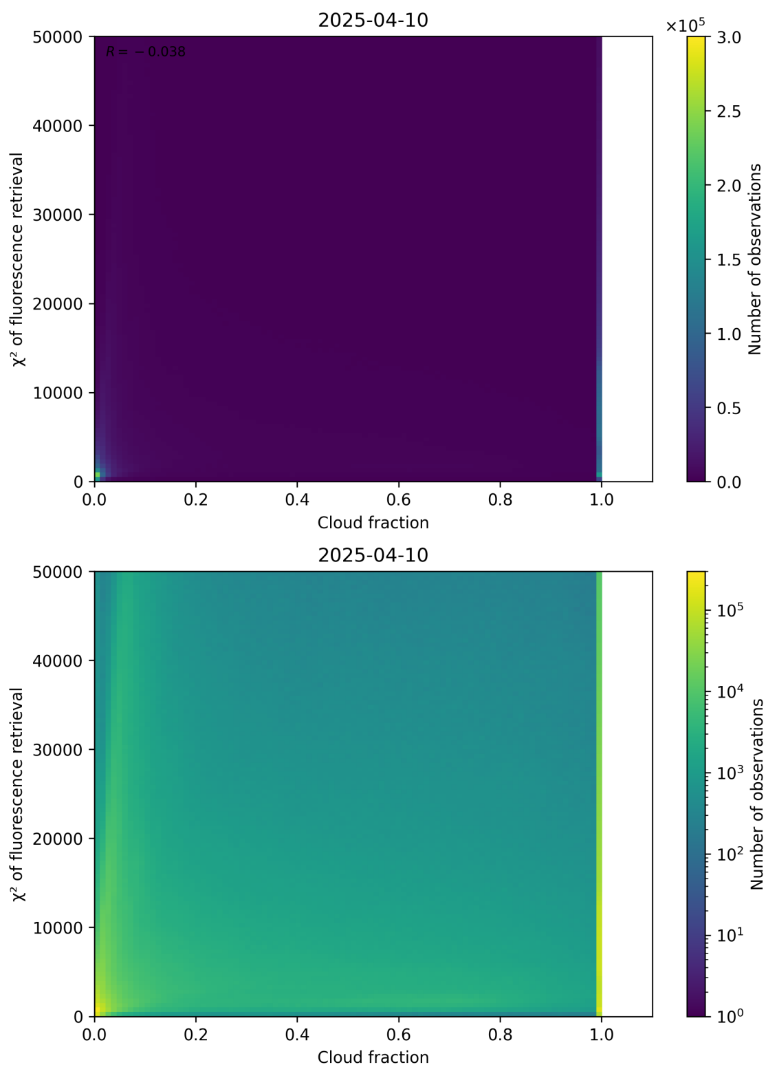
Figure 71: Scatter density plot of “Cloud fraction” against “ \chi^2 of fluorescence retrieval” for 2025-04-09 to 2025-04-11.
