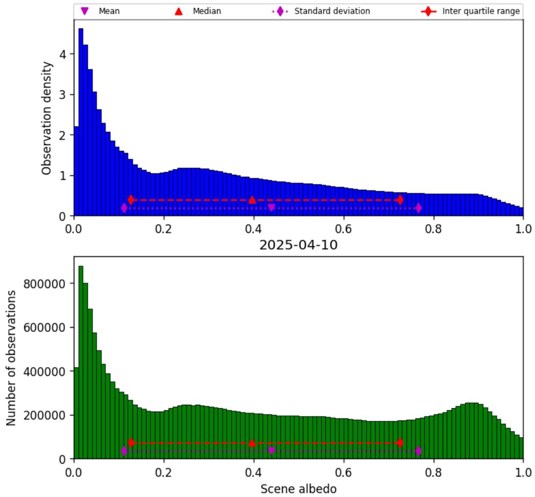
Figure 34: Histogram of “Scene albedo” for 2025-04-09 to 2025-04-11
