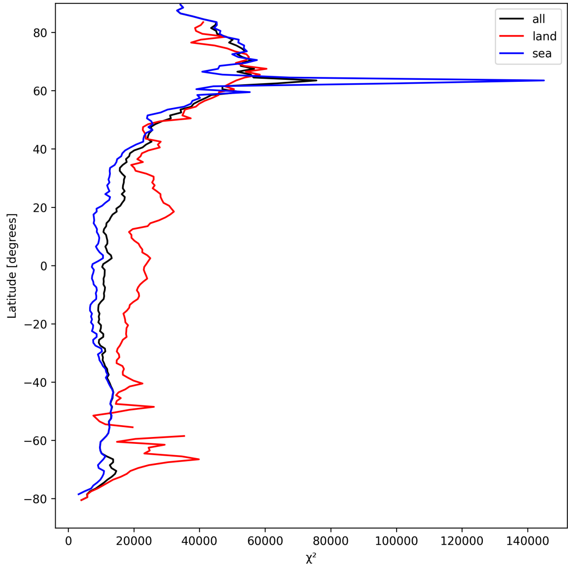
Figure 21: Zonal average of “ \chi^2 ” for 2025-04-09 to 2025-04-11.
