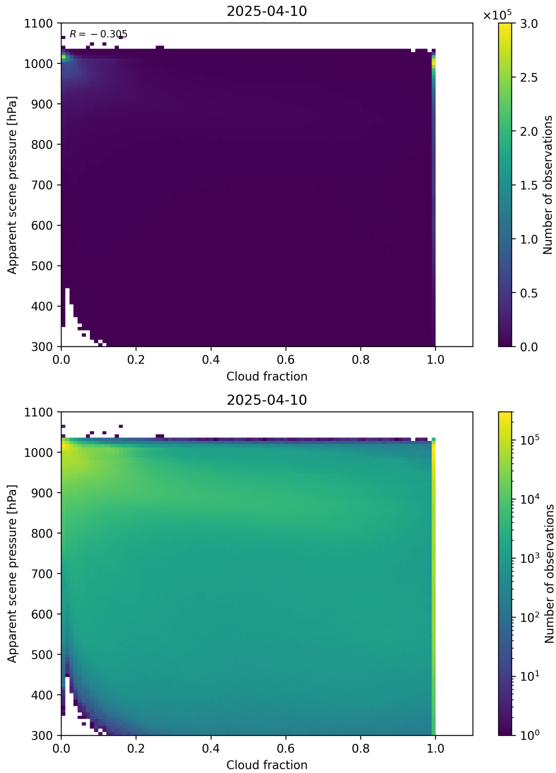
Figure 70: Scatter density plot of “Cloud fraction” against “Apparent scene pressure” for 2025-04-09 to 2025-04-11.
