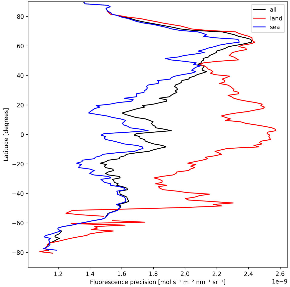
Figure 24: Zonal average of “Fluorescence precision” for 2025-04-09 to 2025-04-11.
