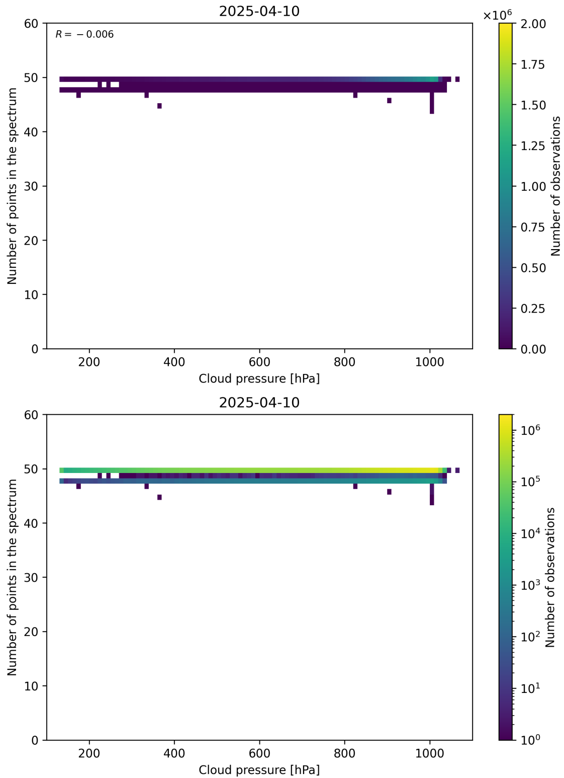
Figure 82: Scatter density plot of “Cloud pressure” against “Number of points in the spectrum” for 2025-04-09 to 2025-04-11.
