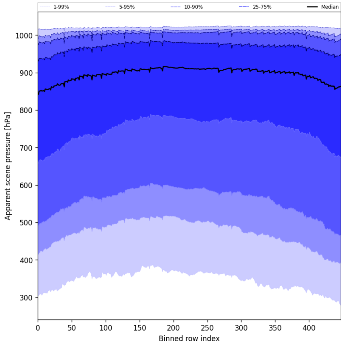
Figure 53: Along track statistics of “Apparent scene pressure” for 2025-04-09 to 2025-04-11
