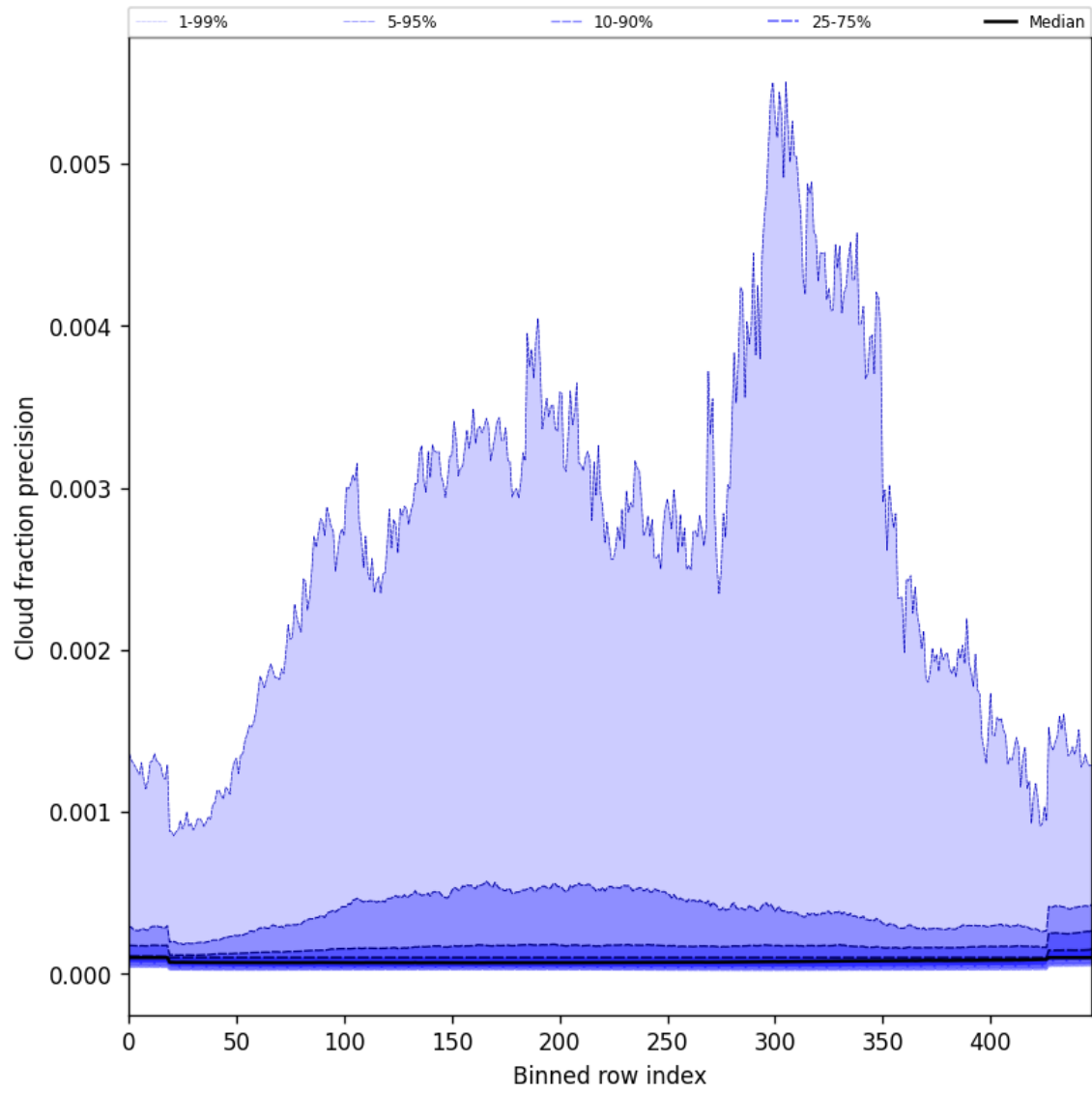
Figure 50: Along track statistics of “Cloud fraction precision” for 2025-04-09 to 2025-04-11
