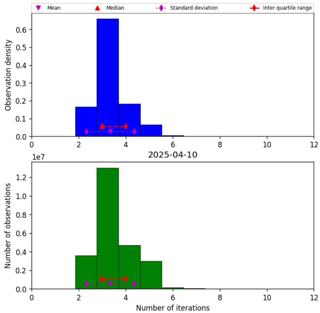
Figure 39: Histogram of “Number of iterations” for 2025-04-09 to 2025-04-11
