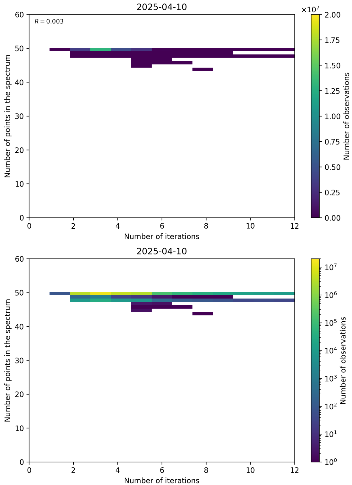
Figure 99: Scatter density plot of “Number of iterations” against “Number of points in the spectrum” for 2025-04-09 to 2025-04-11.
