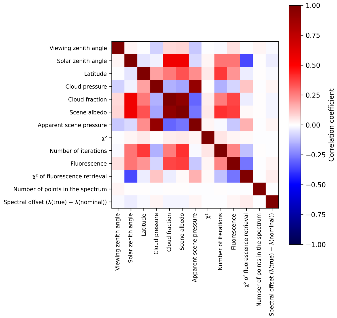
Figure 2: Map of correlation matrix for 2025-04-09 to 2025-04-11.
