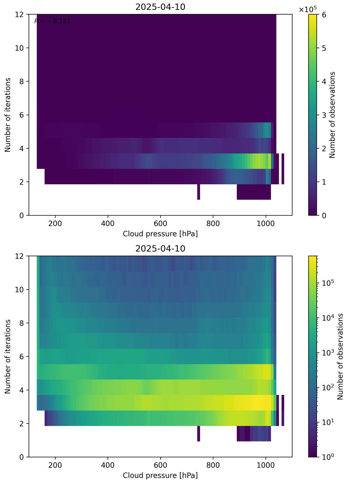
Figure 81: Scatter density plot of “Cloud pressure” against “Number of iterations” for 2025-04-09 to 2025-04-11.
