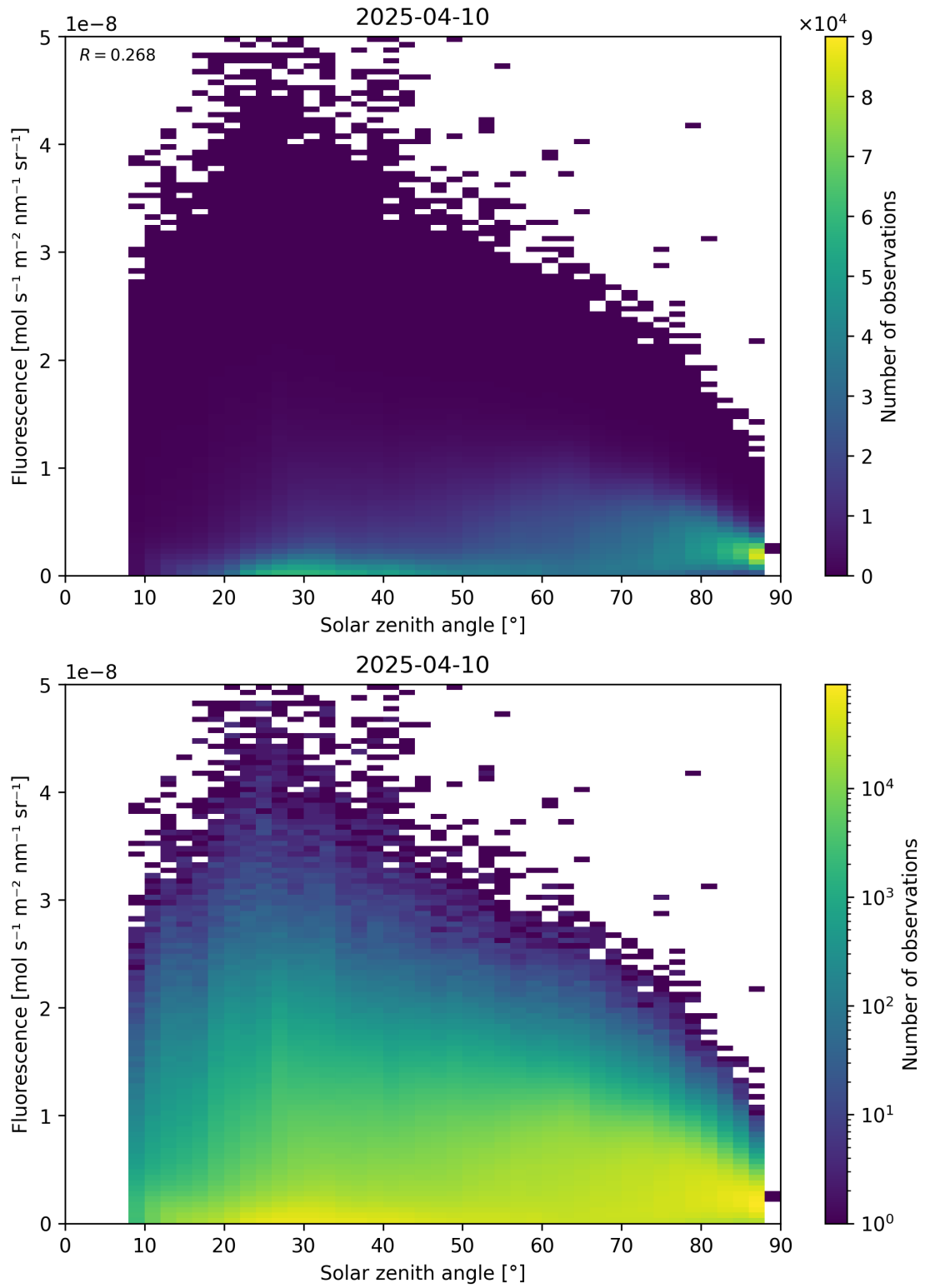
Figure 112: Scatter density plot of “Solar zenith angle” against “Fluorescence” for 2025-04-09 to 2025-04-11.
