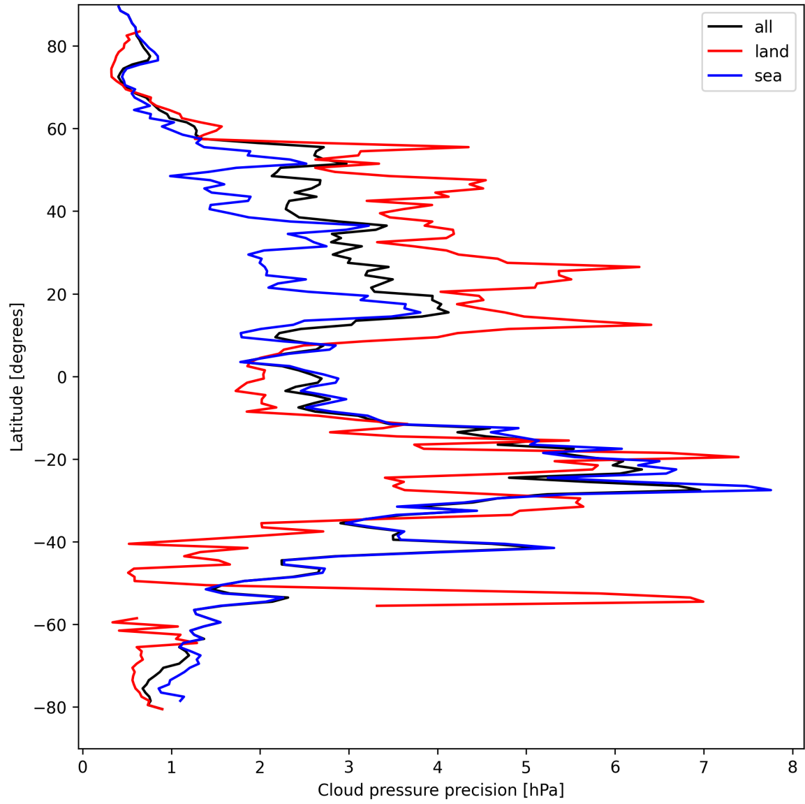
Figure 14: Zonal average of “Cloud pressure precision” for 2025-04-09 to 2025-04-11.
