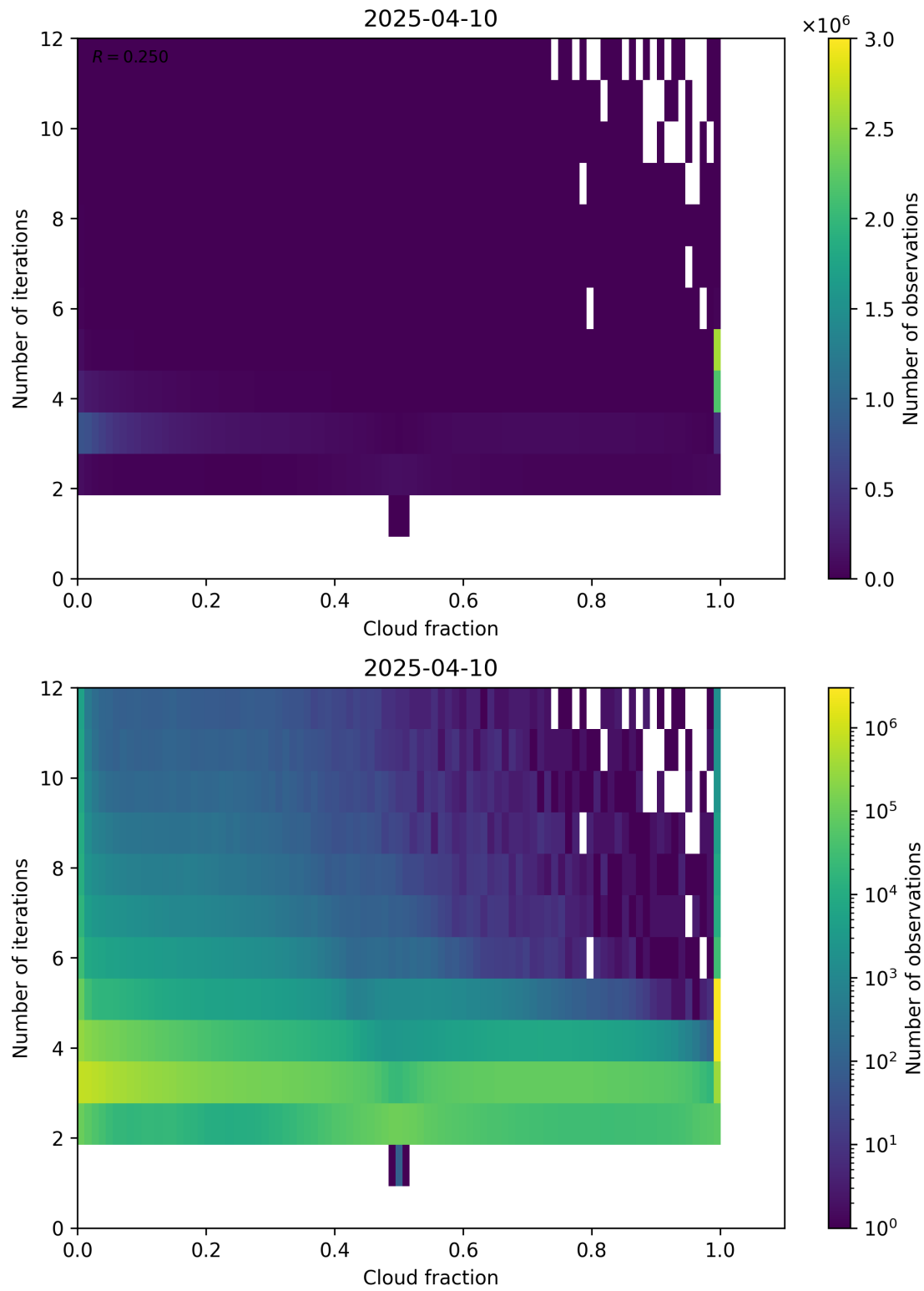
Figure 73: Scatter density plot of “Cloud fraction” against “Number of iterations” for 2025-04-09 to 2025-04-11.
