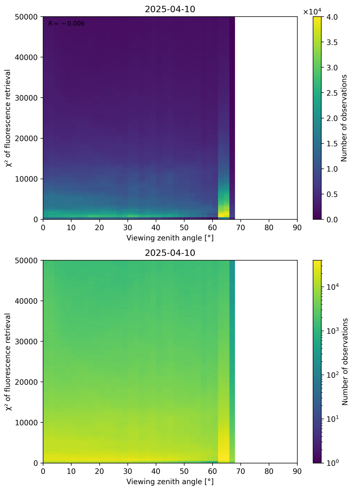
Figure 119: Scatter density plot of “Viewing zenith angle” against “ \chi^2 of fluorescence retrieval” for 2025-04-09 to 2025-04-11.
