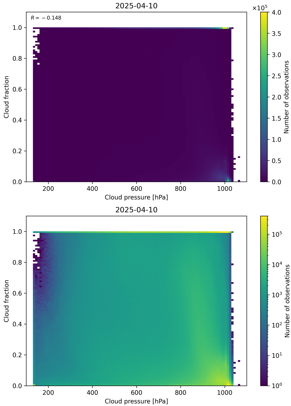
Figure 79: Scatter density plot of “Cloud pressure” against “Cloud fraction” for 2025-04-09 to 2025-04-11.
