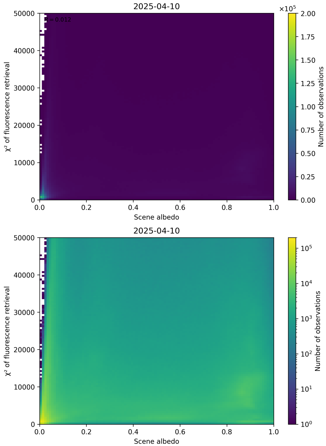
Figure 103: Scatter density plot of “Scene albedo” against “ \chi^2 of fluorescence retrieval” for 2025-04-09 to 2025-04-11.
