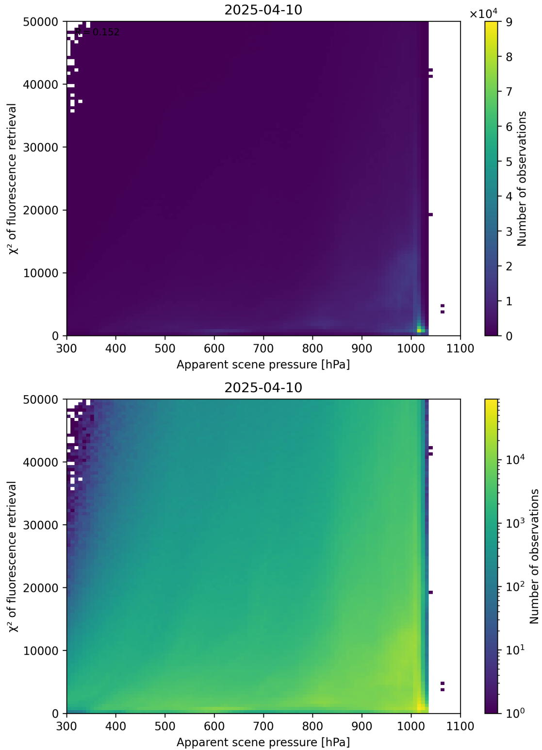
Figure 63: Scatter density plot of “Apparent scene pressure” against “ \chi^2 of fluorescence retrieval” for 2025-04-09 to 2025-04-11.
