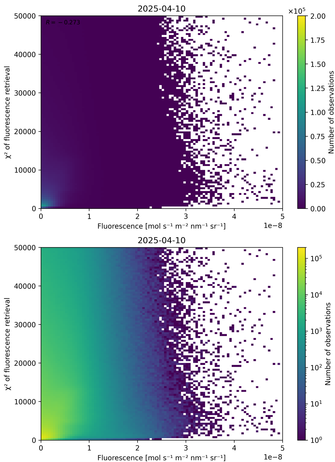
Figure 85: Scatter density plot of “Fluorescence” against “ \chi^2 of fluorescence retrieval” for 2025-04-09 to 2025-04-11.
