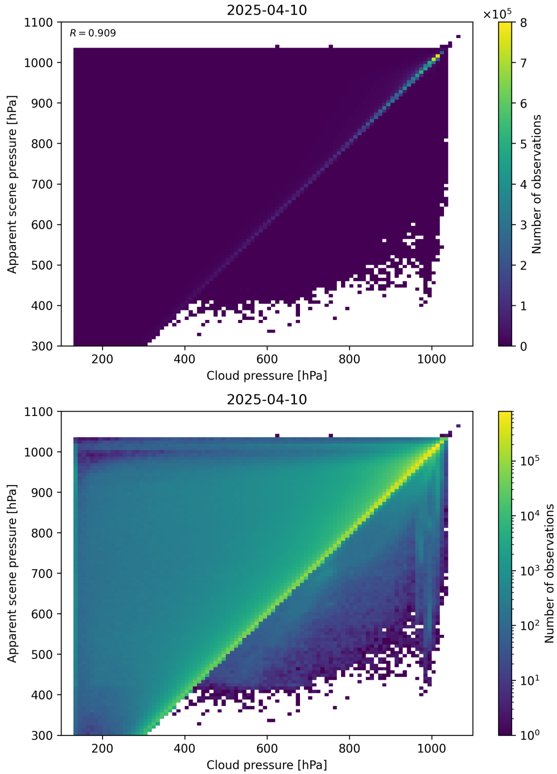
Figure 77: Scatter density plot of “Cloud pressure” against “Apparent scene pressure” for 2025-04-09 to 2025-04-11.
