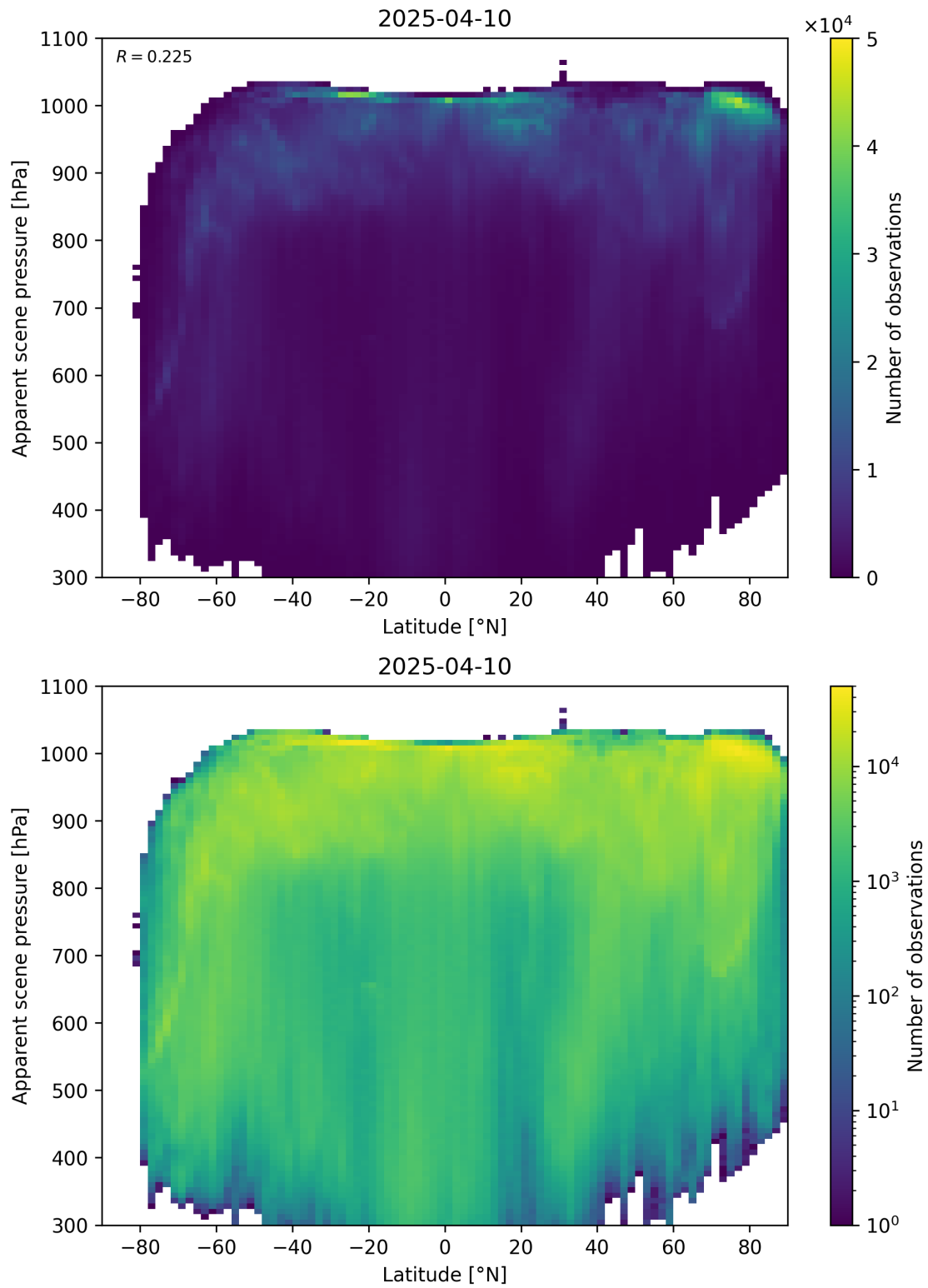
Figure 88: Scatter density plot of “Latitude” against “Apparent scene pressure” for 2025-04-09 to 2025-04-11.
