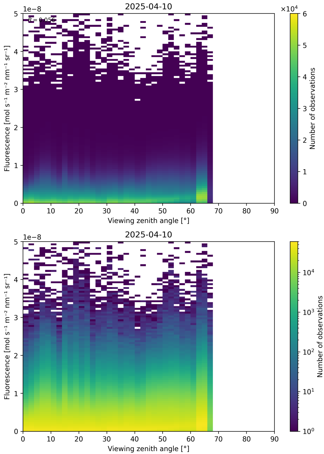
Figure 122: Scatter density plot of “Viewing zenith angle” against “Fluorescence” for 2025-04-09 to 2025-04-11.
