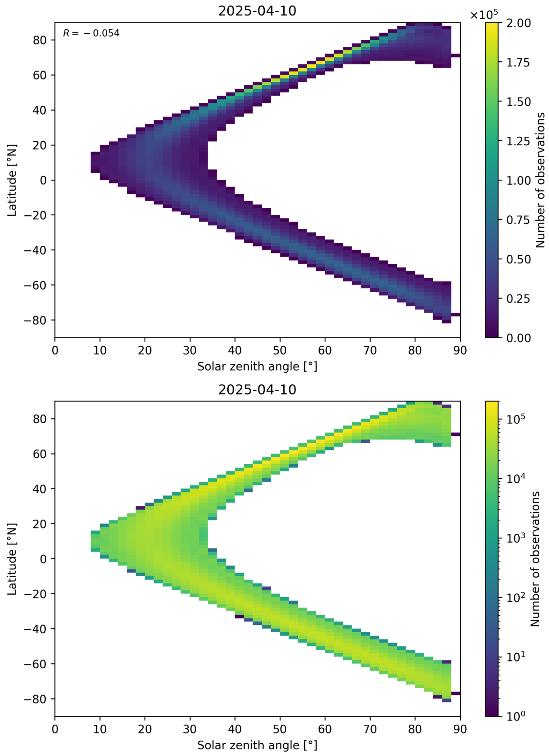
Figure 113: Scatter density plot of “Solar zenith angle” against “Latitude” for 2025-04-09 to 2025-04-11.
