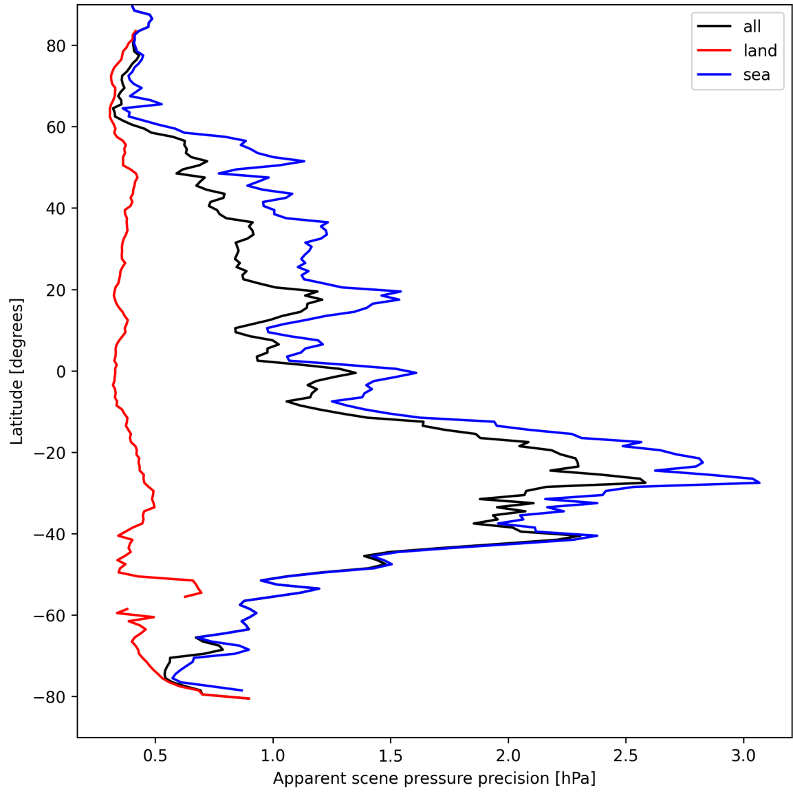
Figure 20: Zonal average of “Apparent scene pressure precision” for 2025-04-09 to 2025-04-11.
