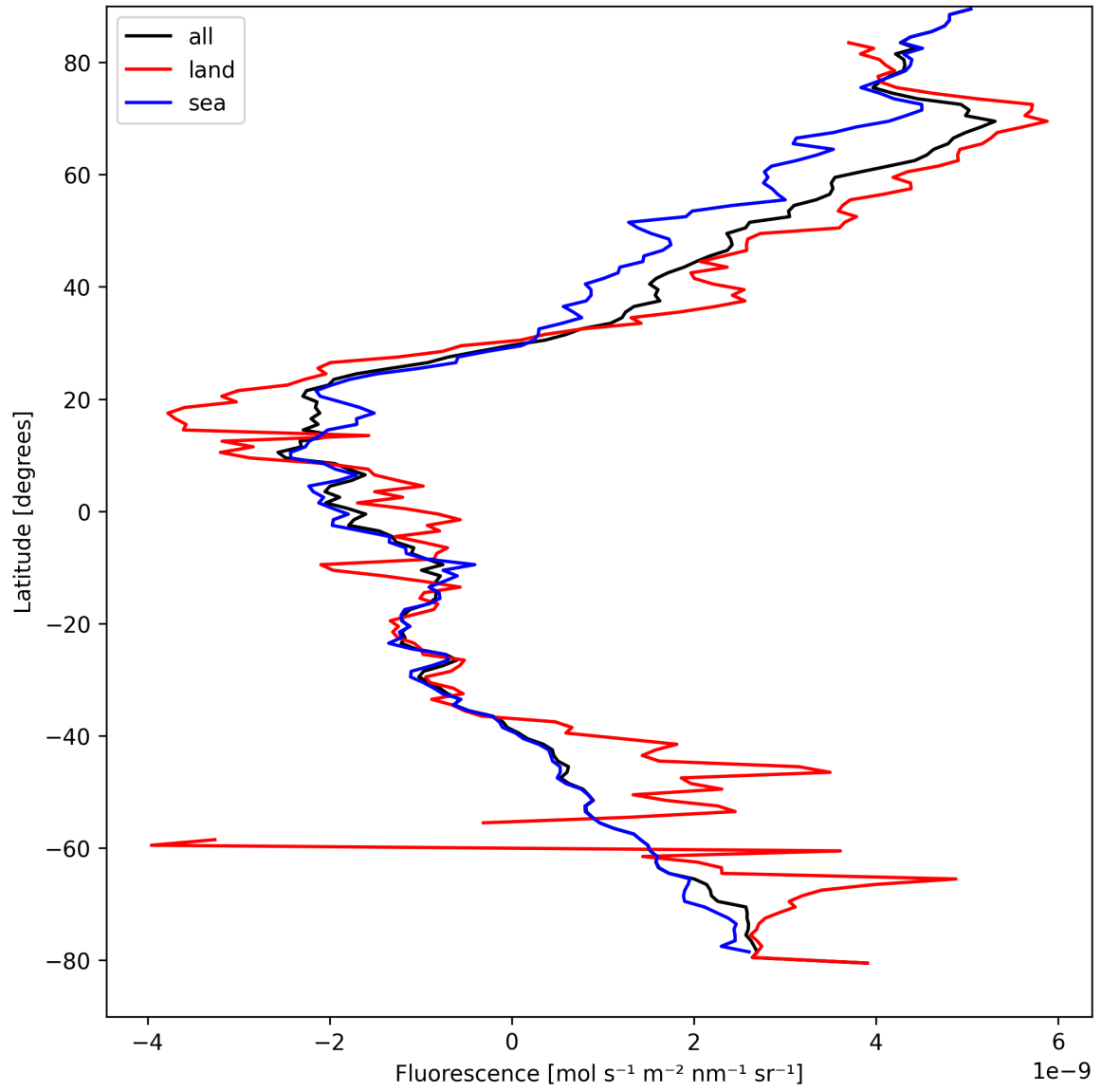
Figure 23: Zonal average of “Fluorescence” for 2025-04-09 to 2025-04-11.
