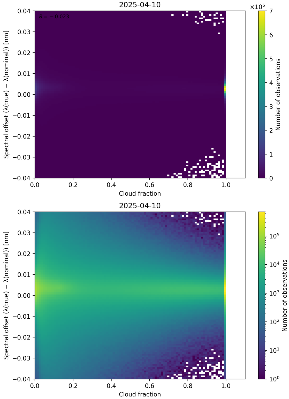
Figure 76: Scatter density plot of “Cloud fraction” against “Spectral offset ( \lambda_{\text{true}} - \lambda_{\text{nominal}} )” for 2025-04-09 to 2025-04-11.
