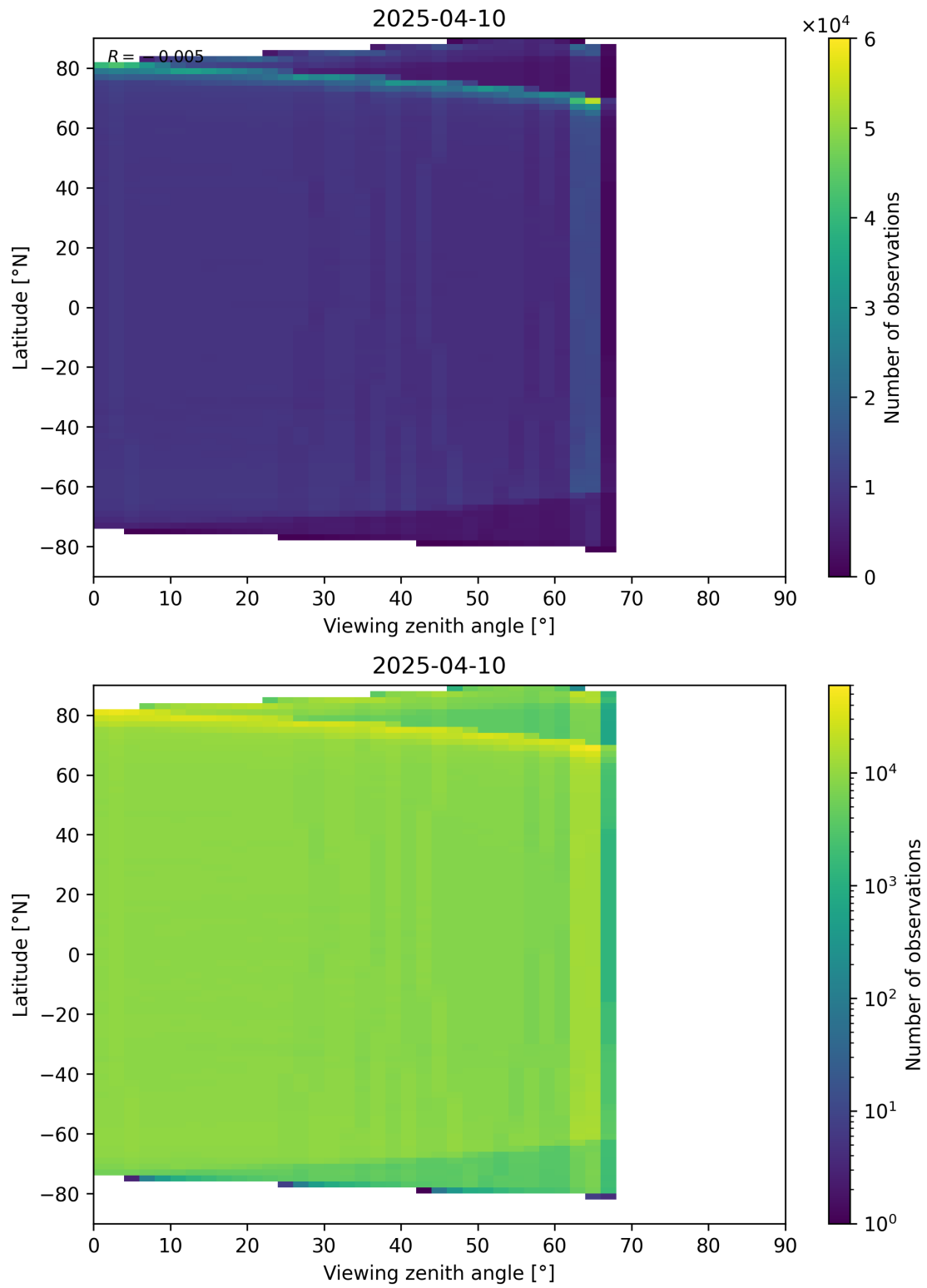
Figure 123: Scatter density plot of “Viewing zenith angle” against “Latitude” for 2025-04-09 to 2025-04-11.
