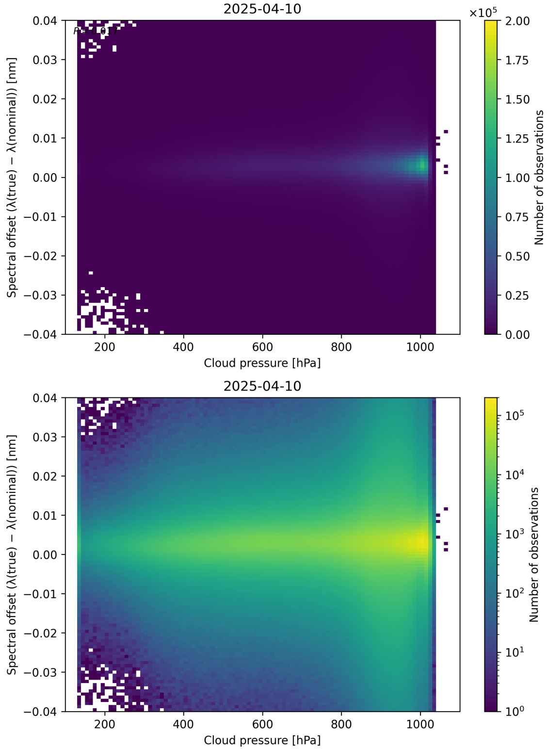
Figure 84: Scatter density plot of “Cloud pressure” against “Spectral offset ( \lambda_{\text{true}} - \lambda_{\text{nominal}} )” for 2025-04-09 to 2025-04-11.
