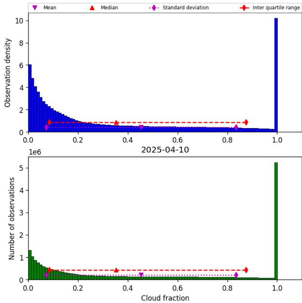
Figure 32: Histogram of “Cloud fraction” for 2025-04-09 to 2025-04-11
