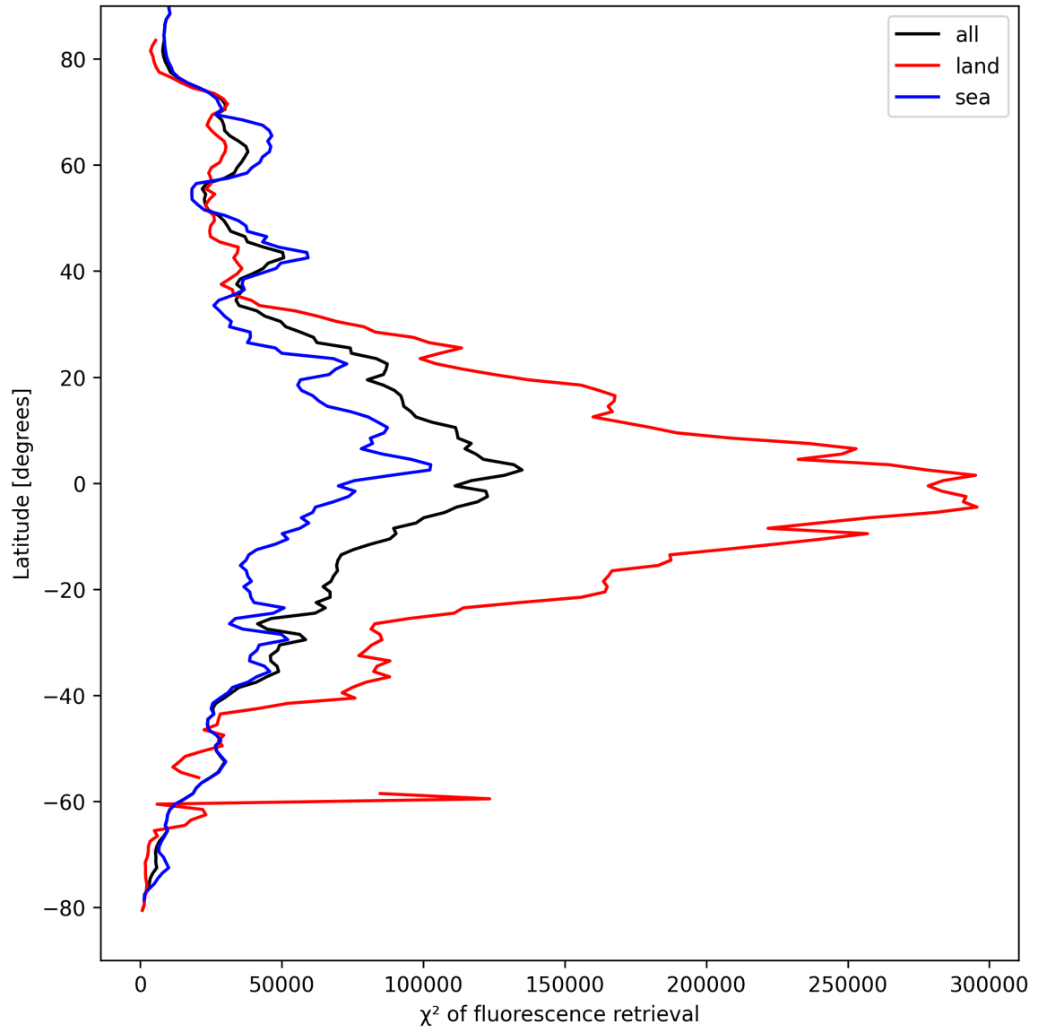
Figure 25: Zonal average of “ \chi^2 of fluorescence retrieval” for 2025-04-09 to 2025-04-11.
