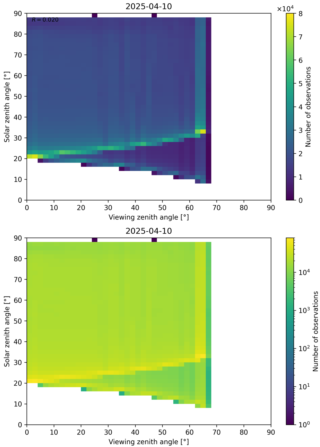
Figure 127: Scatter density plot of “Viewing zenith angle” against “Solar zenith angle” for 2025-04-09 to 2025-04-11.
