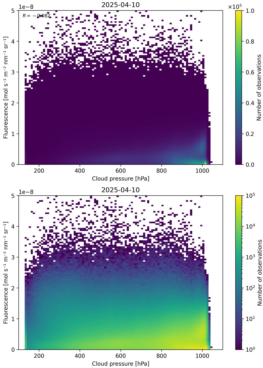
Figure 80: Scatter density plot of “Cloud pressure” against “Fluorescence” for 2025-04-09 to 2025-04-11.
