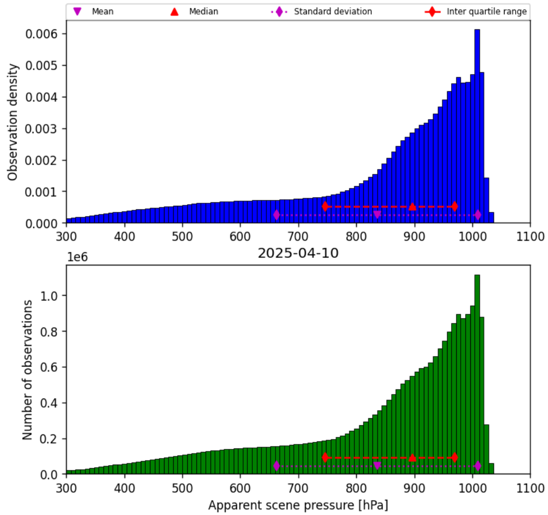
Figure 36: Histogram of “Apparent scene pressure” for 2025-04-09 to 2025-04-11
