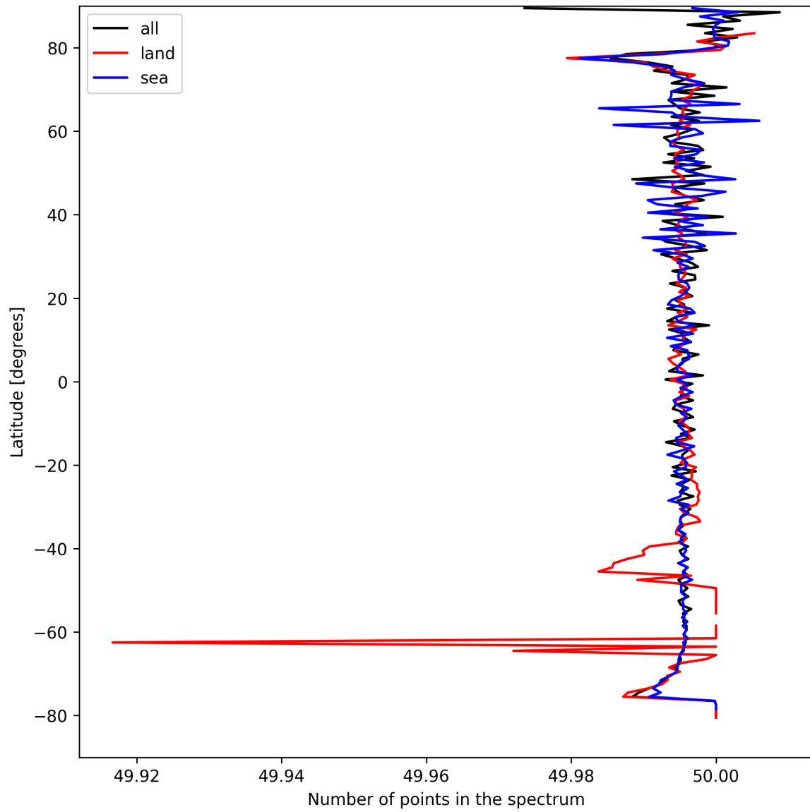
Figure 27: Zonal average of “Number of points in the spectrum” for 2025-04-09 to 2025-04-11.
