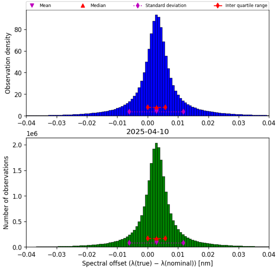
Figure 45: Histogram of “Spectral offset ( \lambda_{\text{true}} - \lambda_{\text{nominal}} )” for 2025-04-09 to 2025-04-11
