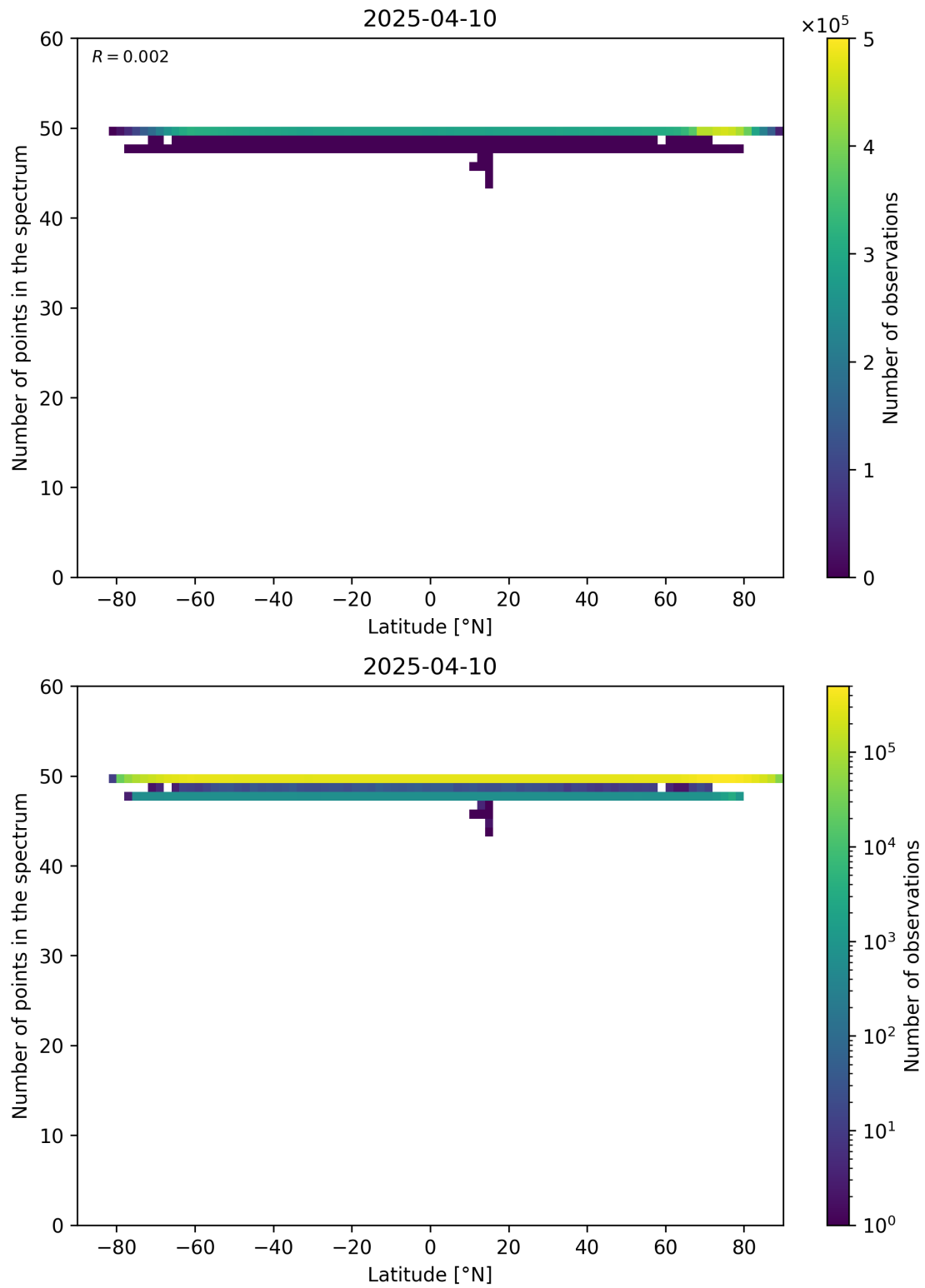
Figure 94: Scatter density plot of “Latitude” against “Number of points in the spectrum” for 2025-04-09 to 2025-04-11.
