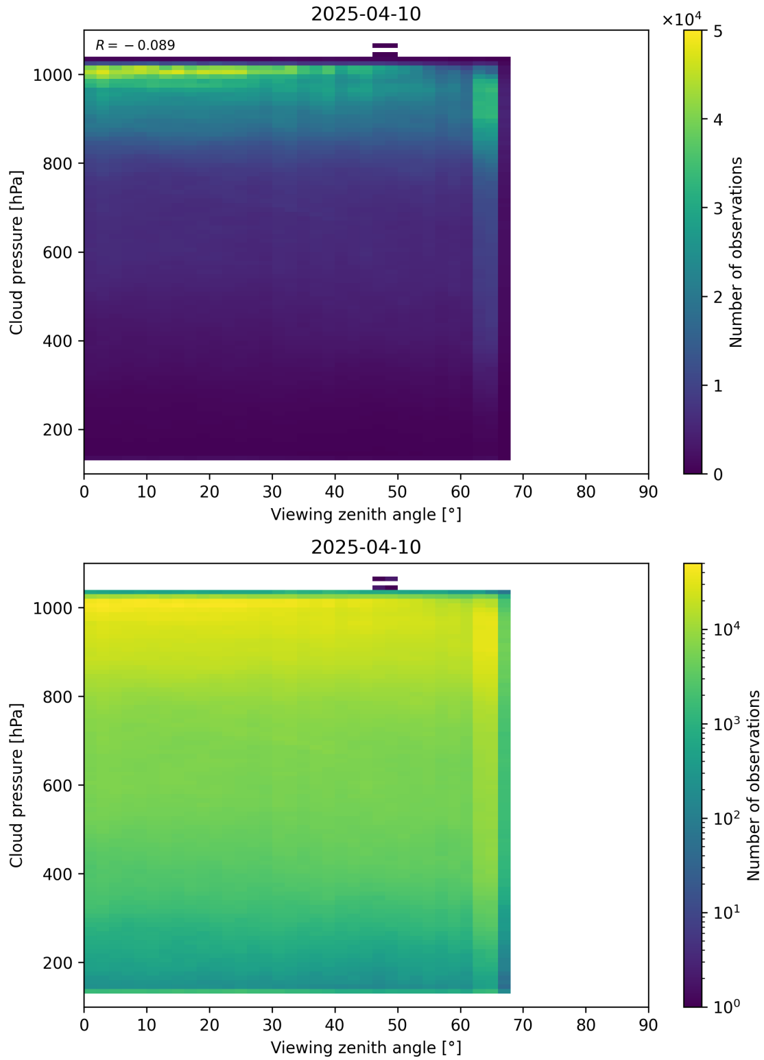
Figure 121: Scatter density plot of “Viewing zenith angle” against “Cloud pressure” for 2025-04-09 to 2025-04-11.
