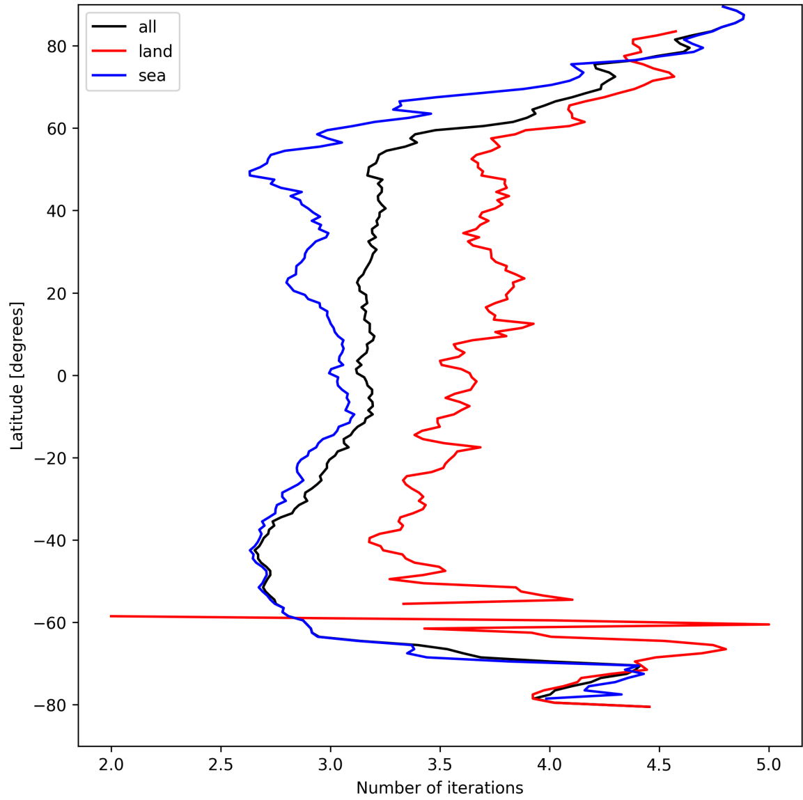
Figure 22: Zonal average of “Number of iterations” for 2025-04-09 to 2025-04-11.
