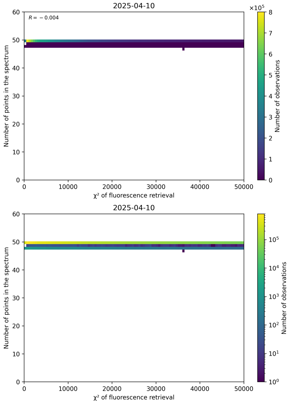
Figure 68: Scatter density plot of " \chi^2 of fluorescence retrieval" against "Number of points in the spectrum" for 2025-04-09 to 2025-04-11.
