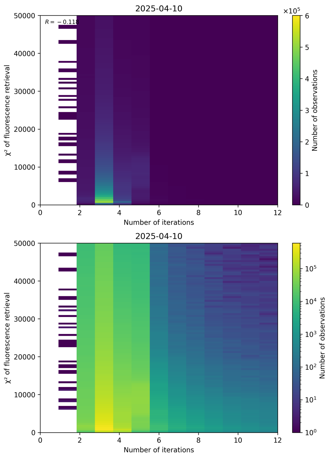
Figure 97: Scatter density plot of “Number of iterations” against “ \chi^2 of fluorescence retrieval” for 2025-04-09 to 2025-04-11.
