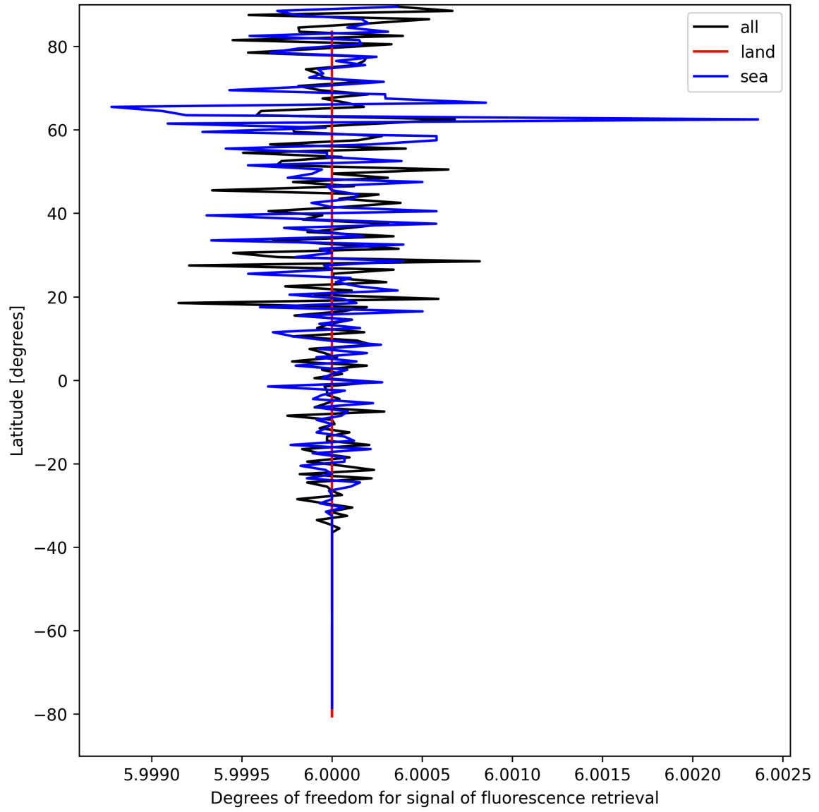
Figure 26: Zonal average of “Degrees of freedom for signal of fluorescence retrieval” for 2025-04-09 to 2025-04-11.
