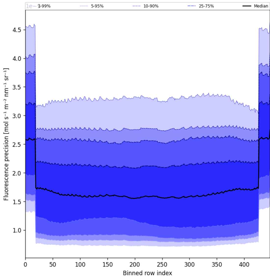
Figure 58: Along track statistics of “Fluorescence precision” for 2025-04-09 to 2025-04-11
