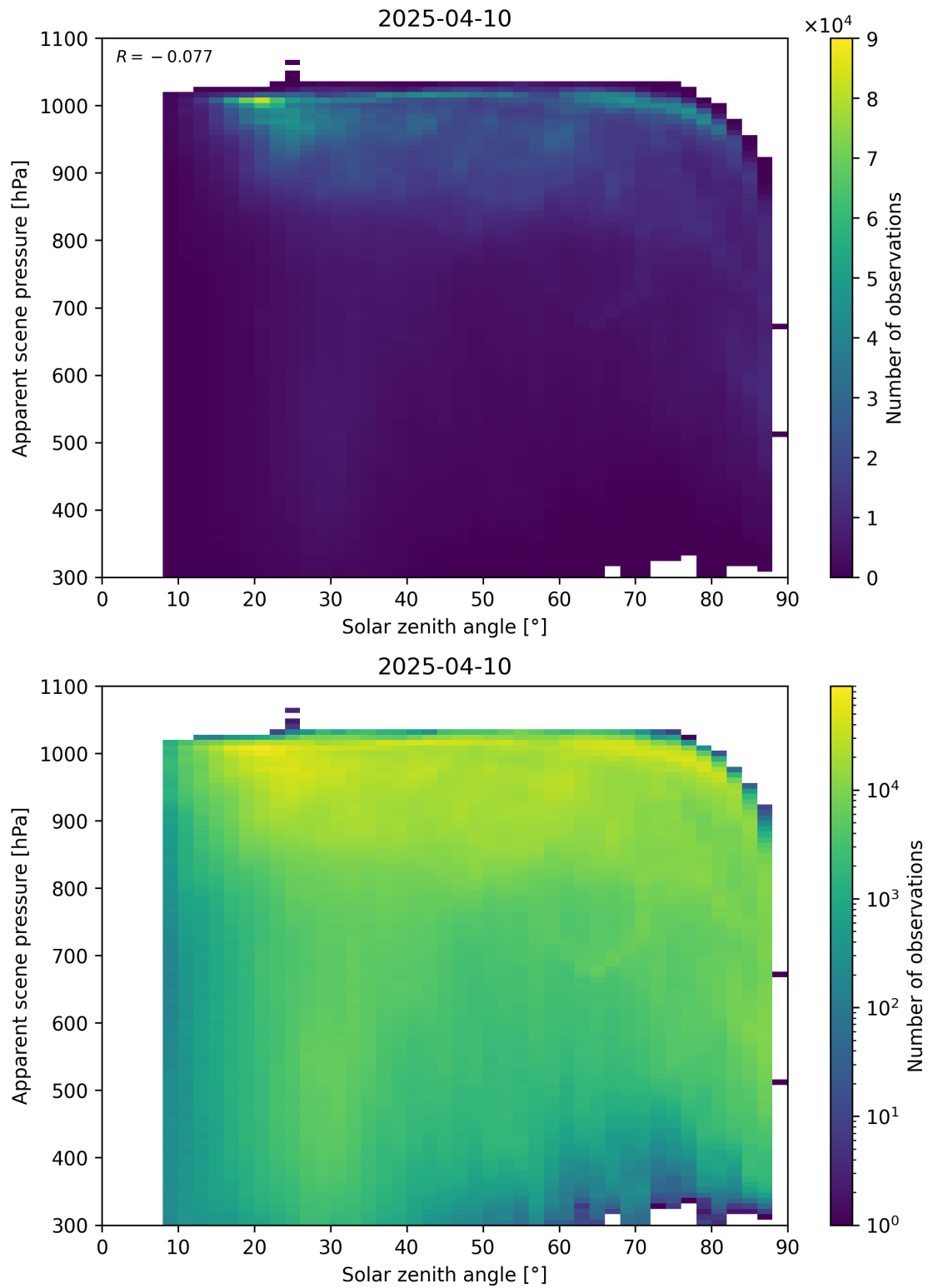
Figure 108: Scatter density plot of “Solar zenith angle” against “Apparent scene pressure” for 2025-04-09 to 2025-04-11.
