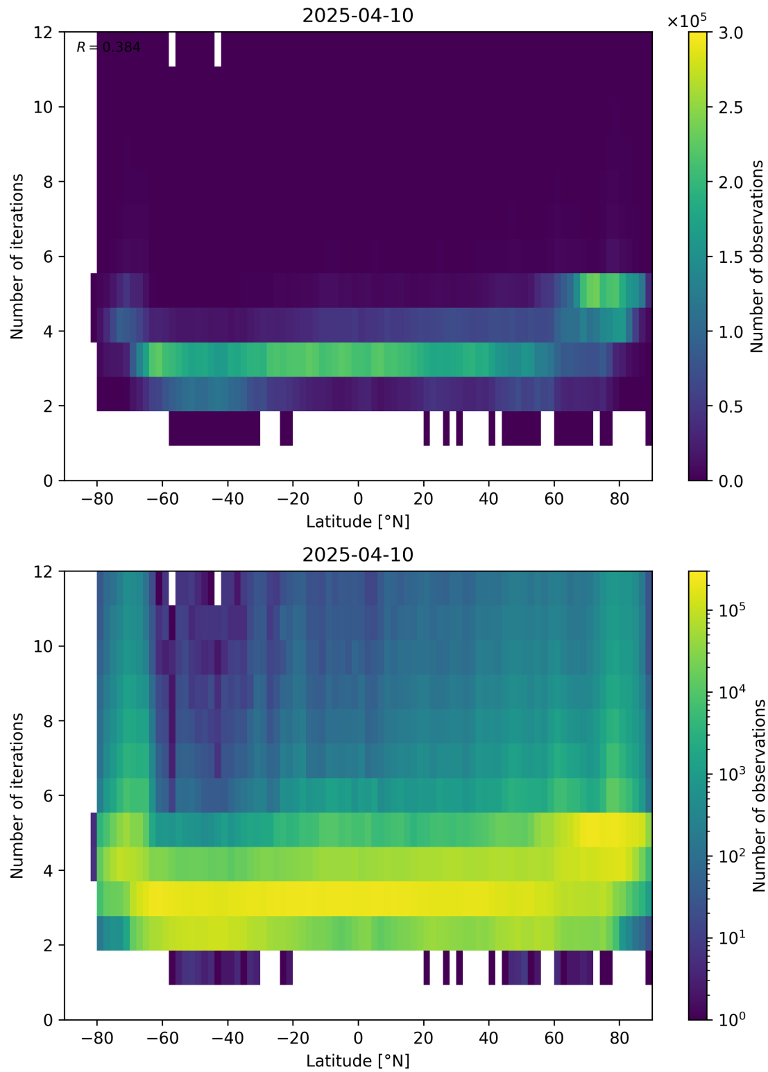
Figure 93: Scatter density plot of “Latitude” against “Number of iterations” for 2025-04-09 to 2025-04-11.
