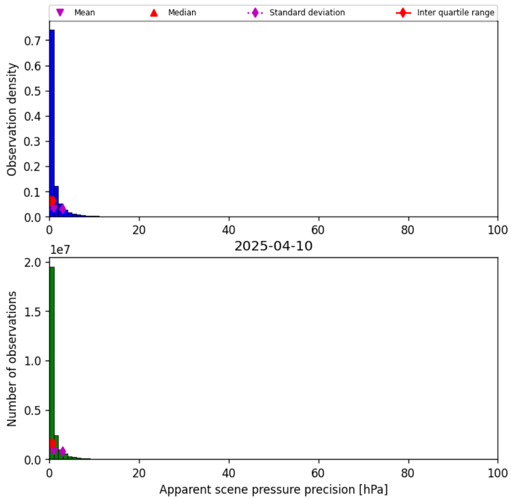
Figure 37: Histogram of “Apparent scene pressure precision” for 2025-04-09 to 2025-04-11
