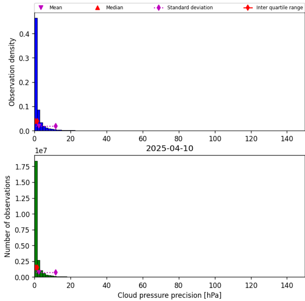
Figure 31: Histogram of “Cloud pressure precision” for 2025-04-09 to 2025-04-11
