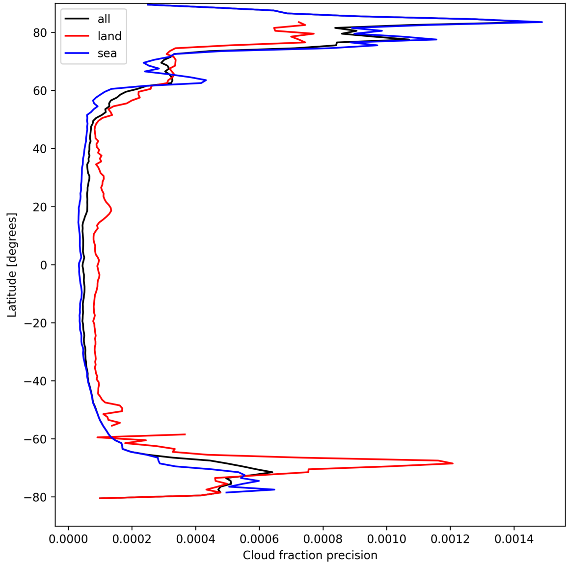
Figure 16: Zonal average of “Cloud fraction precision” for 2025-04-09 to 2025-04-11.
