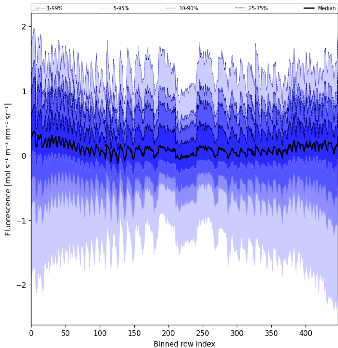
Figure 57: Along track statistics of “Fluorescence” for 2025-04-09 to 2025-04-11
