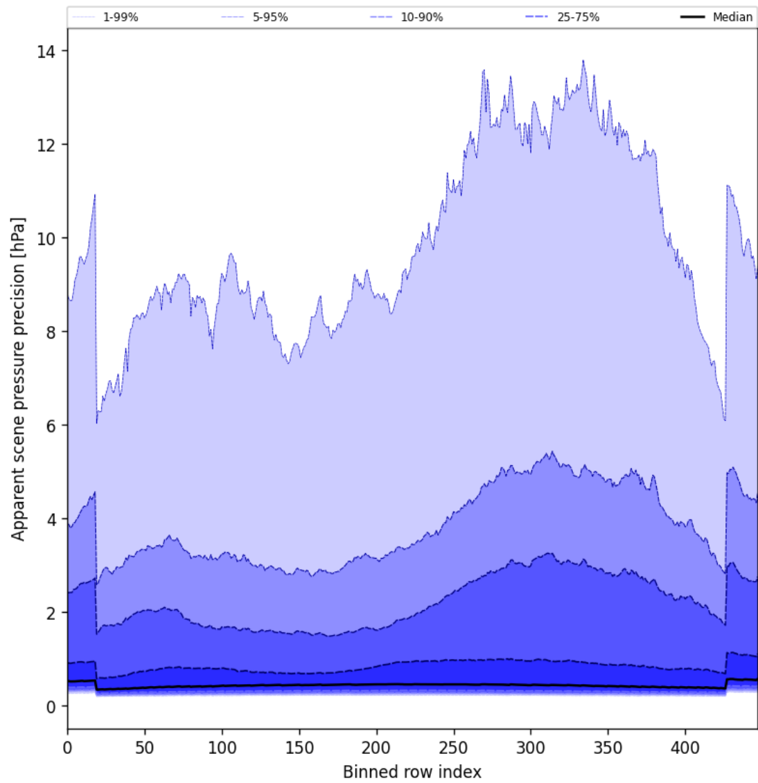
Figure 54: Along track statistics of “Apparent scene pressure precision” for 2025-04-09 to 2025-04-11
