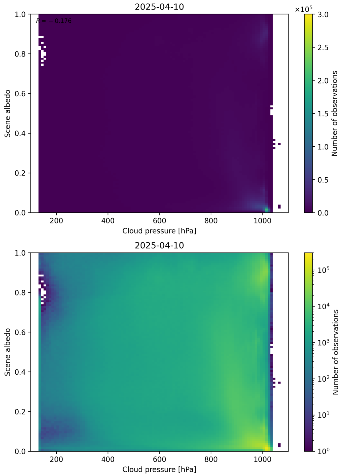
Figure 83: Scatter density plot of “Cloud pressure” against “Scene albedo” for 2025-04-09 to 2025-04-11.
