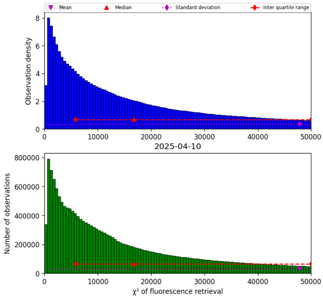
Figure 42: Histogram of “ \chi^2 of fluorescence retrieval” for 2025-04-09 to 2025-04-11
