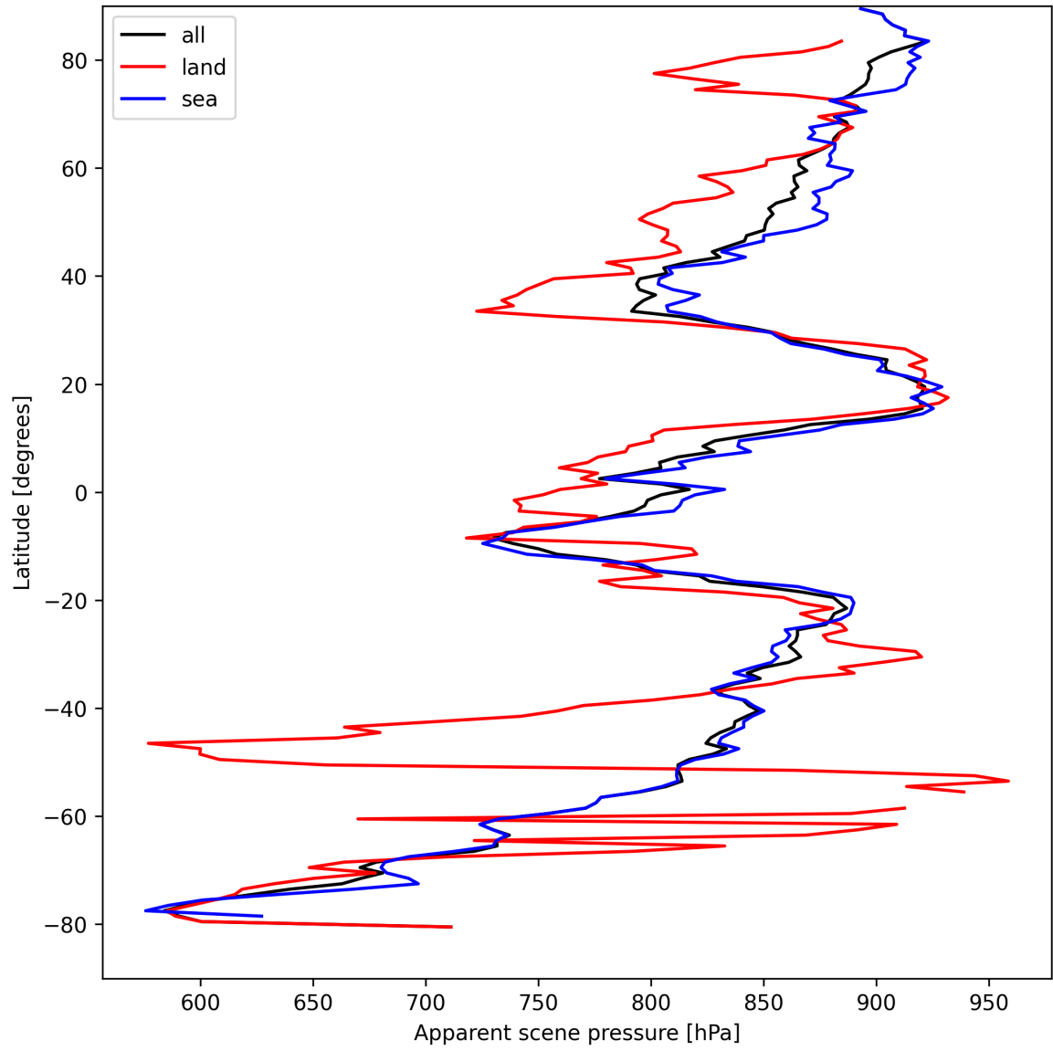
Figure 19: Zonal average of “Apparent scene pressure” for 2025-04-09 to 2025-04-11.
