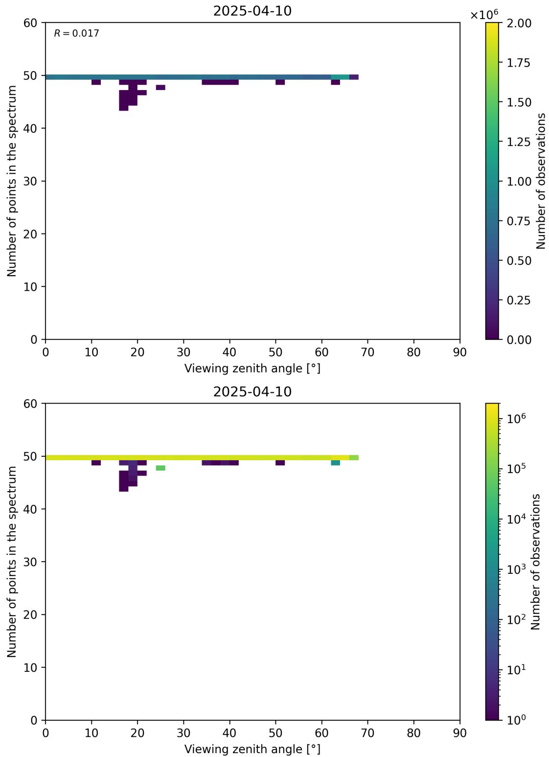
Figure 125: Scatter density plot of “Viewing zenith angle” against “Number of points in the spectrum” for 2025-04-09 to 2025-04-11.
