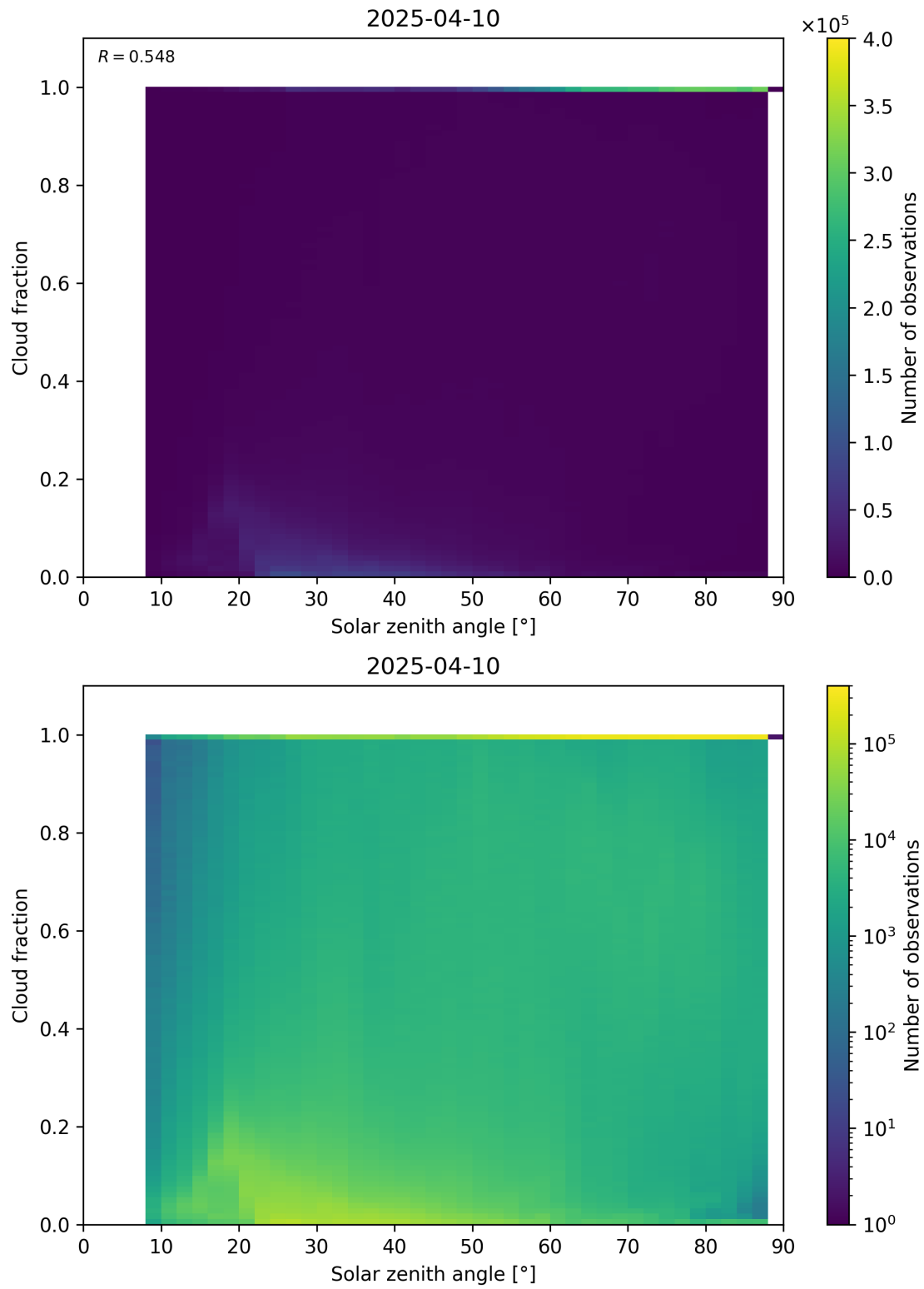
Figure 110: Scatter density plot of “Solar zenith angle” against “Cloud fraction” for 2025-04-09 to 2025-04-11.
