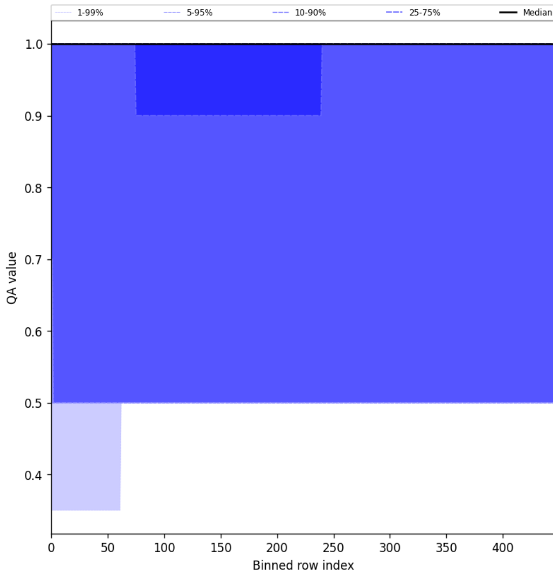
Figure 46: Along track statistics of “QA value” for 2025-04-09 to 2025-04-11
