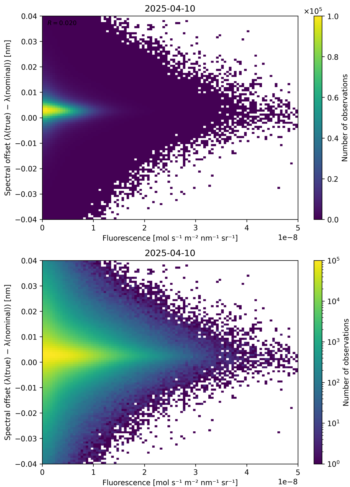
Figure 87: Scatter density plot of “Fluorescence” against “Spectral offset ( \lambda_{\text{true}} - \lambda_{\text{nominal}} )” for 2025-04-09 to 2025-04-11.
