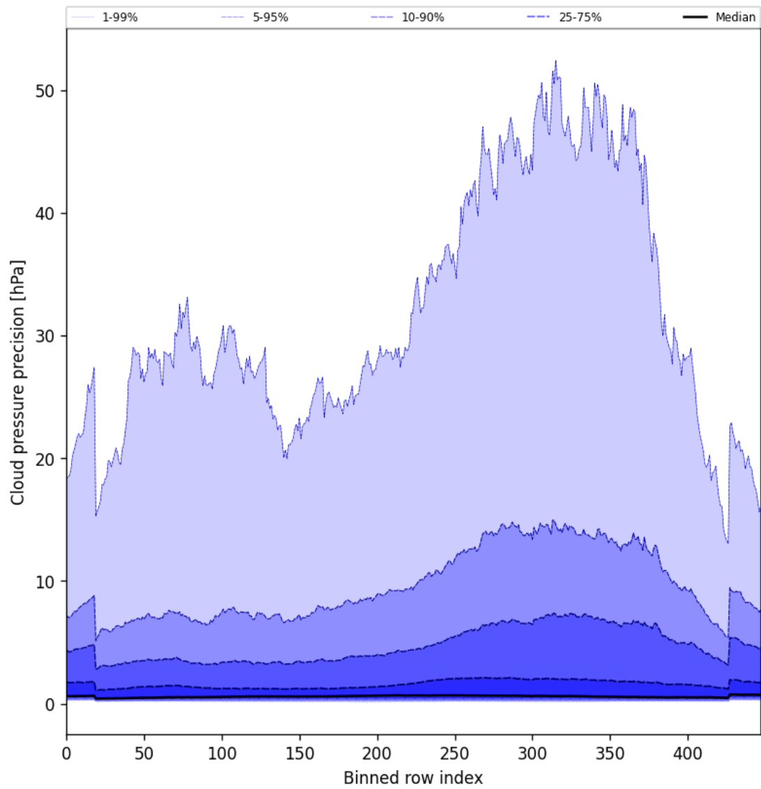
Figure 48: Along track statistics of “Cloud pressure precision” for 2025-04-09 to 2025-04-11
