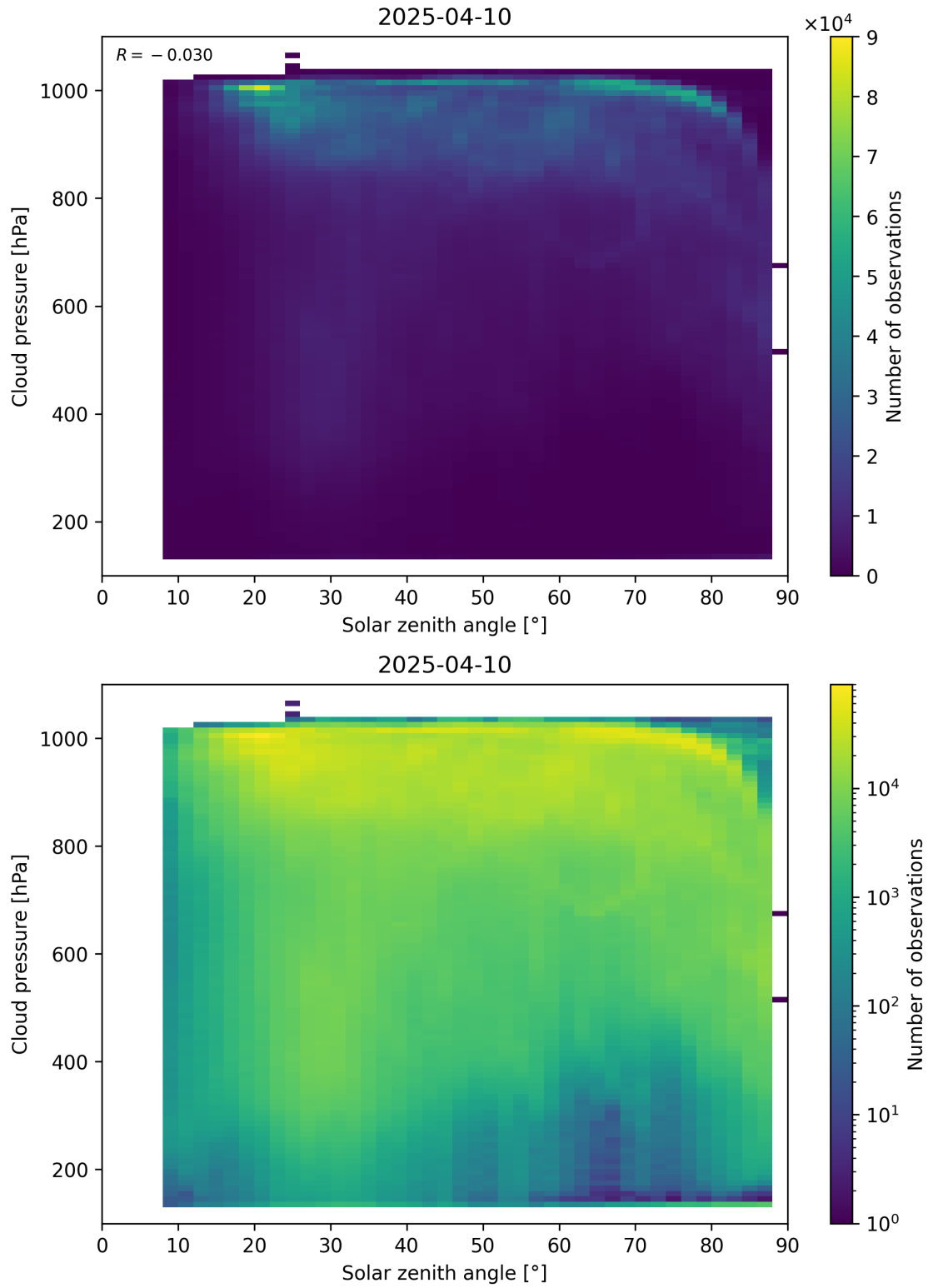
Figure 111: Scatter density plot of “Solar zenith angle” against “Cloud pressure” for 2025-04-09 to 2025-04-11.
