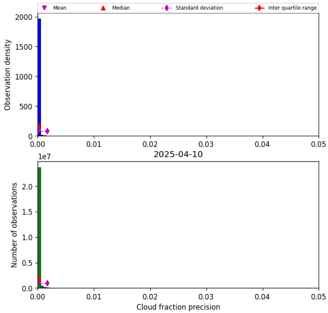
Figure 33: Histogram of “Cloud fraction precision” for 2025-04-09 to 2025-04-11
