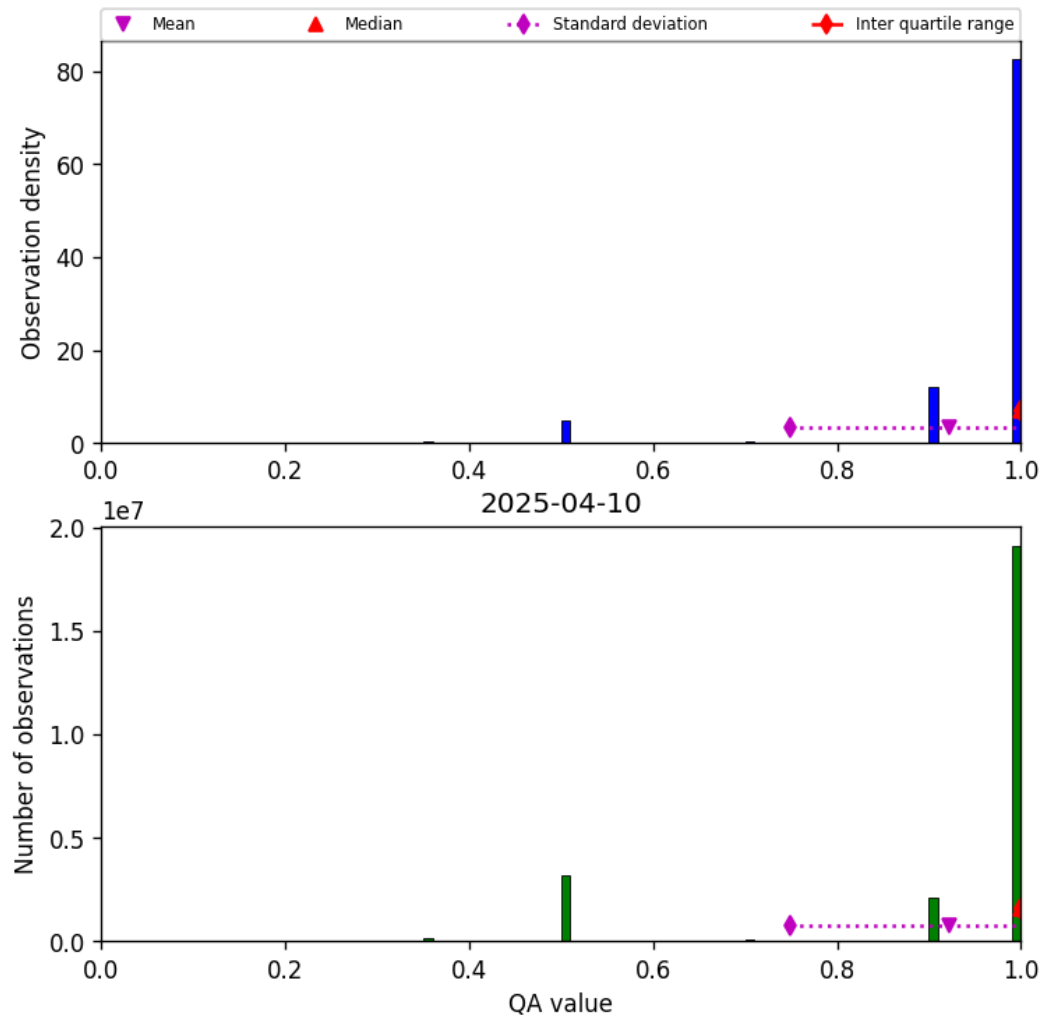
Figure 29: Histogram of “QA value” for 2025-04-09 to 2025-04-11
