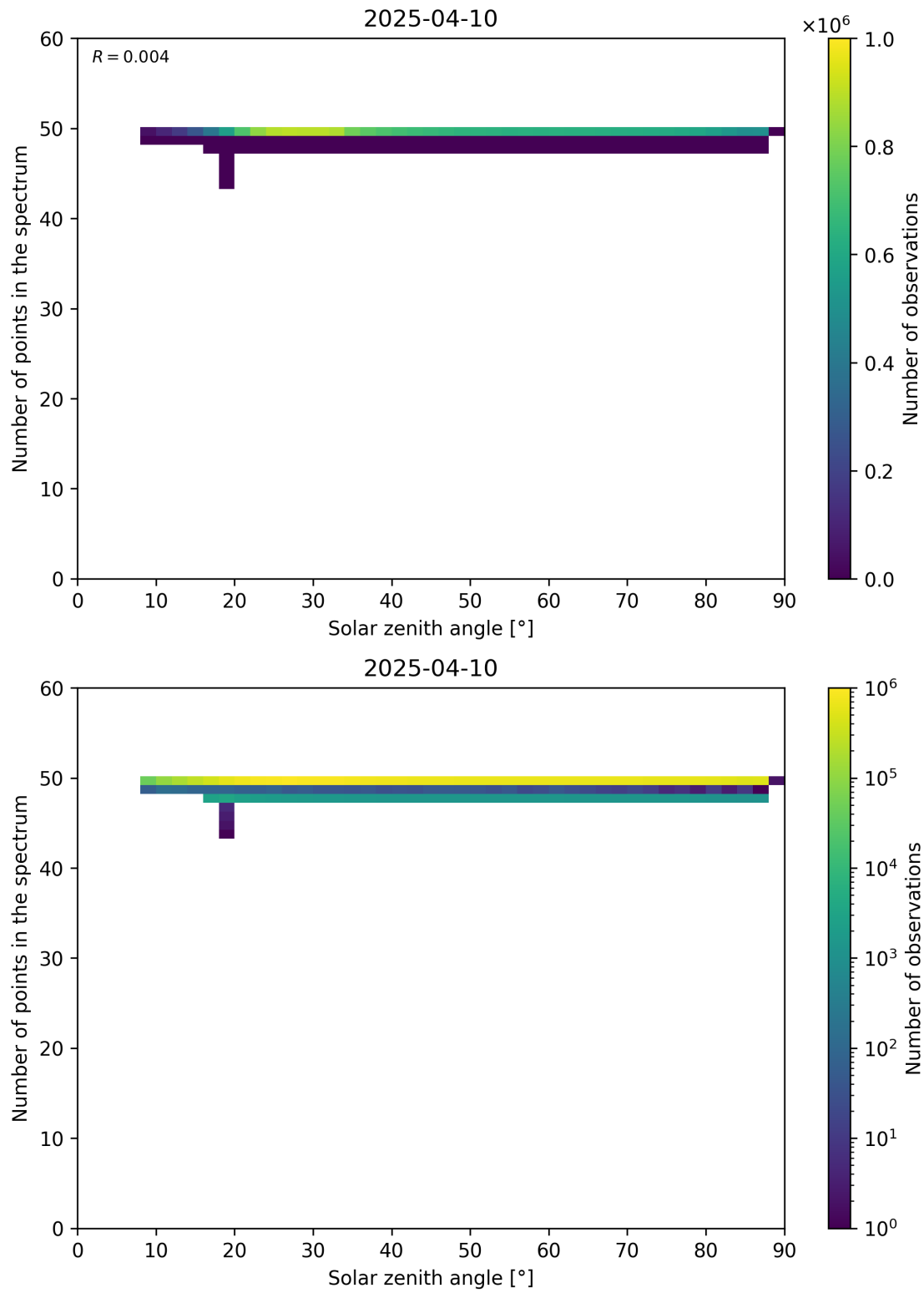
Figure 115: Scatter density plot of “Solar zenith angle” against “Number of points in the spectrum” for 2025-04-09 to 2025-04-11.
