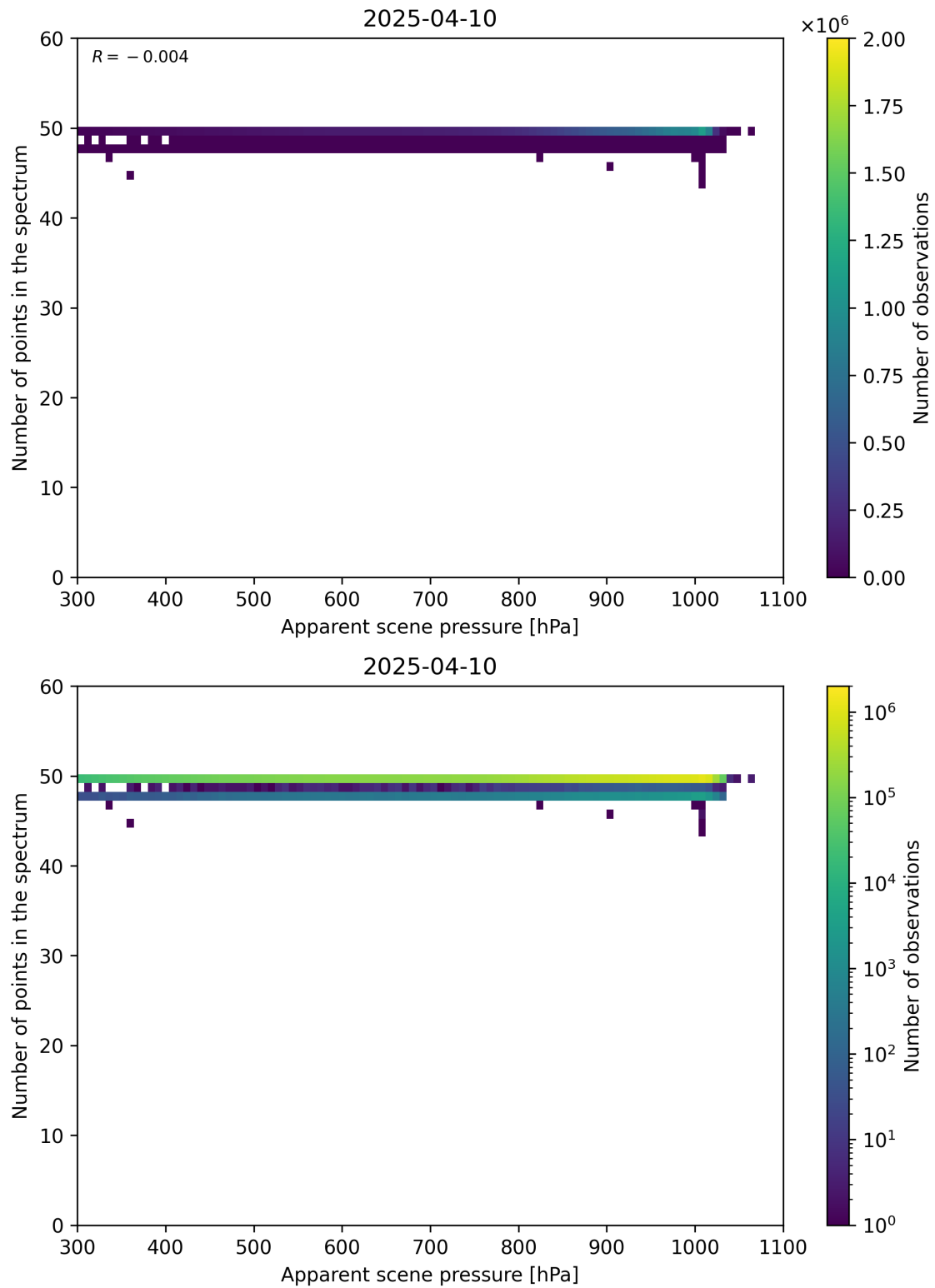
Figure 66: Scatter density plot of “Apparent scene pressure” against “Number of points in the spectrum” for 2025-04-09 to 2025-04-11.
