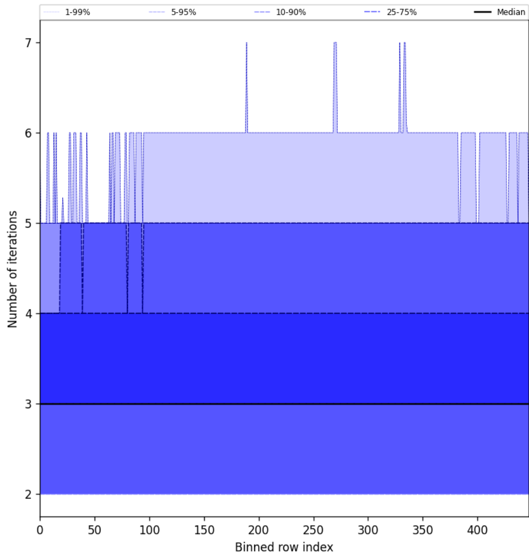
Figure 56: Along track statistics of “Number of iterations” for 2025-04-09 to 2025-04-11
