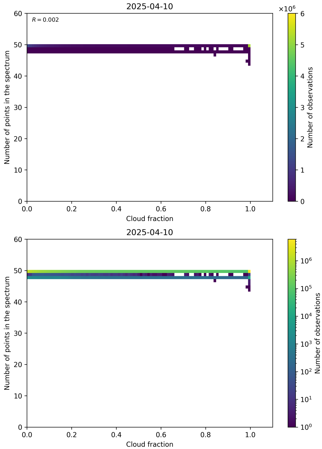
Figure 74: Scatter density plot of “Cloud fraction” against “Number of points in the spectrum” for 2025-04-09 to 2025-04-11.
