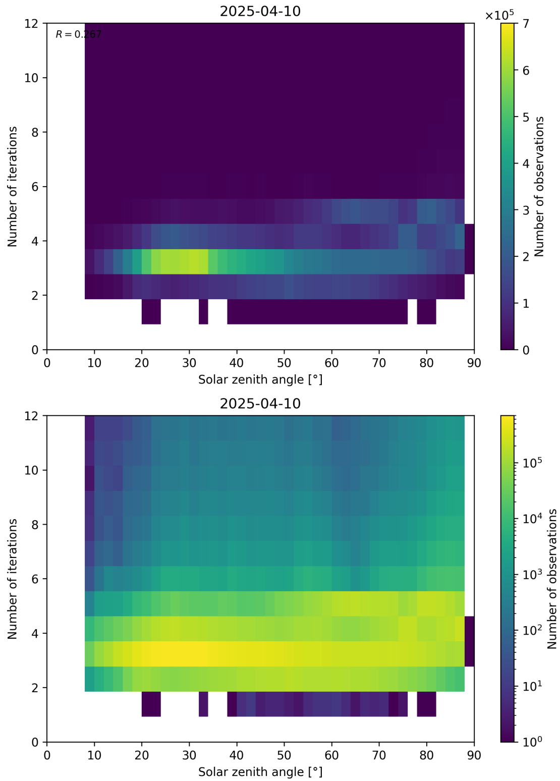
Figure 114: Scatter density plot of “Solar zenith angle” against “Number of iterations” for 2025-04-09 to 2025-04-11.
