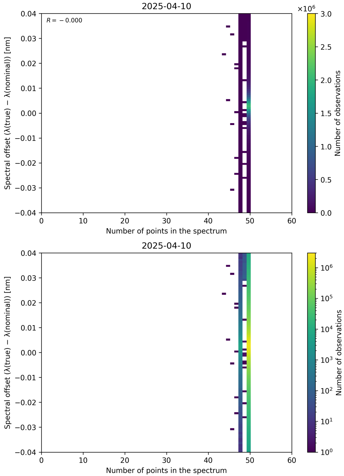
Figure 101: Scatter density plot of “Number of points in the spectrum” against “Spectral offset ( \lambda_{\text{true}} - \lambda_{\text{nominal}} )” for 2025-04-09 to 2025-04-11.
