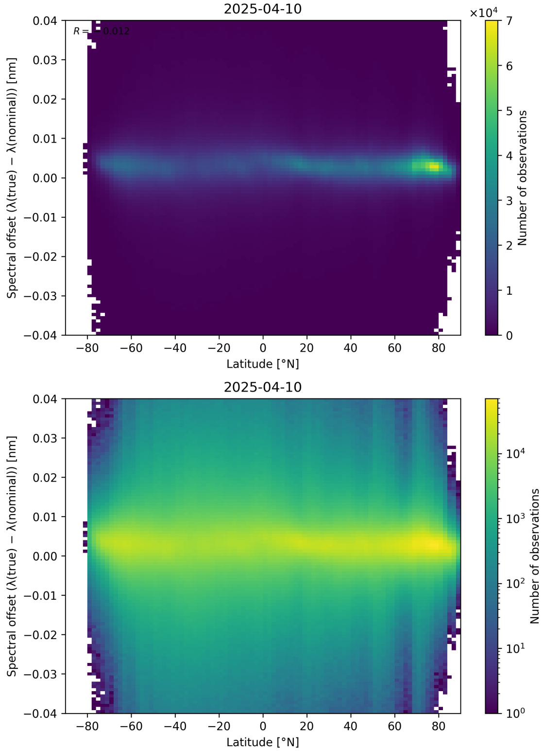
Figure 96: Scatter density plot of “Latitude” against “Spectral offset ( \lambda_{\text{true}} - \lambda_{\text{nominal}} )” for 2025-04-09 to 2025-04-11.
