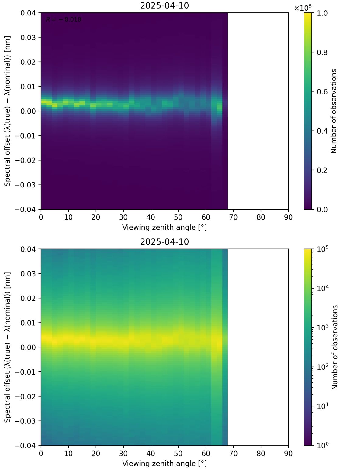
Figure 128: Scatter density plot of “Viewing zenith angle” against “Spectral offset ( \lambda_{\text{true}} - \lambda_{\text{nominal}} )” for 2025-04-09 to 2025-04-11.
