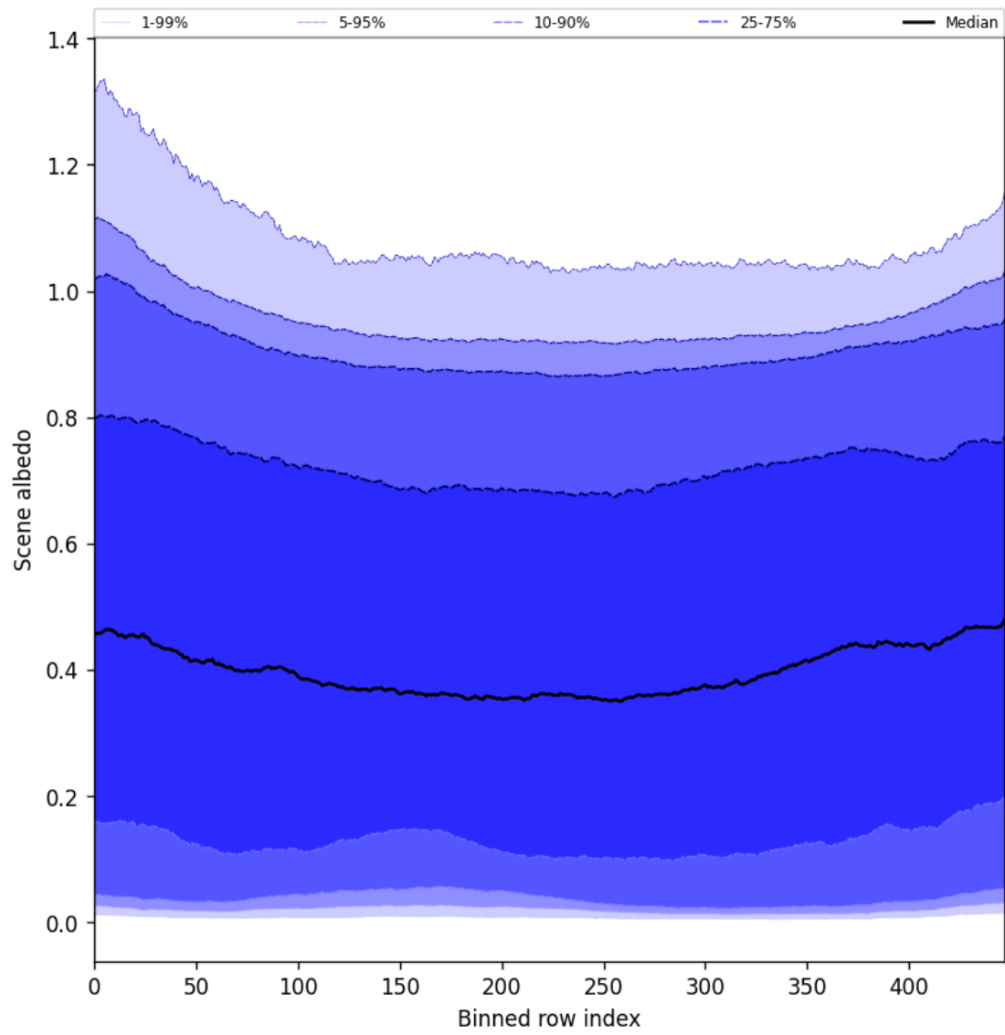
Figure 51: Along track statistics of “Scene albedo” for 2025-04-09 to 2025-04-11
