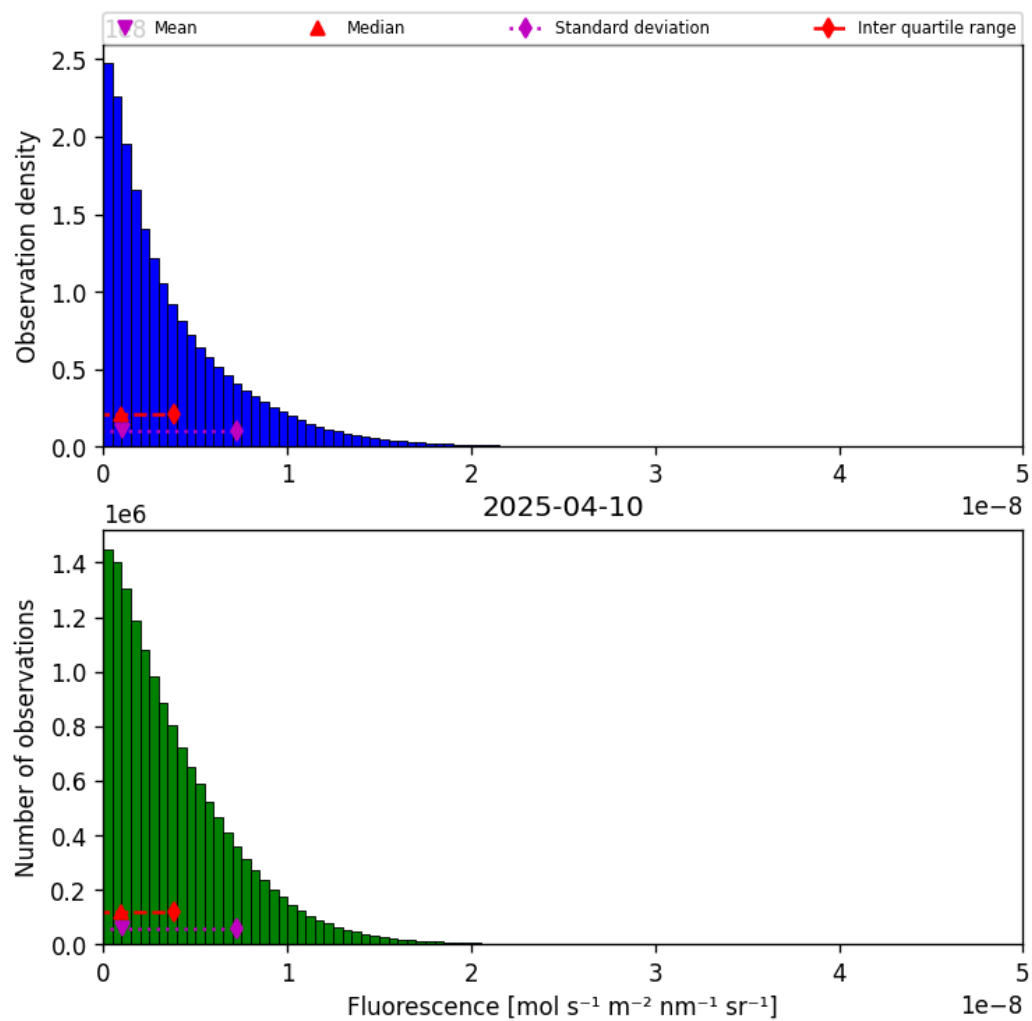
Figure 40: Histogram of “Fluorescence” for 2025-04-09 to 2025-04-11
