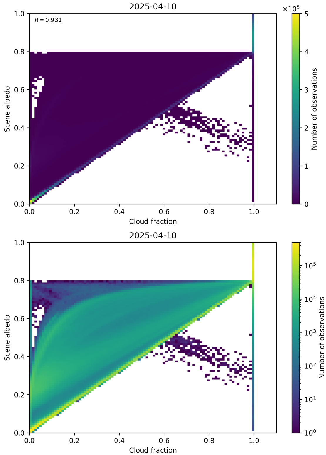
Figure 75: Scatter density plot of “Cloud fraction” against “Scene albedo” for 2025-04-09 to 2025-04-11.
