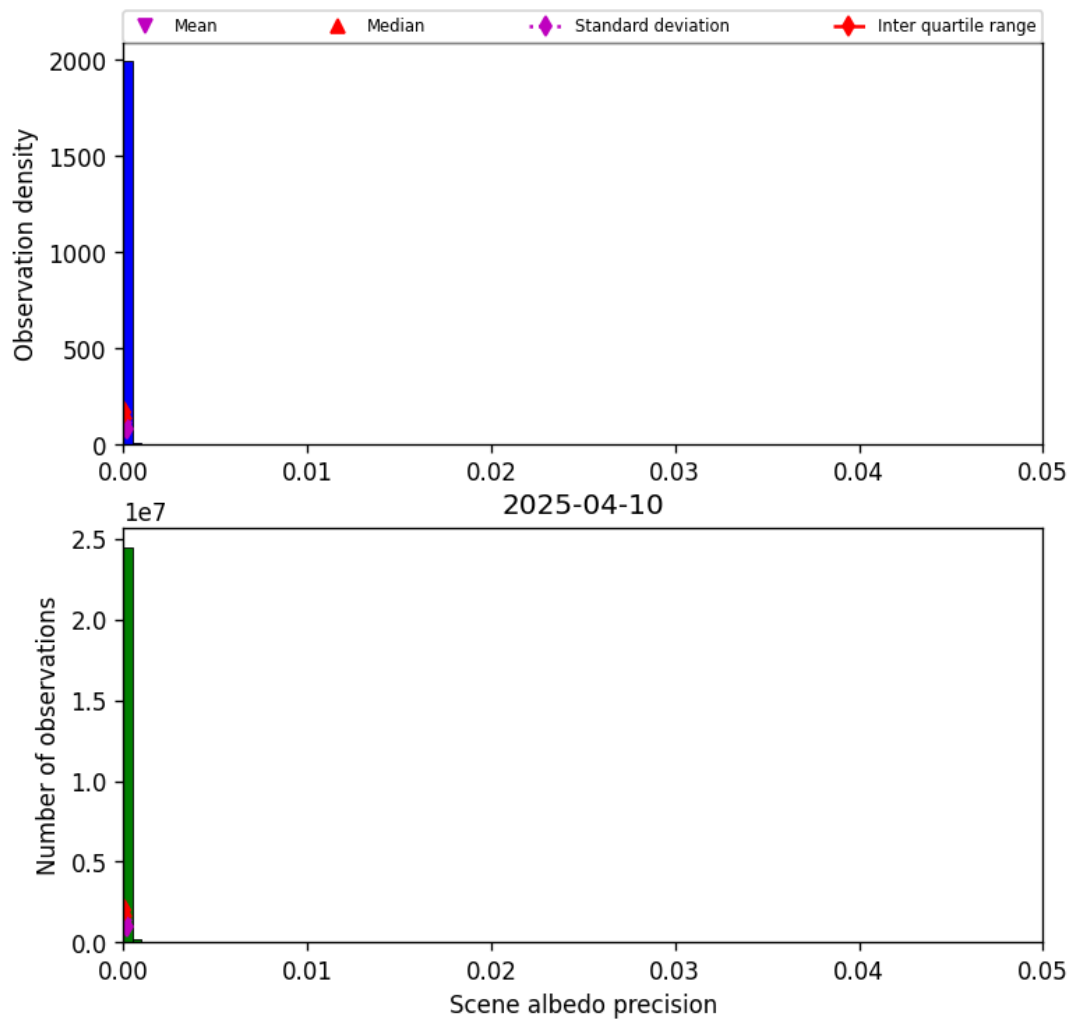
Figure 35: Histogram of “Scene albedo precision” for 2025-04-09 to 2025-04-11
