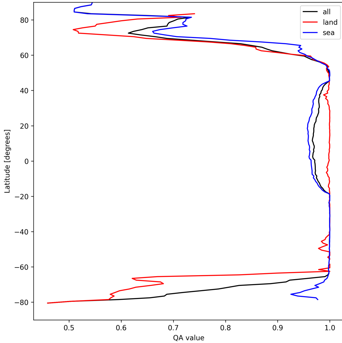
Figure 12: Zonal average of “QA value” for 2025-04-09 to 2025-04-11.
