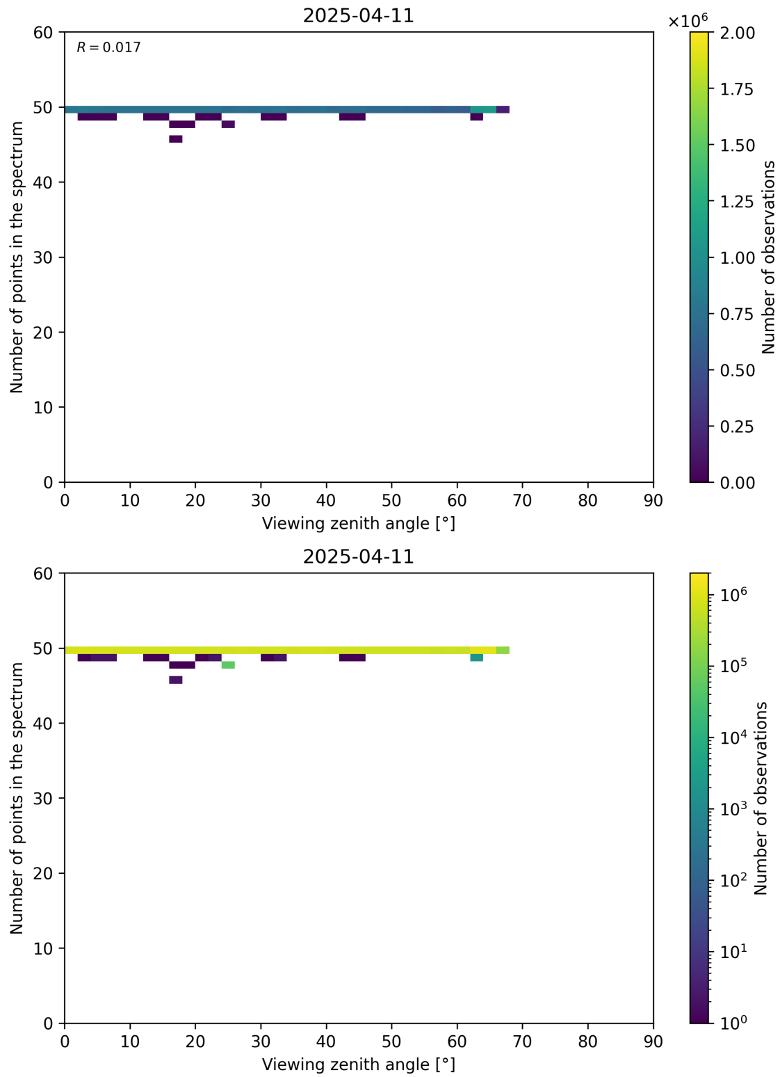
Figure 125: Scatter density plot of “Viewing zenith angle” against “Number of points in the spectrum” for 2025-04-10 to 2025-04-12.
