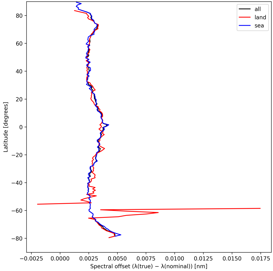
Figure 28: Zonal average of “Spectral offset ( \lambda_{\text{true}} - \lambda_{\text{nominal}} )” for 2025-04-10 to 2025-04-12.
