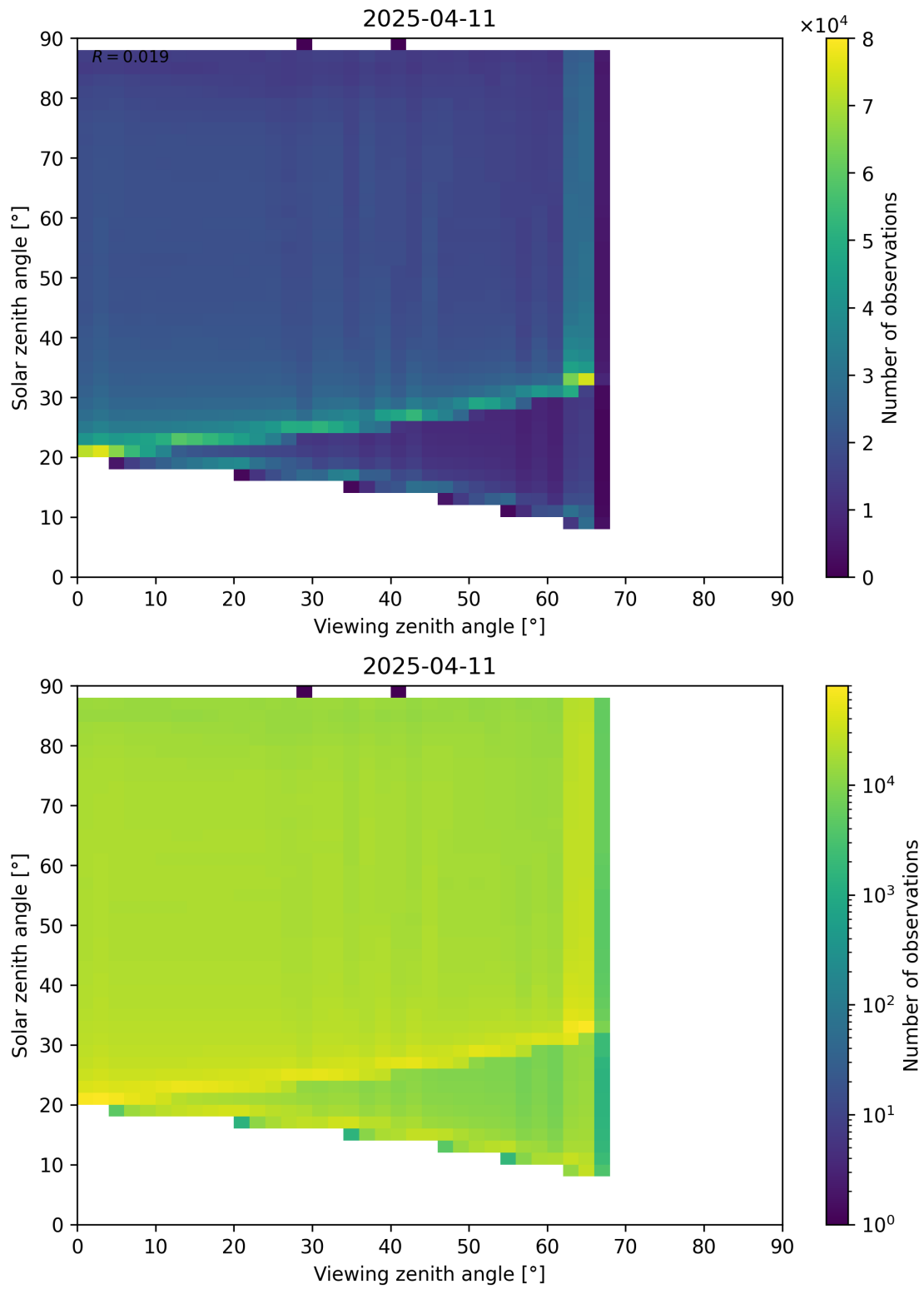
Figure 127: Scatter density plot of “Viewing zenith angle” against “Solar zenith angle” for 2025-04-10 to 2025-04-12.
