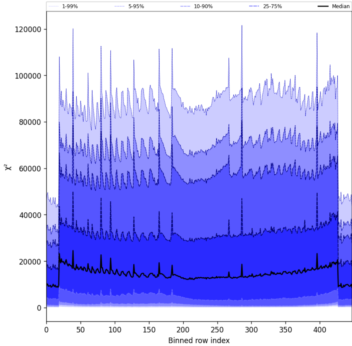
Figure 55: Along track statistics of “ \chi^2 ” for 2025-04-10 to 2025-04-12
