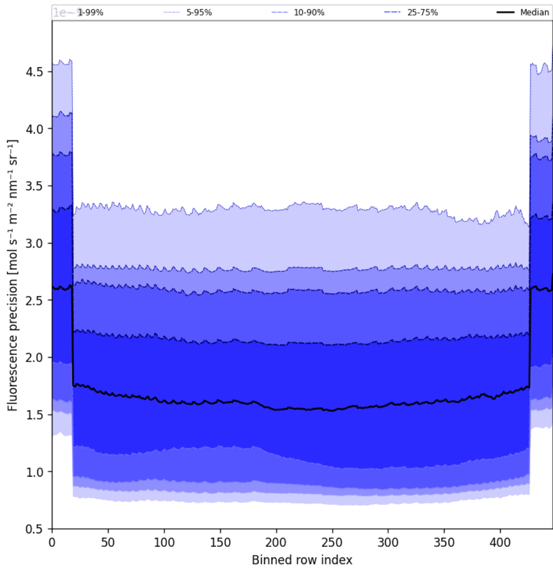
Figure 58: Along track statistics of “Fluorescence precision” for 2025-04-10 to 2025-04-12
