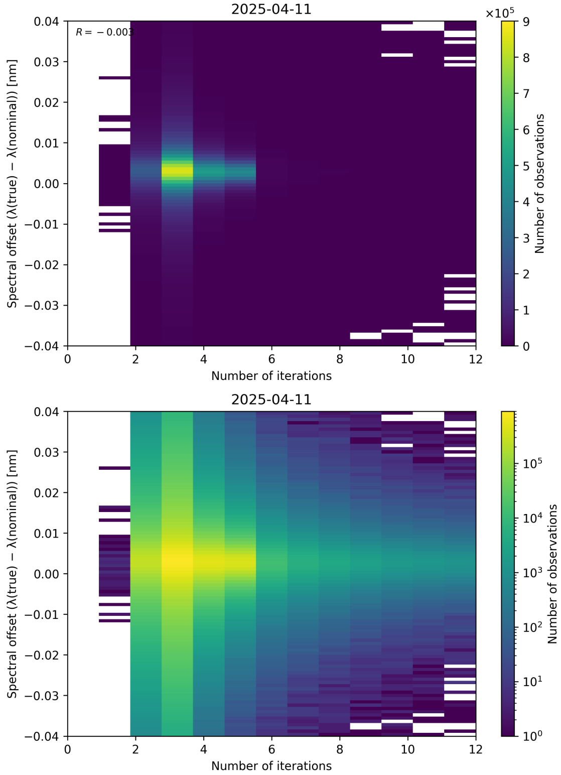
Figure 100: Scatter density plot of “Number of iterations” against “Spectral offset ( \lambda_{\text{true}} - \lambda_{\text{nominal}} )” for 2025-04-10 to 2025-04-12.
