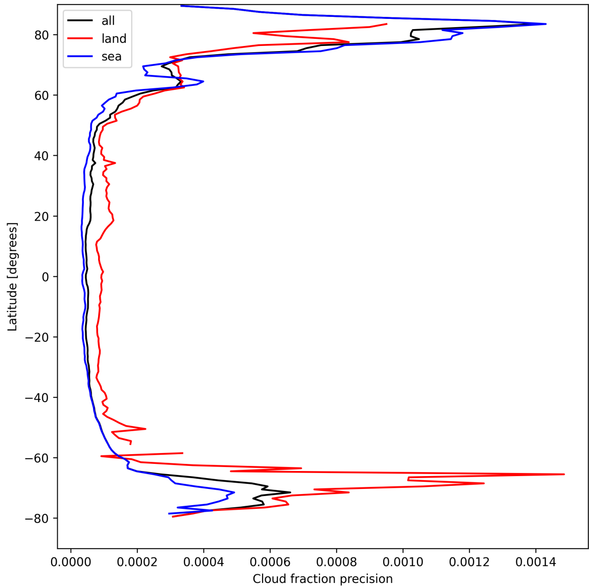
Figure 16: Zonal average of “Cloud fraction precision” for 2025-04-10 to 2025-04-12.
