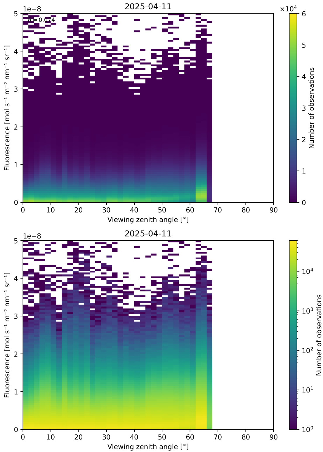
Figure 122: Scatter density plot of “Viewing zenith angle” against “Fluorescence” for 2025-04-10 to 2025-04-12.
