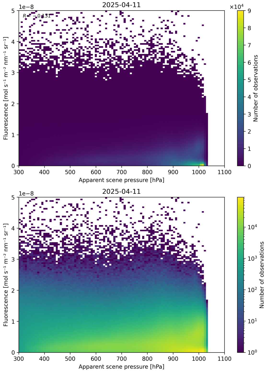
Figure 64: Scatter density plot of “Apparent scene pressure” against “Fluorescence” for 2025-04-10 to 2025-04-12.
