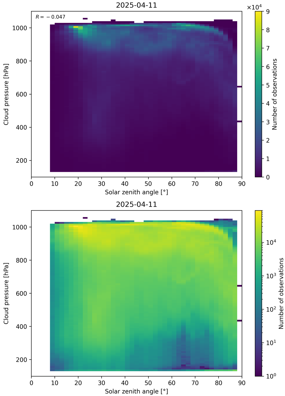
Figure 111: Scatter density plot of “Solar zenith angle” against “Cloud pressure” for 2025-04-10 to 2025-04-12.
