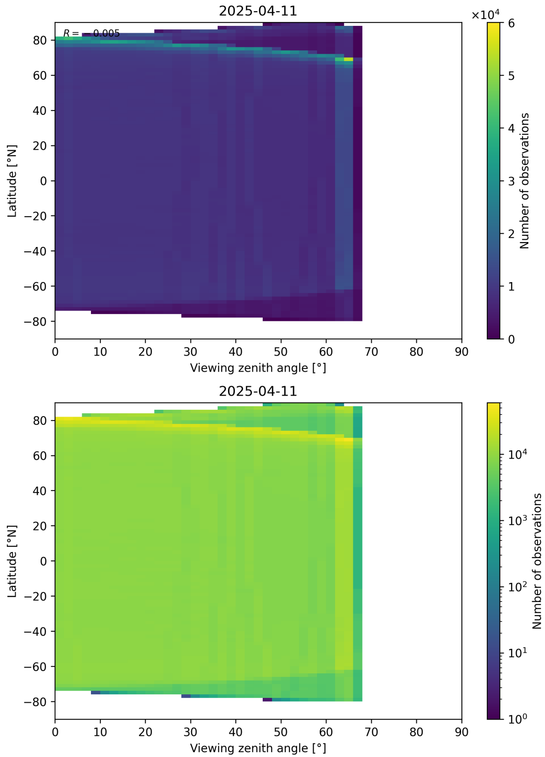
Figure 123: Scatter density plot of “Viewing zenith angle” against “Latitude” for 2025-04-10 to 2025-04-12.
