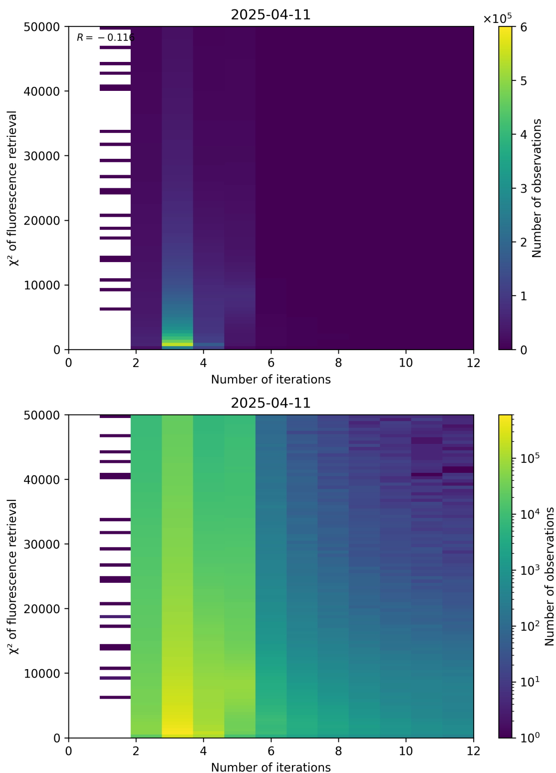
Figure 97: Scatter density plot of “Number of iterations” against “ \chi^2 of fluorescence retrieval” for 2025-04-10 to 2025-04-12.
