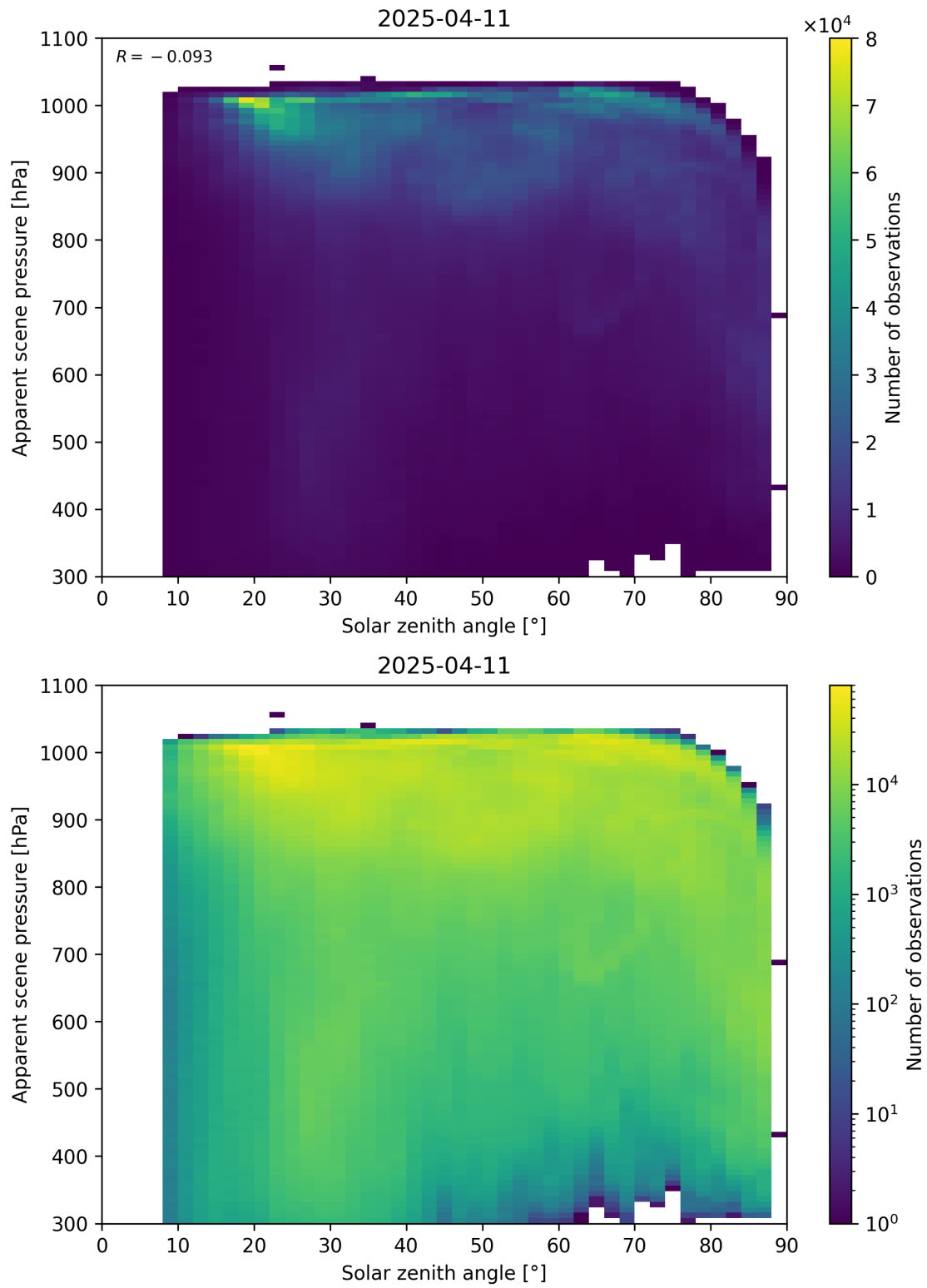
Figure 108: Scatter density plot of “Solar zenith angle” against “Apparent scene pressure” for 2025-04-10 to 2025-04-12.
