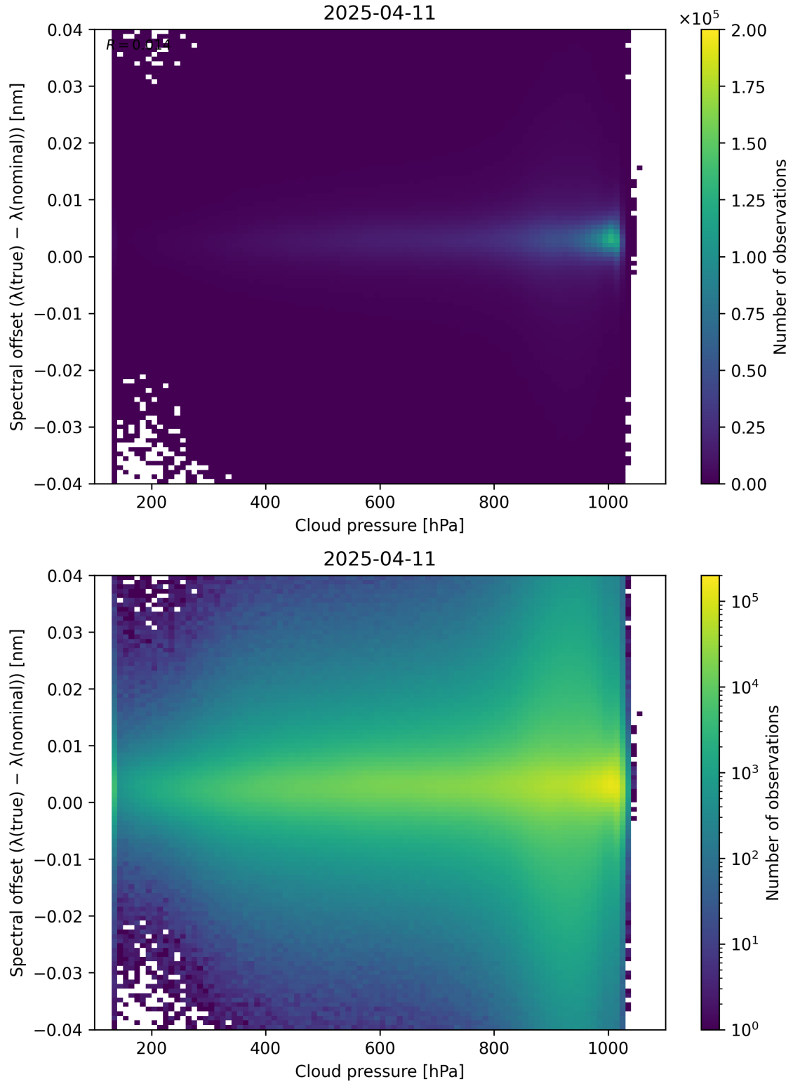
Figure 84: Scatter density plot of “Cloud pressure” against “Spectral offset ( \lambda_{\text{true}} - \lambda_{\text{nominal}} )” for 2025-04-10 to 2025-04-12.
