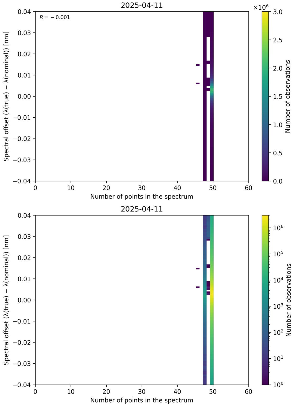
Figure 101: Scatter density plot of “Number of points in the spectrum” against “Spectral offset ( \lambda_{\text{true}} - \lambda_{\text{nominal}} )” for 2025-04-10 to 2025-04-12.
