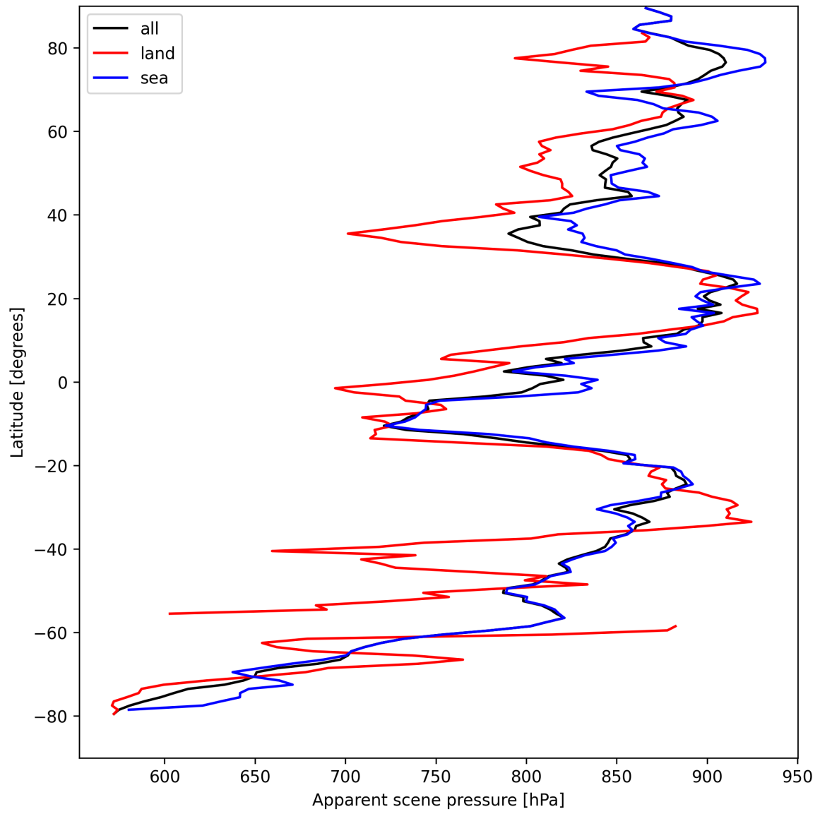
Figure 19: Zonal average of “Apparent scene pressure” for 2025-04-10 to 2025-04-12.
