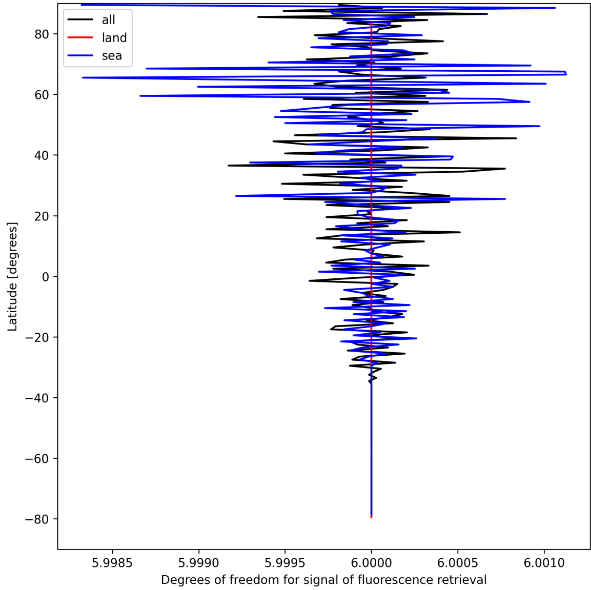
Figure 26: Zonal average of “Degrees of freedom for signal of fluorescence retrieval” for 2025-04-10 to 2025-04-12.
