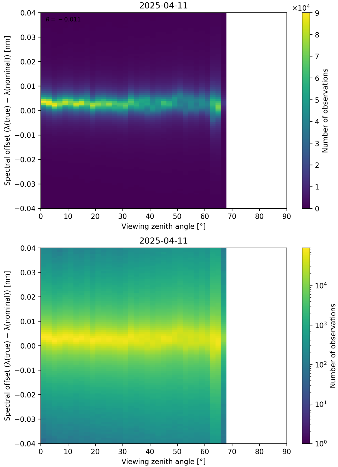
Figure 128: Scatter density plot of “Viewing zenith angle” against “Spectral offset ( \lambda_{\text{true}} - \lambda_{\text{nominal}} )” for 2025-04-10 to 2025-04-12.
