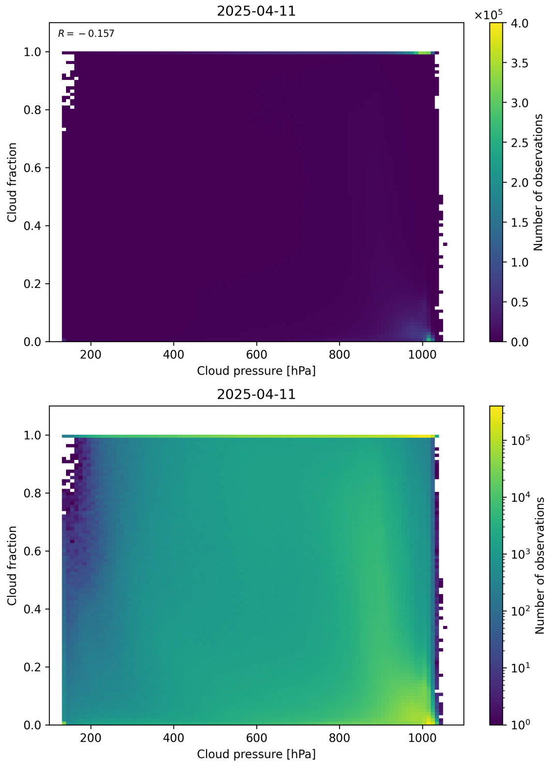
Figure 79: Scatter density plot of “Cloud pressure” against “Cloud fraction” for 2025-04-10 to 2025-04-12.
