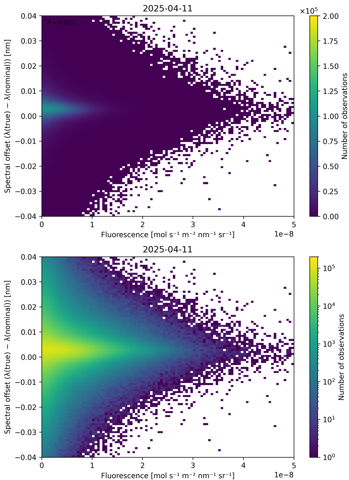
Figure 87: Scatter density plot of “Fluorescence” against “Spectral offset ( \lambda_{\text{true}} - \lambda_{\text{nominal}} )” for 2025-04-10 to 2025-04-12.
