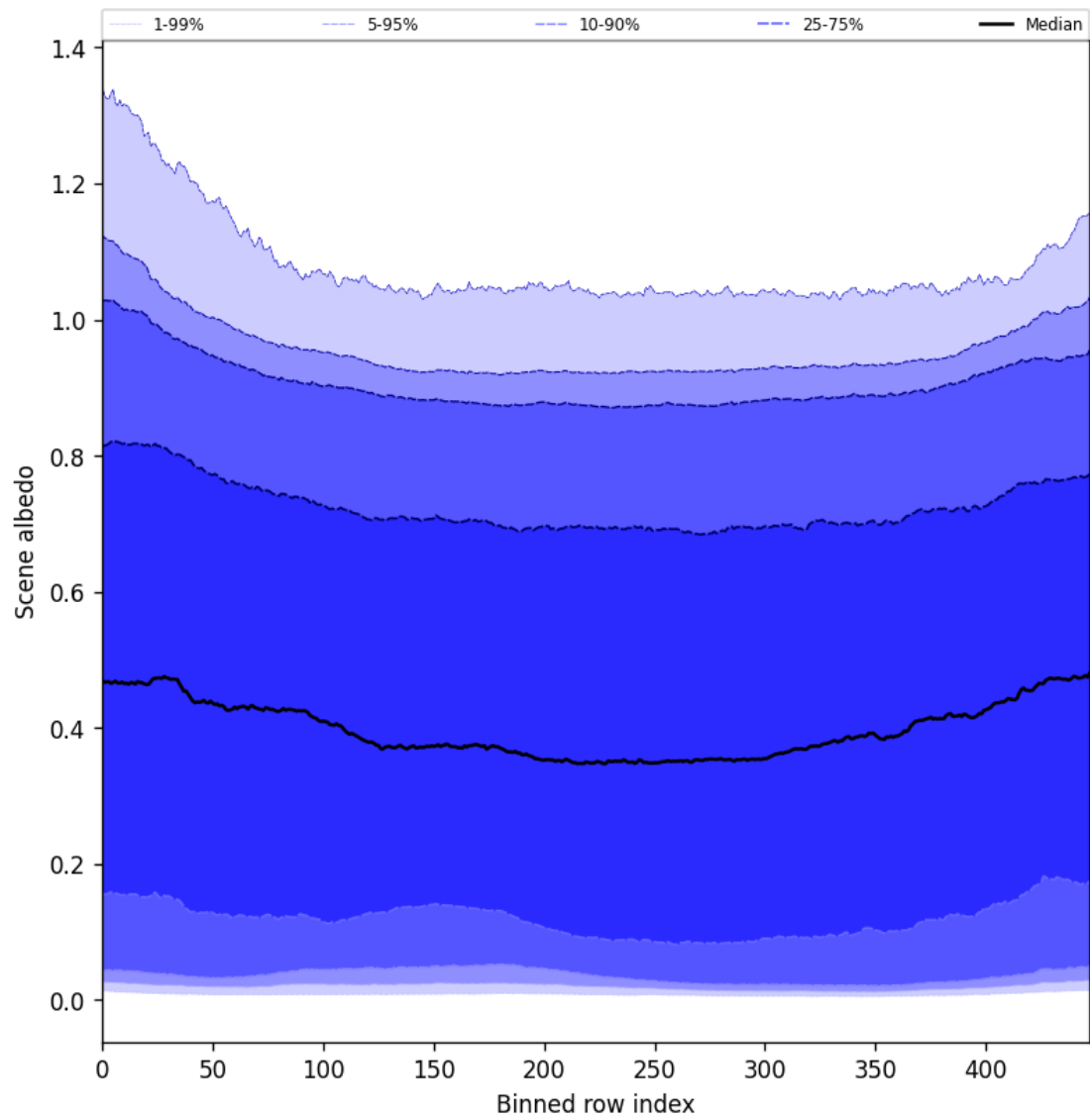
Figure 51: Along track statistics of “Scene albedo” for 2025-04-10 to 2025-04-12
