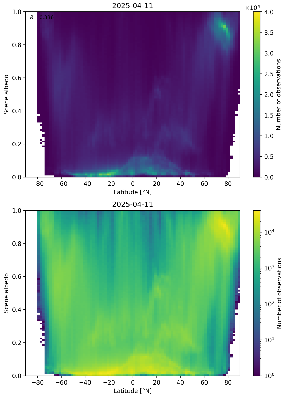
Figure 95: Scatter density plot of “Latitude” against “Scene albedo” for 2025-04-10 to 2025-04-12.
