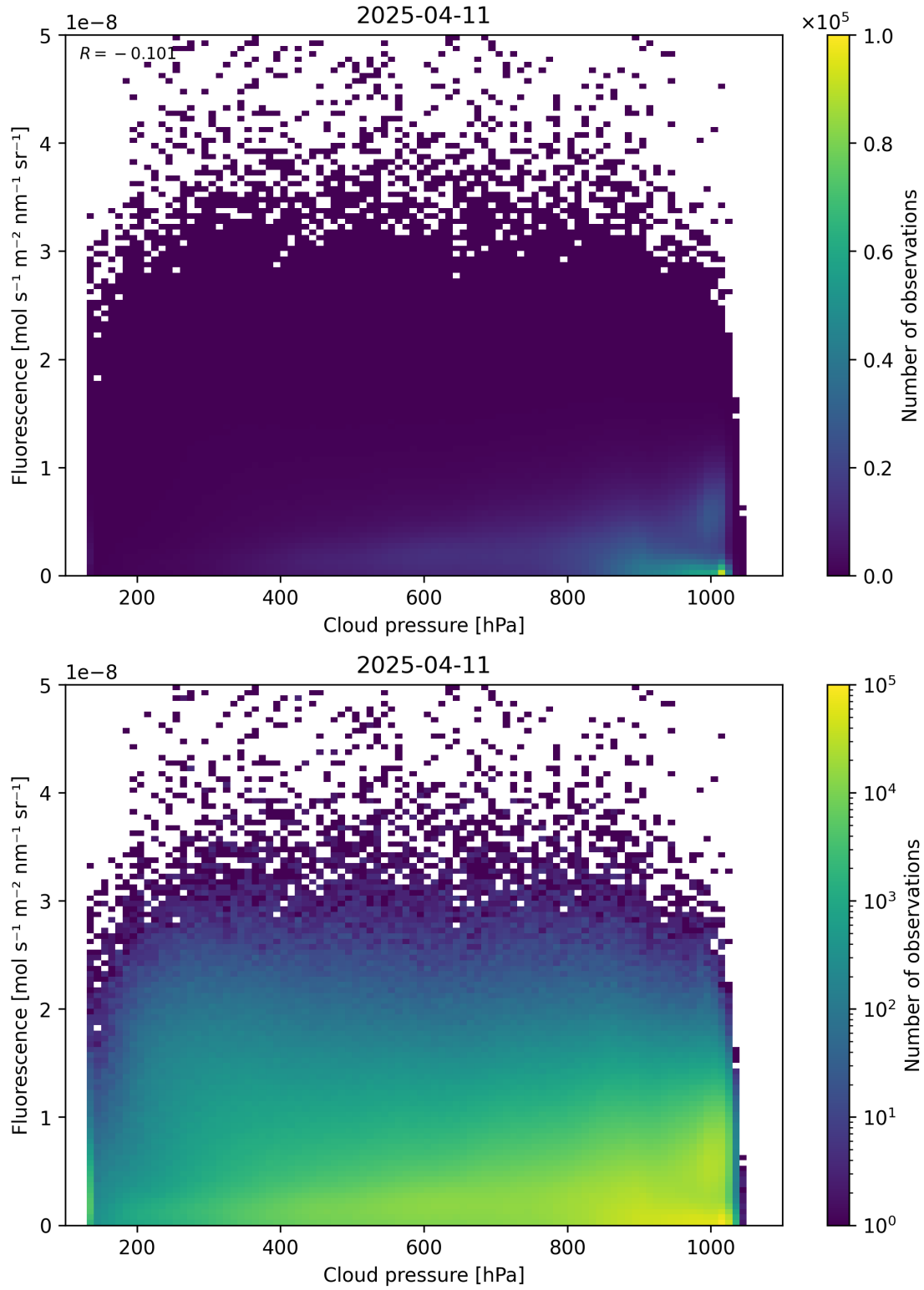
Figure 80: Scatter density plot of “Cloud pressure” against “Fluorescence” for 2025-04-10 to 2025-04-12.
