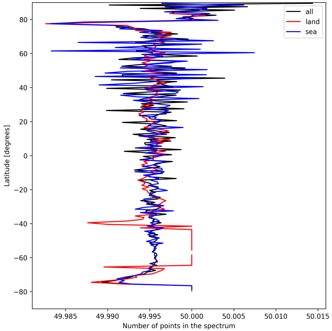
Figure 27: Zonal average of “Number of points in the spectrum” for 2025-04-10 to 2025-04-12.
