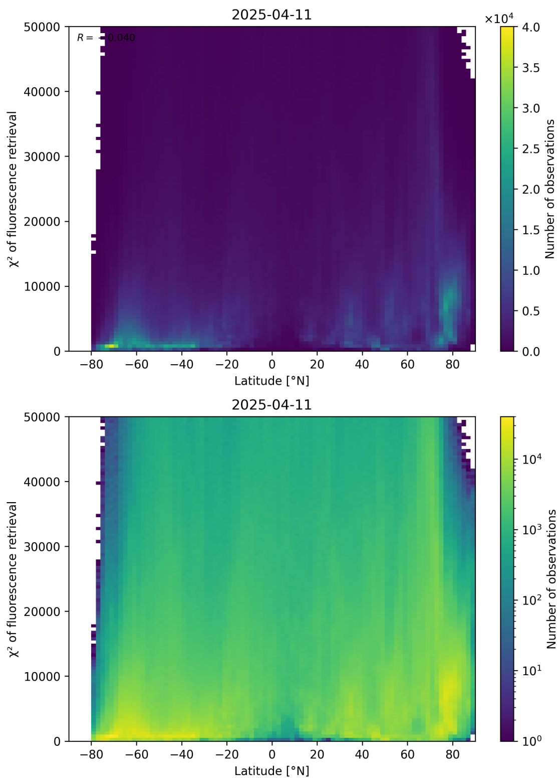
Figure 89: Scatter density plot of “Latitude” against “ \chi^2 of fluorescence retrieval” for 2025-04-10 to 2025-04-12.
