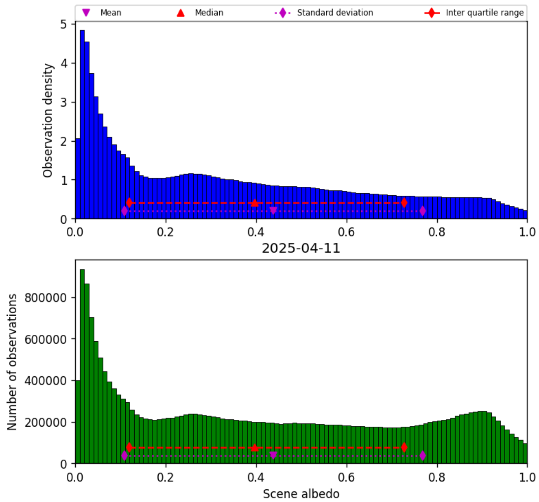
Figure 34: Histogram of “Scene albedo” for 2025-04-10 to 2025-04-12
