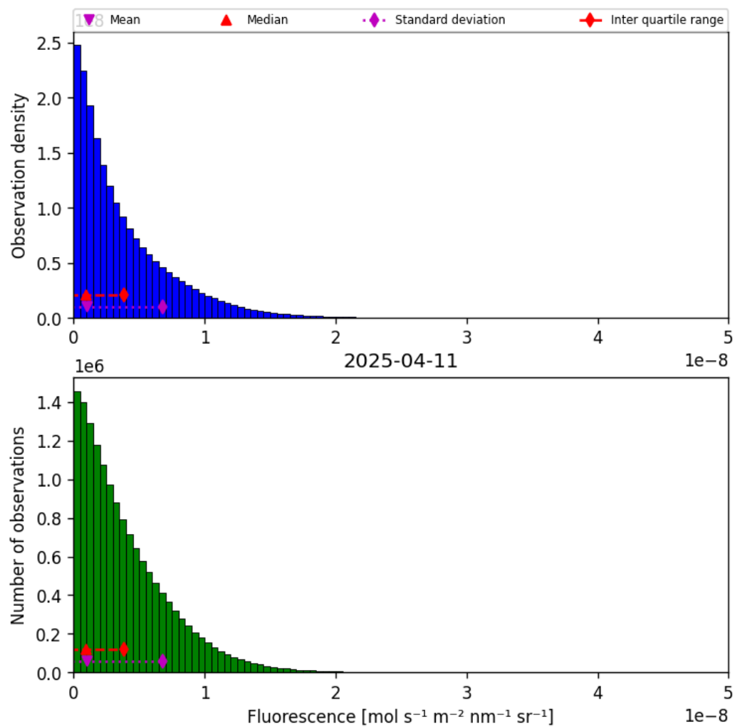
Figure 40: Histogram of “Fluorescence” for 2025-04-10 to 2025-04-12
