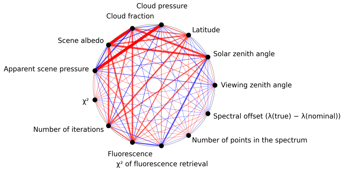
Figure 1: Map of correlation graph for 2025-04-10 to 2025-04-12.
