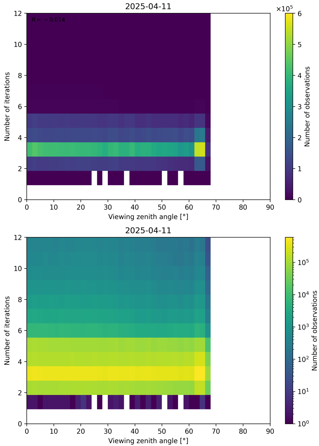
Figure 124: Scatter density plot of “Viewing zenith angle” against “Number of iterations” for 2025-04-10 to 2025-04-12.
