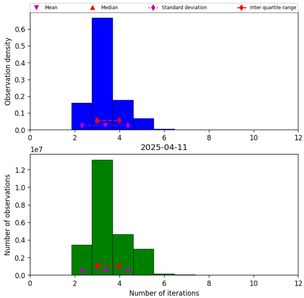
Figure 39: Histogram of “Number of iterations” for 2025-04-10 to 2025-04-12
