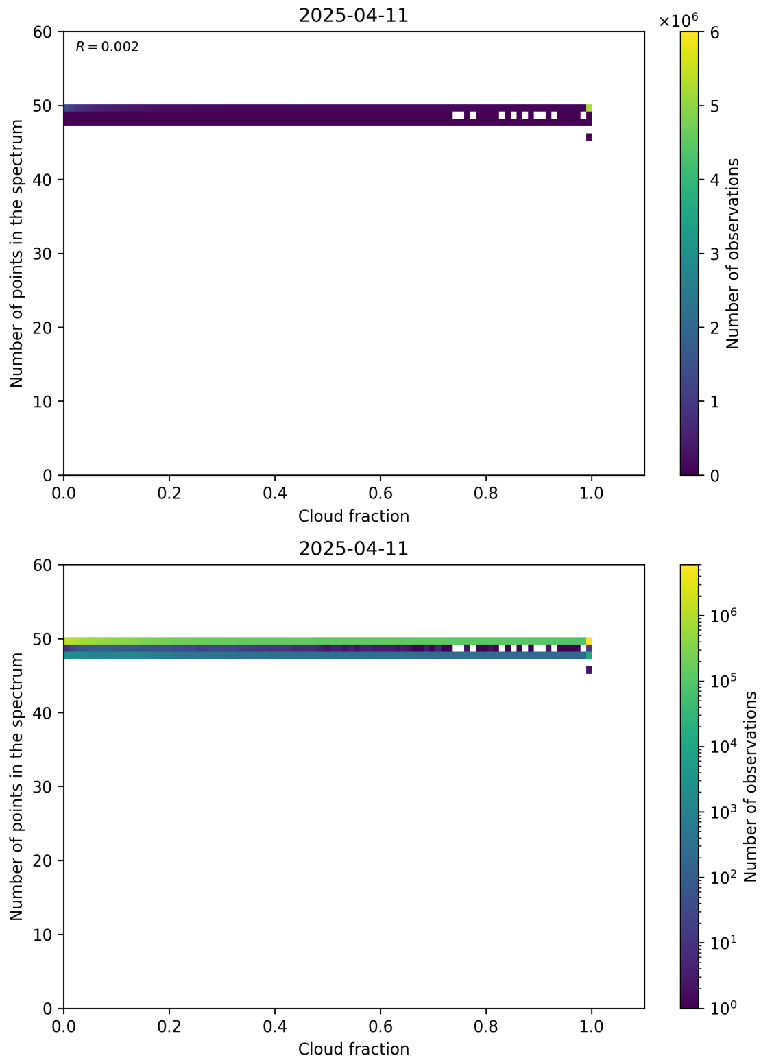
Figure 74: Scatter density plot of “Cloud fraction” against “Number of points in the spectrum” for 2025-04-10 to 2025-04-12.
