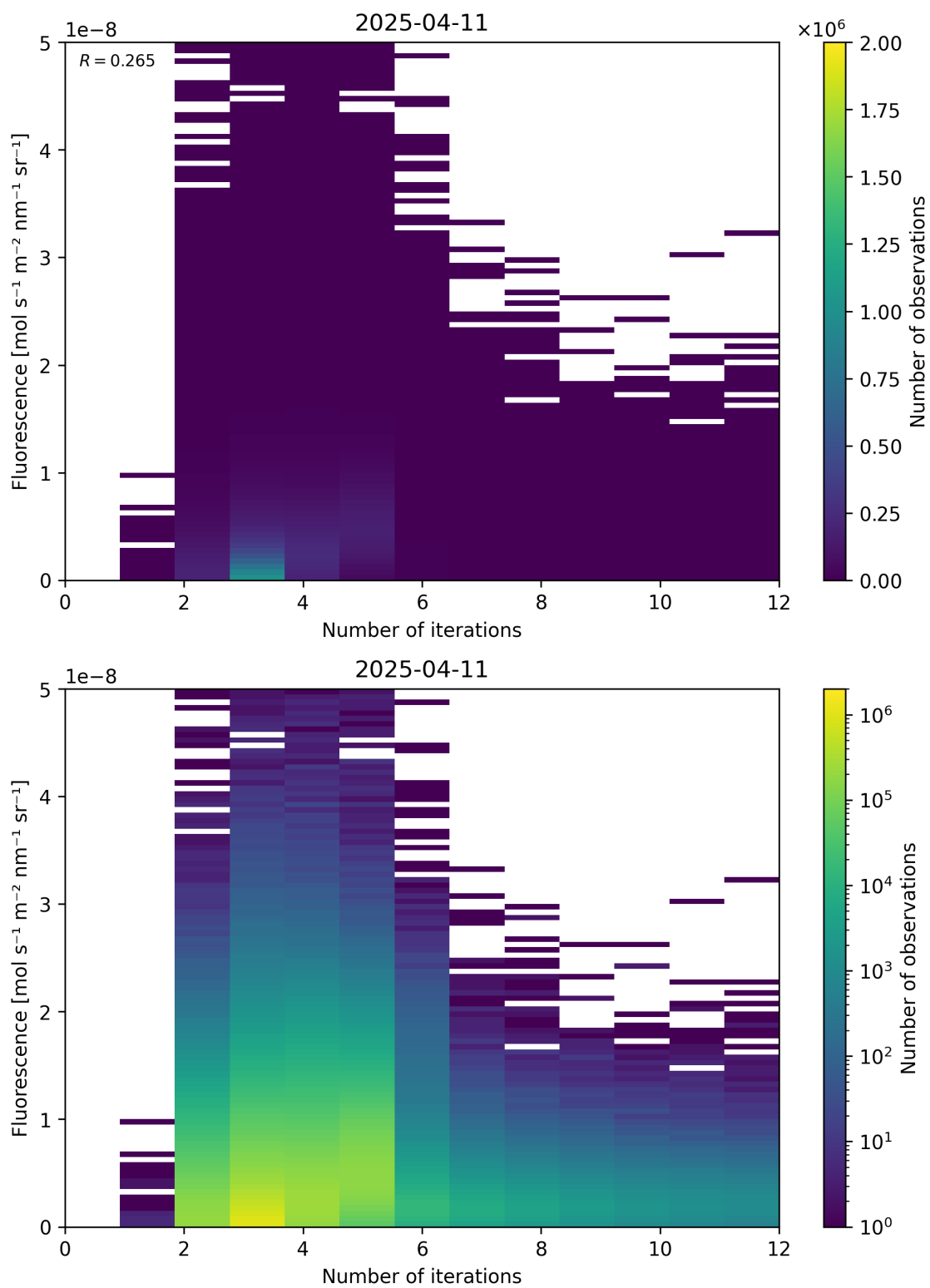
Figure 98: Scatter density plot of “Number of iterations” against “Fluorescence” for 2025-04-10 to 2025-04-12.
