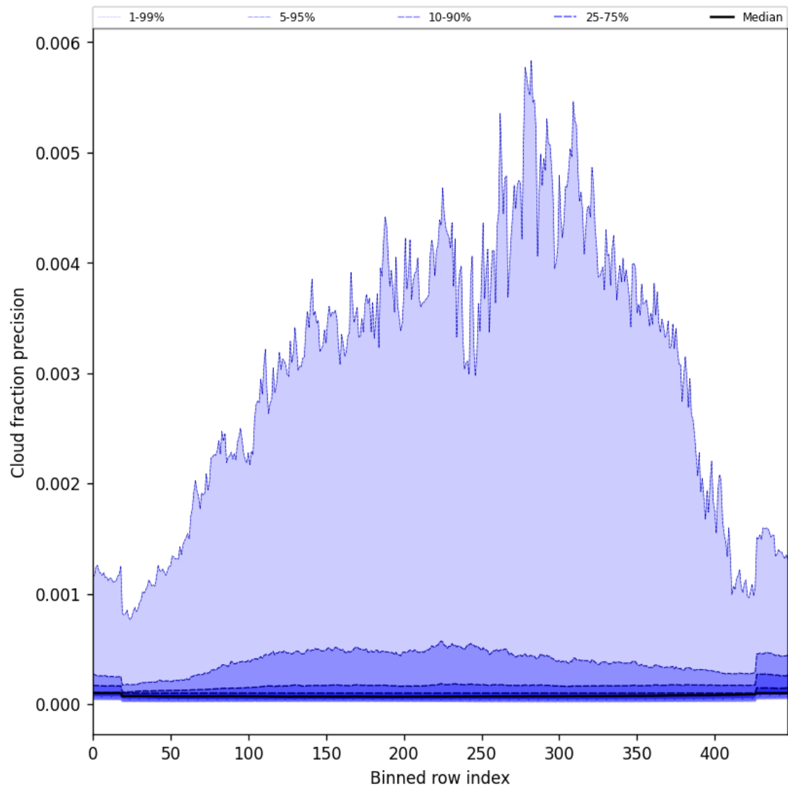
Figure 50: Along track statistics of “Cloud fraction precision” for 2025-04-10 to 2025-04-12
