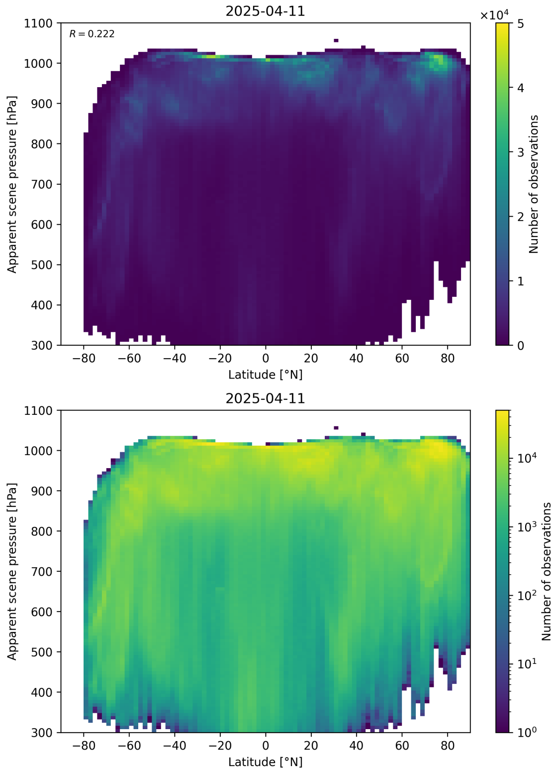
Figure 88: Scatter density plot of “Latitude” against “Apparent scene pressure” for 2025-04-10 to 2025-04-12.
