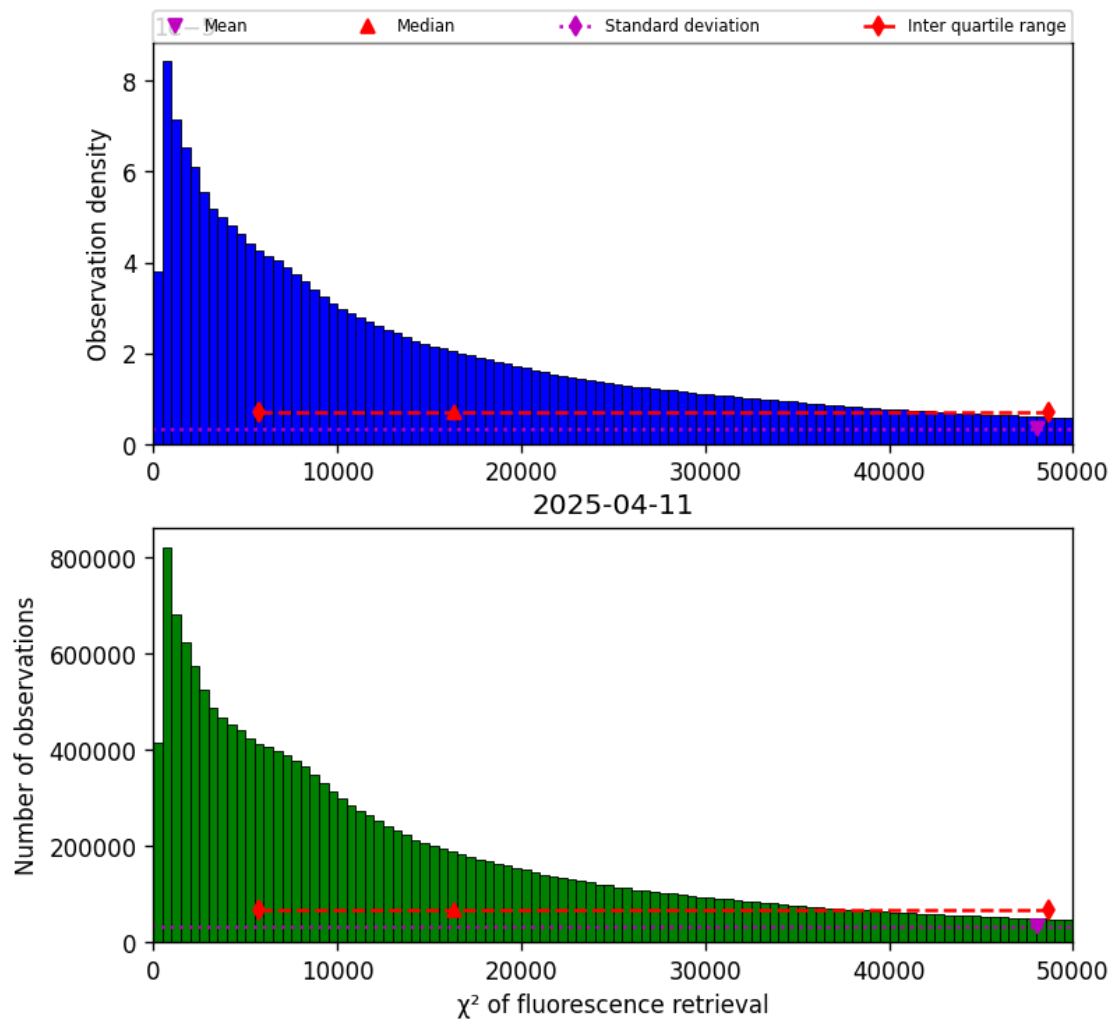
Figure 42: Histogram of “ \chi^2 of fluorescence retrieval” for 2025-04-10 to 2025-04-12
