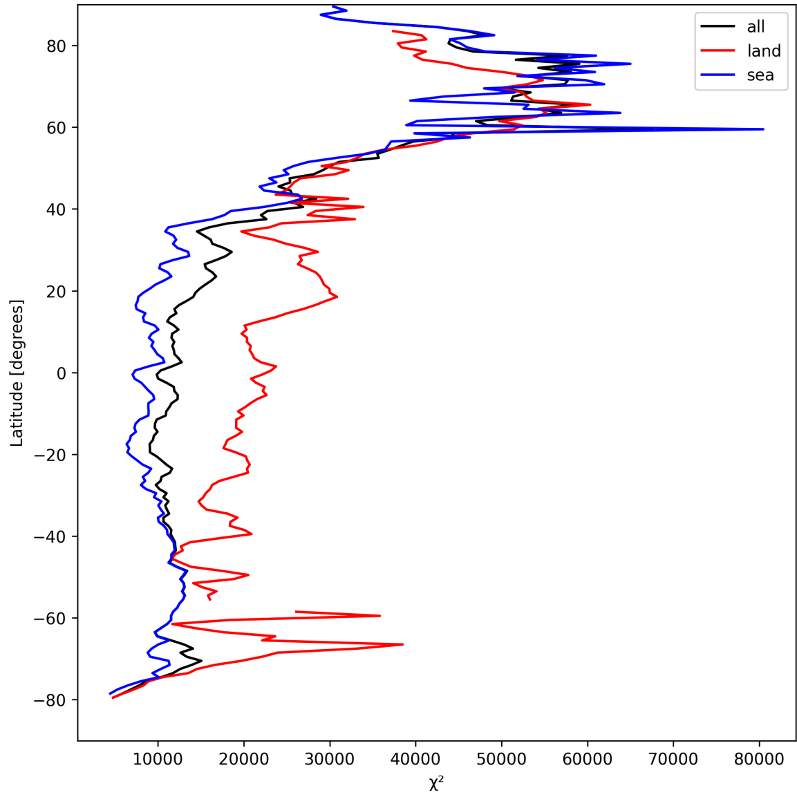
Figure 21: Zonal average of “ \chi^2 ” for 2025-04-10 to 2025-04-12.
