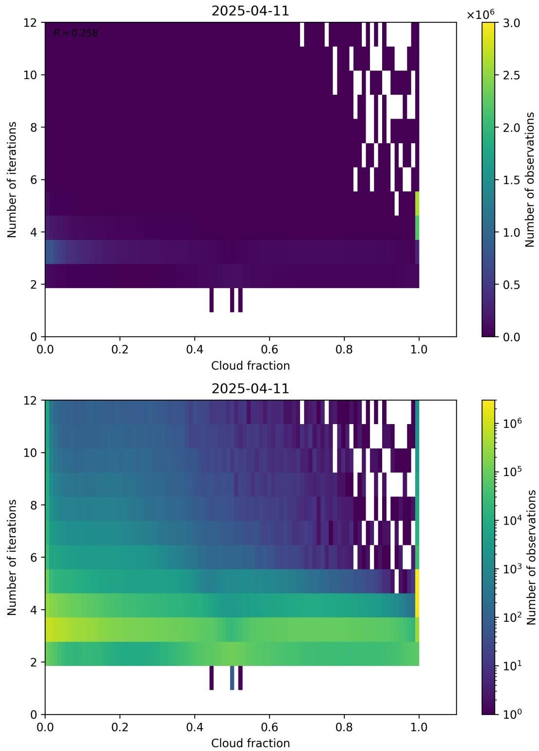
Figure 73: Scatter density plot of “Cloud fraction” against “Number of iterations” for 2025-04-10 to 2025-04-12.
