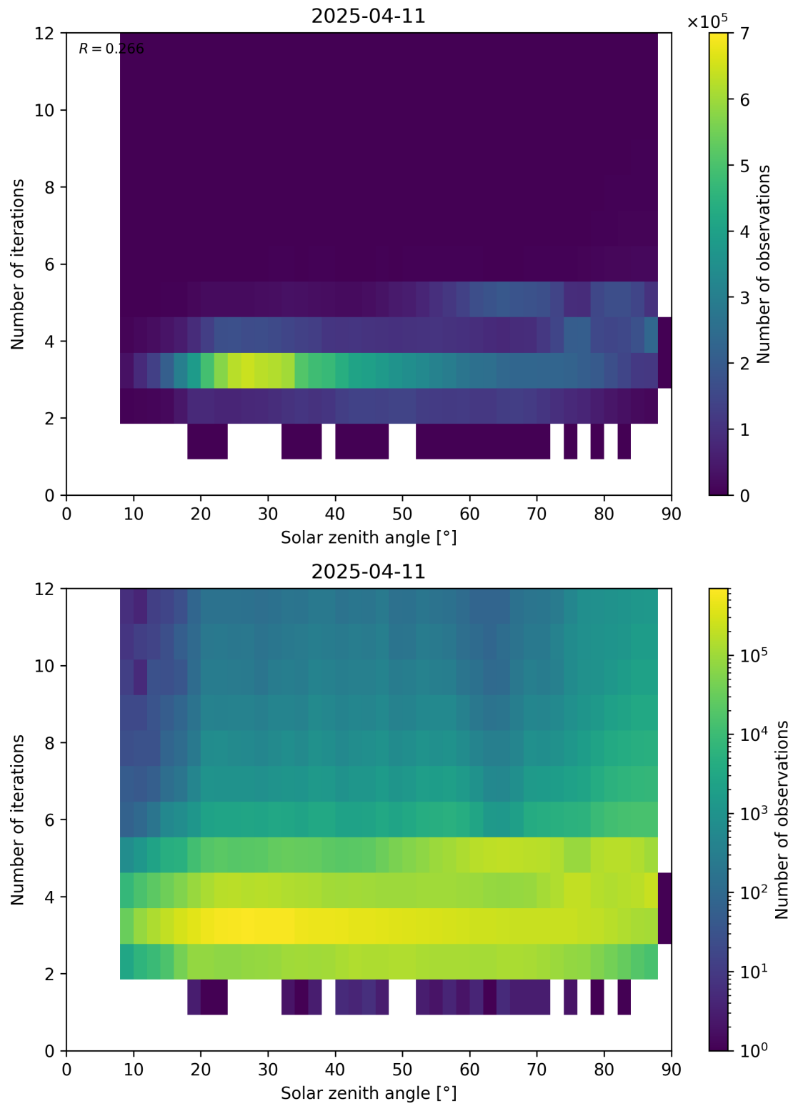
Figure 114: Scatter density plot of “Solar zenith angle” against “Number of iterations” for 2025-04-10 to 2025-04-12.
