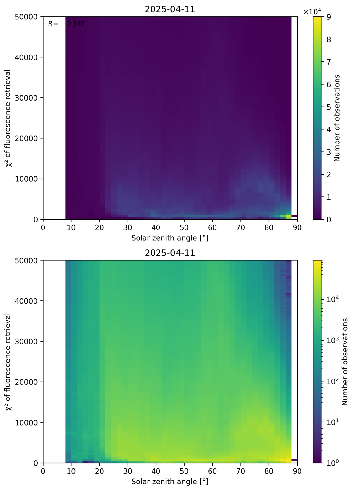
Figure 109: Scatter density plot of “Solar zenith angle” against “ \chi^2 of fluorescence retrieval” for 2025-04-10 to 2025-04-12.
