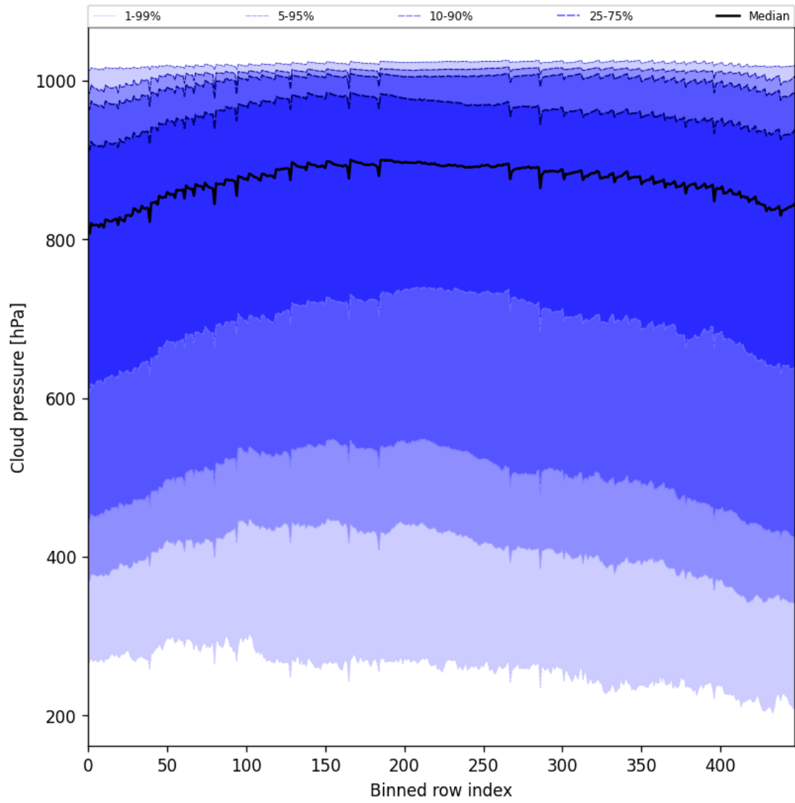
Figure 47: Along track statistics of “Cloud pressure” for 2025-04-10 to 2025-04-12
