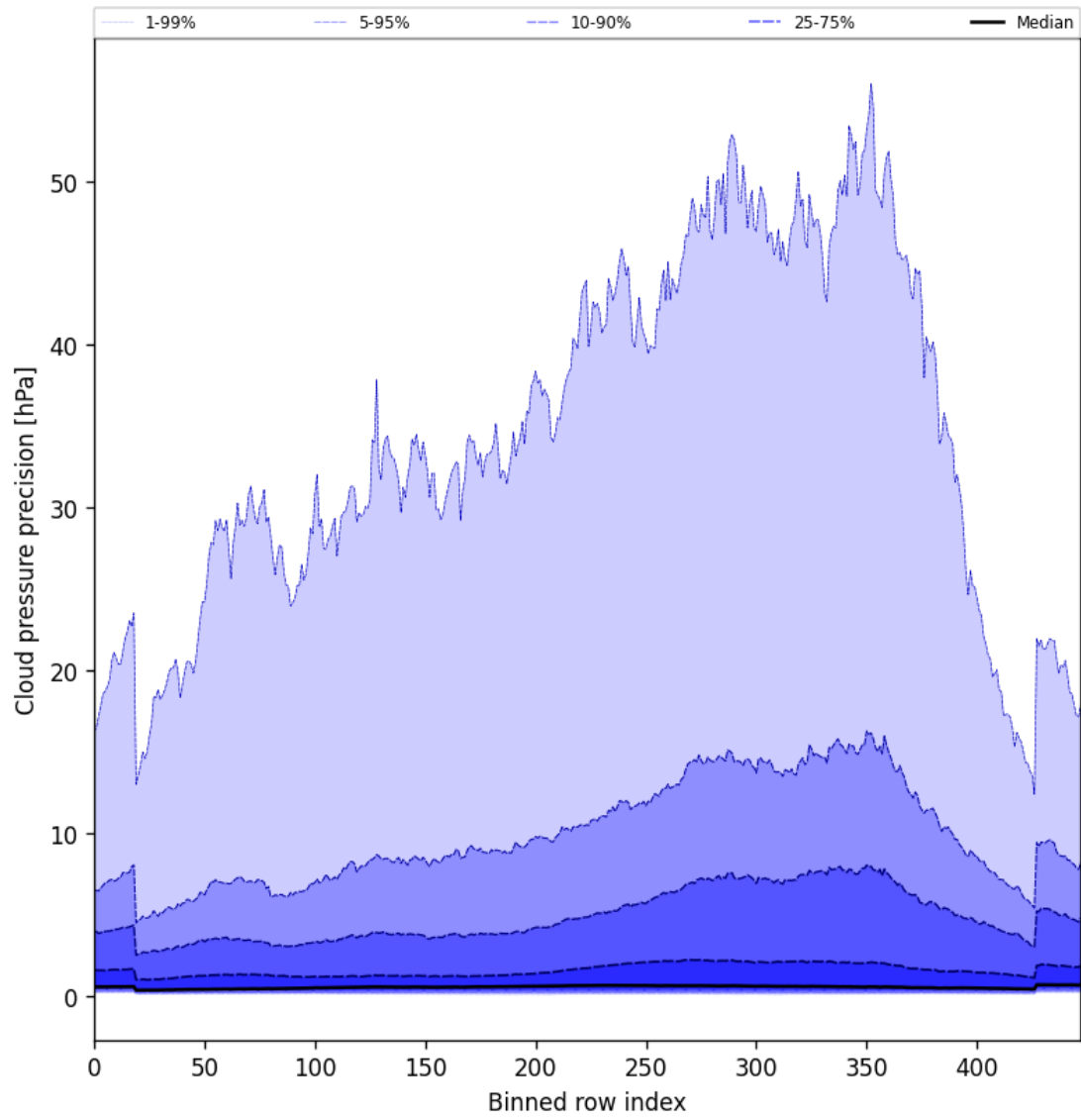
Figure 48: Along track statistics of “Cloud pressure precision” for 2025-04-10 to 2025-04-12
