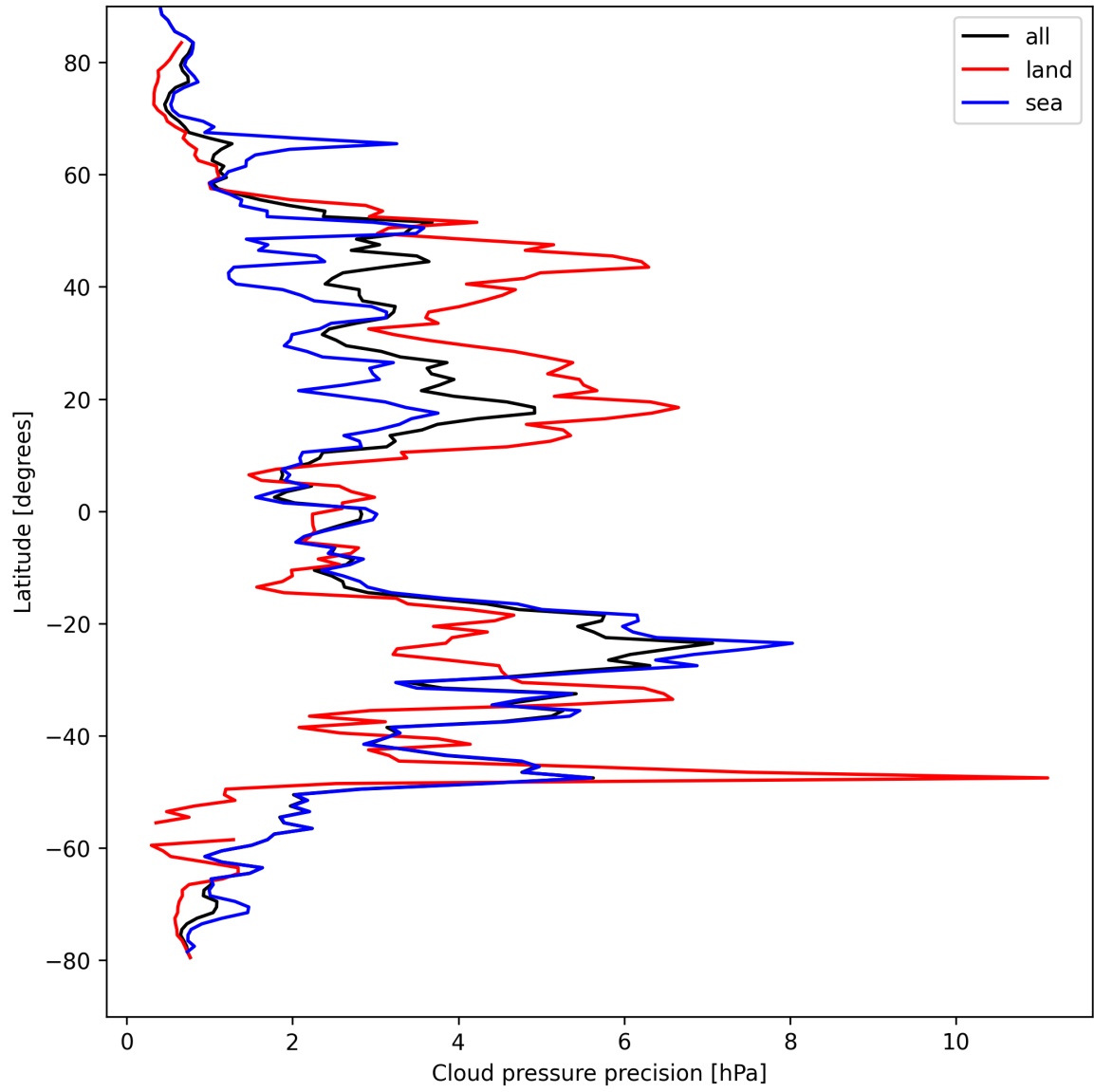
Figure 14: Zonal average of “Cloud pressure precision” for 2025-04-10 to 2025-04-12.
