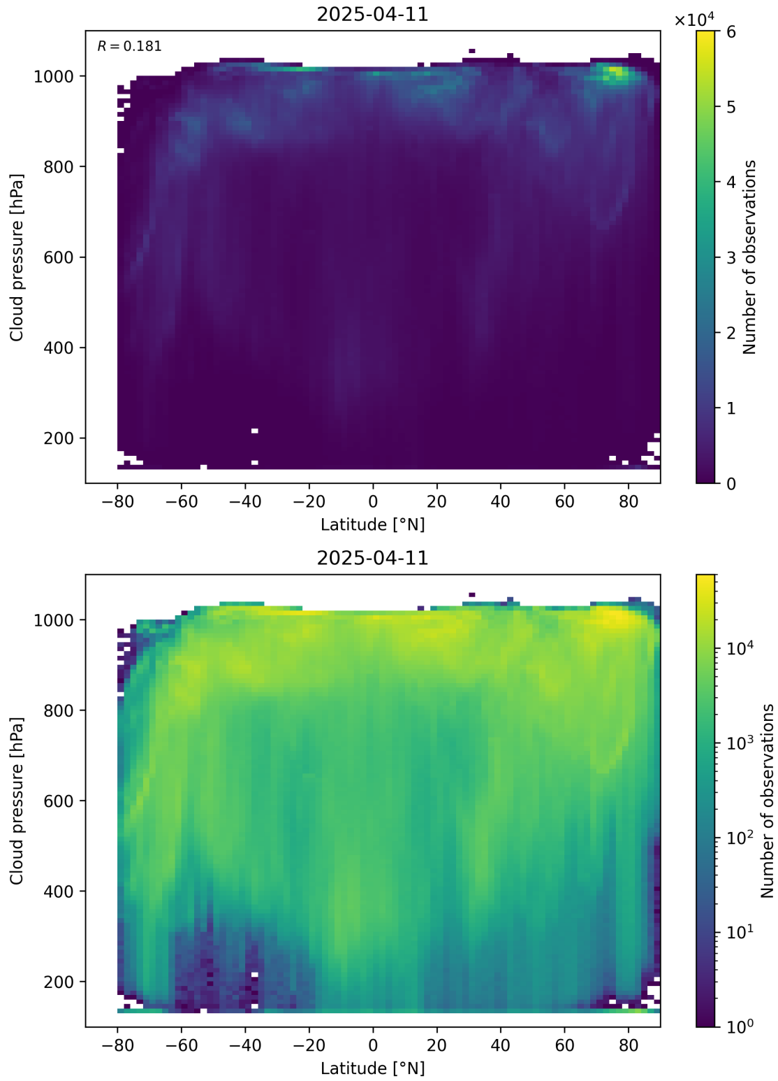
Figure 91: Scatter density plot of “Latitude” against “Cloud pressure” for 2025-04-10 to 2025-04-12.
