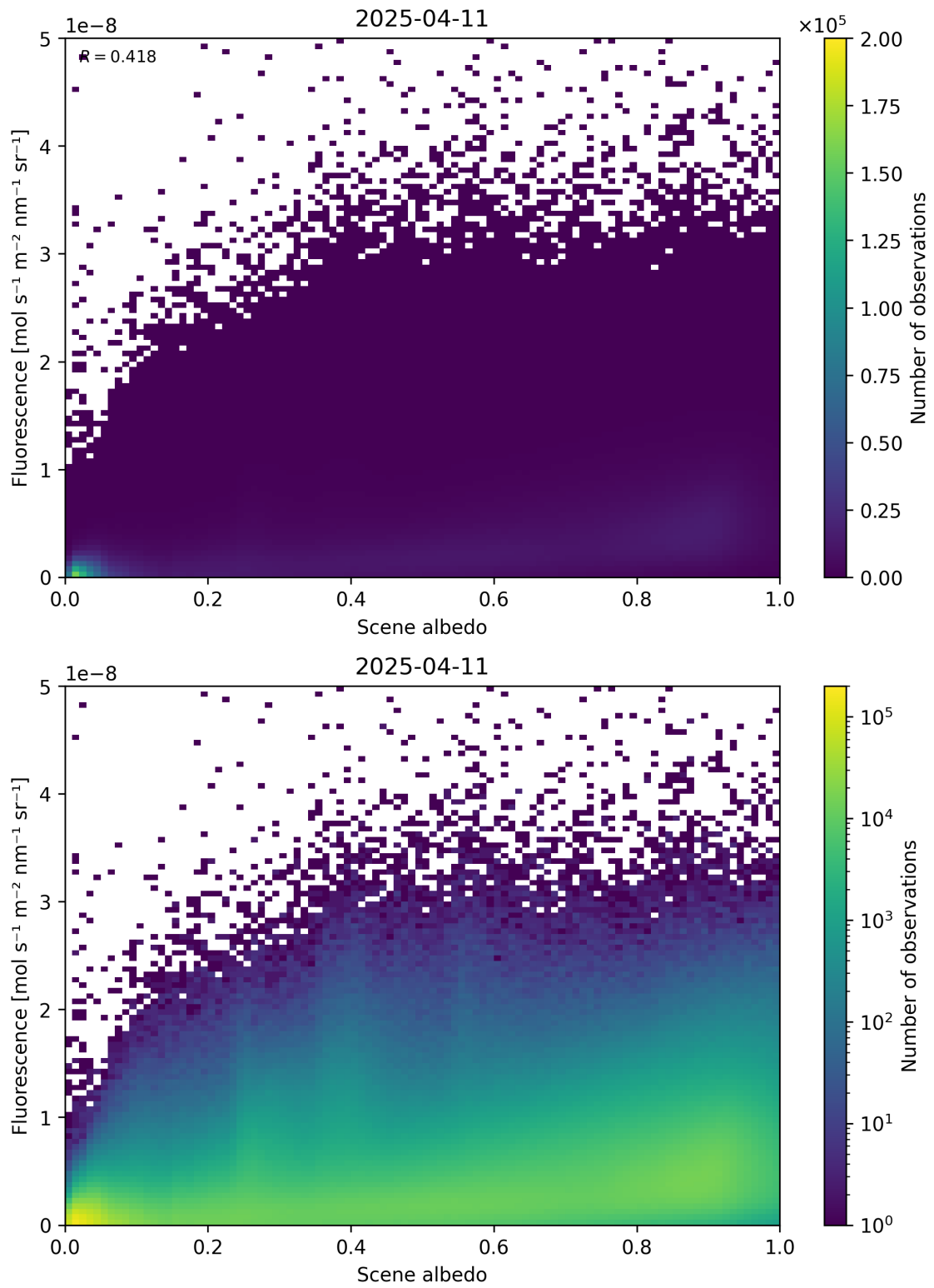
Figure 104: Scatter density plot of “Scene albedo” against “Fluorescence” for 2025-04-10 to 2025-04-12.
