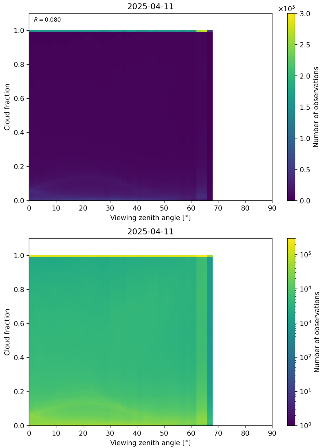
Figure 120: Scatter density plot of “Viewing zenith angle” against “Cloud fraction” for 2025-04-10 to 2025-04-12.
