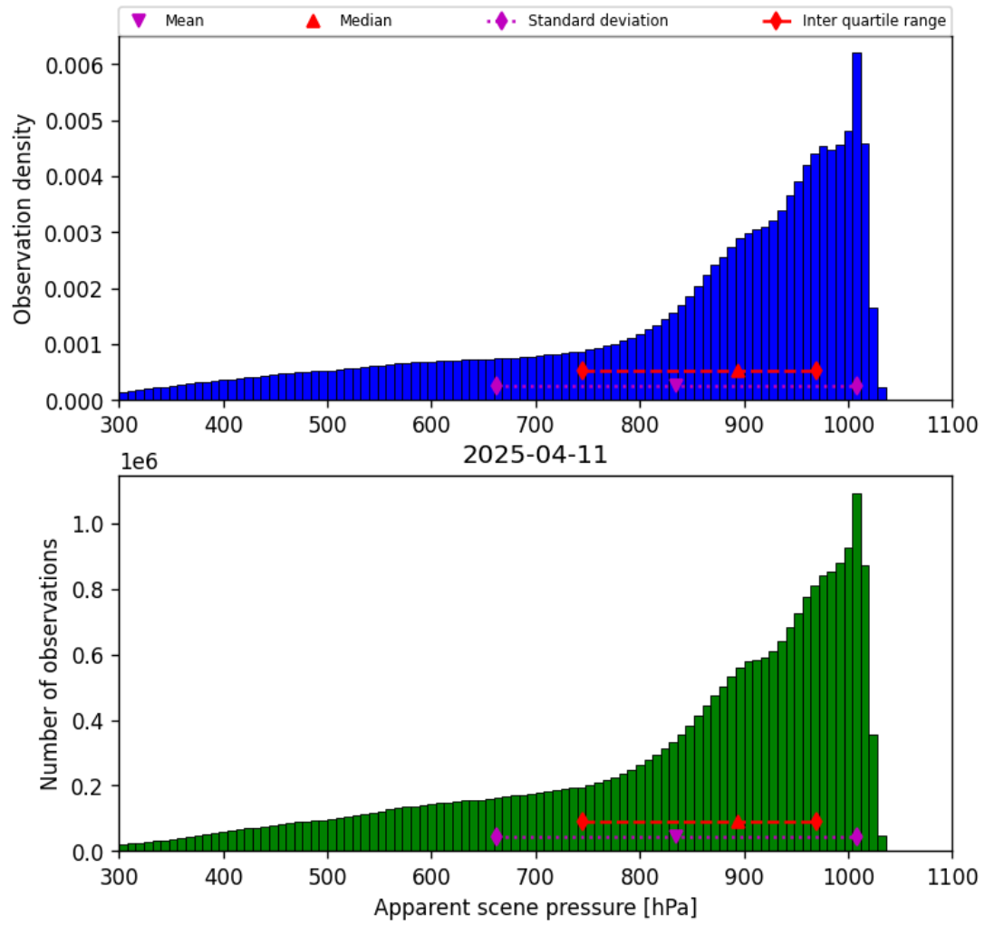
Figure 36: Histogram of “Apparent scene pressure” for 2025-04-10 to 2025-04-12
