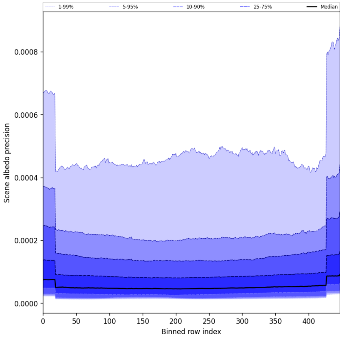
Figure 52: Along track statistics of “Scene albedo precision” for 2025-04-10 to 2025-04-12
