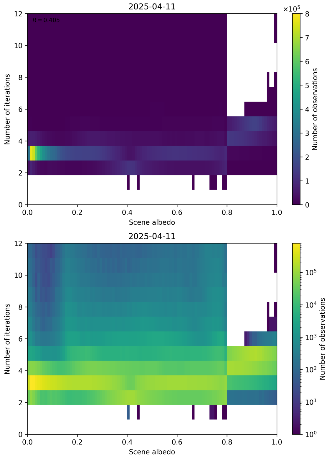
Figure 105: Scatter density plot of “Scene albedo” against “Number of iterations” for 2025-04-10 to 2025-04-12.
