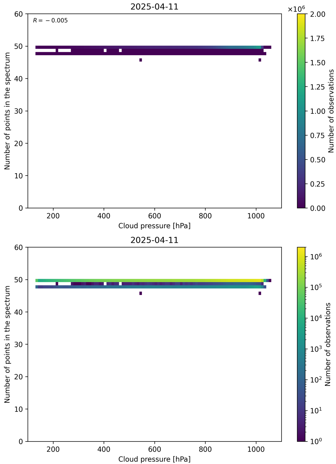
Figure 82: Scatter density plot of “Cloud pressure” against “Number of points in the spectrum” for 2025-04-10 to 2025-04-12.
