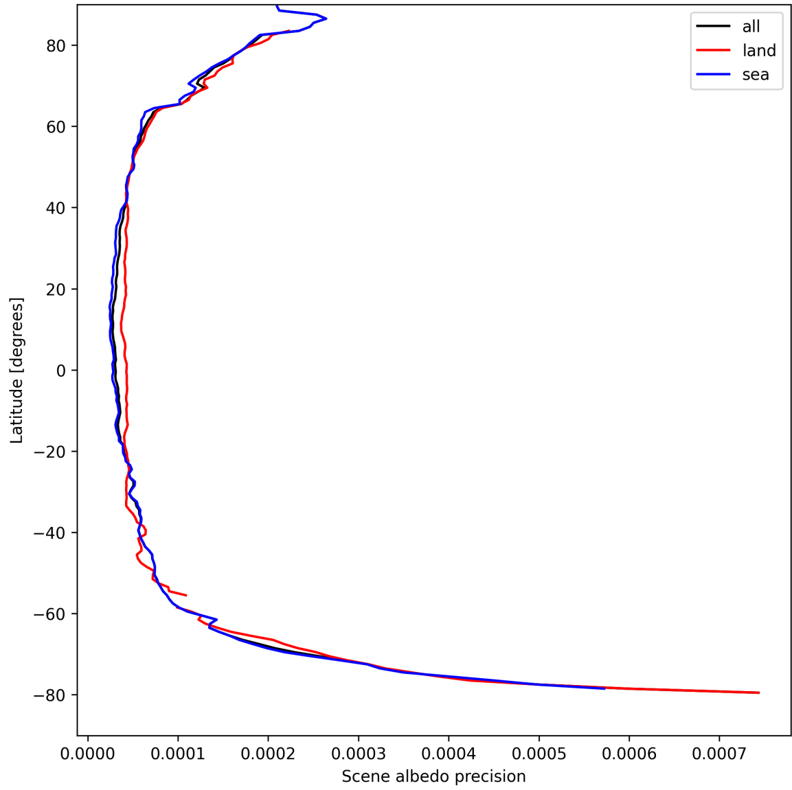
Figure 18: Zonal average of “Scene albedo precision” for 2025-04-10 to 2025-04-12.
