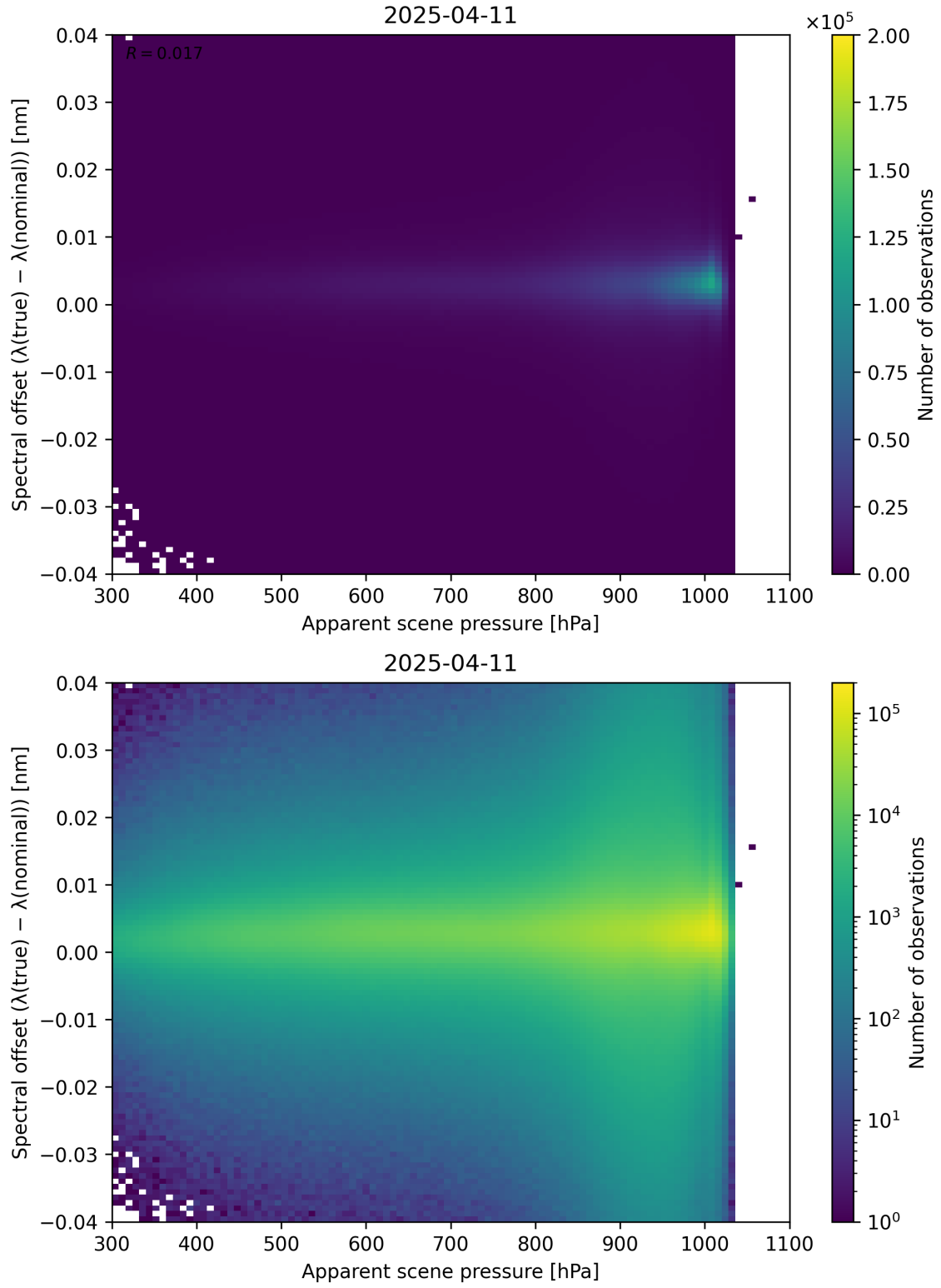
Figure 67: Scatter density plot of “Apparent scene pressure” against “Spectral offset ( \lambda_{\text{true}} - \lambda_{\text{nominal}} )” for 2025-04-10 to 2025-04-12.
