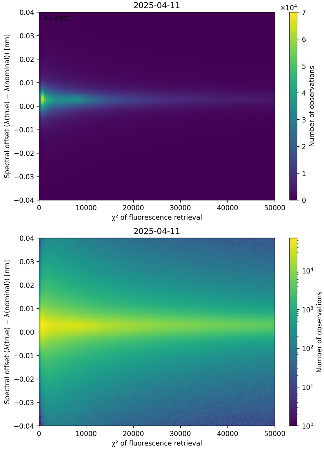
Figure 69: Scatter density plot of “ \chi^2 of fluorescence retrieval” against “Spectral offset ( \lambda_{\text{true}} - \lambda_{\text{nominal}} )” for 2025-04-10 to 2025-04-12.
