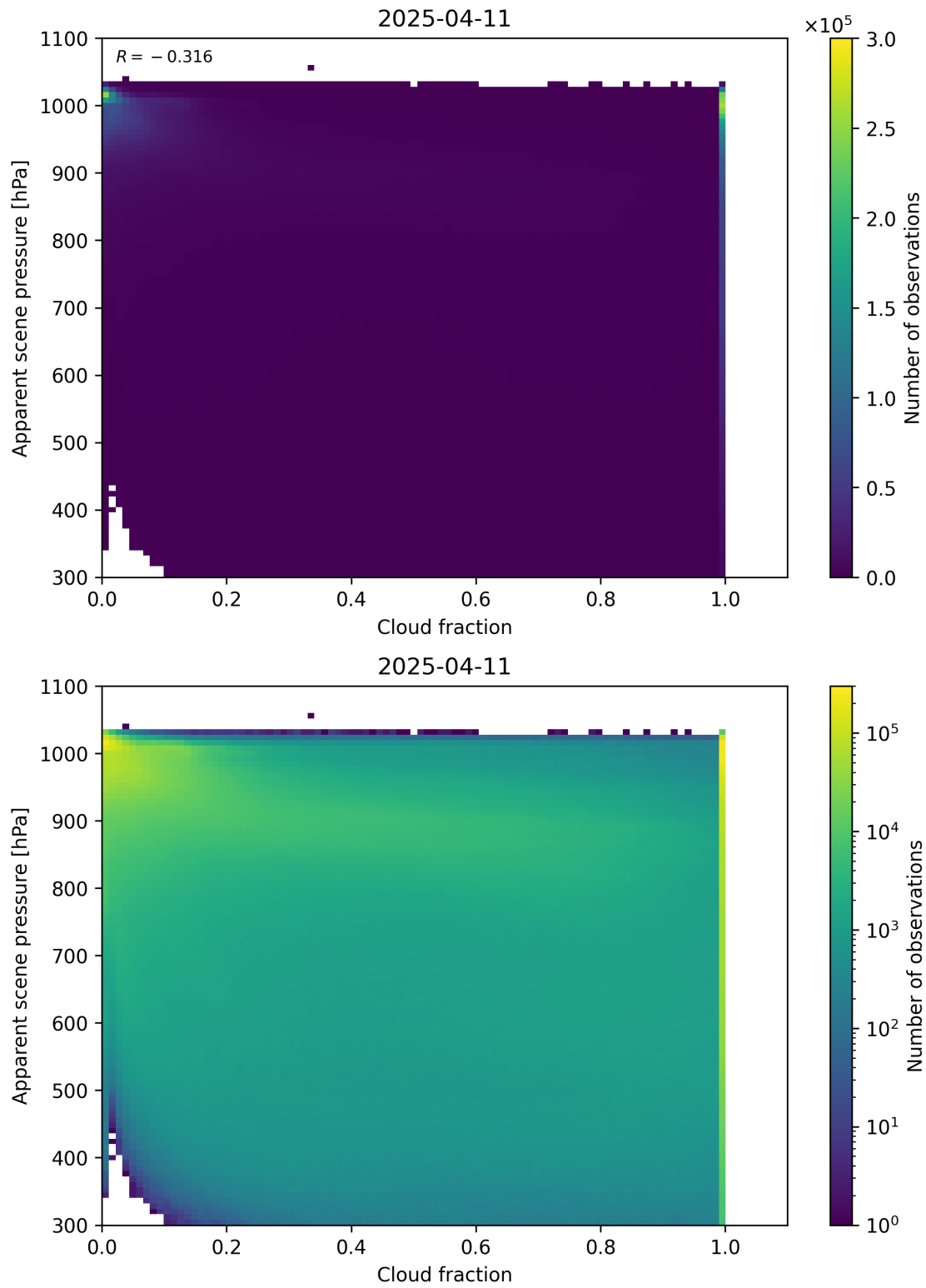
Figure 70: Scatter density plot of “Cloud fraction” against “Apparent scene pressure” for 2025-04-10 to 2025-04-12.
