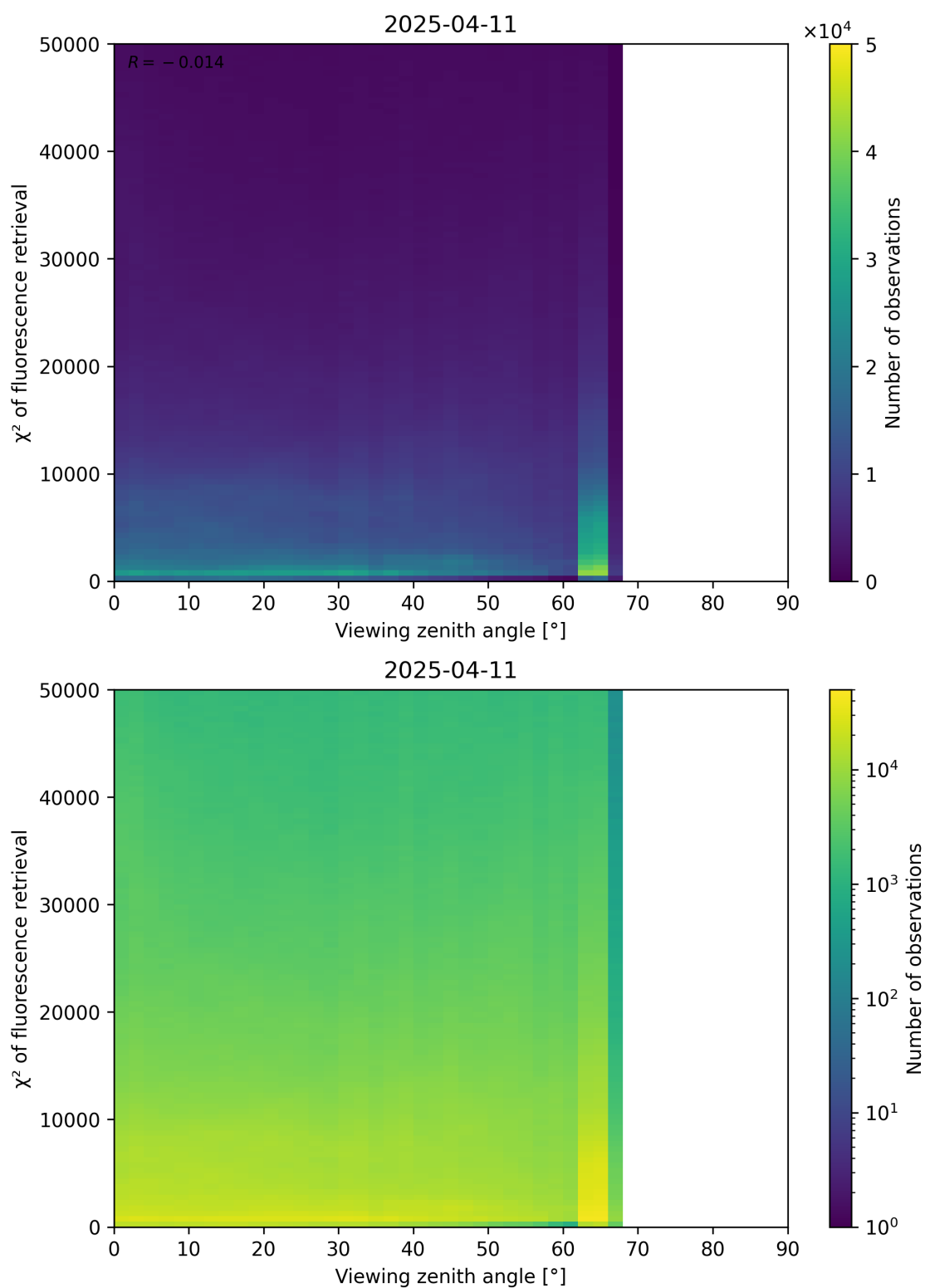
Figure 119: Scatter density plot of “Viewing zenith angle” against “ \chi^2 of fluorescence retrieval” for 2025-04-10 to 2025-04-12.
