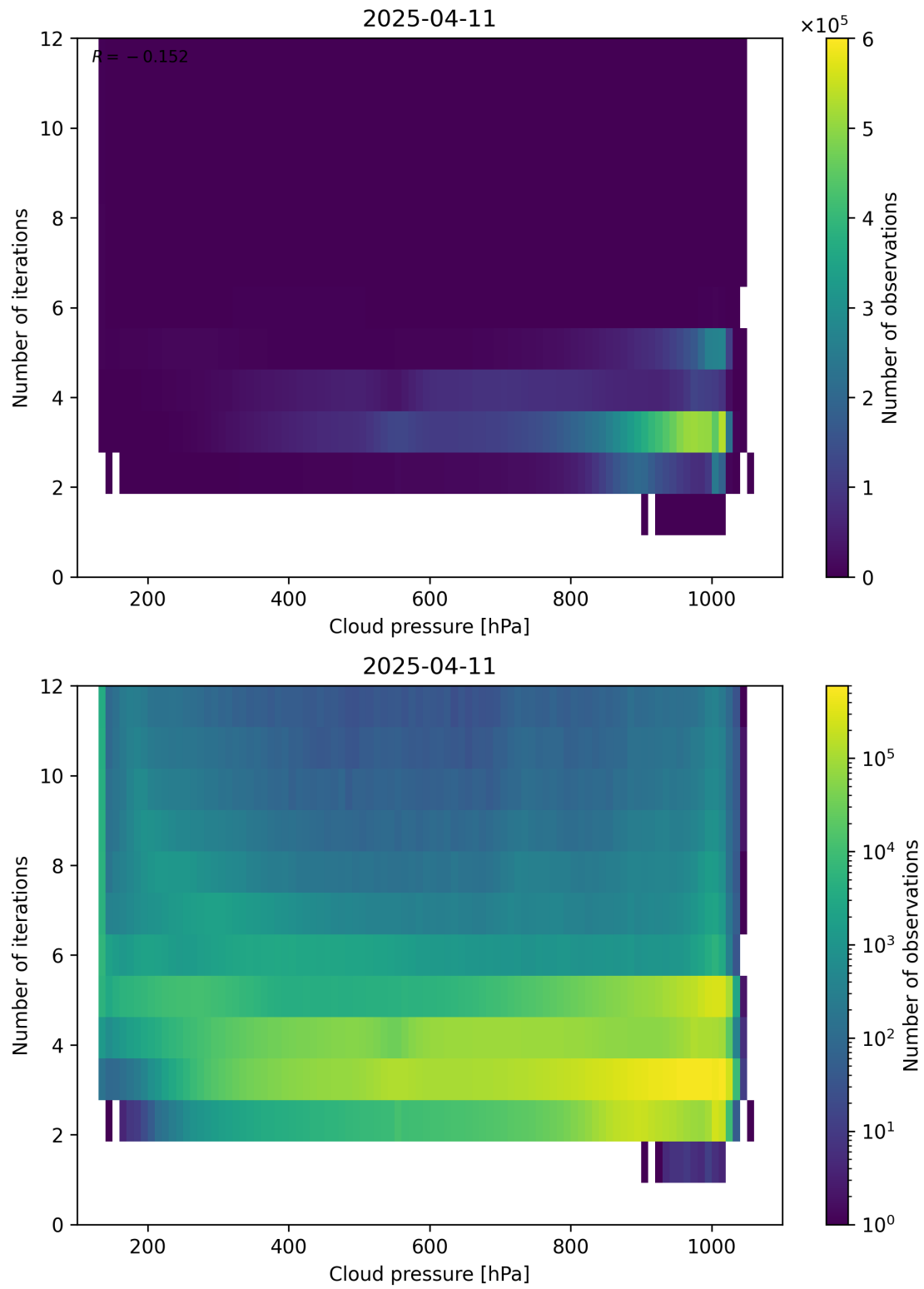
Figure 81: Scatter density plot of “Cloud pressure” against “Number of iterations” for 2025-04-10 to 2025-04-12.
