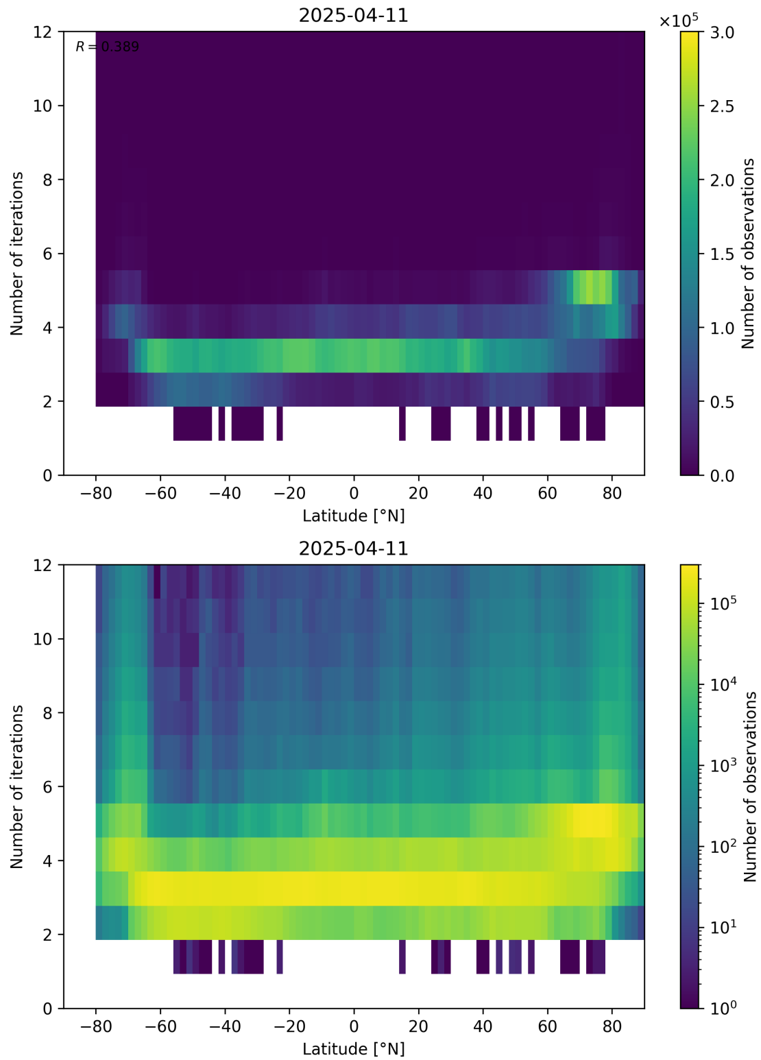
Figure 93: Scatter density plot of “Latitude” against “Number of iterations” for 2025-04-10 to 2025-04-12.
