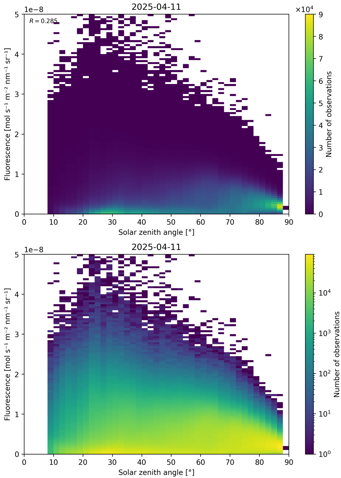
Figure 112: Scatter density plot of “Solar zenith angle” against “Fluorescence” for 2025-04-10 to 2025-04-12.
