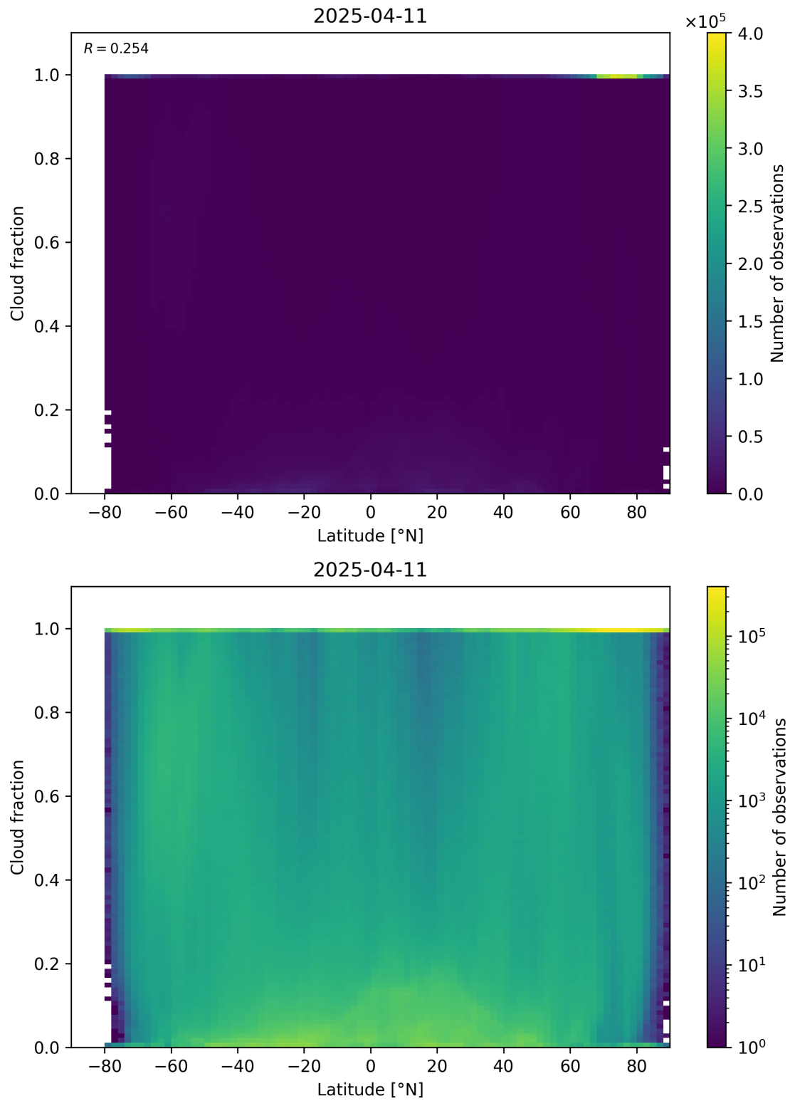
Figure 90: Scatter density plot of “Latitude” against “Cloud fraction” for 2025-04-10 to 2025-04-12.
