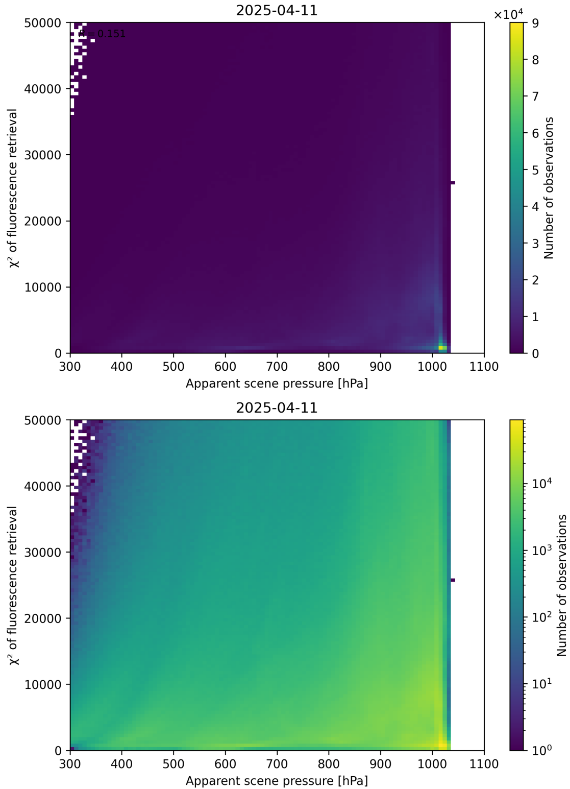
Figure 63: Scatter density plot of “Apparent scene pressure” against “ \chi^2 of fluorescence retrieval” for 2025-04-10 to 2025-04-12.
