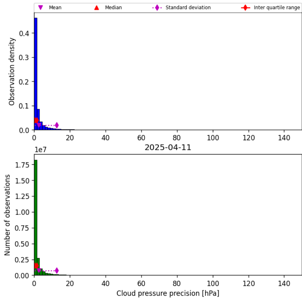
Figure 31: Histogram of “Cloud pressure precision” for 2025-04-10 to 2025-04-12
