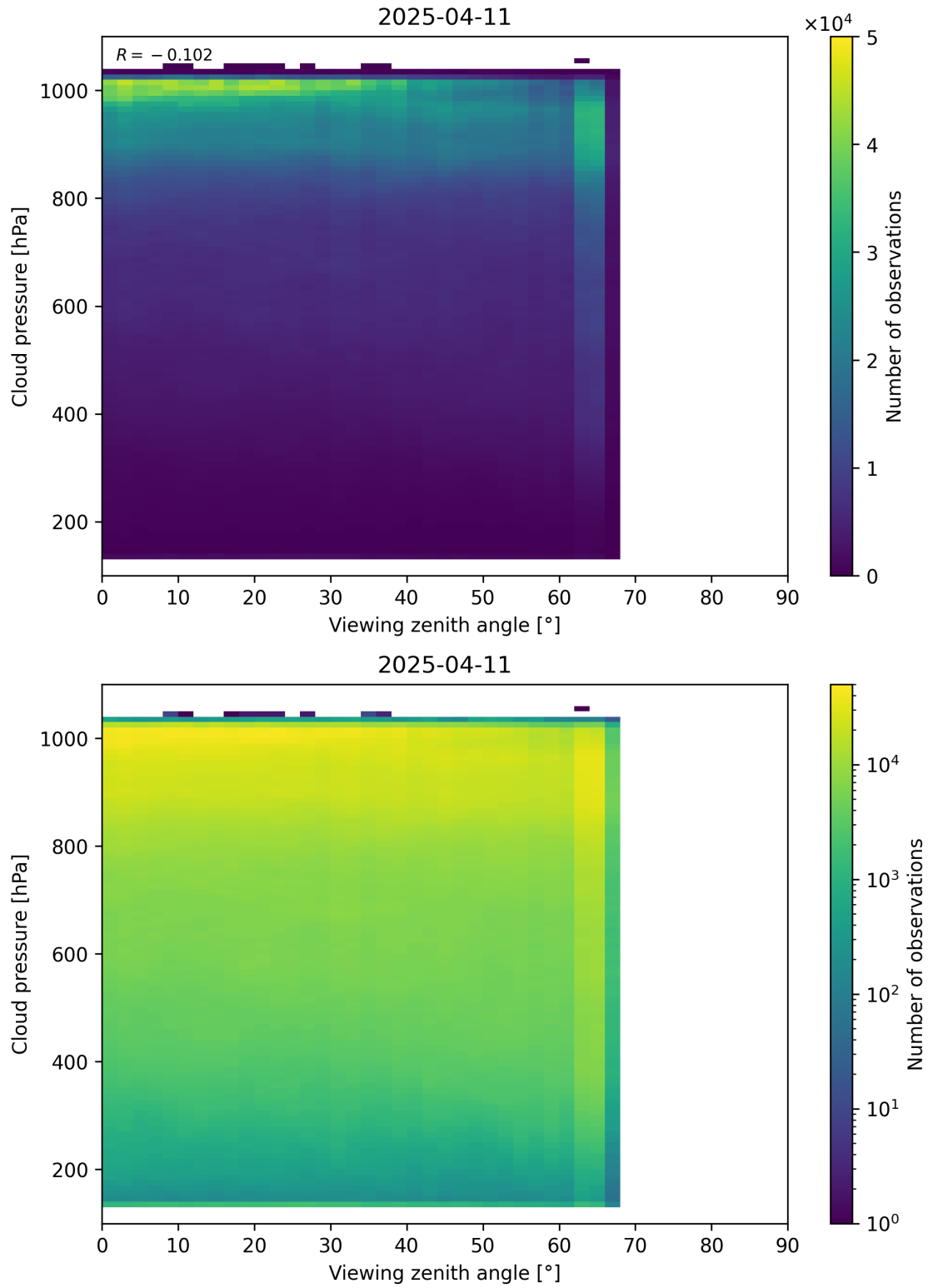
Figure 121: Scatter density plot of “Viewing zenith angle” against “Cloud pressure” for 2025-04-10 to 2025-04-12.
