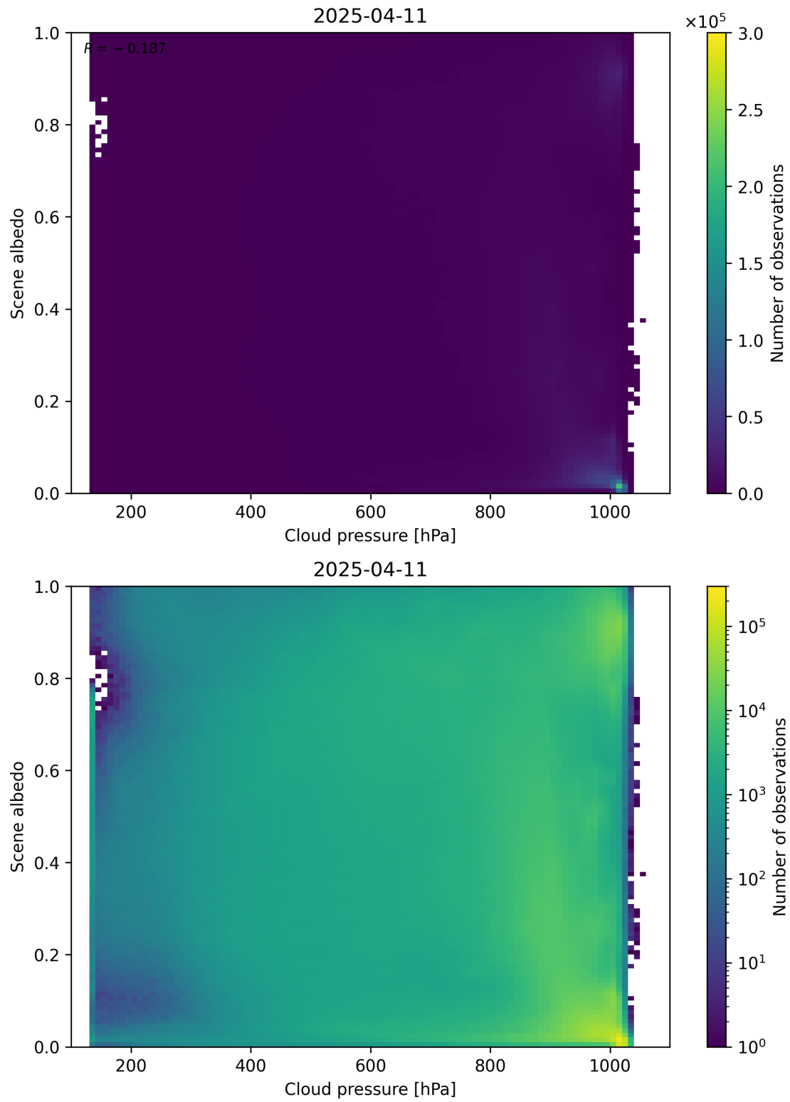
Figure 83: Scatter density plot of “Cloud pressure” against “Scene albedo” for 2025-04-10 to 2025-04-12.
