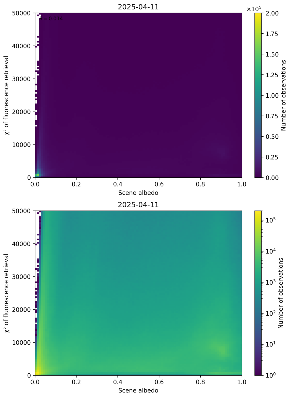
Figure 103: Scatter density plot of “Scene albedo” against “ \chi^2 of fluorescence retrieval” for 2025-04-10 to 2025-04-12.
