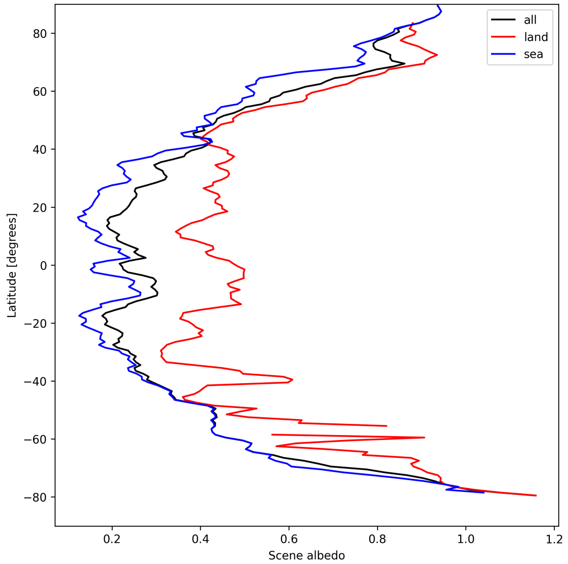
Figure 17: Zonal average of “Scene albedo” for 2025-04-10 to 2025-04-12.
