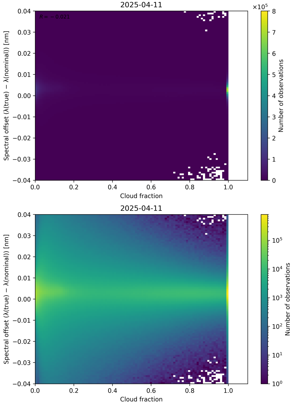
Figure 76: Scatter density plot of “Cloud fraction” against “Spectral offset ( \lambda_{\text{true}} - \lambda_{\text{nominal}} )” for 2025-04-10 to 2025-04-12.
