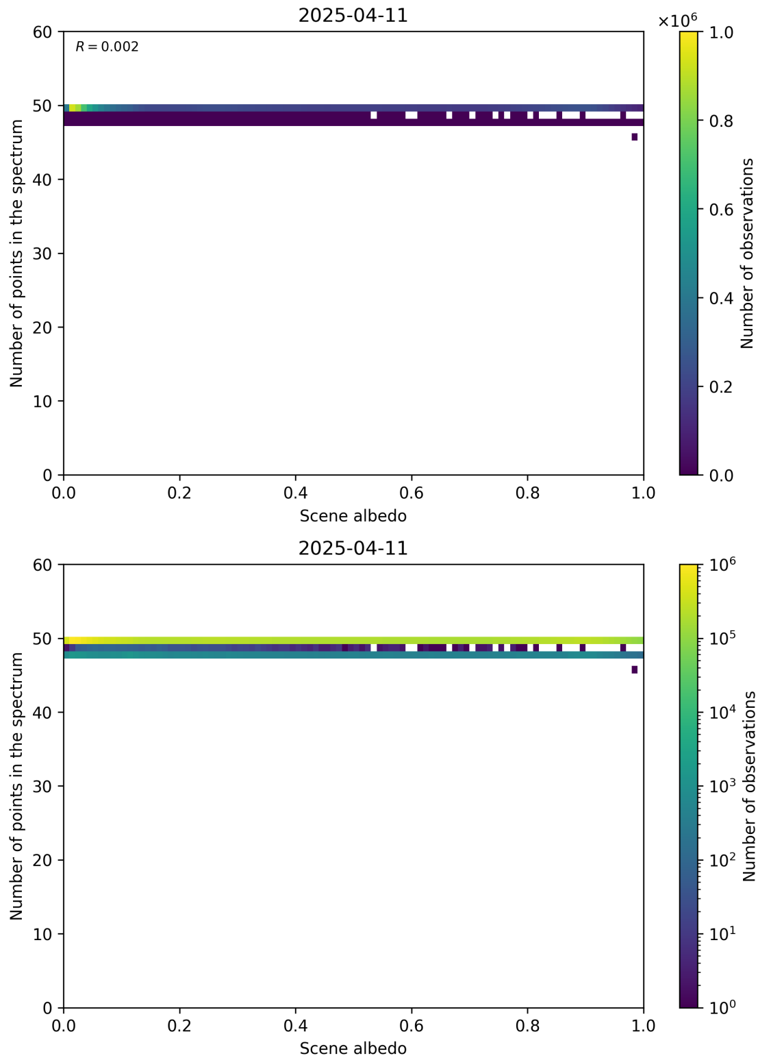
Figure 106: Scatter density plot of “Scene albedo” against “Number of points in the spectrum” for 2025-04-10 to 2025-04-12.
