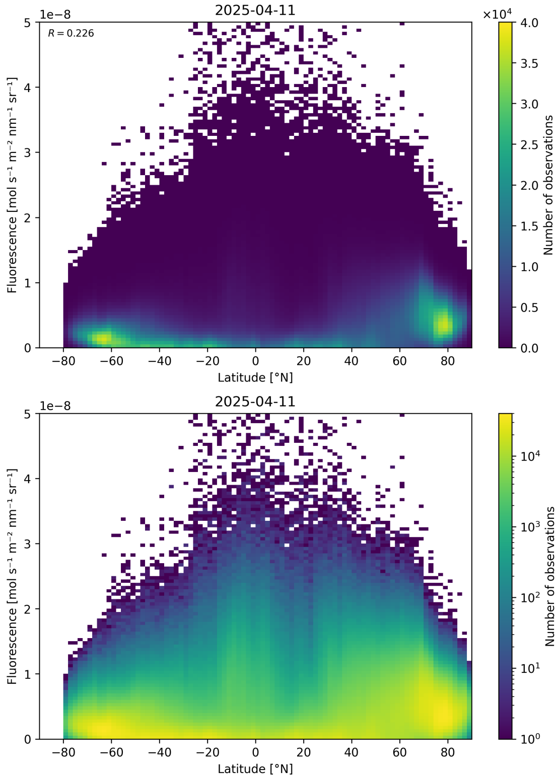
Figure 92: Scatter density plot of “Latitude” against “Fluorescence” for 2025-04-10 to 2025-04-12.
