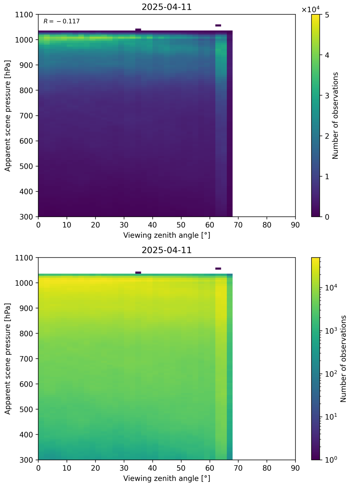
Figure 118: Scatter density plot of “Viewing zenith angle” against “Apparent scene pressure” for 2025-04-10 to 2025-04-12.
