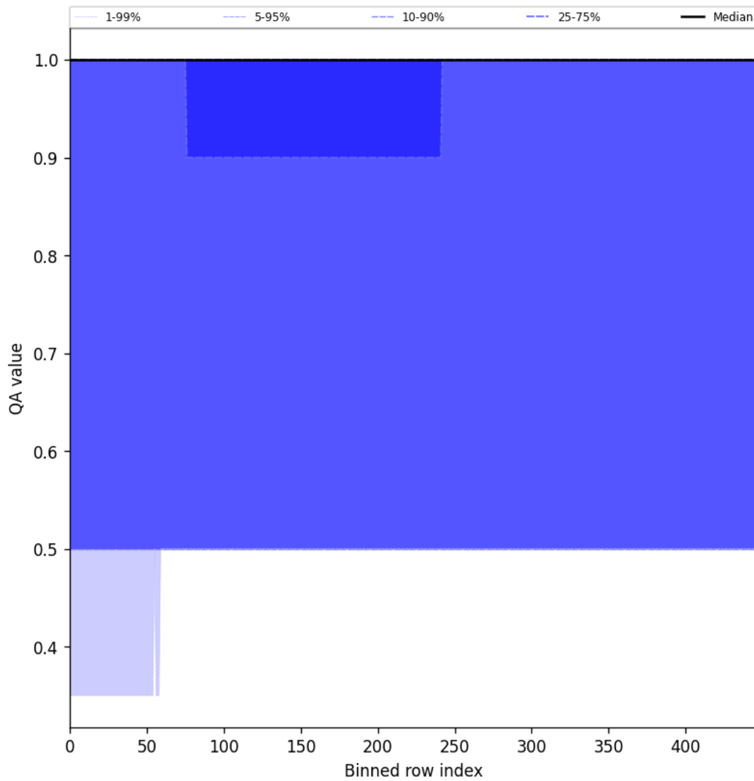
Figure 46: Along track statistics of “QA value” for 2025-04-10 to 2025-04-12
