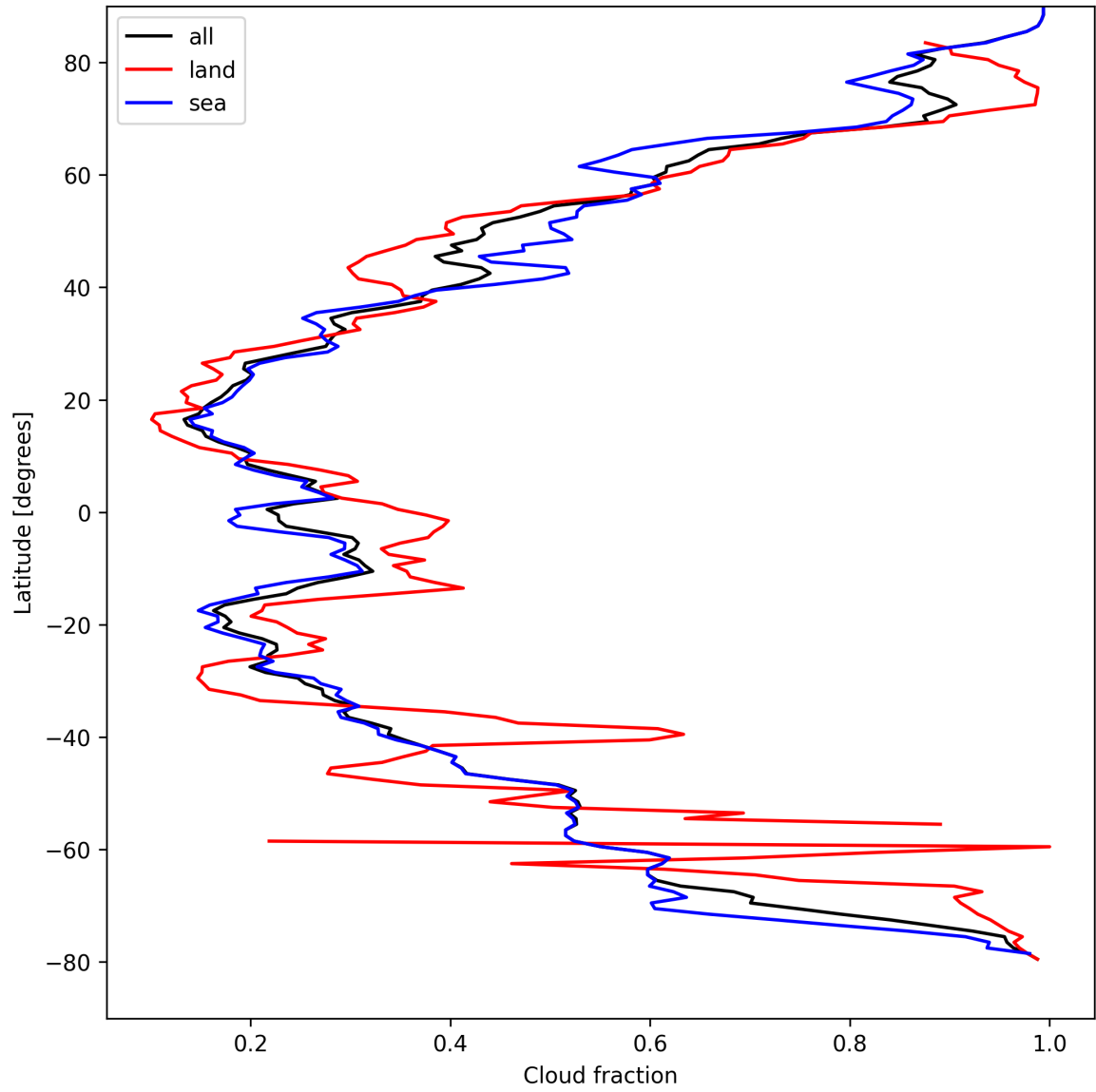
Figure 15: Zonal average of “Cloud fraction” for 2025-04-10 to 2025-04-12.
