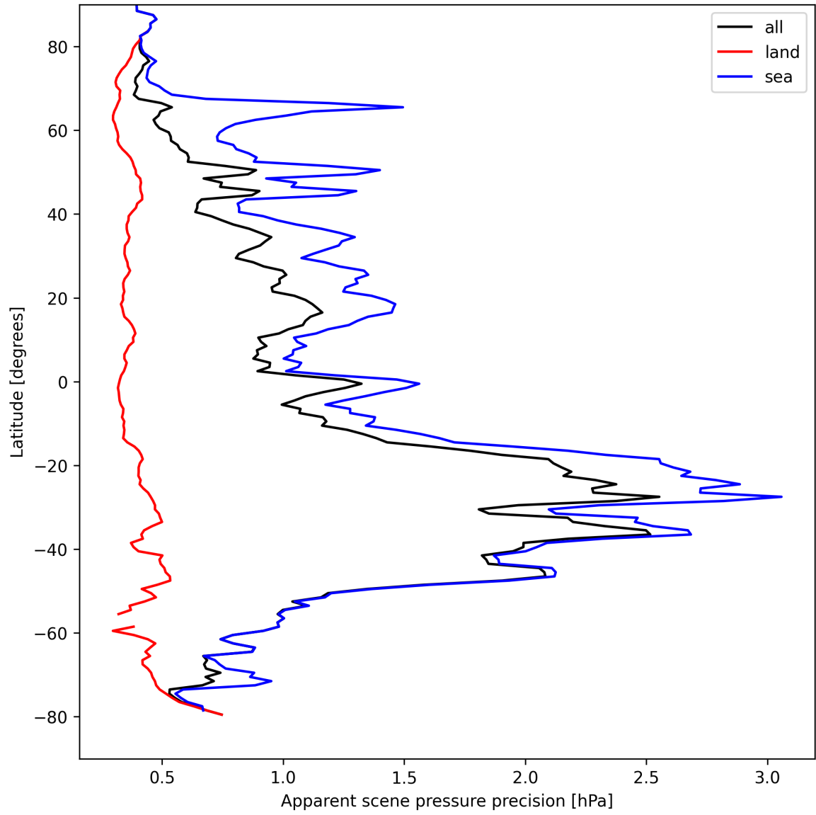
Figure 20: Zonal average of “Apparent scene pressure precision” for 2025-04-10 to 2025-04-12.
