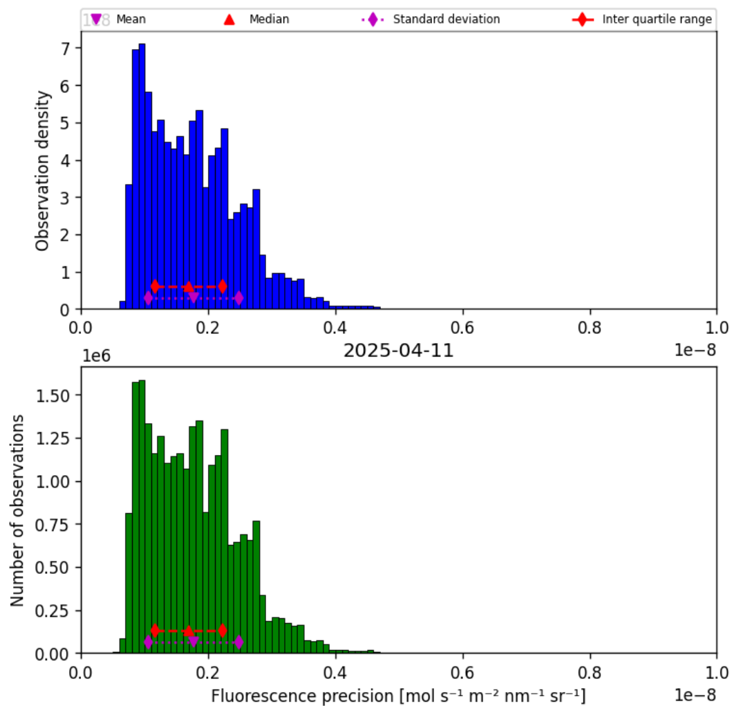
Figure 41: Histogram of “Fluorescence precision” for 2025-04-10 to 2025-04-12
