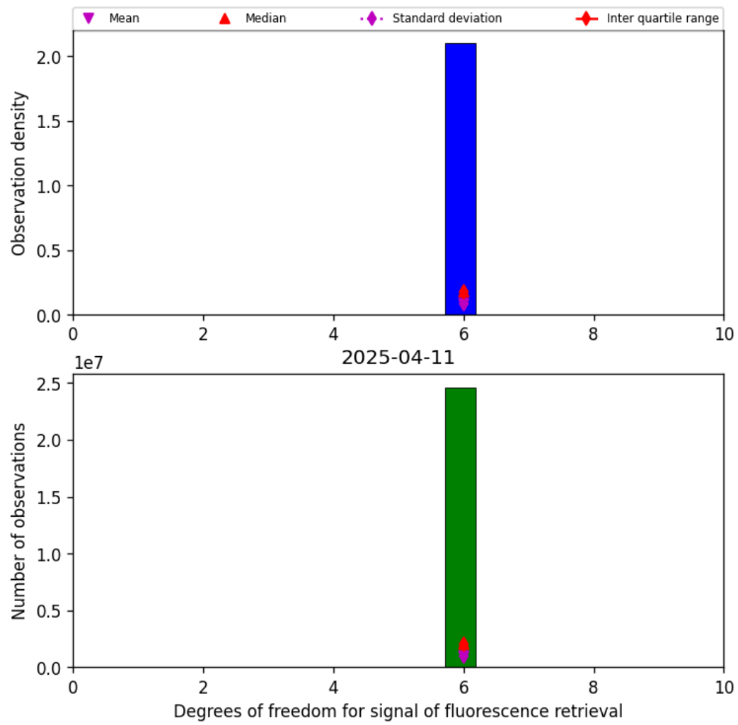
Figure 43: Histogram of “Degrees of freedom for signal of fluorescence retrieval” for 2025-04-10 to 2025-04-12
