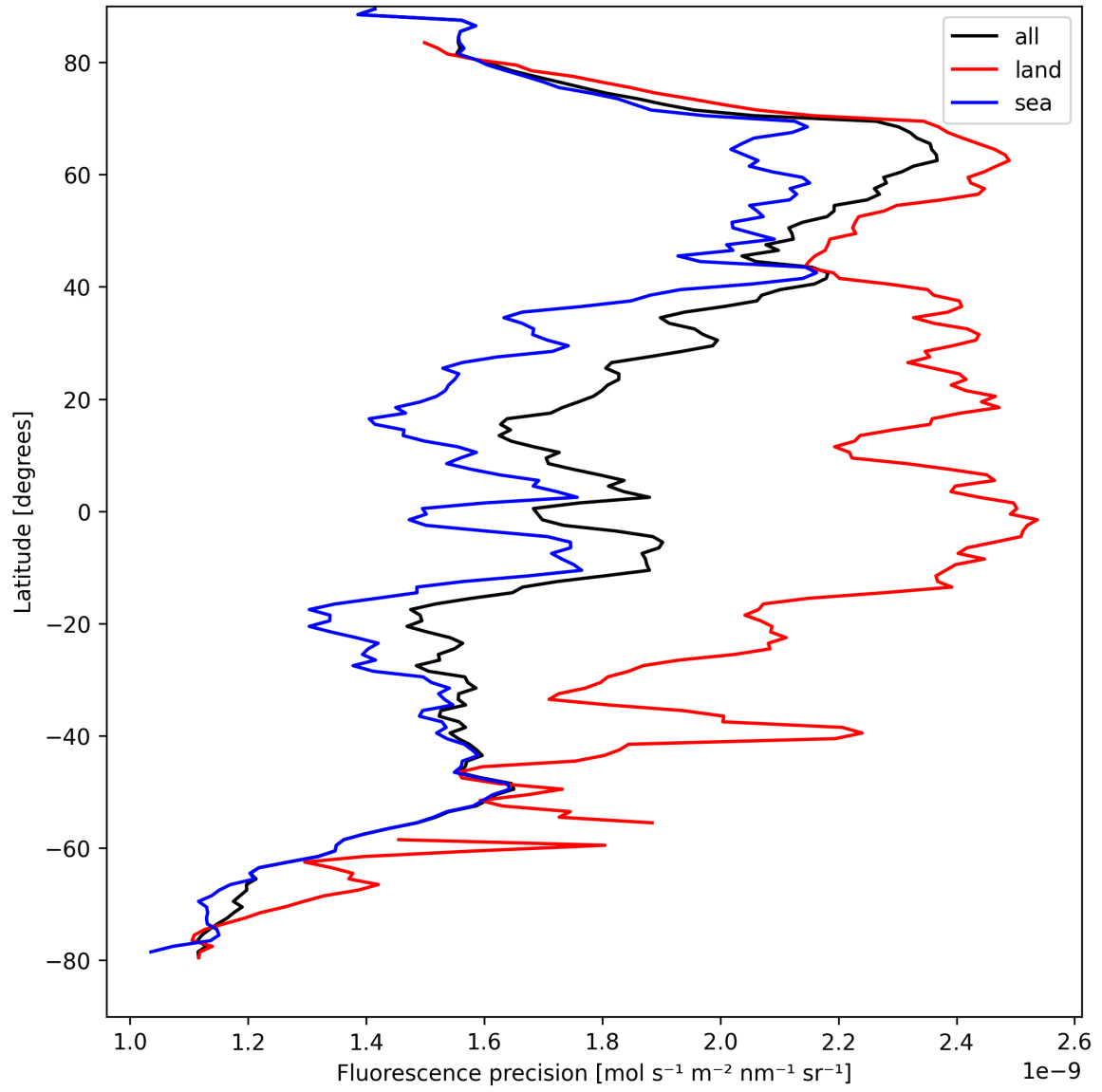
Figure 24: Zonal average of “Fluorescence precision” for 2025-04-10 to 2025-04-12.
