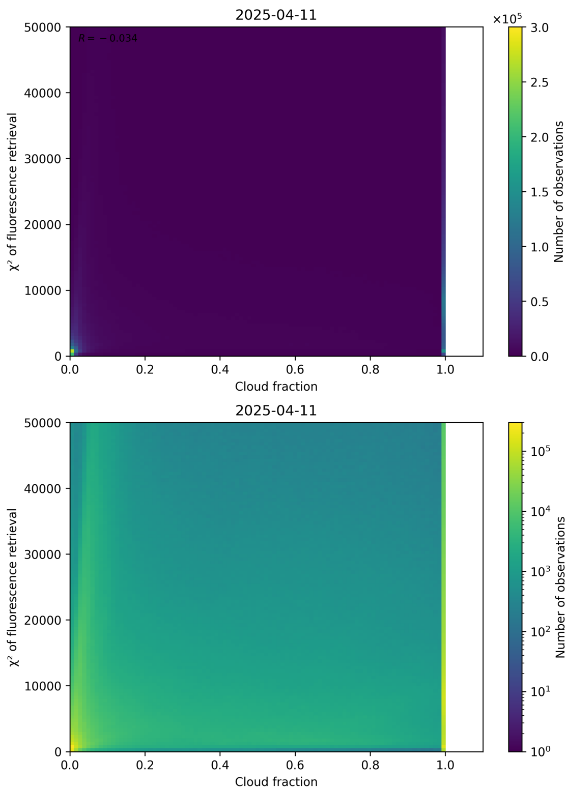
Figure 71: Scatter density plot of “Cloud fraction” against “ \chi^2 of fluorescence retrieval” for 2025-04-10 to 2025-04-12.
