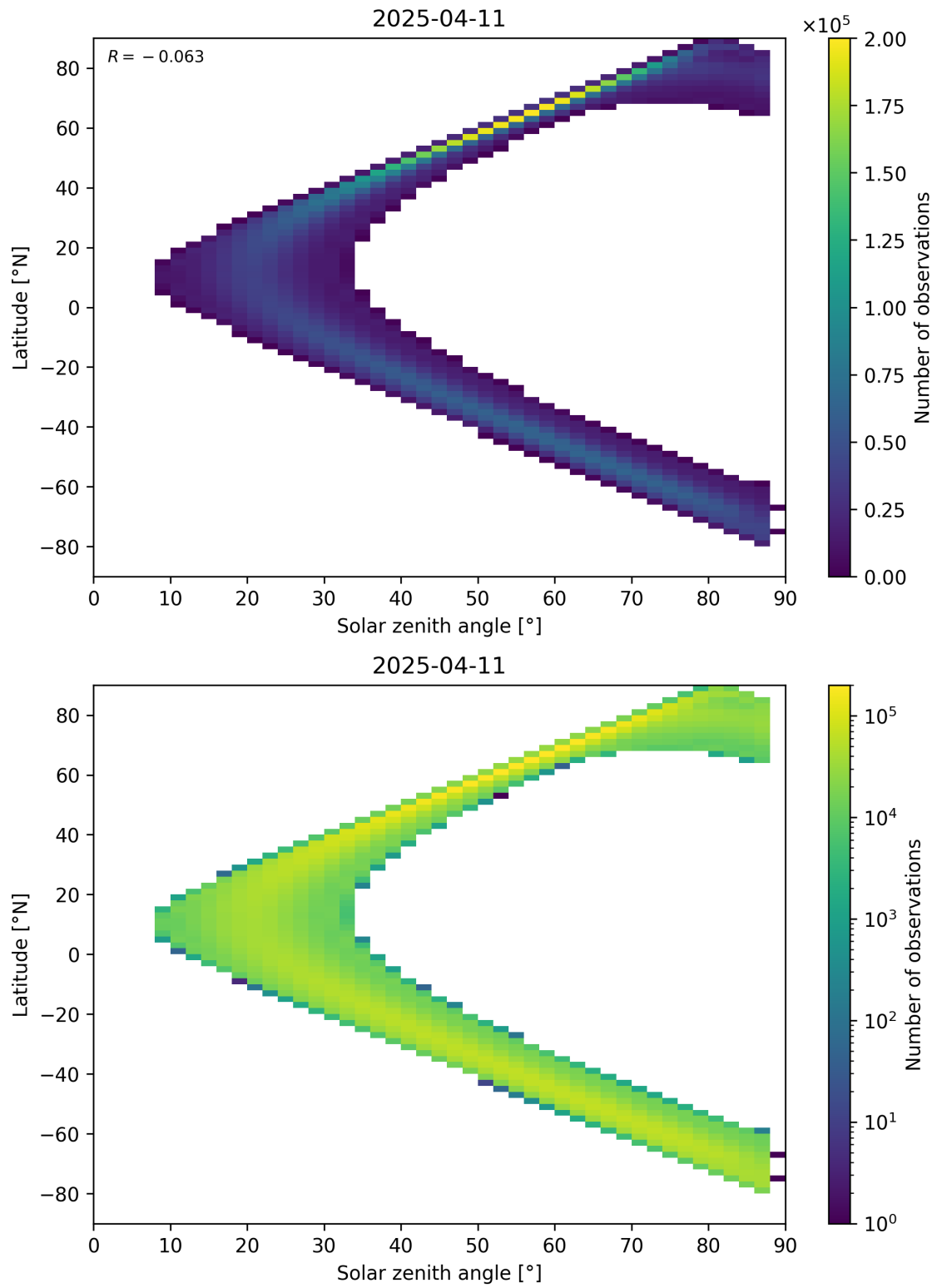
Figure 113: Scatter density plot of “Solar zenith angle” against “Latitude” for 2025-04-10 to 2025-04-12.
