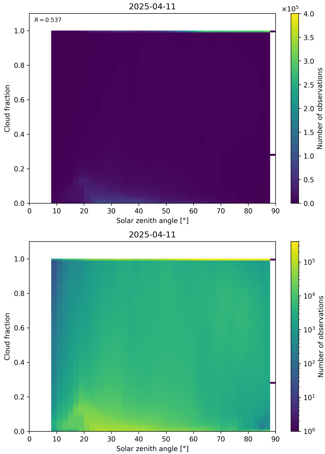
Figure 110: Scatter density plot of “Solar zenith angle” against “Cloud fraction” for 2025-04-10 to 2025-04-12.
