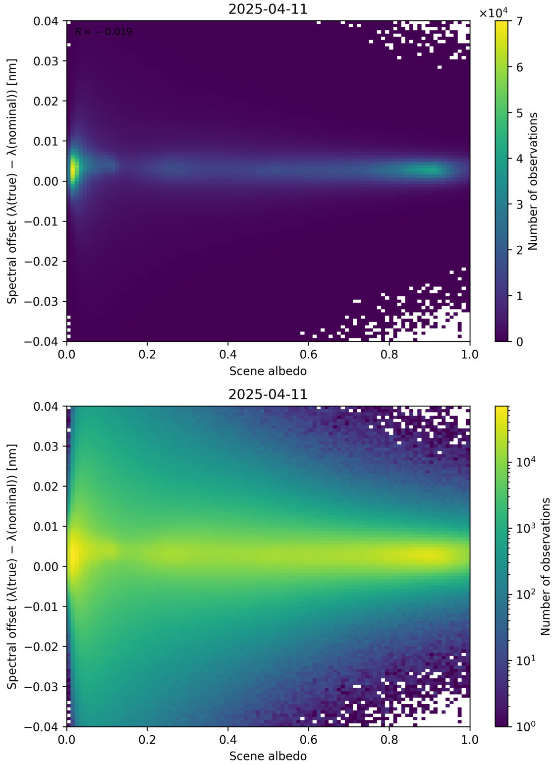
Figure 107: Scatter density plot of “Scene albedo” against “Spectral offset ( \lambda_{\text{true}} - \lambda_{\text{nominal}} )” for 2025-04-10 to 2025-04-12.
