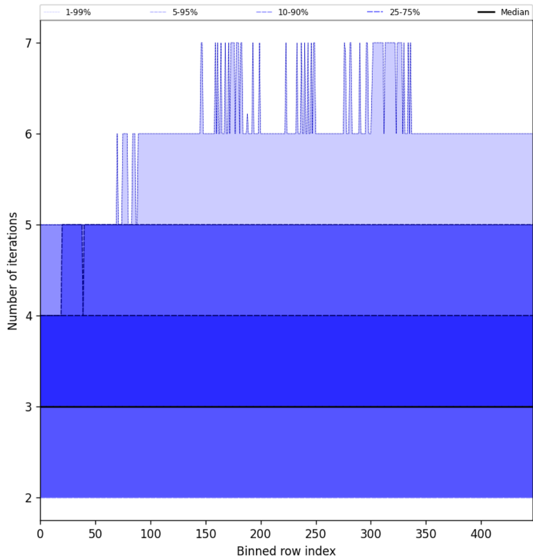
Figure 56: Along track statistics of “Number of iterations” for 2025-04-10 to 2025-04-12
