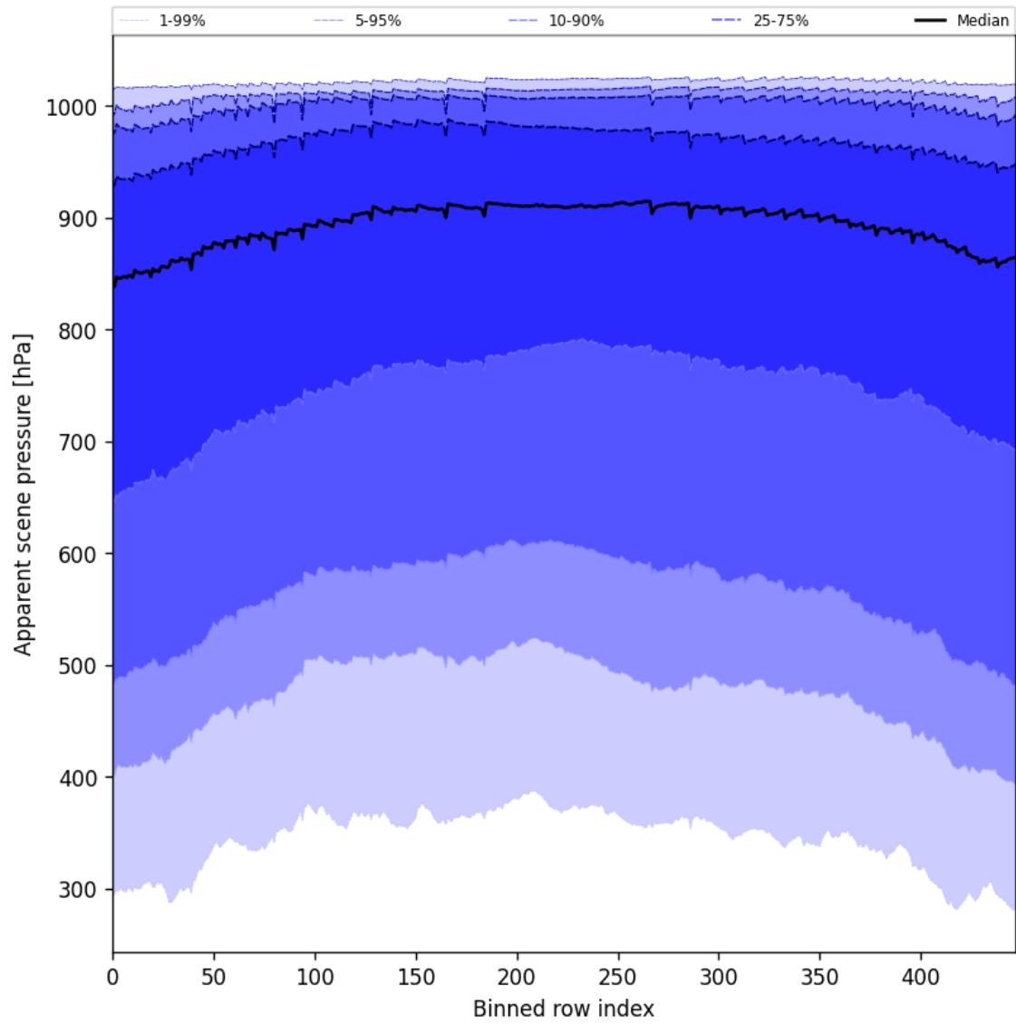
Figure 53: Along track statistics of “Apparent scene pressure” for 2025-04-10 to 2025-04-12
