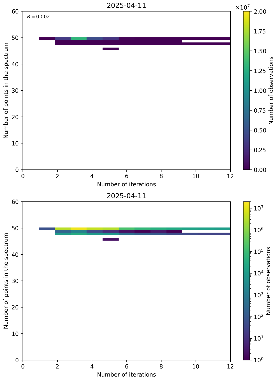
Figure 99: Scatter density plot of “Number of iterations” against “Number of points in the spectrum” for 2025-04-10 to 2025-04-12.
