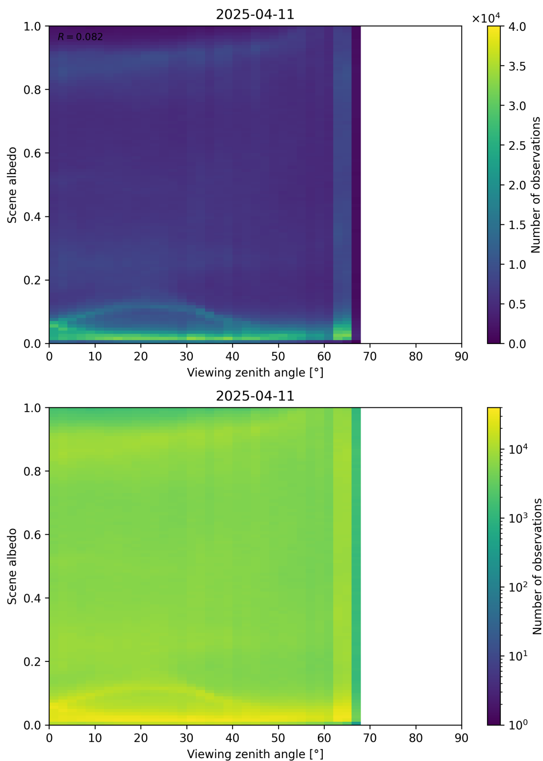
Figure 126: Scatter density plot of “Viewing zenith angle” against “Scene albedo” for 2025-04-10 to 2025-04-12.
