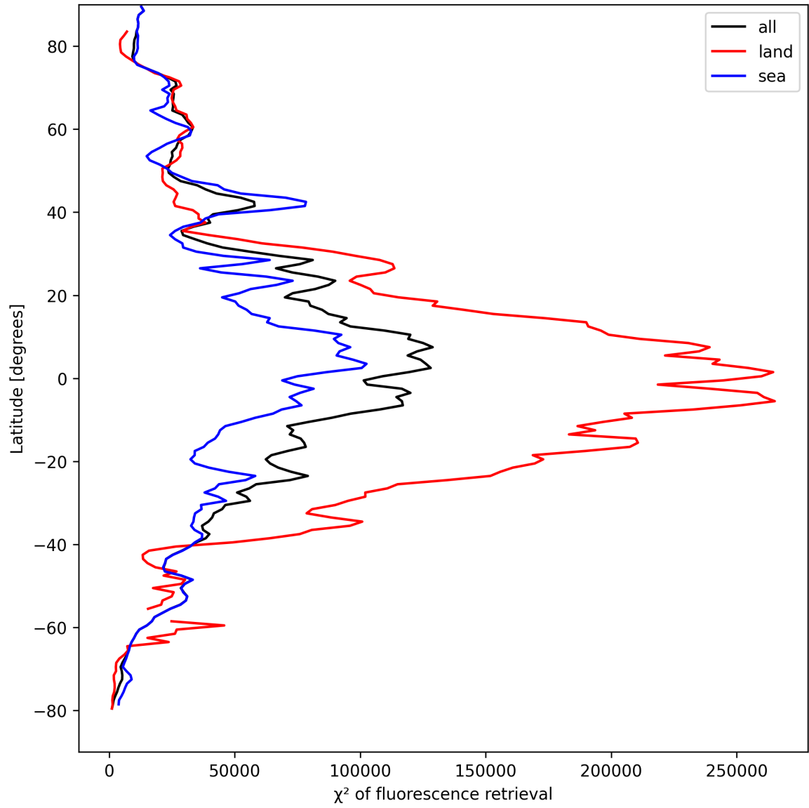
Figure 25: Zonal average of “ \chi^2 of fluorescence retrieval” for 2025-04-10 to 2025-04-12.
