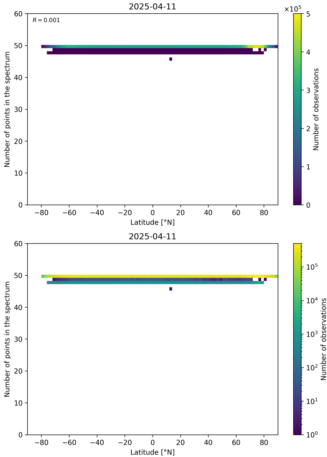
Figure 94: Scatter density plot of “Latitude” against “Number of points in the spectrum” for 2025-04-10 to 2025-04-12.
