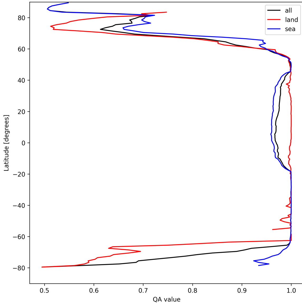
Figure 12: Zonal average of “QA value” for 2025-04-10 to 2025-04-12.
