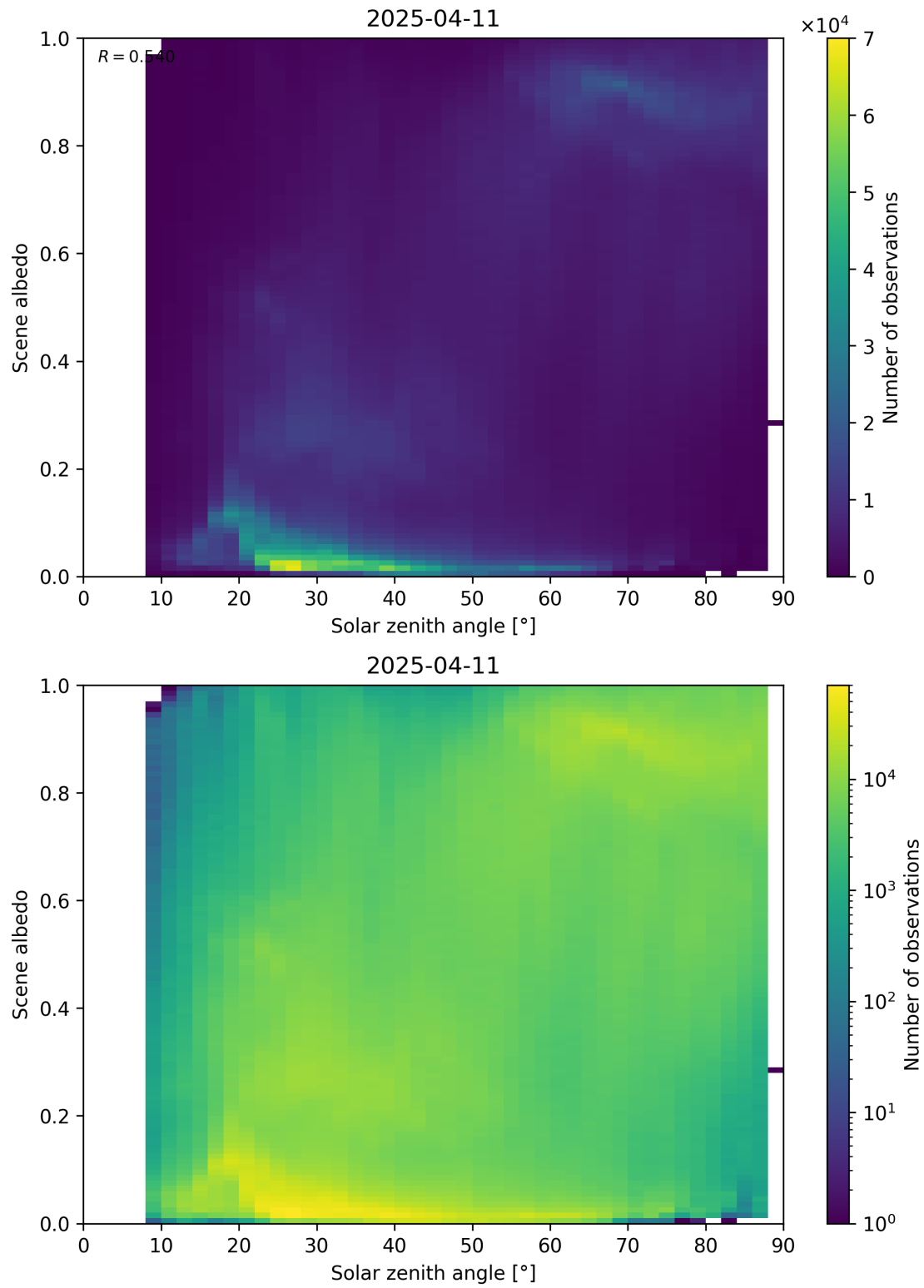
Figure 116: Scatter density plot of “Solar zenith angle” against “Scene albedo” for 2025-04-10 to 2025-04-12.
