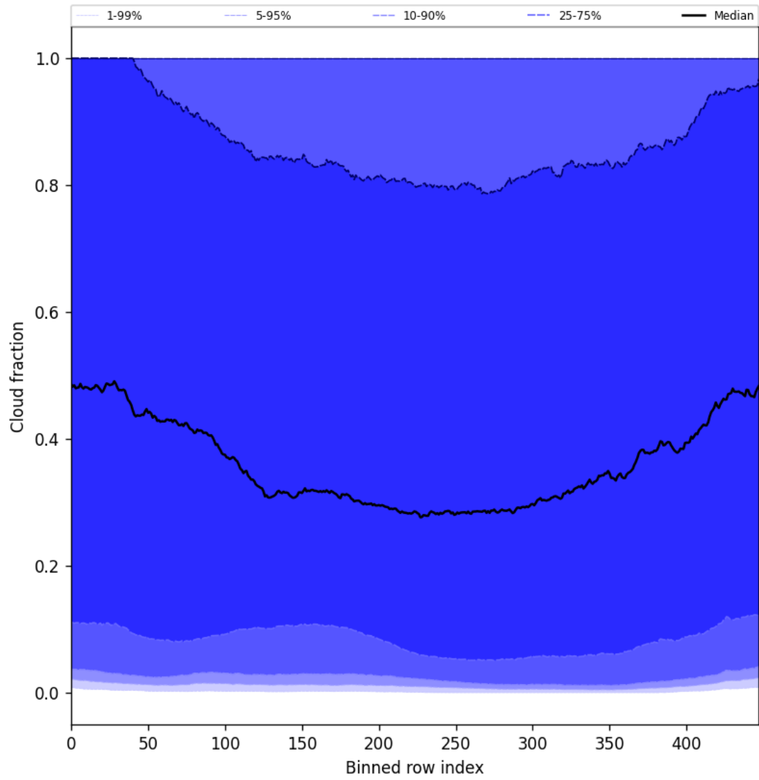
Figure 49: Along track statistics of “Cloud fraction” for 2025-04-10 to 2025-04-12
