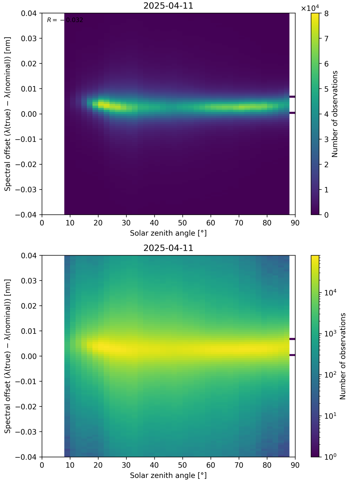
Figure 117: Scatter density plot of “Solar zenith angle” against “Spectral offset ( \lambda_{\text{true}} - \lambda_{\text{nominal}} )” for 2025-04-10 to 2025-04-12.
