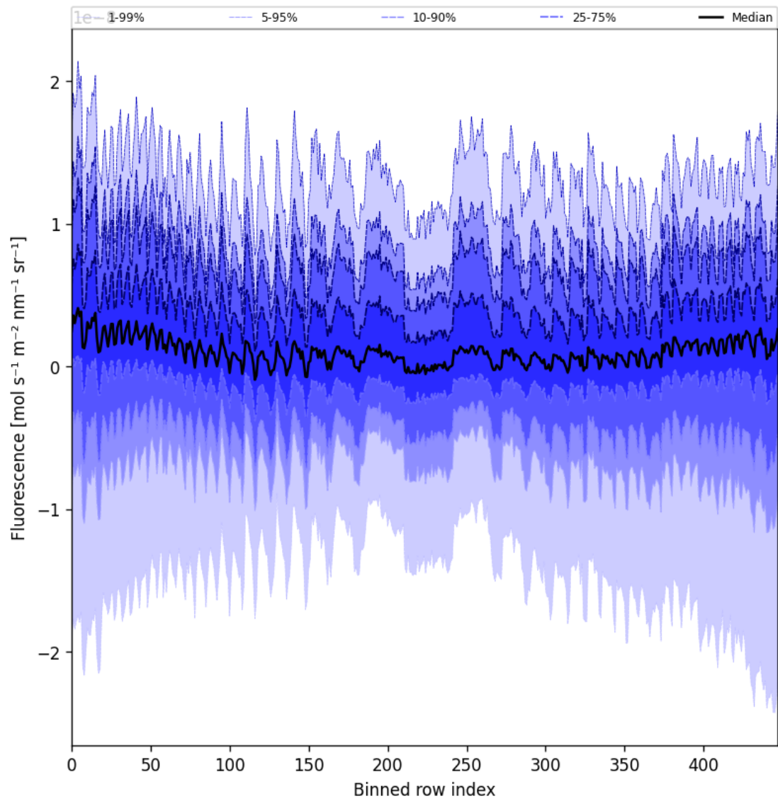
Figure 57: Along track statistics of “Fluorescence” for 2025-04-10 to 2025-04-12
