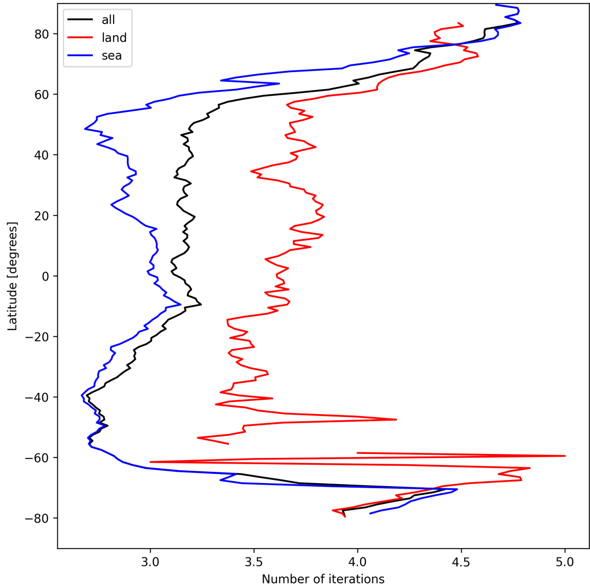
Figure 22: Zonal average of “Number of iterations” for 2025-04-10 to 2025-04-12.
