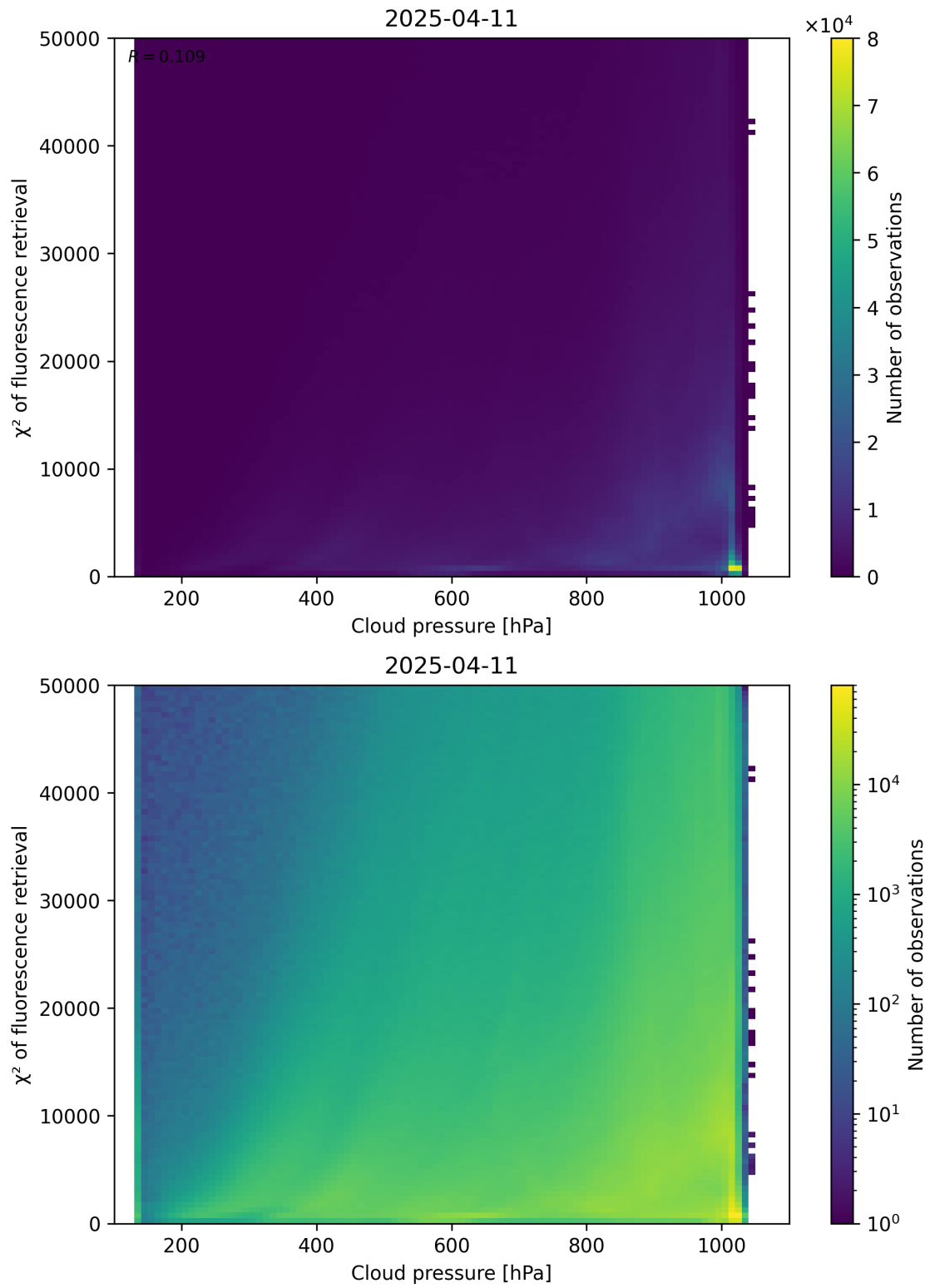
Figure 78: Scatter density plot of “Cloud pressure” against “ \chi^2 of fluorescence retrieval” for 2025-04-10 to 2025-04-12.
