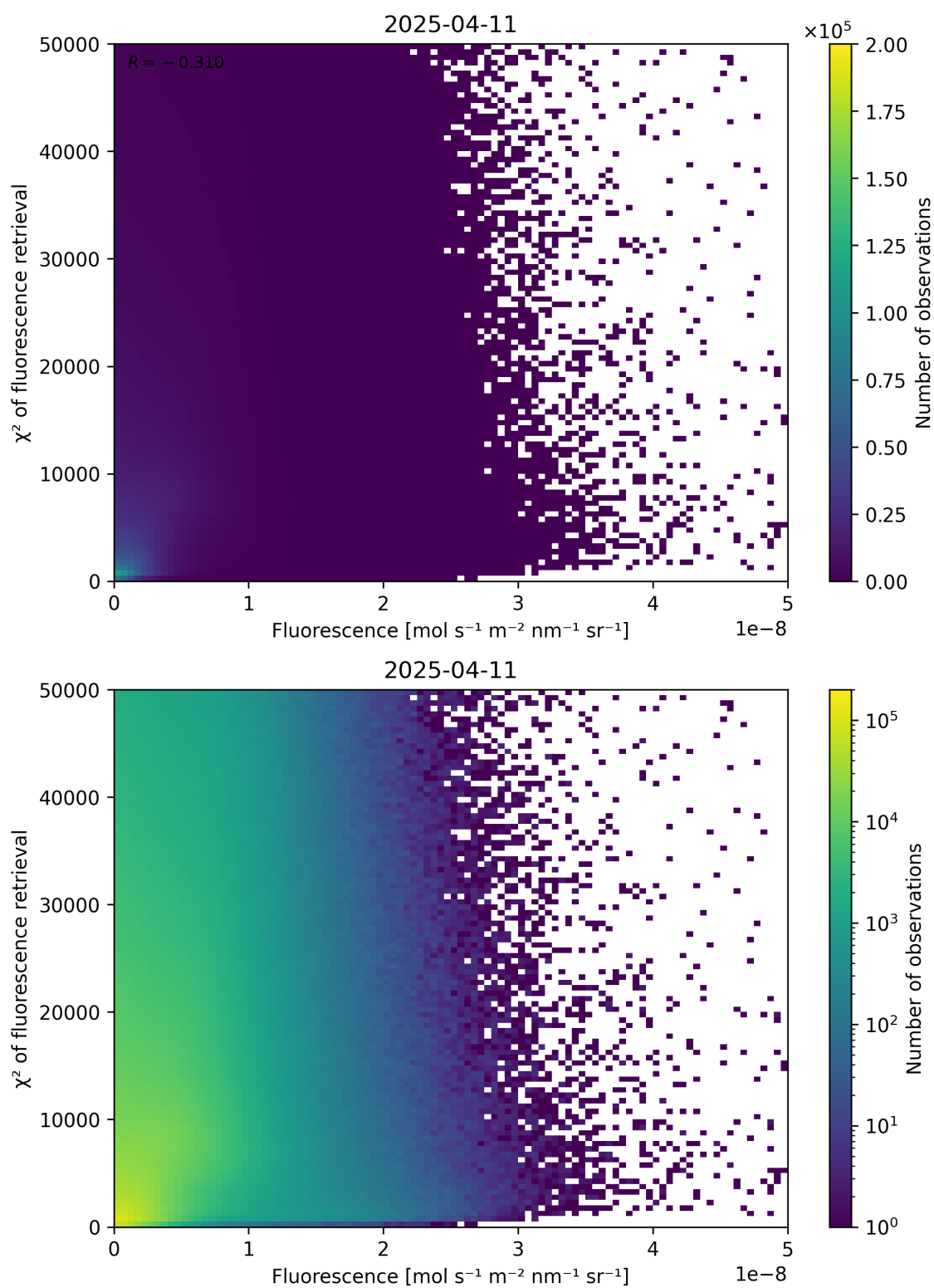
Figure 85: Scatter density plot of “Fluorescence” against “ \chi^2 of fluorescence retrieval” for 2025-04-10 to 2025-04-12.
