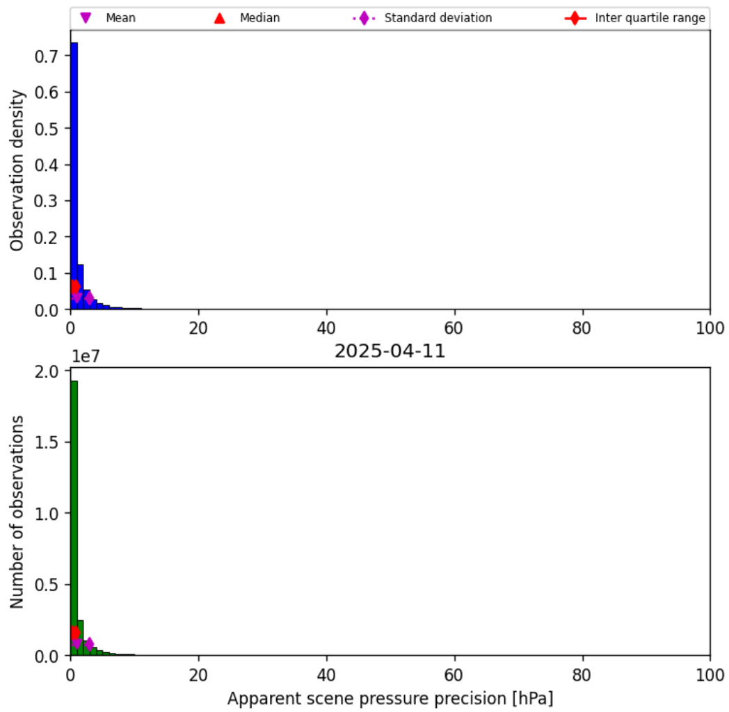
Figure 37: Histogram of “Apparent scene pressure precision” for 2025-04-10 to 2025-04-12
