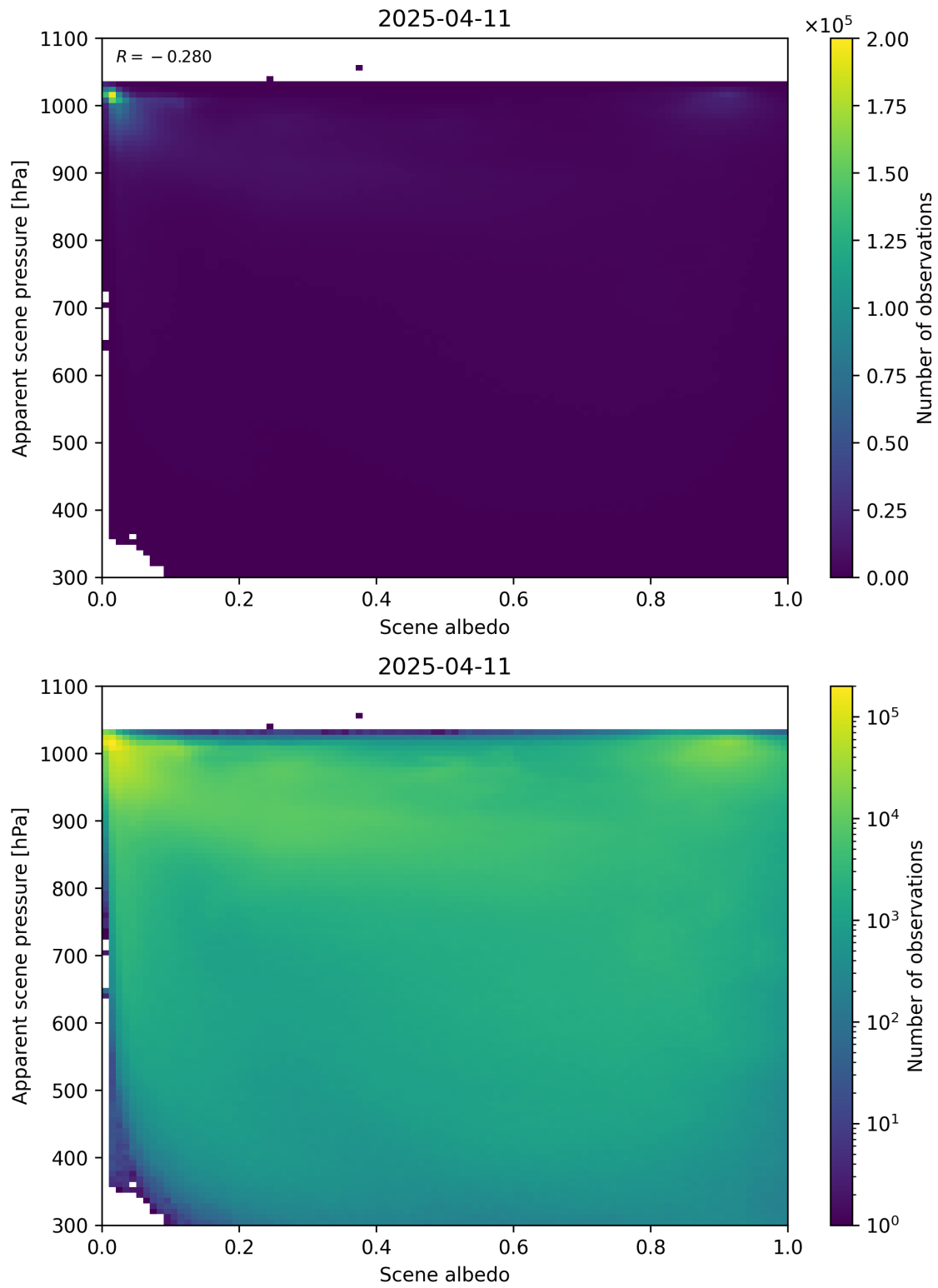
Figure 102: Scatter density plot of “Scene albedo” against “Apparent scene pressure” for 2025-04-10 to 2025-04-12.
