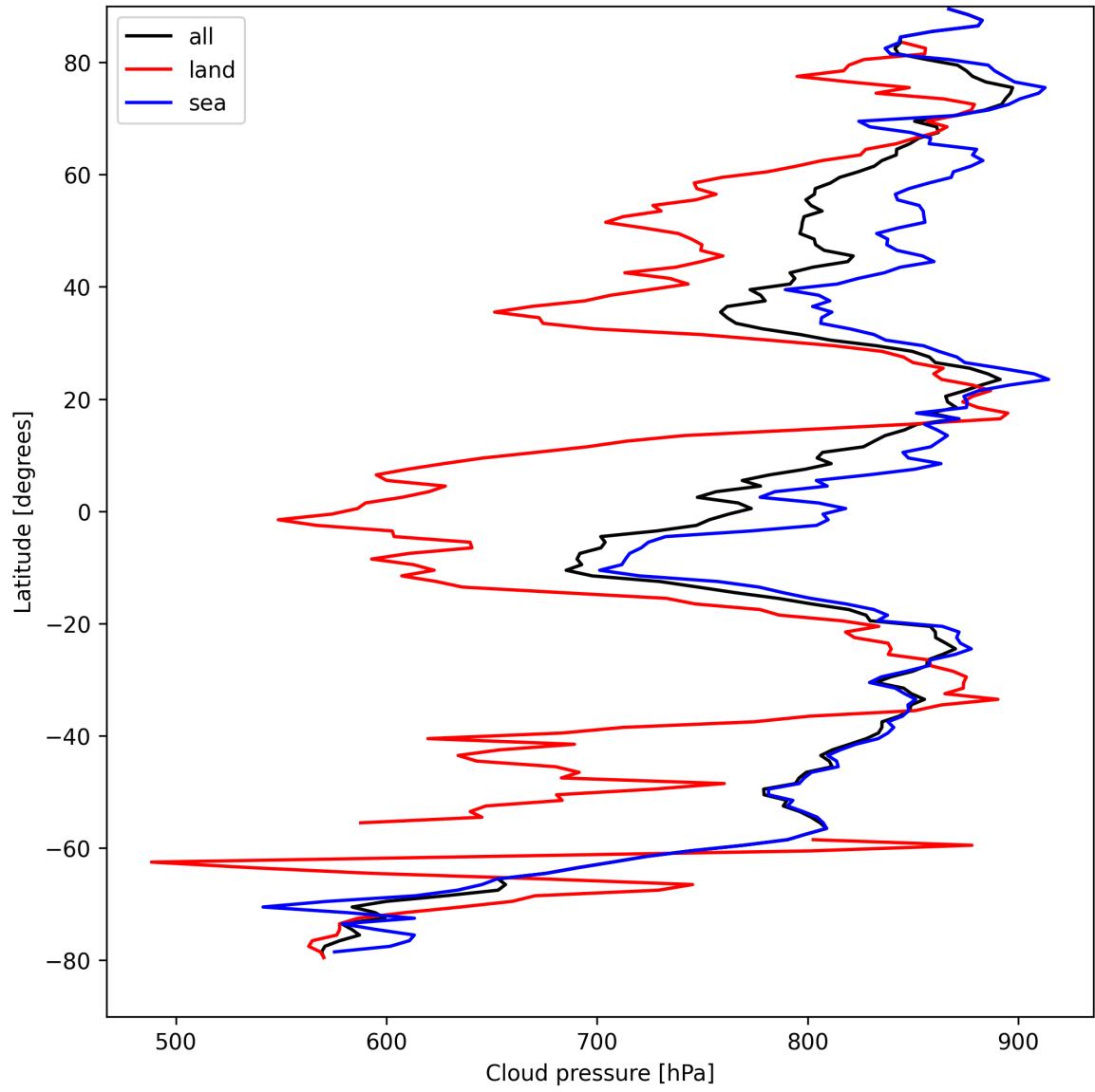
Figure 13: Zonal average of “Cloud pressure” for 2025-04-10 to 2025-04-12.
