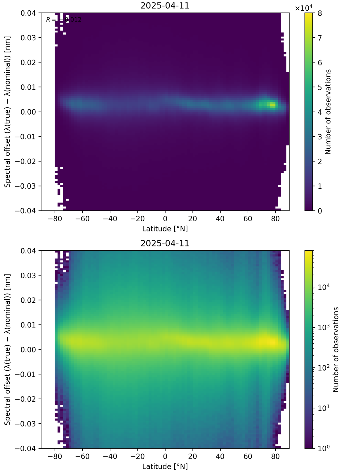
Figure 96: Scatter density plot of “Latitude” against “Spectral offset ( \lambda_{\text{true}} - \lambda_{\text{nominal}} )” for 2025-04-10 to 2025-04-12.
