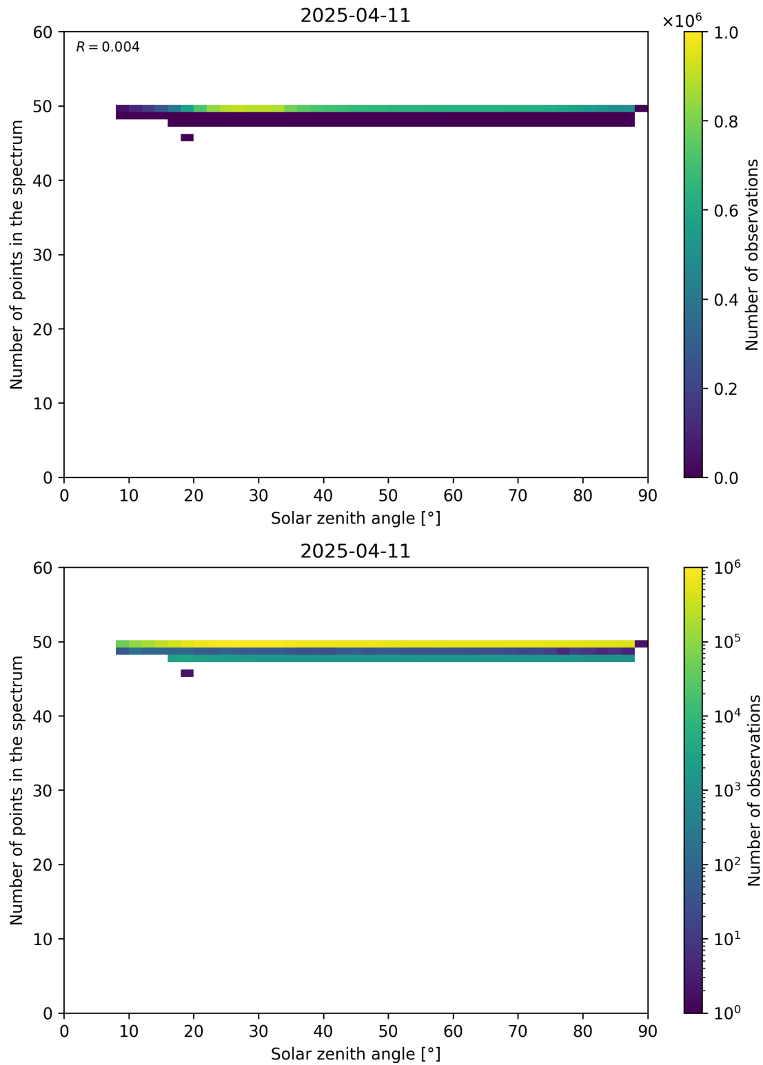
Figure 115: Scatter density plot of “Solar zenith angle” against “Number of points in the spectrum” for 2025-04-10 to 2025-04-12.
