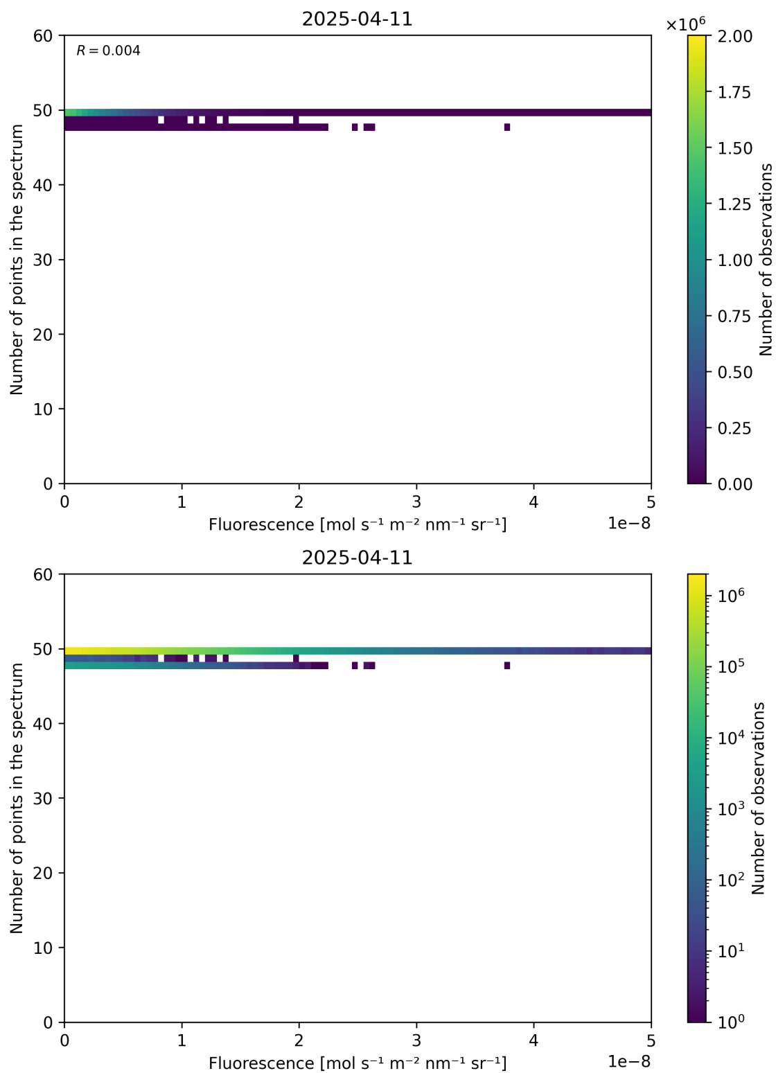
Figure 86: Scatter density plot of “Fluorescence” against “Number of points in the spectrum” for 2025-04-10 to 2025-04-12.
