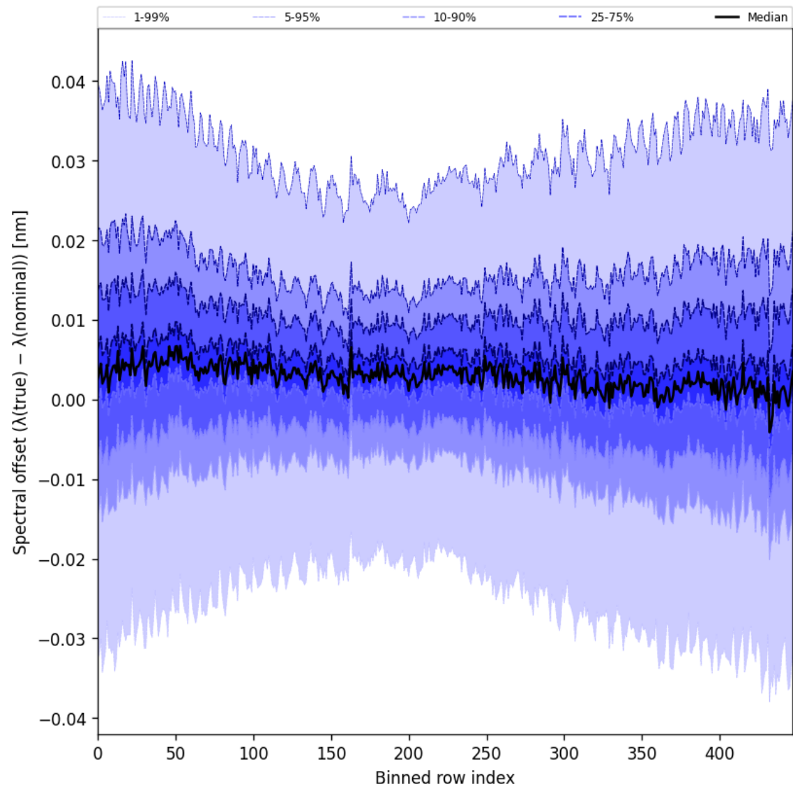
Figure 62: Along track statistics of “Spectral offset ( \lambda_{\text{true}} - \lambda_{\text{nominal}} )” for 2025-04-10 to 2025-04-12
