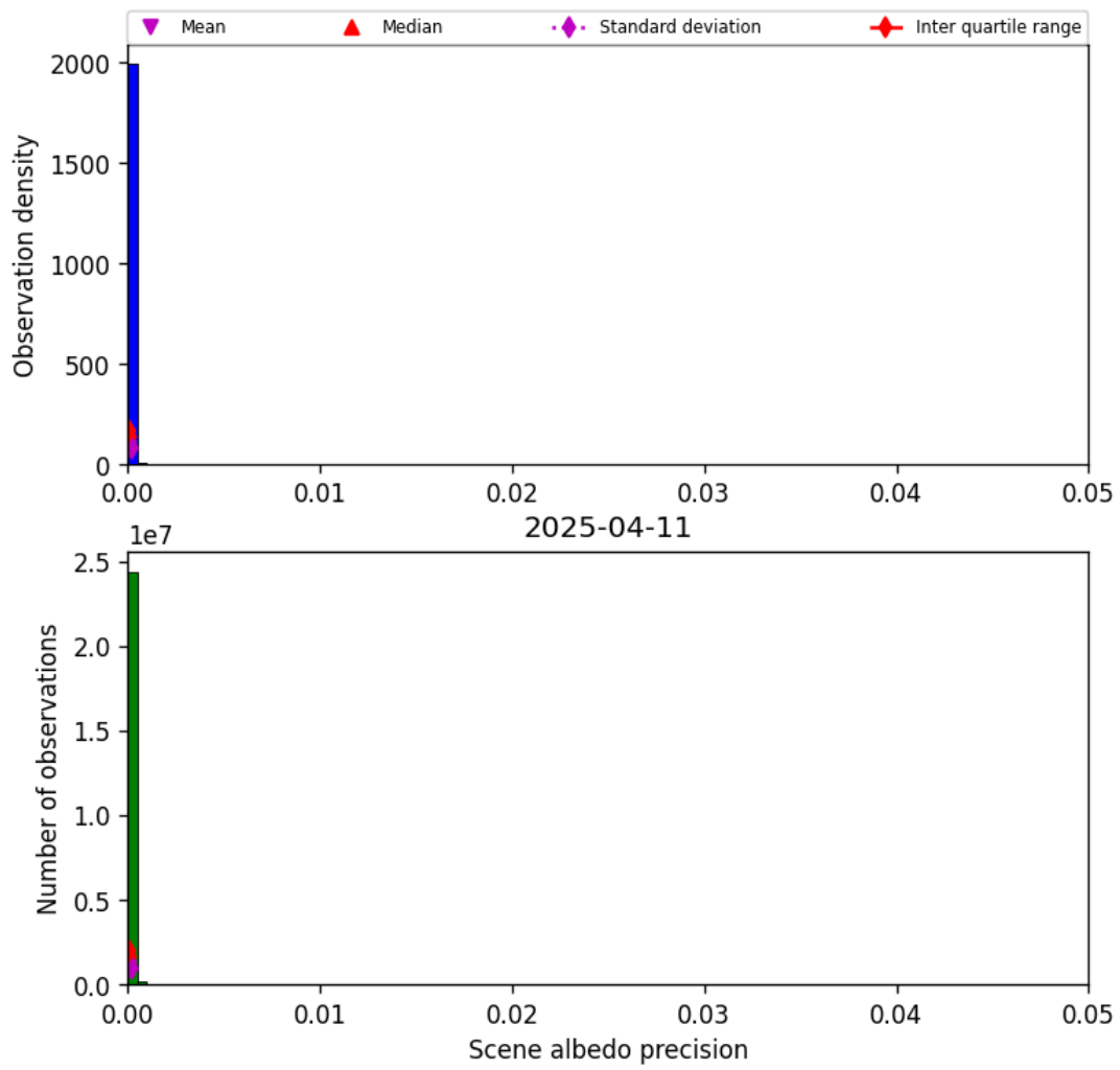
Figure 35: Histogram of “Scene albedo precision” for 2025-04-10 to 2025-04-12
