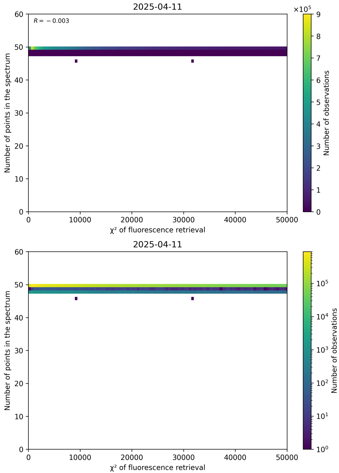
Figure 68: Scatter density plot of “ \chi^2 of fluorescence retrieval” against “Number of points in the spectrum” for 2025-04-10 to 2025-04-12.
