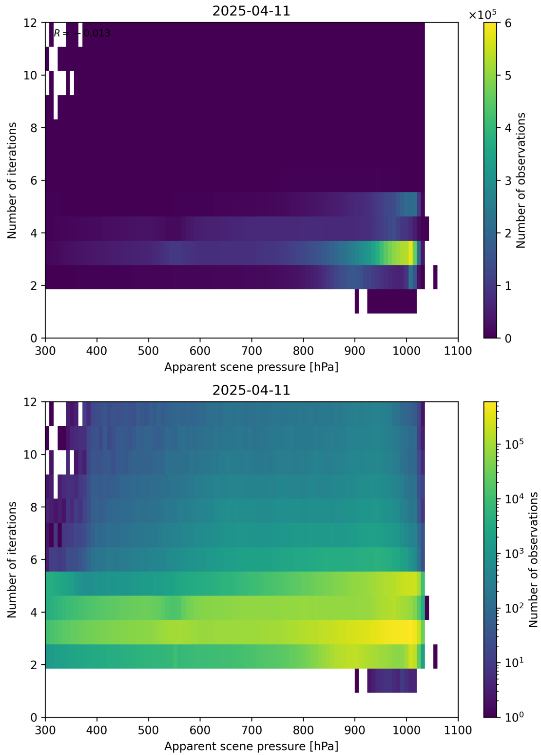
Figure 65: Scatter density plot of “Apparent scene pressure” against “Number of iterations” for 2025-04-10 to 2025-04-12.
