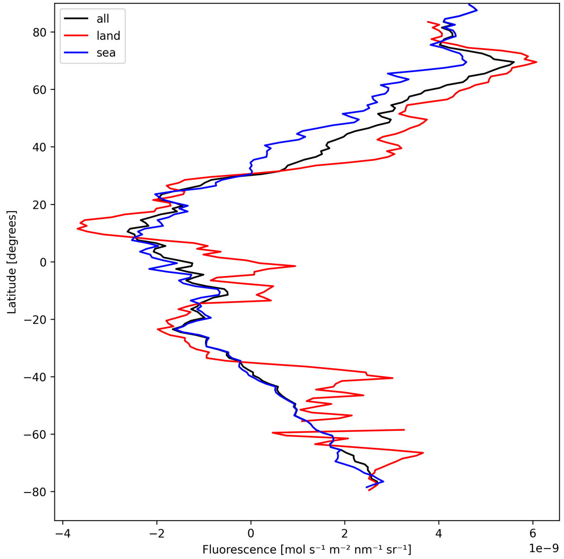
Figure 23: Zonal average of “Fluorescence” for 2025-04-10 to 2025-04-12.
