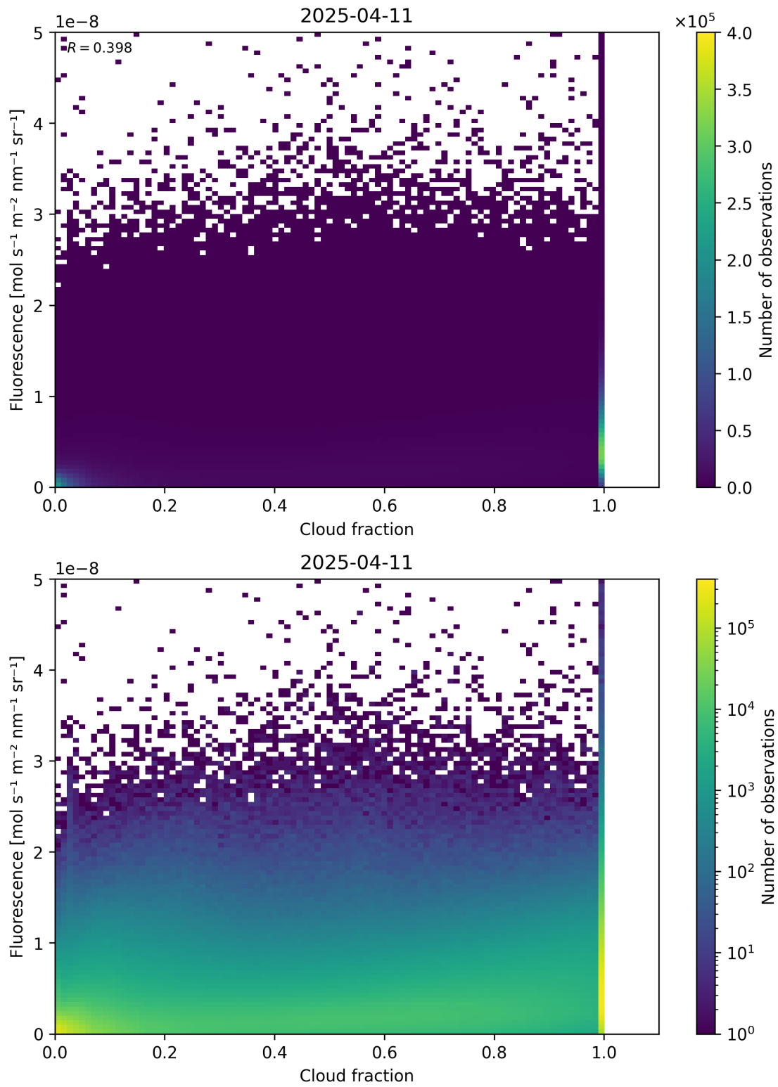
Figure 72: Scatter density plot of “Cloud fraction” against “Fluorescence” for 2025-04-10 to 2025-04-12.
