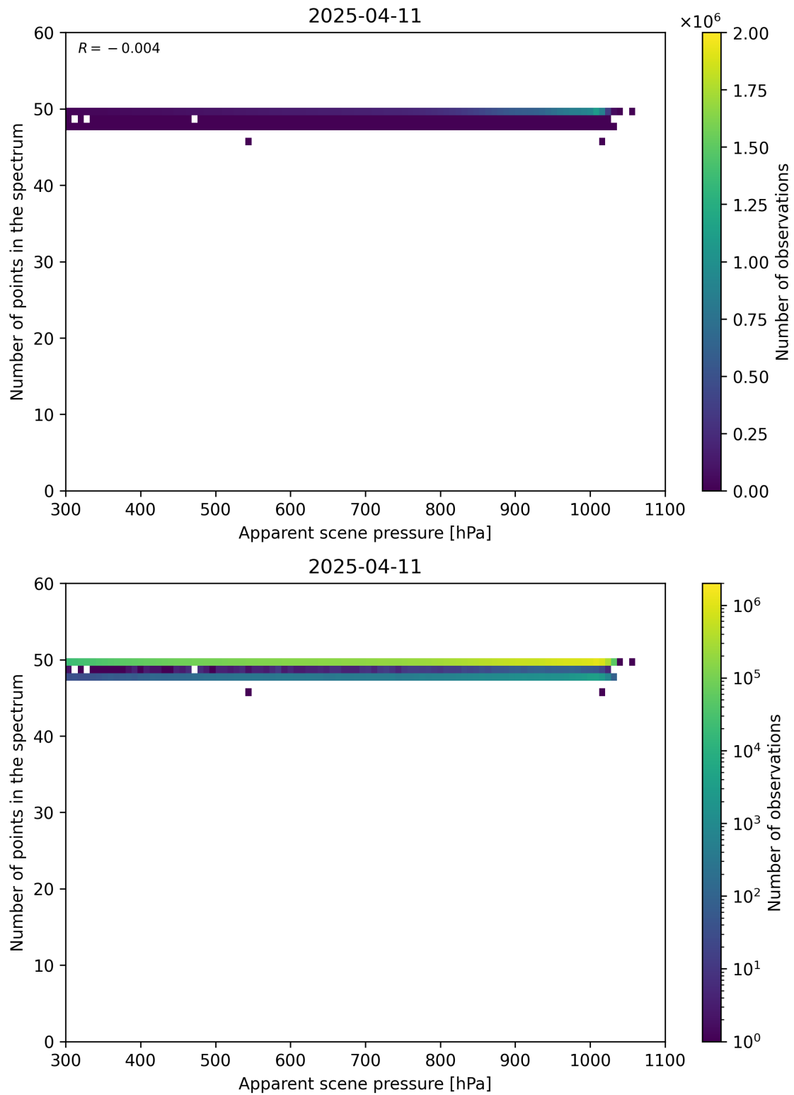
Figure 66: Scatter density plot of “Apparent scene pressure” against “Number of points in the spectrum” for 2025-04-10 to 2025-04-12.
