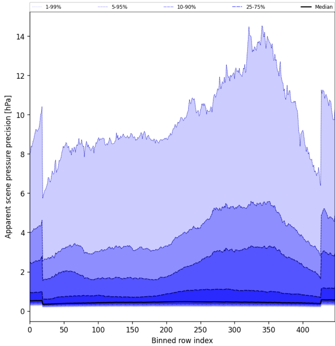
Figure 54: Along track statistics of “Apparent scene pressure precision” for 2025-04-10 to 2025-04-12
