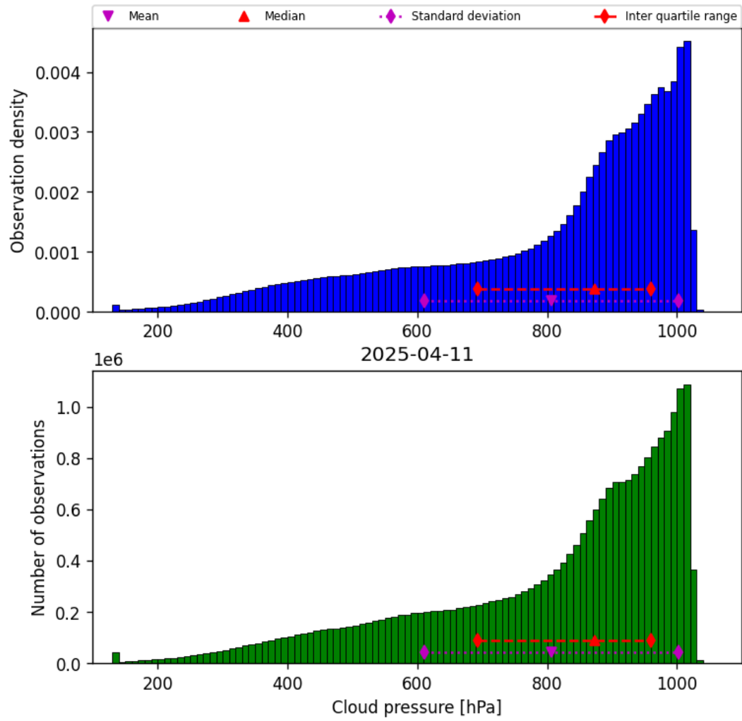
Figure 30: Histogram of “Cloud pressure” for 2025-04-10 to 2025-04-12
