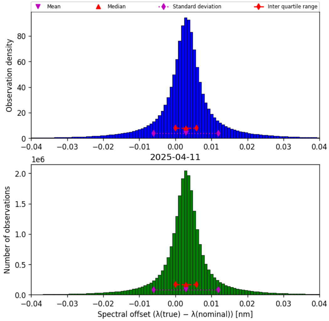
Figure 45: Histogram of “Spectral offset ( \lambda_{\text{true}} - \lambda_{\text{nominal}} )” for 2025-04-10 to 2025-04-12
