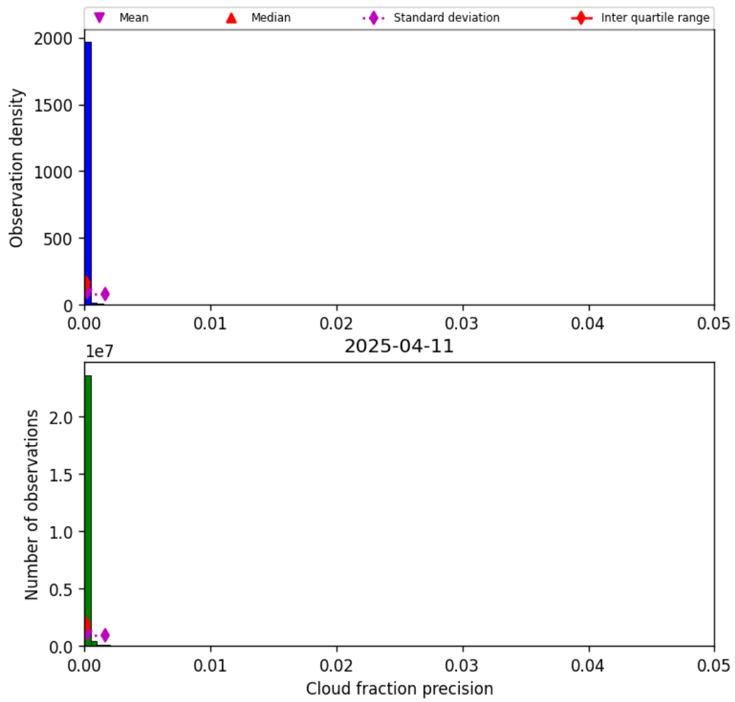
Figure 33: Histogram of “Cloud fraction precision” for 2025-04-10 to 2025-04-12
