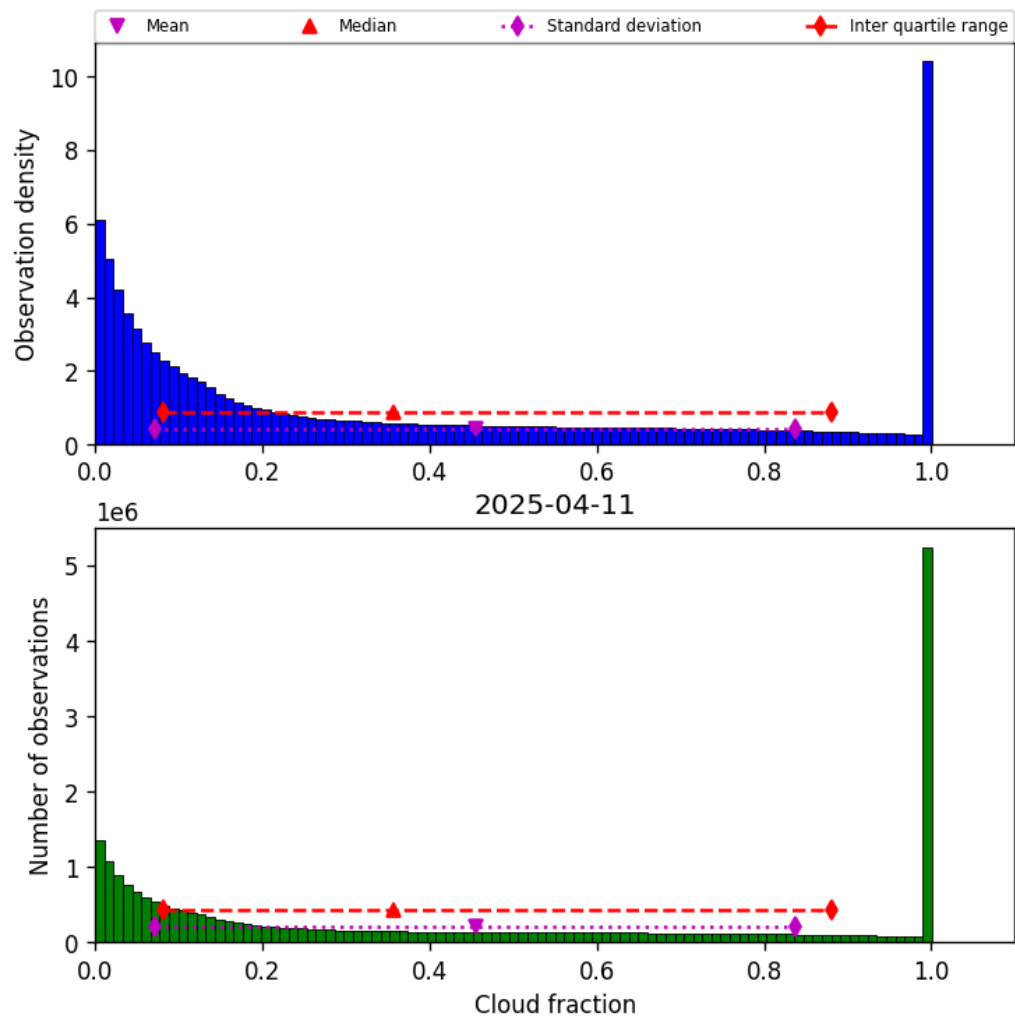
Figure 32: Histogram of “Cloud fraction” for 2025-04-10 to 2025-04-12
