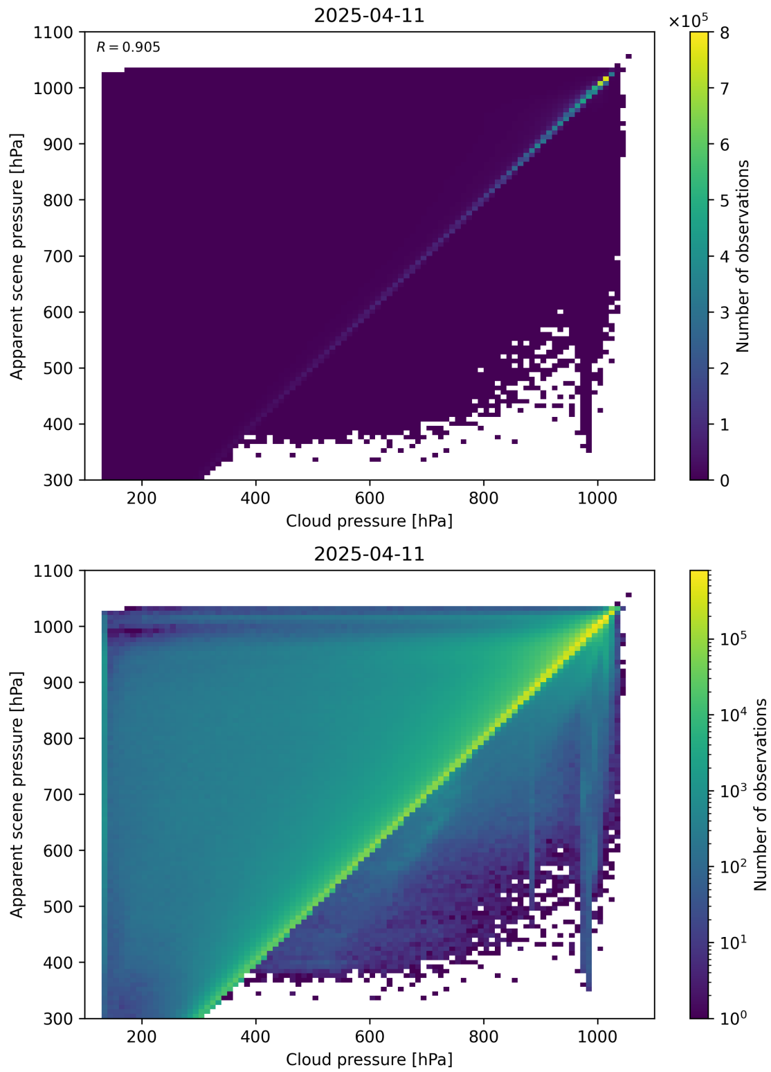
Figure 77: Scatter density plot of “Cloud pressure” against “Apparent scene pressure” for 2025-04-10 to 2025-04-12.
