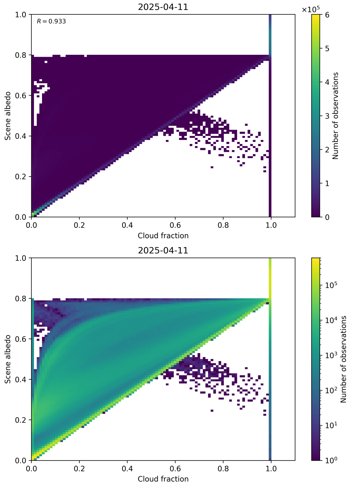
Figure 75: Scatter density plot of “Cloud fraction” against “Scene albedo” for 2025-04-10 to 2025-04-12.
