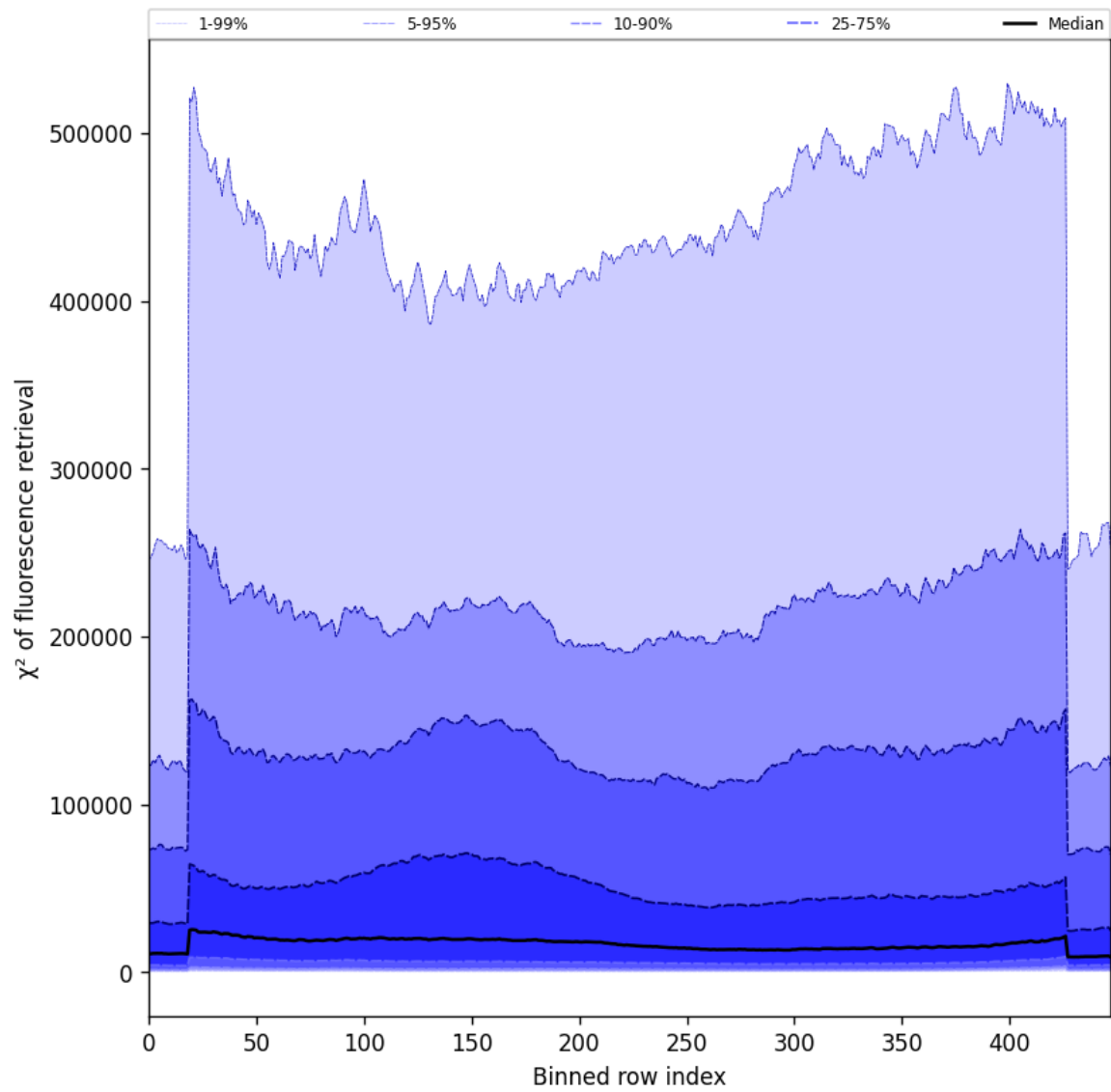
Figure 59: Along track statistics of “ \chi^2 of fluorescence retrieval” for 2025-04-10 to 2025-04-12
