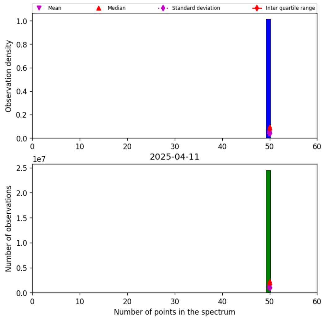
Figure 44: Histogram of “Number of points in the spectrum” for 2025-04-10 to 2025-04-12
