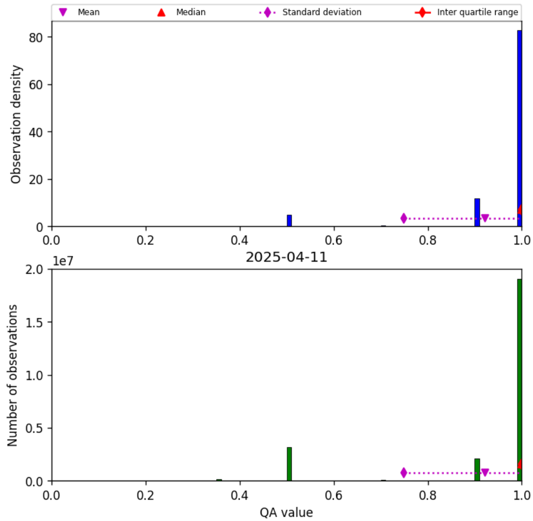
Figure 29: Histogram of “QA value” for 2025-04-10 to 2025-04-12
