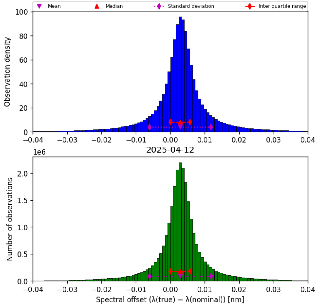
Figure 45: Histogram of “Spectral offset ( \lambda_{\text{true}} - \lambda_{\text{nominal}} )” for 2025-04-11 to 2025-04-13
