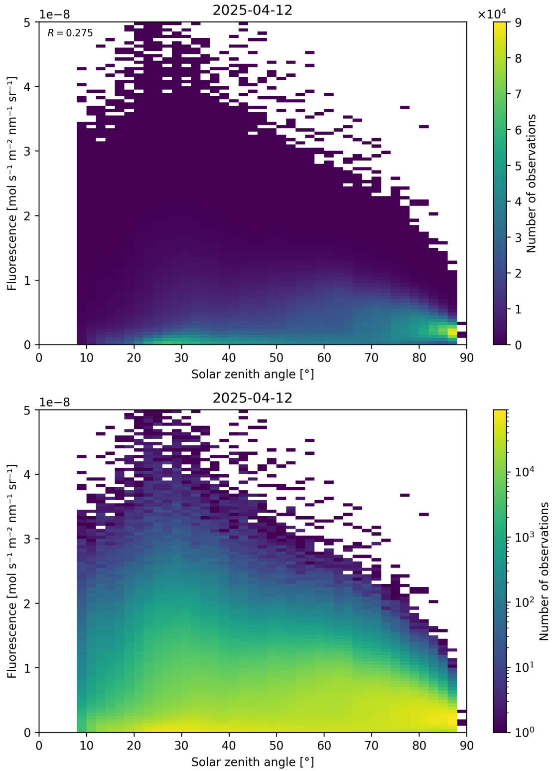
Figure 112: Scatter density plot of “Solar zenith angle” against “Fluorescence” for 2025-04-11 to 2025-04-13.
