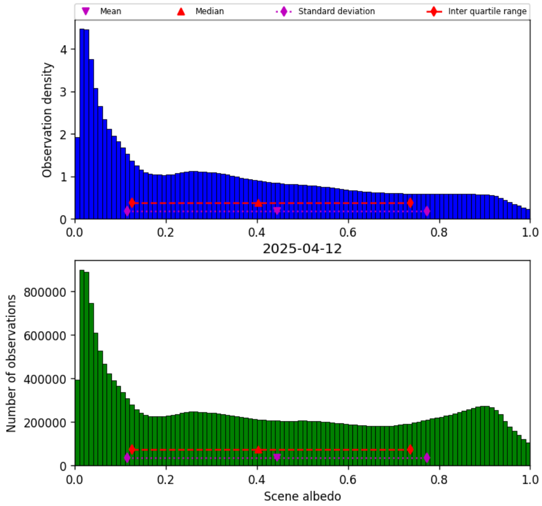
Figure 34: Histogram of “Scene albedo” for 2025-04-11 to 2025-04-13
