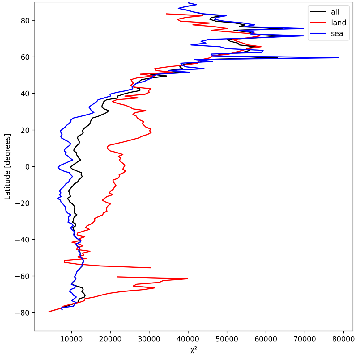
Figure 21: Zonal average of “ \chi^2 ” for 2025-04-11 to 2025-04-13.
