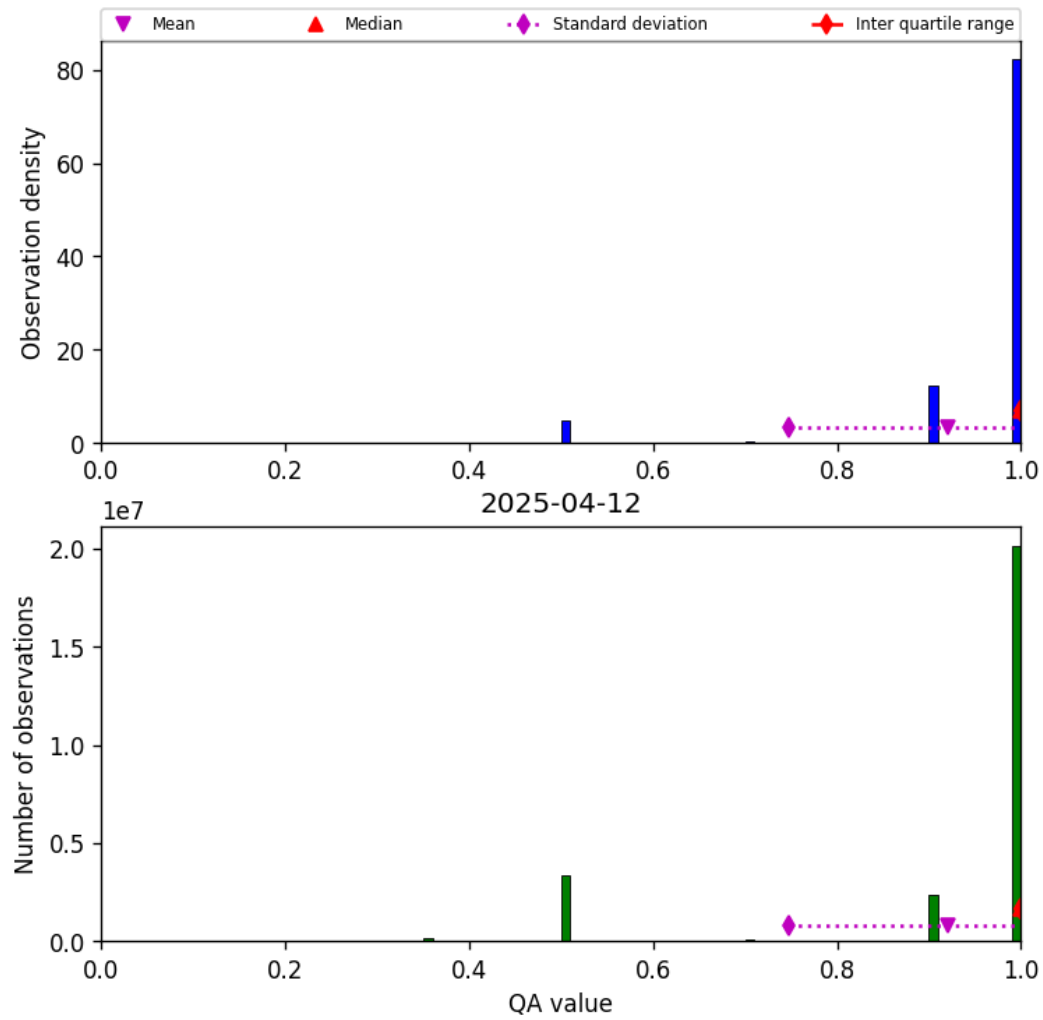
Figure 29: Histogram of “QA value” for 2025-04-11 to 2025-04-13
