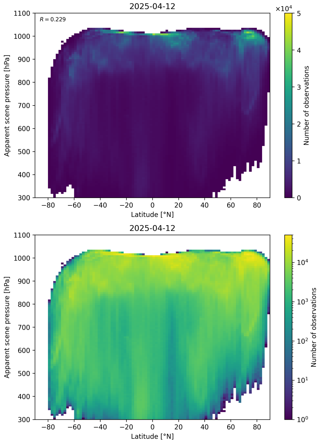
Figure 88: Scatter density plot of “Latitude” against “Apparent scene pressure” for 2025-04-11 to 2025-04-13.
