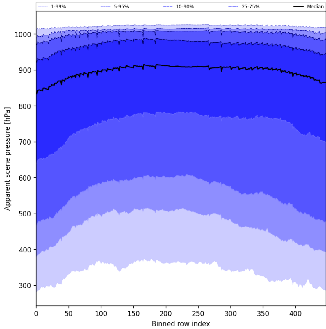
Figure 53: Along track statistics of “Apparent scene pressure” for 2025-04-11 to 2025-04-13
