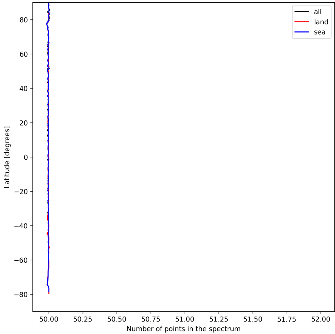
Figure 27: Zonal average of “Number of points in the spectrum” for 2025-04-11 to 2025-04-13.
