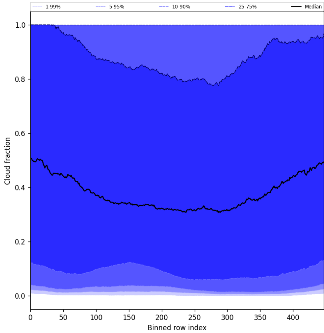
Figure 49: Along track statistics of “Cloud fraction” for 2025-04-11 to 2025-04-13
