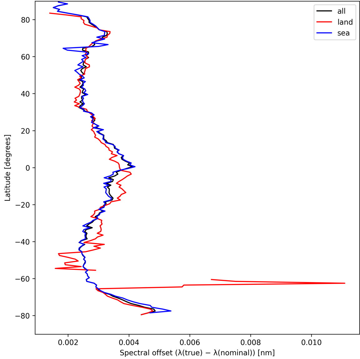
Figure 28: Zonal average of “Spectral offset ( \lambda_{\text{true}} - \lambda_{\text{nominal}} )” for 2025-04-11 to 2025-04-13.
