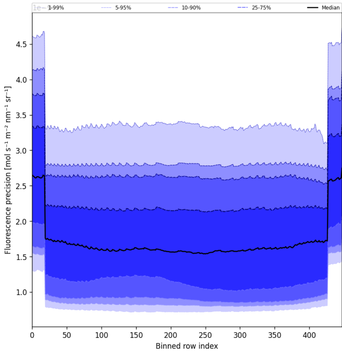
Figure 58: Along track statistics of “Fluorescence precision” for 2025-04-11 to 2025-04-13
