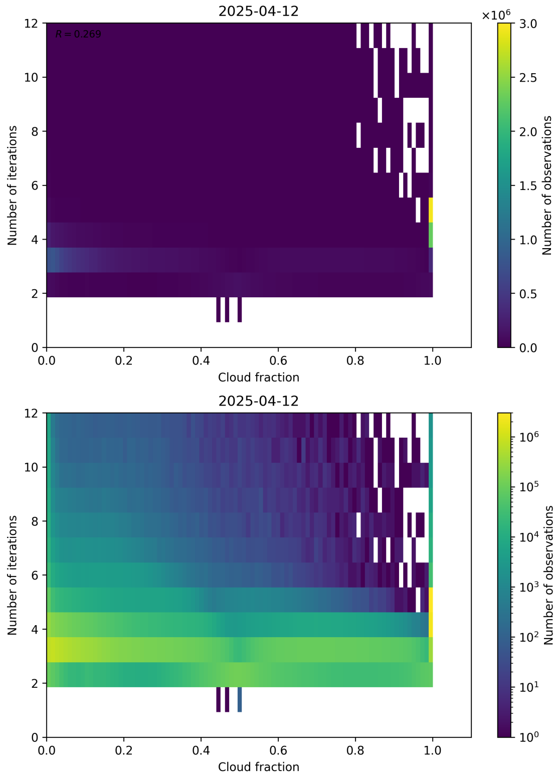
Figure 73: Scatter density plot of “Cloud fraction” against “Number of iterations” for 2025-04-11 to 2025-04-13.
