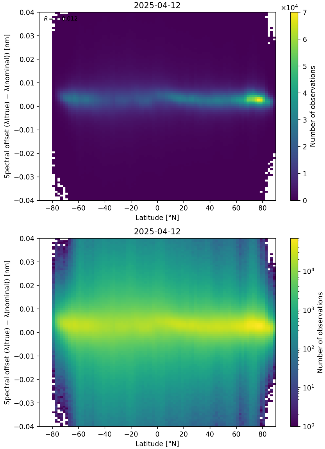
Figure 96: Scatter density plot of “Latitude” against “Spectral offset ( \lambda_{\text{true}} - \lambda_{\text{nominal}} )” for 2025-04-11 to 2025-04-13.
