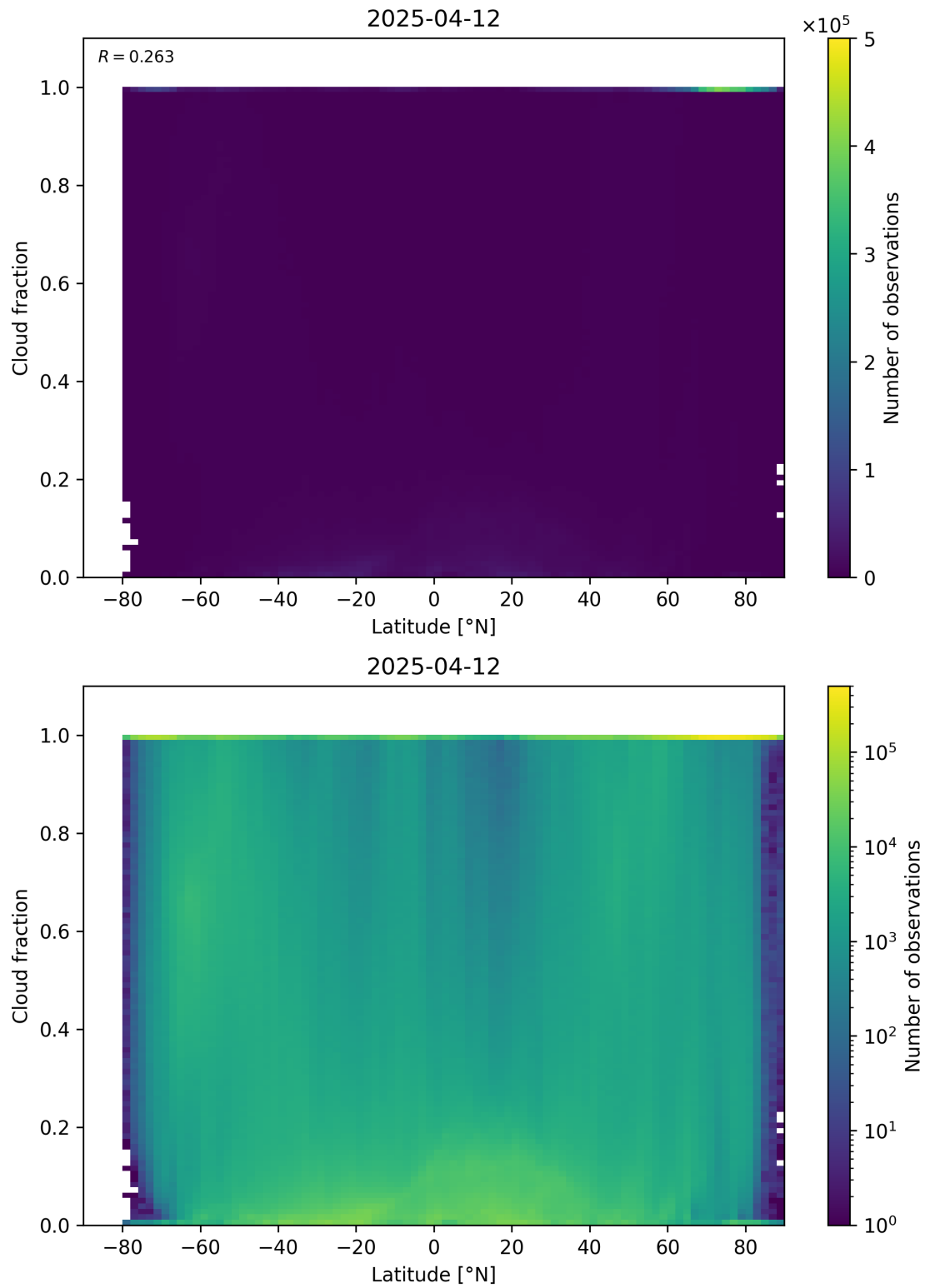
Figure 90: Scatter density plot of “Latitude” against “Cloud fraction” for 2025-04-11 to 2025-04-13.
