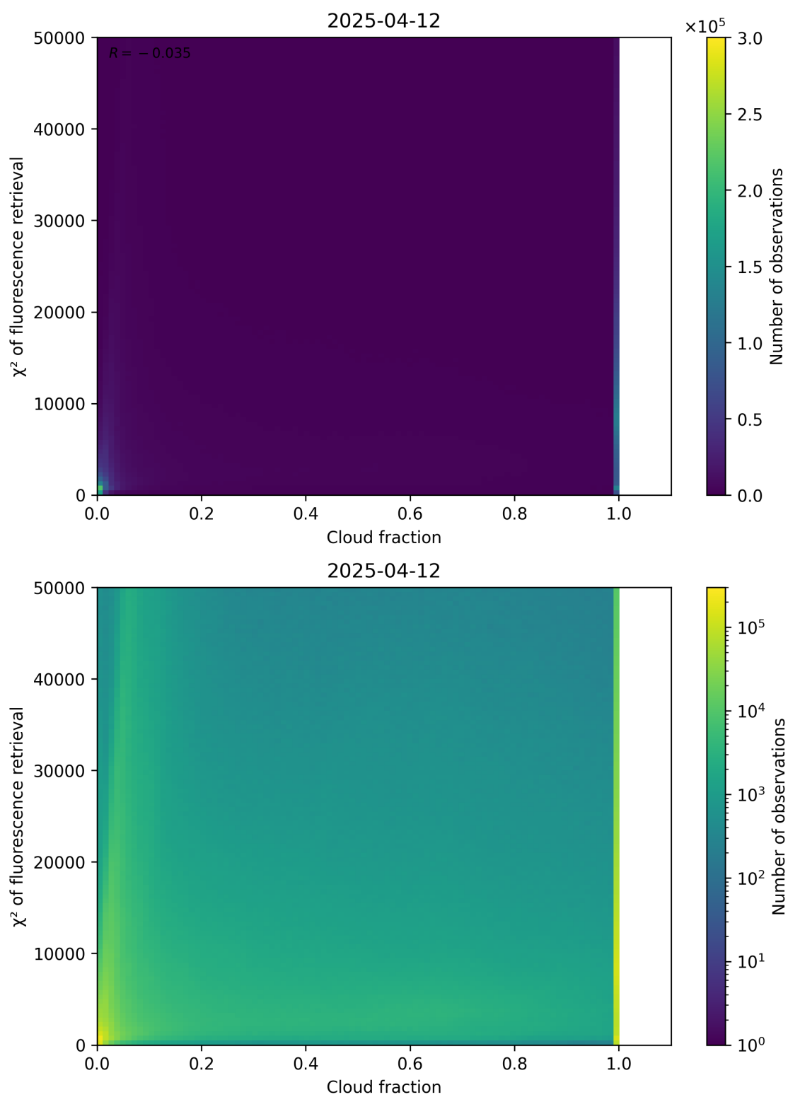
Figure 71: Scatter density plot of “Cloud fraction” against “ \chi^2 of fluorescence retrieval” for 2025-04-11 to 2025-04-13.
