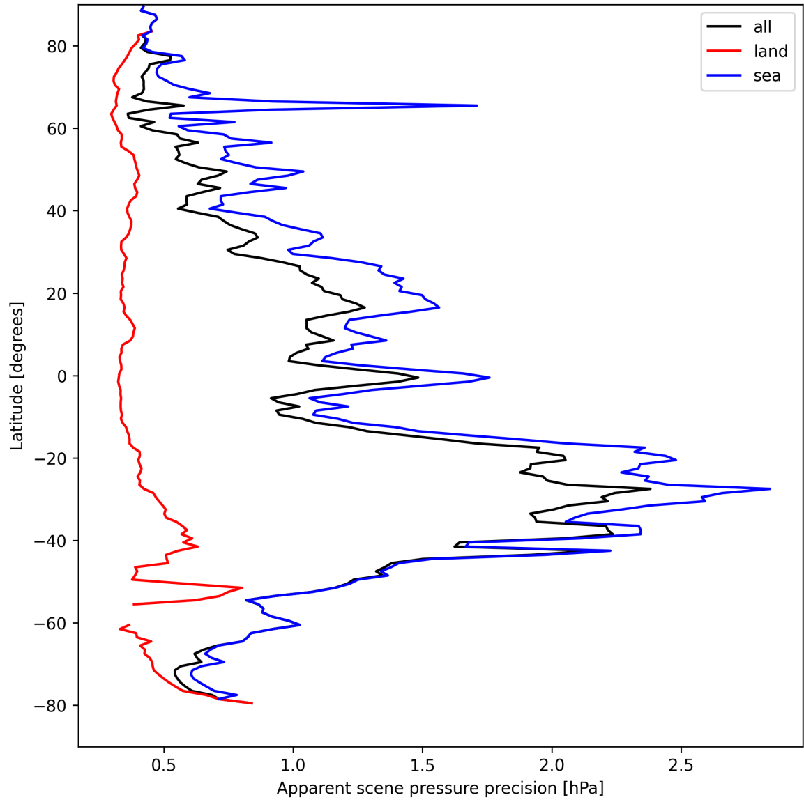
Figure 20: Zonal average of “Apparent scene pressure precision” for 2025-04-11 to 2025-04-13.
