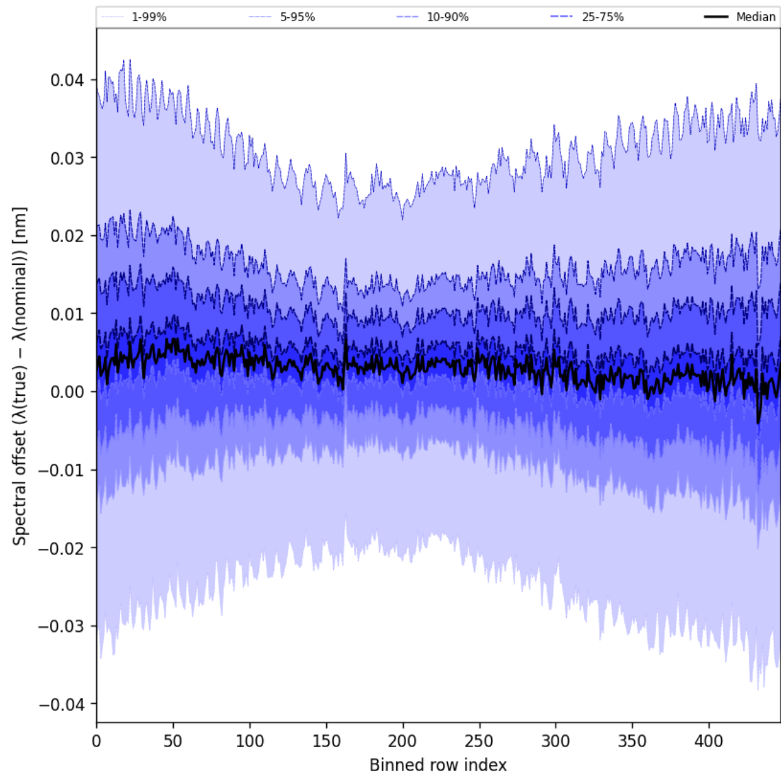
Figure 62: Along track statistics of “Spectral offset ( \lambda_{\text{true}} - \lambda_{\text{nominal}} )” for 2025-04-11 to 2025-04-13
