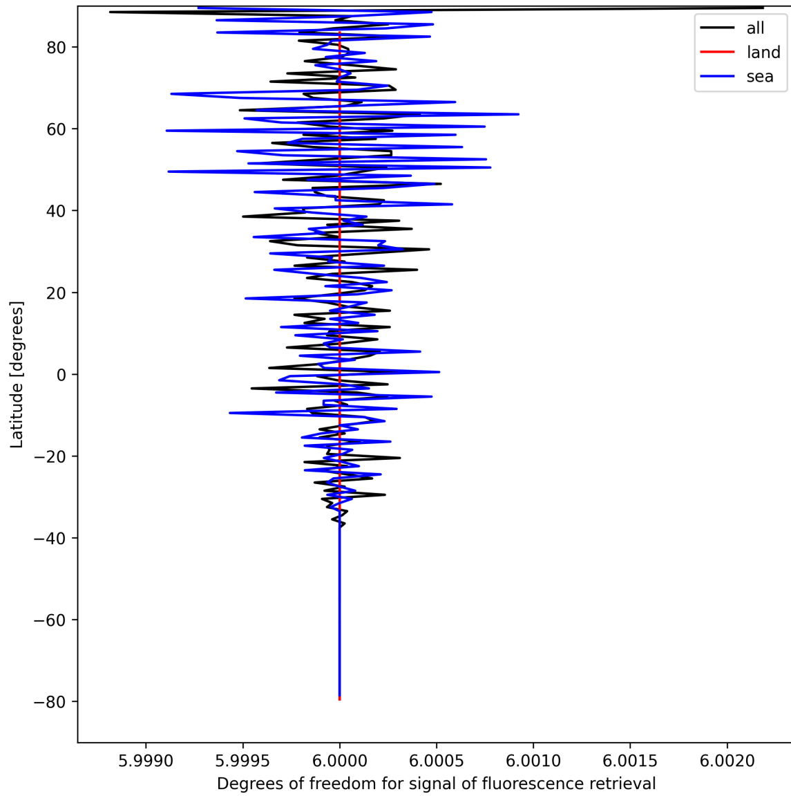
Figure 26: Zonal average of “Degrees of freedom for signal of fluorescence retrieval” for 2025-04-11 to 2025-04-13.
