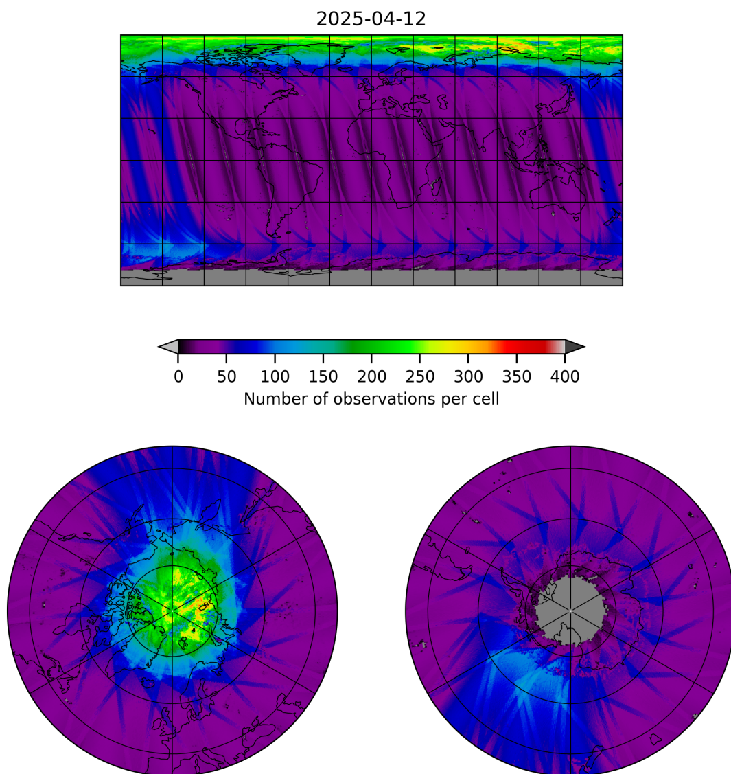
Figure 11: Map of the number of observations for 2025-04-11 to 2025-04-13
