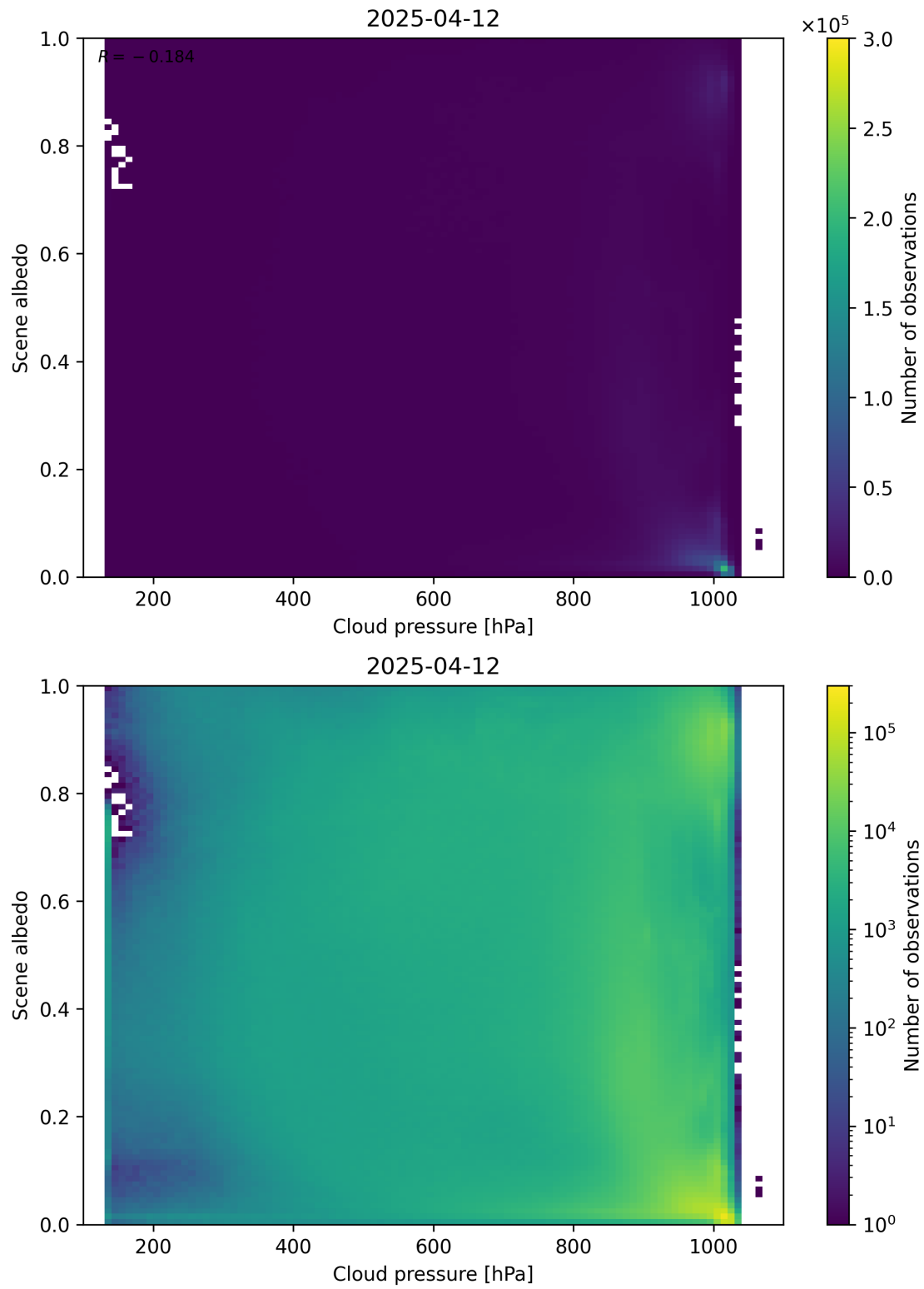
Figure 83: Scatter density plot of “Cloud pressure” against “Scene albedo” for 2025-04-11 to 2025-04-13.
