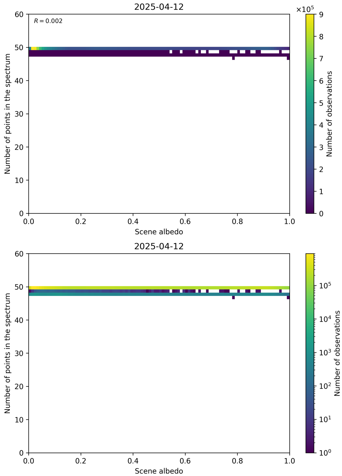
Figure 106: Scatter density plot of “Scene albedo” against “Number of points in the spectrum” for 2025-04-11 to 2025-04-13.
