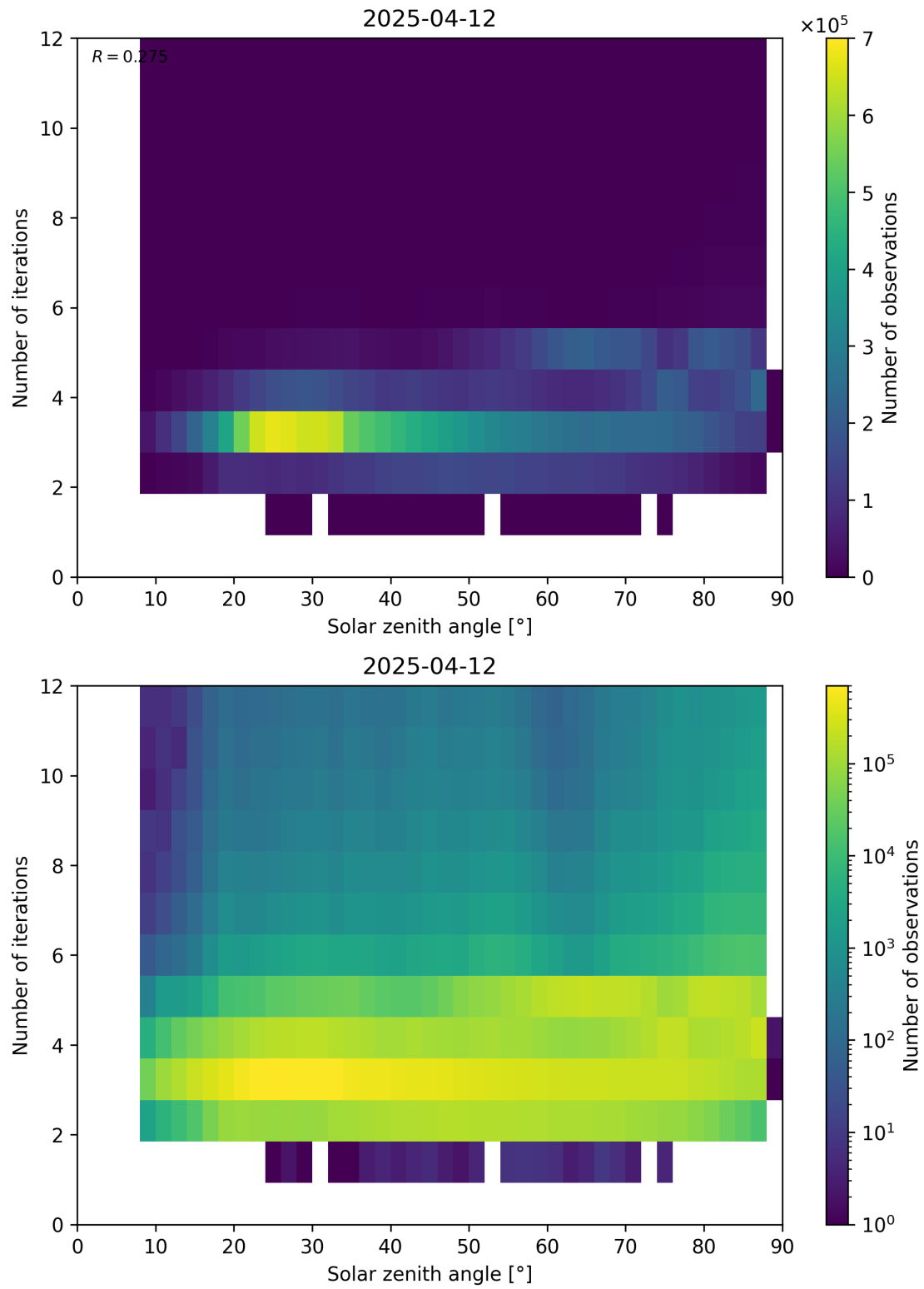
Figure 114: Scatter density plot of “Solar zenith angle” against “Number of iterations” for 2025-04-11 to 2025-04-13.
