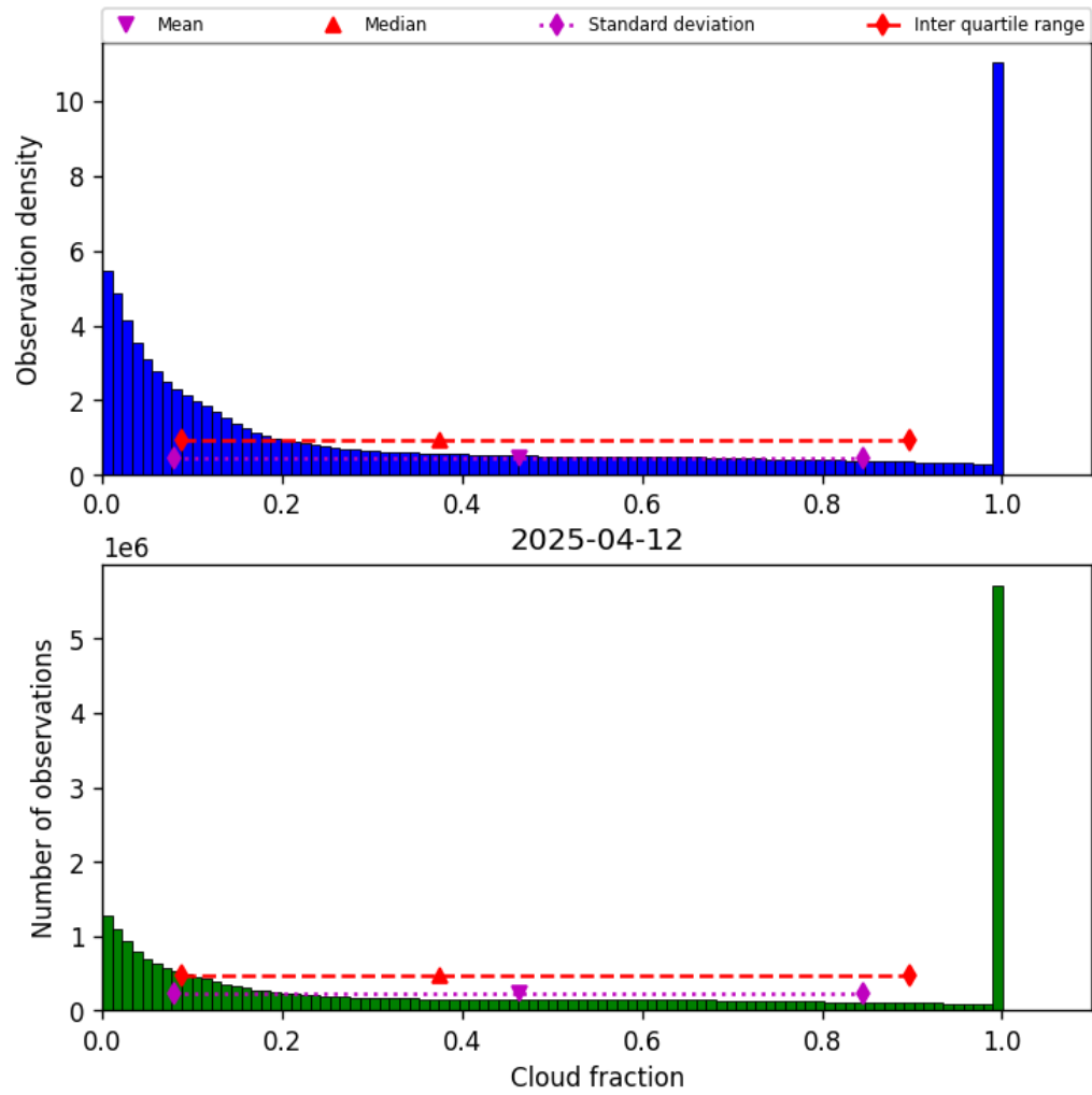
Figure 32: Histogram of “Cloud fraction” for 2025-04-11 to 2025-04-13
