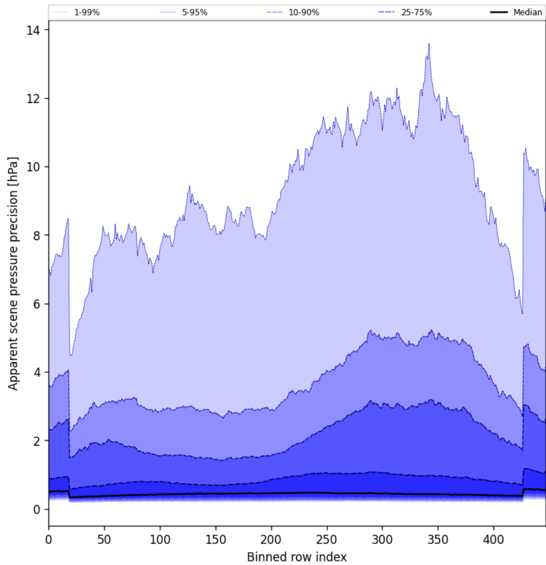
Figure 54: Along track statistics of “Apparent scene pressure precision” for 2025-04-11 to 2025-04-13
