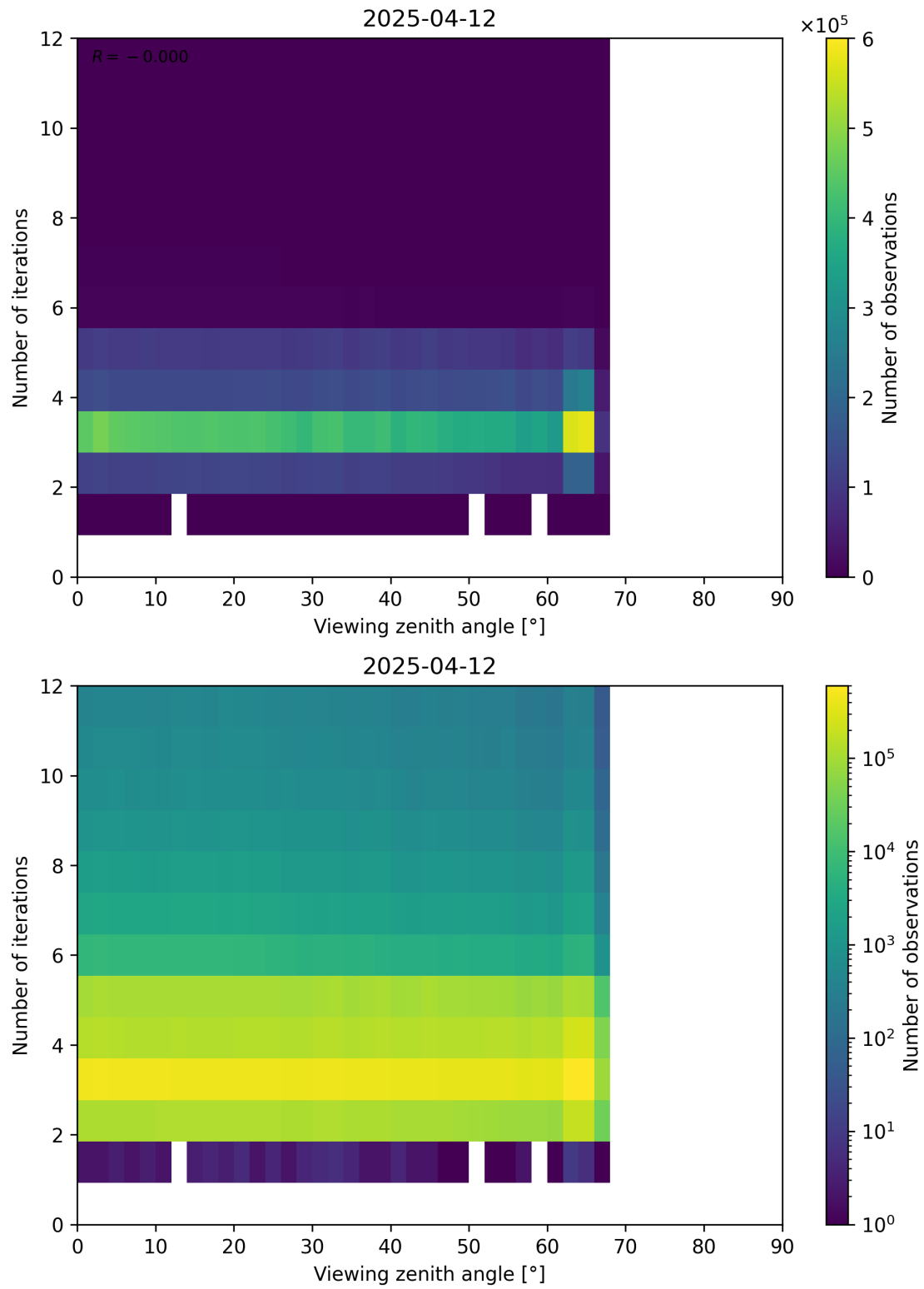
Figure 124: Scatter density plot of “Viewing zenith angle” against “Number of iterations” for 2025-04-11 to 2025-04-13.
