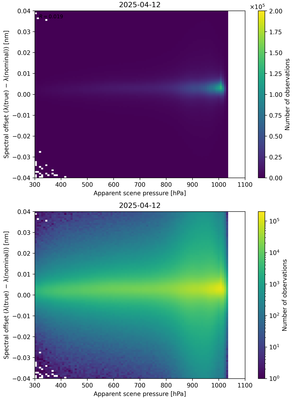
Figure 67: Scatter density plot of “Apparent scene pressure” against “Spectral offset ( \lambda_{\text{true}} - \lambda_{\text{nominal}} )” for 2025-04-11 to 2025-04-13.
