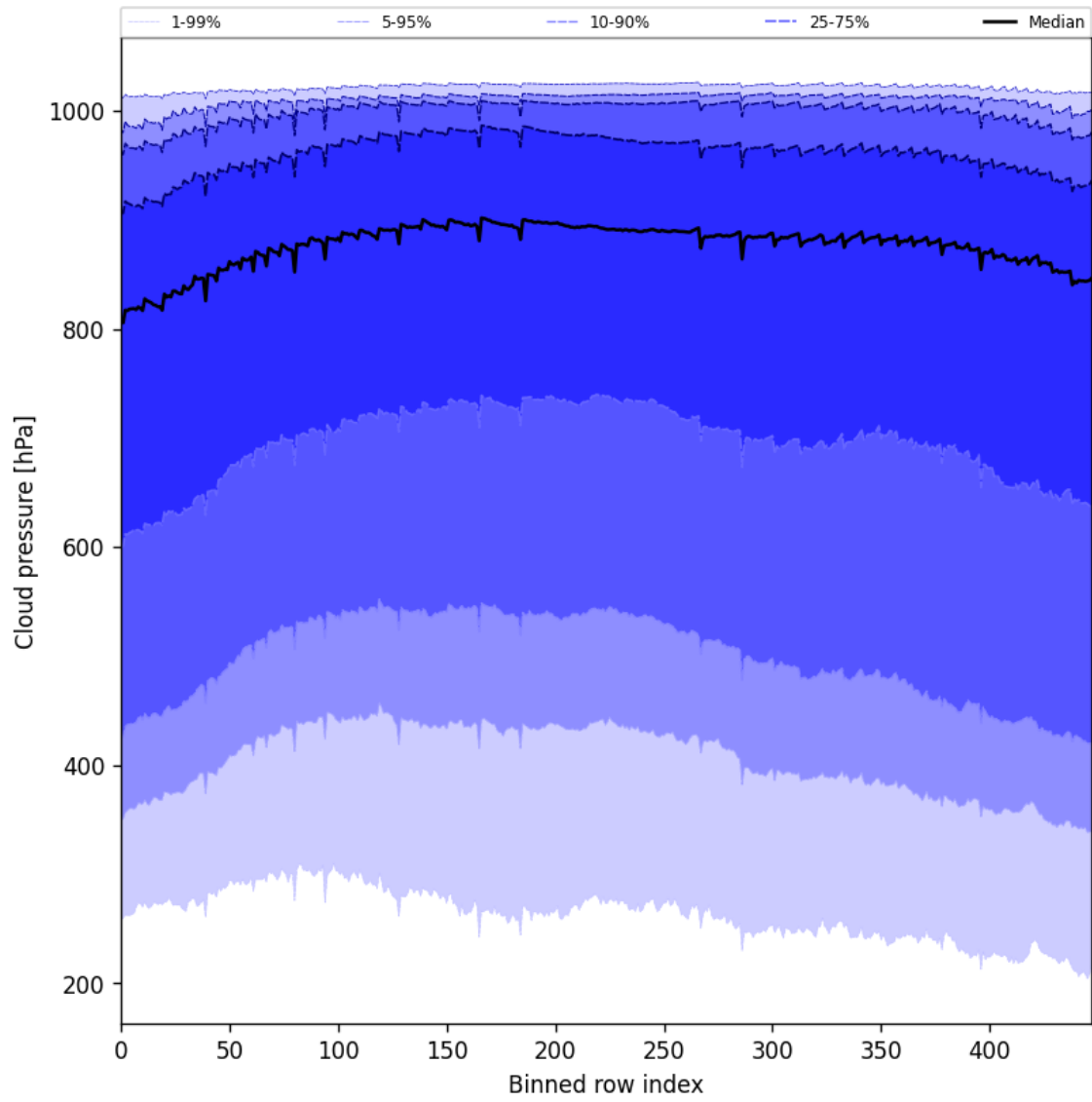
Figure 47: Along track statistics of “Cloud pressure” for 2025-04-11 to 2025-04-13
