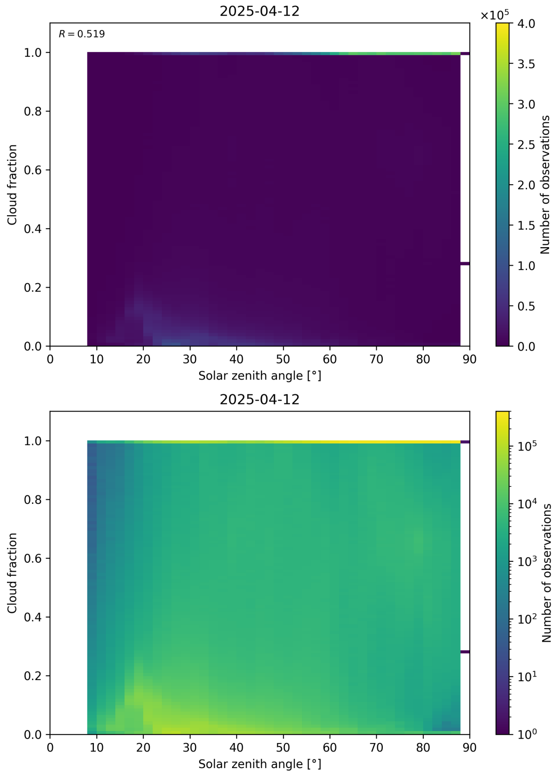
Figure 110: Scatter density plot of “Solar zenith angle” against “Cloud fraction” for 2025-04-11 to 2025-04-13.
