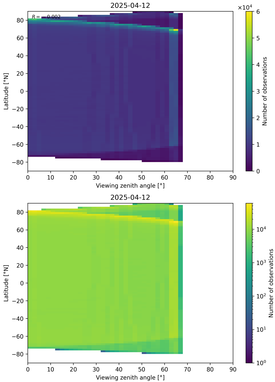
Figure 123: Scatter density plot of “Viewing zenith angle” against “Latitude” for 2025-04-11 to 2025-04-13.
