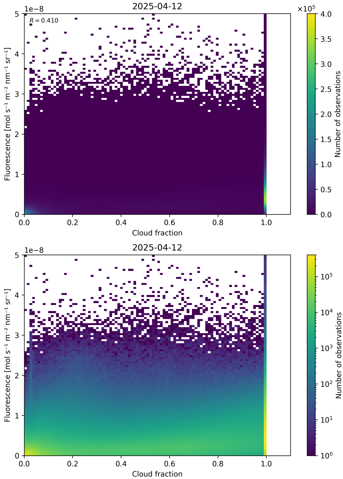
Figure 72: Scatter density plot of “Cloud fraction” against “Fluorescence” for 2025-04-11 to 2025-04-13.
