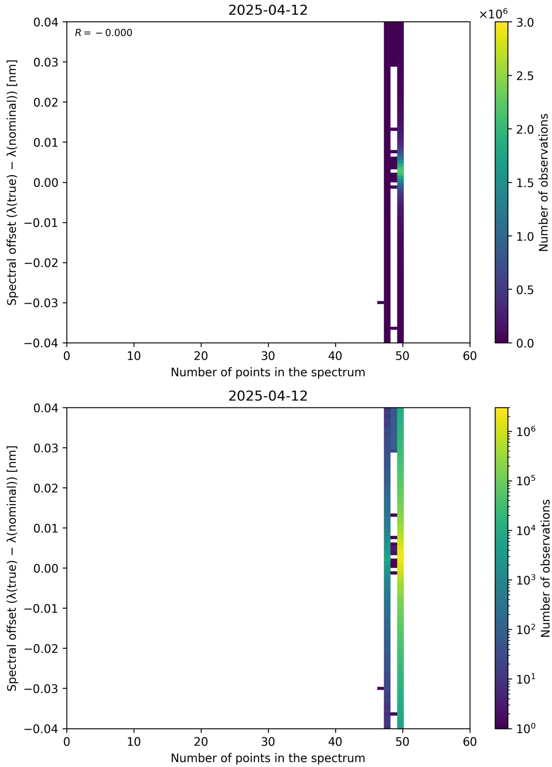
Figure 101: Scatter density plot of “Number of points in the spectrum” against “Spectral offset ( \lambda_{\text{true}} - \lambda_{\text{nominal}} )” for 2025-04-11 to 2025-04-13.
