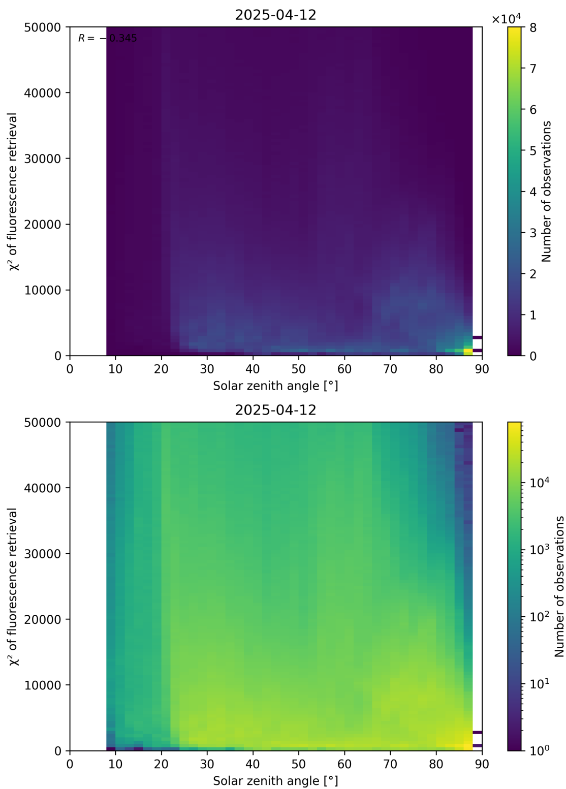
Figure 109: Scatter density plot of “Solar zenith angle” against “ \chi^2 of fluorescence retrieval” for 2025-04-11 to 2025-04-13.
