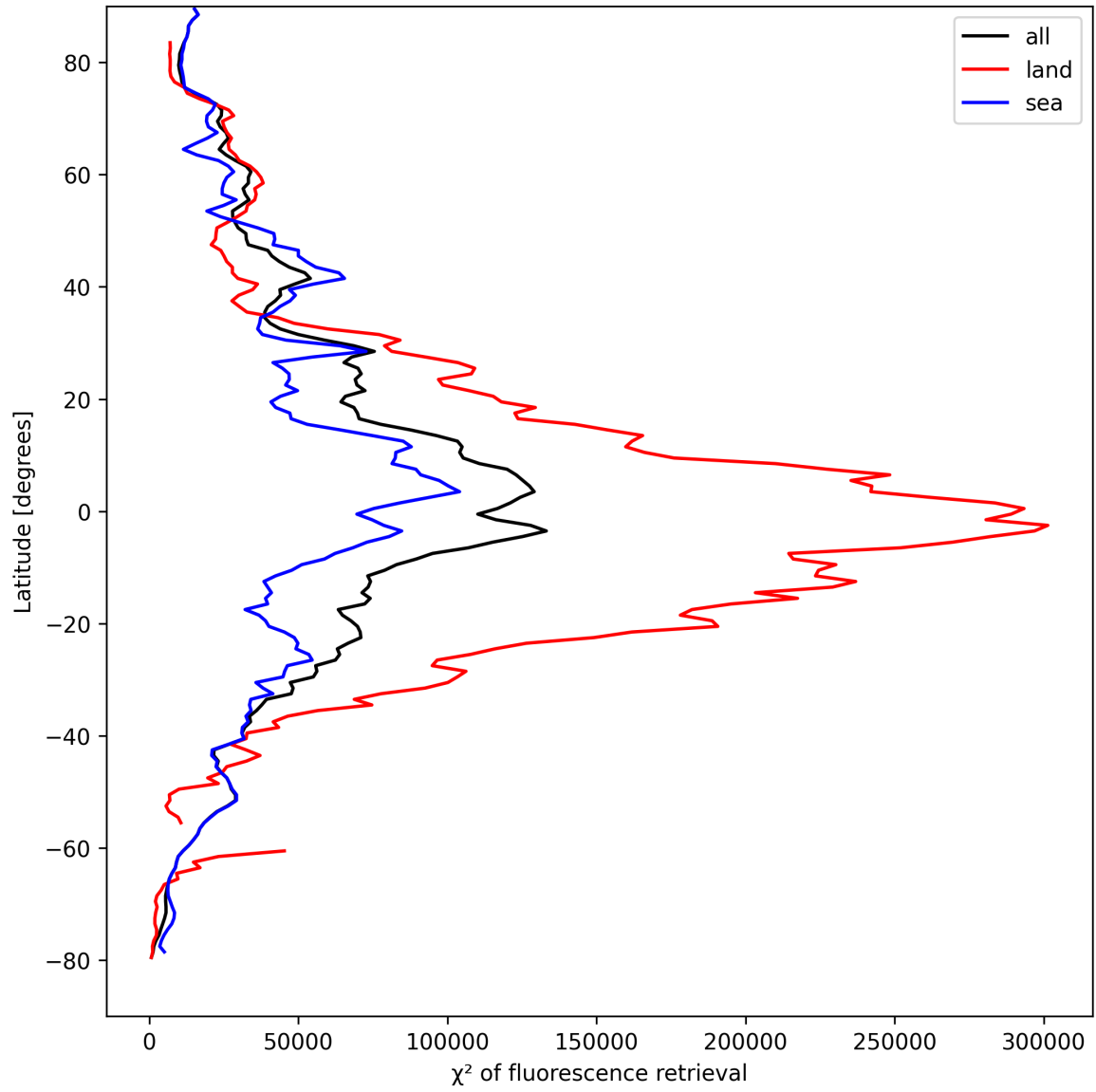
Figure 25: Zonal average of “ \chi^2 of fluorescence retrieval” for 2025-04-11 to 2025-04-13.
