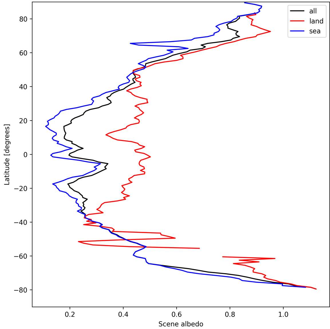
Figure 17: Zonal average of “Scene albedo” for 2025-04-11 to 2025-04-13.
