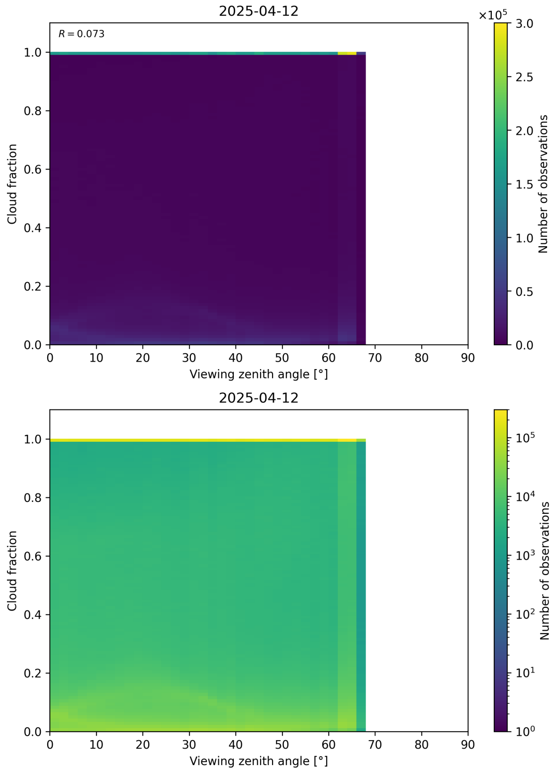
Figure 120: Scatter density plot of “Viewing zenith angle” against “Cloud fraction” for 2025-04-11 to 2025-04-13.
