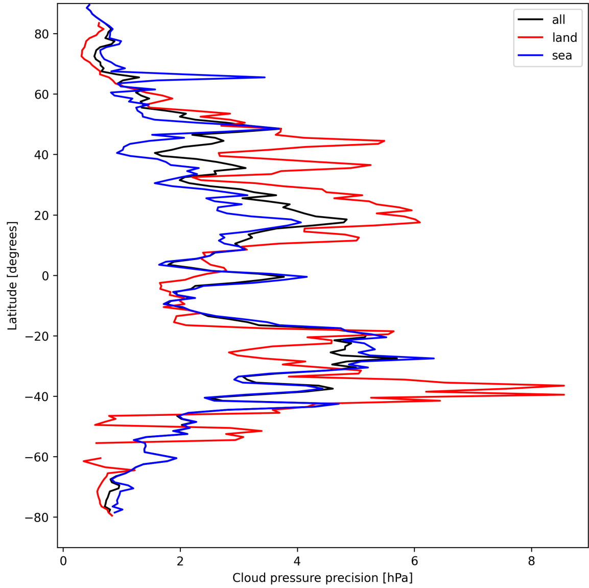
Figure 14: Zonal average of “Cloud pressure precision” for 2025-04-11 to 2025-04-13.
