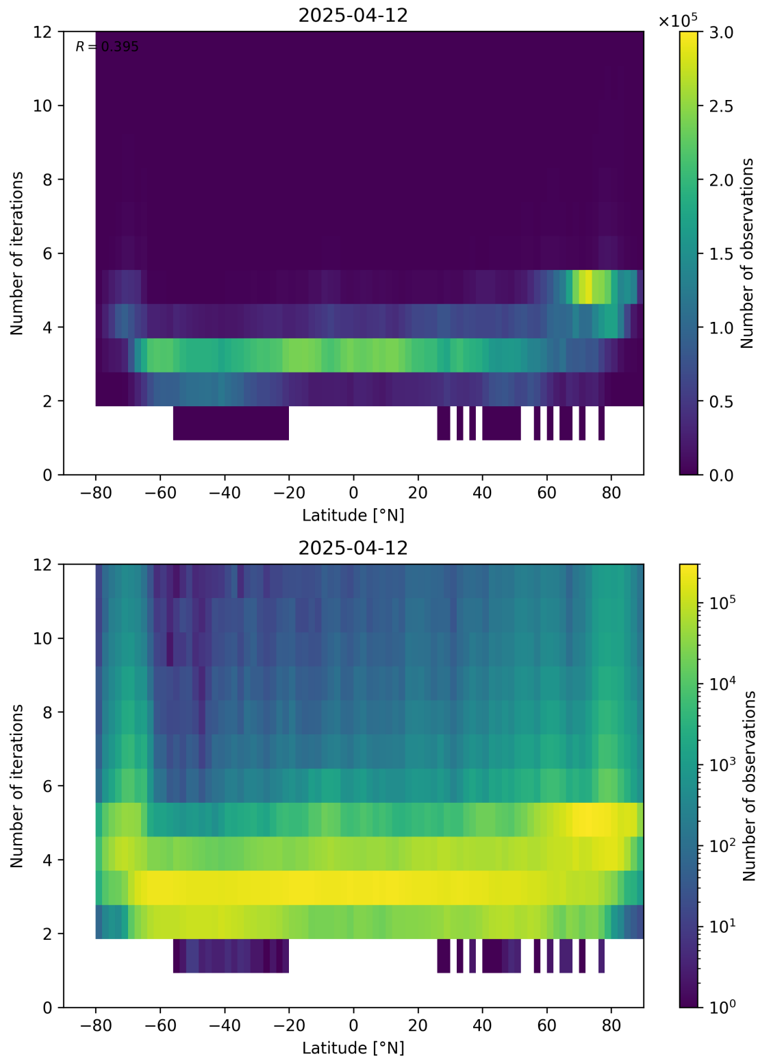
Figure 93: Scatter density plot of “Latitude” against “Number of iterations” for 2025-04-11 to 2025-04-13.
