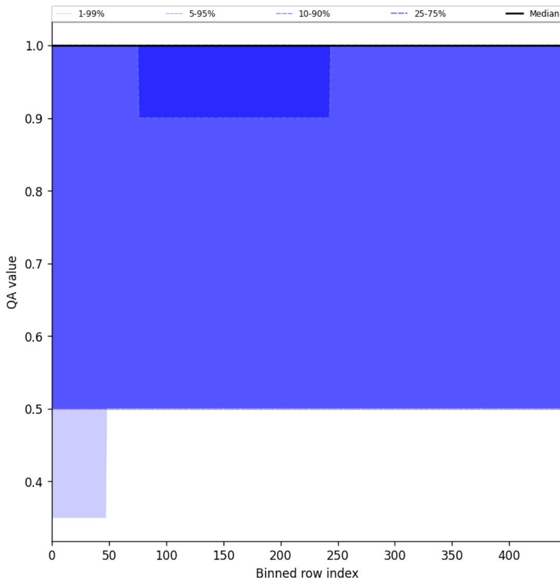
Figure 46: Along track statistics of “QA value” for 2025-04-11 to 2025-04-13
