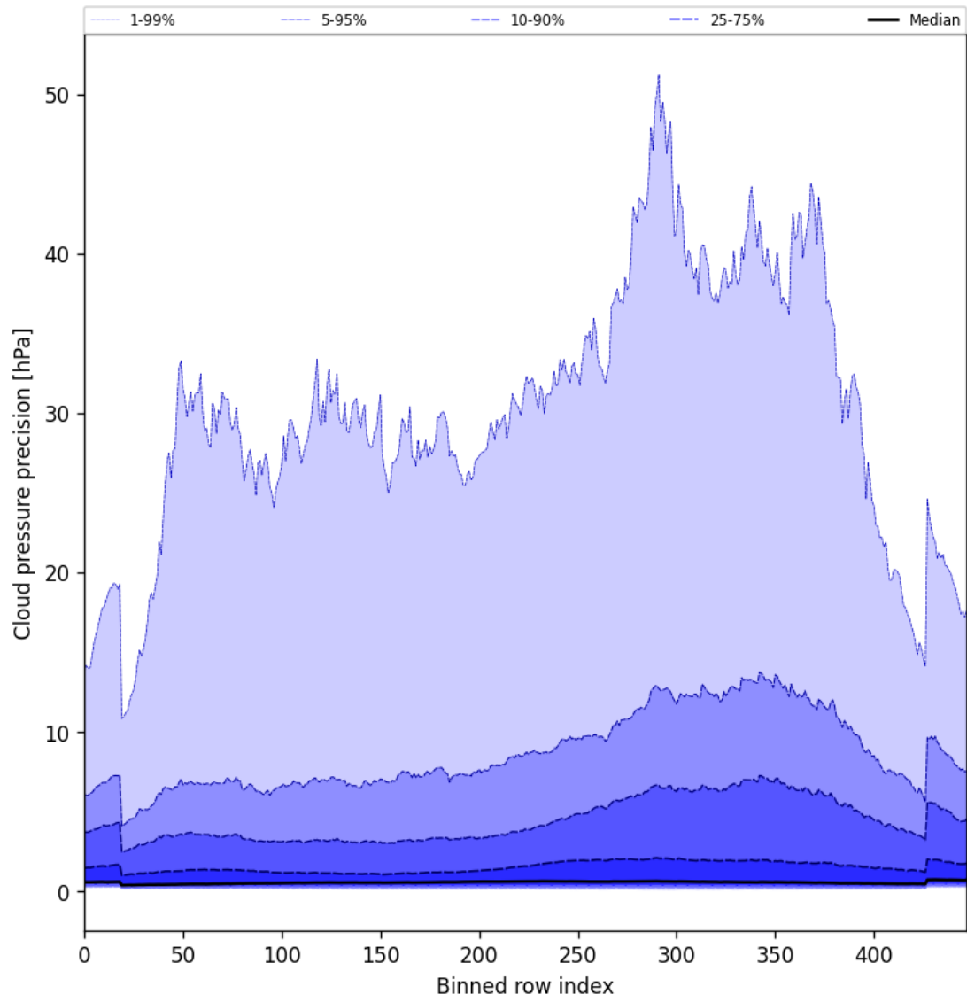
Figure 48: Along track statistics of “Cloud pressure precision” for 2025-04-11 to 2025-04-13
