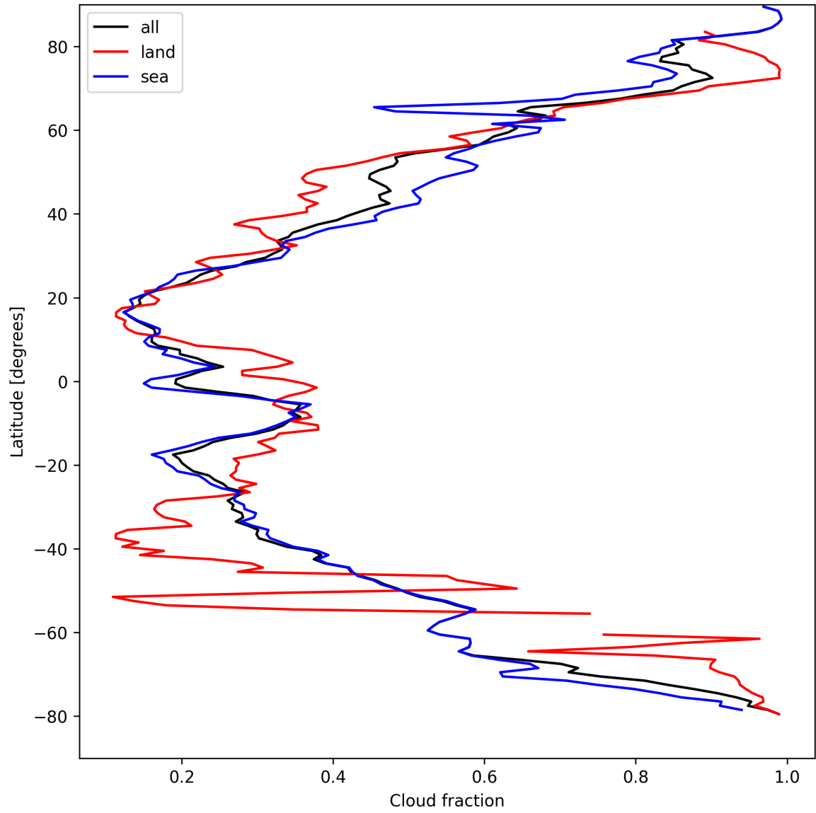
Figure 15: Zonal average of “Cloud fraction” for 2025-04-11 to 2025-04-13.
