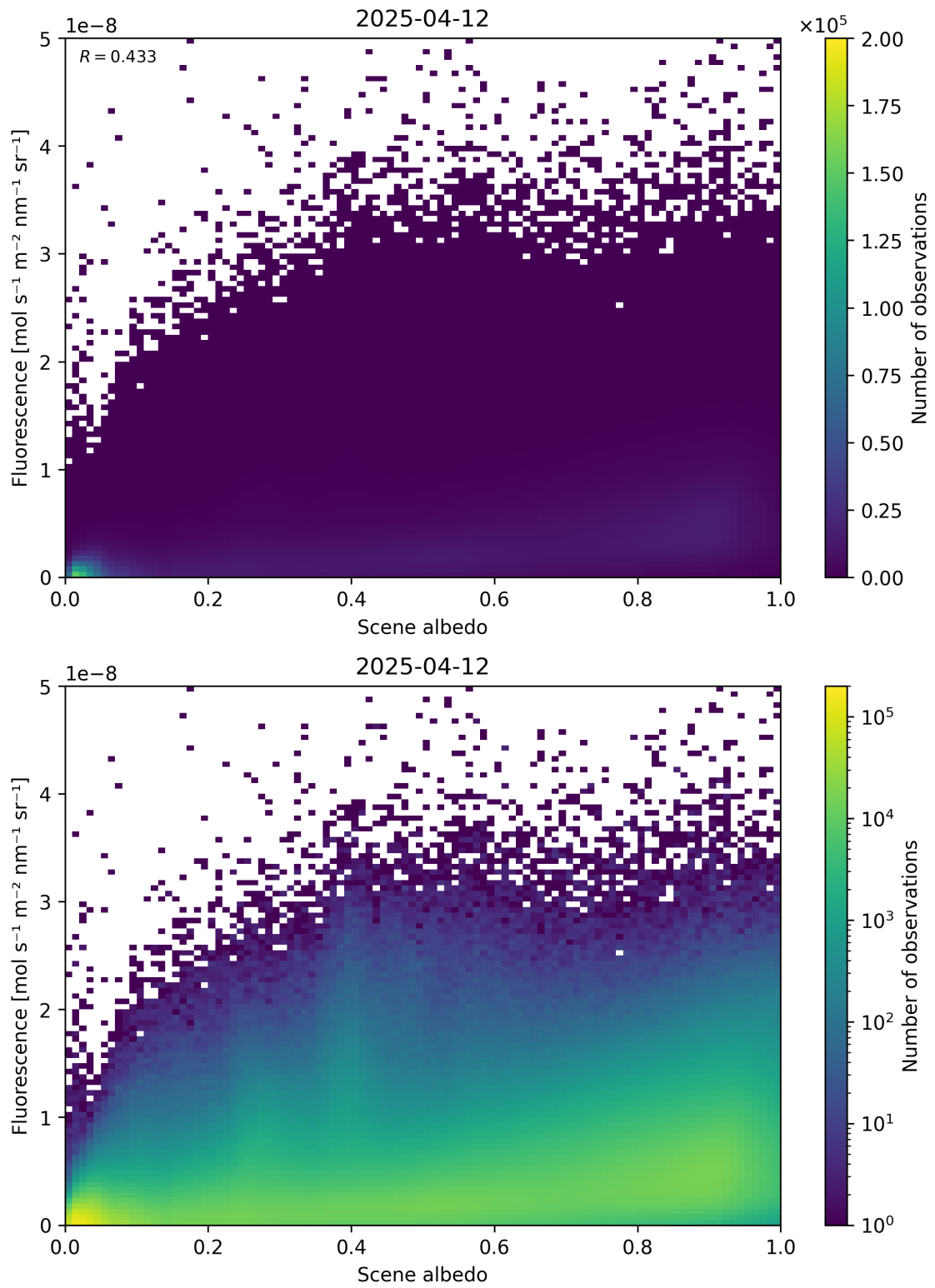
Figure 104: Scatter density plot of “Scene albedo” against “Fluorescence” for 2025-04-11 to 2025-04-13.
