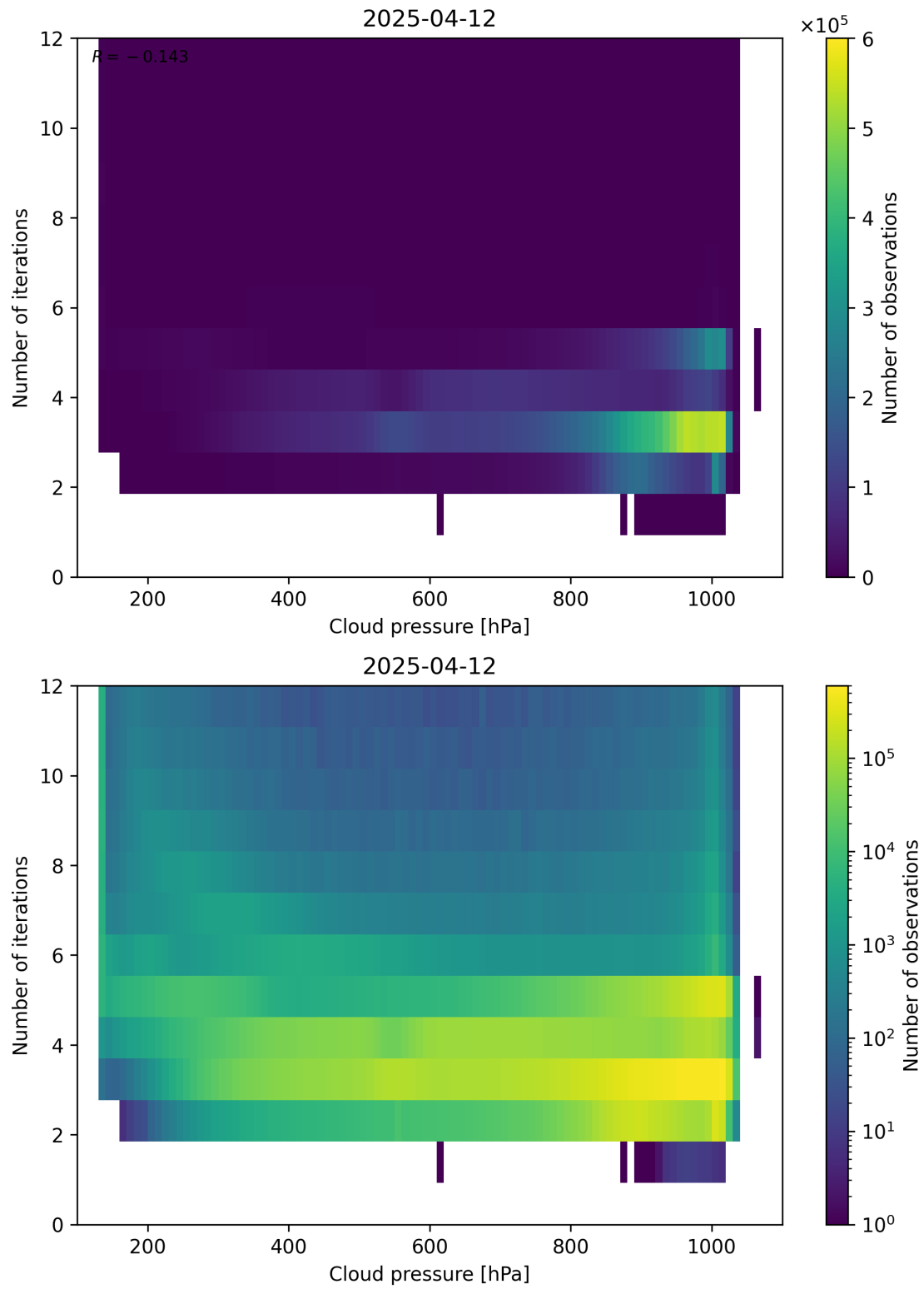
Figure 81: Scatter density plot of “Cloud pressure” against “Number of iterations” for 2025-04-11 to 2025-04-13.
