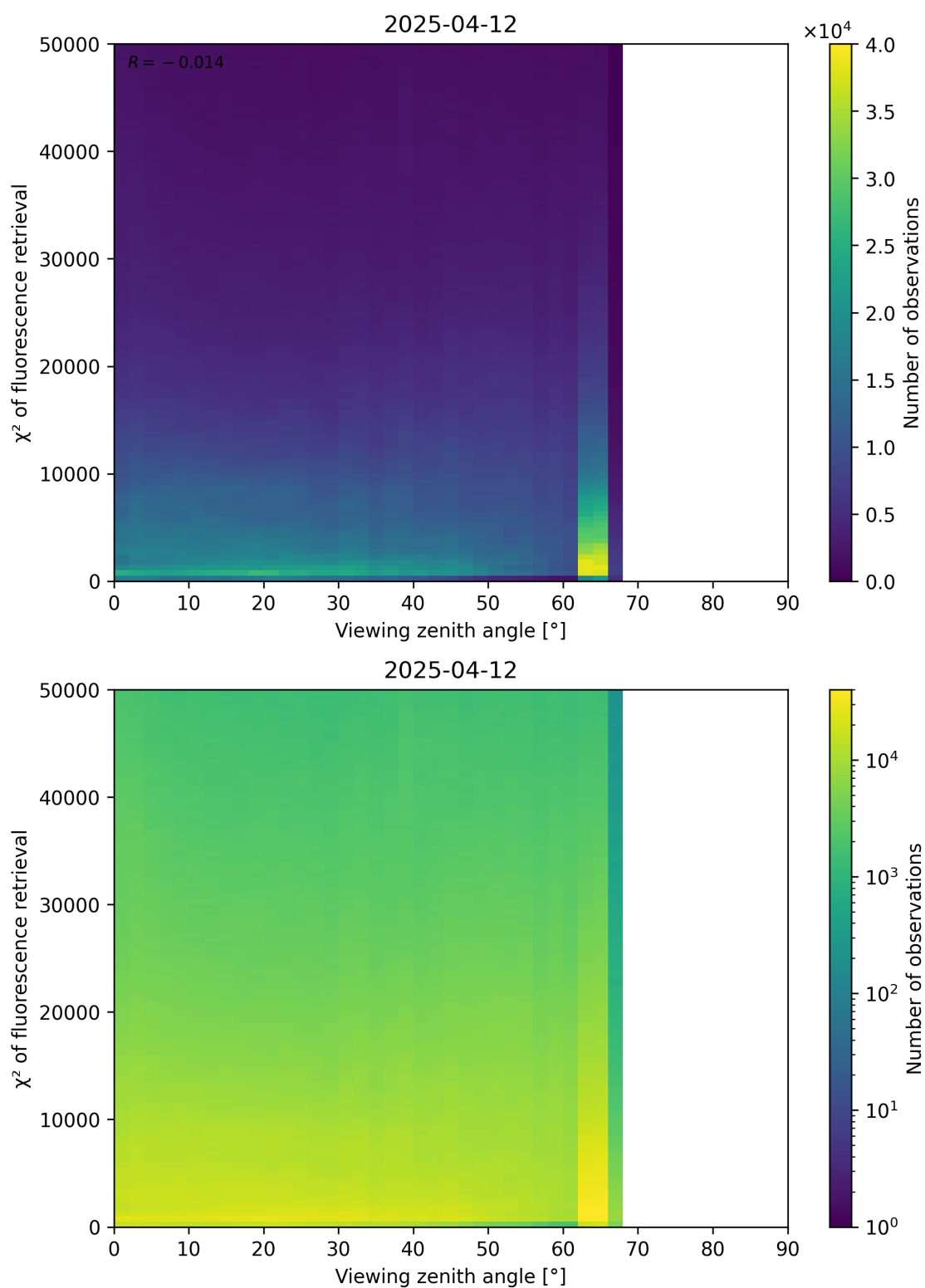
Figure 119: Scatter density plot of “Viewing zenith angle” against “ \chi^2 of fluorescence retrieval” for 2025-04-11 to 2025-04-13.
