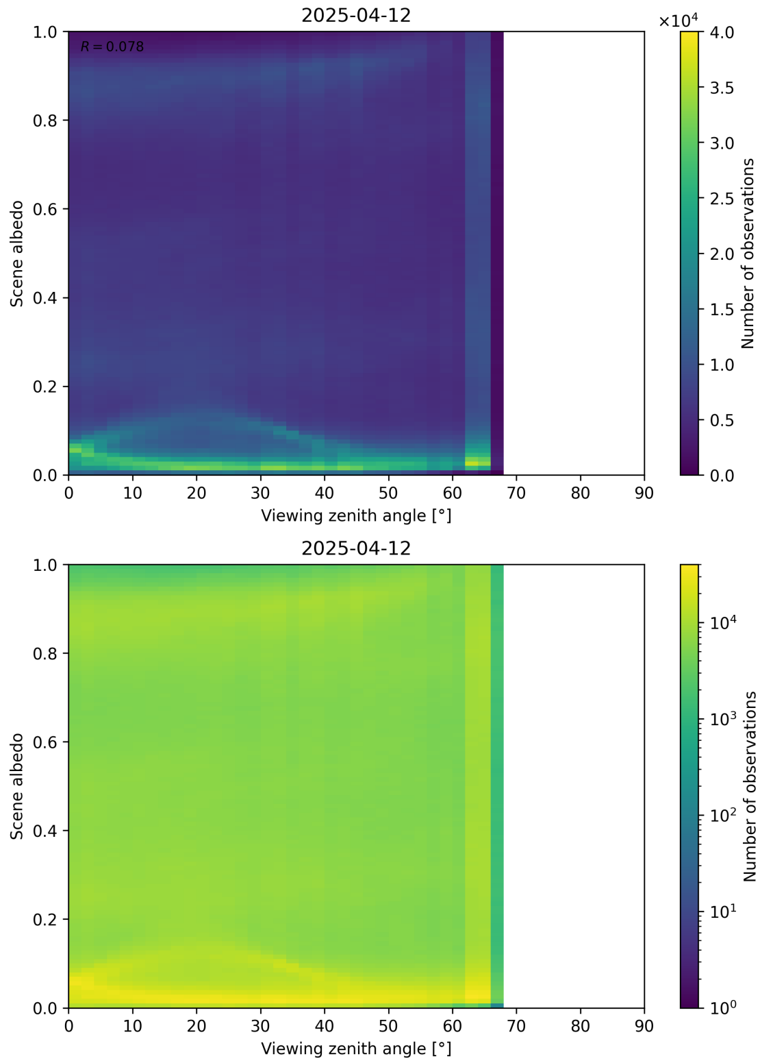
Figure 126: Scatter density plot of “Viewing zenith angle” against “Scene albedo” for 2025-04-11 to 2025-04-13.
