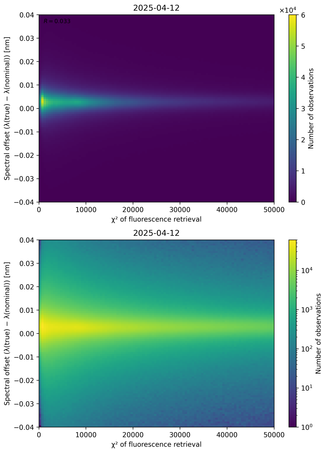
Figure 69: Scatter density plot of “ \chi^2 of fluorescence retrieval” against “Spectral offset ( \lambda_{\text{true}} - \lambda_{\text{nominal}} )” for 2025-04-11 to 2025-04-13.
