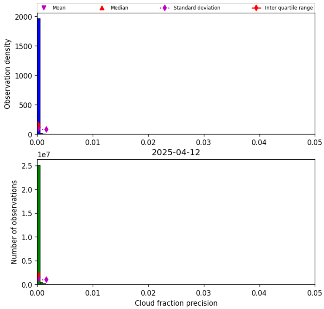
Figure 33: Histogram of “Cloud fraction precision” for 2025-04-11 to 2025-04-13
