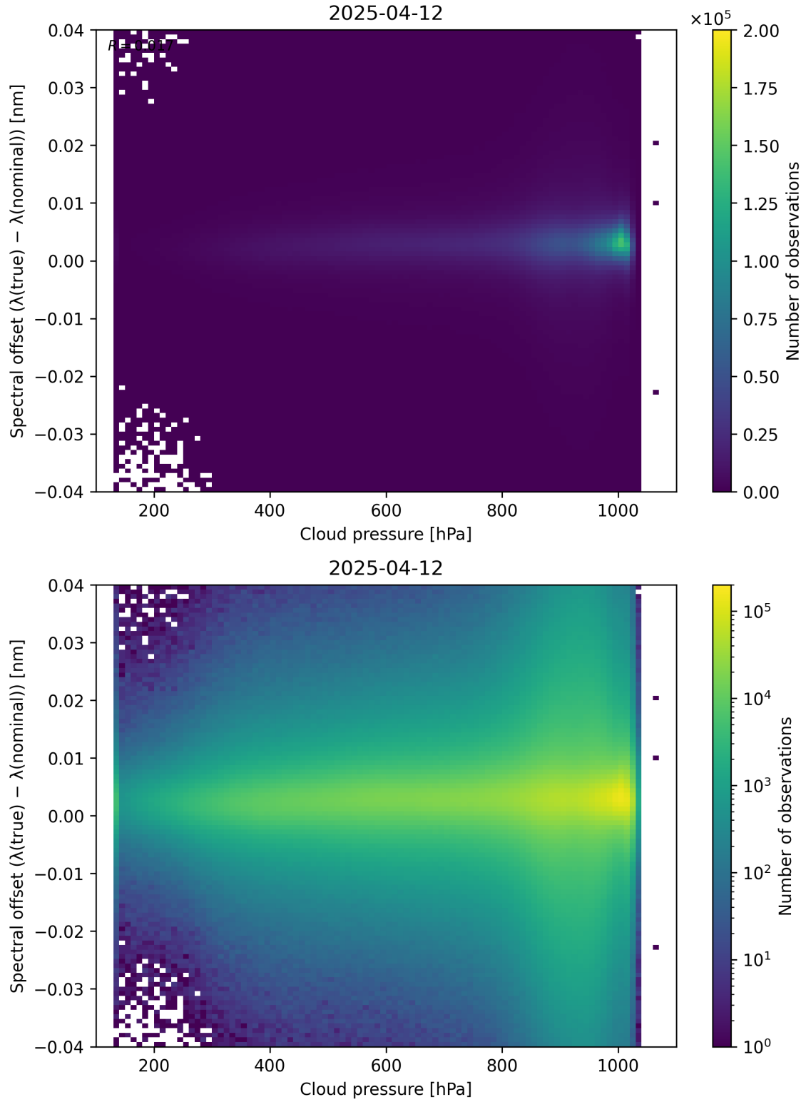
Figure 84: Scatter density plot of “Cloud pressure” against “Spectral offset ( \lambda_{\text{true}} - \lambda_{\text{nominal}} )” for 2025-04-11 to 2025-04-13.
