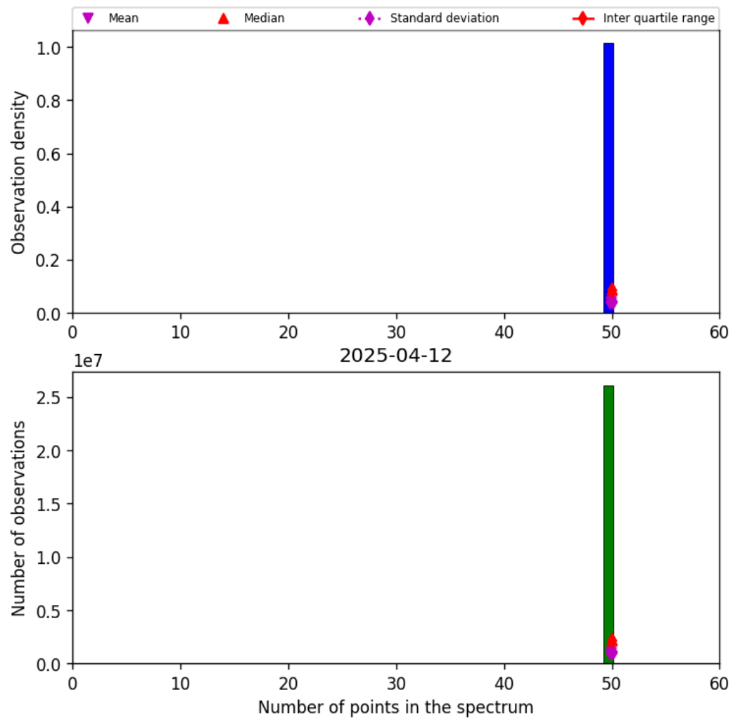
Figure 44: Histogram of “Number of points in the spectrum” for 2025-04-11 to 2025-04-13
