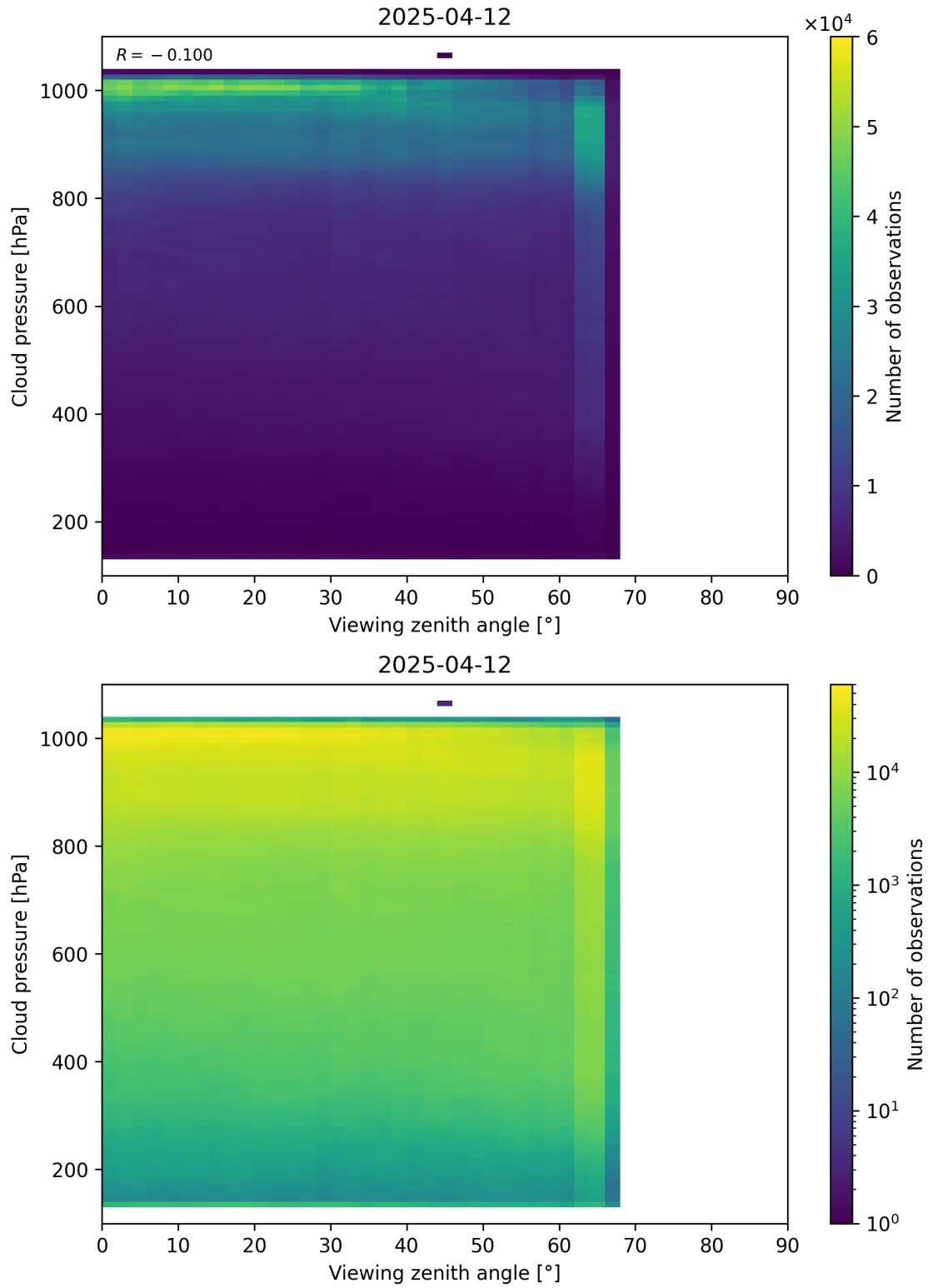
Figure 121: Scatter density plot of “Viewing zenith angle” against “Cloud pressure” for 2025-04-11 to 2025-04-13.
