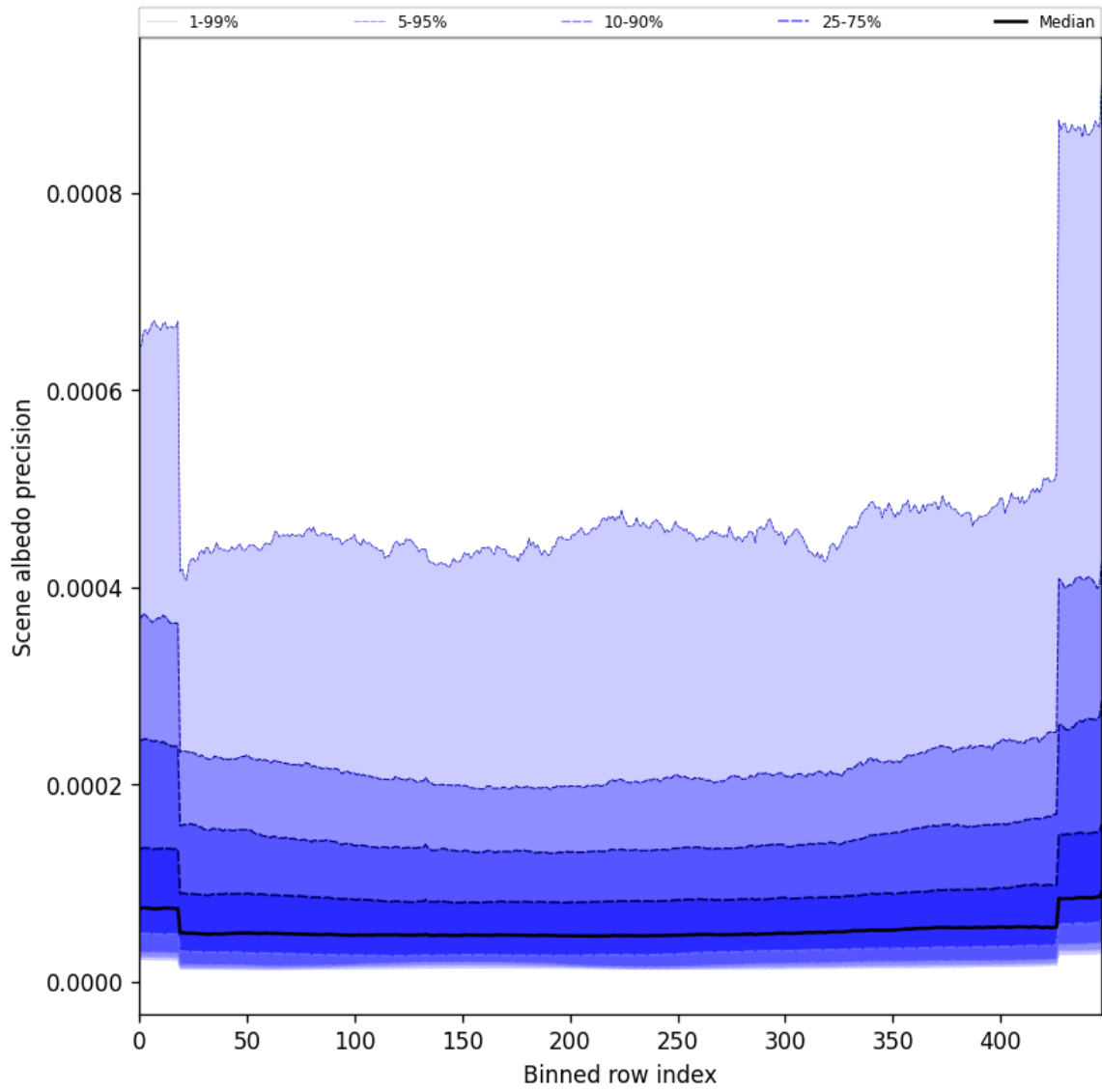
Figure 52: Along track statistics of “Scene albedo precision” for 2025-04-11 to 2025-04-13
