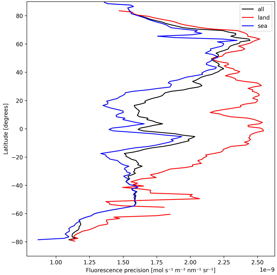
Figure 24: Zonal average of “Fluorescence precision” for 2025-04-11 to 2025-04-13.
