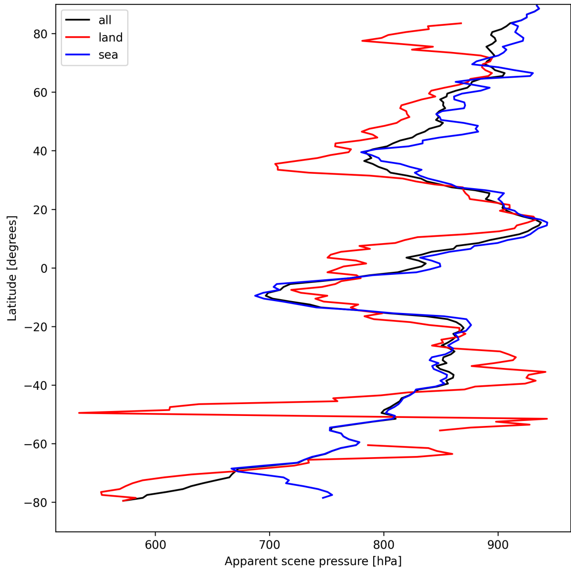
Figure 19: Zonal average of “Apparent scene pressure” for 2025-04-11 to 2025-04-13.
