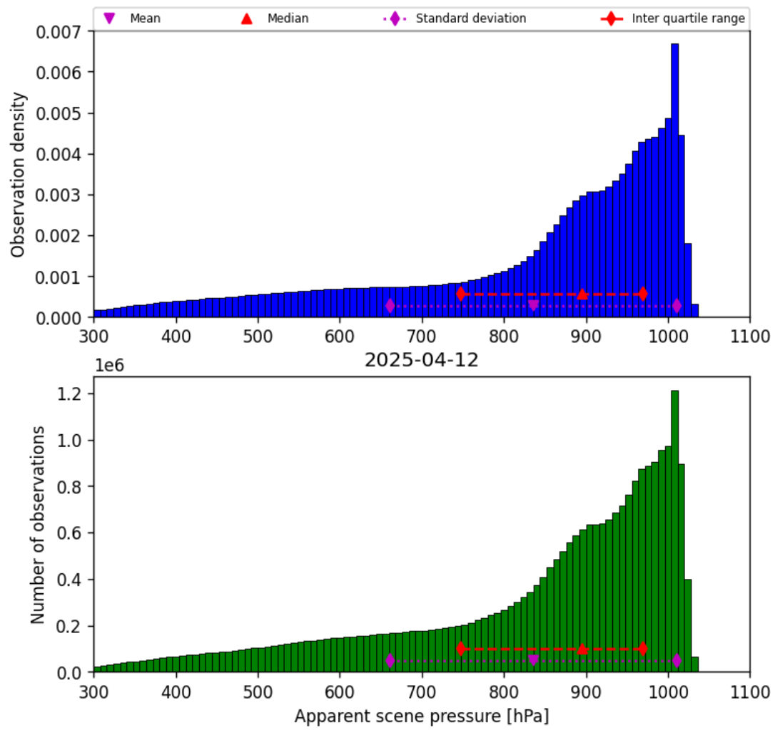
Figure 36: Histogram of “Apparent scene pressure” for 2025-04-11 to 2025-04-13
