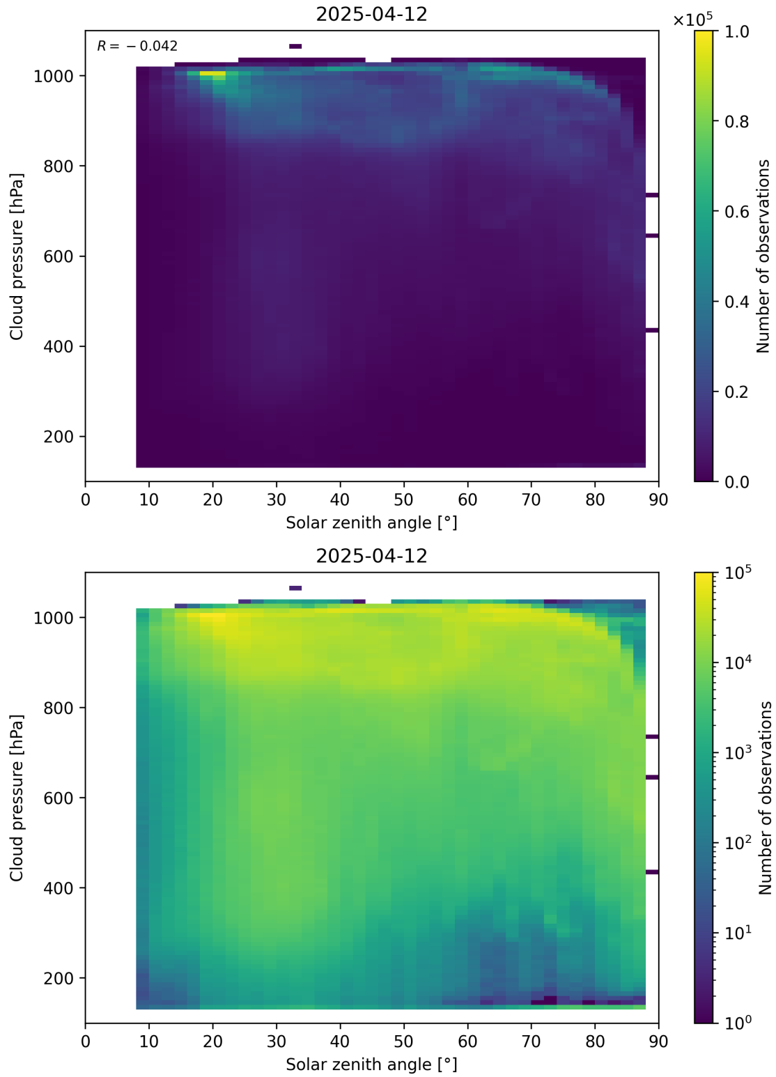
Figure 111: Scatter density plot of “Solar zenith angle” against “Cloud pressure” for 2025-04-11 to 2025-04-13.
