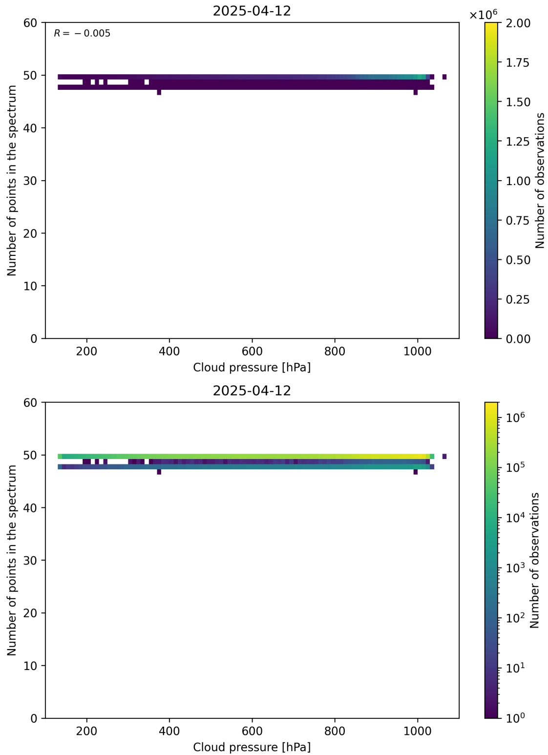
Figure 82: Scatter density plot of “Cloud pressure” against “Number of points in the spectrum” for 2025-04-11 to 2025-04-13.
