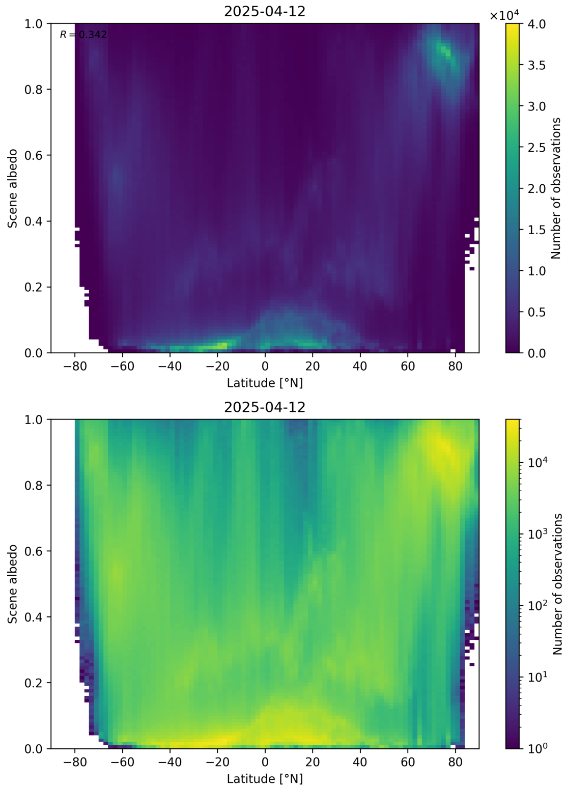
Figure 95: Scatter density plot of “Latitude” against “Scene albedo” for 2025-04-11 to 2025-04-13.
