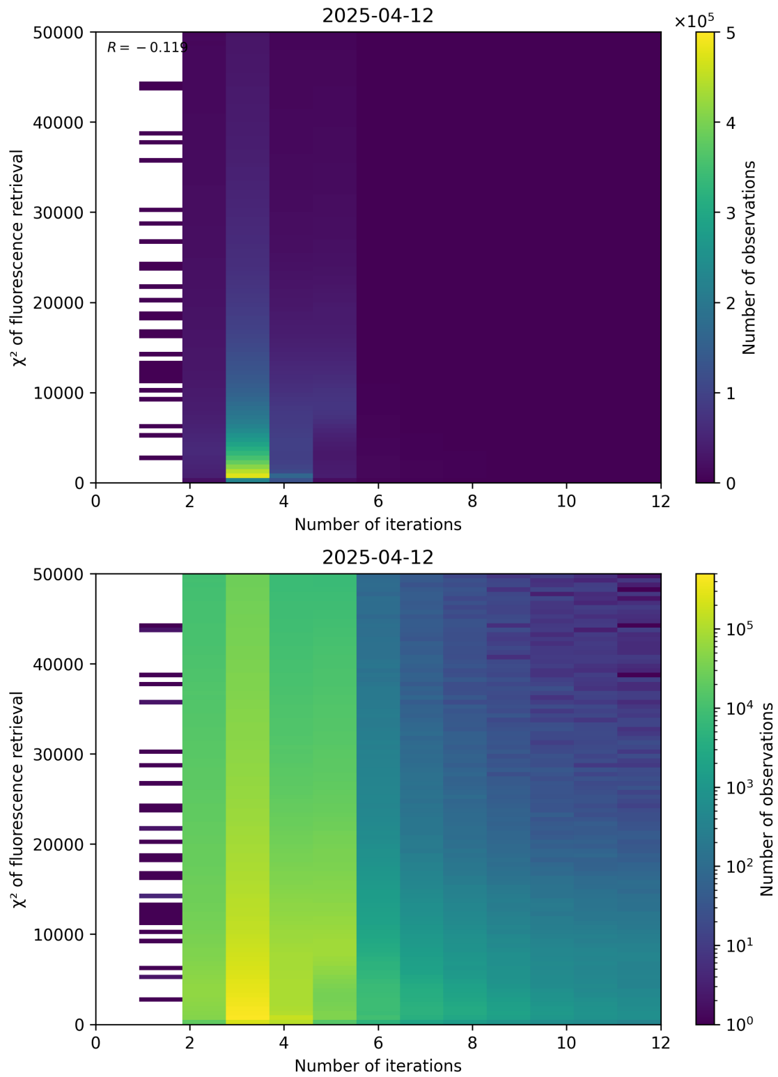
Figure 97: Scatter density plot of “Number of iterations” against “ \chi^2 of fluorescence retrieval” for 2025-04-11 to 2025-04-13.
