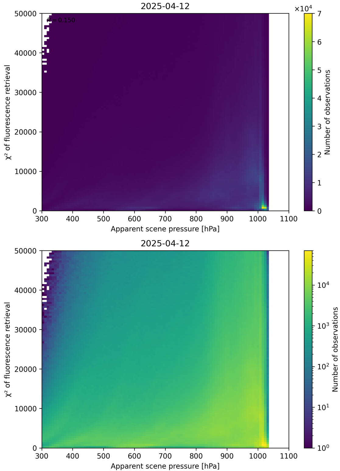
Figure 63: Scatter density plot of “Apparent scene pressure” against “ \chi^2 of fluorescence retrieval” for 2025-04-11 to 2025-04-13.
