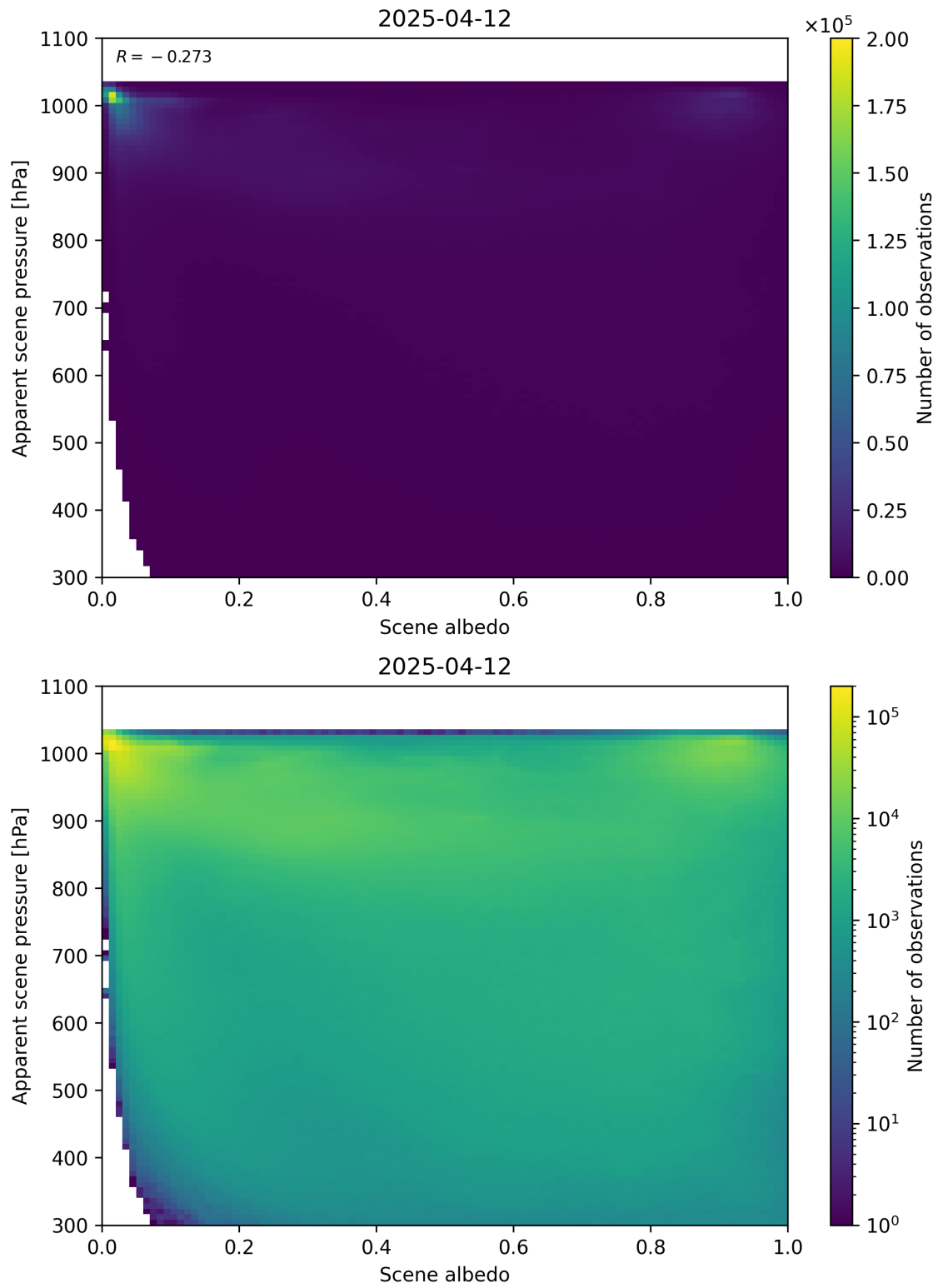
Figure 102: Scatter density plot of “Scene albedo” against “Apparent scene pressure” for 2025-04-11 to 2025-04-13.
