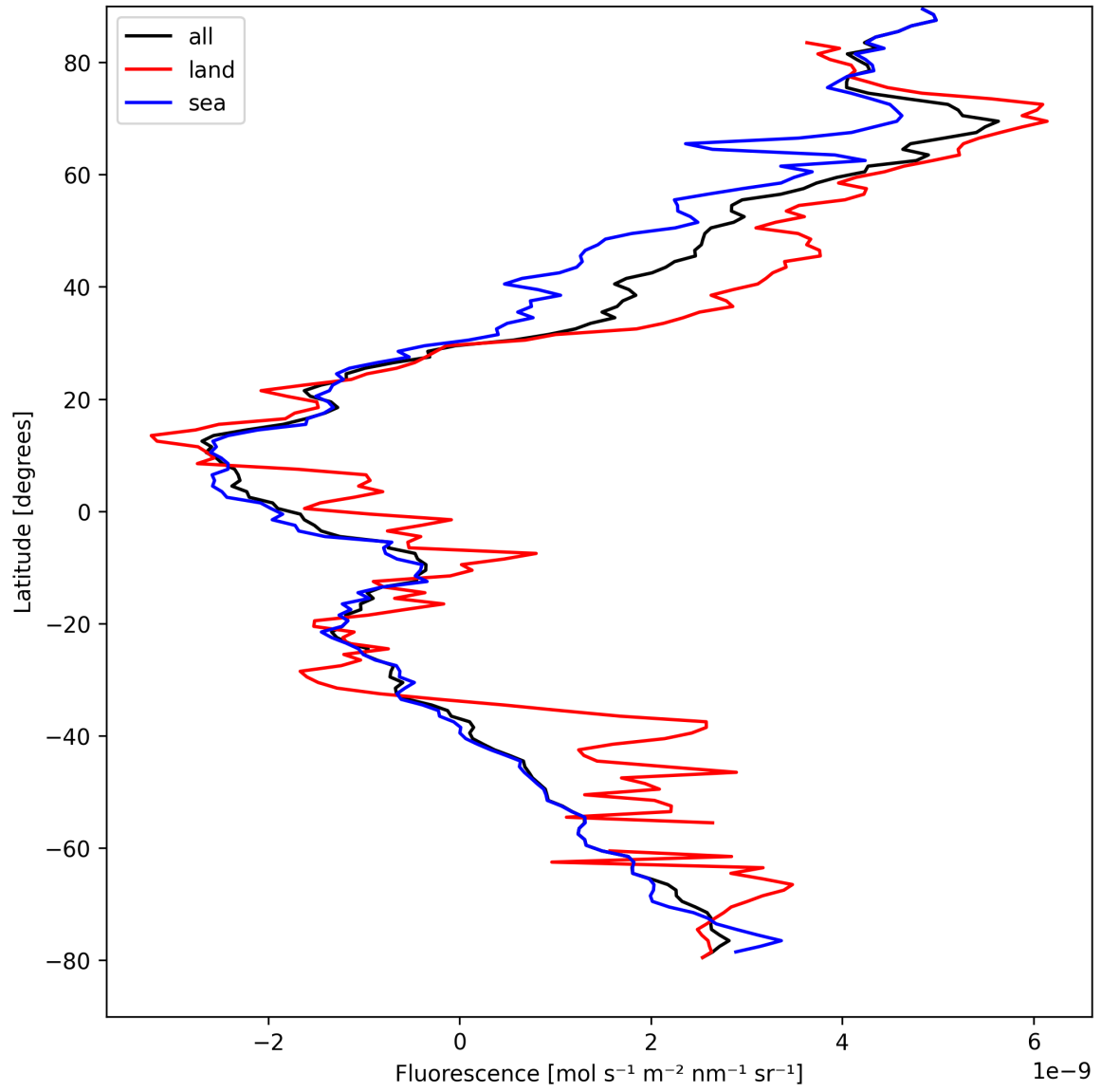
Figure 23: Zonal average of “Fluorescence” for 2025-04-11 to 2025-04-13.
