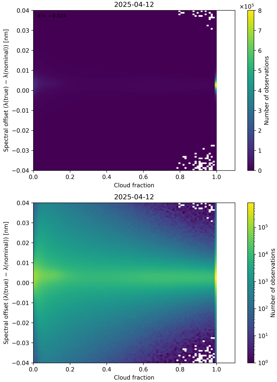
Figure 76: Scatter density plot of “Cloud fraction” against “Spectral offset ( \lambda_{\text{true}} - \lambda_{\text{nominal}} )” for 2025-04-11 to 2025-04-13.
