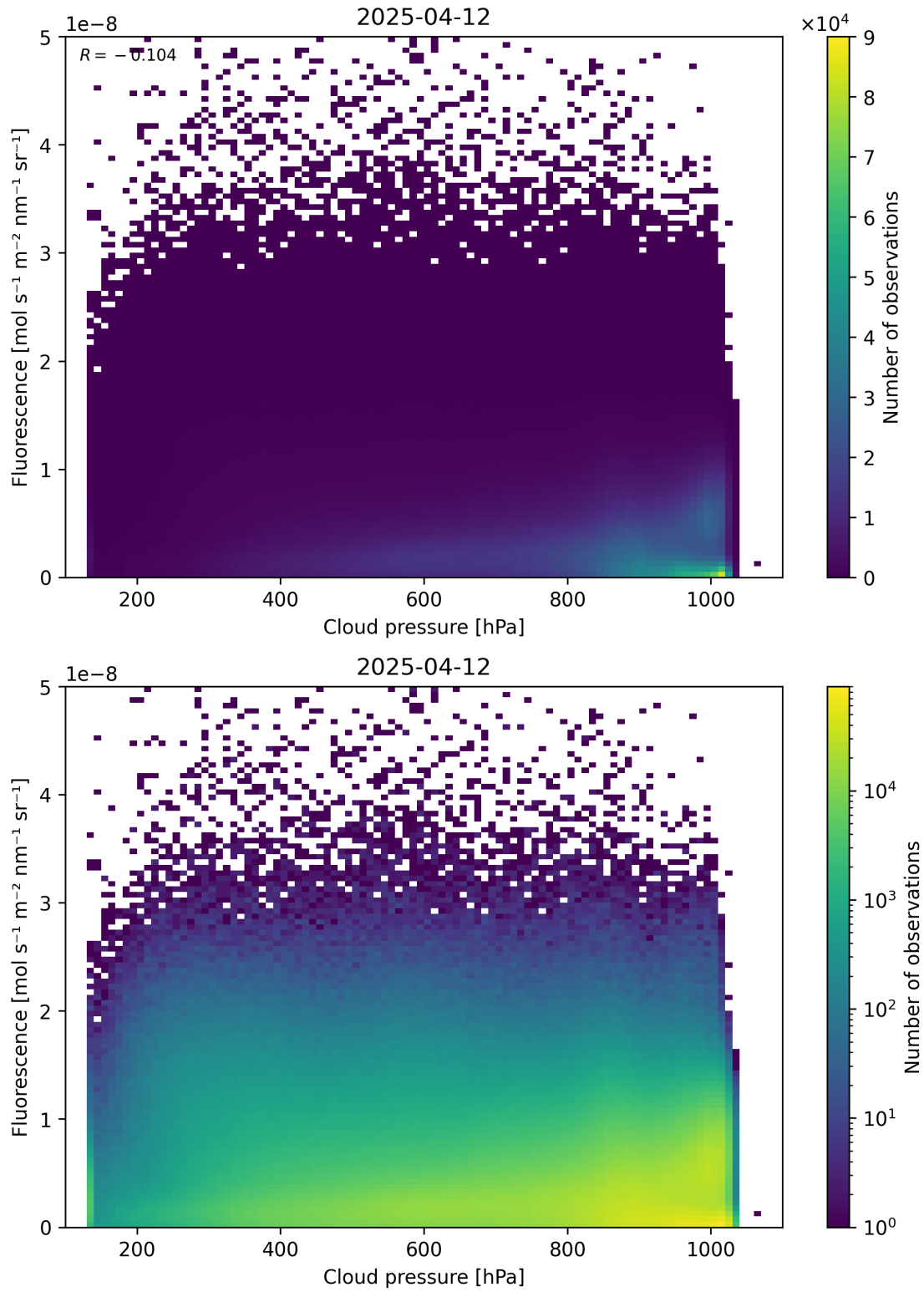
Figure 80: Scatter density plot of “Cloud pressure” against “Fluorescence” for 2025-04-11 to 2025-04-13.
