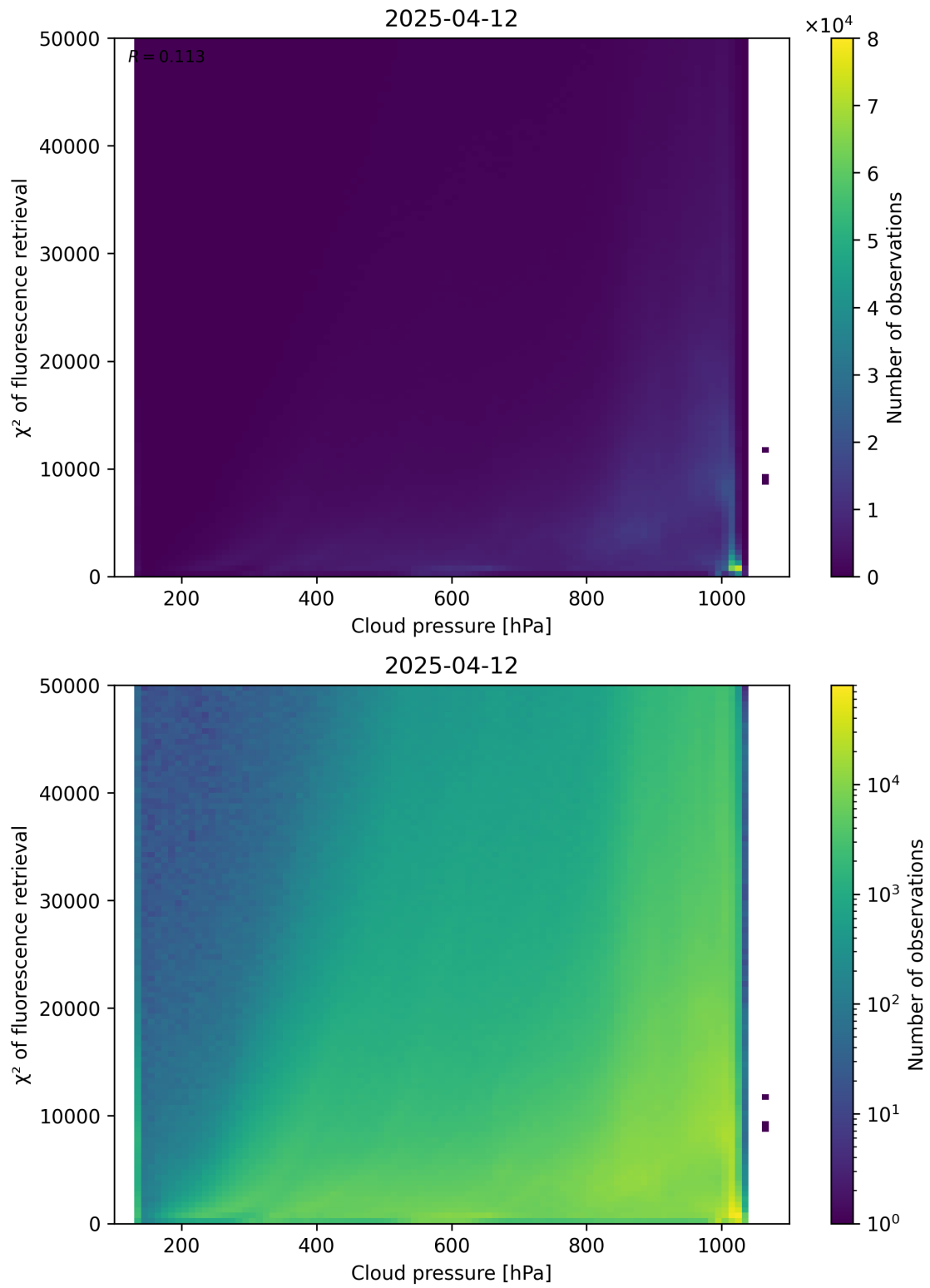
Figure 78: Scatter density plot of “Cloud pressure” against “ \chi^2 of fluorescence retrieval” for 2025-04-11 to 2025-04-13.
