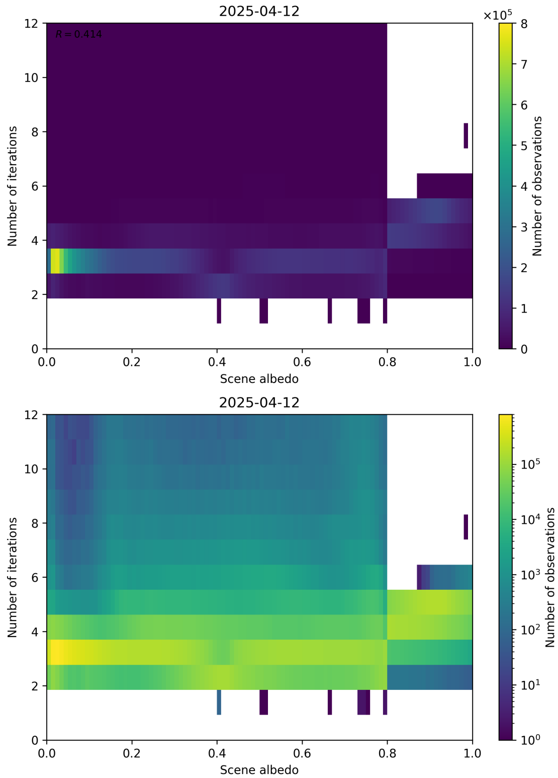
Figure 105: Scatter density plot of “Scene albedo” against “Number of iterations” for 2025-04-11 to 2025-04-13.
