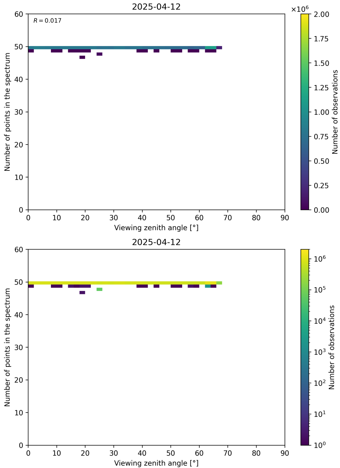
Figure 125: Scatter density plot of “Viewing zenith angle” against “Number of points in the spectrum” for 2025-04-11 to 2025-04-13.
