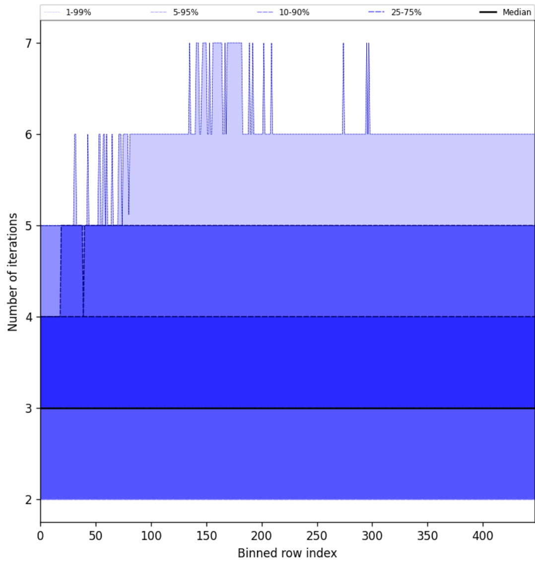
Figure 56: Along track statistics of “Number of iterations” for 2025-04-11 to 2025-04-13
