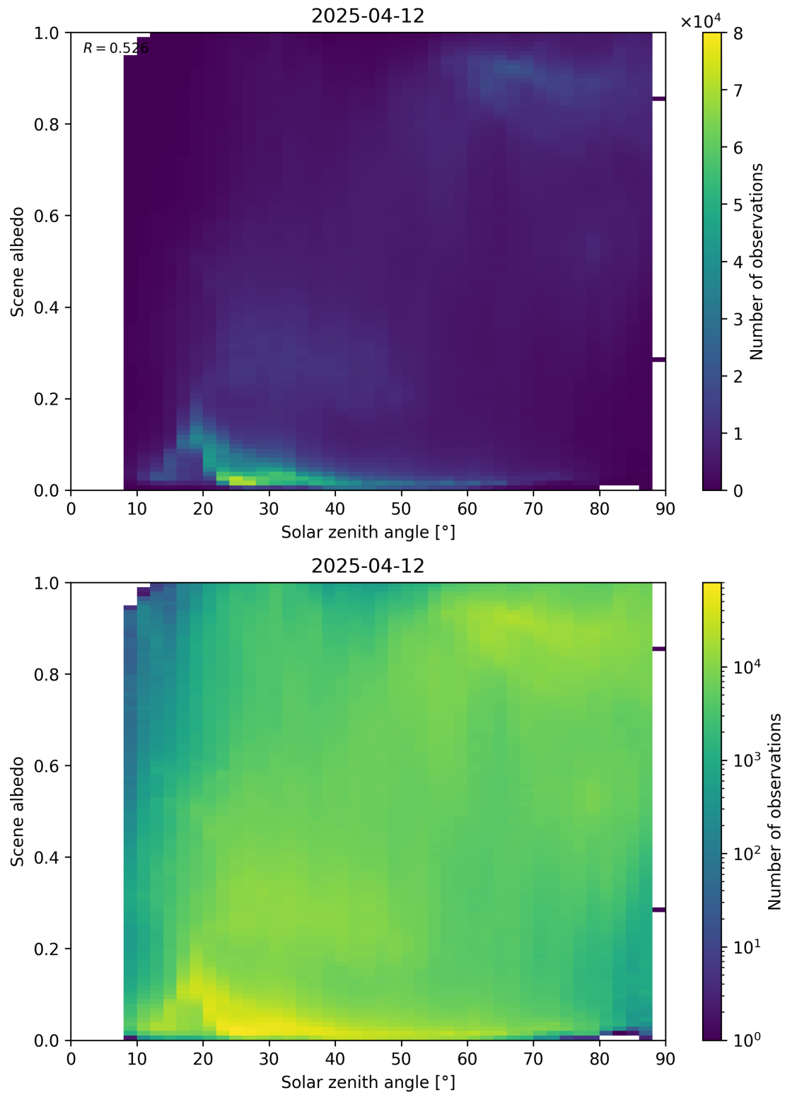
Figure 116: Scatter density plot of “Solar zenith angle” against “Scene albedo” for 2025-04-11 to 2025-04-13.
