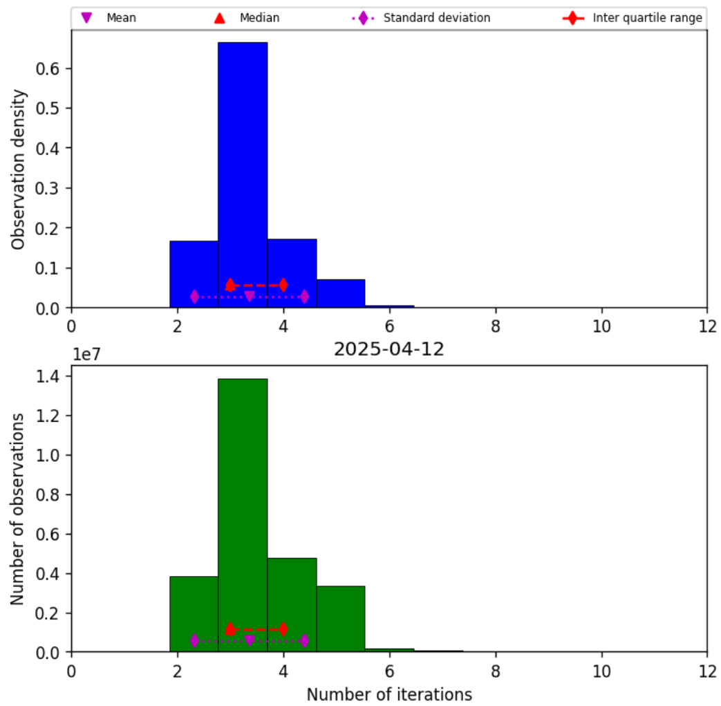
Figure 39: Histogram of “Number of iterations” for 2025-04-11 to 2025-04-13
