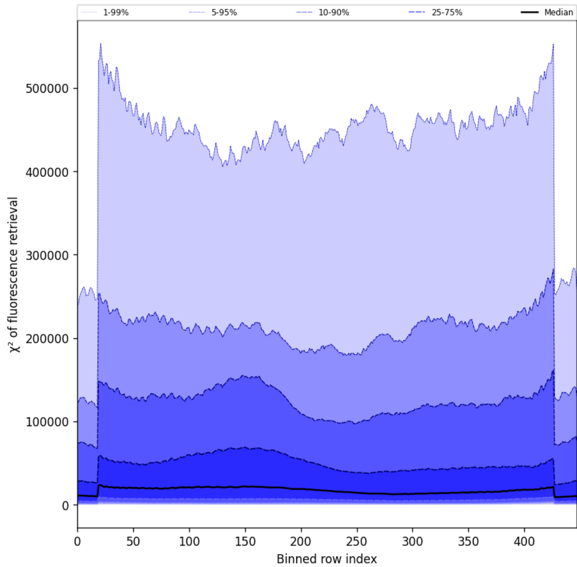
Figure 59: Along track statistics of “ \chi^2 of fluorescence retrieval” for 2025-04-11 to 2025-04-13
