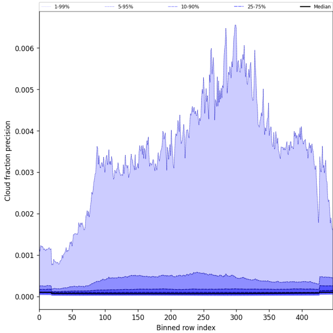
Figure 50: Along track statistics of “Cloud fraction precision” for 2025-04-11 to 2025-04-13
