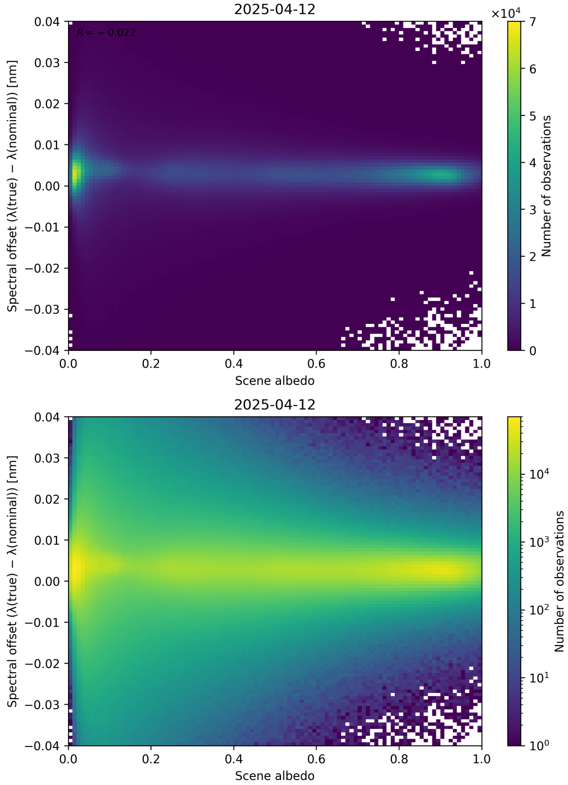
Figure 107: Scatter density plot of “Scene albedo” against “Spectral offset ( \lambda_{\text{true}} - \lambda_{\text{nominal}} )” for 2025-04-11 to 2025-04-13.
