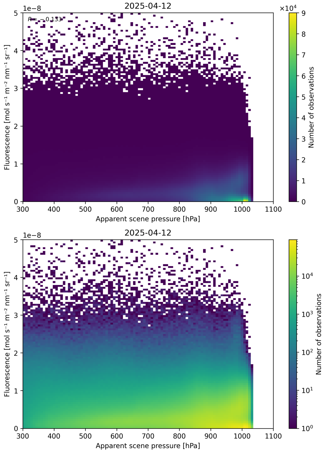
Figure 64: Scatter density plot of “Apparent scene pressure” against “Fluorescence” for 2025-04-11 to 2025-04-13.
