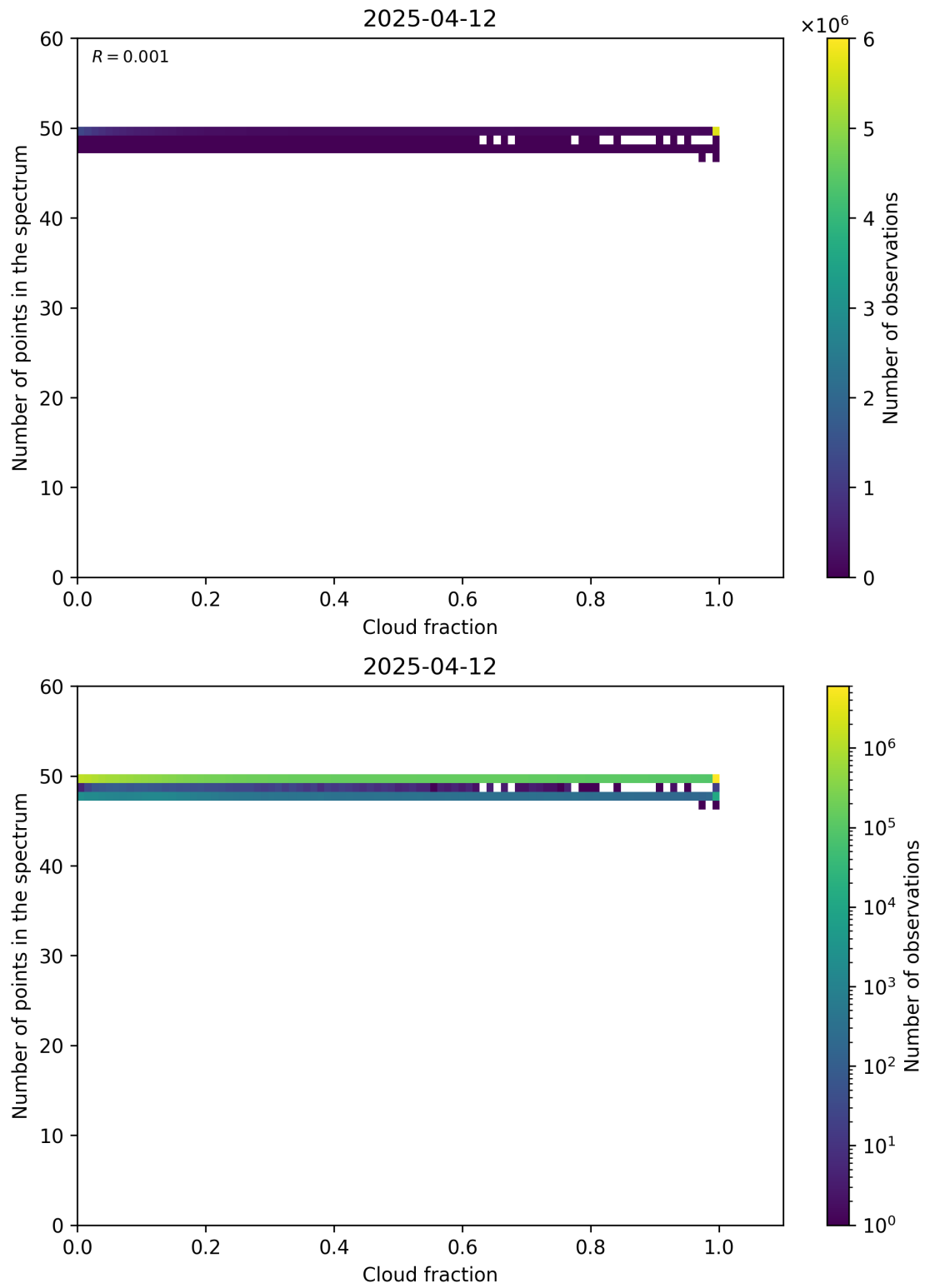
Figure 74: Scatter density plot of “Cloud fraction” against “Number of points in the spectrum” for 2025-04-11 to 2025-04-13.
