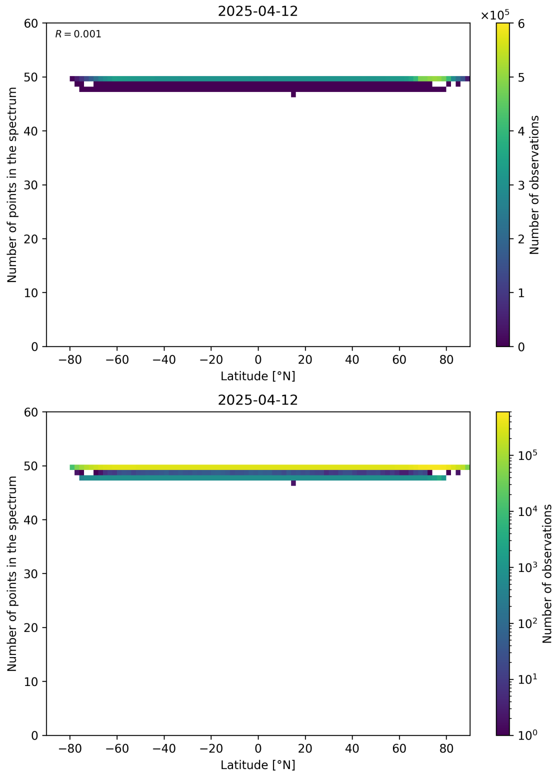
Figure 94: Scatter density plot of “Latitude” against “Number of points in the spectrum” for 2025-04-11 to 2025-04-13.
