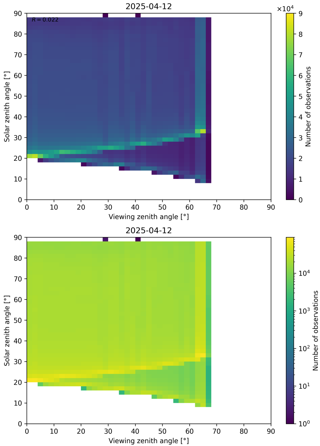
Figure 127: Scatter density plot of “Viewing zenith angle” against “Solar zenith angle” for 2025-04-11 to 2025-04-13.
