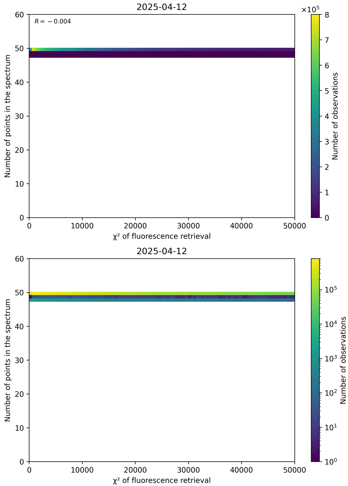
Figure 68: Scatter density plot of " \chi^2 of fluorescence retrieval" against "Number of points in the spectrum" for 2025-04-11 to 2025-04-13.
