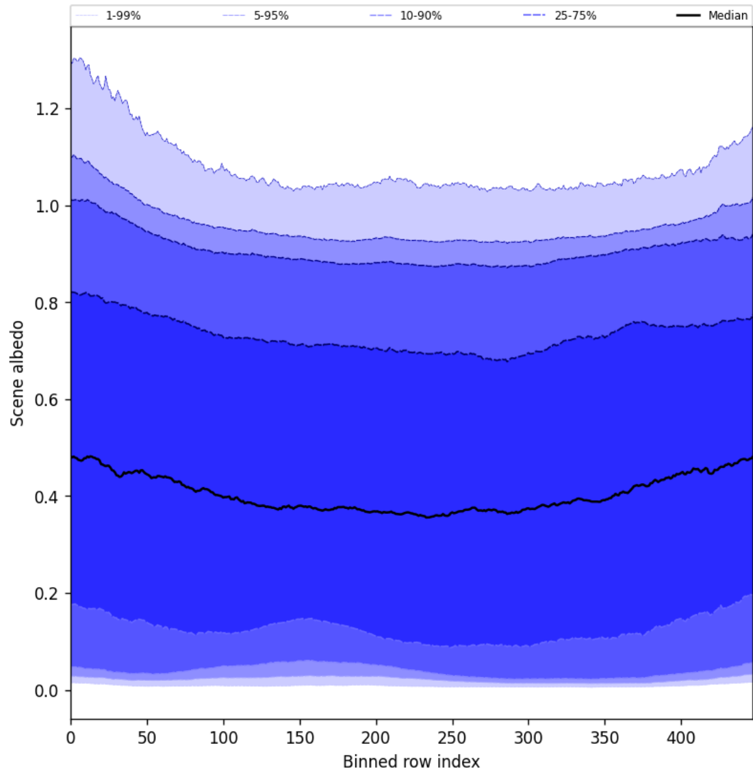
Figure 51: Along track statistics of “Scene albedo” for 2025-04-11 to 2025-04-13
