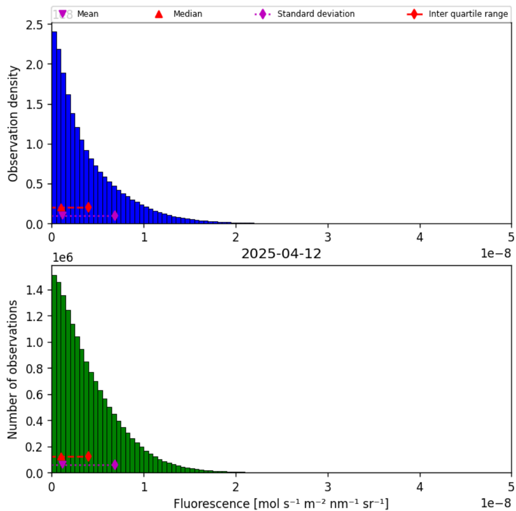
Figure 40: Histogram of “Fluorescence” for 2025-04-11 to 2025-04-13
