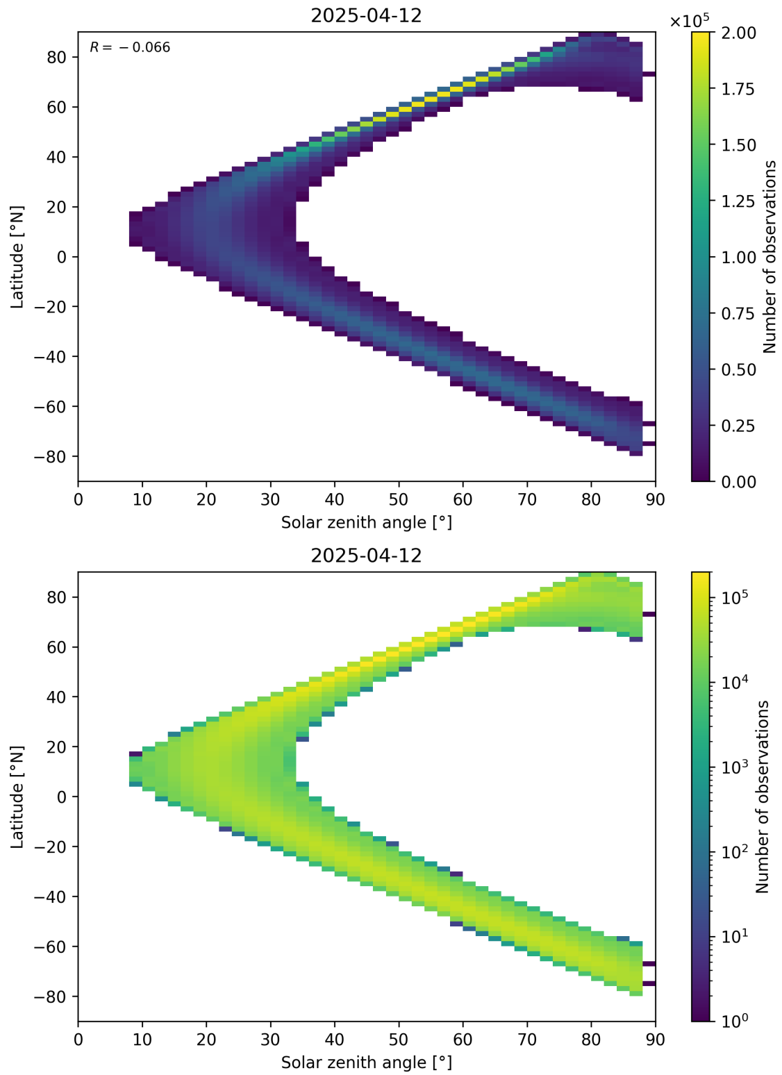
Figure 113: Scatter density plot of “Solar zenith angle” against “Latitude” for 2025-04-11 to 2025-04-13.
