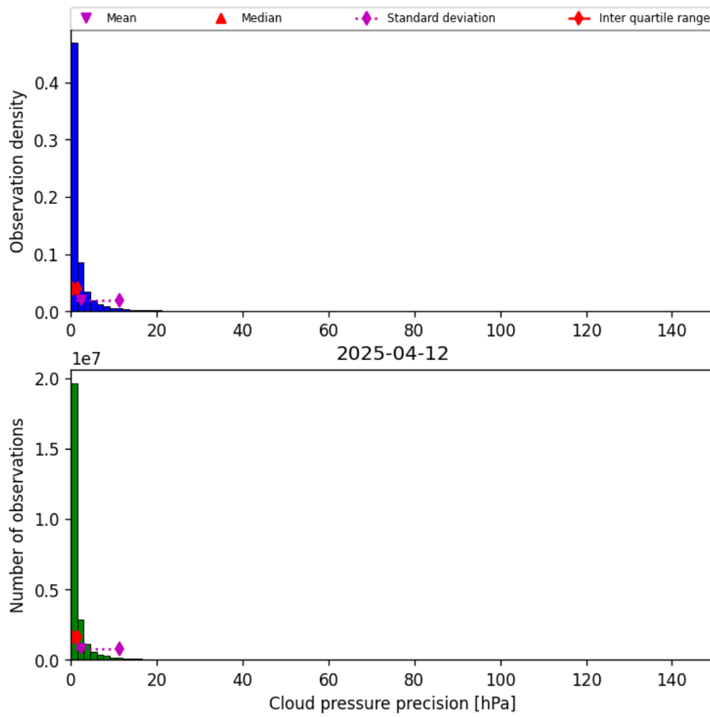
Figure 31: Histogram of “Cloud pressure precision” for 2025-04-11 to 2025-04-13
