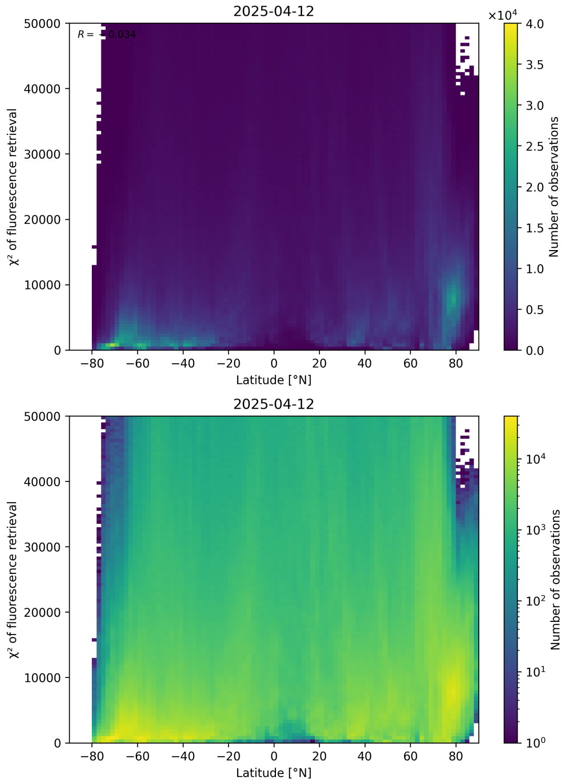
Figure 89: Scatter density plot of “Latitude” against “ \chi^2 of fluorescence retrieval” for 2025-04-11 to 2025-04-13.
