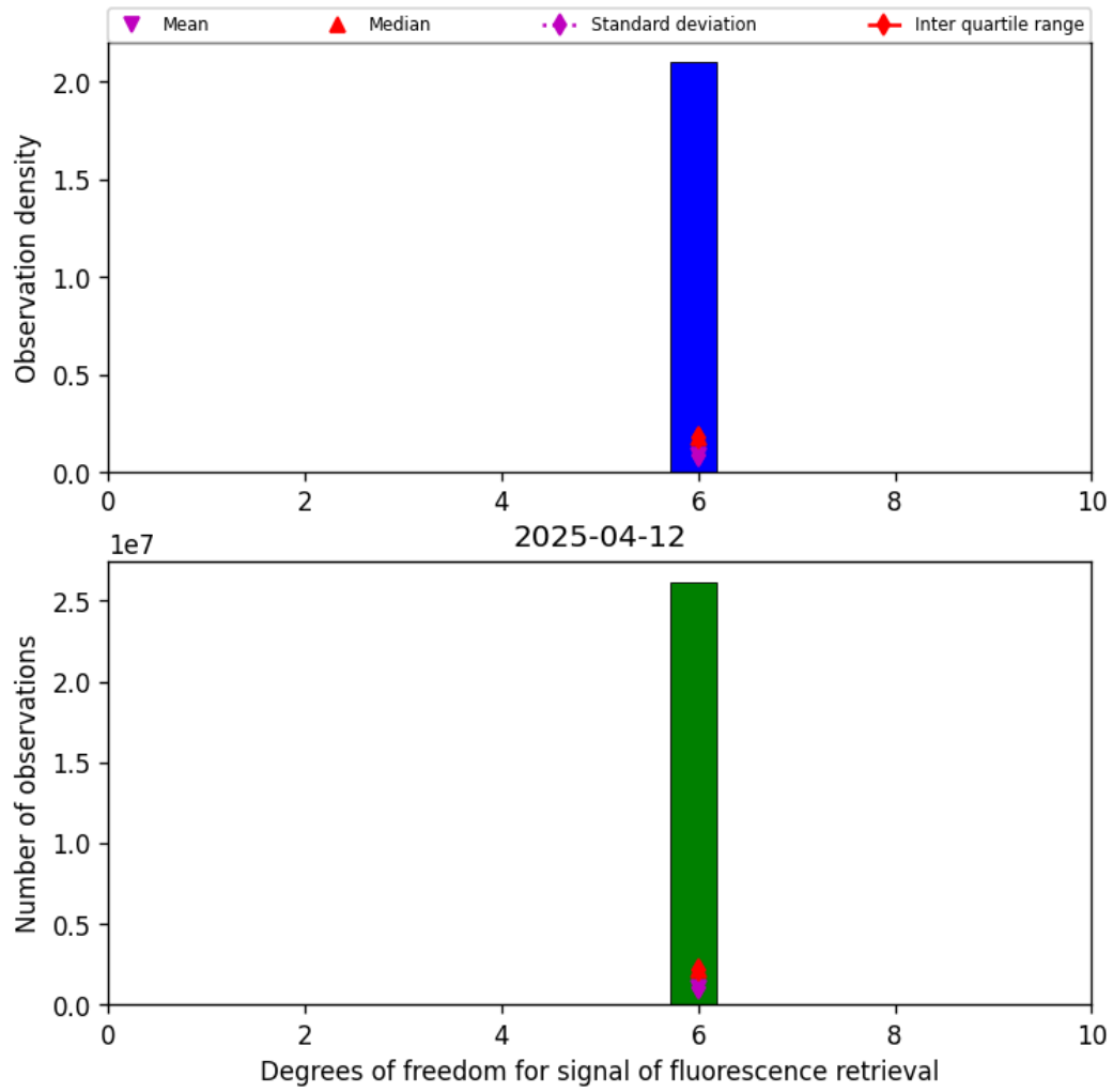
Figure 43: Histogram of "Degrees of freedom for signal of fluorescence retrieval" for 2025-04-11 to 2025-04-13
