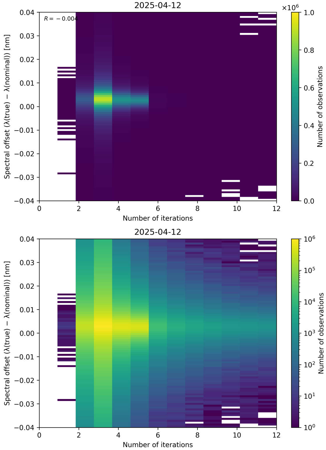
Figure 100: Scatter density plot of “Number of iterations” against “Spectral offset ( \lambda_{\text{true}} - \lambda_{\text{nominal}} )” for 2025-04-11 to 2025-04-13.
