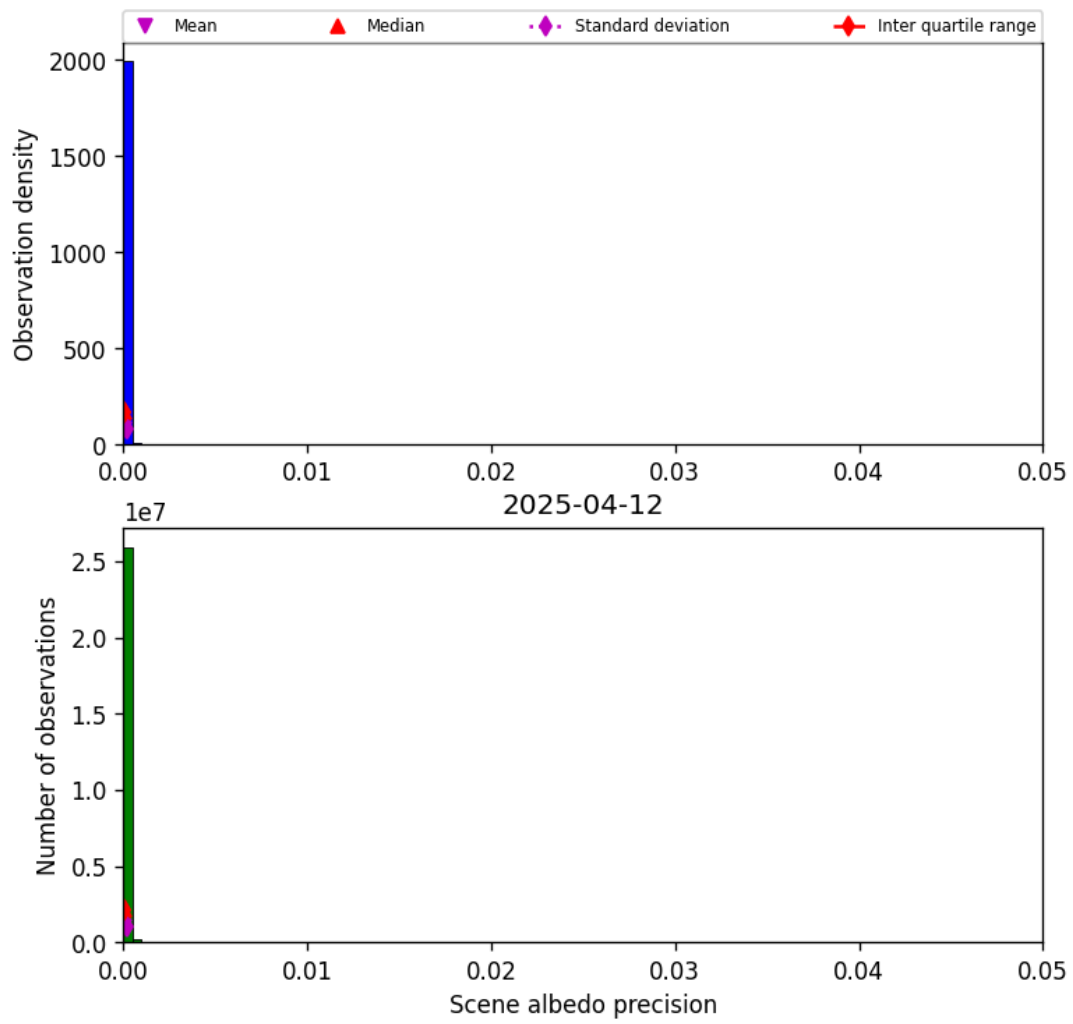
Figure 35: Histogram of “Scene albedo precision” for 2025-04-11 to 2025-04-13
