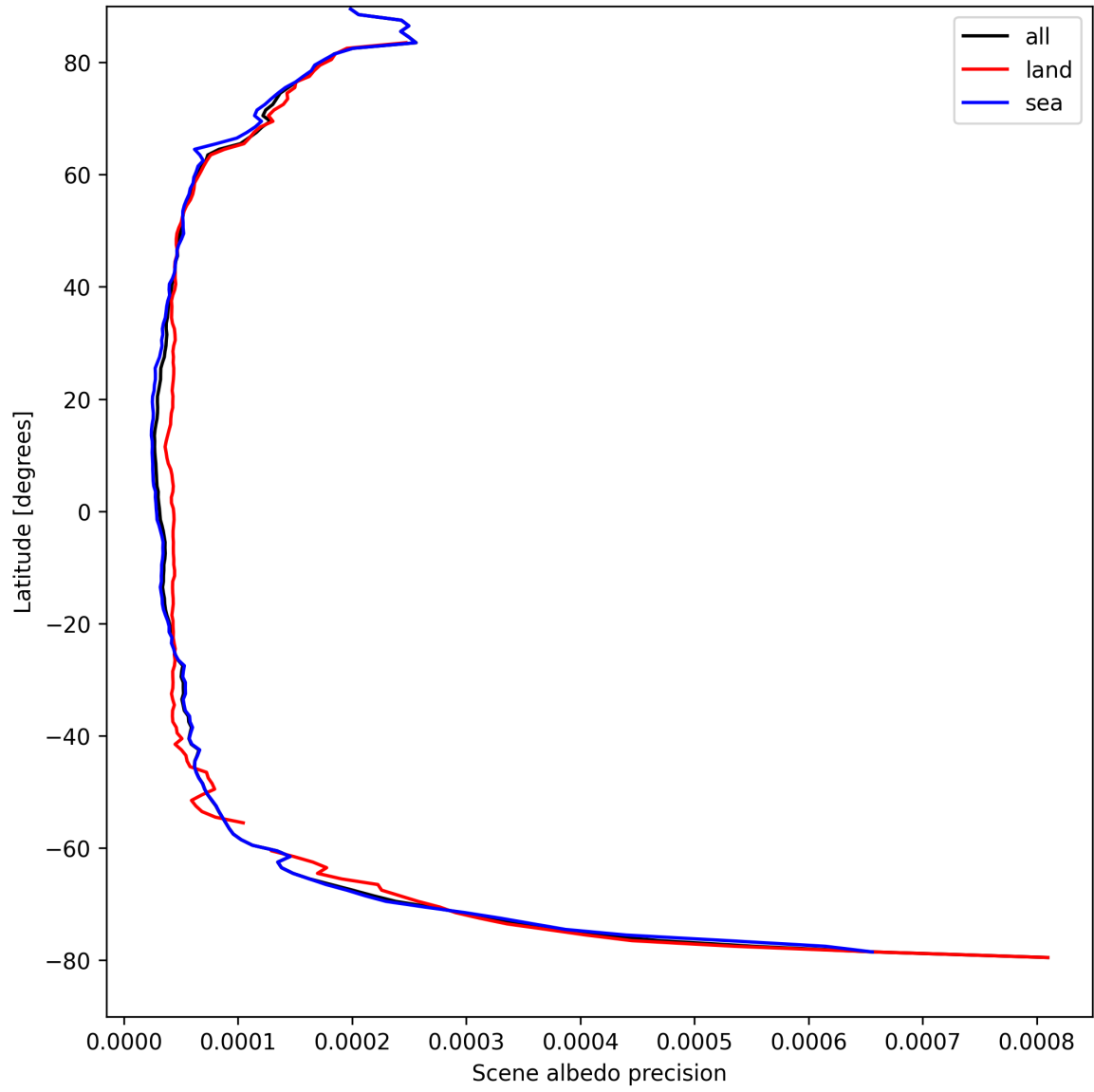
Figure 18: Zonal average of “Scene albedo precision” for 2025-04-11 to 2025-04-13.
