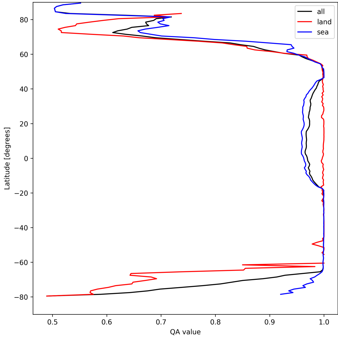
Figure 12: Zonal average of “QA value” for 2025-04-11 to 2025-04-13.
