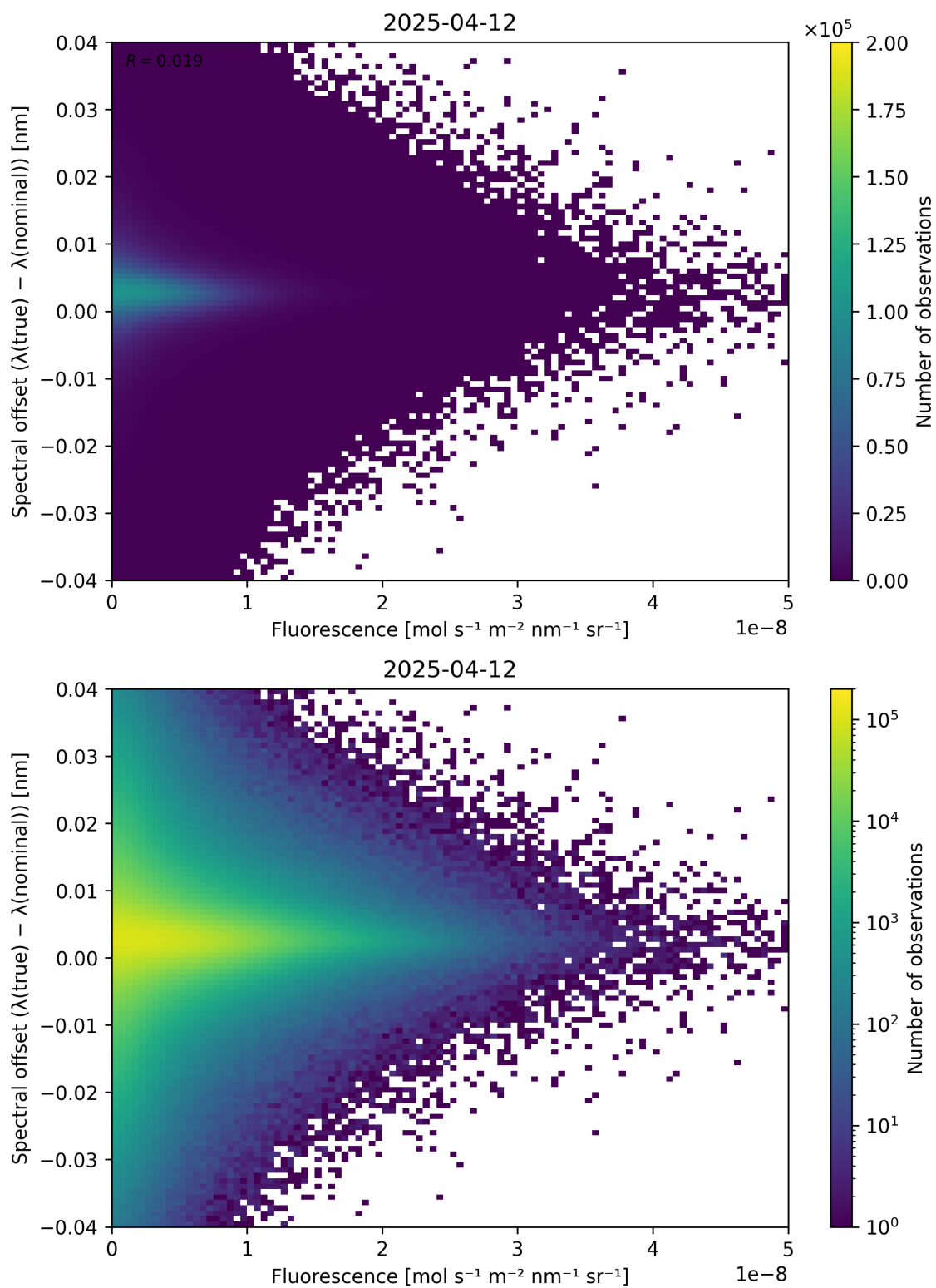
Figure 87: Scatter density plot of “Fluorescence” against “Spectral offset ( \lambda_{\text{true}} - \lambda_{\text{nominal}} )” for 2025-04-11 to 2025-04-13.
