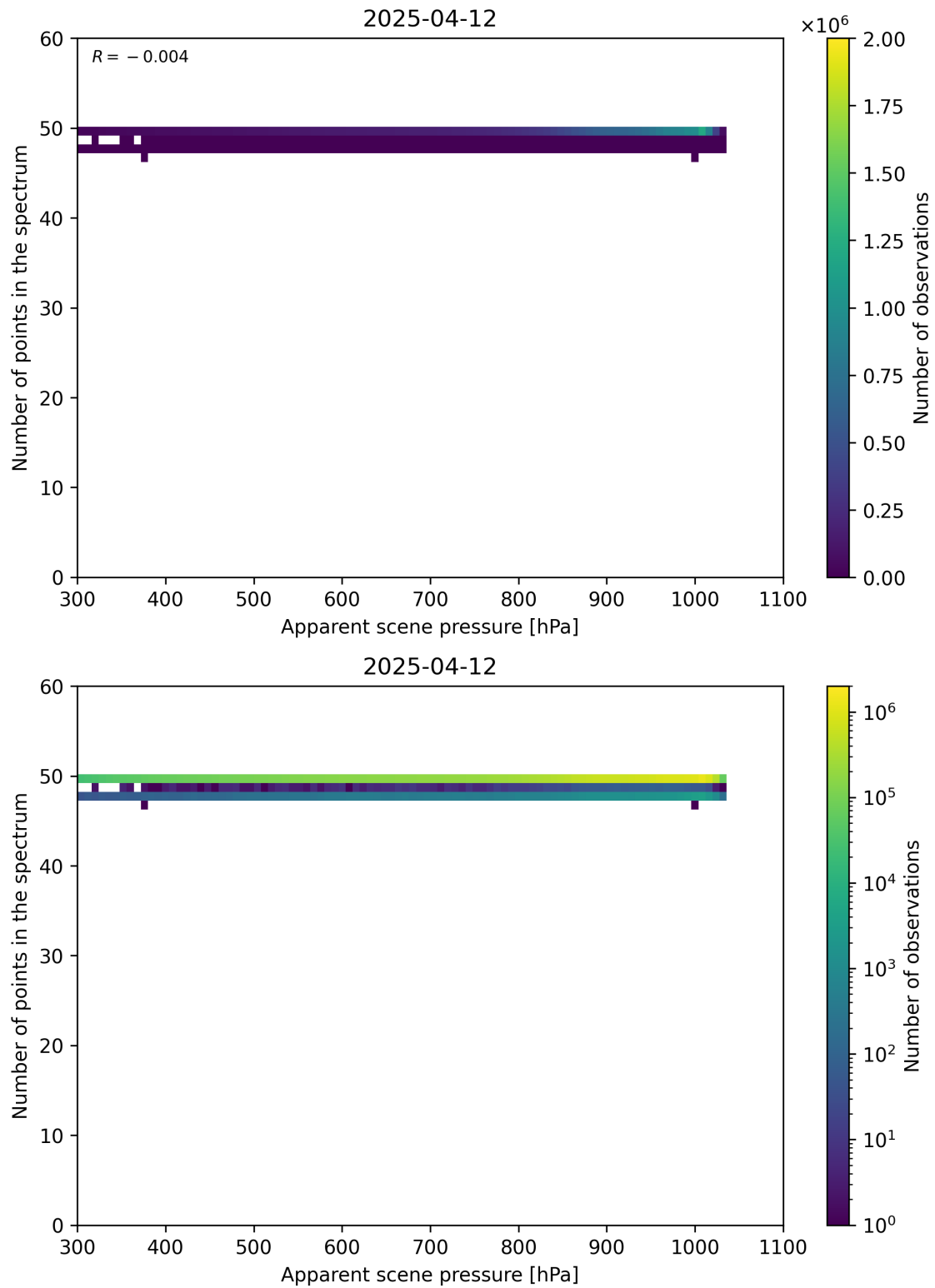
Figure 66: Scatter density plot of “Apparent scene pressure” against “Number of points in the spectrum” for 2025-04-11 to 2025-04-13.
