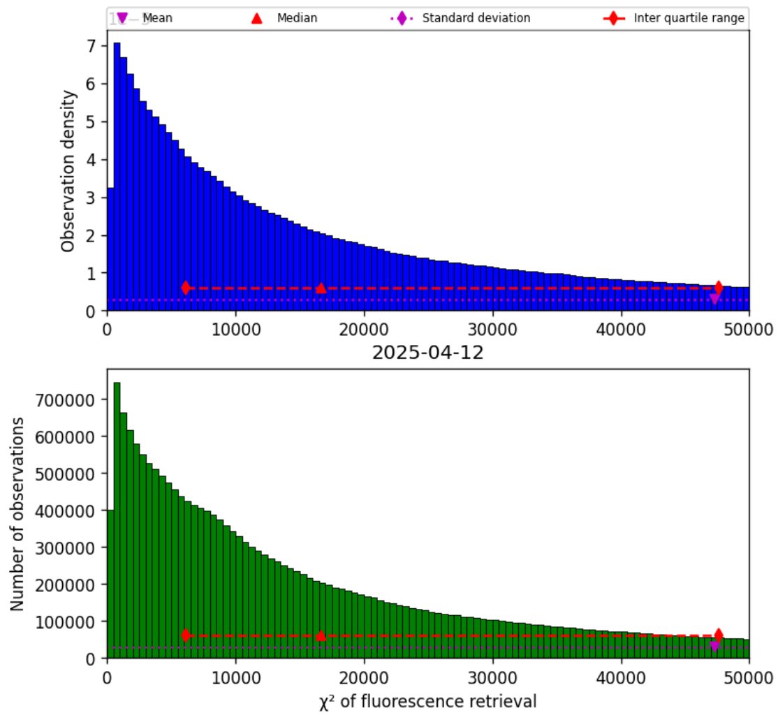
Figure 42: Histogram of “ \chi^2 of fluorescence retrieval” for 2025-04-11 to 2025-04-13
