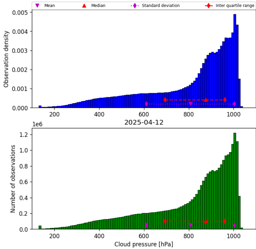
Figure 30: Histogram of “Cloud pressure” for 2025-04-11 to 2025-04-13
