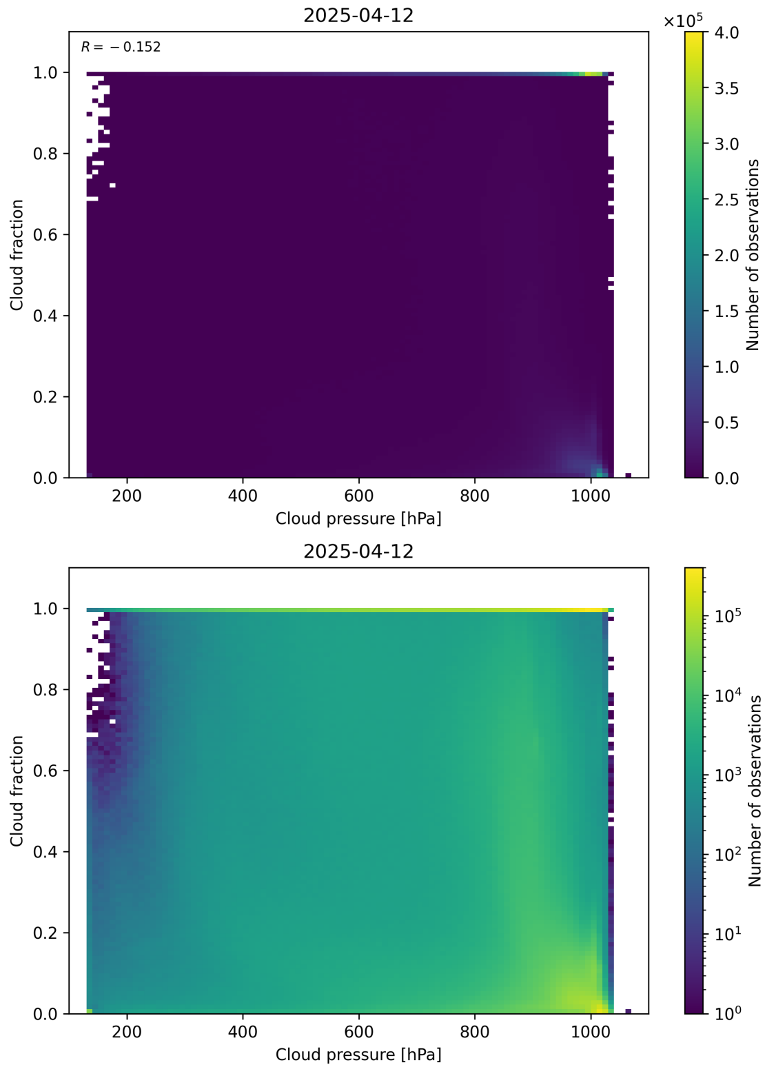
Figure 79: Scatter density plot of “Cloud pressure” against “Cloud fraction” for 2025-04-11 to 2025-04-13.
