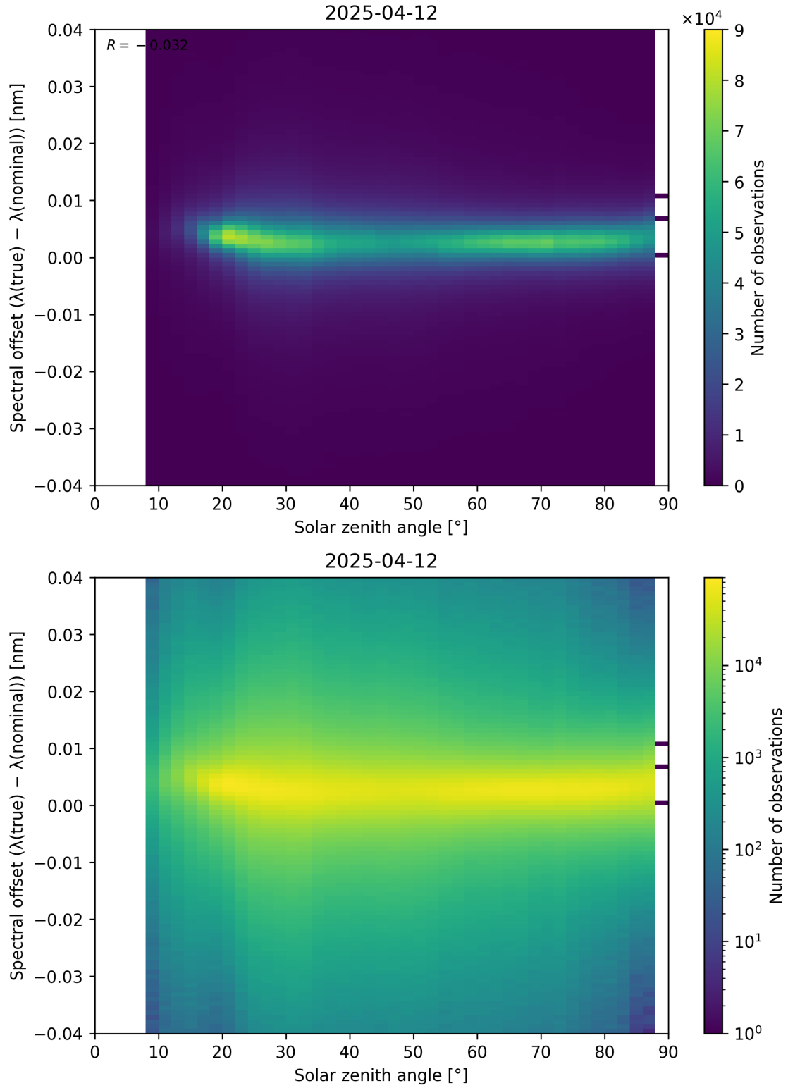
Figure 117: Scatter density plot of “Solar zenith angle” against “Spectral offset ( \lambda_{\text{true}} - \lambda_{\text{nominal}} )” for 2025-04-11 to 2025-04-13.
