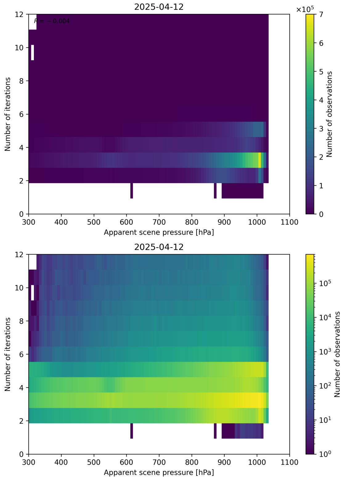
Figure 65: Scatter density plot of “Apparent scene pressure” against “Number of iterations” for 2025-04-11 to 2025-04-13.
