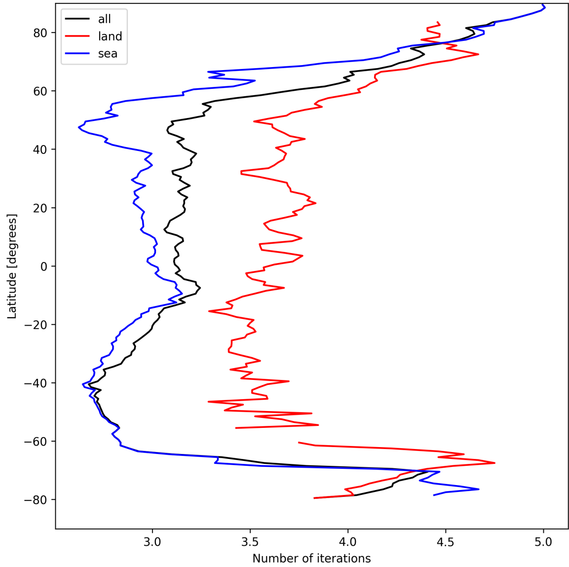
Figure 22: Zonal average of “Number of iterations” for 2025-04-11 to 2025-04-13.
