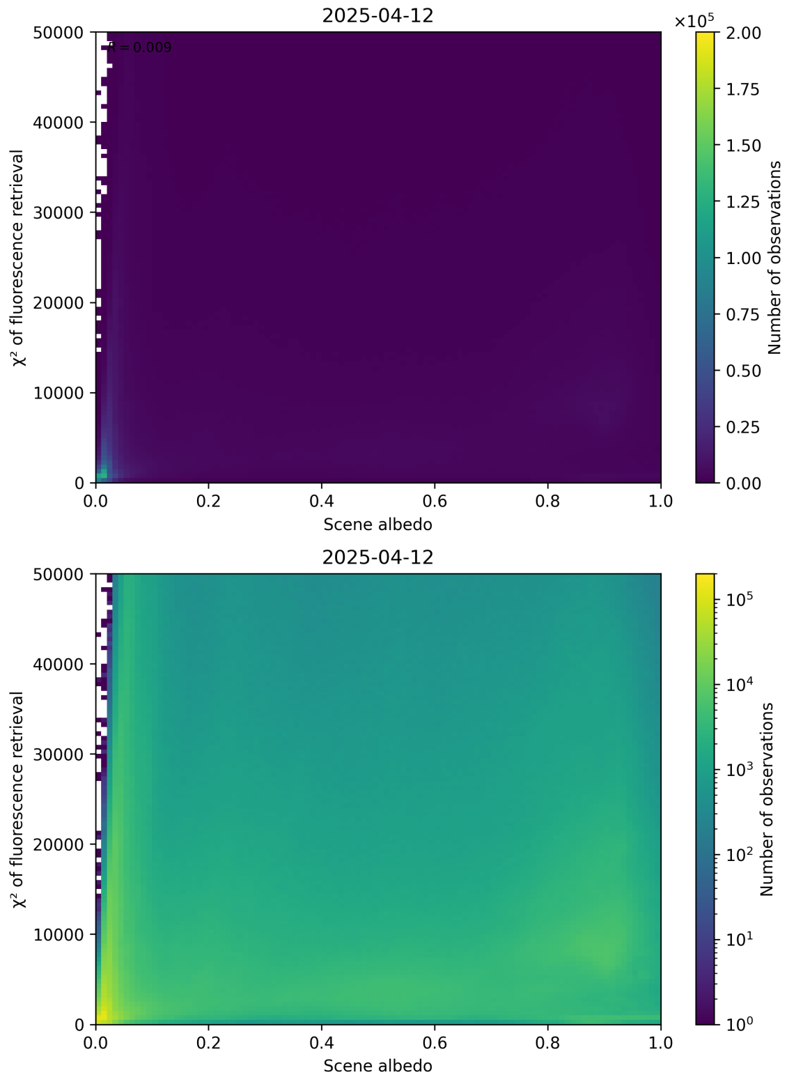
Figure 103: Scatter density plot of “Scene albedo” against “ \chi^2 of fluorescence retrieval” for 2025-04-11 to 2025-04-13.
