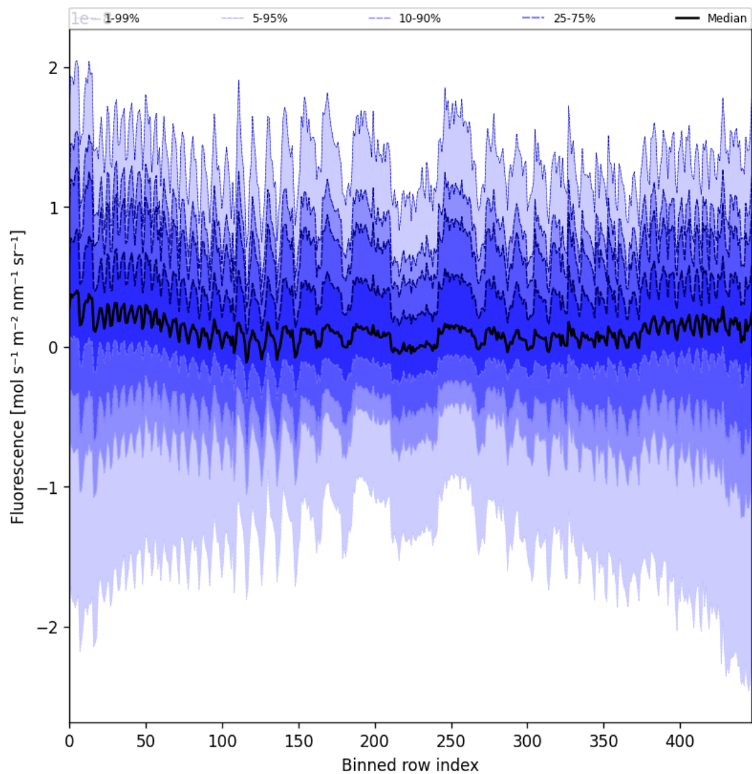
Figure 57: Along track statistics of “Fluorescence” for 2025-04-11 to 2025-04-13
