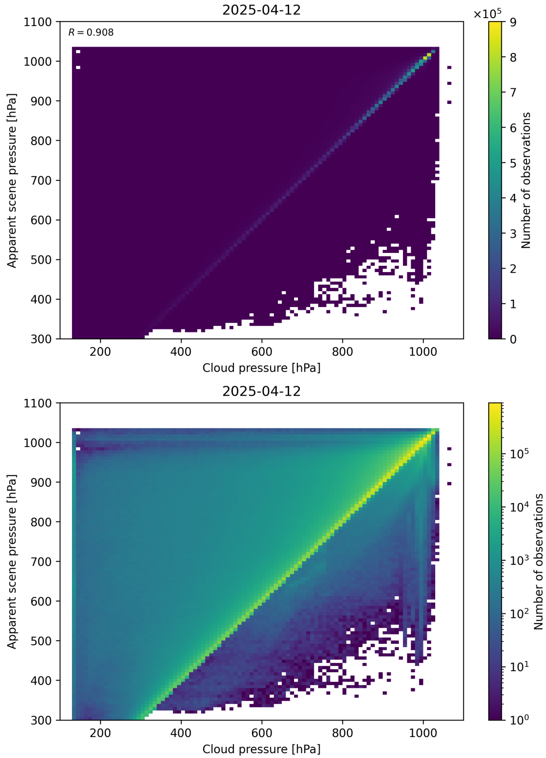
Figure 77: Scatter density plot of “Cloud pressure” against “Apparent scene pressure” for 2025-04-11 to 2025-04-13.
