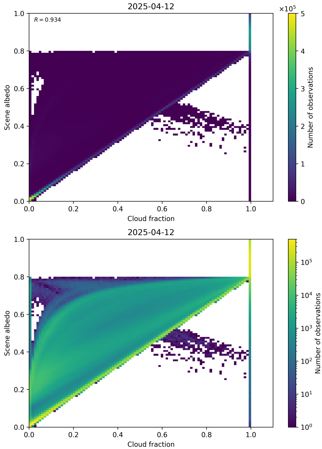
Figure 75: Scatter density plot of “Cloud fraction” against “Scene albedo” for 2025-04-11 to 2025-04-13.
