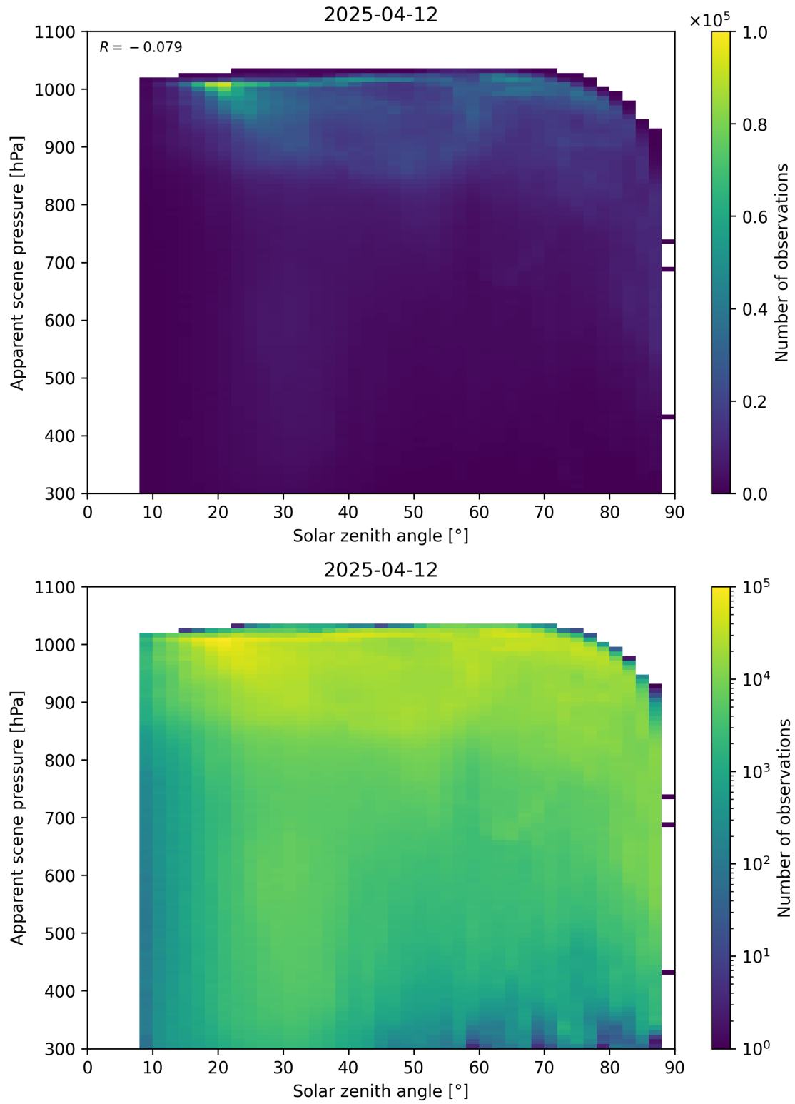
Figure 108: Scatter density plot of “Solar zenith angle” against “Apparent scene pressure” for 2025-04-11 to 2025-04-13.
