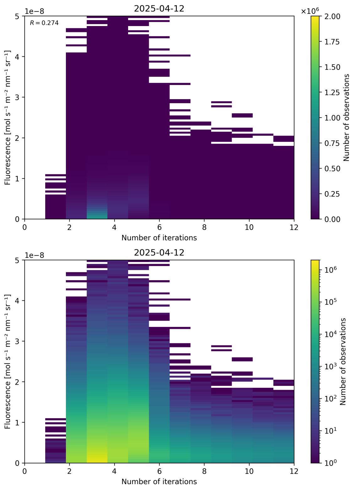
Figure 98: Scatter density plot of “Number of iterations” against “Fluorescence” for 2025-04-11 to 2025-04-13.
