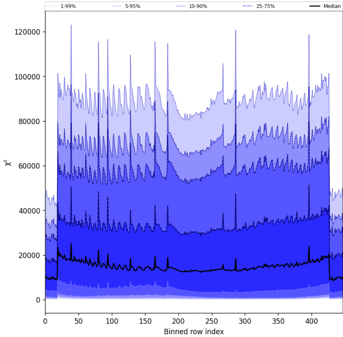
Figure 55: Along track statistics of “ \chi^2 ” for 2025-04-11 to 2025-04-13
