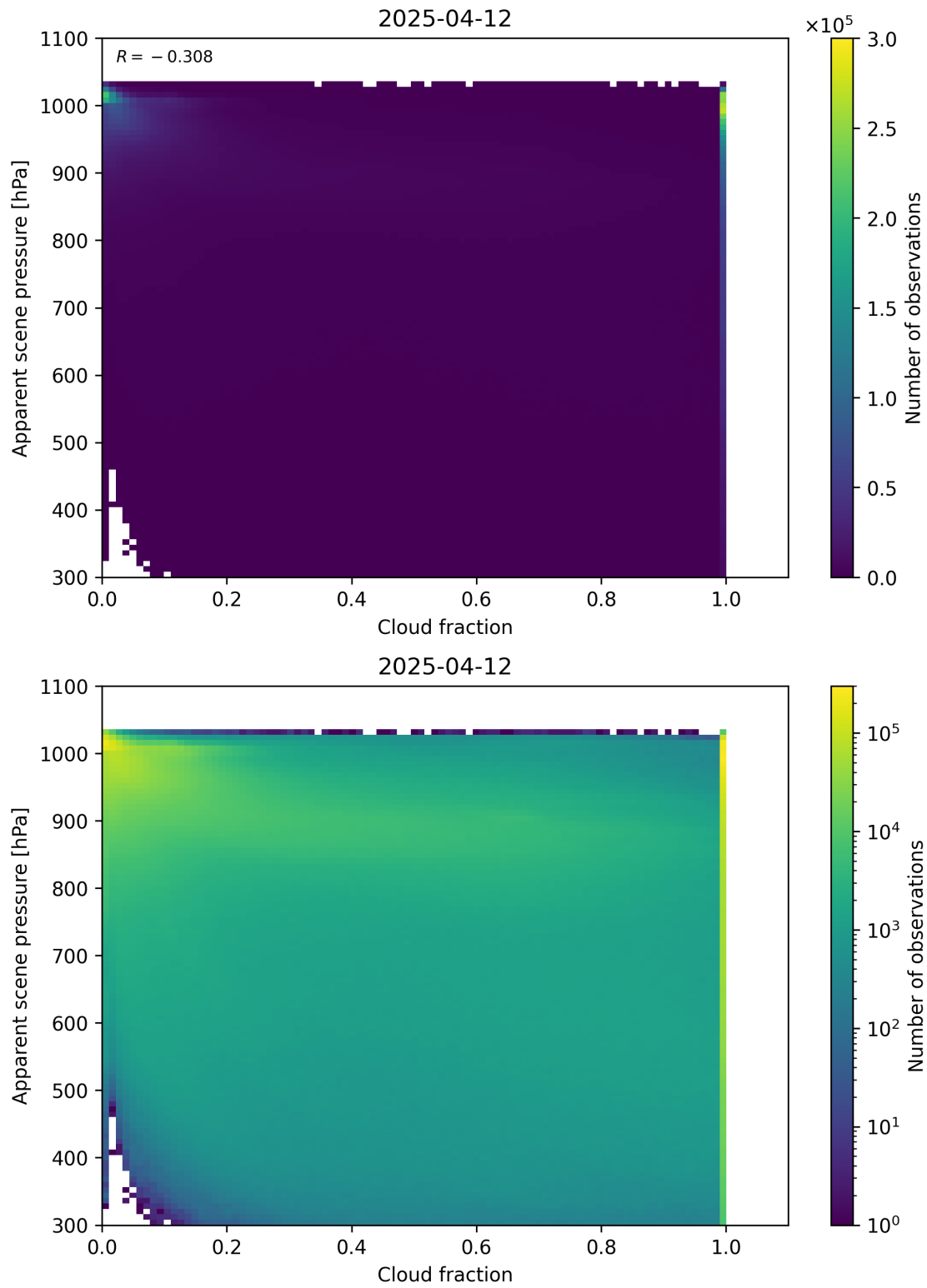
Figure 70: Scatter density plot of “Cloud fraction” against “Apparent scene pressure” for 2025-04-11 to 2025-04-13.
