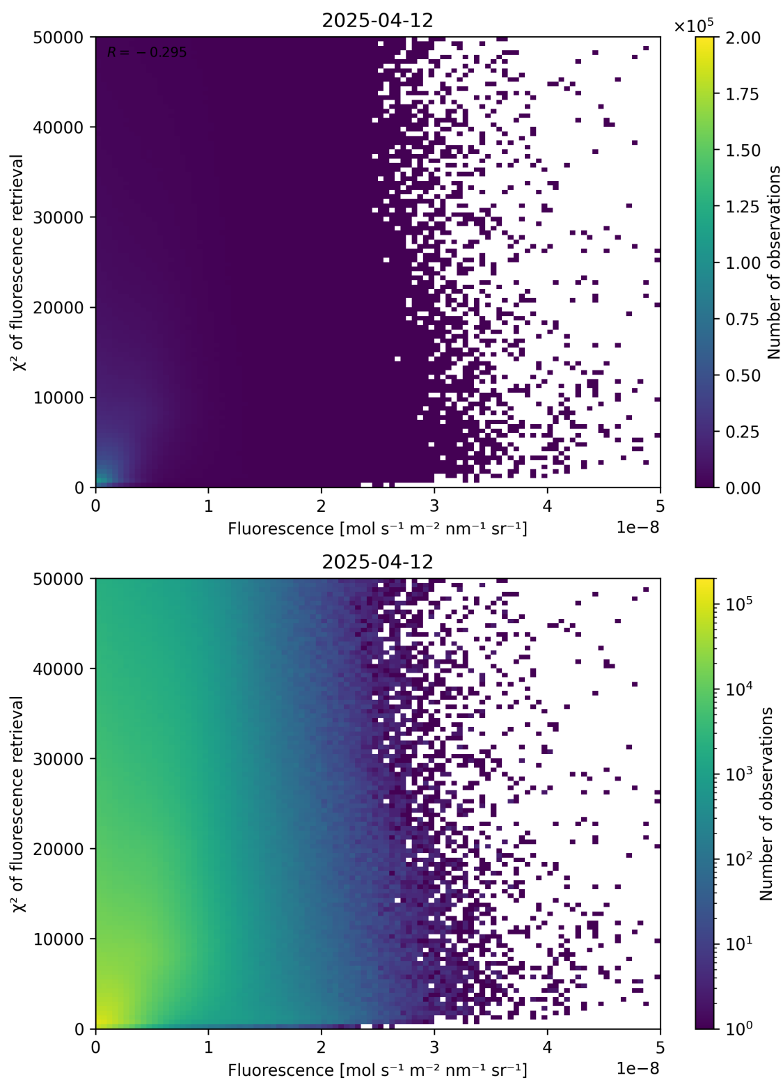
Figure 85: Scatter density plot of “Fluorescence” against “ \chi^2 of fluorescence retrieval” for 2025-04-11 to 2025-04-13.
