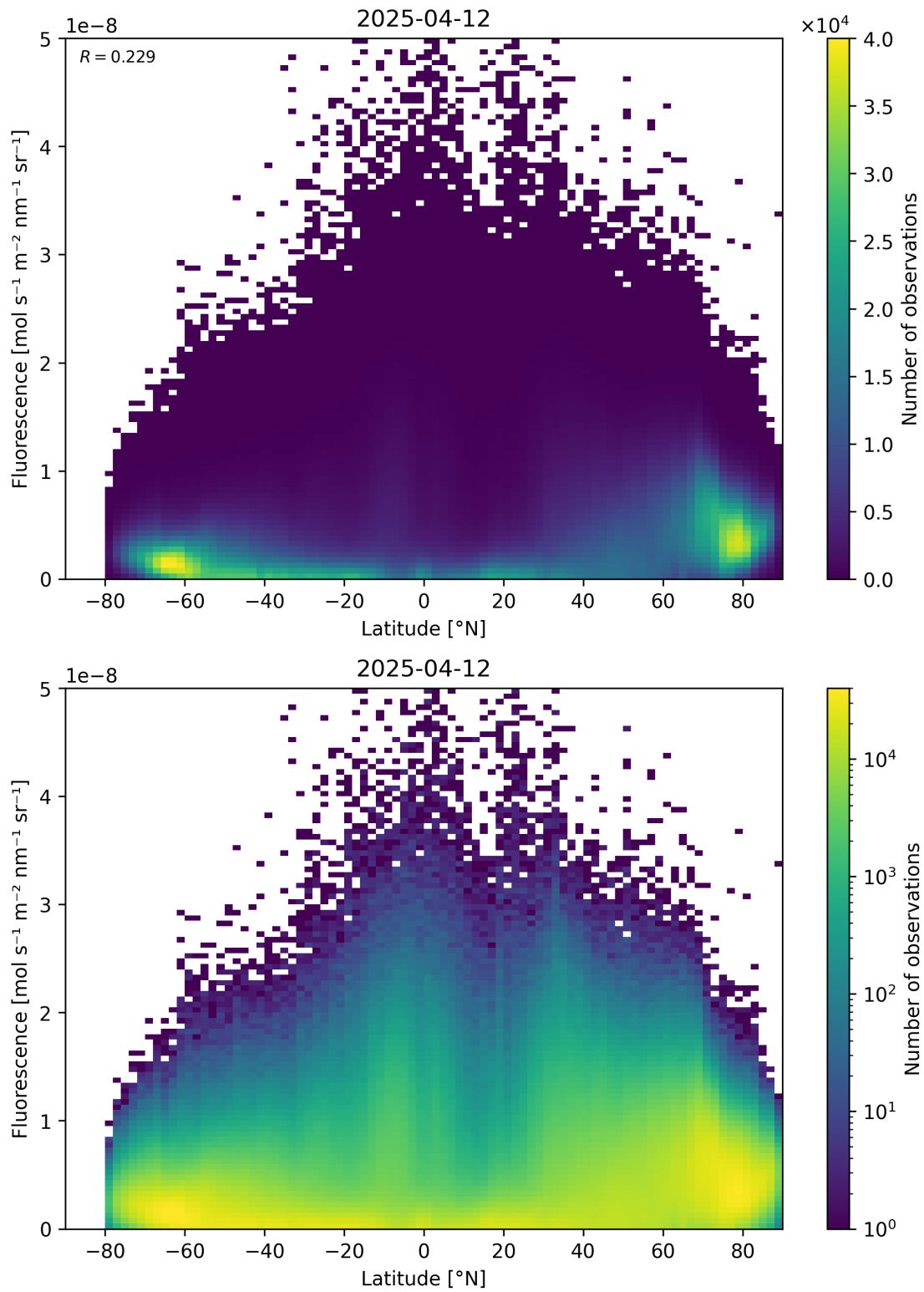
Figure 92: Scatter density plot of “Latitude” against “Fluorescence” for 2025-04-11 to 2025-04-13.
