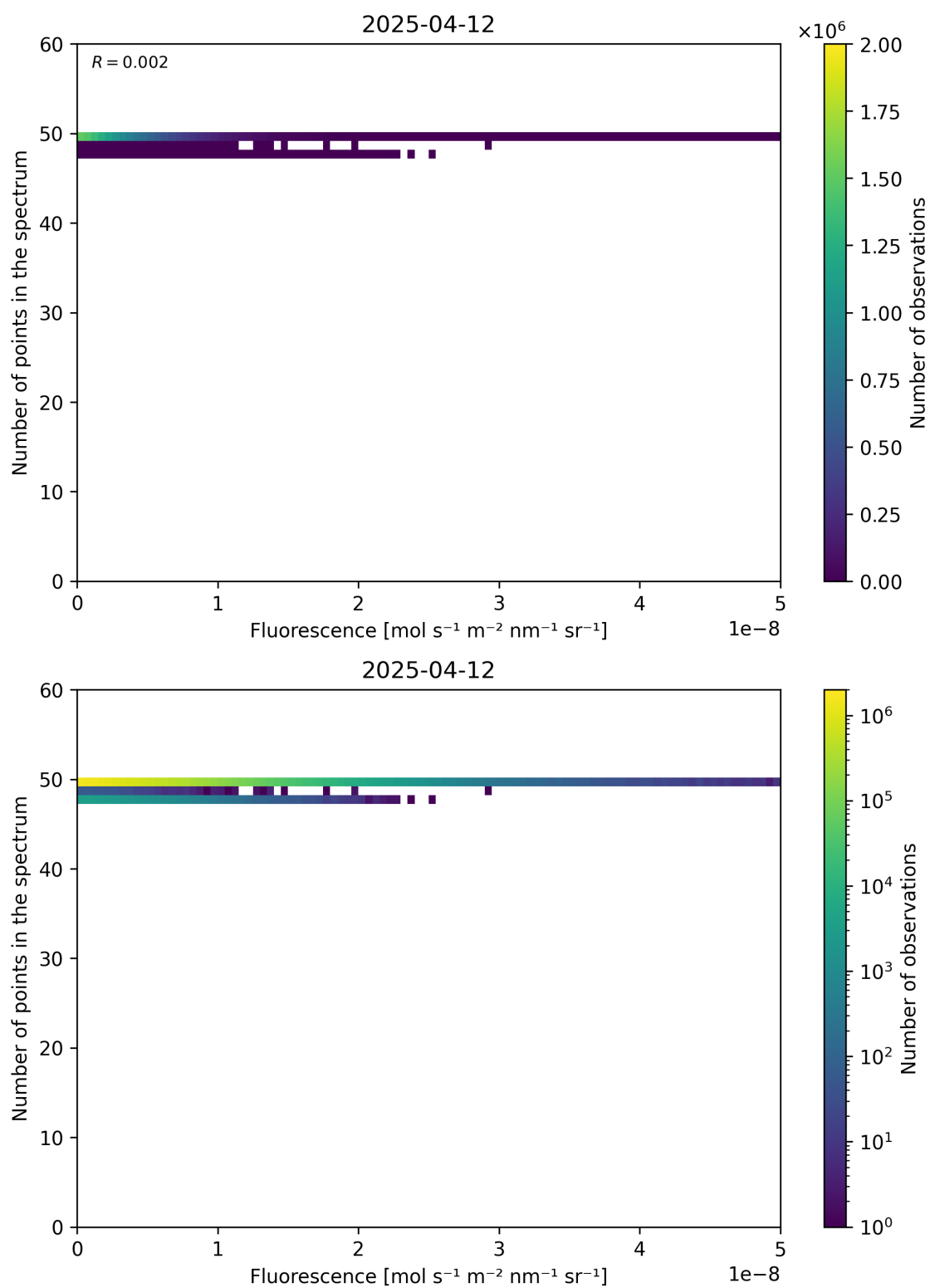
Figure 86: Scatter density plot of “Fluorescence” against “Number of points in the spectrum” for 2025-04-11 to 2025-04-13.
