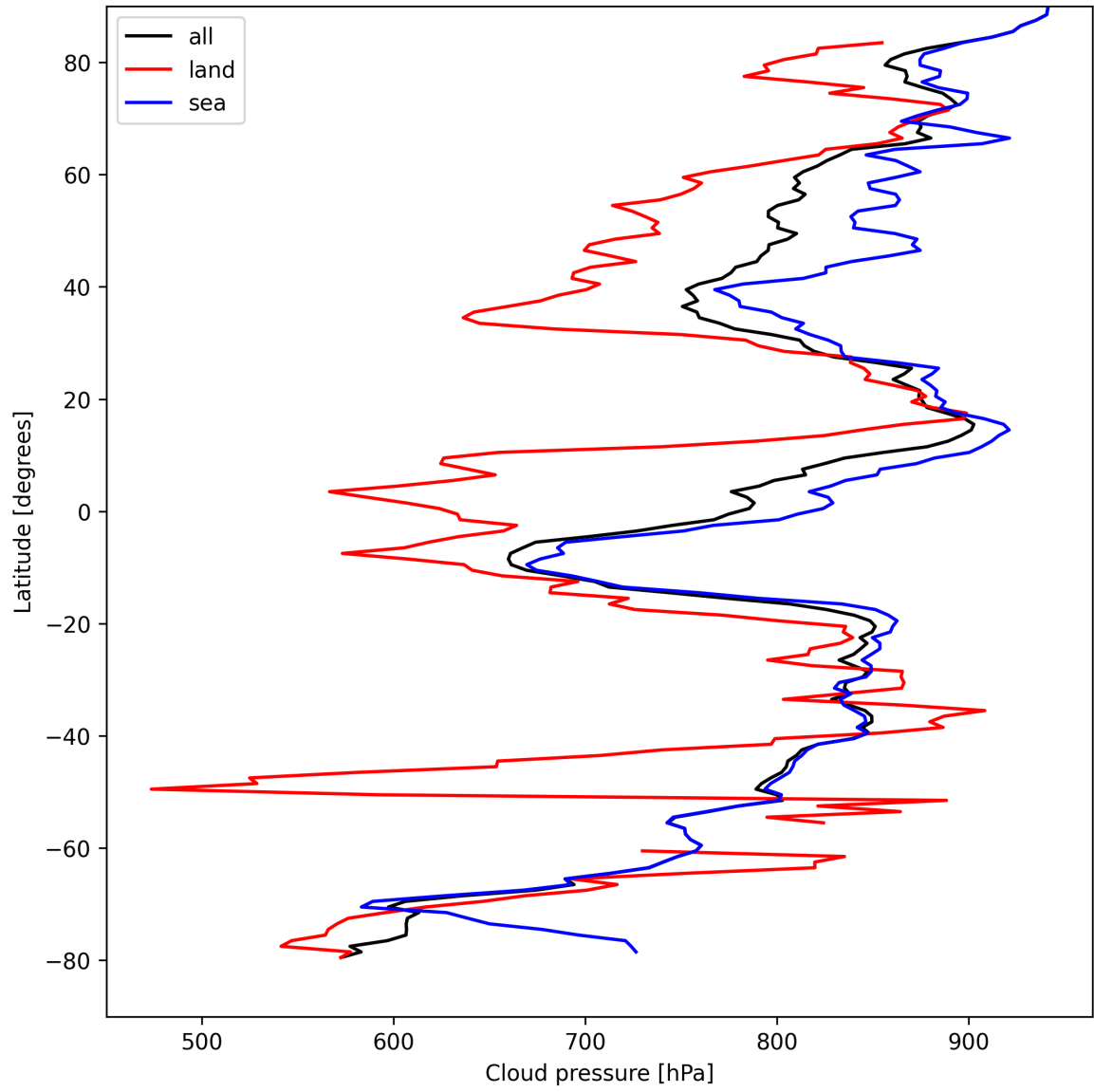
Figure 13: Zonal average of “Cloud pressure” for 2025-04-11 to 2025-04-13.
