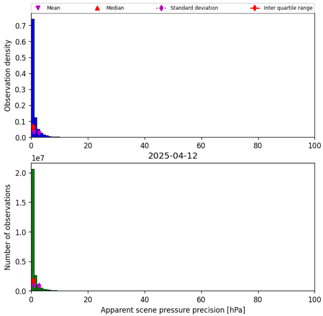
Figure 37: Histogram of “Apparent scene pressure precision” for 2025-04-11 to 2025-04-13
