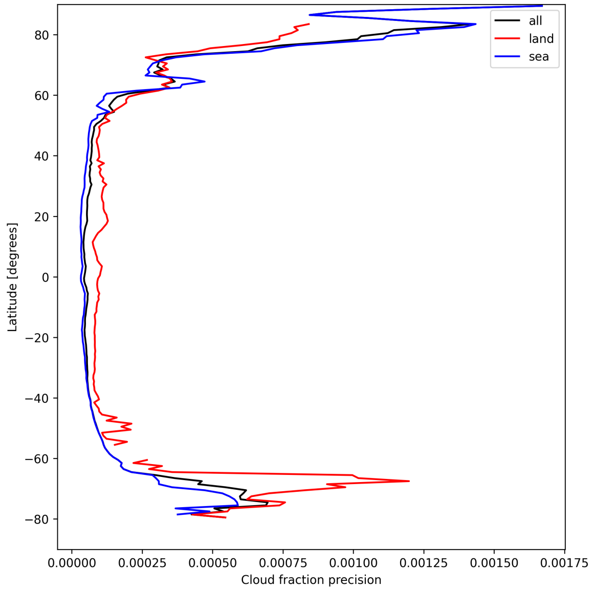
Figure 16: Zonal average of “Cloud fraction precision” for 2025-04-11 to 2025-04-13.
