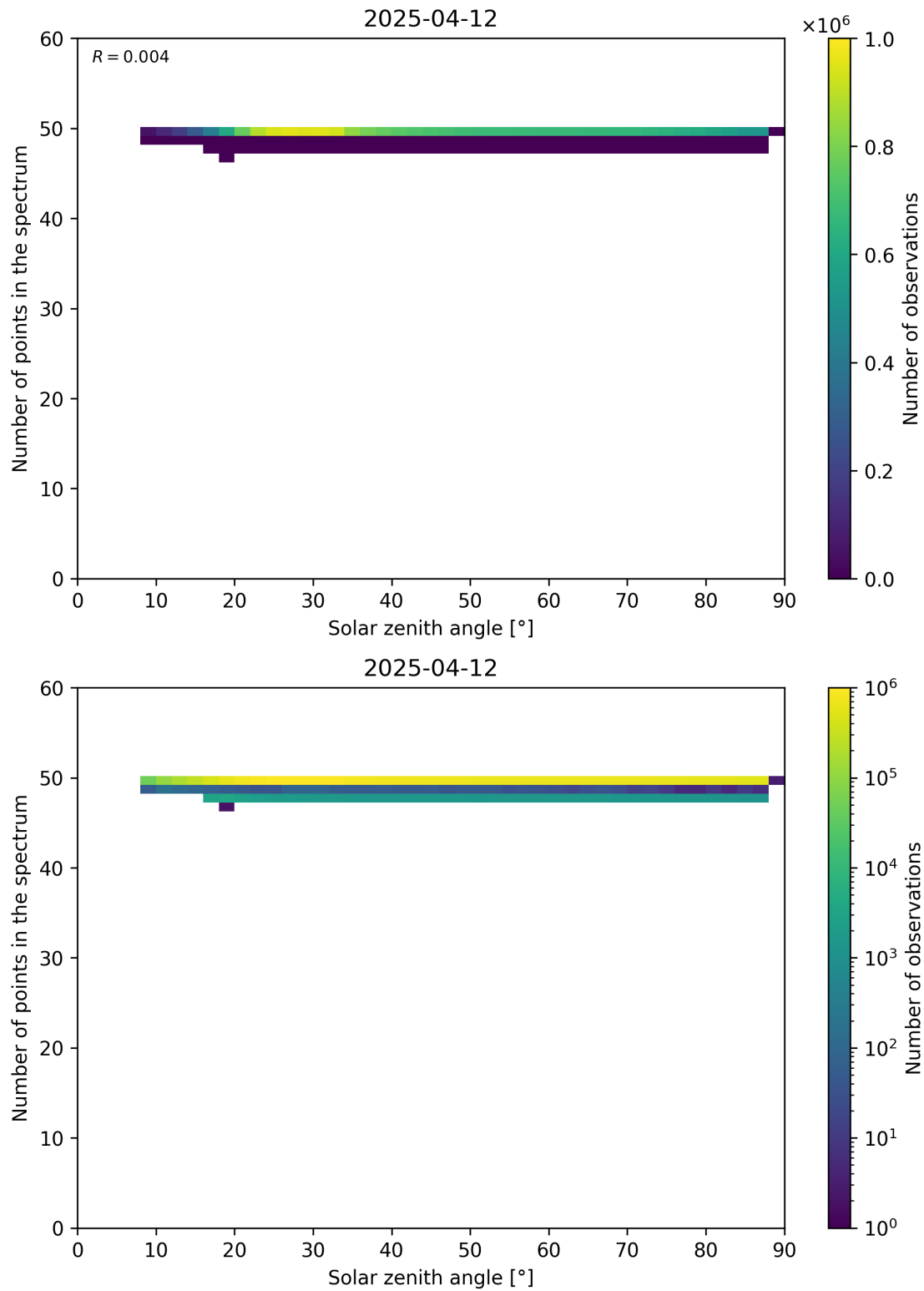
Figure 115: Scatter density plot of “Solar zenith angle” against “Number of points in the spectrum” for 2025-04-11 to 2025-04-13.
