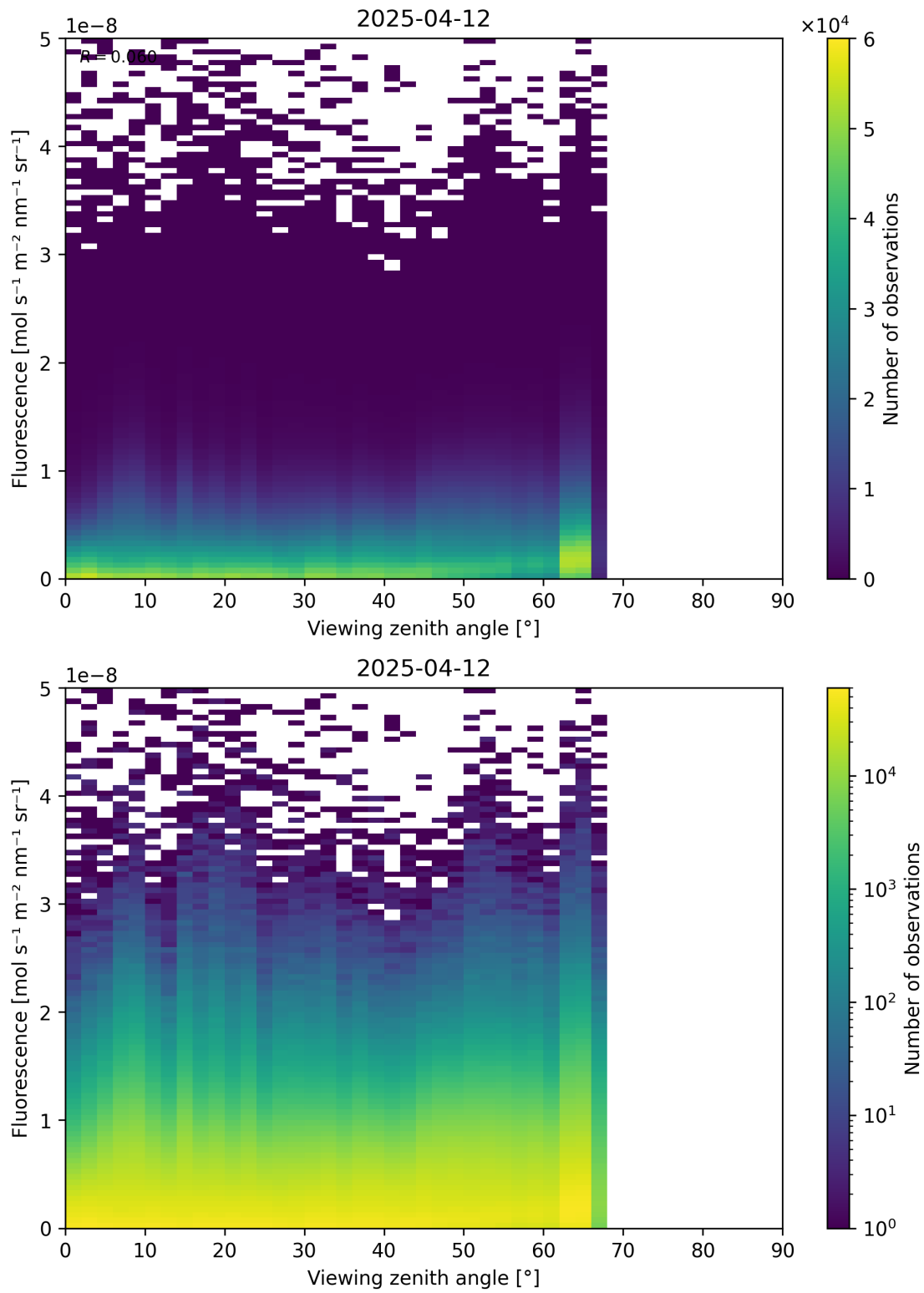
Figure 122: Scatter density plot of “Viewing zenith angle” against “Fluorescence” for 2025-04-11 to 2025-04-13.
