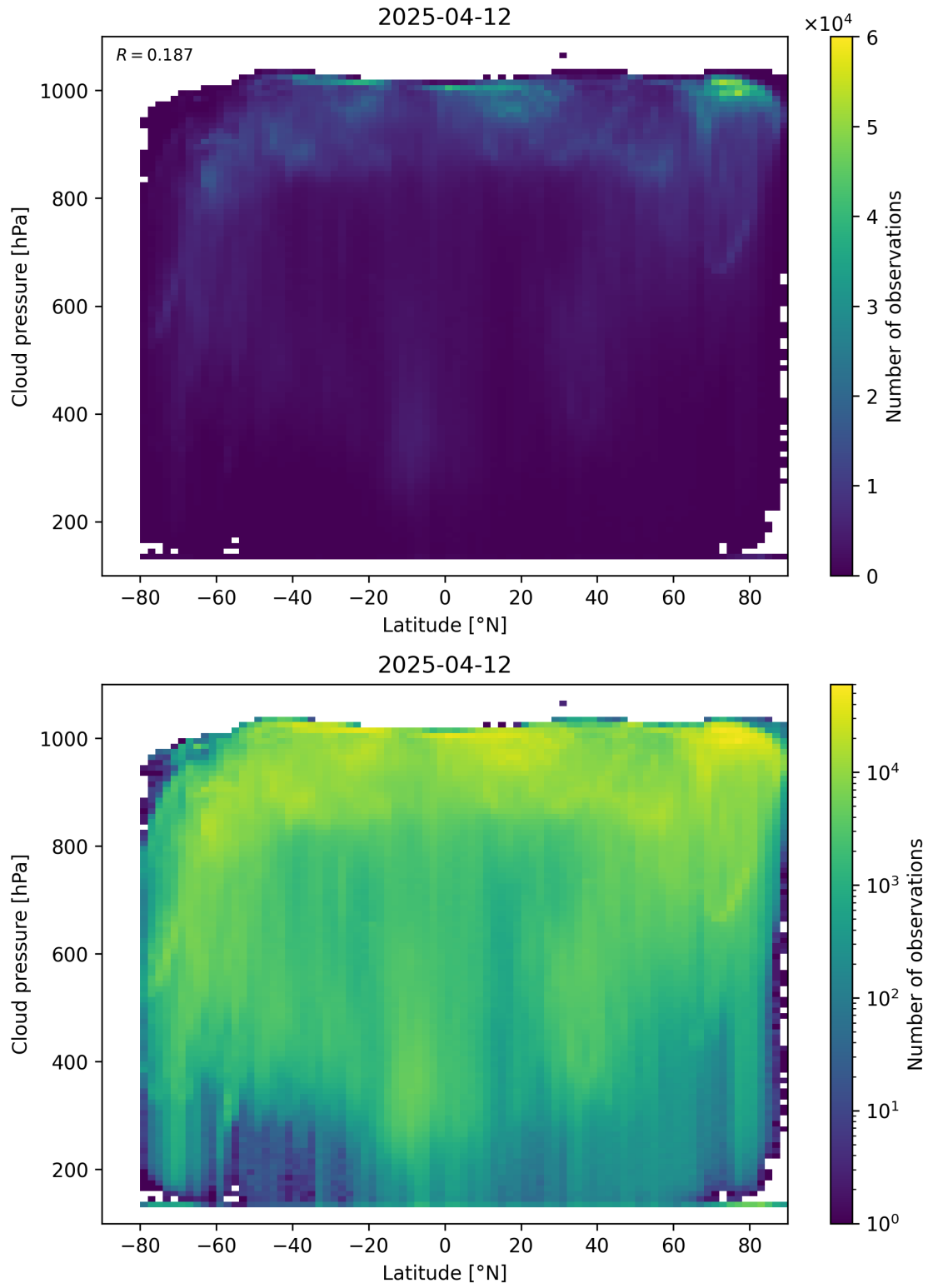
Figure 91: Scatter density plot of “Latitude” against “Cloud pressure” for 2025-04-11 to 2025-04-13.
