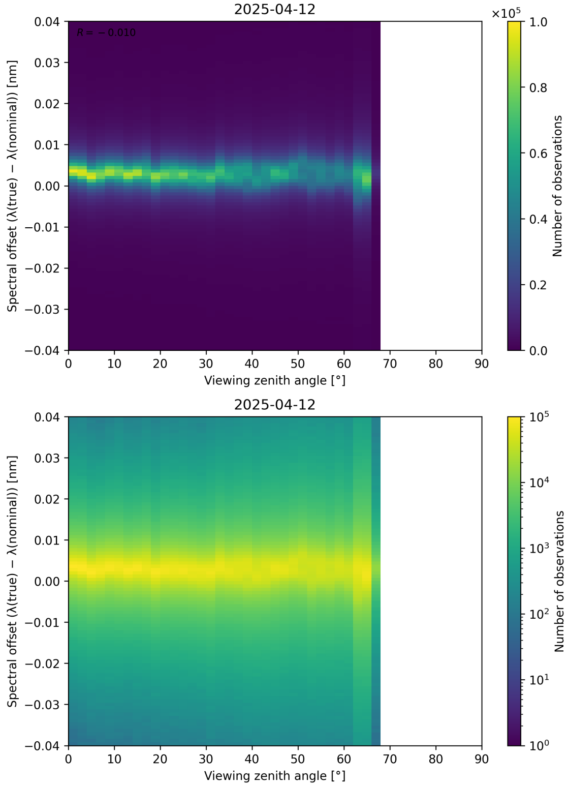
Figure 128: Scatter density plot of “Viewing zenith angle” against “Spectral offset ( \lambda_{\text{true}} - \lambda_{\text{nominal}} )” for 2025-04-11 to 2025-04-13.
