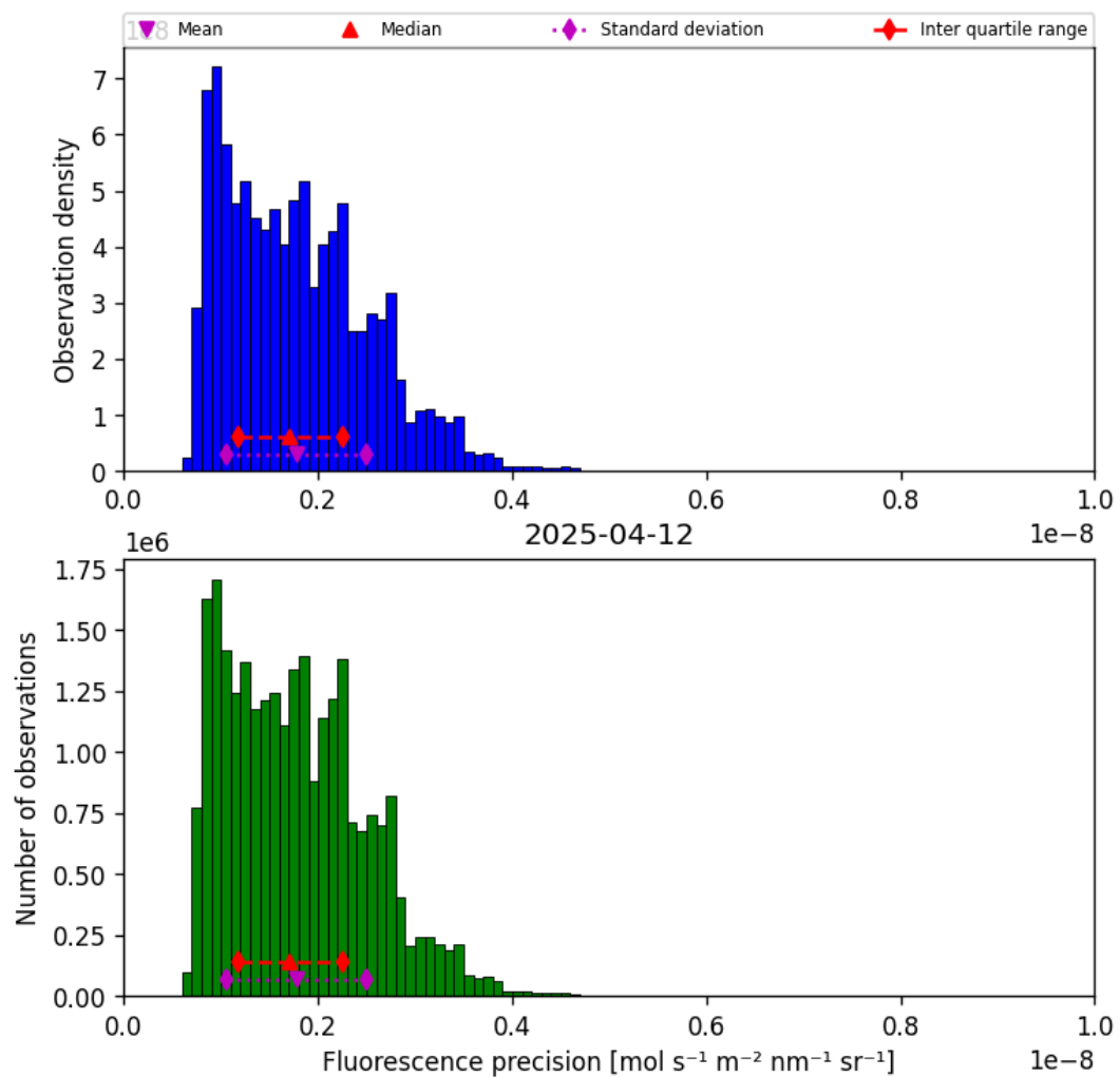
Figure 41: Histogram of “Fluorescence precision” for 2025-04-11 to 2025-04-13
