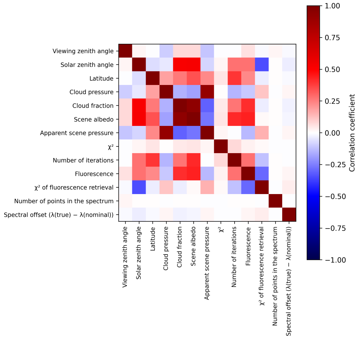
Figure 2: Map of correlation matrix for 2025-04-11 to 2025-04-13.
