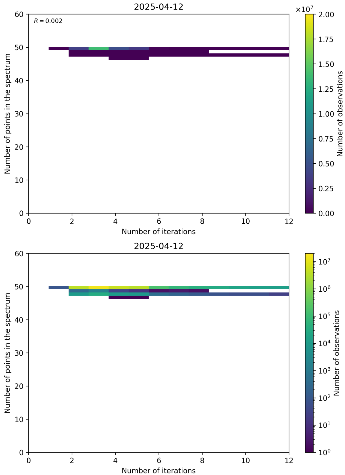
Figure 99: Scatter density plot of “Number of iterations” against “Number of points in the spectrum” for 2025-04-11 to 2025-04-13.
