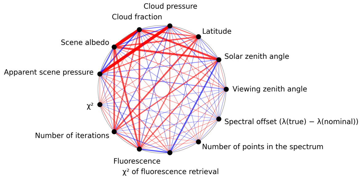
Figure 1: Map of correlation graph for 2025-04-11 to 2025-04-13.
