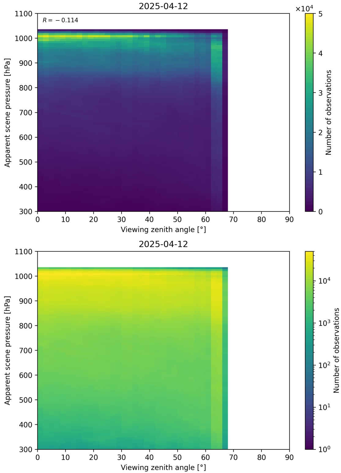
Figure 118: Scatter density plot of “Viewing zenith angle” against “Apparent scene pressure” for 2025-04-11 to 2025-04-13.
