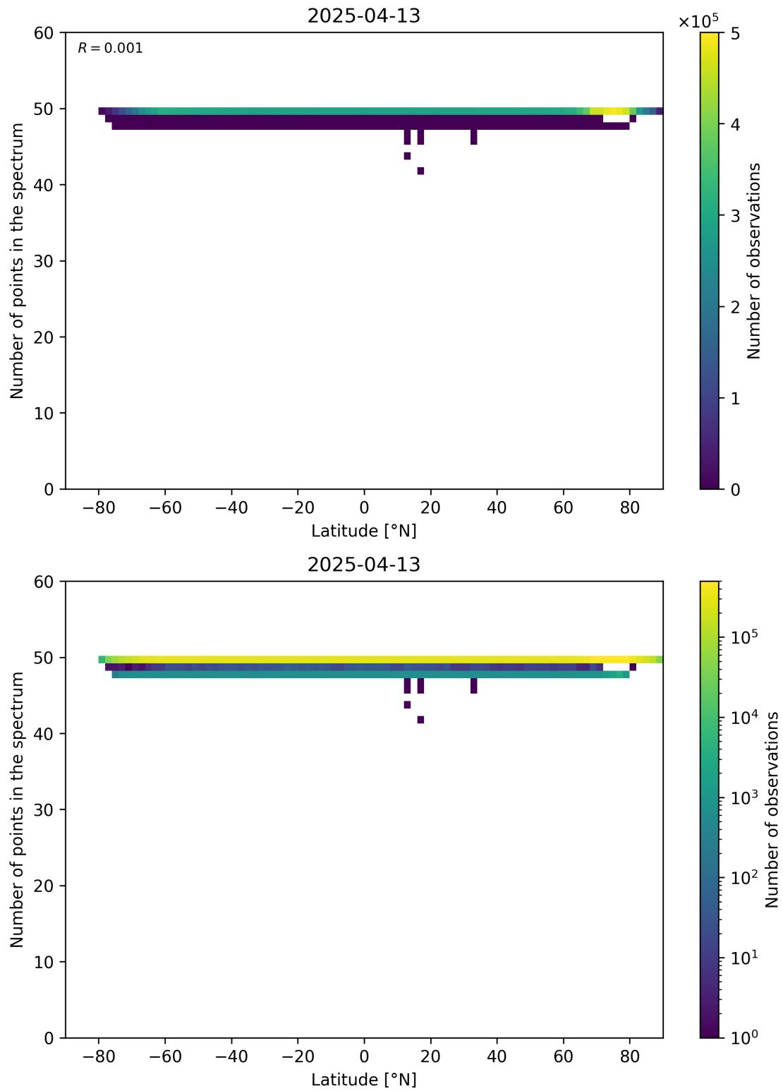
Figure 94: Scatter density plot of “Latitude” against “Number of points in the spectrum” for 2025-04-13 to 2025-04-14.
