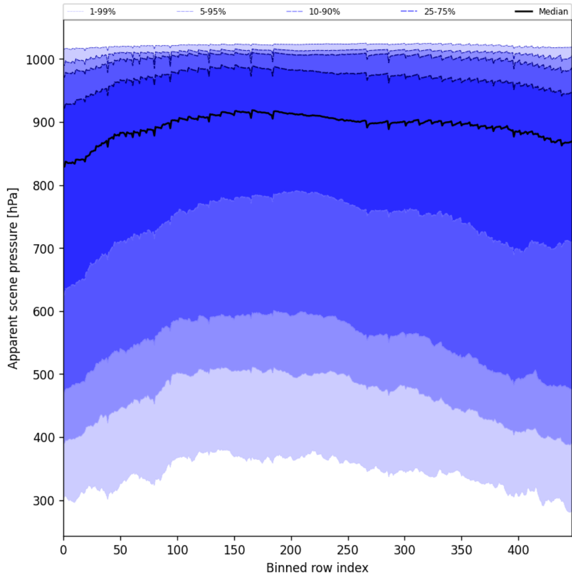
Figure 53: Along track statistics of “Apparent scene pressure” for 2025-04-13 to 2025-04-14
