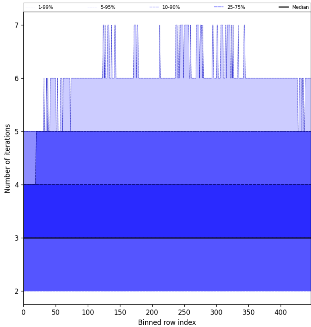
Figure 56: Along track statistics of “Number of iterations” for 2025-04-13 to 2025-04-14
