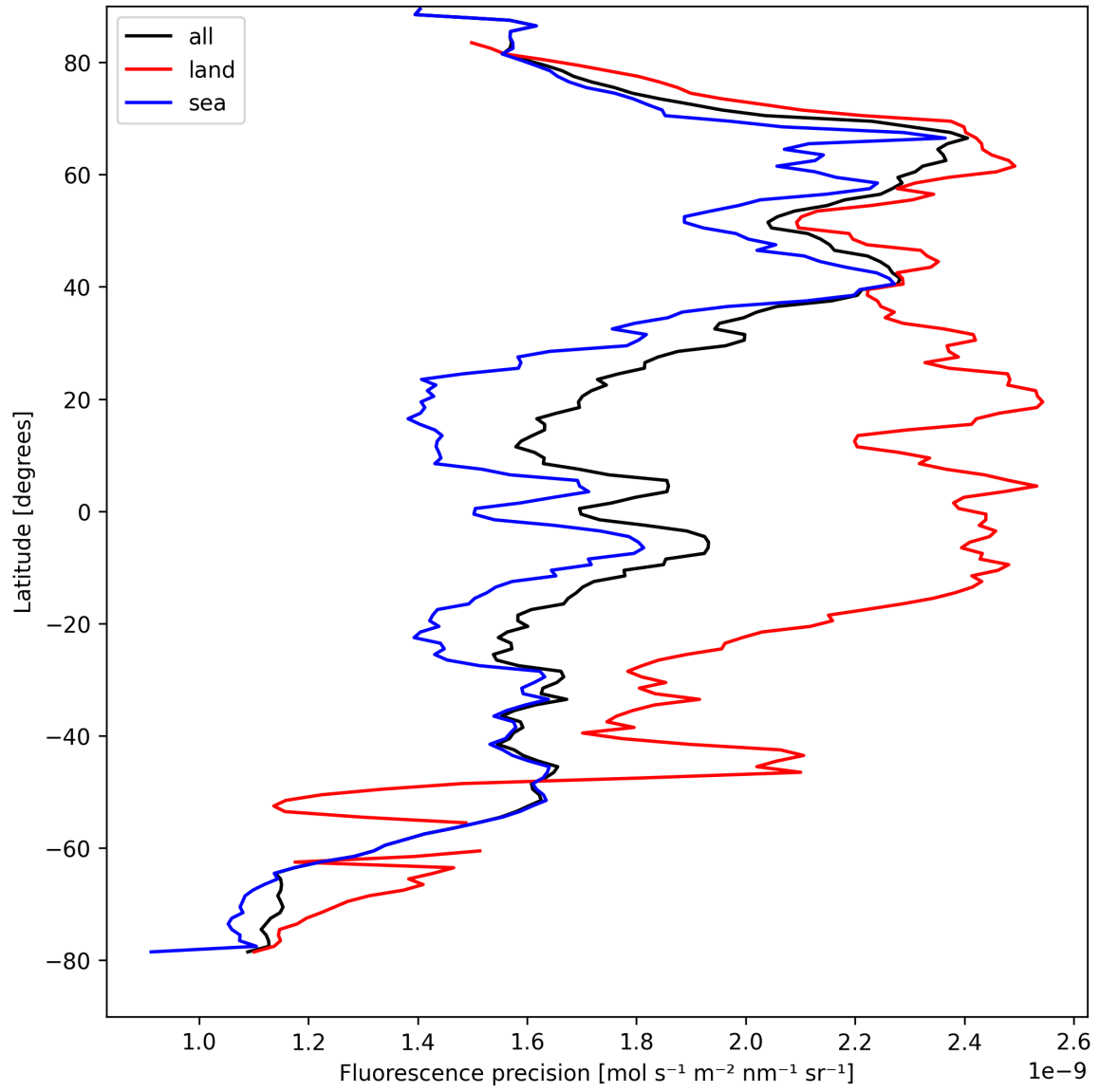
Figure 24: Zonal average of “Fluorescence precision” for 2025-04-13 to 2025-04-14.
