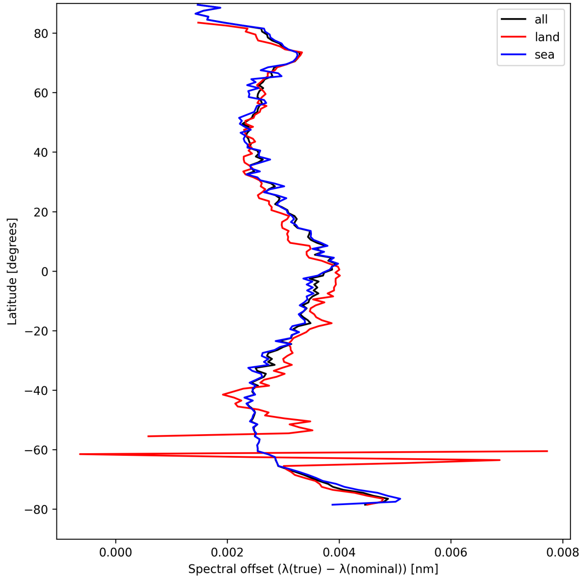
Figure 28: Zonal average of “Spectral offset ( \lambda_{\text{true}} - \lambda_{\text{nominal}} )” for 2025-04-13 to 2025-04-14.
