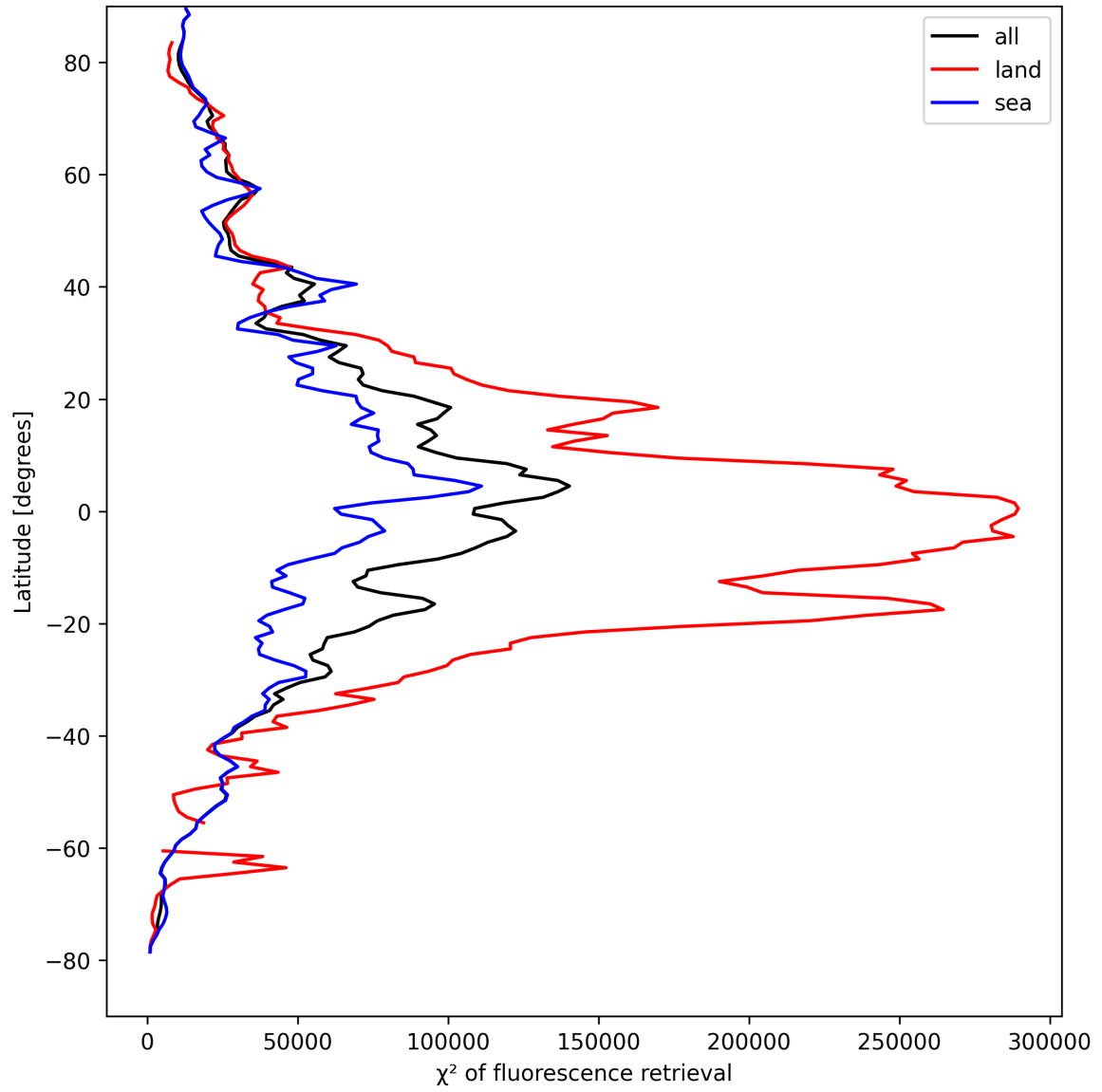
Figure 25: Zonal average of “ \chi^2 of fluorescence retrieval” for 2025-04-13 to 2025-04-14.
