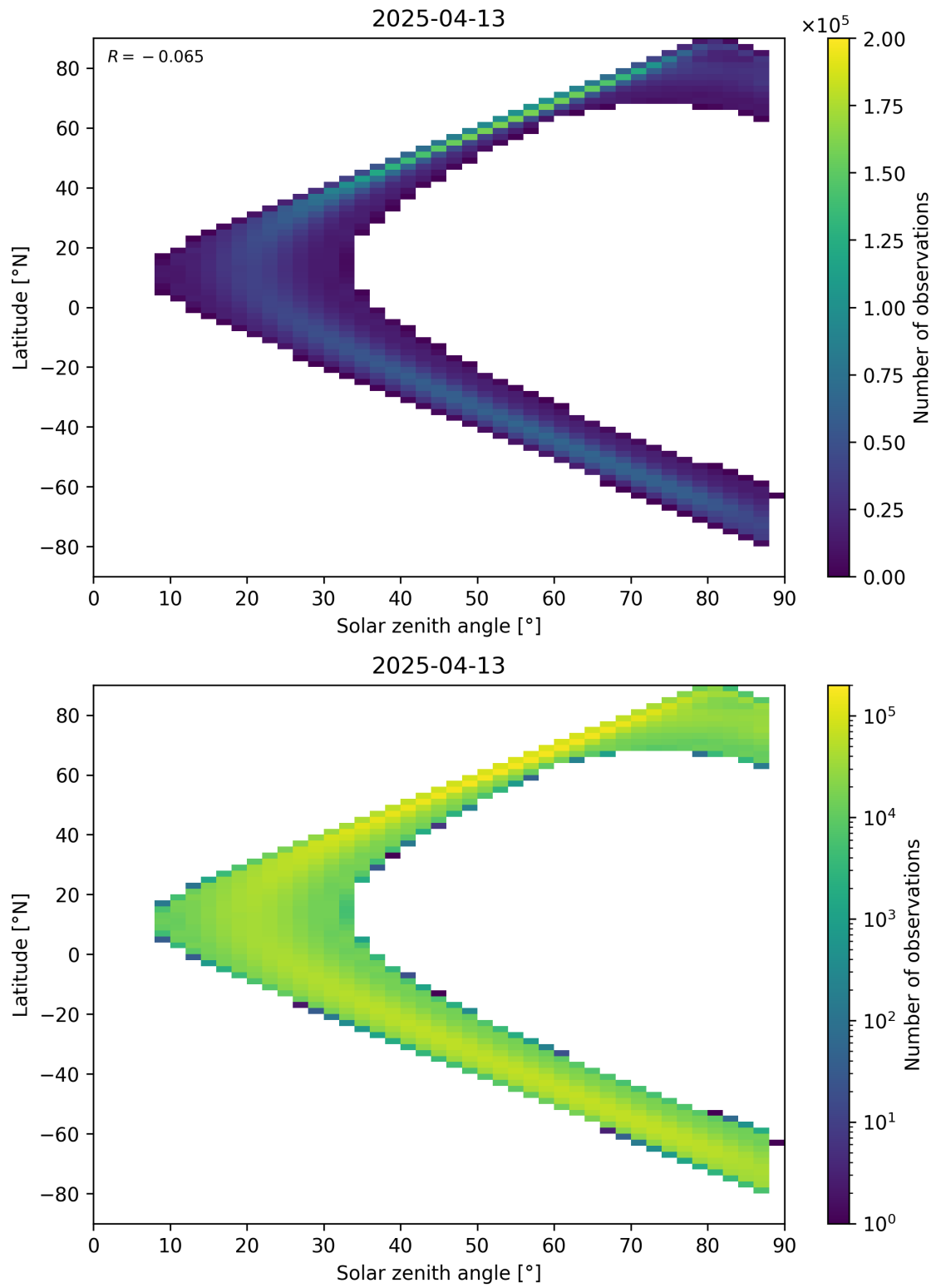
Figure 113: Scatter density plot of “Solar zenith angle” against “Latitude” for 2025-04-13 to 2025-04-14.
