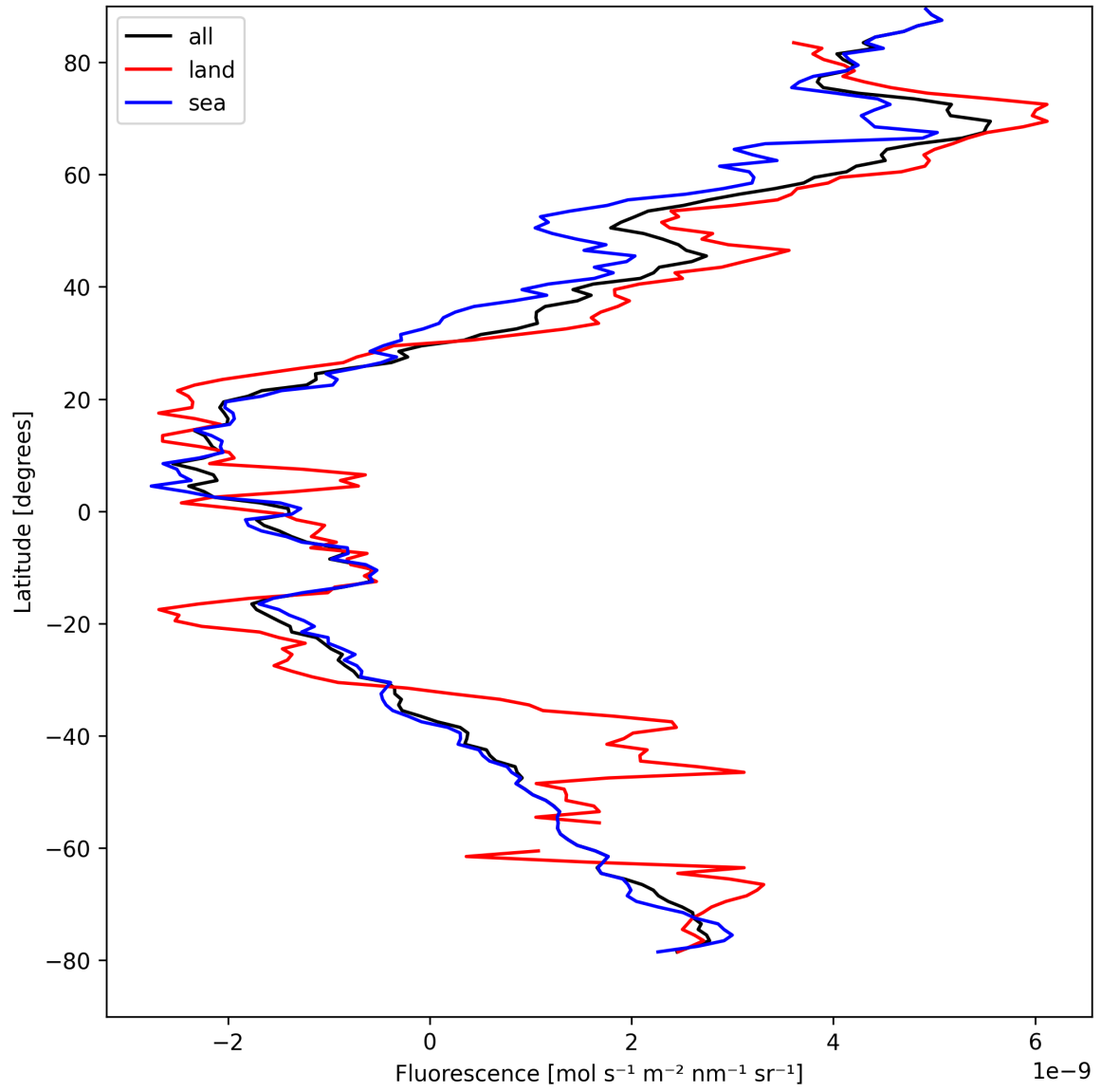
Figure 23: Zonal average of “Fluorescence” for 2025-04-13 to 2025-04-14.
