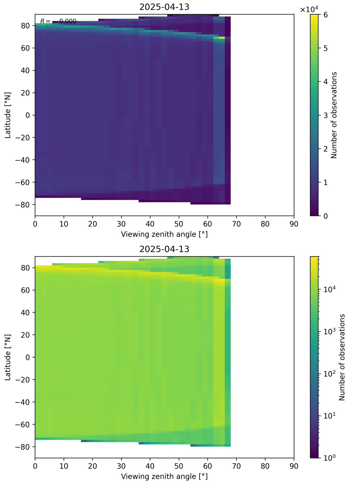
Figure 123: Scatter density plot of “Viewing zenith angle” against “Latitude” for 2025-04-13 to 2025-04-14.
