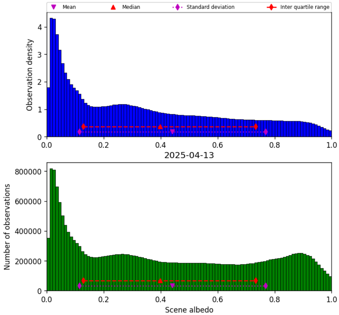
Figure 34: Histogram of “Scene albedo” for 2025-04-13 to 2025-04-14
