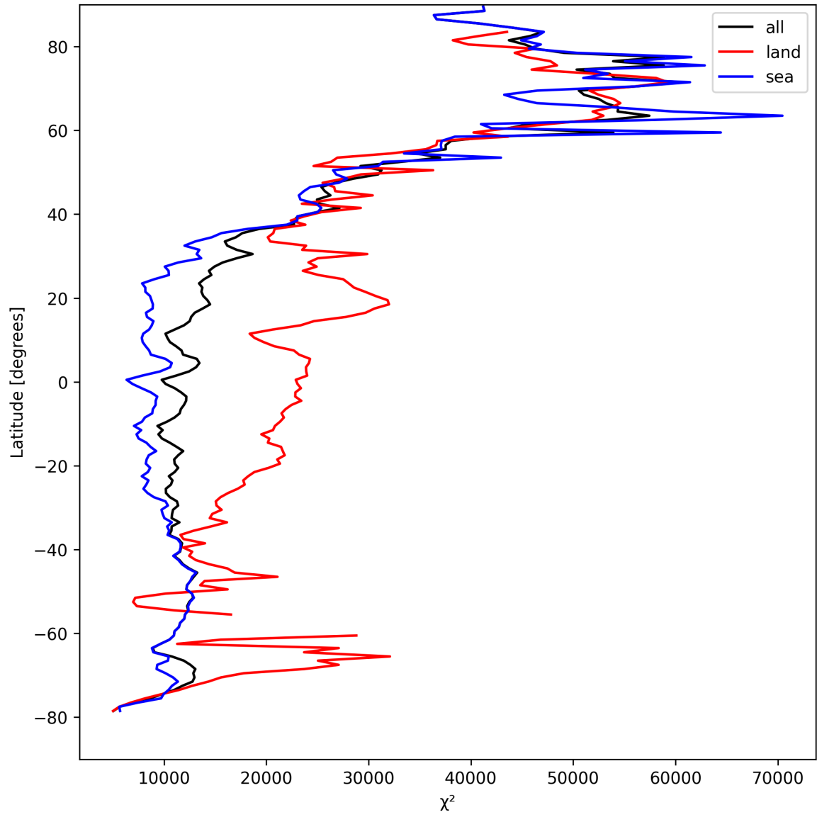
Figure 21: Zonal average of “ \chi^2 ” for 2025-04-13 to 2025-04-14.
