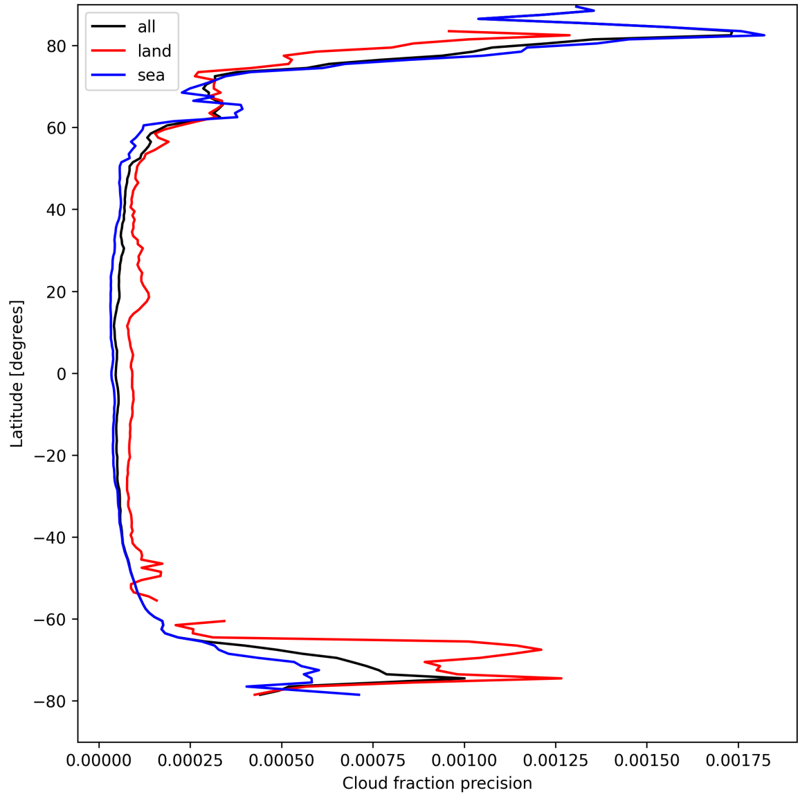
Figure 16: Zonal average of “Cloud fraction precision” for 2025-04-13 to 2025-04-14.
