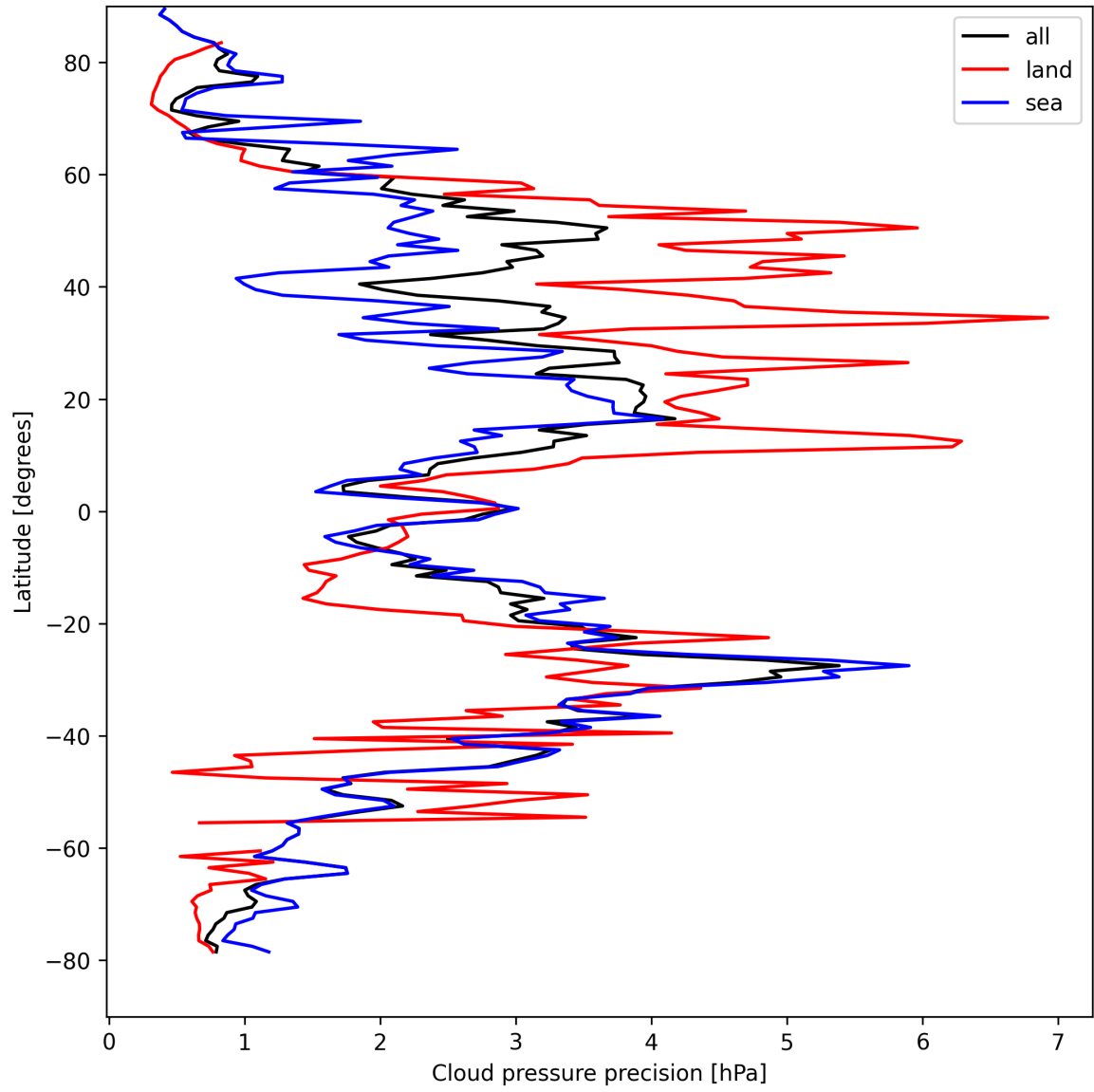
Figure 14: Zonal average of “Cloud pressure precision” for 2025-04-13 to 2025-04-14.
