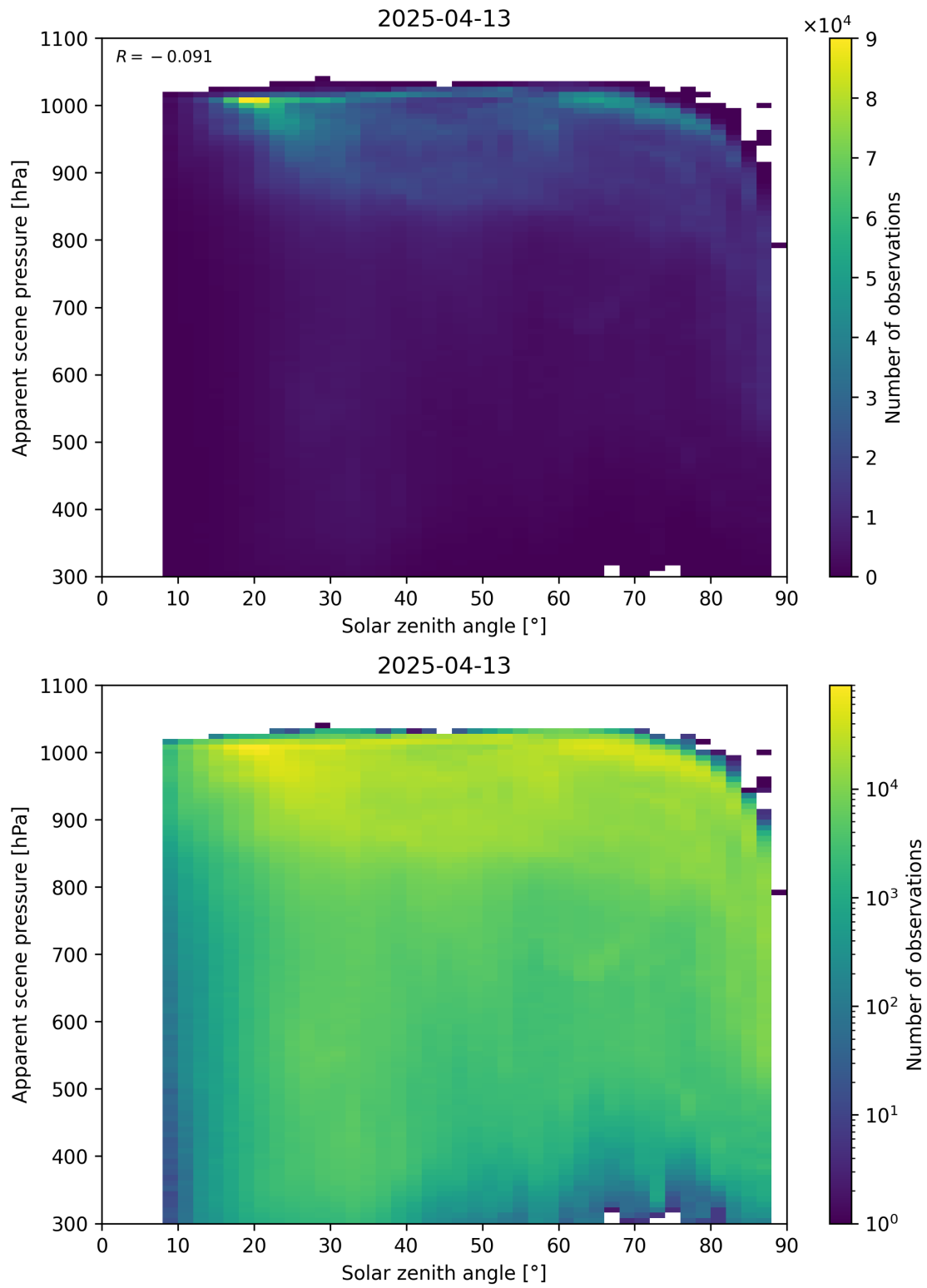
Figure 108: Scatter density plot of “Solar zenith angle” against “Apparent scene pressure” for 2025-04-13 to 2025-04-14.
