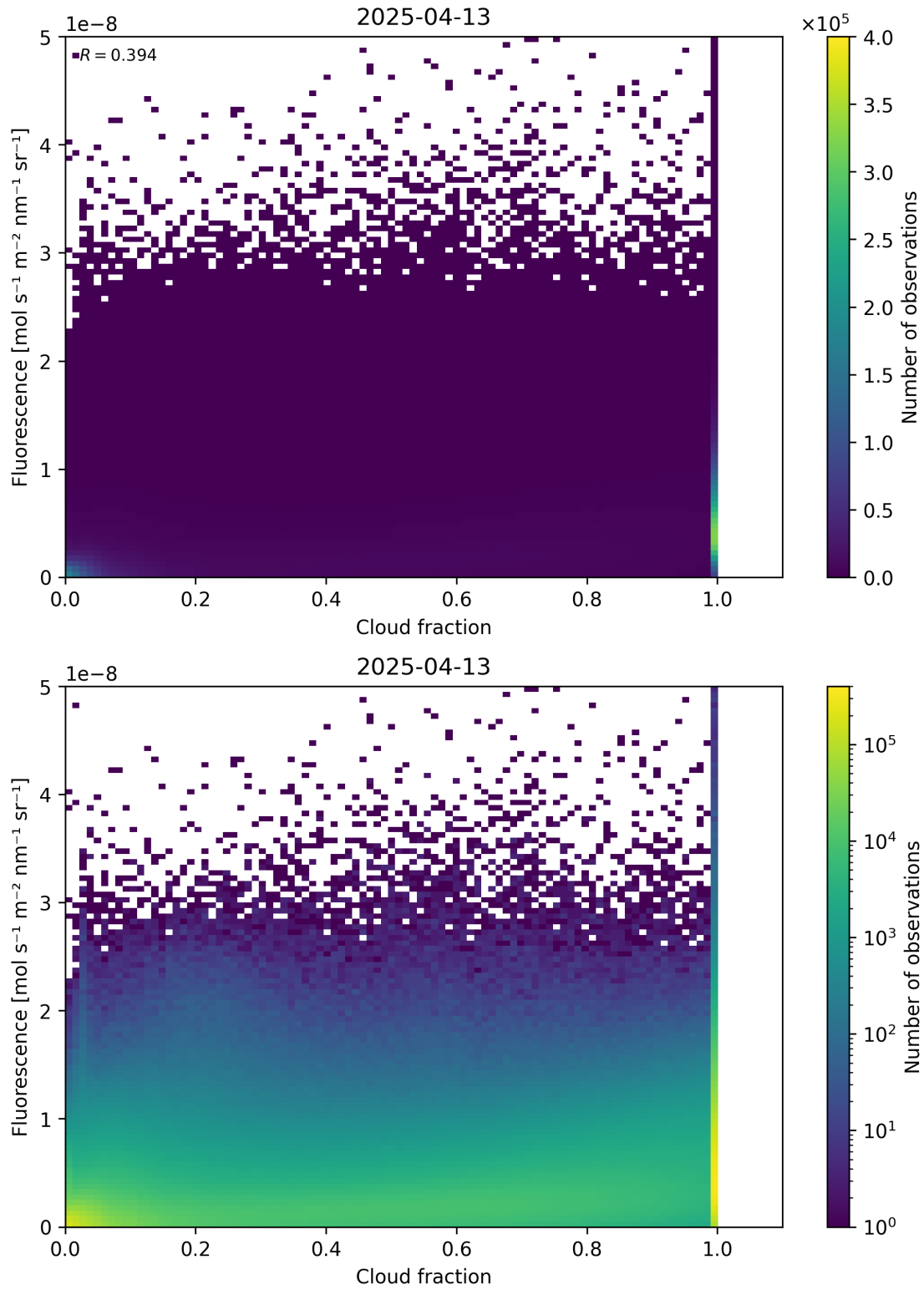
Figure 72: Scatter density plot of “Cloud fraction” against “Fluorescence” for 2025-04-13 to 2025-04-14.
