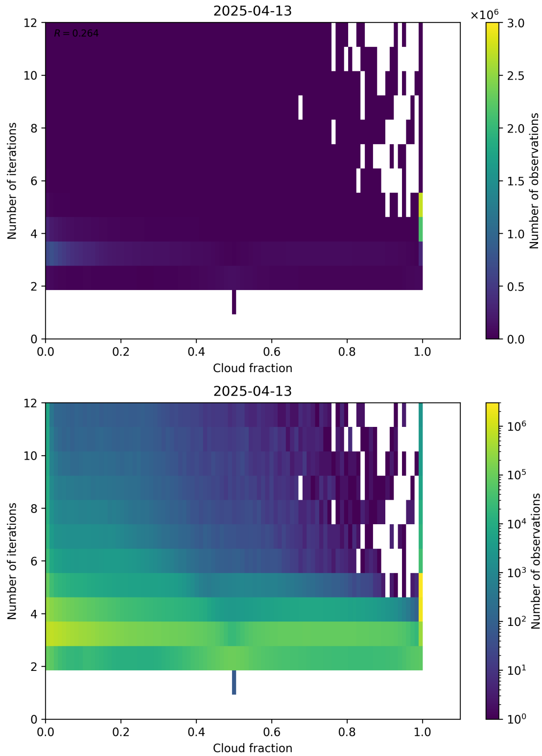
Figure 73: Scatter density plot of “Cloud fraction” against “Number of iterations” for 2025-04-13 to 2025-04-14.
