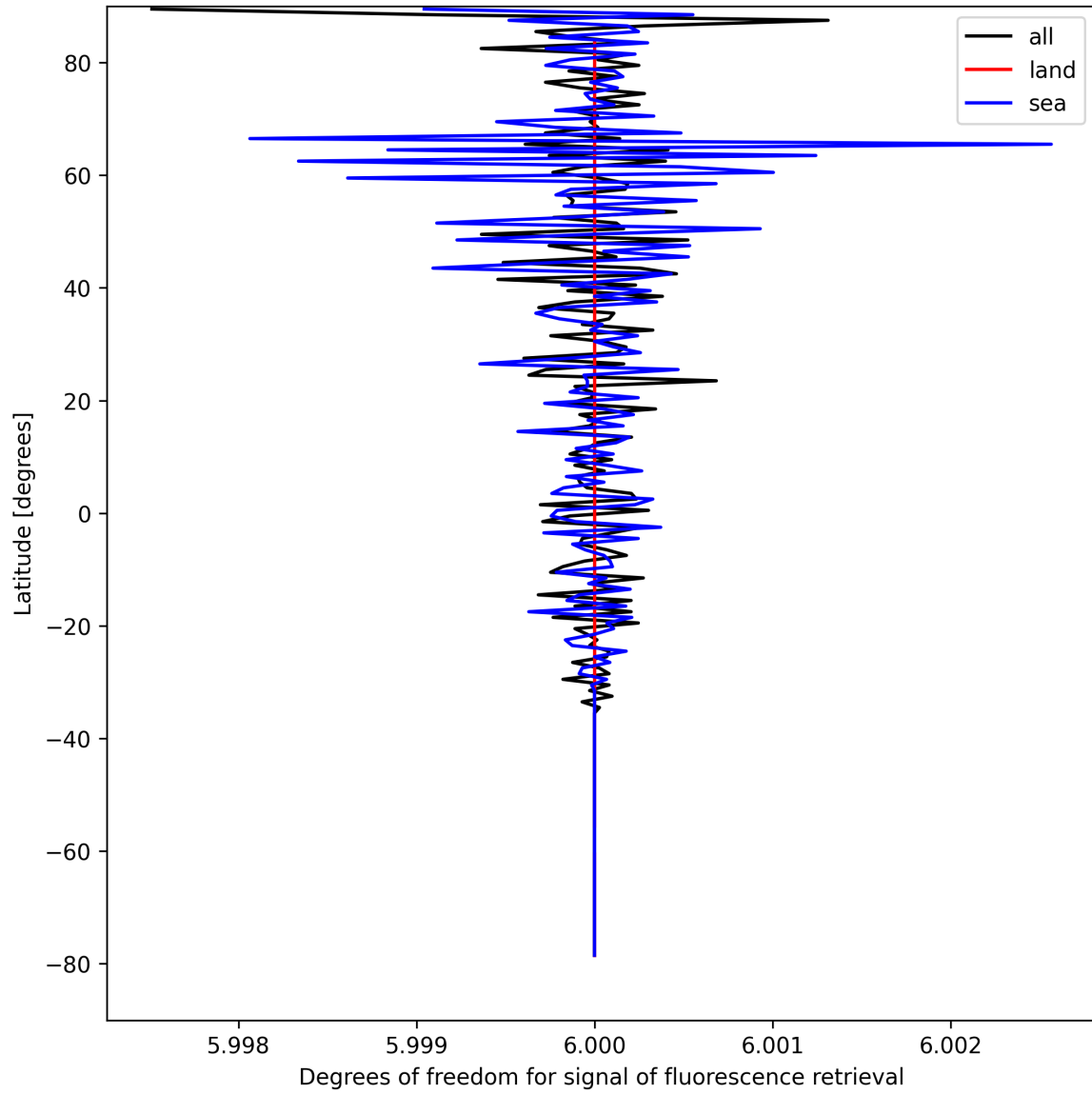
Figure 26: Zonal average of “Degrees of freedom for signal of fluorescence retrieval” for 2025-04-13 to 2025-04-14.
