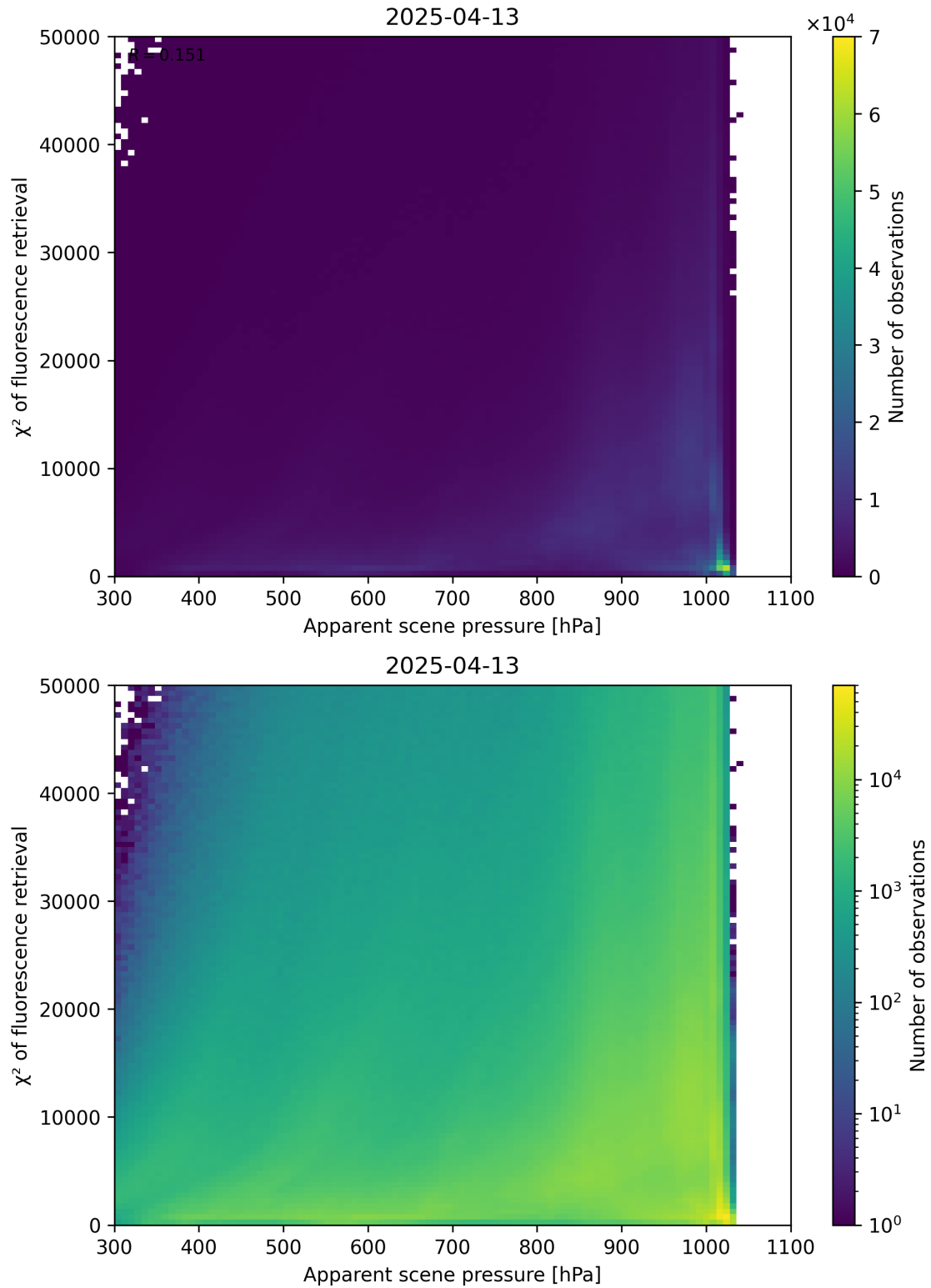
Figure 63: Scatter density plot of “Apparent scene pressure” against “ \chi^2 of fluorescence retrieval” for 2025-04-13 to 2025-04-14.
