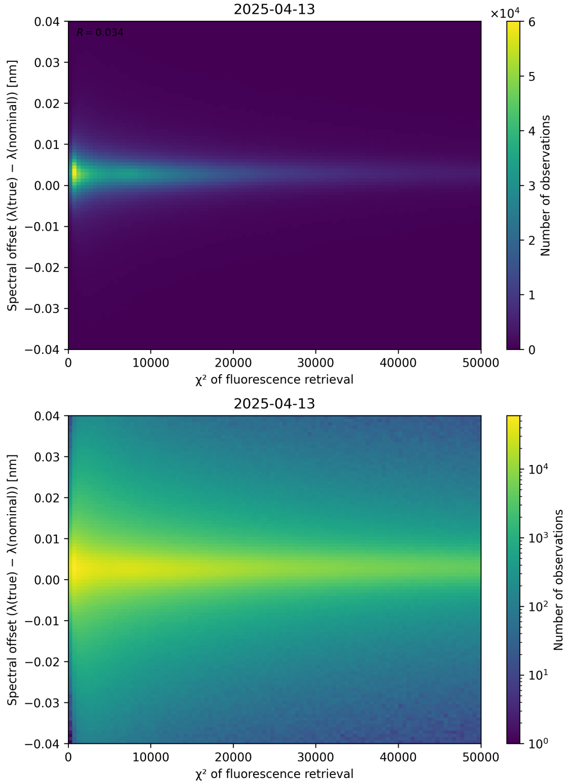
Figure 69: Scatter density plot of “ \chi^2 of fluorescence retrieval” against “Spectral offset ( \lambda_{\text{true}} - \lambda_{\text{nominal}} )” for 2025-04-13 to 2025-04-14.
