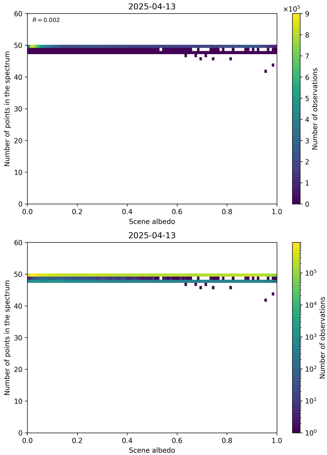
Figure 106: Scatter density plot of “Scene albedo” against “Number of points in the spectrum” for 2025-04-13 to 2025-04-14.
