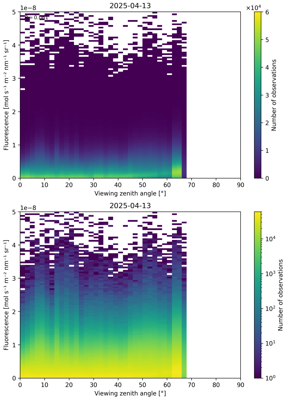
Figure 122: Scatter density plot of “Viewing zenith angle” against “Fluorescence” for 2025-04-13 to 2025-04-14.
