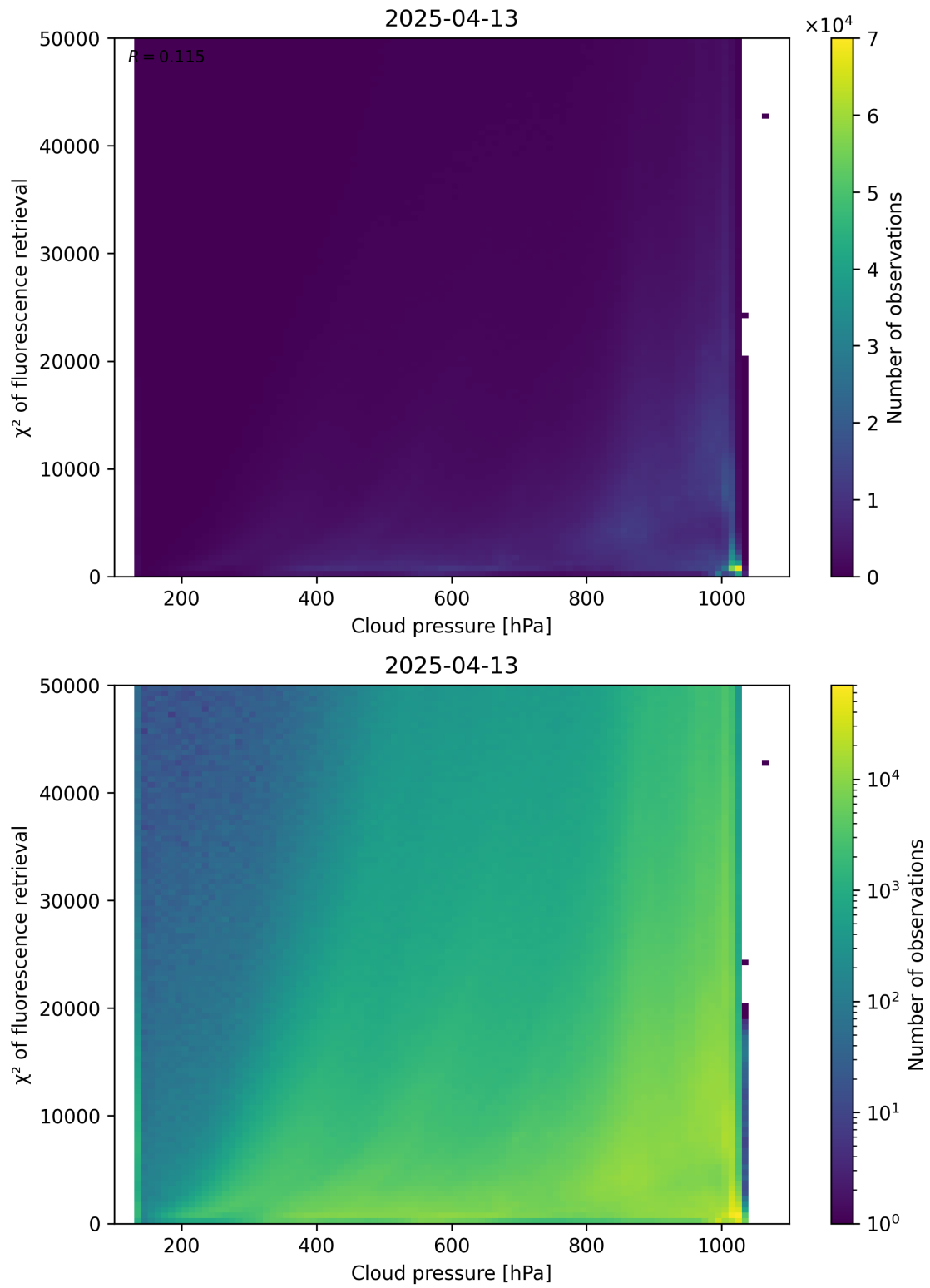
Figure 78: Scatter density plot of “Cloud pressure” against “ \chi^2 of fluorescence retrieval” for 2025-04-13 to 2025-04-14.
