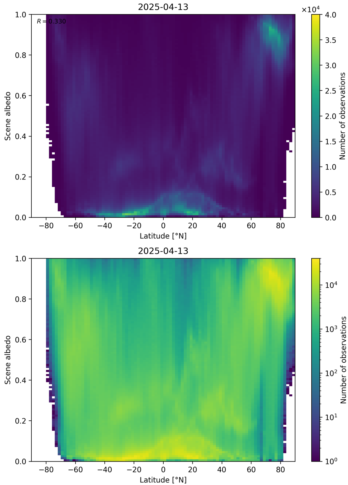
Figure 95: Scatter density plot of “Latitude” against “Scene albedo” for 2025-04-13 to 2025-04-14.
