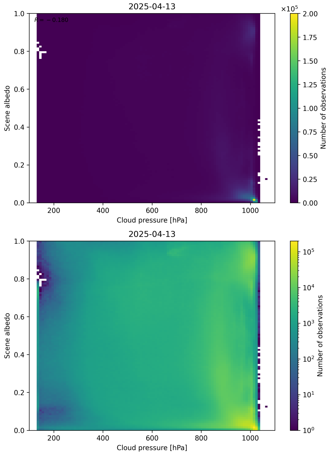
Figure 83: Scatter density plot of “Cloud pressure” against “Scene albedo” for 2025-04-13 to 2025-04-14.
