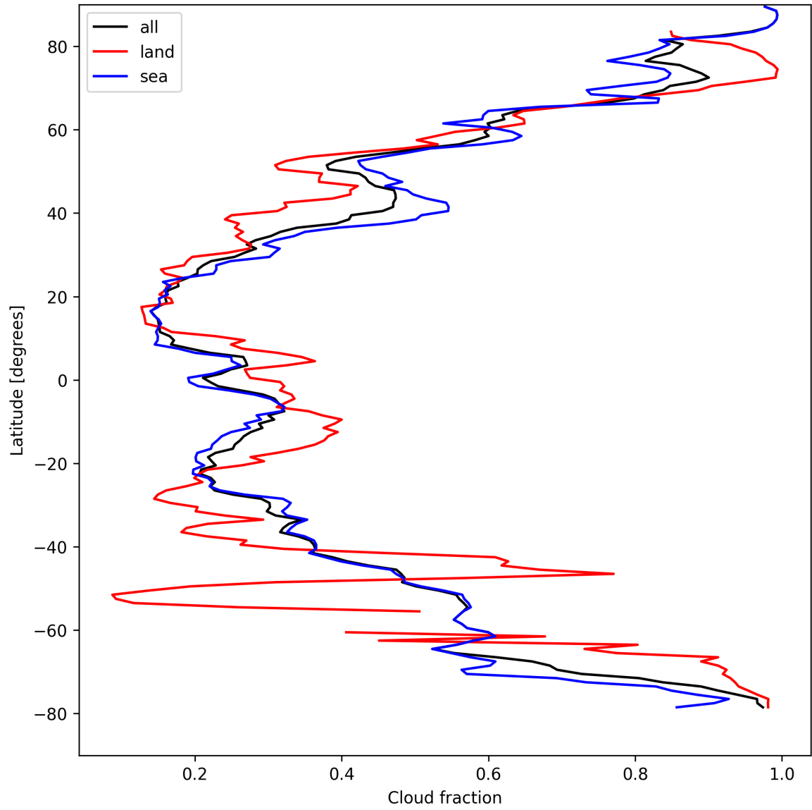
Figure 15: Zonal average of “Cloud fraction” for 2025-04-13 to 2025-04-14.
