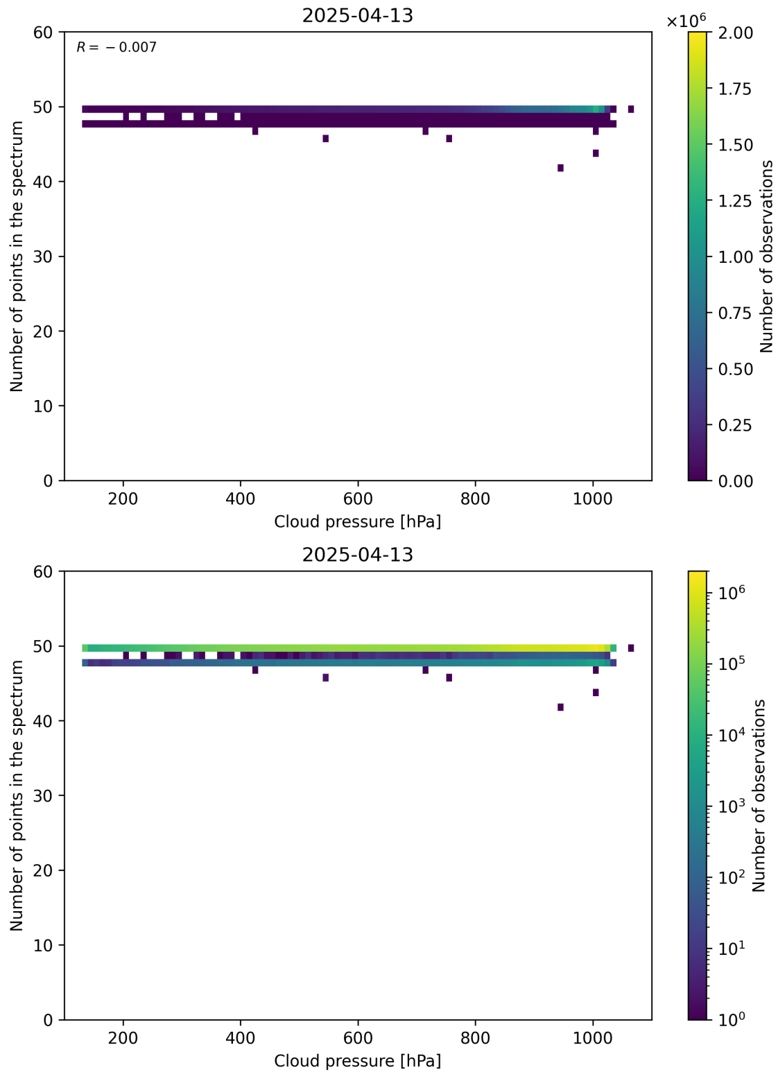
Figure 82: Scatter density plot of “Cloud pressure” against “Number of points in the spectrum” for 2025-04-13 to 2025-04-14.
