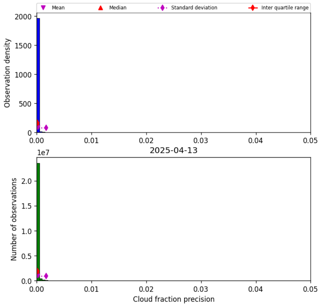
Figure 33: Histogram of “Cloud fraction precision” for 2025-04-13 to 2025-04-14
