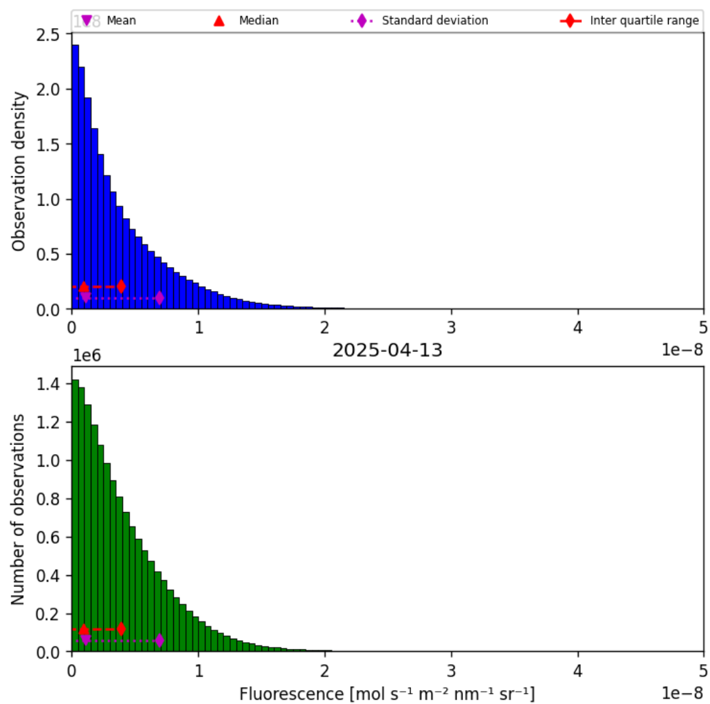
Figure 40: Histogram of “Fluorescence” for 2025-04-13 to 2025-04-14
