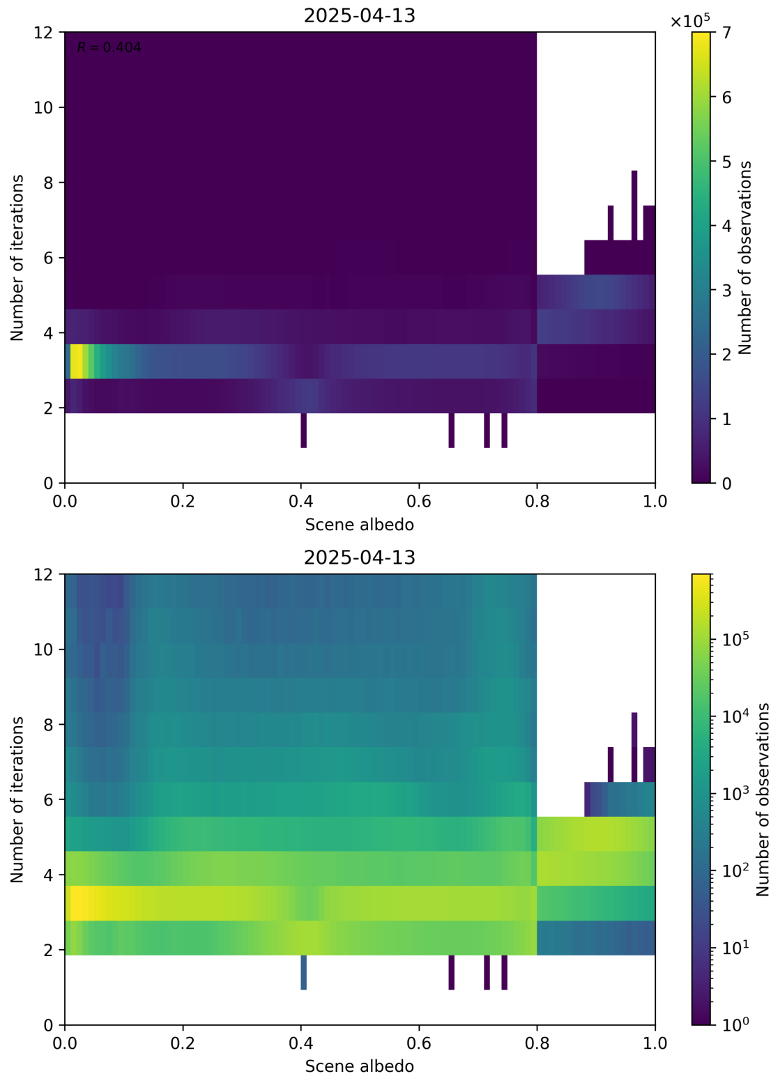
Figure 105: Scatter density plot of “Scene albedo” against “Number of iterations” for 2025-04-13 to 2025-04-14.
