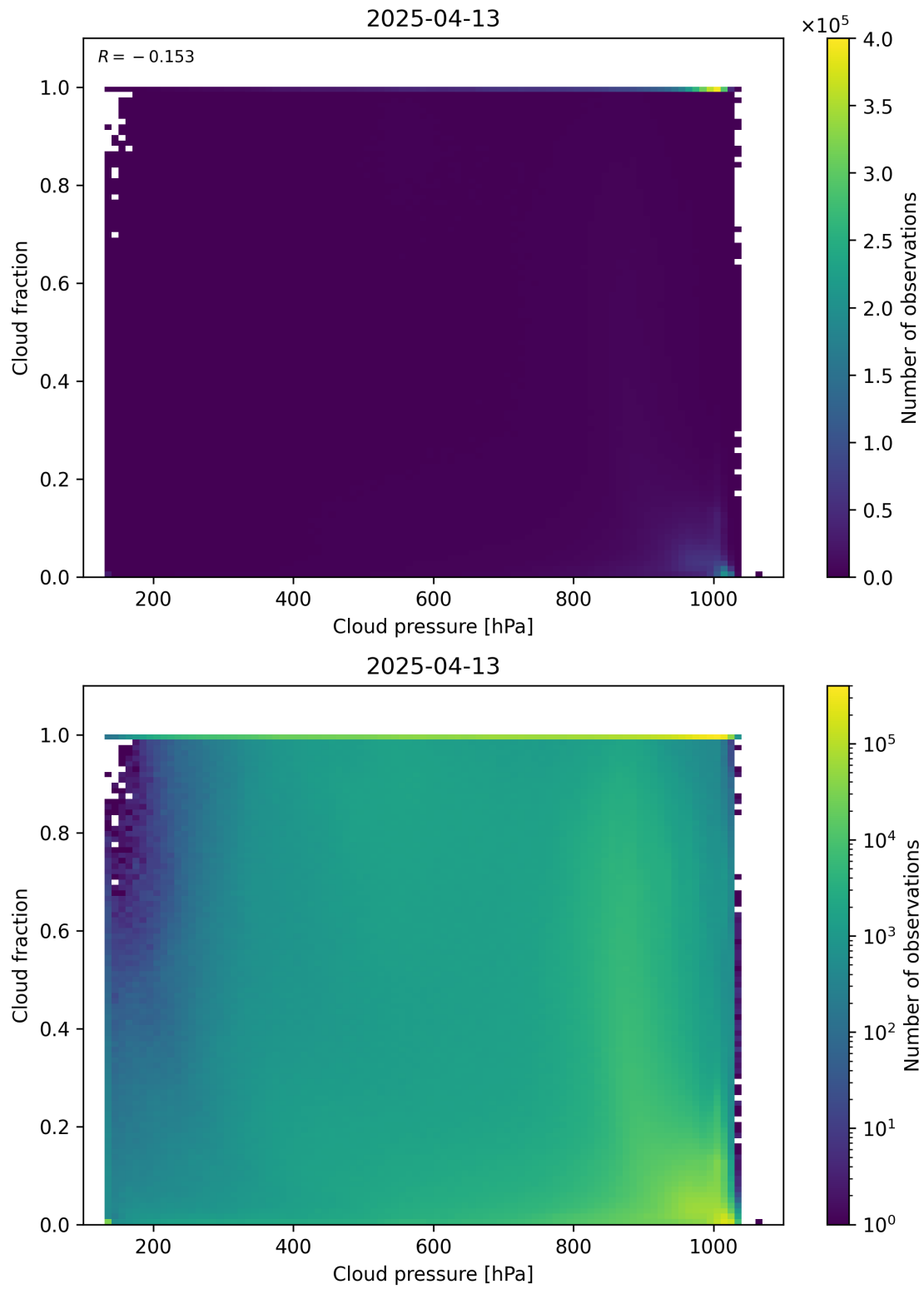
Figure 79: Scatter density plot of “Cloud pressure” against “Cloud fraction” for 2025-04-13 to 2025-04-14.
