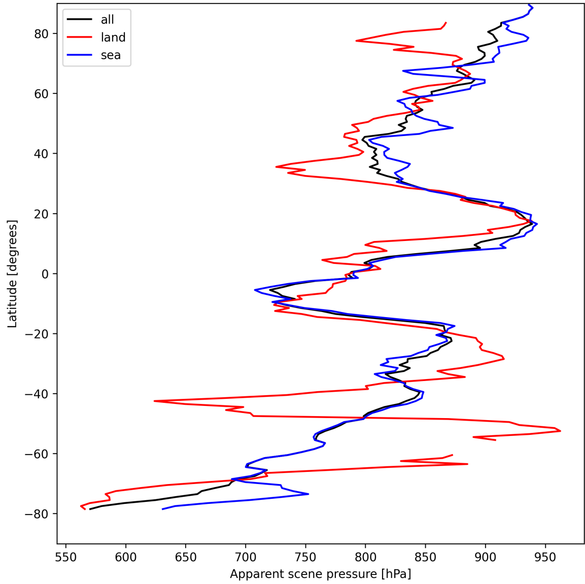
Figure 19: Zonal average of “Apparent scene pressure” for 2025-04-13 to 2025-04-14.
