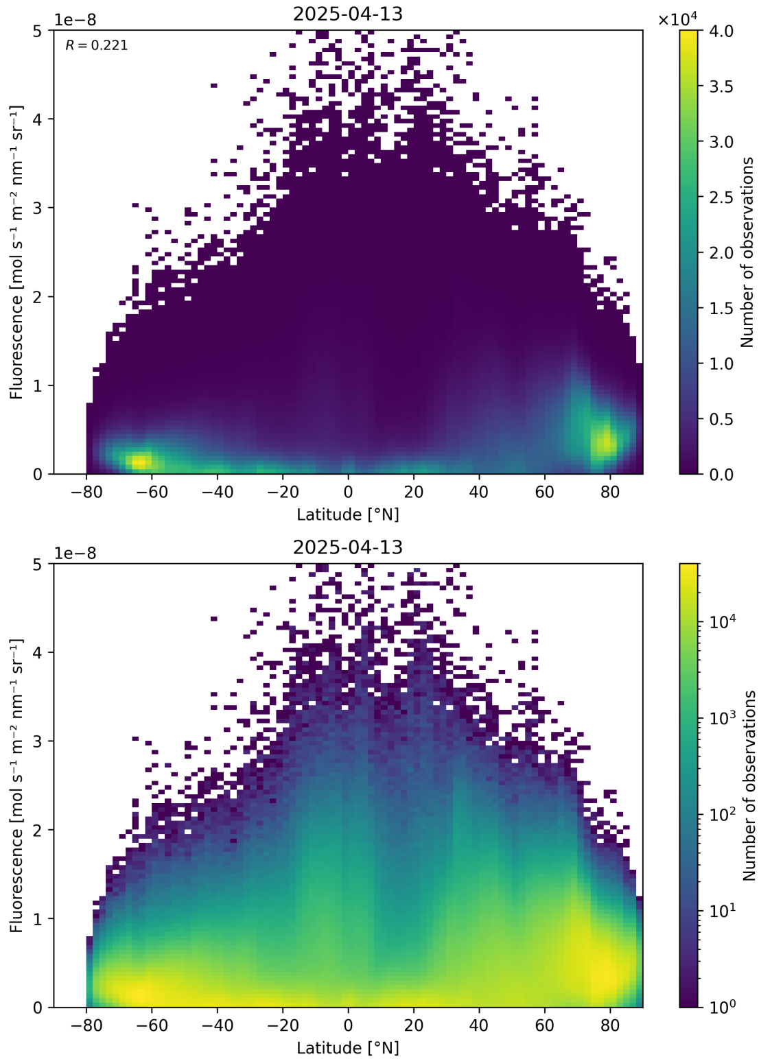
Figure 92: Scatter density plot of “Latitude” against “Fluorescence” for 2025-04-13 to 2025-04-14.
