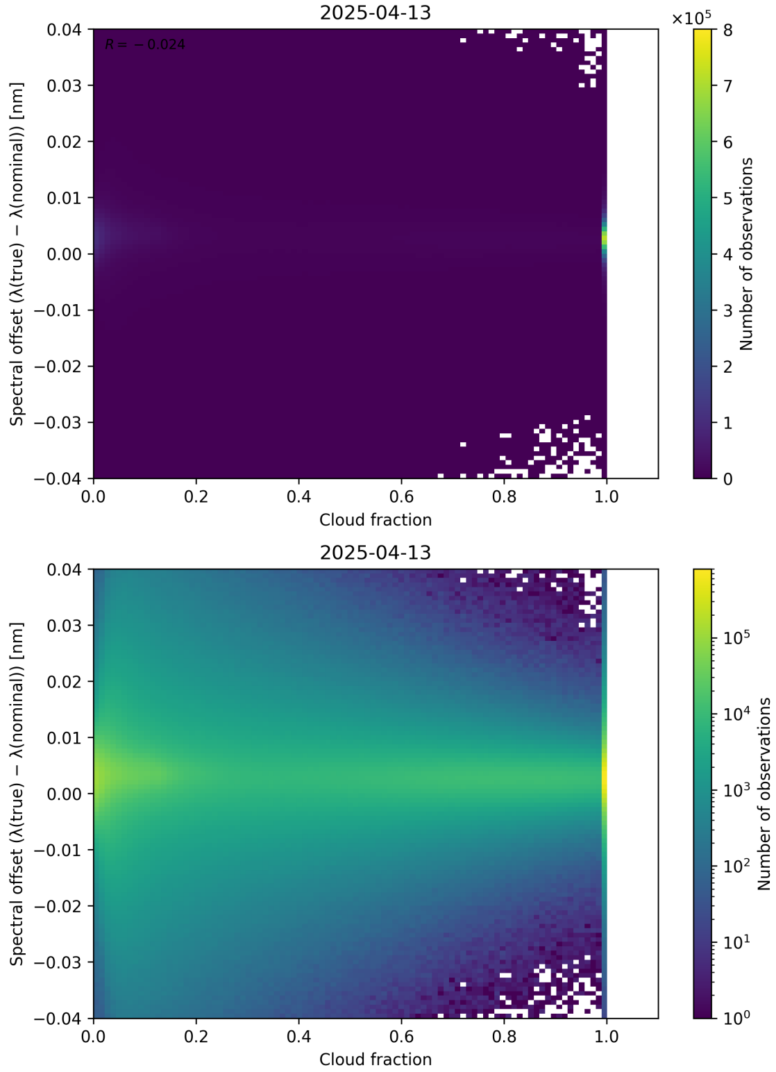
Figure 76: Scatter density plot of “Cloud fraction” against “Spectral offset ( \lambda_{\text{true}} - \lambda_{\text{nominal}} )” for 2025-04-13 to 2025-04-14.
