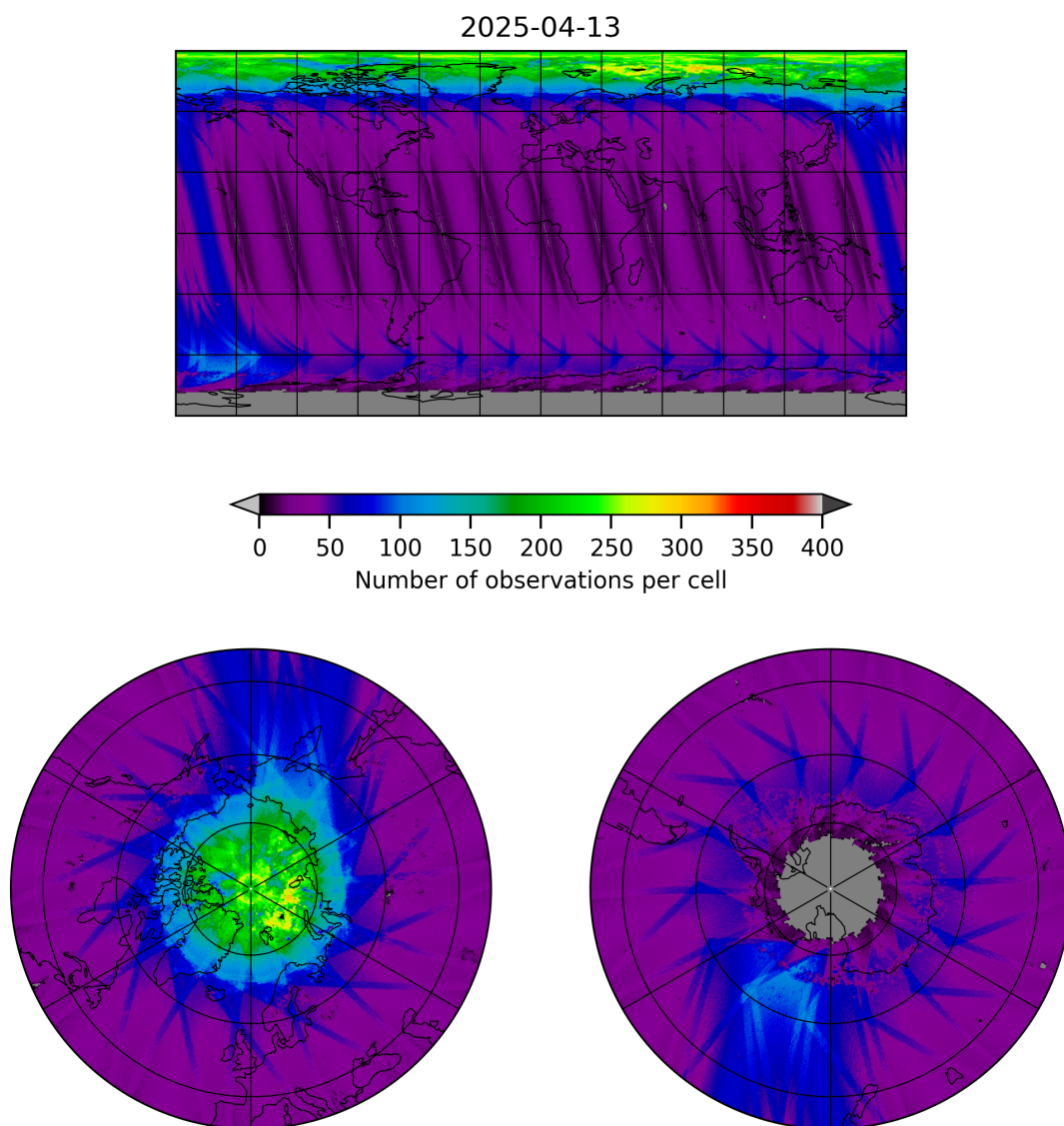
Figure 11: Map of the number of observations for 2025-04-13 to 2025-04-14
