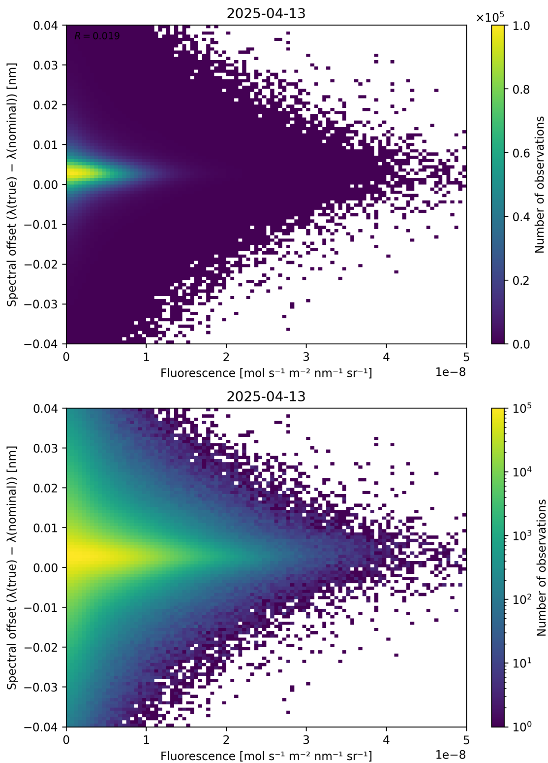
Figure 87: Scatter density plot of “Fluorescence” against “Spectral offset ( \lambda_{\text{true}} - \lambda_{\text{nominal}} )” for 2025-04-13 to 2025-04-14.
