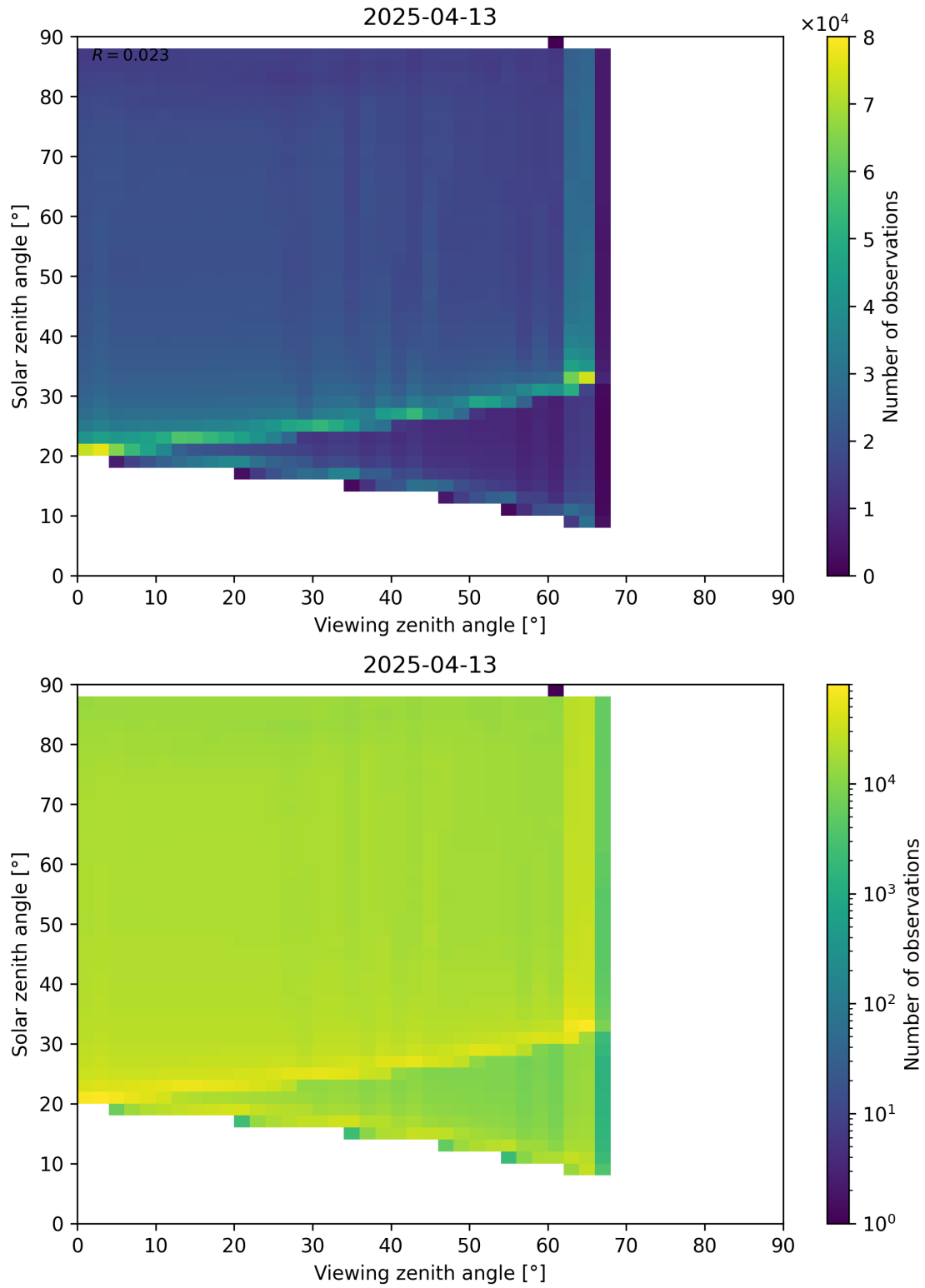
Figure 127: Scatter density plot of “Viewing zenith angle” against “Solar zenith angle” for 2025-04-13 to 2025-04-14.
