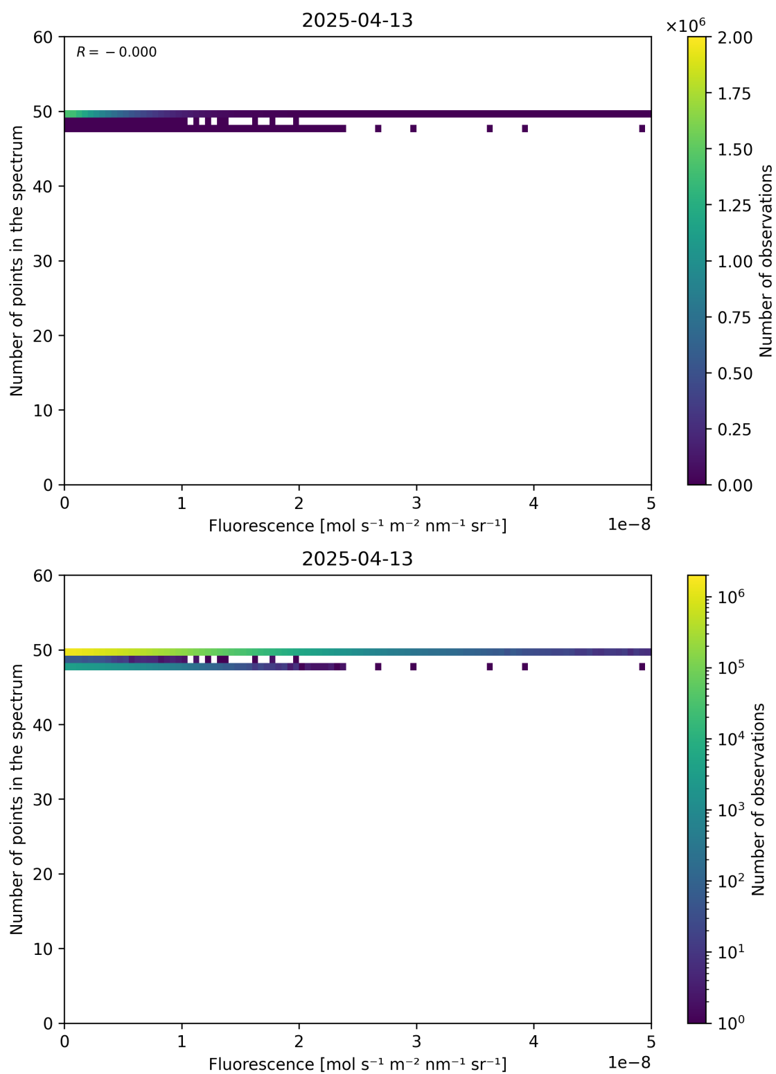
Figure 86: Scatter density plot of “Fluorescence” against “Number of points in the spectrum” for 2025-04-13 to 2025-04-14.
