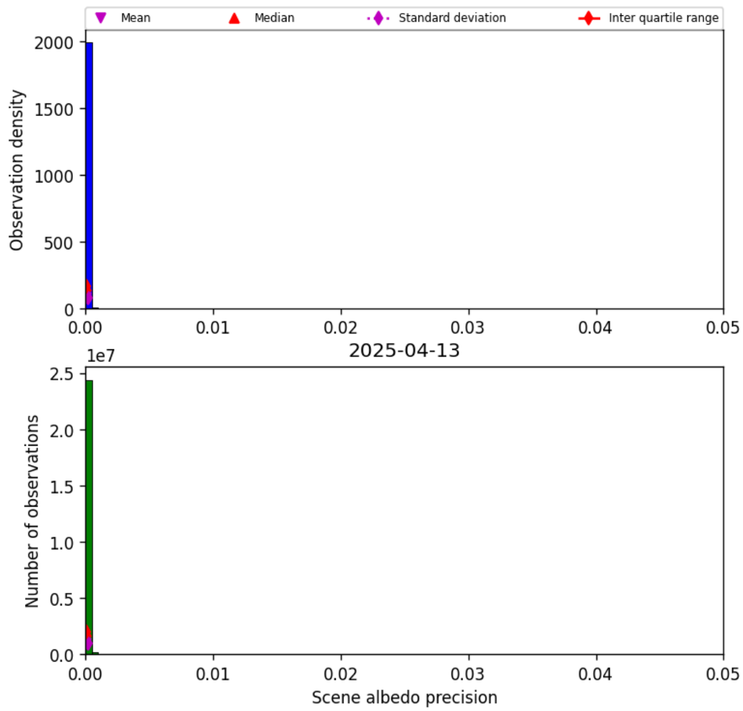
Figure 35: Histogram of “Scene albedo precision” for 2025-04-13 to 2025-04-14
