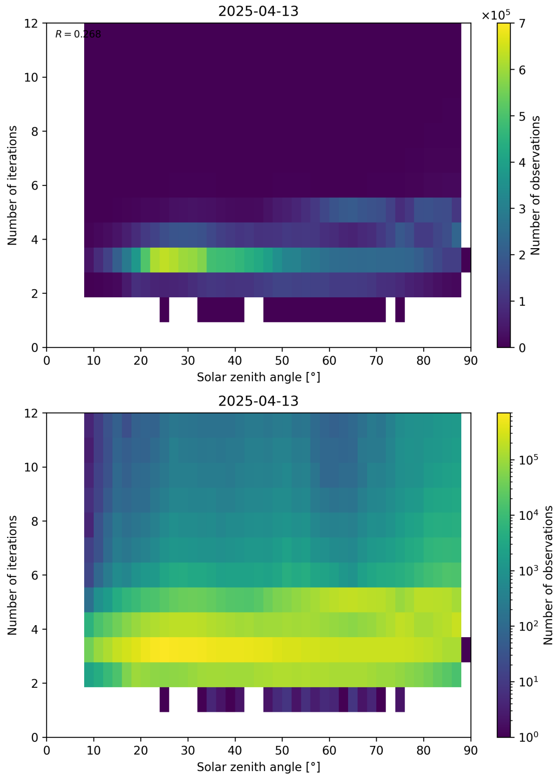
Figure 114: Scatter density plot of “Solar zenith angle” against “Number of iterations” for 2025-04-13 to 2025-04-14.
