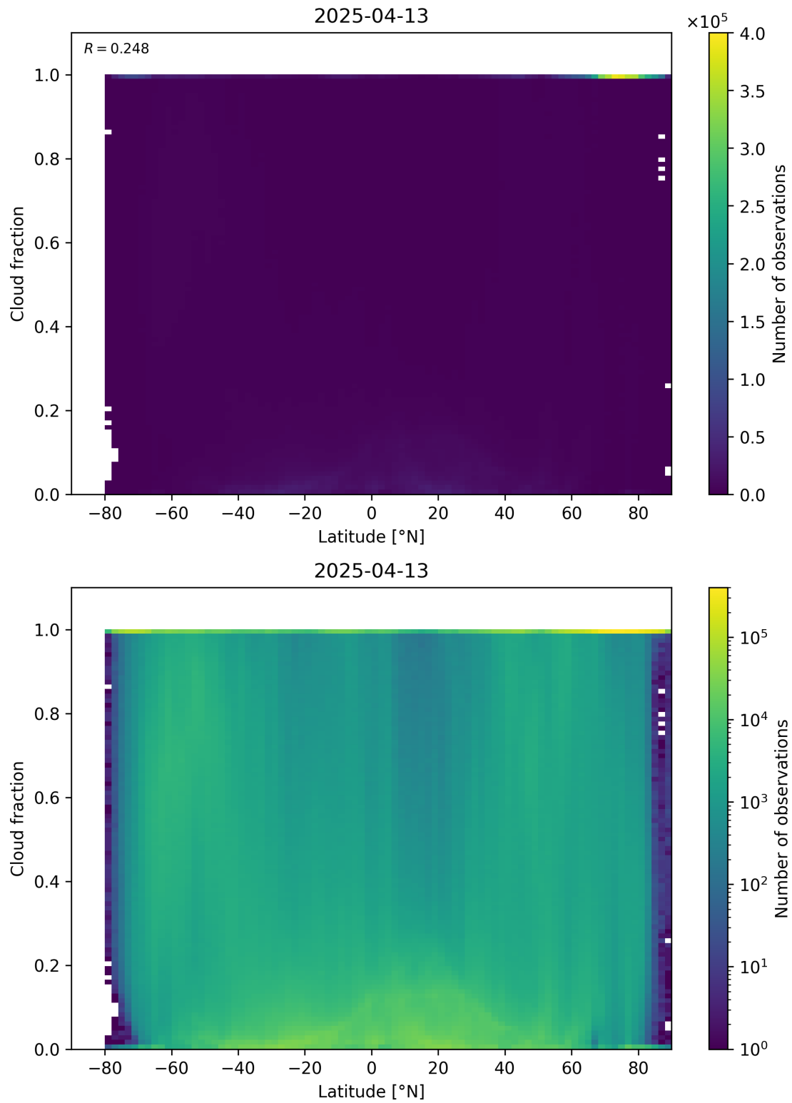
Figure 90: Scatter density plot of “Latitude” against “Cloud fraction” for 2025-04-13 to 2025-04-14.
