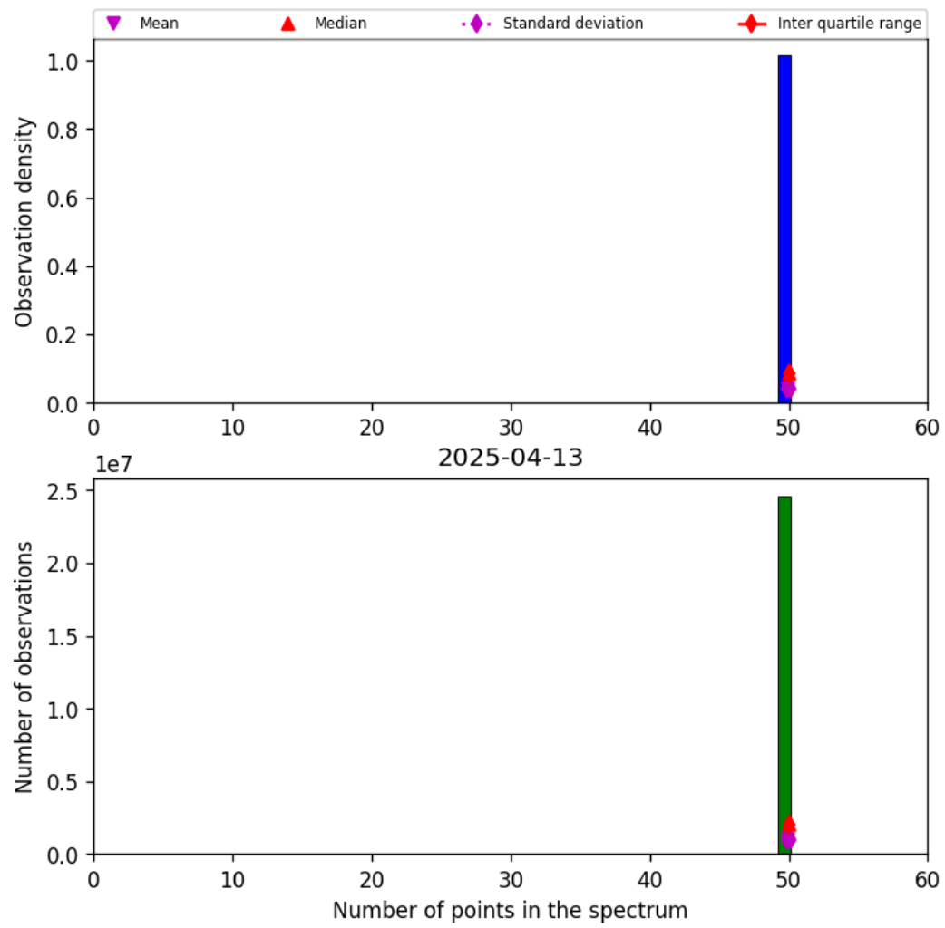
Figure 44: Histogram of “Number of points in the spectrum” for 2025-04-13 to 2025-04-14
