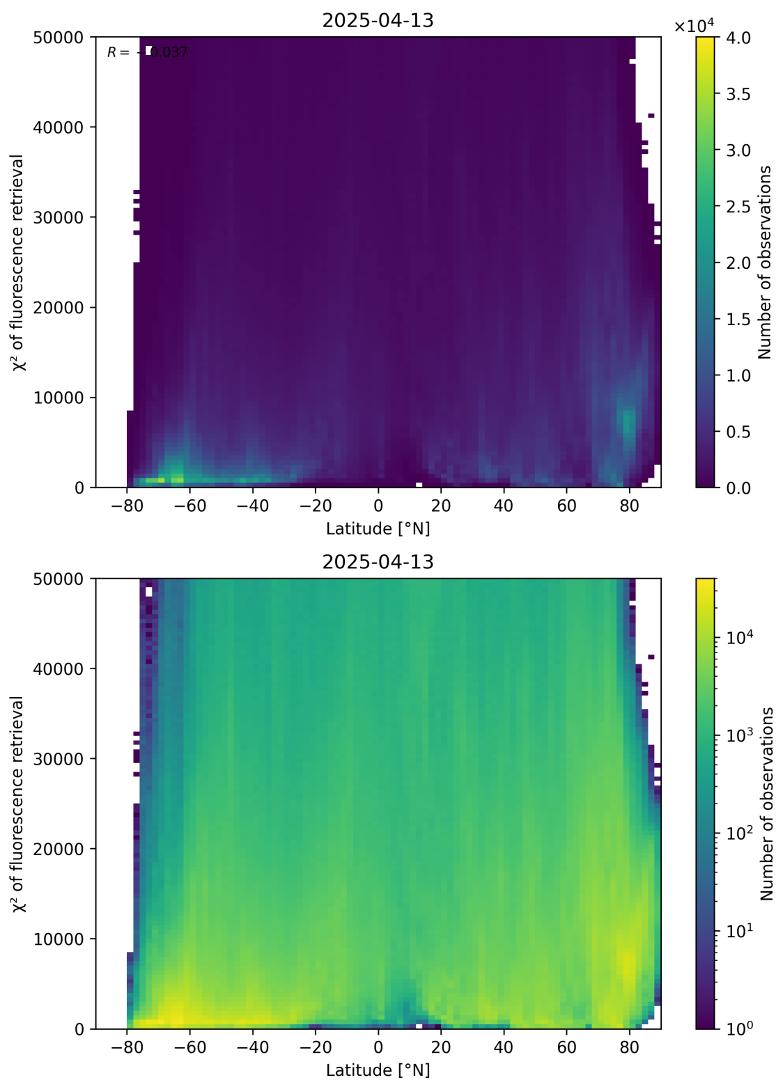
Figure 89: Scatter density plot of “Latitude” against “ \chi^2 of fluorescence retrieval” for 2025-04-13 to 2025-04-14.
