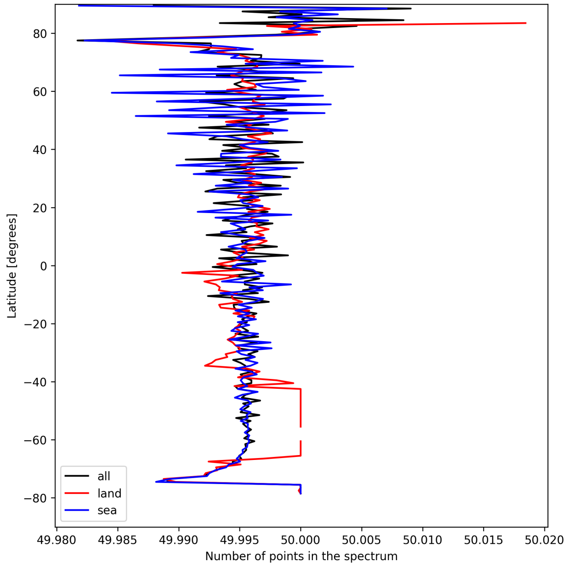
Figure 27: Zonal average of “Number of points in the spectrum” for 2025-04-13 to 2025-04-14.
