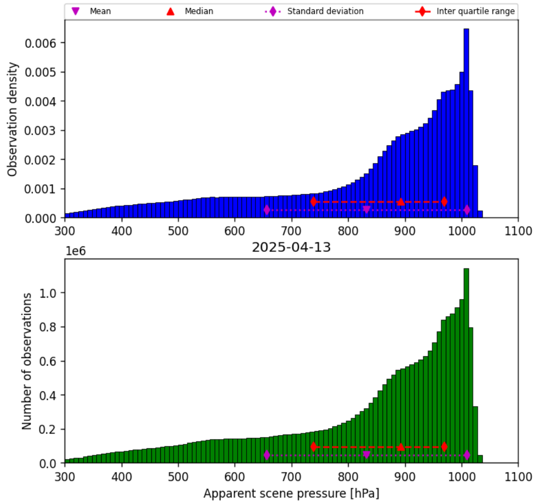
Figure 36: Histogram of “Apparent scene pressure” for 2025-04-13 to 2025-04-14
