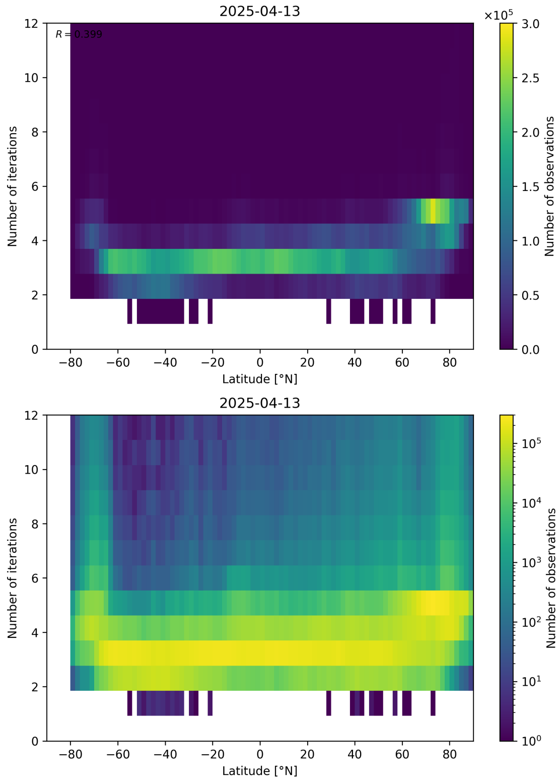
Figure 93: Scatter density plot of “Latitude” against “Number of iterations” for 2025-04-13 to 2025-04-14.
