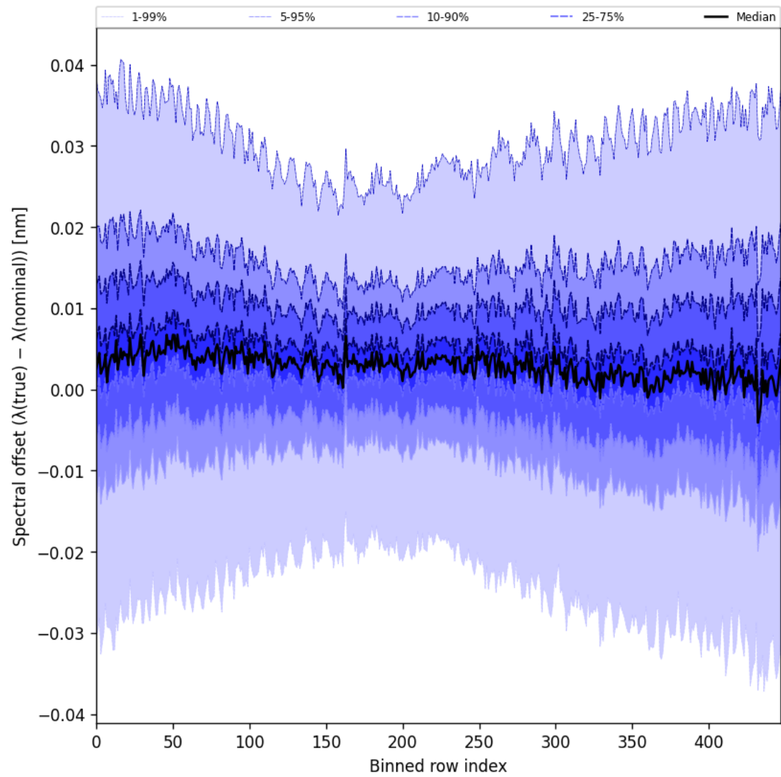
Figure 62: Along track statistics of “Spectral offset ( \lambda_{\text{true}} - \lambda_{\text{nominal}} )” for 2025-04-13 to 2025-04-14
