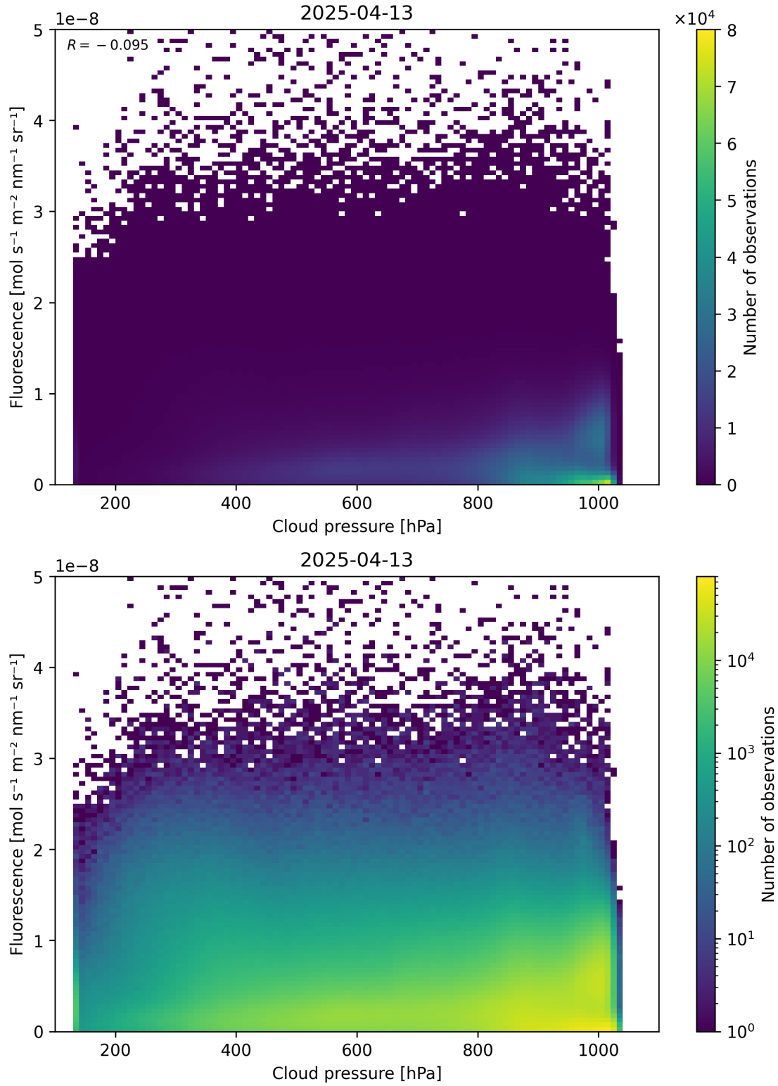
Figure 80: Scatter density plot of “Cloud pressure” against “Fluorescence” for 2025-04-13 to 2025-04-14.
