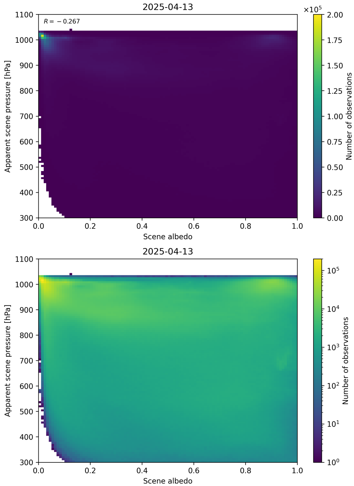
Figure 102: Scatter density plot of “Scene albedo” against “Apparent scene pressure” for 2025-04-13 to 2025-04-14.
