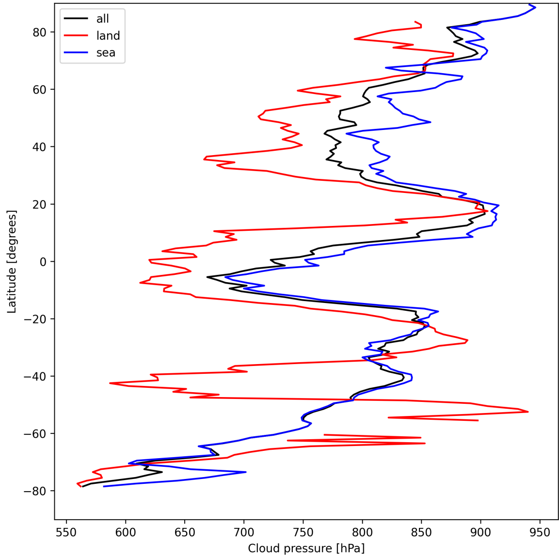
Figure 13: Zonal average of “Cloud pressure” for 2025-04-13 to 2025-04-14.
