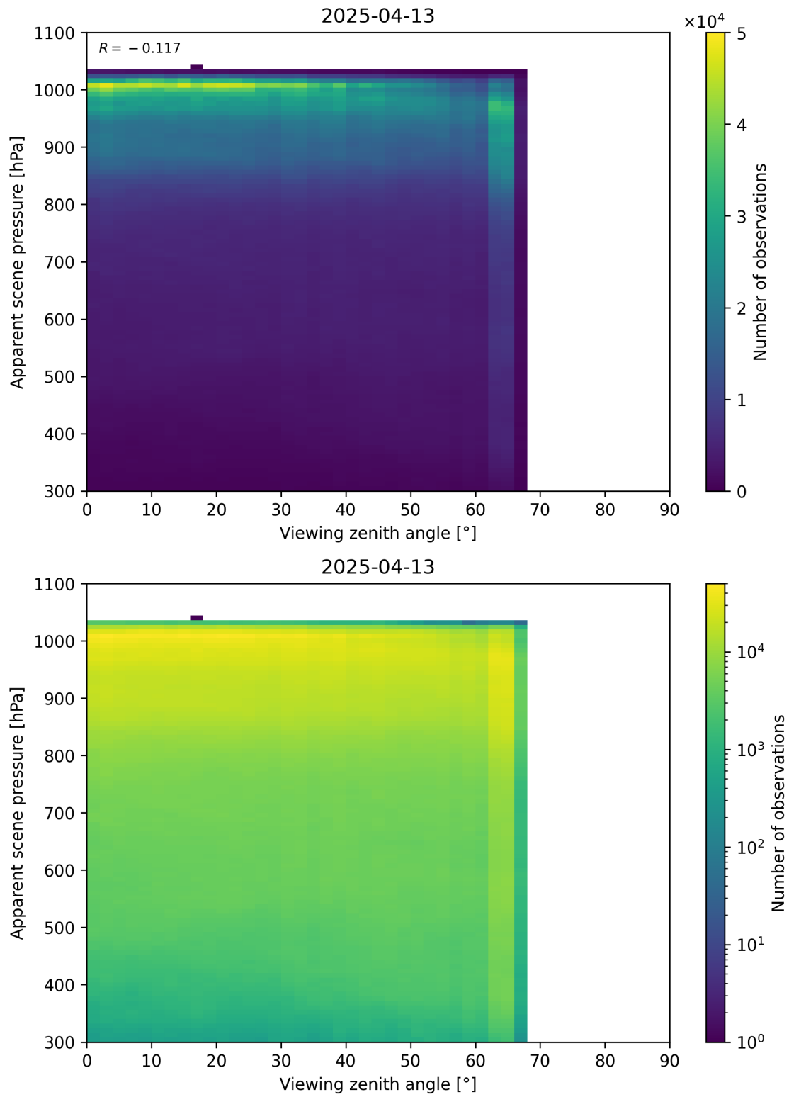
Figure 118: Scatter density plot of “Viewing zenith angle” against “Apparent scene pressure” for 2025-04-13 to 2025-04-14.
