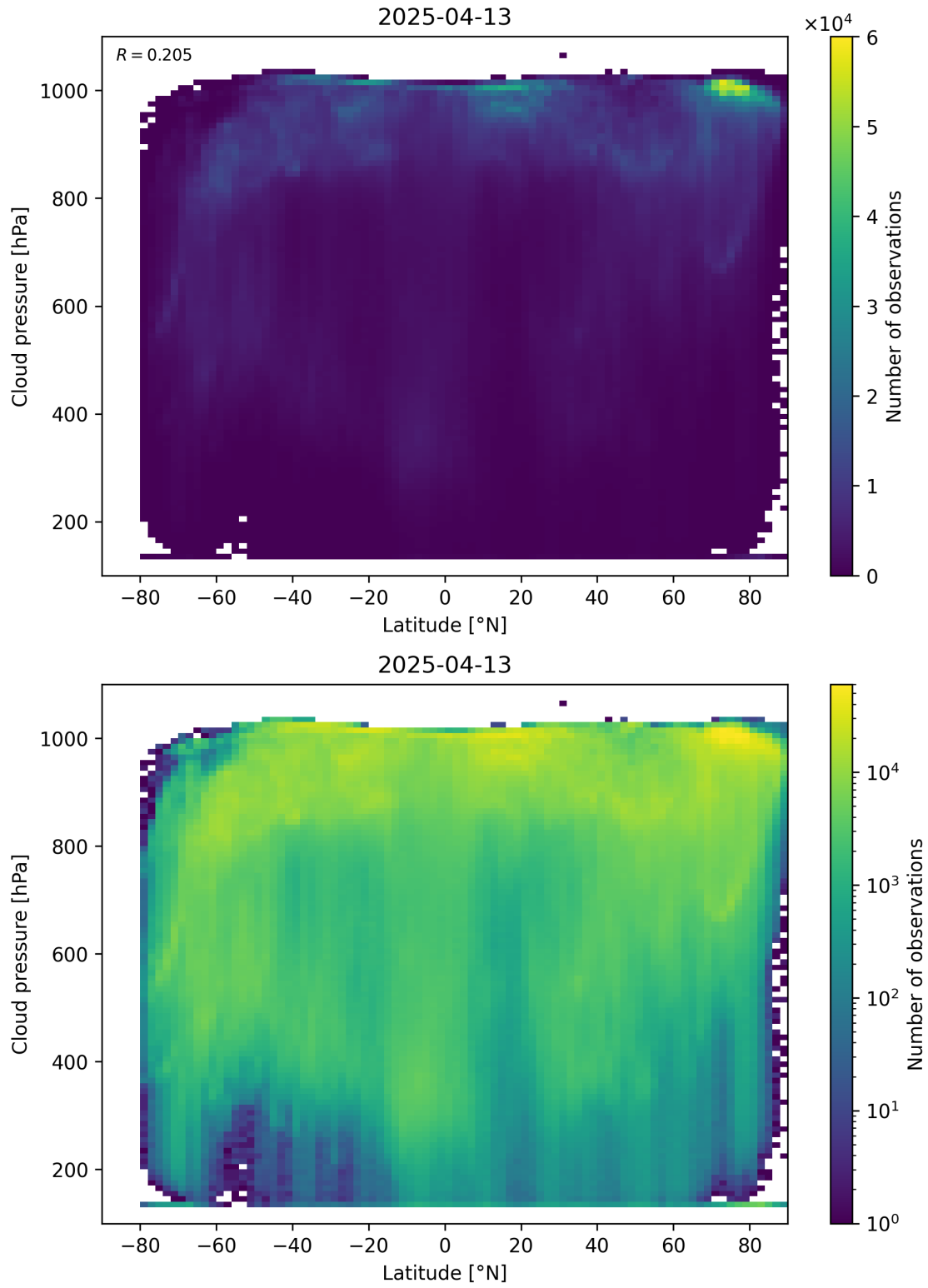
Figure 91: Scatter density plot of “Latitude” against “Cloud pressure” for 2025-04-13 to 2025-04-14.
