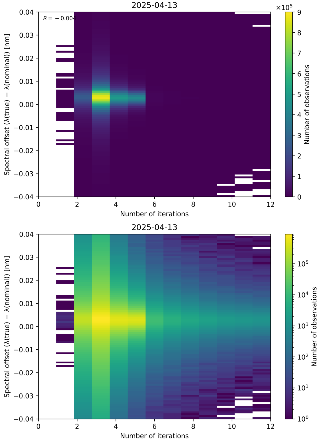
Figure 100: Scatter density plot of “Number of iterations” against “Spectral offset ( \lambda_{\text{true}} - \lambda_{\text{nominal}} )” for 2025-04-13 to 2025-04-14.
