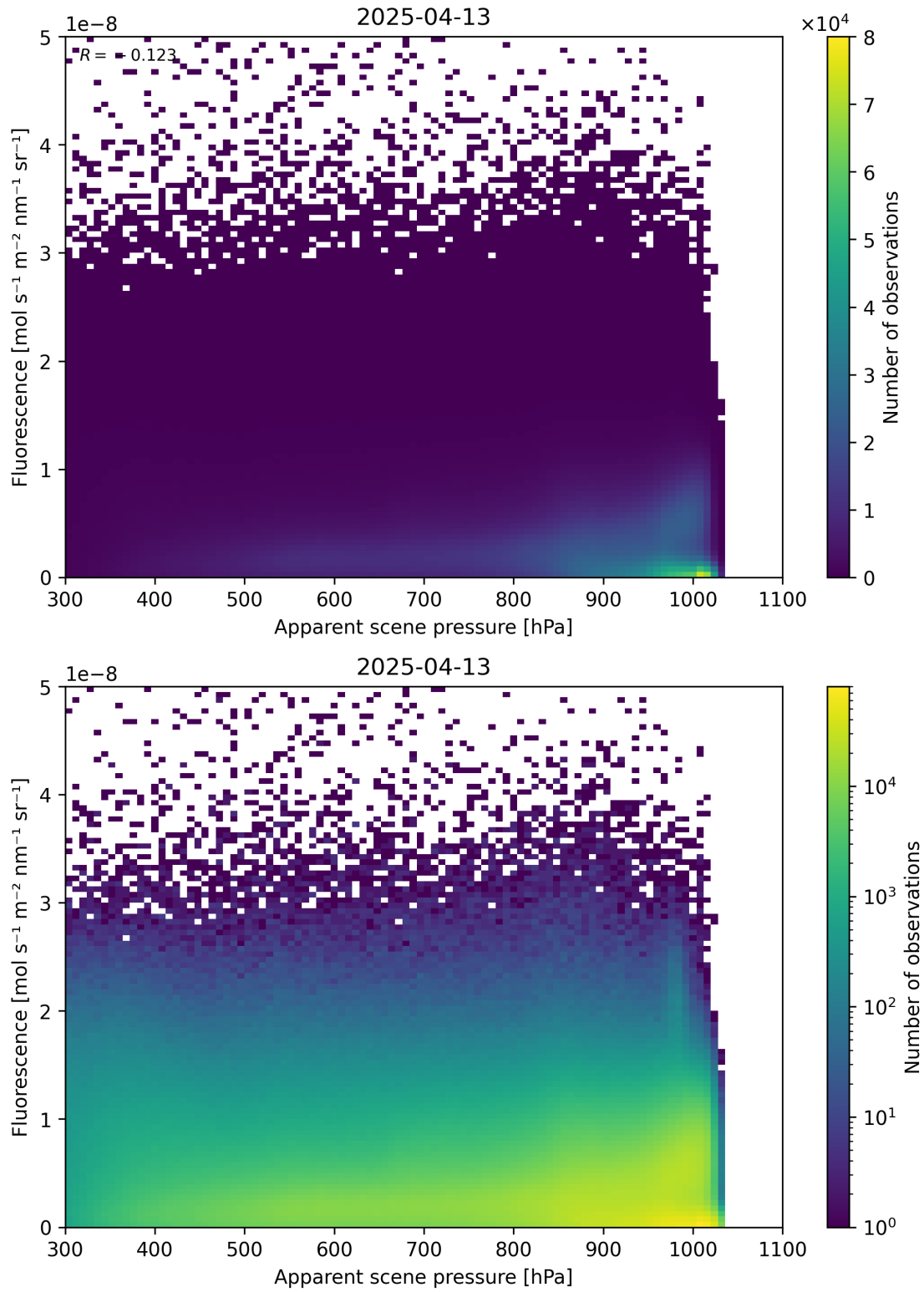
Figure 64: Scatter density plot of “Apparent scene pressure” against “Fluorescence” for 2025-04-13 to 2025-04-14.
