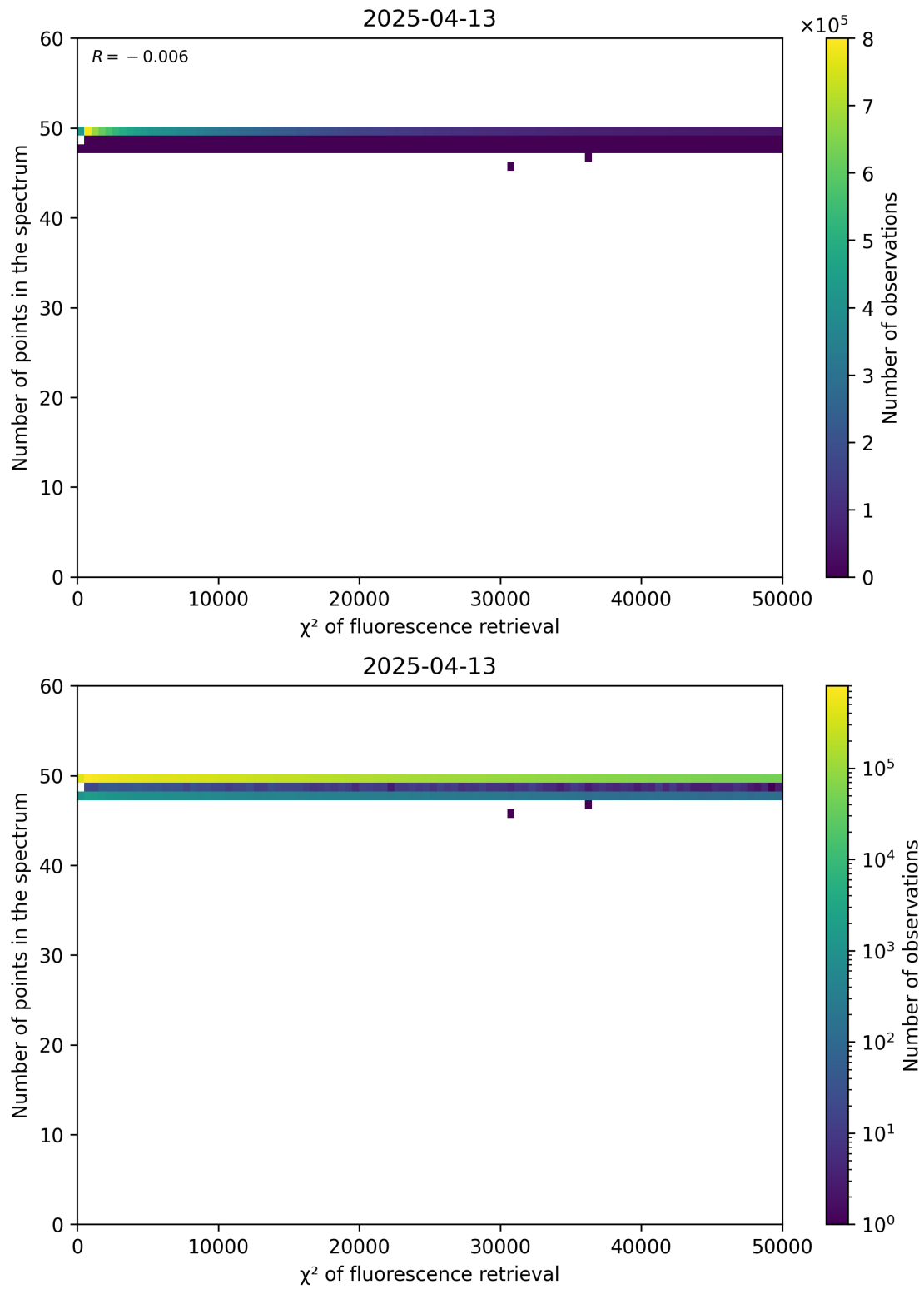
Figure 68: Scatter density plot of “ \chi^2 of fluorescence retrieval” against “Number of points in the spectrum” for 2025-04-13 to 2025-04-14.
