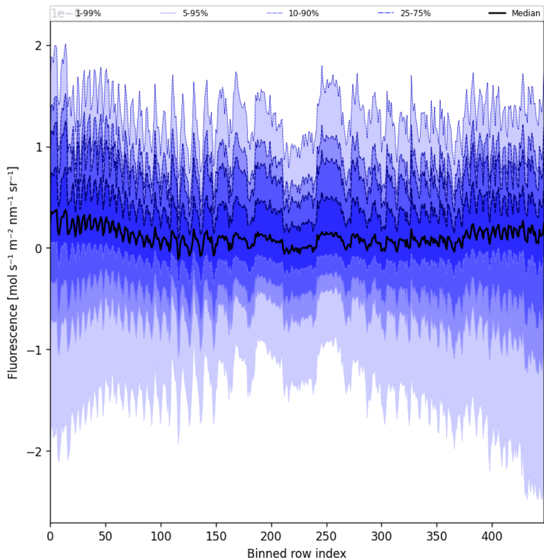
Figure 57: Along track statistics of “Fluorescence” for 2025-04-13 to 2025-04-14
