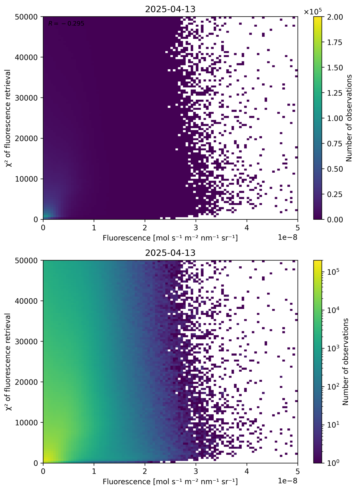
Figure 85: Scatter density plot of “Fluorescence” against “ \chi^2 of fluorescence retrieval” for 2025-04-13 to 2025-04-14.
