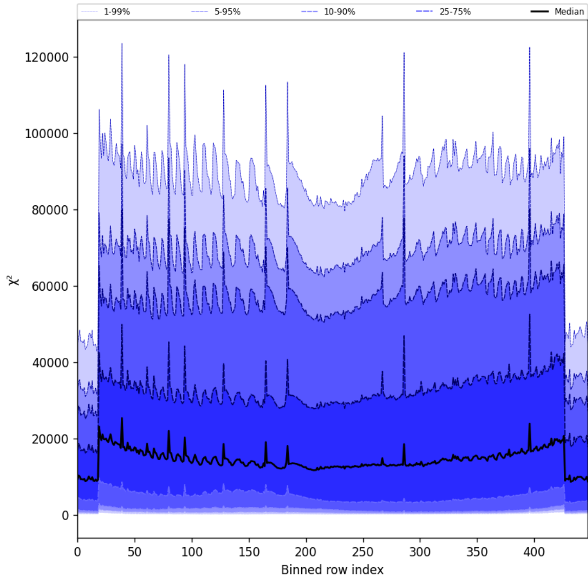
Figure 55: Along track statistics of “ \chi^2 ” for 2025-04-13 to 2025-04-14
