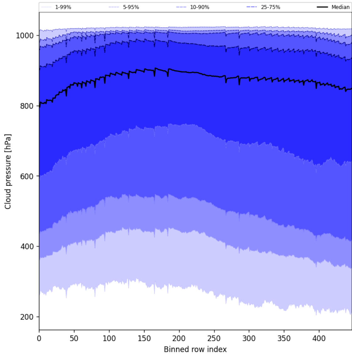
Figure 47: Along track statistics of “Cloud pressure” for 2025-04-13 to 2025-04-14
