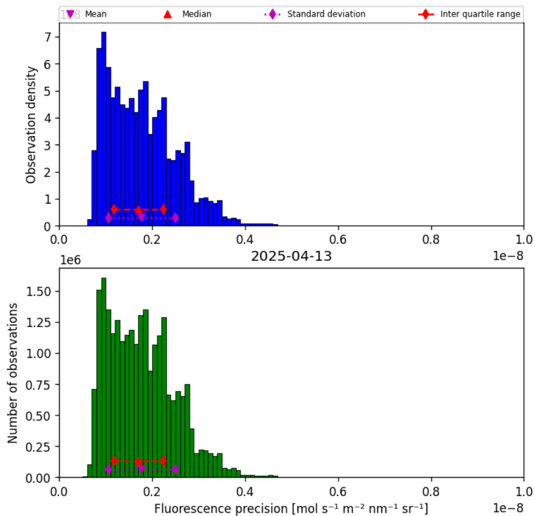
Figure 41: Histogram of “Fluorescence precision” for 2025-04-13 to 2025-04-14
