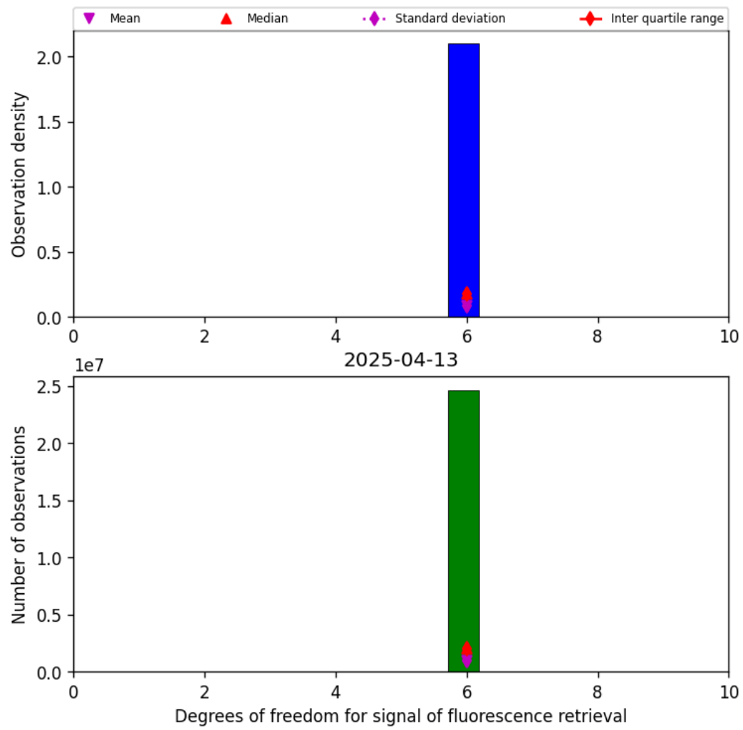
Figure 43: Histogram of “Degrees of freedom for signal of fluorescence retrieval” for 2025-04-13 to 2025-04-14
