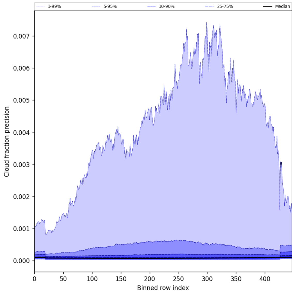
Figure 50: Along track statistics of “Cloud fraction precision” for 2025-04-13 to 2025-04-14
