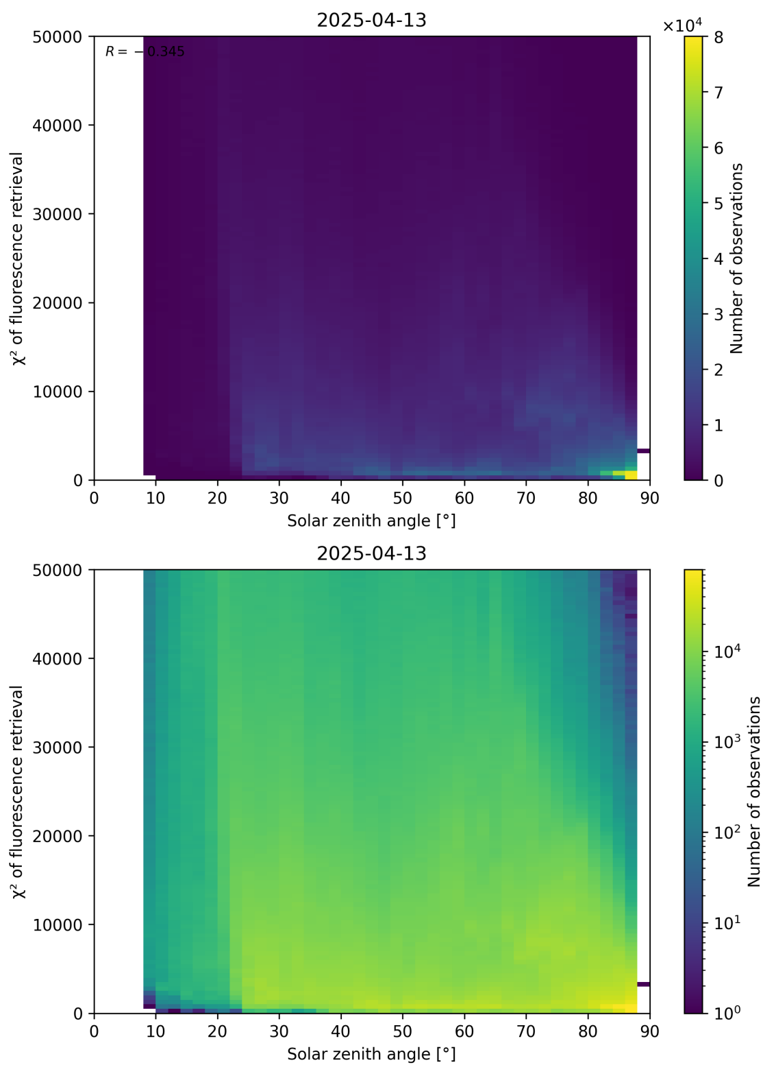
Figure 109: Scatter density plot of “Solar zenith angle” against “ \chi^2 of fluorescence retrieval” for 2025-04-13 to 2025-04-14.
