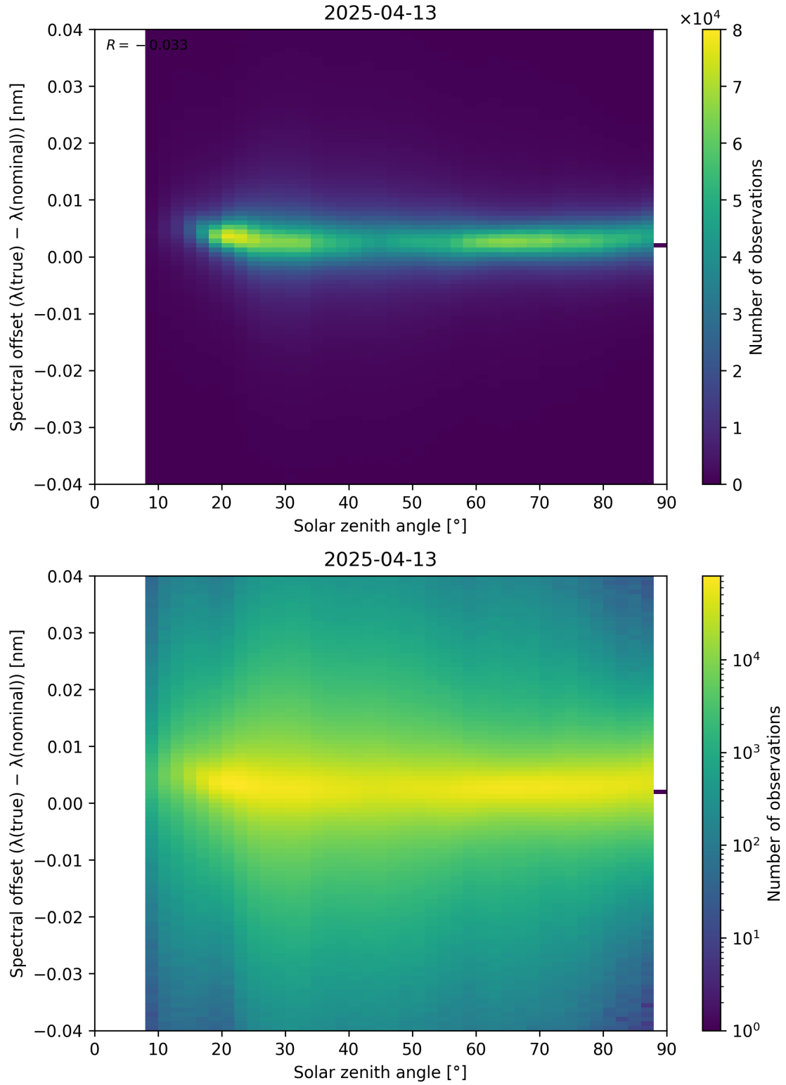
Figure 117: Scatter density plot of “Solar zenith angle” against “Spectral offset ( \lambda_{\text{true}} - \lambda_{\text{nominal}} )” for 2025-04-13 to 2025-04-14.
