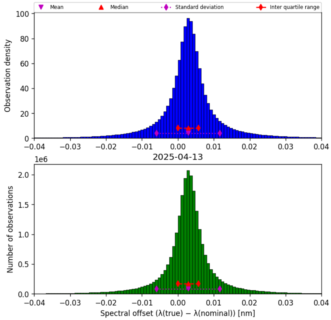
Figure 45: Histogram of “Spectral offset ( \lambda_{\text{true}} - \lambda_{\text{nominal}} )” for 2025-04-13 to 2025-04-14
