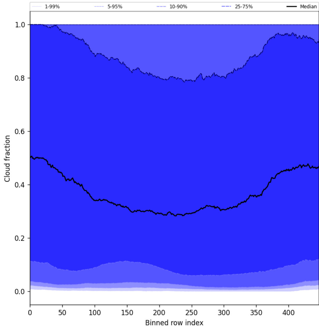
Figure 49: Along track statistics of “Cloud fraction” for 2025-04-13 to 2025-04-14
