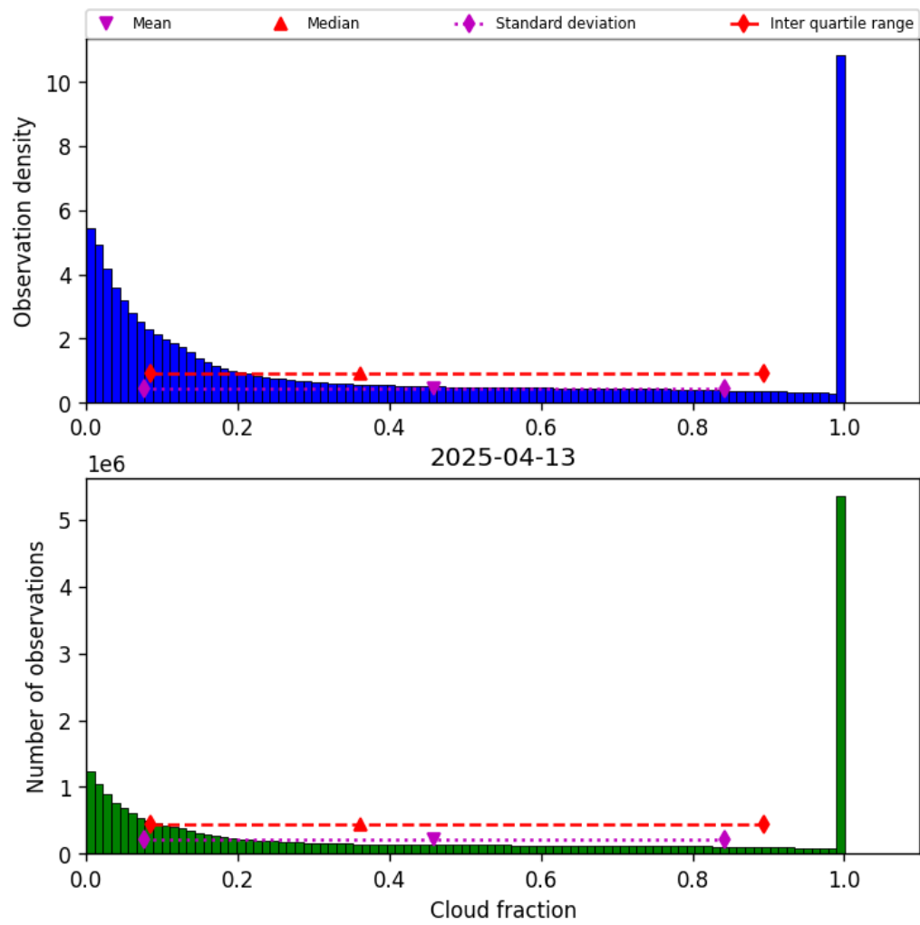
Figure 32: Histogram of “Cloud fraction” for 2025-04-13 to 2025-04-14
