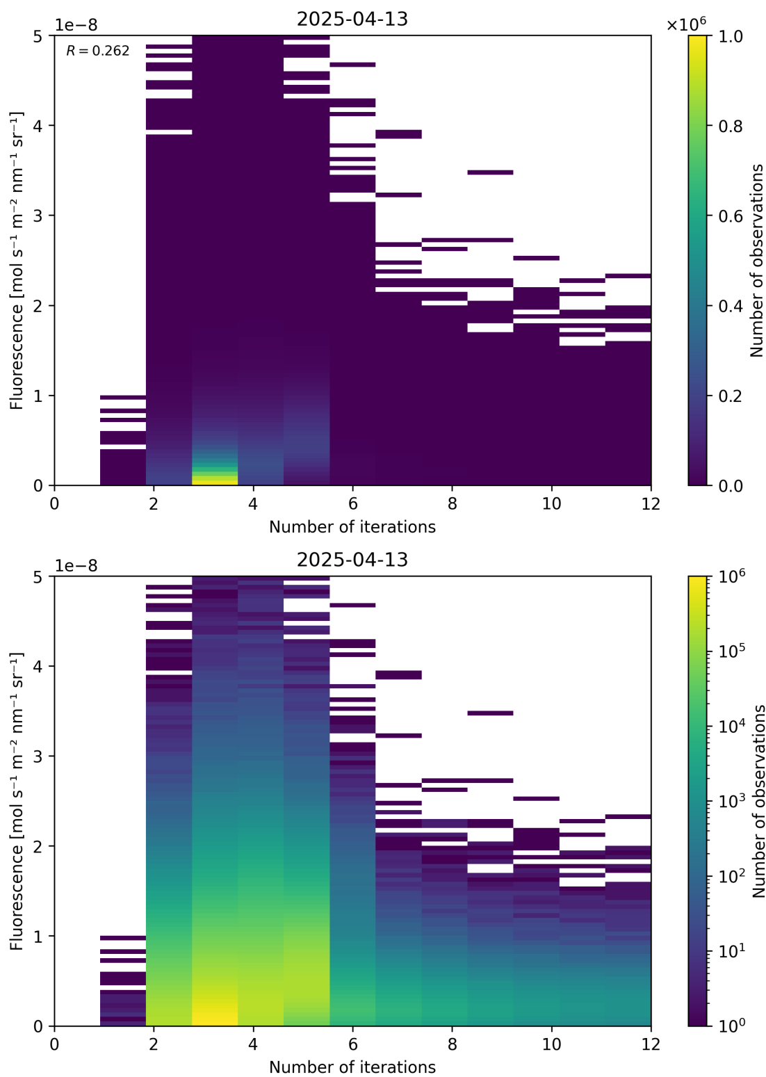
Figure 98: Scatter density plot of “Number of iterations” against “Fluorescence” for 2025-04-13 to 2025-04-14.
