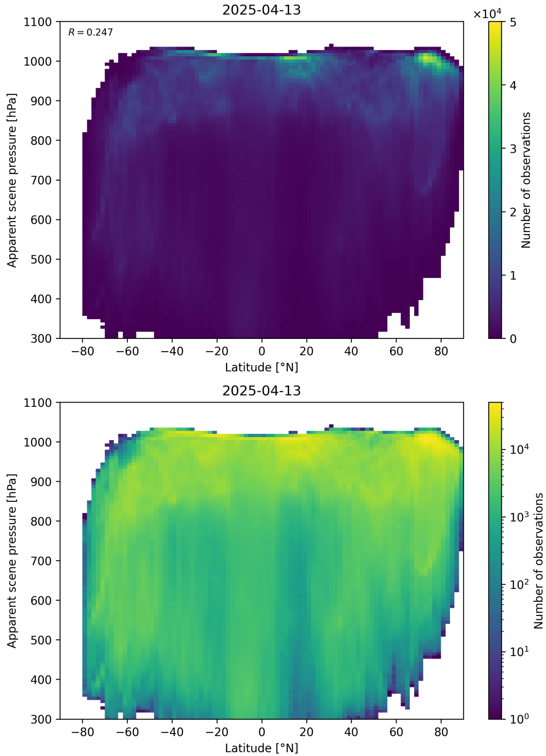
Figure 88: Scatter density plot of “Latitude” against “Apparent scene pressure” for 2025-04-13 to 2025-04-14.
