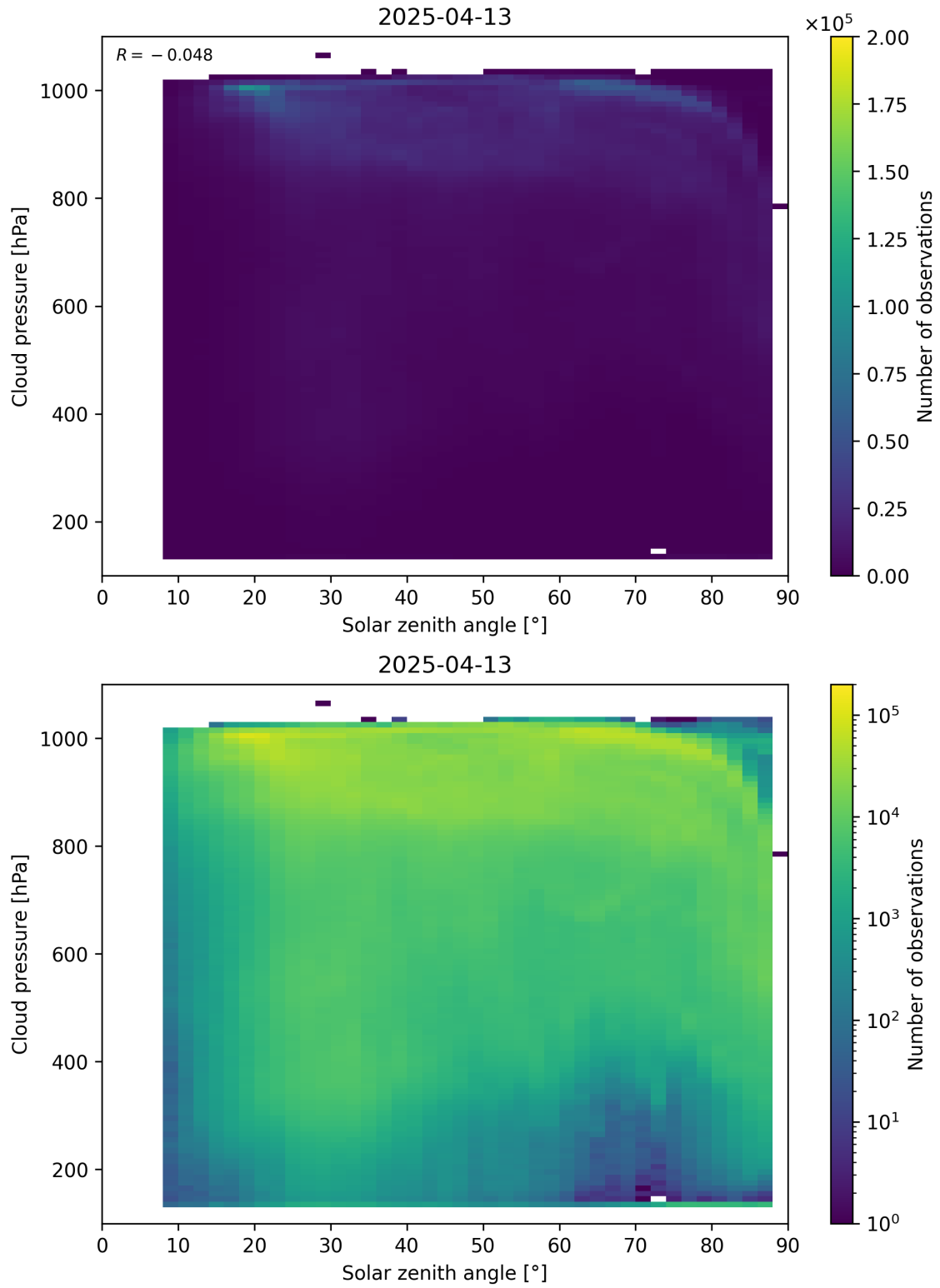
Figure 111: Scatter density plot of “Solar zenith angle” against “Cloud pressure” for 2025-04-13 to 2025-04-14.
