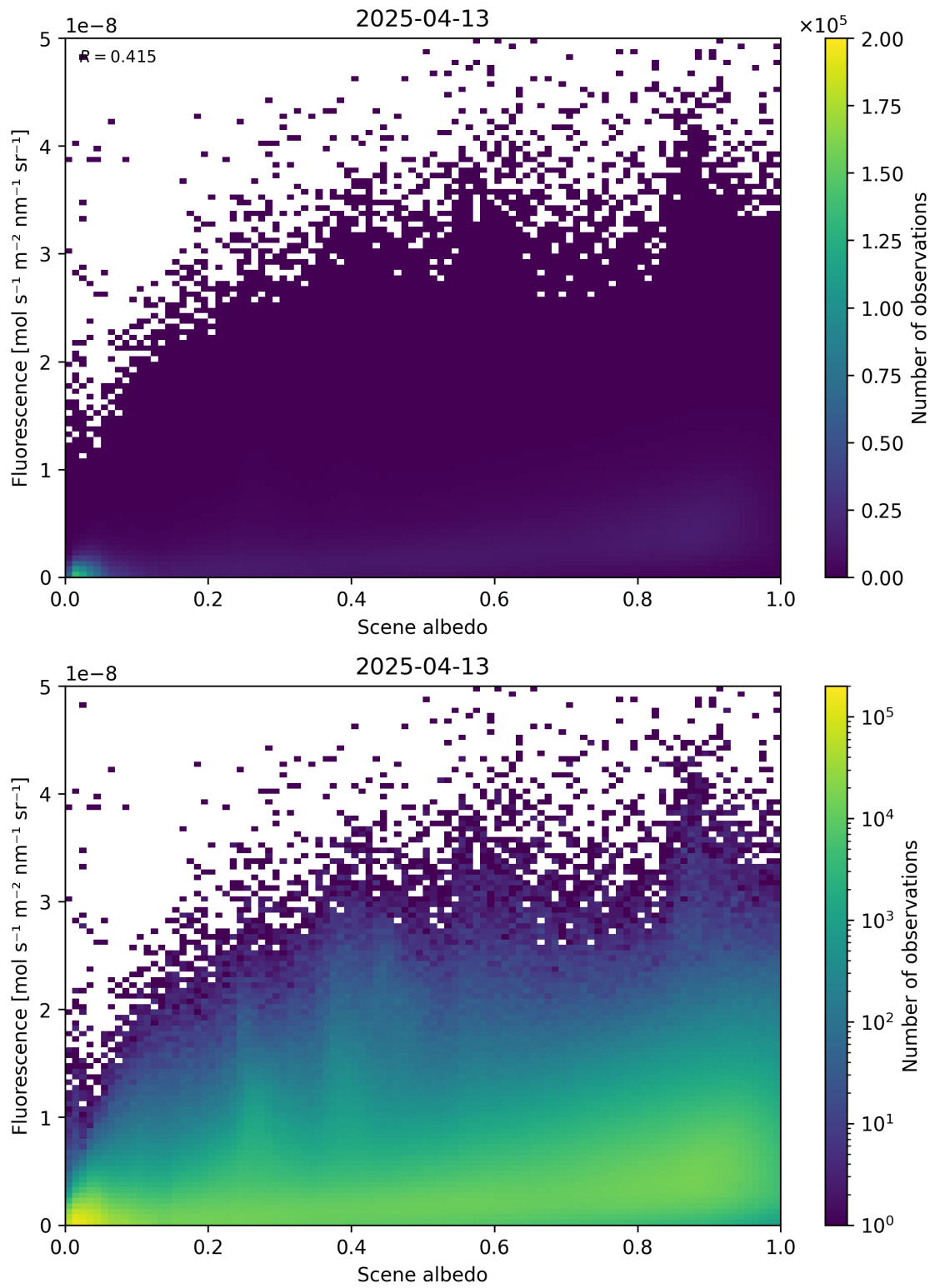
Figure 104: Scatter density plot of “Scene albedo” against “Fluorescence” for 2025-04-13 to 2025-04-14.
