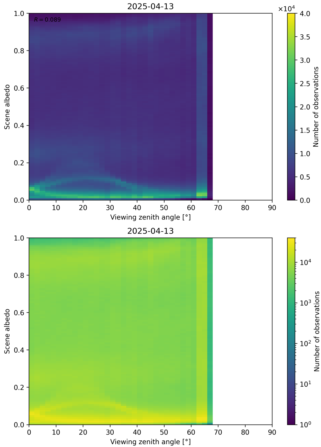
Figure 126: Scatter density plot of “Viewing zenith angle” against “Scene albedo” for 2025-04-13 to 2025-04-14.
