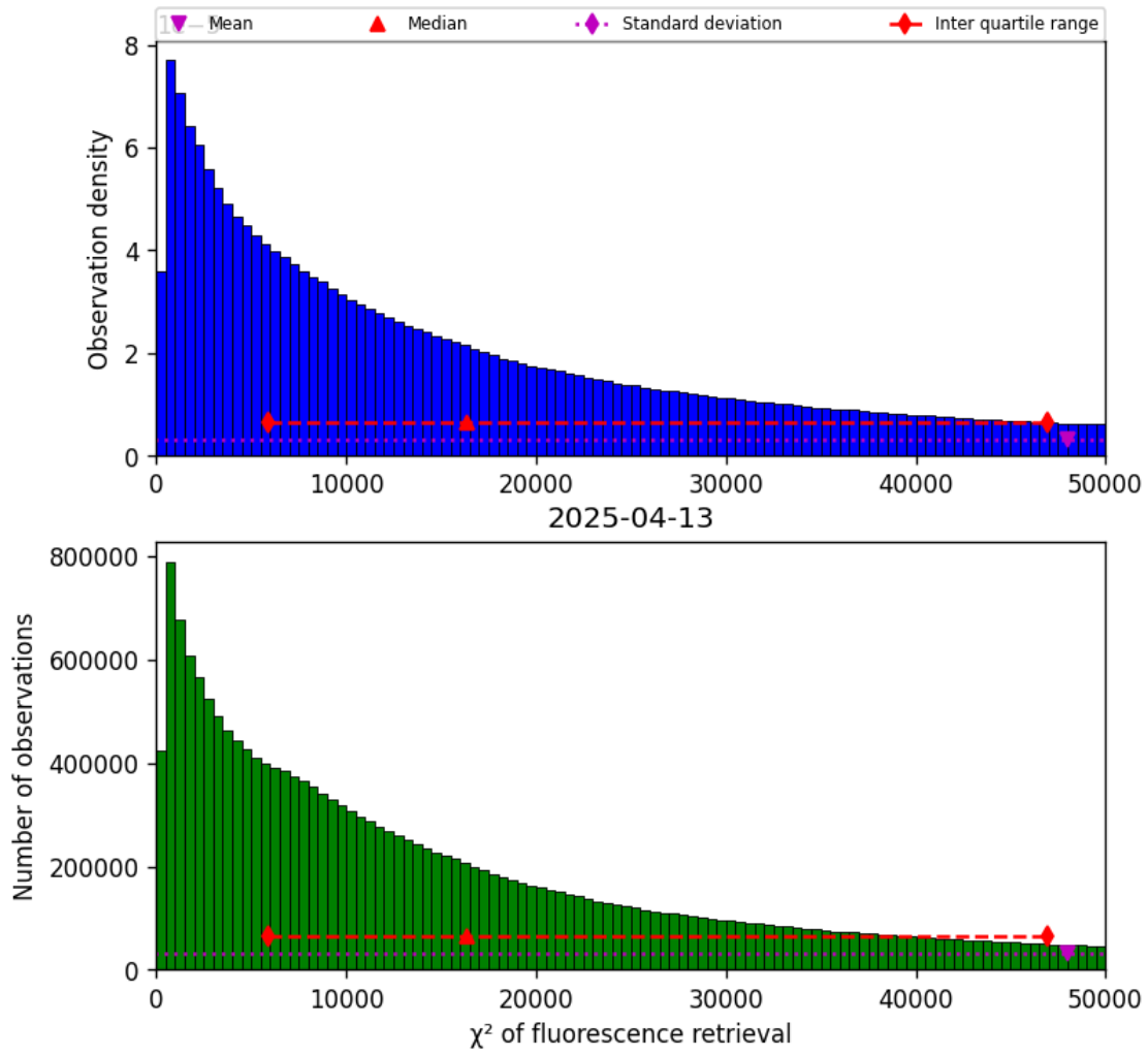
Figure 42: Histogram of “ \chi^2 of fluorescence retrieval” for 2025-04-13 to 2025-04-14
