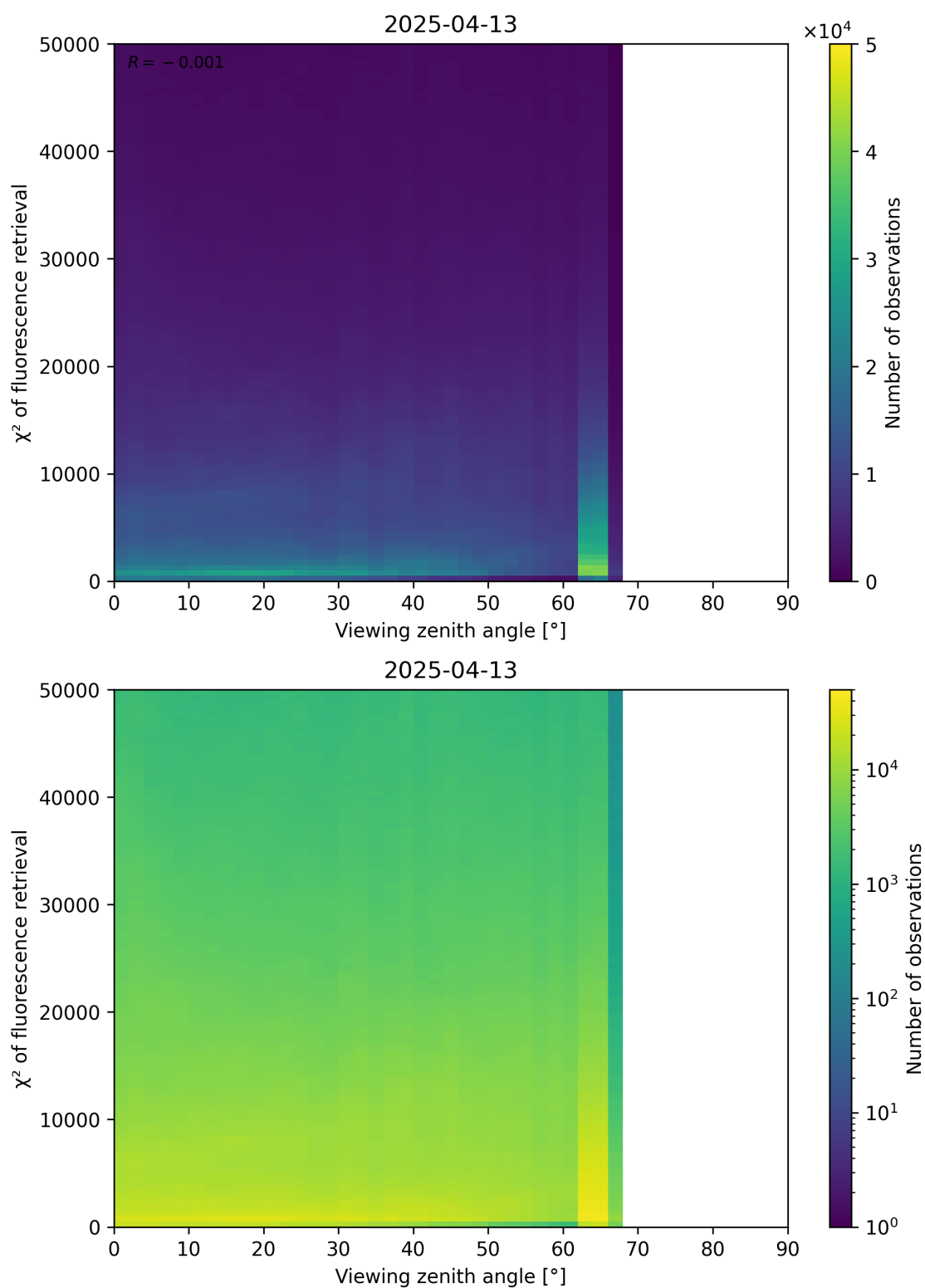
Figure 119: Scatter density plot of “Viewing zenith angle” against “ \chi^2 of fluorescence retrieval” for 2025-04-13 to 2025-04-14.
