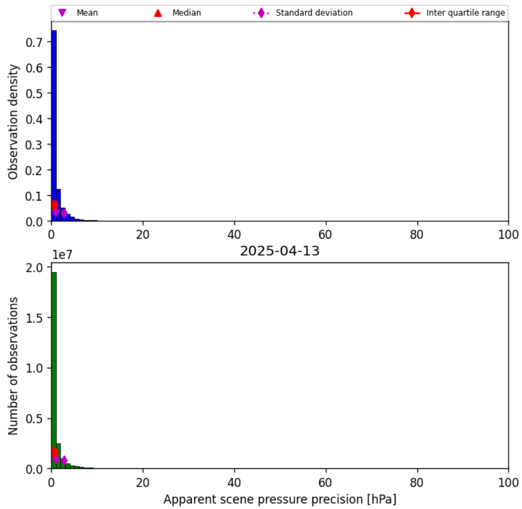
Figure 37: Histogram of “Apparent scene pressure precision” for 2025-04-13 to 2025-04-14
