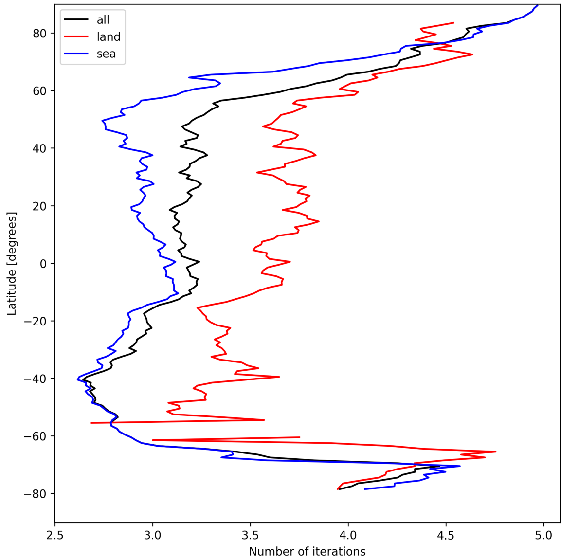
Figure 22: Zonal average of “Number of iterations” for 2025-04-13 to 2025-04-14.
