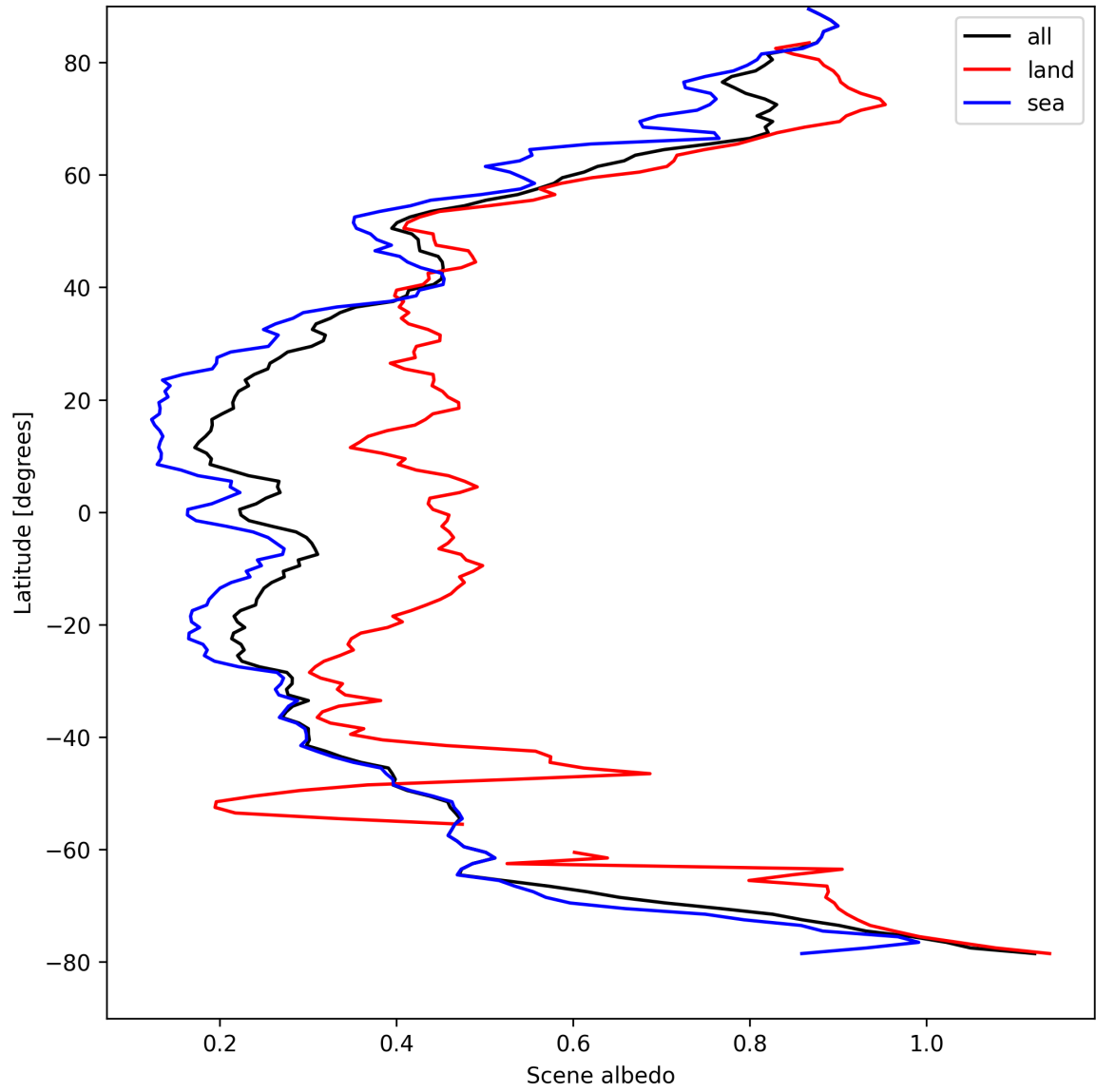
Figure 17: Zonal average of “Scene albedo” for 2025-04-13 to 2025-04-14.
