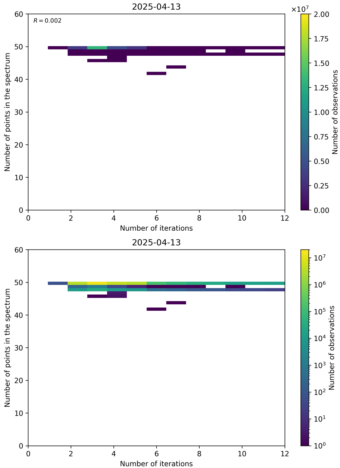
Figure 99: Scatter density plot of “Number of iterations” against “Number of points in the spectrum” for 2025-04-13 to 2025-04-14.
