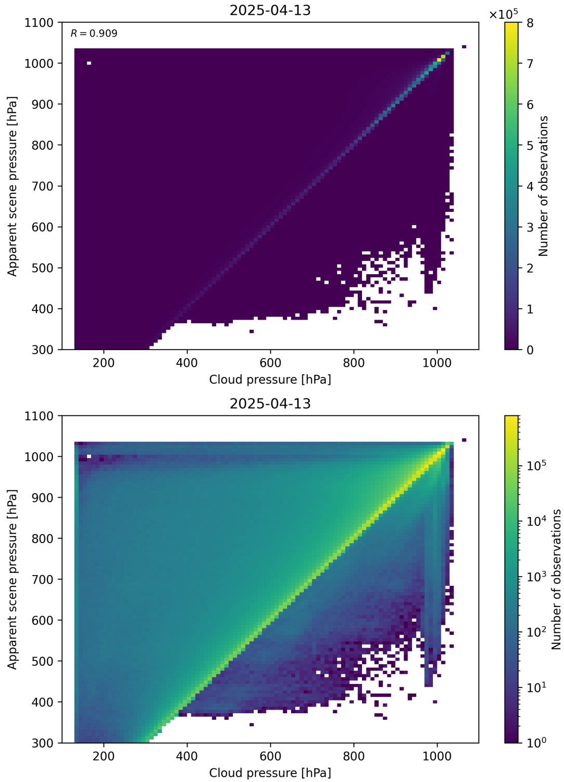
Figure 77: Scatter density plot of “Cloud pressure” against “Apparent scene pressure” for 2025-04-13 to 2025-04-14.
