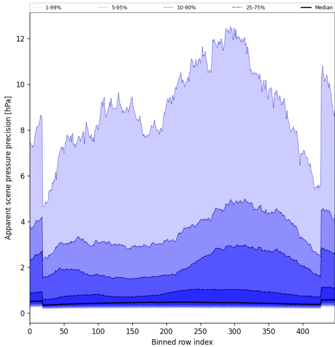
Figure 54: Along track statistics of “Apparent scene pressure precision” for 2025-04-13 to 2025-04-14
