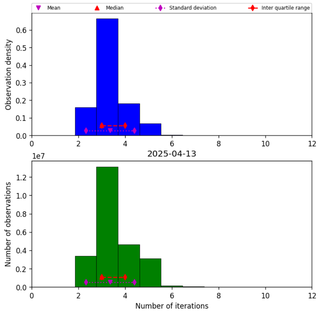
Figure 39: Histogram of “Number of iterations” for 2025-04-13 to 2025-04-14
