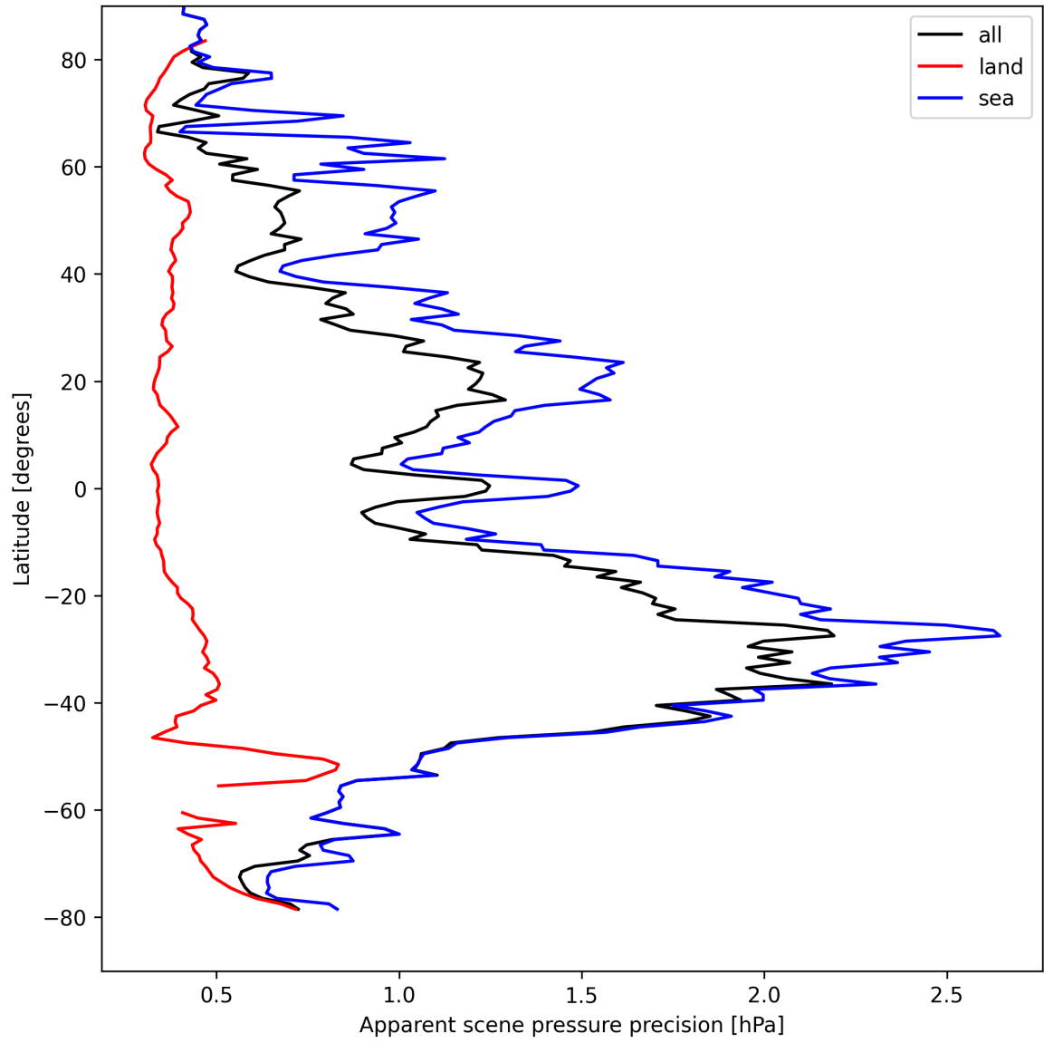
Figure 20: Zonal average of “Apparent scene pressure precision” for 2025-04-13 to 2025-04-14.
