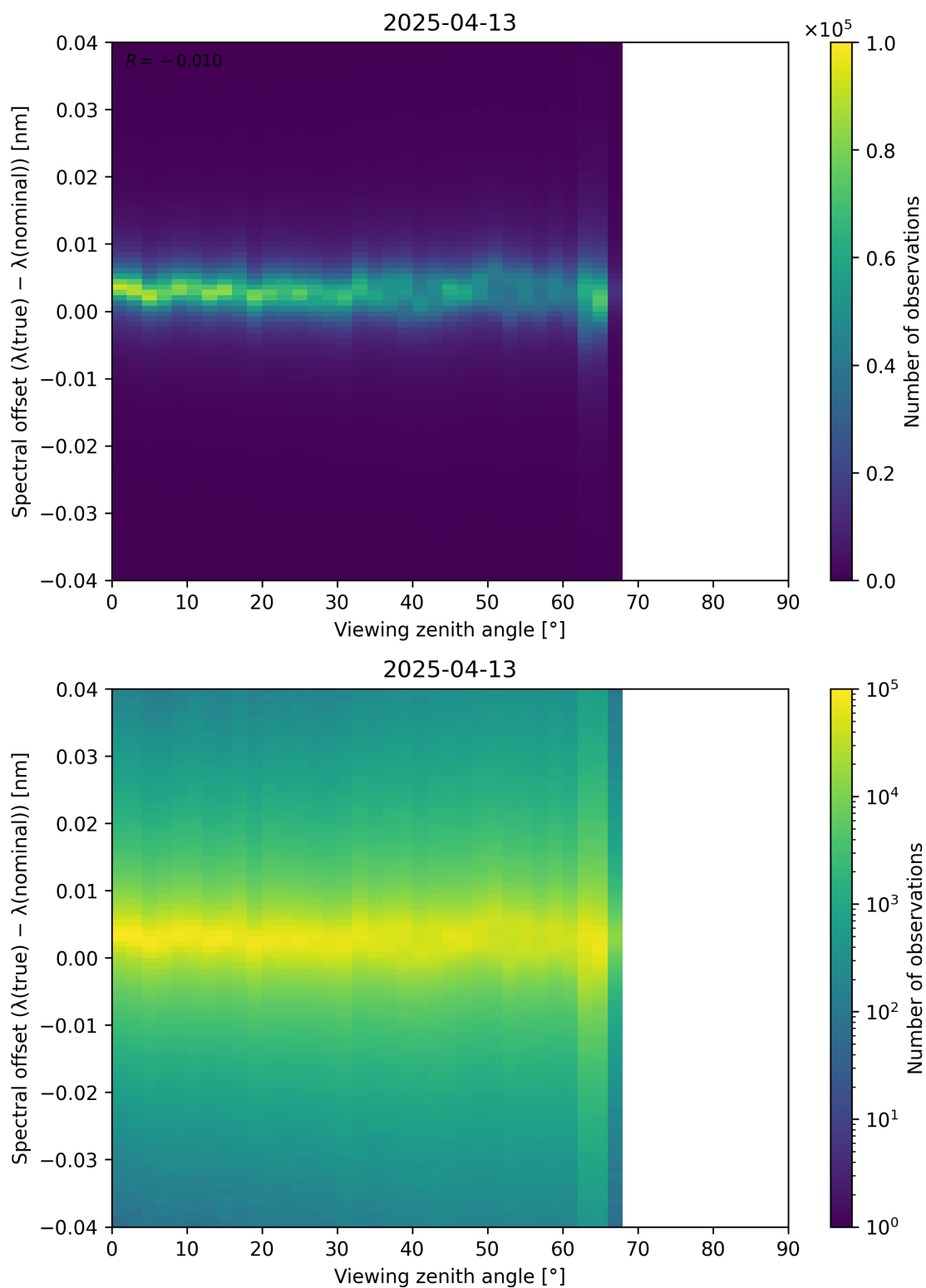
Figure 128: Scatter density plot of “Viewing zenith angle” against “Spectral offset ( \lambda_{\text{true}} - \lambda_{\text{nominal}} )” for 2025-04-13 to 2025-04-14.
