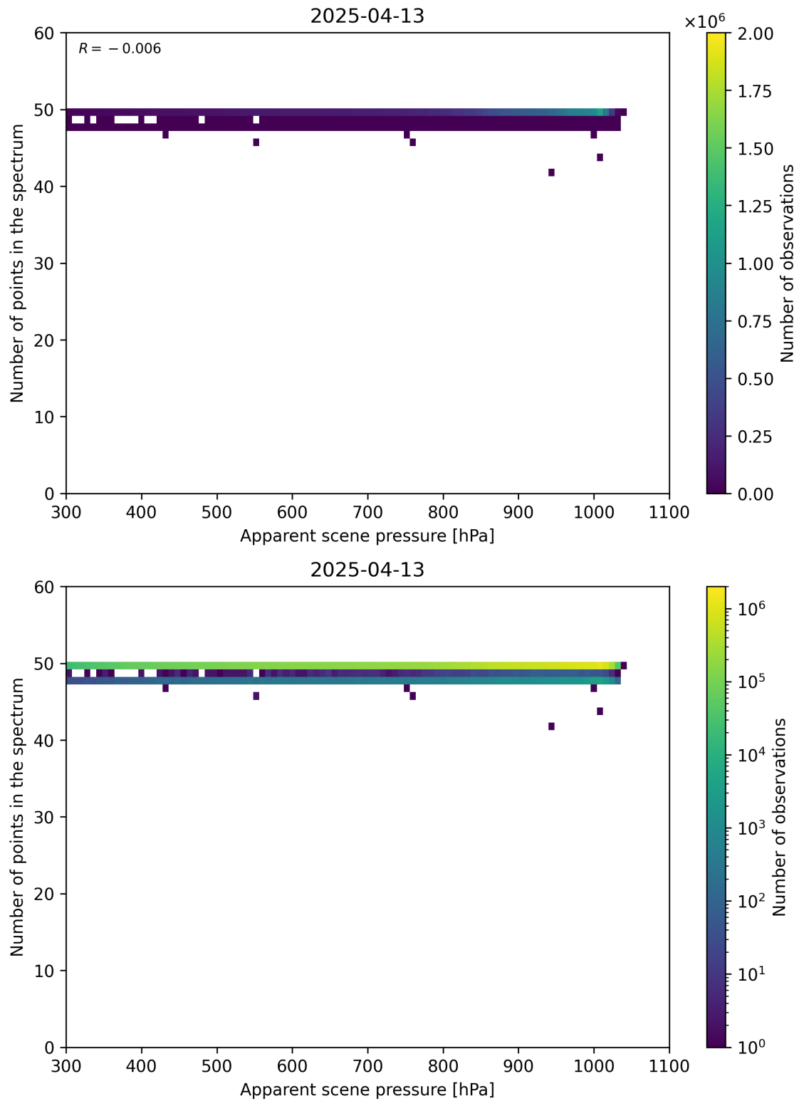
Figure 66: Scatter density plot of “Apparent scene pressure” against “Number of points in the spectrum” for 2025-04-13 to 2025-04-14.
