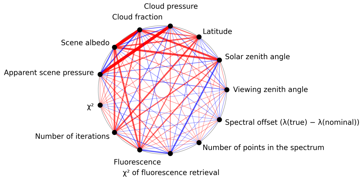
Figure 1: Map of correlation graph for 2025-04-13 to 2025-04-14.
