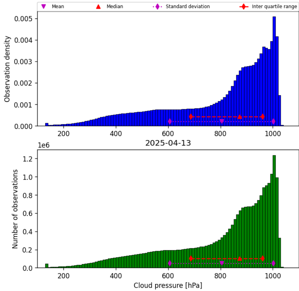
Figure 30: Histogram of “Cloud pressure” for 2025-04-13 to 2025-04-14
