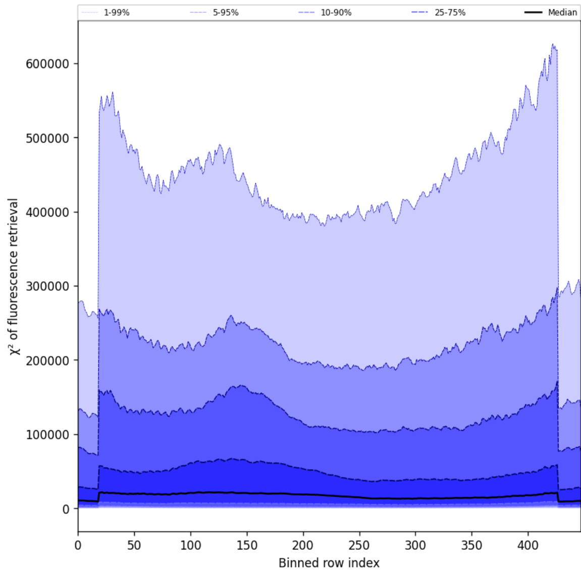
Figure 59: Along track statistics of “ \chi^2 of fluorescence retrieval” for 2025-04-13 to 2025-04-14
