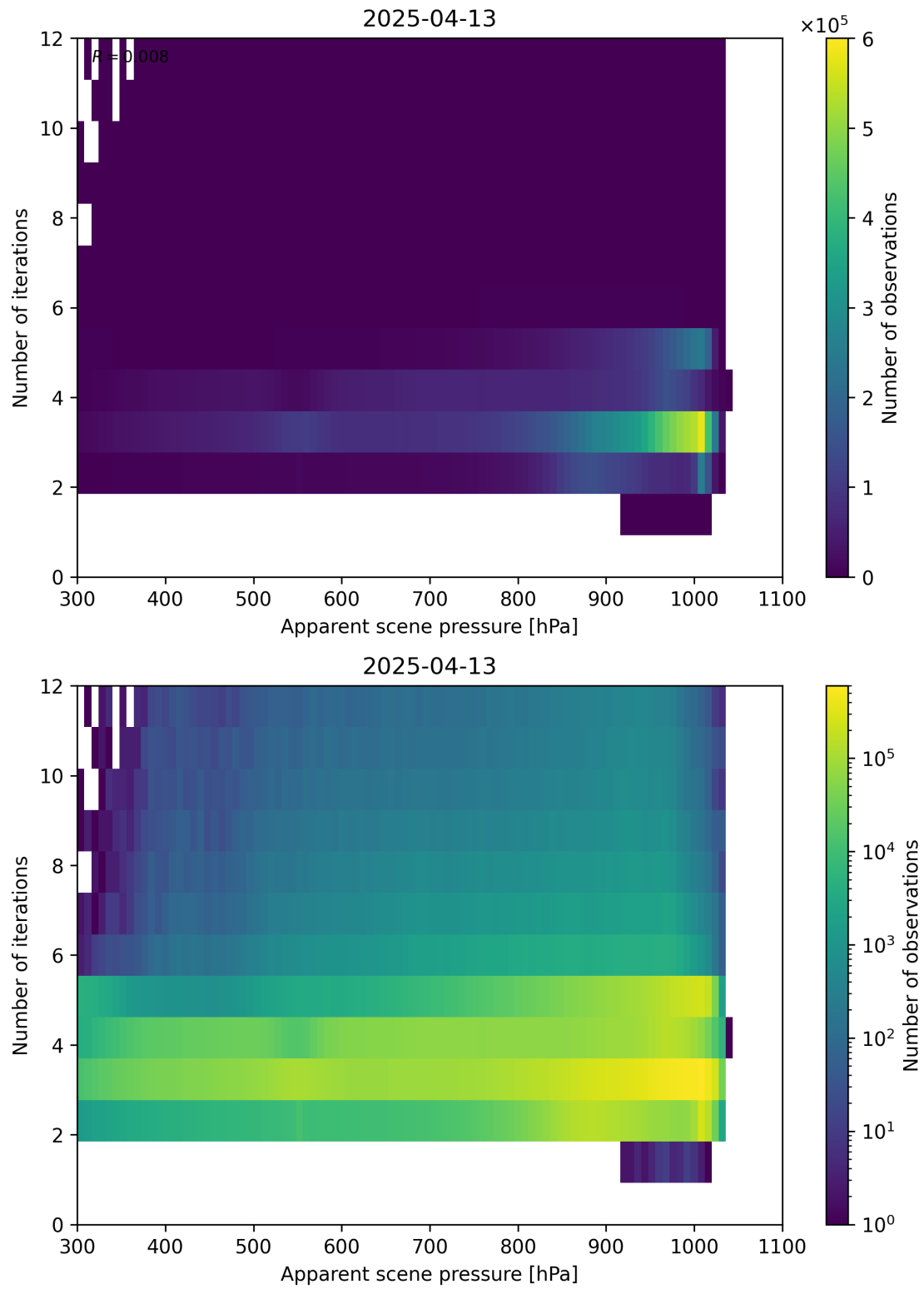
Figure 65: Scatter density plot of “Apparent scene pressure” against “Number of iterations” for 2025-04-13 to 2025-04-14.
