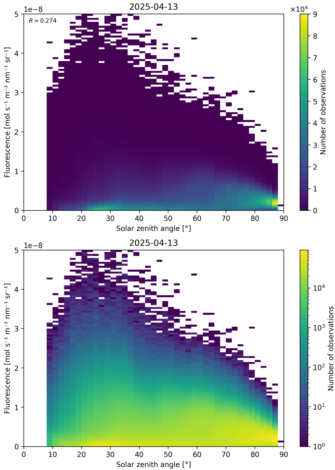
Figure 112: Scatter density plot of “Solar zenith angle” against “Fluorescence” for 2025-04-13 to 2025-04-14.
