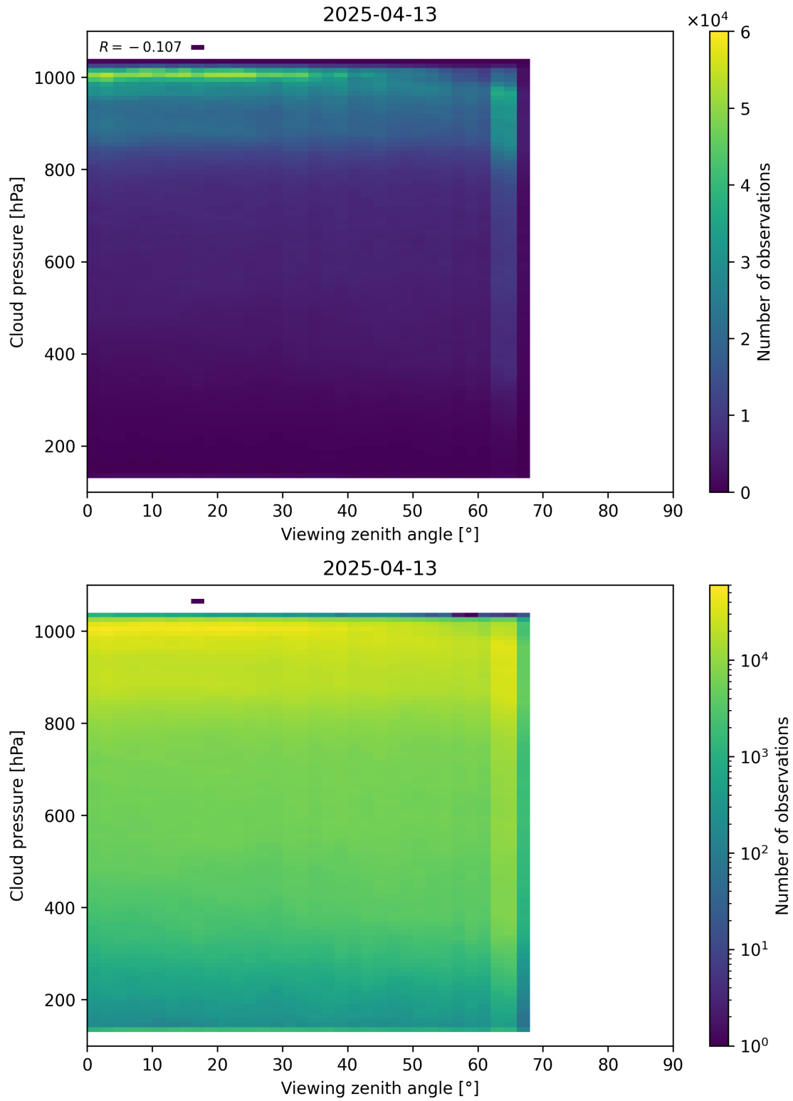
Figure 121: Scatter density plot of “Viewing zenith angle” against “Cloud pressure” for 2025-04-13 to 2025-04-14.
