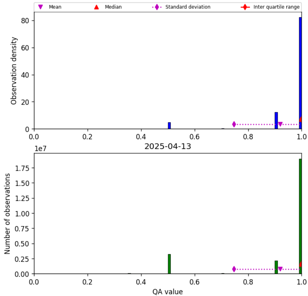
Figure 29: Histogram of “QA value” for 2025-04-13 to 2025-04-14
