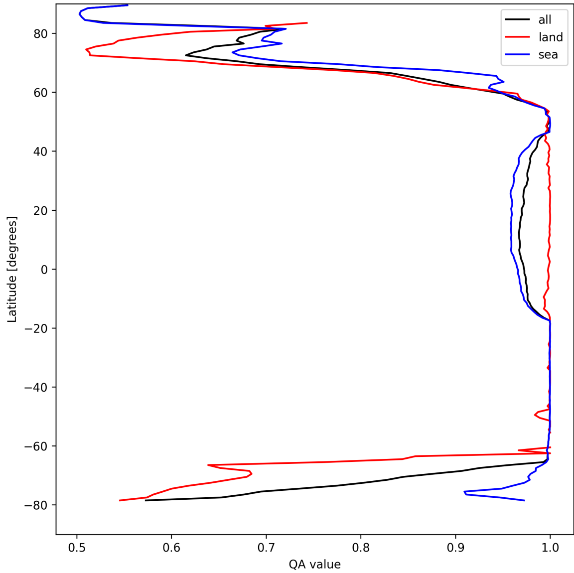
Figure 12: Zonal average of “QA value” for 2025-04-13 to 2025-04-14.
