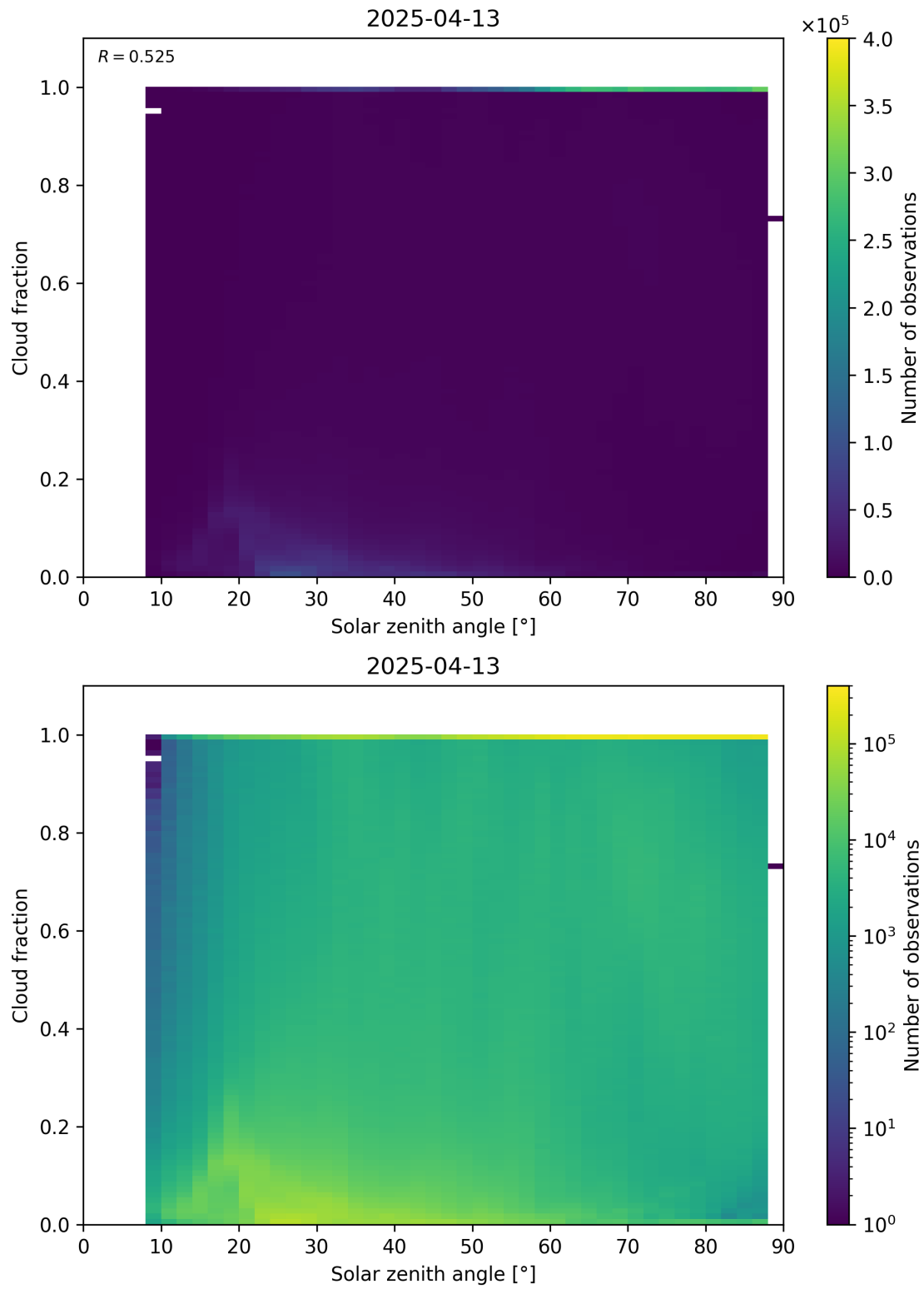
Figure 110: Scatter density plot of “Solar zenith angle” against “Cloud fraction” for 2025-04-13 to 2025-04-14.
