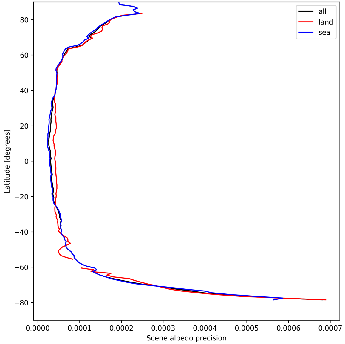
Figure 18: Zonal average of “Scene albedo precision” for 2025-04-13 to 2025-04-14.
