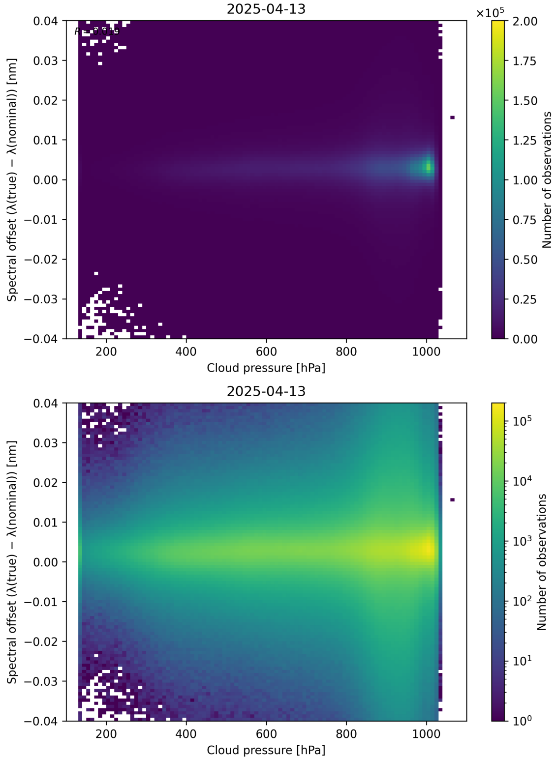
Figure 84: Scatter density plot of “Cloud pressure” against “Spectral offset ( \lambda_{\text{true}} - \lambda_{\text{nominal}} )” for 2025-04-13 to 2025-04-14.
