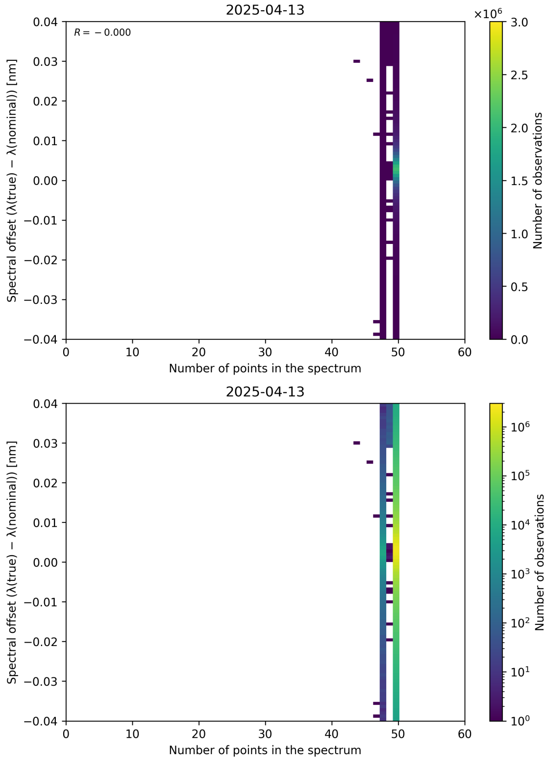
Figure 101: Scatter density plot of “Number of points in the spectrum” against “Spectral offset ( \lambda_{\text{true}} - \lambda_{\text{nominal}} )” for 2025-04-13 to 2025-04-14.
