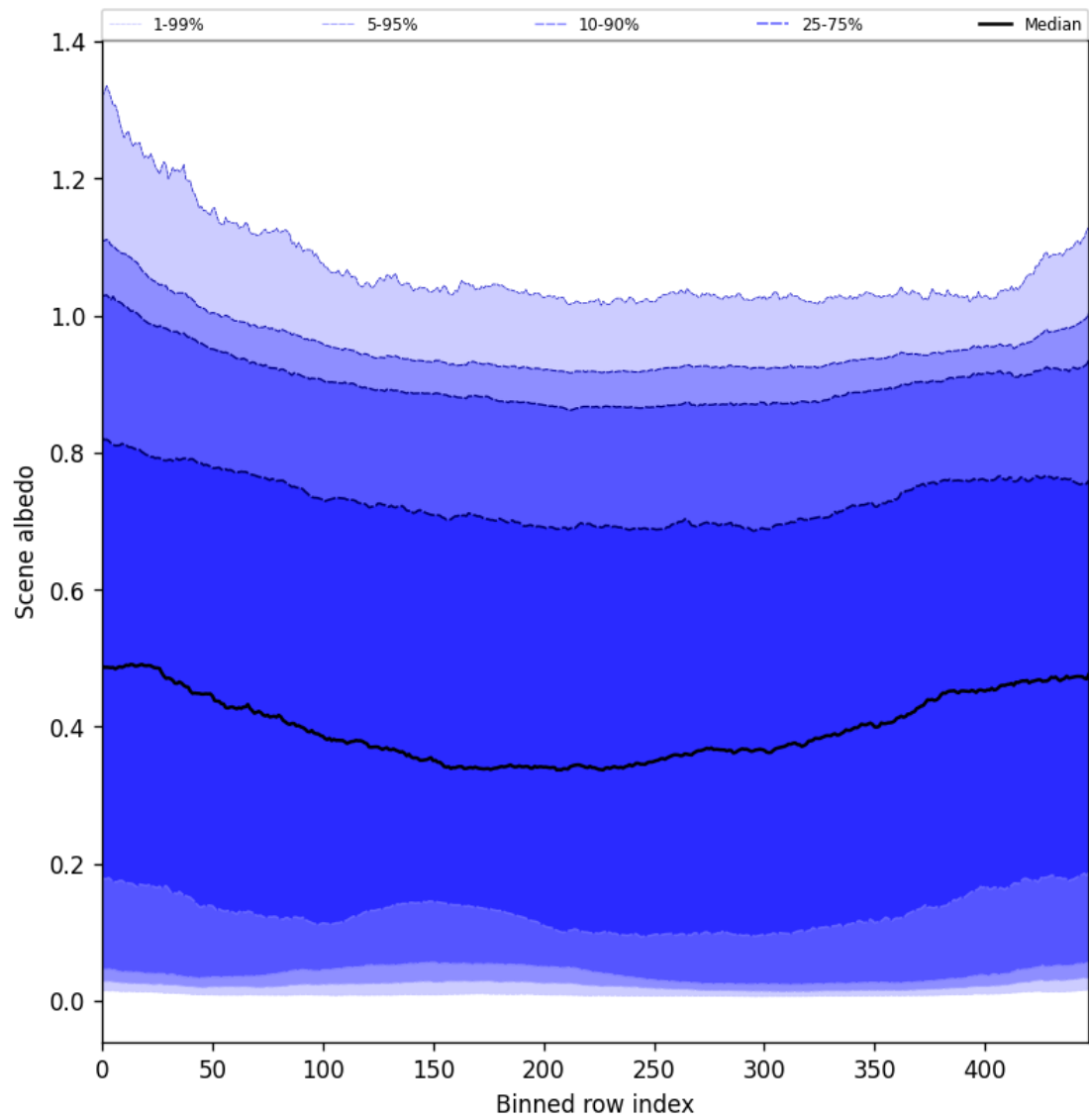
Figure 51: Along track statistics of “Scene albedo” for 2025-04-13 to 2025-04-14
