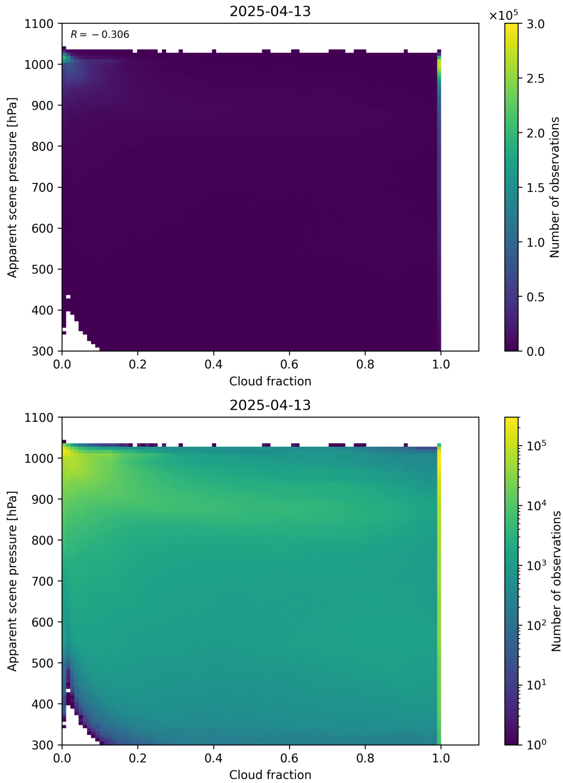
Figure 70: Scatter density plot of “Cloud fraction” against “Apparent scene pressure” for 2025-04-13 to 2025-04-14.
