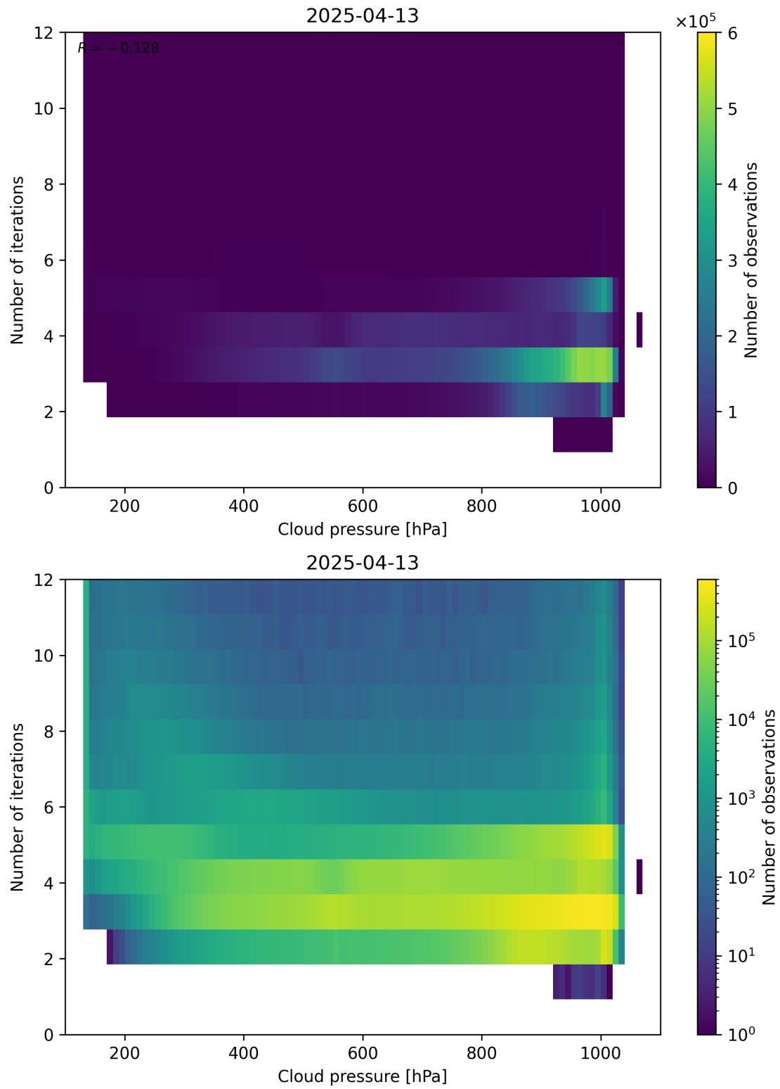
Figure 81: Scatter density plot of “Cloud pressure” against “Number of iterations” for 2025-04-13 to 2025-04-14.
