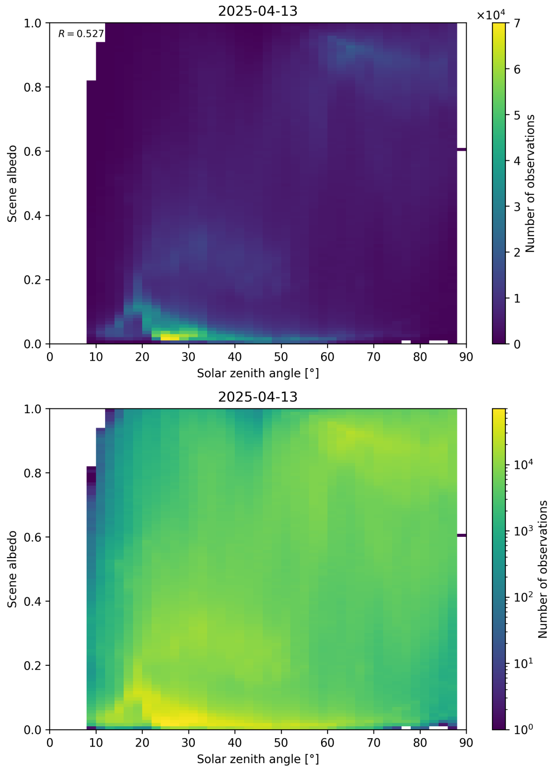
Figure 116: Scatter density plot of “Solar zenith angle” against “Scene albedo” for 2025-04-13 to 2025-04-14.
