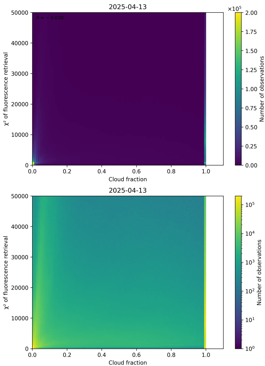
Figure 71: Scatter density plot of “Cloud fraction” against “ \chi^2 of fluorescence retrieval” for 2025-04-13 to 2025-04-14.
