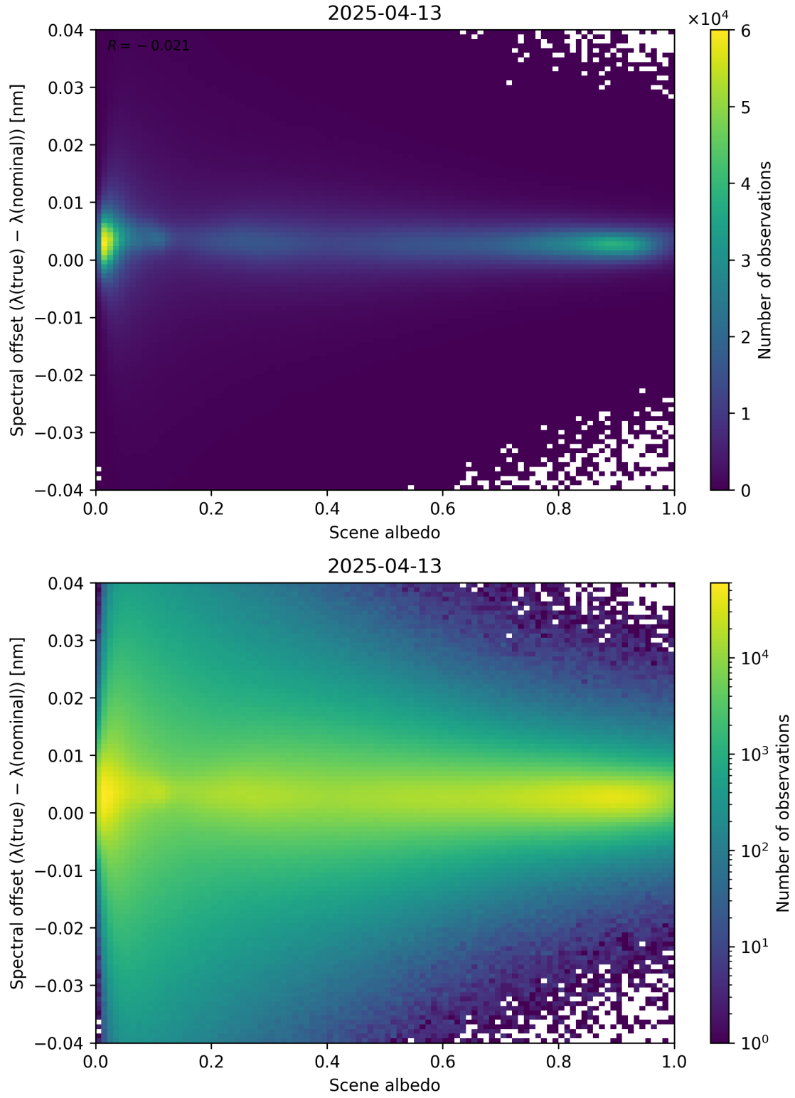
Figure 107: Scatter density plot of “Scene albedo” against “Spectral offset ( \lambda_{\text{true}} - \lambda_{\text{nominal}} )” for 2025-04-13 to 2025-04-14.
