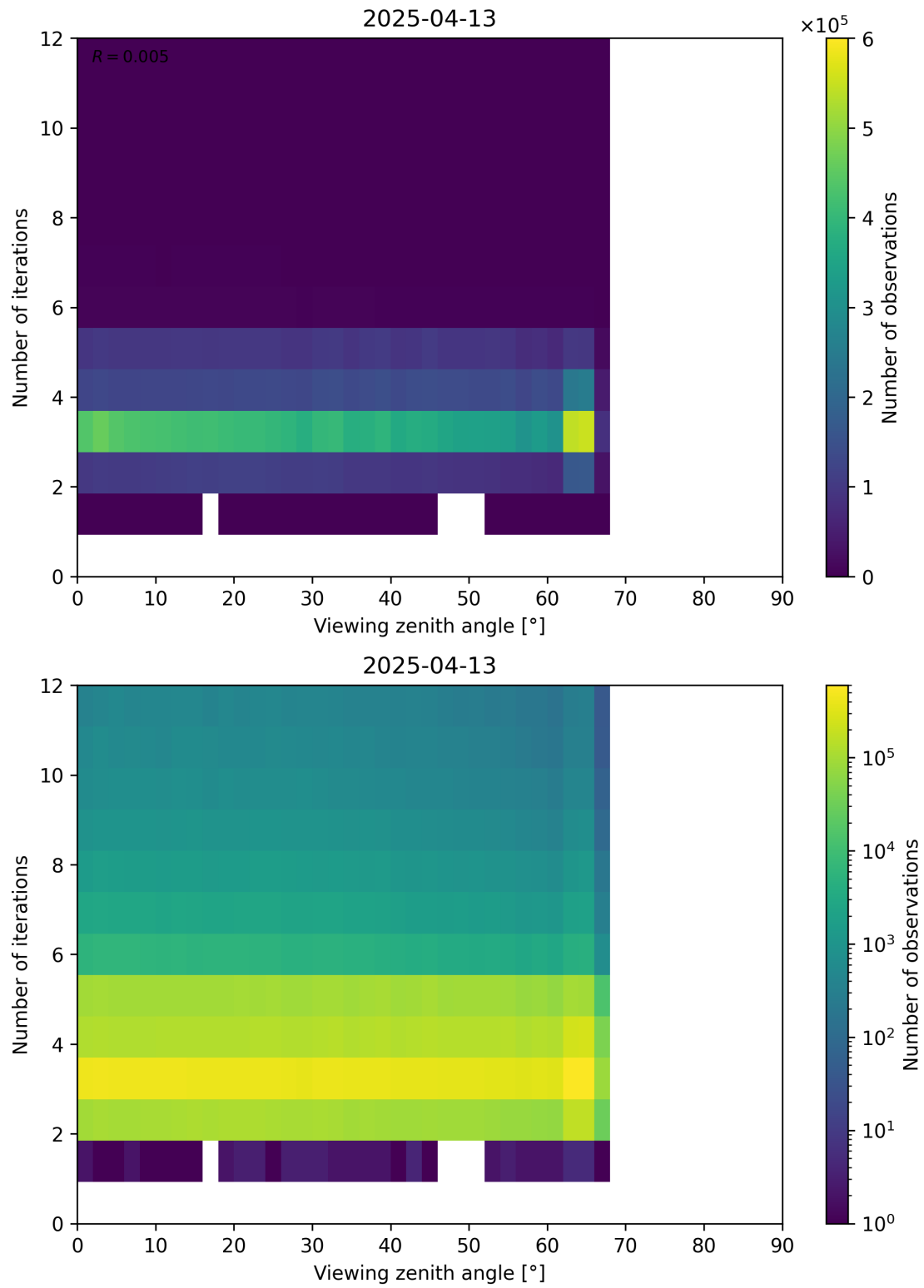
Figure 124: Scatter density plot of “Viewing zenith angle” against “Number of iterations” for 2025-04-13 to 2025-04-14.
