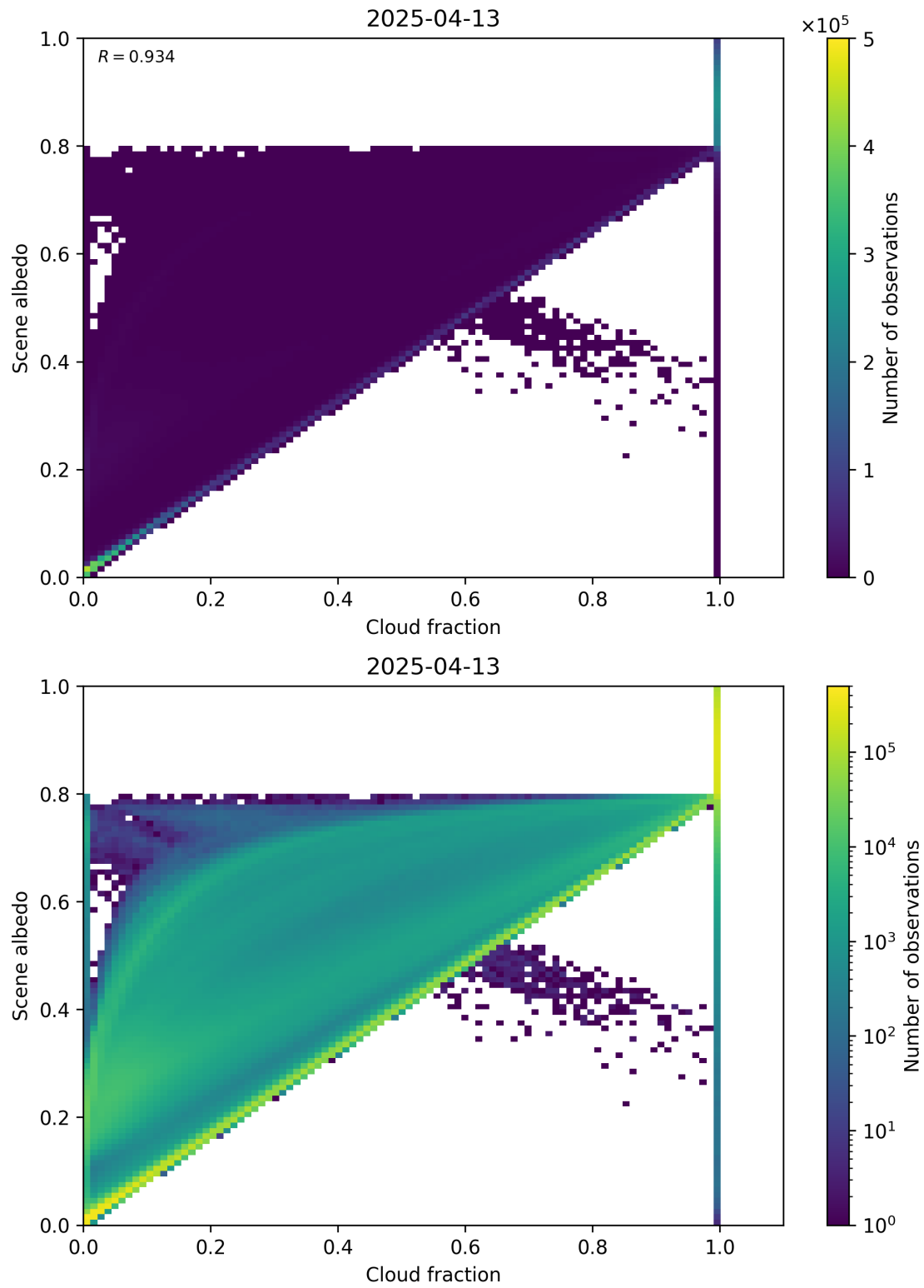
Figure 75: Scatter density plot of “Cloud fraction” against “Scene albedo” for 2025-04-13 to 2025-04-14.
