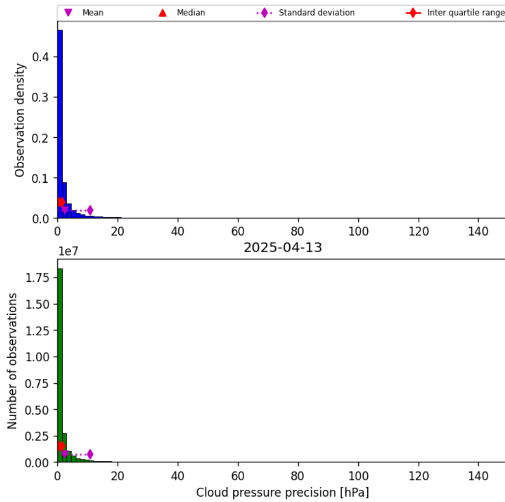
Figure 31: Histogram of “Cloud pressure precision” for 2025-04-13 to 2025-04-14
