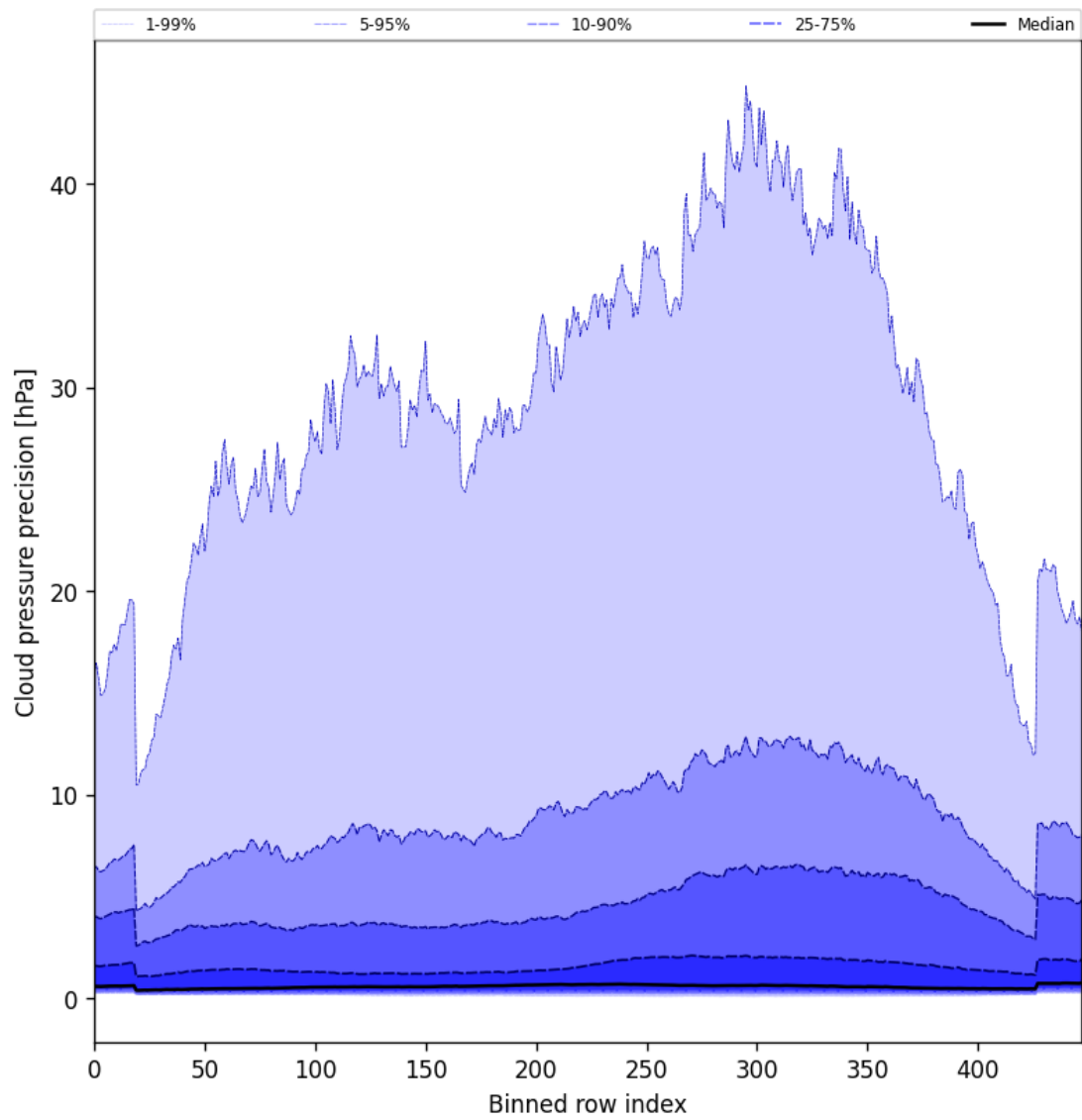
Figure 48: Along track statistics of “Cloud pressure precision” for 2025-04-13 to 2025-04-14
