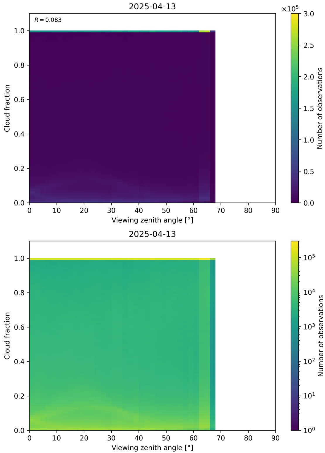
Figure 120: Scatter density plot of “Viewing zenith angle” against “Cloud fraction” for 2025-04-13 to 2025-04-14.
