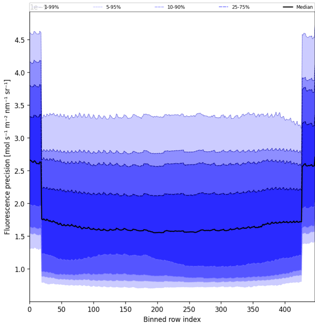
Figure 58: Along track statistics of “Fluorescence precision” for 2025-04-13 to 2025-04-14
