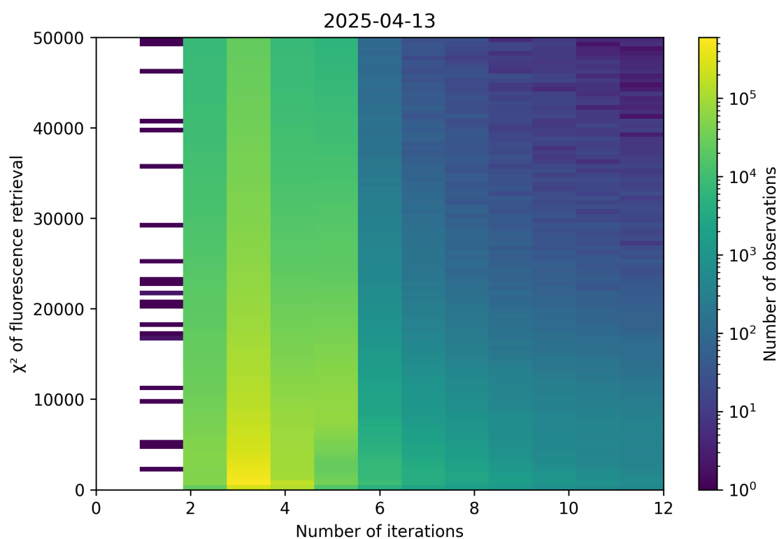
Figure 97: Scatter density plot of “Number of iterations” against “ \chi^2 of fluorescence retrieval” for 2025-04-13 to 2025-04-14.
