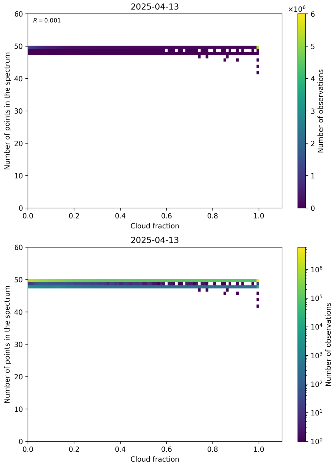
Figure 74: Scatter density plot of “Cloud fraction” against “Number of points in the spectrum” for 2025-04-13 to 2025-04-14.
