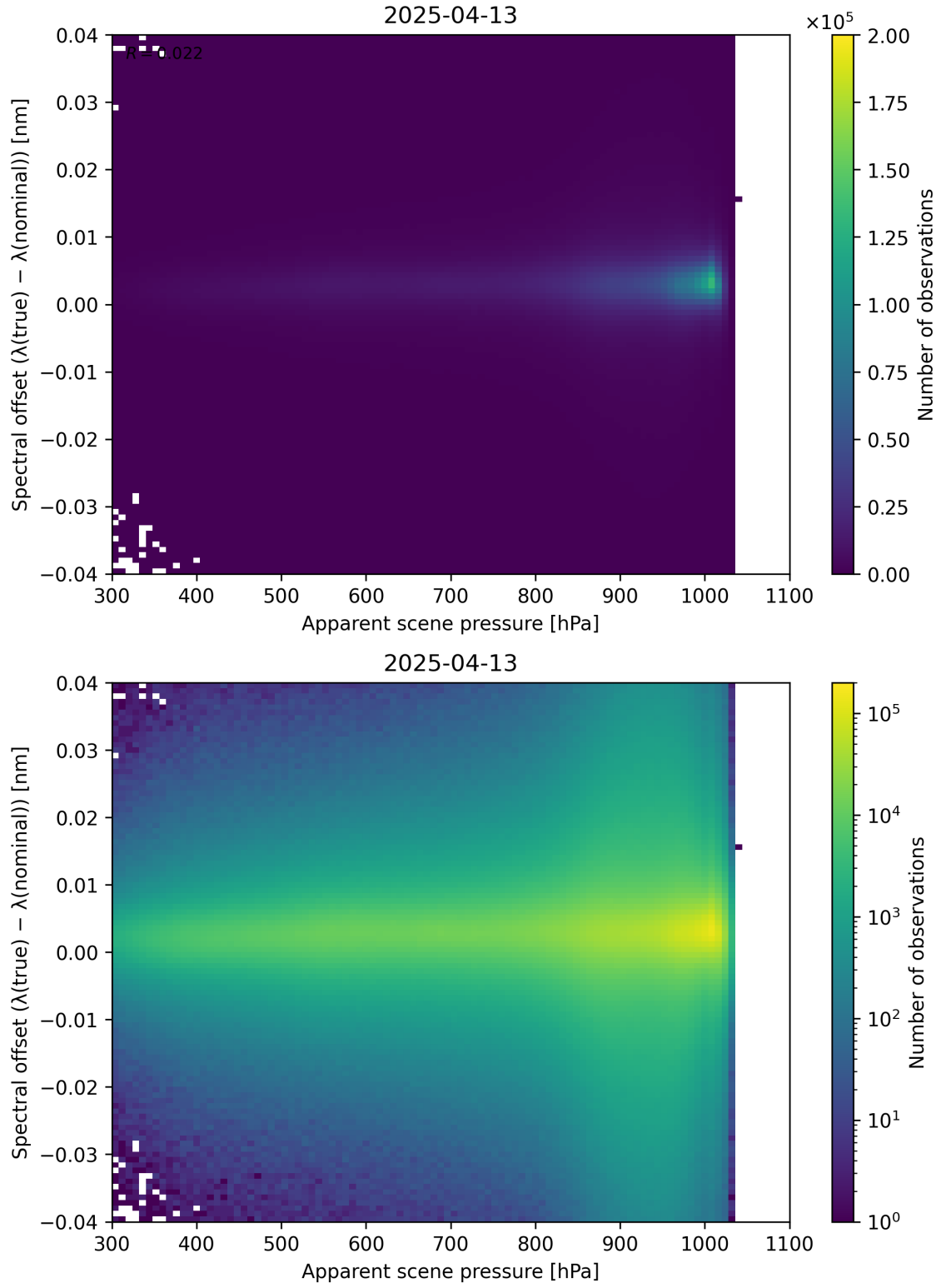
Figure 67: Scatter density plot of “Apparent scene pressure” against “Spectral offset ( \lambda_{\text{true}} - \lambda_{\text{nominal}} )” for 2025-04-13 to 2025-04-14.
