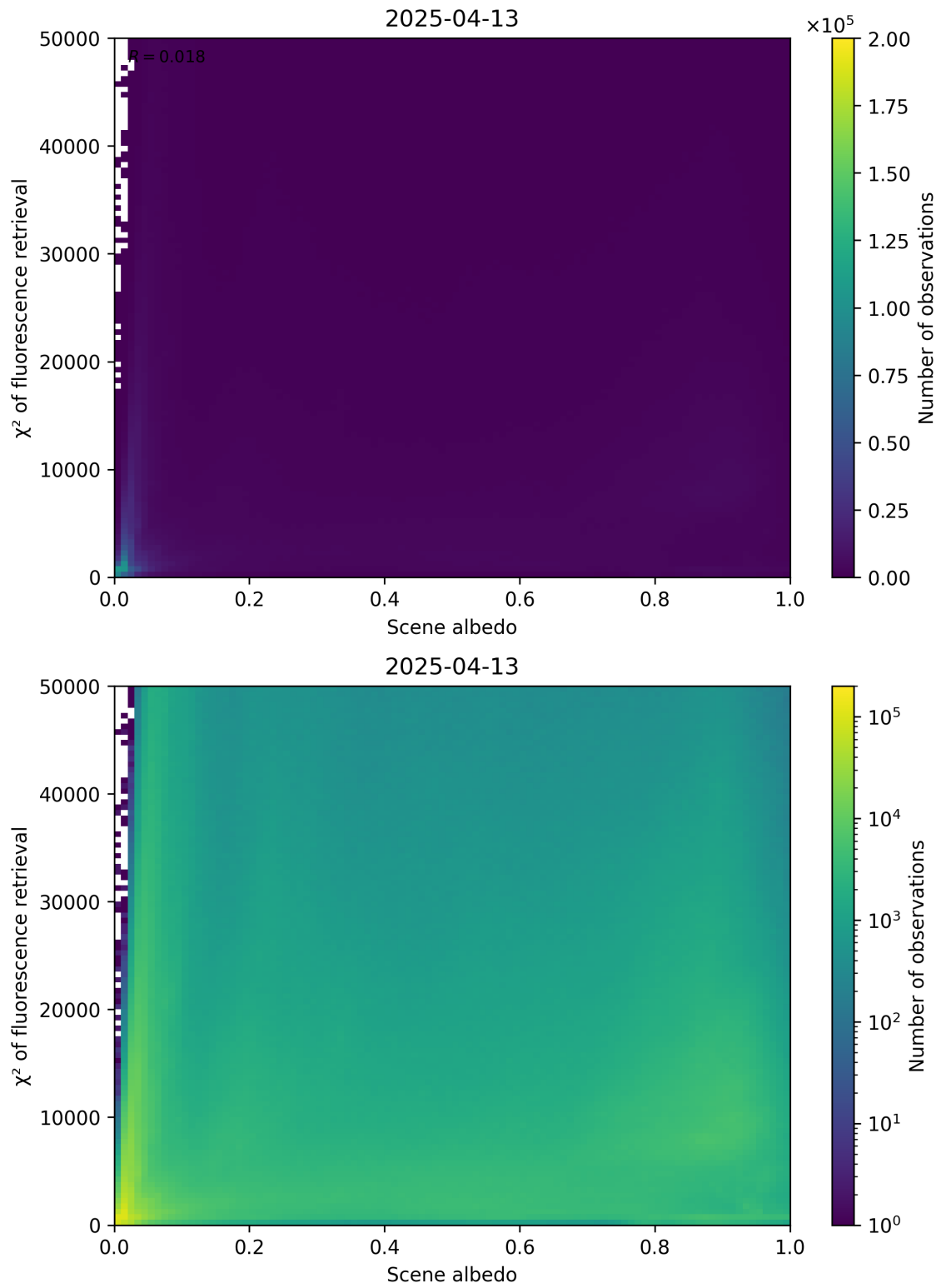
Figure 103: Scatter density plot of “Scene albedo” against “ \chi^2 of fluorescence retrieval” for 2025-04-13 to 2025-04-14.
