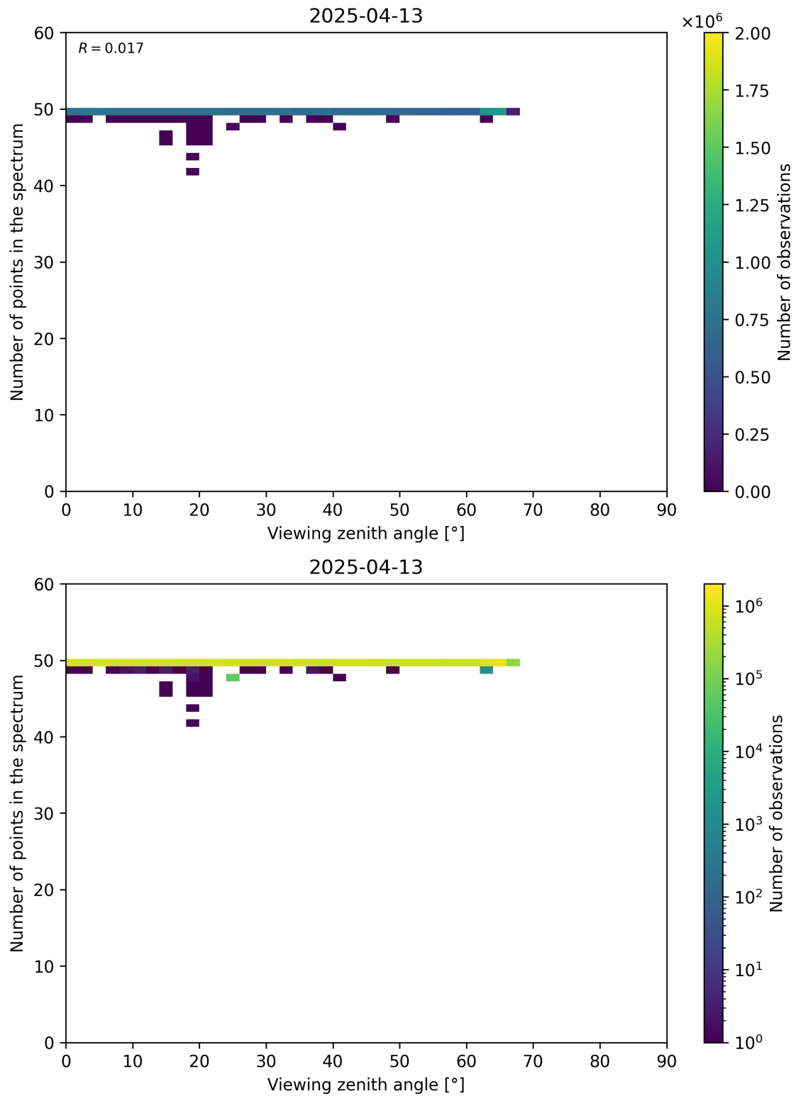
Figure 125: Scatter density plot of “Viewing zenith angle” against “Number of points in the spectrum” for 2025-04-13 to 2025-04-14.
