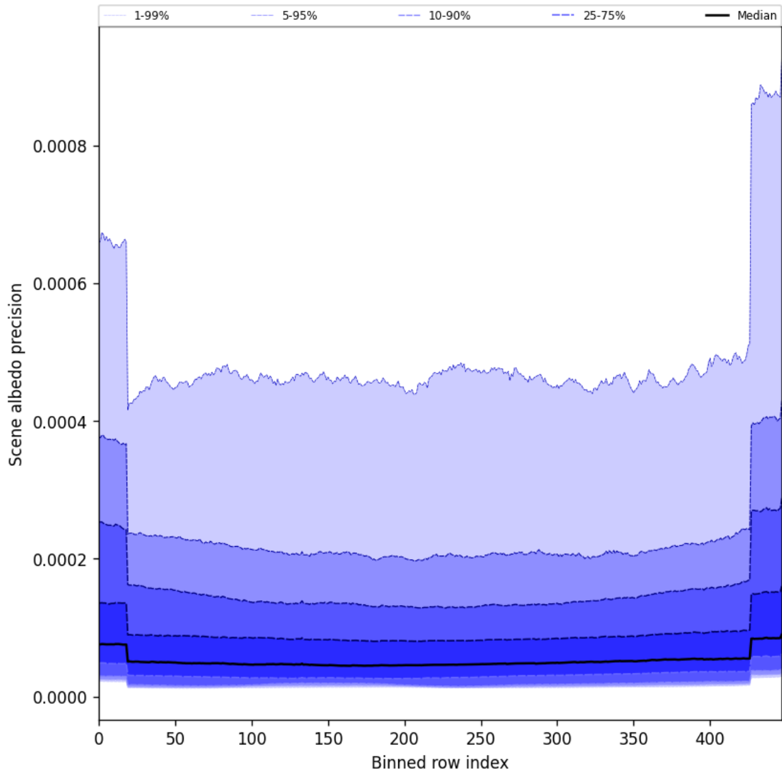
Figure 52: Along track statistics of “Scene albedo precision” for 2025-04-13 to 2025-04-14
