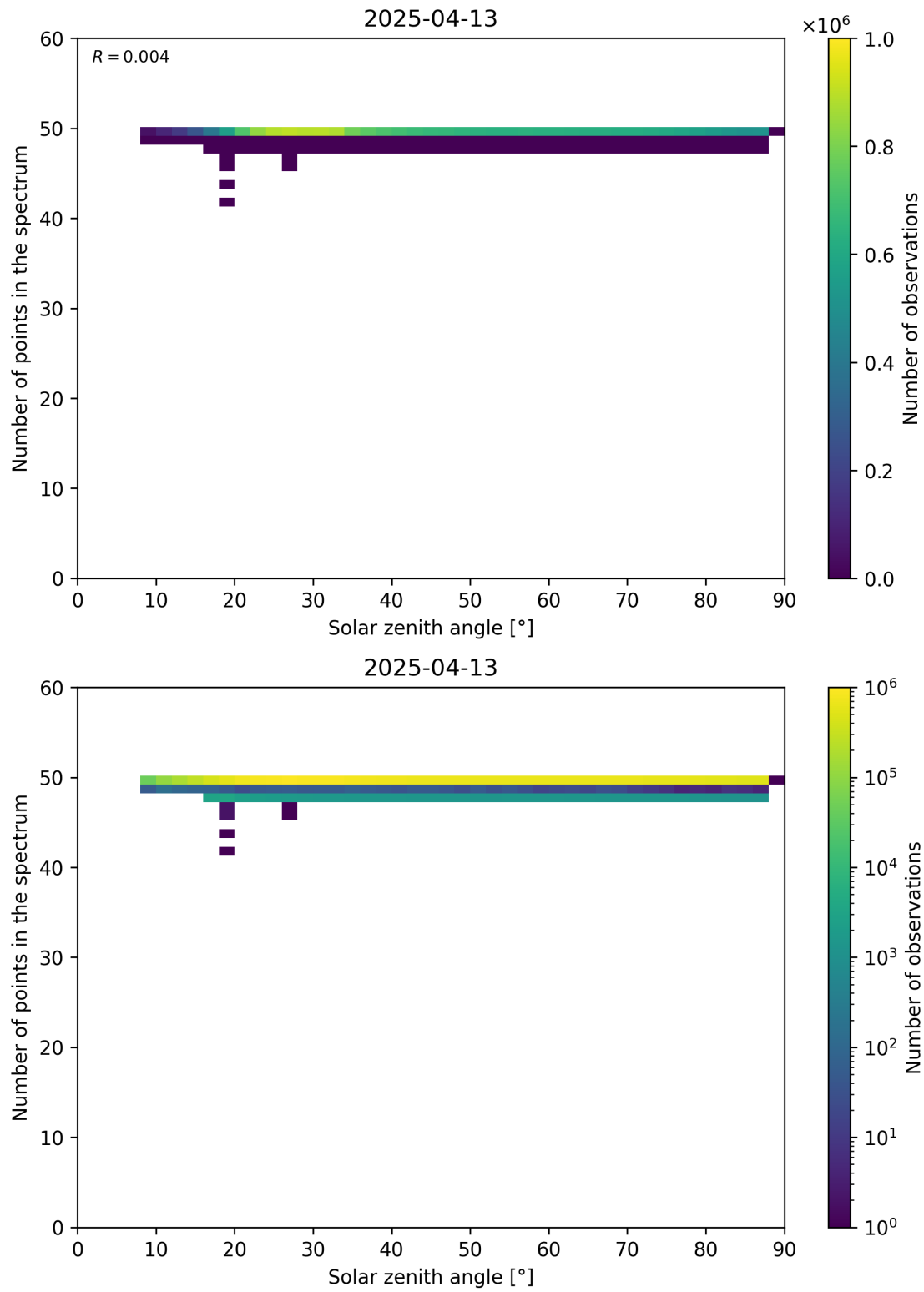
Figure 115: Scatter density plot of “Solar zenith angle” against “Number of points in the spectrum” for 2025-04-13 to 2025-04-14.
