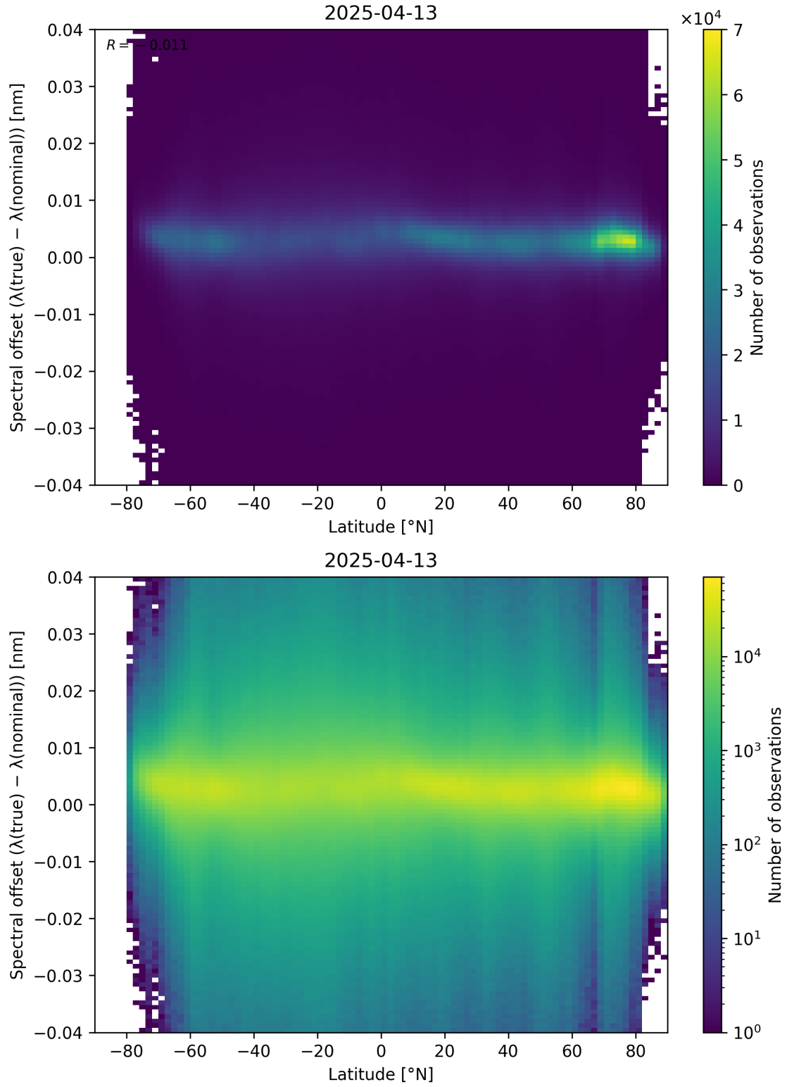
Figure 96: Scatter density plot of “Latitude” against “Spectral offset ( \lambda_{\text{true}} - \lambda_{\text{nominal}} )” for 2025-04-13 to 2025-04-14.
