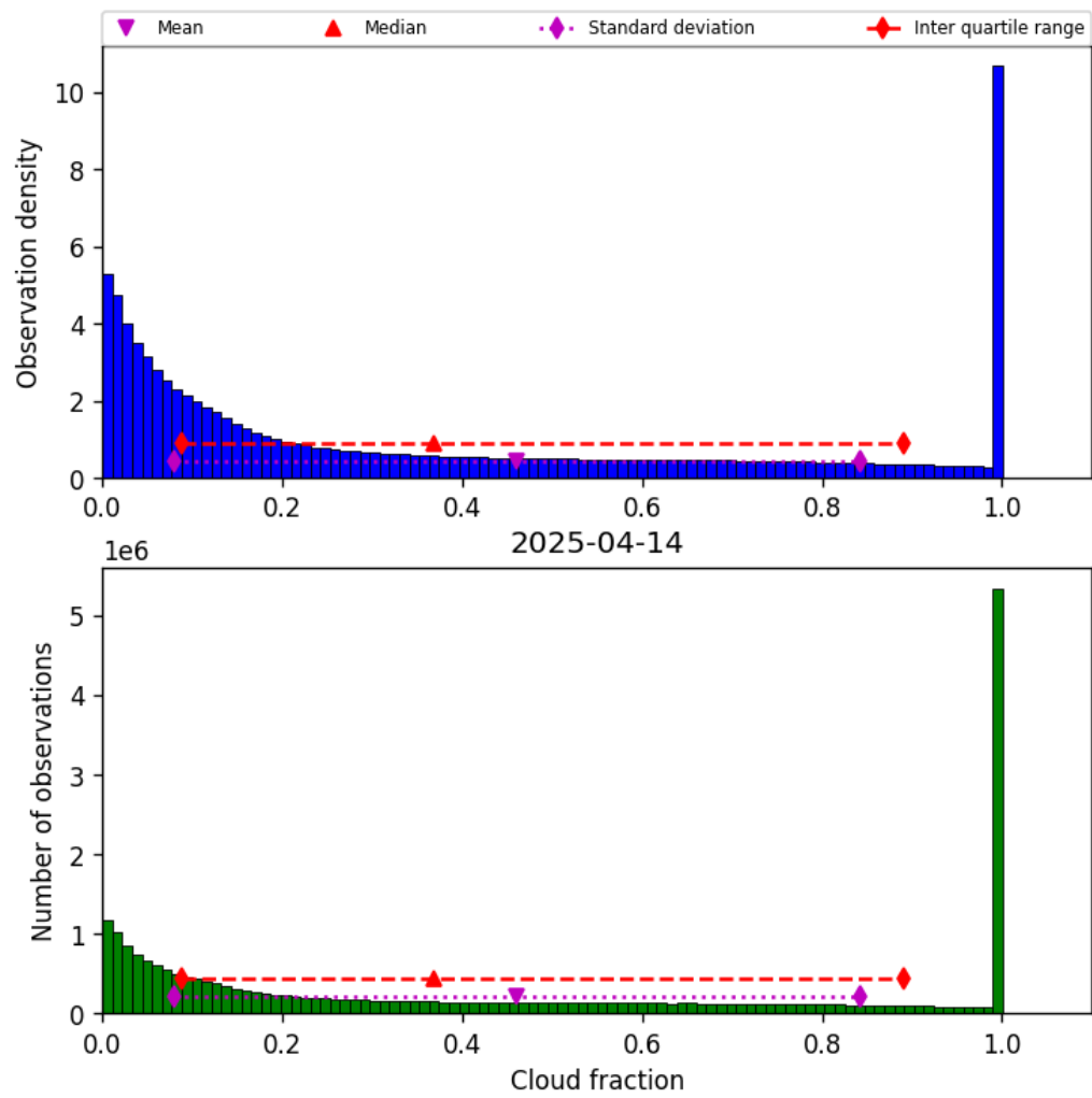
Figure 32: Histogram of “Cloud fraction” for 2025-04-13 to 2025-04-15
