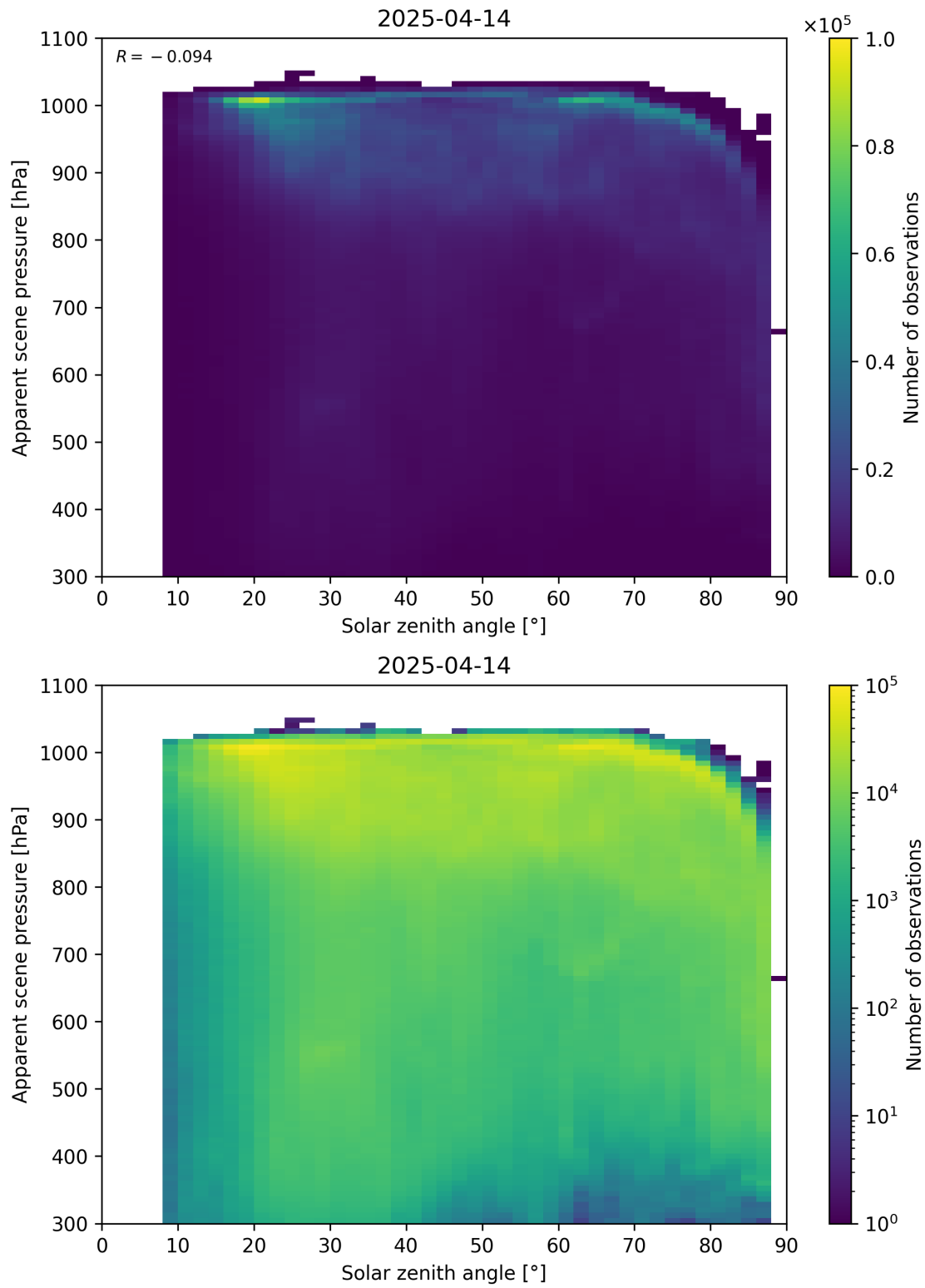
Figure 108: Scatter density plot of “Solar zenith angle” against “Apparent scene pressure” for 2025-04-13 to 2025-04-15.
