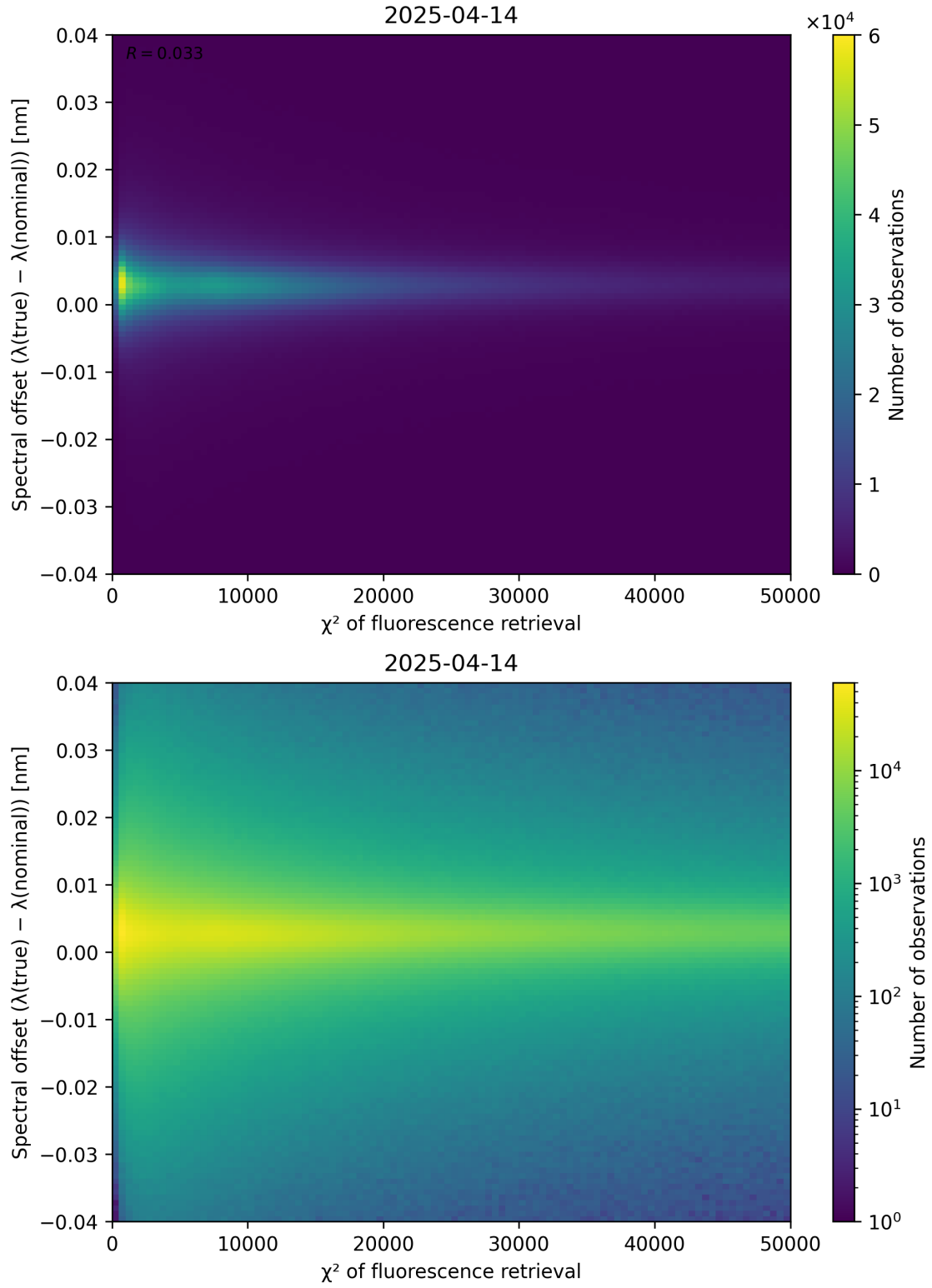
Figure 69: Scatter density plot of “ \chi^2 of fluorescence retrieval” against “Spectral offset ( \lambda_{\text{true}} - \lambda_{\text{nominal}} )” for 2025-04-13 to 2025-04-15.
