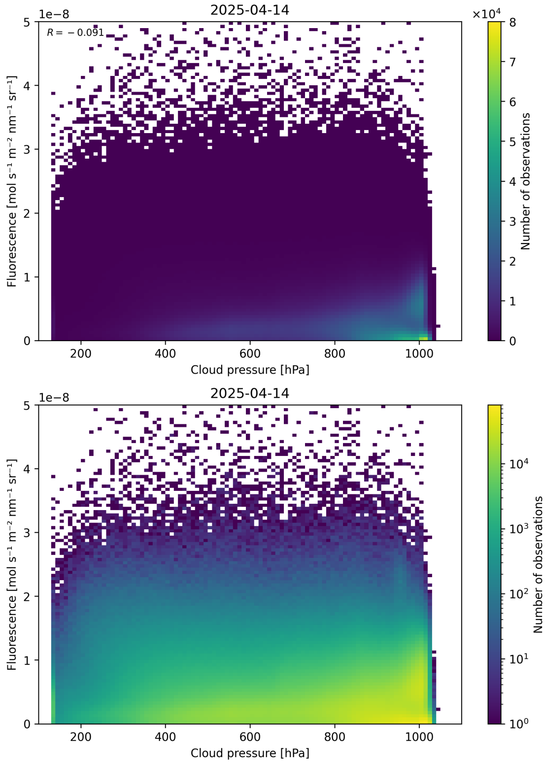
Figure 80: Scatter density plot of “Cloud pressure” against “Fluorescence” for 2025-04-13 to 2025-04-15.
