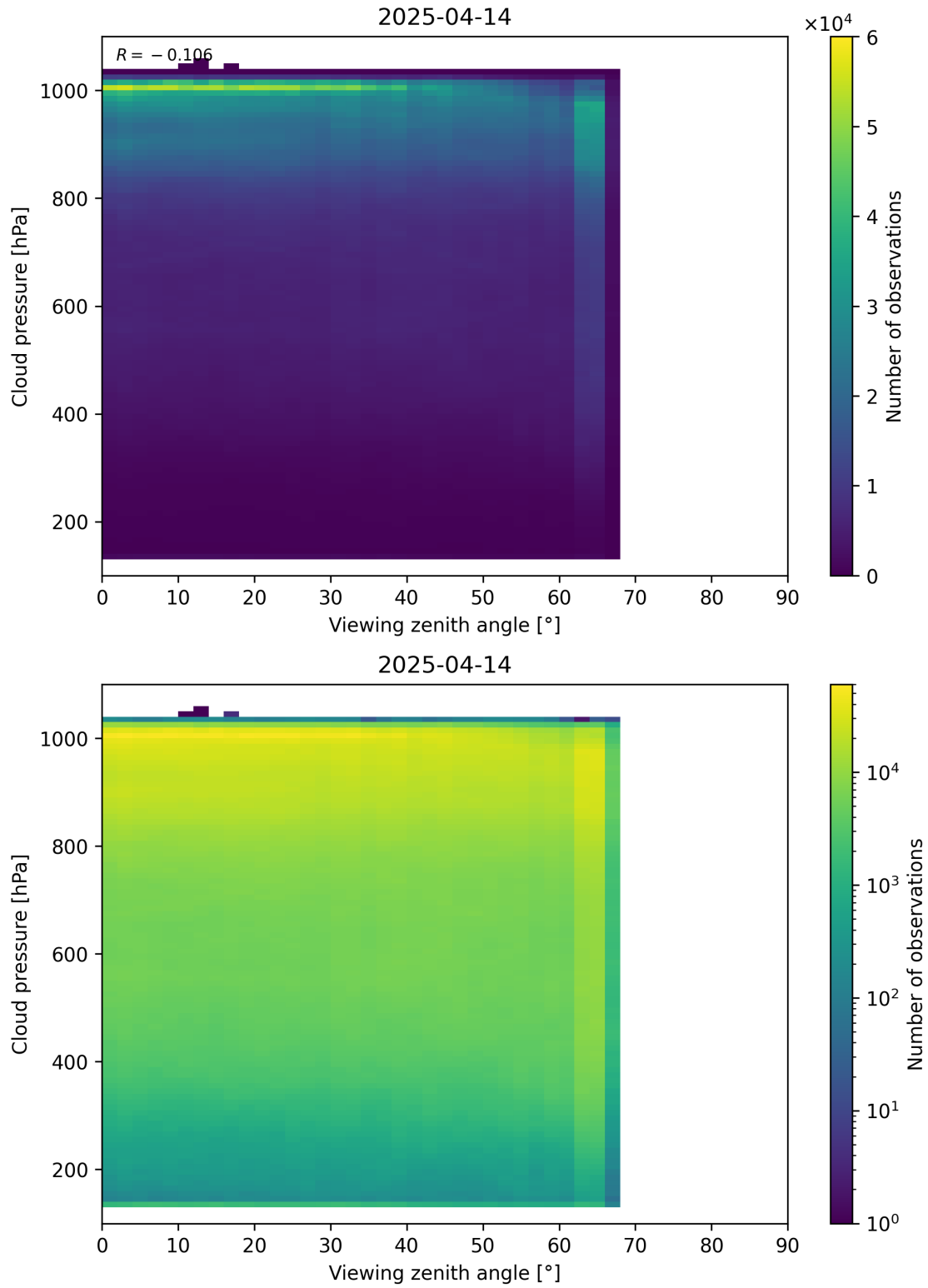
Figure 121: Scatter density plot of “Viewing zenith angle” against “Cloud pressure” for 2025-04-13 to 2025-04-15.
