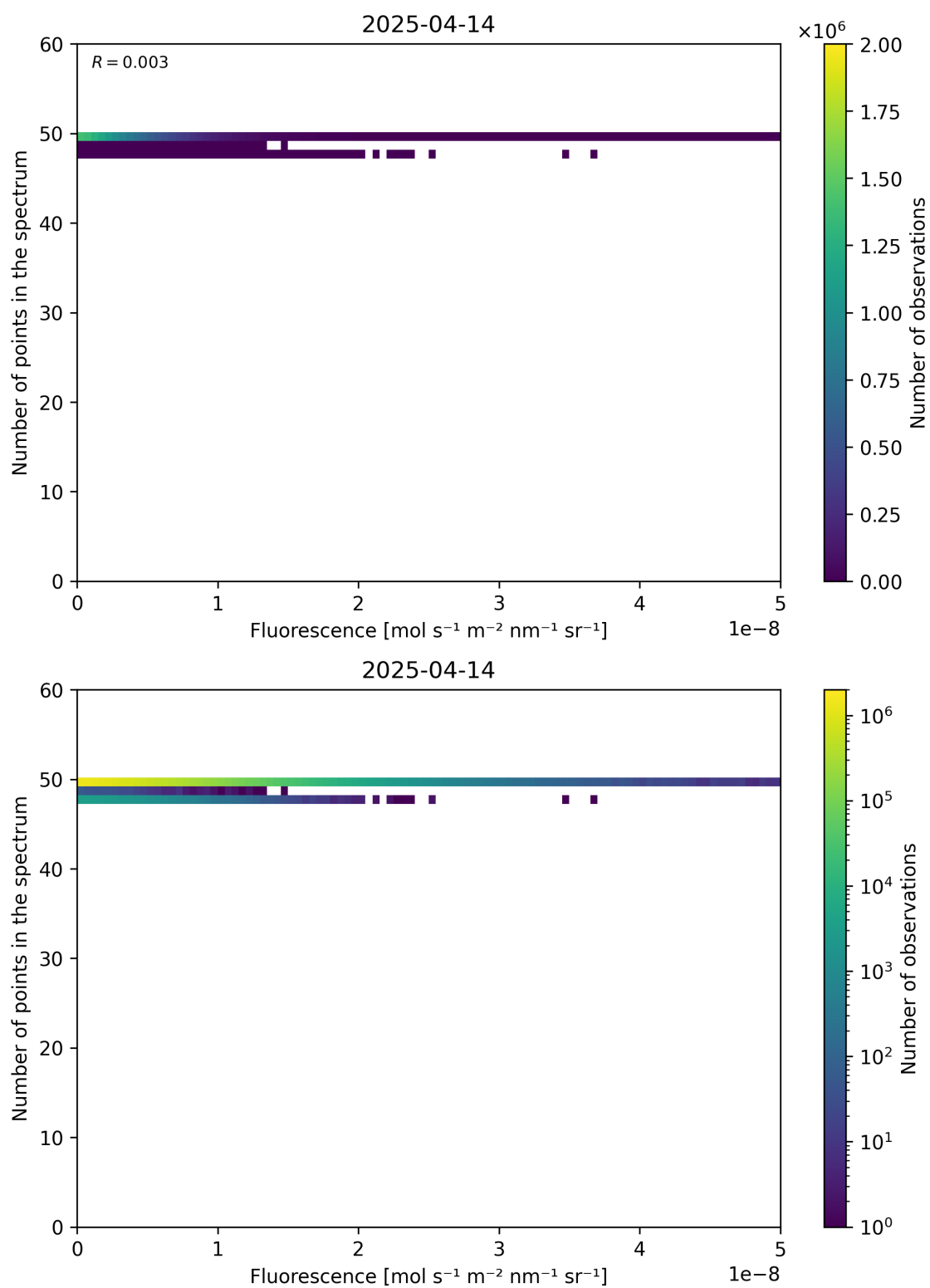
Figure 86: Scatter density plot of “Fluorescence” against “Number of points in the spectrum” for 2025-04-13 to 2025-04-15.
