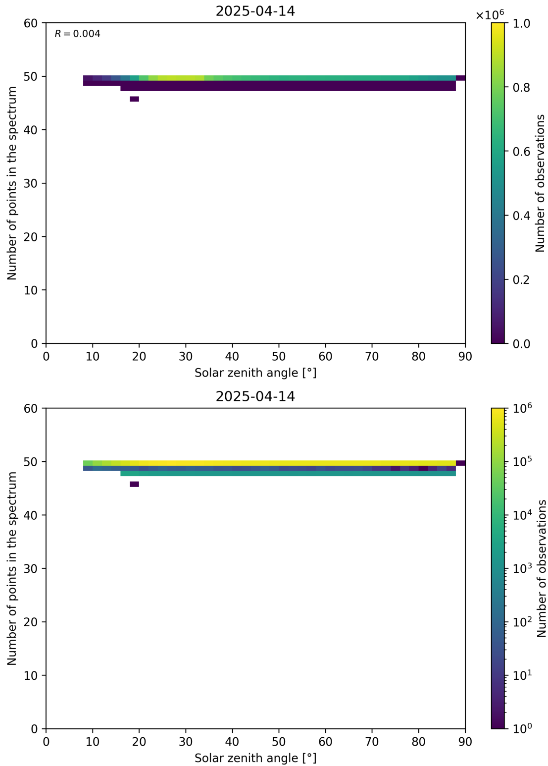
Figure 115: Scatter density plot of “Solar zenith angle” against “Number of points in the spectrum” for 2025-04-13 to 2025-04-15.
