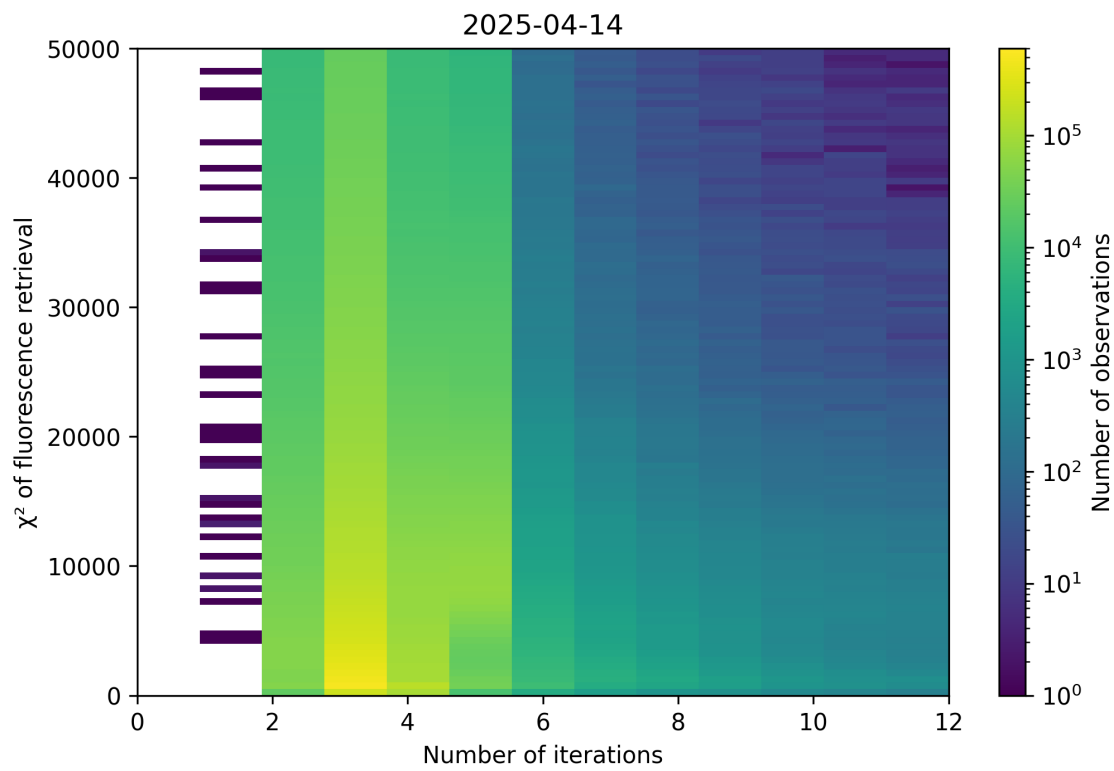
Figure 97: Scatter density plot of “Number of iterations” against “ \chi^2 of fluorescence retrieval” for 2025-04-13 to 2025-04-15.
