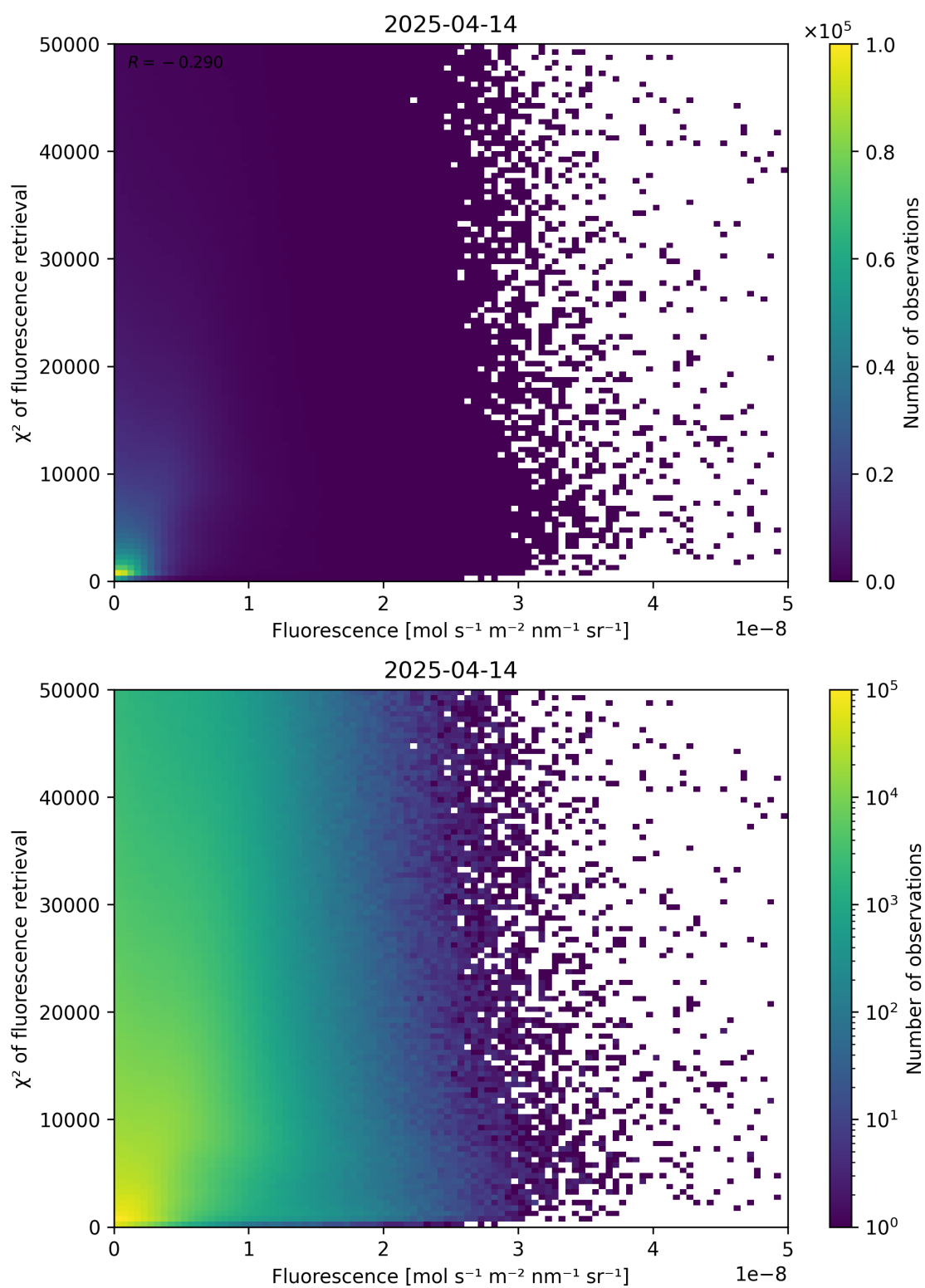
Figure 85: Scatter density plot of “Fluorescence” against “ \chi^2 of fluorescence retrieval” for 2025-04-13 to 2025-04-15.
