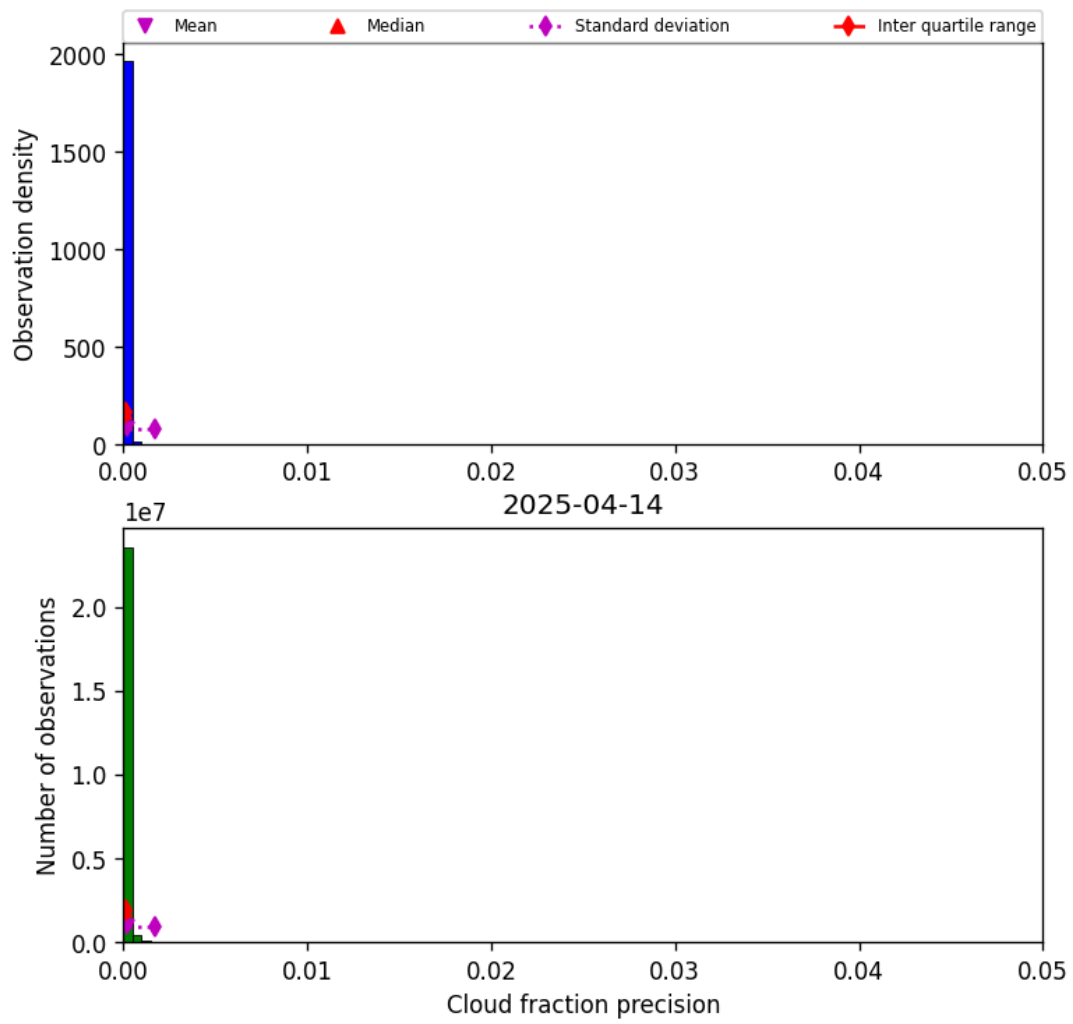
Figure 33: Histogram of “Cloud fraction precision” for 2025-04-13 to 2025-04-15
