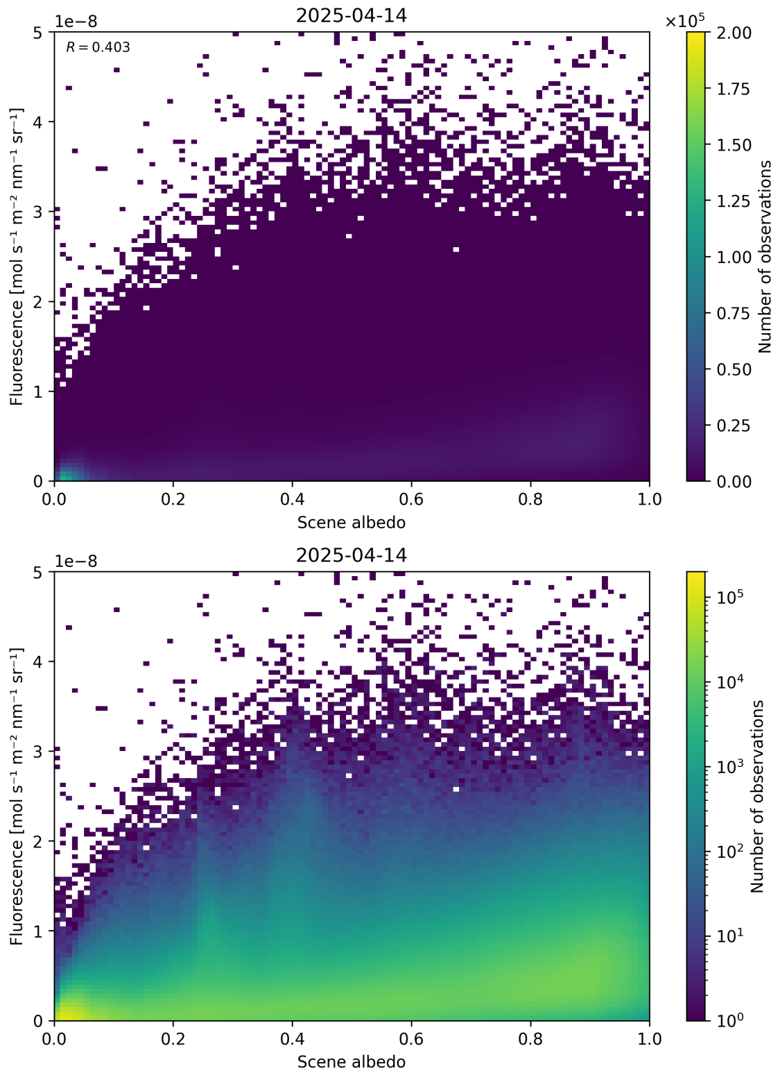
Figure 104: Scatter density plot of "Scene albedo" against "Fluorescence" for 2025-04-13 to 2025-04-15.
