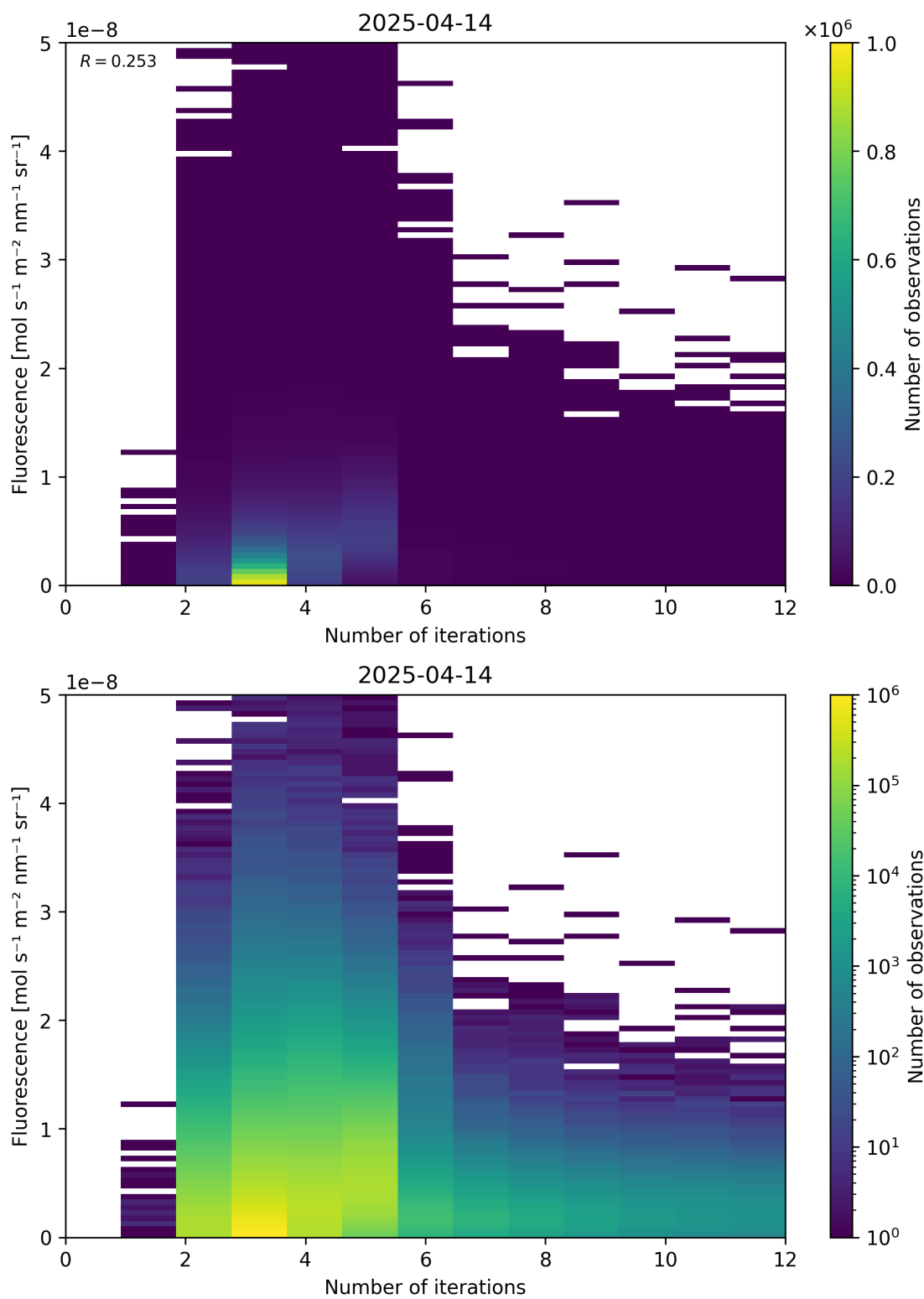
Figure 98: Scatter density plot of “Number of iterations” against “Fluorescence” for 2025-04-13 to 2025-04-15.
