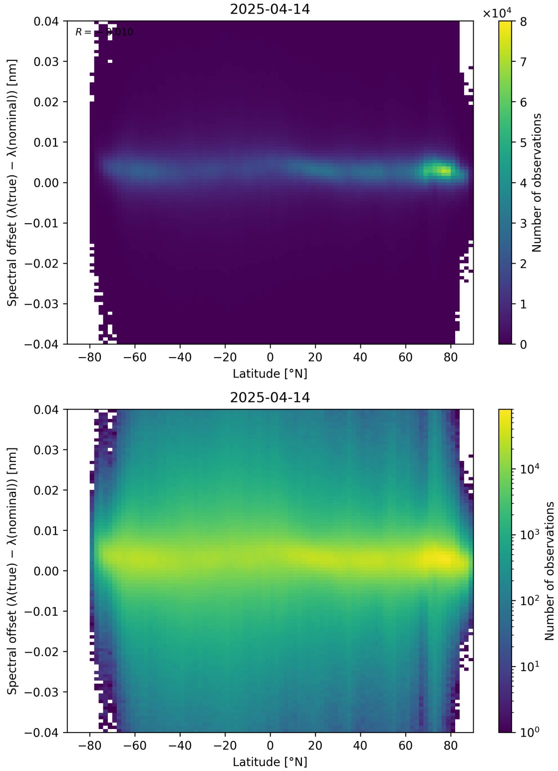
Figure 96: Scatter density plot of “Latitude” against “Spectral offset ( \lambda_{\text{true}} - \lambda_{\text{nominal}} )” for 2025-04-13 to 2025-04-15.
