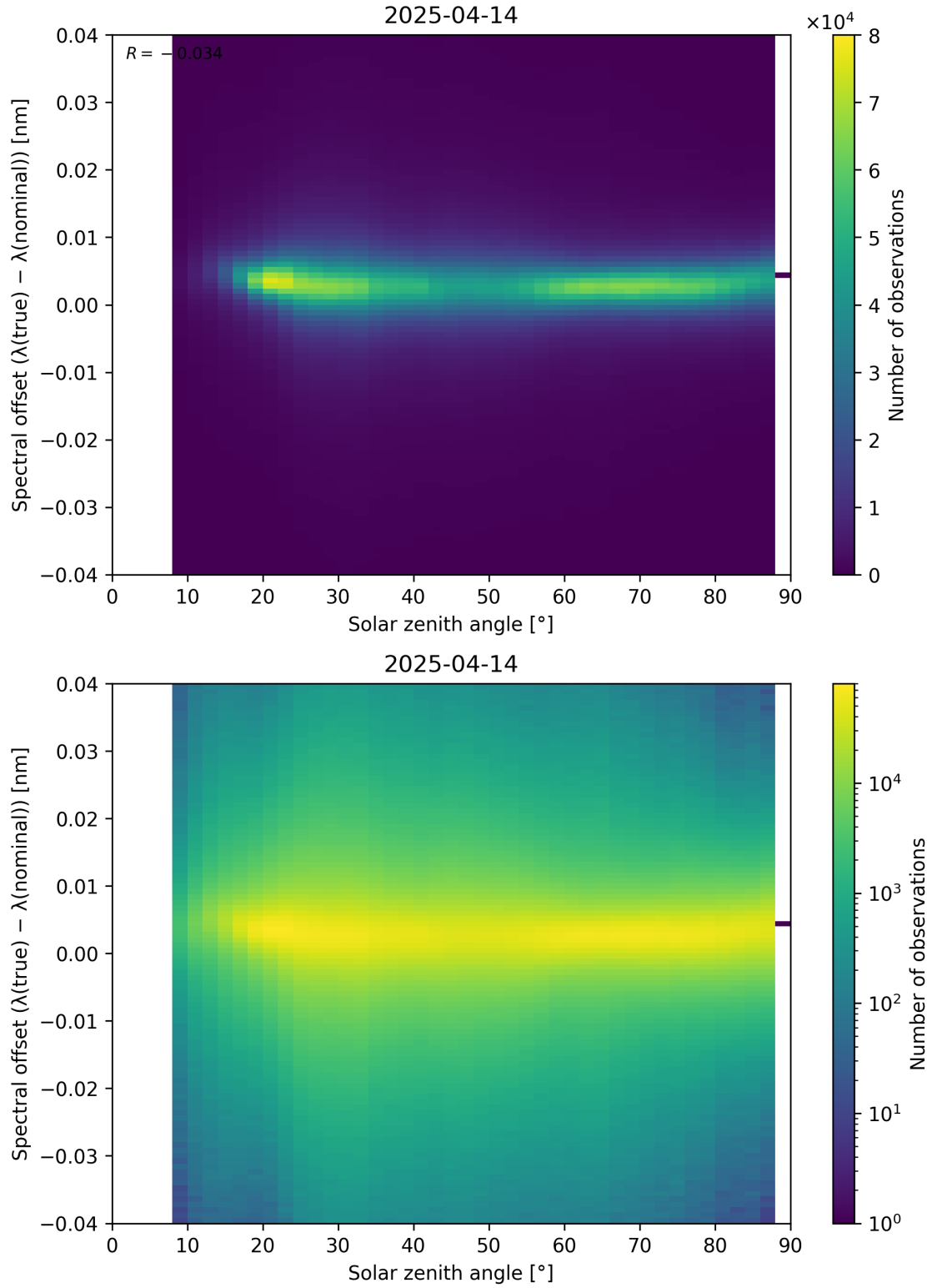
Figure 117: Scatter density plot of “Solar zenith angle” against “Spectral offset ( \lambda_{\text{true}} - \lambda_{\text{nominal}} )” for 2025-04-13 to 2025-04-15.
