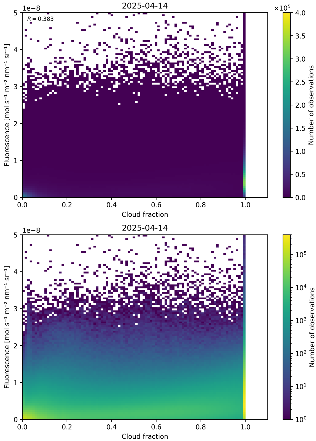
Figure 72: Scatter density plot of “Cloud fraction” against “Fluorescence” for 2025-04-13 to 2025-04-15.
