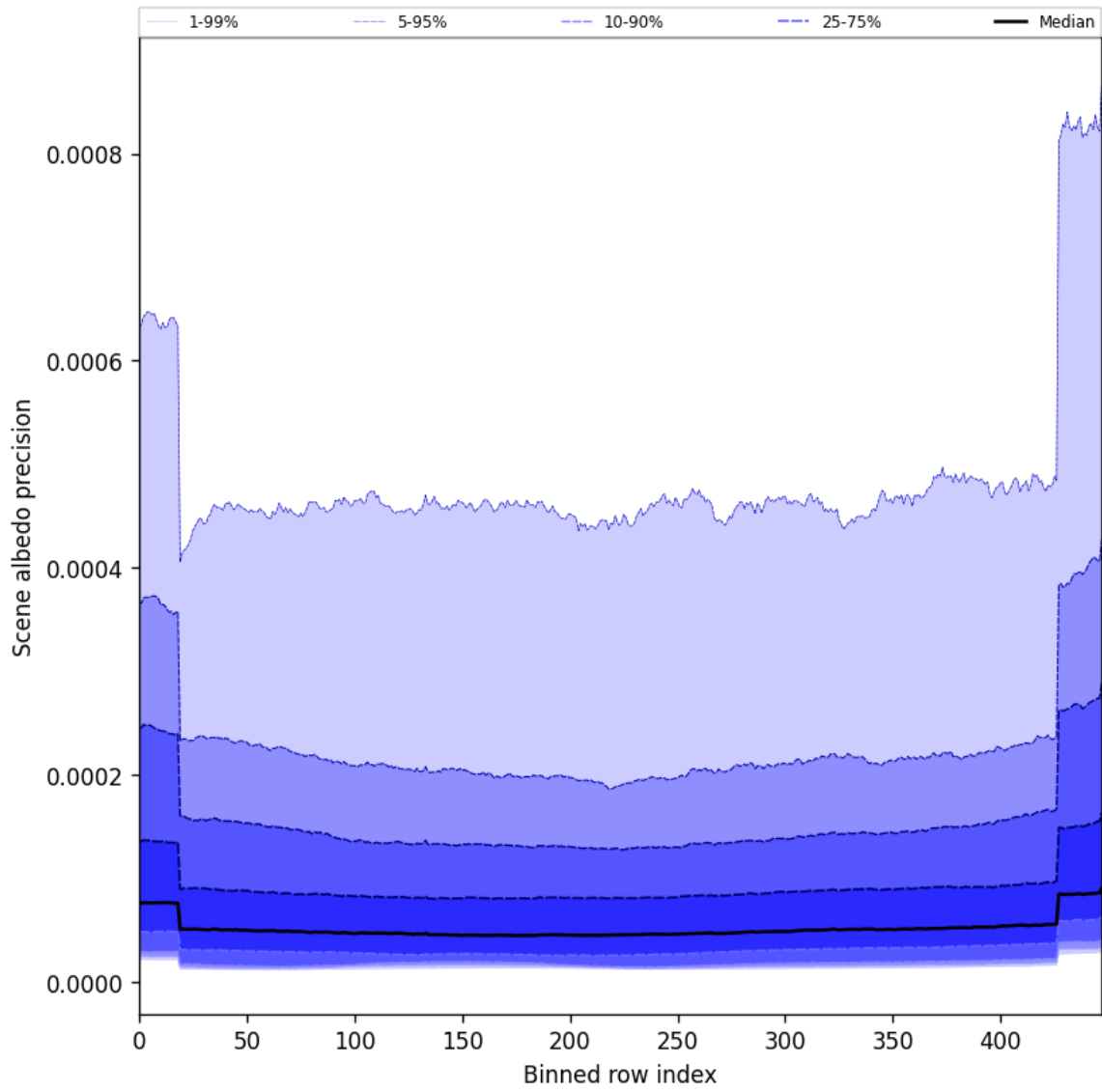
Figure 52: Along track statistics of “Scene albedo precision” for 2025-04-13 to 2025-04-15
