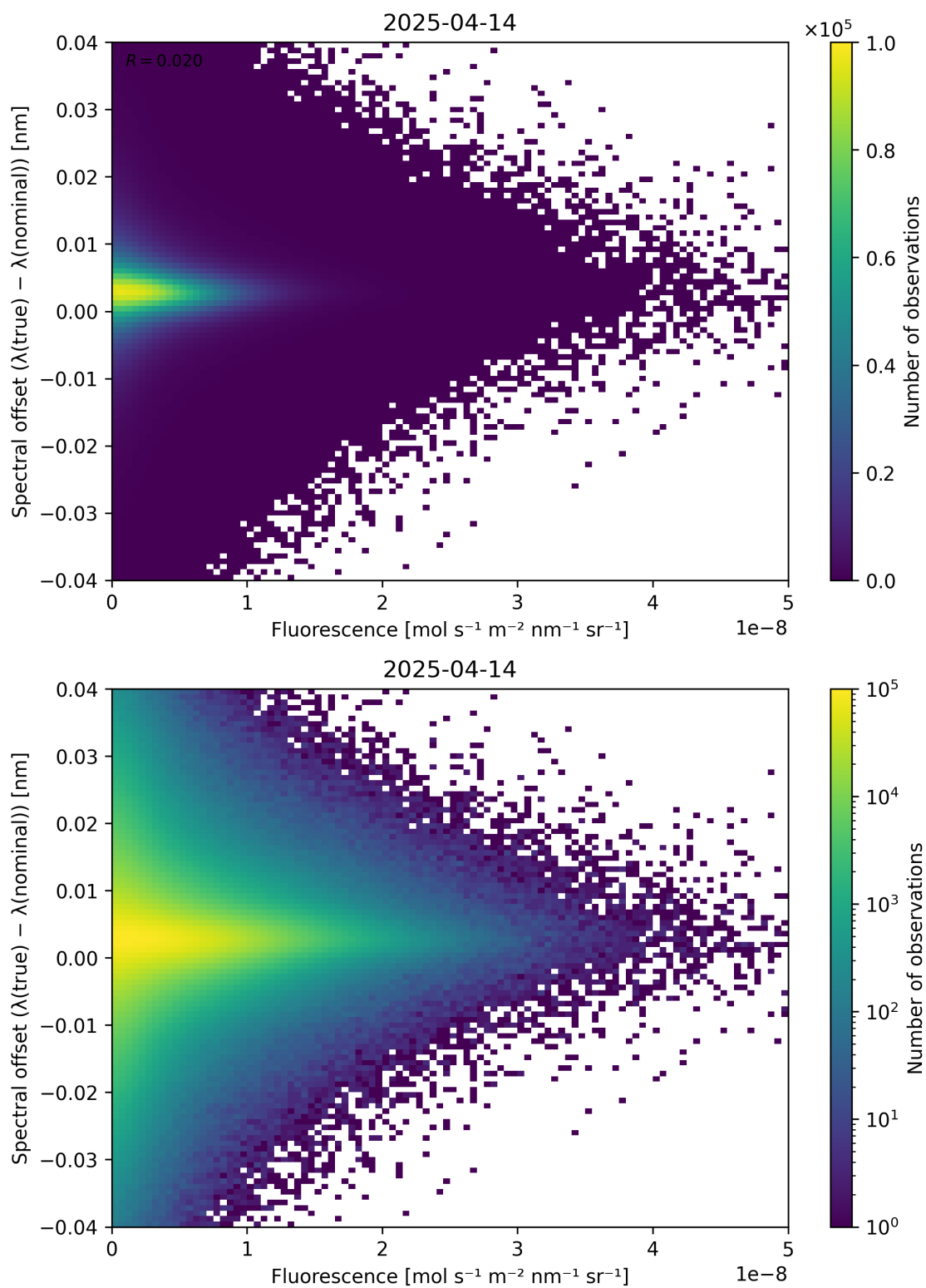
Figure 87: Scatter density plot of “Fluorescence” against “Spectral offset ( \lambda_{\text{true}} - \lambda_{\text{nominal}} )” for 2025-04-13 to 2025-04-15.
