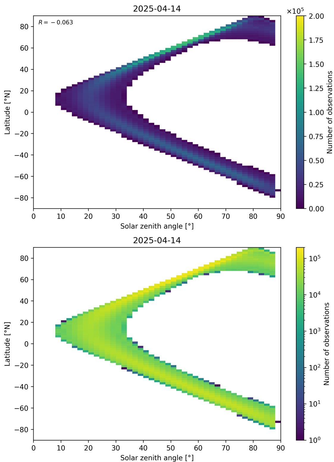
Figure 113: Scatter density plot of “Solar zenith angle” against “Latitude” for 2025-04-13 to 2025-04-15.
