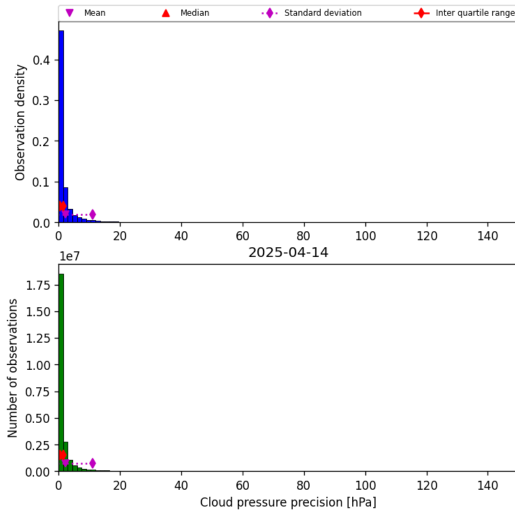
Figure 31: Histogram of “Cloud pressure precision” for 2025-04-13 to 2025-04-15
