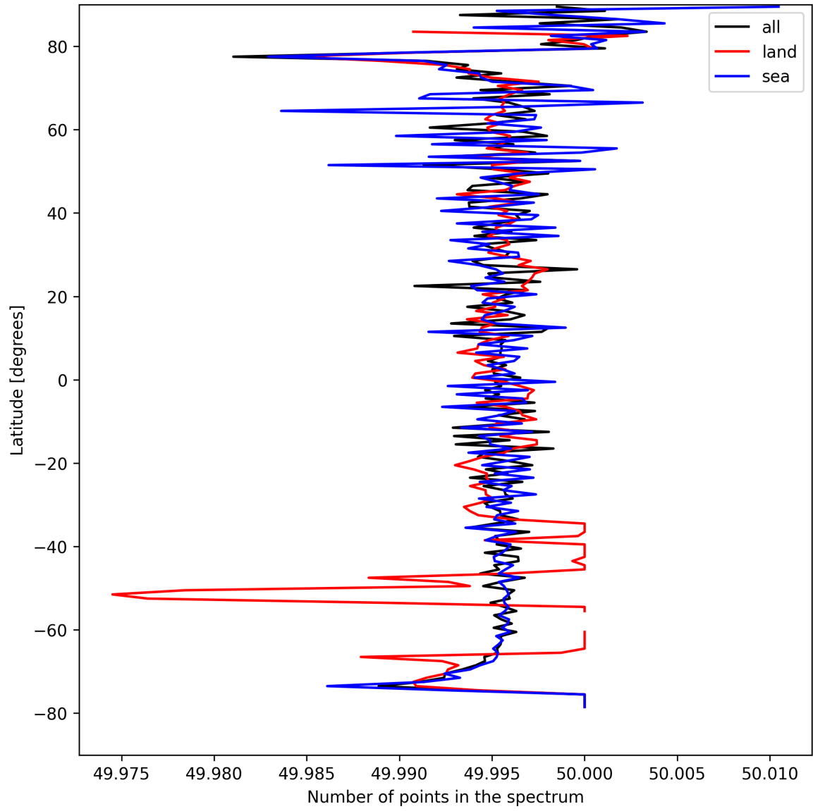
Figure 27: Zonal average of “Number of points in the spectrum” for 2025-04-13 to 2025-04-15.
