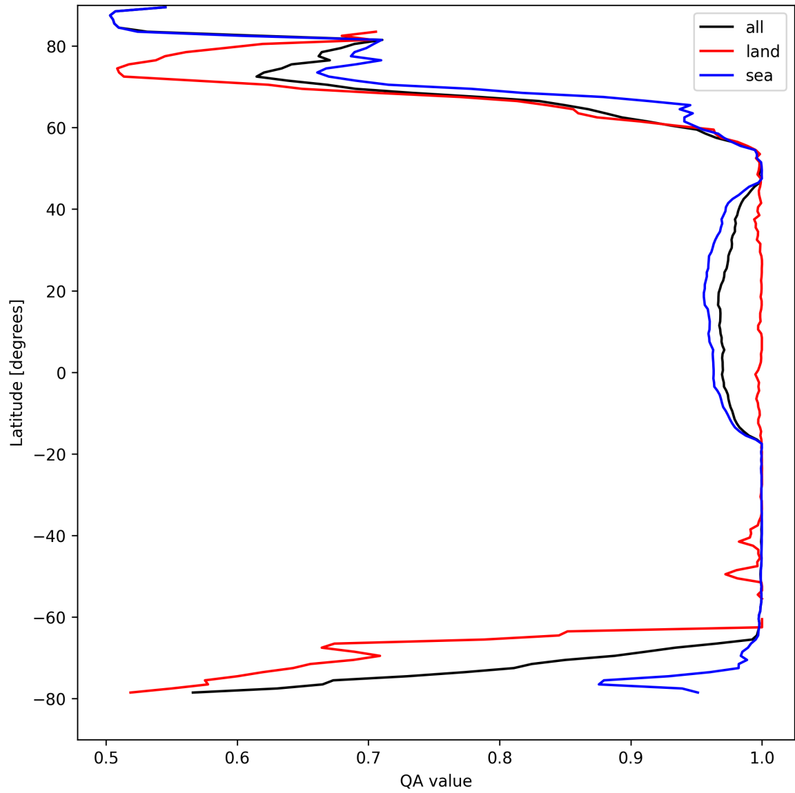
Figure 12: Zonal average of “QA value” for 2025-04-13 to 2025-04-15.
