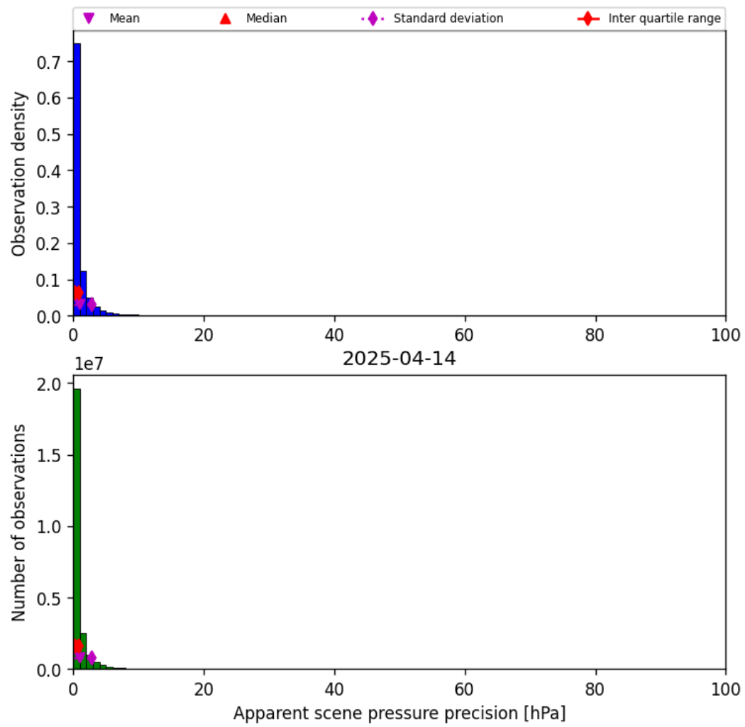
Figure 37: Histogram of “Apparent scene pressure precision” for 2025-04-13 to 2025-04-15
