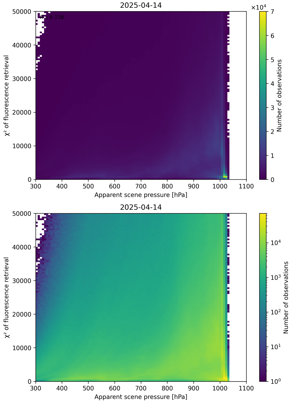
Figure 63: Scatter density plot of “Apparent scene pressure” against “ \chi^2 of fluorescence retrieval” for 2025-04-13 to 2025-04-15.
