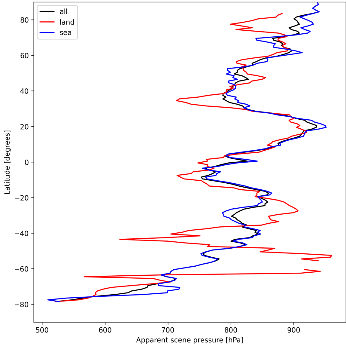
Figure 19: Zonal average of “Apparent scene pressure” for 2025-04-13 to 2025-04-15.
