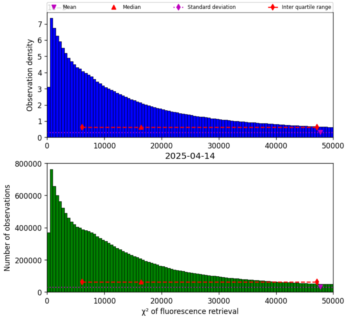
Figure 42: Histogram of “ \chi^2 of fluorescence retrieval” for 2025-04-13 to 2025-04-15
