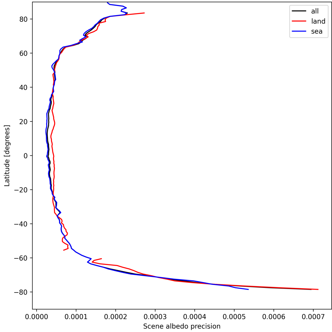
Figure 18: Zonal average of “Scene albedo precision” for 2025-04-13 to 2025-04-15.
