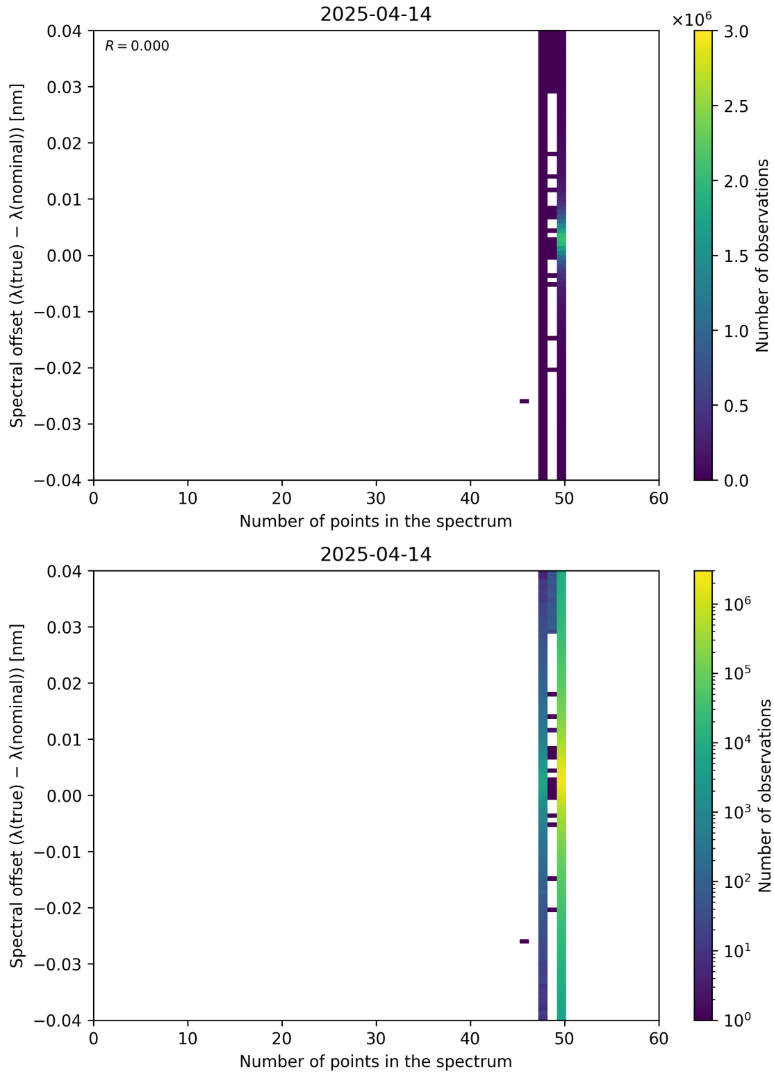
Figure 101: Scatter density plot of “Number of points in the spectrum” against “Spectral offset ( \lambda_{\text{true}} - \lambda_{\text{nominal}} )” for 2025-04-13 to 2025-04-15.
