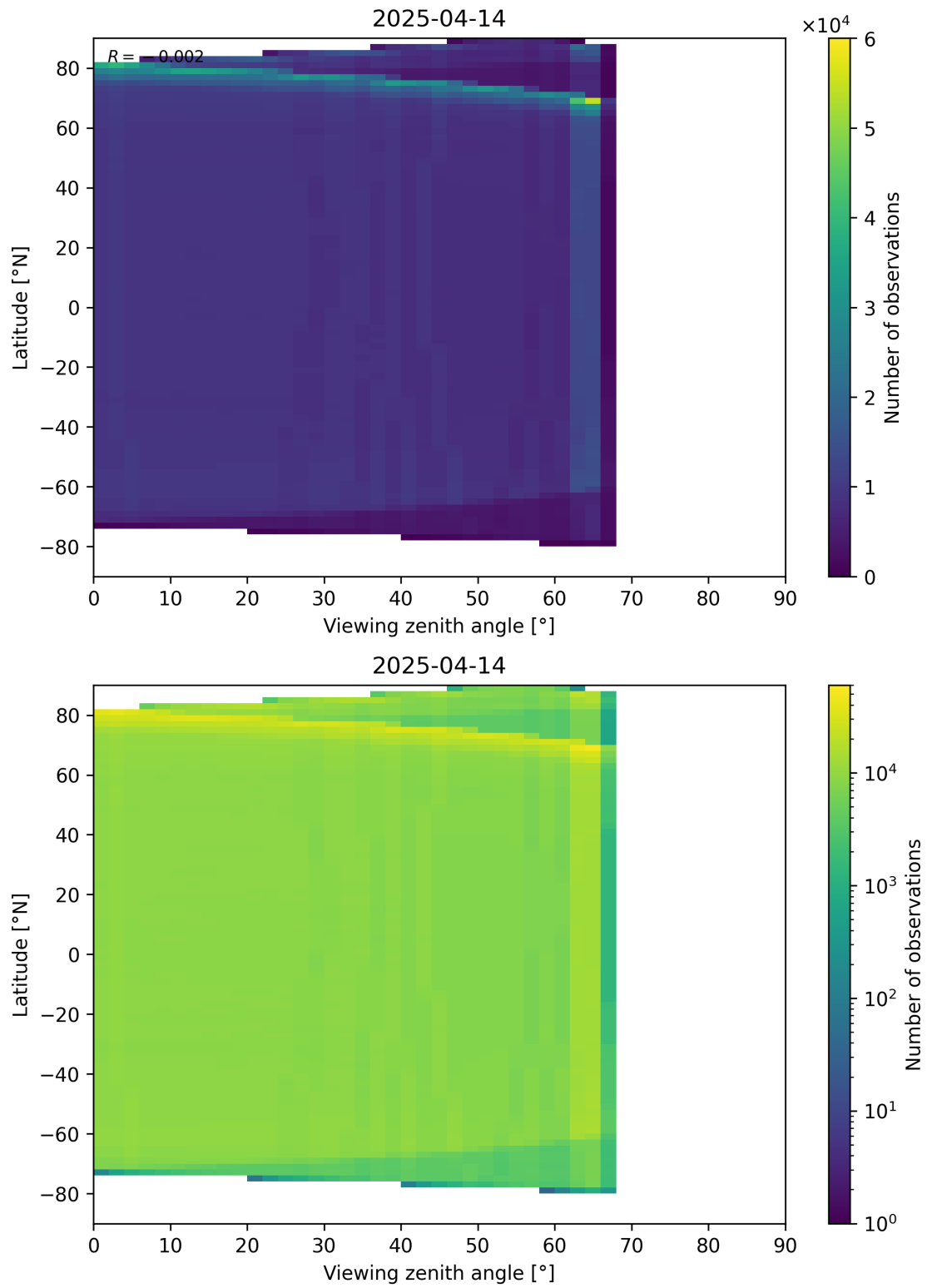
Figure 123: Scatter density plot of “Viewing zenith angle” against “Latitude” for 2025-04-13 to 2025-04-15.
