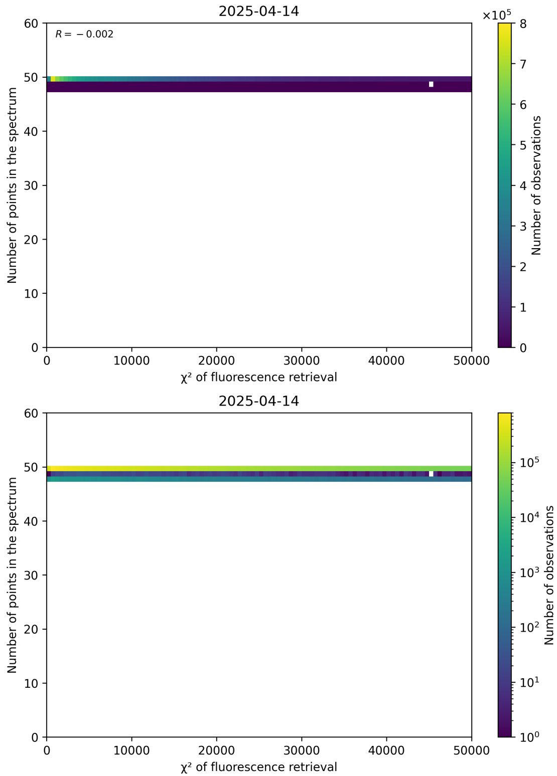
Figure 68: Scatter density plot of " \chi^2 of fluorescence retrieval" against "Number of points in the spectrum" for 2025-04-13 to 2025-04-15.
