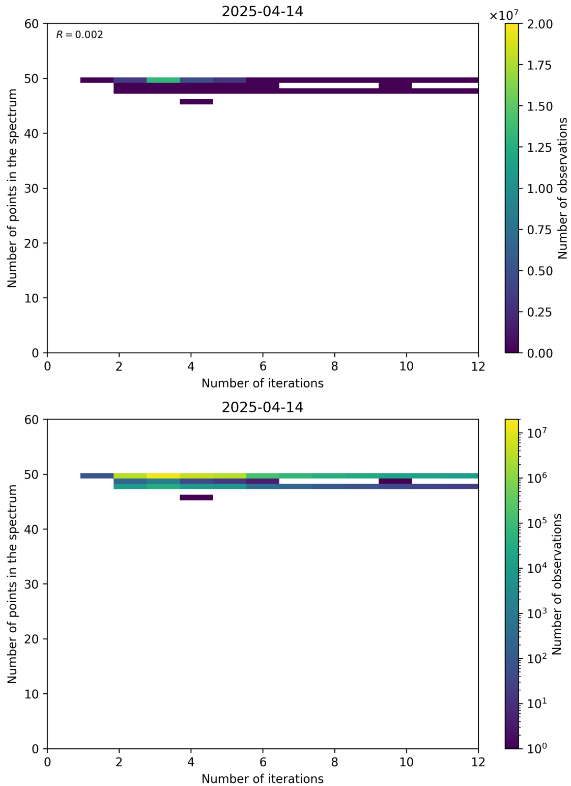
Figure 99: Scatter density plot of “Number of iterations” against “Number of points in the spectrum” for 2025-04-13 to 2025-04-15.
