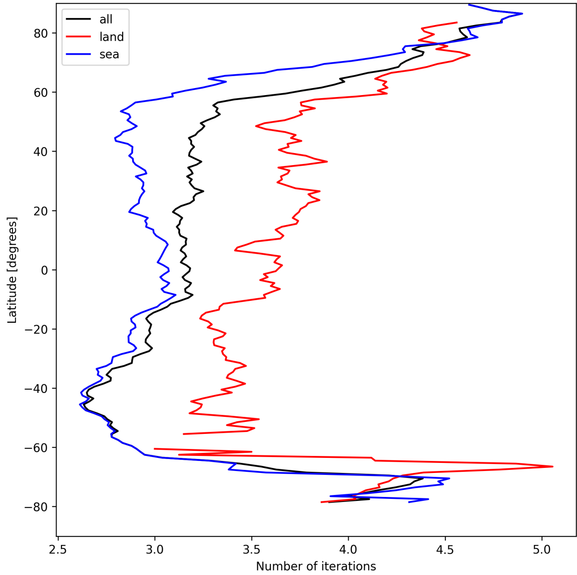
Figure 22: Zonal average of “Number of iterations” for 2025-04-13 to 2025-04-15.
