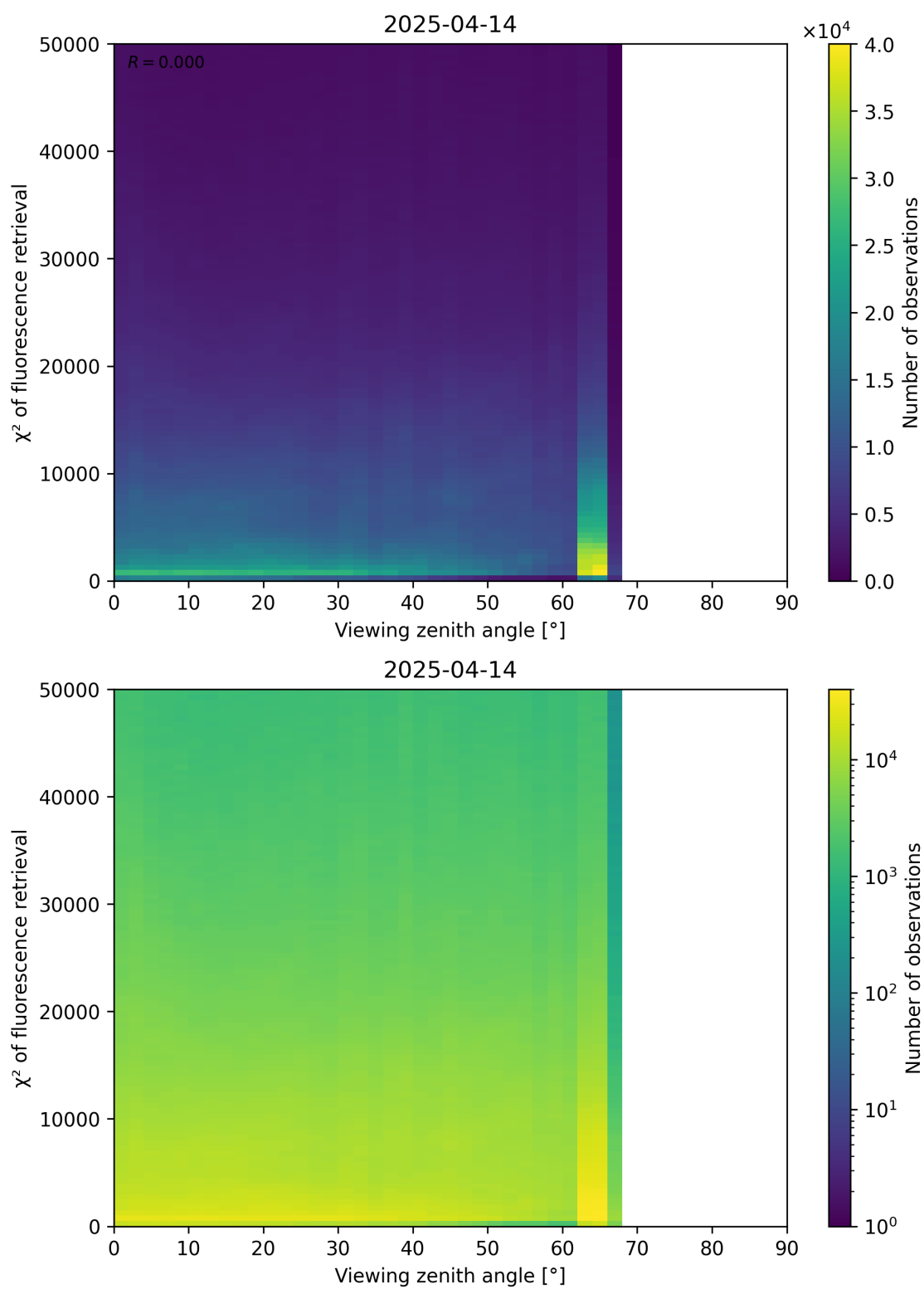
Figure 119: Scatter density plot of “Viewing zenith angle” against “ \chi^2 of fluorescence retrieval” for 2025-04-13 to 2025-04-15.
