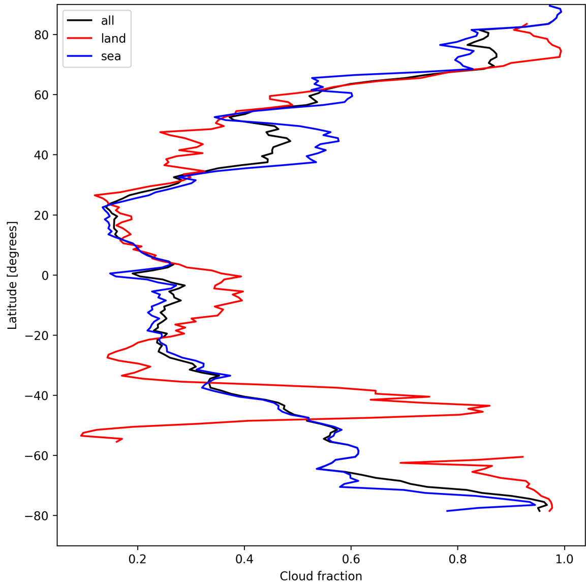
Figure 15: Zonal average of “Cloud fraction” for 2025-04-13 to 2025-04-15.
