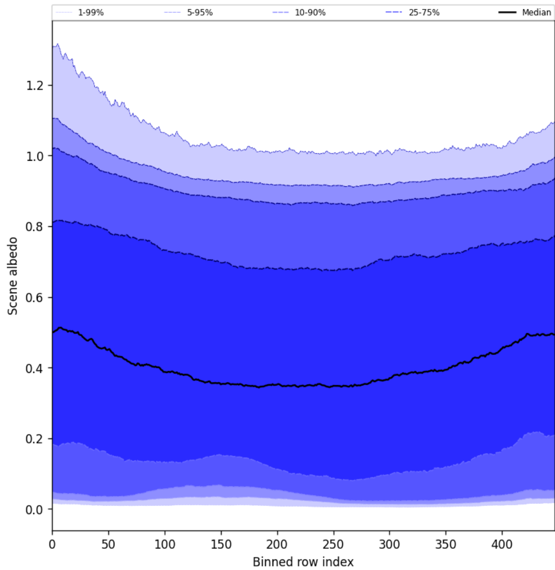
Figure 51: Along track statistics of “Scene albedo” for 2025-04-13 to 2025-04-15
