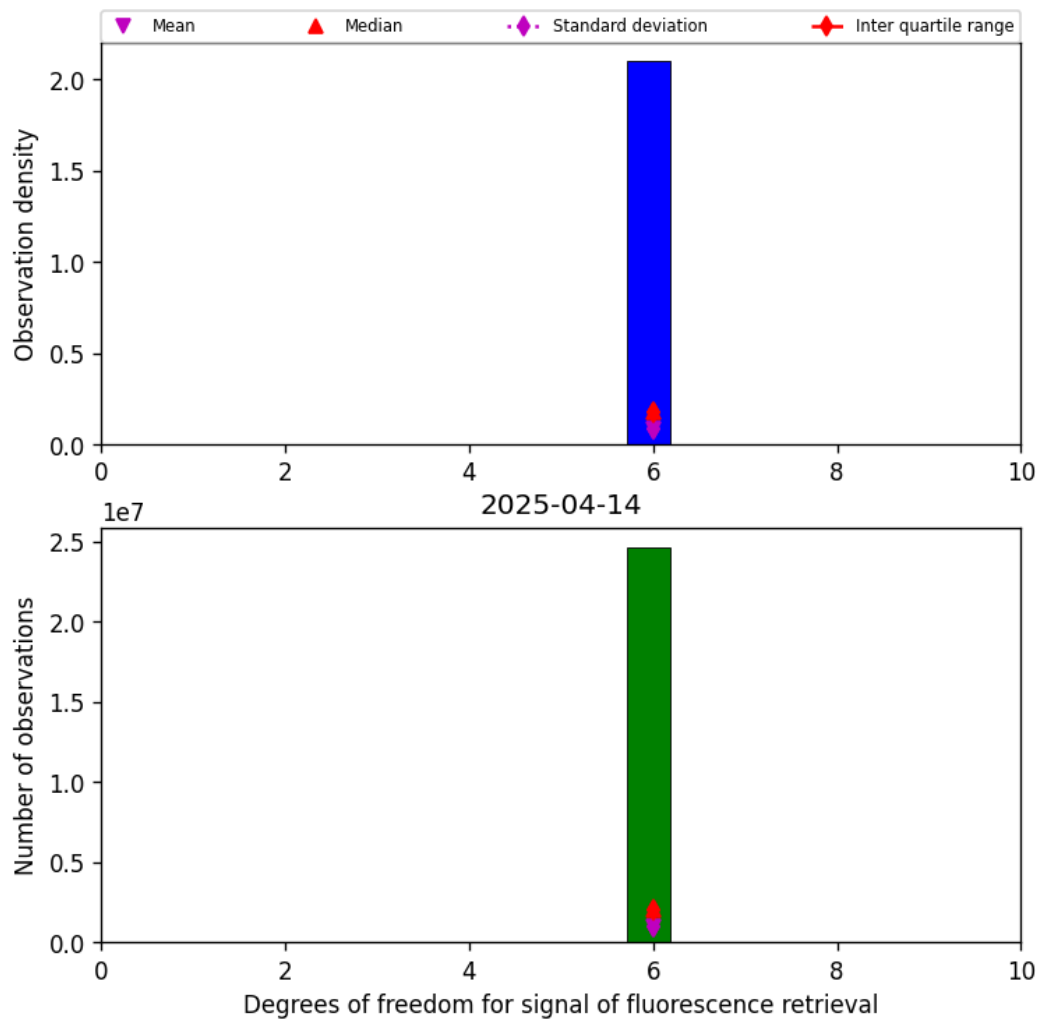
Figure 43: Histogram of "Degrees of freedom for signal of fluorescence retrieval" for 2025-04-13 to 2025-04-15
