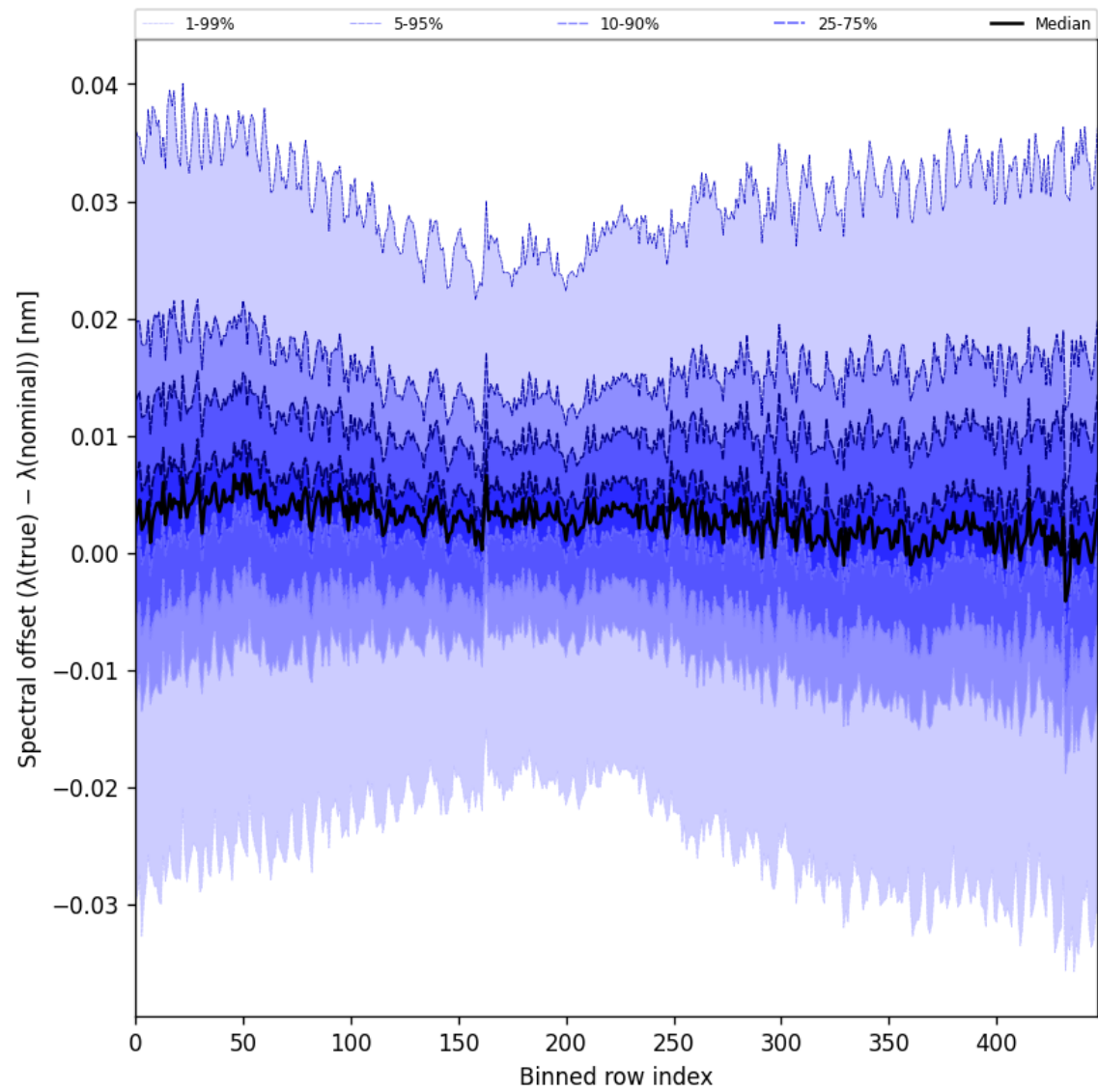
Figure 62: Along track statistics of “Spectral offset ( \lambda_{\text{true}} - \lambda_{\text{nominal}} )” for 2025-04-13 to 2025-04-15
