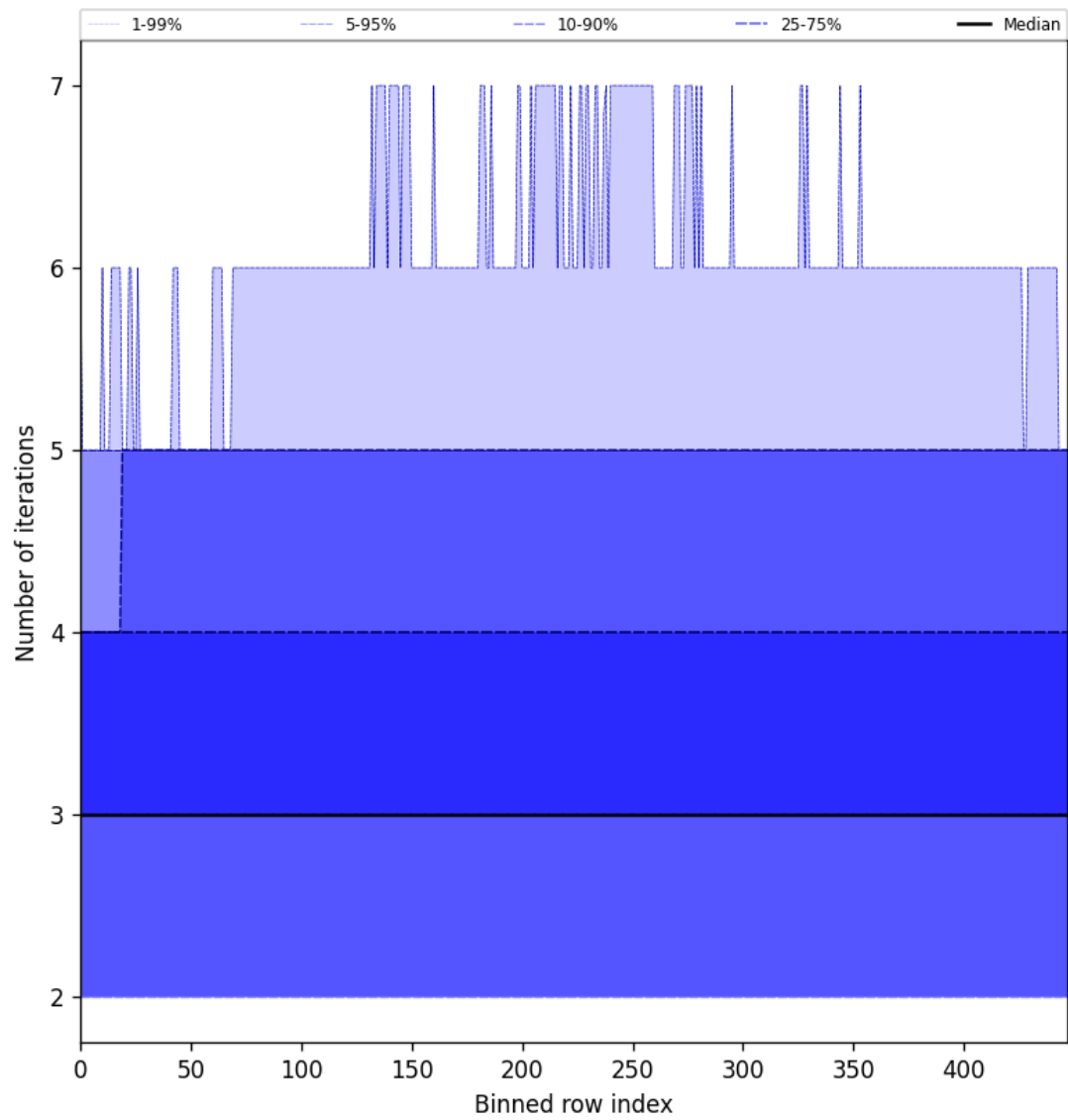
Figure 56: Along track statistics of “Number of iterations” for 2025-04-13 to 2025-04-15
