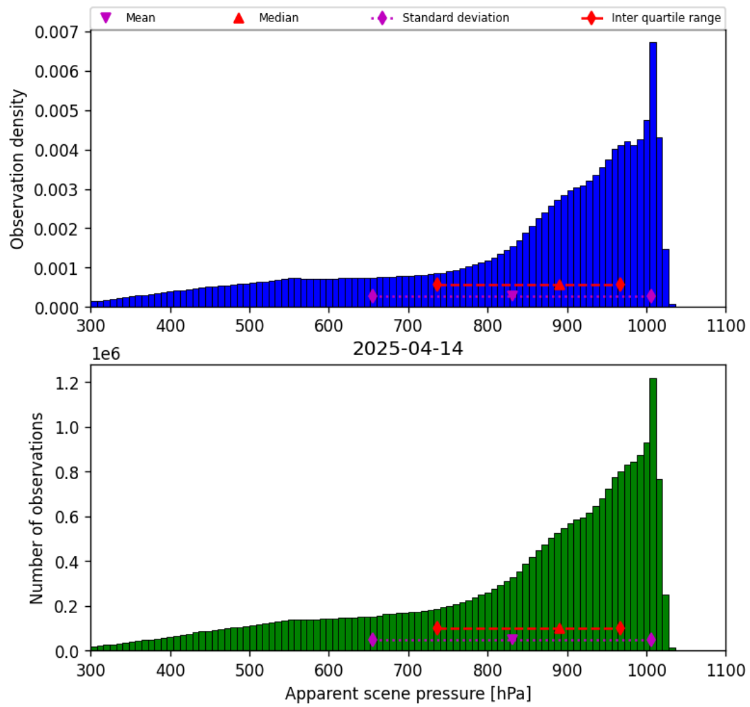
Figure 36: Histogram of “Apparent scene pressure” for 2025-04-13 to 2025-04-15
