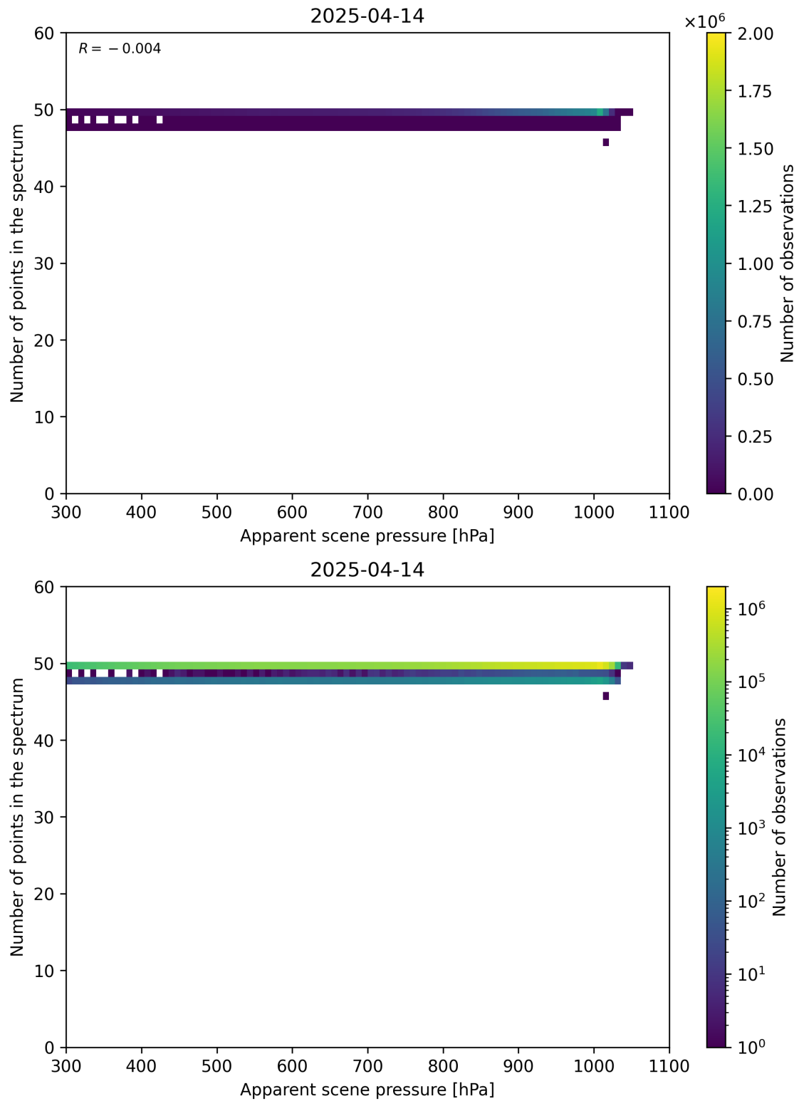
Figure 66: Scatter density plot of “Apparent scene pressure” against “Number of points in the spectrum” for 2025-04-13 to 2025-04-15.
