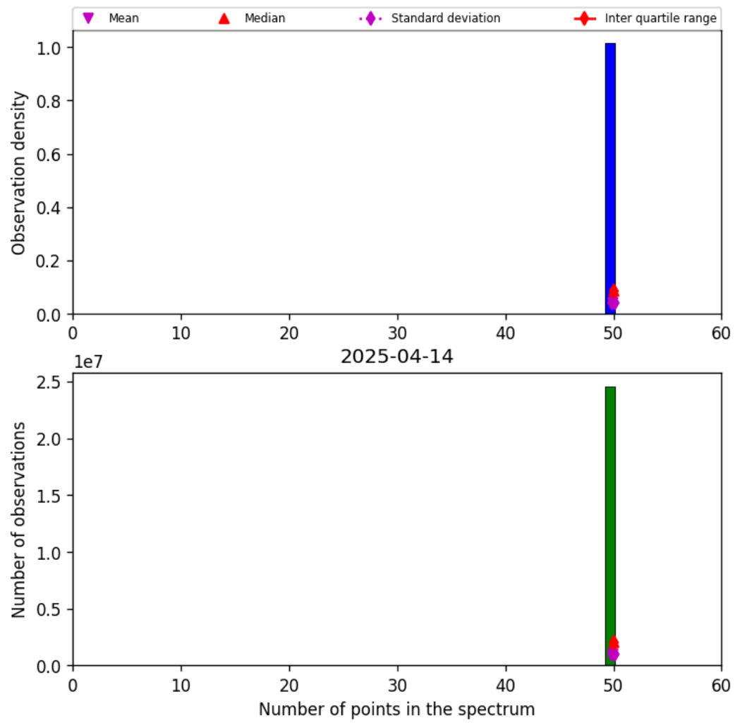
Figure 44: Histogram of “Number of points in the spectrum” for 2025-04-13 to 2025-04-15
