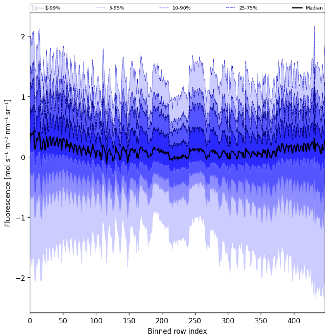
Figure 57: Along track statistics of “Fluorescence” for 2025-04-13 to 2025-04-15
