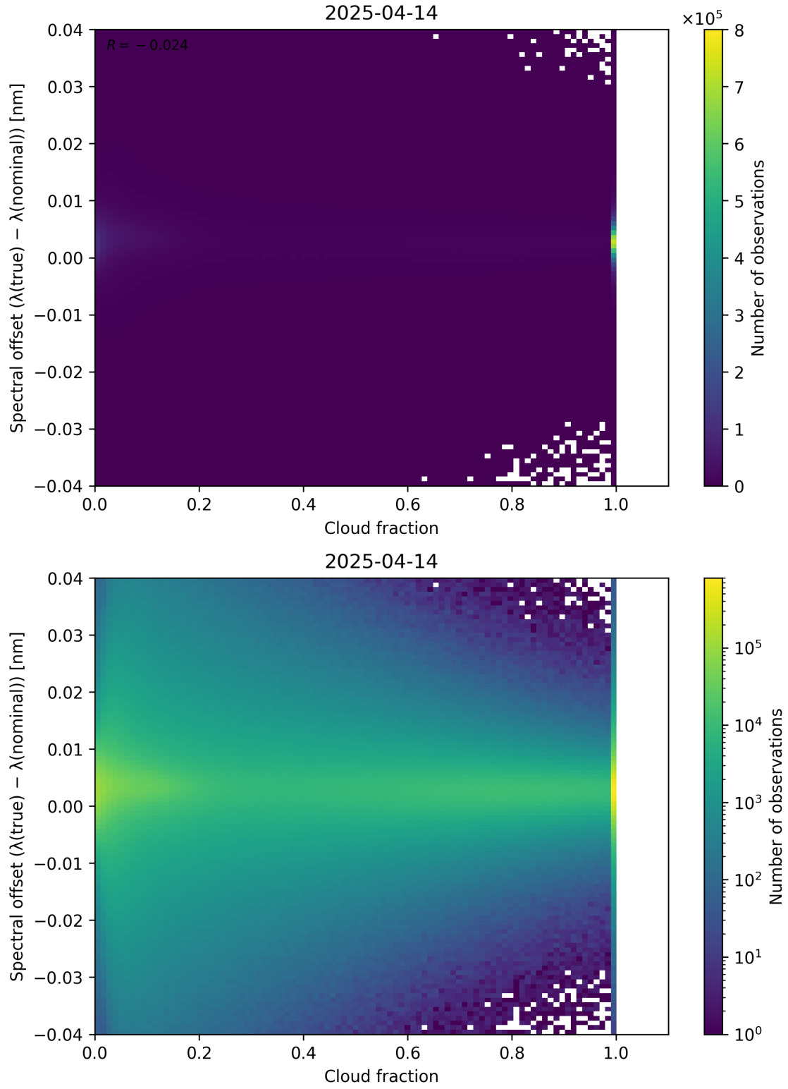
Figure 76: Scatter density plot of “Cloud fraction” against “Spectral offset ( \lambda_{\text{true}} - \lambda_{\text{nominal}} )” for 2025-04-13 to 2025-04-15.
