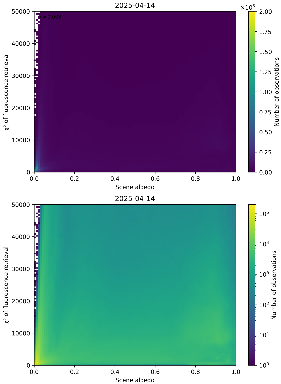
Figure 103: Scatter density plot of “Scene albedo” against “ \chi^2 of fluorescence retrieval” for 2025-04-13 to 2025-04-15.
