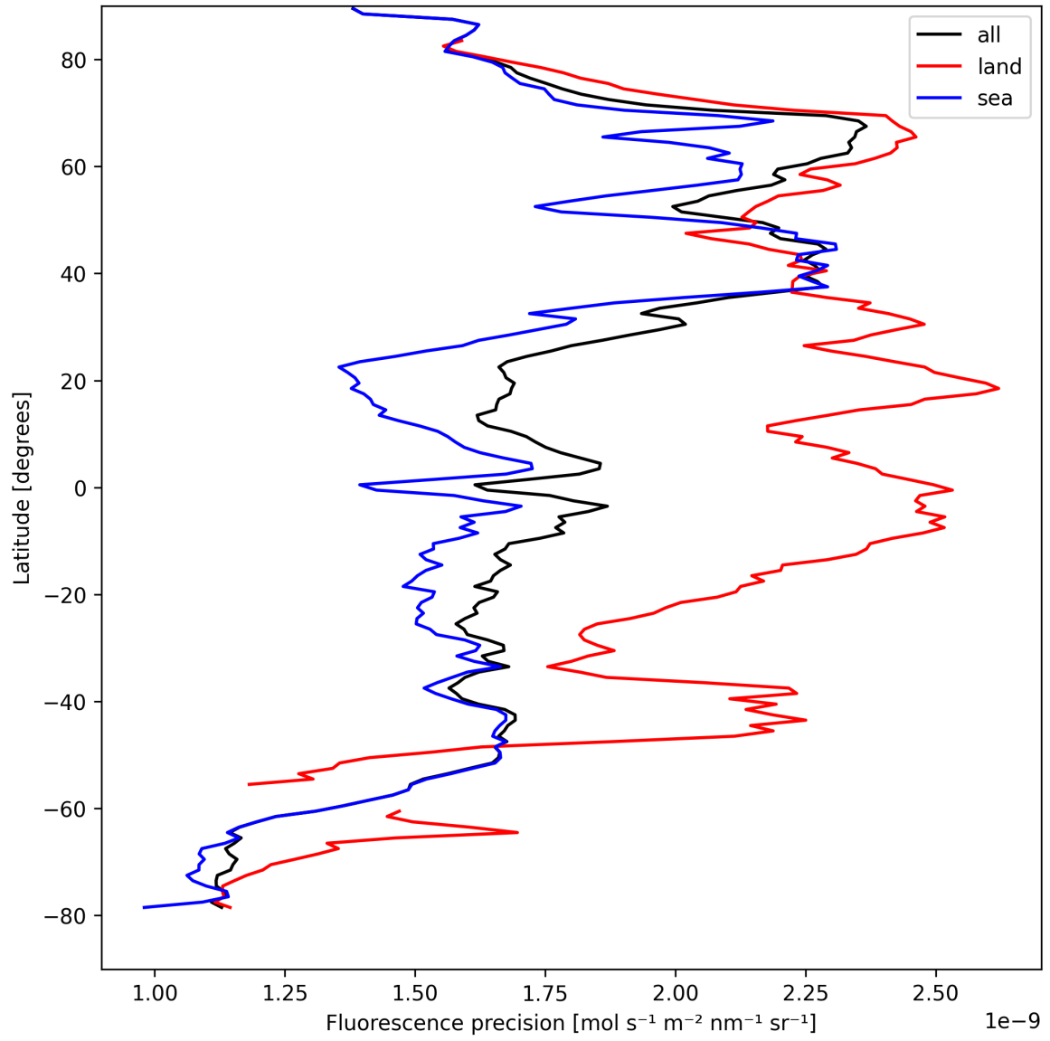
Figure 24: Zonal average of “Fluorescence precision” for 2025-04-13 to 2025-04-15.
