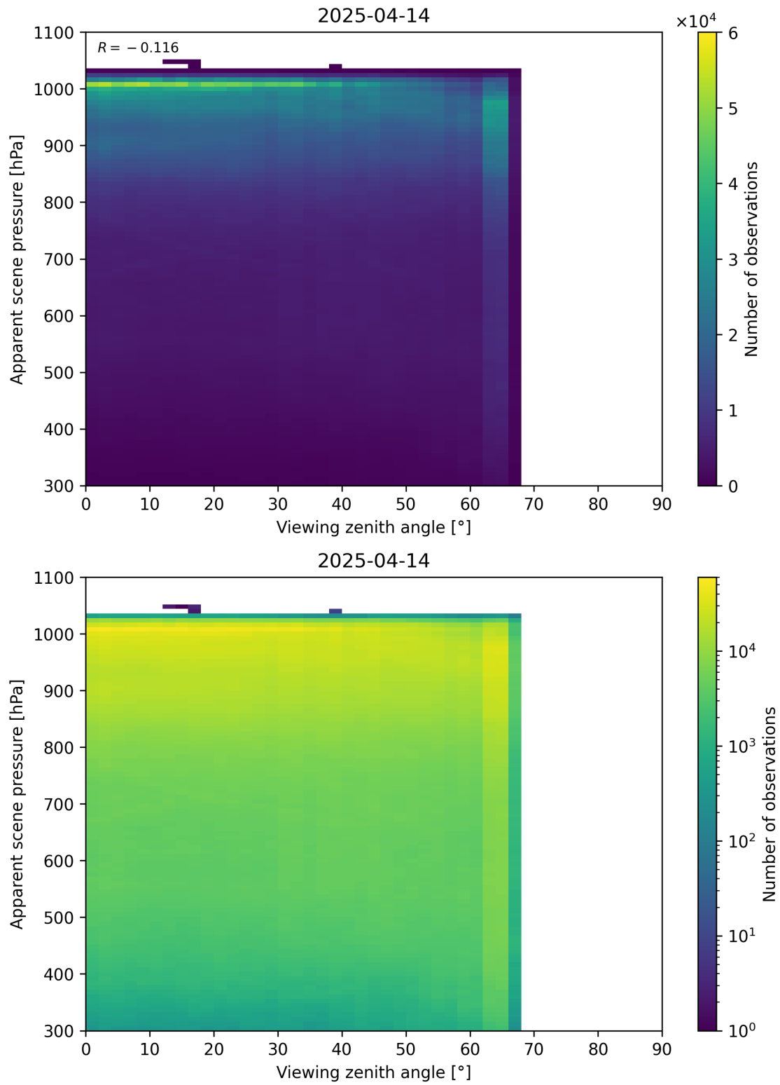
Figure 118: Scatter density plot of “Viewing zenith angle” against “Apparent scene pressure” for 2025-04-13 to 2025-04-15.
