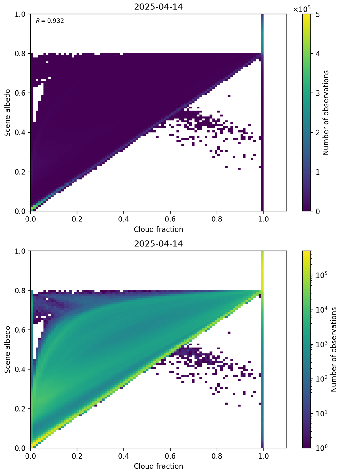
Figure 75: Scatter density plot of “Cloud fraction” against “Scene albedo” for 2025-04-13 to 2025-04-15.
