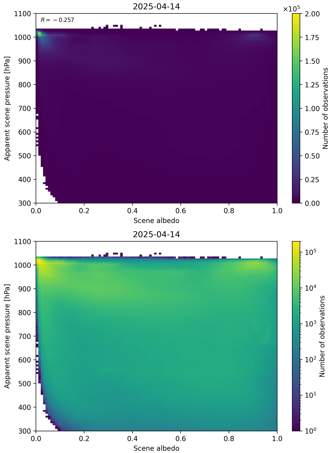
Figure 102: Scatter density plot of “Scene albedo” against “Apparent scene pressure” for 2025-04-13 to 2025-04-15.
