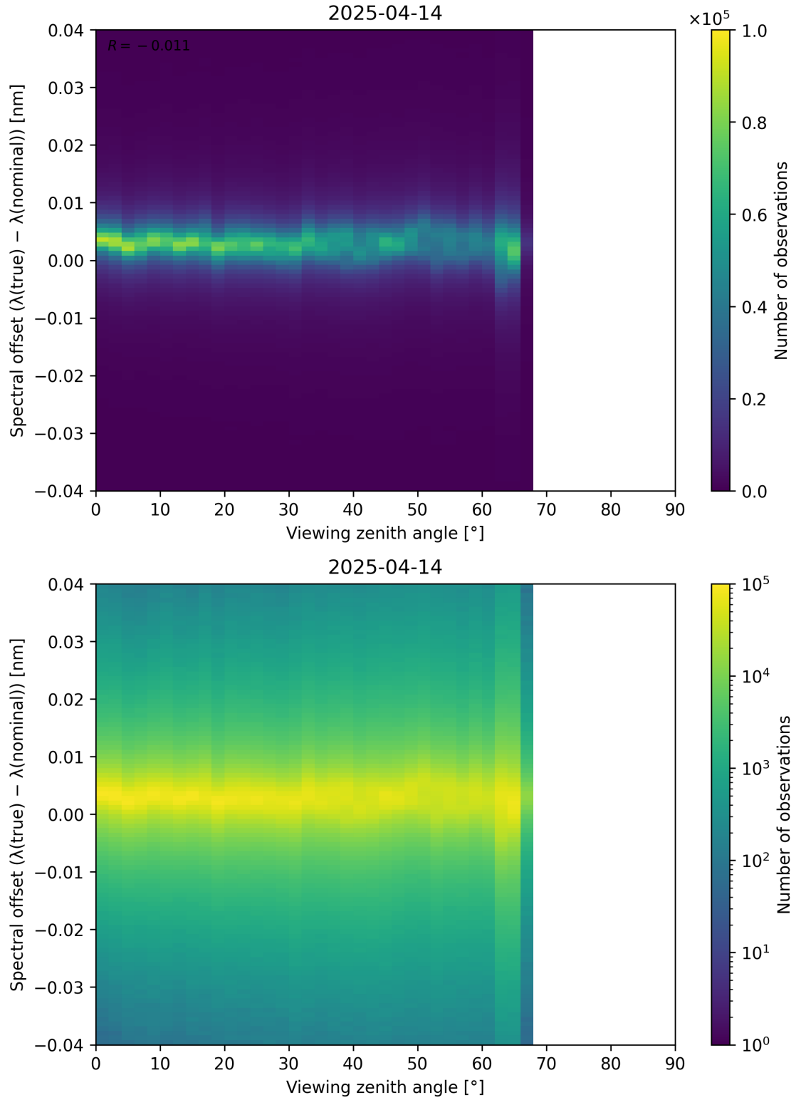
Figure 128: Scatter density plot of “Viewing zenith angle” against “Spectral offset ( \lambda_{\text{true}} - \lambda_{\text{nominal}} )” for 2025-04-13 to 2025-04-15.
