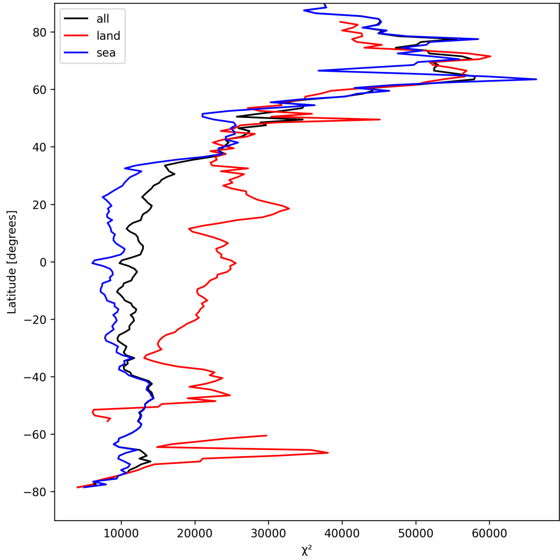
Figure 21: Zonal average of “ \chi^2 ” for 2025-04-13 to 2025-04-15.
