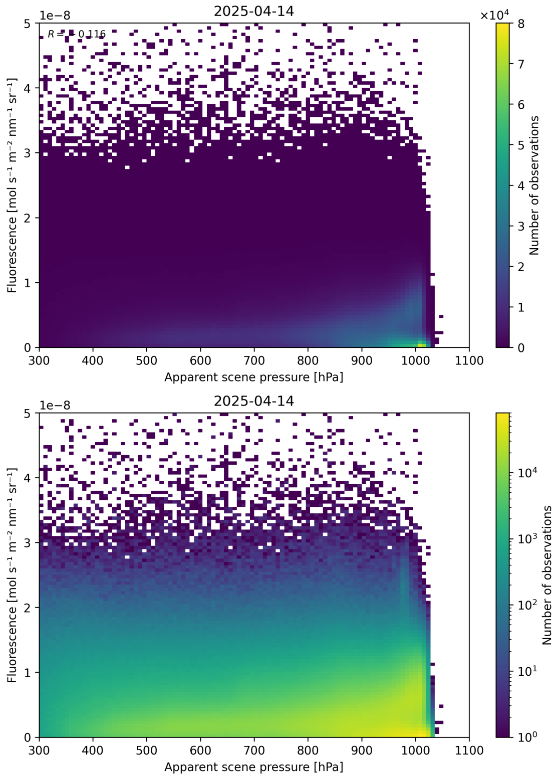
Figure 64: Scatter density plot of “Apparent scene pressure” against “Fluorescence” for 2025-04-13 to 2025-04-15.
