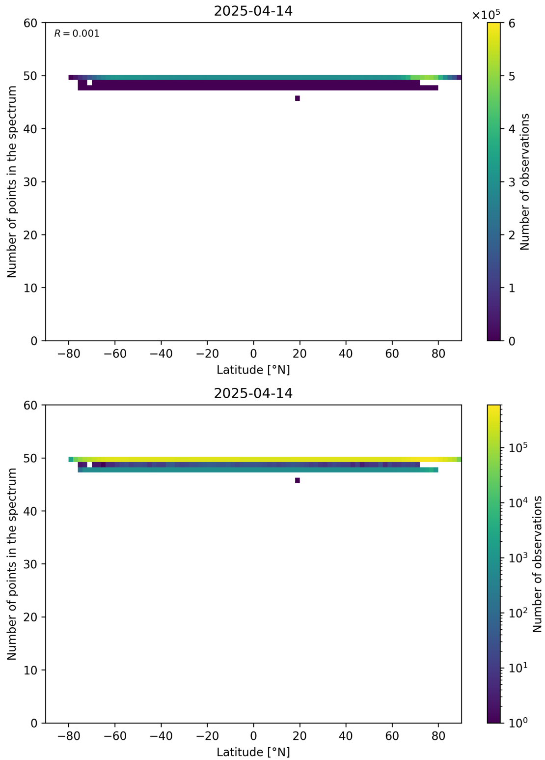
Figure 94: Scatter density plot of “Latitude” against “Number of points in the spectrum” for 2025-04-13 to 2025-04-15.
