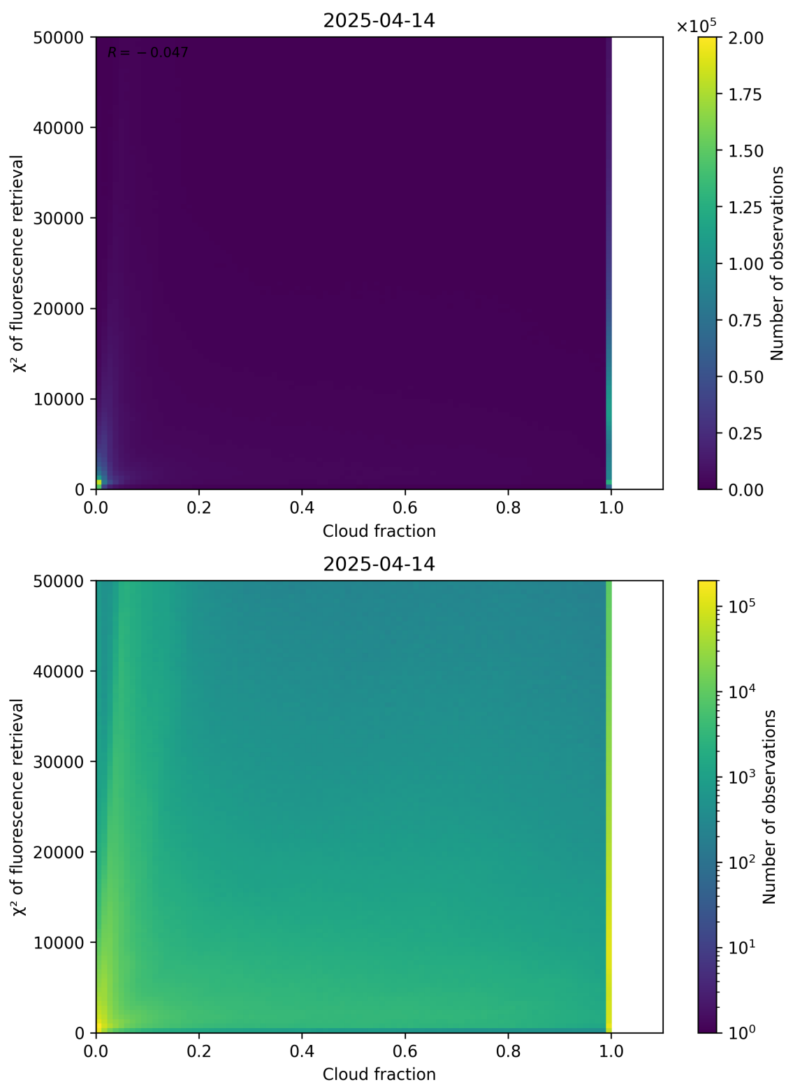
Figure 71: Scatter density plot of “Cloud fraction” against “ \chi^2 of fluorescence retrieval” for 2025-04-13 to 2025-04-15.
