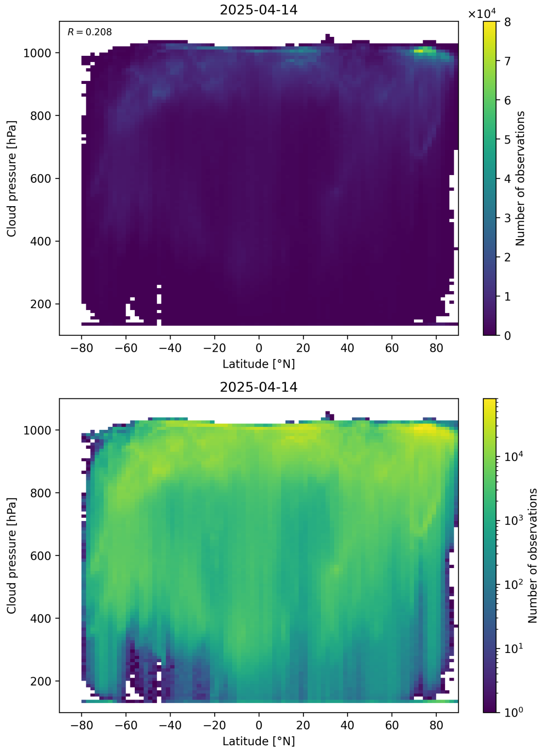
Figure 91: Scatter density plot of “Latitude” against “Cloud pressure” for 2025-04-13 to 2025-04-15.
