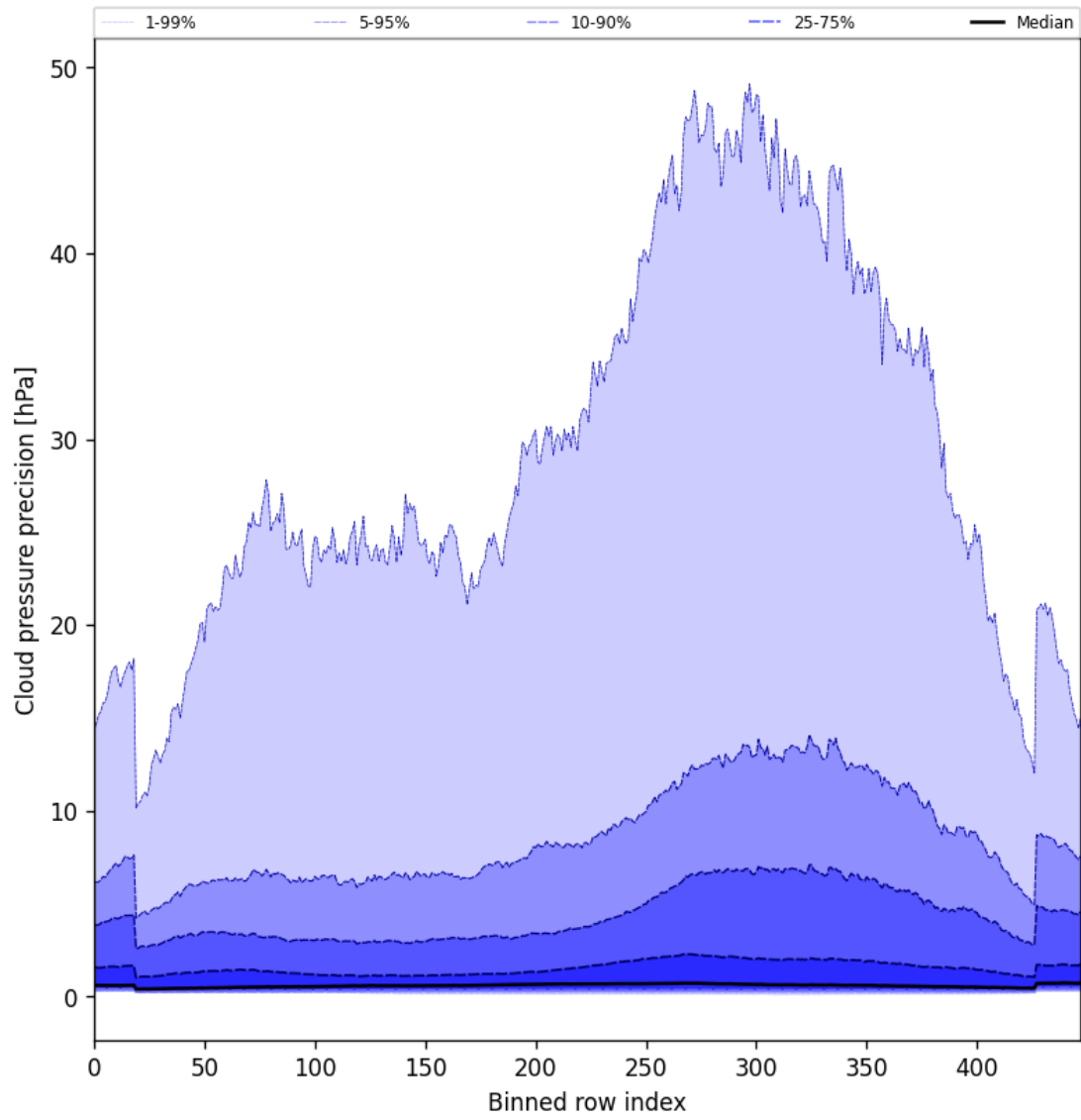
Figure 48: Along track statistics of “Cloud pressure precision” for 2025-04-13 to 2025-04-15
