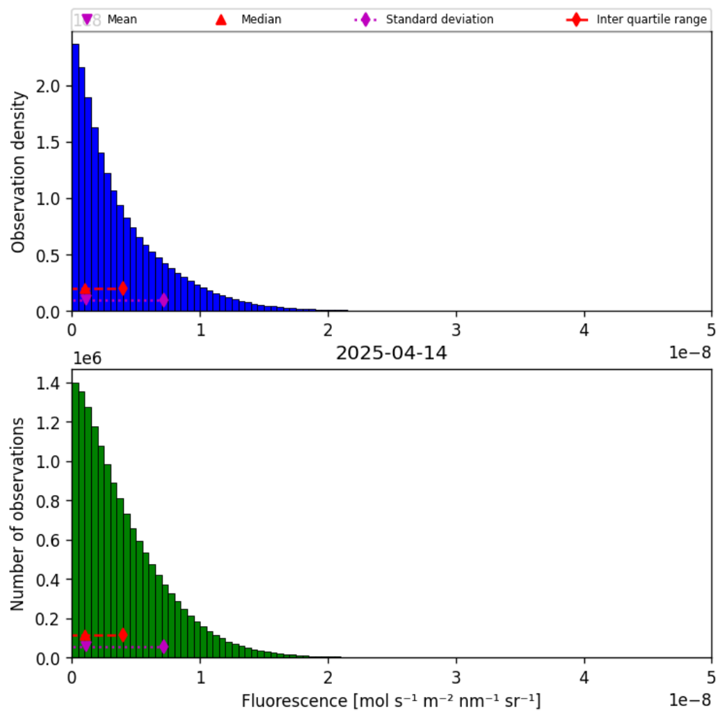
Figure 40: Histogram of “Fluorescence” for 2025-04-13 to 2025-04-15
