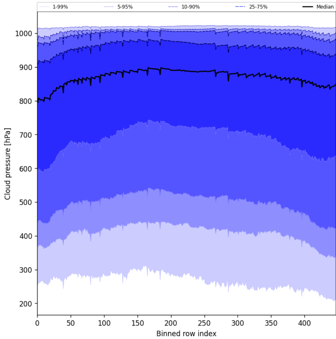
Figure 47: Along track statistics of “Cloud pressure” for 2025-04-13 to 2025-04-15
