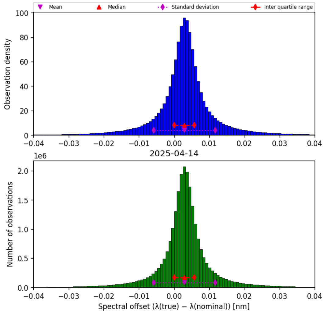
Figure 45: Histogram of “Spectral offset ( \lambda_{\text{true}} - \lambda_{\text{nominal}} )” for 2025-04-13 to 2025-04-15
