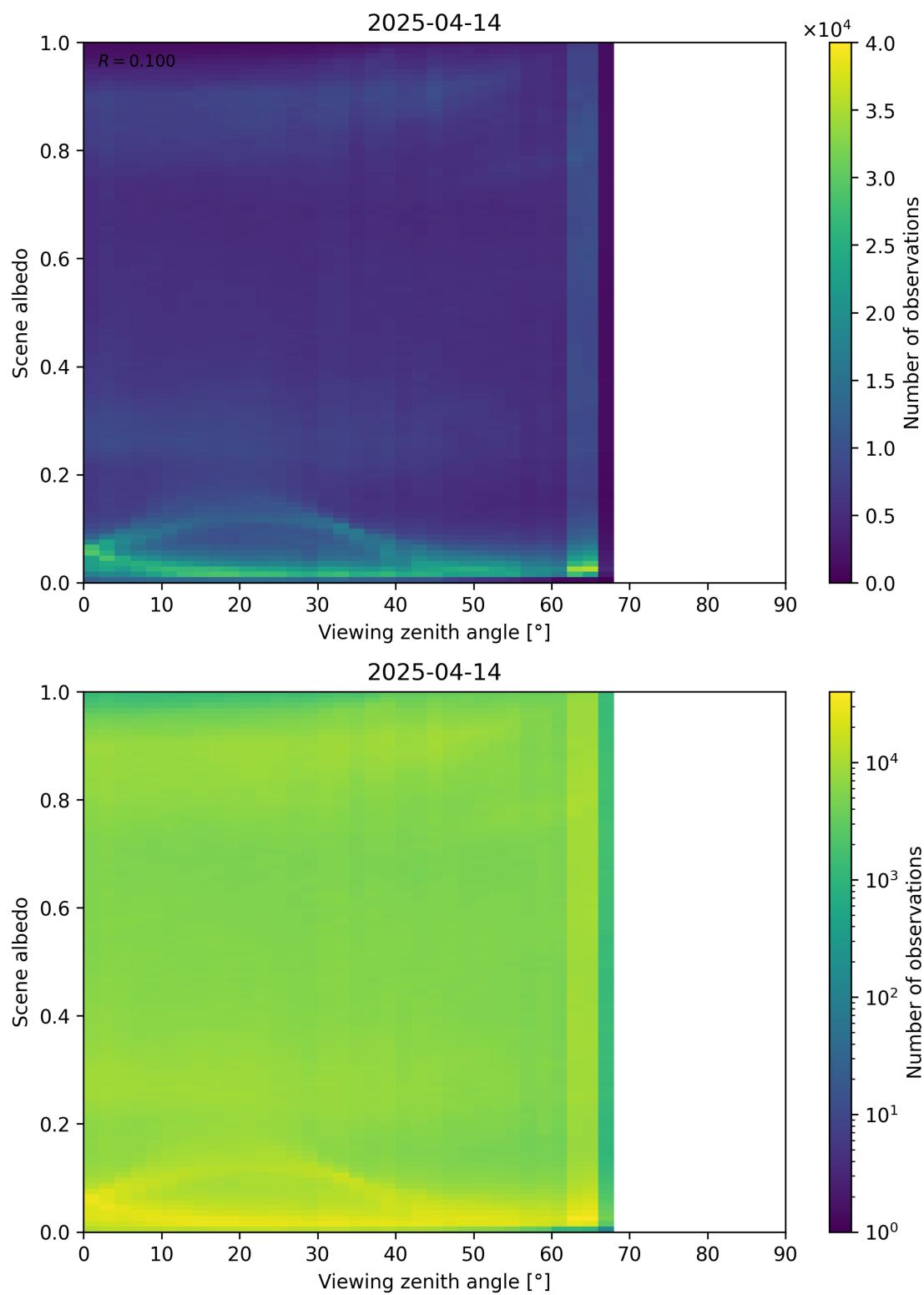
Figure 126: Scatter density plot of “Viewing zenith angle” against “Scene albedo” for 2025-04-13 to 2025-04-15.
