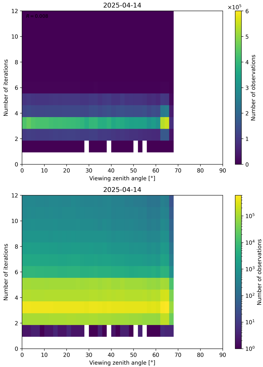
Figure 124: Scatter density plot of “Viewing zenith angle” against “Number of iterations” for 2025-04-13 to 2025-04-15.
