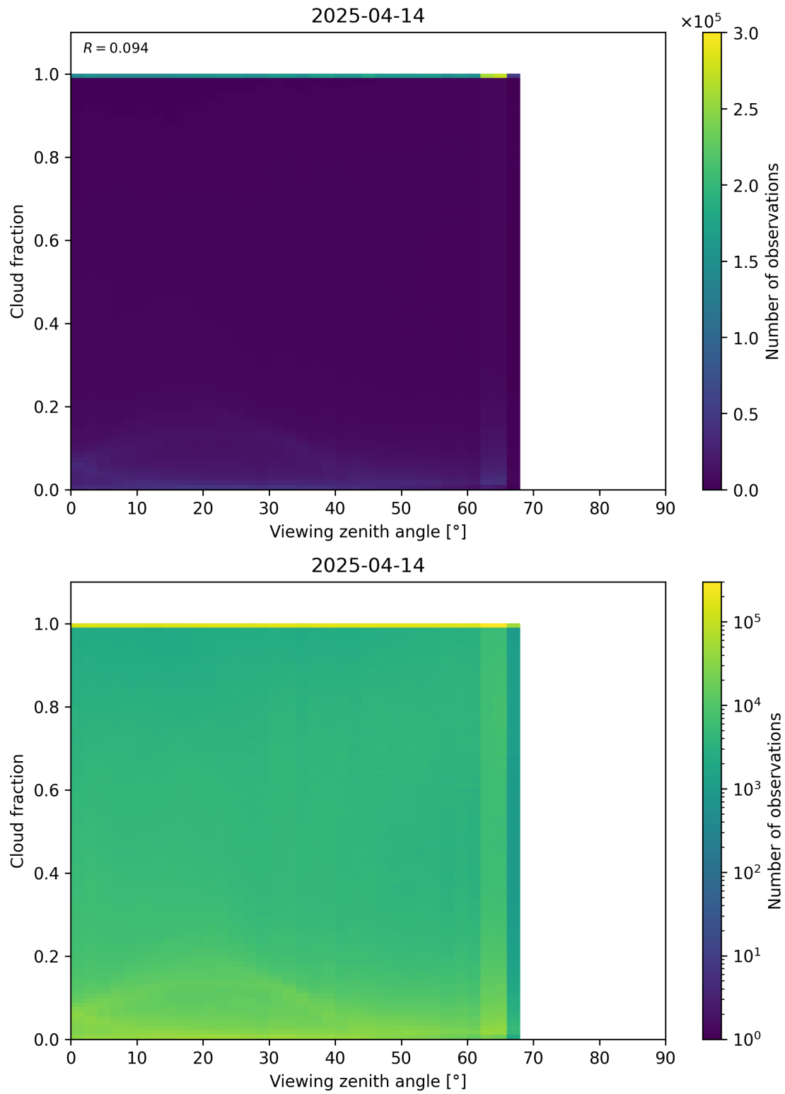
Figure 120: Scatter density plot of “Viewing zenith angle” against “Cloud fraction” for 2025-04-13 to 2025-04-15.
