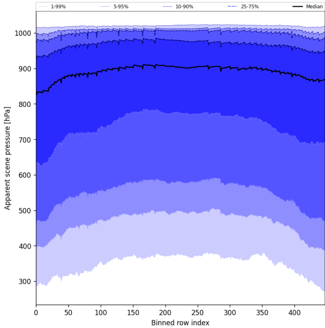
Figure 53: Along track statistics of “Apparent scene pressure” for 2025-04-13 to 2025-04-15
