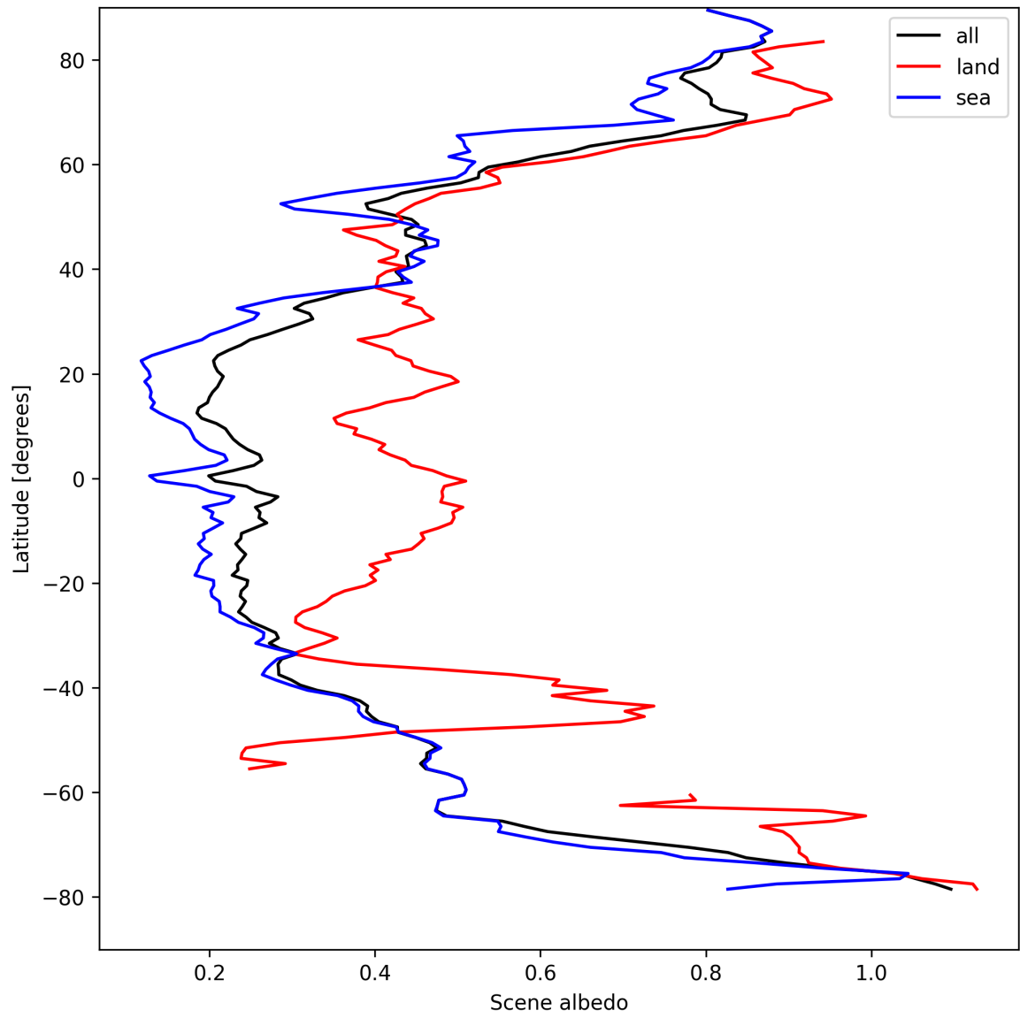
Figure 17: Zonal average of “Scene albedo” for 2025-04-13 to 2025-04-15.
