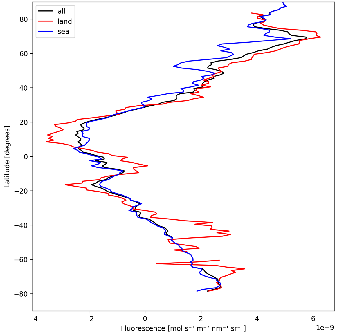
Figure 23: Zonal average of “Fluorescence” for 2025-04-13 to 2025-04-15.
