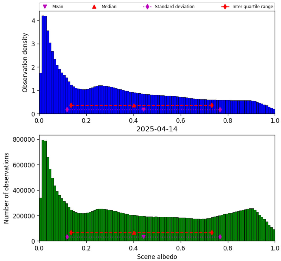
Figure 34: Histogram of “Scene albedo” for 2025-04-13 to 2025-04-15
