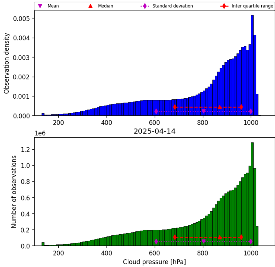
Figure 30: Histogram of “Cloud pressure” for 2025-04-13 to 2025-04-15
