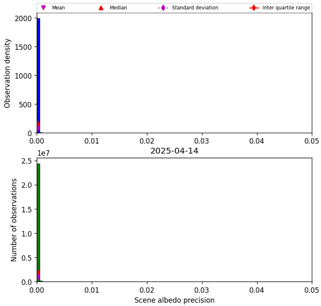
Figure 35: Histogram of “Scene albedo precision” for 2025-04-13 to 2025-04-15
