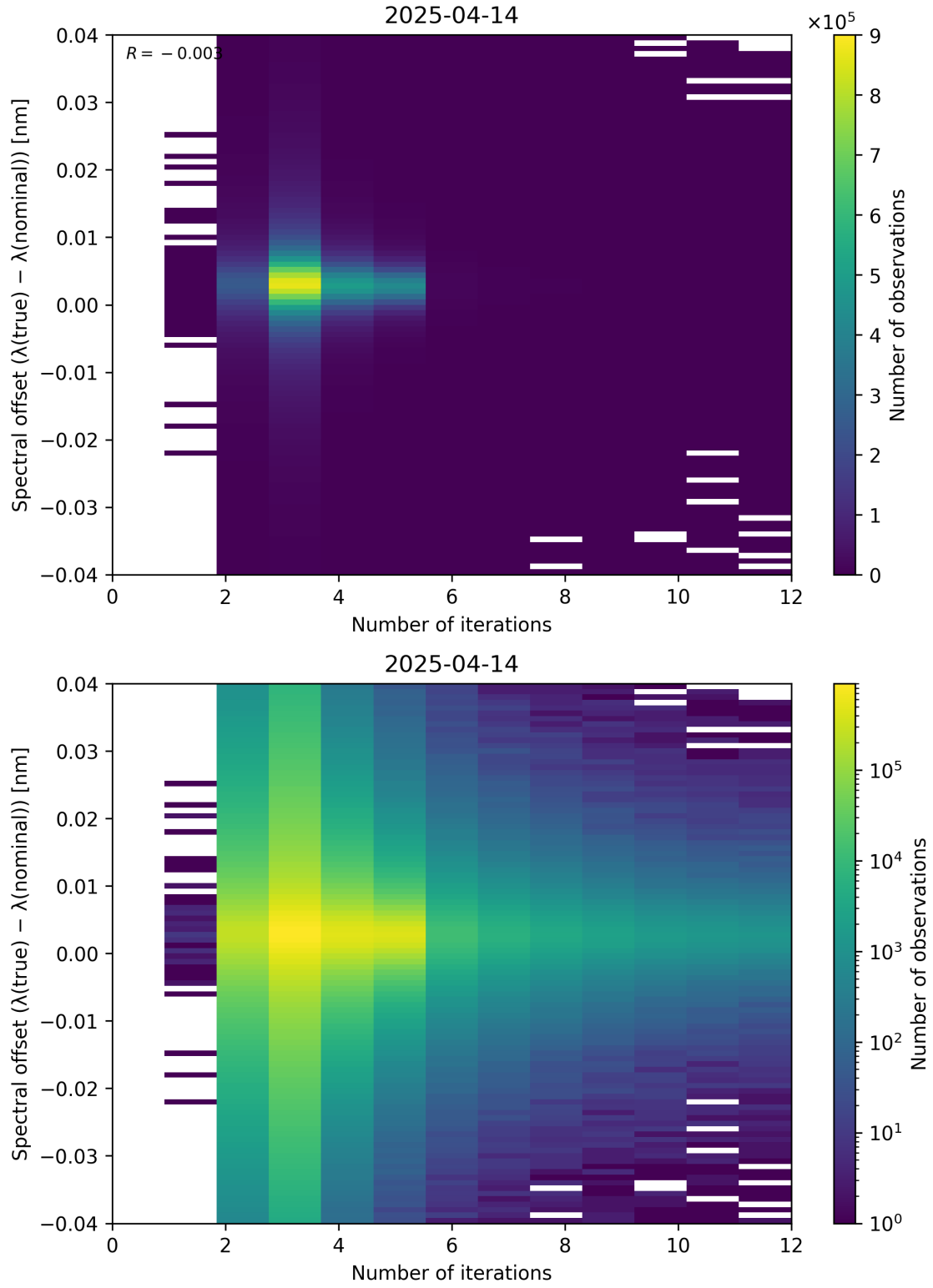
Figure 100: Scatter density plot of “Number of iterations” against “Spectral offset ( \lambda_{\text{true}} - \lambda_{\text{nominal}} )” for 2025-04-13 to 2025-04-15.
