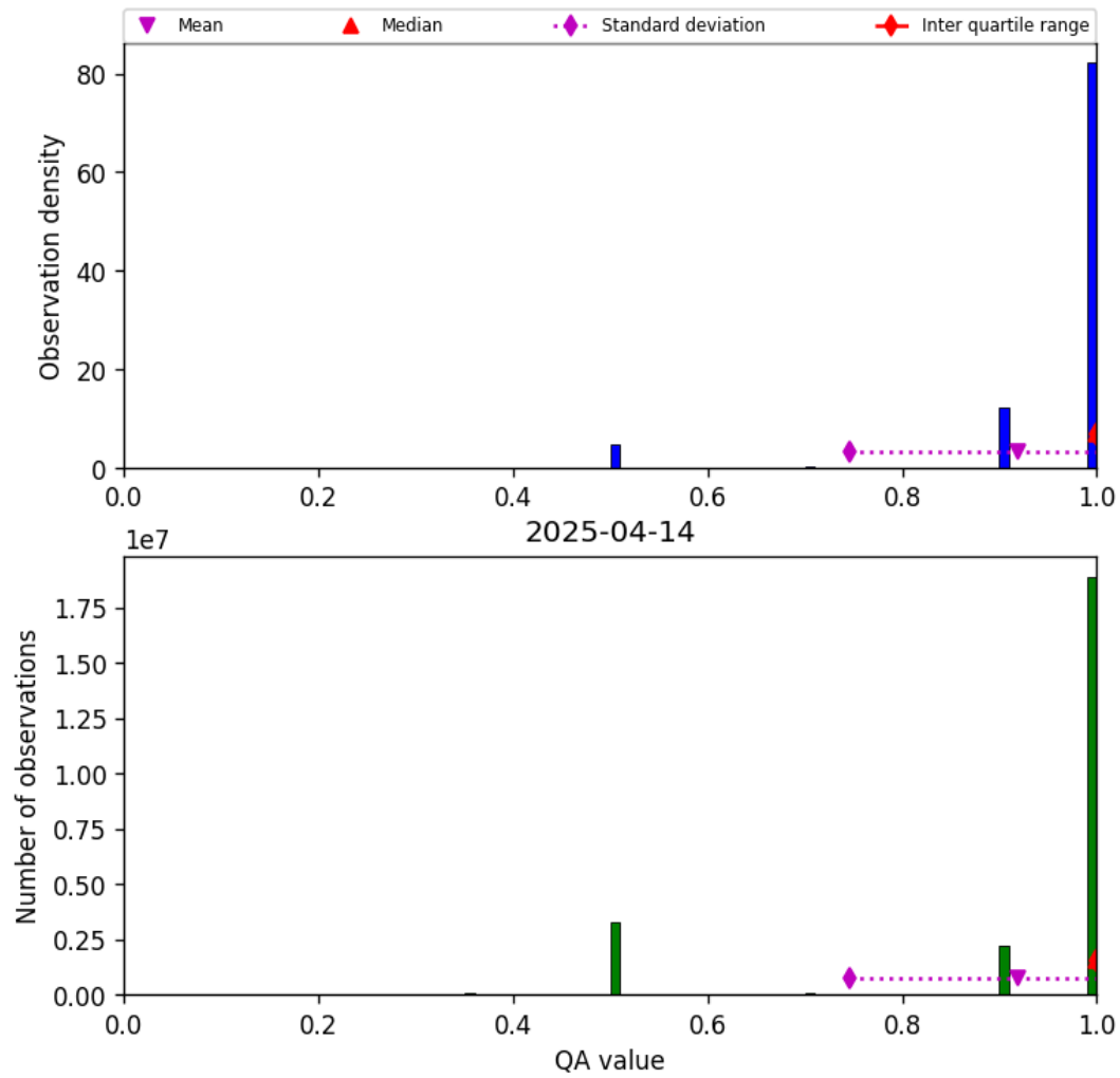
Figure 29: Histogram of “QA value” for 2025-04-13 to 2025-04-15
