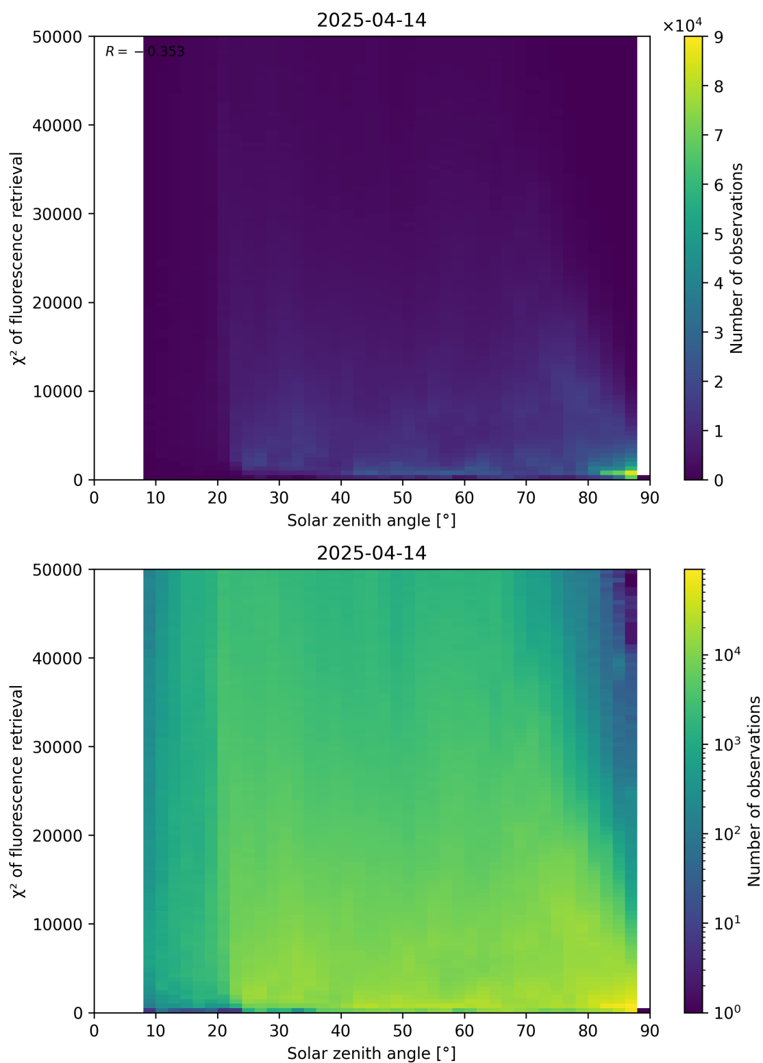
Figure 109: Scatter density plot of “Solar zenith angle” against “ \chi^2 of fluorescence retrieval” for 2025-04-13 to 2025-04-15.
