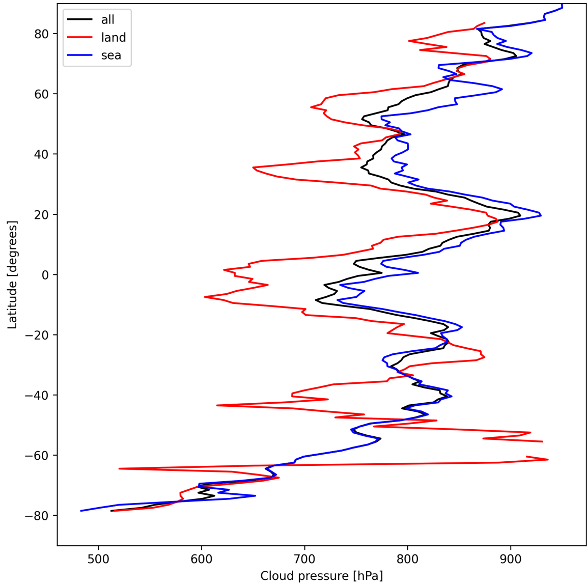
Figure 13: Zonal average of “Cloud pressure” for 2025-04-13 to 2025-04-15.
