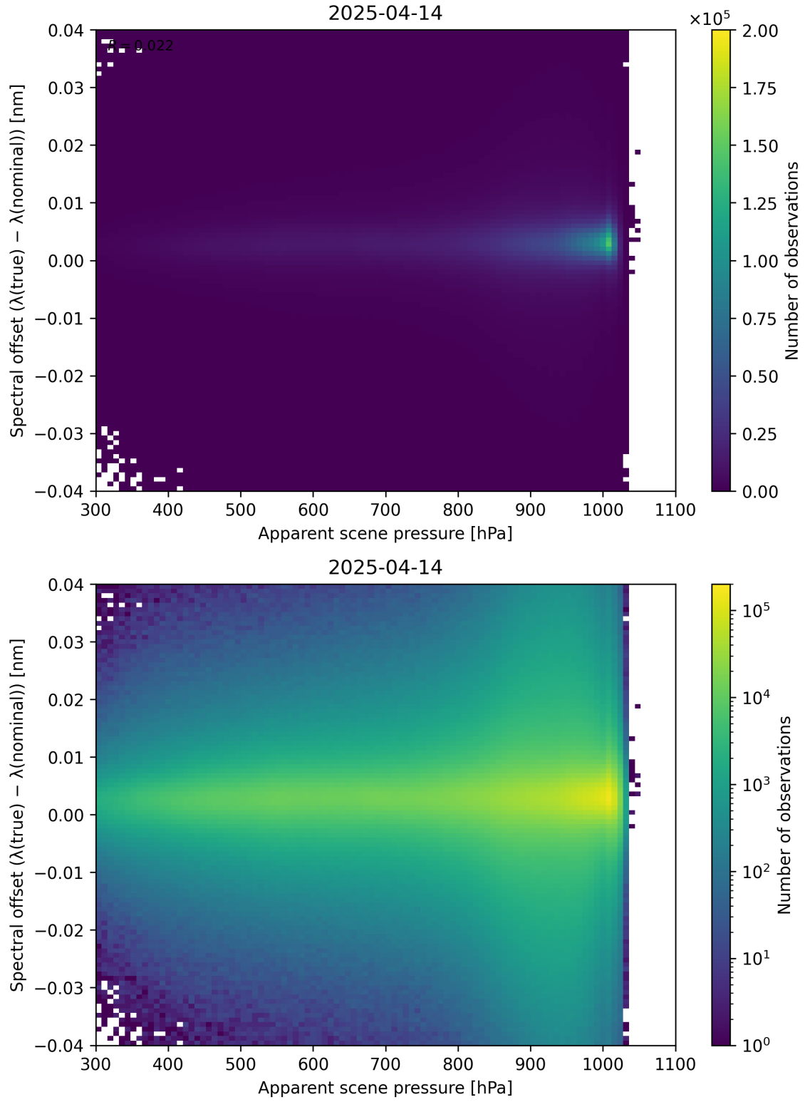
Figure 67: Scatter density plot of “Apparent scene pressure” against “Spectral offset ( \lambda_{\text{true}} - \lambda_{\text{nominal}} )” for 2025-04-13 to 2025-04-15.
