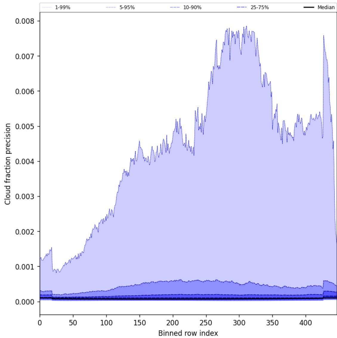
Figure 50: Along track statistics of “Cloud fraction precision” for 2025-04-13 to 2025-04-15
