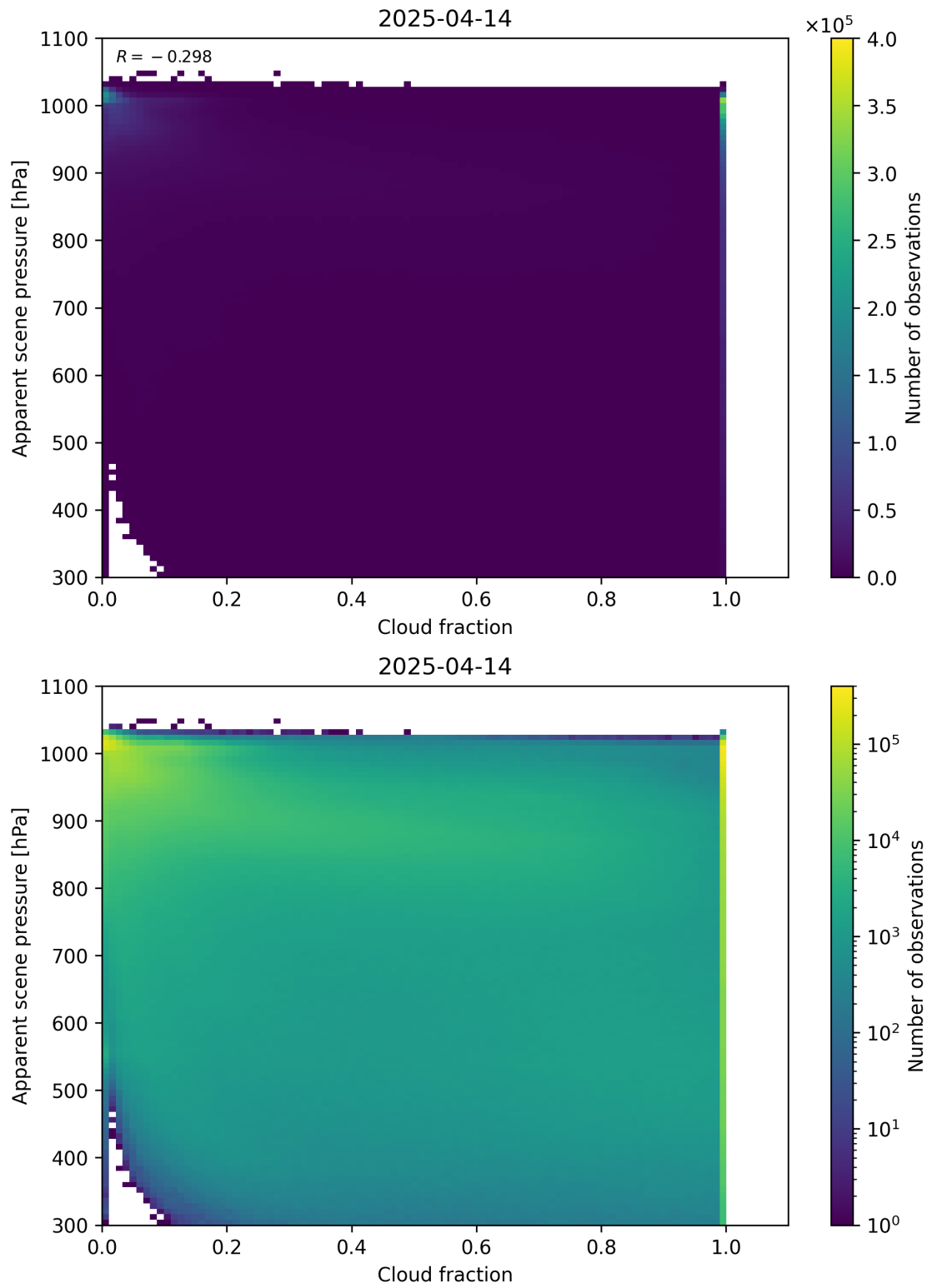
Figure 70: Scatter density plot of “Cloud fraction” against “Apparent scene pressure” for 2025-04-13 to 2025-04-15.
