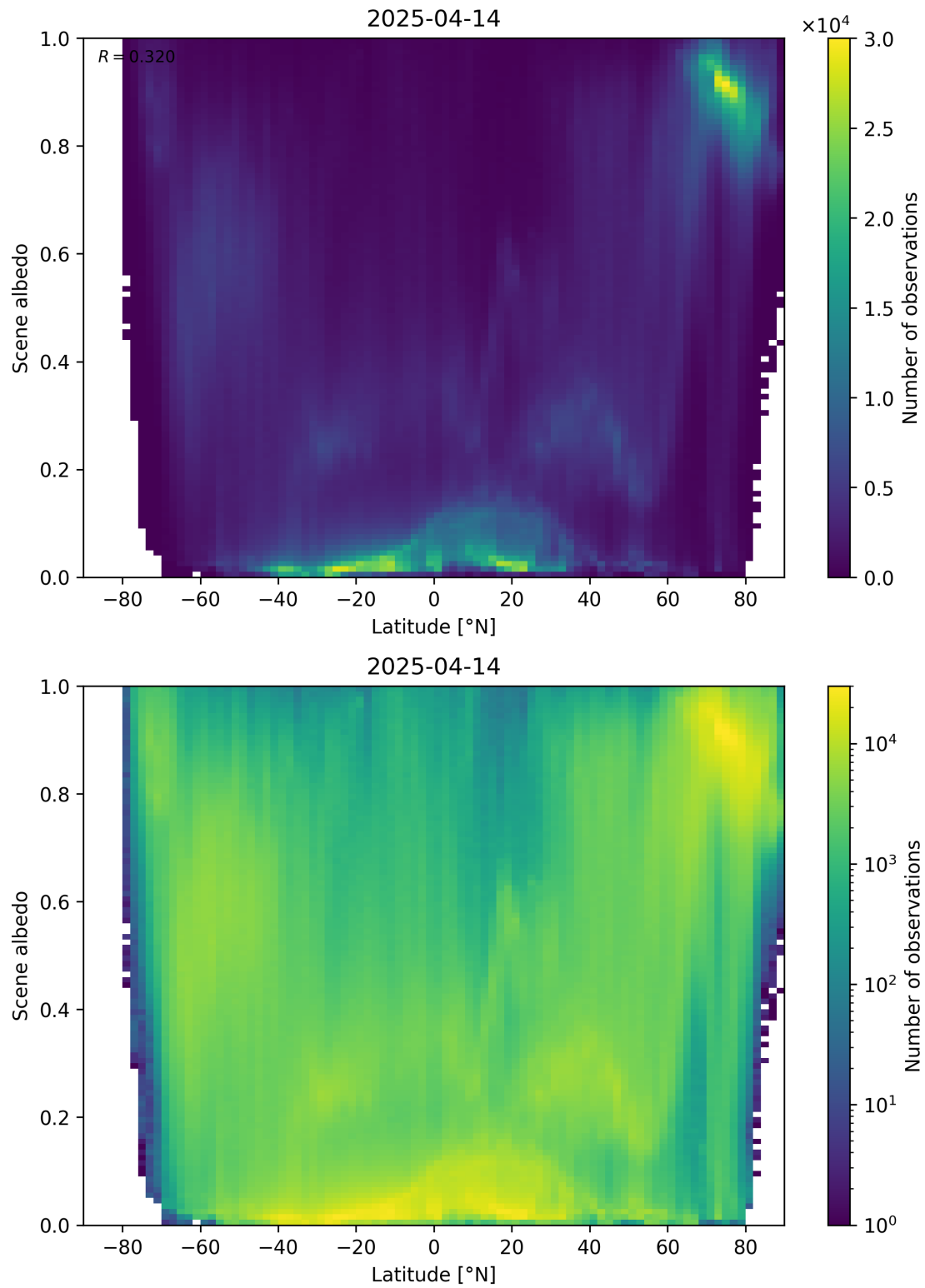
Figure 95: Scatter density plot of “Latitude” against “Scene albedo” for 2025-04-13 to 2025-04-15.
