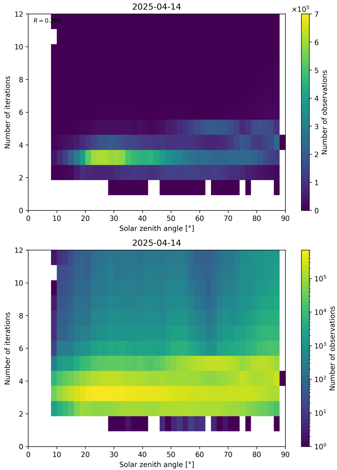
Figure 114: Scatter density plot of “Solar zenith angle” against “Number of iterations” for 2025-04-13 to 2025-04-15.
