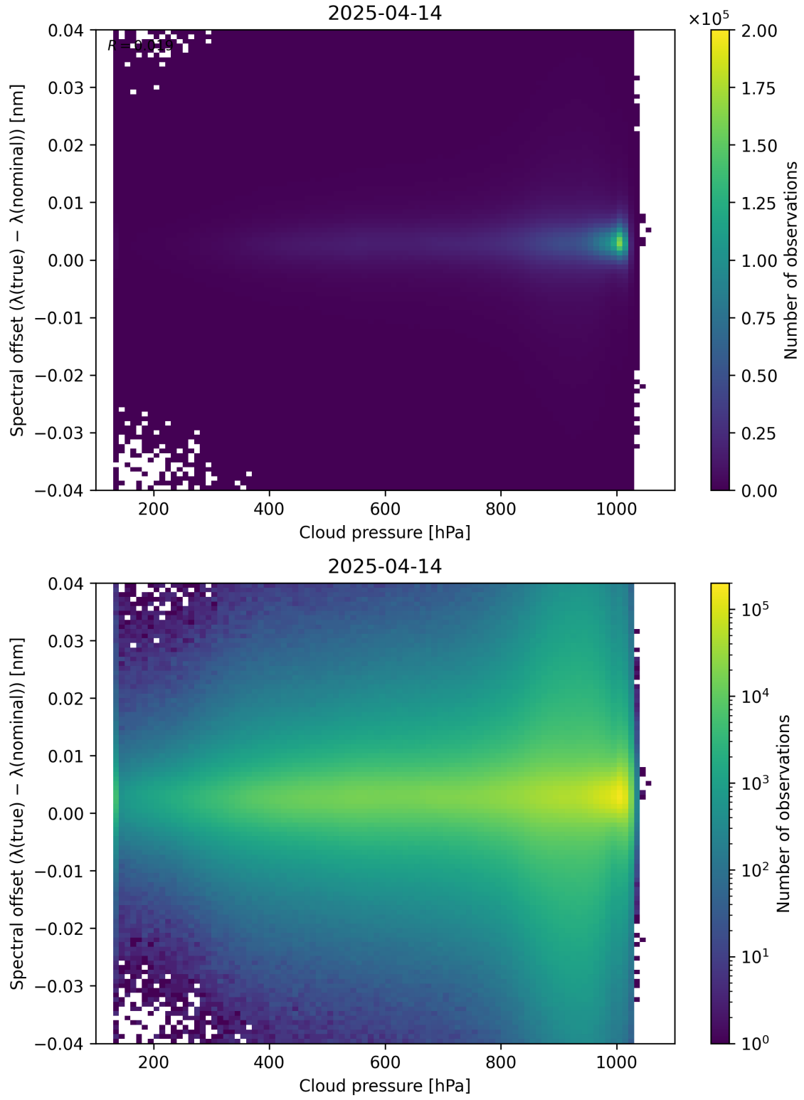
Figure 84: Scatter density plot of “Cloud pressure” against “Spectral offset ( \lambda_{\text{true}} - \lambda_{\text{nominal}} )” for 2025-04-13 to 2025-04-15.
