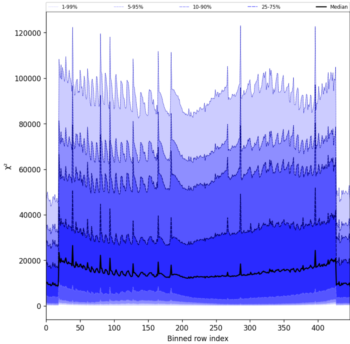
Figure 55: Along track statistics of “ \chi^2 ” for 2025-04-13 to 2025-04-15
