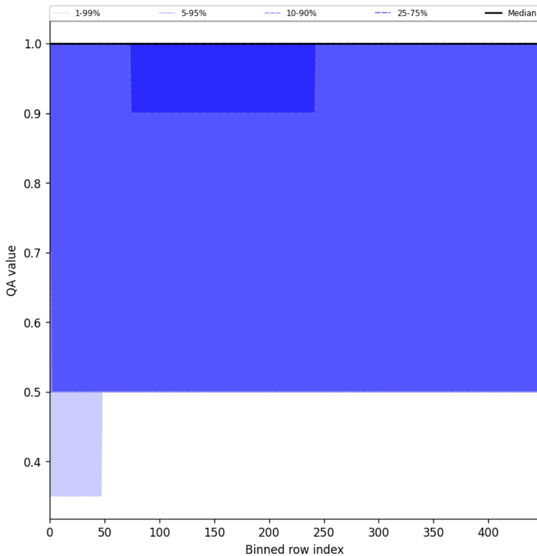
Figure 46: Along track statistics of “QA value” for 2025-04-13 to 2025-04-15
