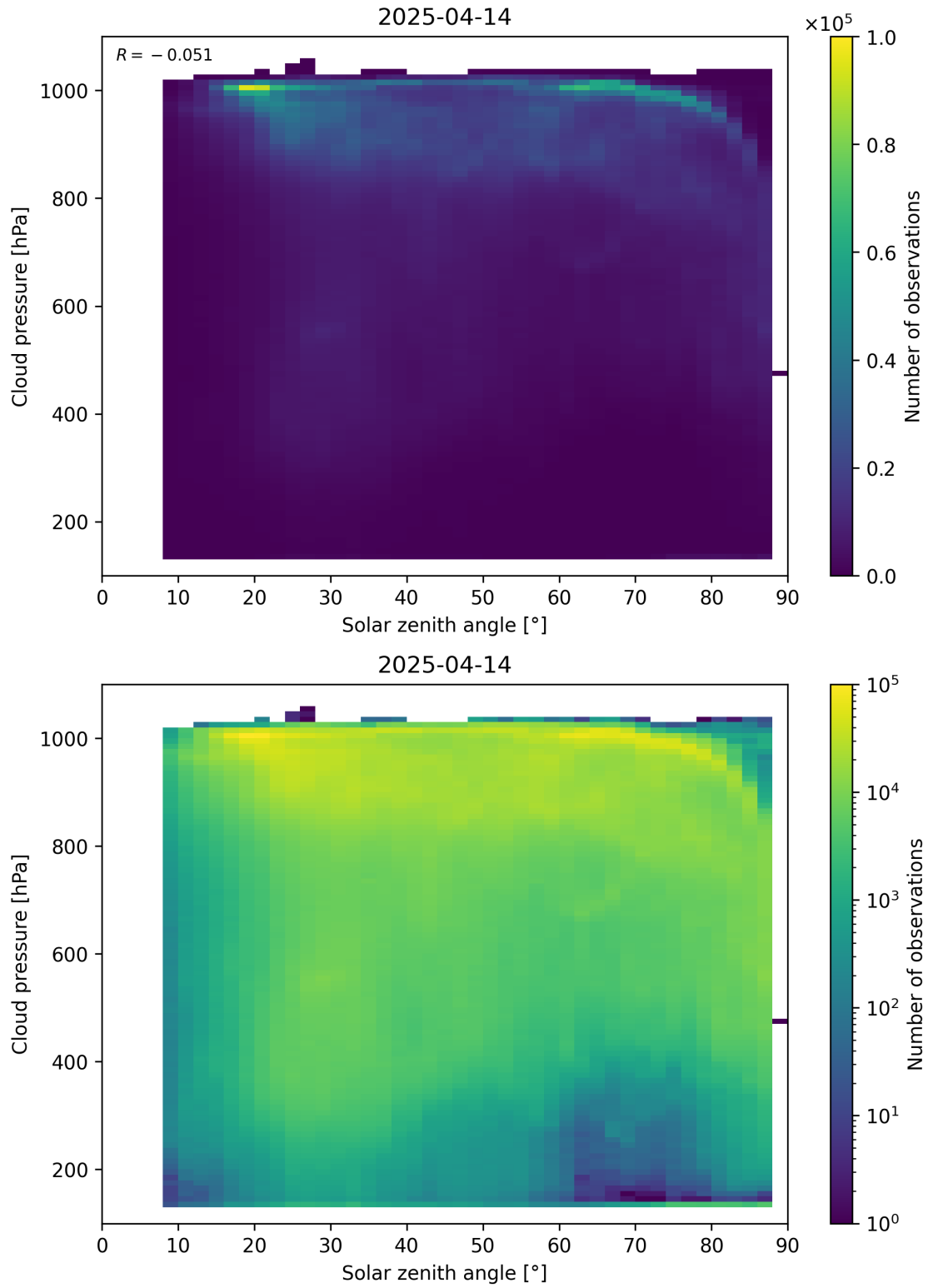
Figure 111: Scatter density plot of “Solar zenith angle” against “Cloud pressure” for 2025-04-13 to 2025-04-15.
