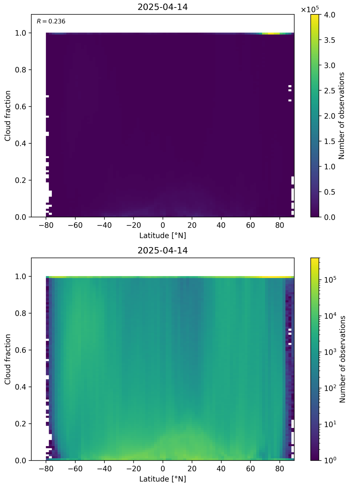
Figure 90: Scatter density plot of “Latitude” against “Cloud fraction” for 2025-04-13 to 2025-04-15.
