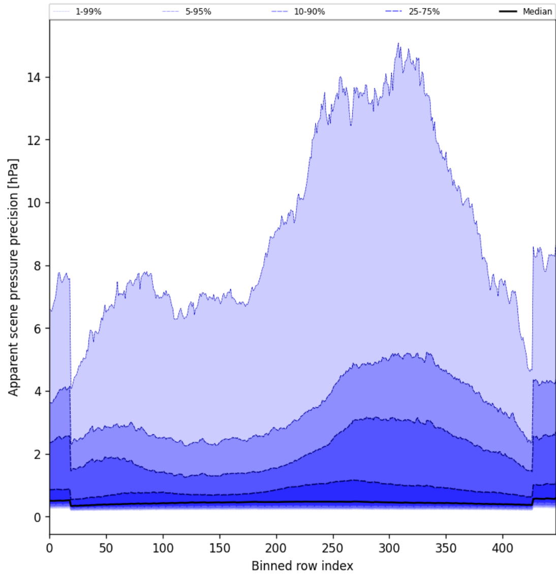
Figure 54: Along track statistics of “Apparent scene pressure precision” for 2025-04-13 to 2025-04-15
