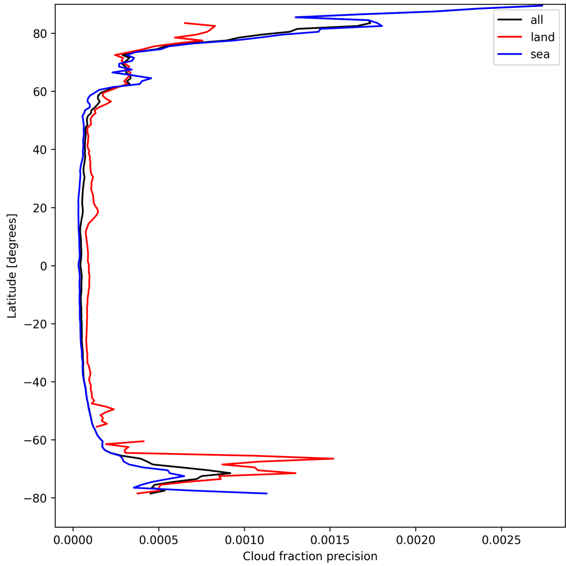
Figure 16: Zonal average of “Cloud fraction precision” for 2025-04-13 to 2025-04-15.
