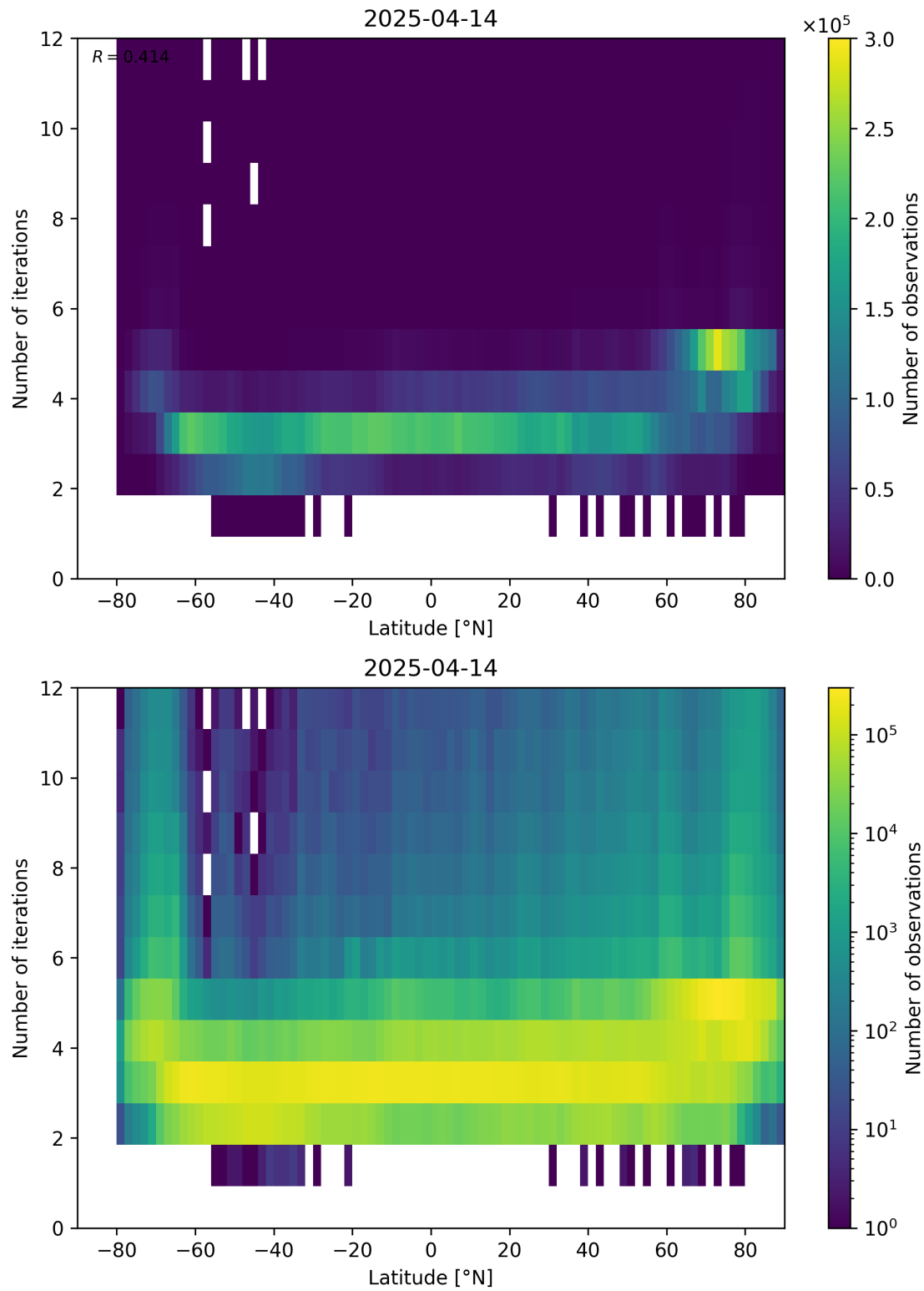
Figure 93: Scatter density plot of “Latitude” against “Number of iterations” for 2025-04-13 to 2025-04-15.
