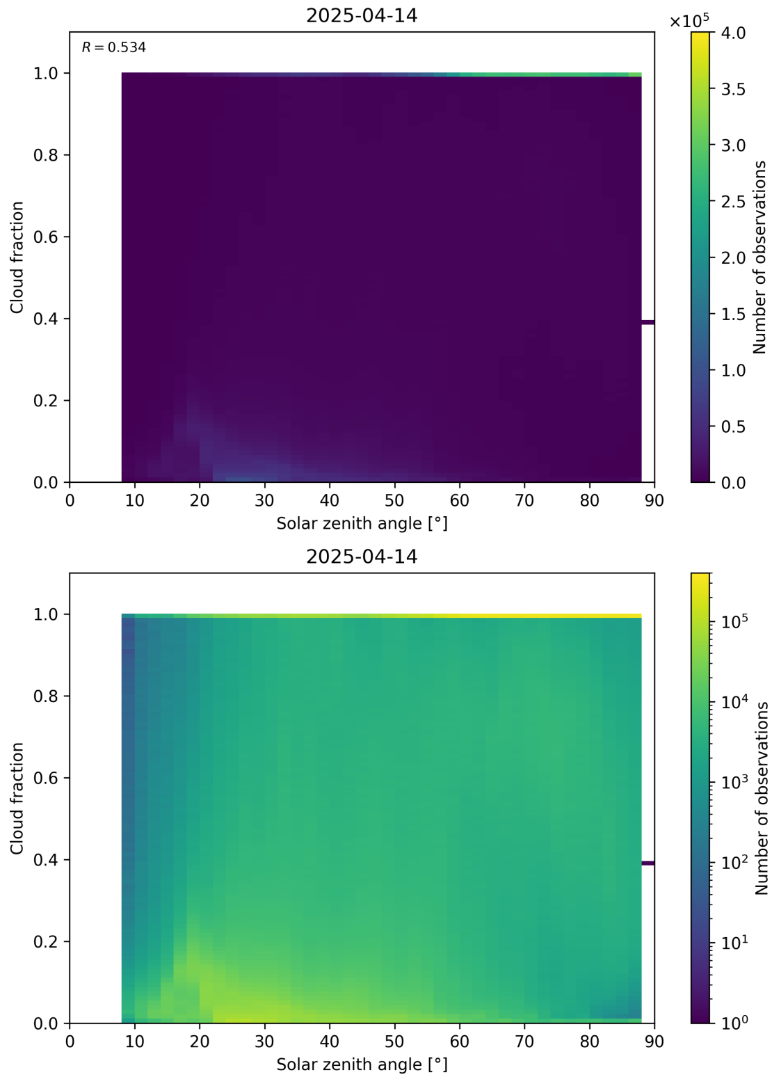
Figure 110: Scatter density plot of “Solar zenith angle” against “Cloud fraction” for 2025-04-13 to 2025-04-15.
