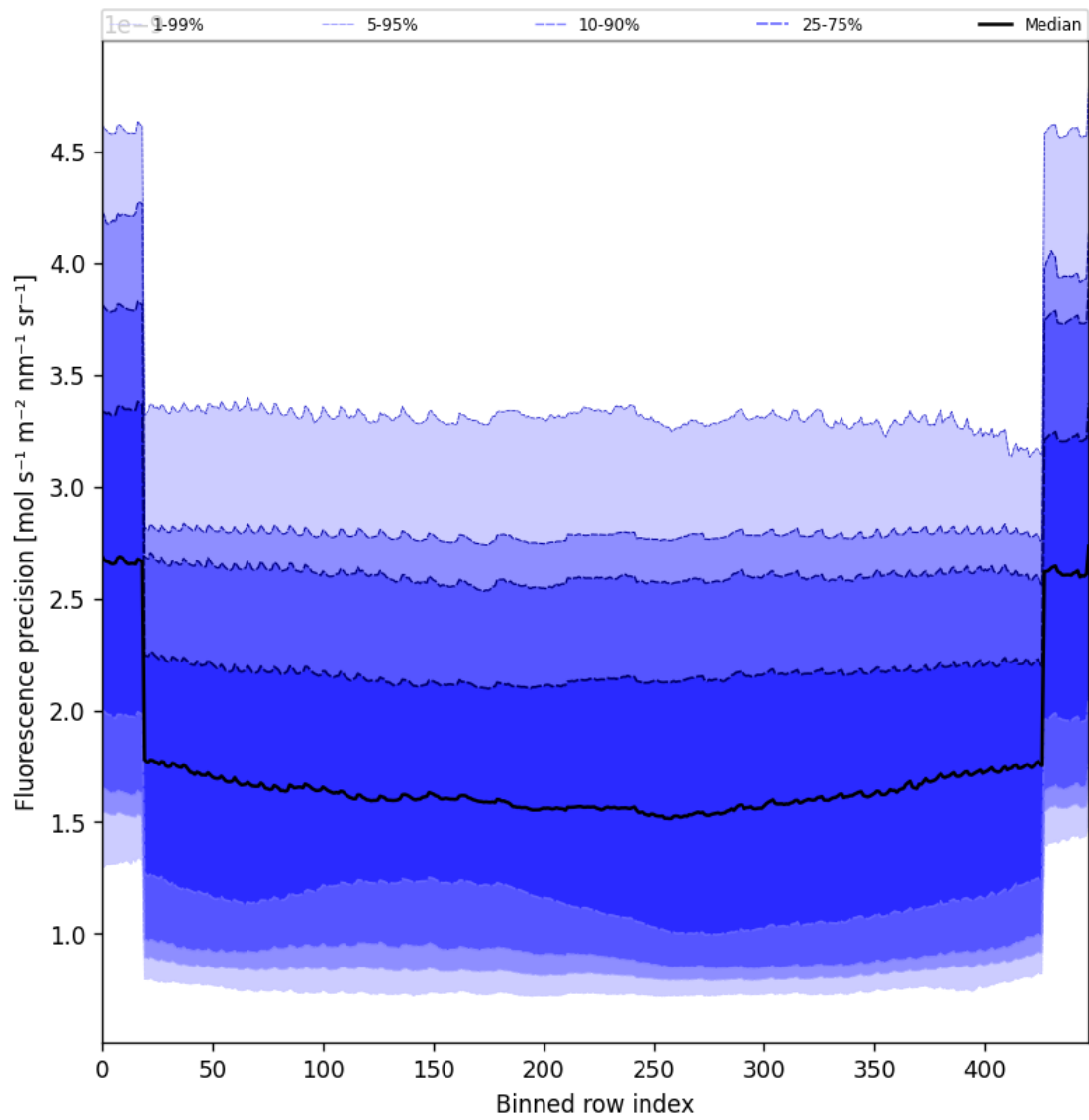
Figure 58: Along track statistics of “Fluorescence precision” for 2025-04-13 to 2025-04-15
