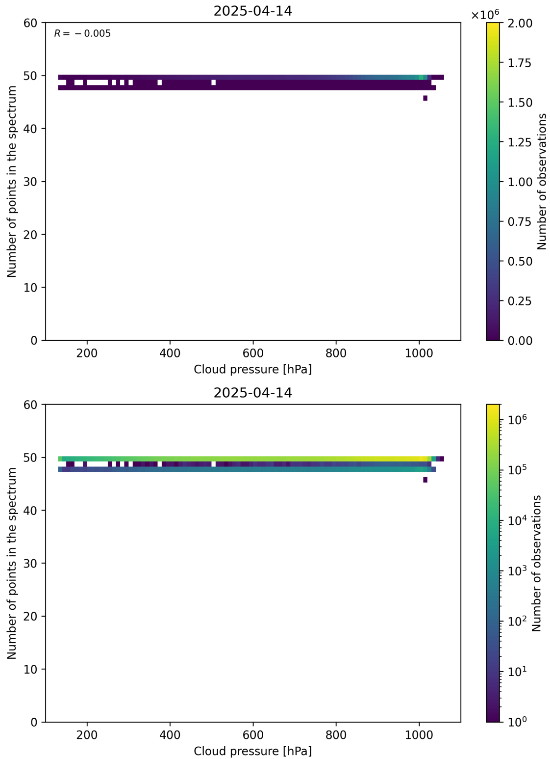
Figure 82: Scatter density plot of “Cloud pressure” against “Number of points in the spectrum” for 2025-04-13 to 2025-04-15.
