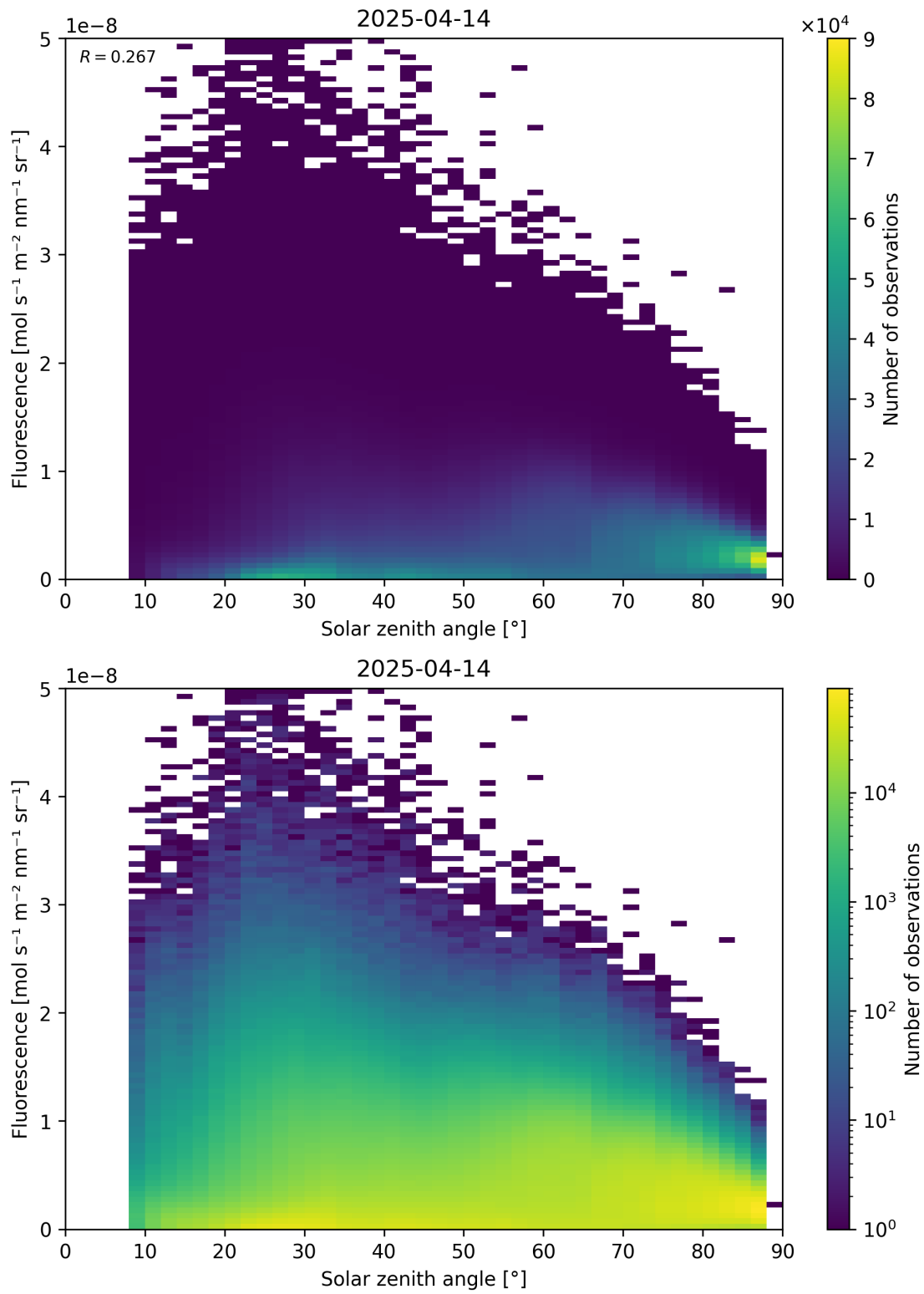
Figure 112: Scatter density plot of “Solar zenith angle” against “Fluorescence” for 2025-04-13 to 2025-04-15.
