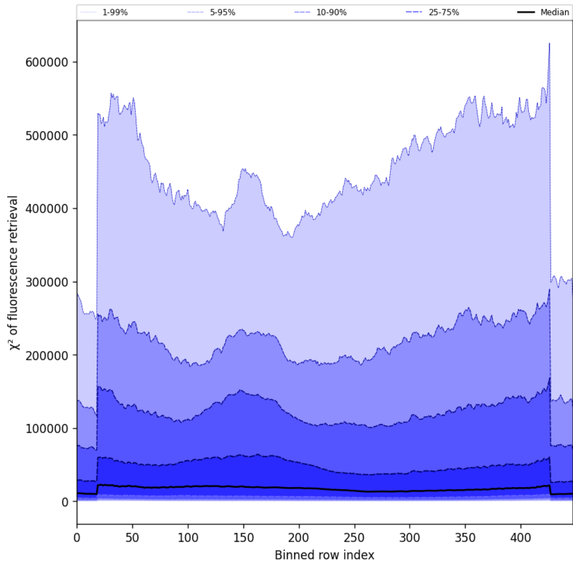
Figure 59: Along track statistics of “ \chi^2 of fluorescence retrieval” for 2025-04-13 to 2025-04-15
