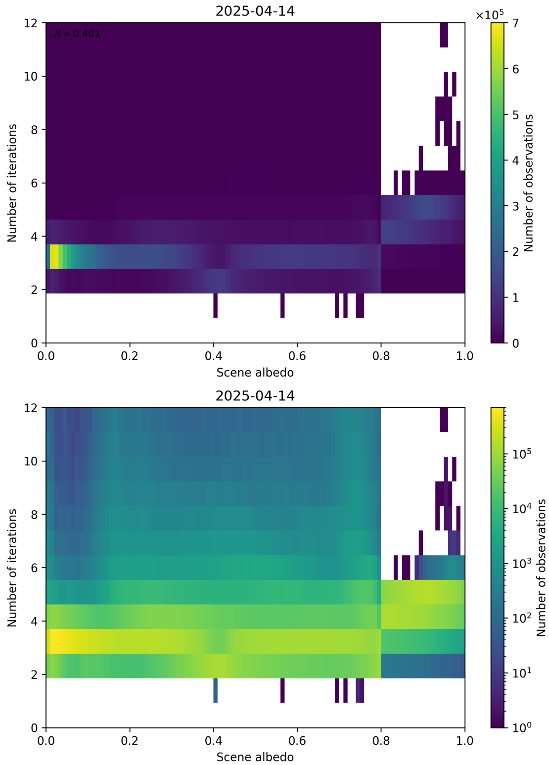
Figure 105: Scatter density plot of “Scene albedo” against “Number of iterations” for 2025-04-13 to 2025-04-15.
