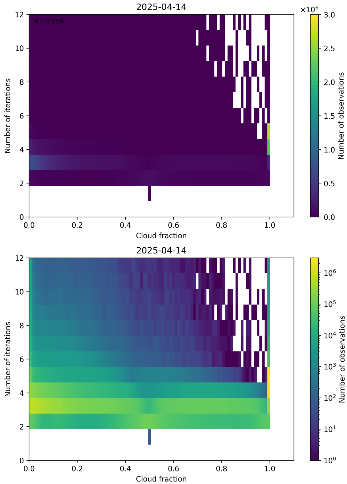
Figure 73: Scatter density plot of “Cloud fraction” against “Number of iterations” for 2025-04-13 to 2025-04-15.
