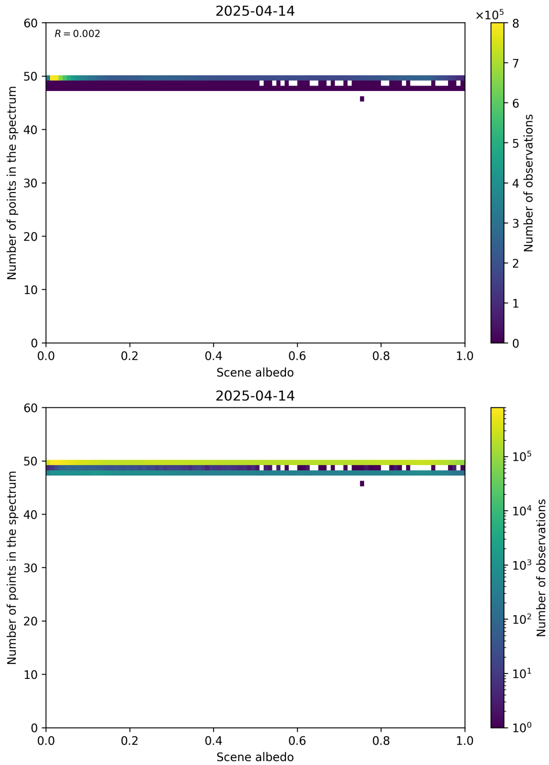
Figure 106: Scatter density plot of “Scene albedo” against “Number of points in the spectrum” for 2025-04-13 to 2025-04-15.
