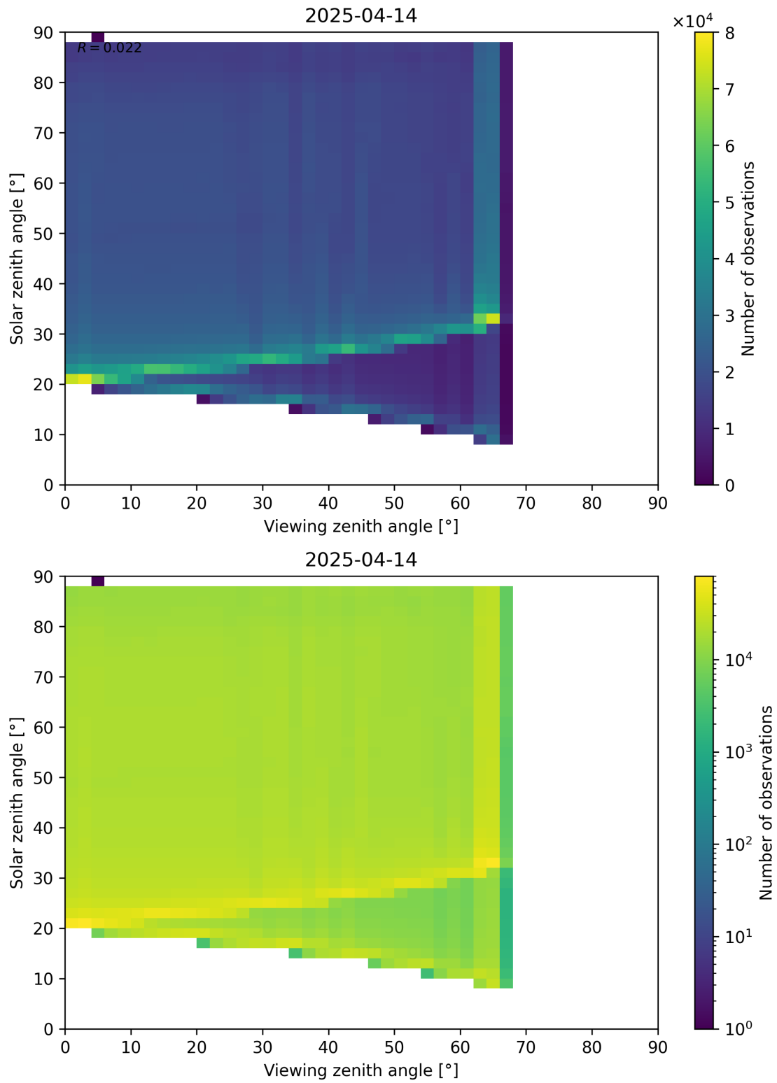
Figure 127: Scatter density plot of “Viewing zenith angle” against “Solar zenith angle” for 2025-04-13 to 2025-04-15.
