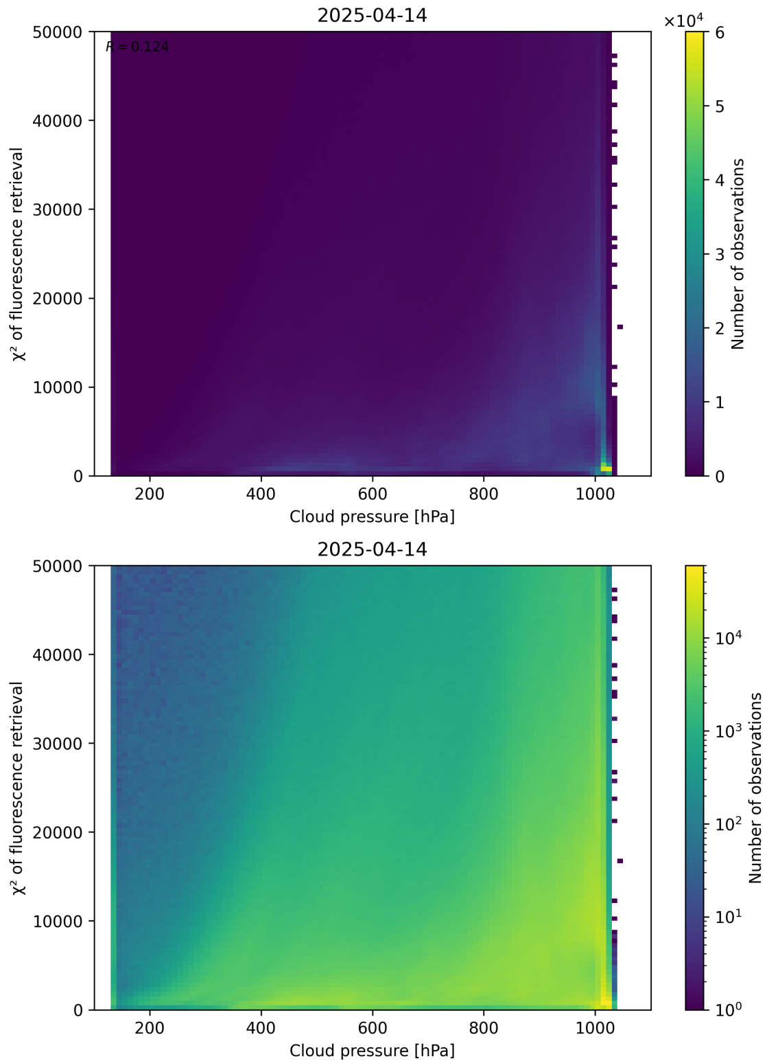
Figure 78: Scatter density plot of “Cloud pressure” against “ \chi^2 of fluorescence retrieval” for 2025-04-13 to 2025-04-15.
