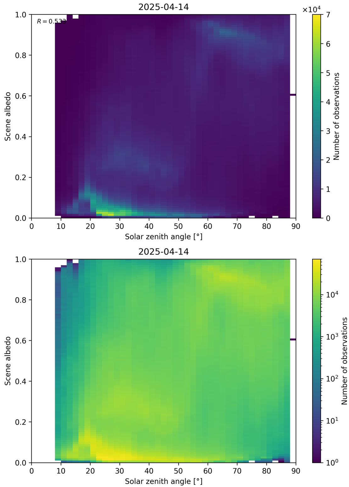
Figure 116: Scatter density plot of “Solar zenith angle” against “Scene albedo” for 2025-04-13 to 2025-04-15.
