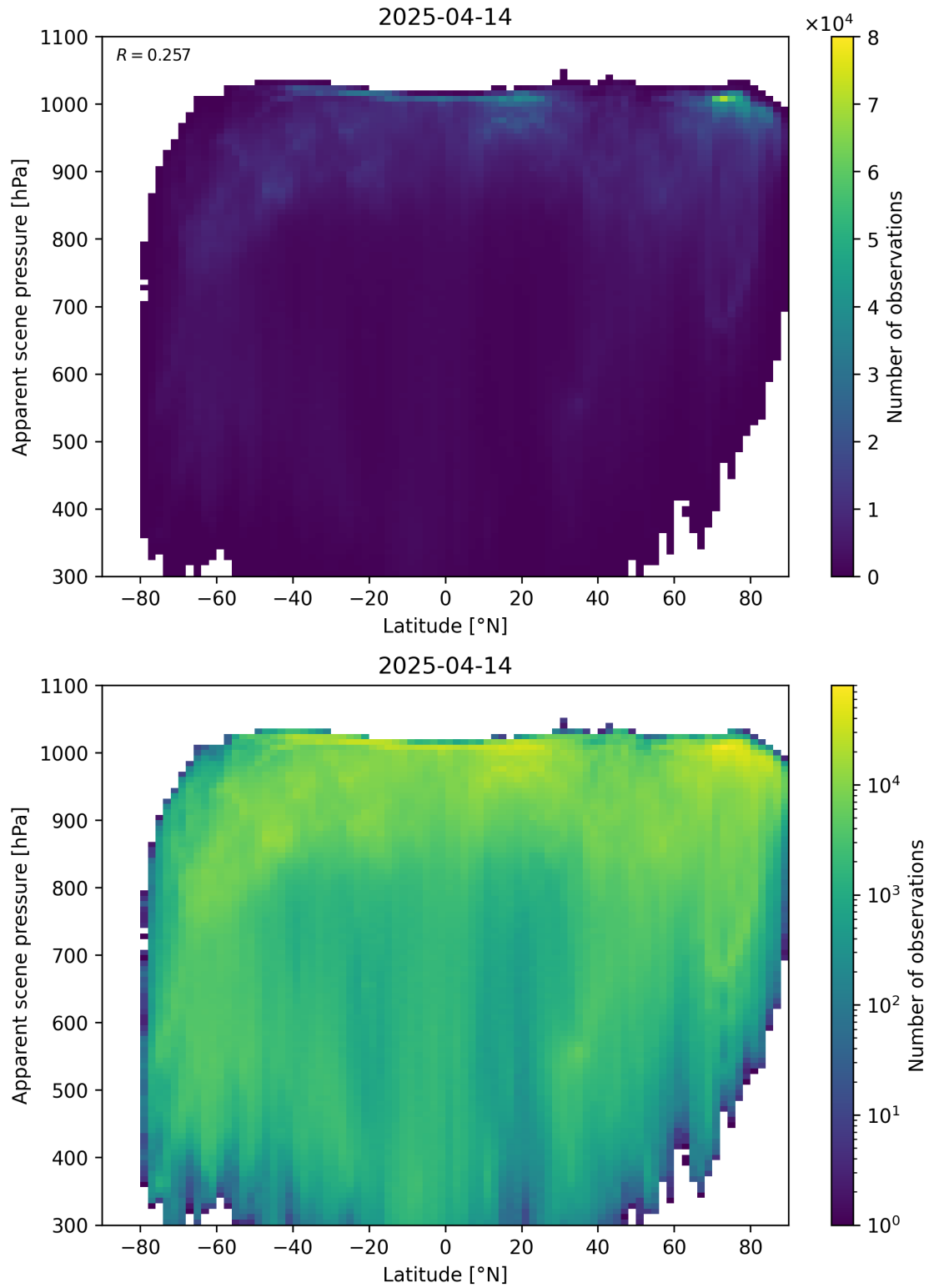
Figure 88: Scatter density plot of “Latitude” against “Apparent scene pressure” for 2025-04-13 to 2025-04-15.
