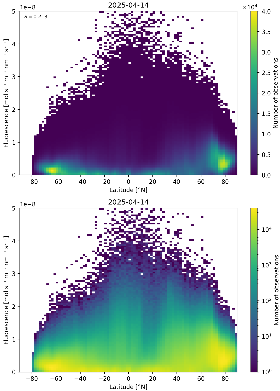
Figure 92: Scatter density plot of “Latitude” against “Fluorescence” for 2025-04-13 to 2025-04-15.
