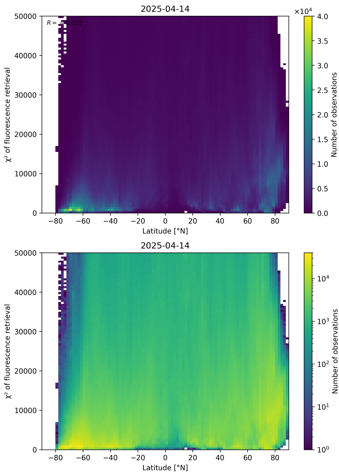
Figure 89: Scatter density plot of “Latitude” against “ \chi^2 of fluorescence retrieval” for 2025-04-13 to 2025-04-15.
