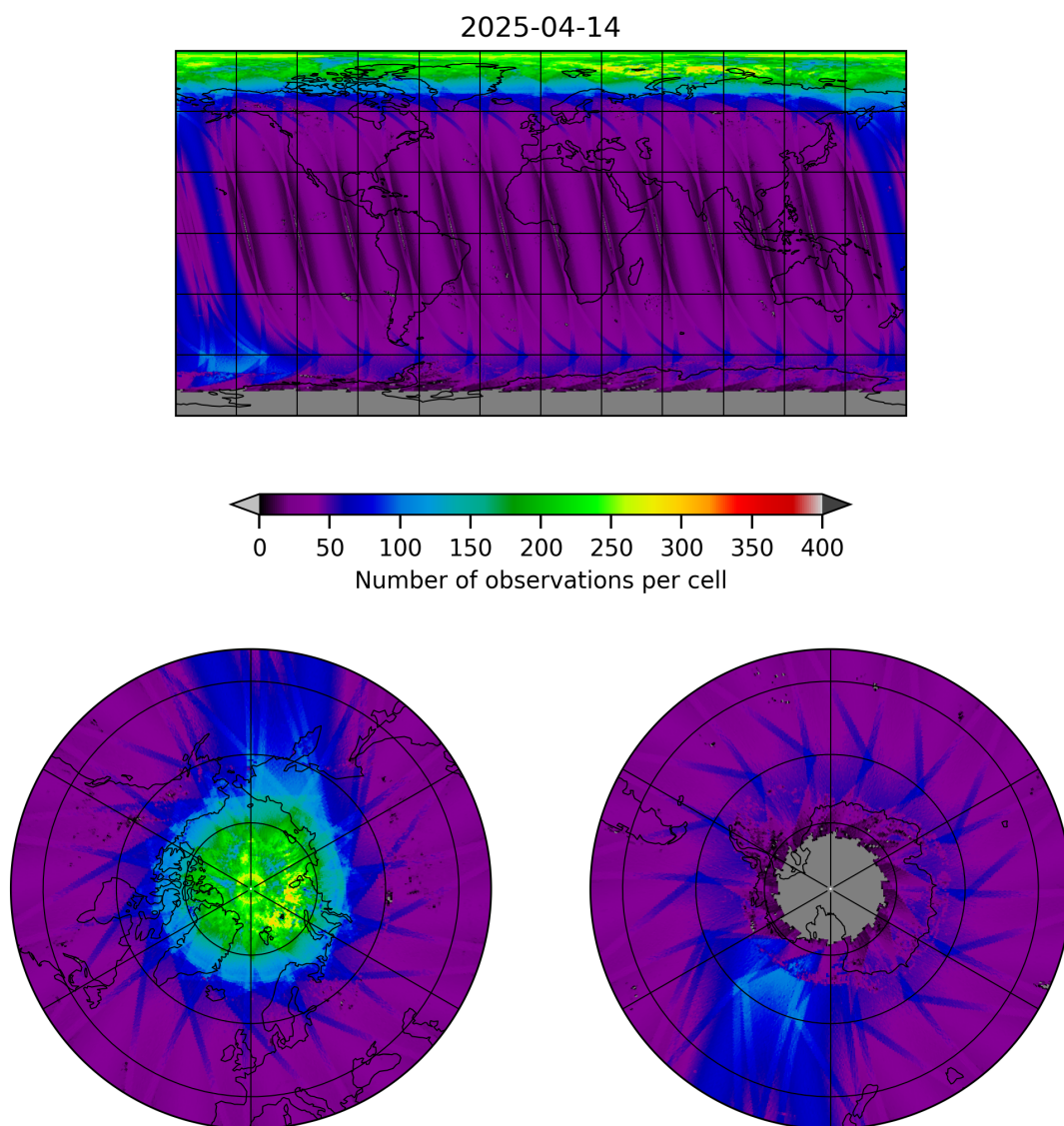
Figure 11: Map of the number of observations for 2025-04-13 to 2025-04-15
