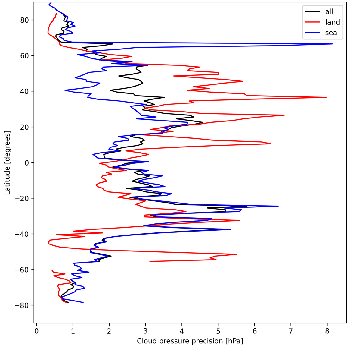
Figure 14: Zonal average of “Cloud pressure precision” for 2025-04-13 to 2025-04-15.
