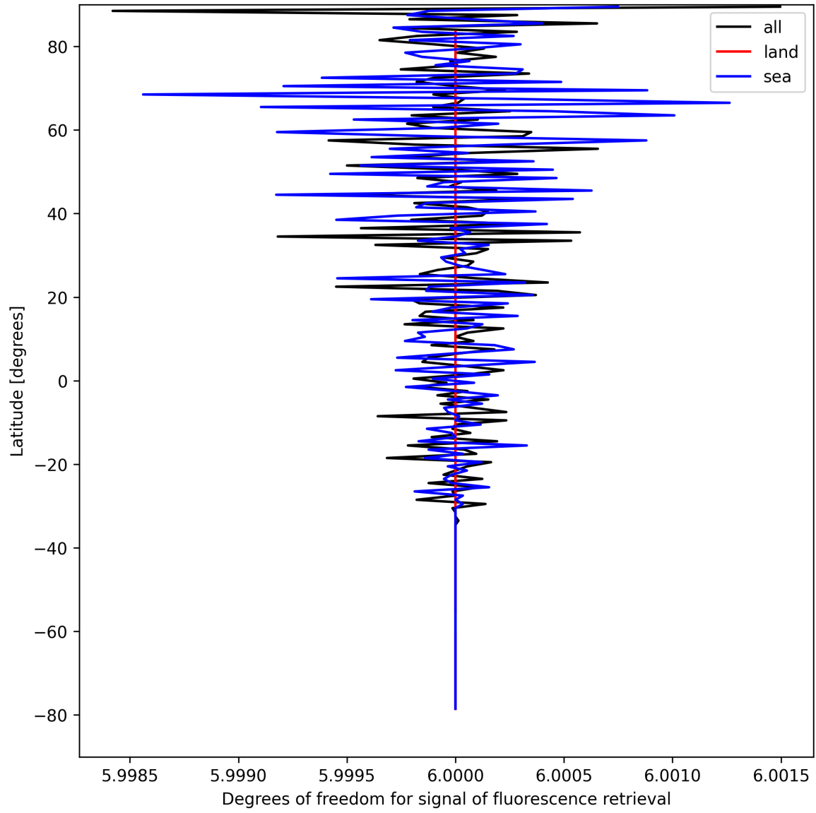
Figure 26: Zonal average of “Degrees of freedom for signal of fluorescence retrieval” for 2025-04-13 to 2025-04-15.
