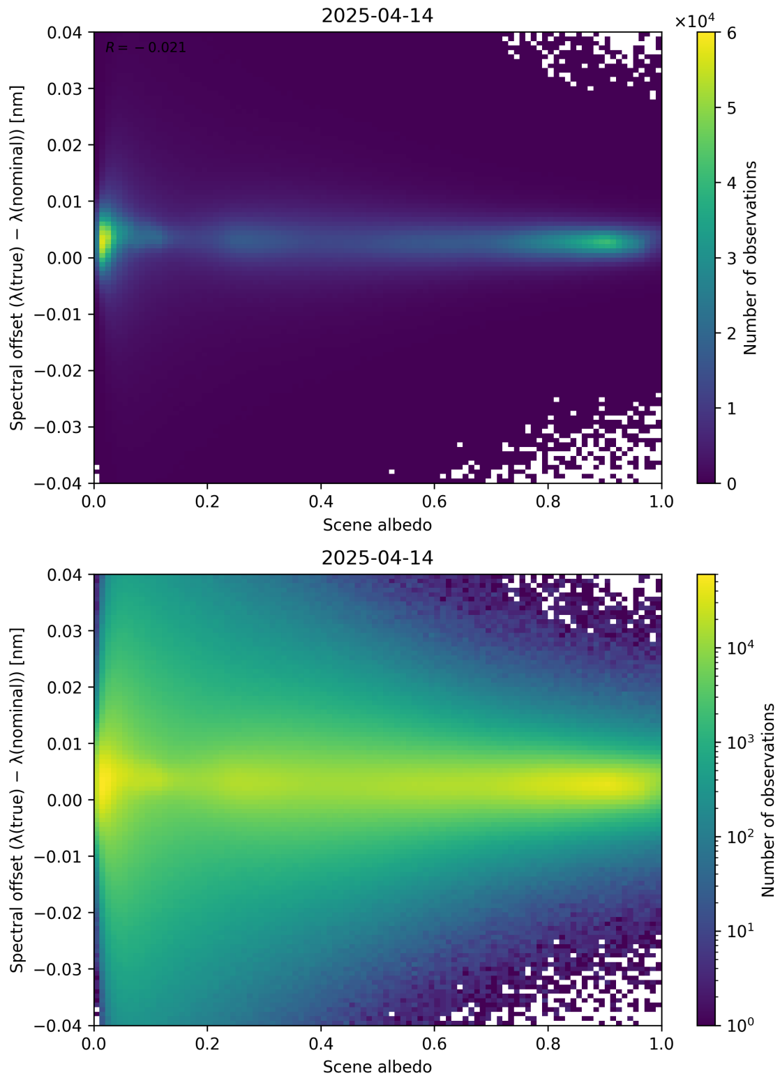
Figure 107: Scatter density plot of “Scene albedo” against “Spectral offset ( \lambda_{\text{true}} - \lambda_{\text{nominal}} )” for 2025-04-13 to 2025-04-15.
