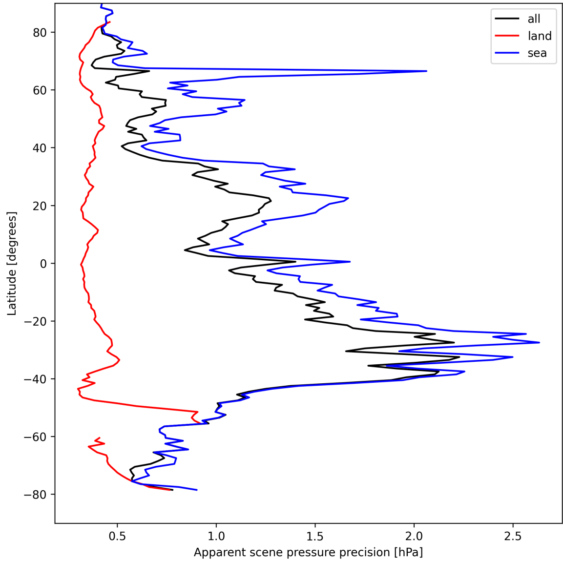
Figure 20: Zonal average of “Apparent scene pressure precision” for 2025-04-13 to 2025-04-15.
