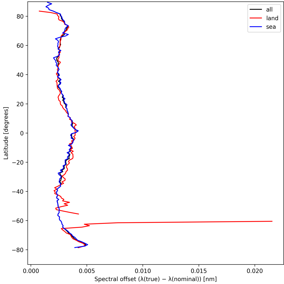
Figure 28: Zonal average of “Spectral offset ( \lambda_{\text{true}} - \lambda_{\text{nominal}} )” for 2025-04-13 to 2025-04-15.
