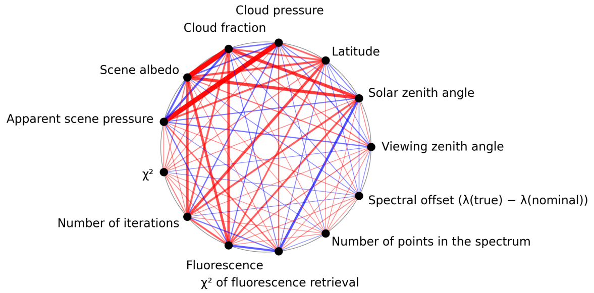
Figure 1: Map of correlation graph for 2025-04-13 to 2025-04-15.
