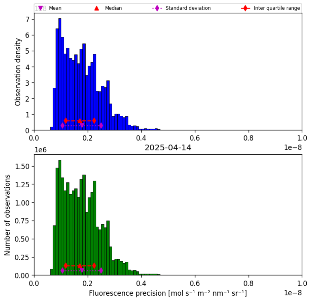
Figure 41: Histogram of “Fluorescence precision” for 2025-04-13 to 2025-04-15
