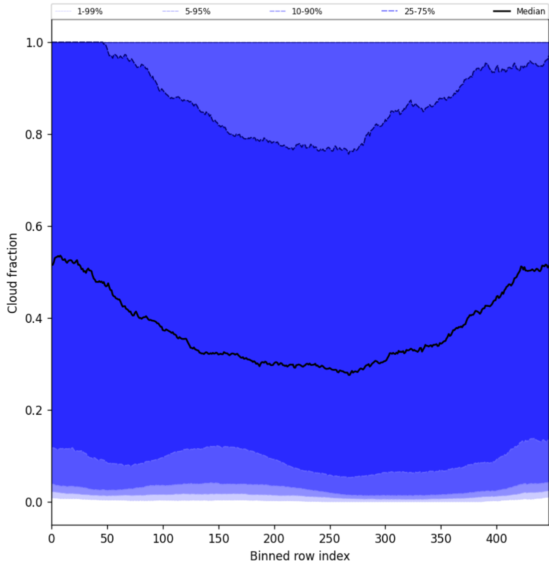
Figure 49: Along track statistics of “Cloud fraction” for 2025-04-13 to 2025-04-15
