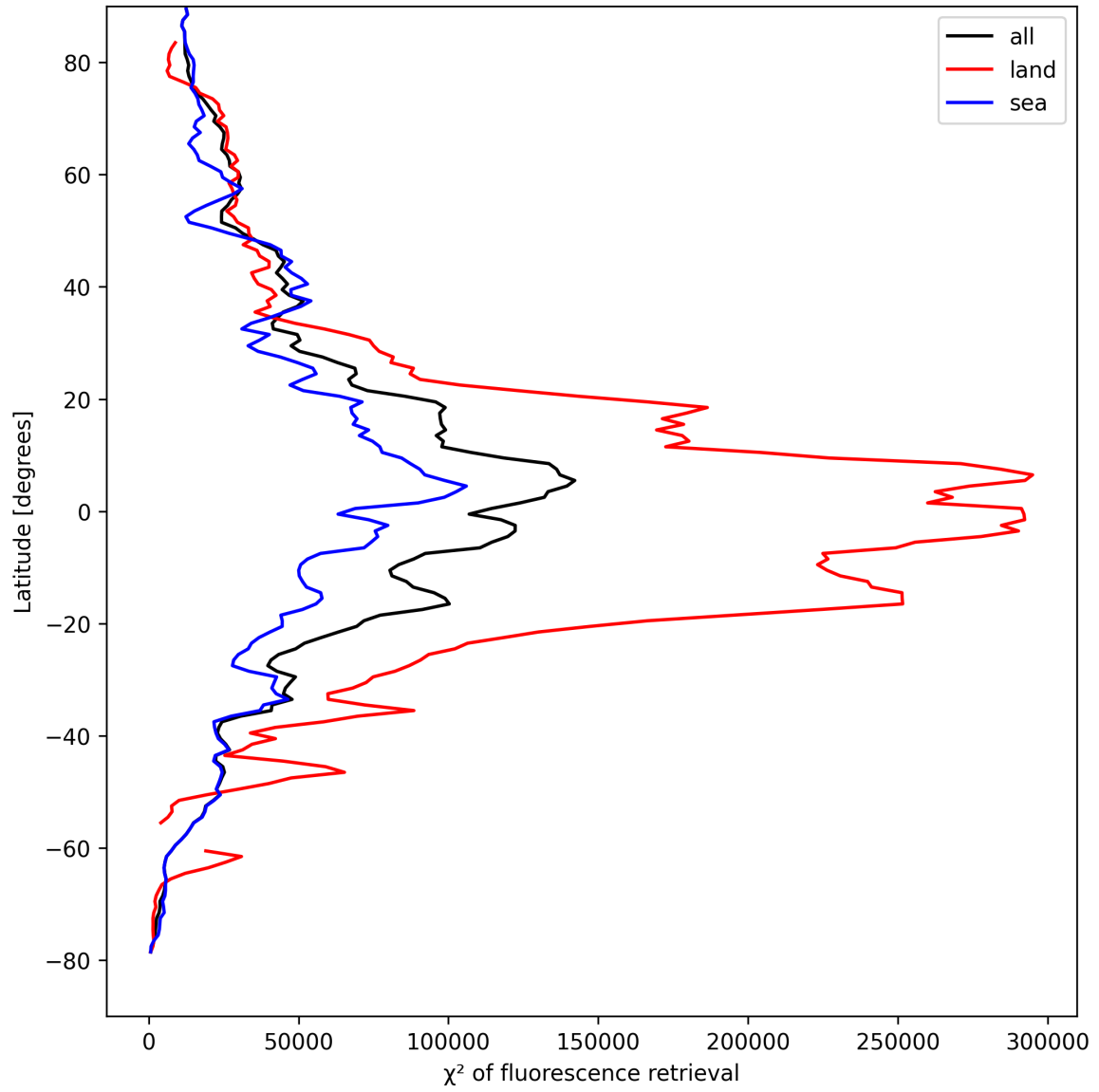
Figure 25: Zonal average of “ \chi^2 of fluorescence retrieval” for 2025-04-13 to 2025-04-15.
