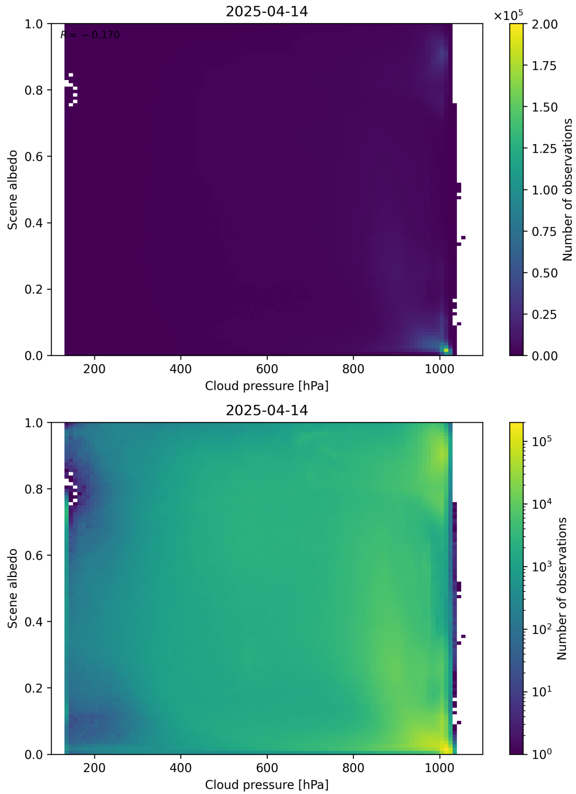
Figure 83: Scatter density plot of “Cloud pressure” against “Scene albedo” for 2025-04-13 to 2025-04-15.
