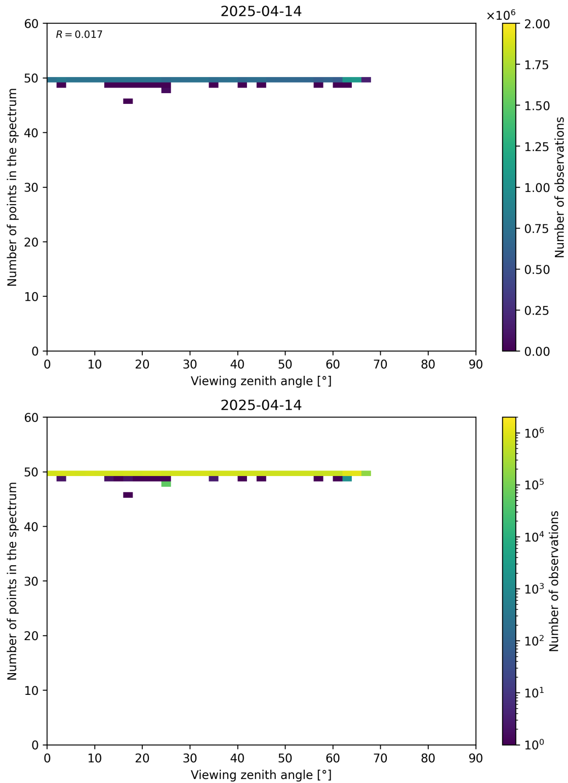
Figure 125: Scatter density plot of “Viewing zenith angle” against “Number of points in the spectrum” for 2025-04-13 to 2025-04-15.
