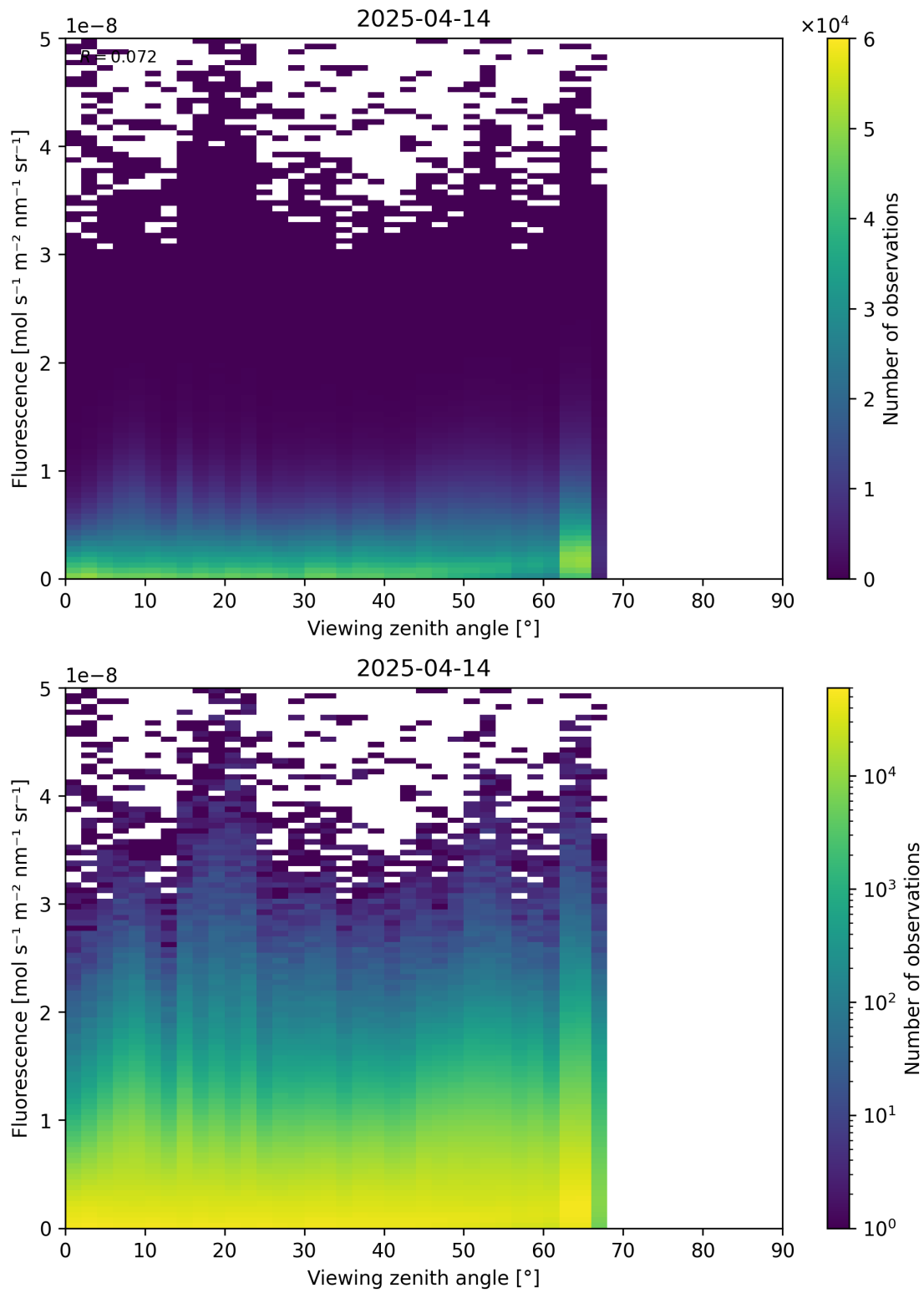
Figure 122: Scatter density plot of “Viewing zenith angle” against “Fluorescence” for 2025-04-13 to 2025-04-15.
