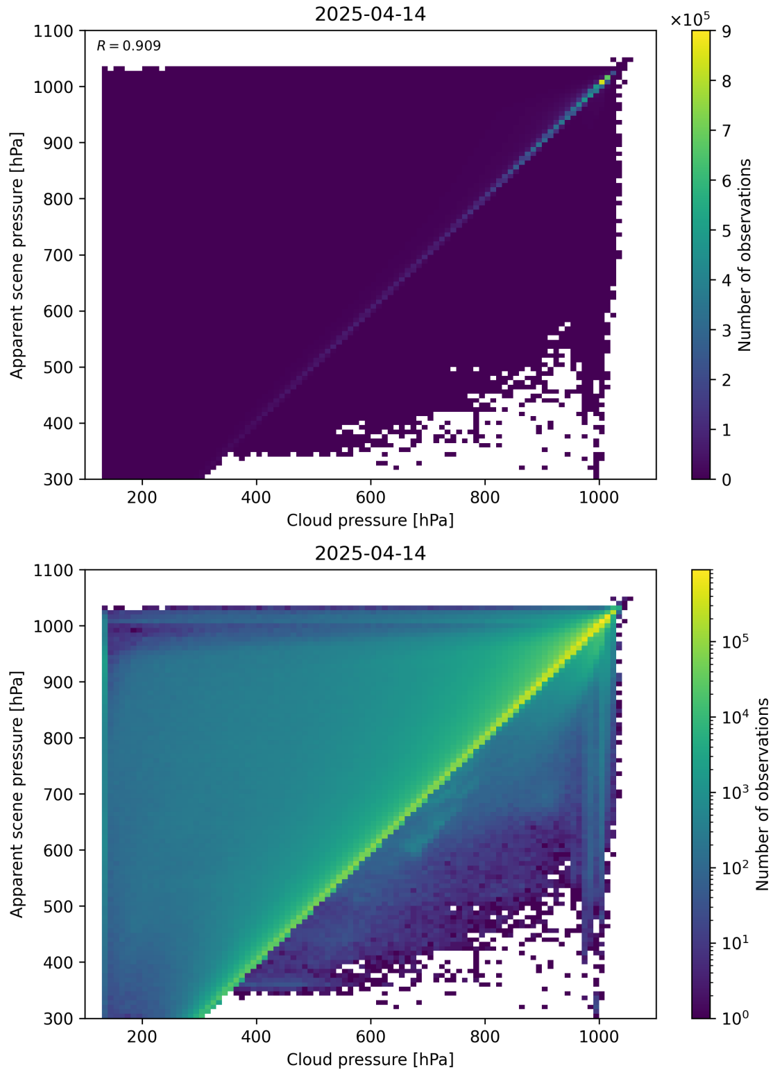
Figure 77: Scatter density plot of “Cloud pressure” against “Apparent scene pressure” for 2025-04-13 to 2025-04-15.
