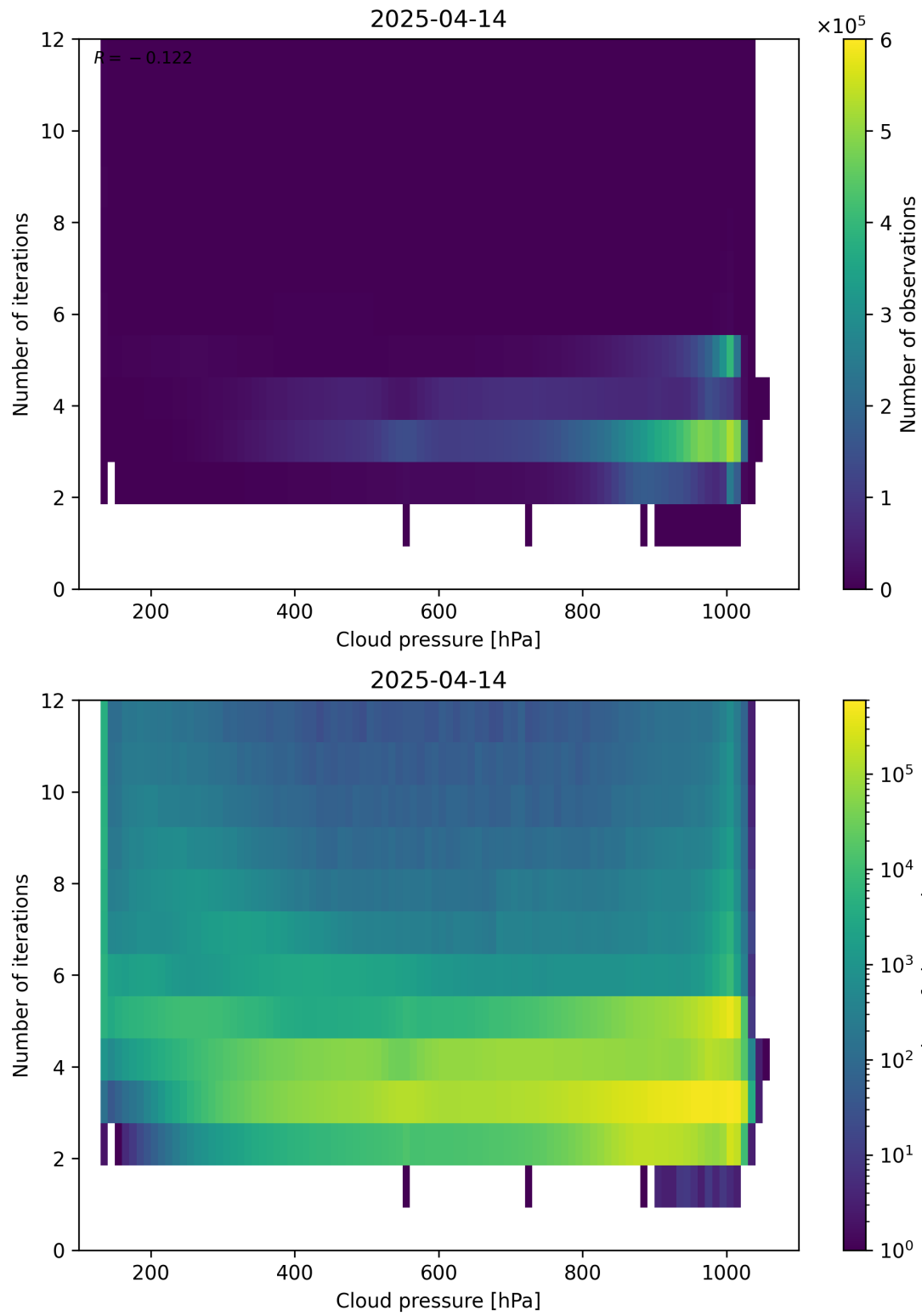
Figure 81: Scatter density plot of “Cloud pressure” against “Number of iterations” for 2025-04-13 to 2025-04-15.
