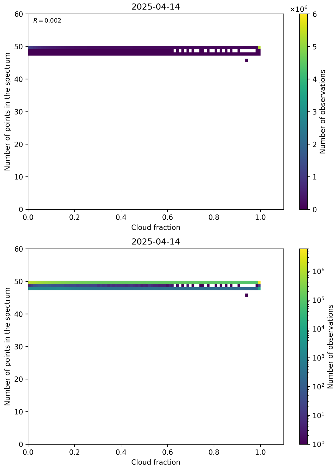
Figure 74: Scatter density plot of “Cloud fraction” against “Number of points in the spectrum” for 2025-04-13 to 2025-04-15.
