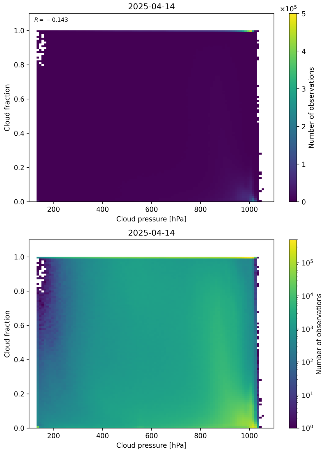
Figure 79: Scatter density plot of “Cloud pressure” against “Cloud fraction” for 2025-04-13 to 2025-04-15.
