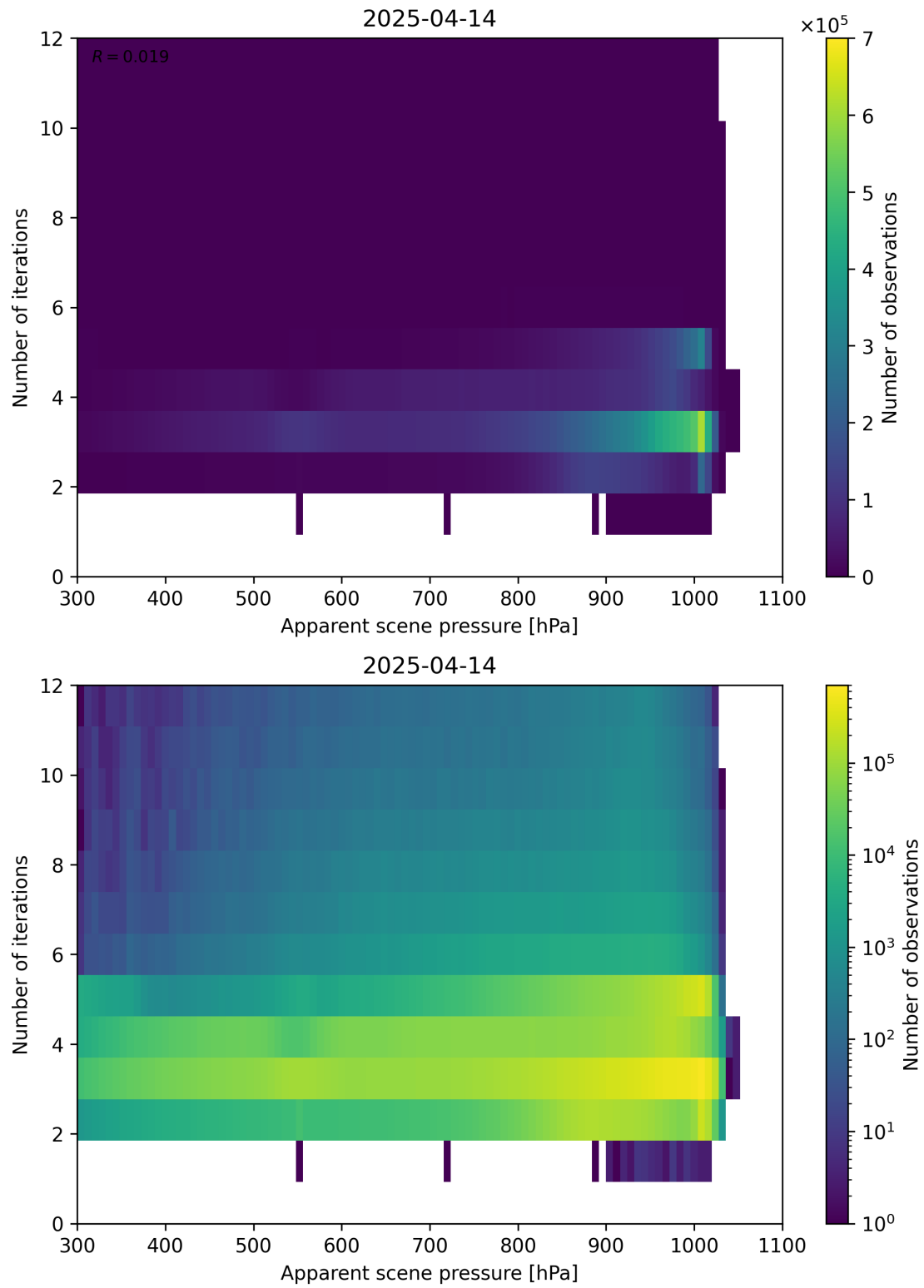
Figure 65: Scatter density plot of “Apparent scene pressure” against “Number of iterations” for 2025-04-13 to 2025-04-15.
