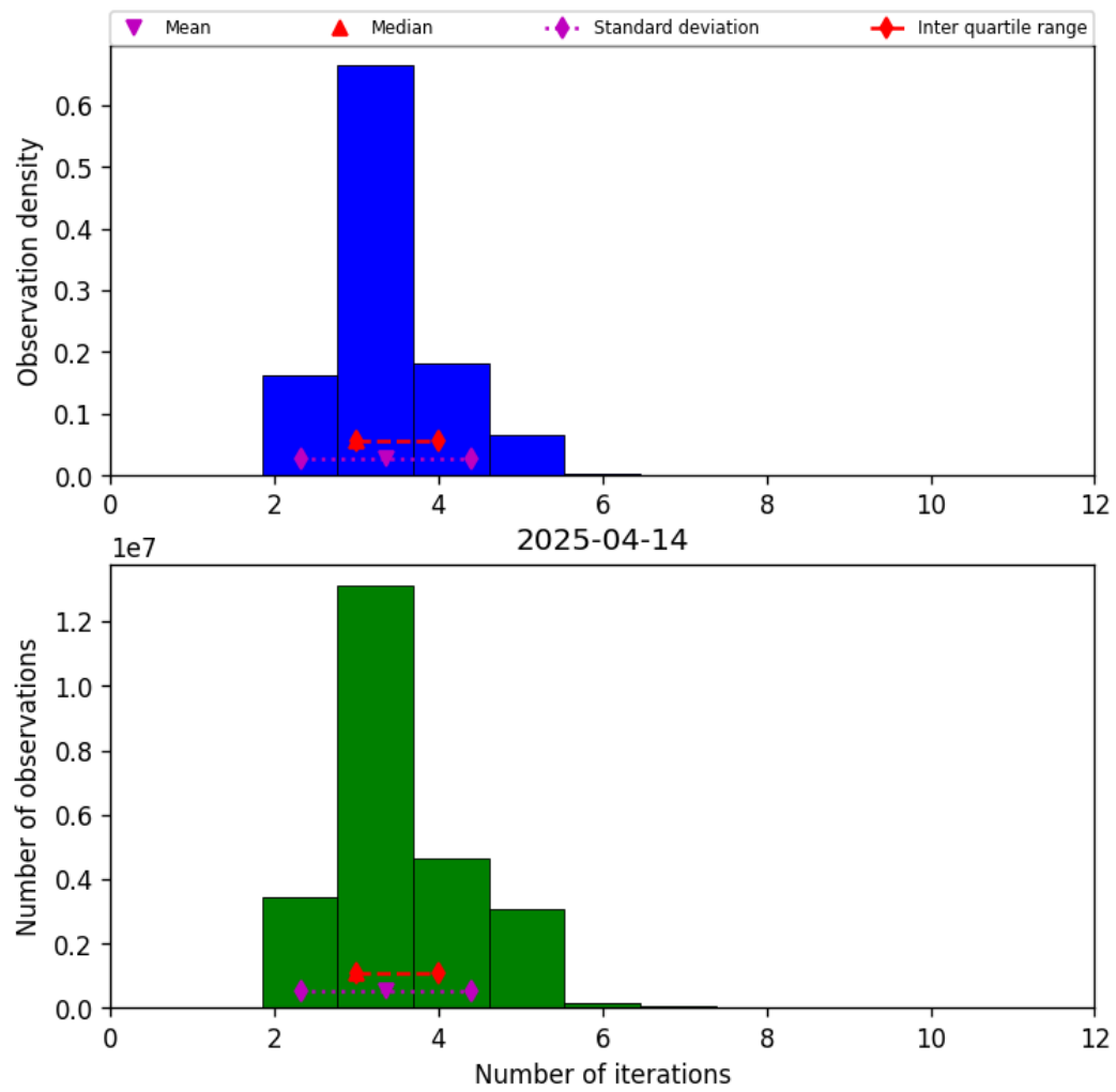
Figure 39: Histogram of “Number of iterations” for 2025-04-13 to 2025-04-15
