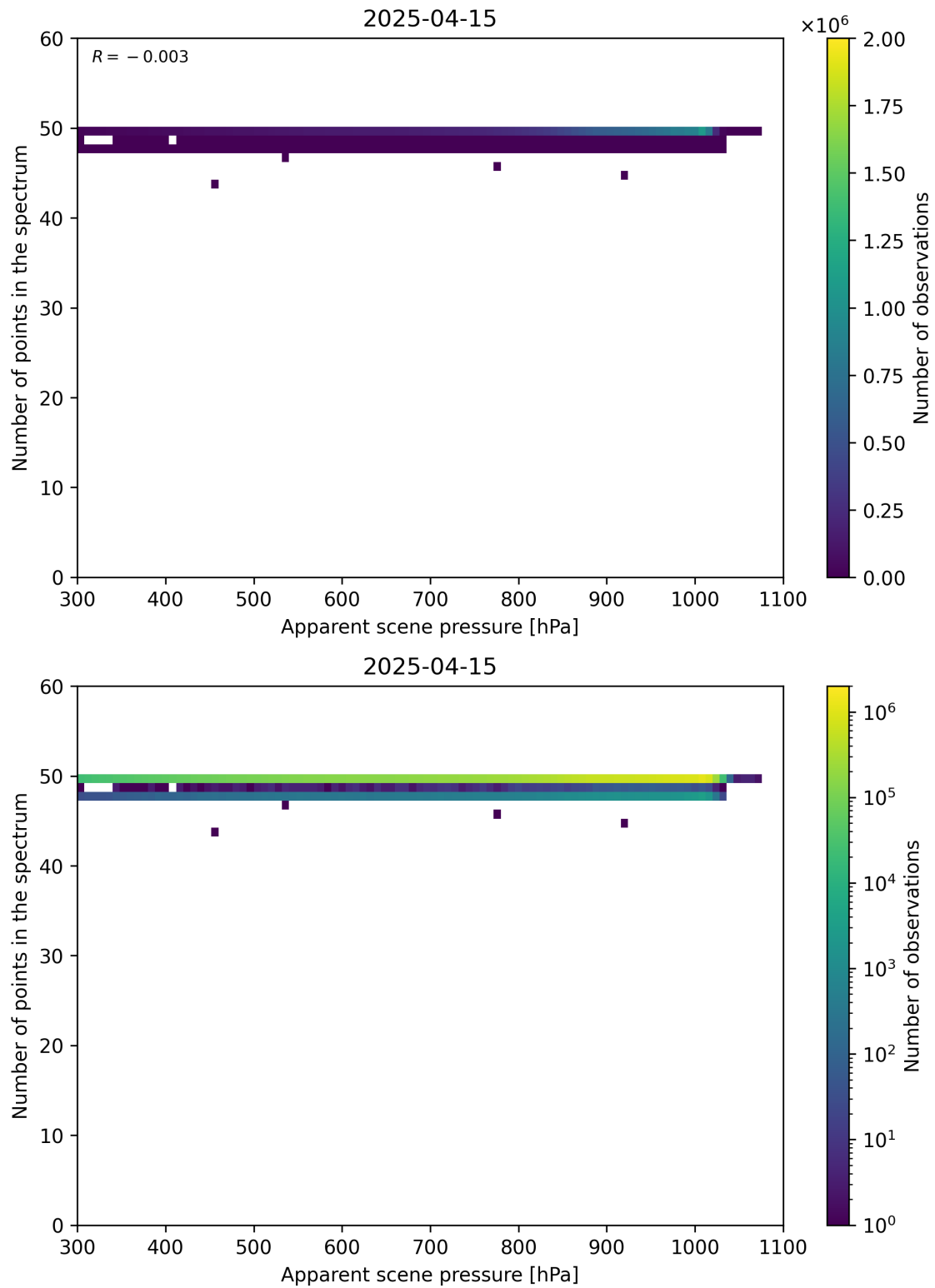
Figure 66: Scatter density plot of “Apparent scene pressure” against “Number of points in the spectrum” for 2025-04-14 to 2025-04-16.
