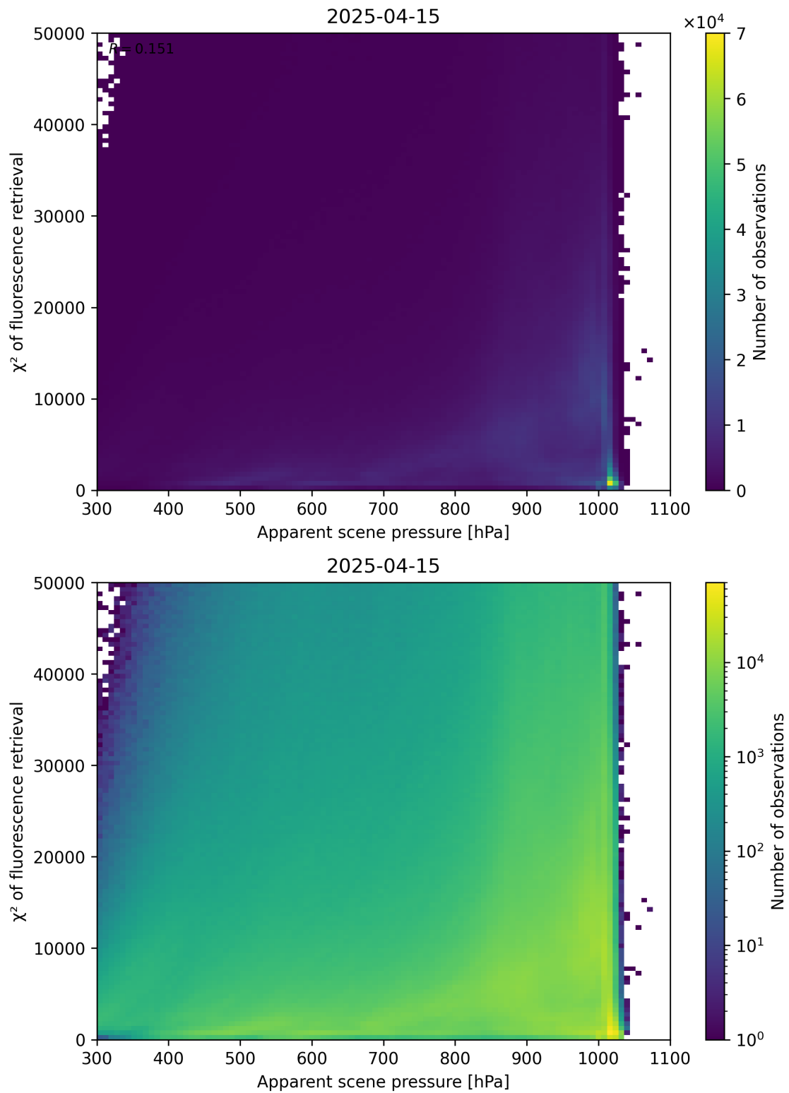
Figure 63: Scatter density plot of “Apparent scene pressure” against “ \chi^2 of fluorescence retrieval” for 2025-04-14 to 2025-04-16.
