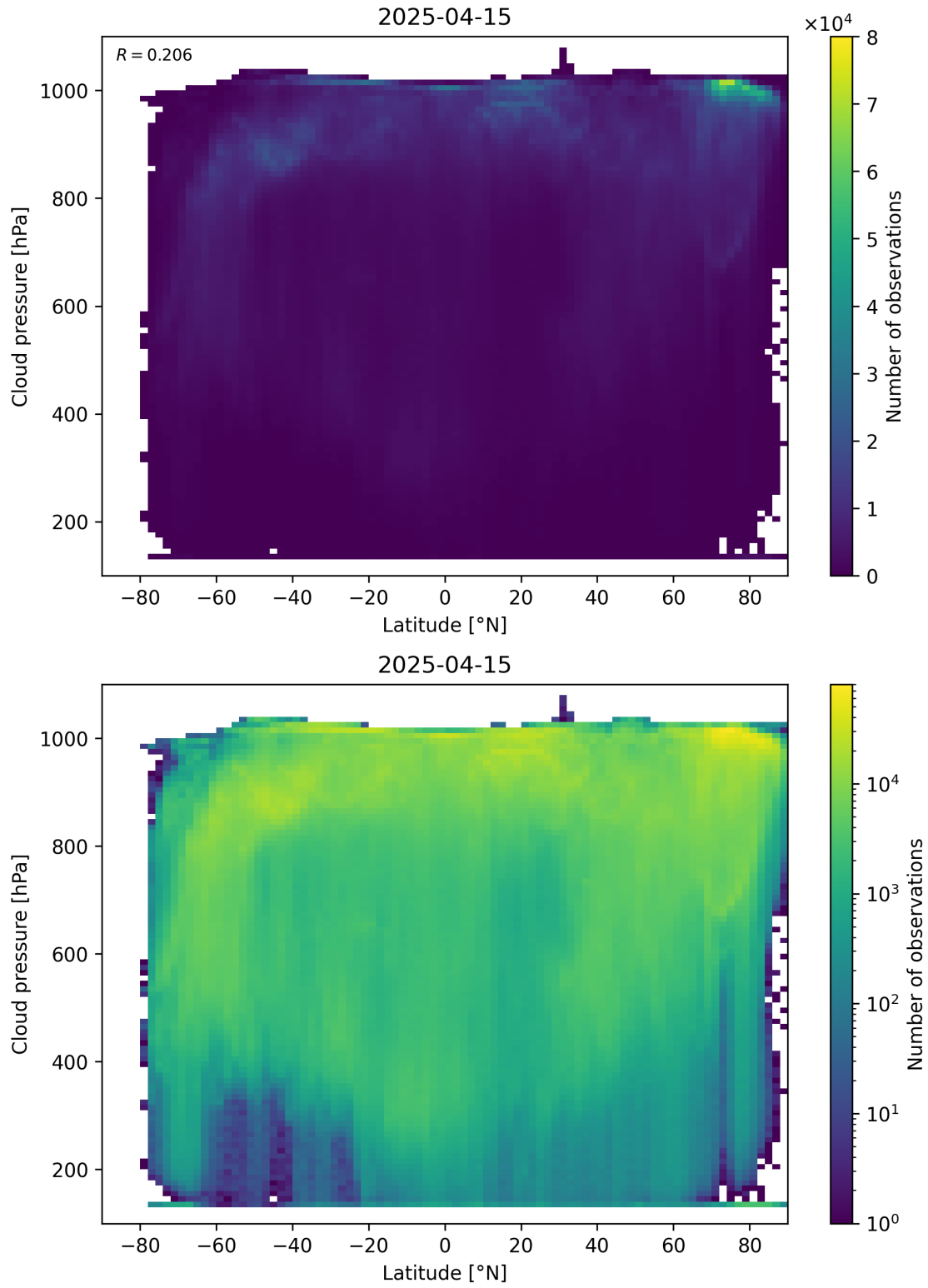
Figure 91: Scatter density plot of “Latitude” against “Cloud pressure” for 2025-04-14 to 2025-04-16.
