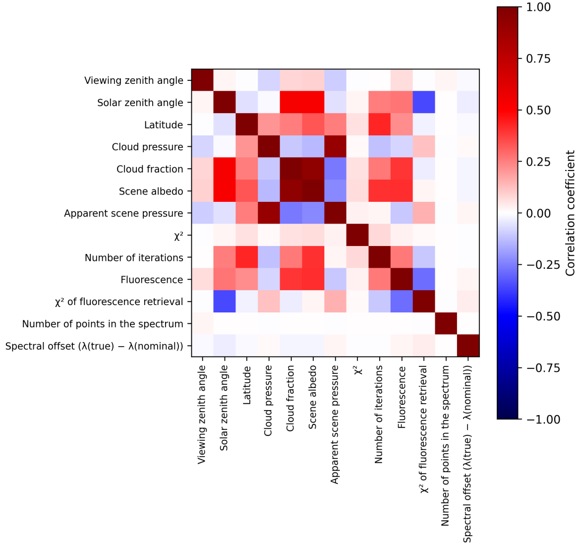
Figure 2: Map of correlation matrix for 2025-04-14 to 2025-04-16.
