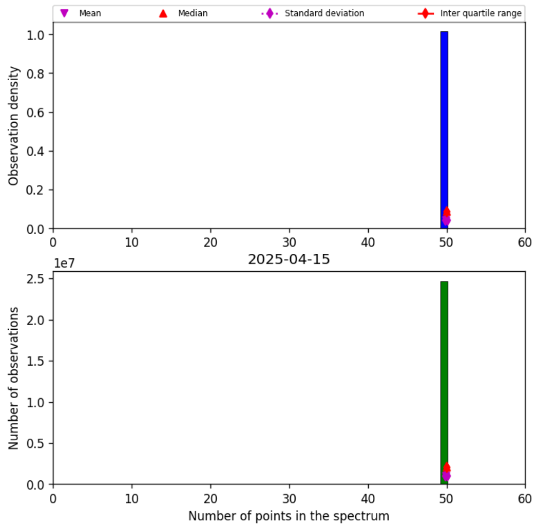
Figure 44: Histogram of “Number of points in the spectrum” for 2025-04-14 to 2025-04-16
