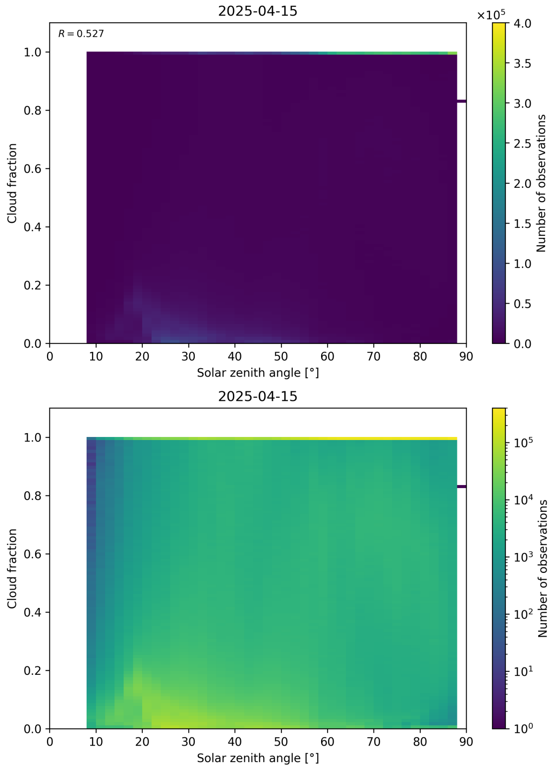
Figure 110: Scatter density plot of “Solar zenith angle” against “Cloud fraction” for 2025-04-14 to 2025-04-16.
