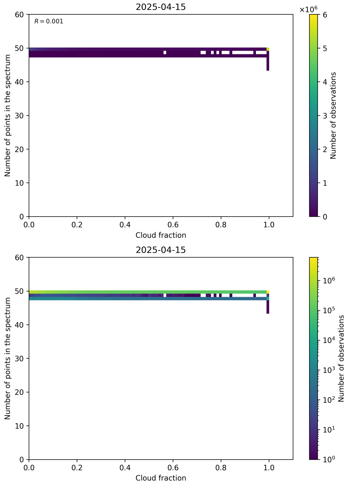
Figure 74: Scatter density plot of “Cloud fraction” against “Number of points in the spectrum” for 2025-04-14 to 2025-04-16.
