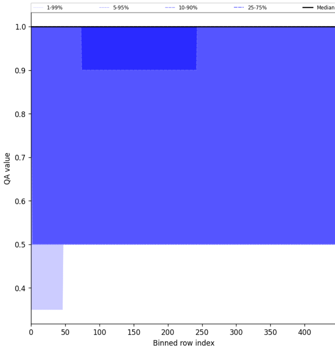
Figure 46: Along track statistics of “QA value” for 2025-04-14 to 2025-04-16
