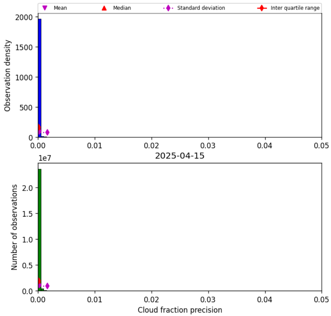
Figure 33: Histogram of “Cloud fraction precision” for 2025-04-14 to 2025-04-16
