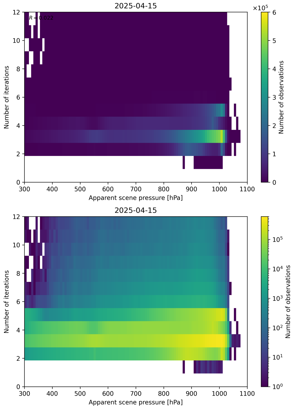
Figure 65: Scatter density plot of “Apparent scene pressure” against “Number of iterations” for 2025-04-14 to 2025-04-16.
