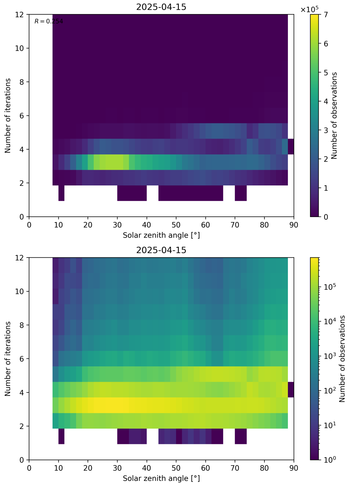
Figure 114: Scatter density plot of “Solar zenith angle” against “Number of iterations” for 2025-04-14 to 2025-04-16.
