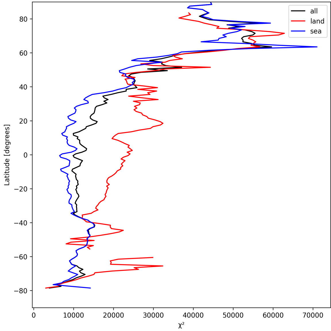
Figure 21: Zonal average of “ \chi^2 ” for 2025-04-14 to 2025-04-16.
