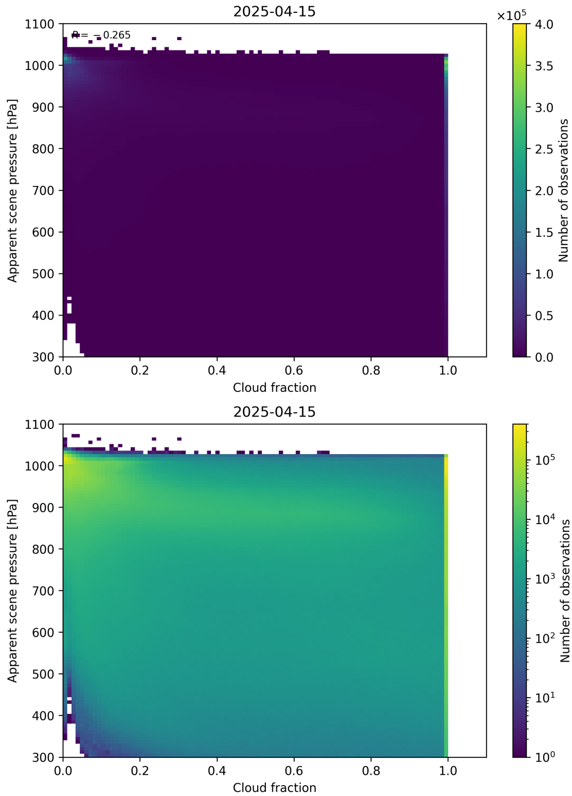
Figure 70: Scatter density plot of “Cloud fraction” against “Apparent scene pressure” for 2025-04-14 to 2025-04-16.
