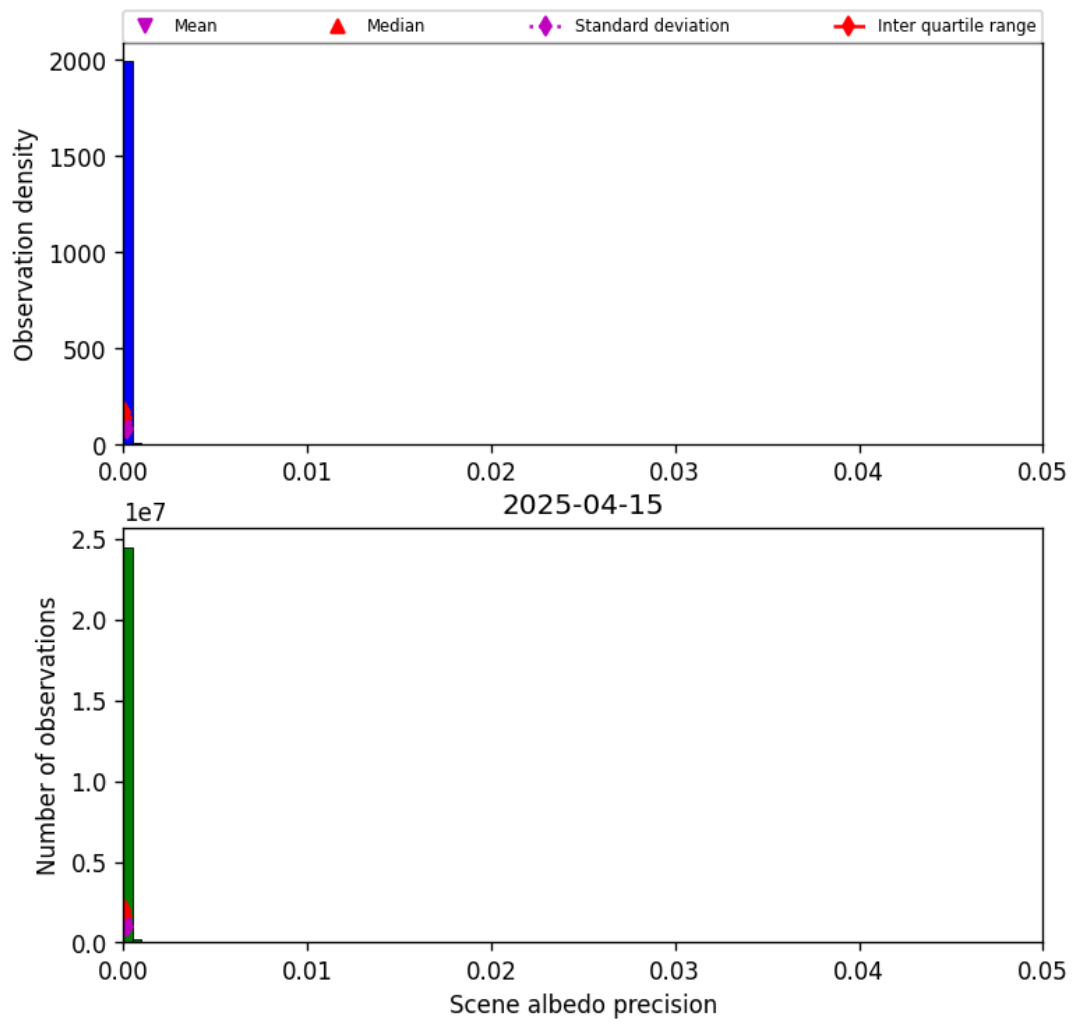
Figure 35: Histogram of “Scene albedo precision” for 2025-04-14 to 2025-04-16
