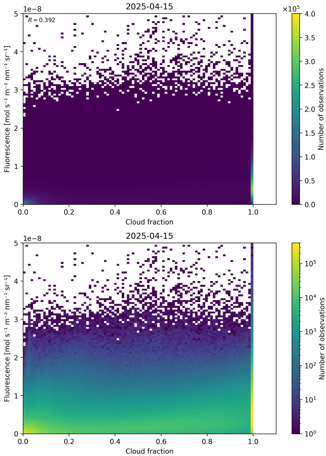
Figure 72: Scatter density plot of “Cloud fraction” against “Fluorescence” for 2025-04-14 to 2025-04-16.
