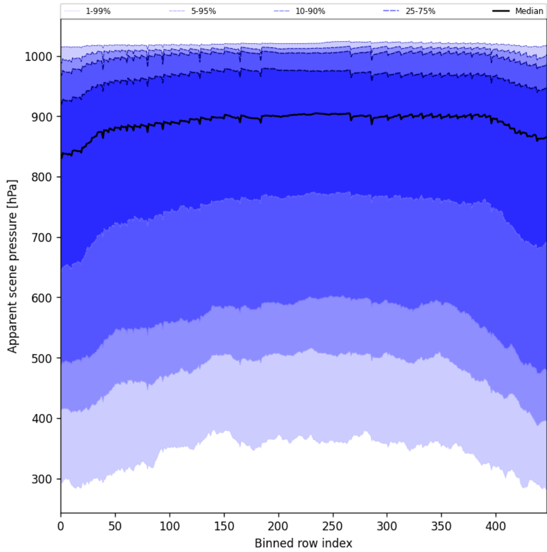
Figure 53: Along track statistics of “Apparent scene pressure” for 2025-04-14 to 2025-04-16
