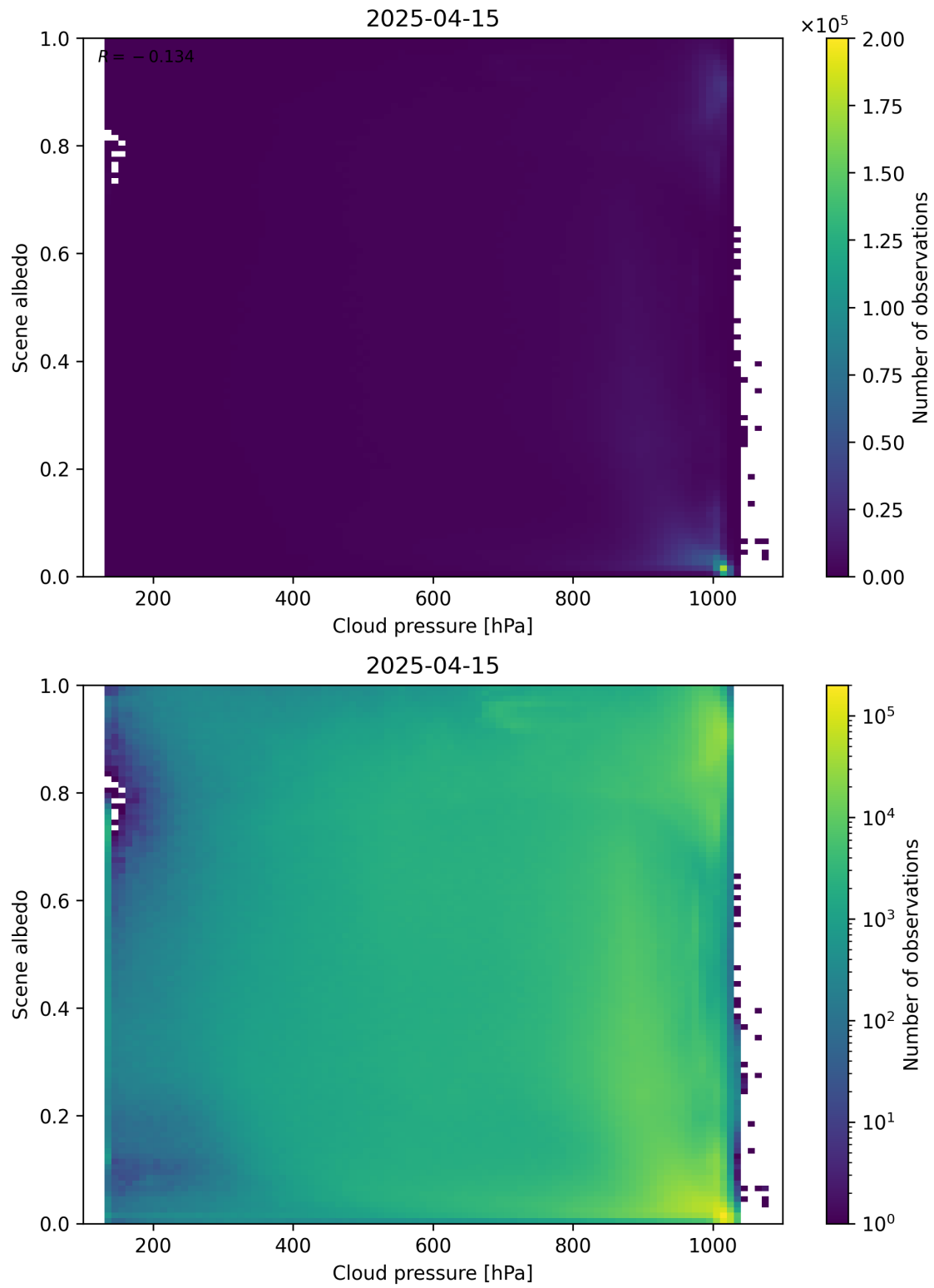
Figure 83: Scatter density plot of “Cloud pressure” against “Scene albedo” for 2025-04-14 to 2025-04-16.
