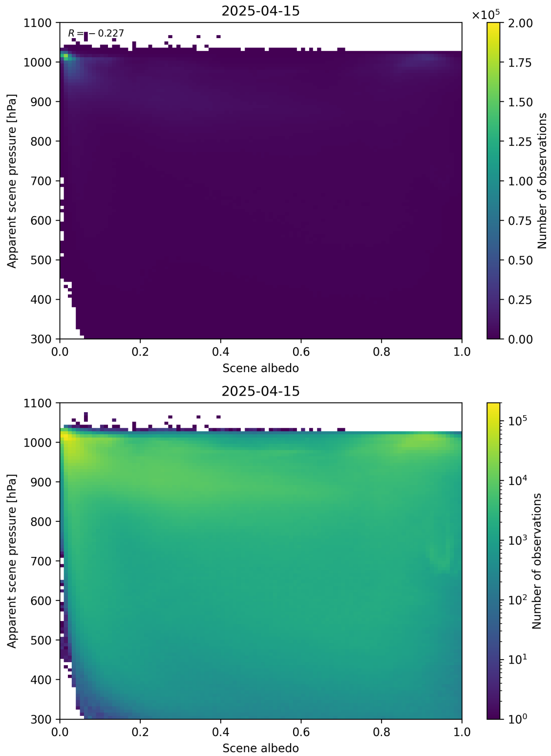
Figure 102: Scatter density plot of “Scene albedo” against “Apparent scene pressure” for 2025-04-14 to 2025-04-16.
