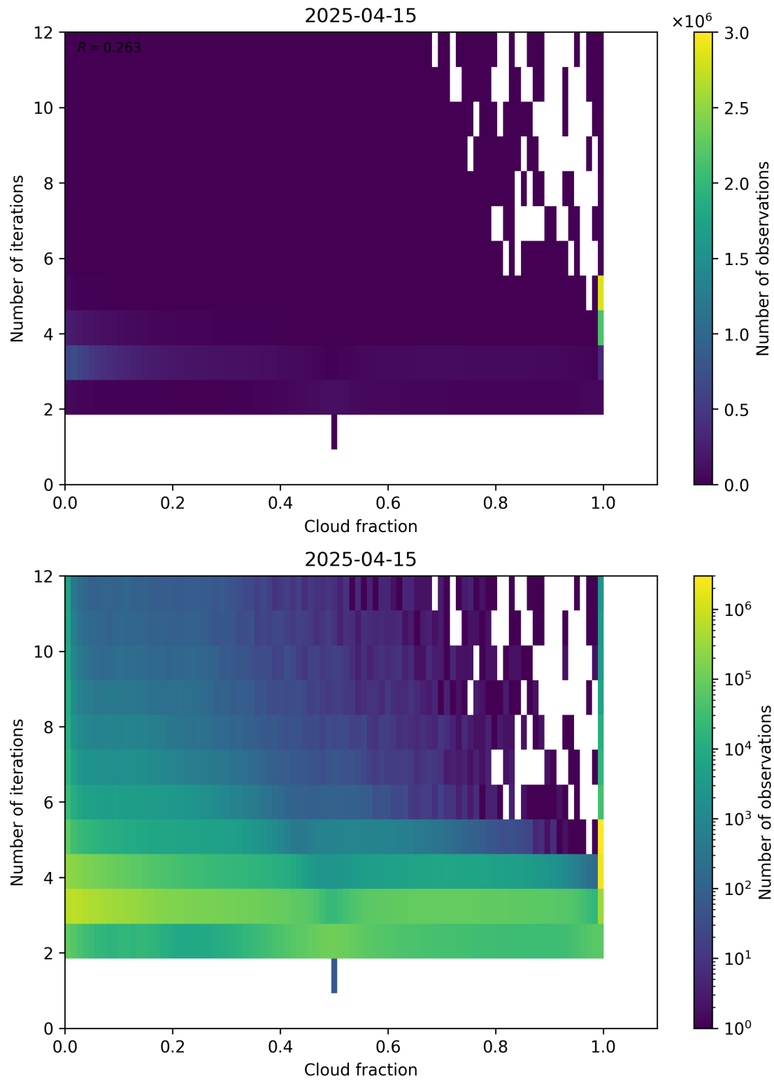
Figure 73: Scatter density plot of “Cloud fraction” against “Number of iterations” for 2025-04-14 to 2025-04-16.
