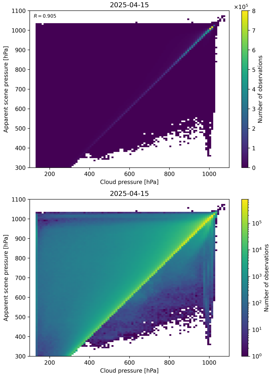
Figure 77: Scatter density plot of “Cloud pressure” against “Apparent scene pressure” for 2025-04-14 to 2025-04-16.
