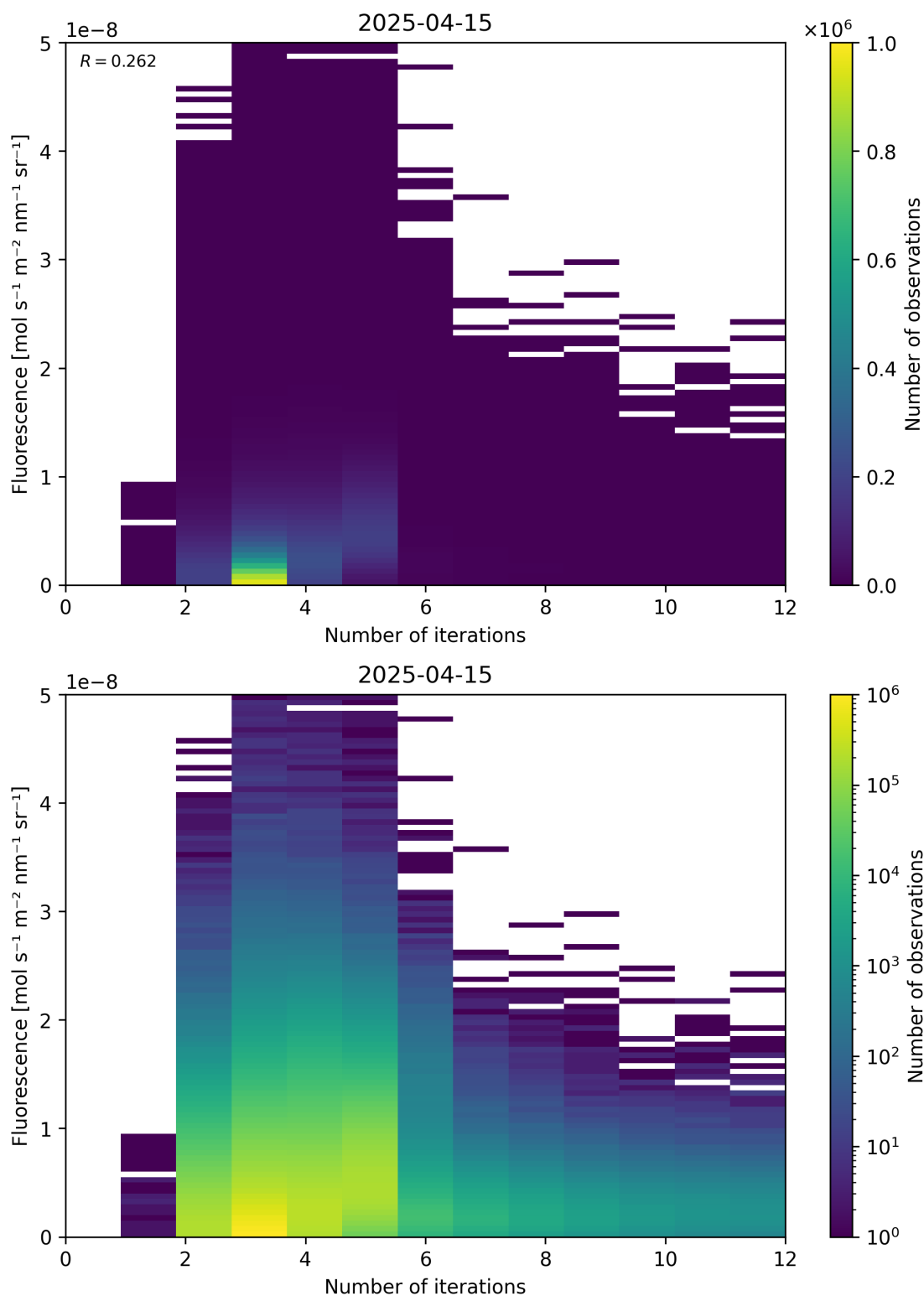
Figure 98: Scatter density plot of “Number of iterations” against “Fluorescence” for 2025-04-14 to 2025-04-16.
