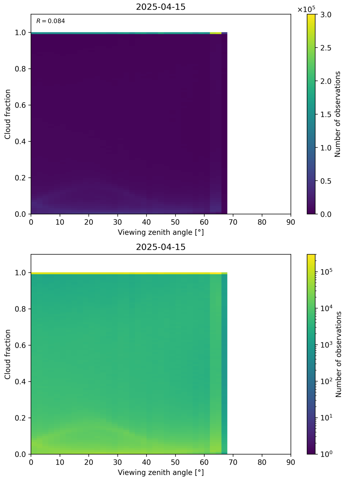
Figure 120: Scatter density plot of “Viewing zenith angle” against “Cloud fraction” for 2025-04-14 to 2025-04-16.
