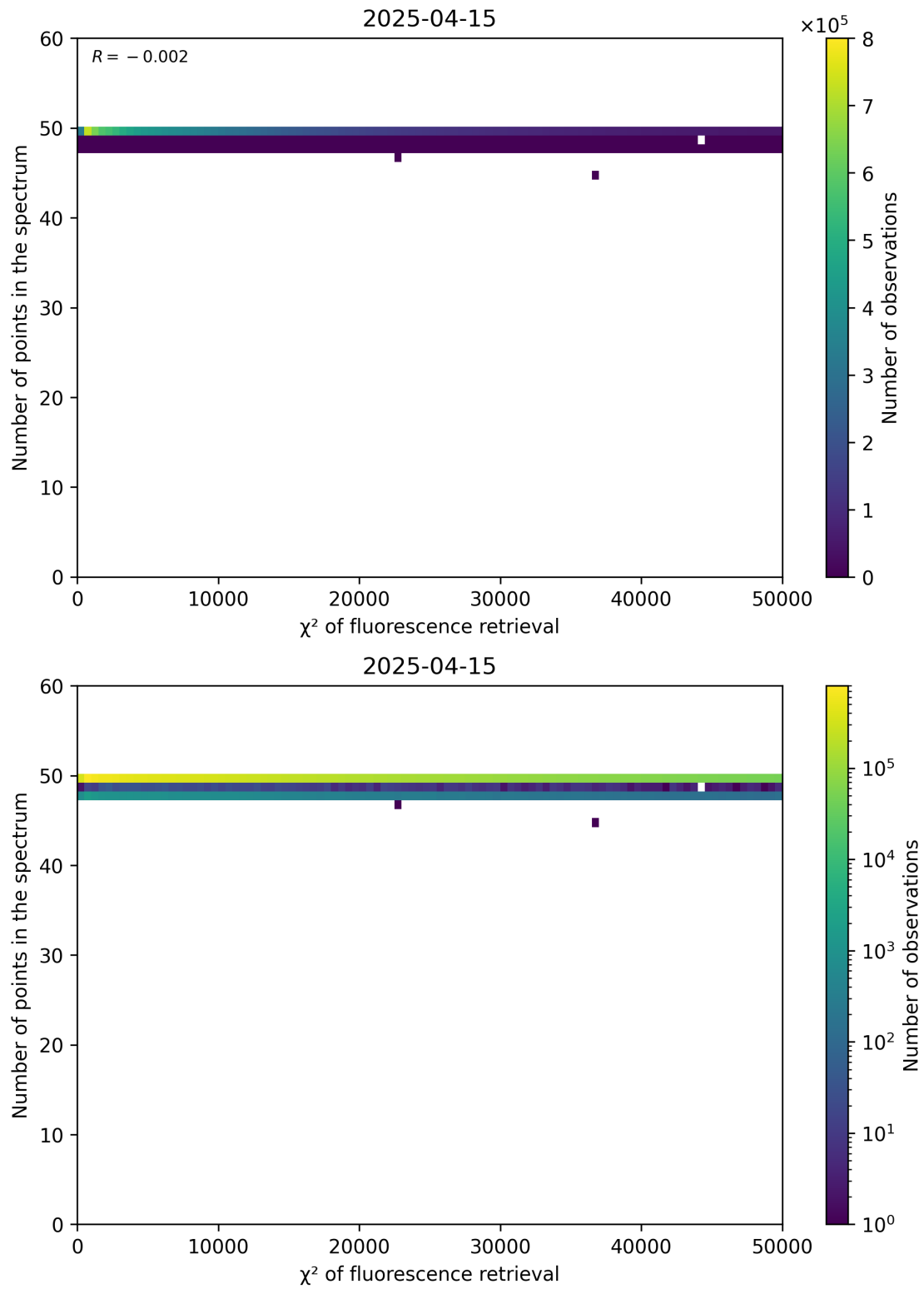
Figure 68: Scatter density plot of “ \chi^2 of fluorescence retrieval” against “Number of points in the spectrum” for 2025-04-14 to 2025-04-16.
