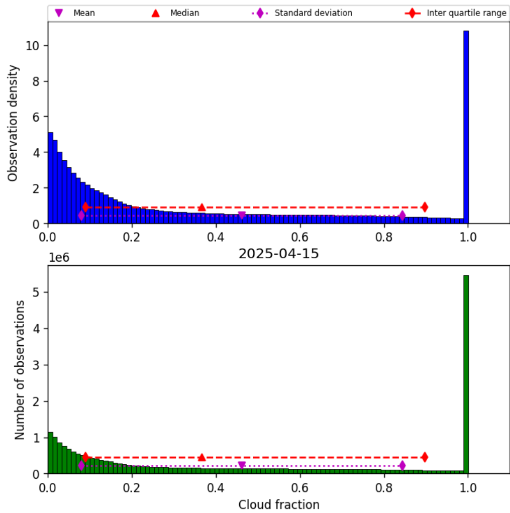
Figure 32: Histogram of “Cloud fraction” for 2025-04-14 to 2025-04-16
