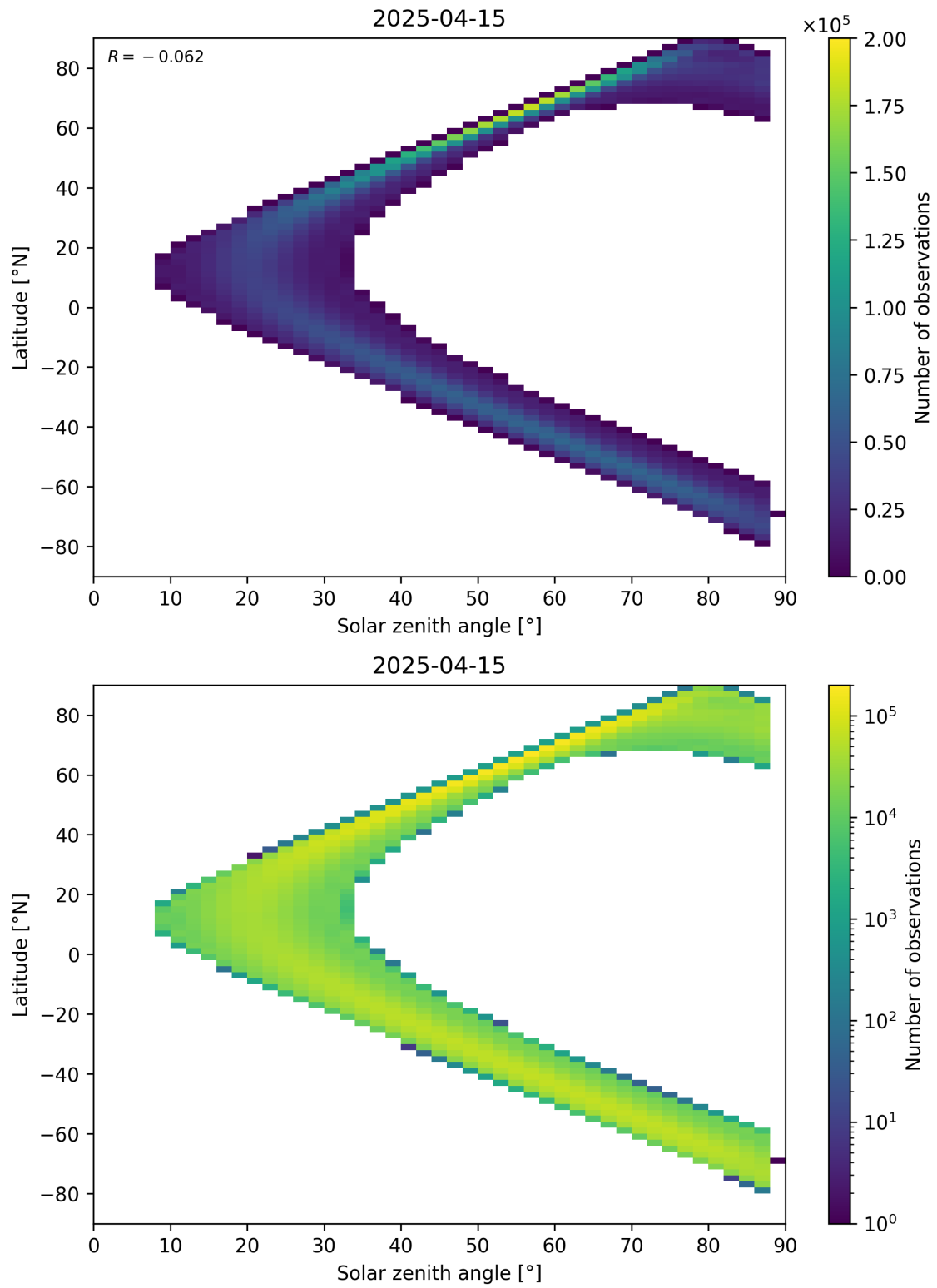
Figure 113: Scatter density plot of “Solar zenith angle” against “Latitude” for 2025-04-14 to 2025-04-16.
