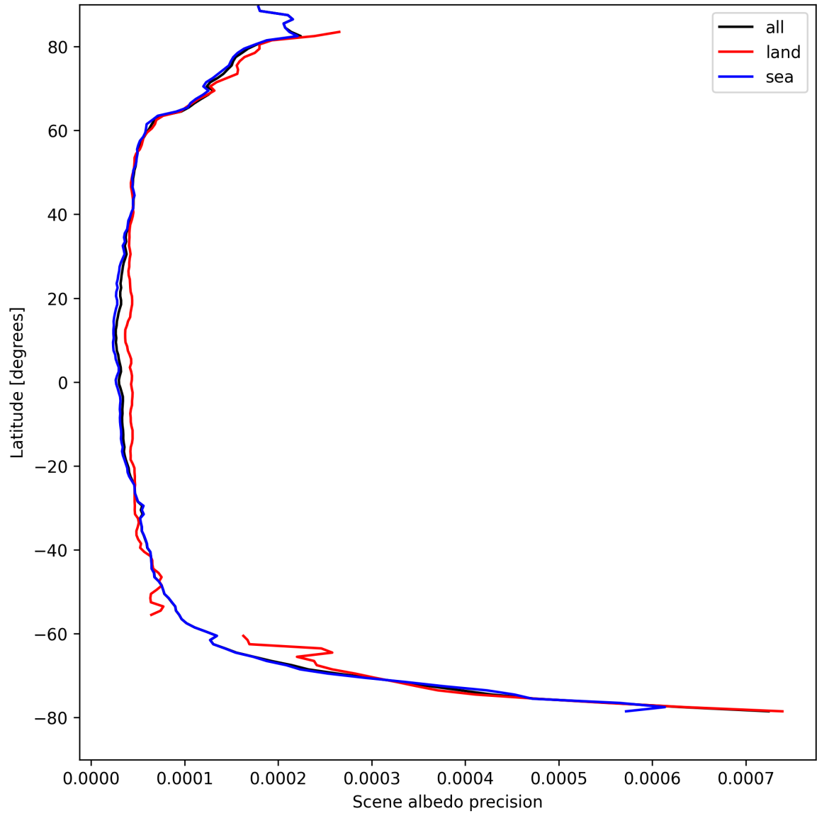
Figure 18: Zonal average of “Scene albedo precision” for 2025-04-14 to 2025-04-16.
