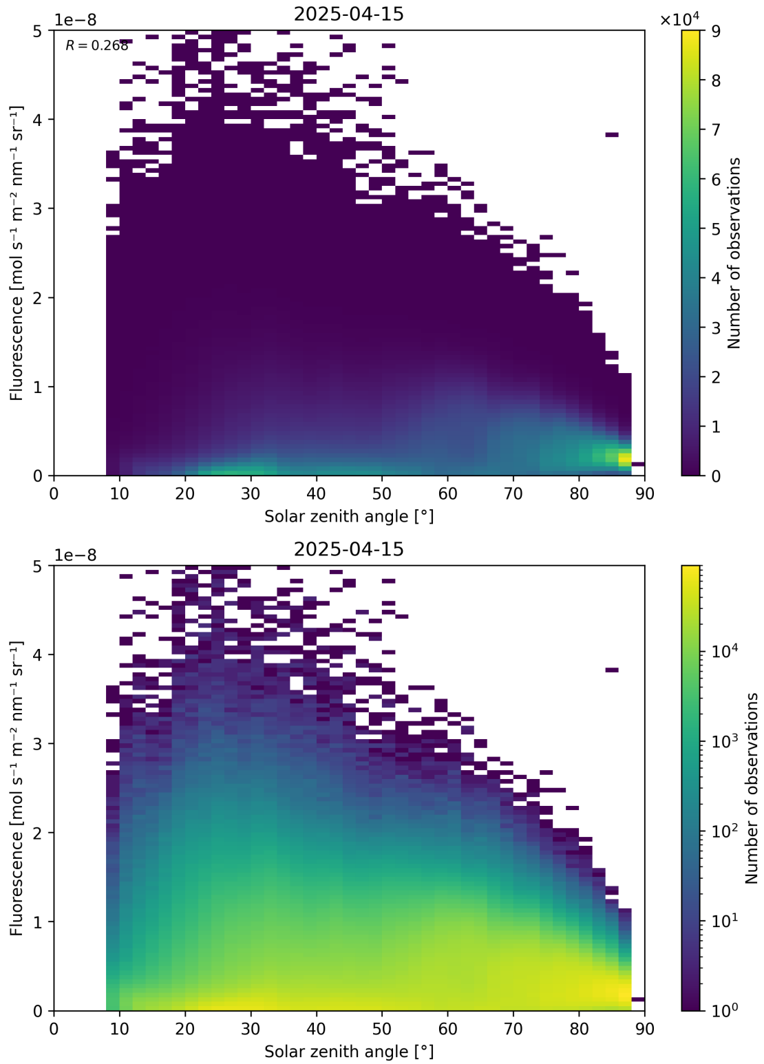
Figure 112: Scatter density plot of “Solar zenith angle” against “Fluorescence” for 2025-04-14 to 2025-04-16.
