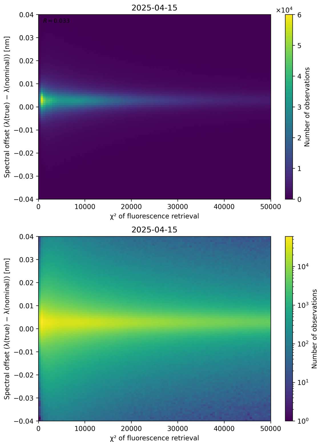
Figure 69: Scatter density plot of “ \chi^2 of fluorescence retrieval” against “Spectral offset ( \lambda_{\text{true}} - \lambda_{\text{nominal}} )” for 2025-04-14 to 2025-04-16.
