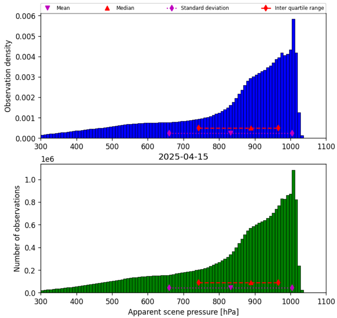
Figure 36: Histogram of “Apparent scene pressure” for 2025-04-14 to 2025-04-16
