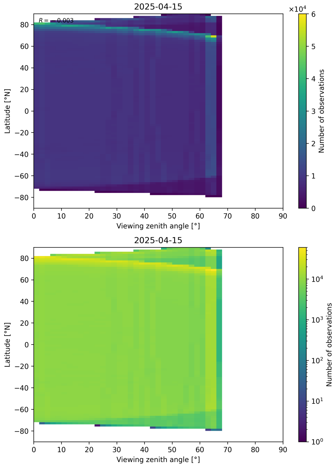
Figure 123: Scatter density plot of “Viewing zenith angle” against “Latitude” for 2025-04-14 to 2025-04-16.
