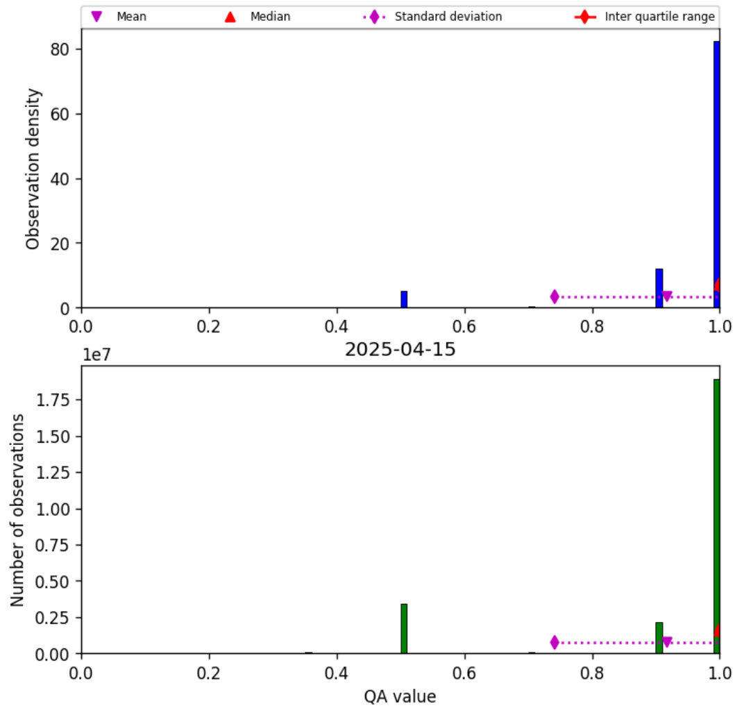
Figure 29: Histogram of “QA value” for 2025-04-14 to 2025-04-16
