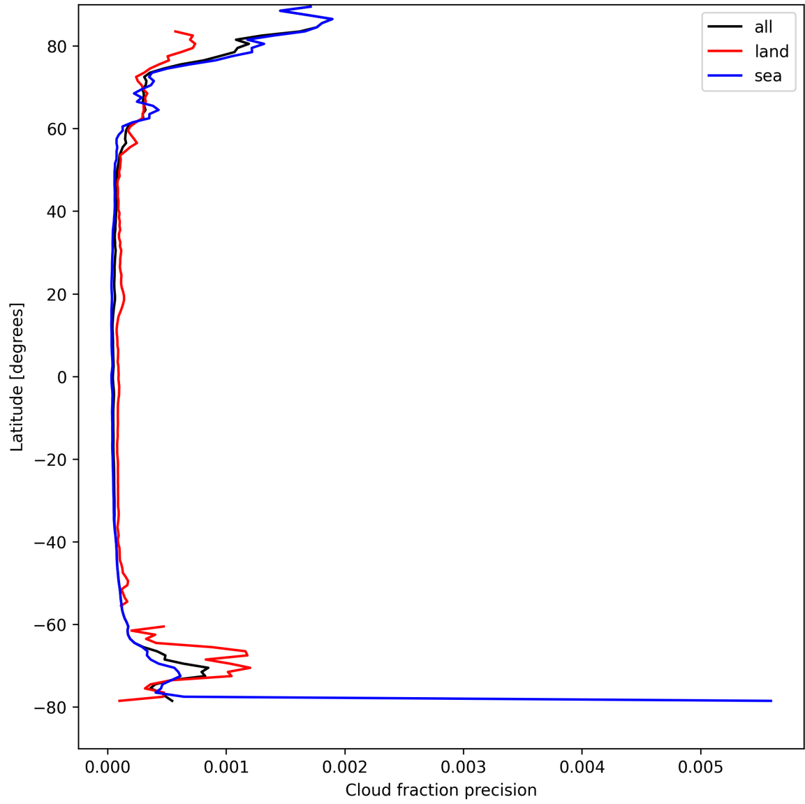
Figure 16: Zonal average of “Cloud fraction precision” for 2025-04-14 to 2025-04-16.
