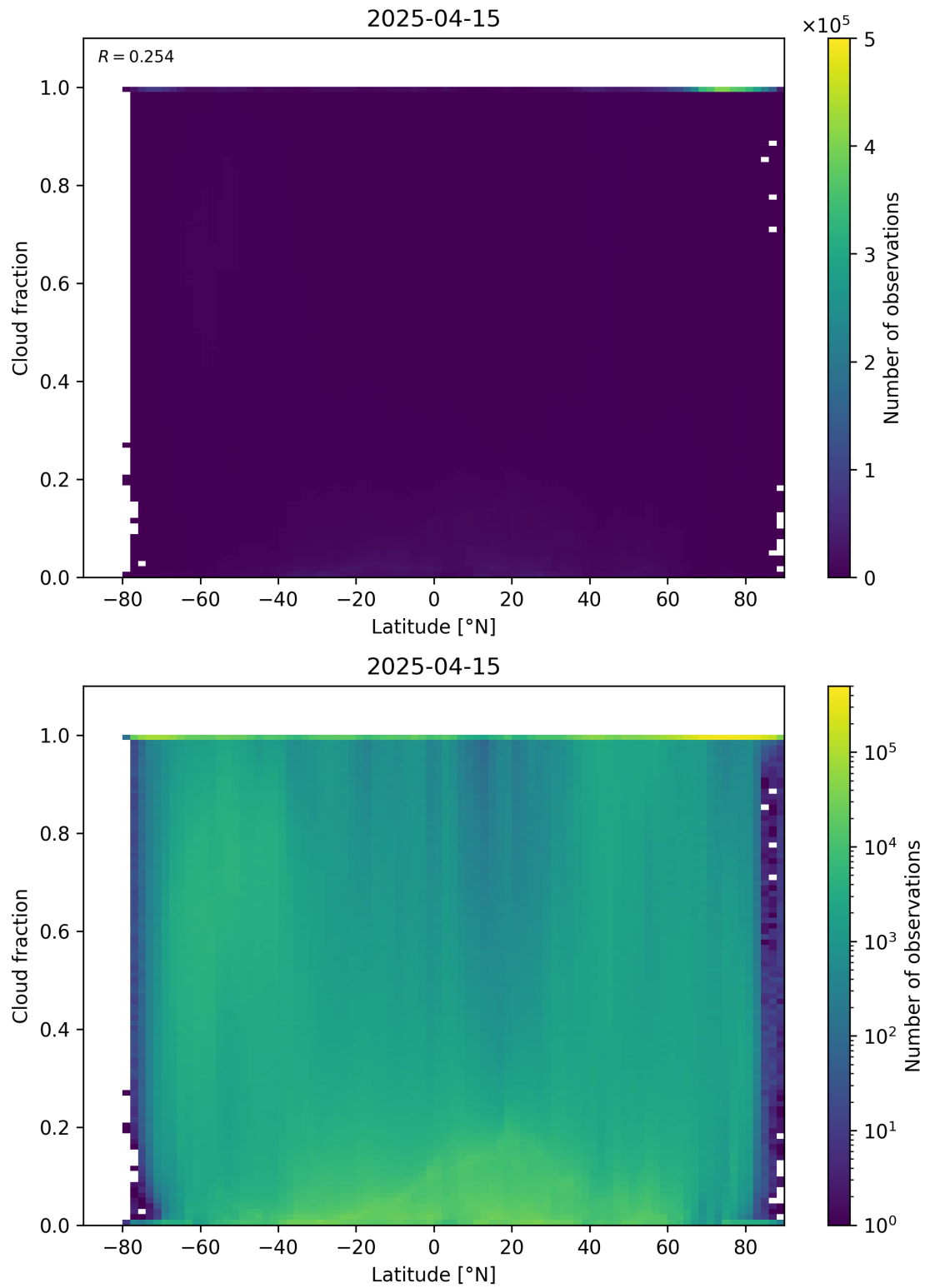
Figure 90: Scatter density plot of “Latitude” against “Cloud fraction” for 2025-04-14 to 2025-04-16.
