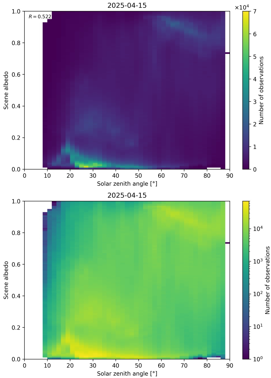
Figure 116: Scatter density plot of “Solar zenith angle” against “Scene albedo” for 2025-04-14 to 2025-04-16.
