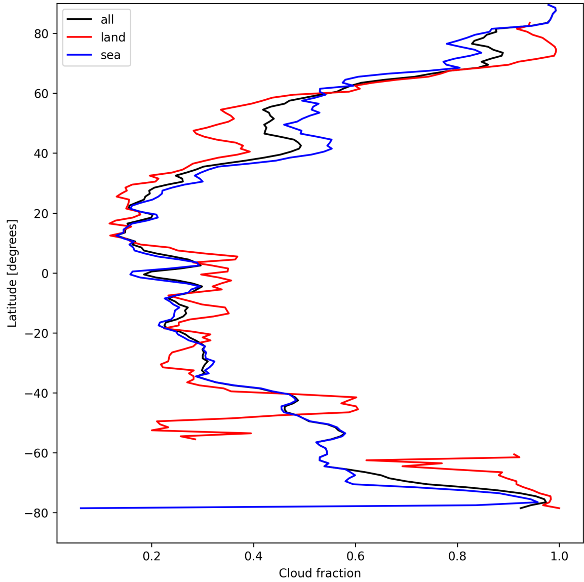
Figure 15: Zonal average of “Cloud fraction” for 2025-04-14 to 2025-04-16.
