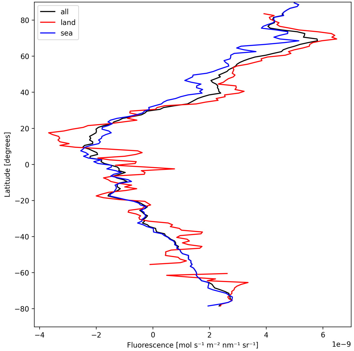
Figure 23: Zonal average of “Fluorescence” for 2025-04-14 to 2025-04-16.
