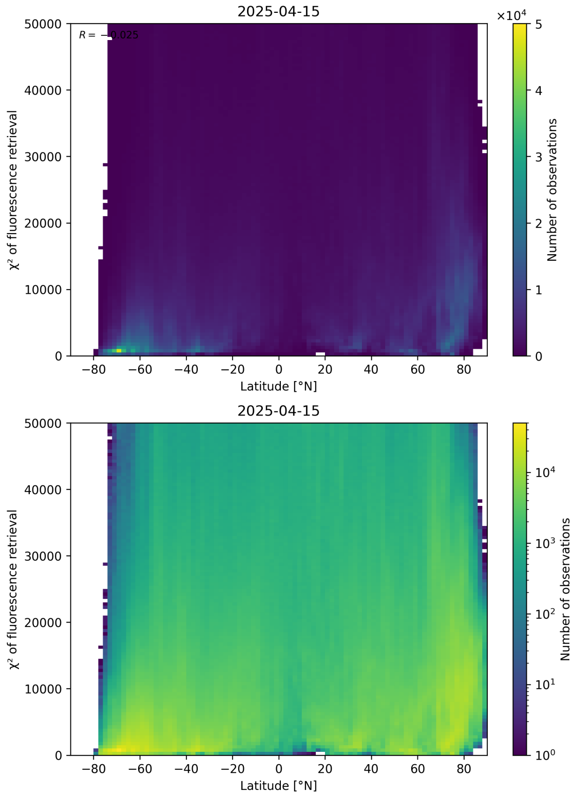
Figure 89: Scatter density plot of “Latitude” against “ \chi^2 of fluorescence retrieval” for 2025-04-14 to 2025-04-16.
