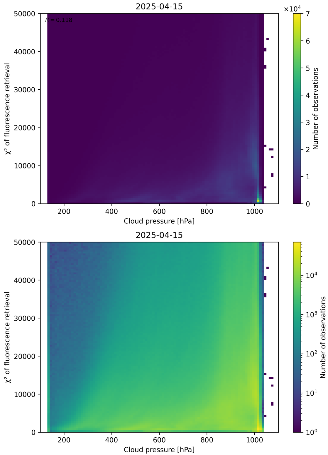
Figure 78: Scatter density plot of “Cloud pressure” against “ \chi^2 of fluorescence retrieval” for 2025-04-14 to 2025-04-16.
