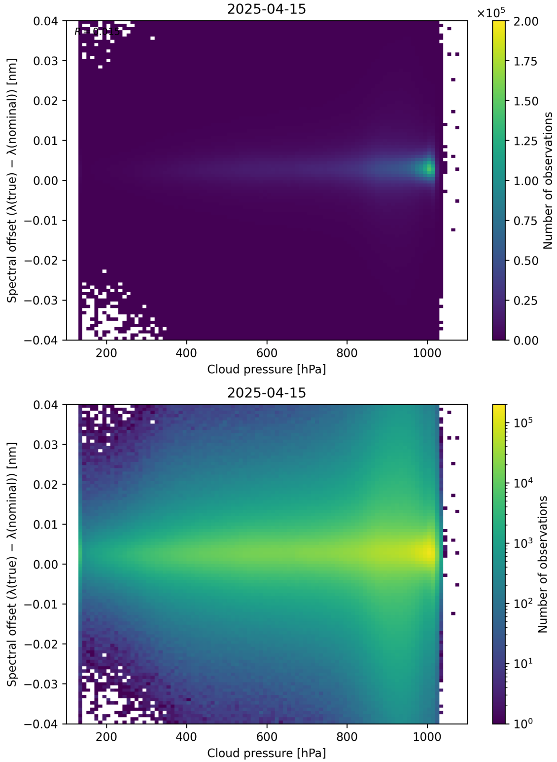
Figure 84: Scatter density plot of “Cloud pressure” against “Spectral offset ( \lambda_{\text{true}} - \lambda_{\text{nominal}} )” for 2025-04-14 to 2025-04-16.
