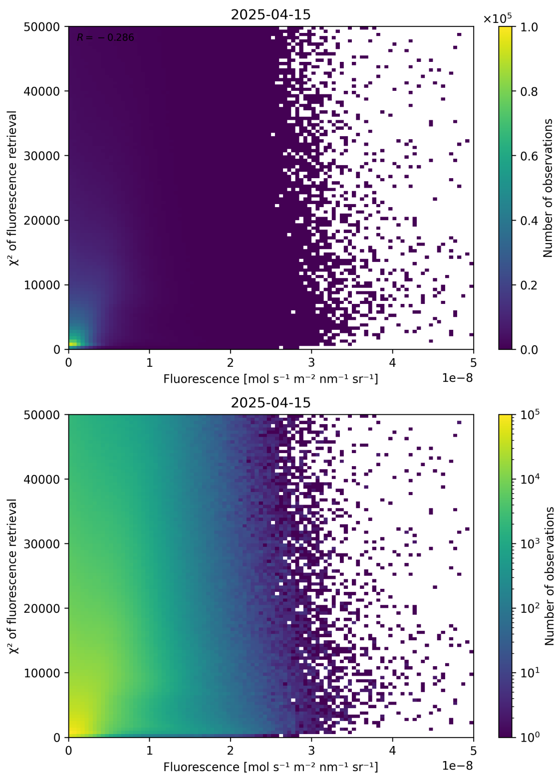
Figure 85: Scatter density plot of “Fluorescence” against “ \chi^2 of fluorescence retrieval” for 2025-04-14 to 2025-04-16.
