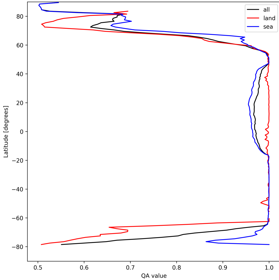
Figure 12: Zonal average of “QA value” for 2025-04-14 to 2025-04-16.
