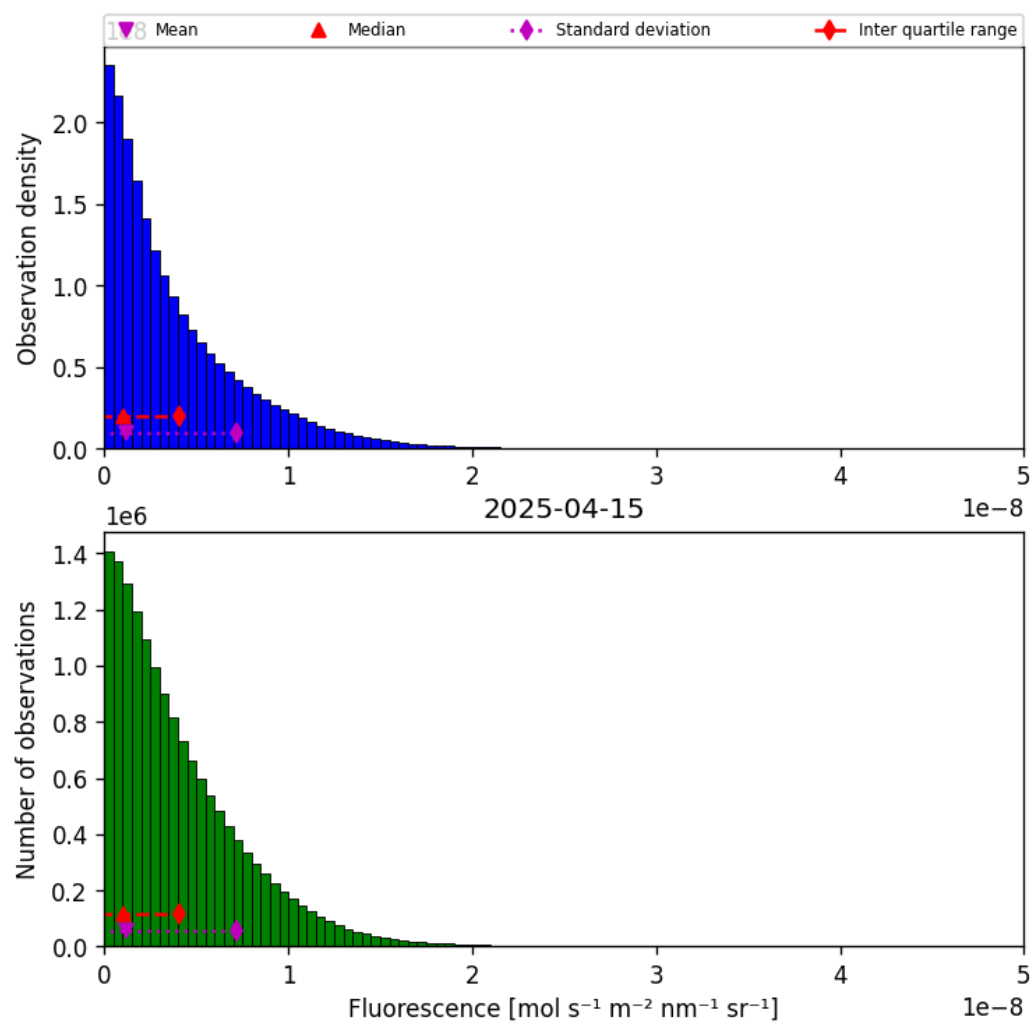
Figure 40: Histogram of “Fluorescence” for 2025-04-14 to 2025-04-16
