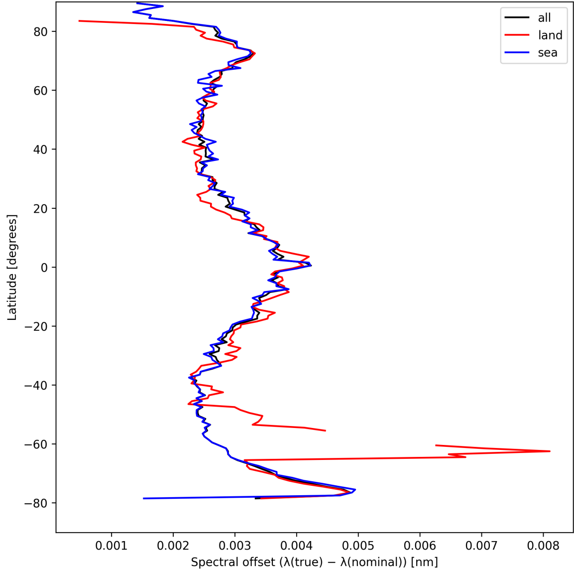
Figure 28: Zonal average of “Spectral offset ( \lambda_{\text{true}} - \lambda_{\text{nominal}} )” for 2025-04-14 to 2025-04-16.
