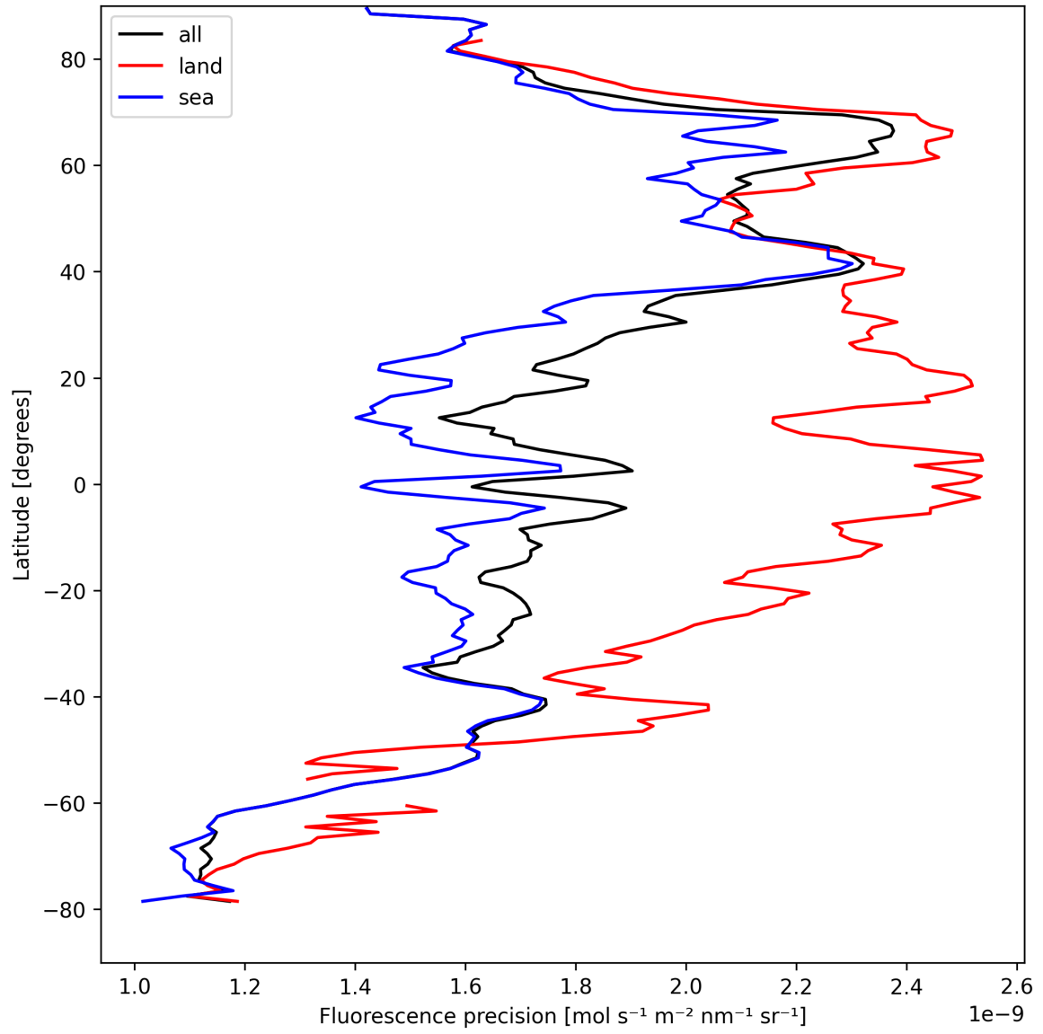
Figure 24: Zonal average of “Fluorescence precision” for 2025-04-14 to 2025-04-16.
