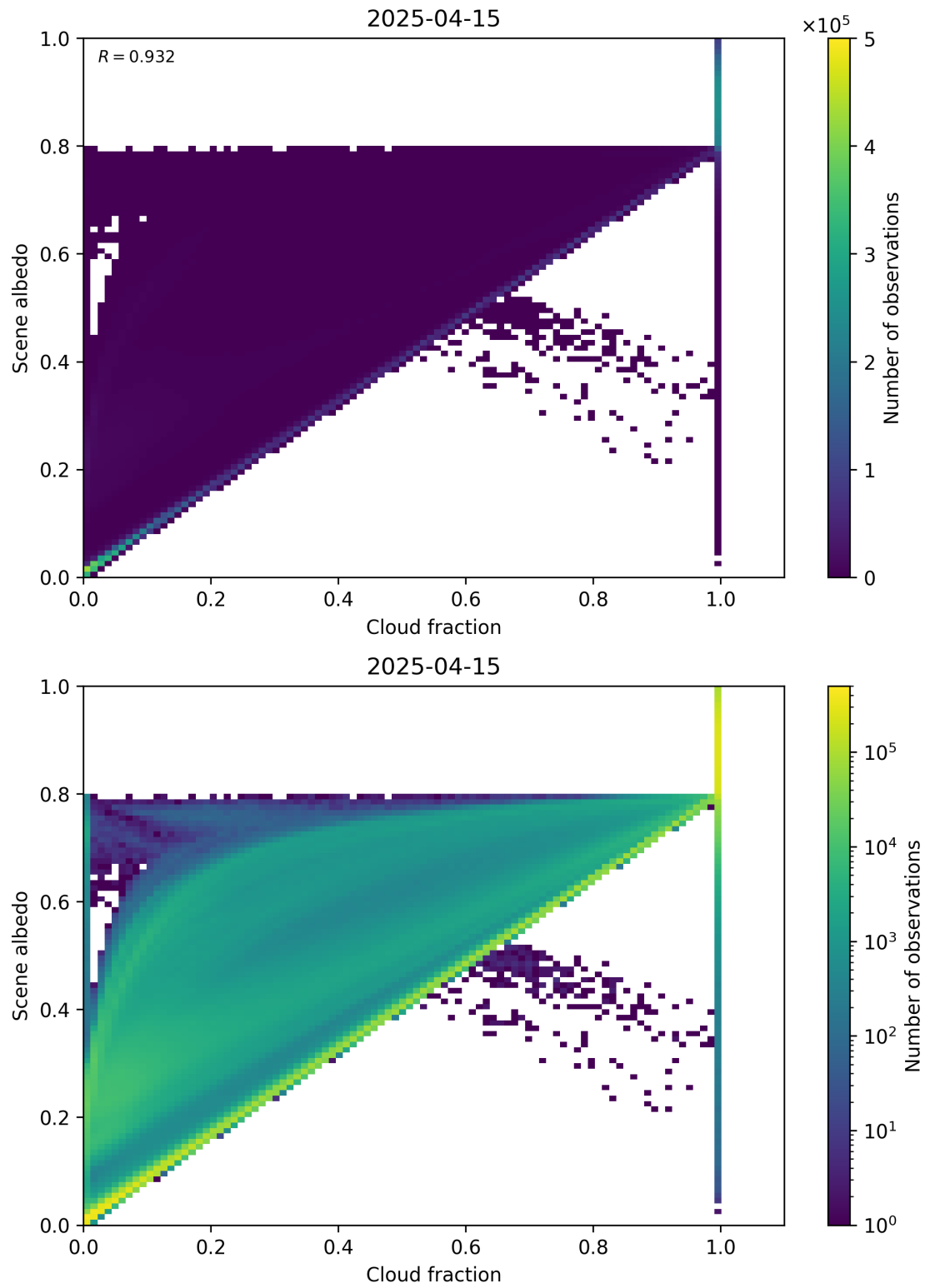
Figure 75: Scatter density plot of “Cloud fraction” against “Scene albedo” for 2025-04-14 to 2025-04-16.
