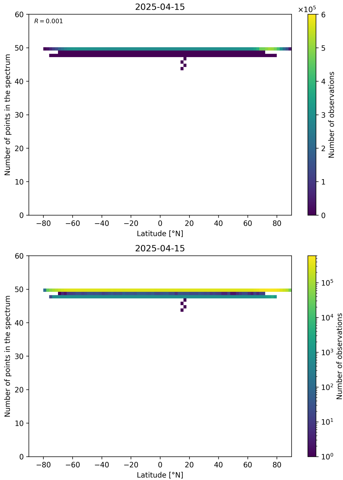
Figure 94: Scatter density plot of “Latitude” against “Number of points in the spectrum” for 2025-04-14 to 2025-04-16.
