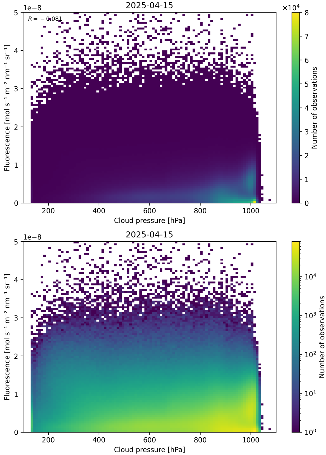
Figure 80: Scatter density plot of “Cloud pressure” against “Fluorescence” for 2025-04-14 to 2025-04-16.
