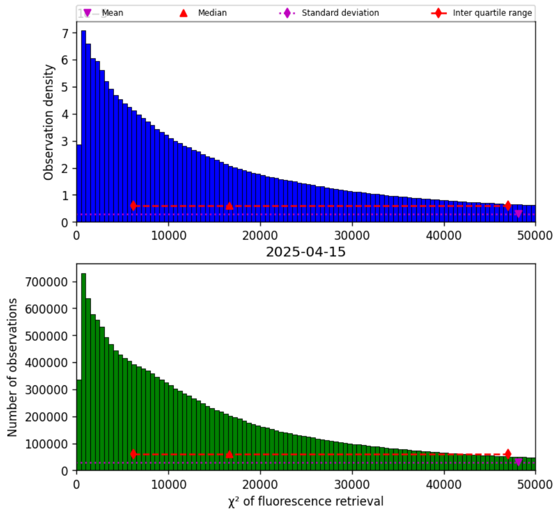
Figure 42: Histogram of “ \chi^2 of fluorescence retrieval” for 2025-04-14 to 2025-04-16
