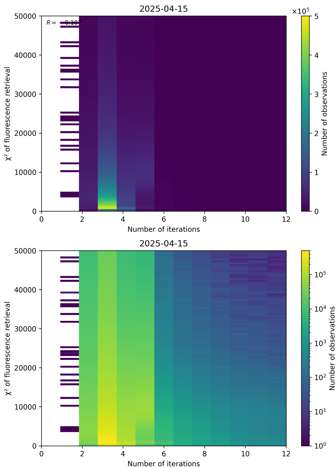
Figure 97: Scatter density plot of “Number of iterations” against “ \chi^2 of fluorescence retrieval” for 2025-04-14 to 2025-04-16.
