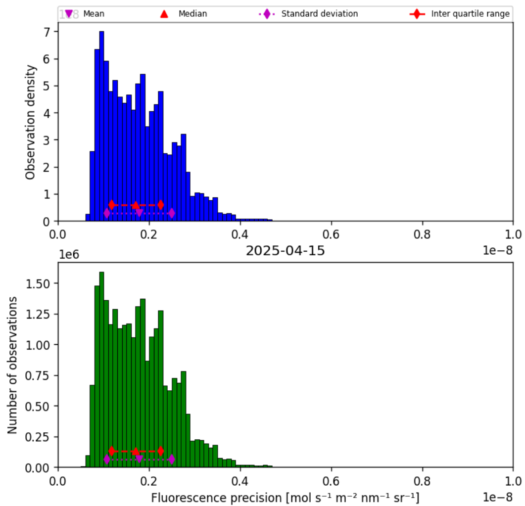
Figure 41: Histogram of “Fluorescence precision” for 2025-04-14 to 2025-04-16
