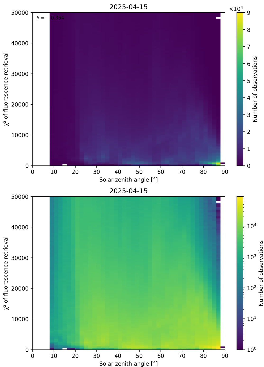
Figure 109: Scatter density plot of “Solar zenith angle” against “ \chi^2 of fluorescence retrieval” for 2025-04-14 to 2025-04-16.
