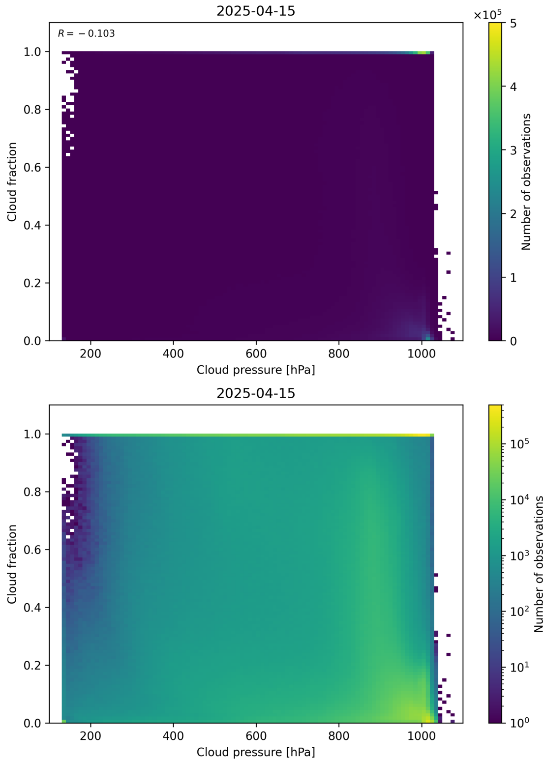
Figure 79: Scatter density plot of “Cloud pressure” against “Cloud fraction” for 2025-04-14 to 2025-04-16.
