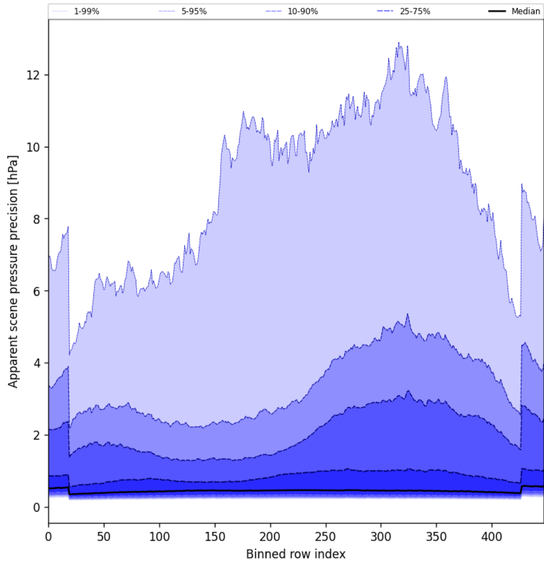
Figure 54: Along track statistics of “Apparent scene pressure precision” for 2025-04-14 to 2025-04-16
