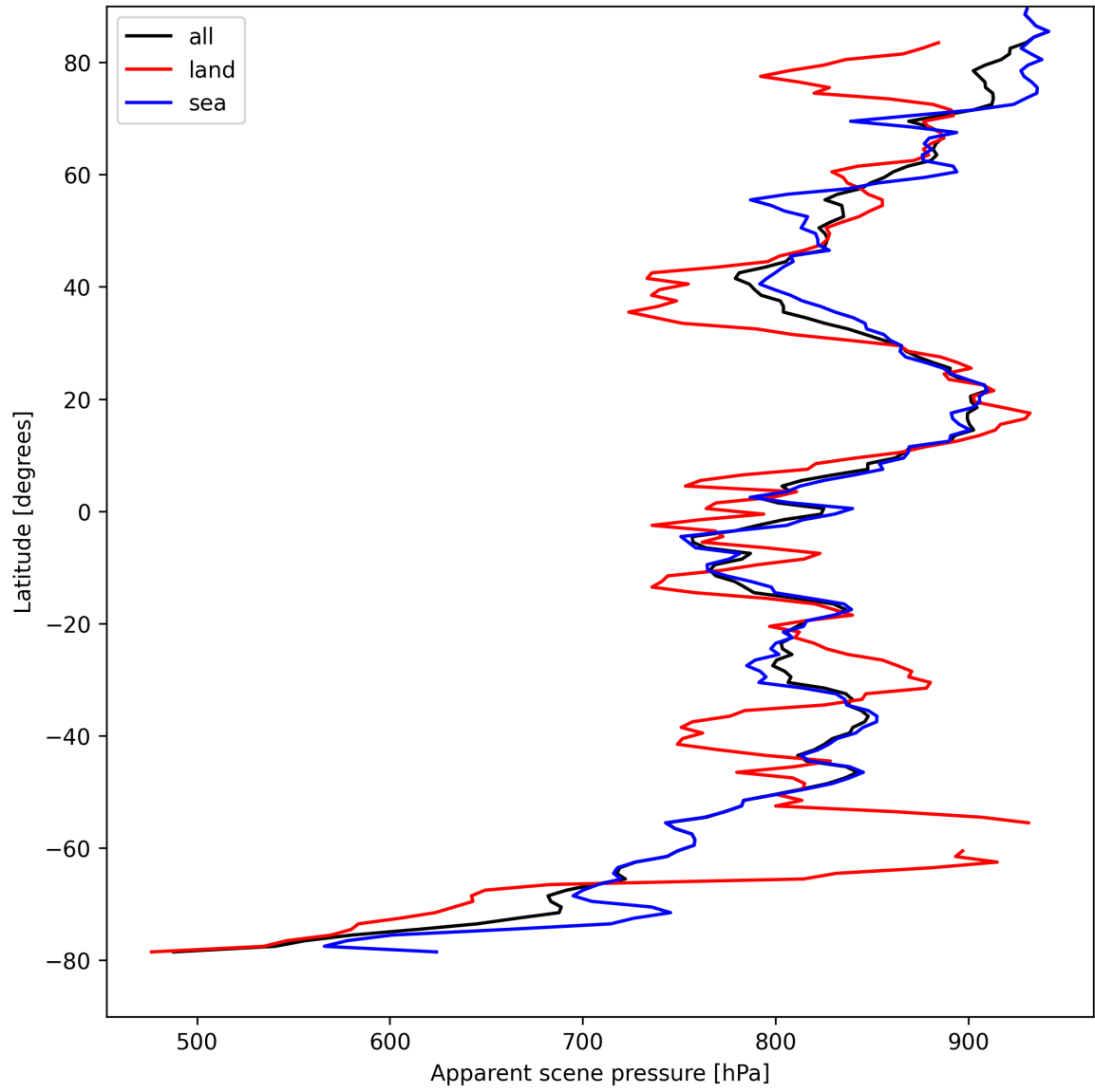
Figure 19: Zonal average of “Apparent scene pressure” for 2025-04-14 to 2025-04-16.
