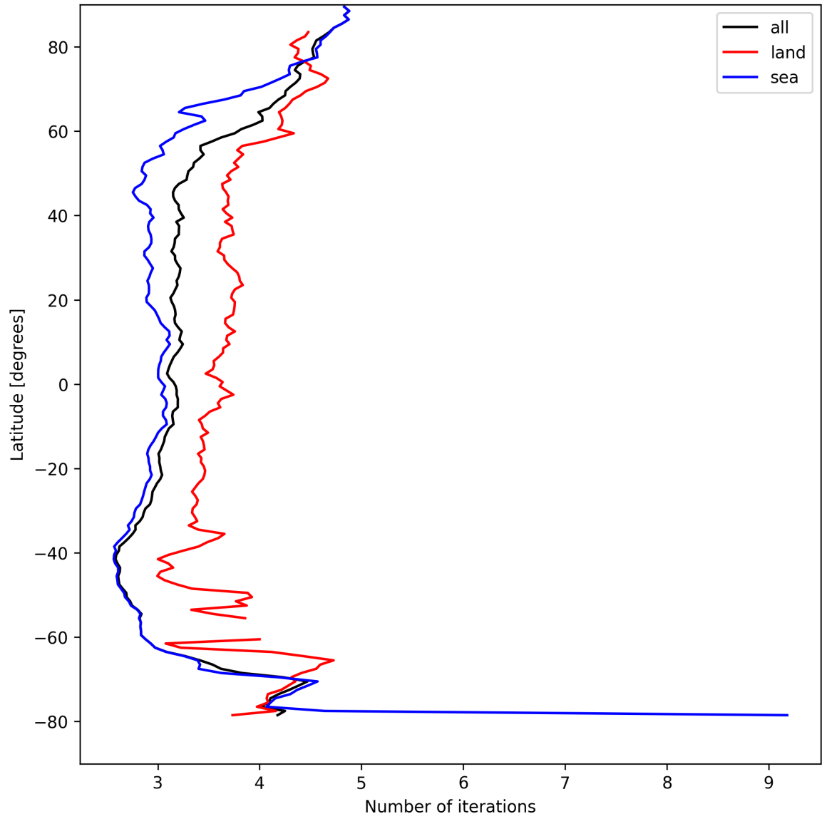
Figure 22: Zonal average of “Number of iterations” for 2025-04-14 to 2025-04-16.
