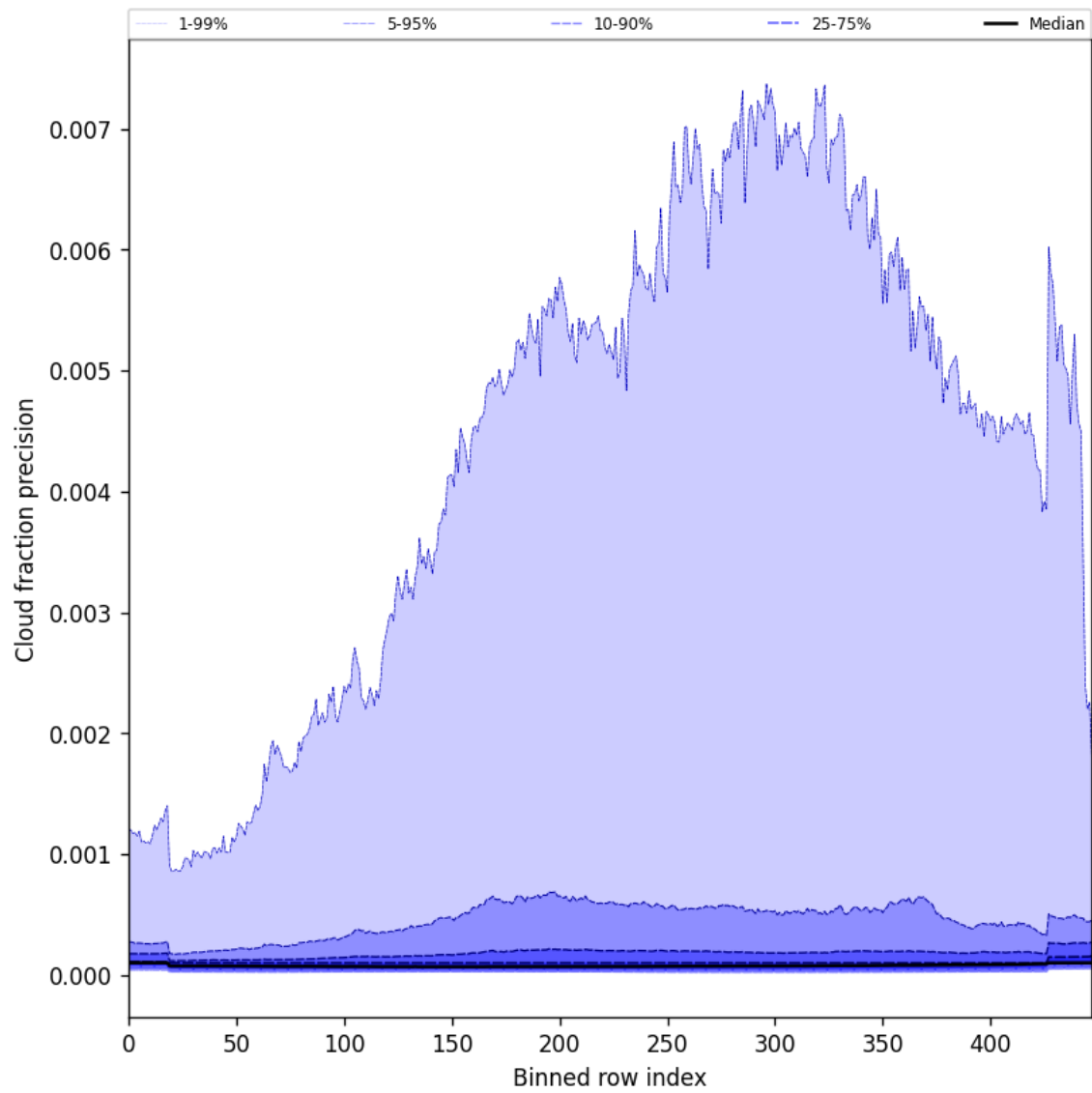
Figure 50: Along track statistics of “Cloud fraction precision” for 2025-04-14 to 2025-04-16
