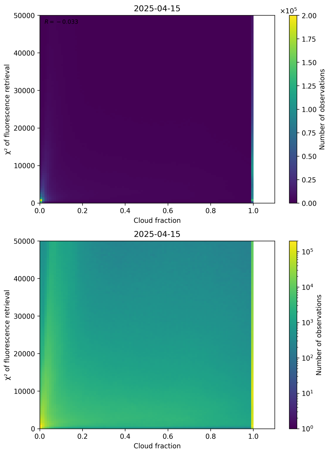
Figure 71: Scatter density plot of “Cloud fraction” against “ \chi^2 of fluorescence retrieval” for 2025-04-14 to 2025-04-16.
