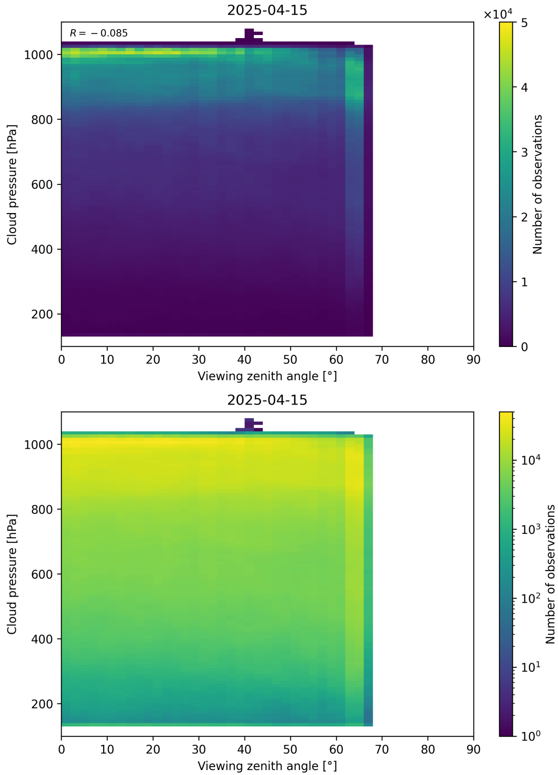
Figure 121: Scatter density plot of “Viewing zenith angle” against “Cloud pressure” for 2025-04-14 to 2025-04-16.
