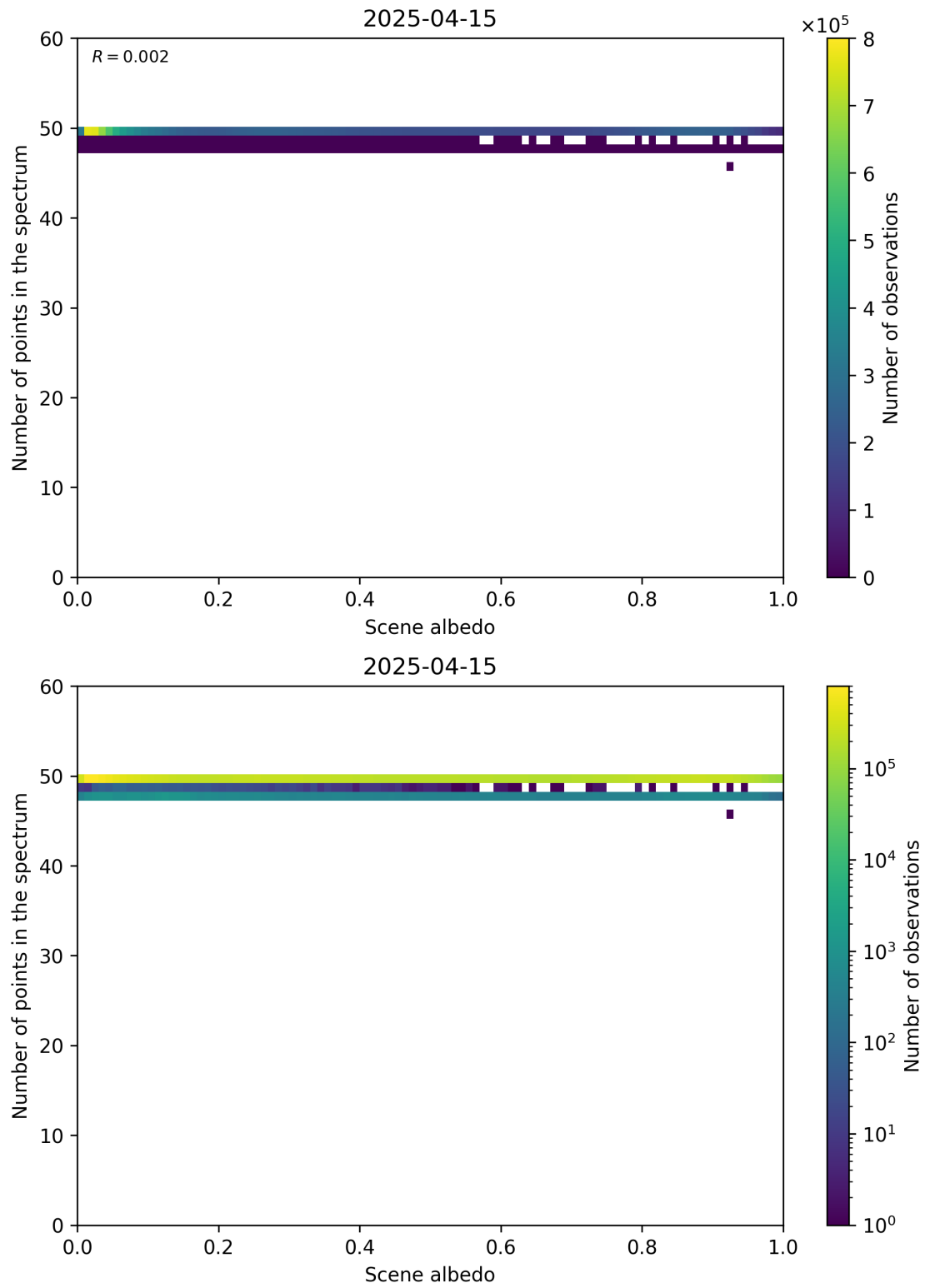
Figure 106: Scatter density plot of “Scene albedo” against “Number of points in the spectrum” for 2025-04-14 to 2025-04-16.
