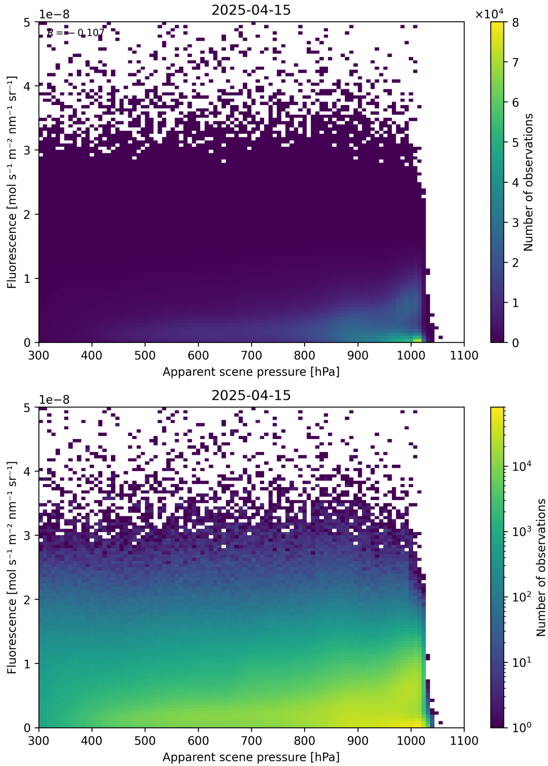
Figure 64: Scatter density plot of “Apparent scene pressure” against “Fluorescence” for 2025-04-14 to 2025-04-16.
