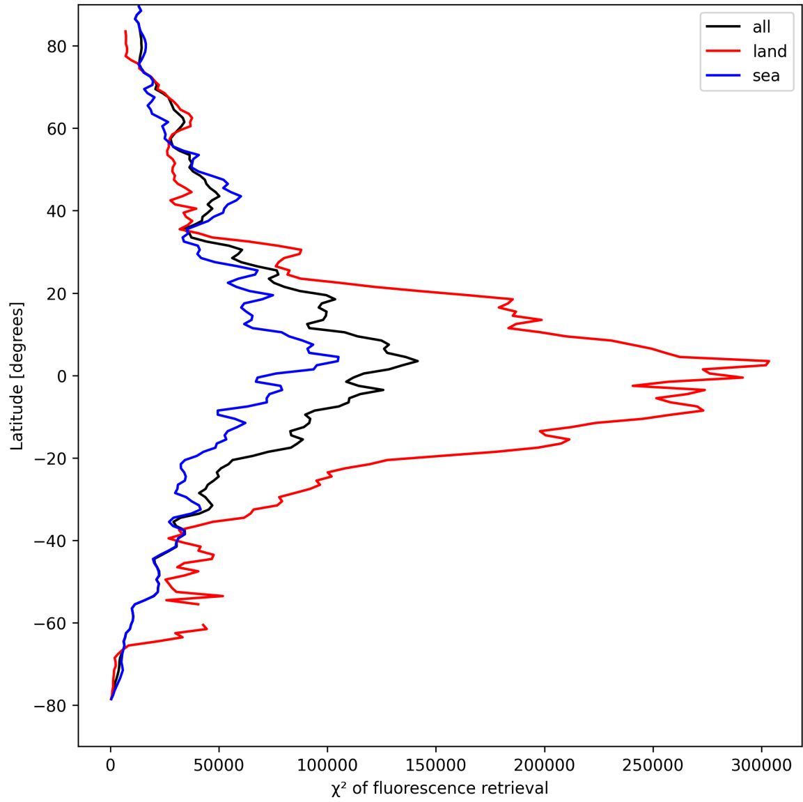
Figure 25: Zonal average of “ \chi^2 of fluorescence retrieval” for 2025-04-14 to 2025-04-16.
