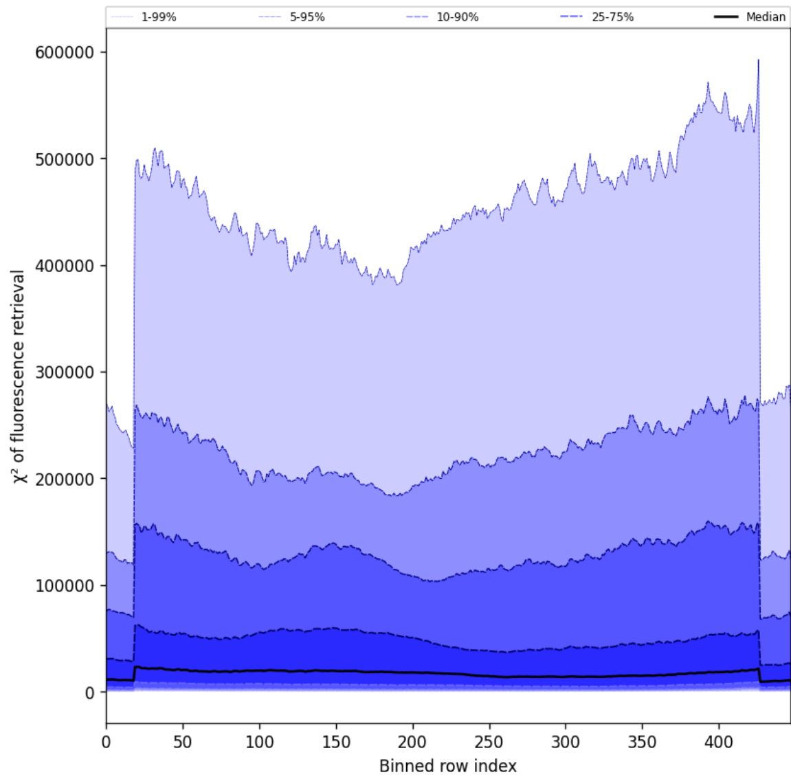
Figure 59: Along track statistics of “ \chi^2 of fluorescence retrieval” for 2025-04-14 to 2025-04-16
