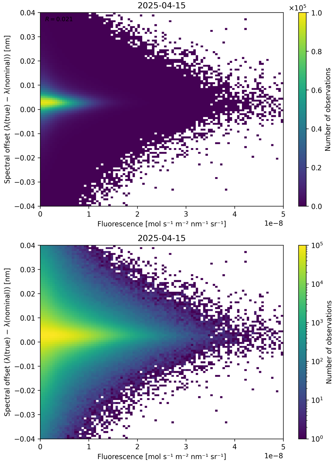
Figure 87: Scatter density plot of “Fluorescence” against “Spectral offset ( \lambda_{\text{true}} - \lambda_{\text{nominal}} )” for 2025-04-14 to 2025-04-16.
