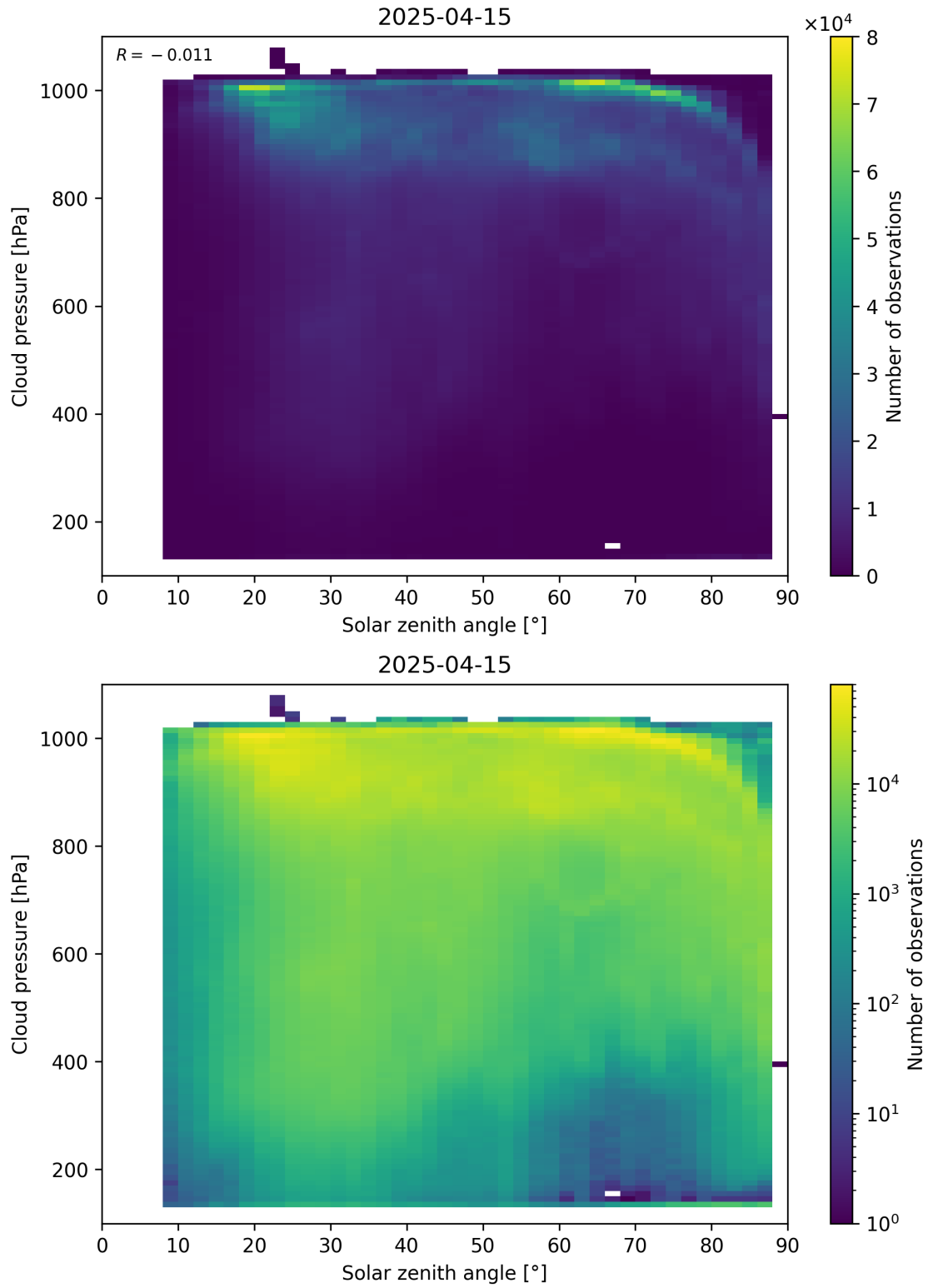
Figure 111: Scatter density plot of “Solar zenith angle” against “Cloud pressure” for 2025-04-14 to 2025-04-16.
