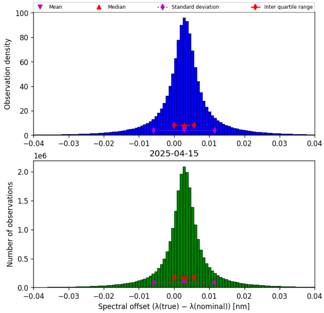
Figure 45: Histogram of “Spectral offset ( \lambda_{\text{true}} - \lambda_{\text{nominal}} )” for 2025-04-14 to 2025-04-16
