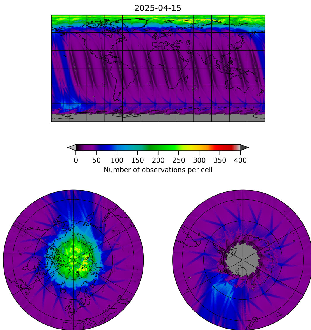
Figure 11: Map of the number of observations for 2025-04-14 to 2025-04-16
