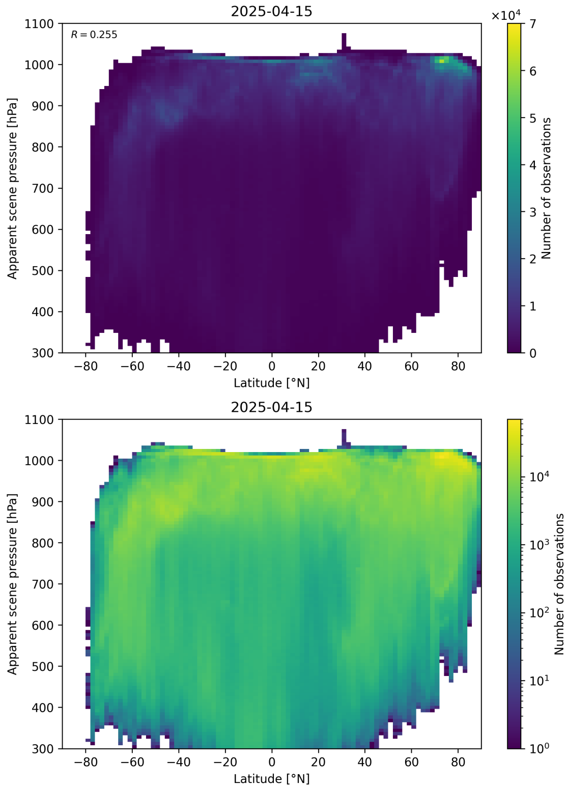
Figure 88: Scatter density plot of “Latitude” against “Apparent scene pressure” for 2025-04-14 to 2025-04-16.
