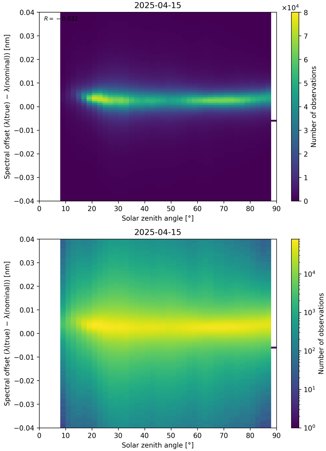
Figure 117: Scatter density plot of “Solar zenith angle” against “Spectral offset ( \lambda_{\text{true}} - \lambda_{\text{nominal}} )” for 2025-04-14 to 2025-04-16.
