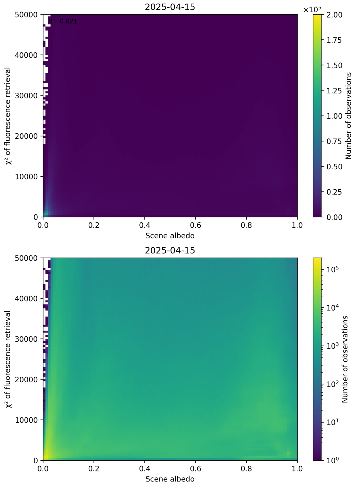
Figure 103: Scatter density plot of “Scene albedo” against “ \chi^2 of fluorescence retrieval” for 2025-04-14 to 2025-04-16.
