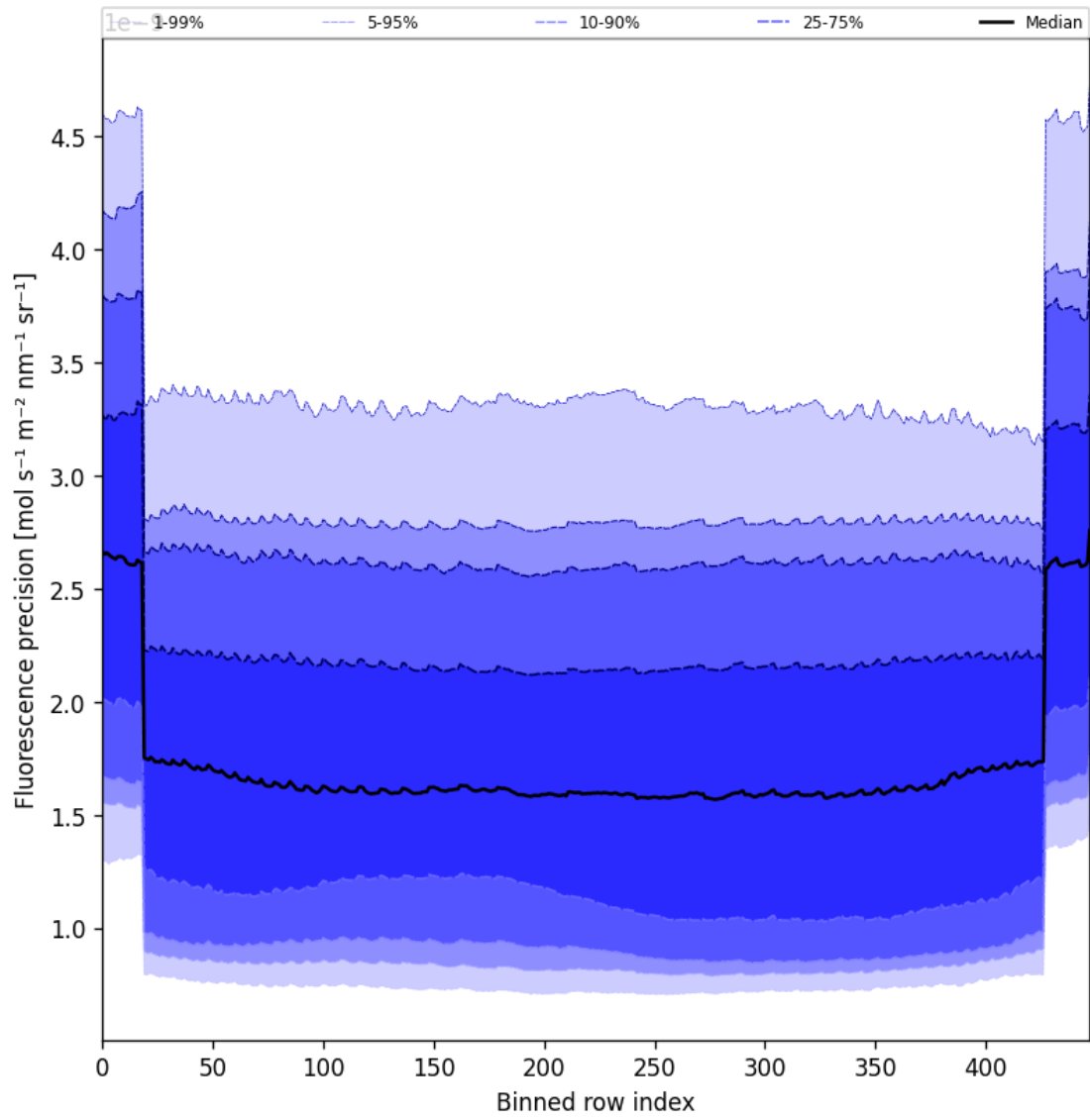
Figure 58: Along track statistics of “Fluorescence precision” for 2025-04-14 to 2025-04-16
