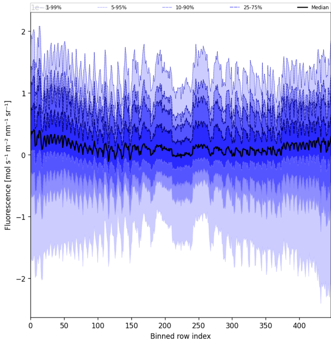
Figure 57: Along track statistics of “Fluorescence” for 2025-04-14 to 2025-04-16
