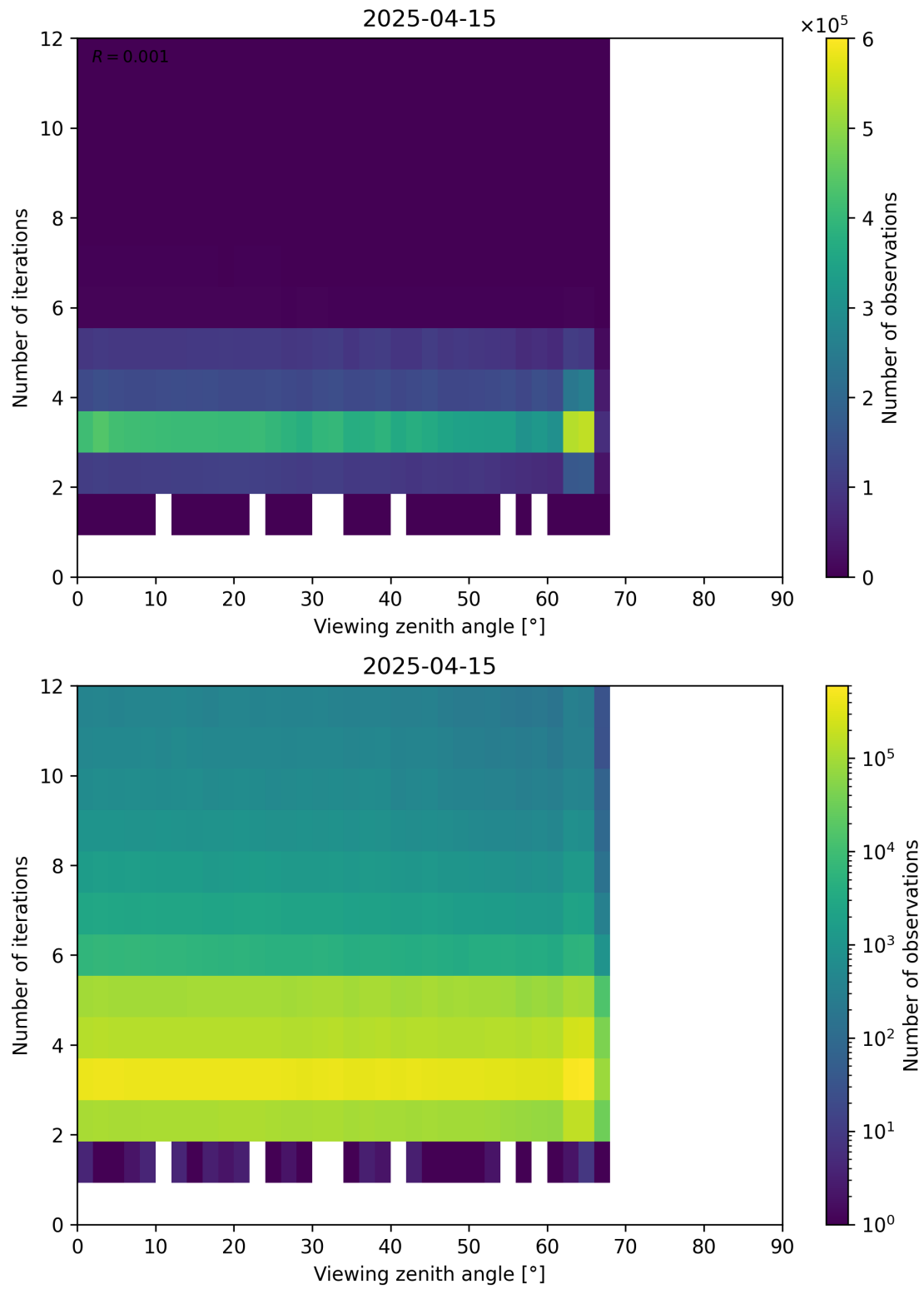
Figure 124: Scatter density plot of “Viewing zenith angle” against “Number of iterations” for 2025-04-14 to 2025-04-16.
