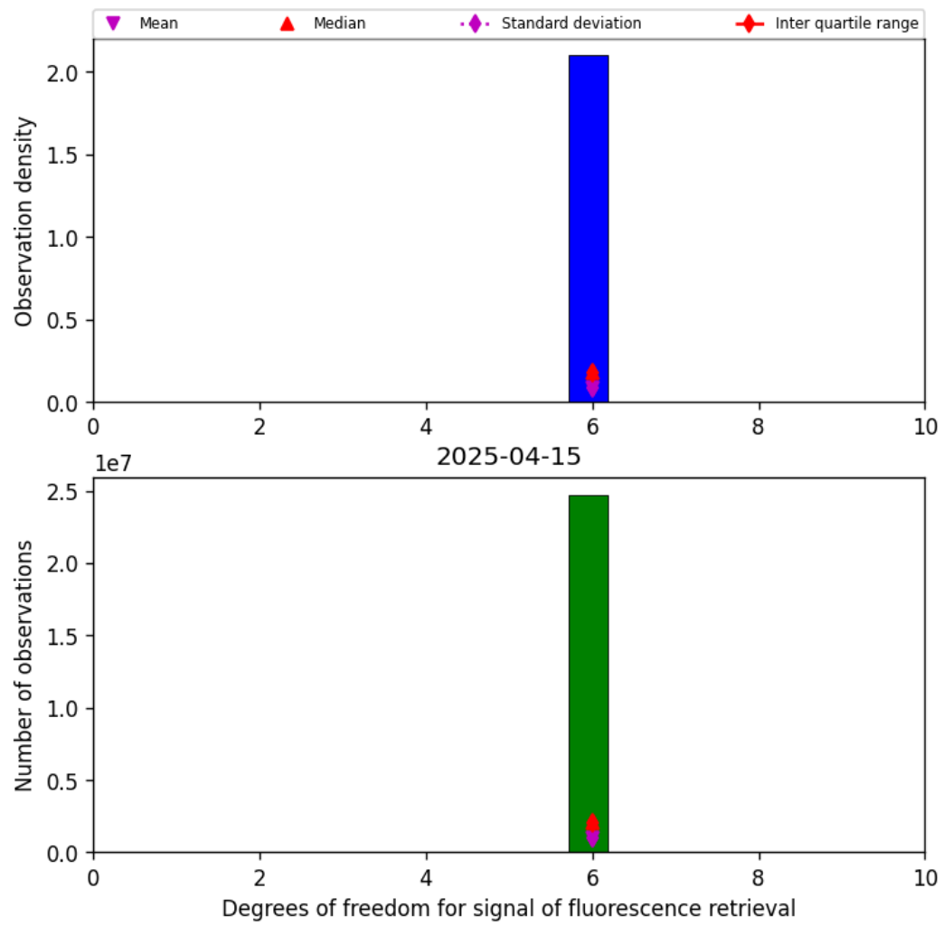
Figure 43: Histogram of "Degrees of freedom for signal of fluorescence retrieval" for 2025-04-14 to 2025-04-16
