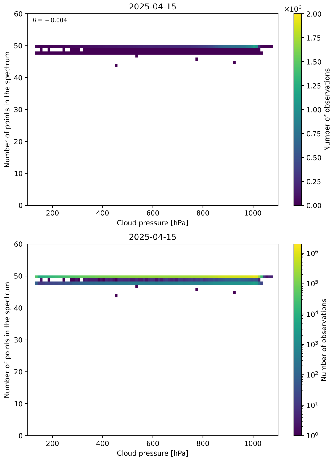
Figure 82: Scatter density plot of “Cloud pressure” against “Number of points in the spectrum” for 2025-04-14 to 2025-04-16.
