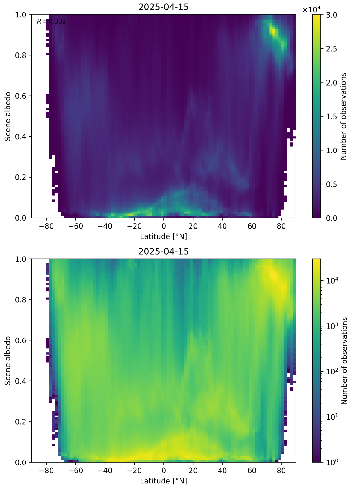
Figure 95: Scatter density plot of “Latitude” against “Scene albedo” for 2025-04-14 to 2025-04-16.
