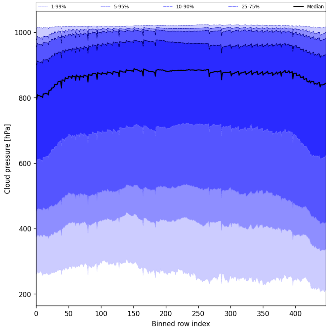
Figure 47: Along track statistics of “Cloud pressure” for 2025-04-14 to 2025-04-16
