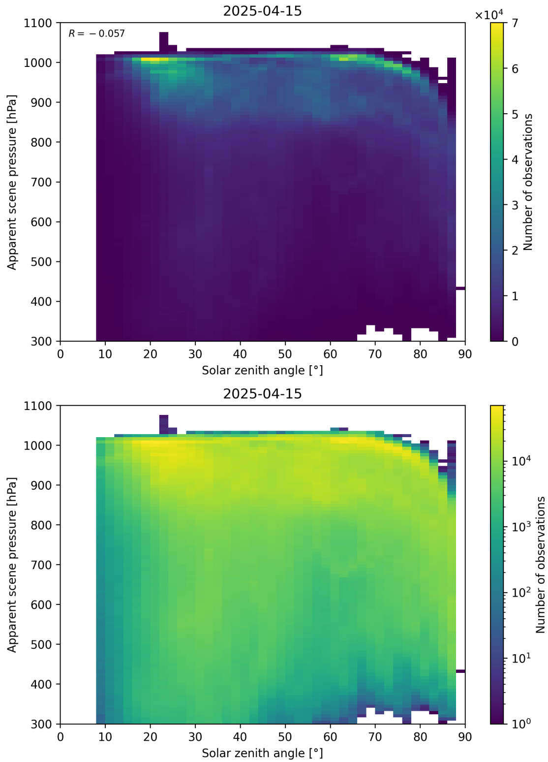
Figure 108: Scatter density plot of “Solar zenith angle” against “Apparent scene pressure” for 2025-04-14 to 2025-04-16.
