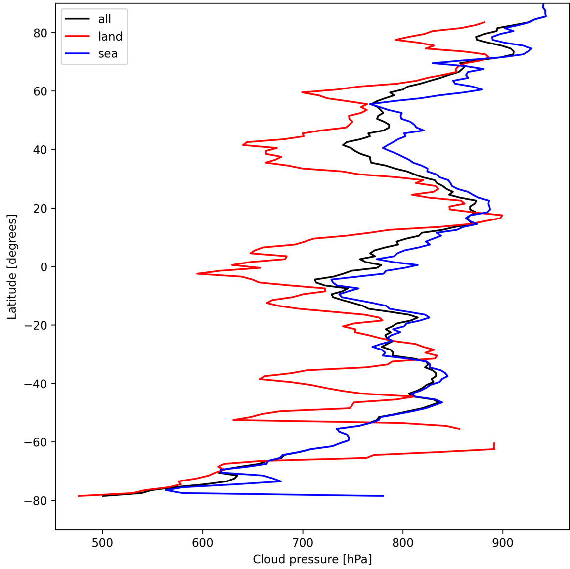
Figure 13: Zonal average of “Cloud pressure” for 2025-04-14 to 2025-04-16.
