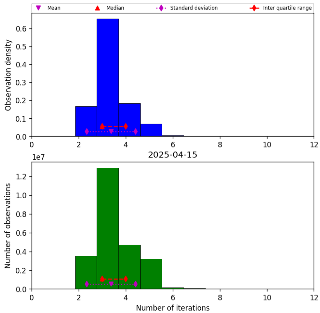
Figure 39: Histogram of “Number of iterations” for 2025-04-14 to 2025-04-16
