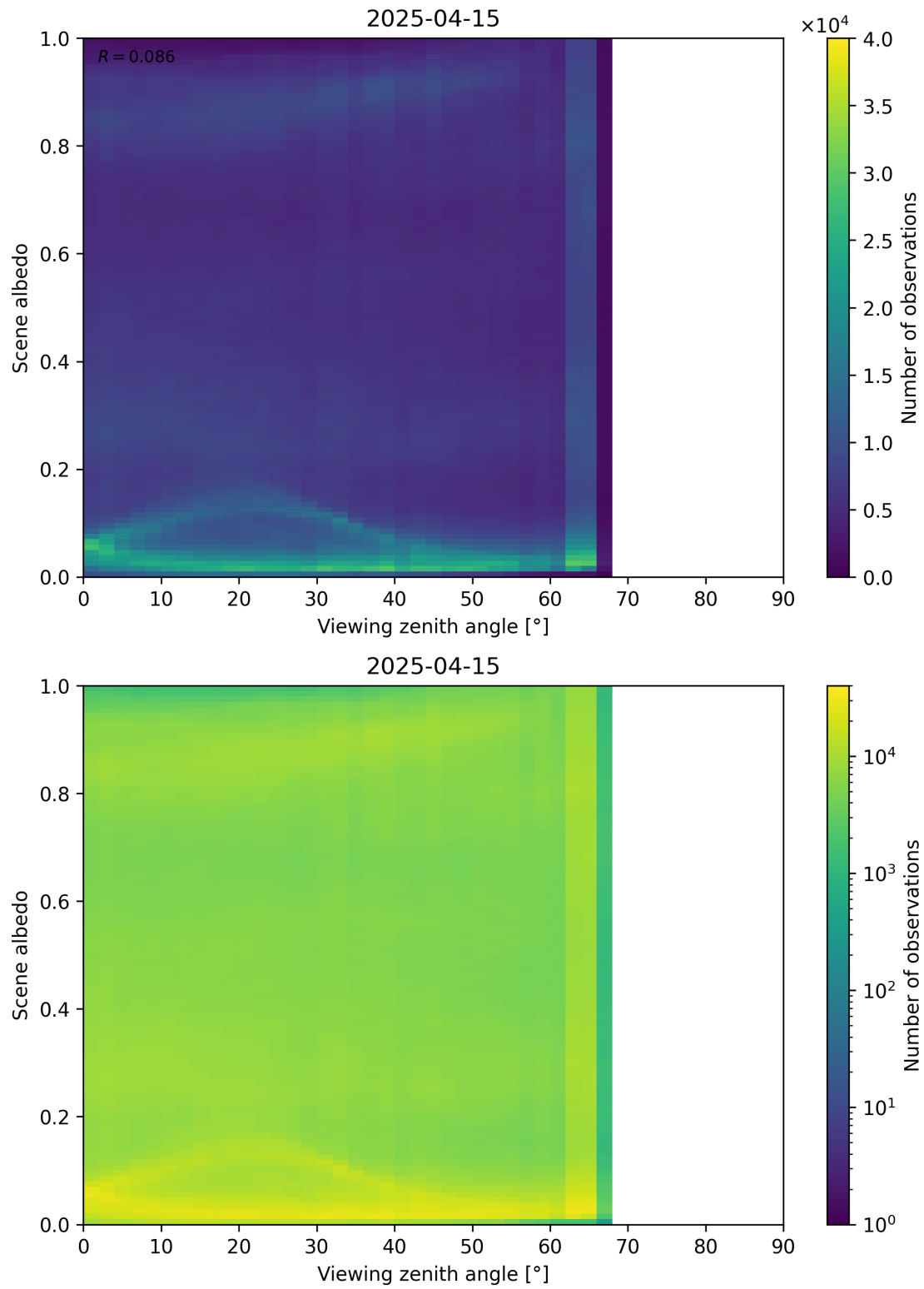
Figure 126: Scatter density plot of “Viewing zenith angle” against “Scene albedo” for 2025-04-14 to 2025-04-16.
