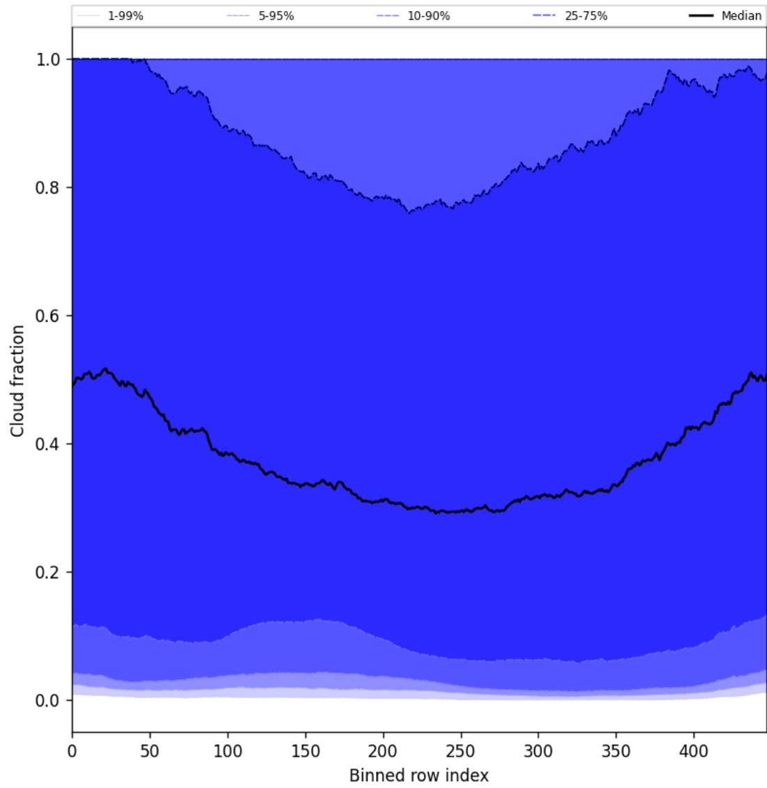
Figure 49: Along track statistics of “Cloud fraction” for 2025-04-14 to 2025-04-16
