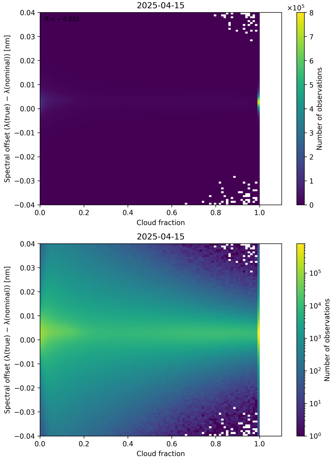
Figure 76: Scatter density plot of “Cloud fraction” against “Spectral offset ( \lambda_{\text{true}} - \lambda_{\text{nominal}} )” for 2025-04-14 to 2025-04-16.
