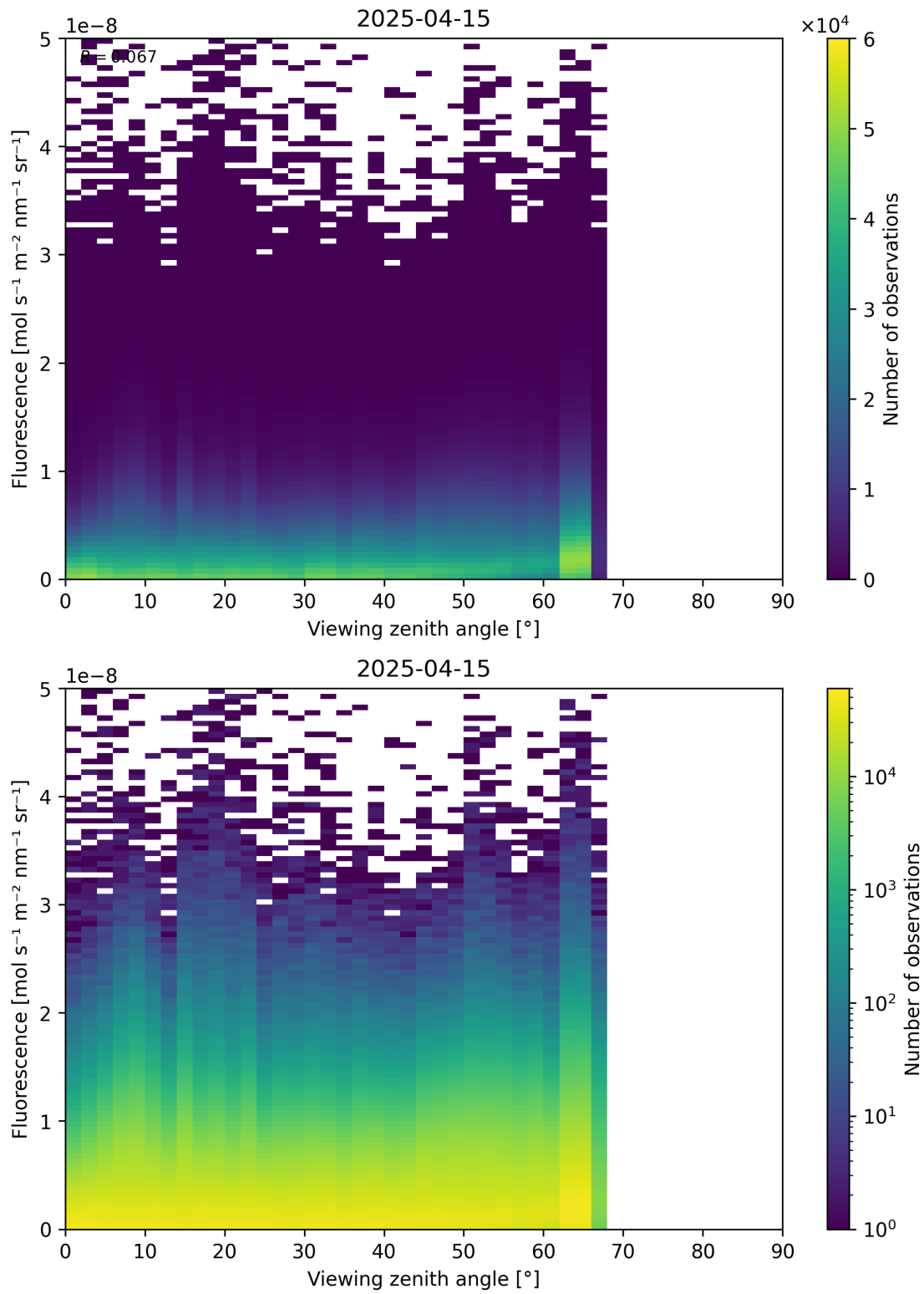
Figure 122: Scatter density plot of “Viewing zenith angle” against “Fluorescence” for 2025-04-14 to 2025-04-16.
