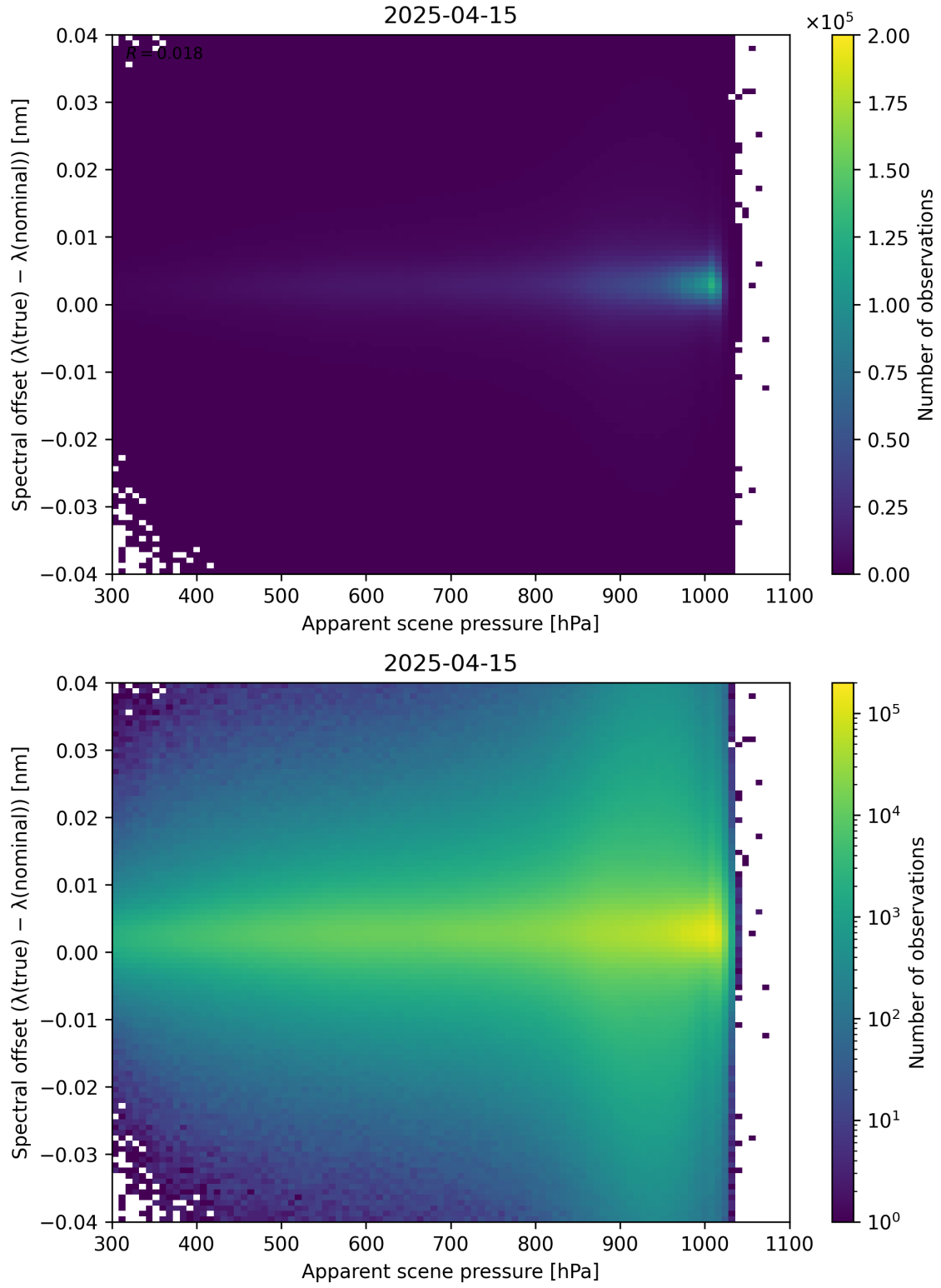
Figure 67: Scatter density plot of “Apparent scene pressure” against “Spectral offset ( \lambda_{\text{true}} - \lambda_{\text{nominal}} )” for 2025-04-14 to 2025-04-16.
