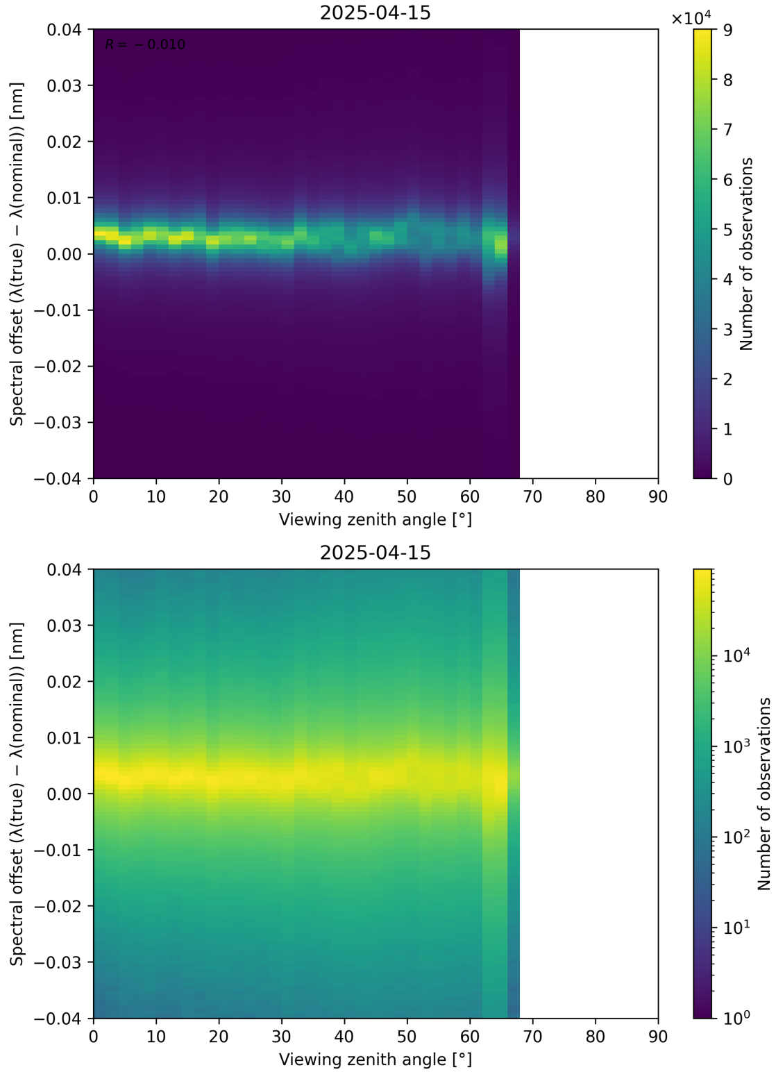
Figure 128: Scatter density plot of “Viewing zenith angle” against “Spectral offset ( \lambda_{\text{true}} - \lambda_{\text{nominal}} )” for 2025-04-14 to 2025-04-16.
