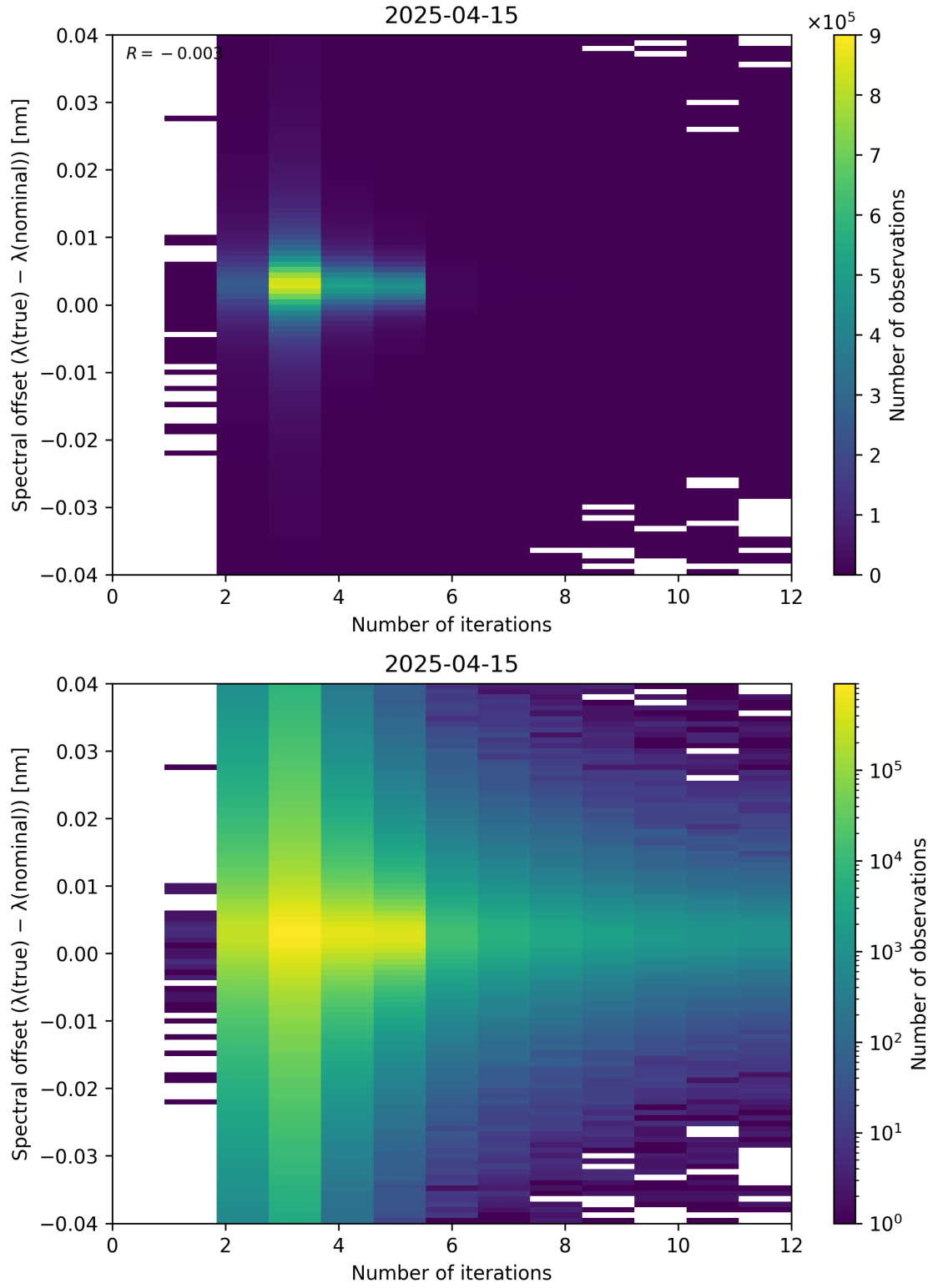
Figure 100: Scatter density plot of “Number of iterations” against “Spectral offset ( \lambda_{\text{true}} - \lambda_{\text{nominal}} )” for 2025-04-14 to 2025-04-16.
