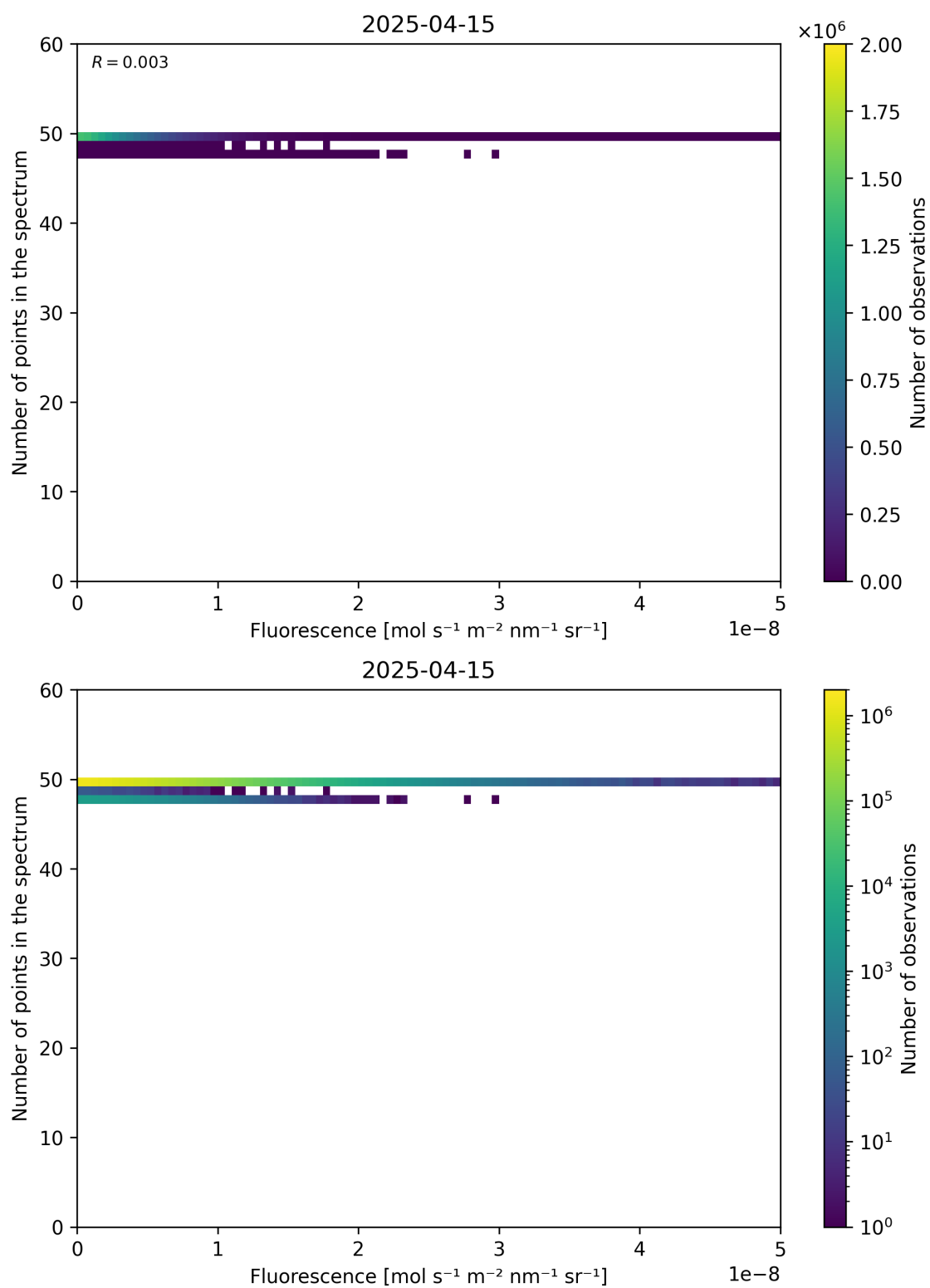
Figure 86: Scatter density plot of “Fluorescence” against “Number of points in the spectrum” for 2025-04-14 to 2025-04-16.
