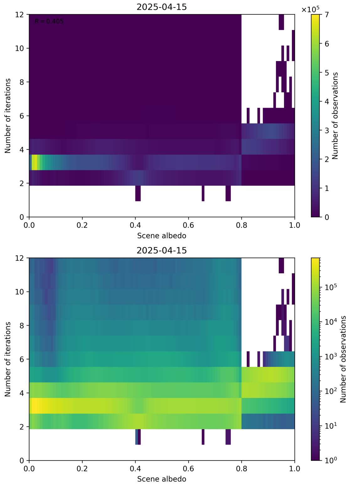
Figure 105: Scatter density plot of “Scene albedo” against “Number of iterations” for 2025-04-14 to 2025-04-16.
