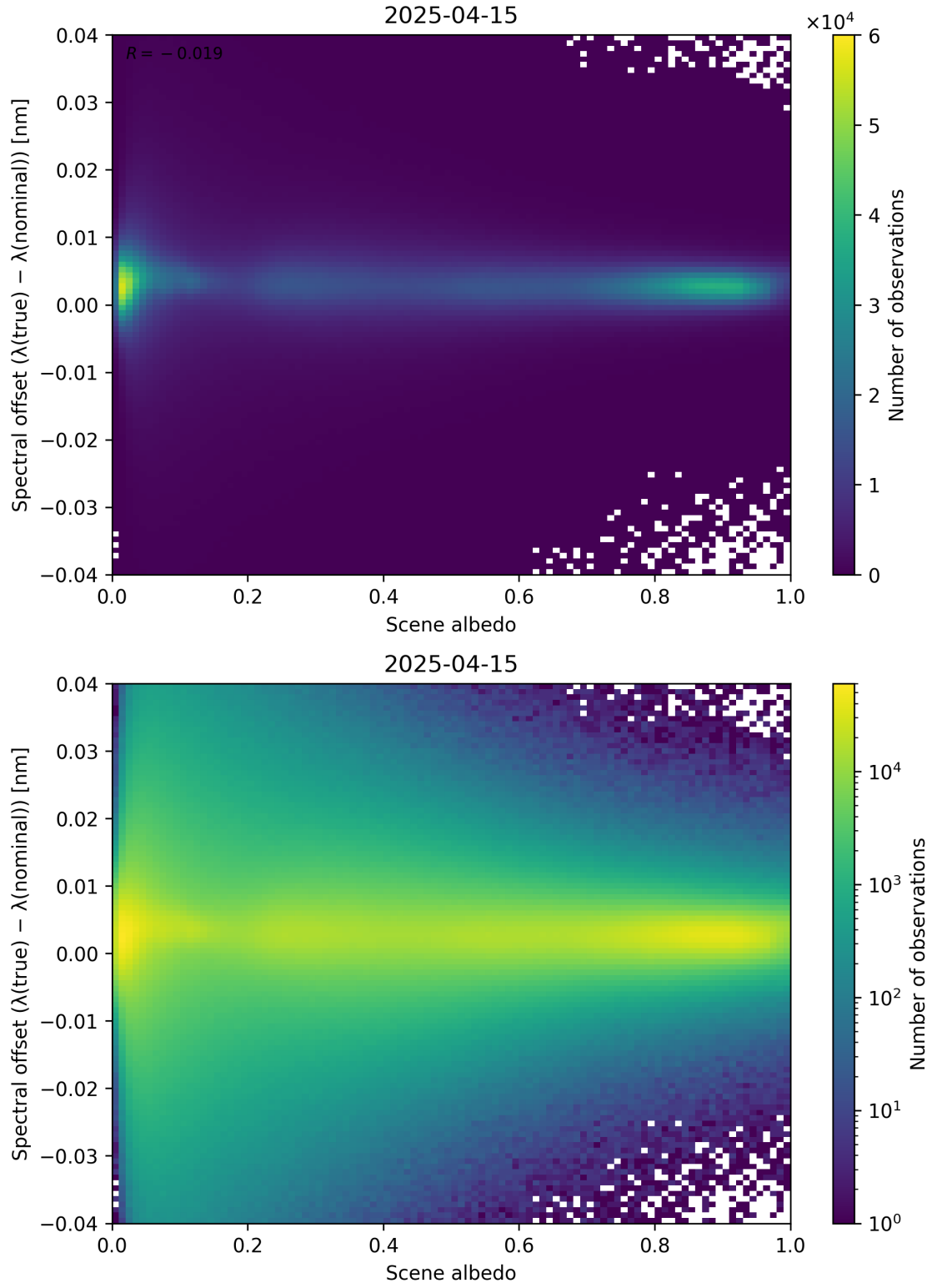
Figure 107: Scatter density plot of “Scene albedo” against “Spectral offset ( \lambda_{\text{true}} - \lambda_{\text{nominal}} )” for 2025-04-14 to 2025-04-16.
