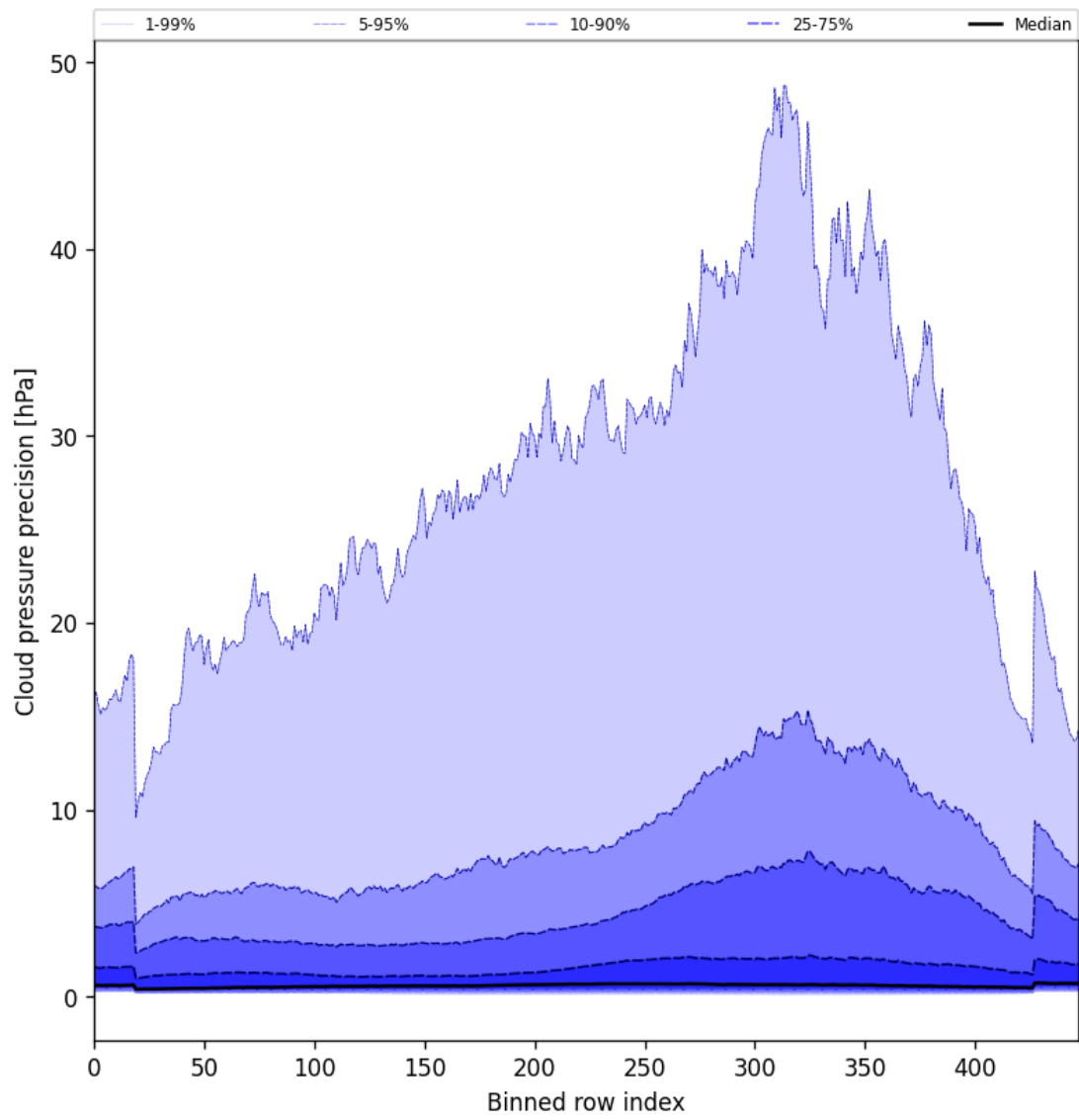
Figure 48: Along track statistics of “Cloud pressure precision” for 2025-04-14 to 2025-04-16
