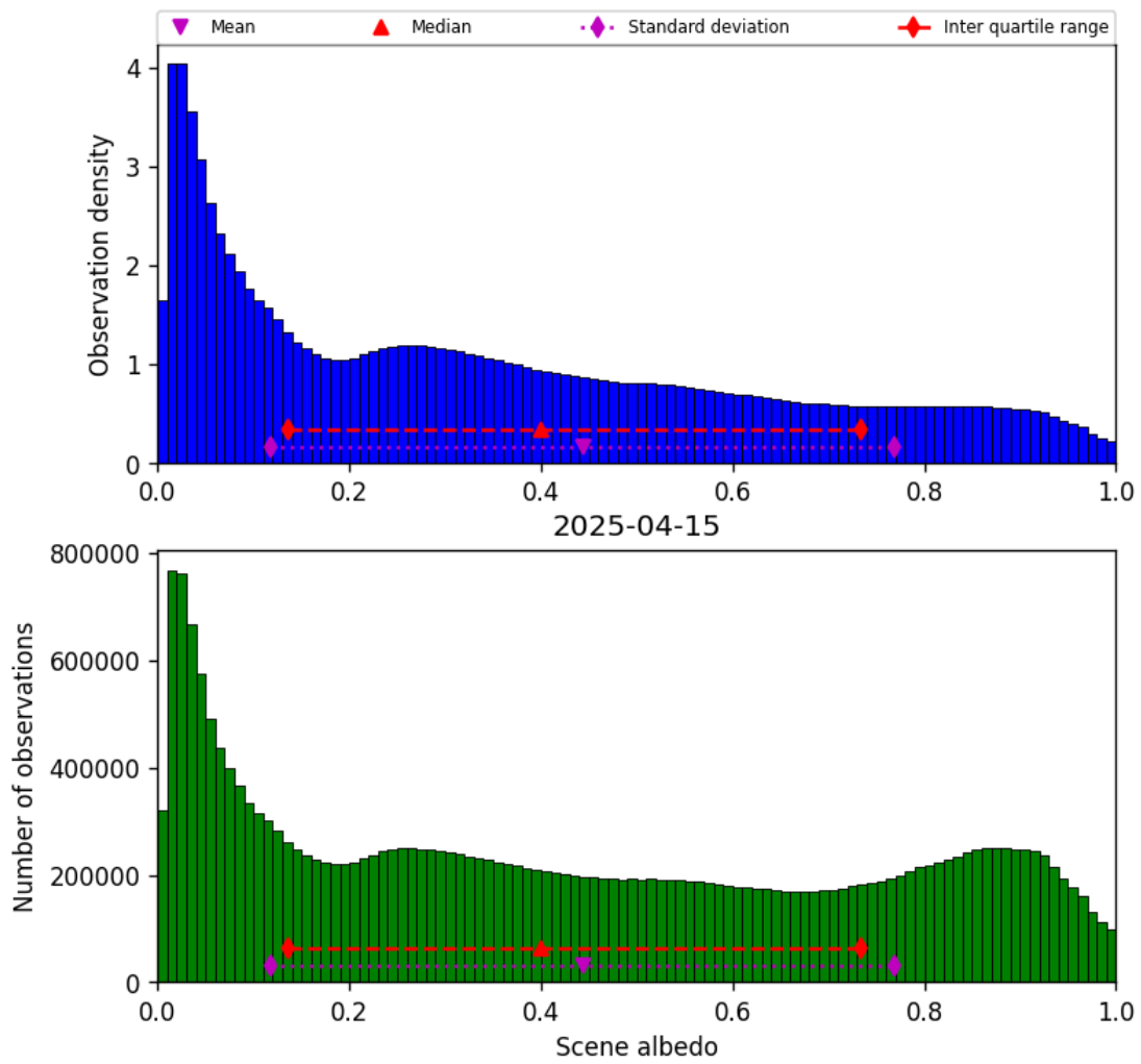
Figure 34: Histogram of “Scene albedo” for 2025-04-14 to 2025-04-16
