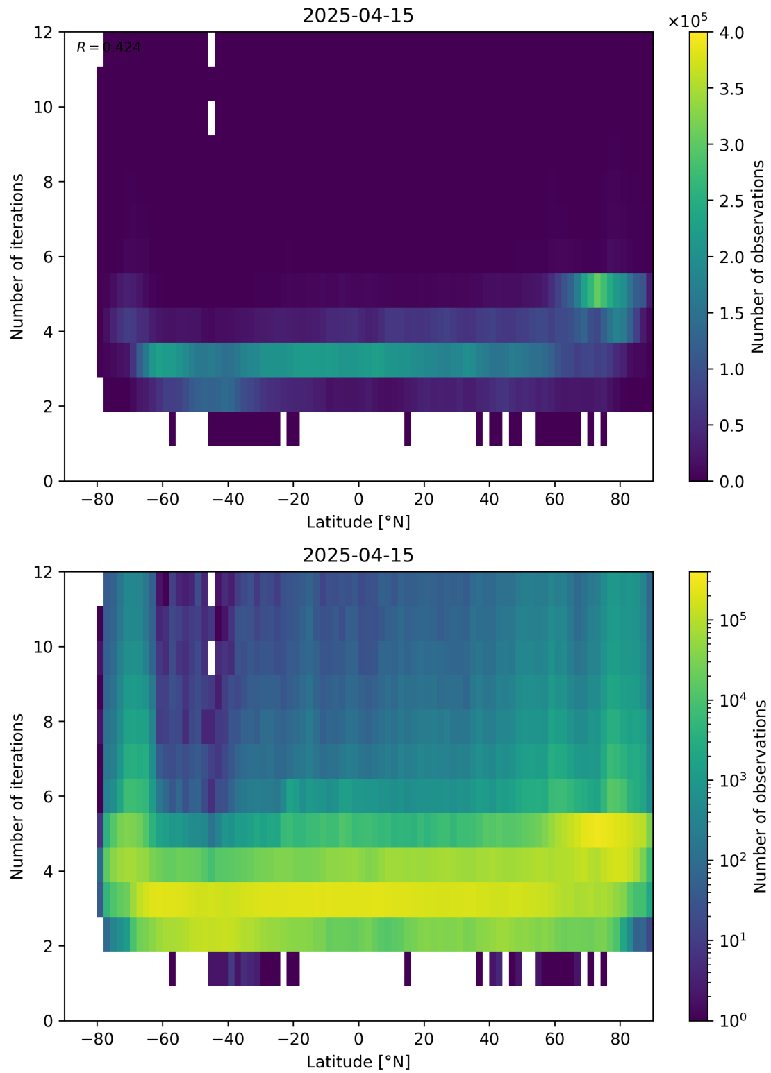
Figure 93: Scatter density plot of “Latitude” against “Number of iterations” for 2025-04-14 to 2025-04-16.
