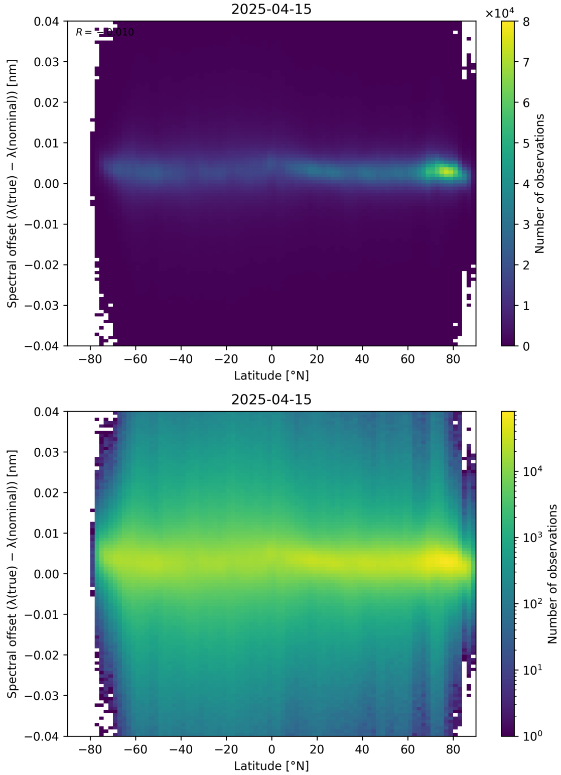
Figure 96: Scatter density plot of “Latitude” against “Spectral offset ( \lambda_{\text{true}} - \lambda_{\text{nominal}} )” for 2025-04-14 to 2025-04-16.
