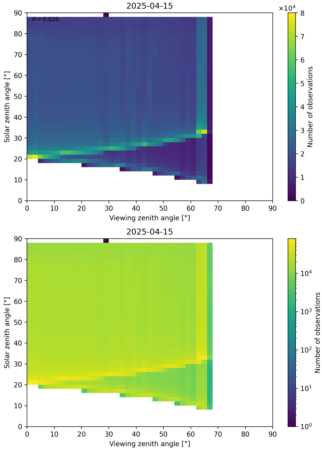
Figure 127: Scatter density plot of “Viewing zenith angle” against “Solar zenith angle” for 2025-04-14 to 2025-04-16.
