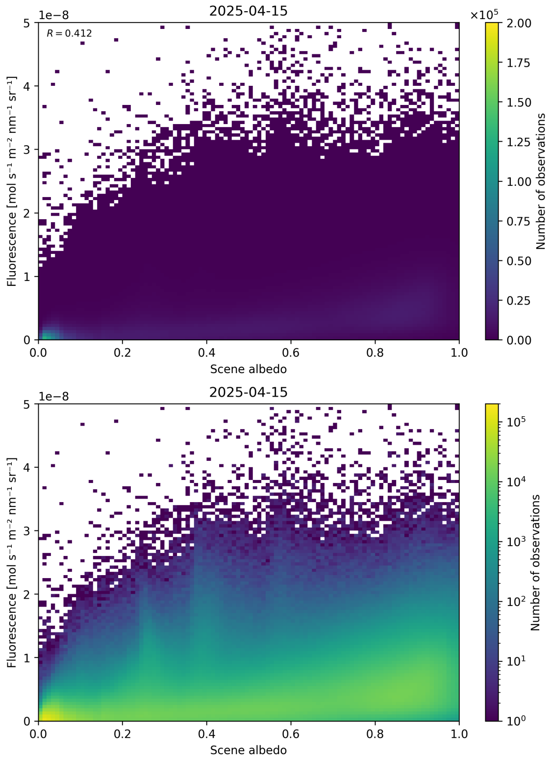
Figure 104: Scatter density plot of “Scene albedo” against “Fluorescence” for 2025-04-14 to 2025-04-16.
