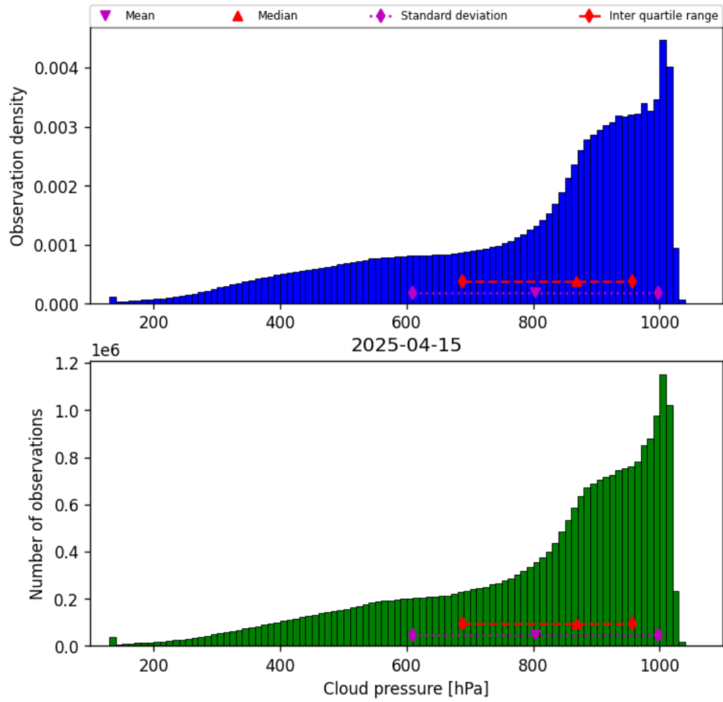
Figure 30: Histogram of “Cloud pressure” for 2025-04-14 to 2025-04-16
