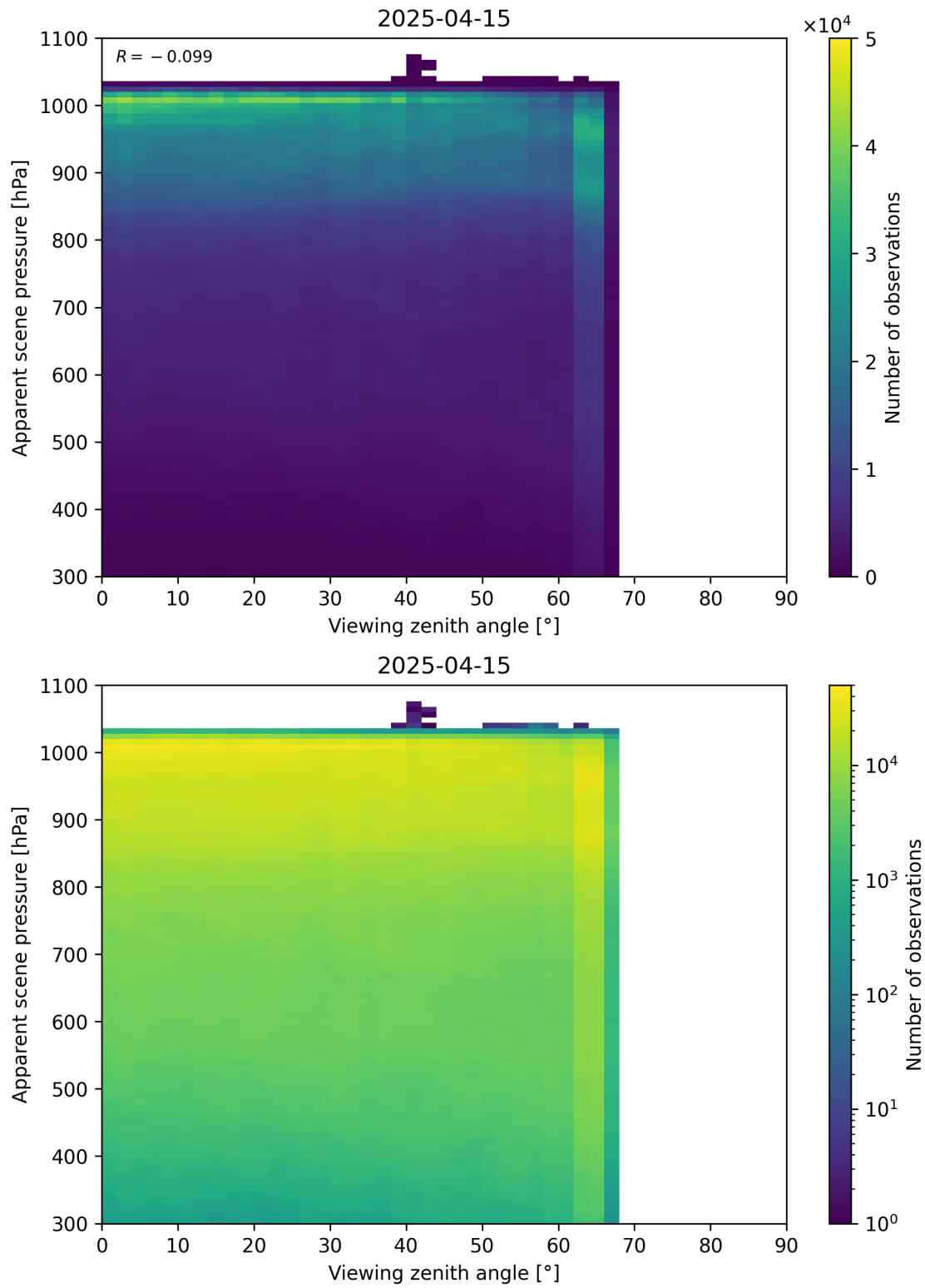
Figure 118: Scatter density plot of “Viewing zenith angle” against “Apparent scene pressure” for 2025-04-14 to 2025-04-16.
