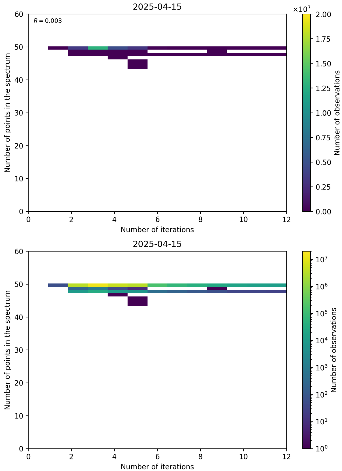
Figure 99: Scatter density plot of “Number of iterations” against “Number of points in the spectrum” for 2025-04-14 to 2025-04-16.
