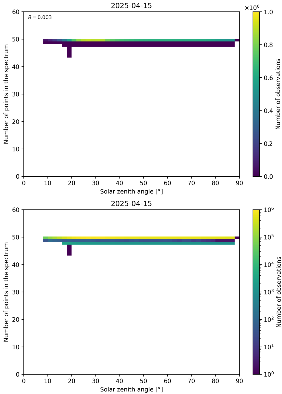
Figure 115: Scatter density plot of “Solar zenith angle” against “Number of points in the spectrum” for 2025-04-14 to 2025-04-16.
