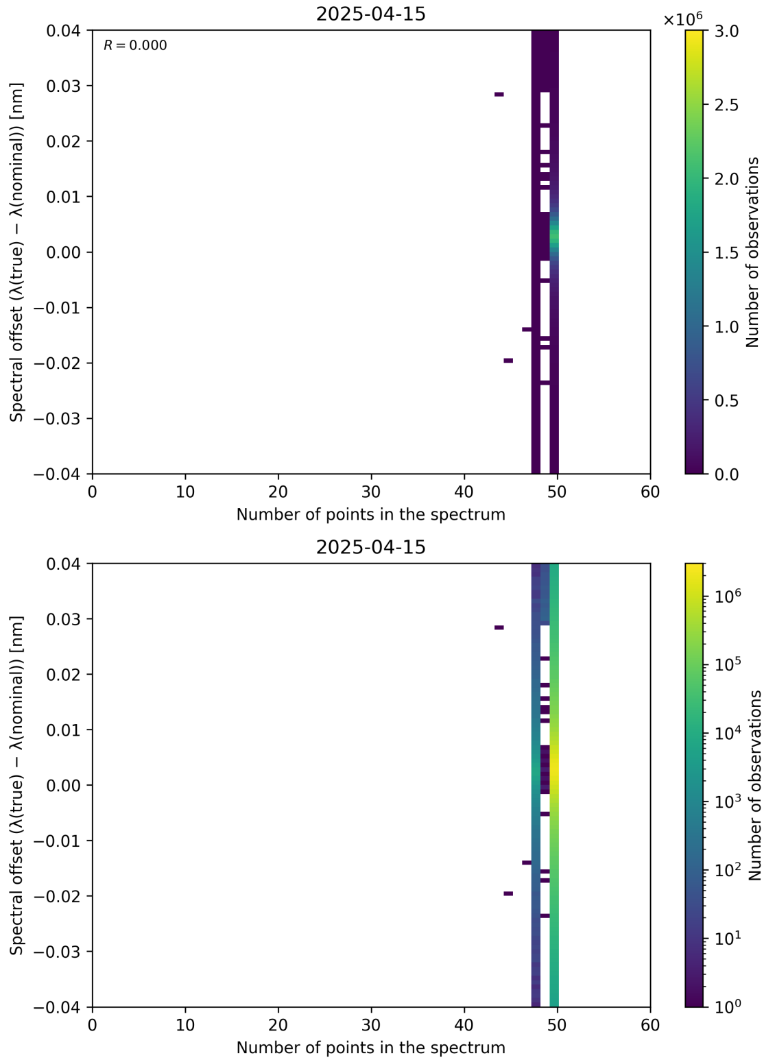
Figure 101: Scatter density plot of “Number of points in the spectrum” against “Spectral offset ( \lambda_{\text{true}} - \lambda_{\text{nominal}} )” for 2025-04-14 to 2025-04-16.
