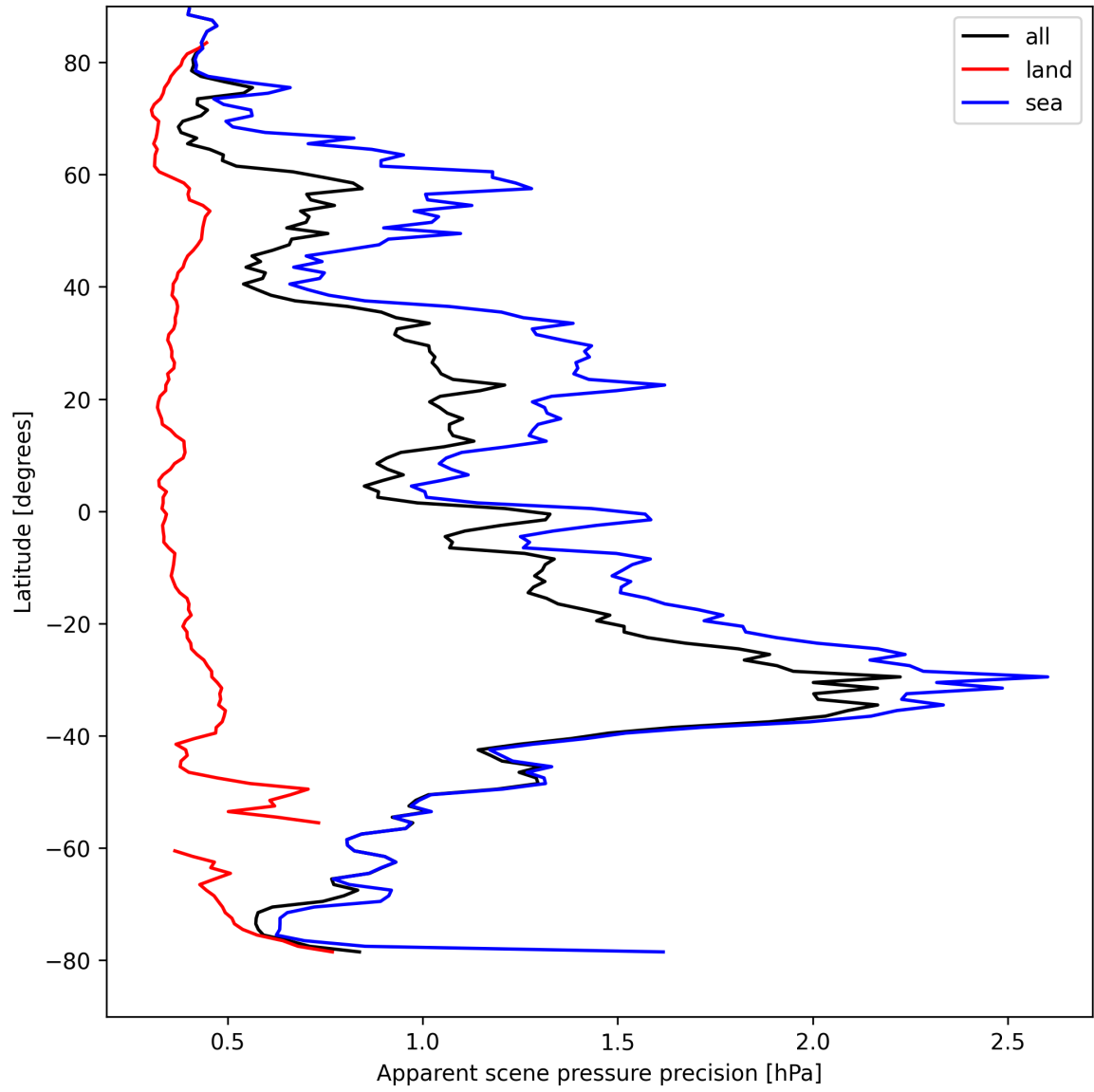
Figure 20: Zonal average of “Apparent scene pressure precision” for 2025-04-14 to 2025-04-16.
