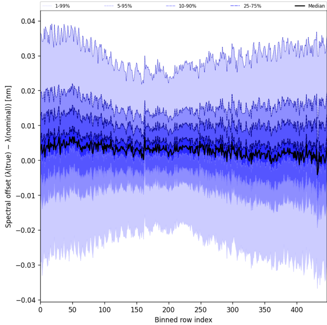
Figure 62: Along track statistics of “Spectral offset ( \lambda_{\text{true}} - \lambda_{\text{nominal}} )” for 2025-04-14 to 2025-04-16
