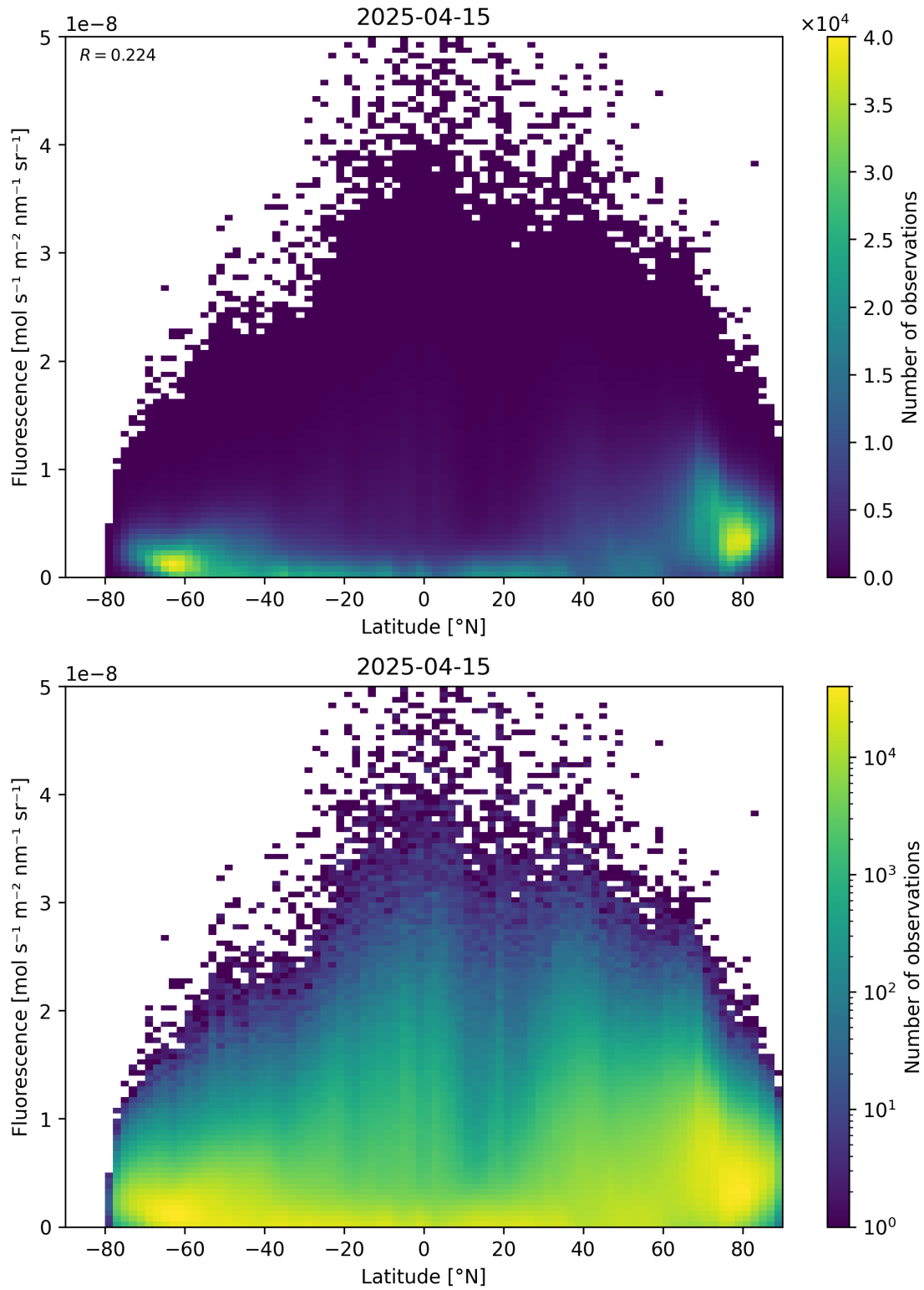
Figure 92: Scatter density plot of “Latitude” against “Fluorescence” for 2025-04-14 to 2025-04-16.
