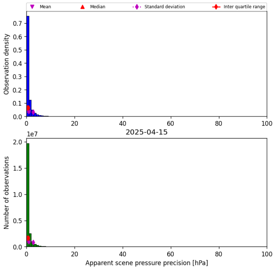
Figure 37: Histogram of “Apparent scene pressure precision” for 2025-04-14 to 2025-04-16
