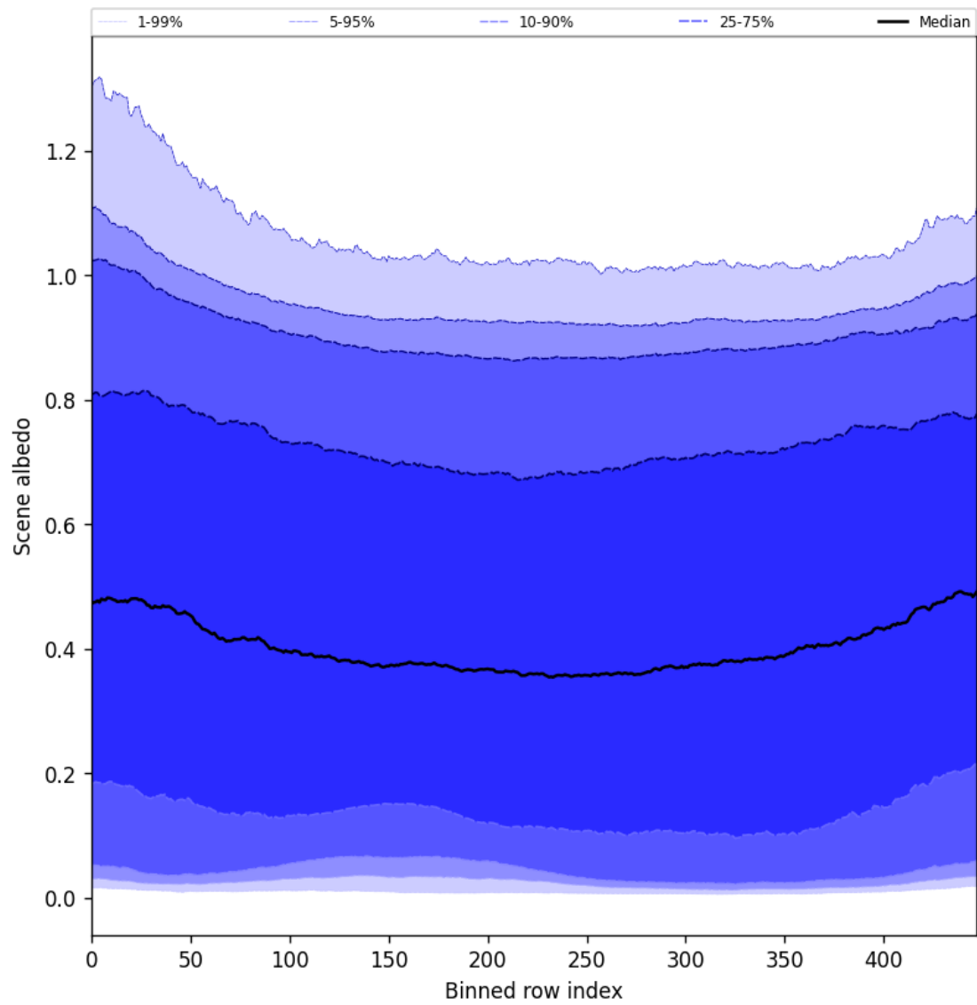
Figure 51: Along track statistics of “Scene albedo” for 2025-04-14 to 2025-04-16
