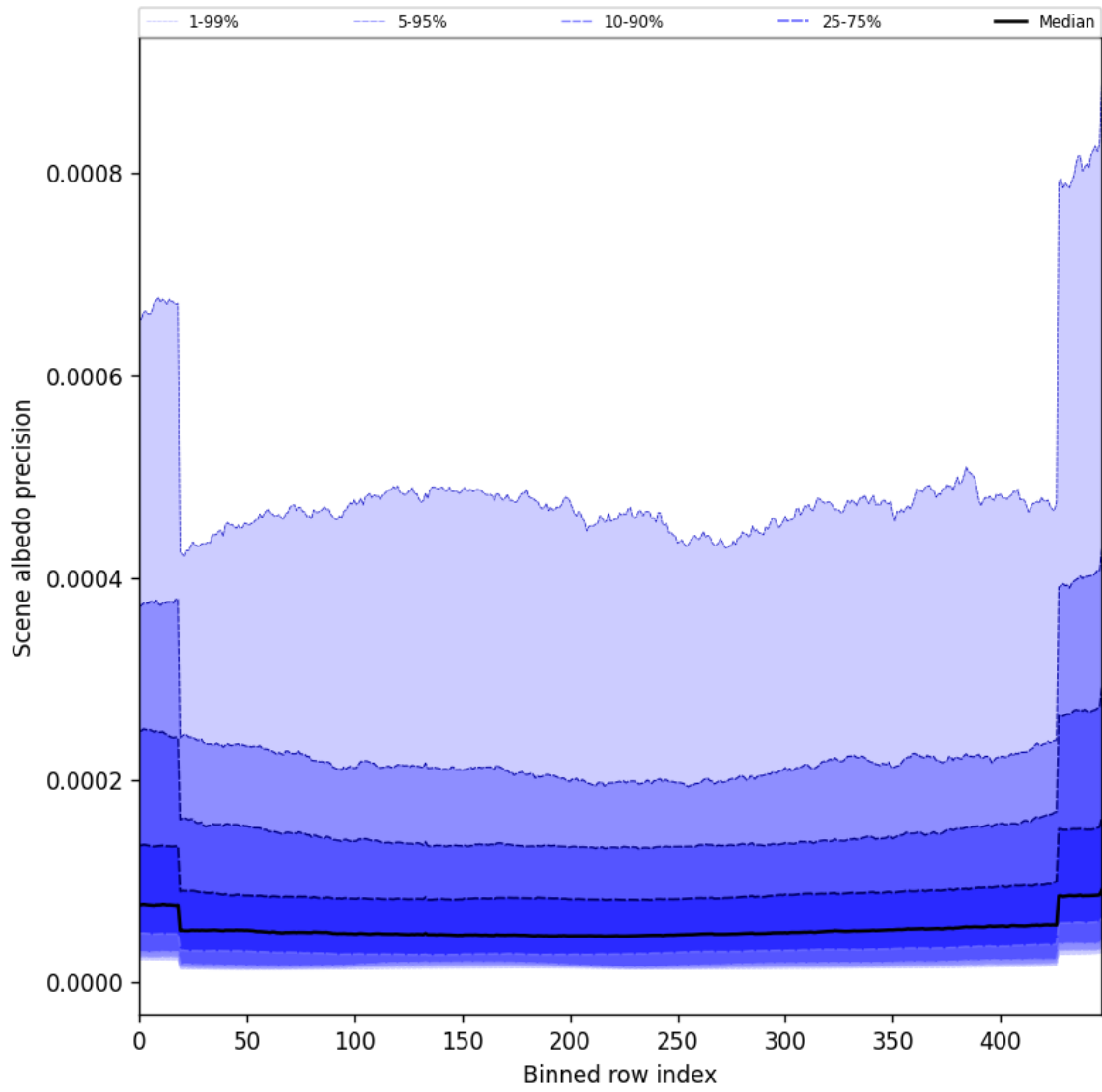
Figure 52: Along track statistics of “Scene albedo precision” for 2025-04-14 to 2025-04-16
