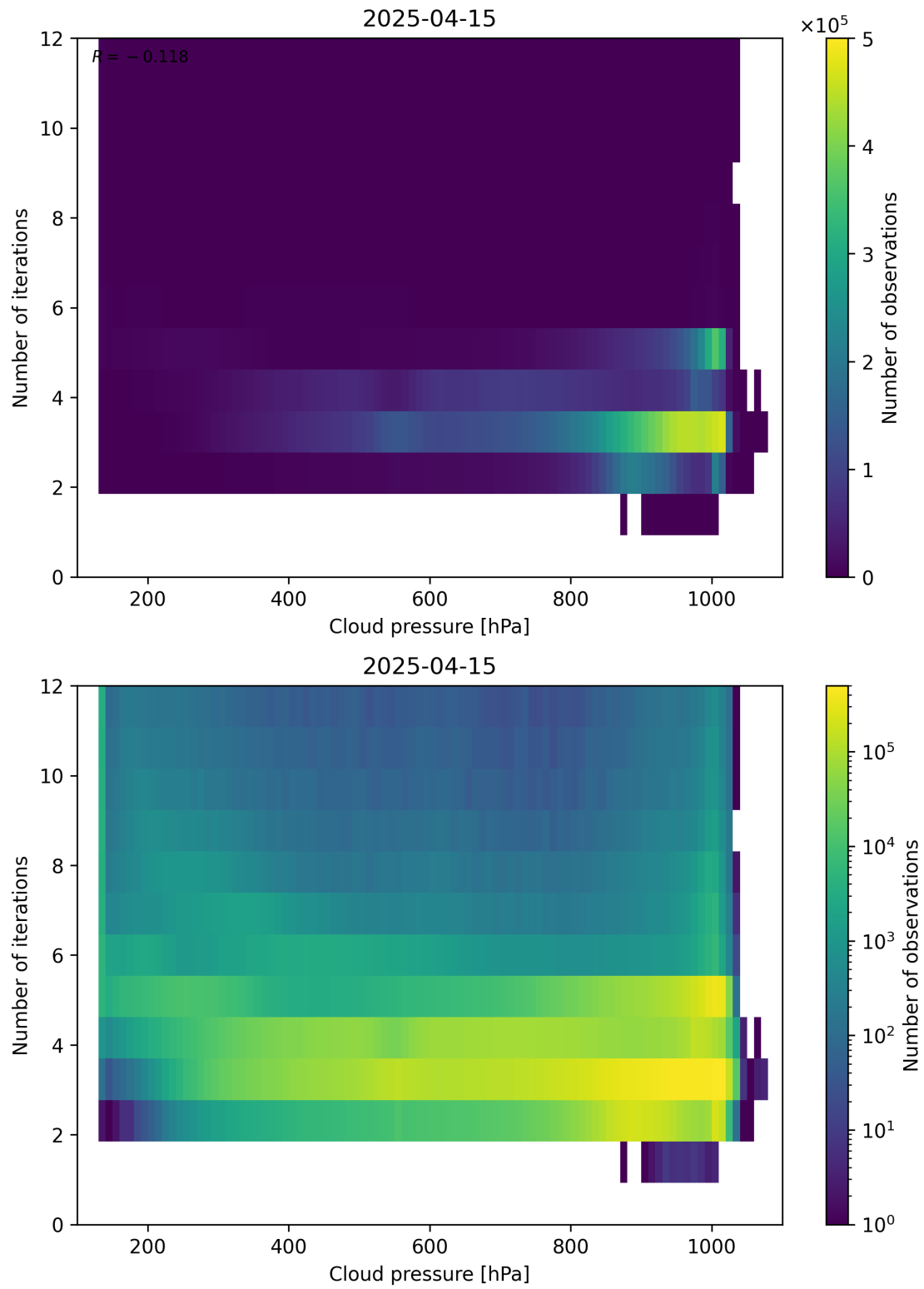
Figure 81: Scatter density plot of “Cloud pressure” against “Number of iterations” for 2025-04-14 to 2025-04-16.
