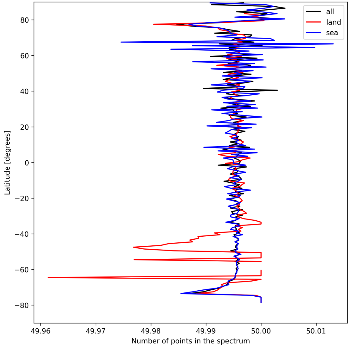
Figure 27: Zonal average of “Number of points in the spectrum” for 2025-04-14 to 2025-04-16.
