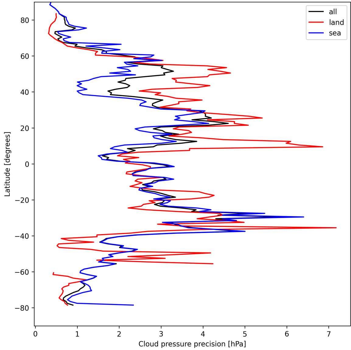
Figure 14: Zonal average of “Cloud pressure precision” for 2025-04-14 to 2025-04-16.
