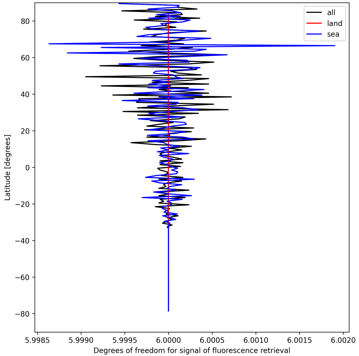
Figure 26: Zonal average of “Degrees of freedom for signal of fluorescence retrieval” for 2025-04-14 to 2025-04-16.
