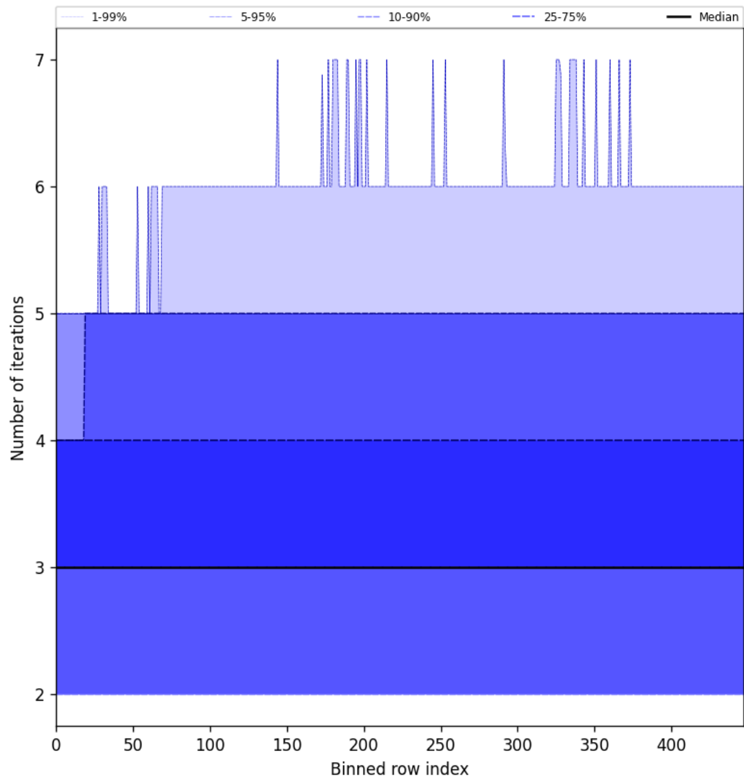
Figure 56: Along track statistics of “Number of iterations” for 2025-04-14 to 2025-04-16
