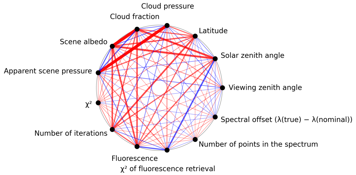
Figure 1: Map of correlation graph for 2025-04-14 to 2025-04-16.
