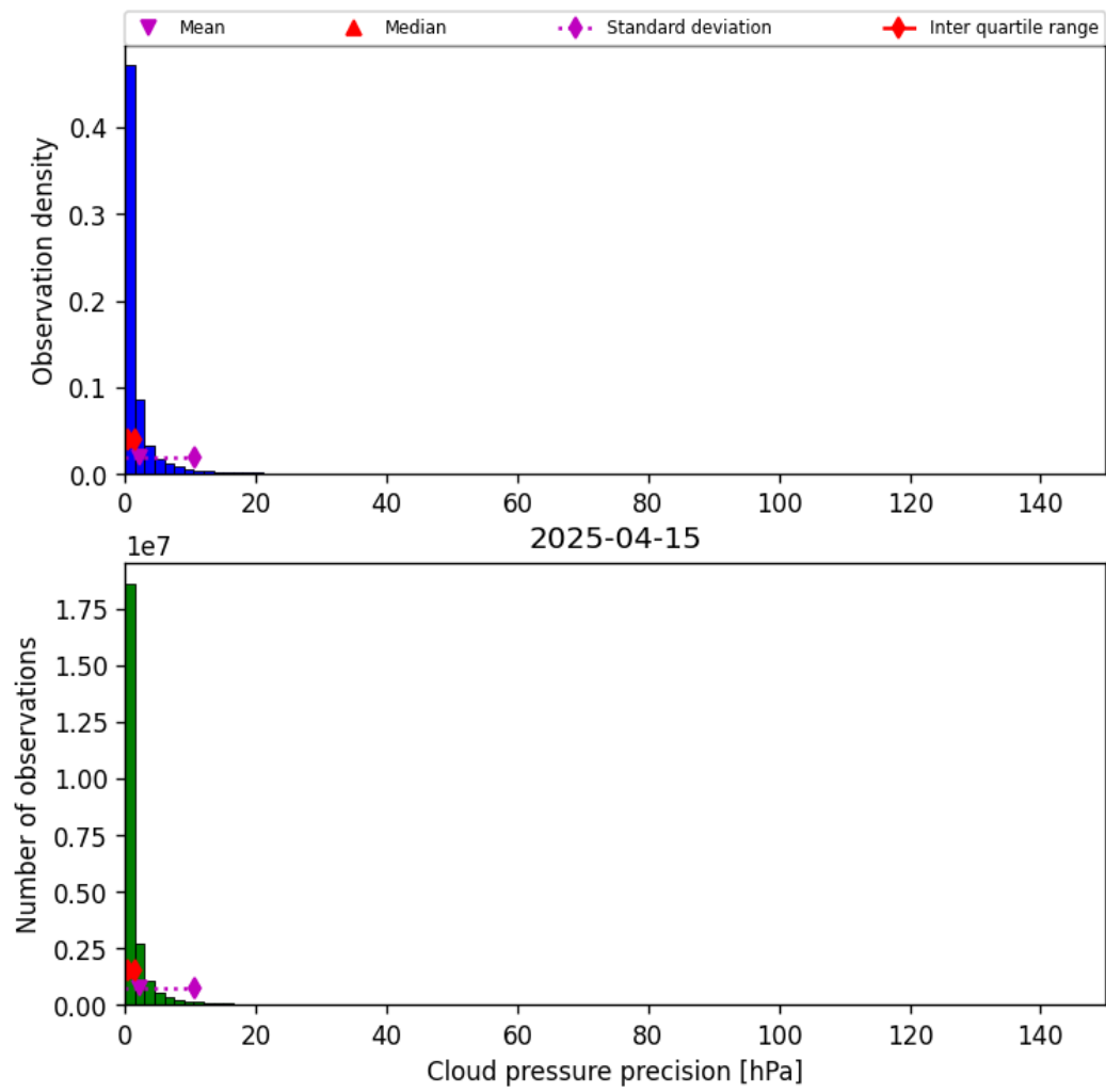
Figure 31: Histogram of “Cloud pressure precision” for 2025-04-14 to 2025-04-16
