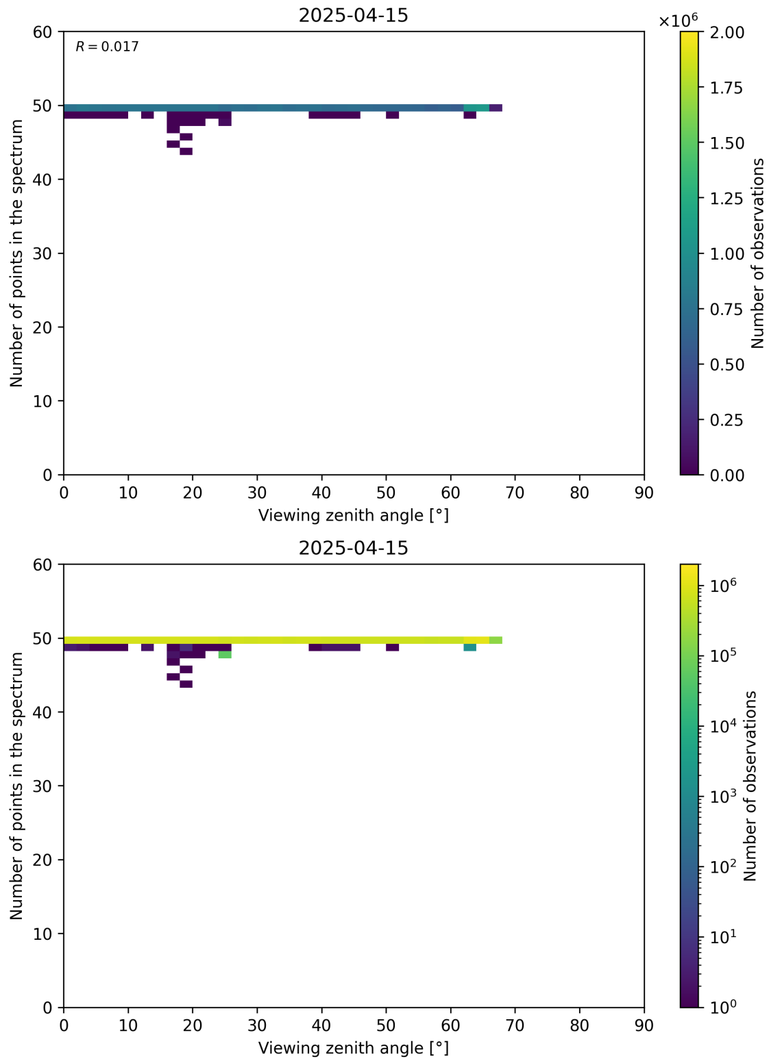
Figure 125: Scatter density plot of “Viewing zenith angle” against “Number of points in the spectrum” for 2025-04-14 to 2025-04-16.
