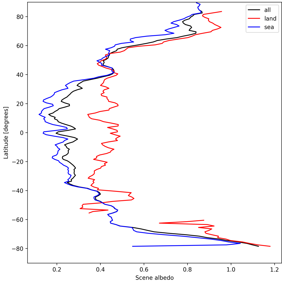
Figure 17: Zonal average of “Scene albedo” for 2025-04-14 to 2025-04-16.
