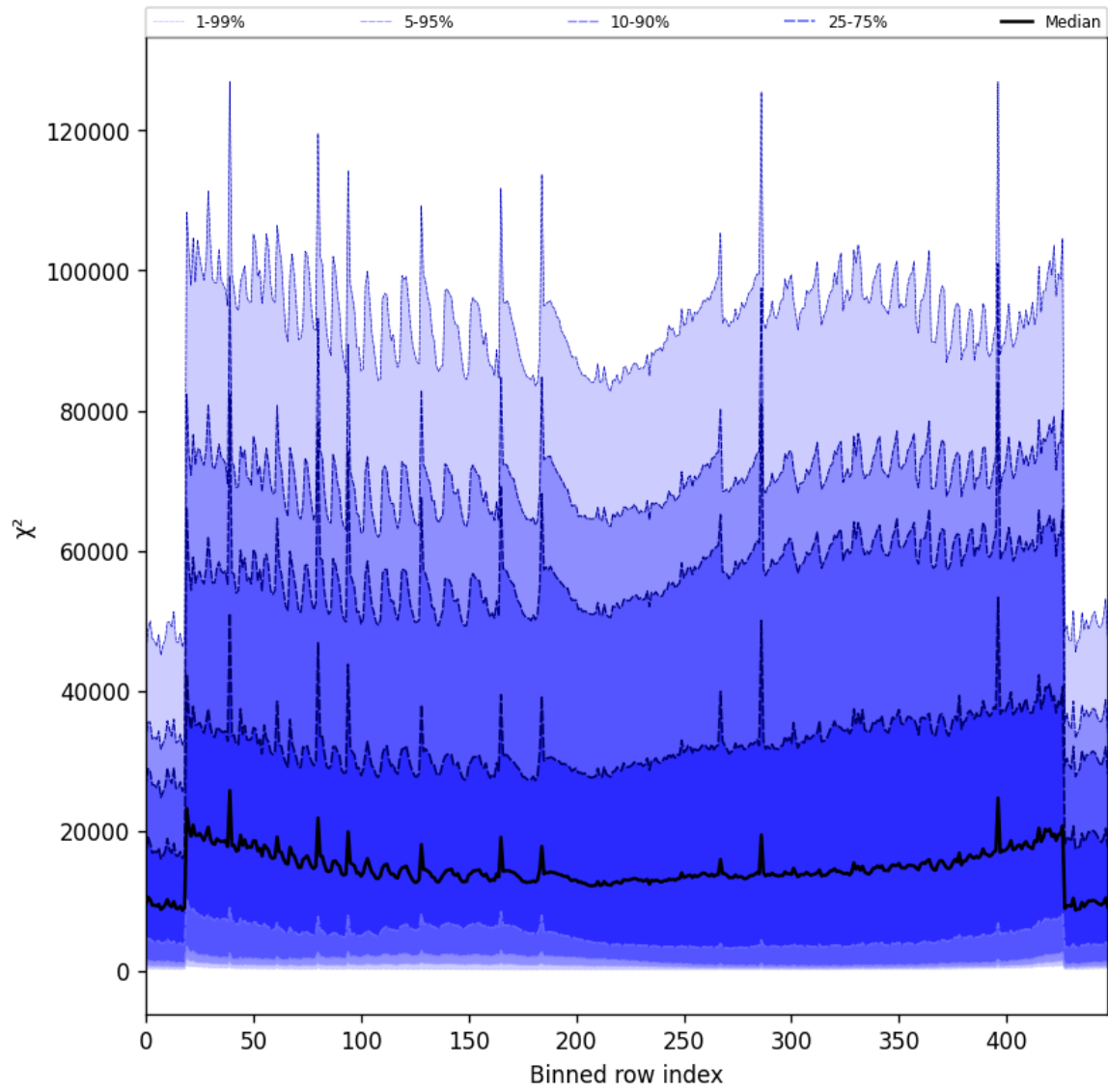
Figure 55: Along track statistics of “ \chi^2 ” for 2025-04-14 to 2025-04-16
