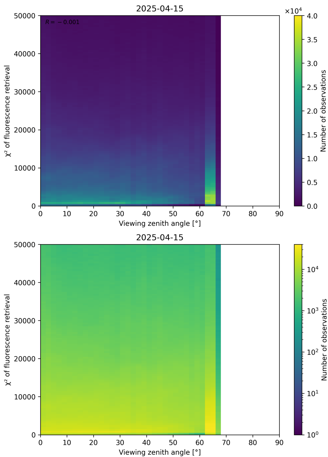
Figure 119: Scatter density plot of “Viewing zenith angle” against “ \chi^2 of fluorescence retrieval” for 2025-04-14 to 2025-04-16.
