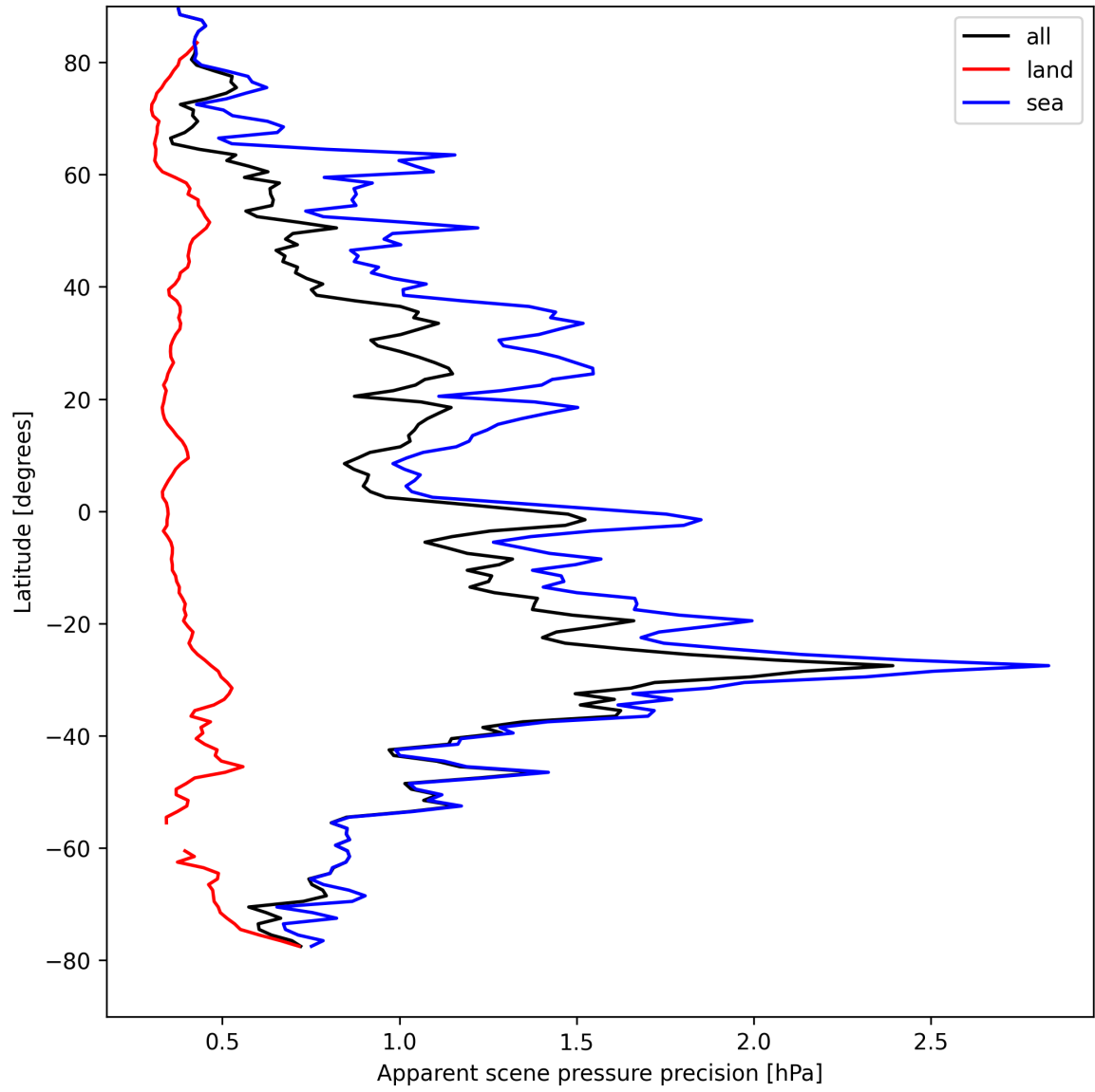
Figure 20: Zonal average of “Apparent scene pressure precision” for 2025-04-15 to 2025-04-17.
