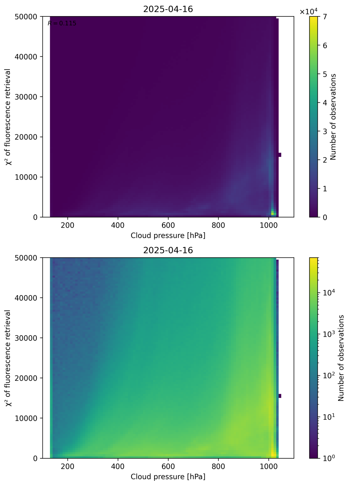
Figure 78: Scatter density plot of “Cloud pressure” against “ \chi^2 of fluorescence retrieval” for 2025-04-15 to 2025-04-17.
