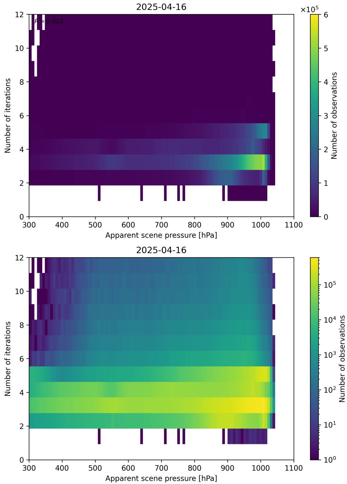
Figure 65: Scatter density plot of “Apparent scene pressure” against “Number of iterations” for 2025-04-15 to 2025-04-17.
