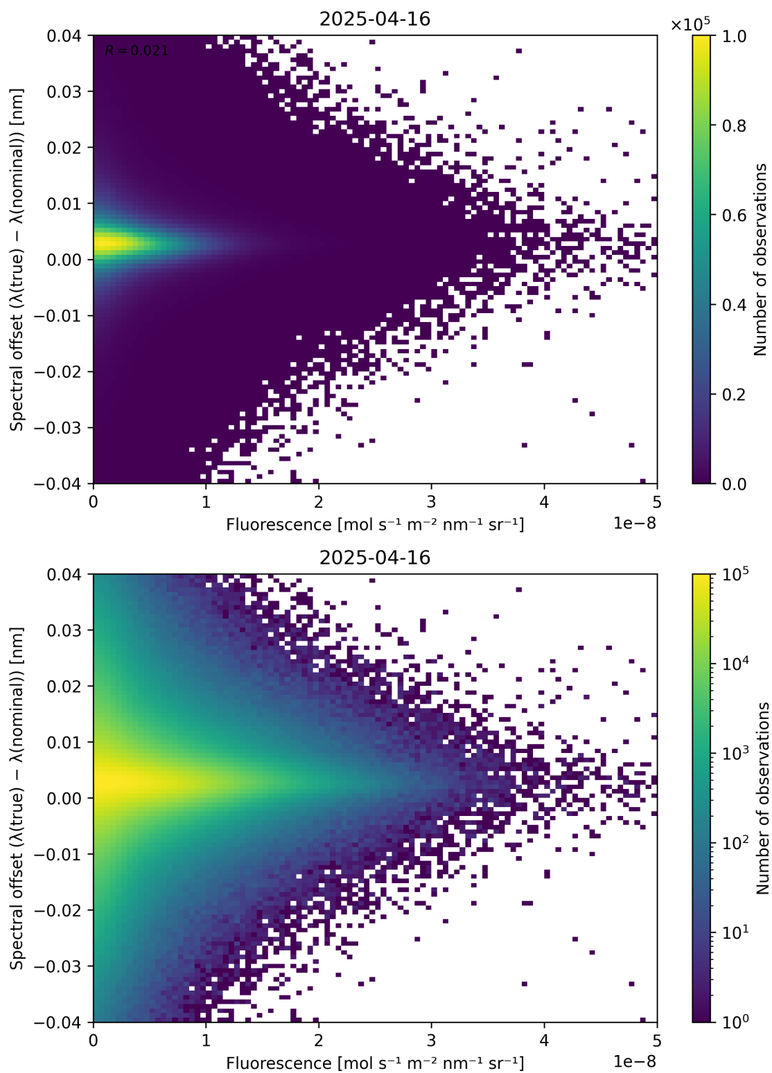
Figure 87: Scatter density plot of “Fluorescence” against “Spectral offset ( \lambda_{\text{true}} - \lambda_{\text{nominal}} )” for 2025-04-15 to 2025-04-17.
