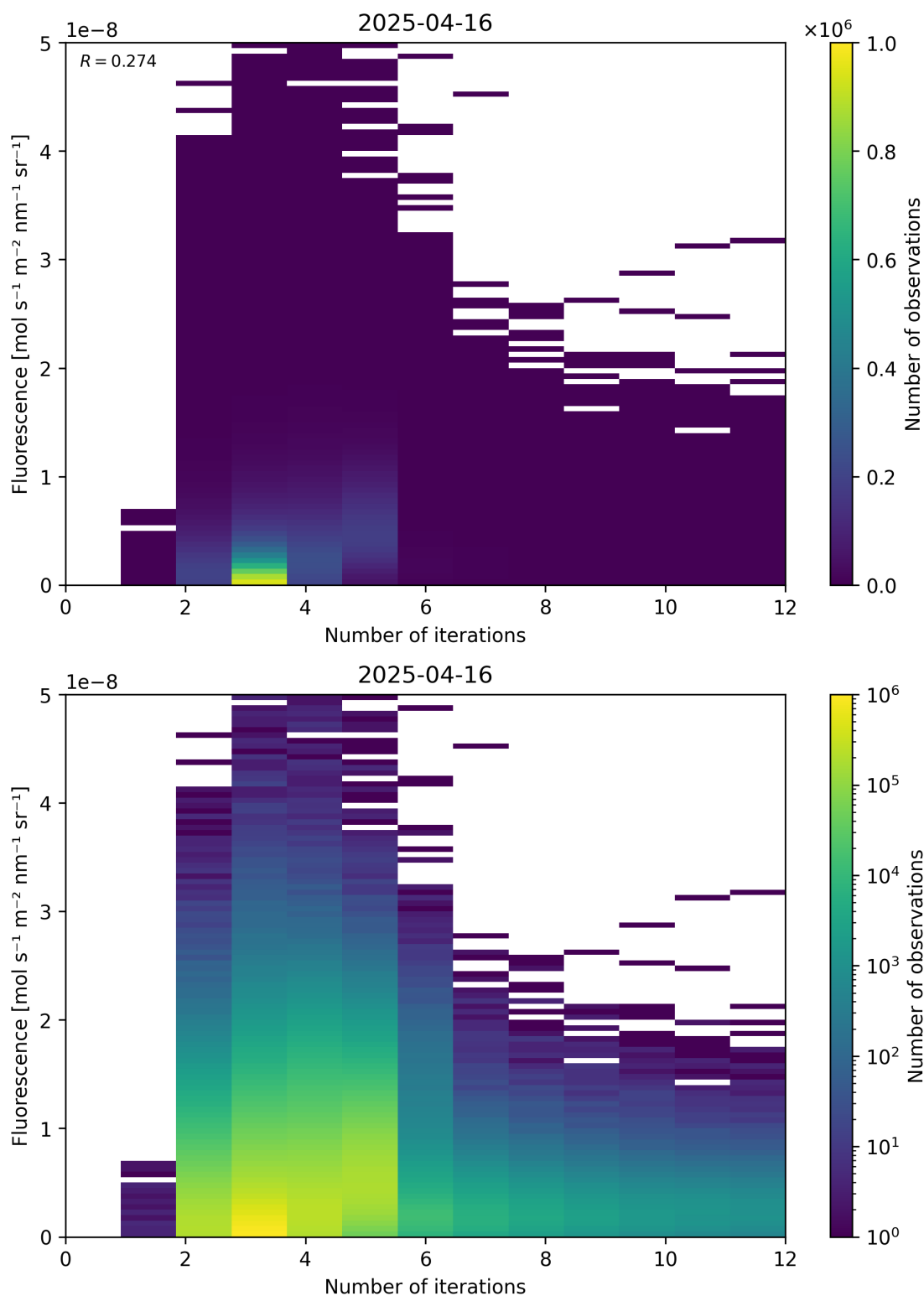
Figure 98: Scatter density plot of “Number of iterations” against “Fluorescence” for 2025-04-15 to 2025-04-17.
