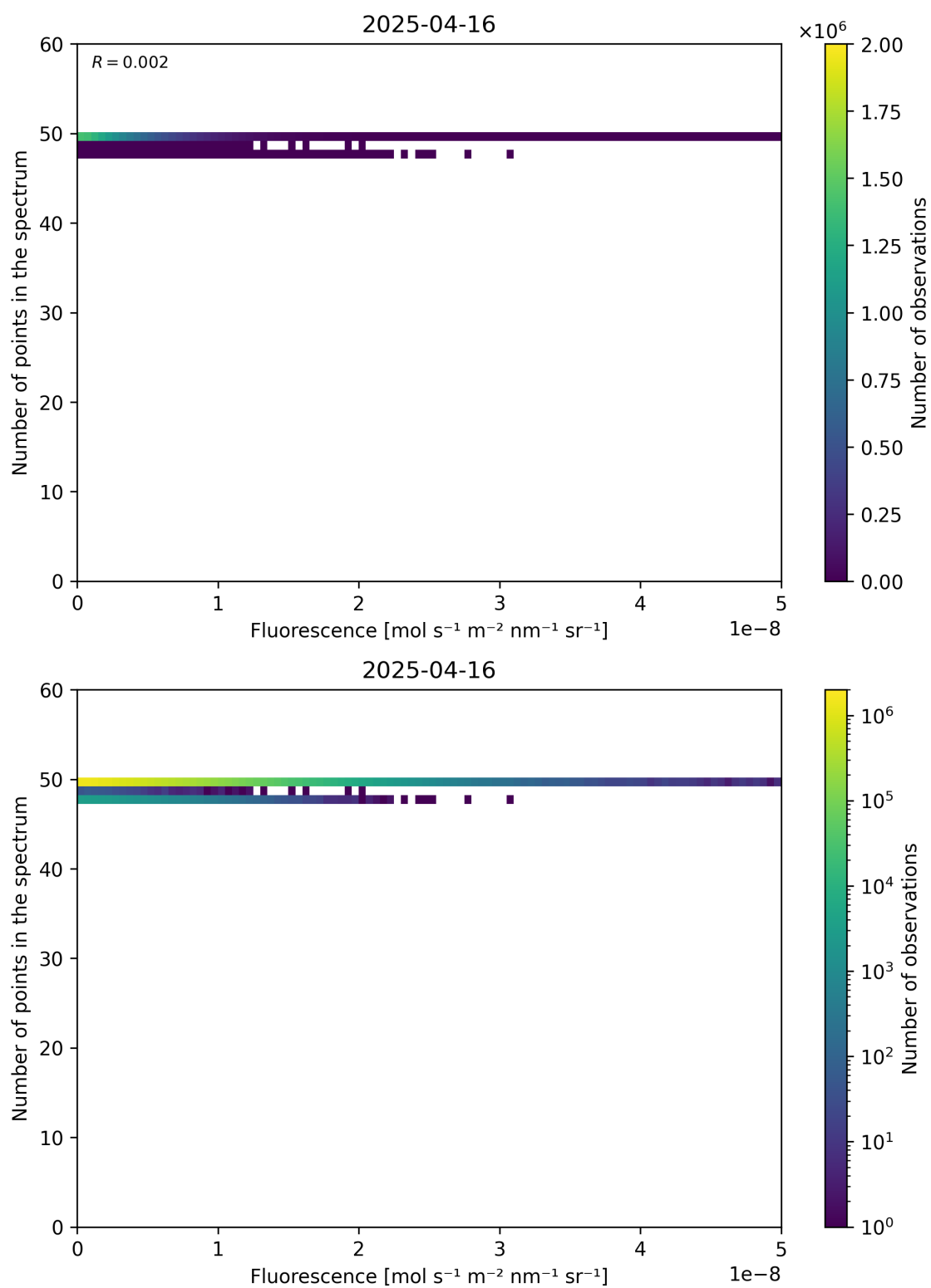
Figure 86: Scatter density plot of “Fluorescence” against “Number of points in the spectrum” for 2025-04-15 to 2025-04-17.
