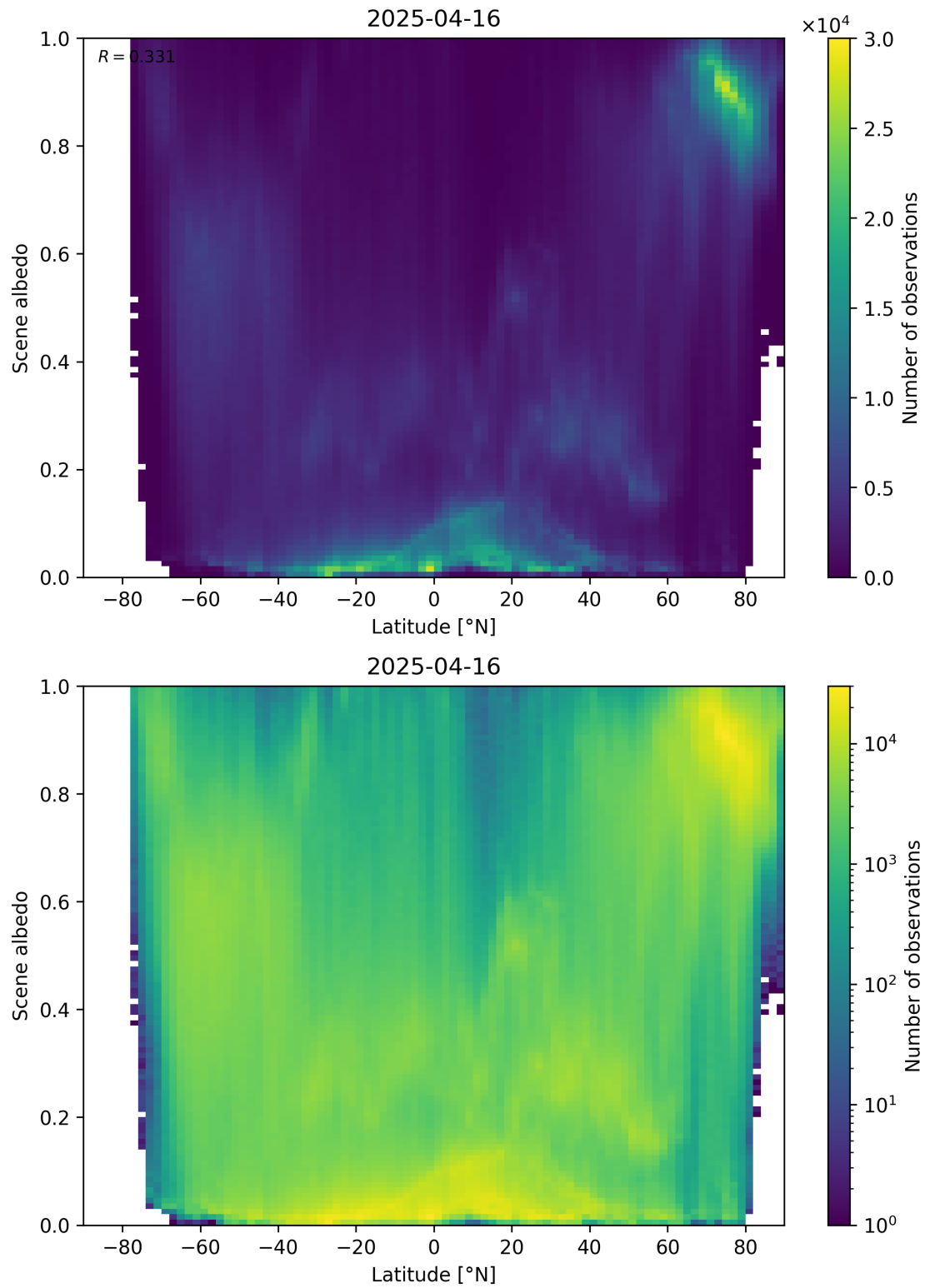
Figure 95: Scatter density plot of “Latitude” against “Scene albedo” for 2025-04-15 to 2025-04-17.
