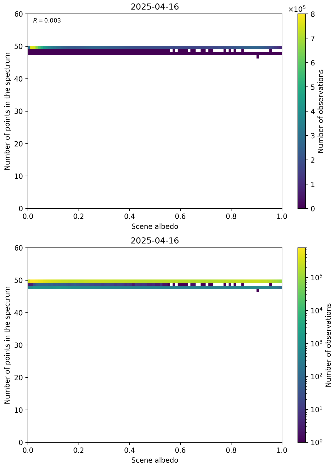
Figure 106: Scatter density plot of “Scene albedo” against “Number of points in the spectrum” for 2025-04-15 to 2025-04-17.
