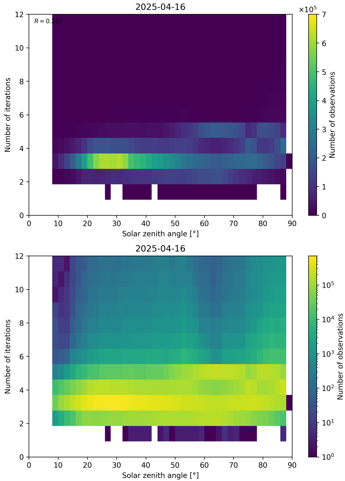
Figure 114: Scatter density plot of “Solar zenith angle” against “Number of iterations” for 2025-04-15 to 2025-04-17.
