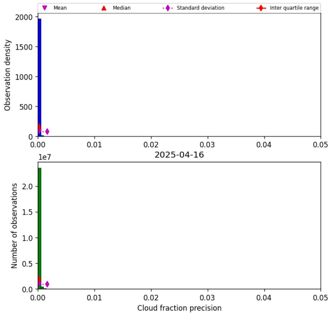
Figure 33: Histogram of “Cloud fraction precision” for 2025-04-15 to 2025-04-17
