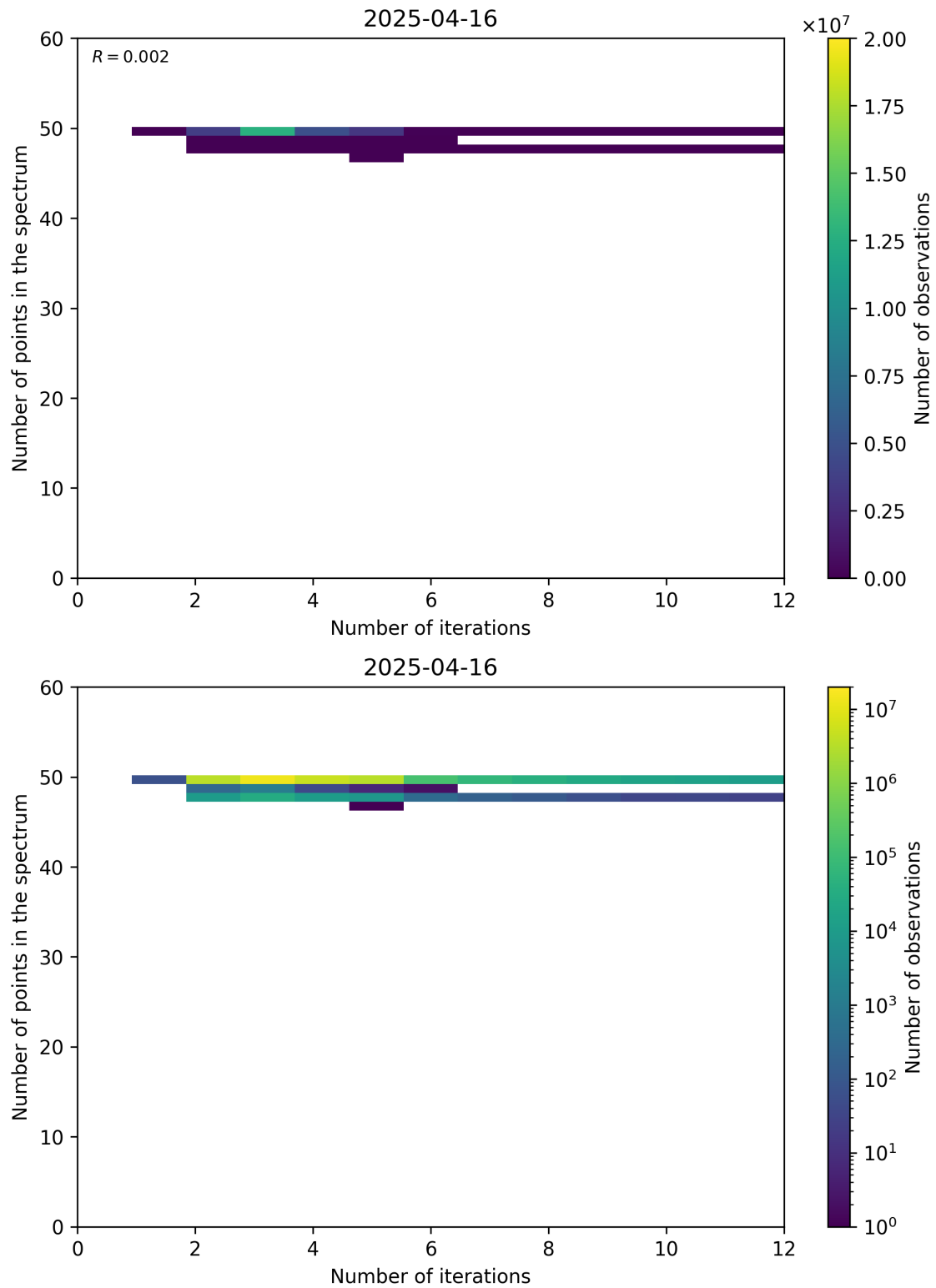
Figure 99: Scatter density plot of “Number of iterations” against “Number of points in the spectrum” for 2025-04-15 to 2025-04-17.
