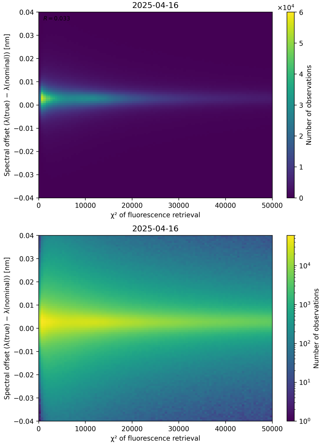
Figure 69: Scatter density plot of “ \chi^2 of fluorescence retrieval” against “Spectral offset ( \lambda_{\text{true}} - \lambda_{\text{nominal}} )” for 2025-04-15 to 2025-04-17.
