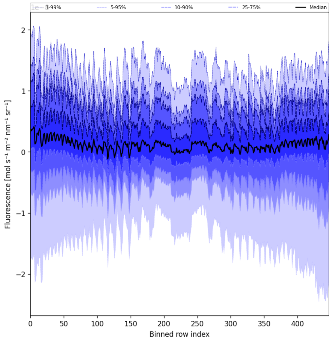
Figure 57: Along track statistics of “Fluorescence” for 2025-04-15 to 2025-04-17
