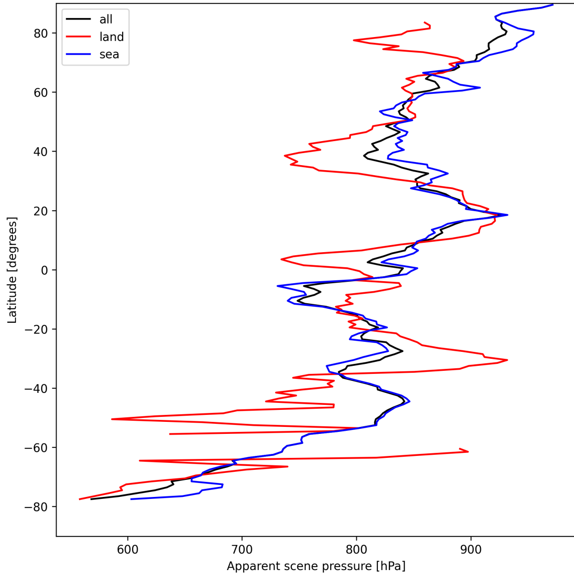
Figure 19: Zonal average of “Apparent scene pressure” for 2025-04-15 to 2025-04-17.
