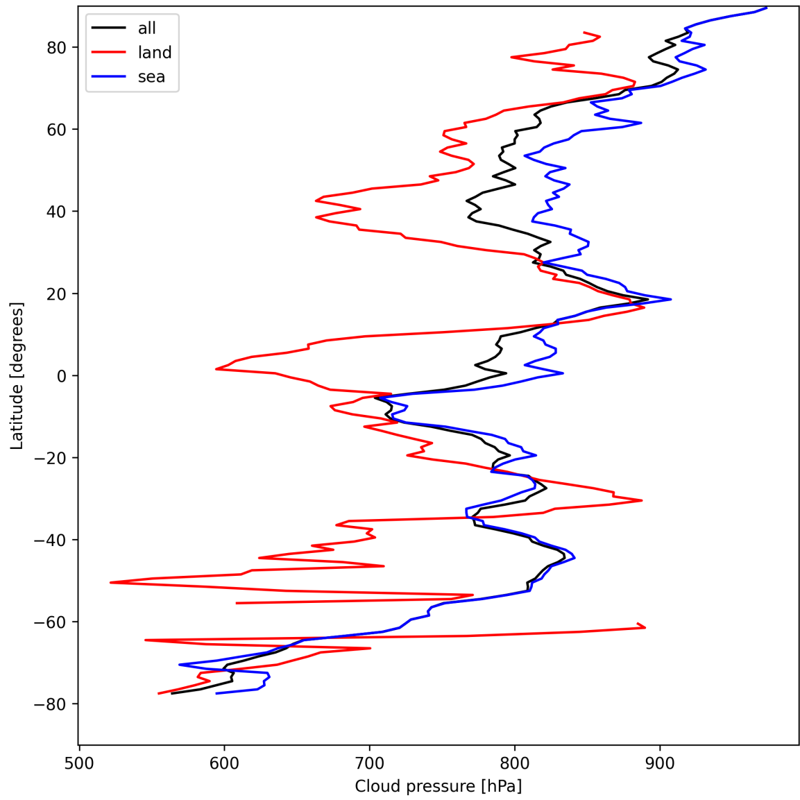
Figure 13: Zonal average of “Cloud pressure” for 2025-04-15 to 2025-04-17.
