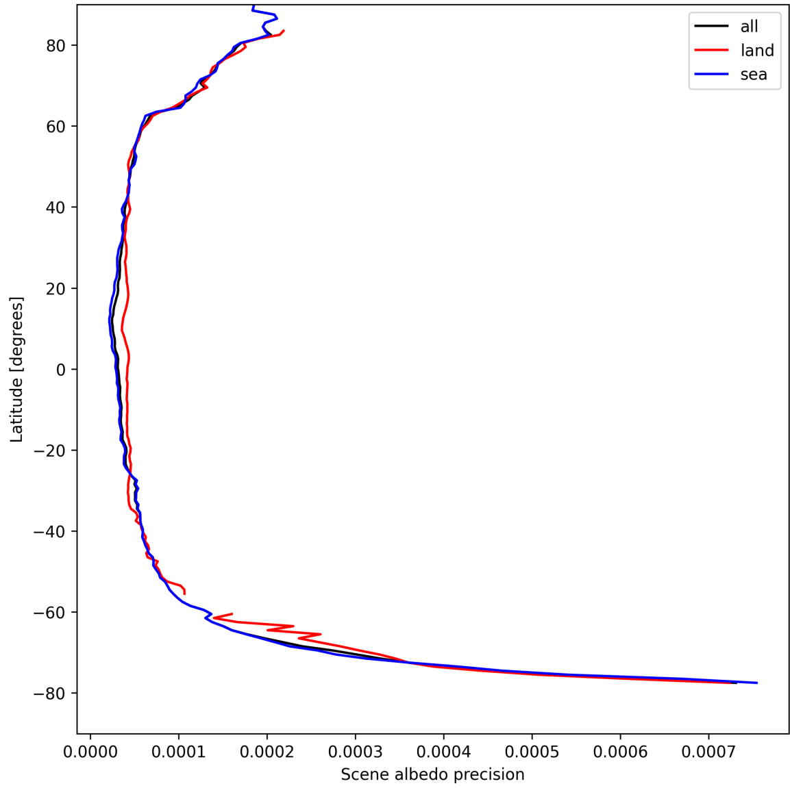
Figure 18: Zonal average of “Scene albedo precision” for 2025-04-15 to 2025-04-17.
