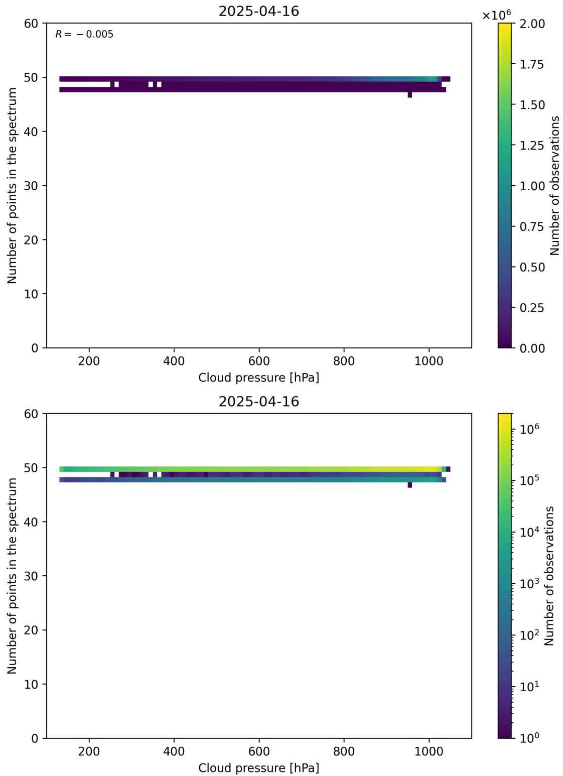
Figure 82: Scatter density plot of “Cloud pressure” against “Number of points in the spectrum” for 2025-04-15 to 2025-04-17.
