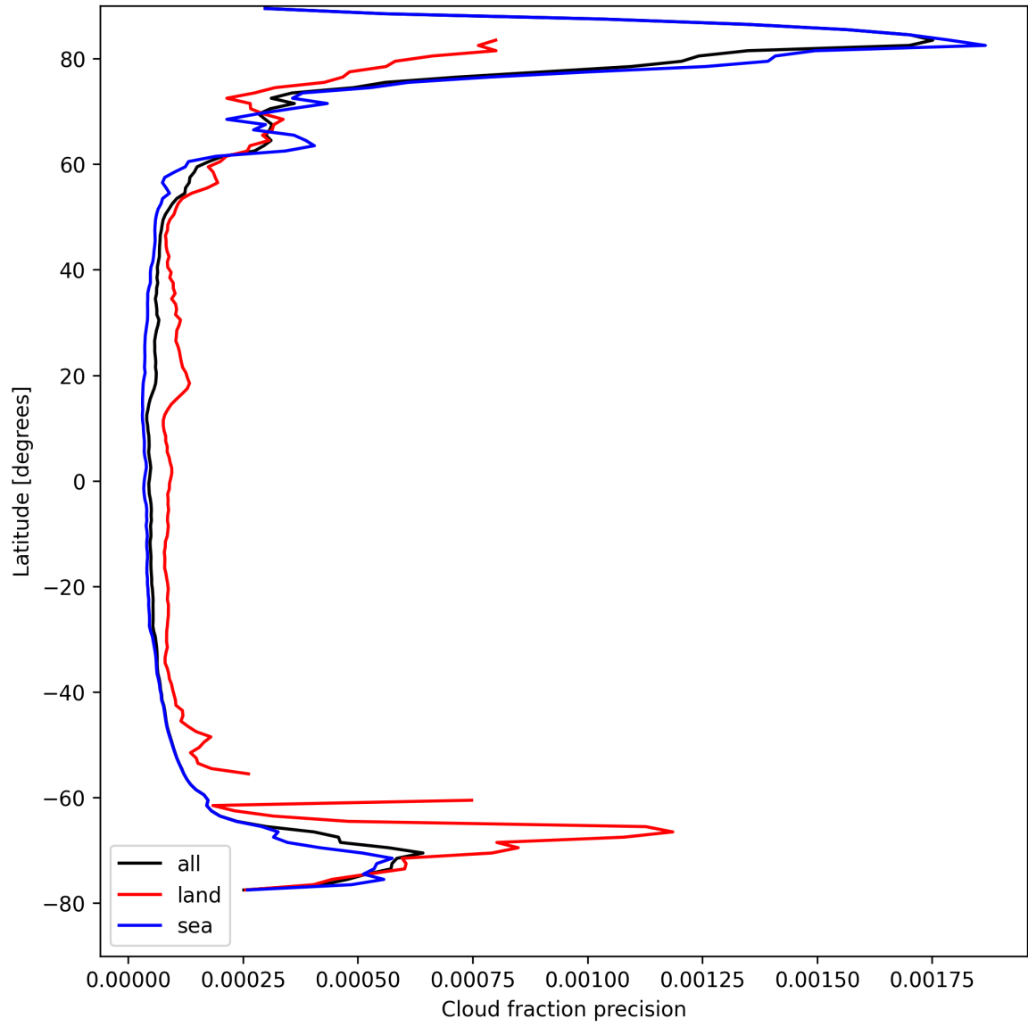
Figure 16: Zonal average of “Cloud fraction precision” for 2025-04-15 to 2025-04-17.
