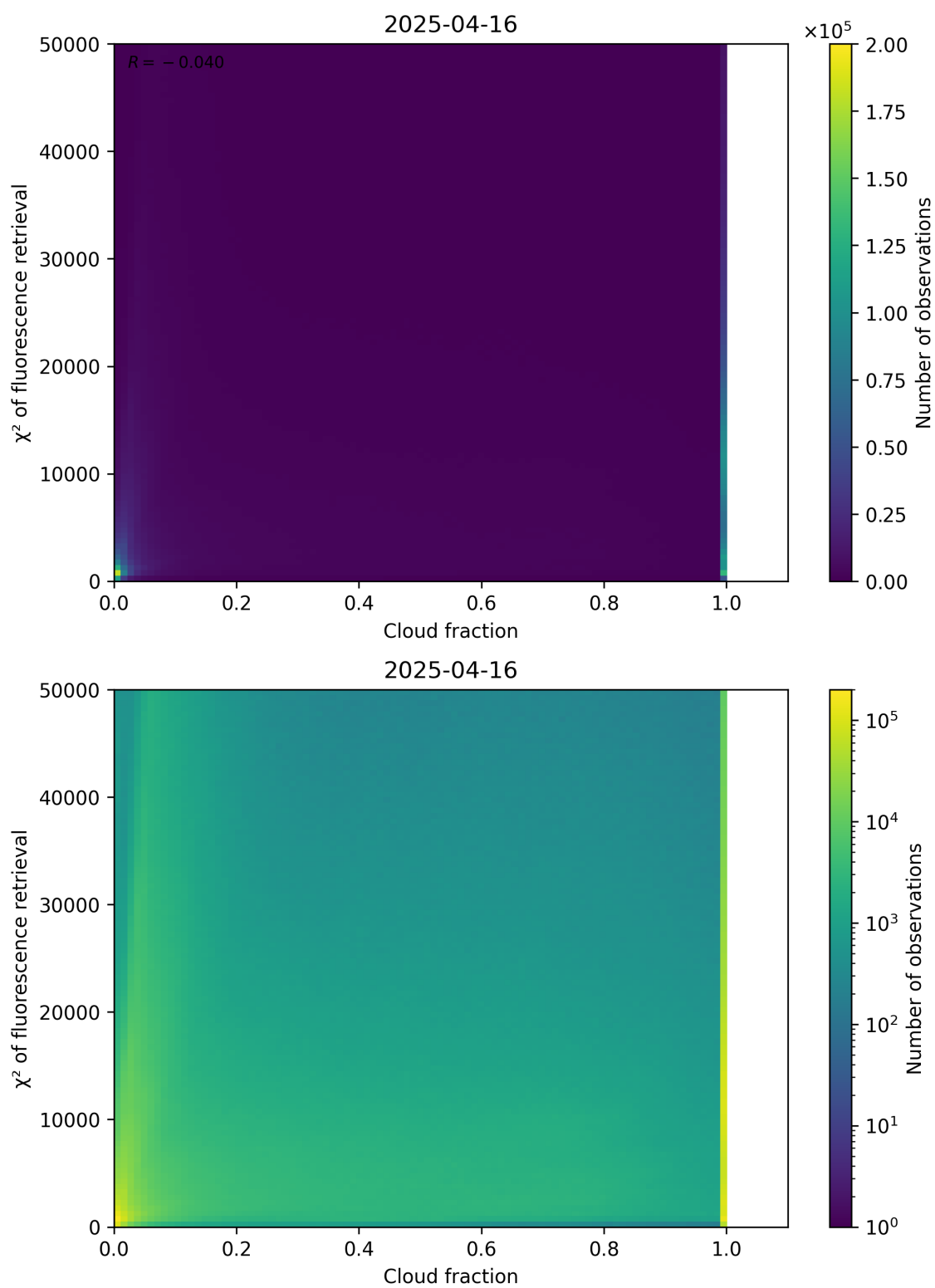
Figure 71: Scatter density plot of “Cloud fraction” against “ \chi^2 of fluorescence retrieval” for 2025-04-15 to 2025-04-17.
