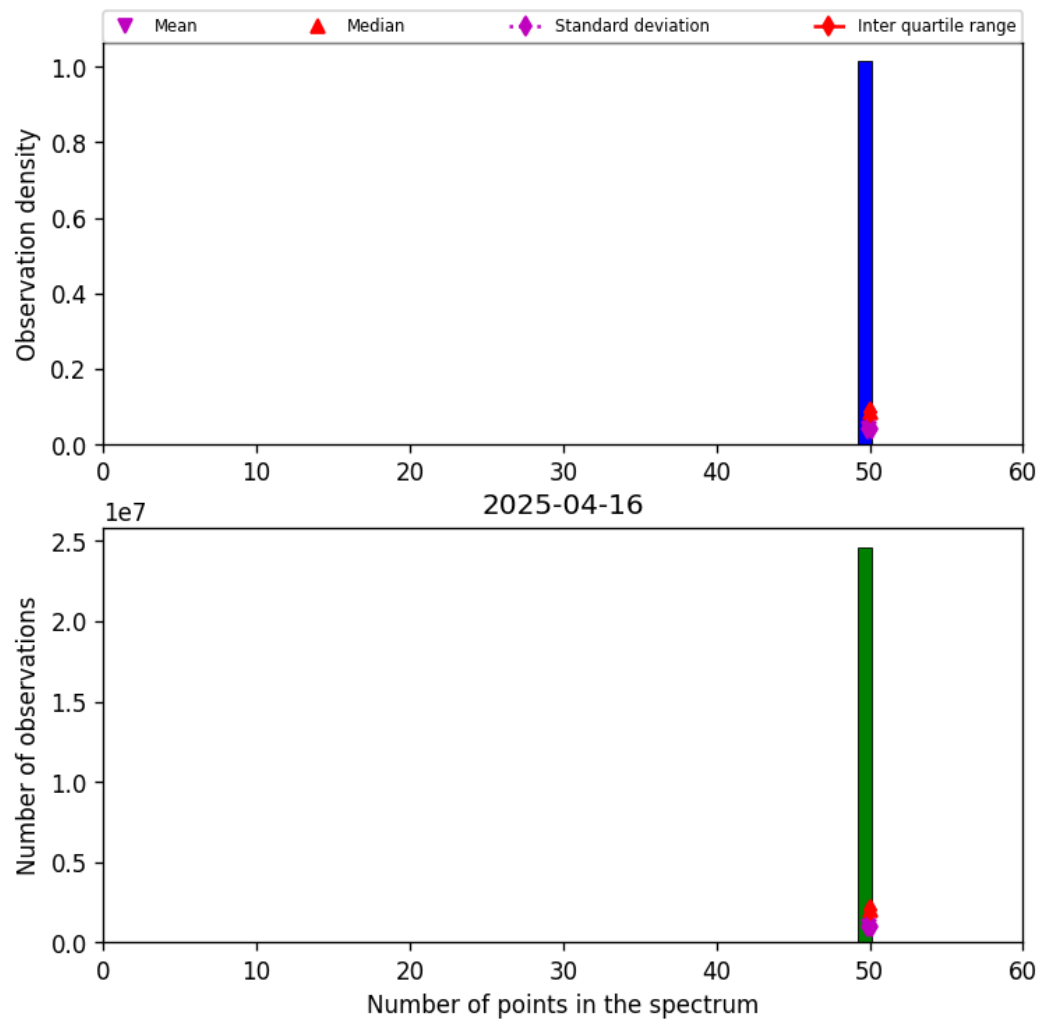
Figure 44: Histogram of “Number of points in the spectrum” for 2025-04-15 to 2025-04-17
