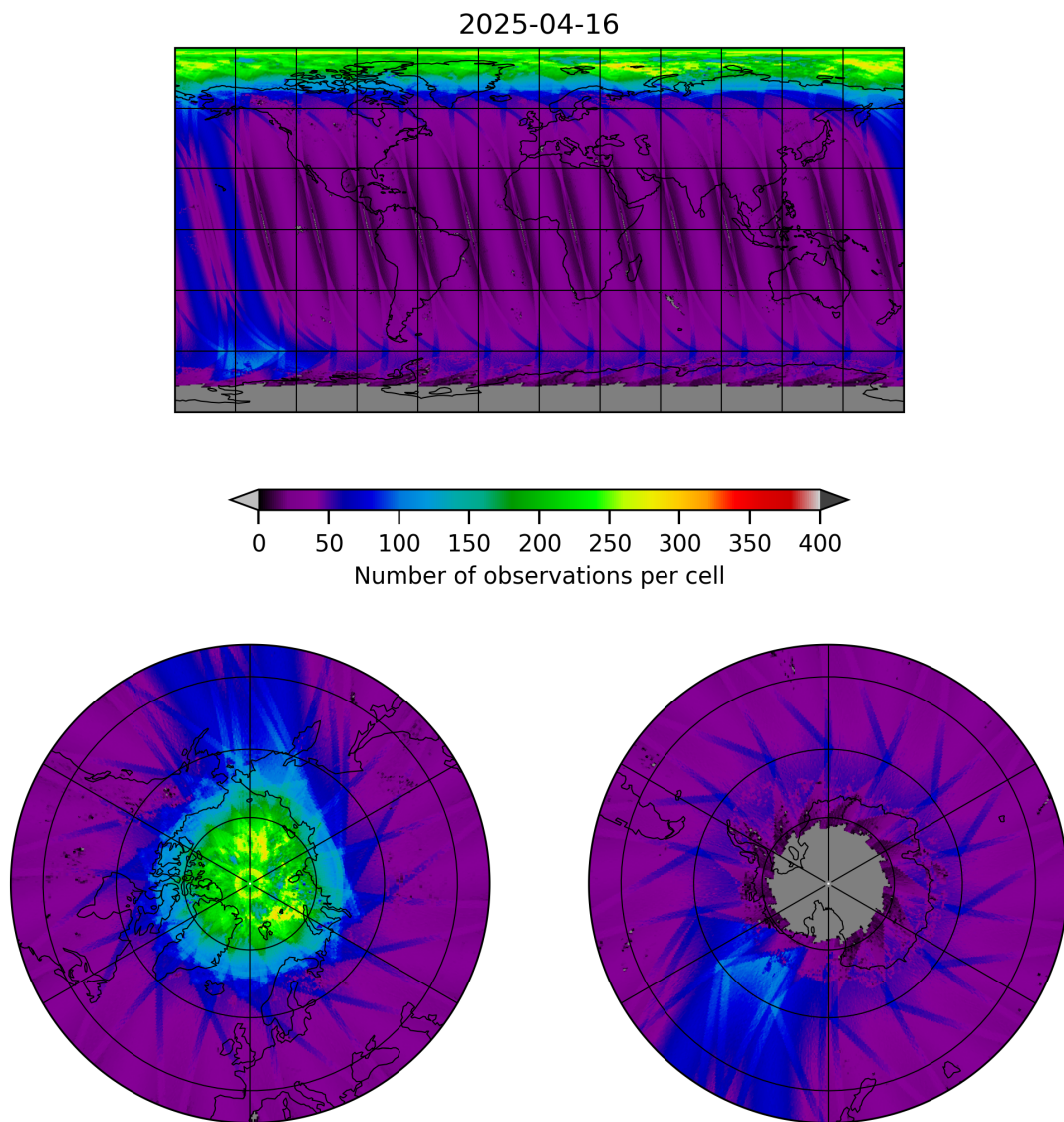
Figure 11: Map of the number of observations for 2025-04-15 to 2025-04-17
