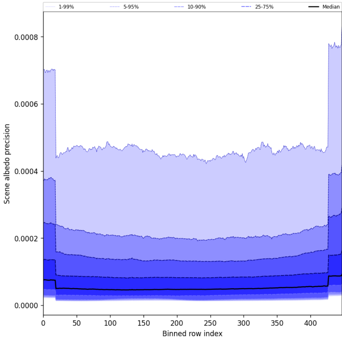
Figure 52: Along track statistics of “Scene albedo precision” for 2025-04-15 to 2025-04-17
