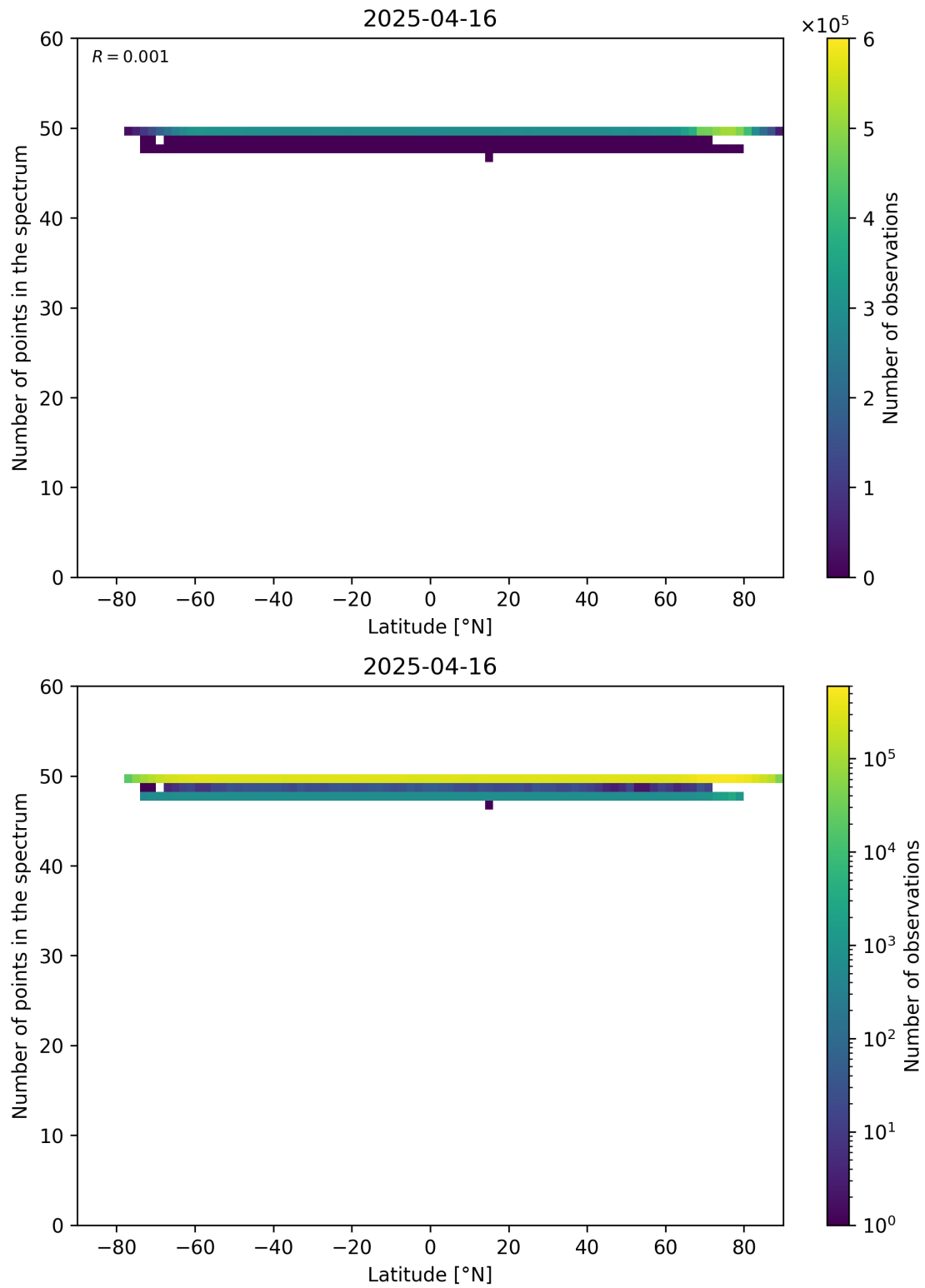
Figure 94: Scatter density plot of “Latitude” against “Number of points in the spectrum” for 2025-04-15 to 2025-04-17.
