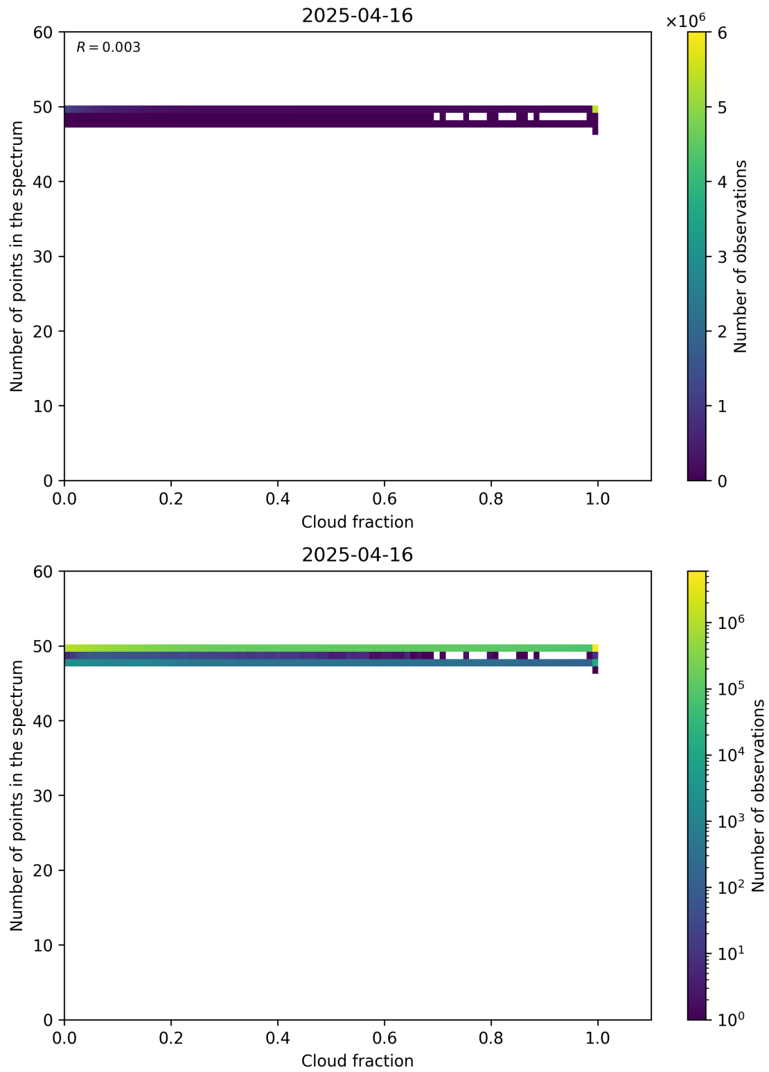
Figure 74: Scatter density plot of “Cloud fraction” against “Number of points in the spectrum” for 2025-04-15 to 2025-04-17.
