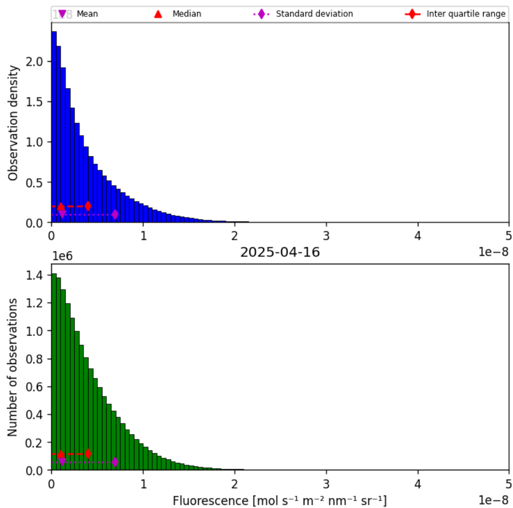
Figure 40: Histogram of “Fluorescence” for 2025-04-15 to 2025-04-17
