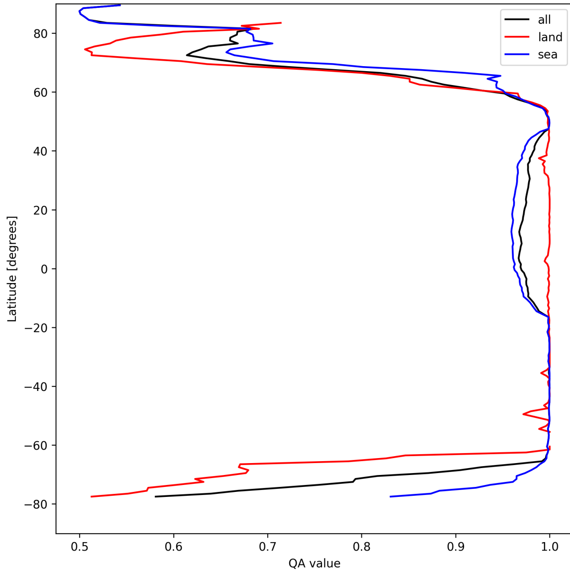
Figure 12: Zonal average of “QA value” for 2025-04-15 to 2025-04-17.
