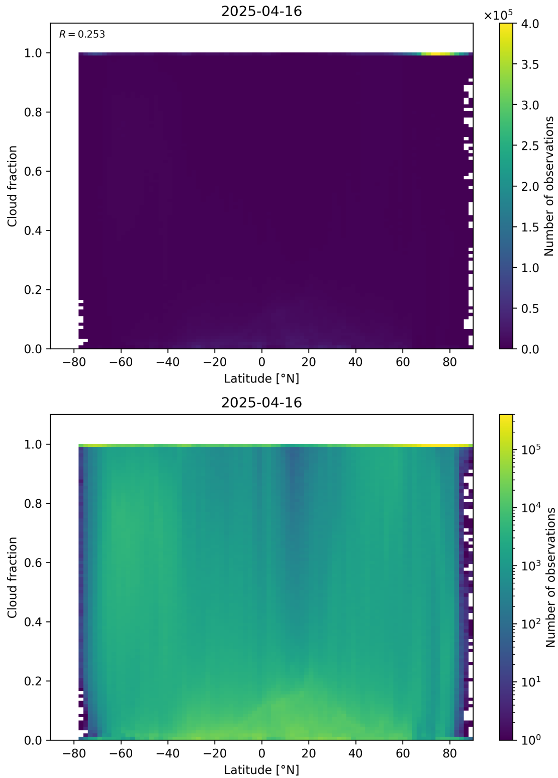
Figure 90: Scatter density plot of “Latitude” against “Cloud fraction” for 2025-04-15 to 2025-04-17.
