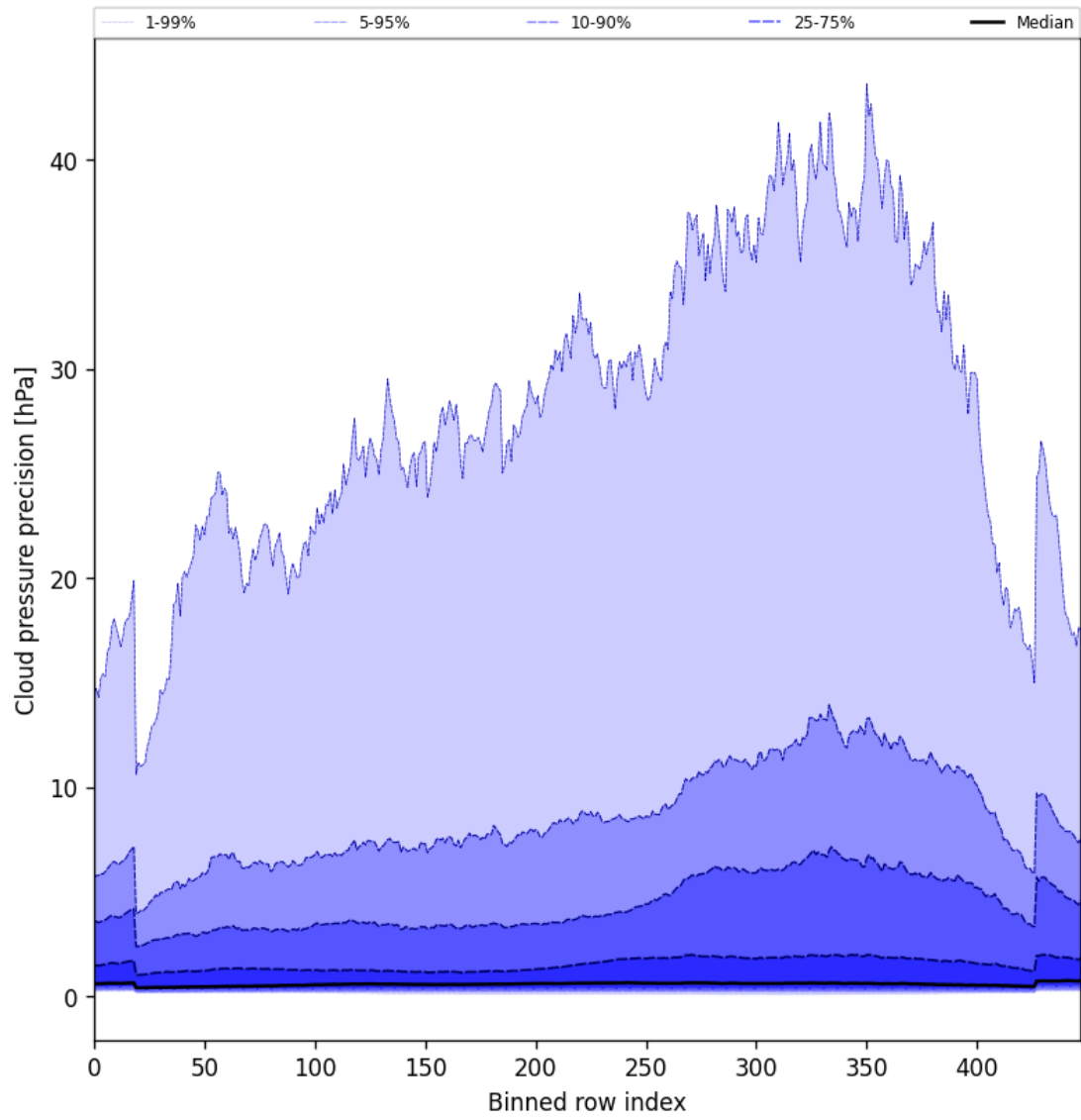
Figure 48: Along track statistics of “Cloud pressure precision” for 2025-04-15 to 2025-04-17
