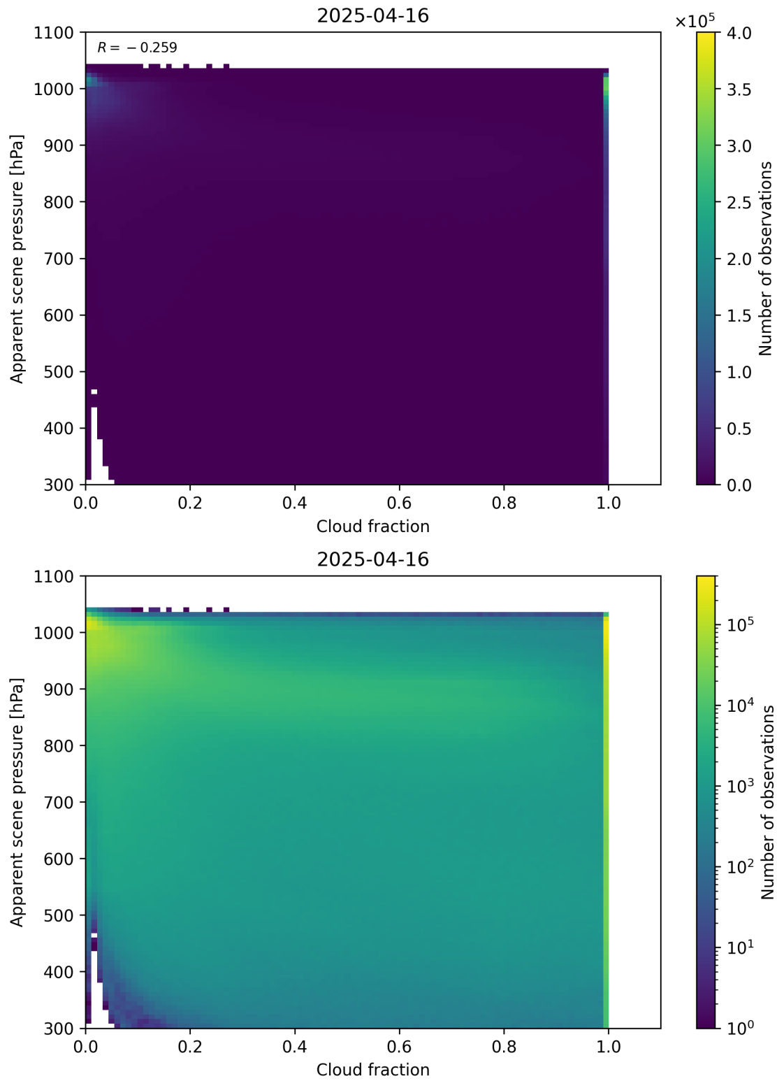
Figure 70: Scatter density plot of “Cloud fraction” against “Apparent scene pressure” for 2025-04-15 to 2025-04-17.
