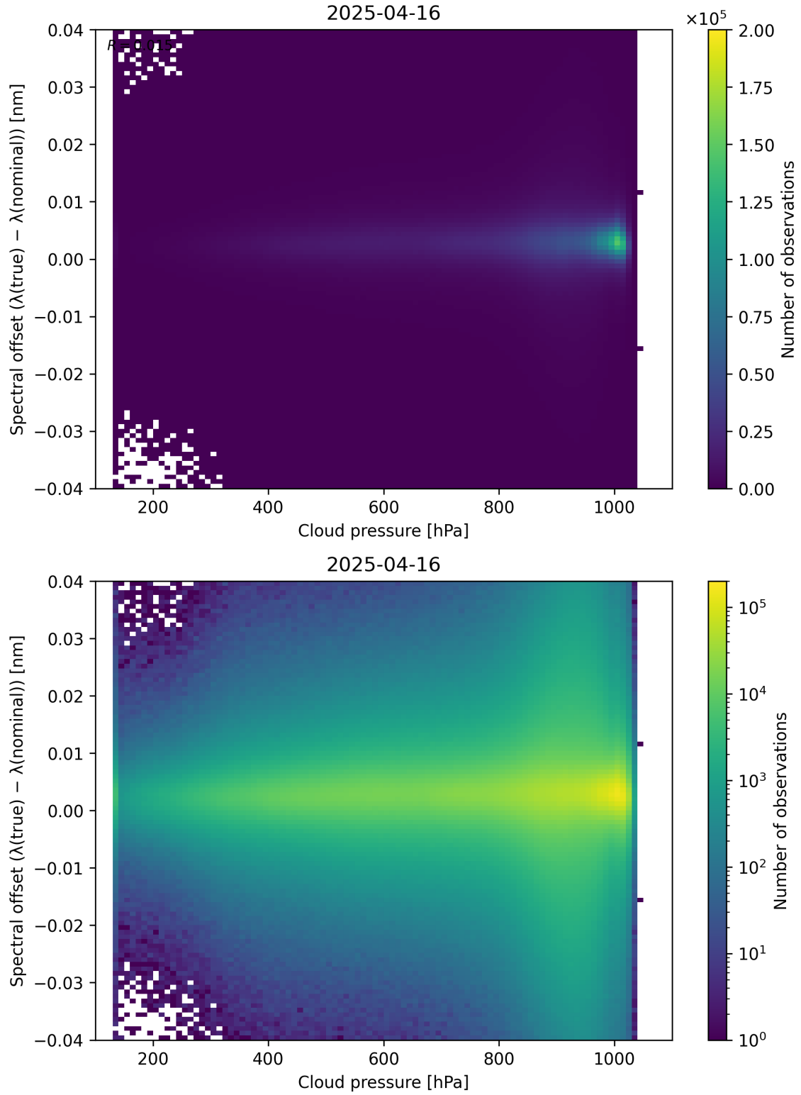
Figure 84: Scatter density plot of “Cloud pressure” against “Spectral offset ( \lambda_{\text{true}} - \lambda_{\text{nominal}} )” for 2025-04-15 to 2025-04-17.
