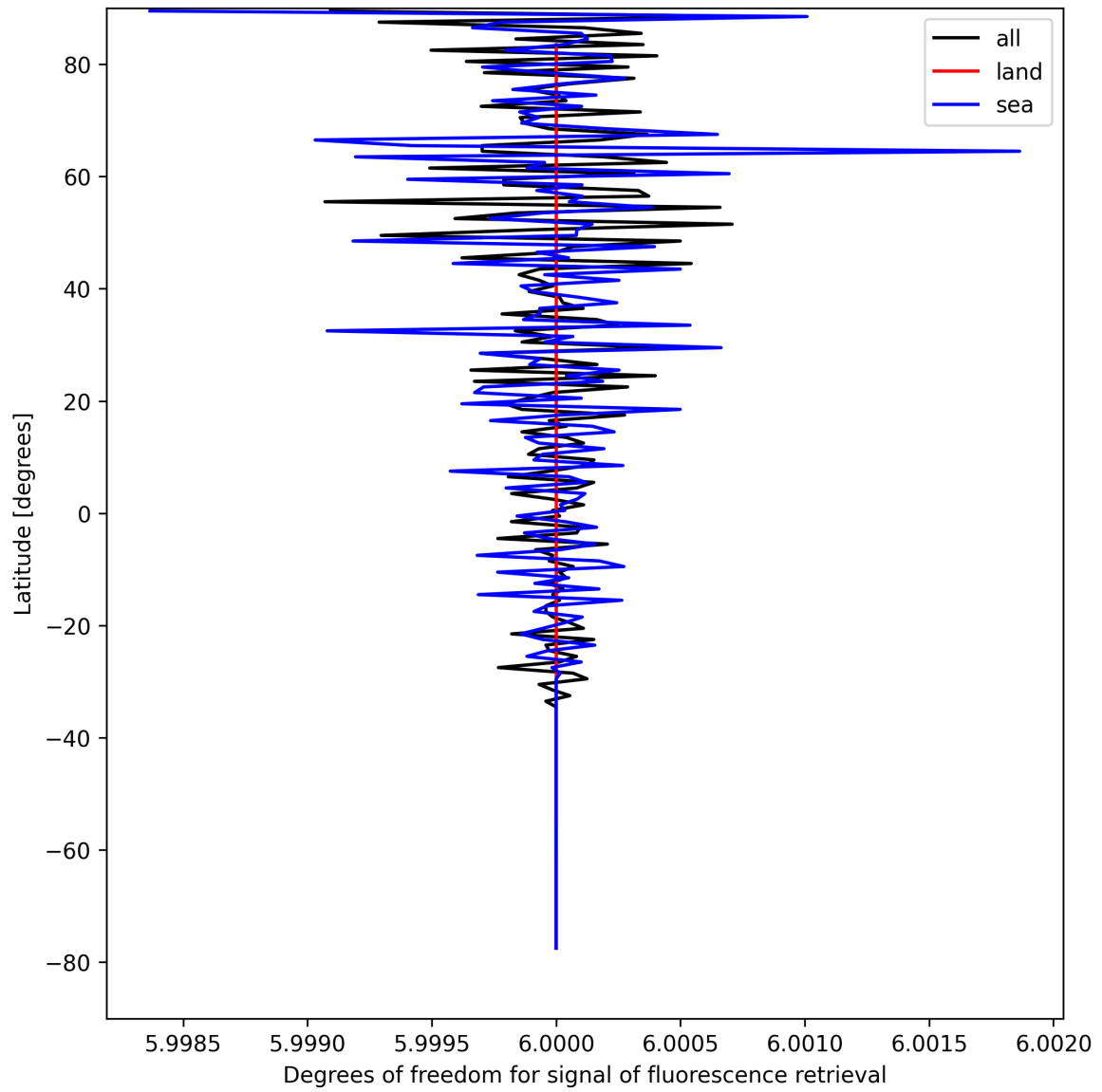
Figure 26: Zonal average of “Degrees of freedom for signal of fluorescence retrieval” for 2025-04-15 to 2025-04-17.
