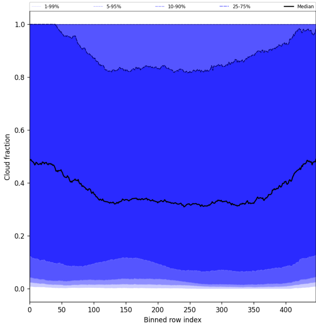
Figure 49: Along track statistics of “Cloud fraction” for 2025-04-15 to 2025-04-17
