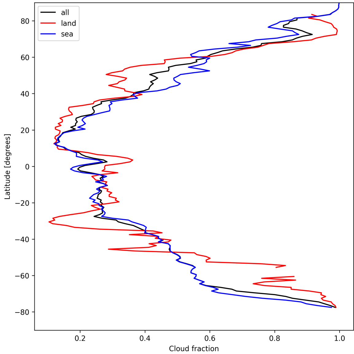
Figure 15: Zonal average of “Cloud fraction” for 2025-04-15 to 2025-04-17.
