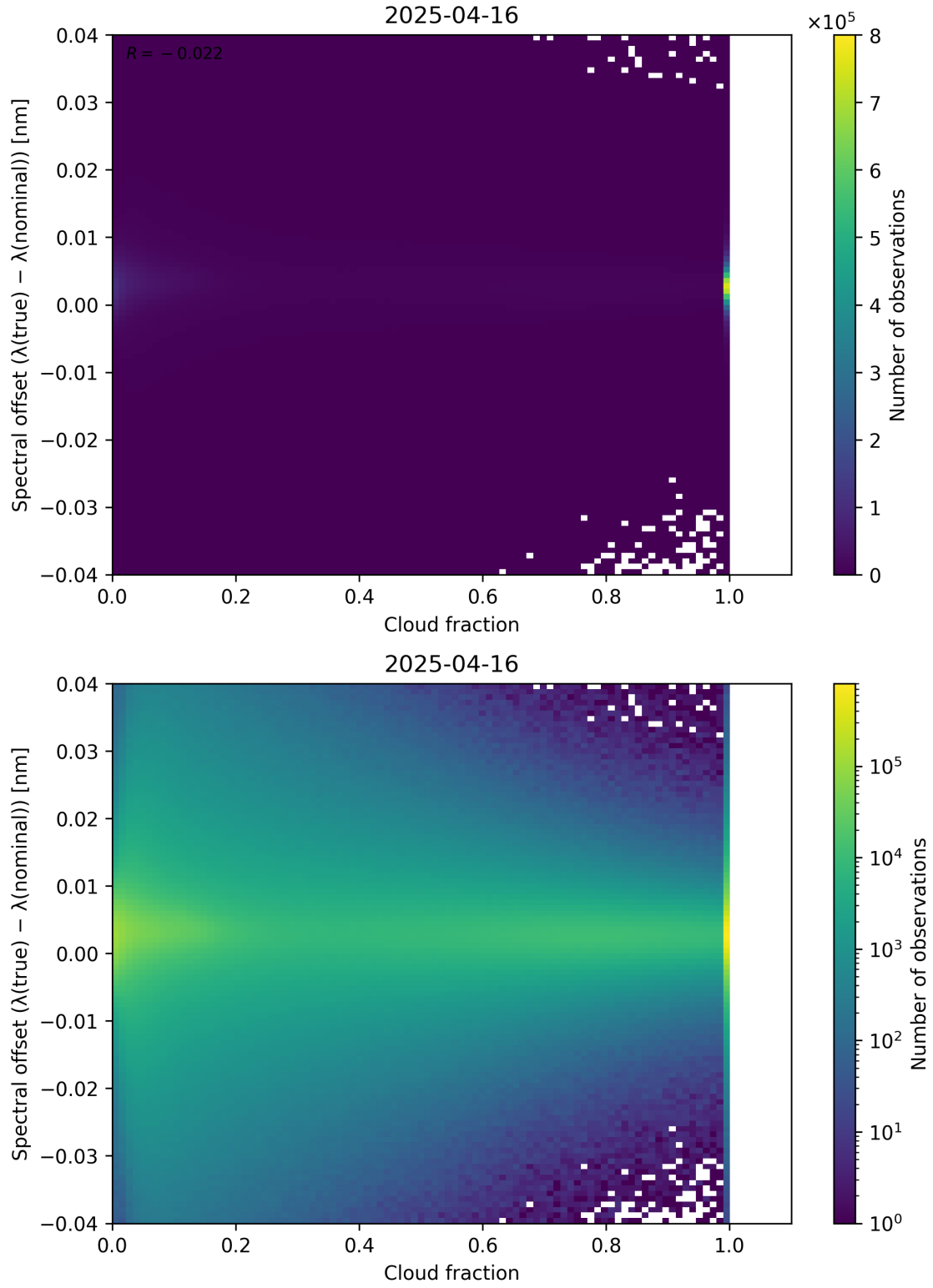
Figure 76: Scatter density plot of “Cloud fraction” against “Spectral offset ( \lambda_{\text{true}} - \lambda_{\text{nominal}} )” for 2025-04-15 to 2025-04-17.
