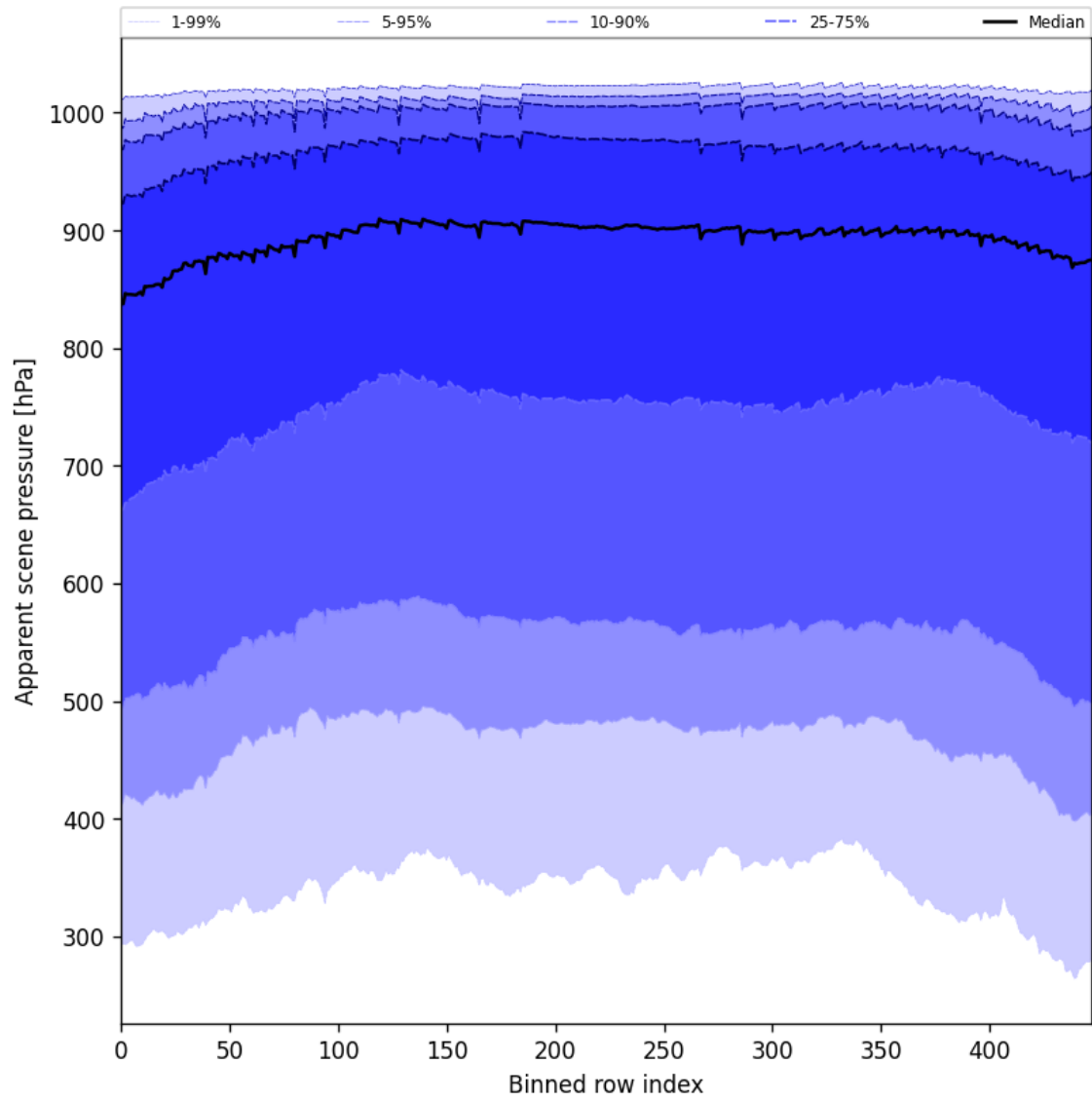
Figure 53: Along track statistics of “Apparent scene pressure” for 2025-04-15 to 2025-04-17
