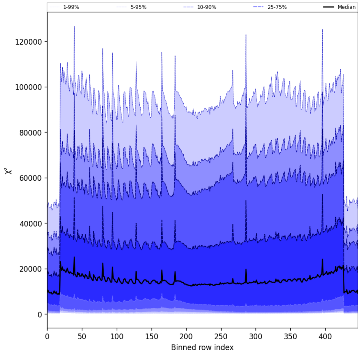
Figure 55: Along track statistics of “ \chi^2 ” for 2025-04-15 to 2025-04-17
