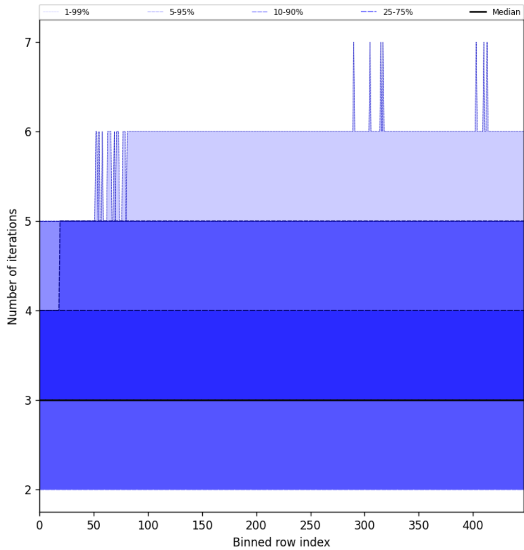
Figure 56: Along track statistics of “Number of iterations” for 2025-04-15 to 2025-04-17
