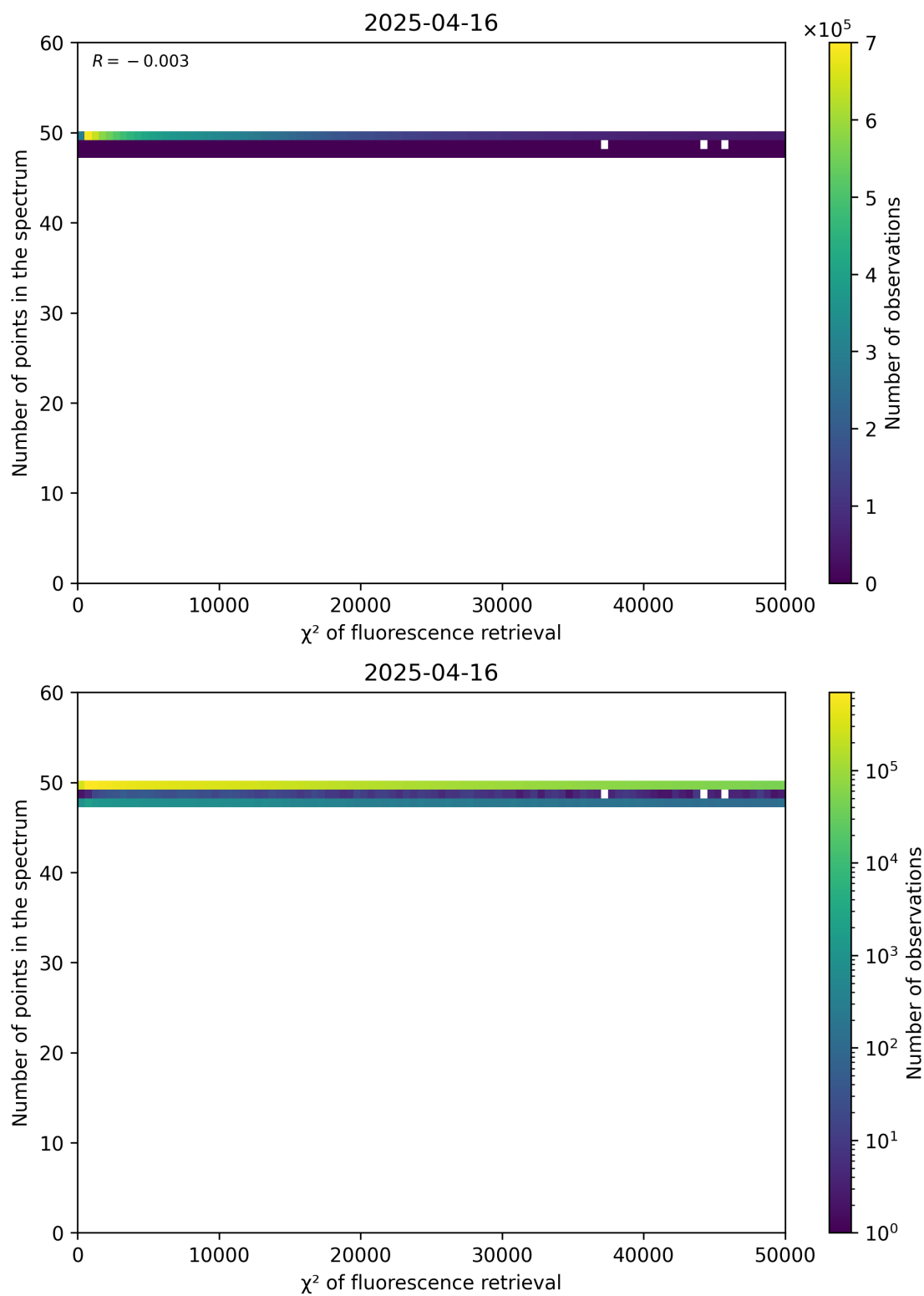
Figure 68: Scatter density plot of " \chi^2 of fluorescence retrieval" against "Number of points in the spectrum" for 2025-04-15 to 2025-04-17.
