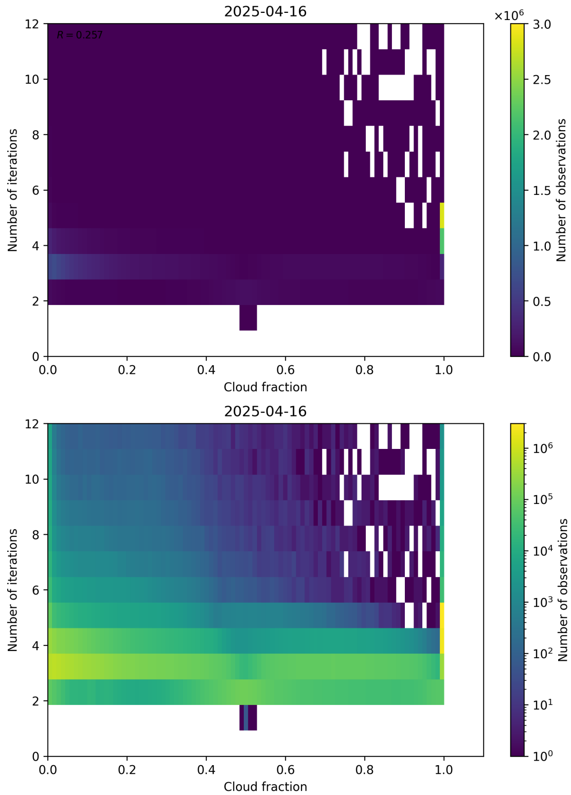
Figure 73: Scatter density plot of “Cloud fraction” against “Number of iterations” for 2025-04-15 to 2025-04-17.
