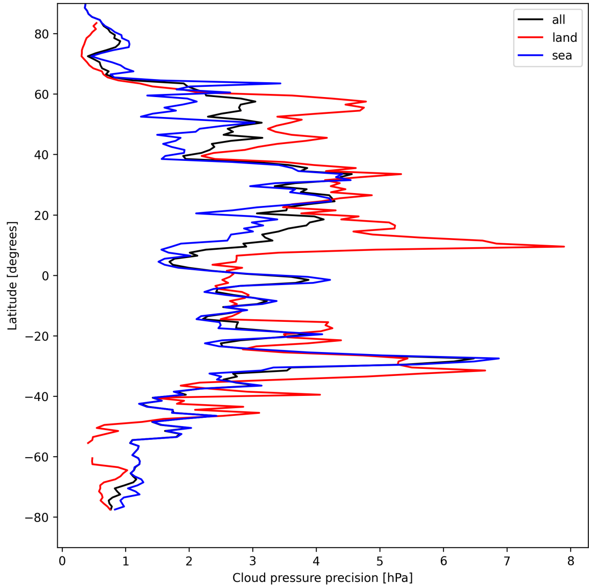
Figure 14: Zonal average of “Cloud pressure precision” for 2025-04-15 to 2025-04-17.
