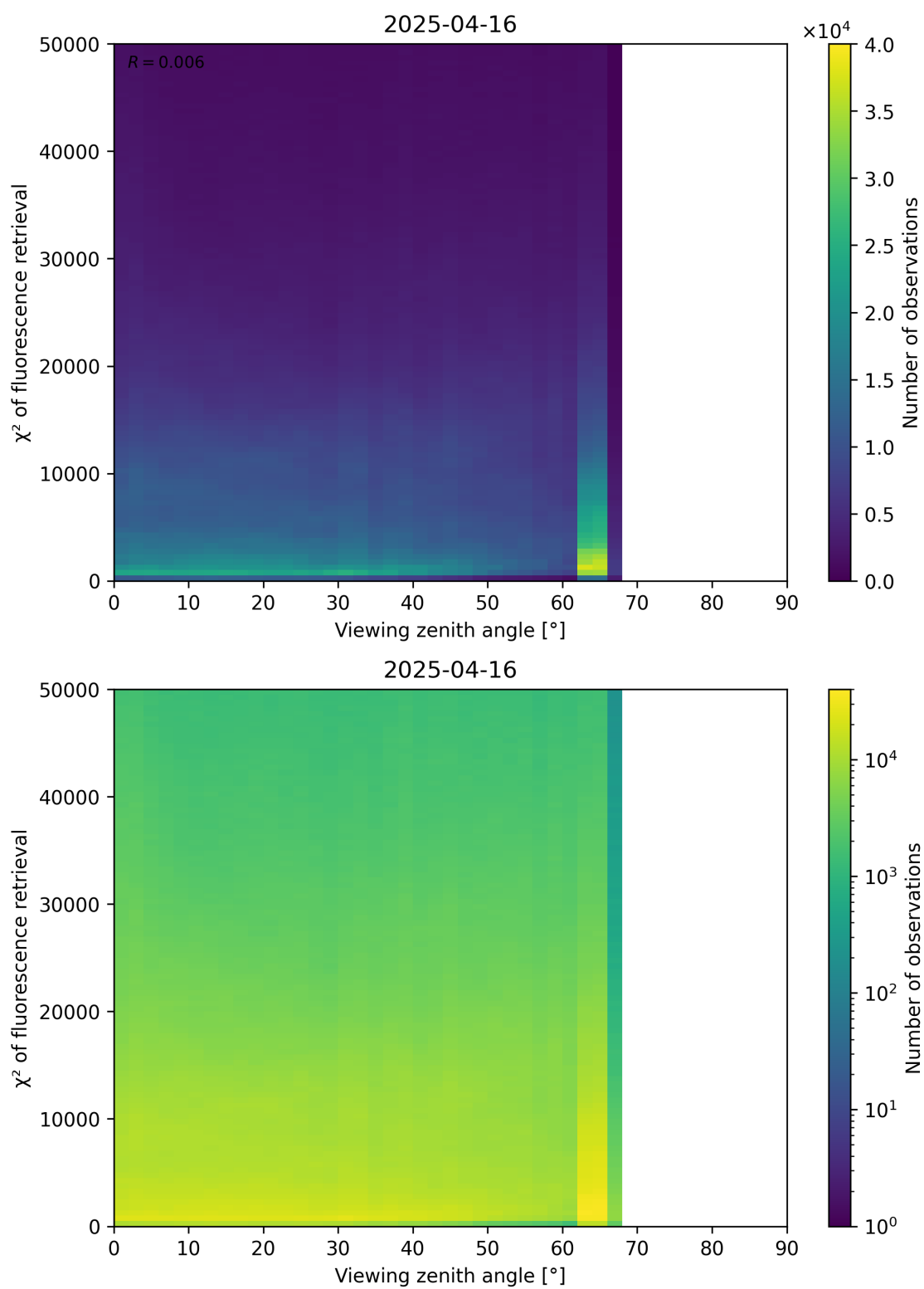
Figure 119: Scatter density plot of “Viewing zenith angle” against “ \chi^2 of fluorescence retrieval” for 2025-04-15 to 2025-04-17.
