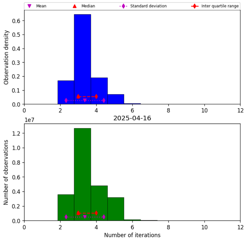
Figure 39: Histogram of “Number of iterations” for 2025-04-15 to 2025-04-17
