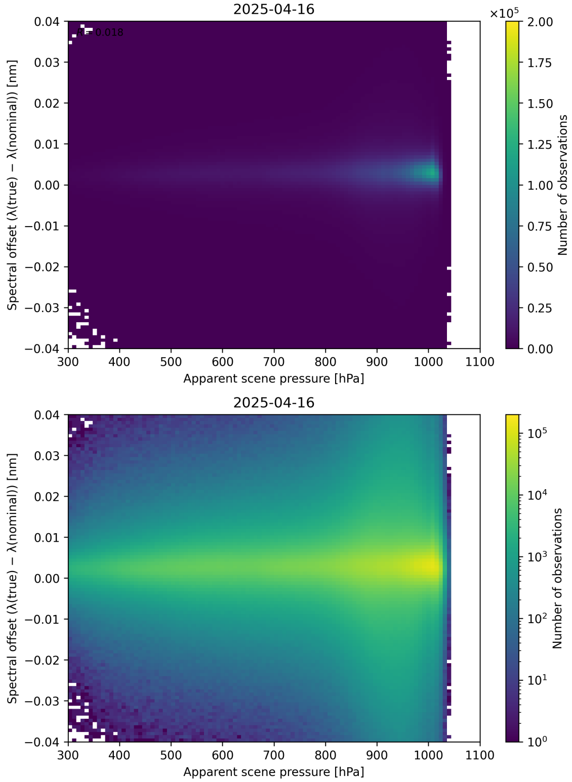
Figure 67: Scatter density plot of “Apparent scene pressure” against “Spectral offset ( \lambda_{\text{true}} - \lambda_{\text{nominal}} )” for 2025-04-15 to 2025-04-17.
