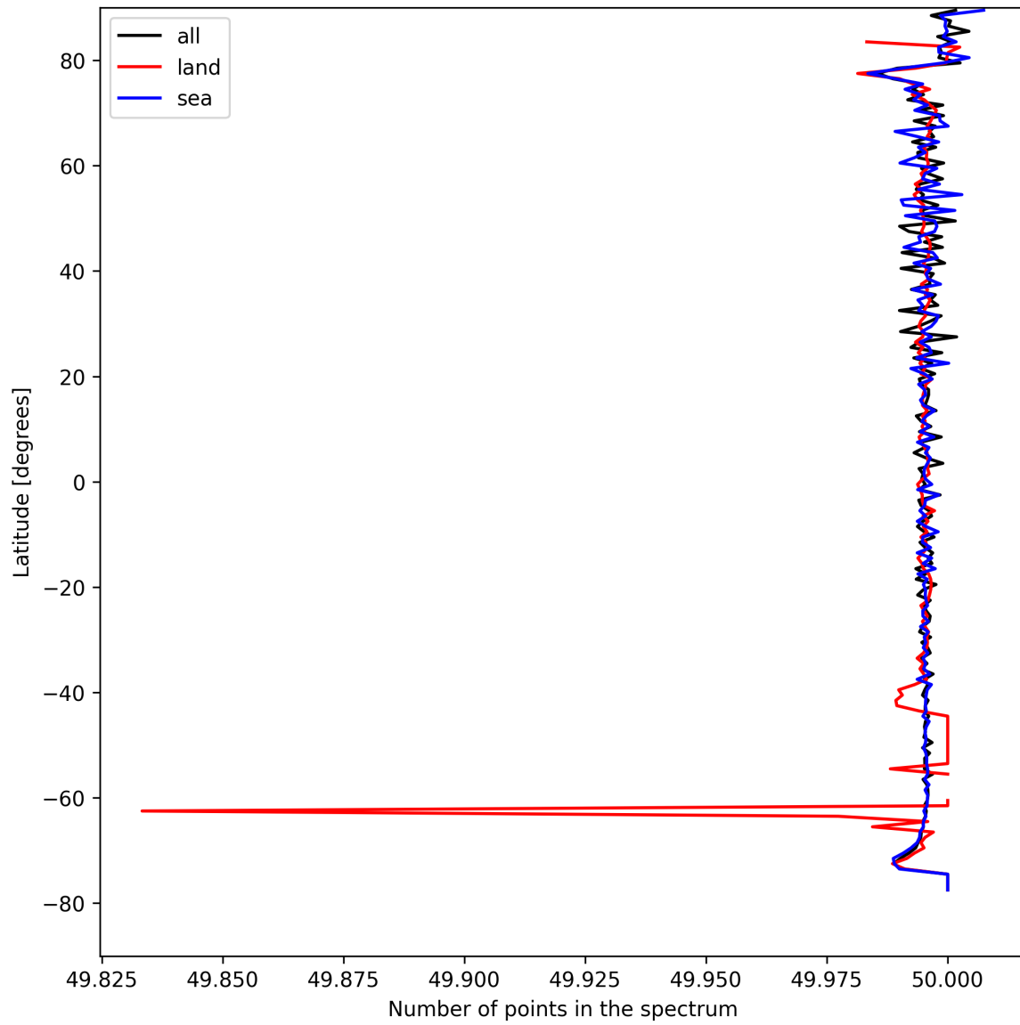
Figure 27: Zonal average of “Number of points in the spectrum” for 2025-04-15 to 2025-04-17.
