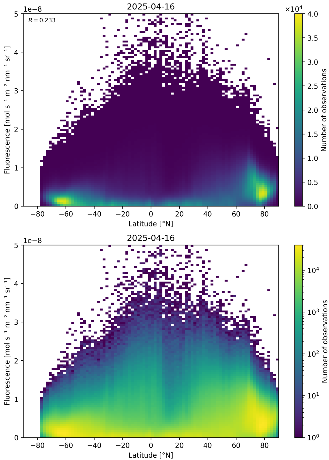
Figure 92: Scatter density plot of “Latitude” against “Fluorescence” for 2025-04-15 to 2025-04-17.
