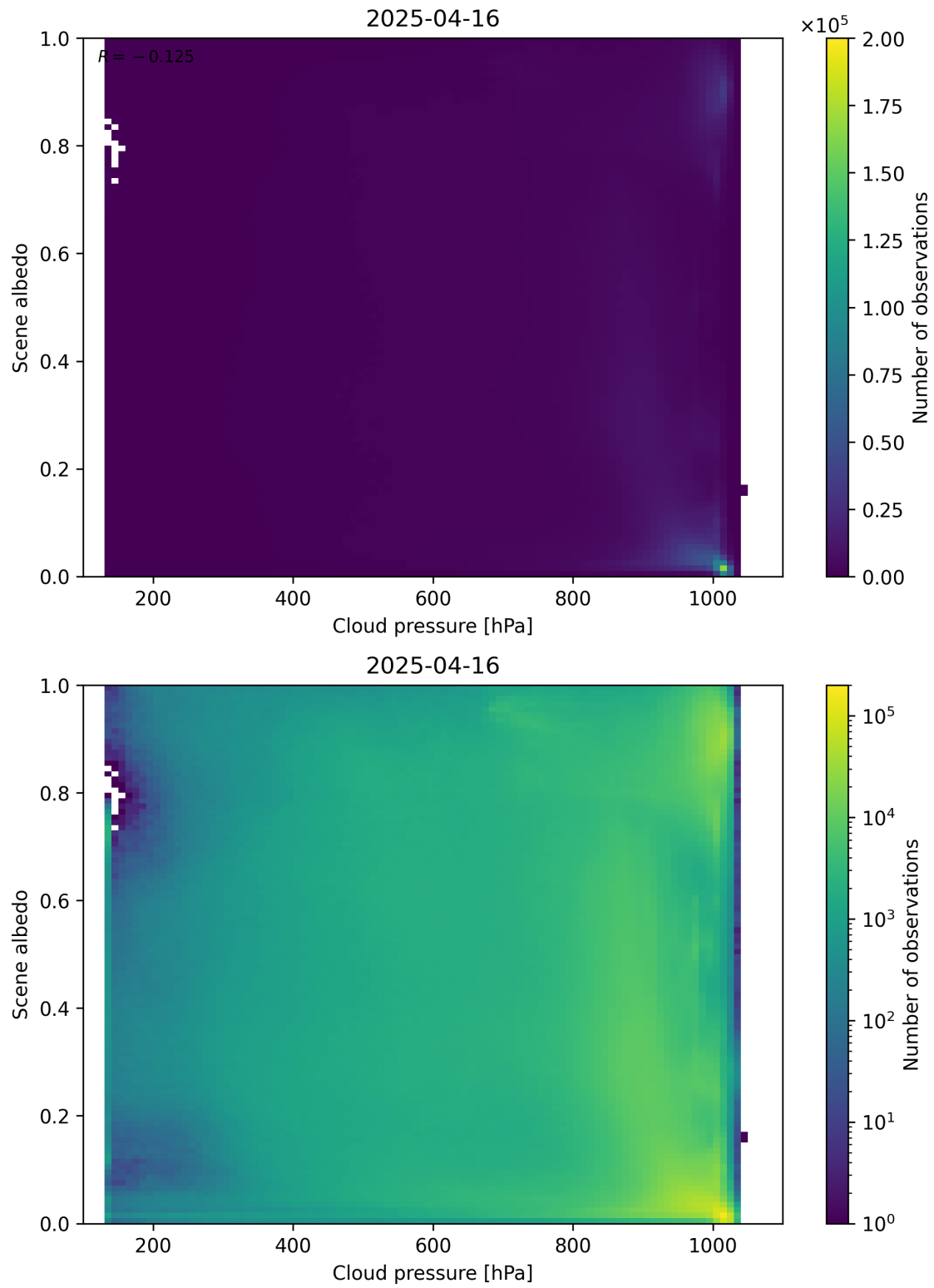
Figure 83: Scatter density plot of “Cloud pressure” against “Scene albedo” for 2025-04-15 to 2025-04-17.
