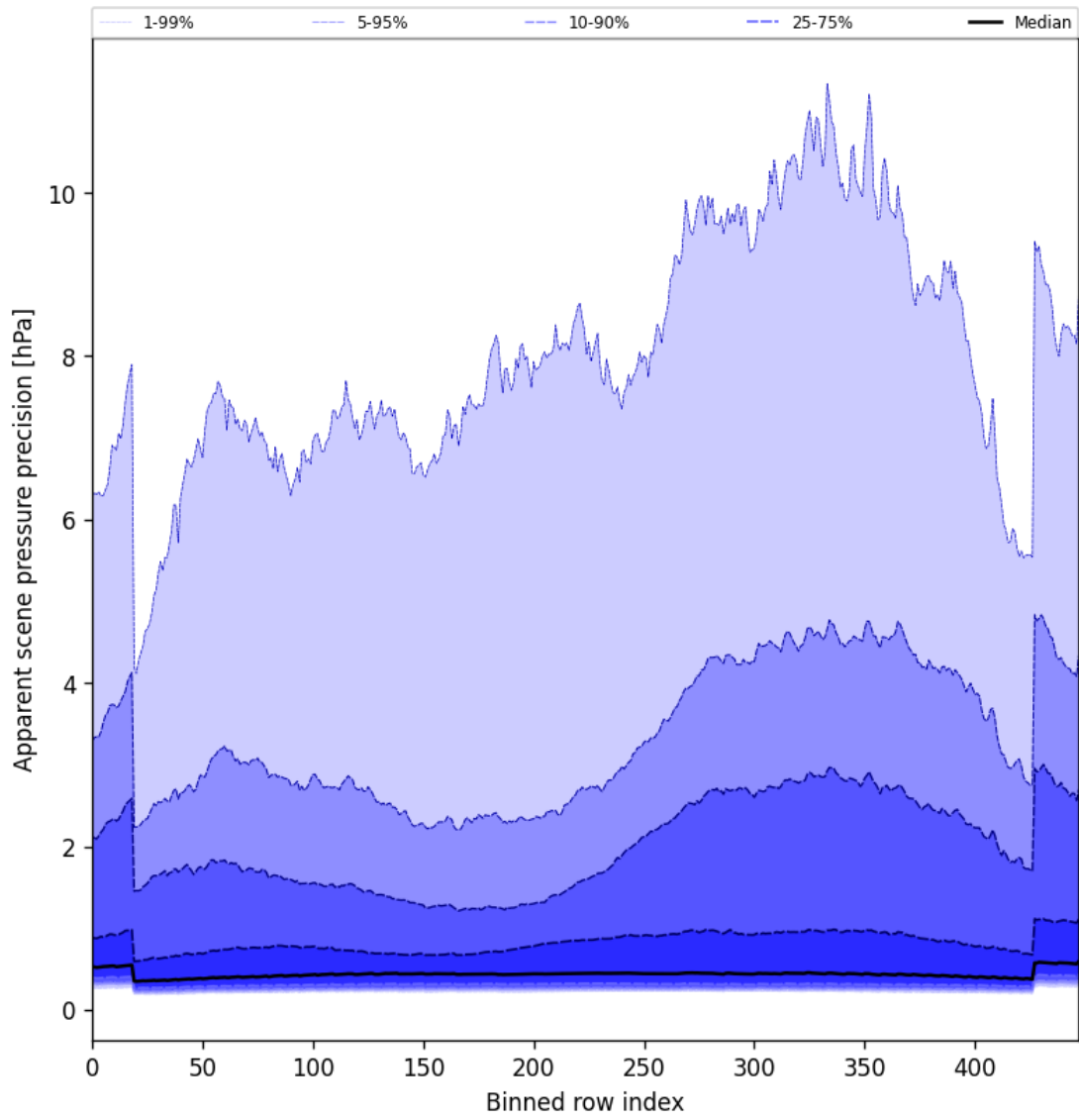
Figure 54: Along track statistics of “Apparent scene pressure precision” for 2025-04-15 to 2025-04-17
