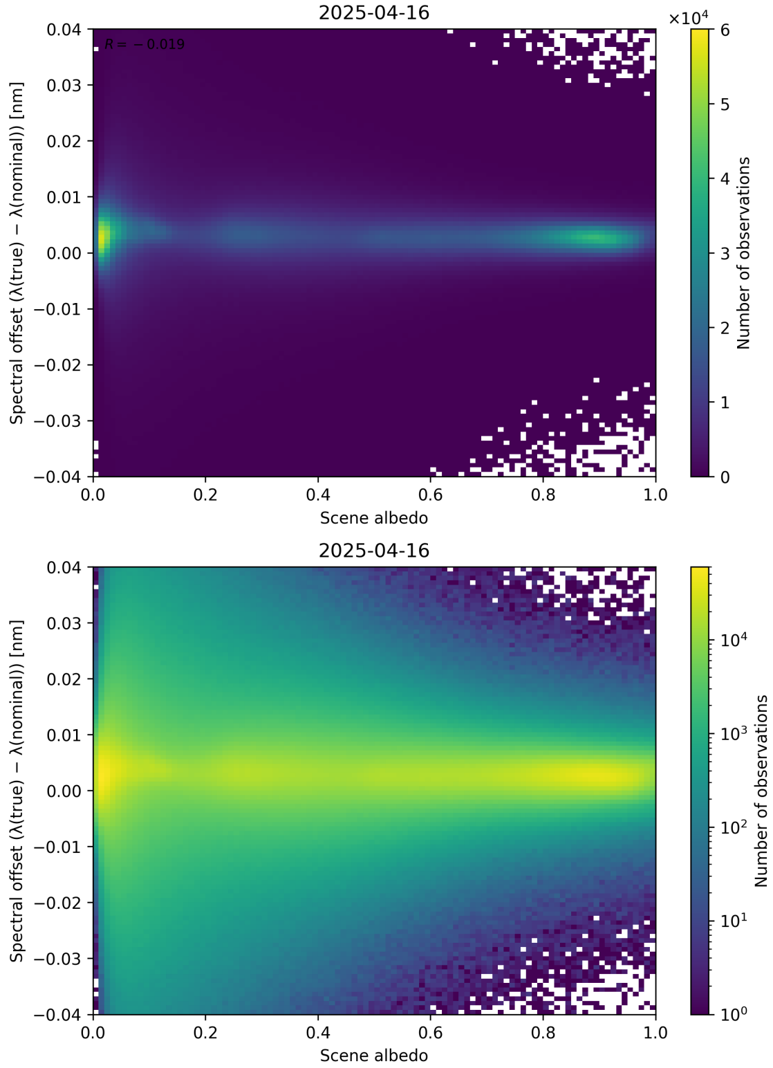
Figure 107: Scatter density plot of “Scene albedo” against “Spectral offset ( \lambda_{\text{true}} - \lambda_{\text{nominal}} )” for 2025-04-15 to 2025-04-17.
