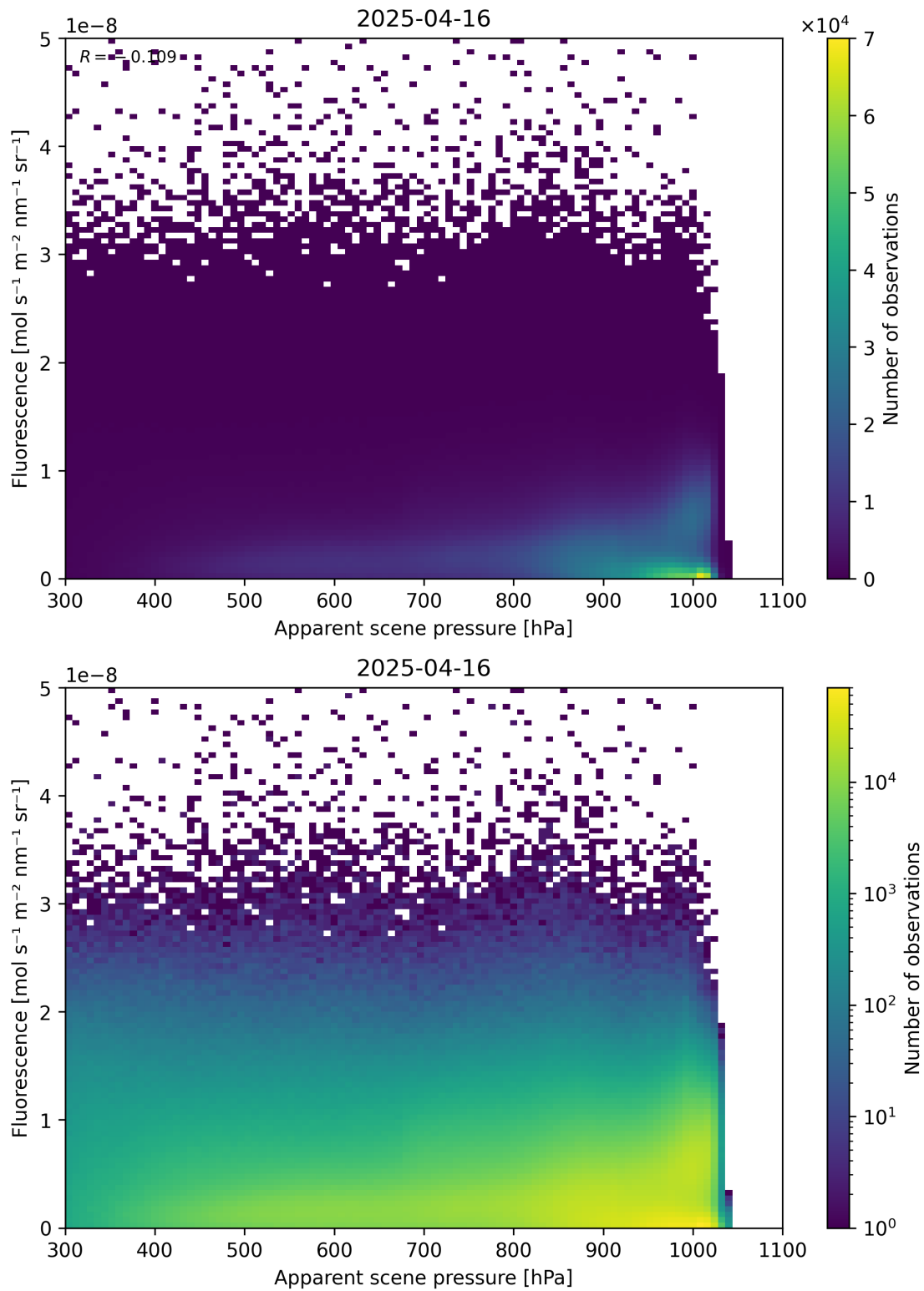
Figure 64: Scatter density plot of “Apparent scene pressure” against “Fluorescence” for 2025-04-15 to 2025-04-17.
