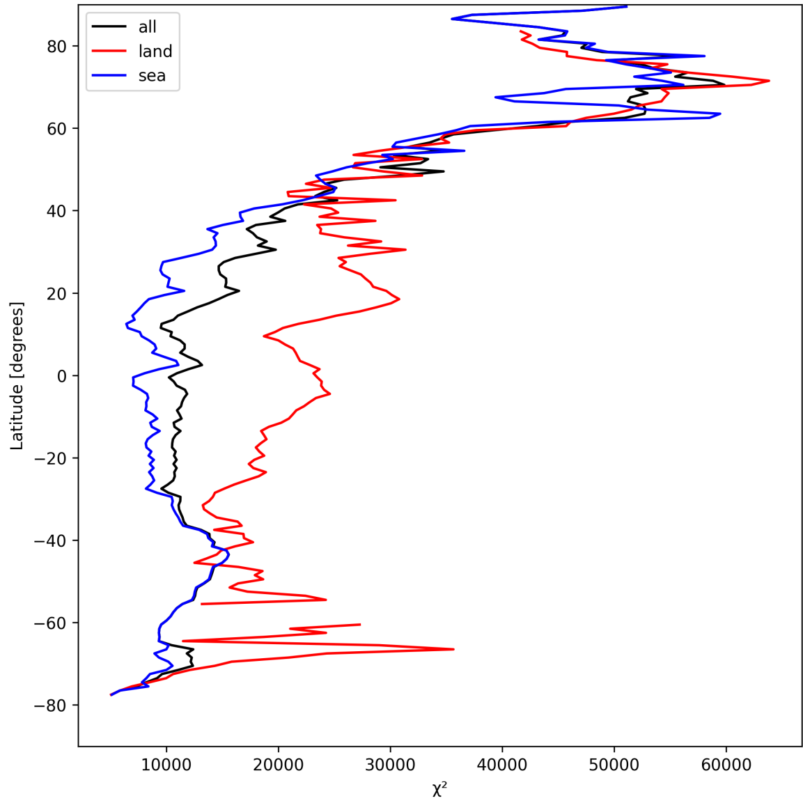
Figure 21: Zonal average of “ \chi^2 ” for 2025-04-15 to 2025-04-17.
