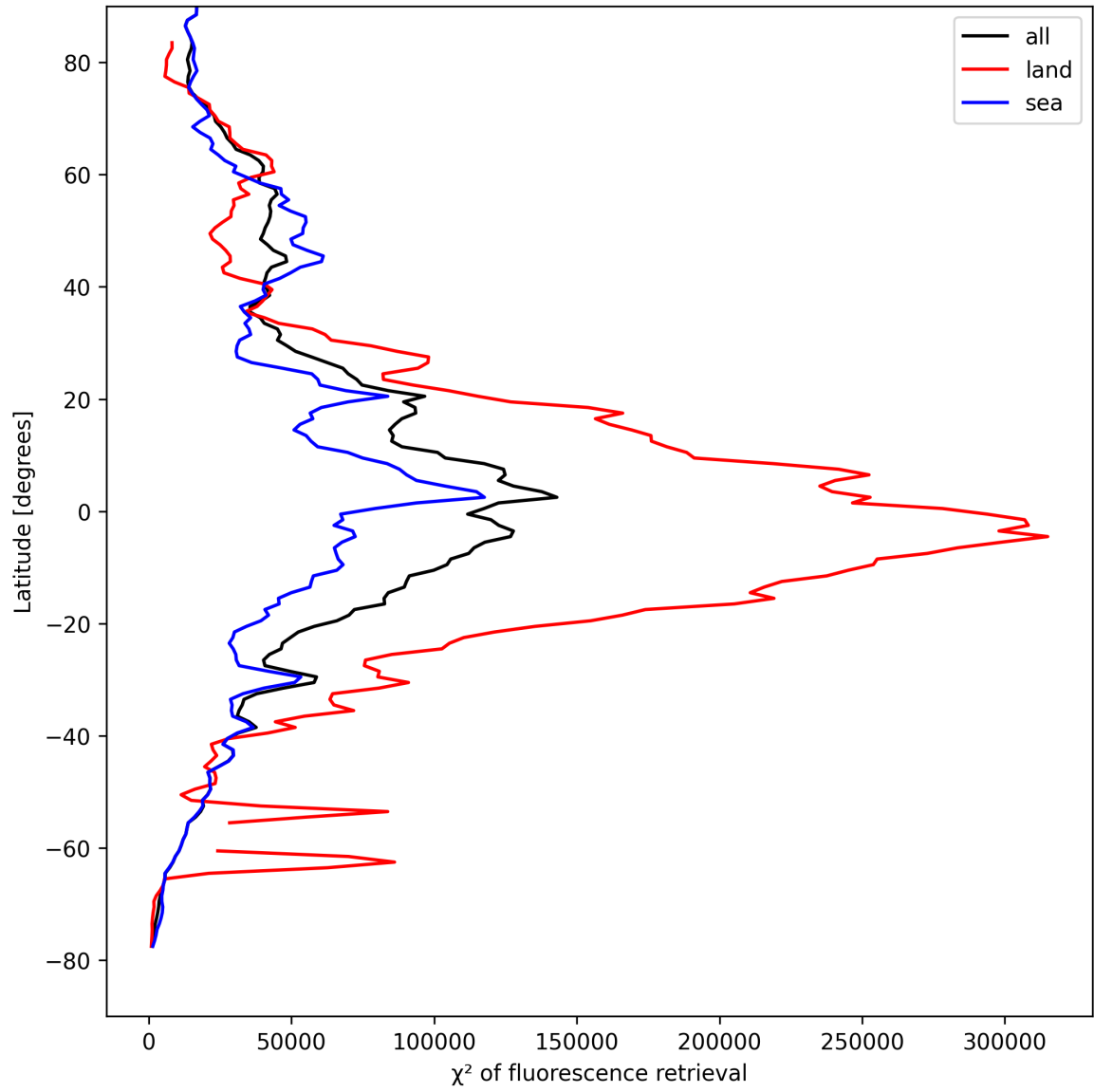
Figure 25: Zonal average of “ \chi^2 of fluorescence retrieval” for 2025-04-15 to 2025-04-17.
