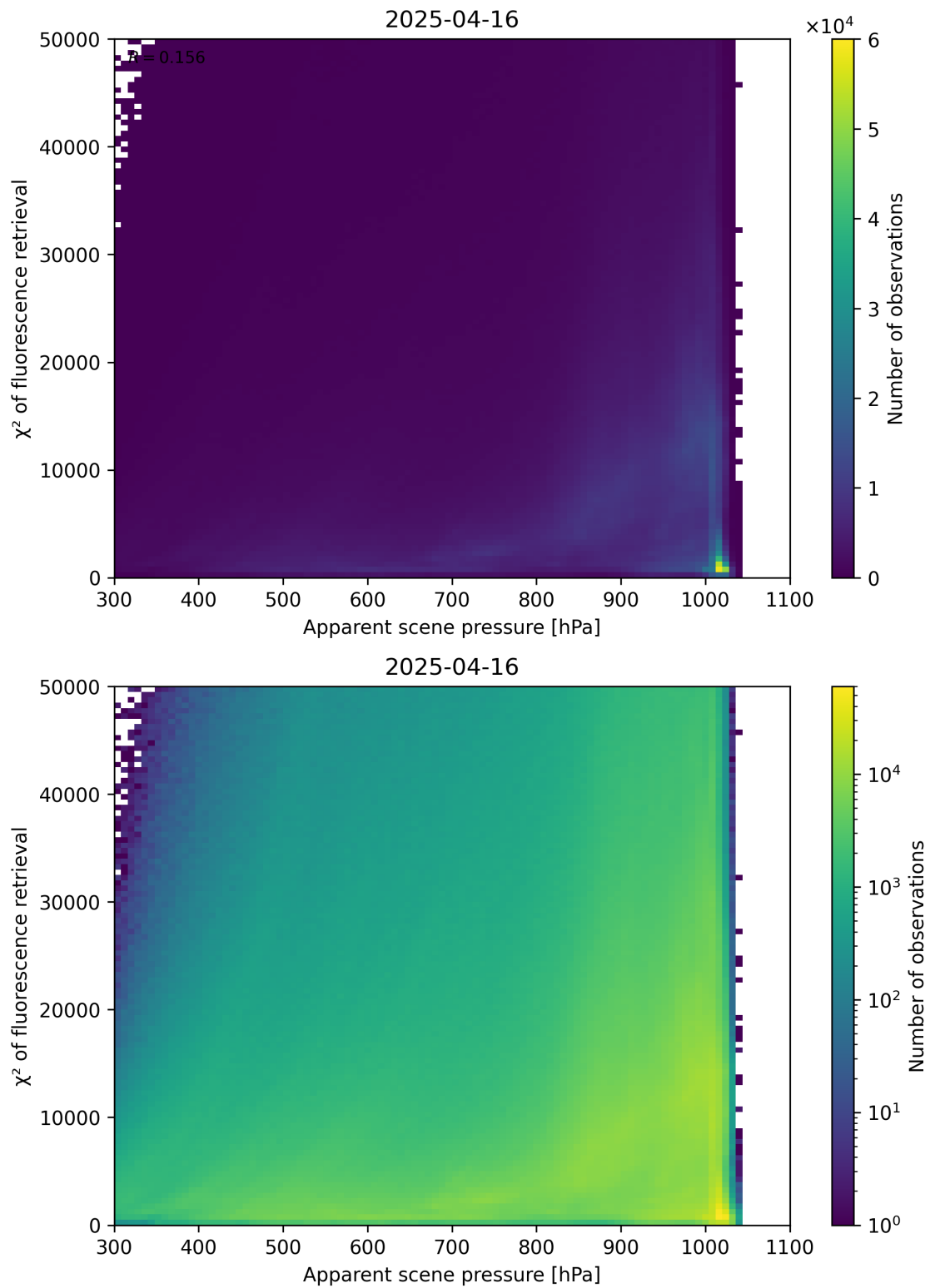
Figure 63: Scatter density plot of “Apparent scene pressure” against “ \chi^2 of fluorescence retrieval” for 2025-04-15 to 2025-04-17.
