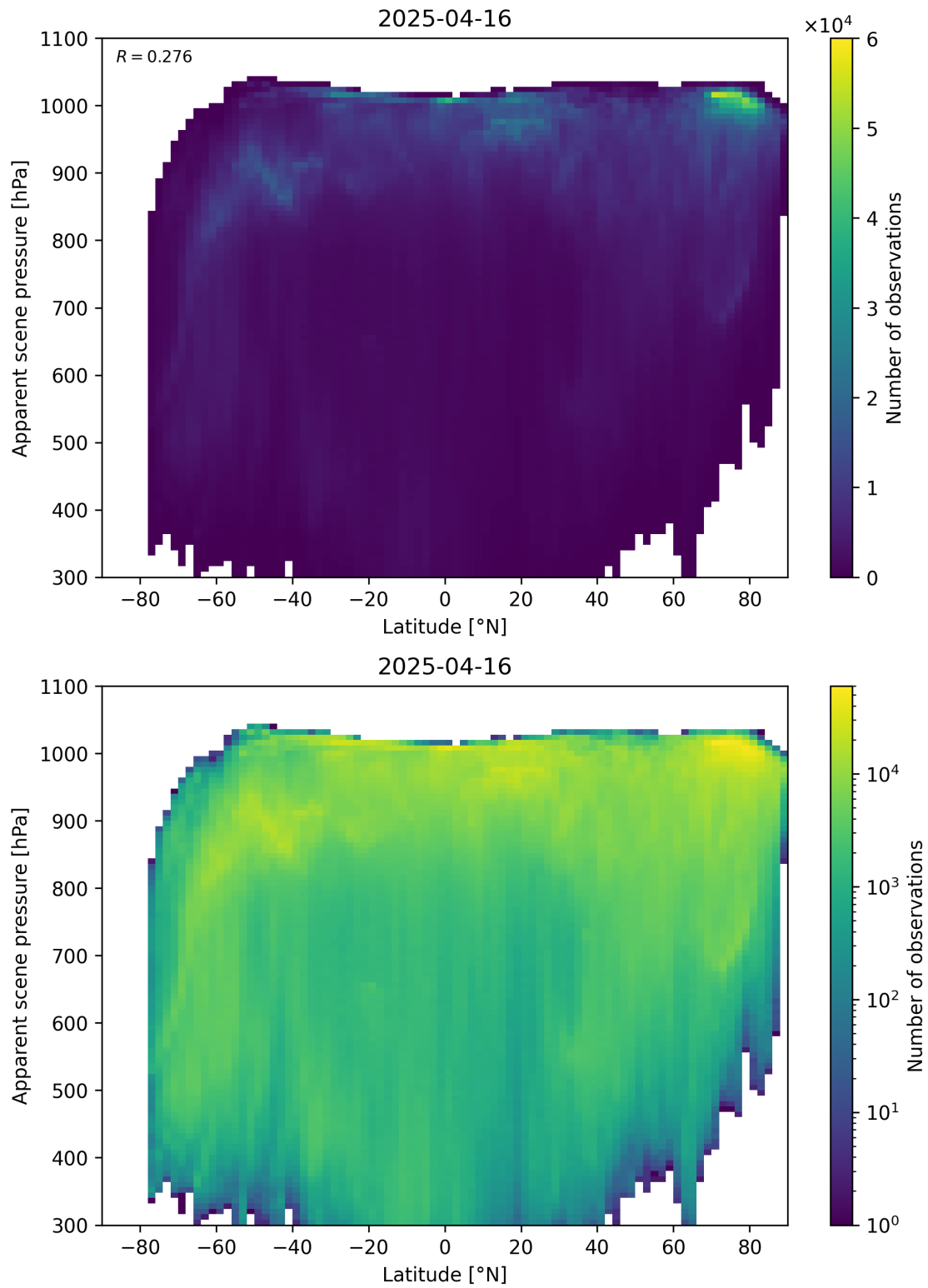
Figure 88: Scatter density plot of “Latitude” against “Apparent scene pressure” for 2025-04-15 to 2025-04-17.
