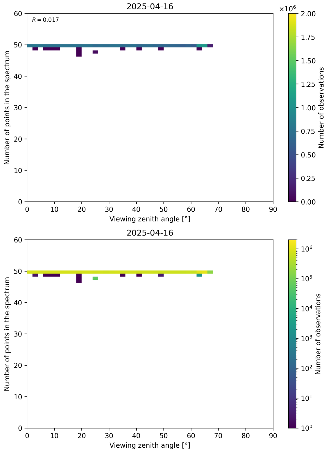
Figure 125: Scatter density plot of “Viewing zenith angle” against “Number of points in the spectrum” for 2025-04-15 to 2025-04-17.
