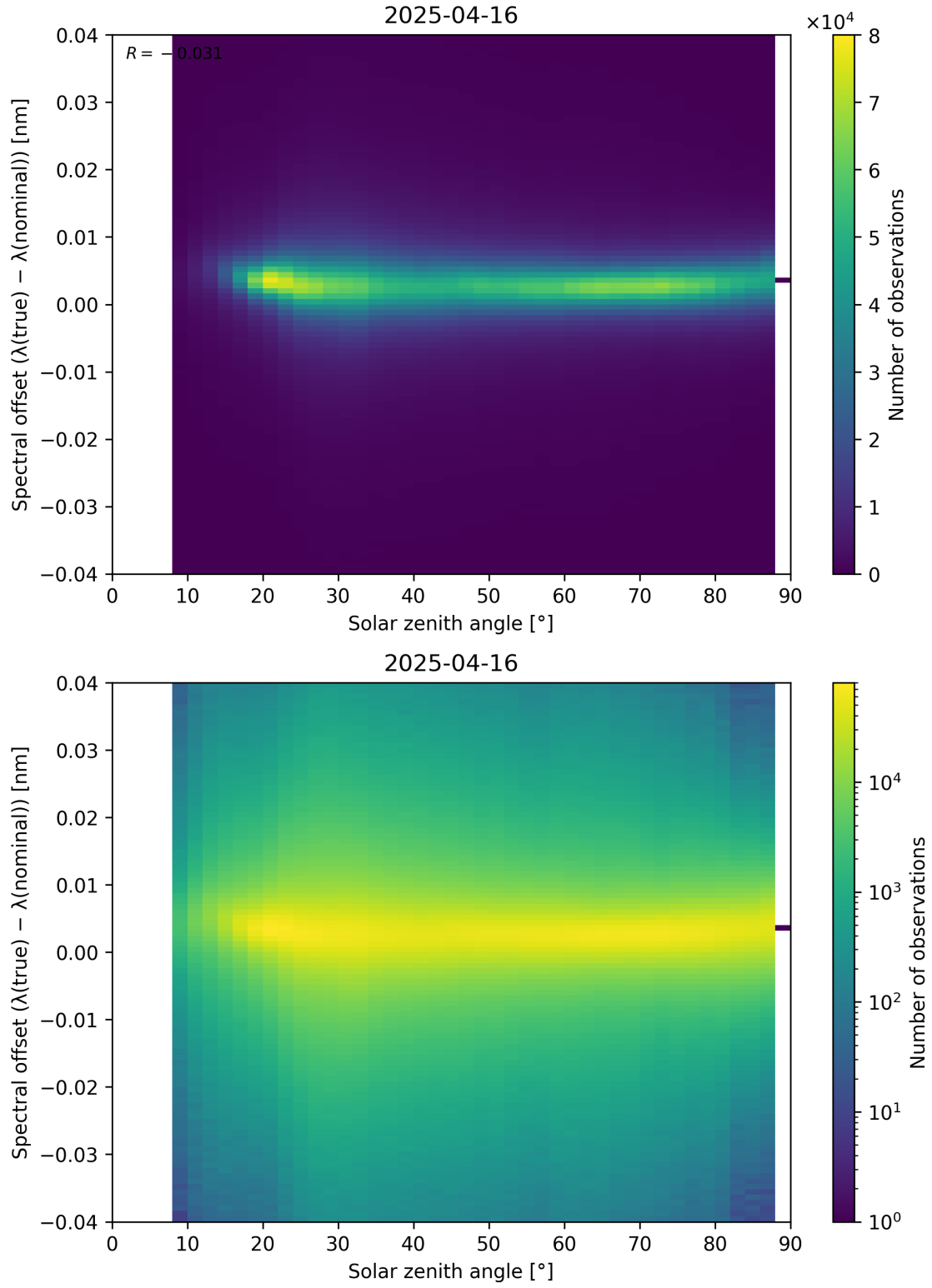
Figure 117: Scatter density plot of “Solar zenith angle” against “Spectral offset ( \lambda_{\text{true}} - \lambda_{\text{nominal}} )” for 2025-04-15 to 2025-04-17.
