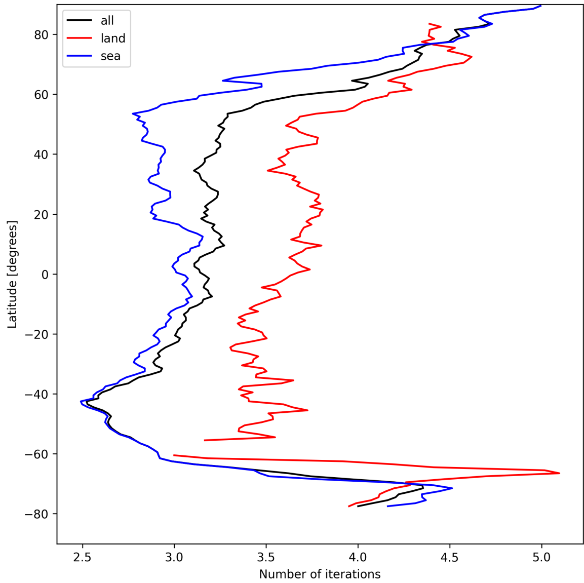
Figure 22: Zonal average of “Number of iterations” for 2025-04-15 to 2025-04-17.
