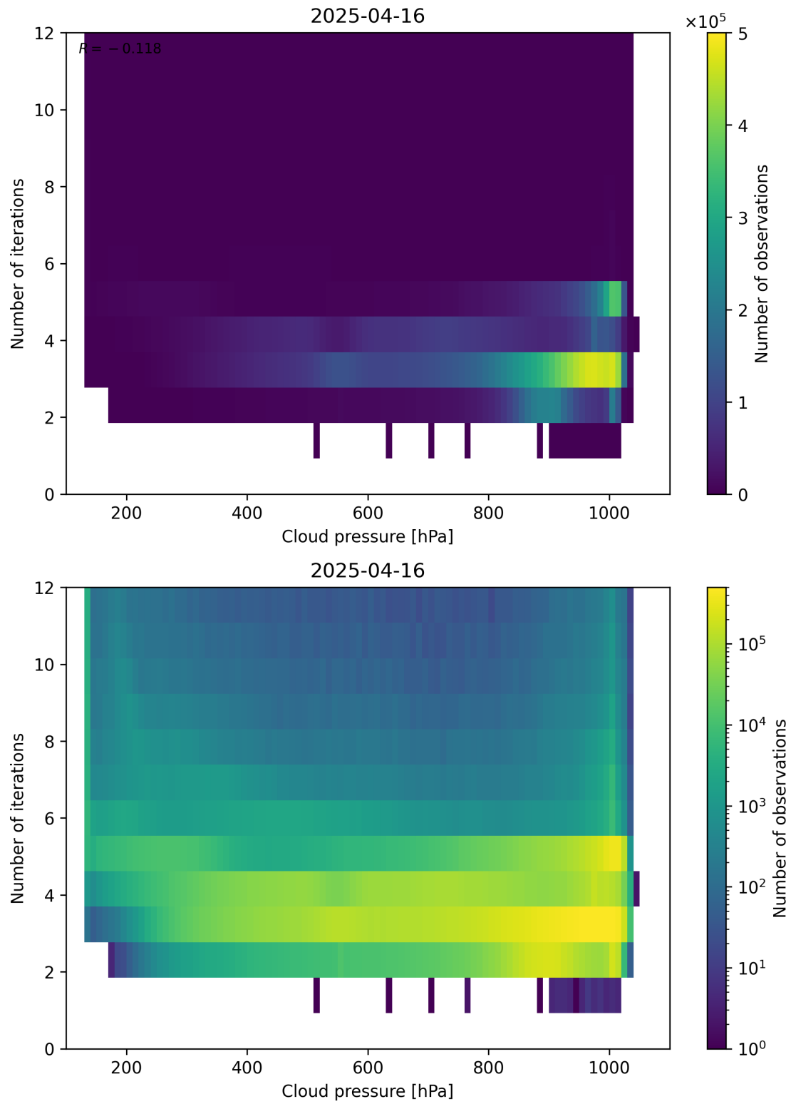
Figure 81: Scatter density plot of “Cloud pressure” against “Number of iterations” for 2025-04-15 to 2025-04-17.
