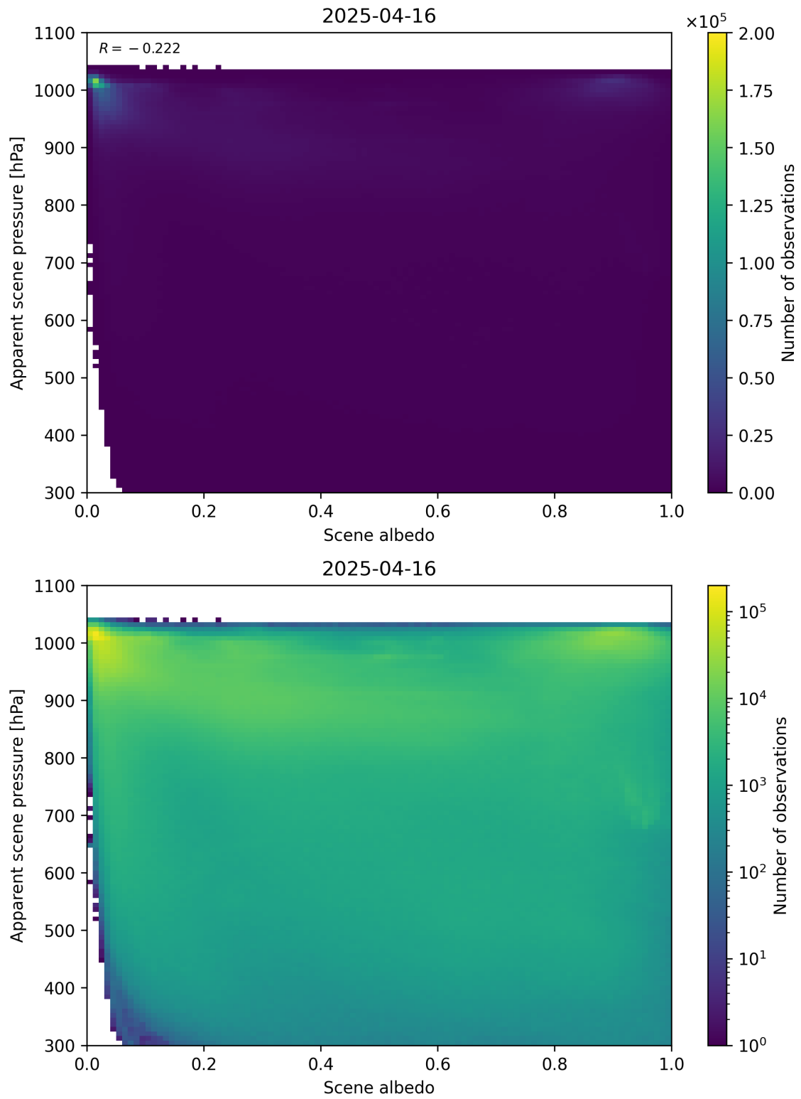
Figure 102: Scatter density plot of “Scene albedo” against “Apparent scene pressure” for 2025-04-15 to 2025-04-17.
