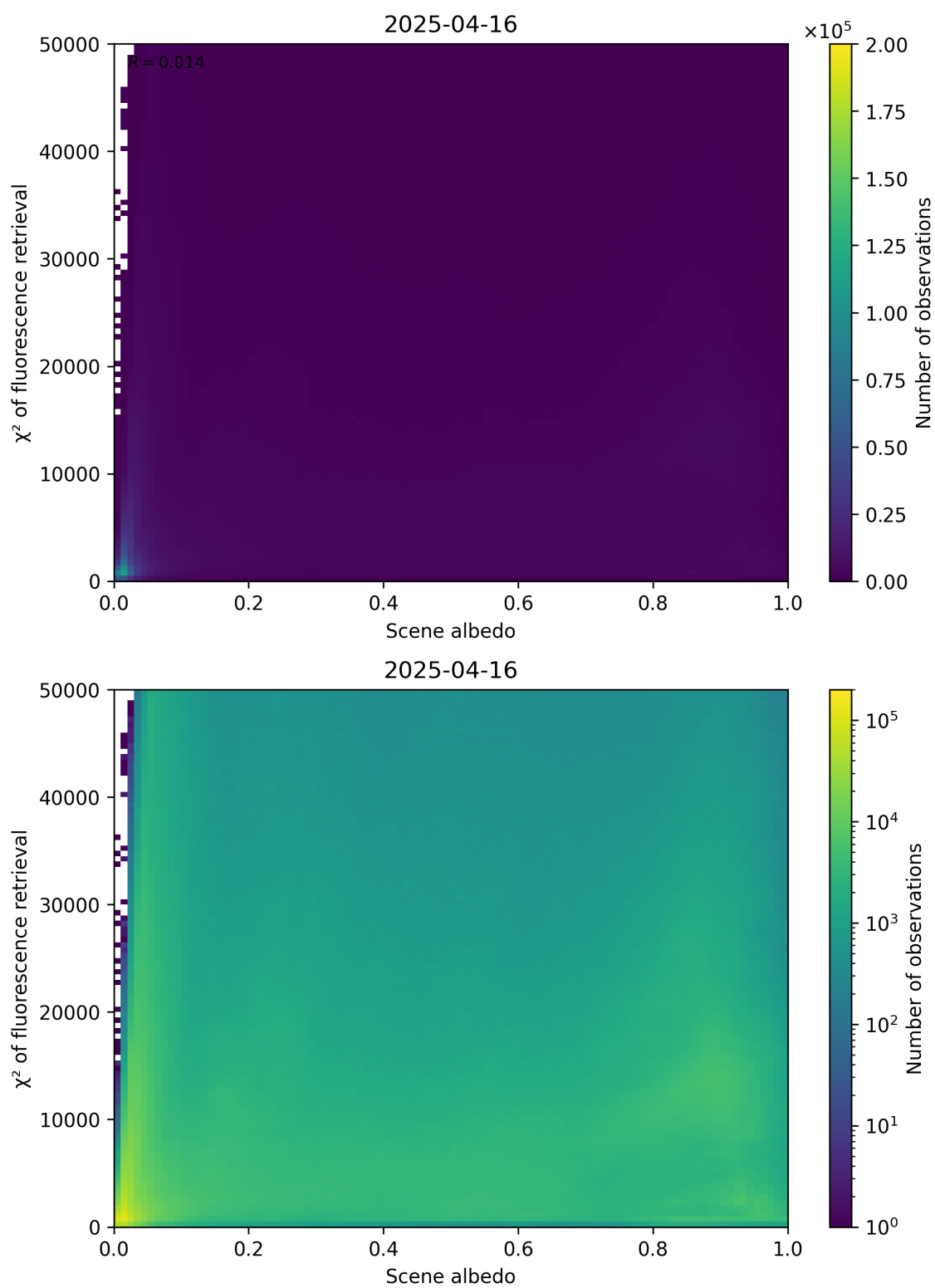
Figure 103: Scatter density plot of “Scene albedo” against “ \chi^2 of fluorescence retrieval” for 2025-04-15 to 2025-04-17.
