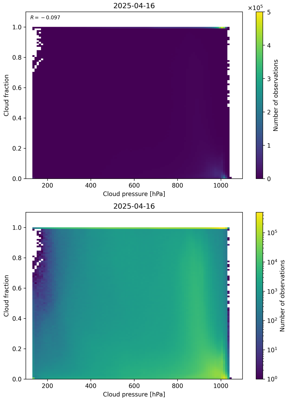
Figure 79: Scatter density plot of “Cloud pressure” against “Cloud fraction” for 2025-04-15 to 2025-04-17.
