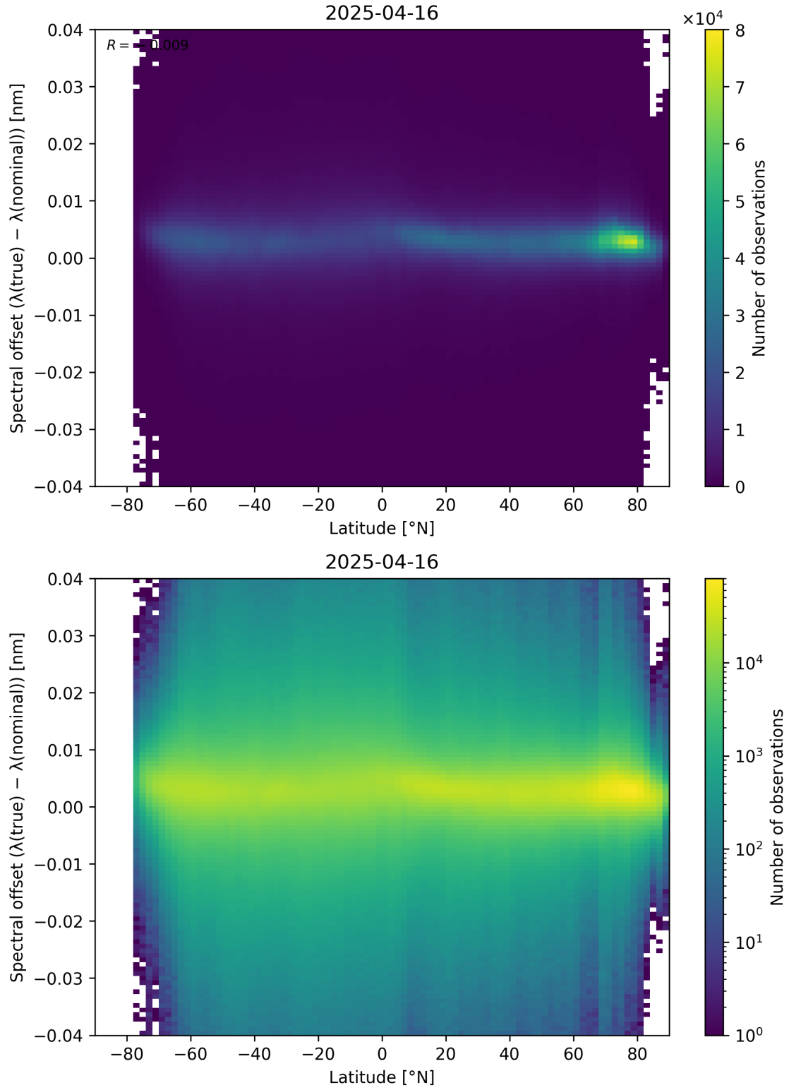
Figure 96: Scatter density plot of “Latitude” against “Spectral offset ( \lambda_{\text{true}} - \lambda_{\text{nominal}} )” for 2025-04-15 to 2025-04-17.
