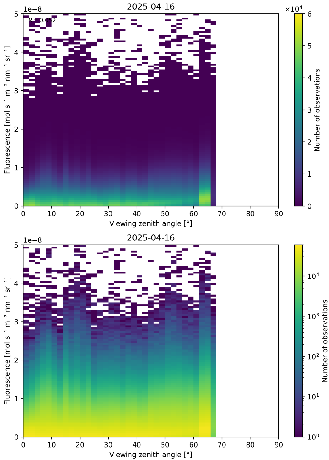
Figure 122: Scatter density plot of “Viewing zenith angle” against “Fluorescence” for 2025-04-15 to 2025-04-17.
