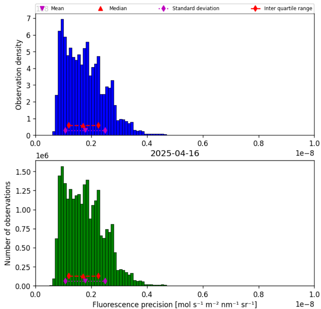
Figure 41: Histogram of “Fluorescence precision” for 2025-04-15 to 2025-04-17
