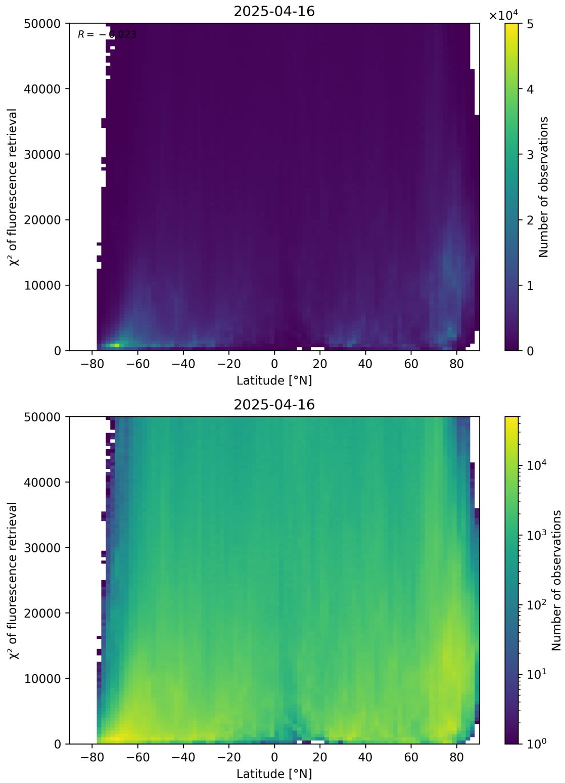
Figure 89: Scatter density plot of “Latitude” against “ \chi^2 of fluorescence retrieval” for 2025-04-15 to 2025-04-17.
