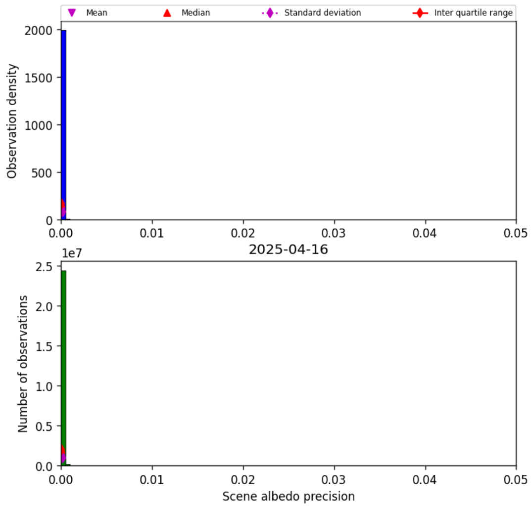
Figure 35: Histogram of “Scene albedo precision” for 2025-04-15 to 2025-04-17
