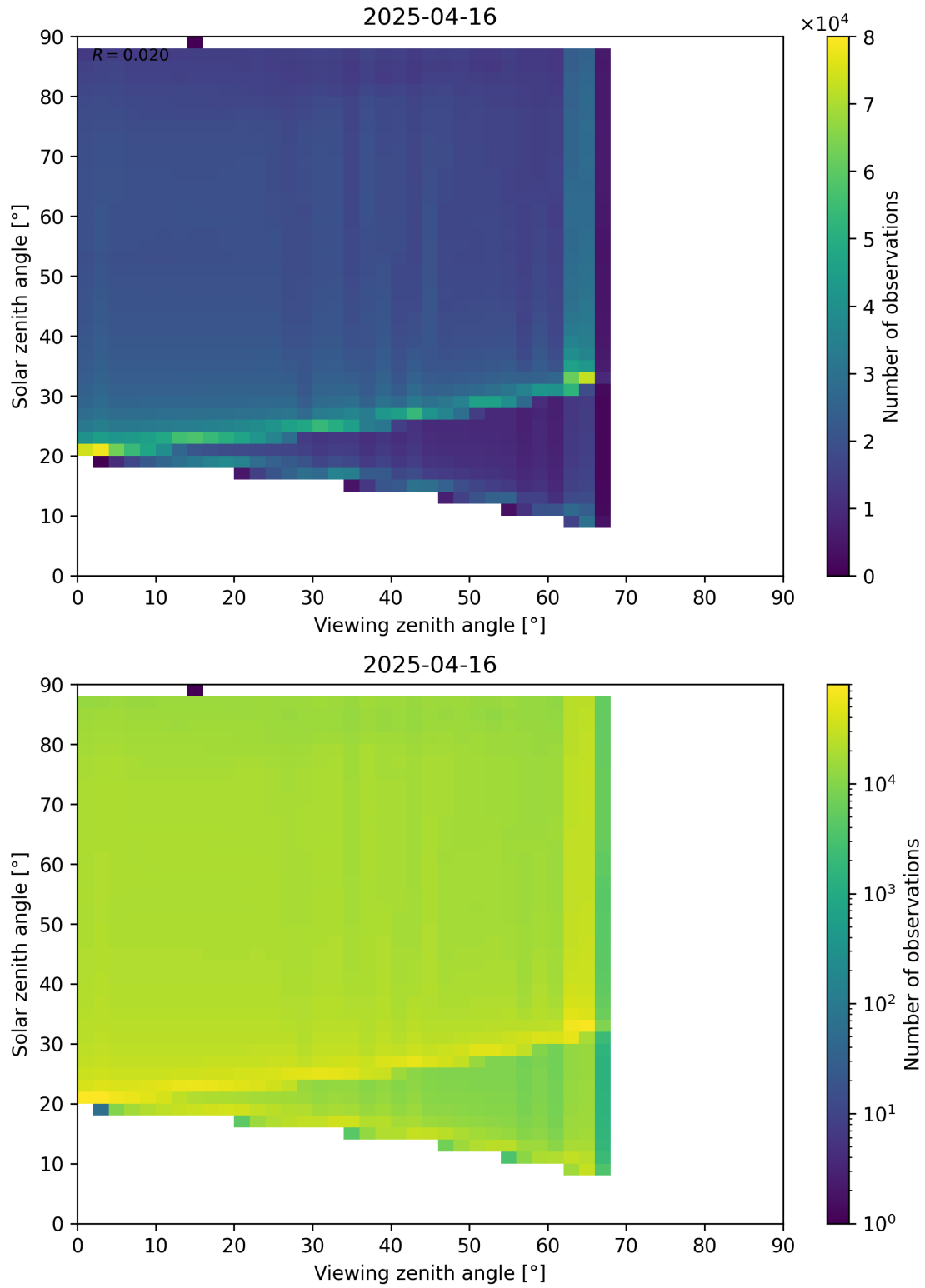
Figure 127: Scatter density plot of “Viewing zenith angle” against “Solar zenith angle” for 2025-04-15 to 2025-04-17.
