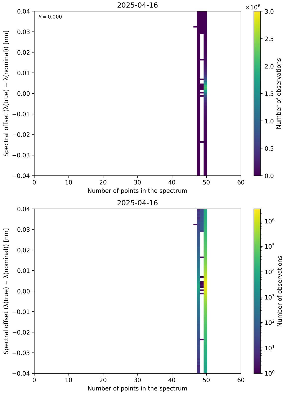
Figure 101: Scatter density plot of “Number of points in the spectrum” against “Spectral offset ( \lambda_{\text{true}} - \lambda_{\text{nominal}} )” for 2025-04-15 to 2025-04-17.
