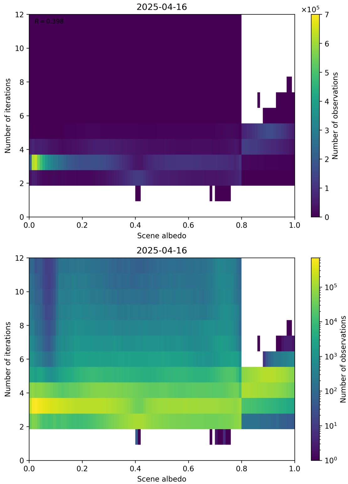
Figure 105: Scatter density plot of “Scene albedo” against “Number of iterations” for 2025-04-15 to 2025-04-17.
