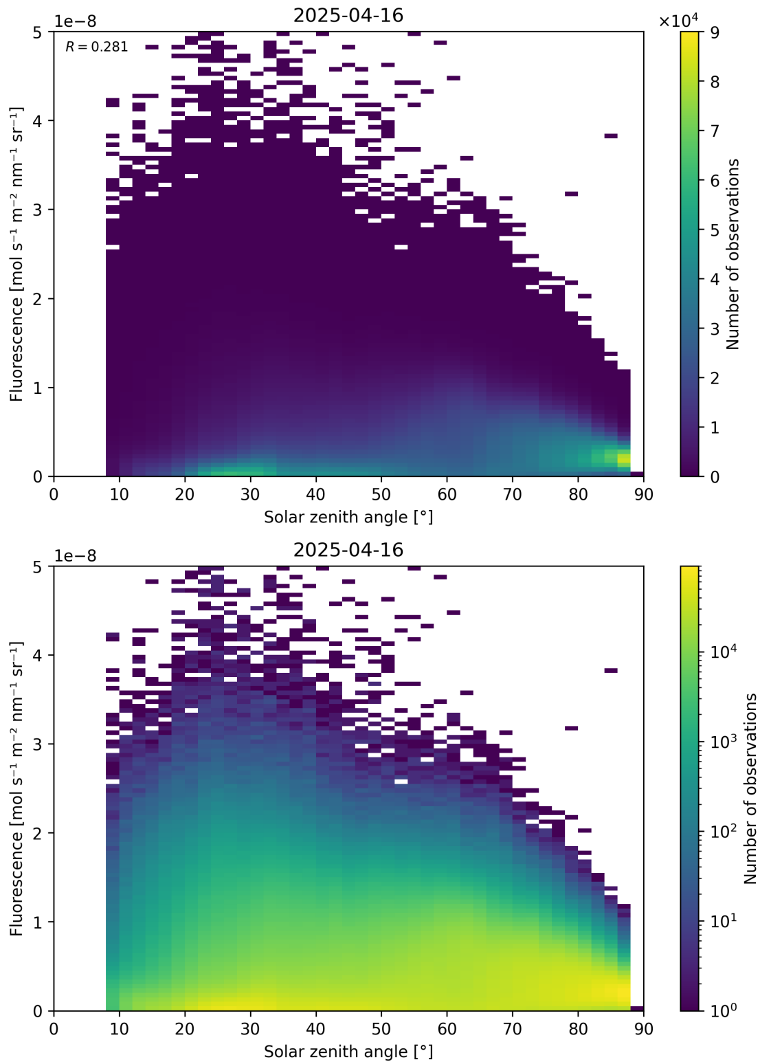
Figure 112: Scatter density plot of “Solar zenith angle” against “Fluorescence” for 2025-04-15 to 2025-04-17.
