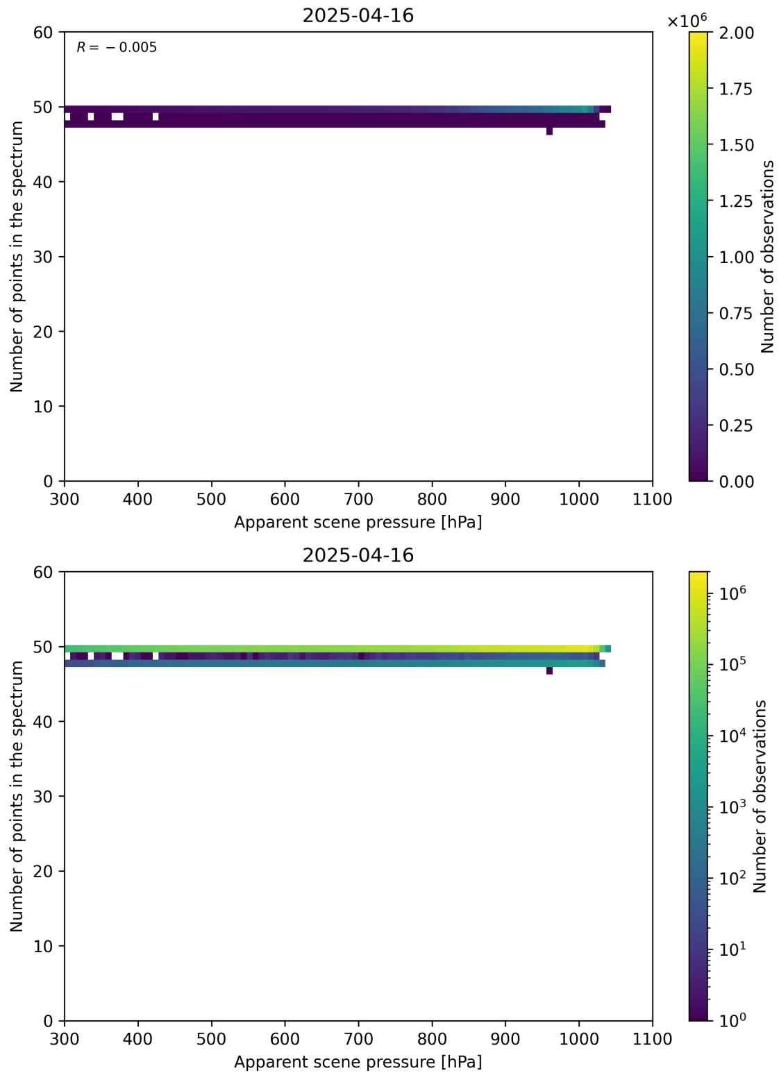
Figure 66: Scatter density plot of “Apparent scene pressure” against “Number of points in the spectrum” for 2025-04-15 to 2025-04-17.
