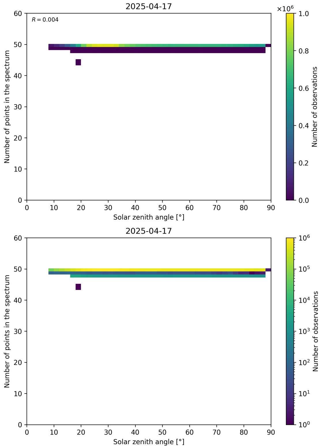
Figure 115: Scatter density plot of “Solar zenith angle” against “Number of points in the spectrum” for 2025-04-16 to 2025-04-18.
