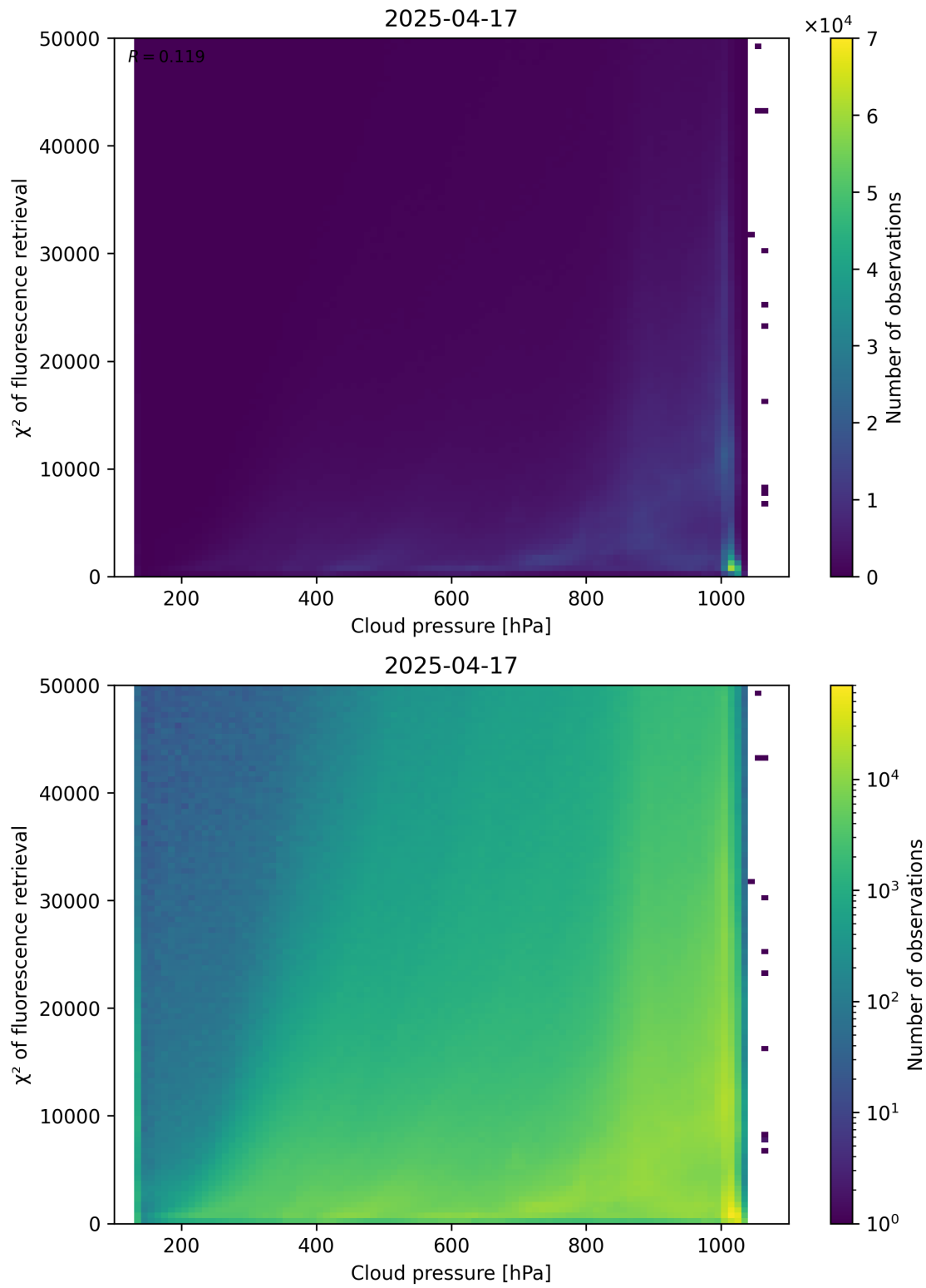
Figure 78: Scatter density plot of “Cloud pressure” against “ \chi^2 of fluorescence retrieval” for 2025-04-16 to 2025-04-18.
