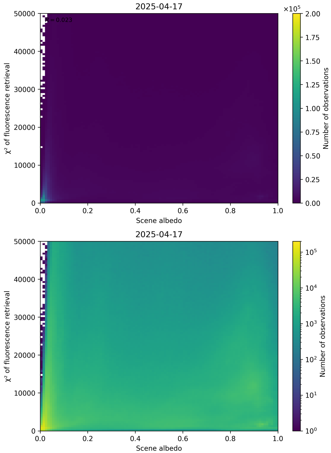
Figure 103: Scatter density plot of “Scene albedo” against “ \chi^2 of fluorescence retrieval” for 2025-04-16 to 2025-04-18.
