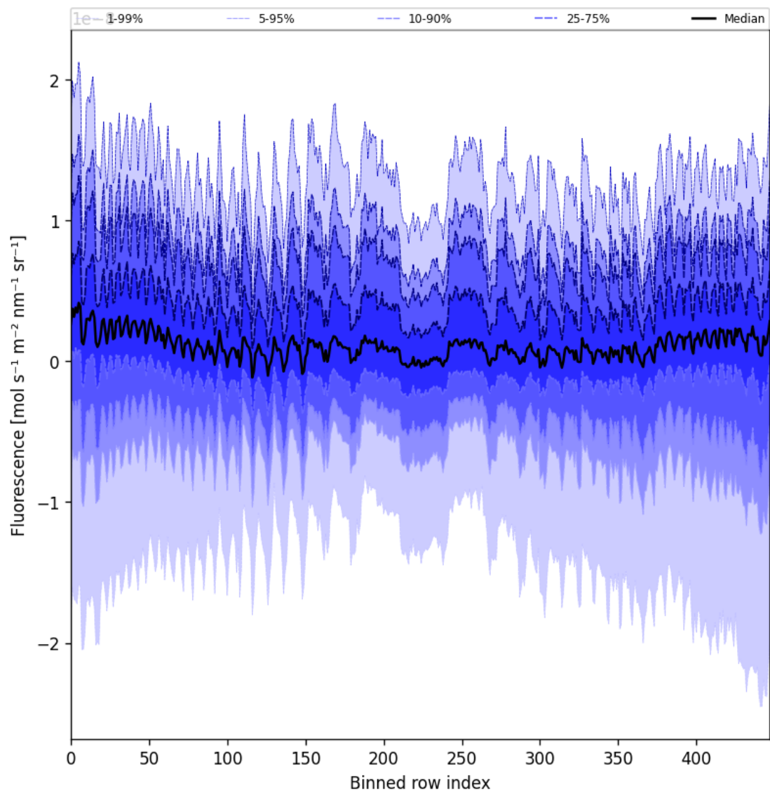
Figure 57: Along track statistics of “Fluorescence” for 2025-04-16 to 2025-04-18
