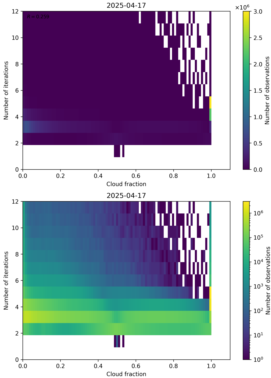
Figure 73: Scatter density plot of “Cloud fraction” against “Number of iterations” for 2025-04-16 to 2025-04-18.
