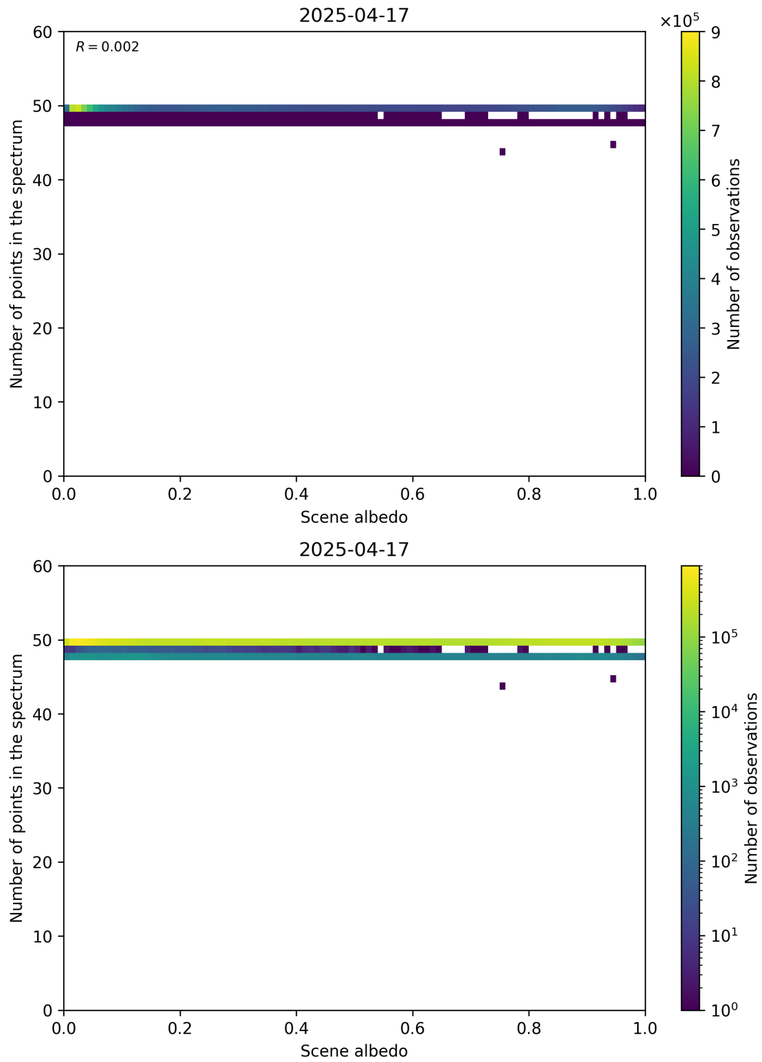
Figure 106: Scatter density plot of “Scene albedo” against “Number of points in the spectrum” for 2025-04-16 to 2025-04-18.
