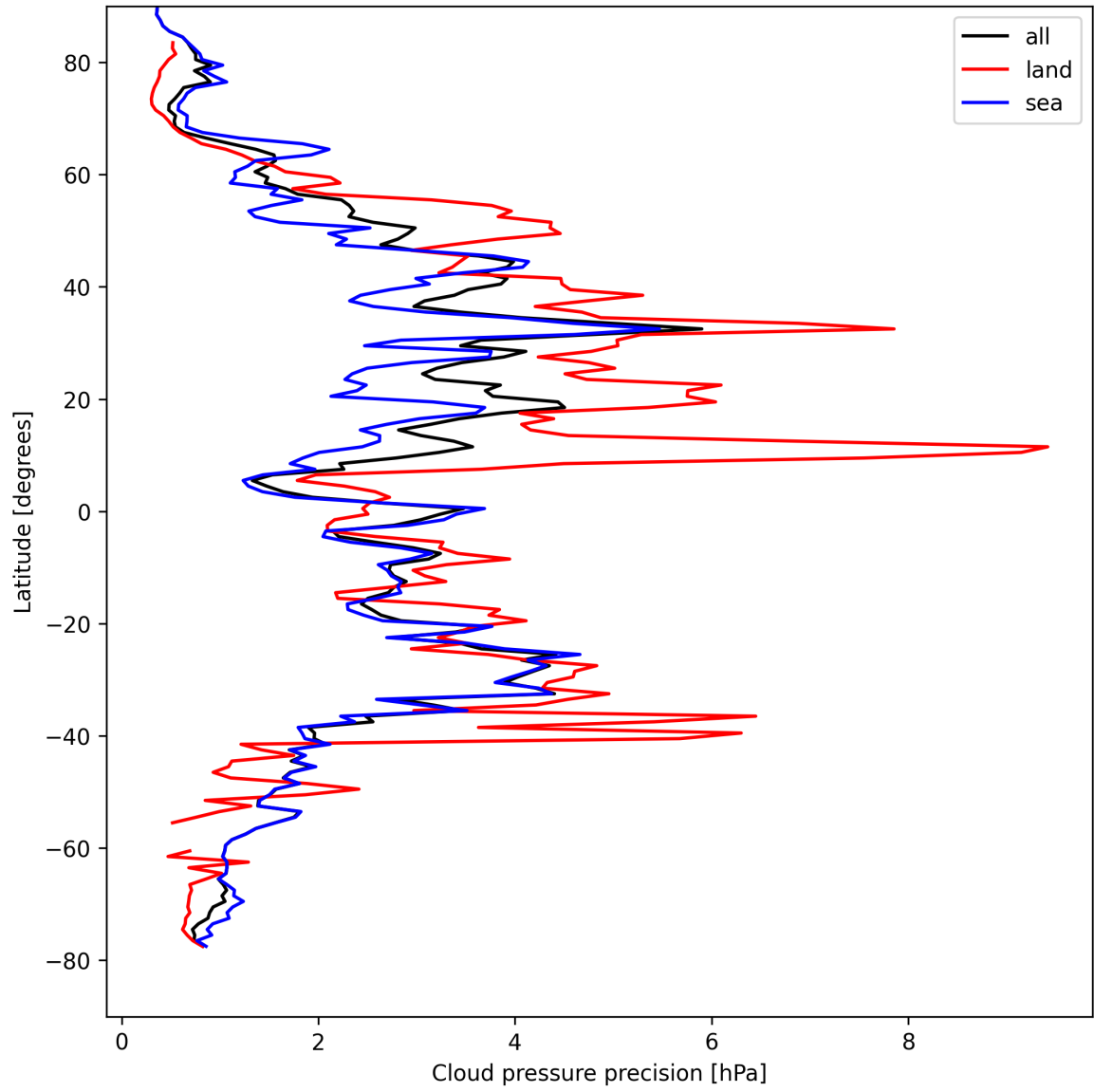
Figure 14: Zonal average of "Cloud pressure precision" for 2025-04-16 to 2025-04-18.
