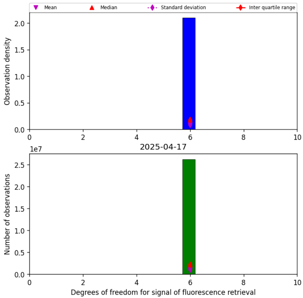
Figure 43: Histogram of “Degrees of freedom for signal of fluorescence retrieval” for 2025-04-16 to 2025-04-18
