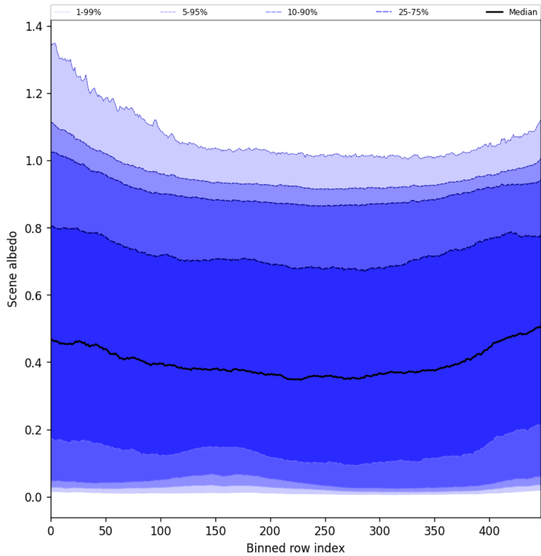
Figure 51: Along track statistics of “Scene albedo” for 2025-04-16 to 2025-04-18
