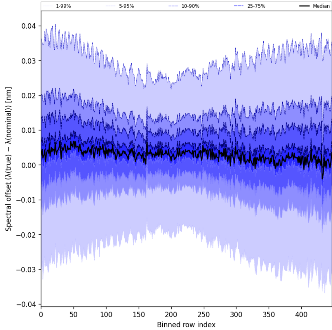
Figure 62: Along track statistics of “Spectral offset ( \lambda_{\text{true}} - \lambda_{\text{nominal}} )” for 2025-04-16 to 2025-04-18
