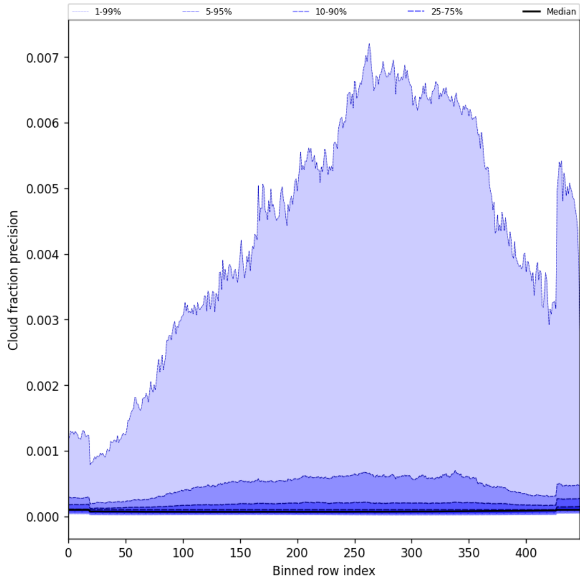
Figure 50: Along track statistics of “Cloud fraction precision” for 2025-04-16 to 2025-04-18
