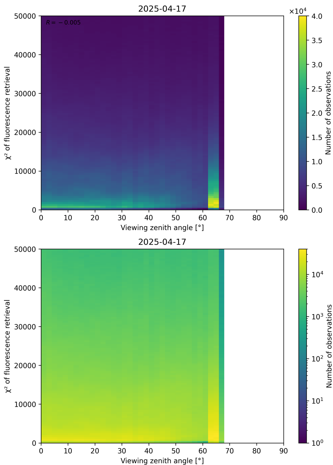
Figure 119: Scatter density plot of “Viewing zenith angle” against “ \chi^2 of fluorescence retrieval” for 2025-04-16 to 2025-04-18.
