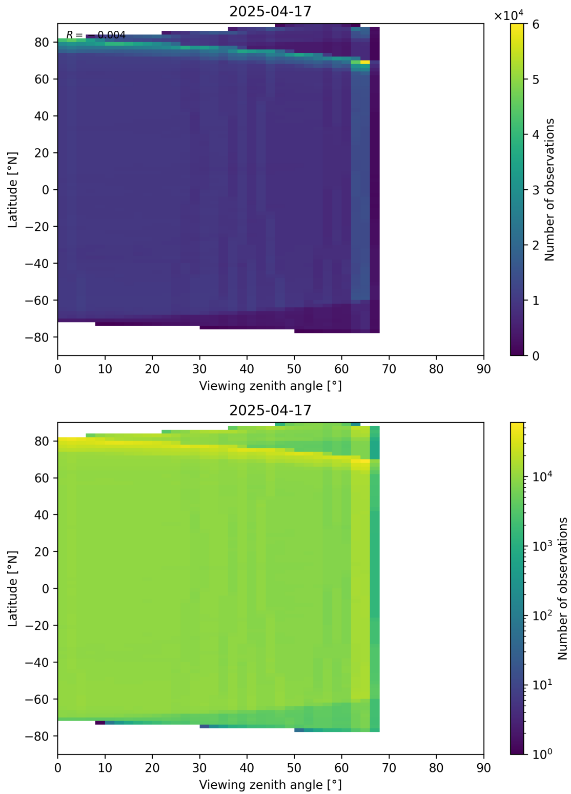
Figure 123: Scatter density plot of “Viewing zenith angle” against “Latitude” for 2025-04-16 to 2025-04-18.
