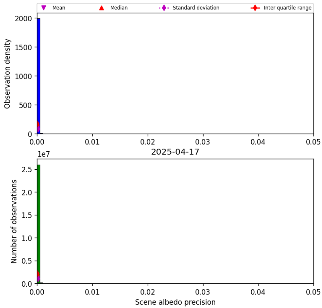
Figure 35: Histogram of “Scene albedo precision” for 2025-04-16 to 2025-04-18
