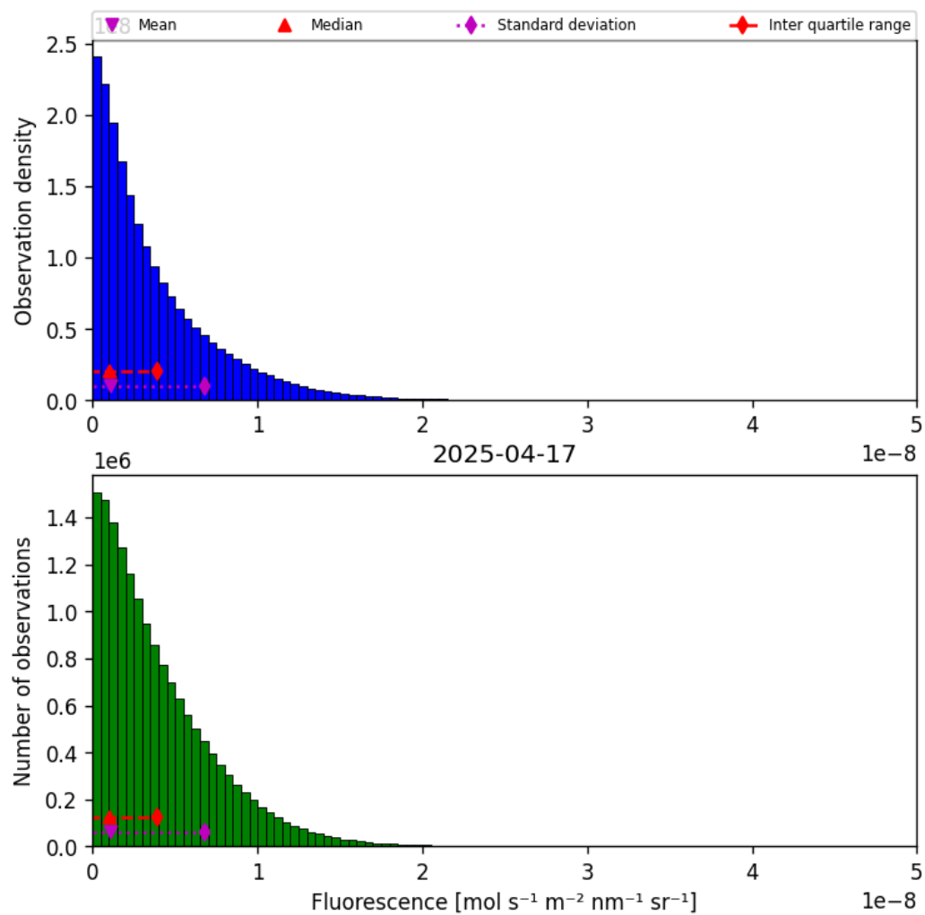
Figure 40: Histogram of “Fluorescence” for 2025-04-16 to 2025-04-18
