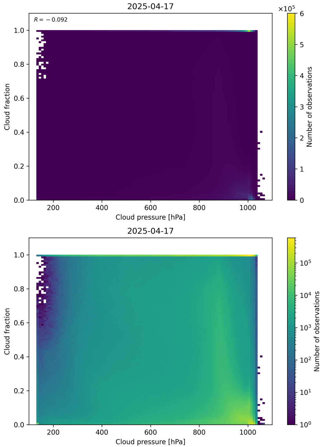
Figure 79: Scatter density plot of “Cloud pressure” against “Cloud fraction” for 2025-04-16 to 2025-04-18.
