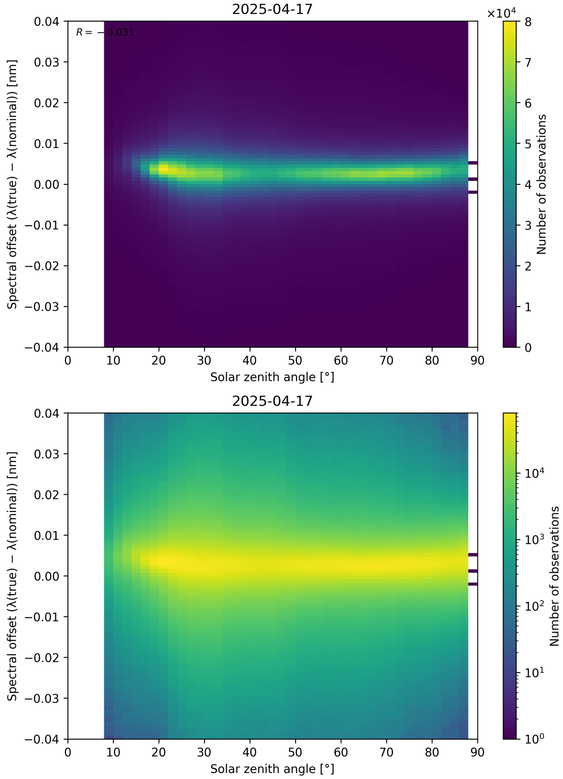
Figure 117: Scatter density plot of “Solar zenith angle” against “Spectral offset ( \lambda_{\text{true}} - \lambda_{\text{nominal}} )” for 2025-04-16 to 2025-04-18.
