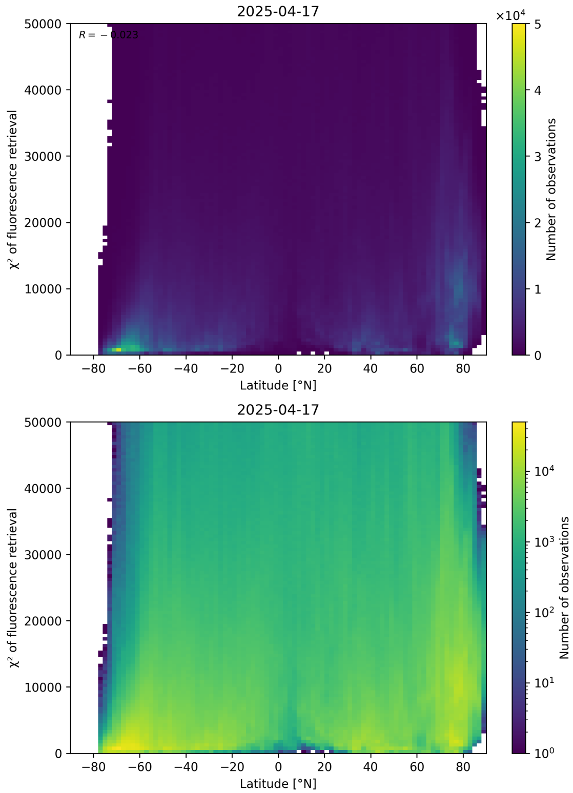
Figure 89: Scatter density plot of “Latitude” against “ \chi^2 of fluorescence retrieval” for 2025-04-16 to 2025-04-18.
