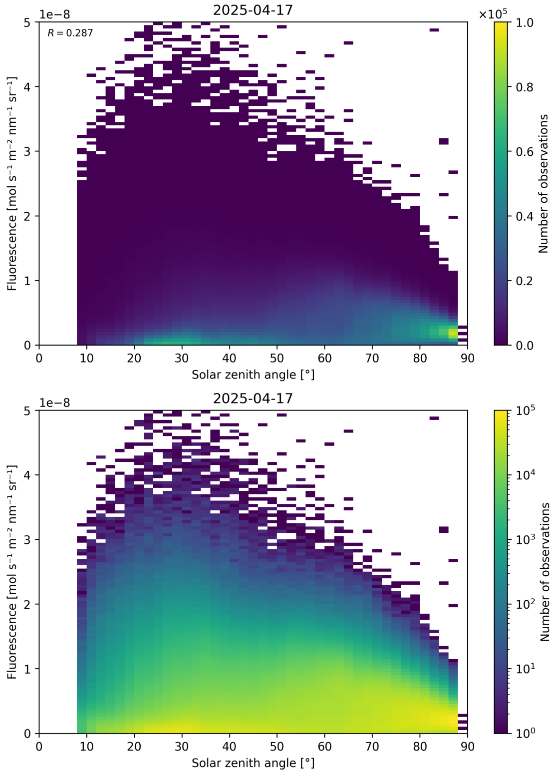
Figure 112: Scatter density plot of “Solar zenith angle” against “Fluorescence” for 2025-04-16 to 2025-04-18.
