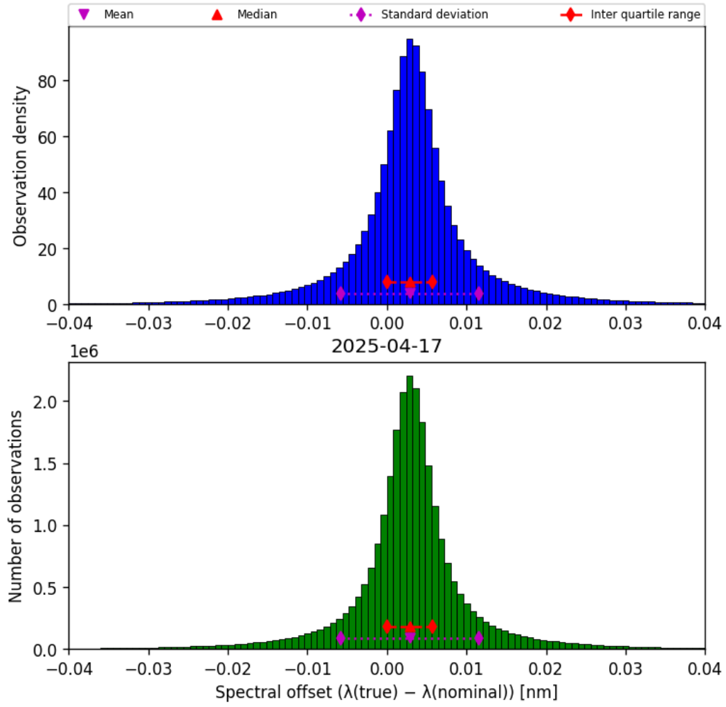
Figure 45: Histogram of “Spectral offset ( \lambda_{\text{true}} - \lambda_{\text{nominal}} )” for 2025-04-16 to 2025-04-18
