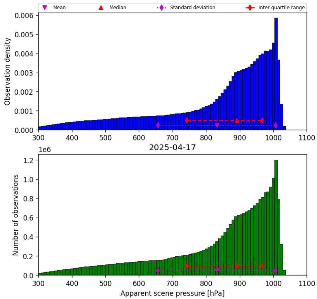
Figure 36: Histogram of “Apparent scene pressure” for 2025-04-16 to 2025-04-18
