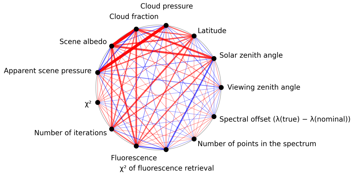
Figure 1: Map of correlation graph for 2025-04-16 to 2025-04-18.
