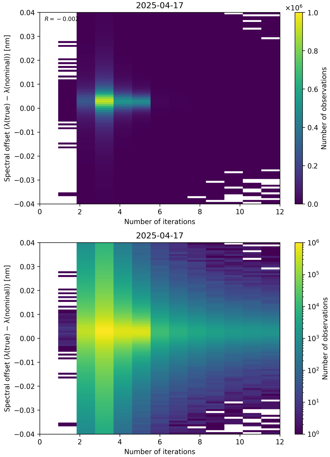
Figure 100: Scatter density plot of “Number of iterations” against “Spectral offset ( \lambda_{\text{true}} - \lambda_{\text{nominal}} )” for 2025-04-16 to 2025-04-18.
