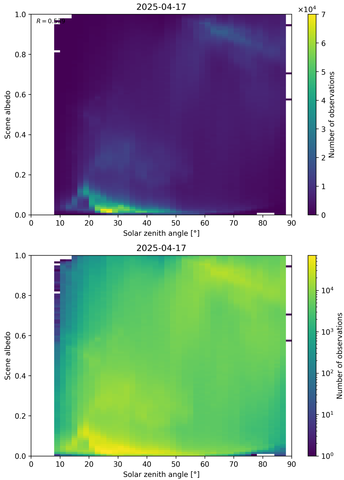
Figure 116: Scatter density plot of “Solar zenith angle” against “Scene albedo” for 2025-04-16 to 2025-04-18.
