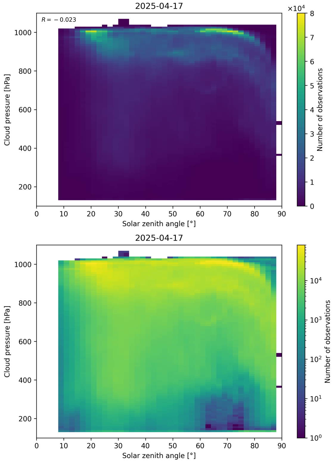
Figure 111: Scatter density plot of “Solar zenith angle” against “Cloud pressure” for 2025-04-16 to 2025-04-18.
