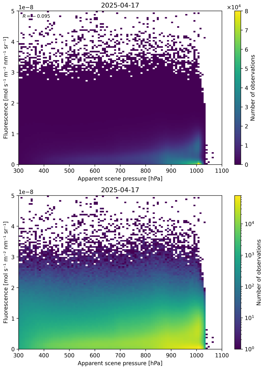
Figure 64: Scatter density plot of “Apparent scene pressure” against “Fluorescence” for 2025-04-16 to 2025-04-18.
