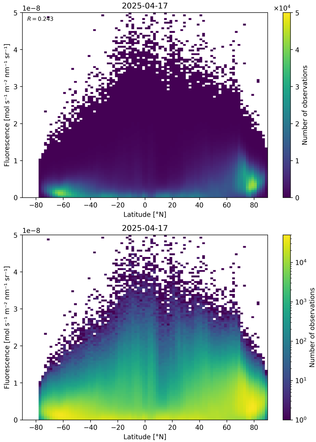
Figure 92: Scatter density plot of “Latitude” against “Fluorescence” for 2025-04-16 to 2025-04-18.
