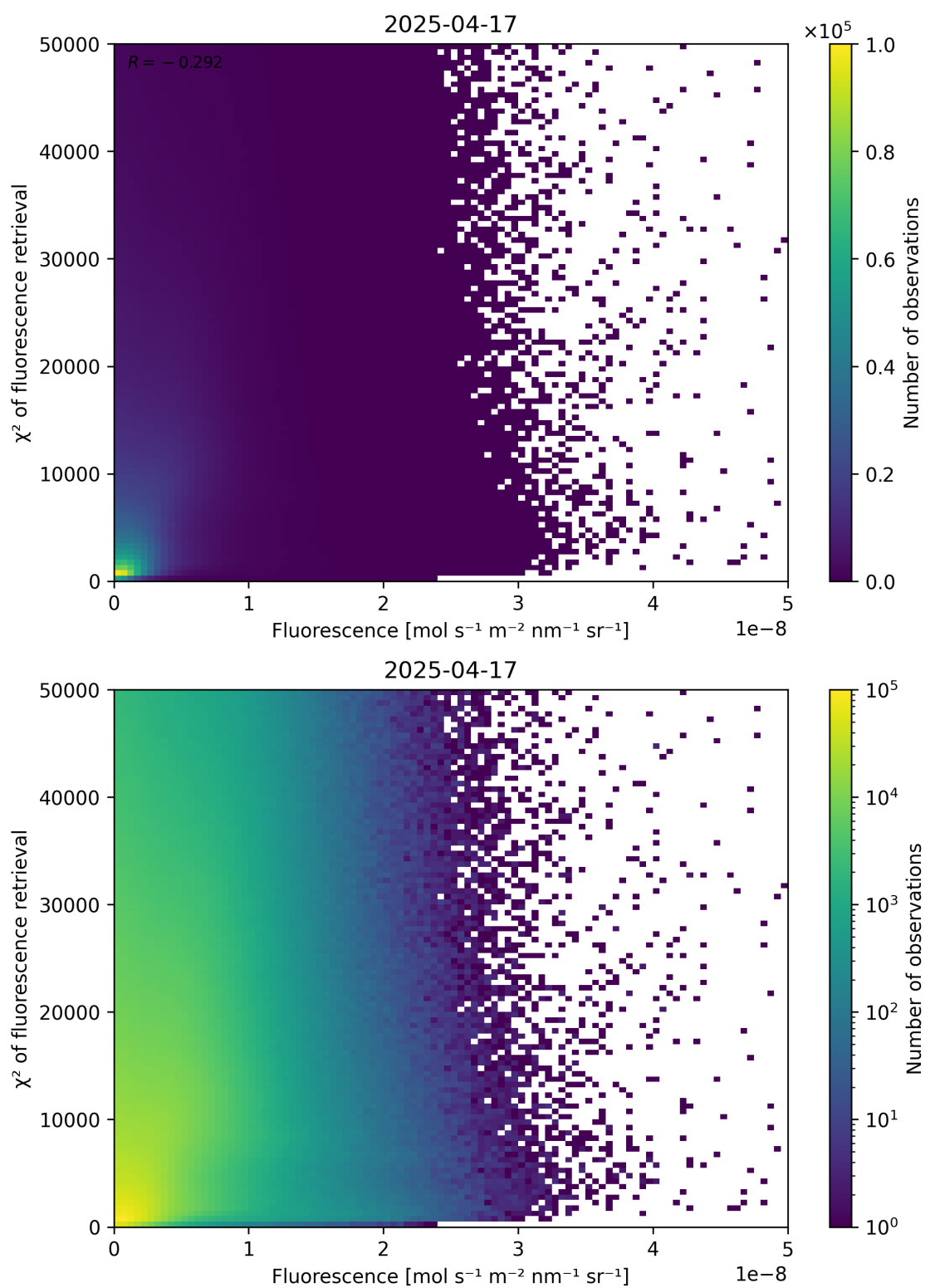
Figure 85: Scatter density plot of “Fluorescence” against “ \chi^2 of fluorescence retrieval” for 2025-04-16 to 2025-04-18.
