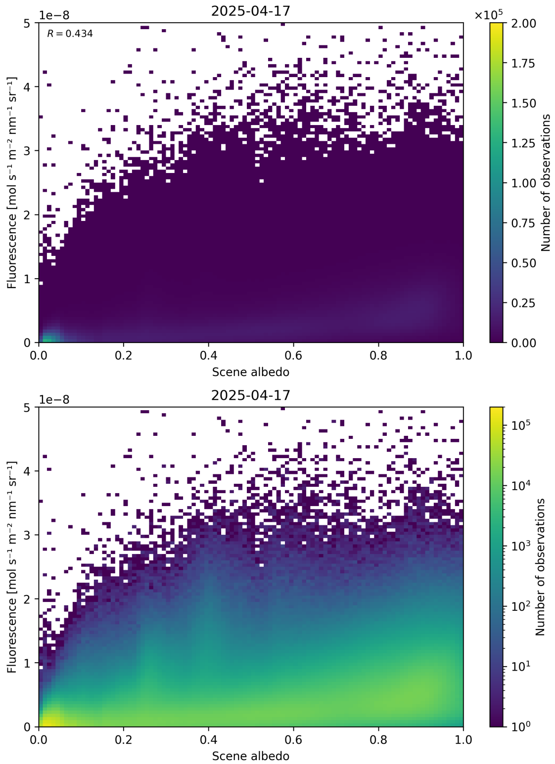
Figure 104: Scatter density plot of “Scene albedo” against “Fluorescence” for 2025-04-16 to 2025-04-18.
