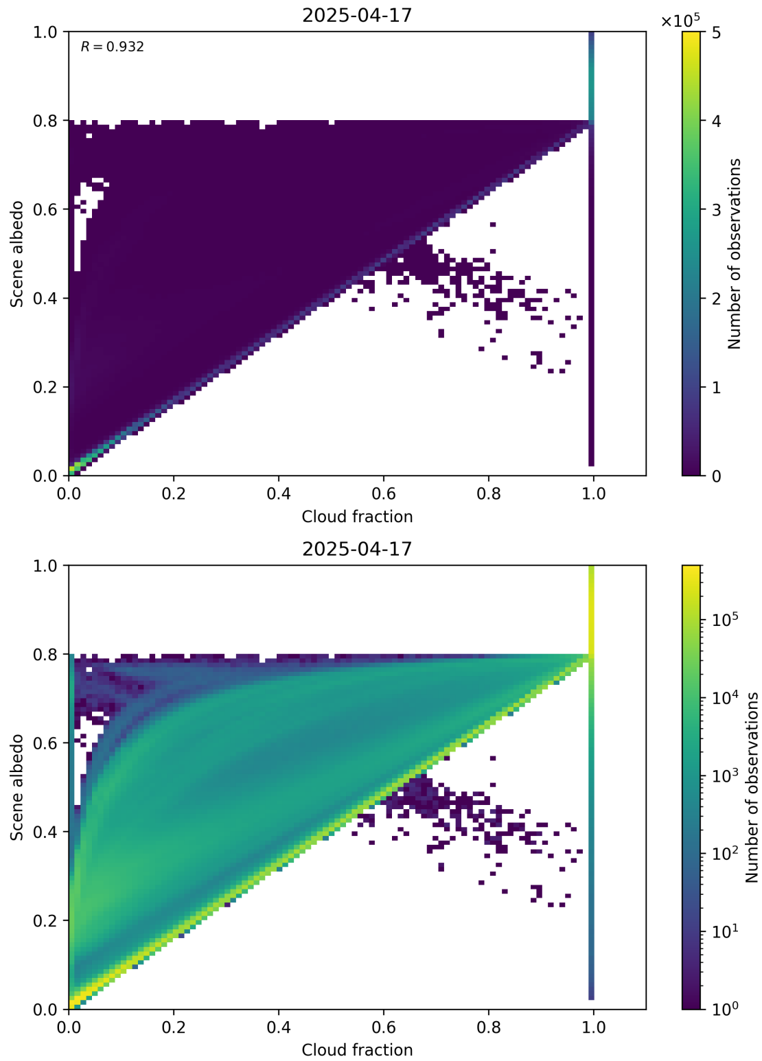
Figure 75: Scatter density plot of “Cloud fraction” against “Scene albedo” for 2025-04-16 to 2025-04-18.
