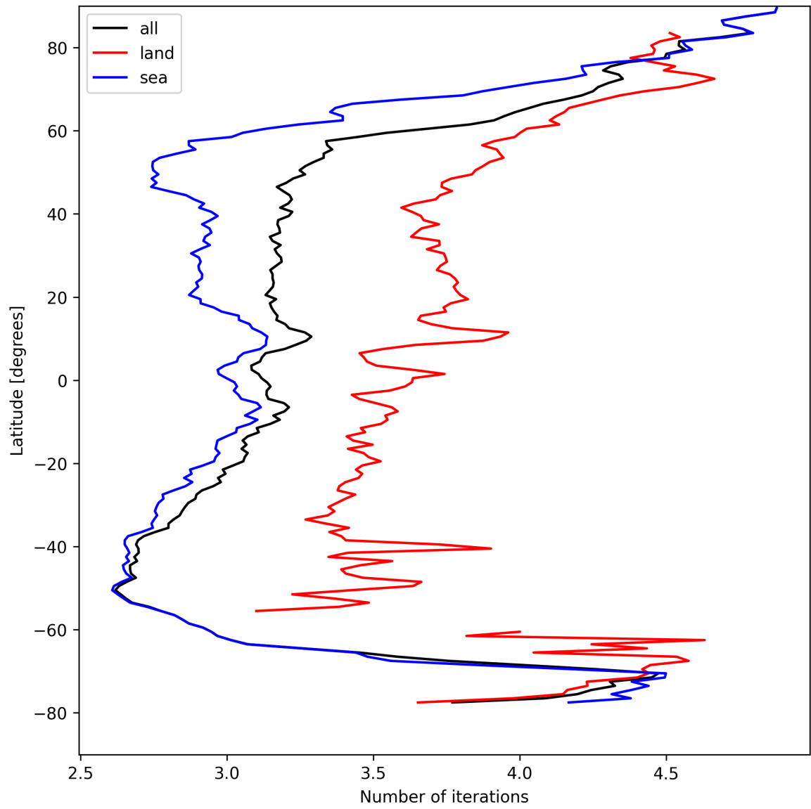
Figure 22: Zonal average of “Number of iterations” for 2025-04-16 to 2025-04-18.
