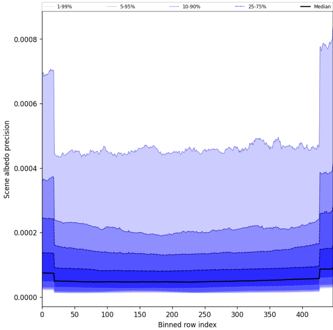
Figure 52: Along track statistics of “Scene albedo precision” for 2025-04-16 to 2025-04-18
