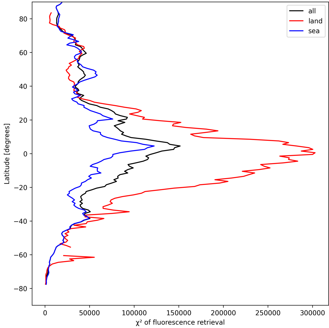
Figure 25: Zonal average of “ \chi^2 of fluorescence retrieval” for 2025-04-16 to 2025-04-18.
