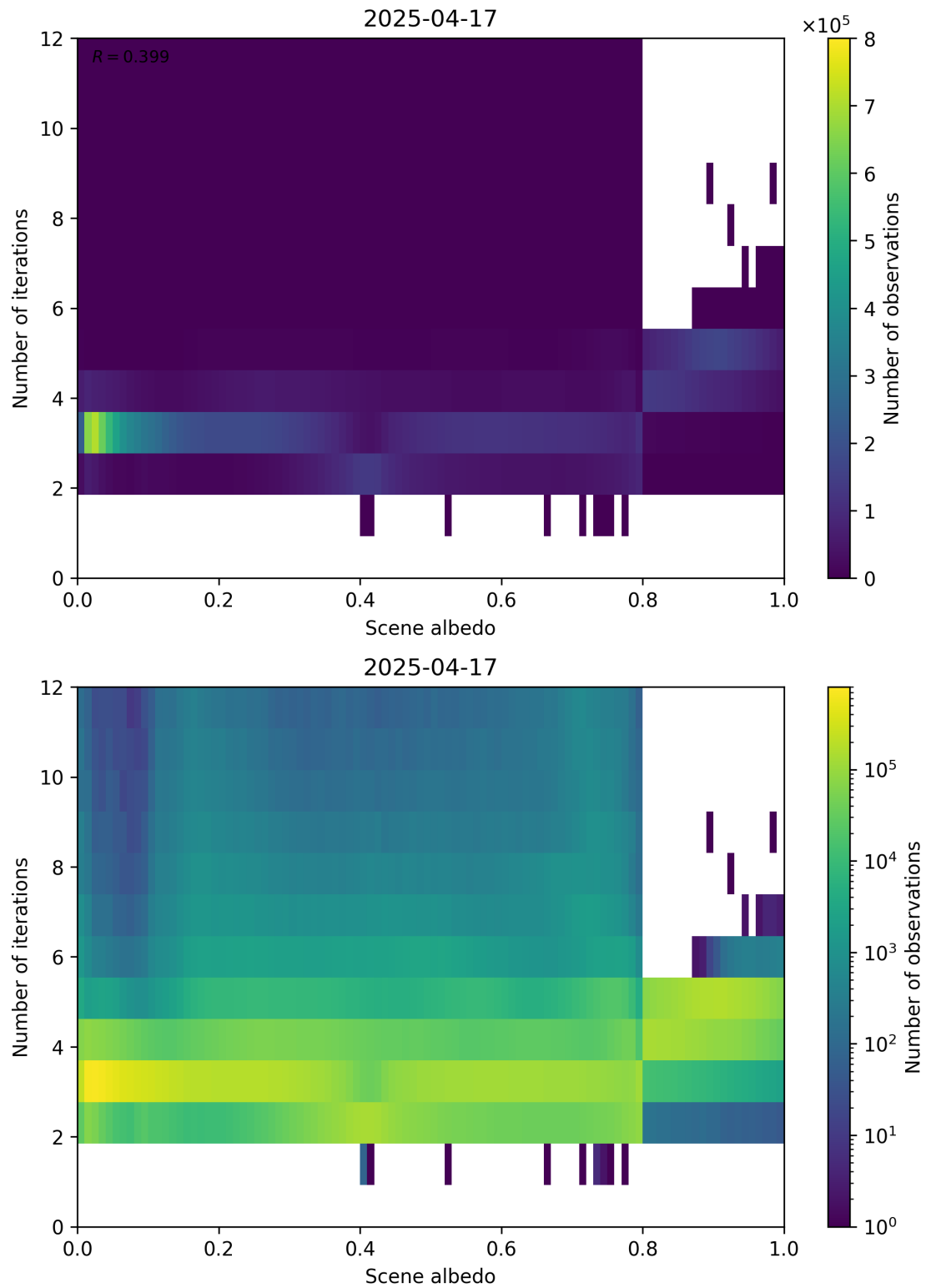
Figure 105: Scatter density plot of “Scene albedo” against “Number of iterations” for 2025-04-16 to 2025-04-18.
