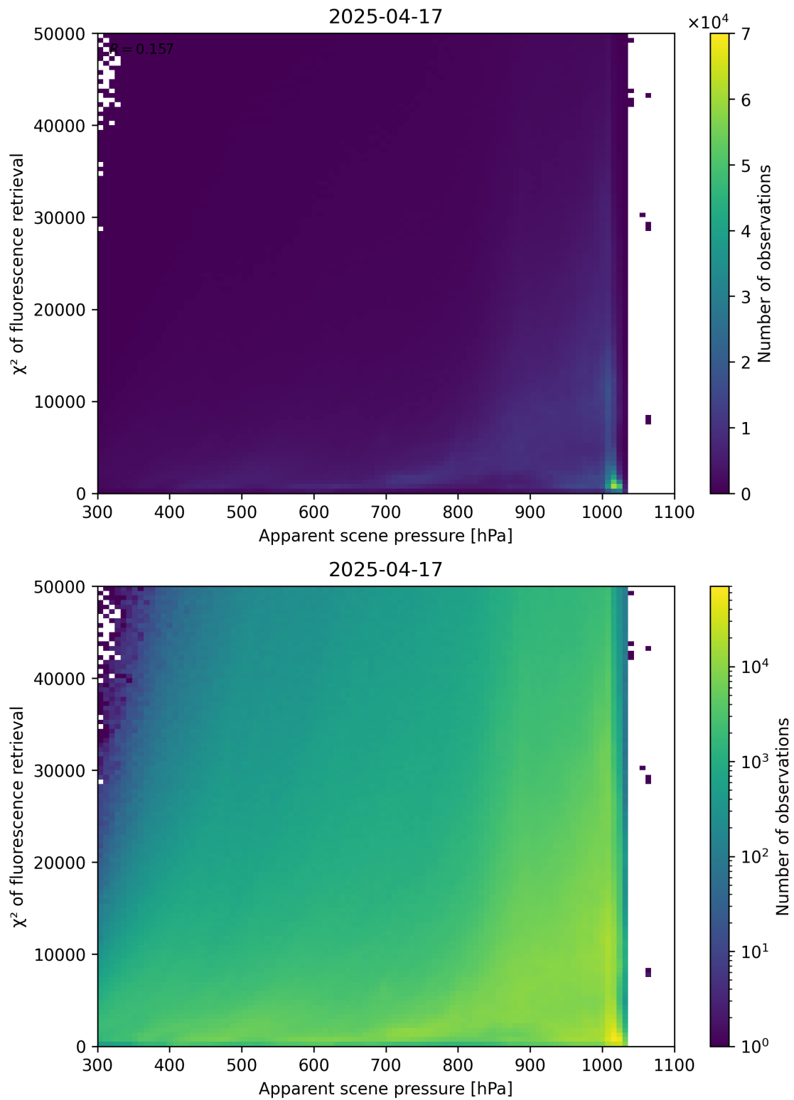
Figure 63: Scatter density plot of “Apparent scene pressure” against “ \chi^2 of fluorescence retrieval” for 2025-04-16 to 2025-04-18.
