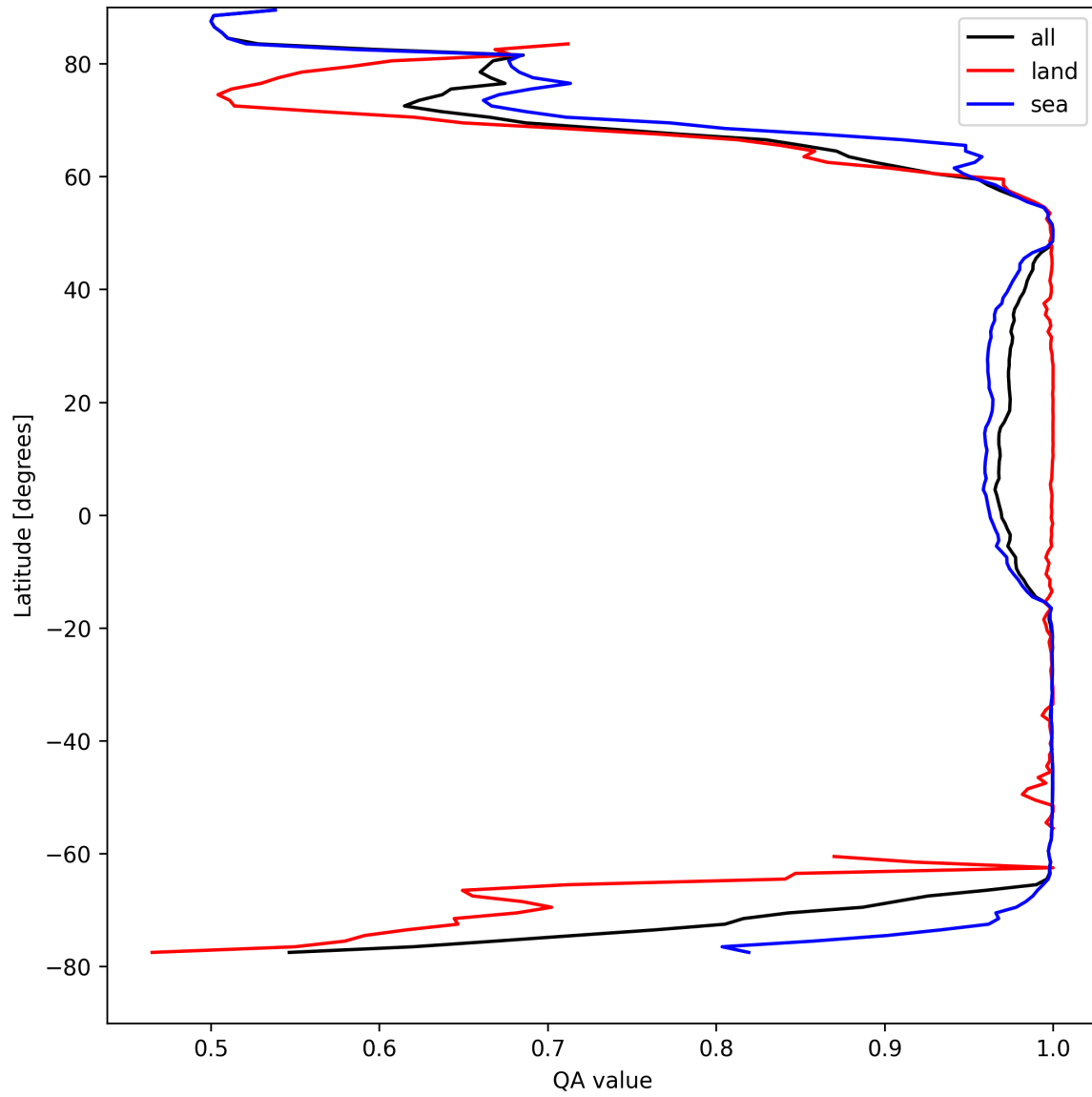
Figure 12: Zonal average of “QA value” for 2025-04-16 to 2025-04-18.
