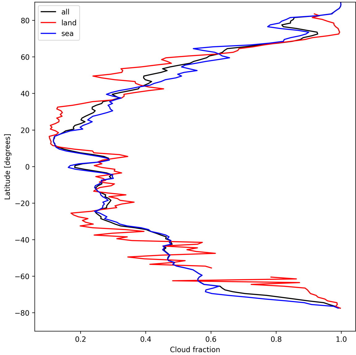
Figure 15: Zonal average of “Cloud fraction” for 2025-04-16 to 2025-04-18.
