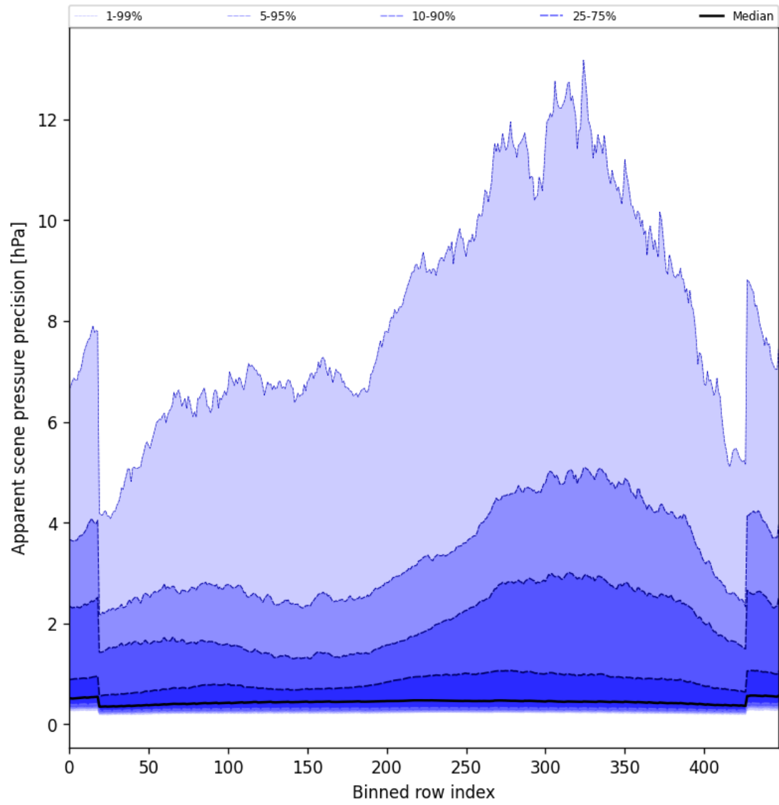
Figure 54: Along track statistics of “Apparent scene pressure precision” for 2025-04-16 to 2025-04-18
