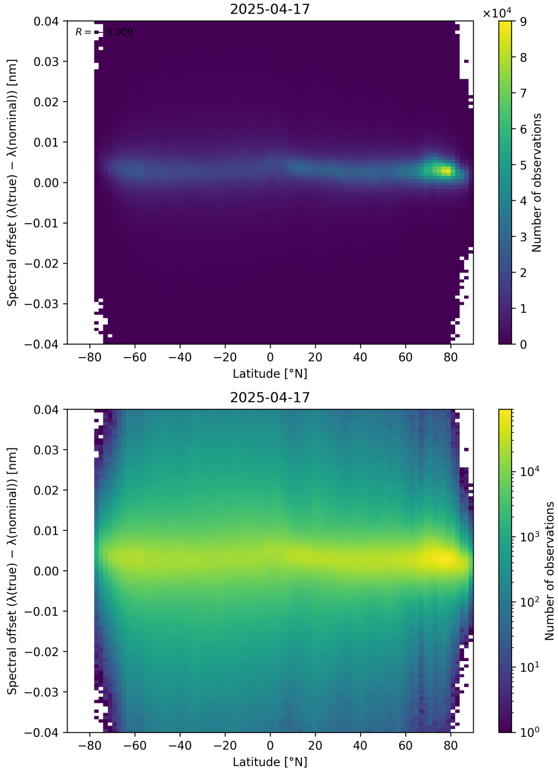
Figure 96: Scatter density plot of “Latitude” against “Spectral offset ( \lambda_{\text{true}} - \lambda_{\text{nominal}} )” for 2025-04-16 to 2025-04-18.
