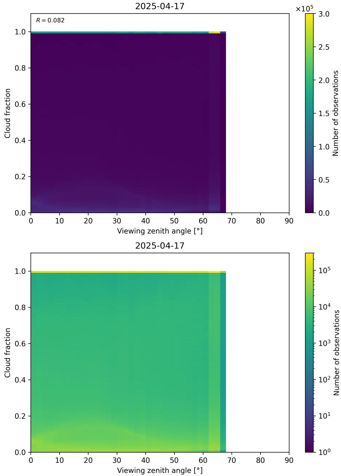
Figure 120: Scatter density plot of “Viewing zenith angle” against “Cloud fraction” for 2025-04-16 to 2025-04-18.
