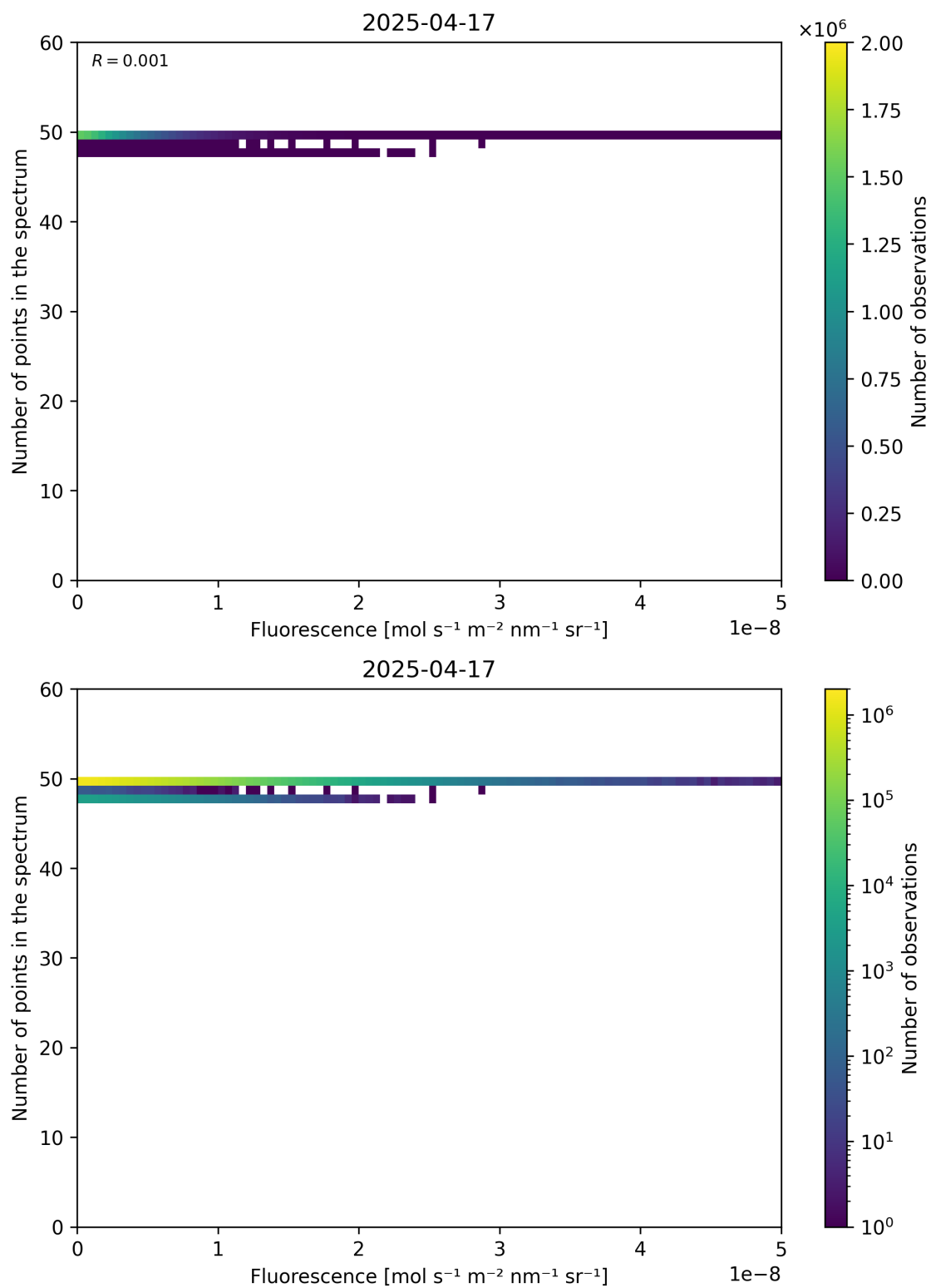
Figure 86: Scatter density plot of “Fluorescence” against “Number of points in the spectrum” for 2025-04-16 to 2025-04-18.
