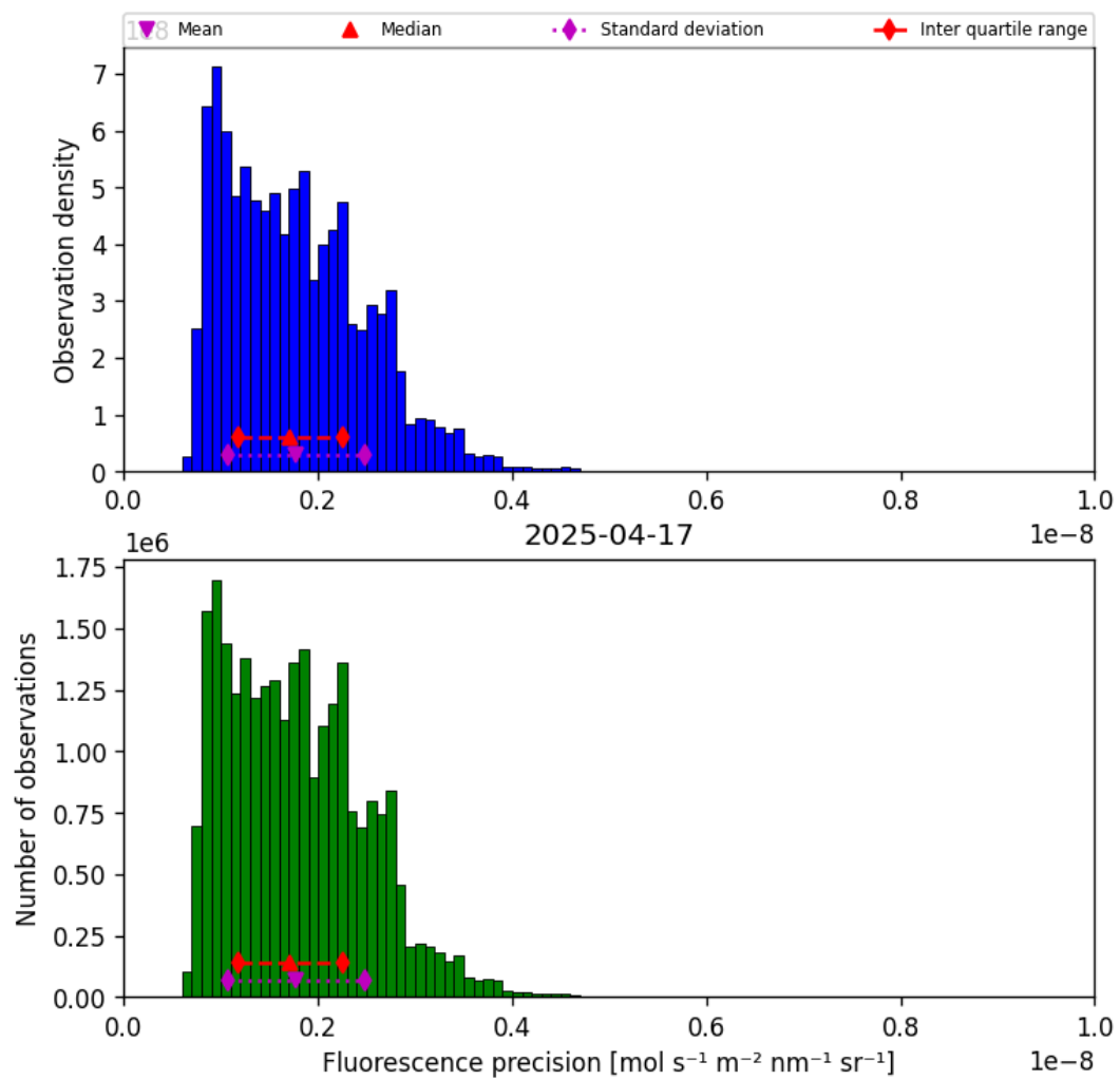
Figure 41: Histogram of “Fluorescence precision” for 2025-04-16 to 2025-04-18
