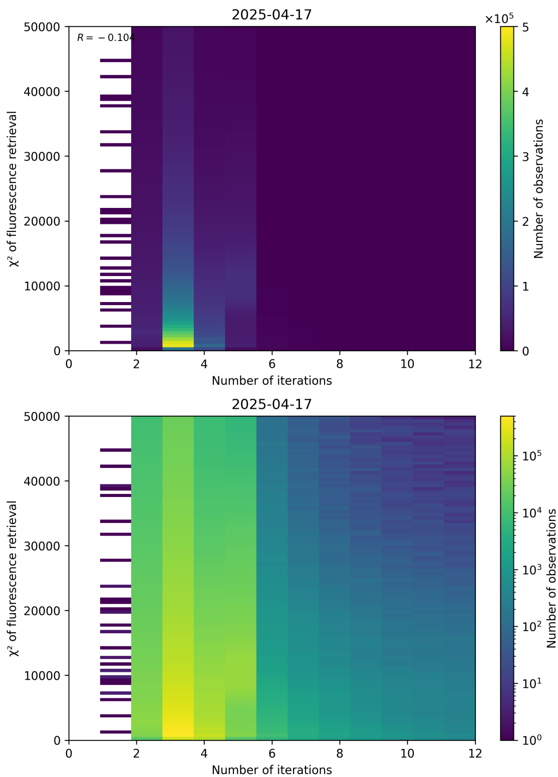
Figure 97: Scatter density plot of “Number of iterations” against “ \chi^2 of fluorescence retrieval” for 2025-04-16 to 2025-04-18.
