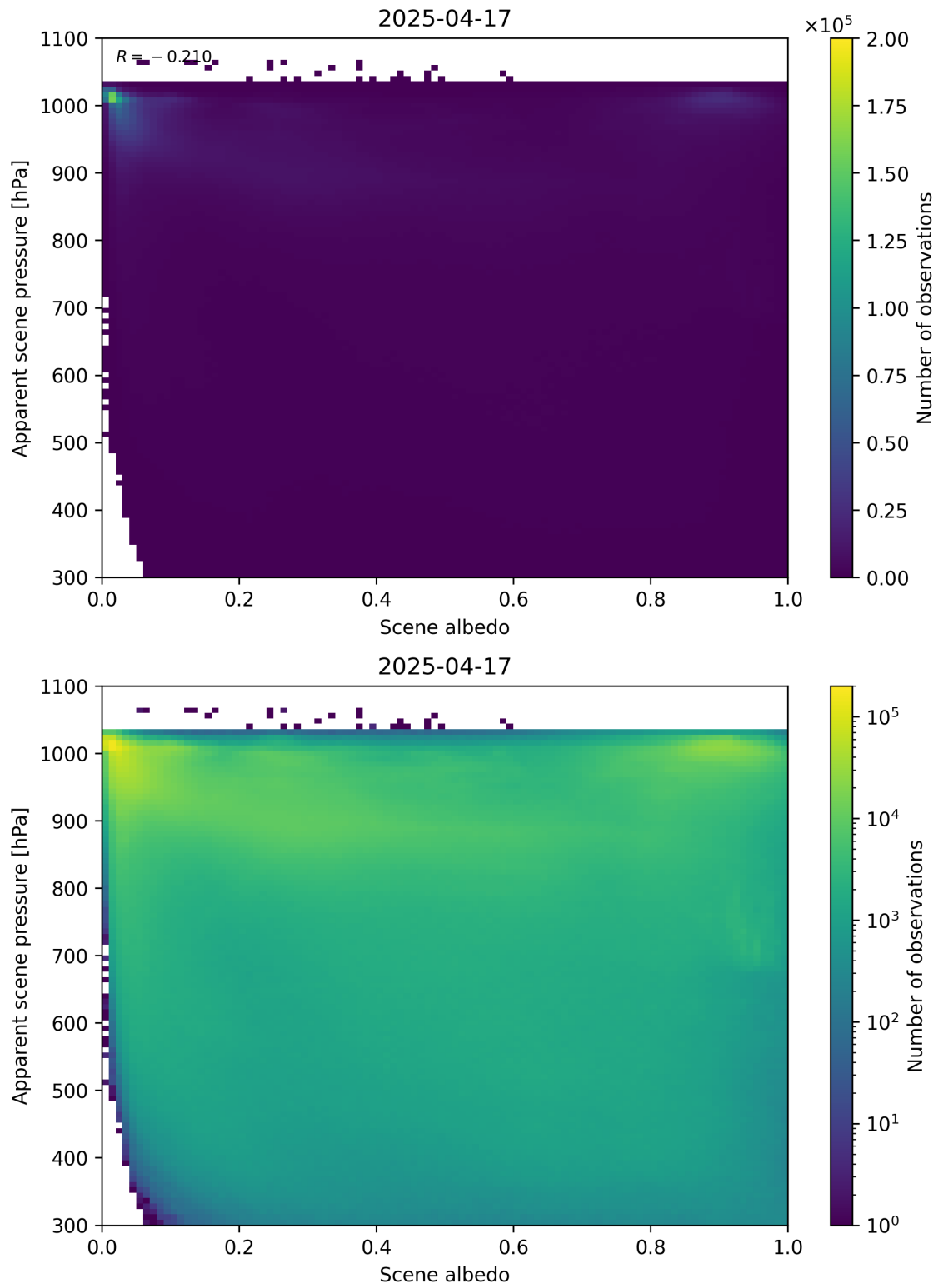
Figure 102: Scatter density plot of “Scene albedo” against “Apparent scene pressure” for 2025-04-16 to 2025-04-18.
