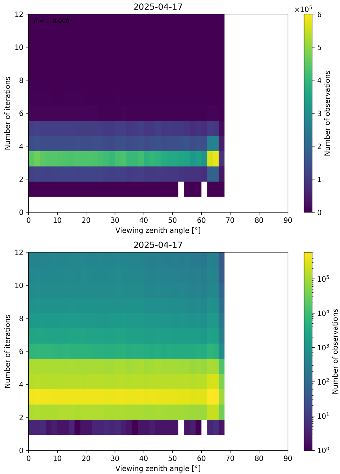
Figure 124: Scatter density plot of “Viewing zenith angle” against “Number of iterations” for 2025-04-16 to 2025-04-18.
