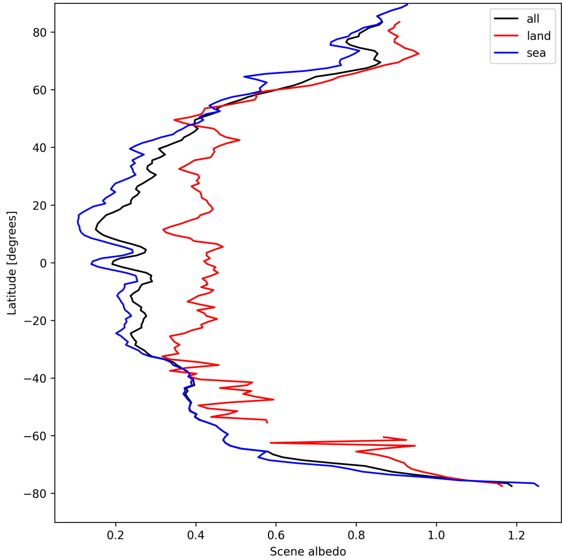
Figure 17: Zonal average of “Scene albedo” for 2025-04-16 to 2025-04-18.
