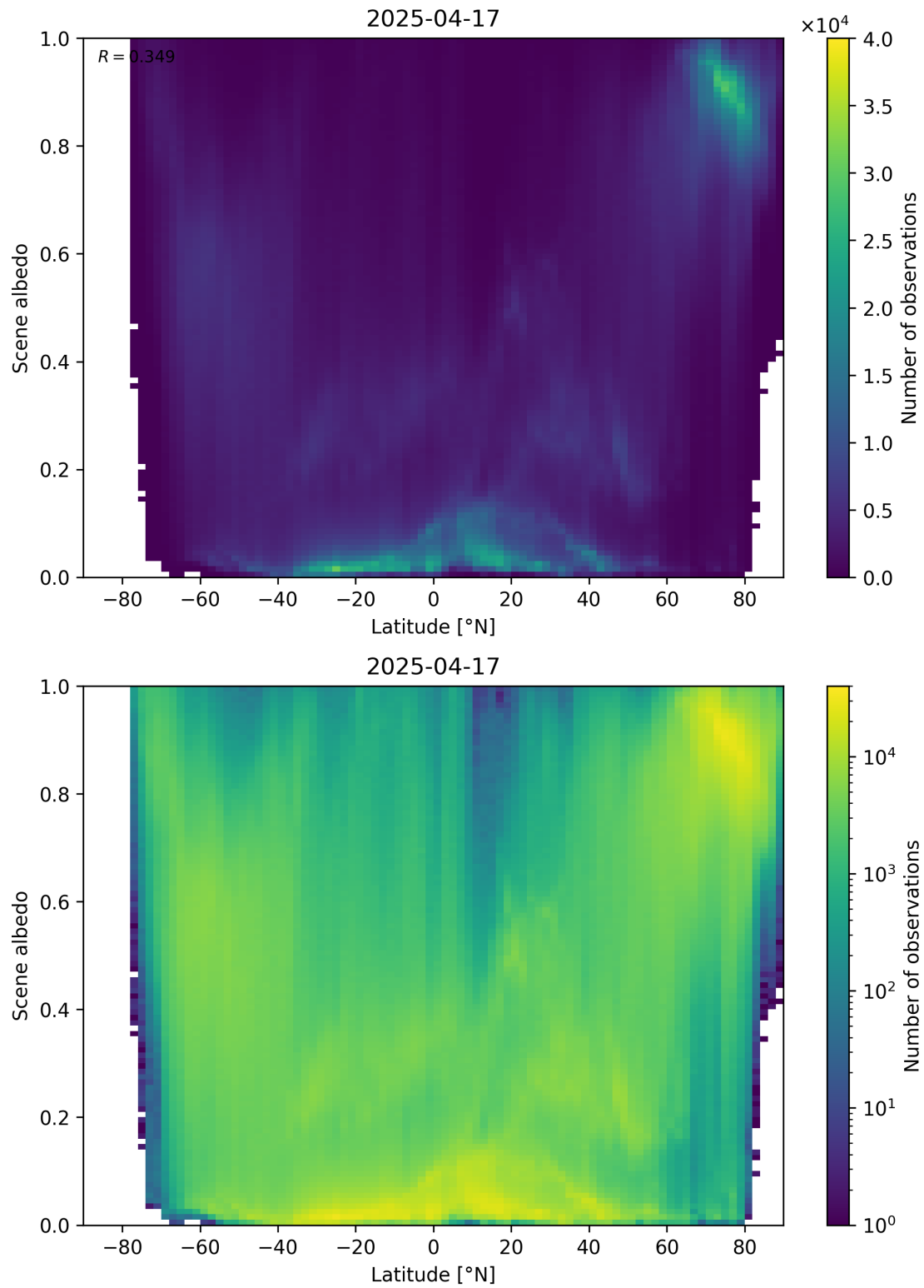
Figure 95: Scatter density plot of “Latitude” against “Scene albedo” for 2025-04-16 to 2025-04-18.
