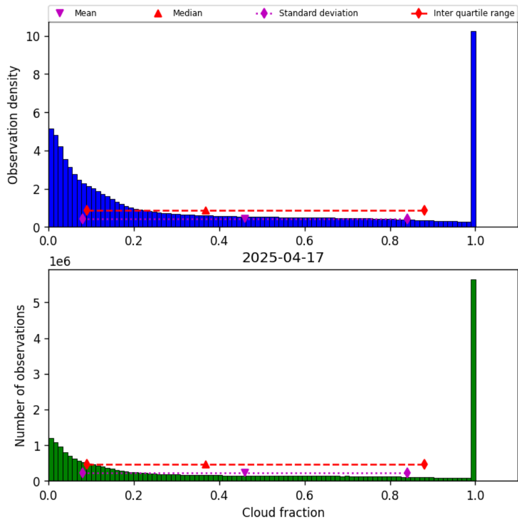
Figure 32: Histogram of “Cloud fraction” for 2025-04-16 to 2025-04-18
