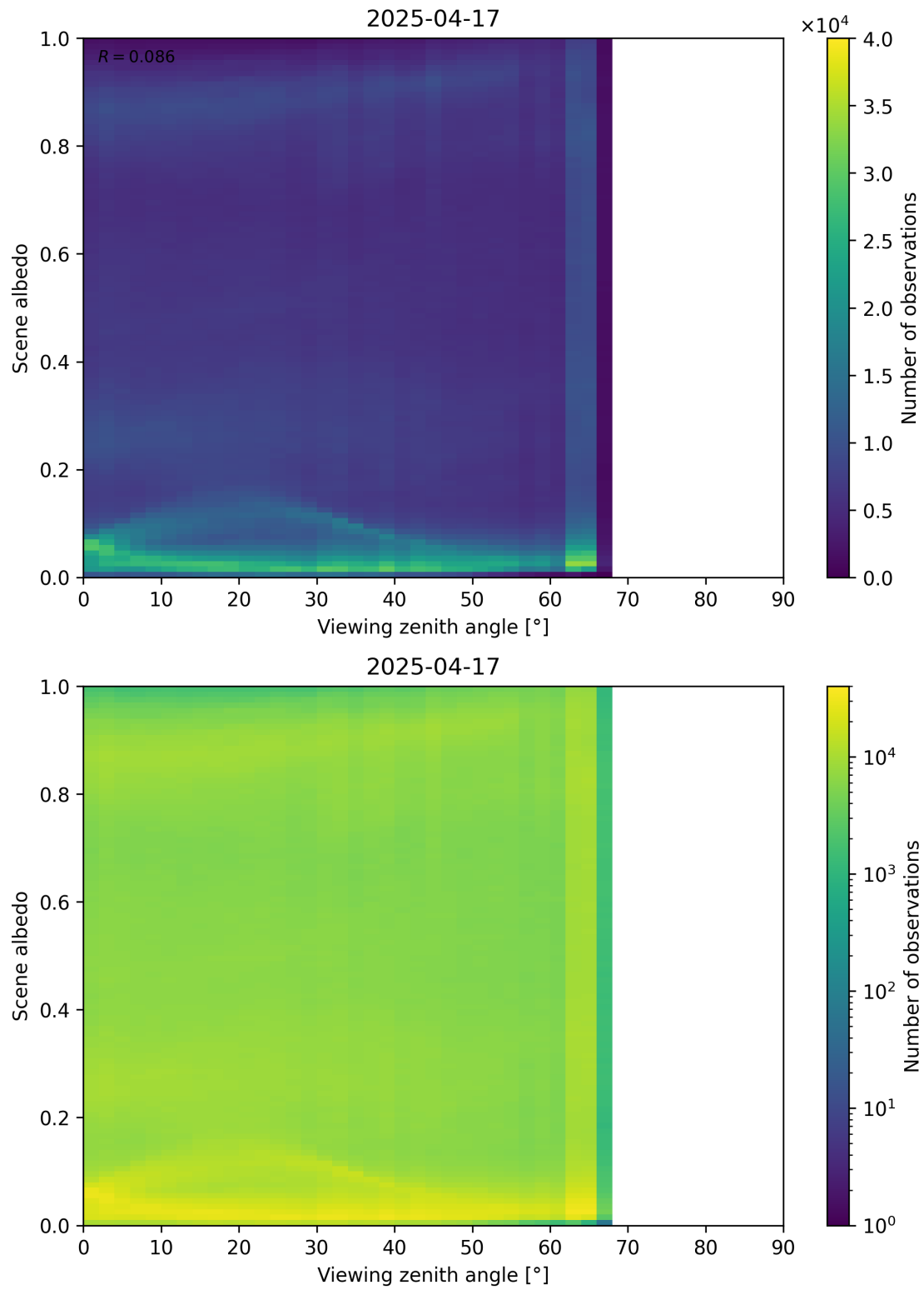
Figure 126: Scatter density plot of “Viewing zenith angle” against “Scene albedo” for 2025-04-16 to 2025-04-18.
