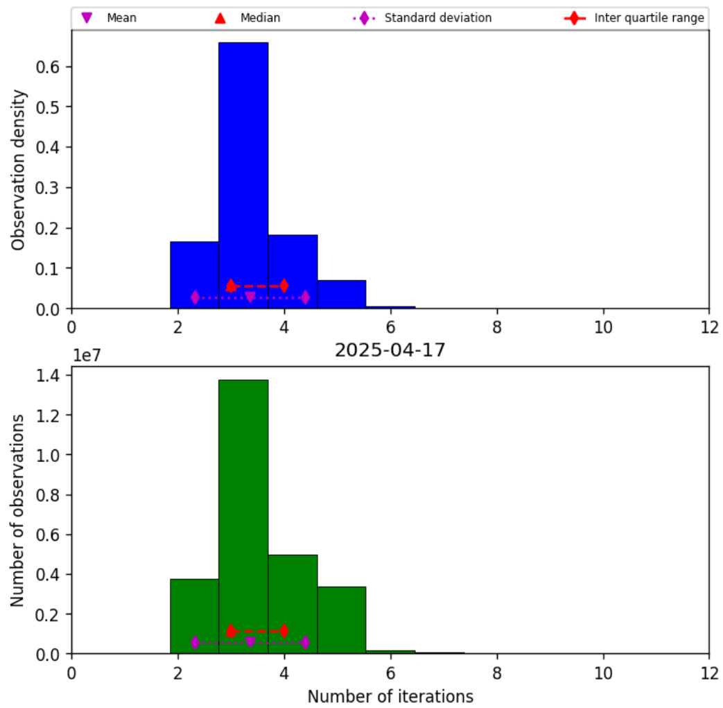
Figure 39: Histogram of “Number of iterations” for 2025-04-16 to 2025-04-18
