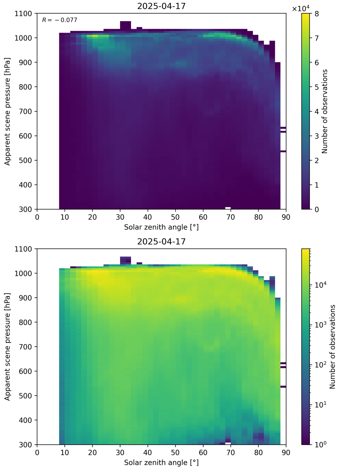
Figure 108: Scatter density plot of “Solar zenith angle” against “Apparent scene pressure” for 2025-04-16 to 2025-04-18.
