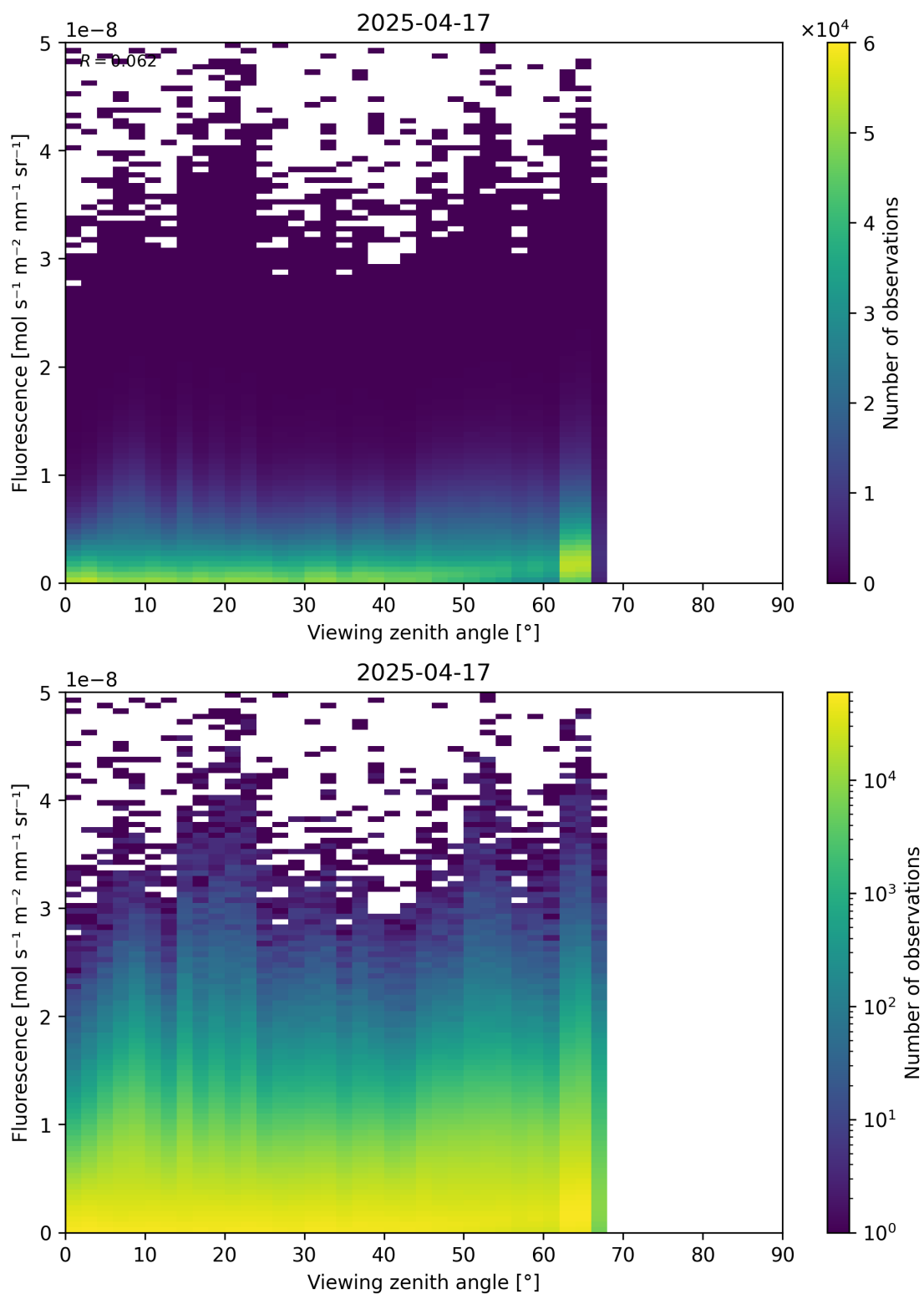
Figure 122: Scatter density plot of “Viewing zenith angle” against “Fluorescence” for 2025-04-16 to 2025-04-18.
