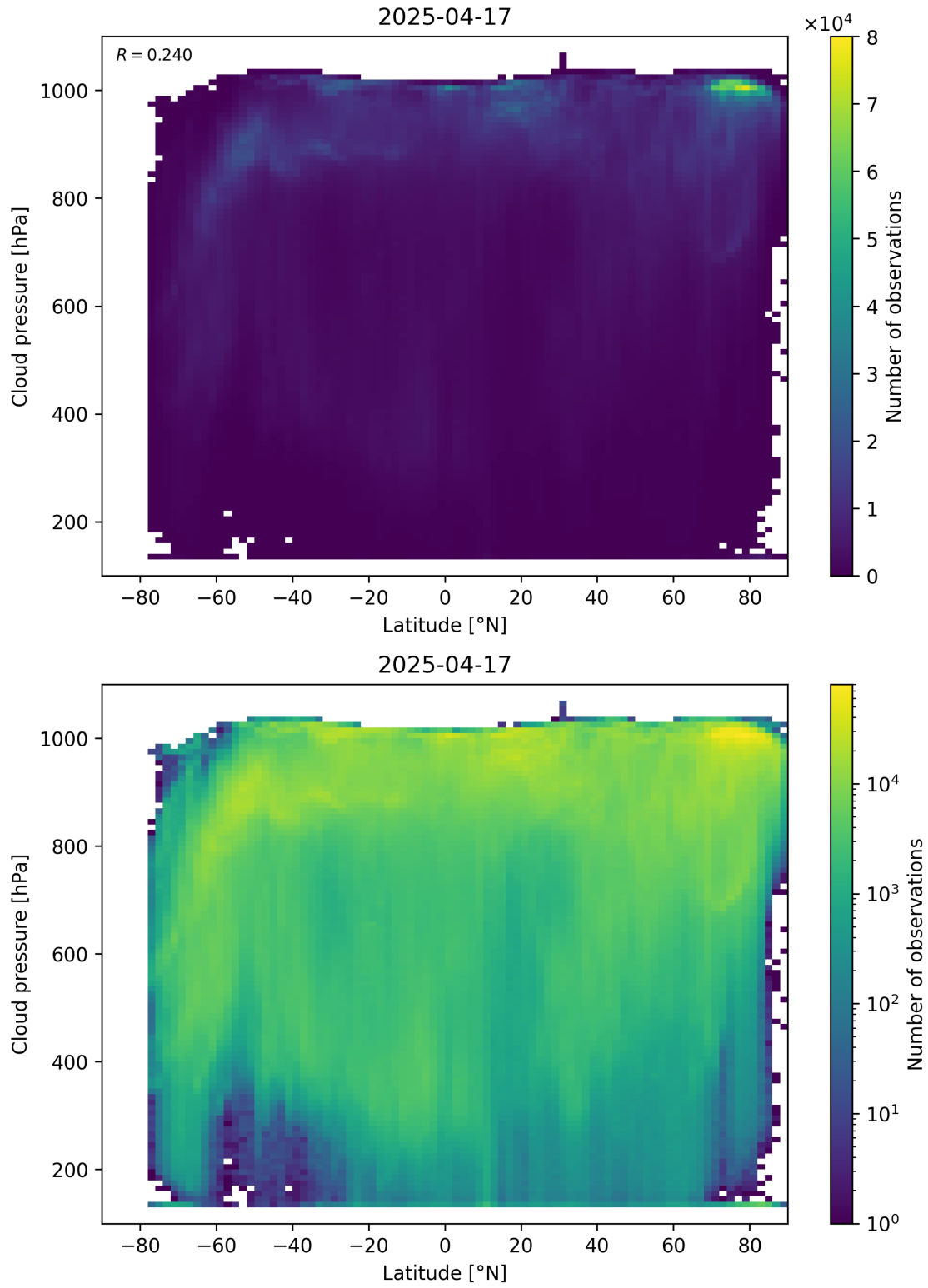
Figure 91: Scatter density plot of “Latitude” against “Cloud pressure” for 2025-04-16 to 2025-04-18.
