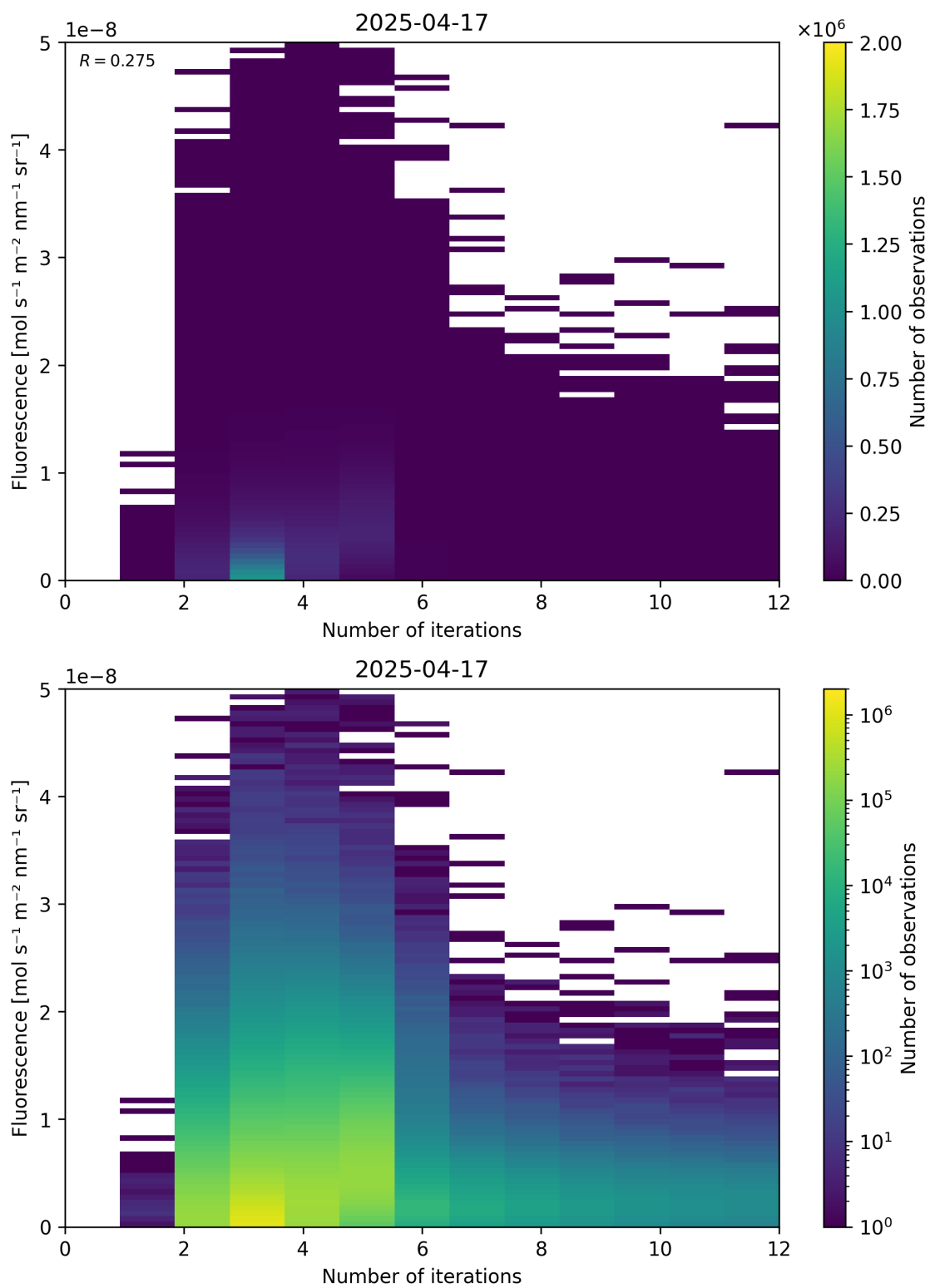
Figure 98: Scatter density plot of “Number of iterations” against “Fluorescence” for 2025-04-16 to 2025-04-18.
