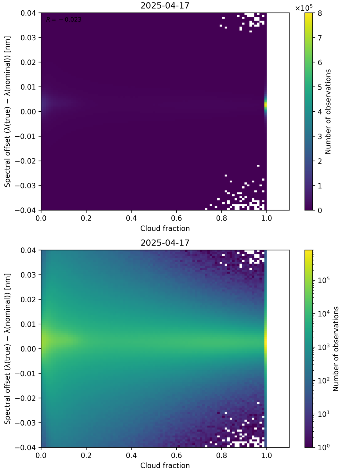
Figure 76: Scatter density plot of “Cloud fraction” against “Spectral offset ( \lambda_{\text{true}} - \lambda_{\text{nominal}} )” for 2025-04-16 to 2025-04-18.
