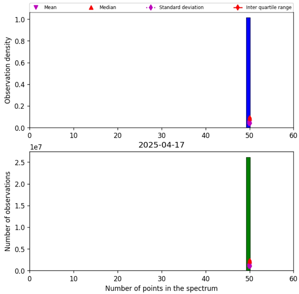
Figure 44: Histogram of “Number of points in the spectrum” for 2025-04-16 to 2025-04-18
