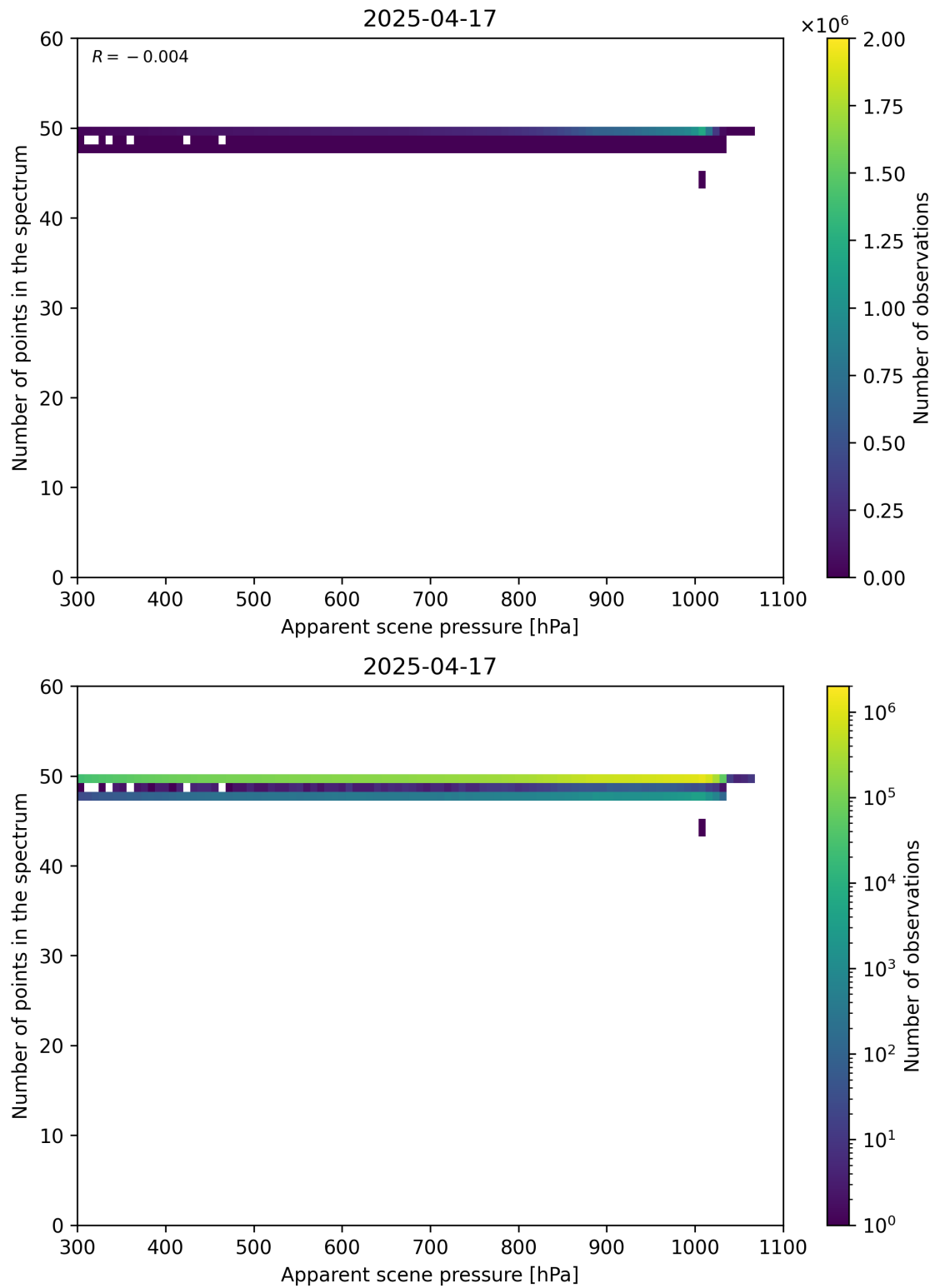
Figure 66: Scatter density plot of “Apparent scene pressure” against “Number of points in the spectrum” for 2025-04-16 to 2025-04-18.
