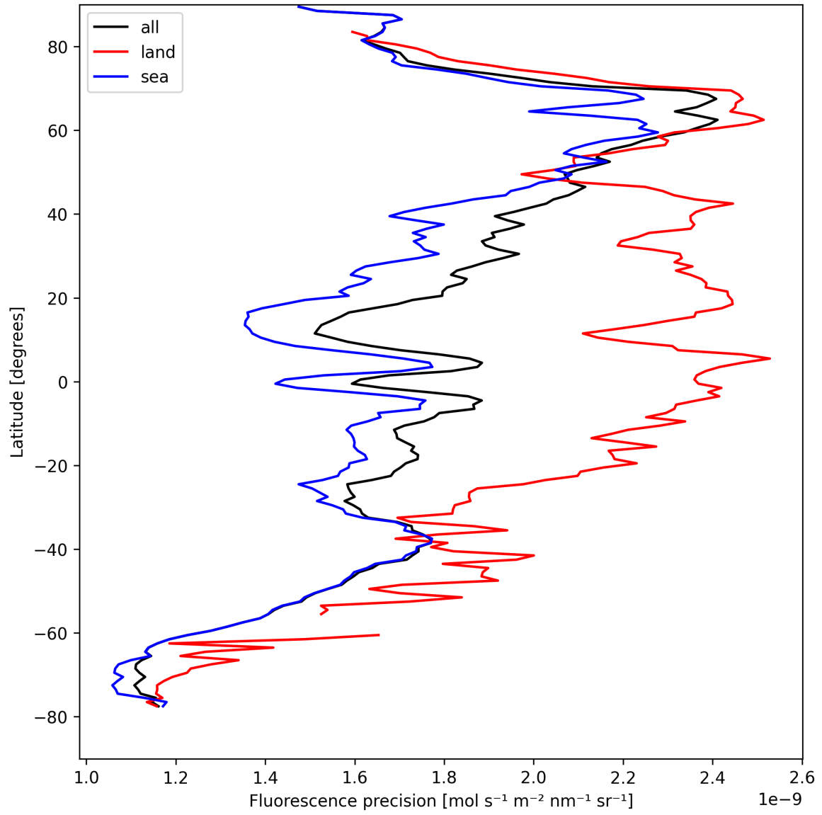
Figure 24: Zonal average of “Fluorescence precision” for 2025-04-16 to 2025-04-18.
