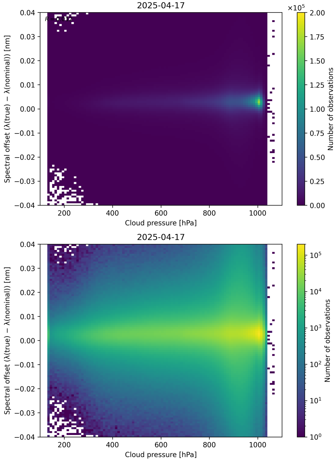
Figure 84: Scatter density plot of “Cloud pressure” against “Spectral offset ( \lambda_{\text{true}} - \lambda_{\text{nominal}} )” for 2025-04-16 to 2025-04-18.
