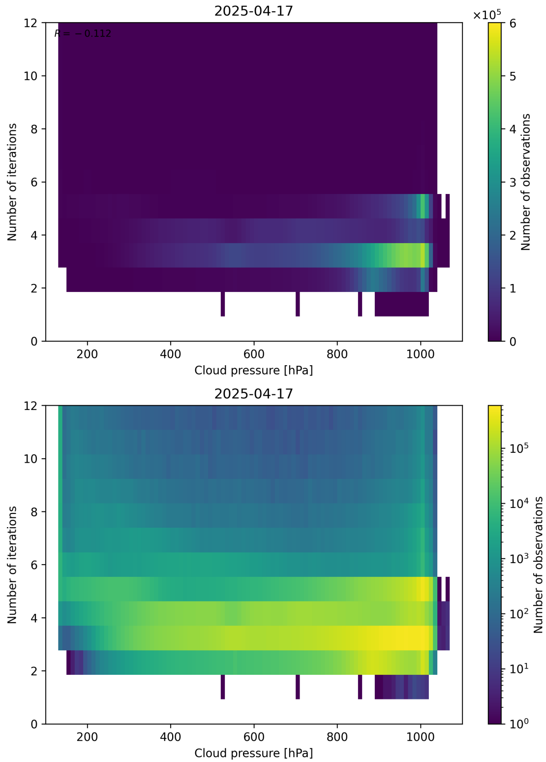
Figure 81: Scatter density plot of “Cloud pressure” against “Number of iterations” for 2025-04-16 to 2025-04-18.
