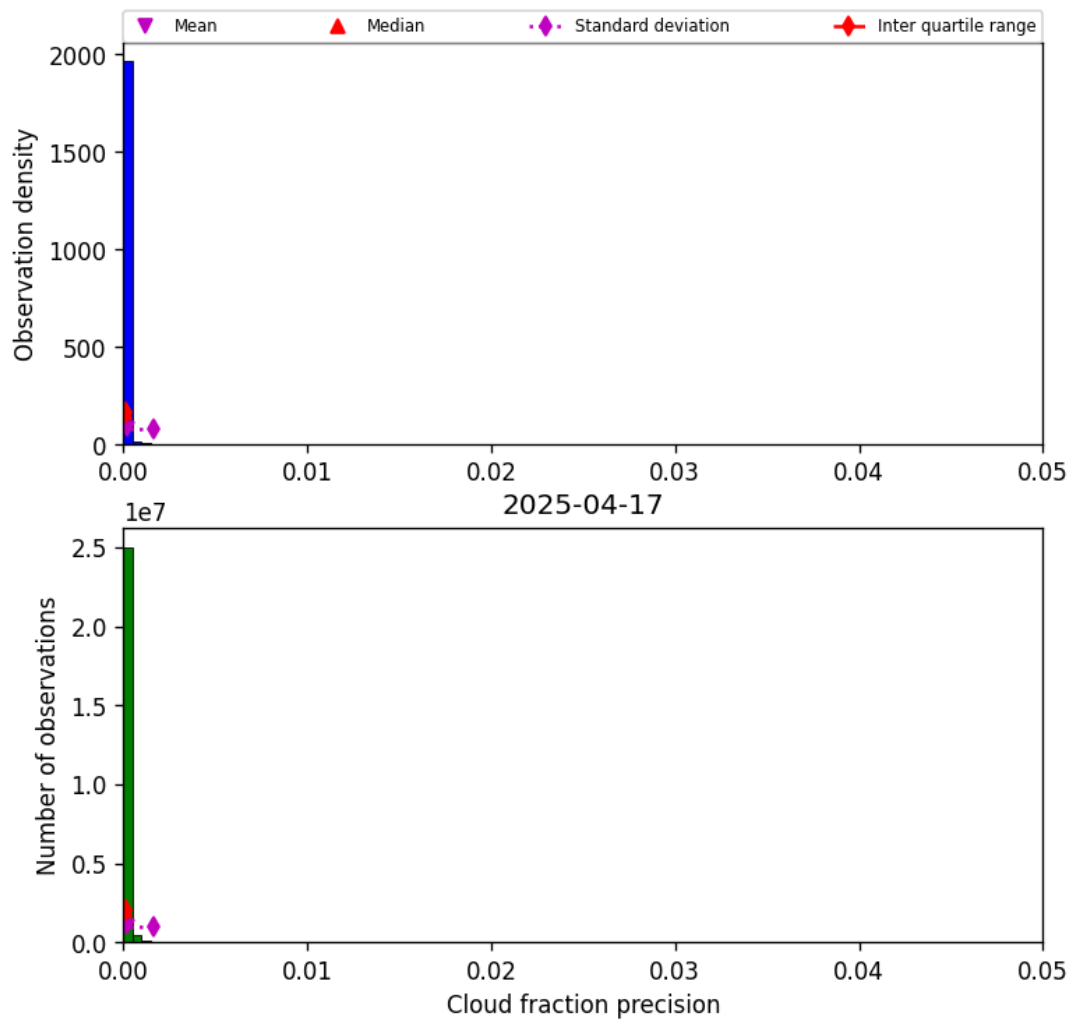
Figure 33: Histogram of “Cloud fraction precision” for 2025-04-16 to 2025-04-18
