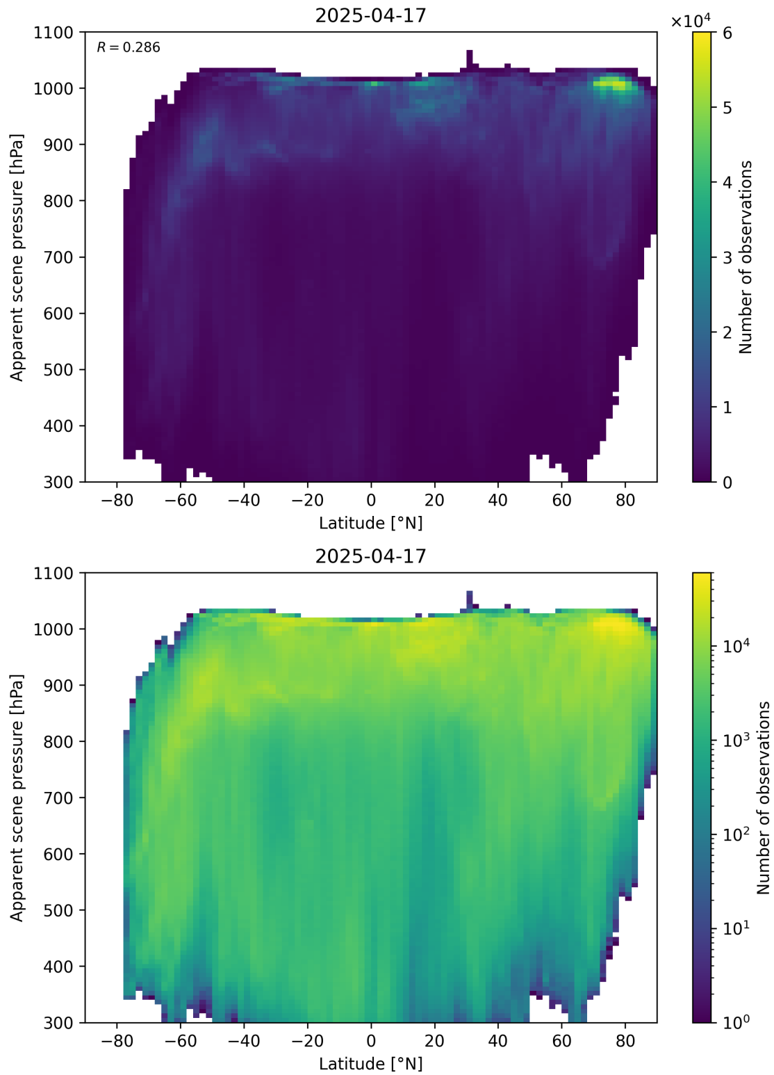
Figure 88: Scatter density plot of “Latitude” against “Apparent scene pressure” for 2025-04-16 to 2025-04-18.
