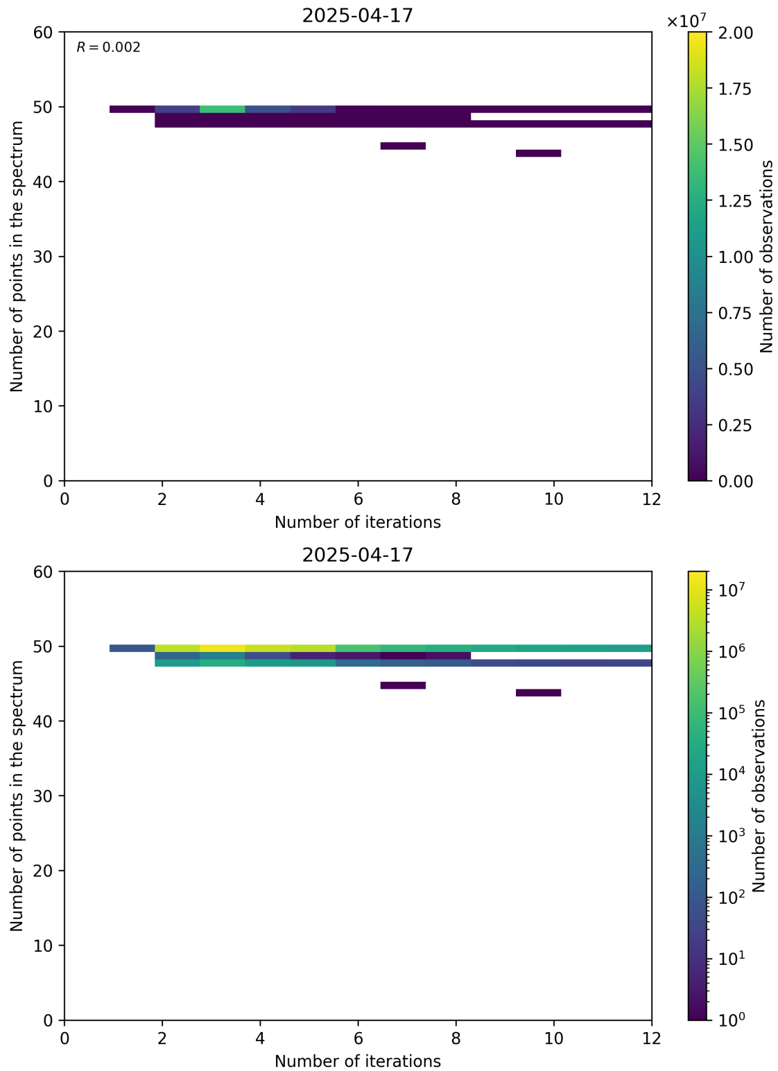
Figure 99: Scatter density plot of “Number of iterations” against “Number of points in the spectrum” for 2025-04-16 to 2025-04-18.
