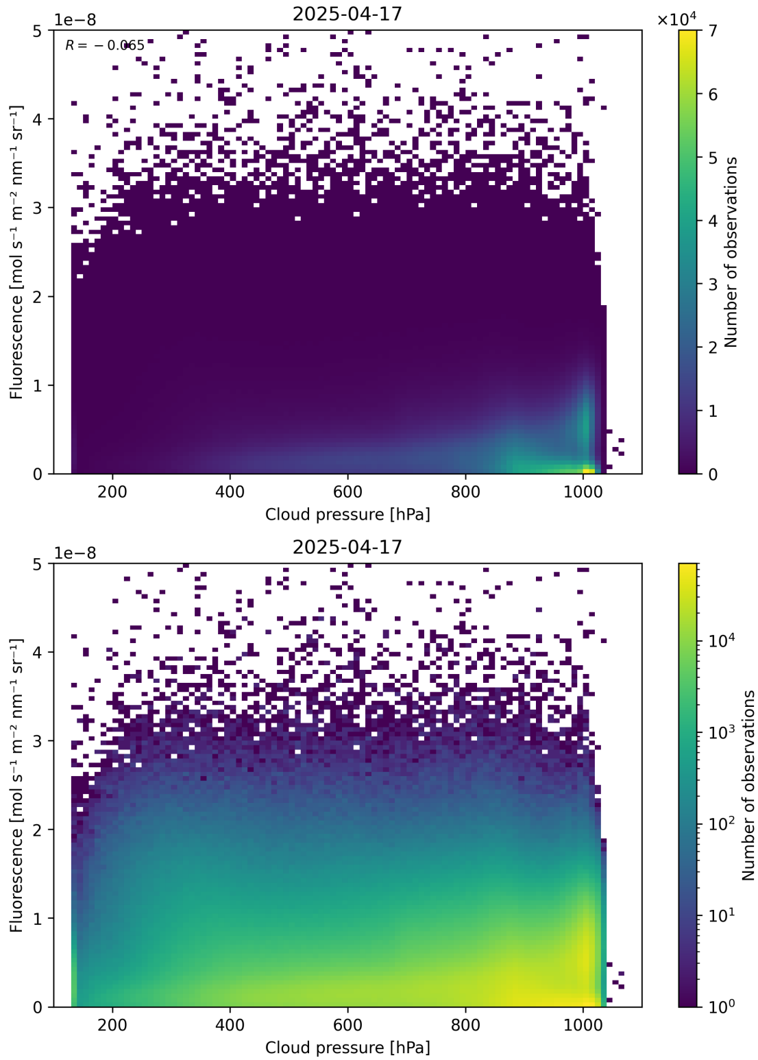
Figure 80: Scatter density plot of “Cloud pressure” against “Fluorescence” for 2025-04-16 to 2025-04-18.
