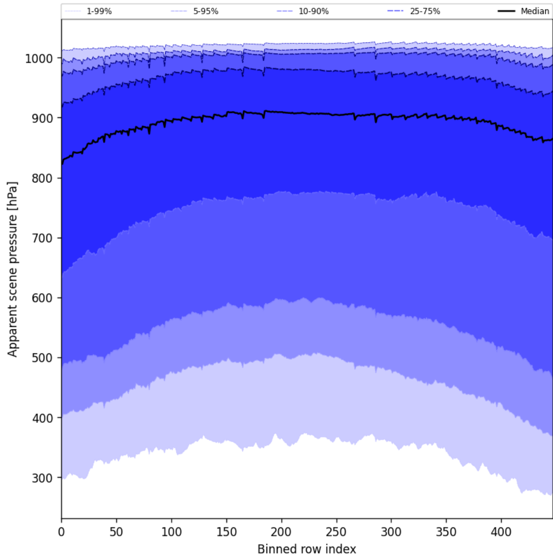
Figure 53: Along track statistics of “Apparent scene pressure” for 2025-04-16 to 2025-04-18
