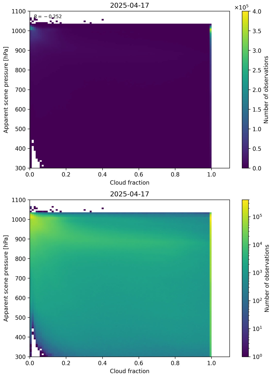
Figure 70: Scatter density plot of “Cloud fraction” against “Apparent scene pressure” for 2025-04-16 to 2025-04-18.
