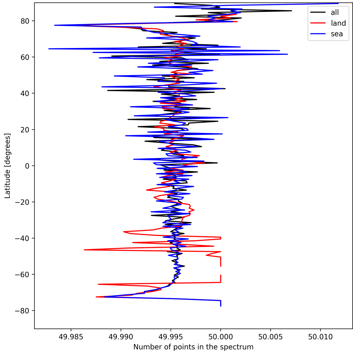
Figure 27: Zonal average of “Number of points in the spectrum” for 2025-04-16 to 2025-04-18.
