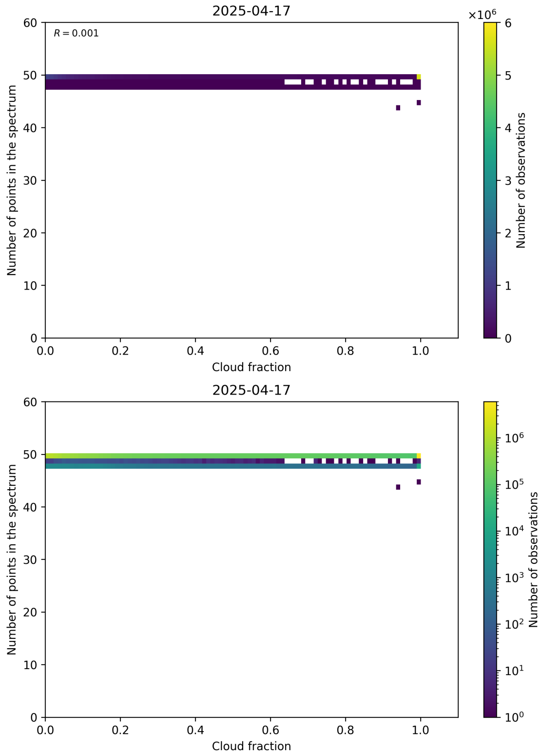
Figure 74: Scatter density plot of “Cloud fraction” against “Number of points in the spectrum” for 2025-04-16 to 2025-04-18.
