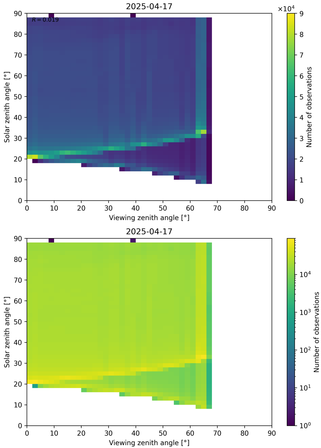
Figure 127: Scatter density plot of “Viewing zenith angle” against “Solar zenith angle” for 2025-04-16 to 2025-04-18.
