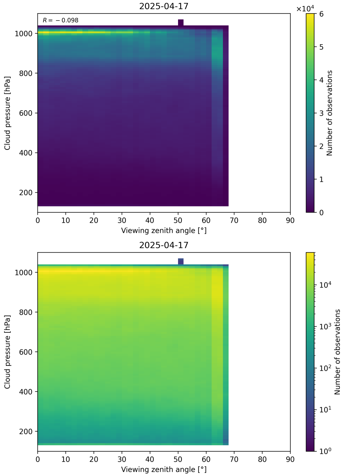
Figure 121: Scatter density plot of “Viewing zenith angle” against “Cloud pressure” for 2025-04-16 to 2025-04-18.
