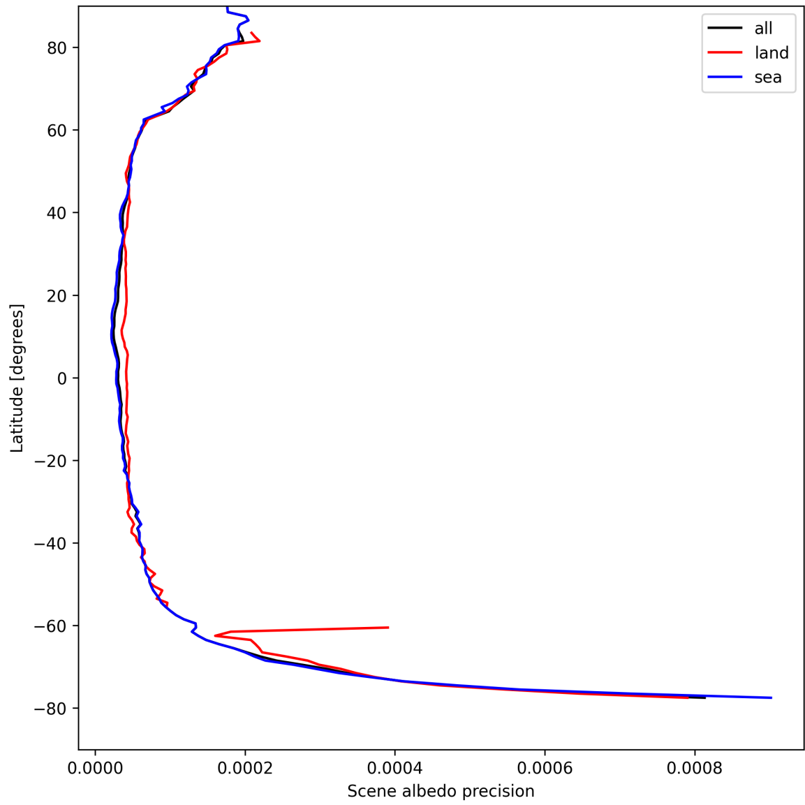
Figure 18: Zonal average of “Scene albedo precision” for 2025-04-16 to 2025-04-18.
