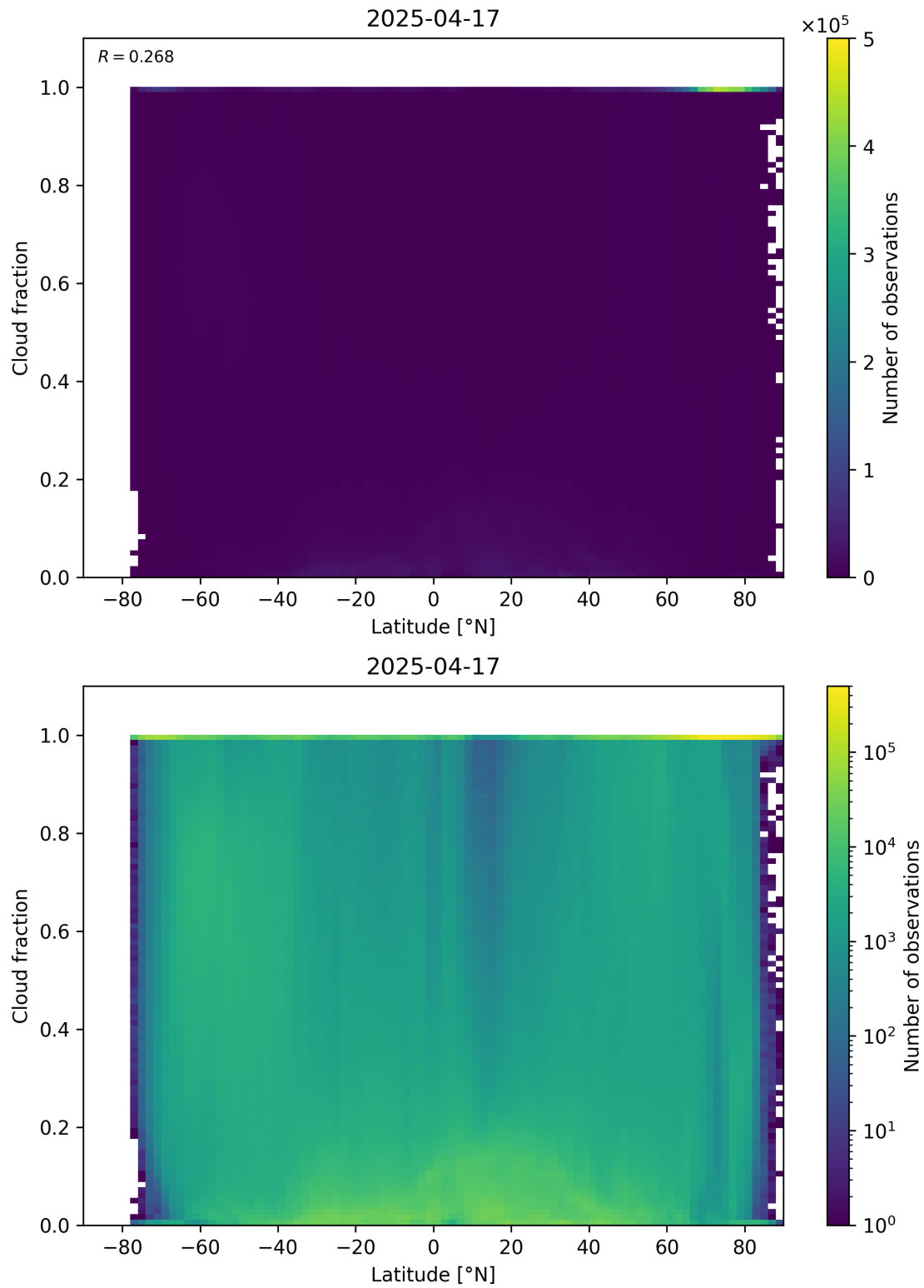
Figure 90: Scatter density plot of “Latitude” against “Cloud fraction” for 2025-04-16 to 2025-04-18.
