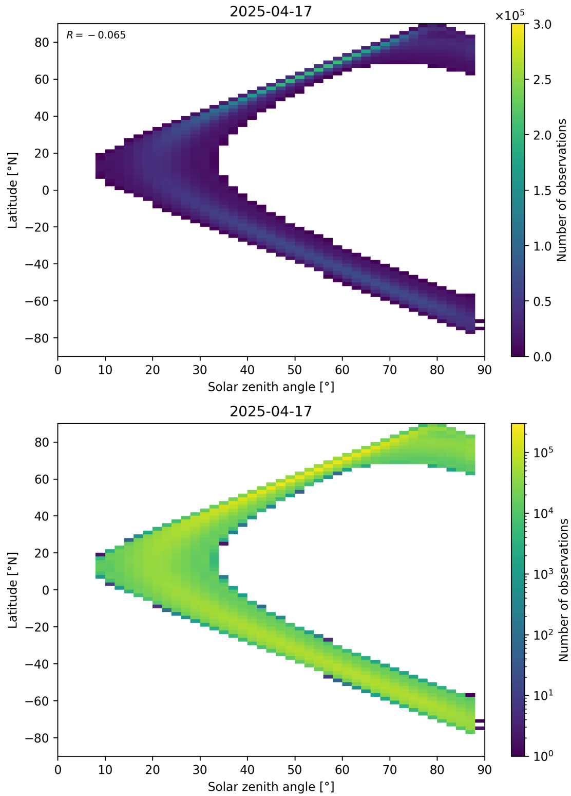
Figure 113: Scatter density plot of “Solar zenith angle” against “Latitude” for 2025-04-16 to 2025-04-18.
