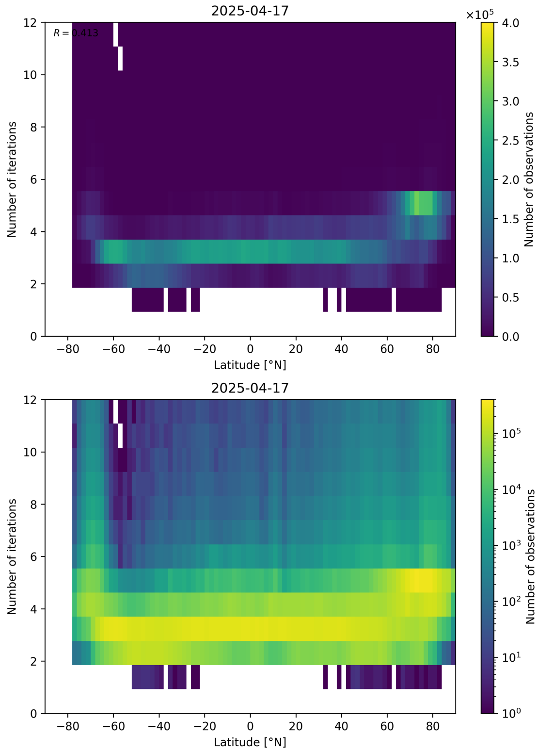
Figure 93: Scatter density plot of “Latitude” against “Number of iterations” for 2025-04-16 to 2025-04-18.
