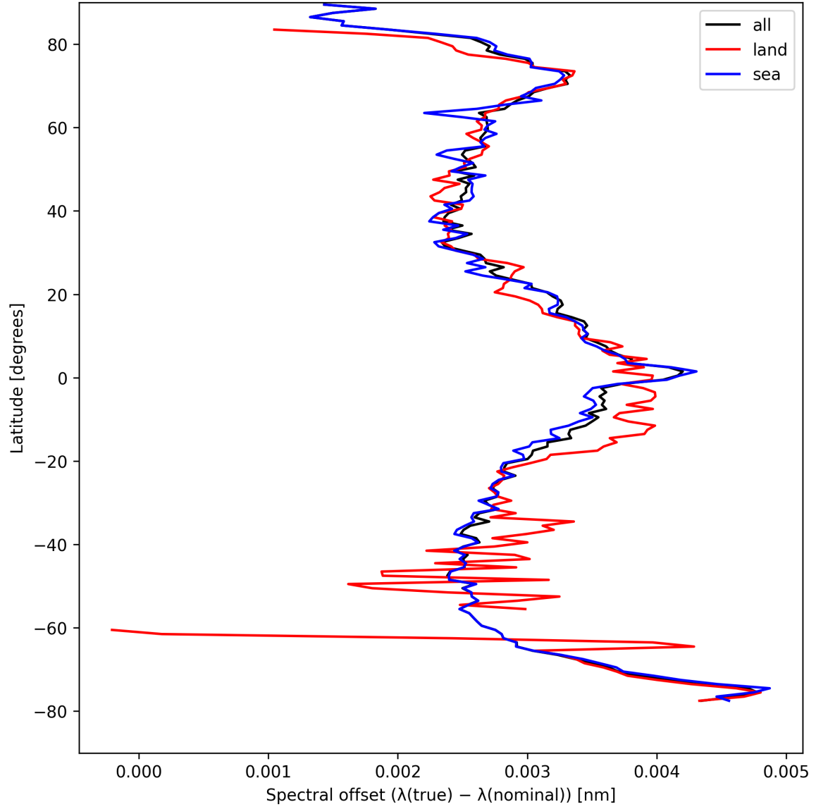
Figure 28: Zonal average of “Spectral offset ( \lambda_{\text{true}} - \lambda_{\text{nominal}} )” for 2025-04-16 to 2025-04-18.
