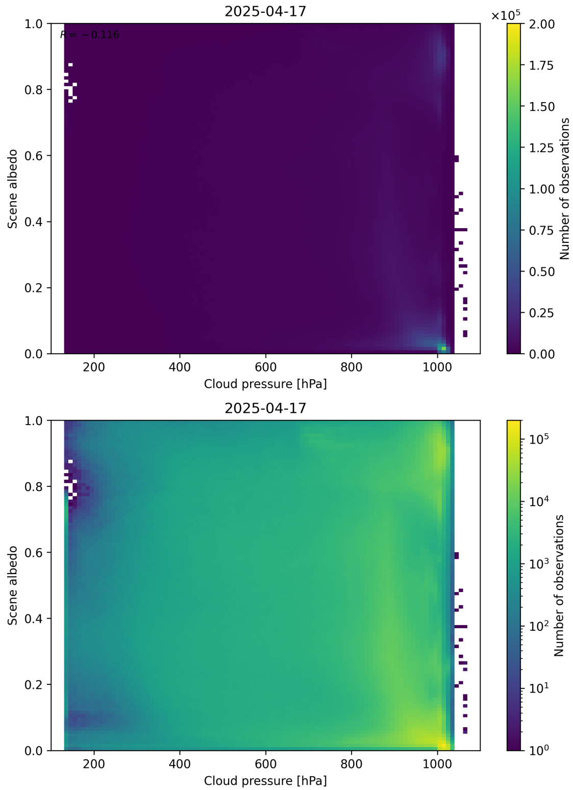
Figure 83: Scatter density plot of “Cloud pressure” against “Scene albedo” for 2025-04-16 to 2025-04-18.
