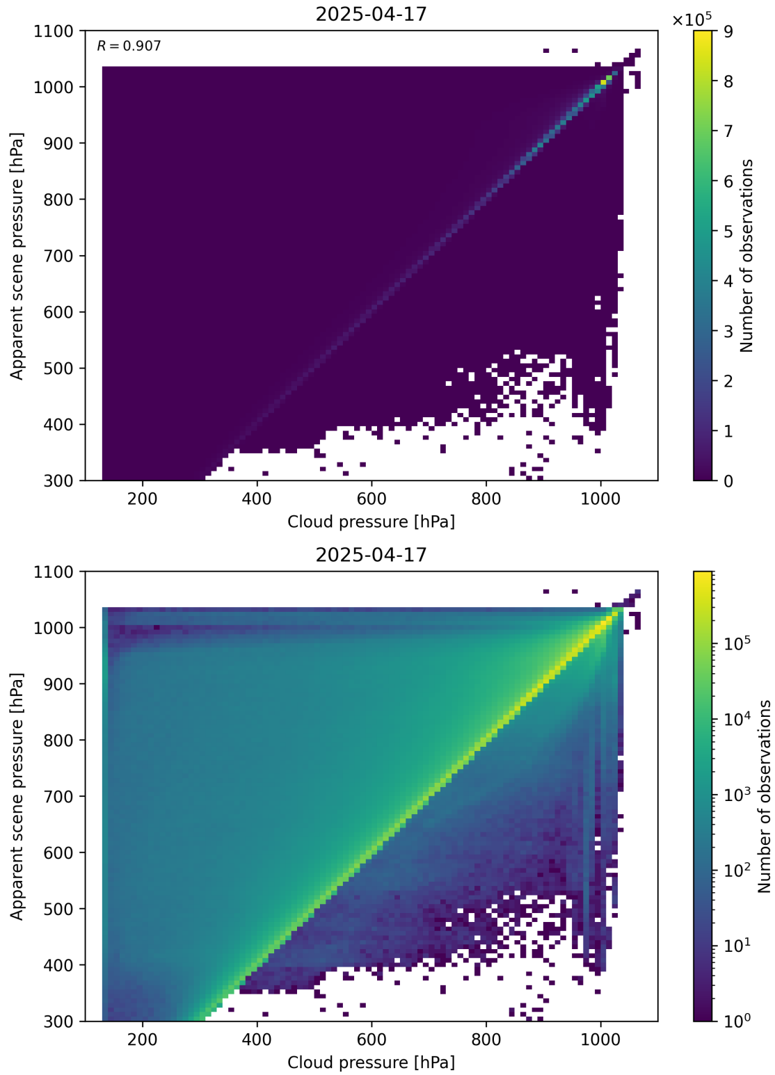
Figure 77: Scatter density plot of “Cloud pressure” against “Apparent scene pressure” for 2025-04-16 to 2025-04-18.
