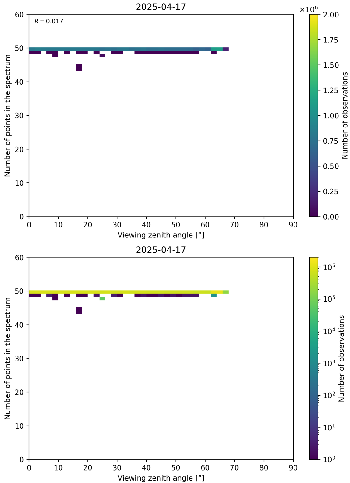
Figure 125: Scatter density plot of “Viewing zenith angle” against “Number of points in the spectrum” for 2025-04-16 to 2025-04-18.
