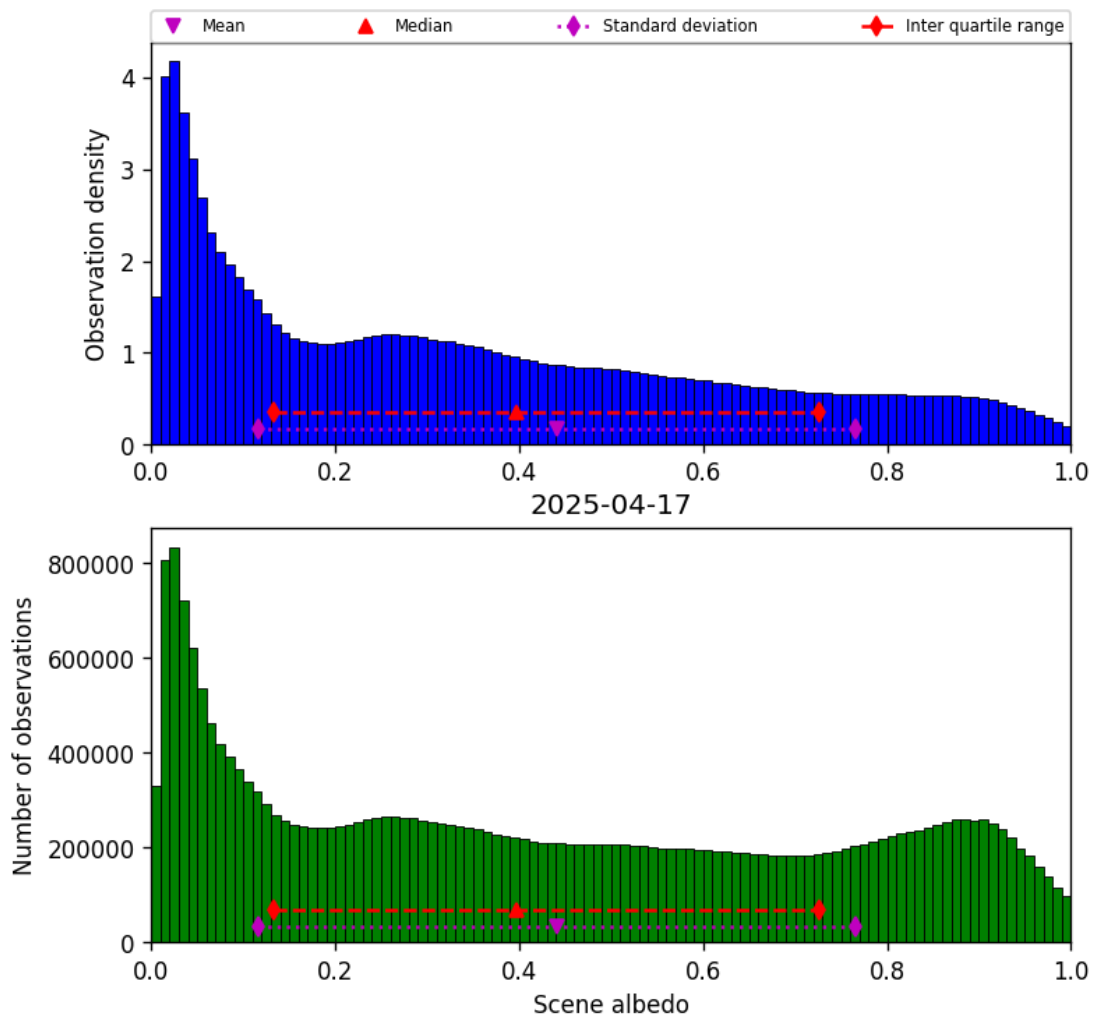
Figure 34: Histogram of “Scene albedo” for 2025-04-16 to 2025-04-18
