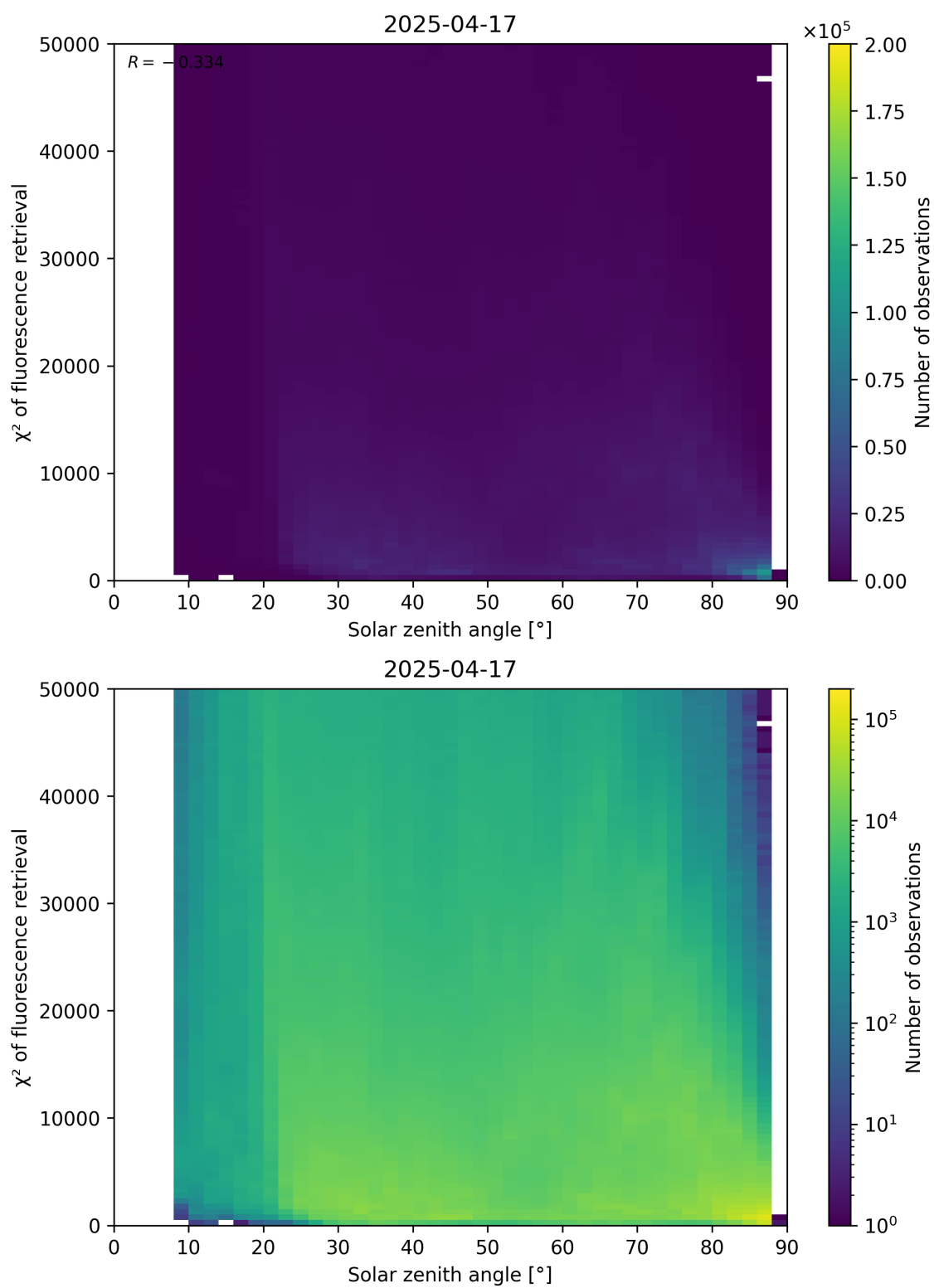
Figure 109: Scatter density plot of “Solar zenith angle” against “ \chi^2 of fluorescence retrieval” for 2025-04-16 to 2025-04-18.
