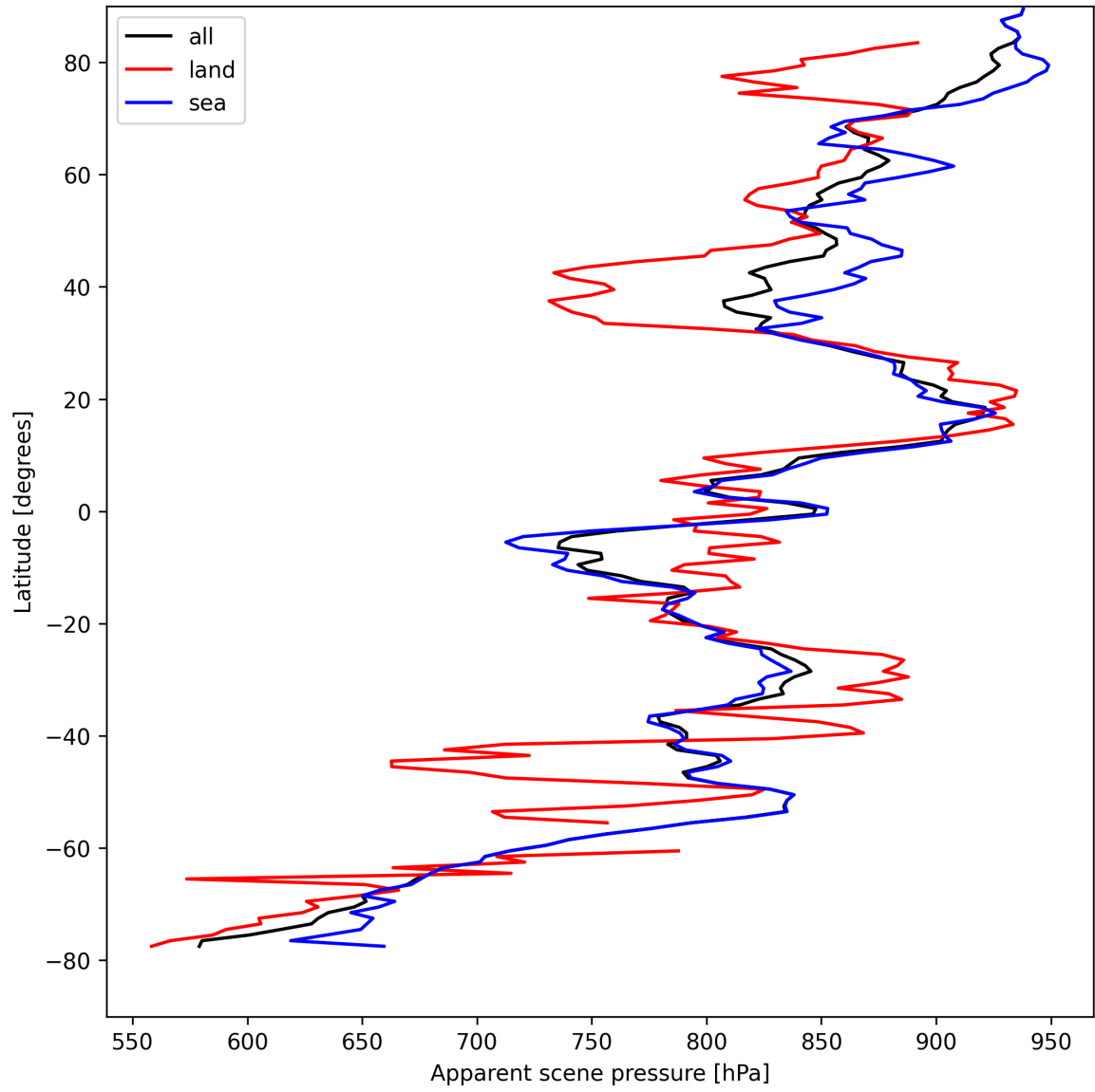
Figure 19: Zonal average of “Apparent scene pressure” for 2025-04-16 to 2025-04-18.
