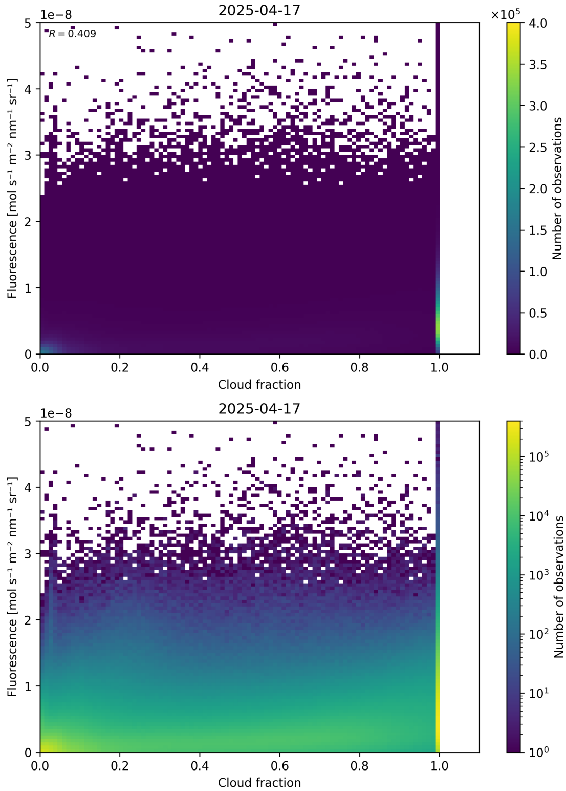
Figure 72: Scatter density plot of “Cloud fraction” against “Fluorescence” for 2025-04-16 to 2025-04-18.
