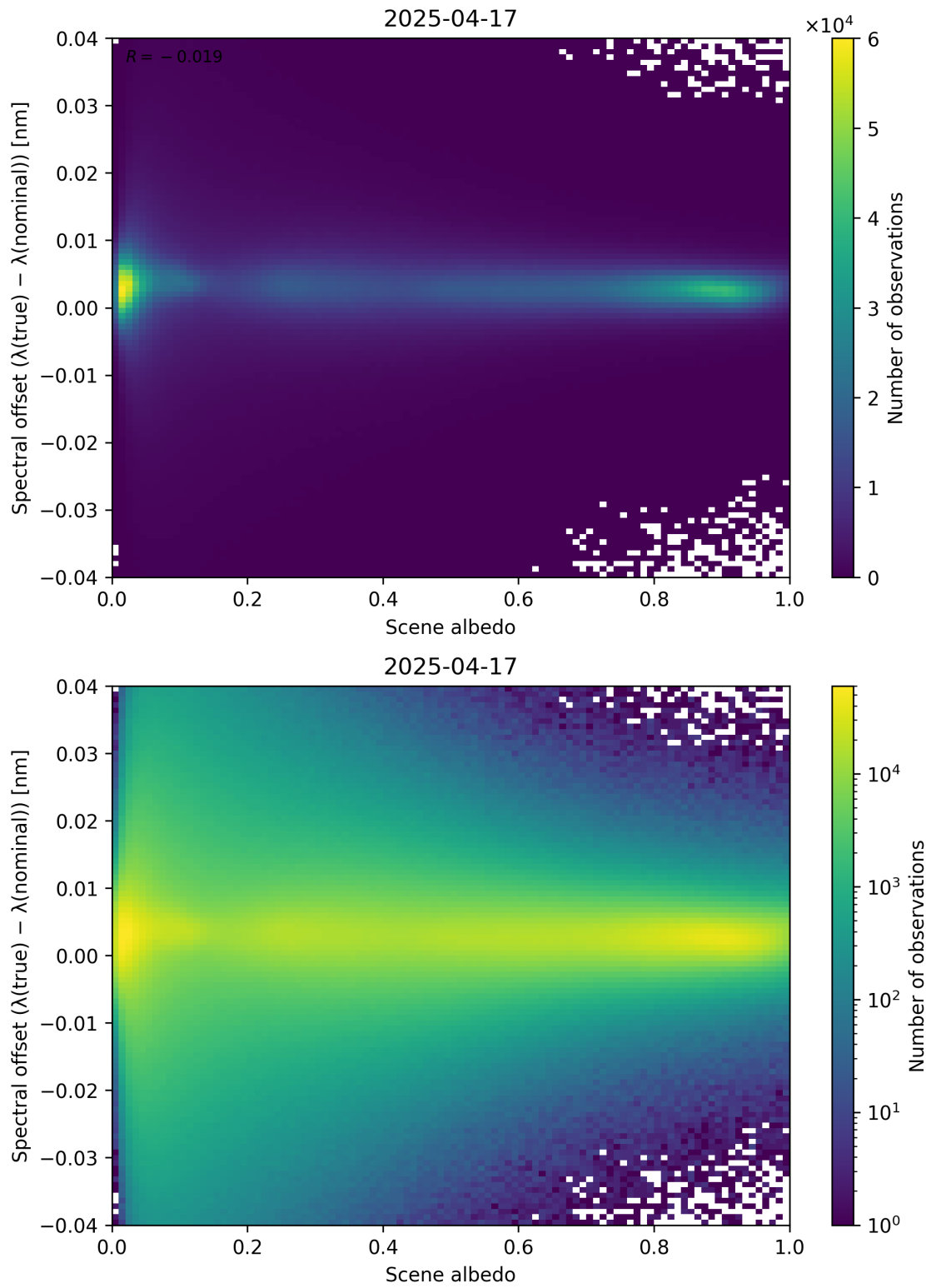
Figure 107: Scatter density plot of “Scene albedo” against “Spectral offset ( \lambda_{\text{true}} - \lambda_{\text{nominal}} )” for 2025-04-16 to 2025-04-18.
