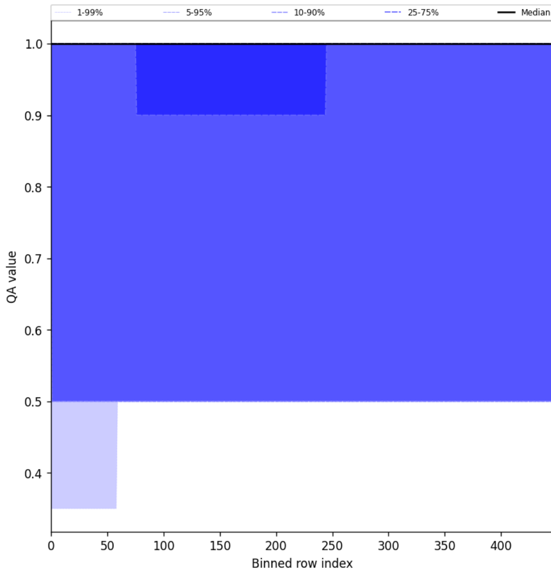
Figure 46: Along track statistics of “QA value” for 2025-04-16 to 2025-04-18
