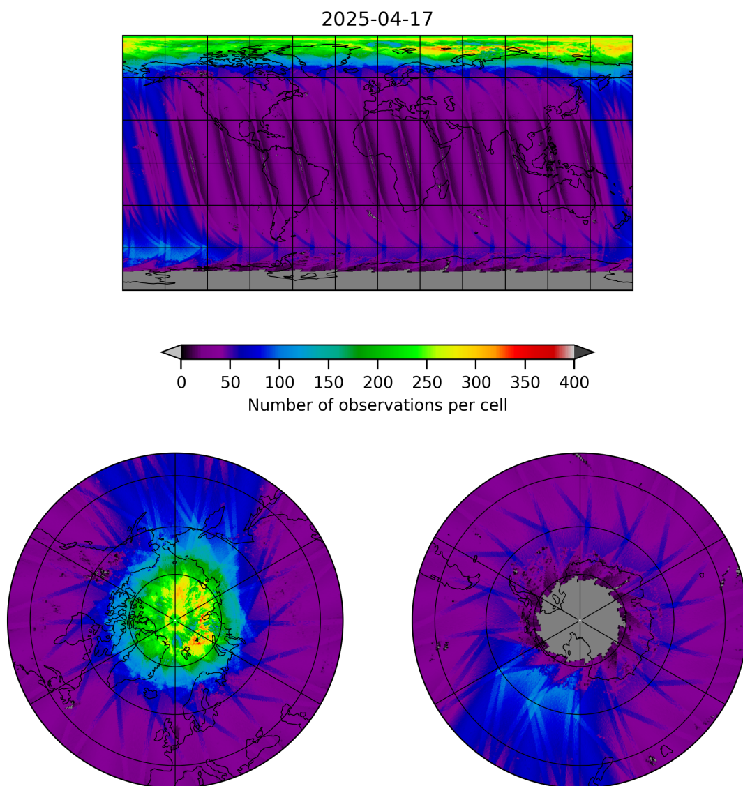
Figure 11: Map of the number of observations for 2025-04-16 to 2025-04-18
