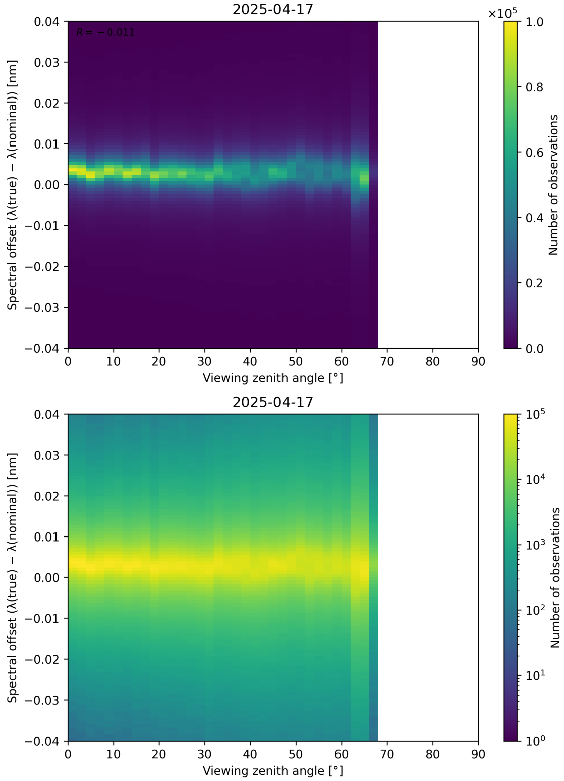
Figure 128: Scatter density plot of “Viewing zenith angle” against “Spectral offset ( \lambda_{\text{true}} - \lambda_{\text{nominal}} )” for 2025-04-16 to 2025-04-18.
