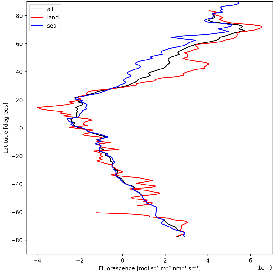
Figure 23: Zonal average of “Fluorescence” for 2025-04-16 to 2025-04-18.
