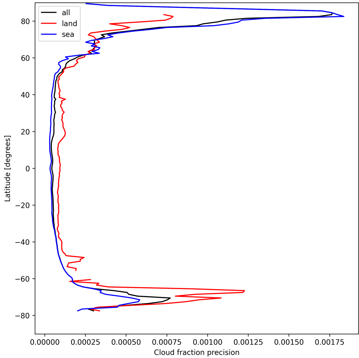
Figure 16: Zonal average of “Cloud fraction precision” for 2025-04-16 to 2025-04-18.
