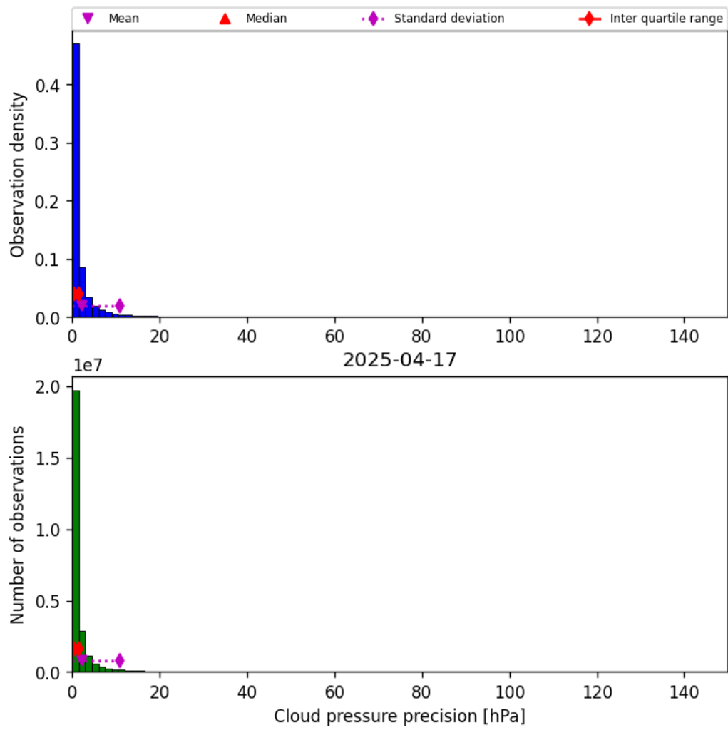
Figure 31: Histogram of “Cloud pressure precision” for 2025-04-16 to 2025-04-18
