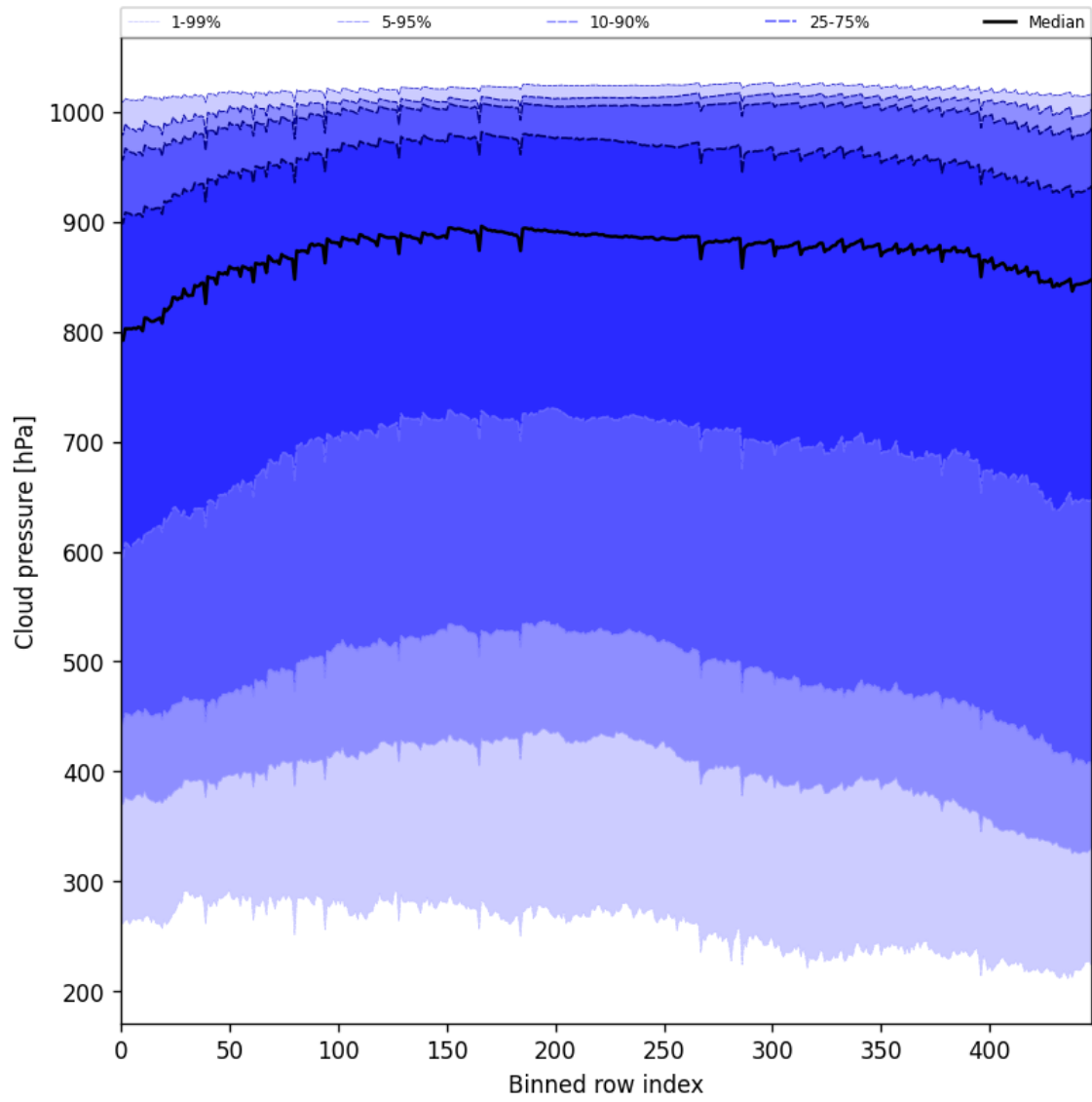
Figure 47: Along track statistics of “Cloud pressure” for 2025-04-16 to 2025-04-18
