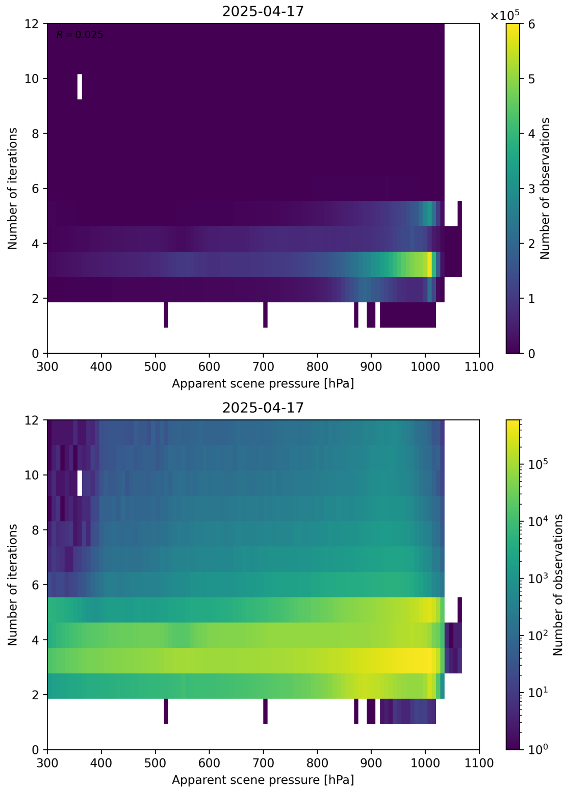
Figure 65: Scatter density plot of “Apparent scene pressure” against “Number of iterations” for 2025-04-16 to 2025-04-18.
