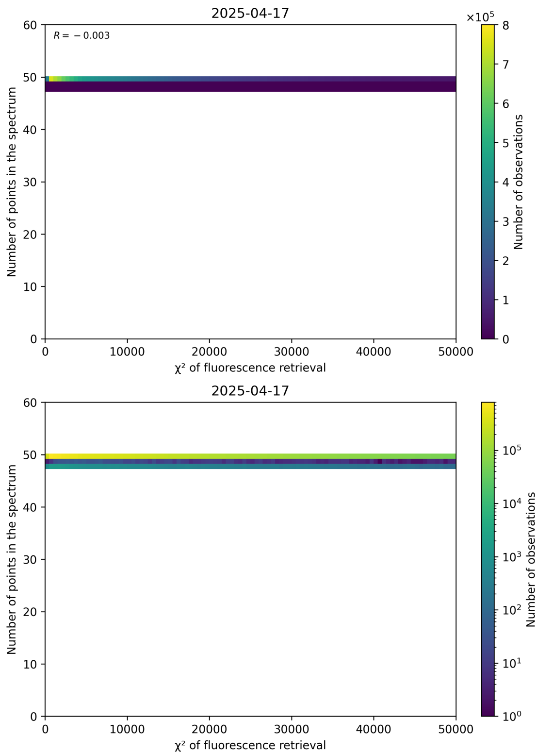
Figure 68: Scatter density plot of “ \chi^2 of fluorescence retrieval” against “Number of points in the spectrum” for 2025-04-16 to 2025-04-18.
