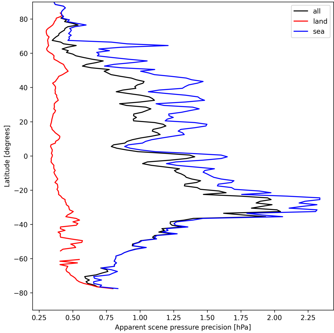
Figure 20: Zonal average of “Apparent scene pressure precision” for 2025-04-16 to 2025-04-18.
