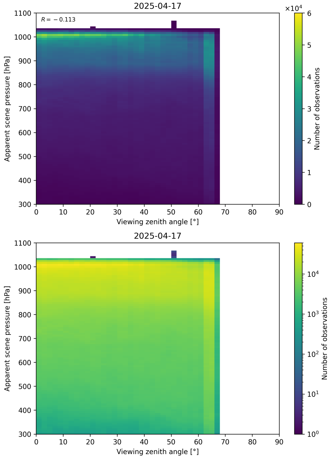
Figure 118: Scatter density plot of “Viewing zenith angle” against “Apparent scene pressure” for 2025-04-16 to 2025-04-18.
