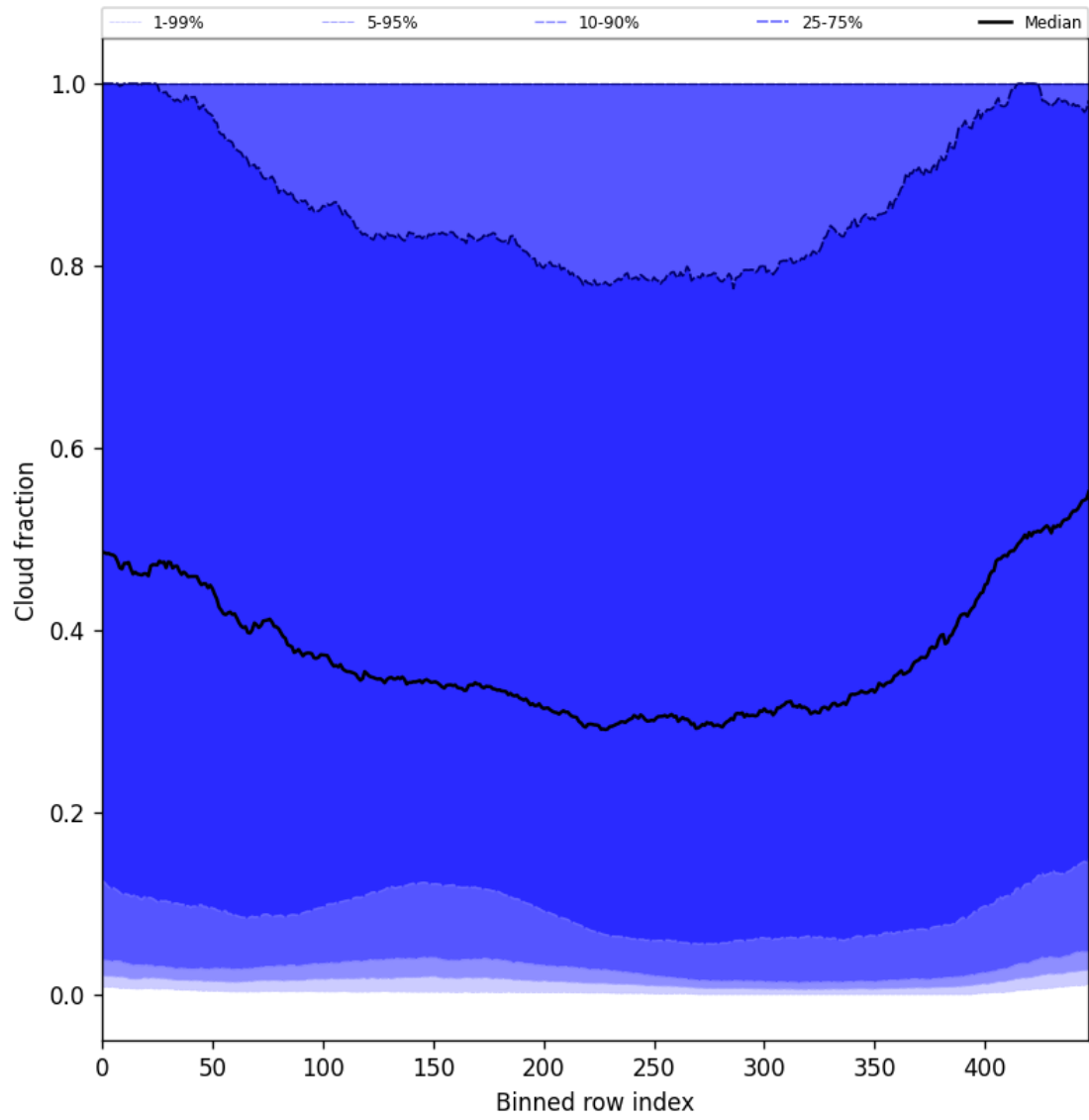
Figure 49: Along track statistics of “Cloud fraction” for 2025-04-16 to 2025-04-18
