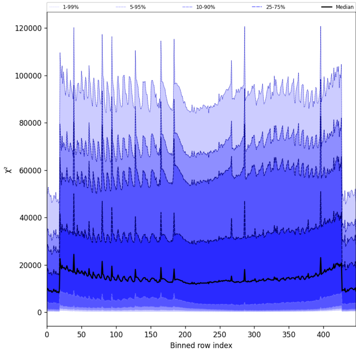
Figure 55: Along track statistics of “ \chi^2 ” for 2025-04-16 to 2025-04-18
