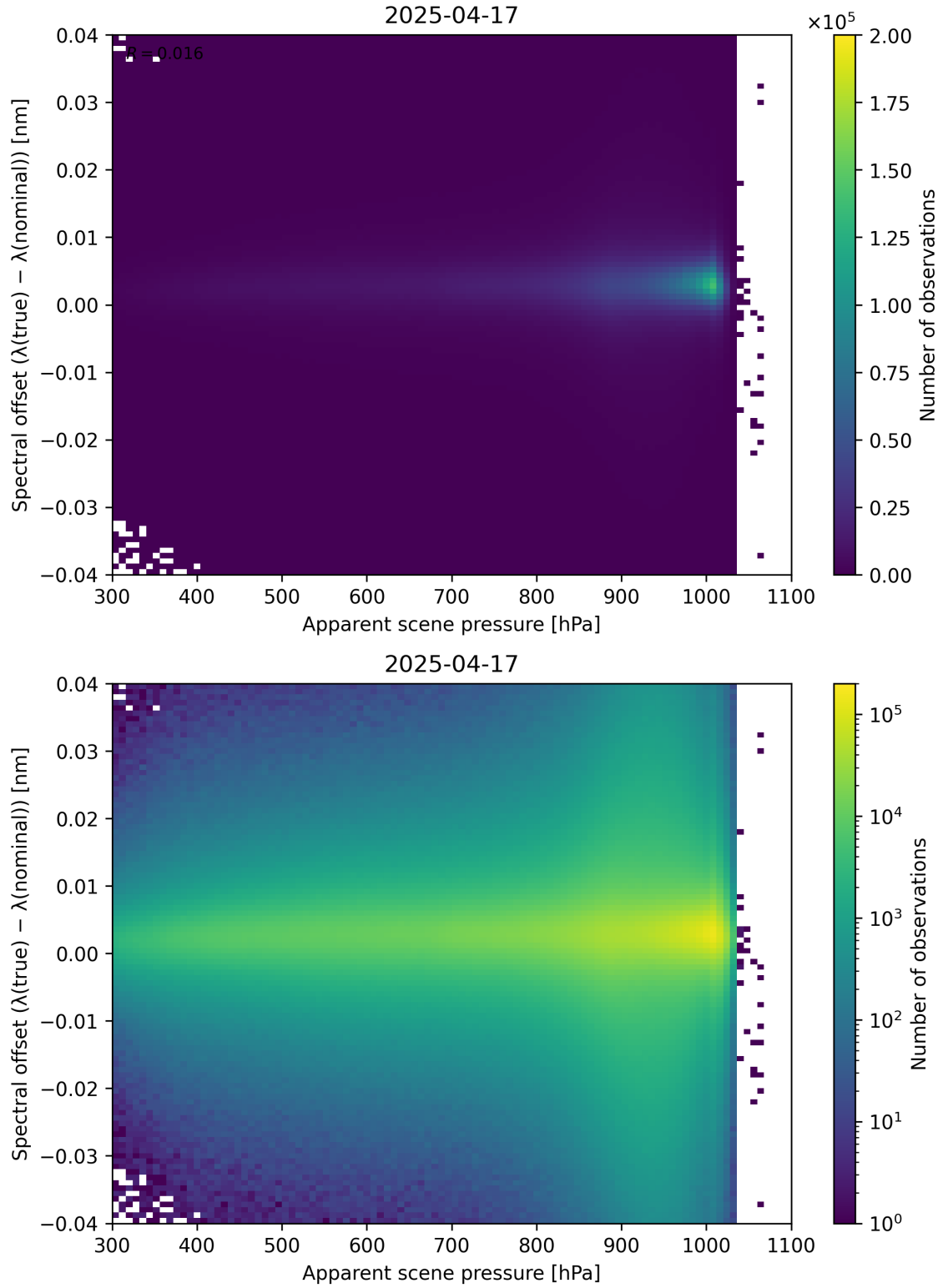
Figure 67: Scatter density plot of “Apparent scene pressure” against “Spectral offset ( \lambda_{\text{true}} - \lambda_{\text{nominal}} )” for 2025-04-16 to 2025-04-18.
