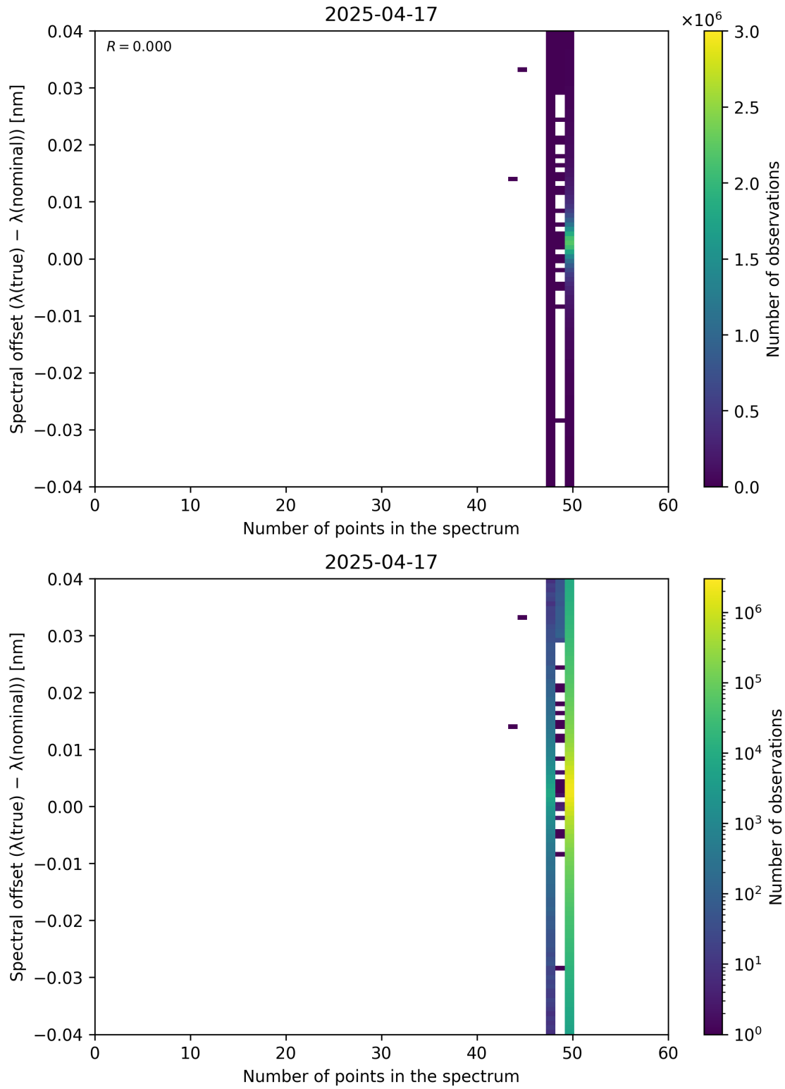
Figure 101: Scatter density plot of “Number of points in the spectrum” against “Spectral offset ( \lambda_{\text{true}} - \lambda_{\text{nominal}} )” for 2025-04-16 to 2025-04-18.
