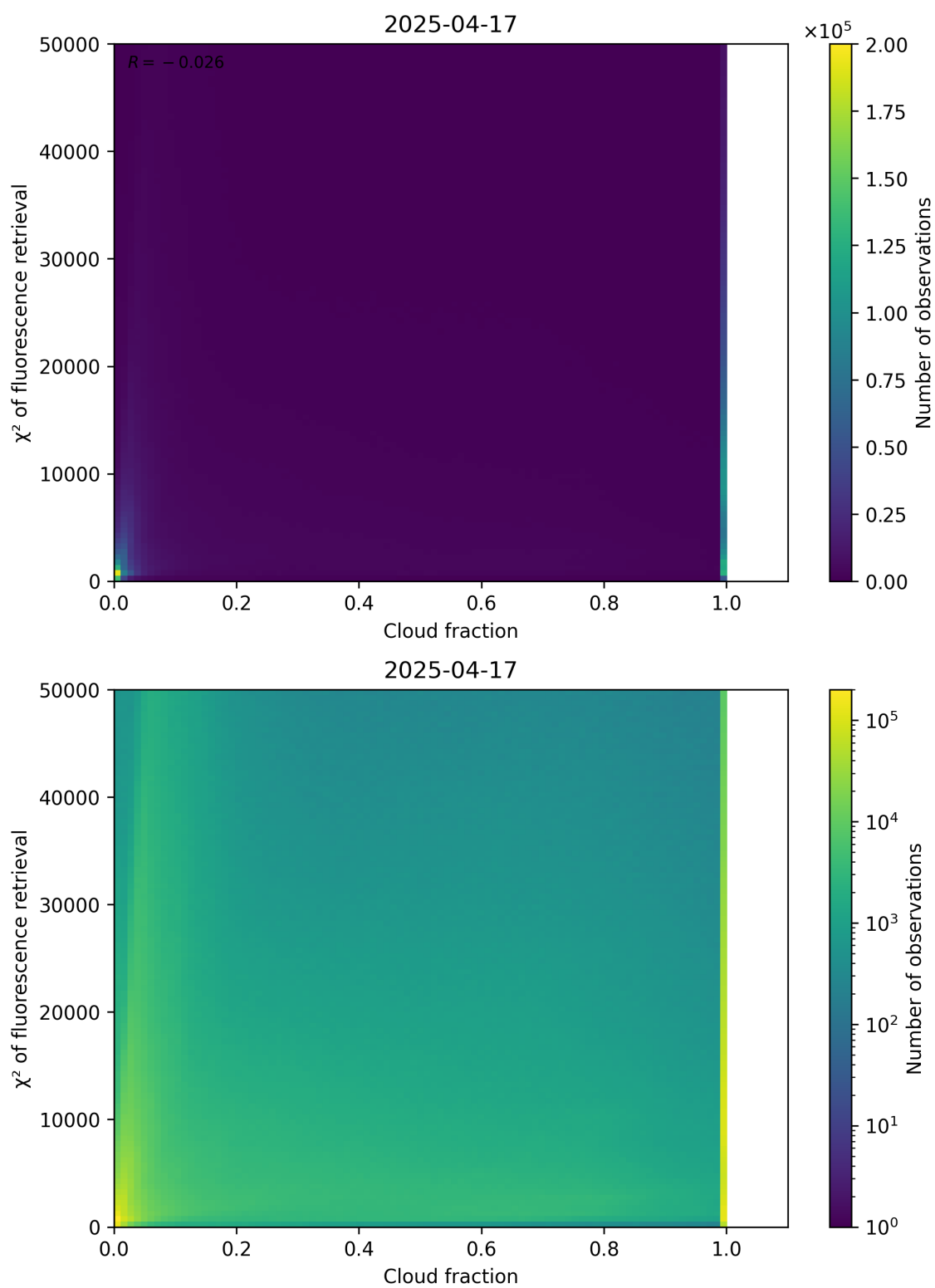
Figure 71: Scatter density plot of “Cloud fraction” against “ \chi^2 of fluorescence retrieval” for 2025-04-16 to 2025-04-18.
