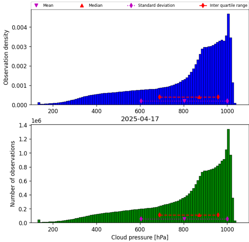
Figure 30: Histogram of “Cloud pressure” for 2025-04-16 to 2025-04-18
