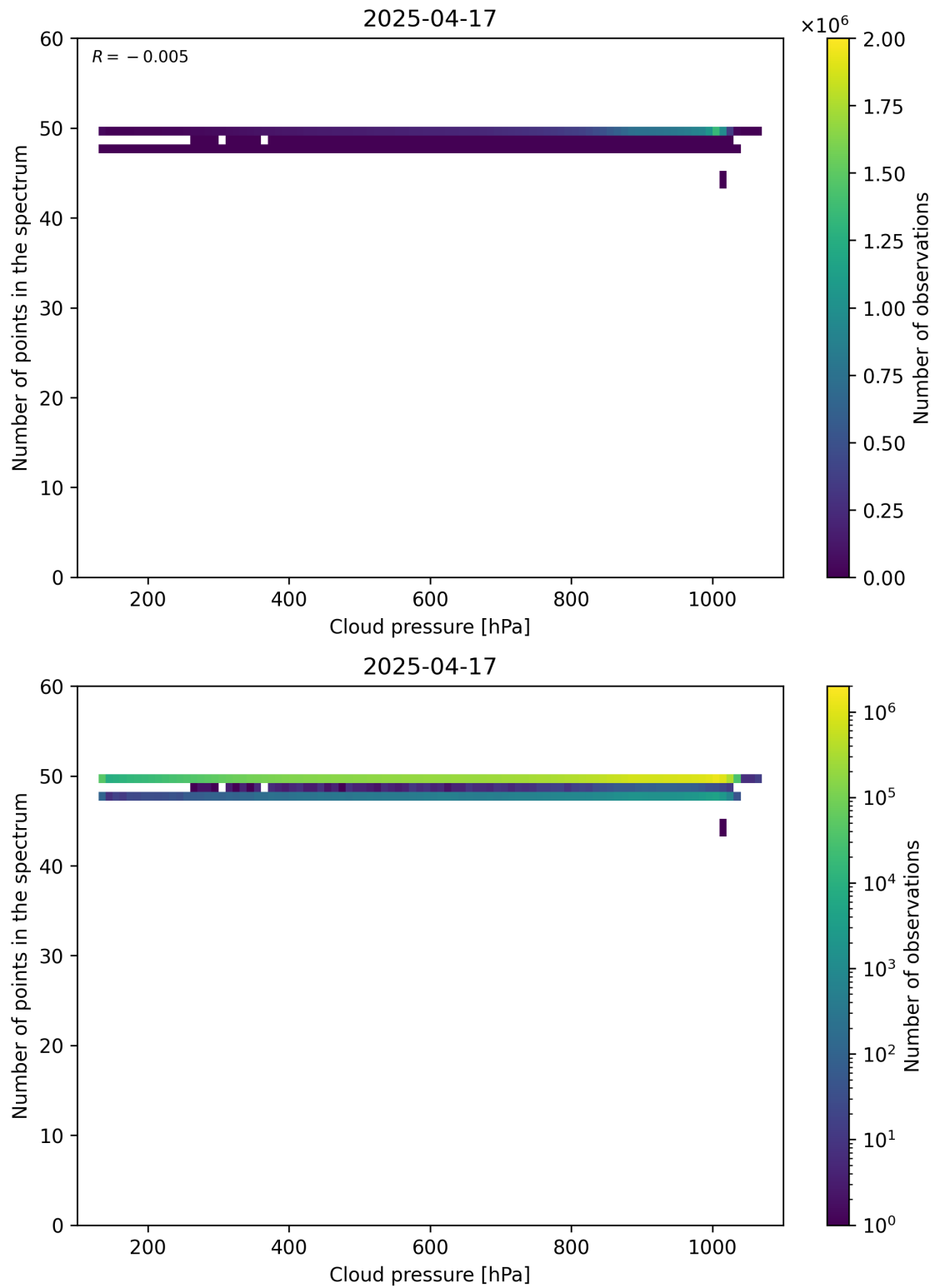
Figure 82: Scatter density plot of “Cloud pressure” against “Number of points in the spectrum” for 2025-04-16 to 2025-04-18.
