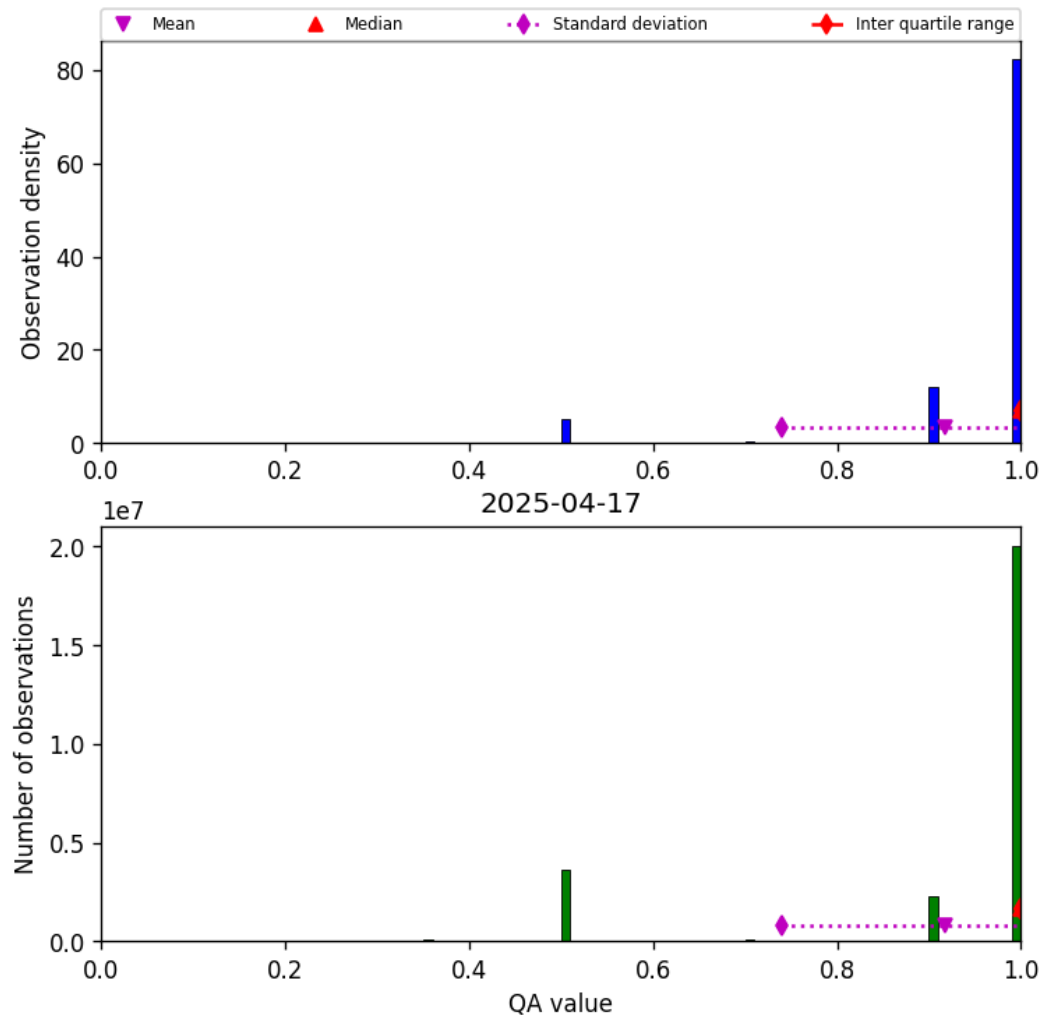
Figure 29: Histogram of “QA value” for 2025-04-16 to 2025-04-18
