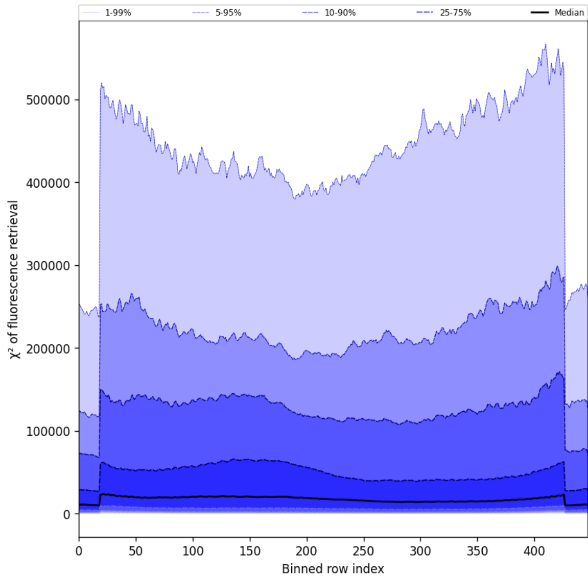
Figure 59: Along track statistics of “ \chi^2 of fluorescence retrieval” for 2025-04-16 to 2025-04-18
