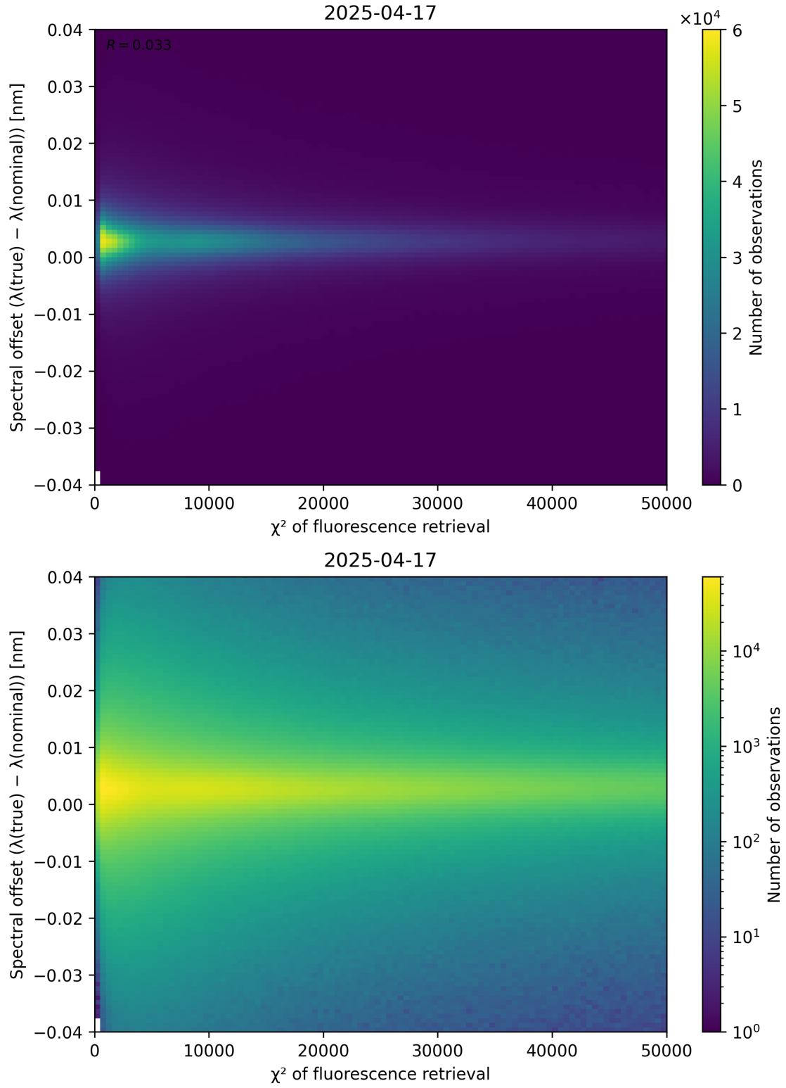
Figure 69: Scatter density plot of “ \chi^2 of fluorescence retrieval” against “Spectral offset ( \lambda_{\text{true}} - \lambda_{\text{nominal}} )” for 2025-04-16 to 2025-04-18.
