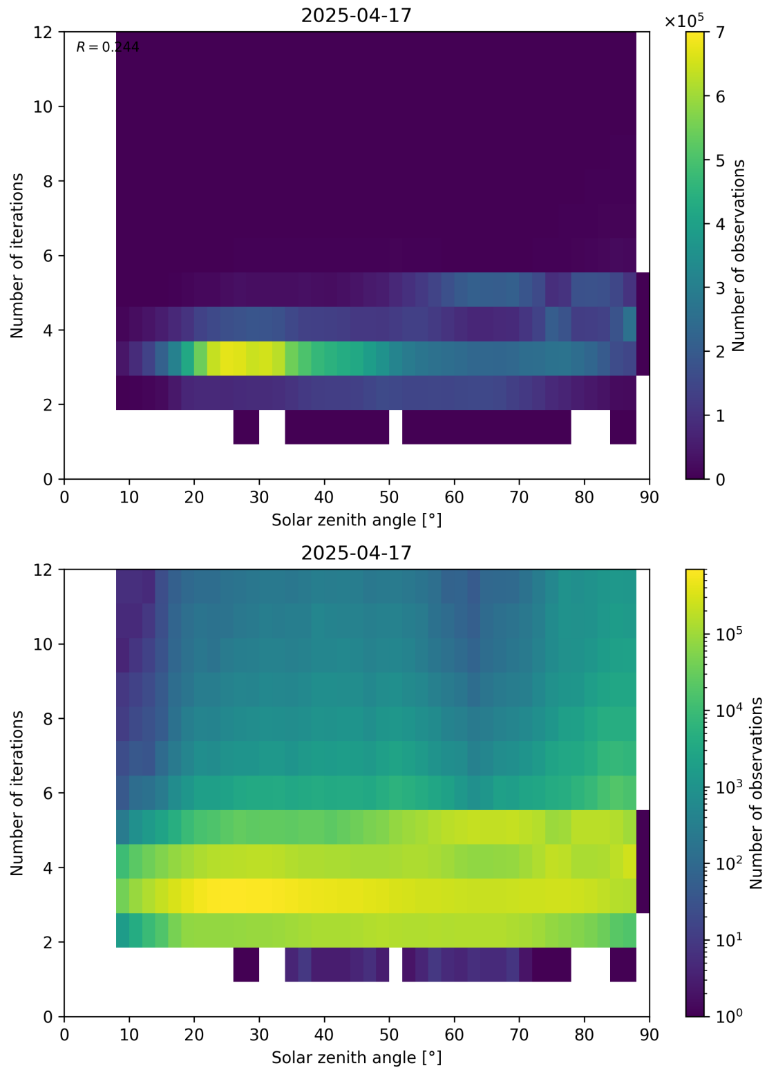
Figure 114: Scatter density plot of “Solar zenith angle” against “Number of iterations” for 2025-04-16 to 2025-04-18.
