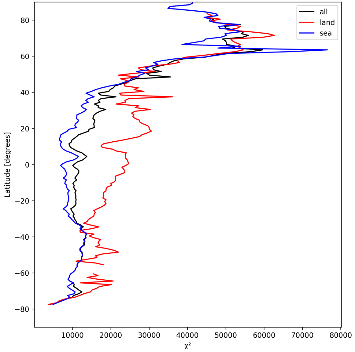
Figure 21: Zonal average of “ \chi^2 ” for 2025-04-16 to 2025-04-18.
