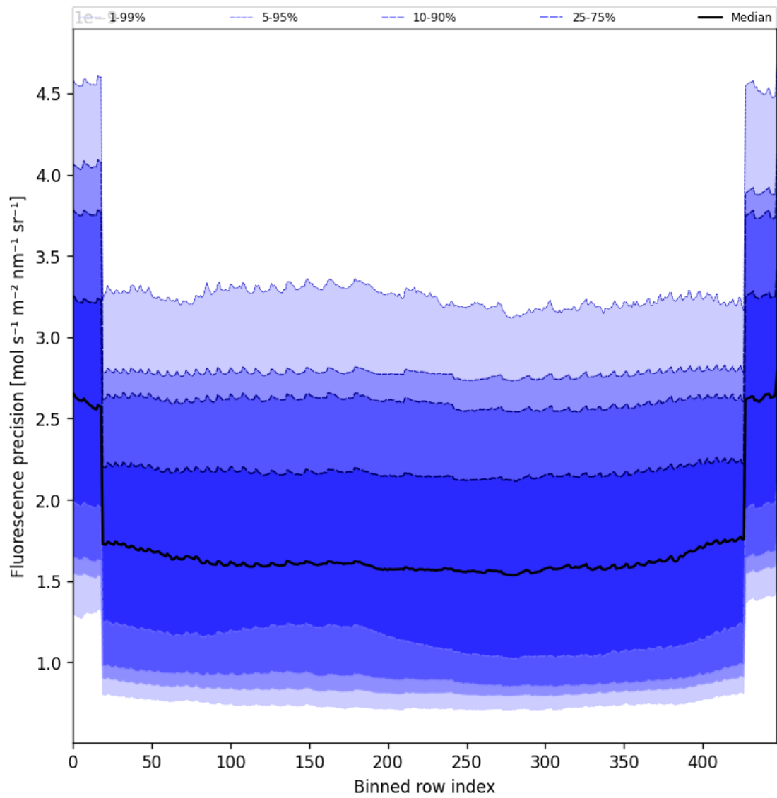
Figure 58: Along track statistics of “Fluorescence precision” for 2025-04-16 to 2025-04-18
