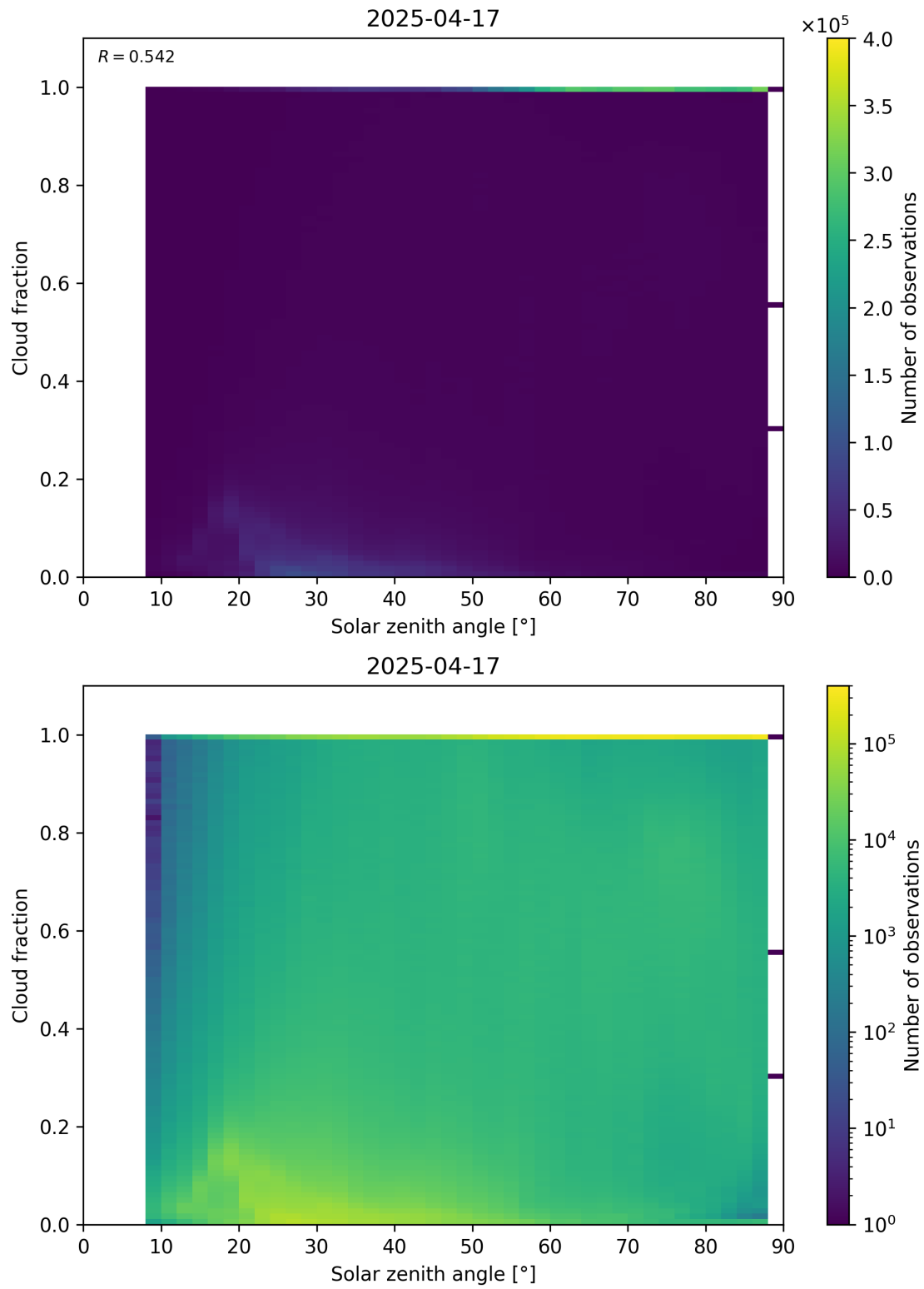
Figure 110: Scatter density plot of “Solar zenith angle” against “Cloud fraction” for 2025-04-16 to 2025-04-18.
