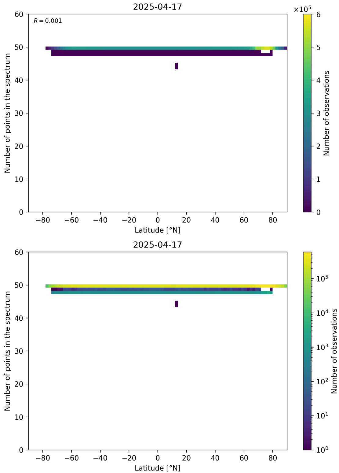
Figure 94: Scatter density plot of “Latitude” against “Number of points in the spectrum” for 2025-04-16 to 2025-04-18.
