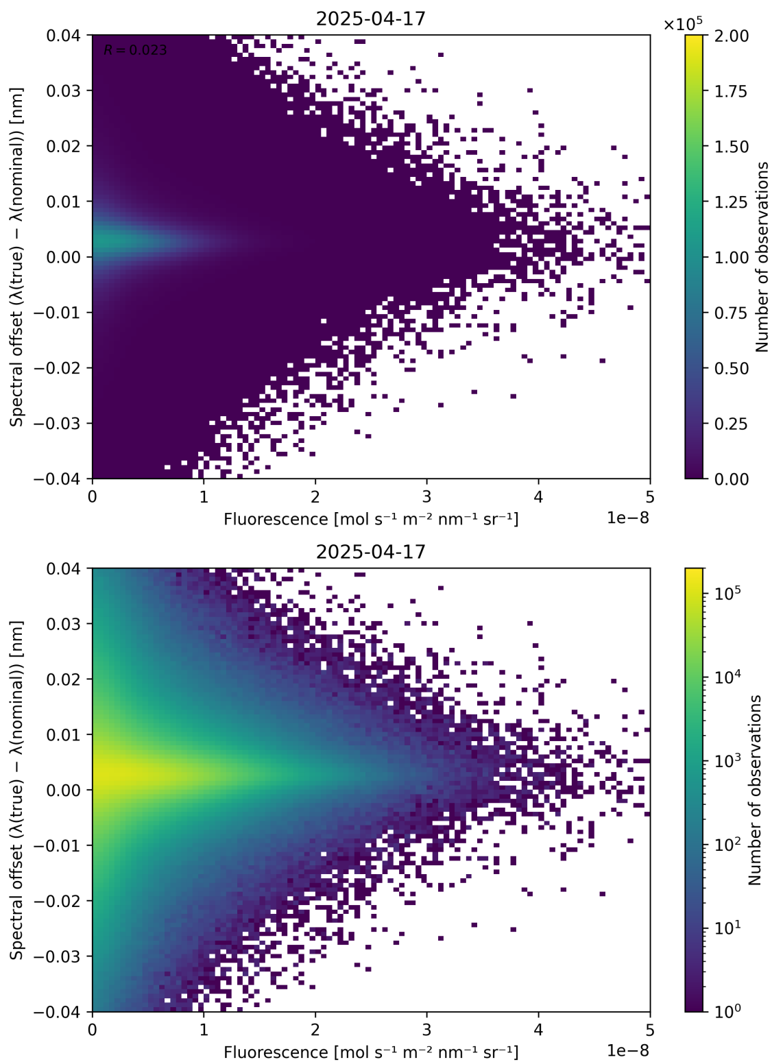
Figure 87: Scatter density plot of “Fluorescence” against “Spectral offset ( \lambda_{\text{true}} - \lambda_{\text{nominal}} )” for 2025-04-16 to 2025-04-18.
