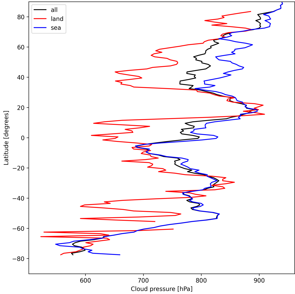
Figure 13: Zonal average of “Cloud pressure” for 2025-04-16 to 2025-04-18.
