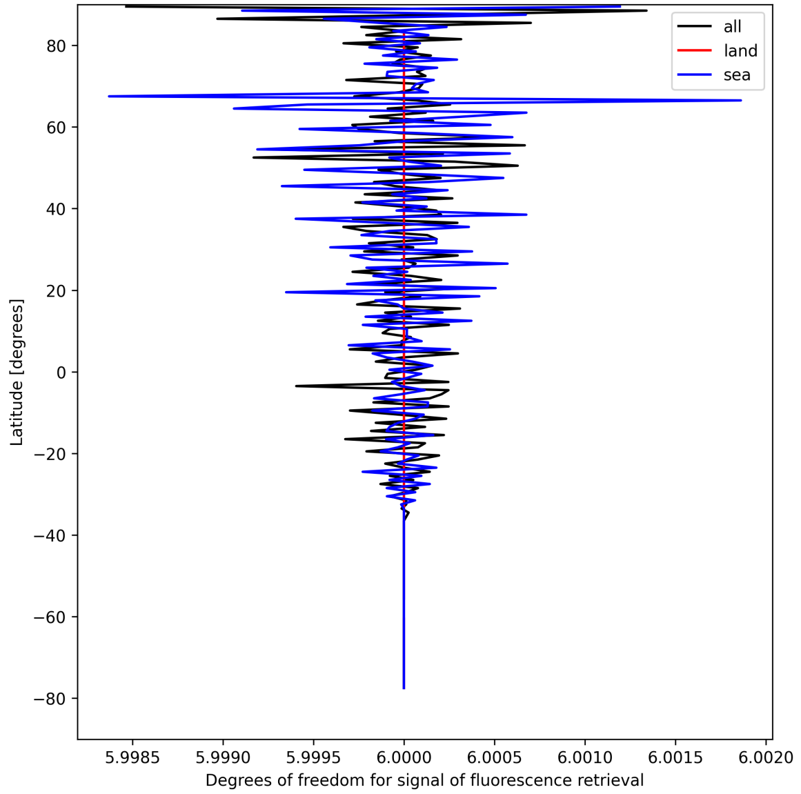
Figure 26: Zonal average of “Degrees of freedom for signal of fluorescence retrieval” for 2025-04-16 to 2025-04-18.
