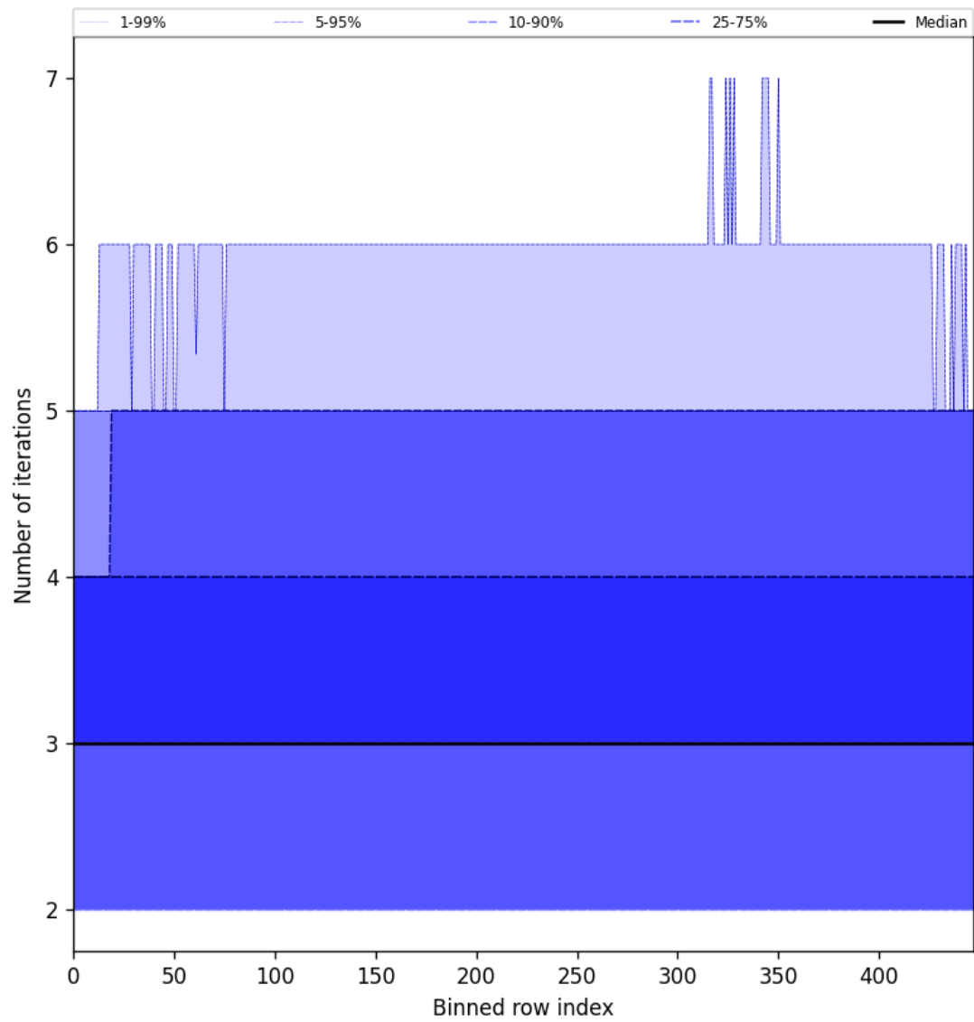
Figure 56: Along track statistics of “Number of iterations” for 2025-04-16 to 2025-04-18
