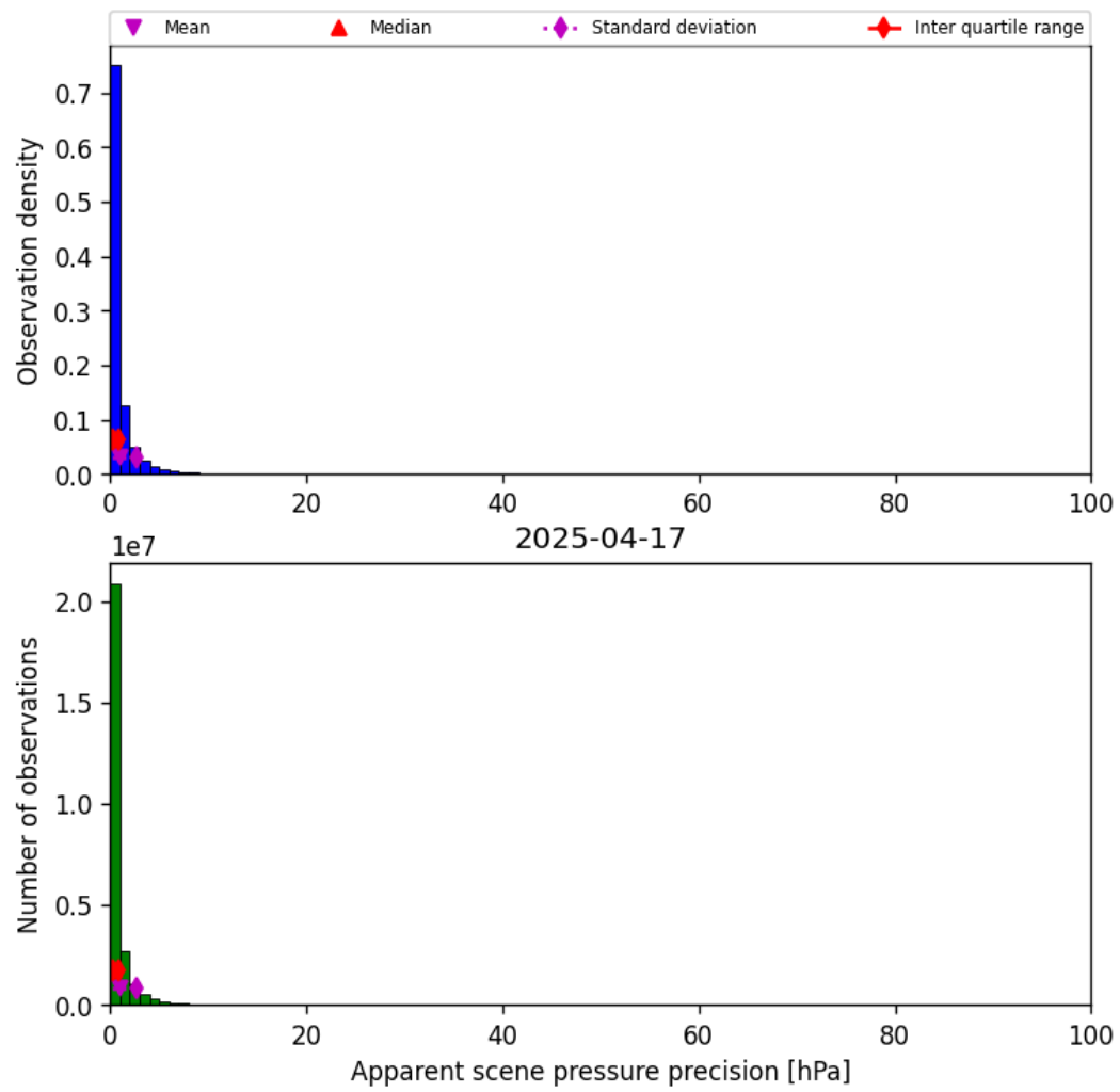
Figure 37: Histogram of “Apparent scene pressure precision” for 2025-04-16 to 2025-04-18
