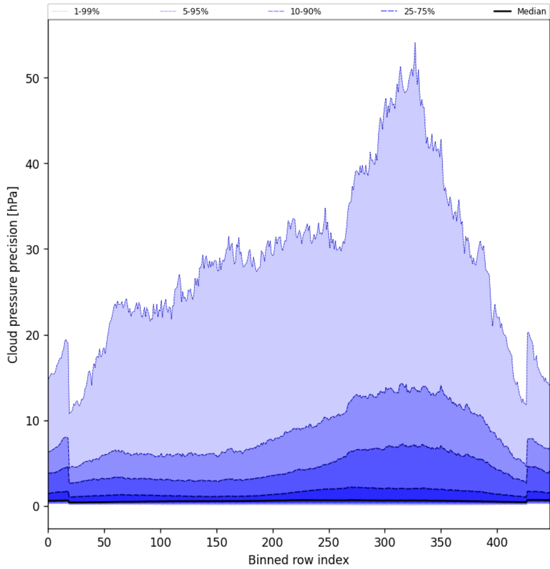
Figure 48: Along track statistics of “Cloud pressure precision” for 2025-04-16 to 2025-04-18
