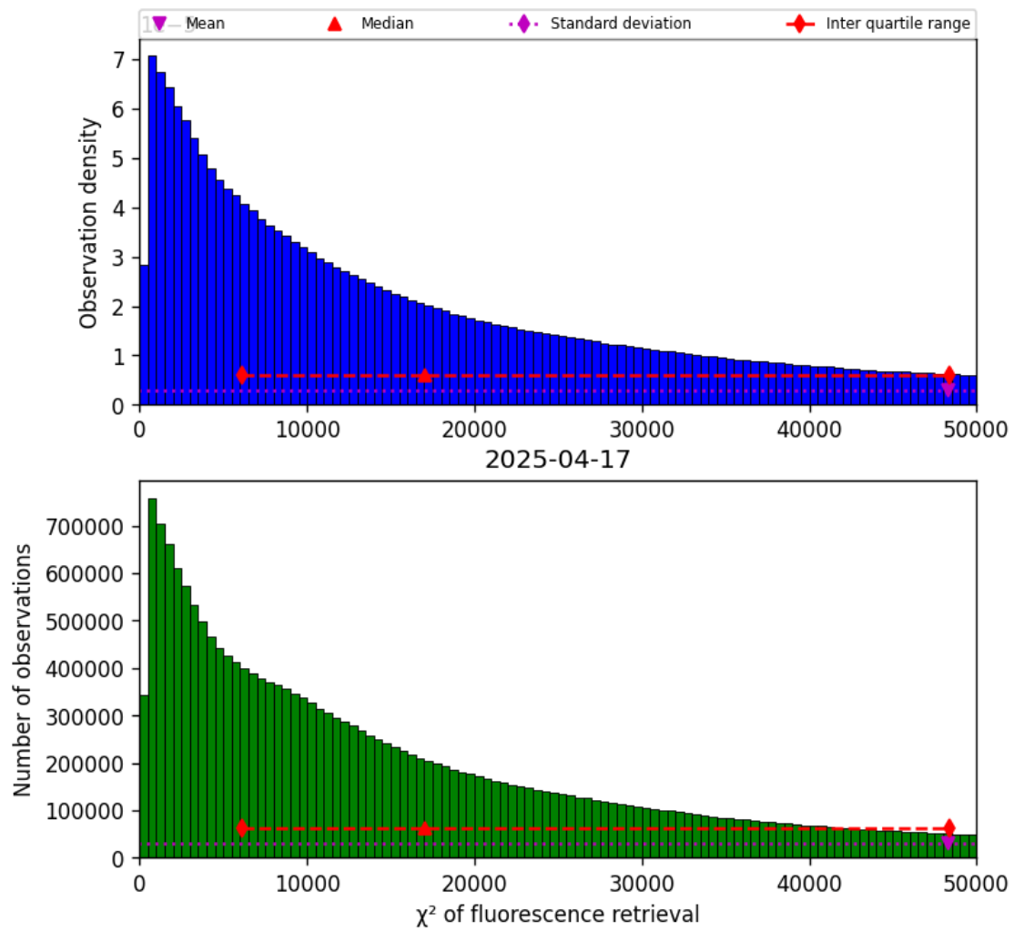
Figure 42: Histogram of “ \chi^2 of fluorescence retrieval” for 2025-04-16 to 2025-04-18
