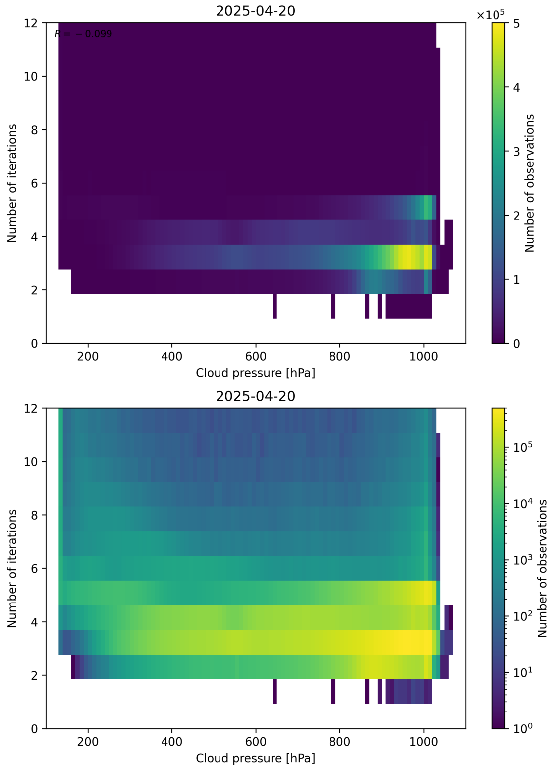
Figure 81: Scatter density plot of “Cloud pressure” against “Number of iterations” for 2025-04-19 to 2025-04-21.
