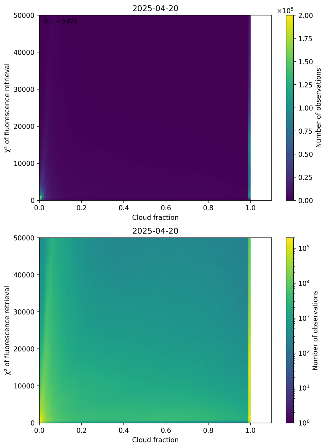
Figure 71: Scatter density plot of “Cloud fraction” against “ \chi^2 of fluorescence retrieval” for 2025-04-19 to 2025-04-21.
