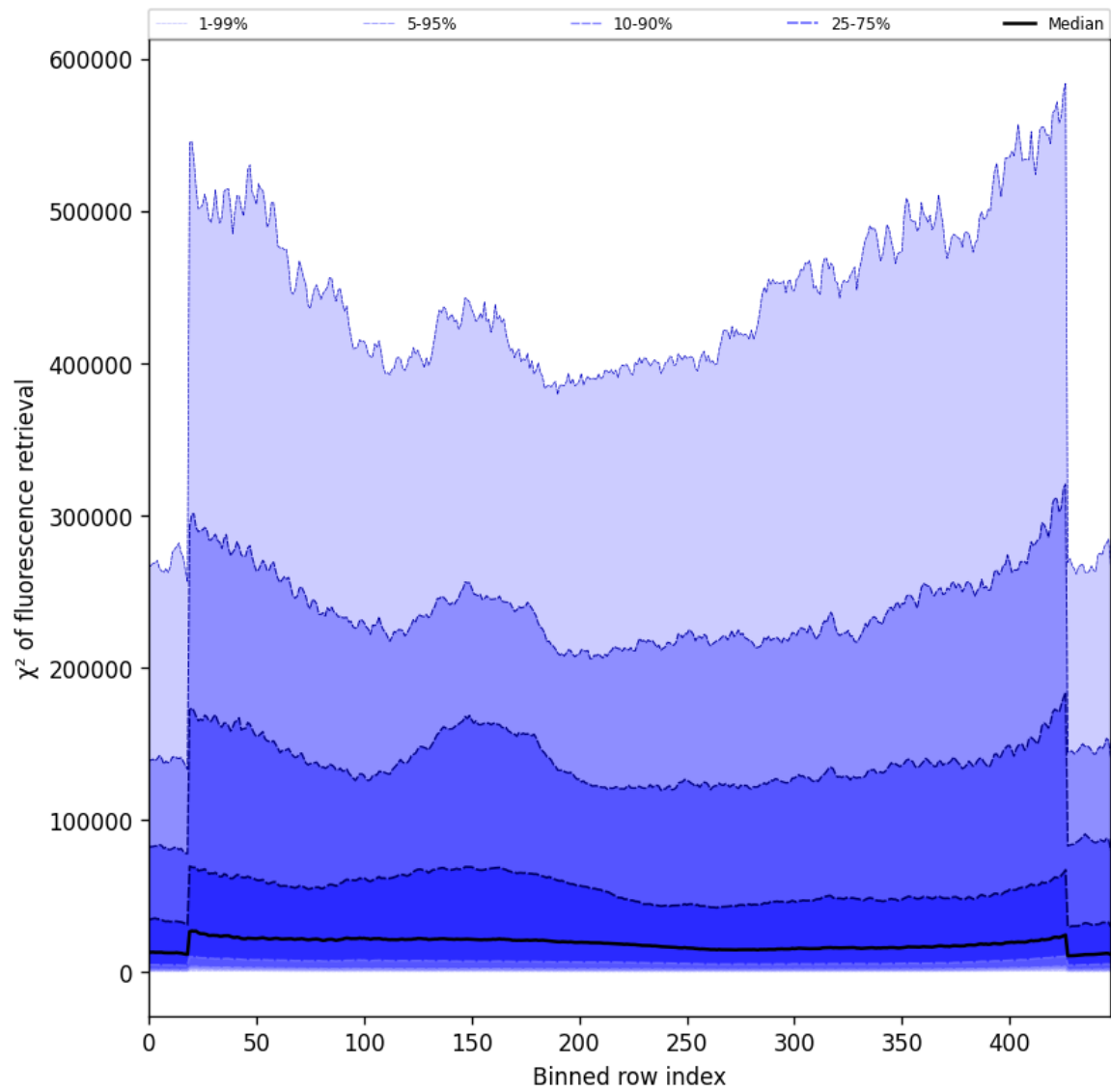
Figure 59: Along track statistics of “ \chi^2 of fluorescence retrieval” for 2025-04-19 to 2025-04-21
