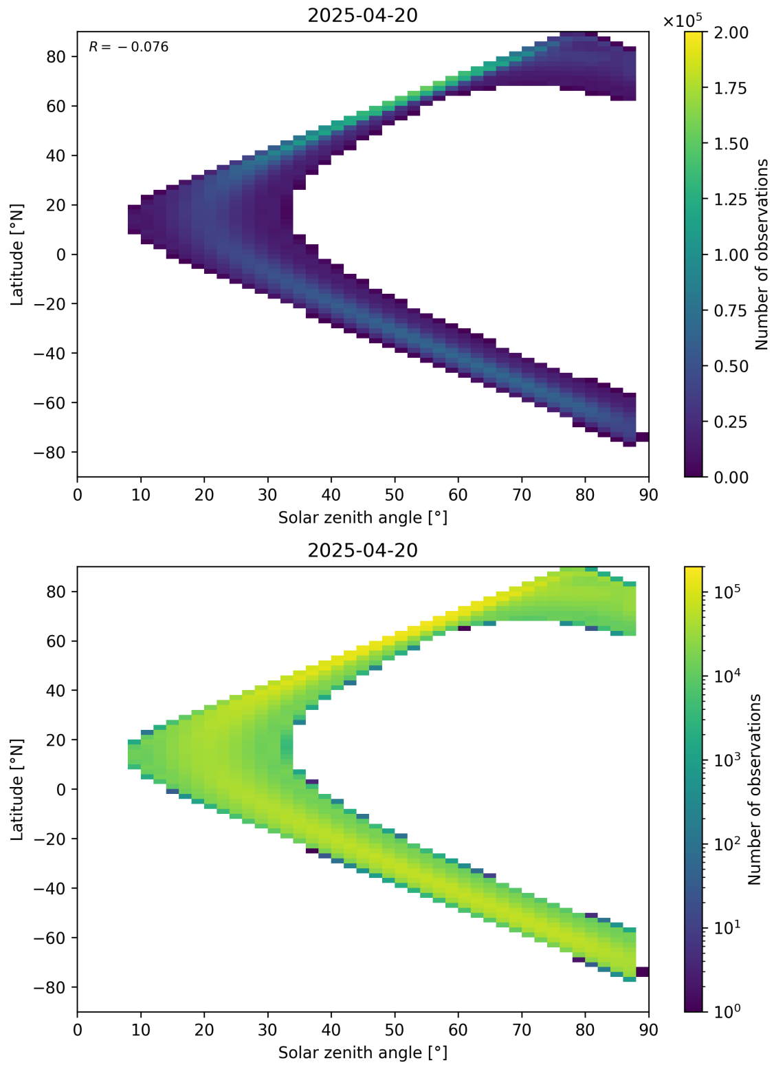
Figure 113: Scatter density plot of “Solar zenith angle” against “Latitude” for 2025-04-19 to 2025-04-21.
