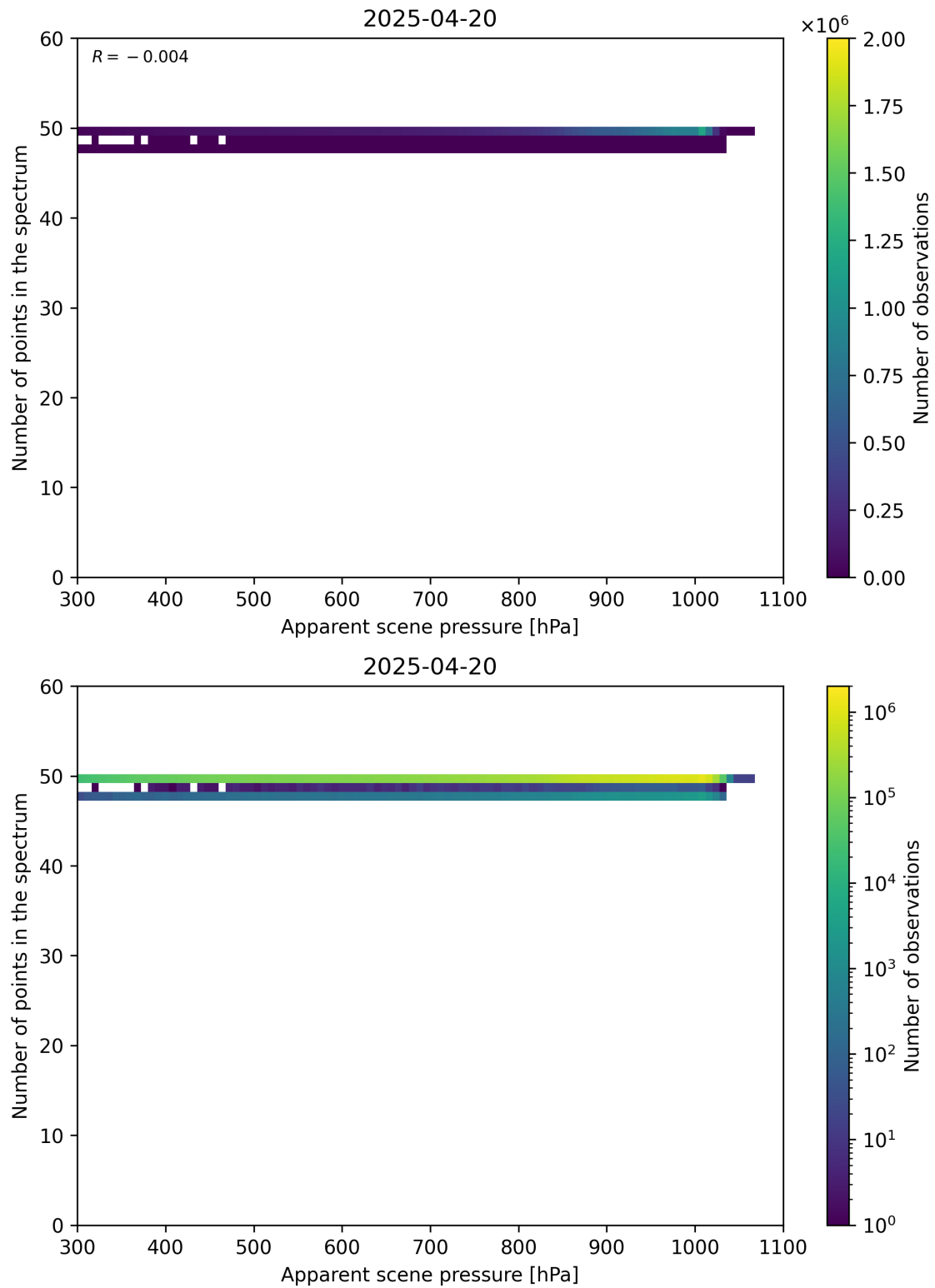
Figure 66: Scatter density plot of “Apparent scene pressure” against “Number of points in the spectrum” for 2025-04-19 to 2025-04-21.
