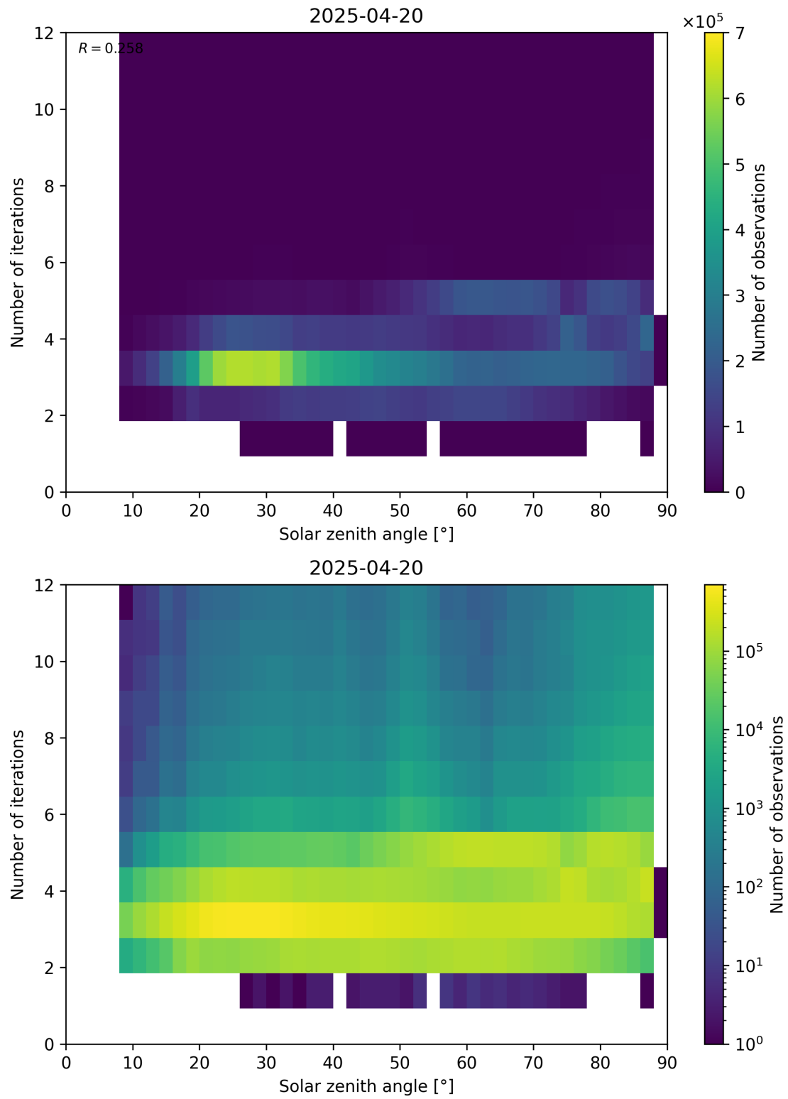
Figure 114: Scatter density plot of “Solar zenith angle” against “Number of iterations” for 2025-04-19 to 2025-04-21.
