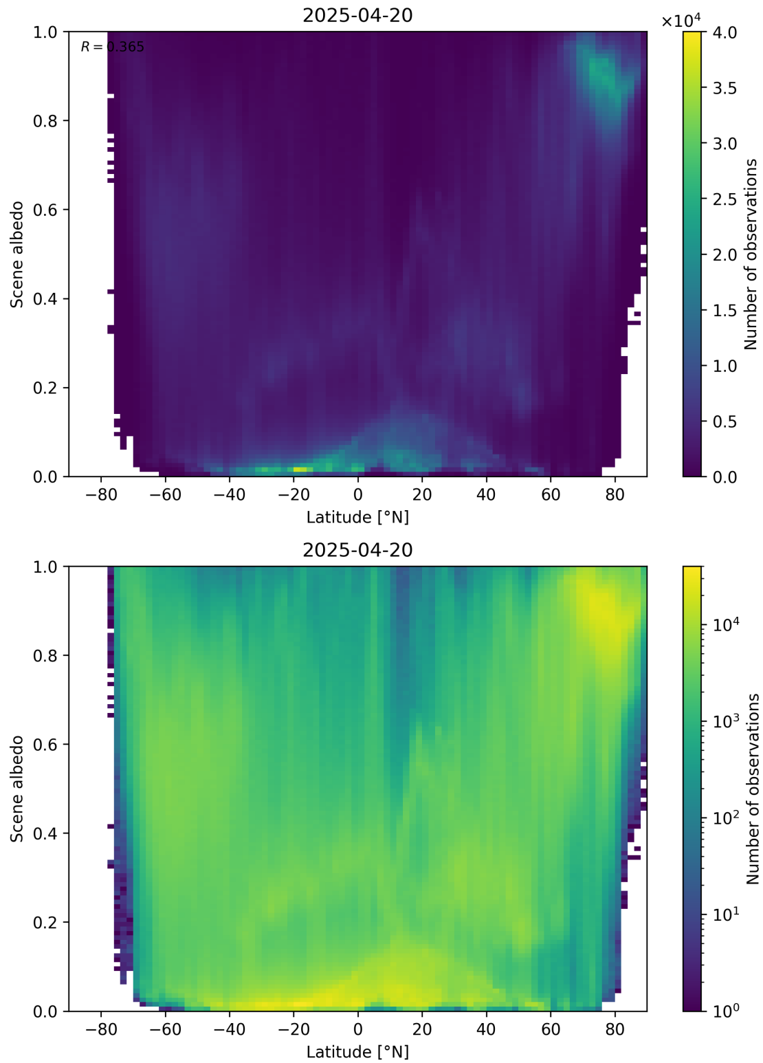
Figure 95: Scatter density plot of “Latitude” against “Scene albedo” for 2025-04-19 to 2025-04-21.
