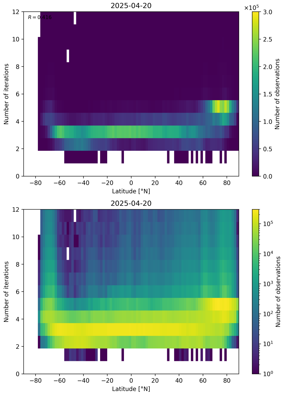
Figure 93: Scatter density plot of “Latitude” against “Number of iterations” for 2025-04-19 to 2025-04-21.
