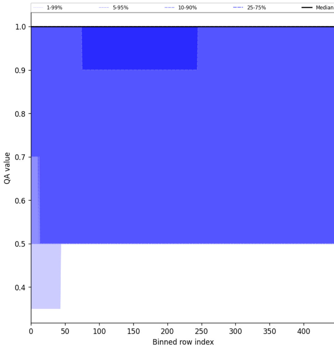
Figure 46: Along track statistics of “QA value” for 2025-04-19 to 2025-04-21
