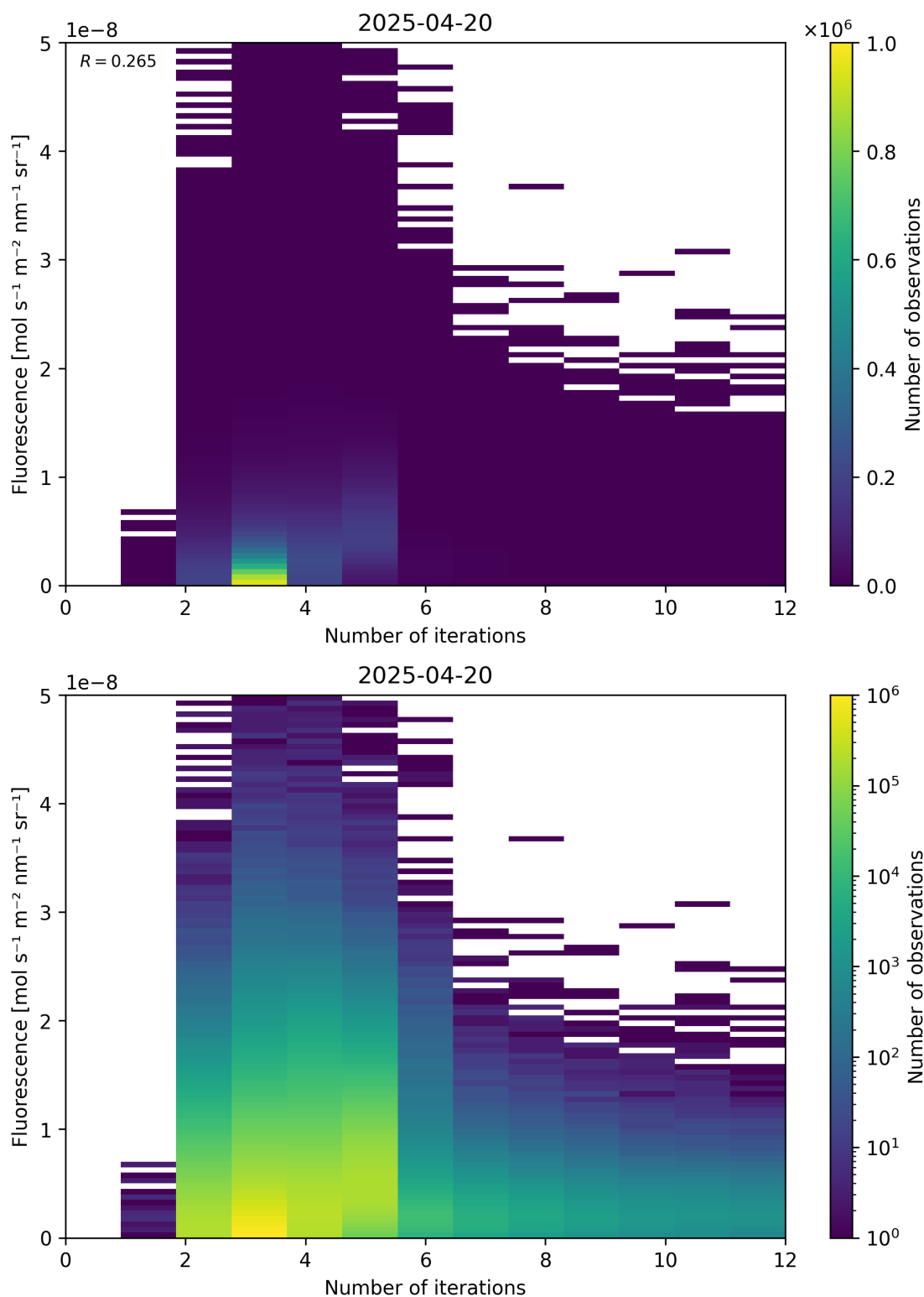
Figure 98: Scatter density plot of “Number of iterations” against “Fluorescence” for 2025-04-19 to 2025-04-21.
