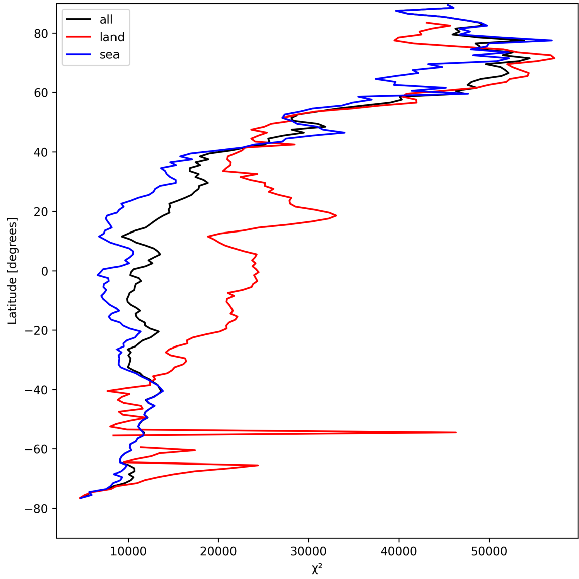
Figure 21: Zonal average of “ \chi^2 ” for 2025-04-19 to 2025-04-21.
