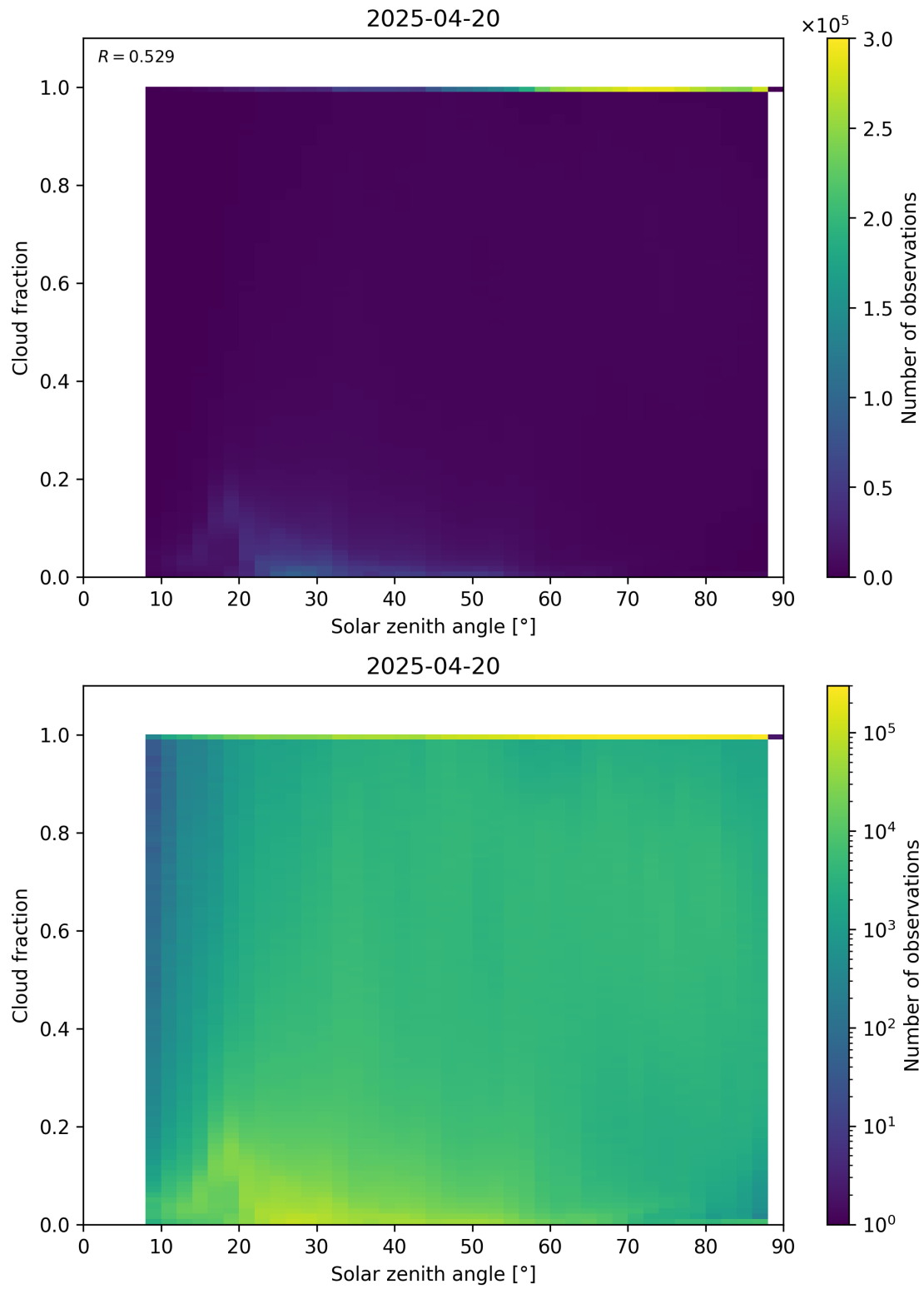
Figure 110: Scatter density plot of “Solar zenith angle” against “Cloud fraction” for 2025-04-19 to 2025-04-21.
