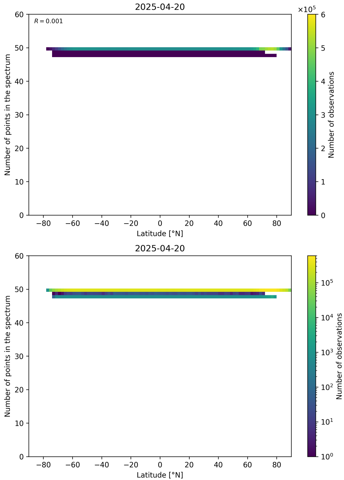
Figure 94: Scatter density plot of “Latitude” against “Number of points in the spectrum” for 2025-04-19 to 2025-04-21.
