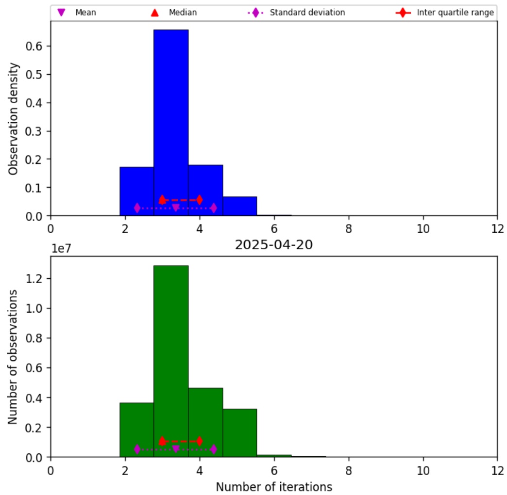
Figure 39: Histogram of “Number of iterations” for 2025-04-19 to 2025-04-21
