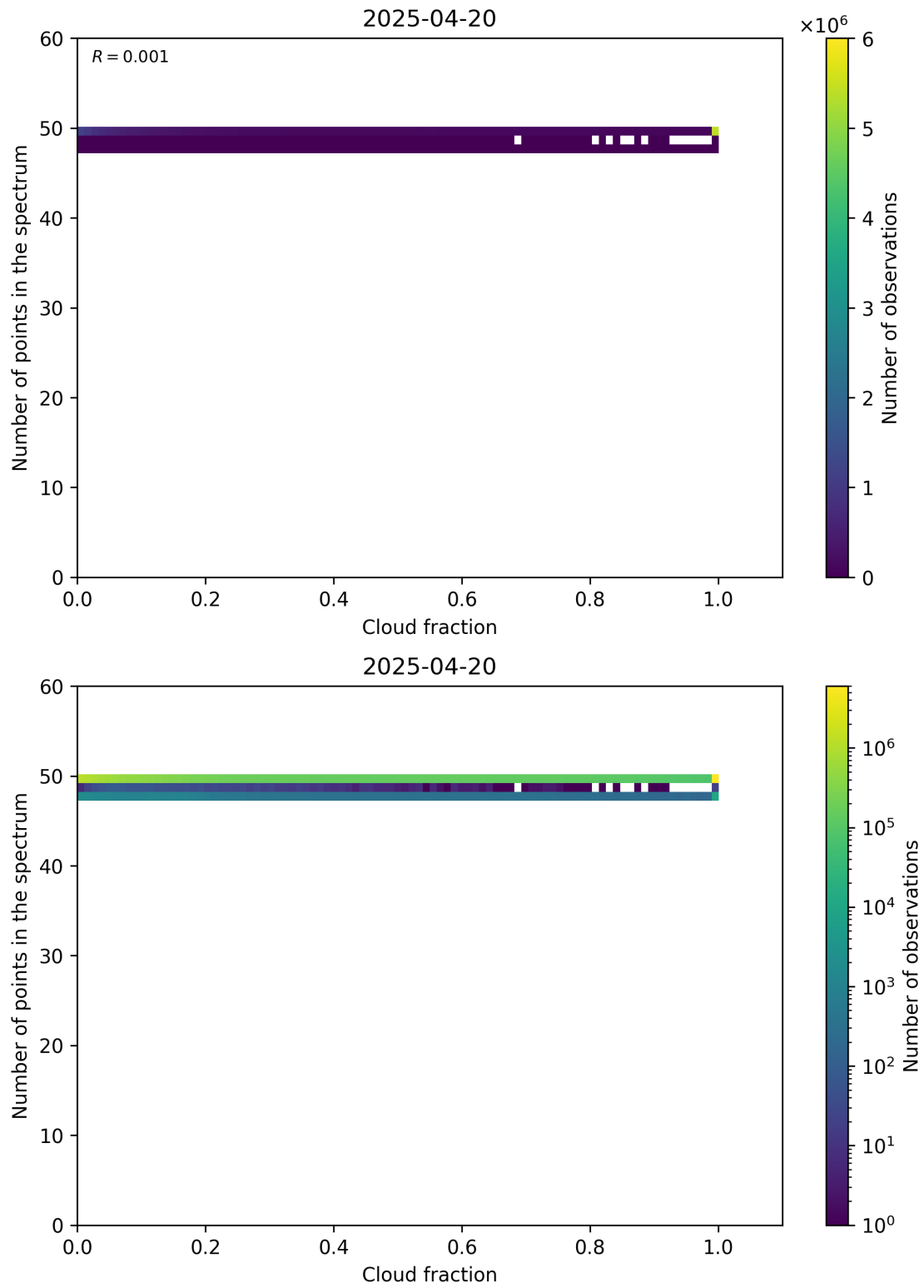
Figure 74: Scatter density plot of “Cloud fraction” against “Number of points in the spectrum” for 2025-04-19 to 2025-04-21.
