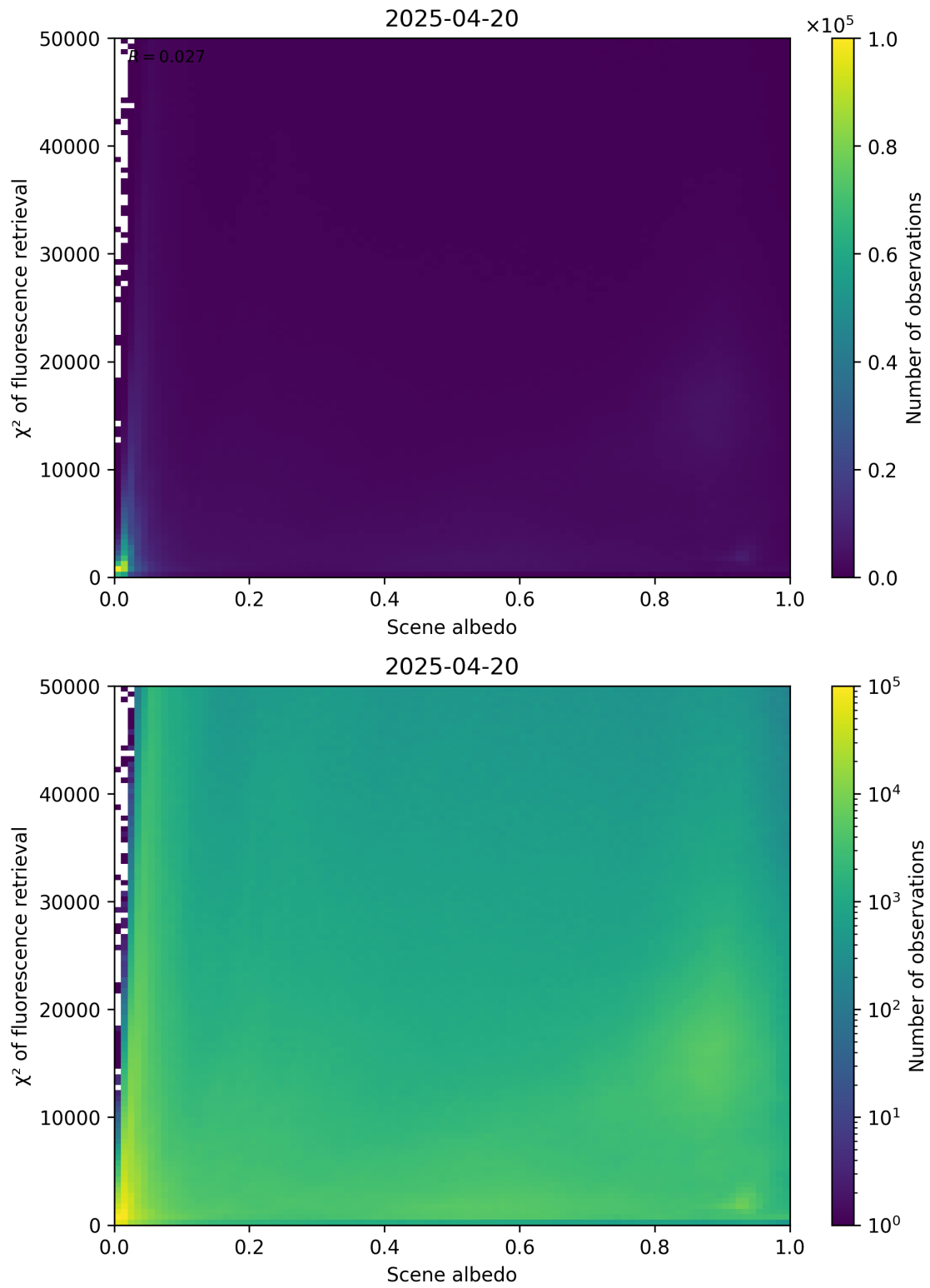
Figure 103: Scatter density plot of “Scene albedo” against “ \chi^2 of fluorescence retrieval” for 2025-04-19 to 2025-04-21.
