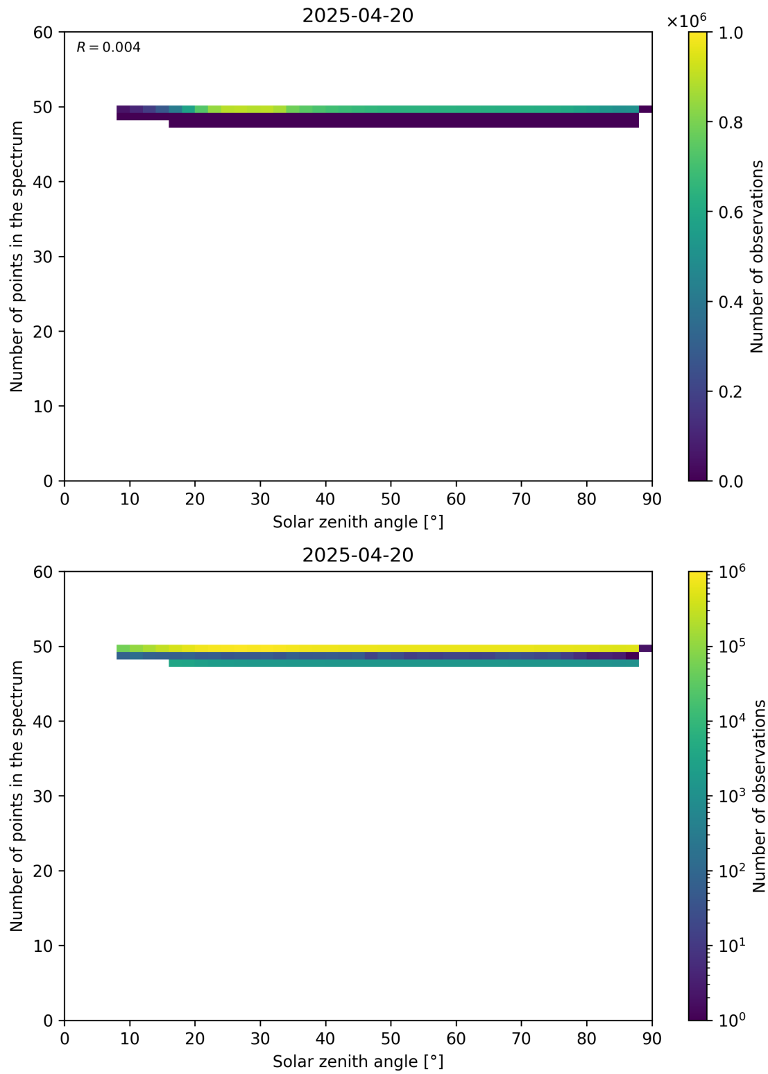
Figure 115: Scatter density plot of “Solar zenith angle” against “Number of points in the spectrum” for 2025-04-19 to 2025-04-21.
