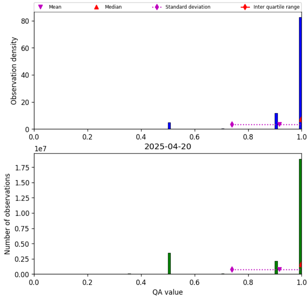
Figure 29: Histogram of “QA value” for 2025-04-19 to 2025-04-21
