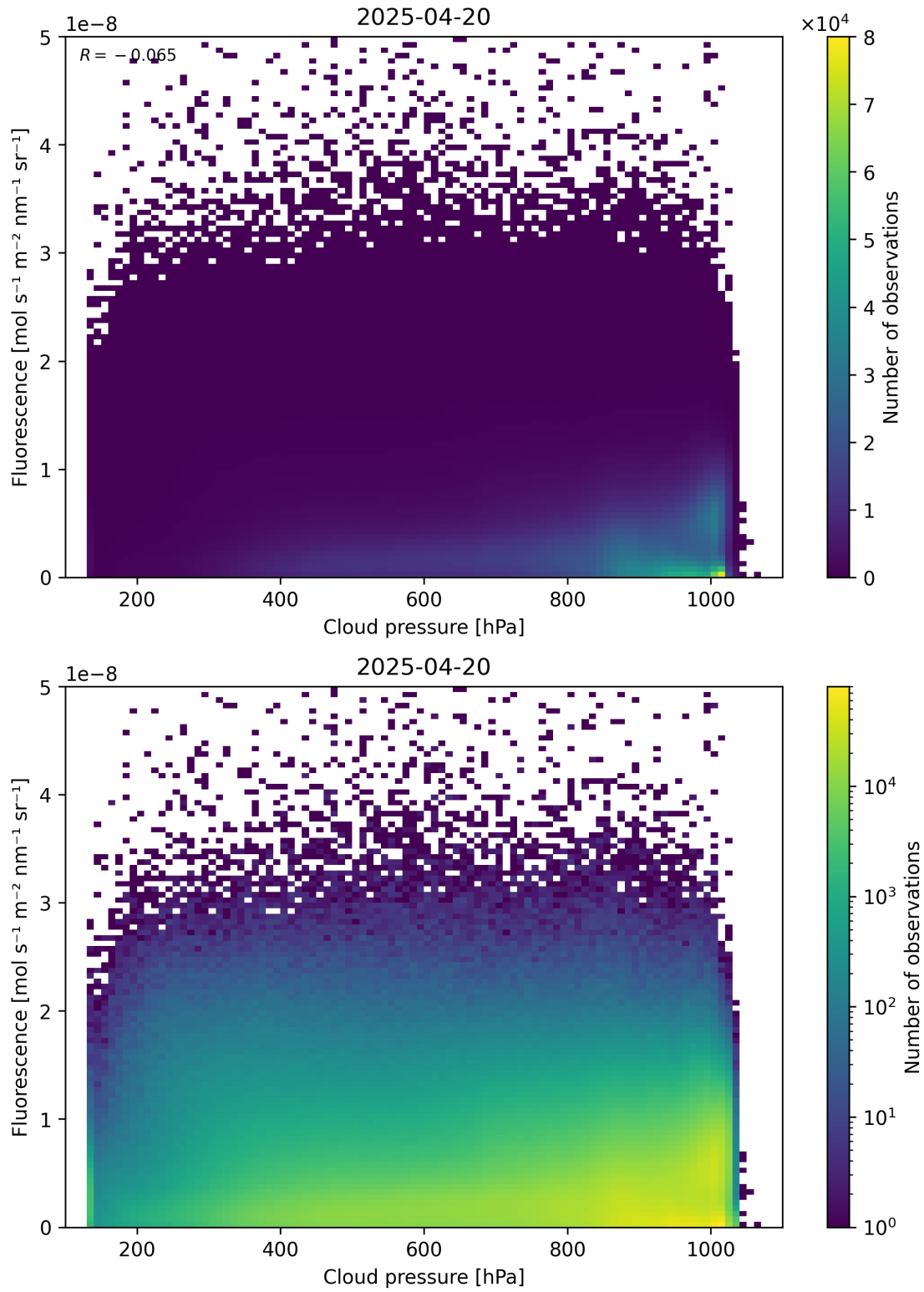
Figure 80: Scatter density plot of “Cloud pressure” against “Fluorescence” for 2025-04-19 to 2025-04-21.
