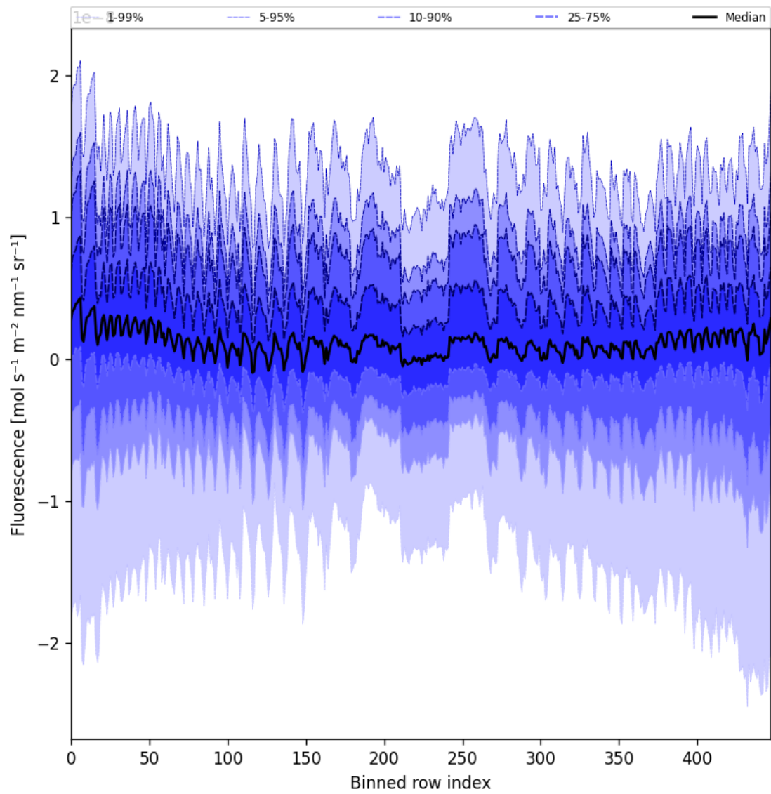
Figure 57: Along track statistics of “Fluorescence” for 2025-04-19 to 2025-04-21
