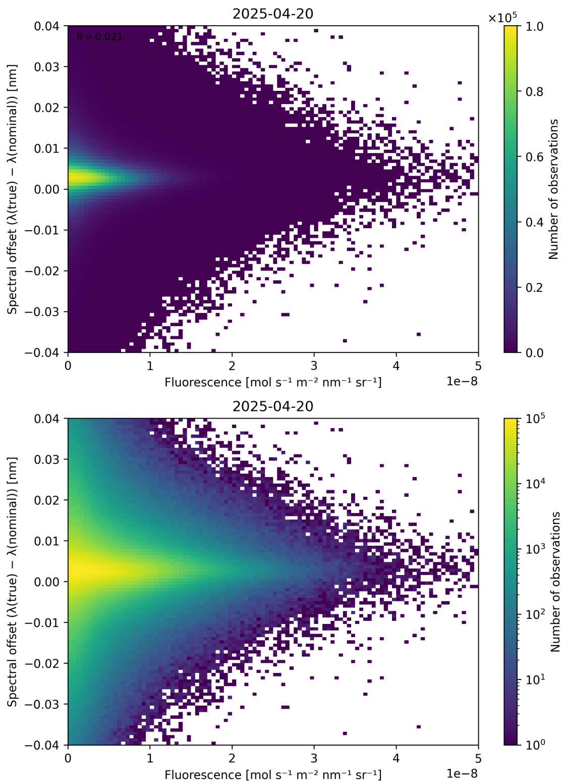
Figure 87: Scatter density plot of “Fluorescence” against “Spectral offset ( \lambda_{\text{true}} - \lambda_{\text{nominal}} )” for 2025-04-19 to 2025-04-21.
