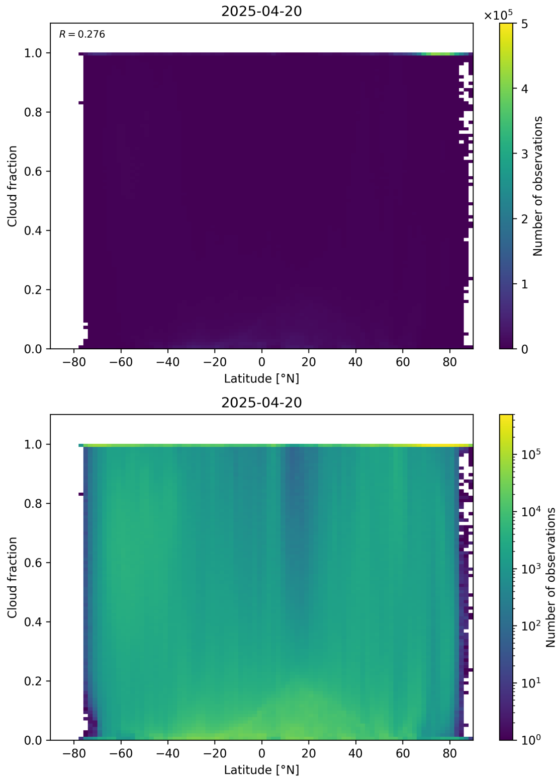
Figure 90: Scatter density plot of “Latitude” against “Cloud fraction” for 2025-04-19 to 2025-04-21.
