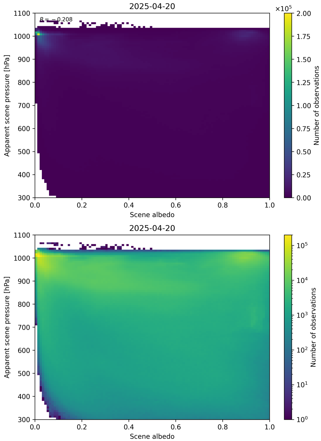
Figure 102: Scatter density plot of “Scene albedo” against “Apparent scene pressure” for 2025-04-19 to 2025-04-21.
