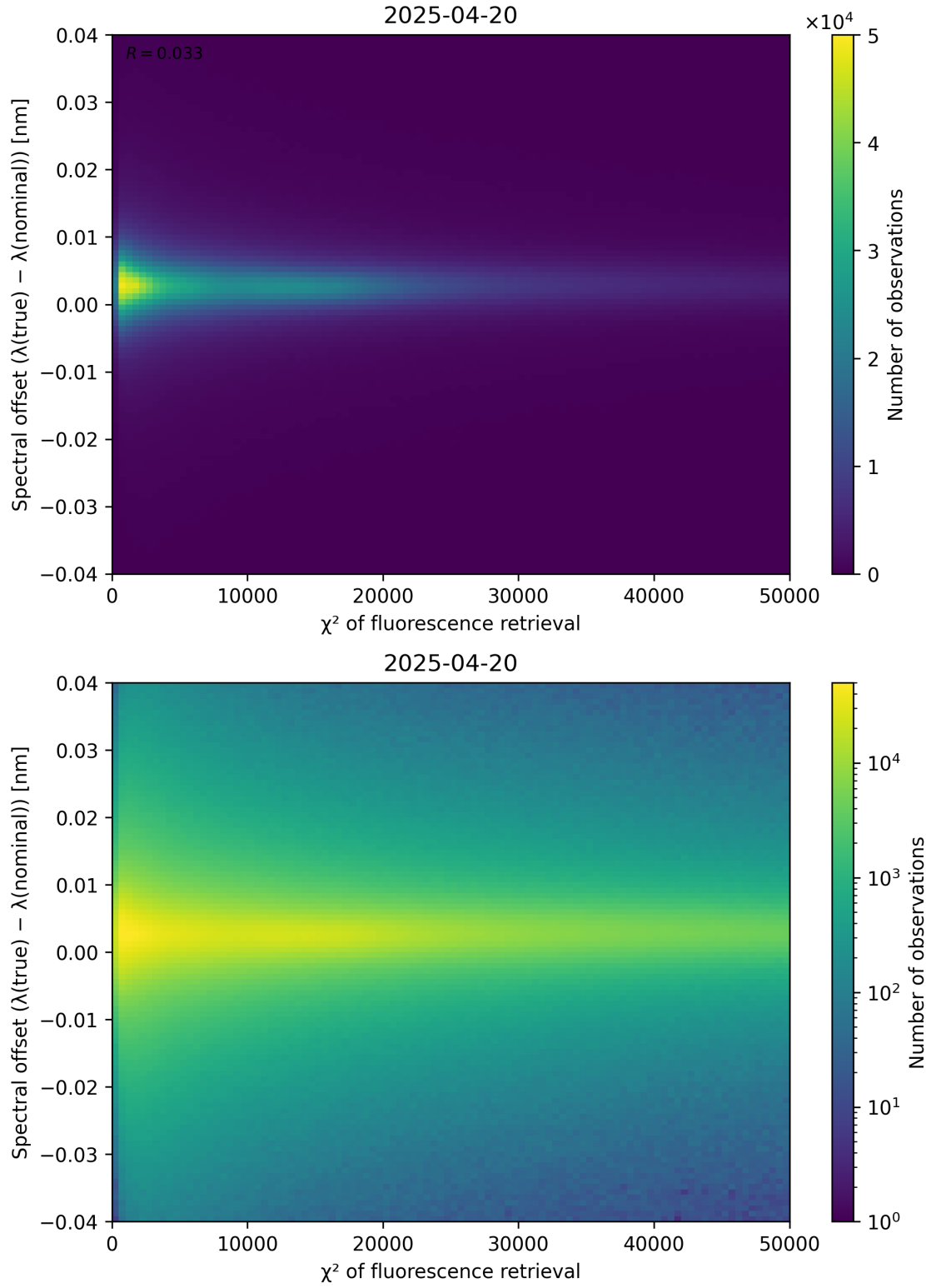
Figure 69: Scatter density plot of " \chi^2 of fluorescence retrieval" against "Spectral offset ( \lambda_{\text{true}} - \lambda_{\text{nominal}} )" for 2025-04-19 to 2025-04-21.
