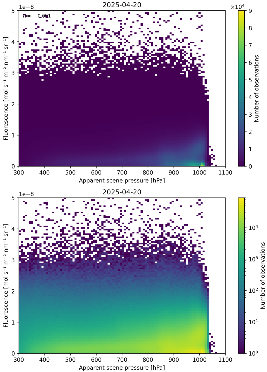
Figure 64: Scatter density plot of “Apparent scene pressure” against “Fluorescence” for 2025-04-19 to 2025-04-21.
