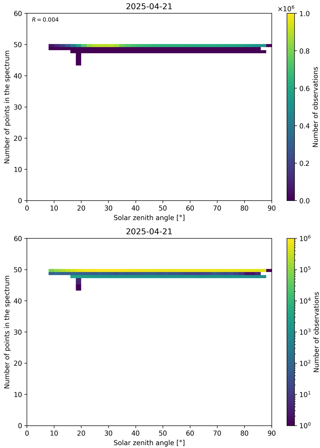
Figure 115: Scatter density plot of “Solar zenith angle” against “Number of points in the spectrum” for 2025-04-20 to 2025-04-22.
