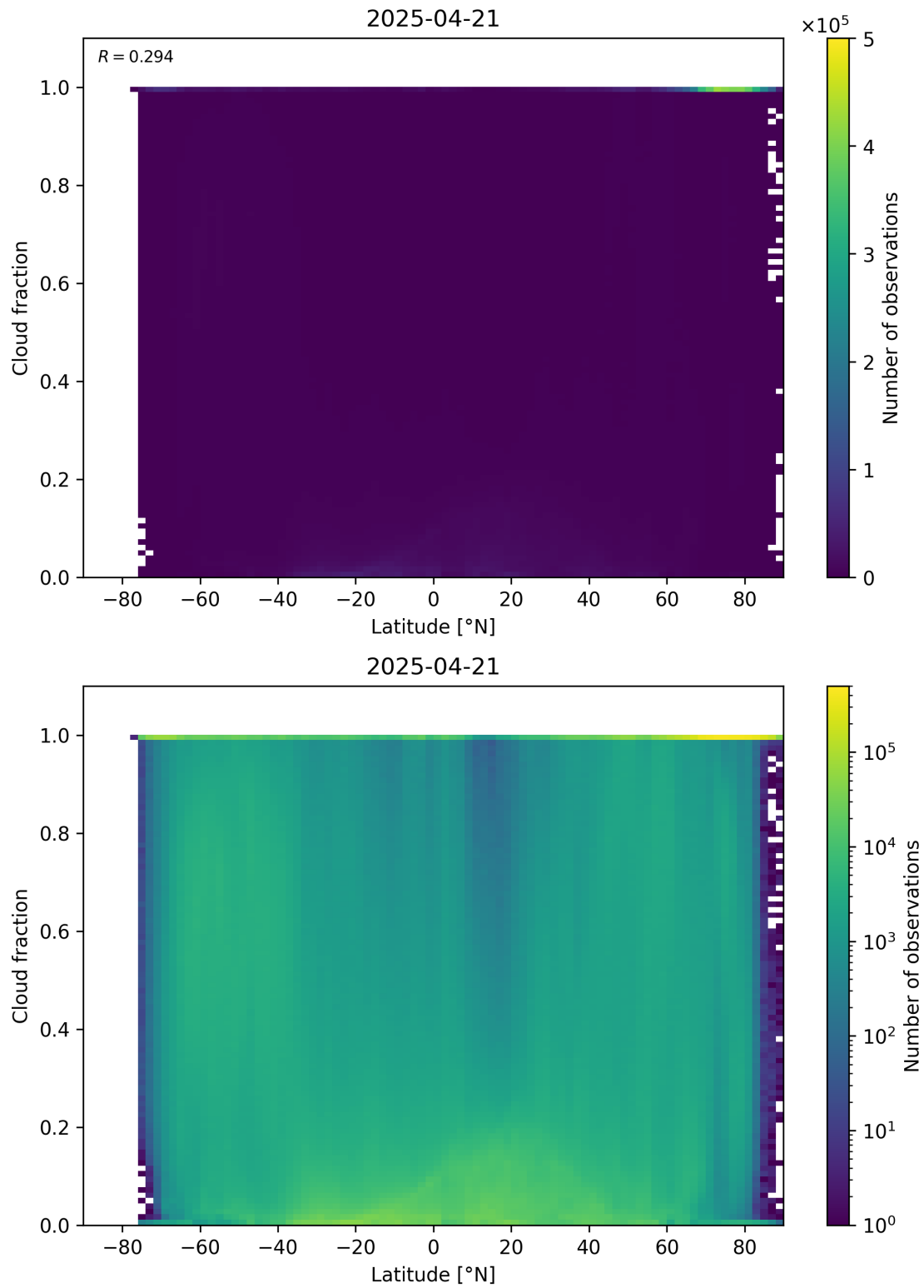
Figure 90: Scatter density plot of “Latitude” against “Cloud fraction” for 2025-04-20 to 2025-04-22.
