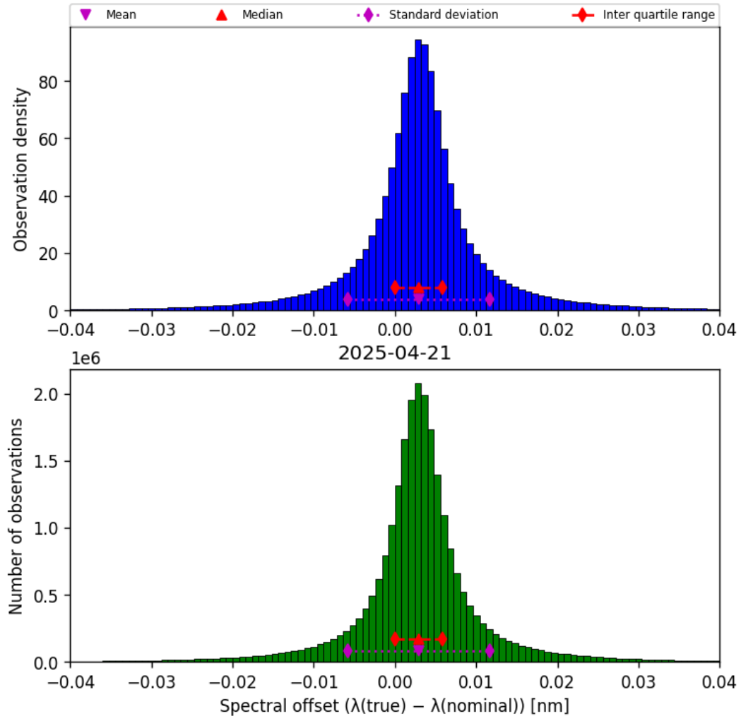
Figure 45: Histogram of “Spectral offset ( \lambda_{\text{true}} - \lambda_{\text{nominal}} )” for 2025-04-20 to 2025-04-22
