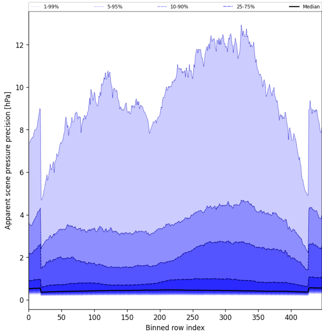
Figure 54: Along track statistics of “Apparent scene pressure precision” for 2025-04-20 to 2025-04-22
