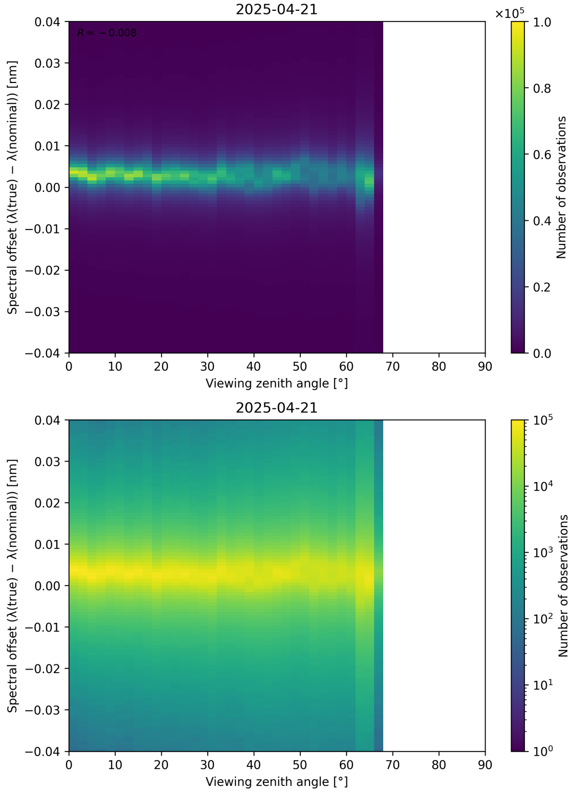
Figure 128: Scatter density plot of “Viewing zenith angle” against “Spectral offset ( \lambda_{\text{true}} - \lambda_{\text{nominal}} )” for 2025-04-20 to 2025-04-22.
