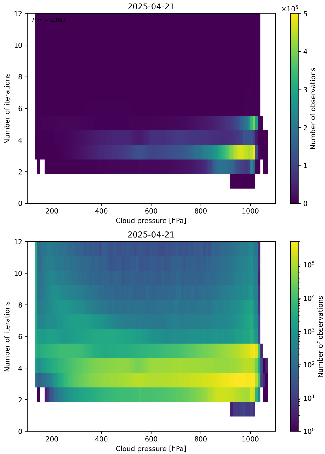
Figure 81: Scatter density plot of “Cloud pressure” against “Number of iterations” for 2025-04-20 to 2025-04-22.
