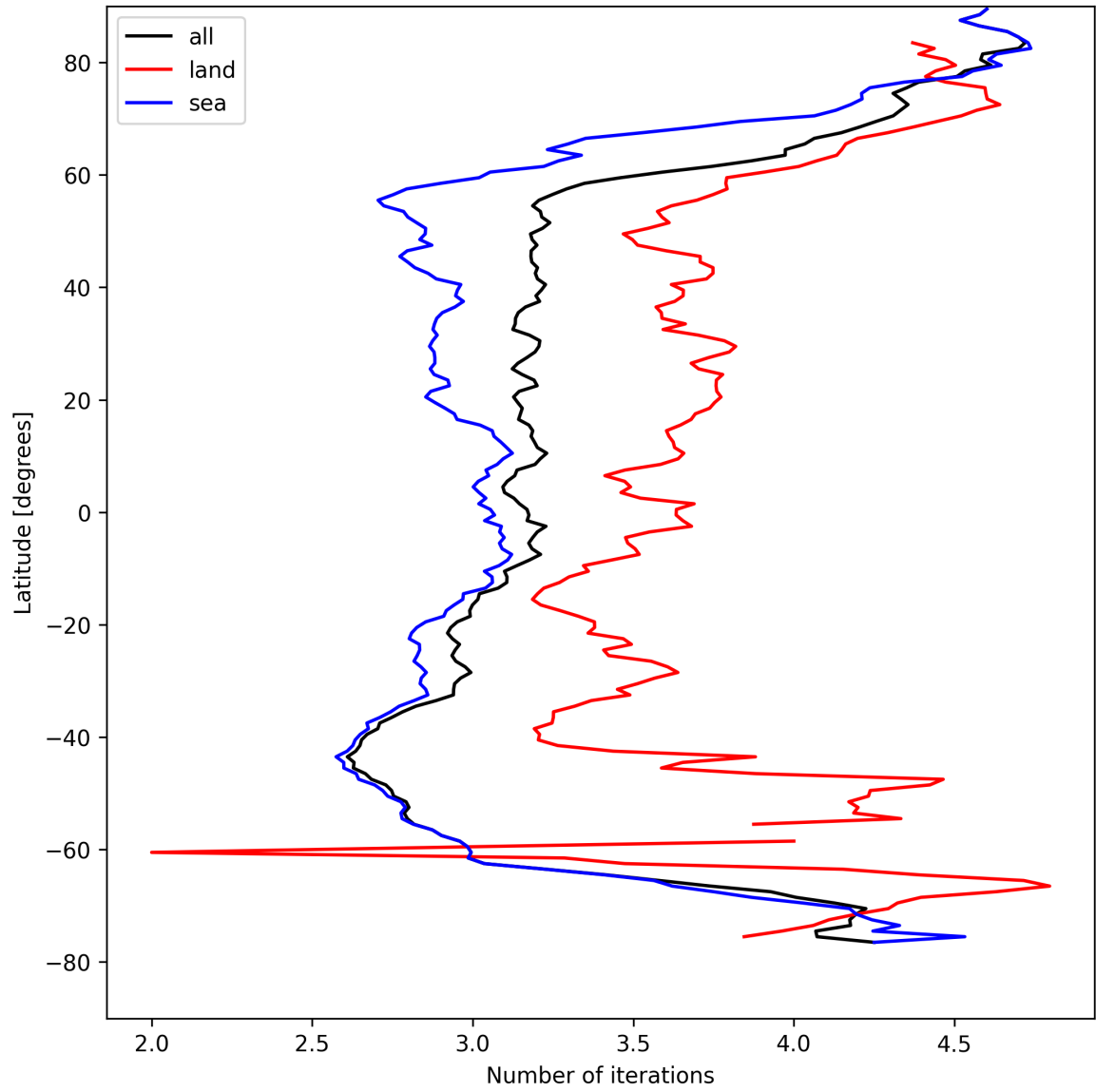
Figure 22: Zonal average of “Number of iterations” for 2025-04-20 to 2025-04-22.
