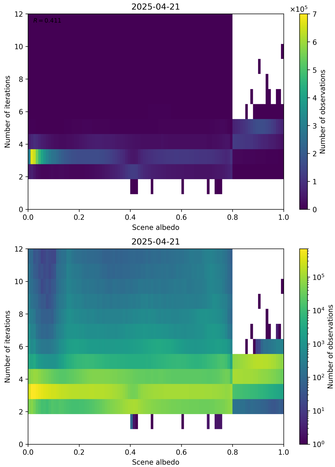
Figure 105: Scatter density plot of “Scene albedo” against “Number of iterations” for 2025-04-20 to 2025-04-22.
