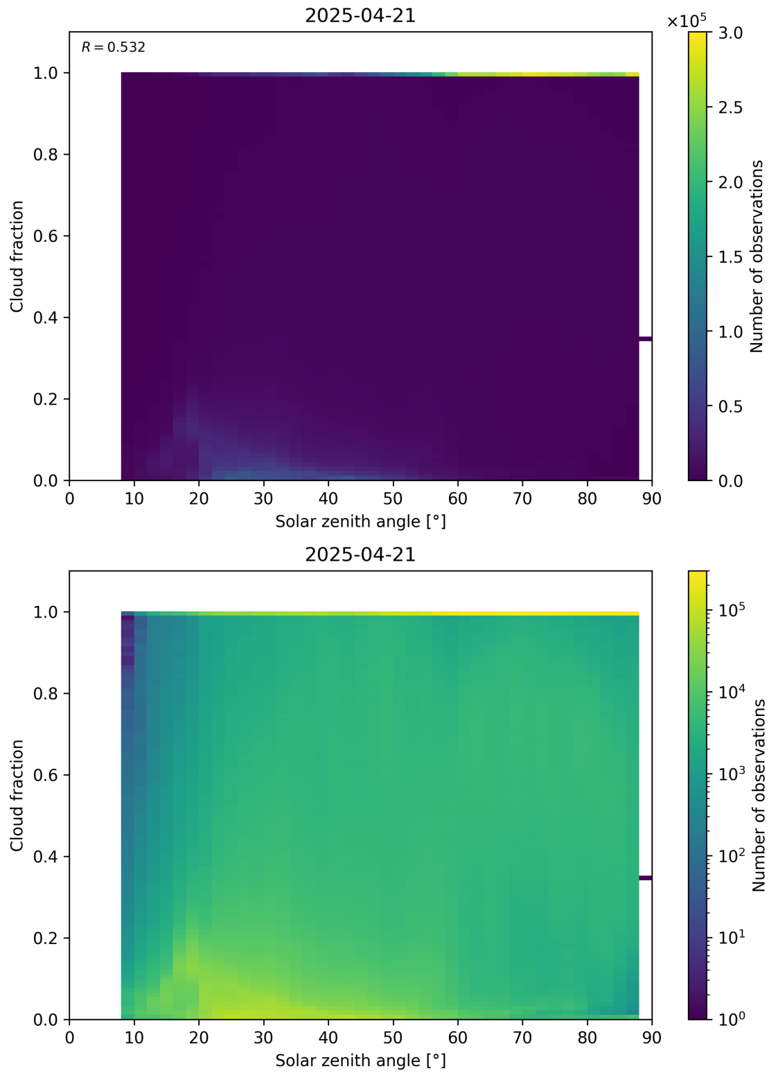
Figure 110: Scatter density plot of “Solar zenith angle” against “Cloud fraction” for 2025-04-20 to 2025-04-22.
