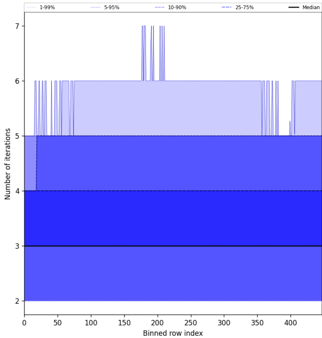
Figure 56: Along track statistics of “Number of iterations” for 2025-04-20 to 2025-04-22
