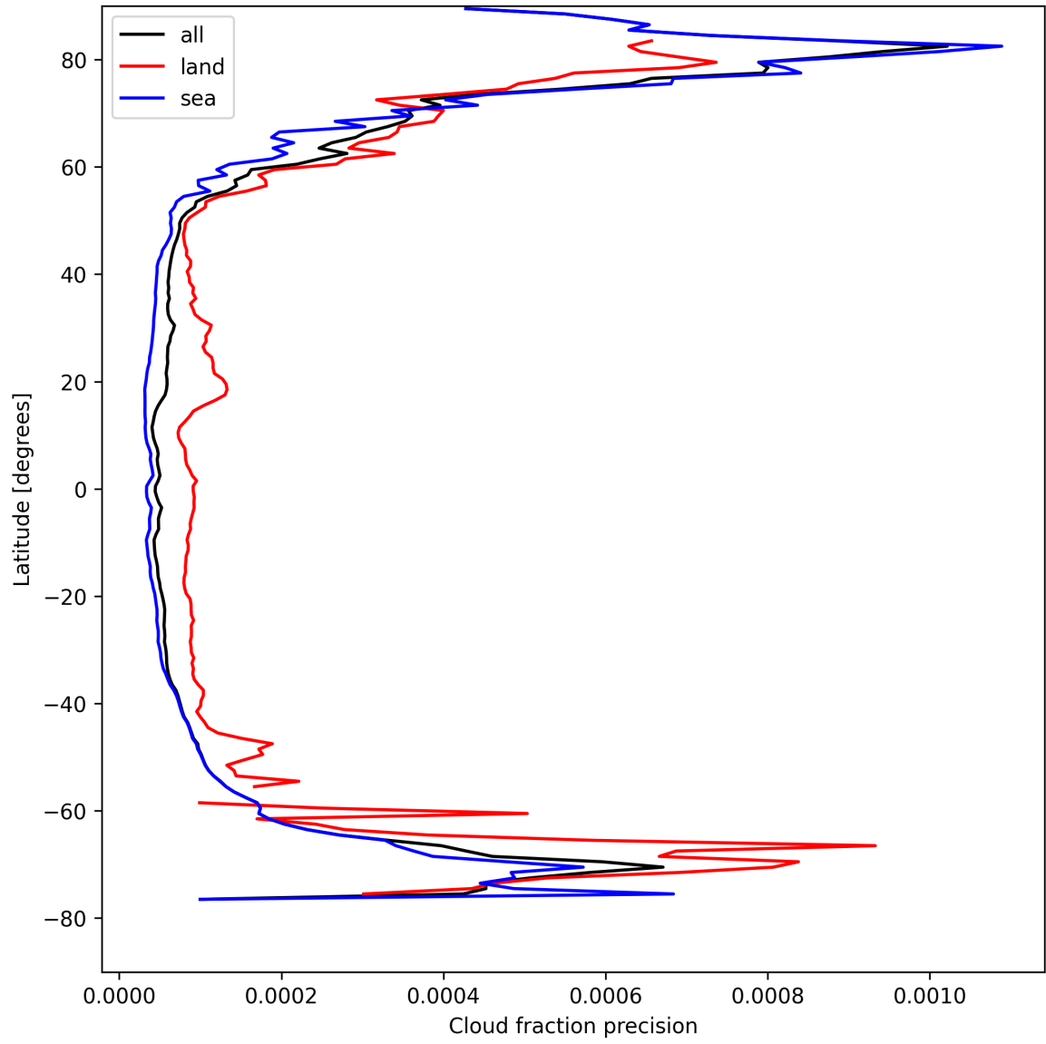
Figure 16: Zonal average of “Cloud fraction precision” for 2025-04-20 to 2025-04-22.
