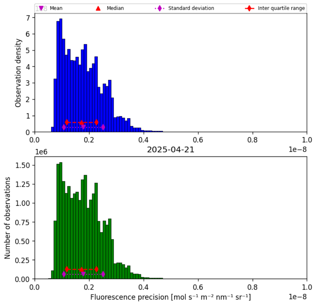
Figure 41: Histogram of “Fluorescence precision” for 2025-04-20 to 2025-04-22
