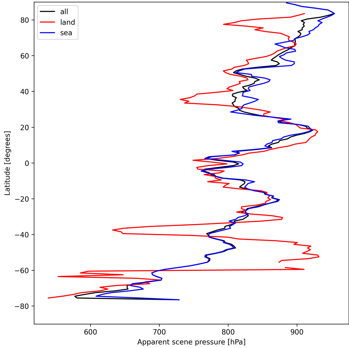
Figure 19: Zonal average of “Apparent scene pressure” for 2025-04-20 to 2025-04-22.
