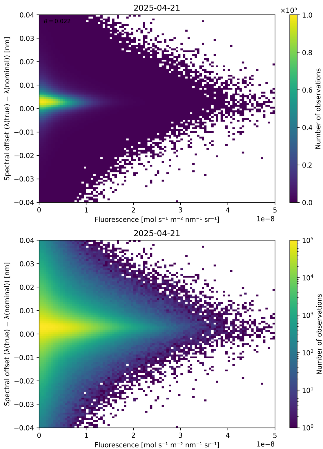
Figure 87: Scatter density plot of “Fluorescence” against “Spectral offset ( \lambda_{\text{true}} - \lambda_{\text{nominal}} )” for 2025-04-20 to 2025-04-22.
