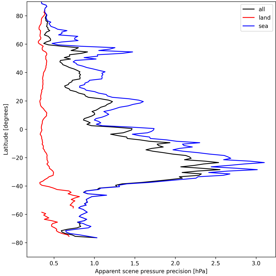
Figure 20: Zonal average of “Apparent scene pressure precision” for 2025-04-20 to 2025-04-22.
