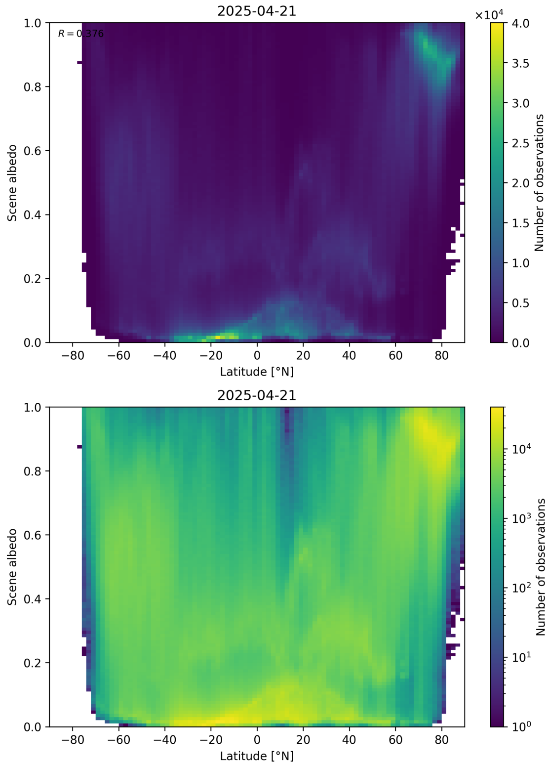
Figure 95: Scatter density plot of “Latitude” against “Scene albedo” for 2025-04-20 to 2025-04-22.
