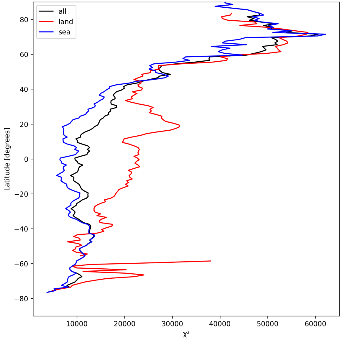
Figure 21: Zonal average of “ \chi^2 ” for 2025-04-20 to 2025-04-22.
