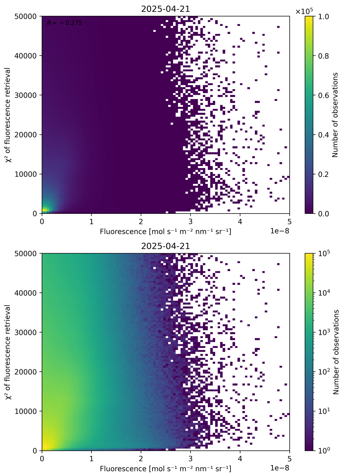
Figure 85: Scatter density plot of “Fluorescence” against “ \chi^2 of fluorescence retrieval” for 2025-04-20 to 2025-04-22.
