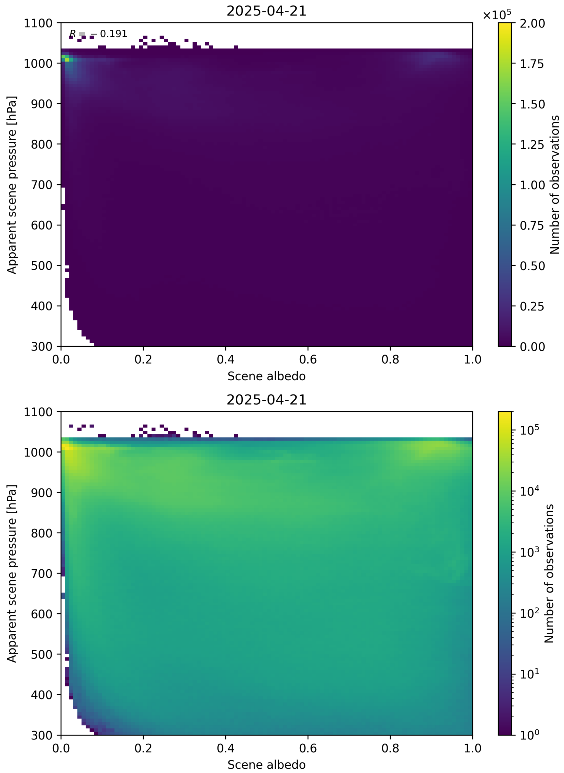
Figure 102: Scatter density plot of “Scene albedo” against “Apparent scene pressure” for 2025-04-20 to 2025-04-22.
