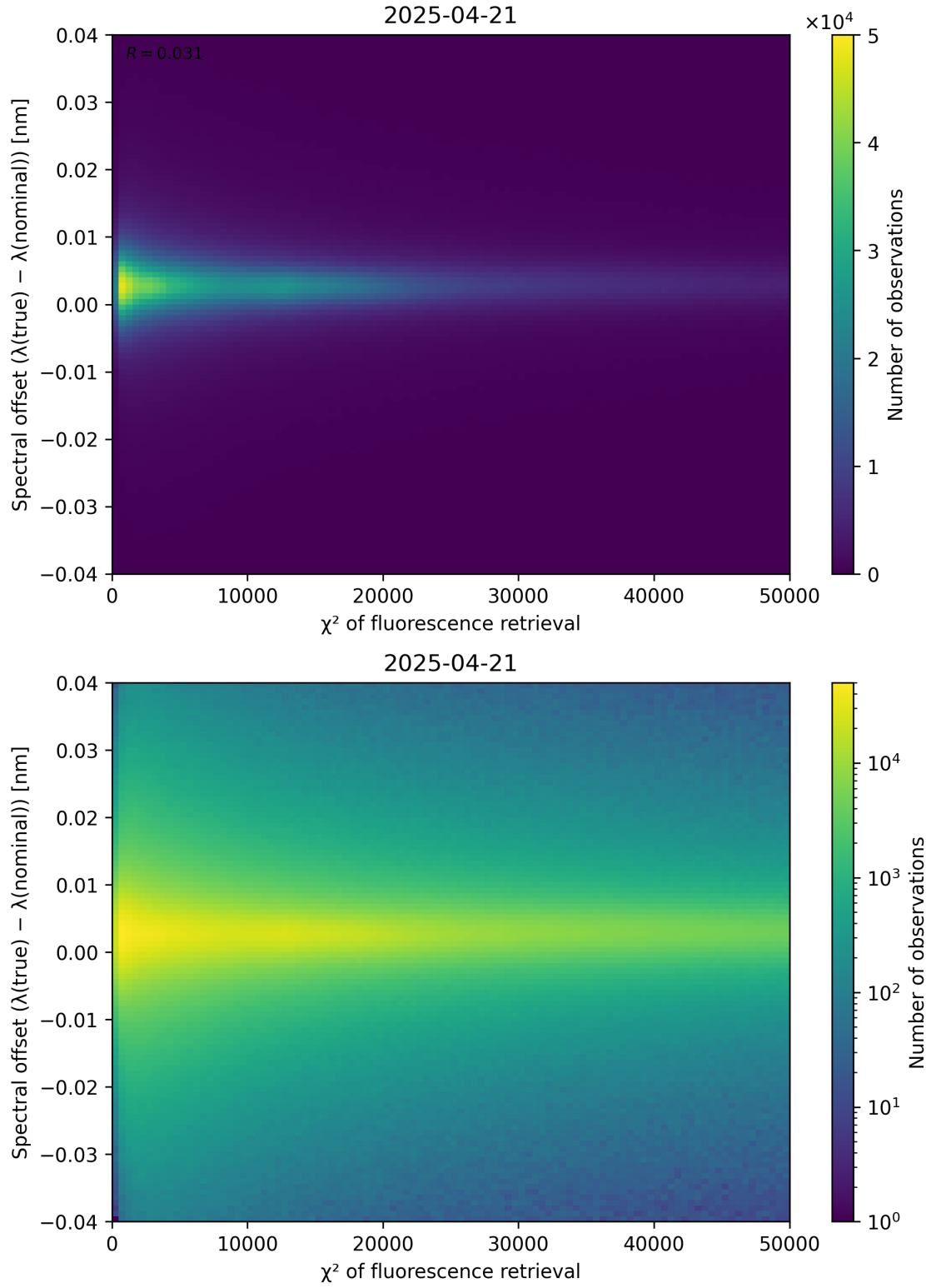
Figure 69: Scatter density plot of “ \chi^2 of fluorescence retrieval” against “Spectral offset ( \lambda_{\text{true}} - \lambda_{\text{nominal}} )” for 2025-04-20 to 2025-04-22.
