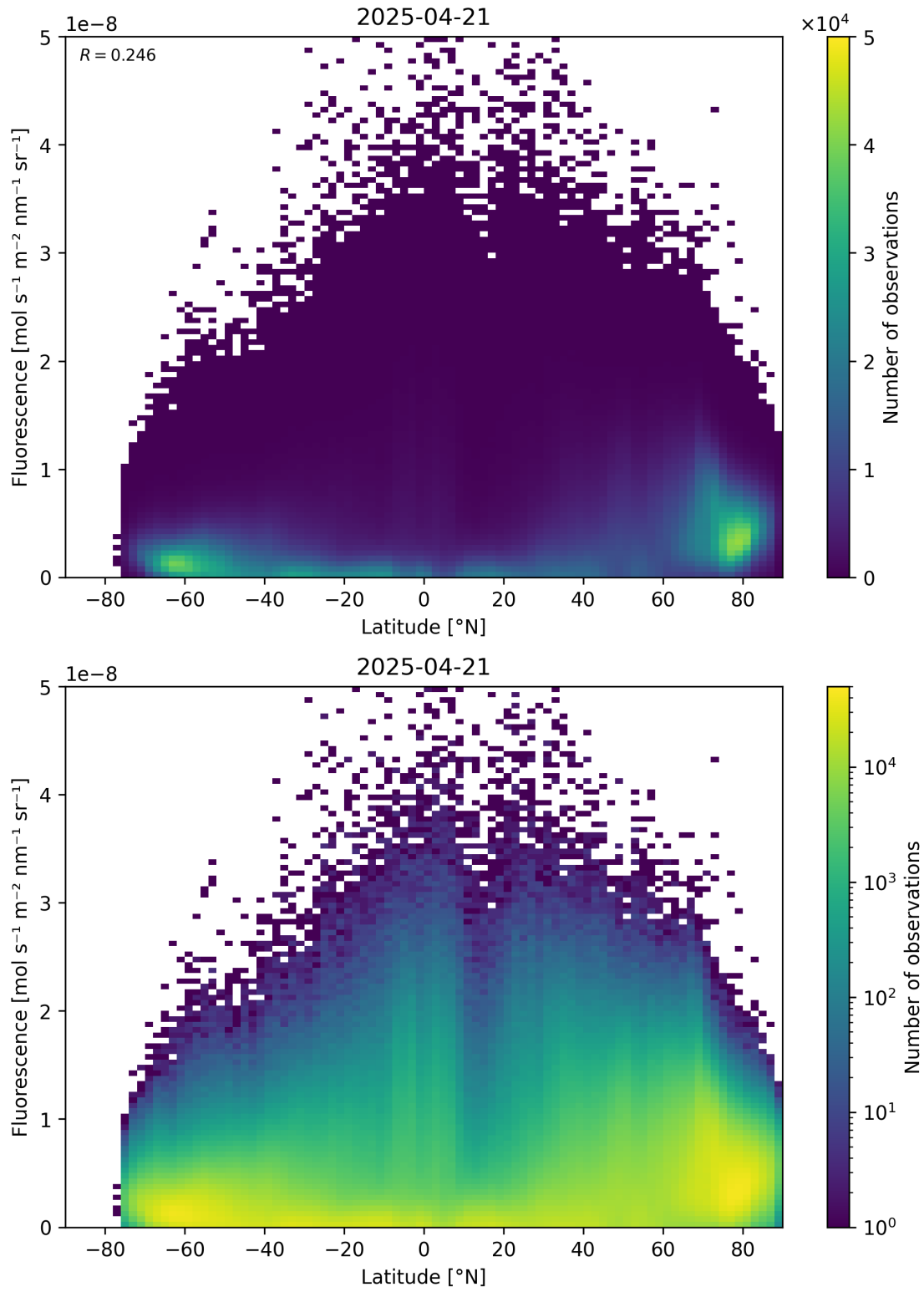
Figure 92: Scatter density plot of “Latitude” against “Fluorescence” for 2025-04-20 to 2025-04-22.
