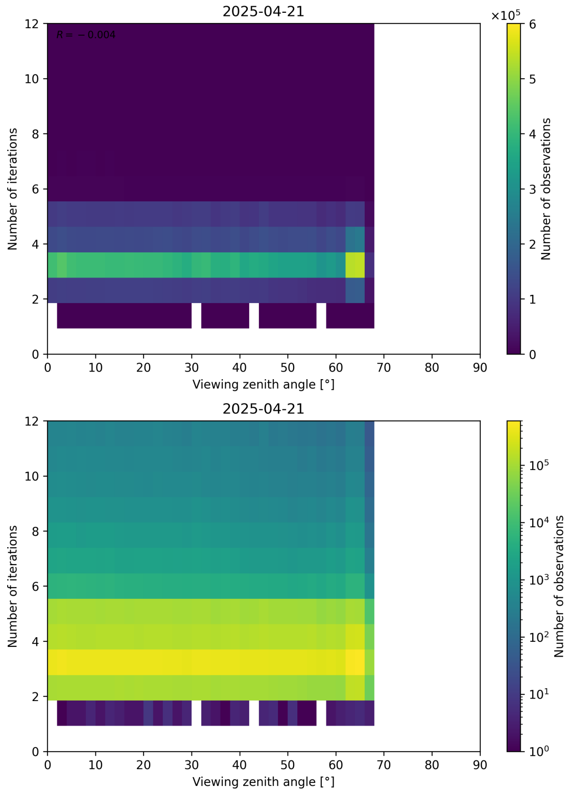
Figure 124: Scatter density plot of “Viewing zenith angle” against “Number of iterations” for 2025-04-20 to 2025-04-22.
