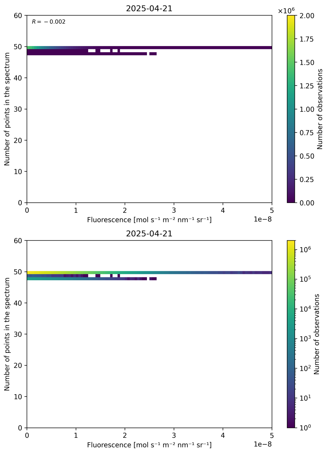
Figure 86: Scatter density plot of “Fluorescence” against “Number of points in the spectrum” for 2025-04-20 to 2025-04-22.
