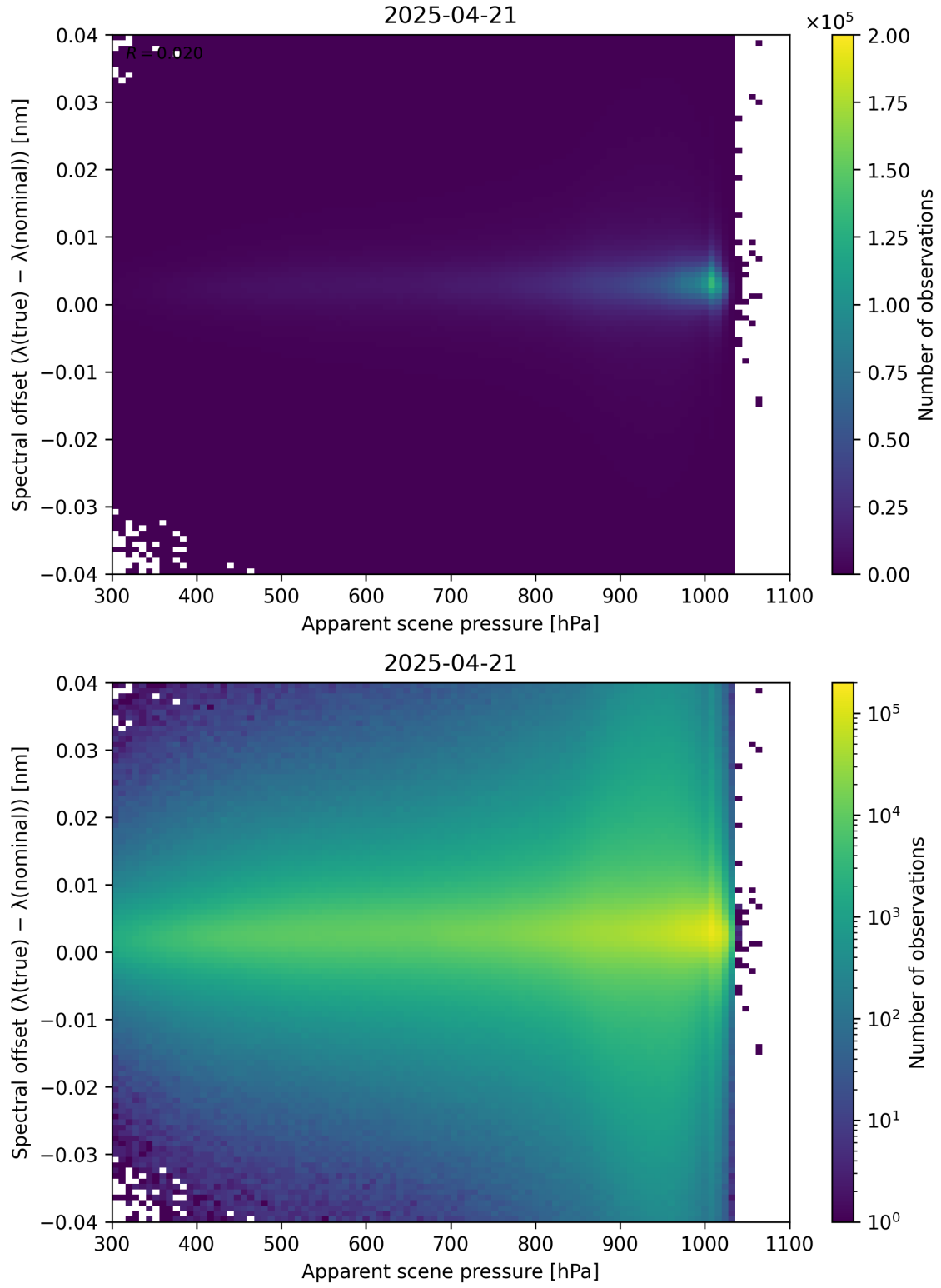
Figure 67: Scatter density plot of “Apparent scene pressure” against “Spectral offset ( \lambda_{\text{true}} - \lambda_{\text{nominal}} )” for 2025-04-20 to 2025-04-22.
