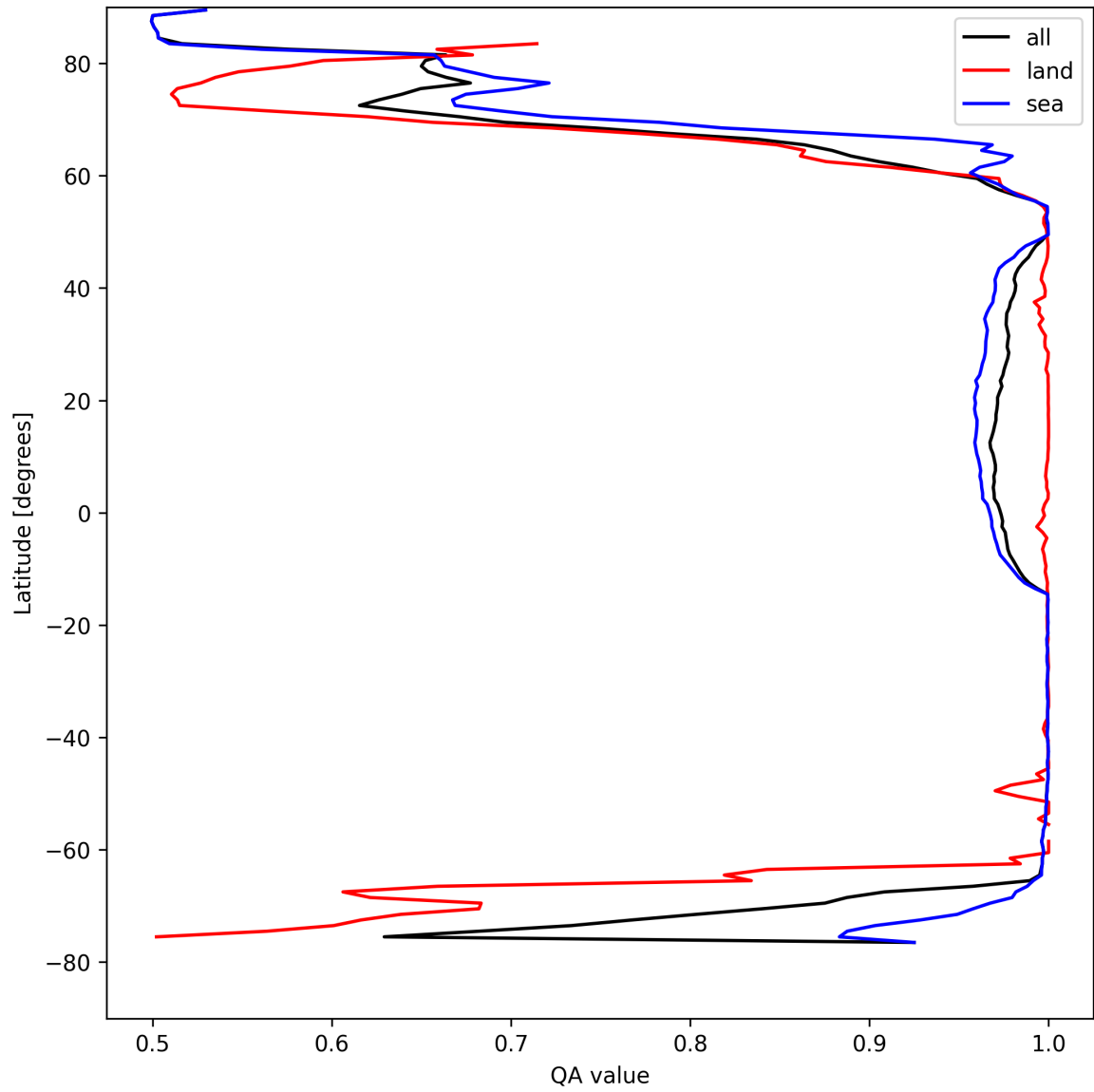
Figure 12: Zonal average of “QA value” for 2025-04-20 to 2025-04-22.
