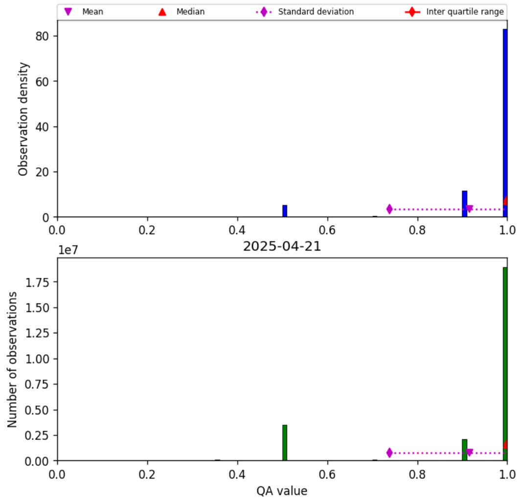
Figure 29: Histogram of “QA value” for 2025-04-20 to 2025-04-22
