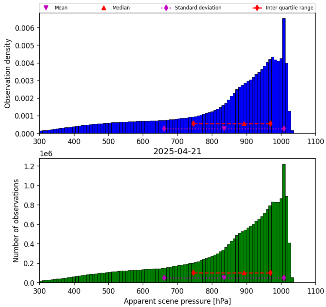
Figure 36: Histogram of “Apparent scene pressure” for 2025-04-20 to 2025-04-22
