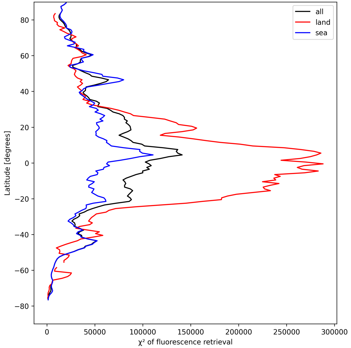
Figure 25: Zonal average of “ \chi^2 of fluorescence retrieval” for 2025-04-20 to 2025-04-22.
