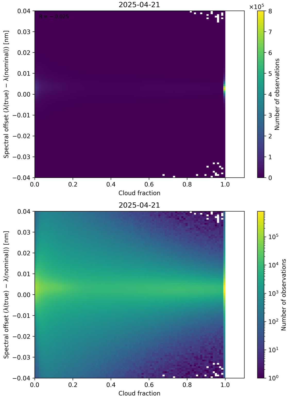
Figure 76: Scatter density plot of “Cloud fraction” against “Spectral offset ( \lambda_{\text{true}} - \lambda_{\text{nominal}} )” for 2025-04-20 to 2025-04-22.
