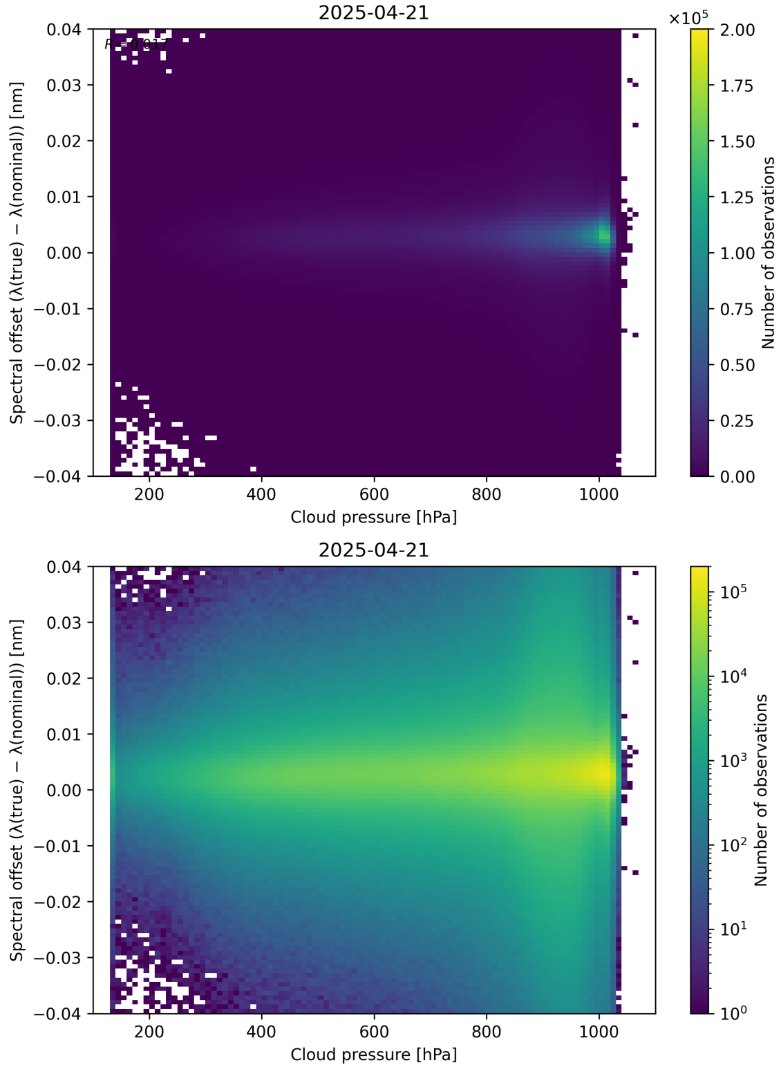
Figure 84: Scatter density plot of “Cloud pressure” against “Spectral offset ( \lambda_{\text{true}} - \lambda_{\text{nominal}} )” for 2025-04-20 to 2025-04-22.
