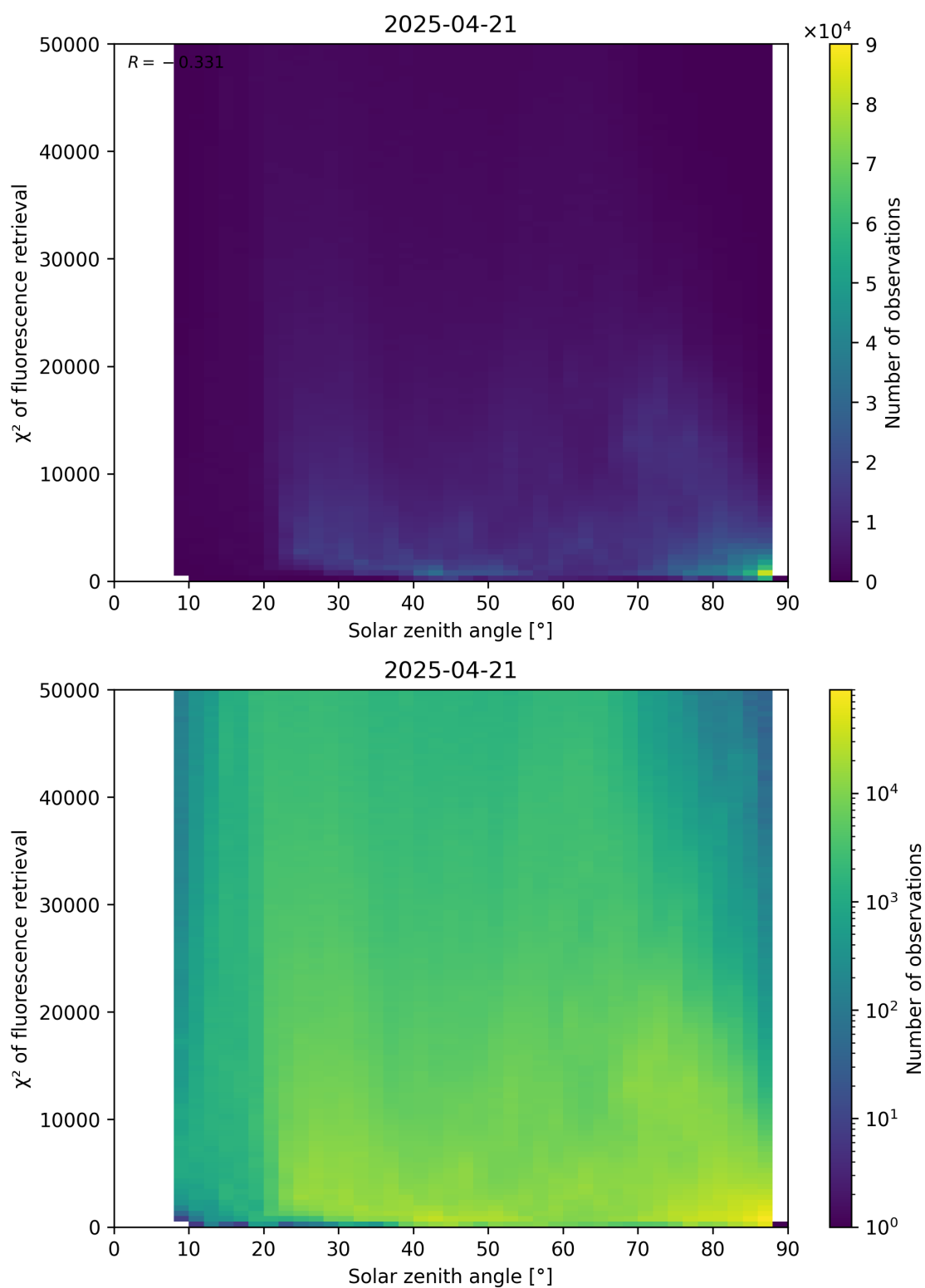
Figure 109: Scatter density plot of “Solar zenith angle” against “ \chi^2 of fluorescence retrieval” for 2025-04-20 to 2025-04-22.
