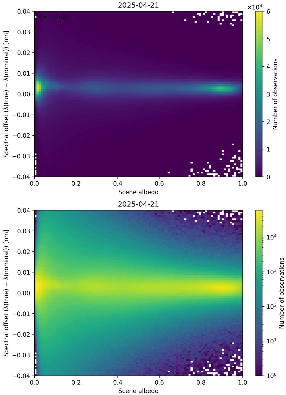
Figure 107: Scatter density plot of “Scene albedo” against “Spectral offset ( \lambda_{\text{true}} - \lambda_{\text{nominal}} )” for 2025-04-20 to 2025-04-22.
