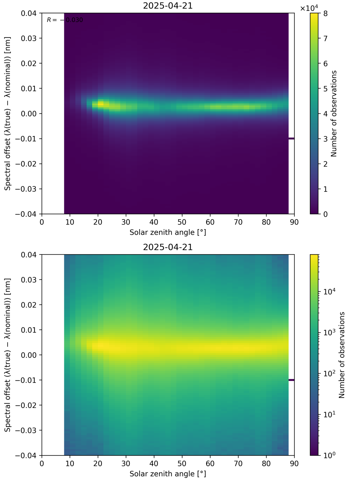
Figure 117: Scatter density plot of “Solar zenith angle” against “Spectral offset ( \lambda_{\text{true}} - \lambda_{\text{nominal}} )” for 2025-04-20 to 2025-04-22.
