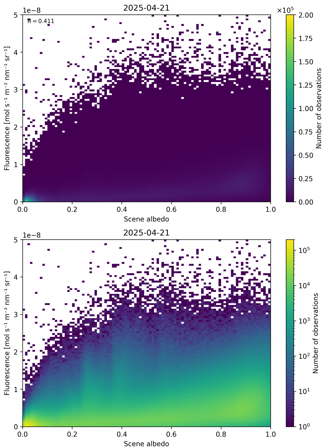
Figure 104: Scatter density plot of “Scene albedo” against “Fluorescence” for 2025-04-20 to 2025-04-22.
