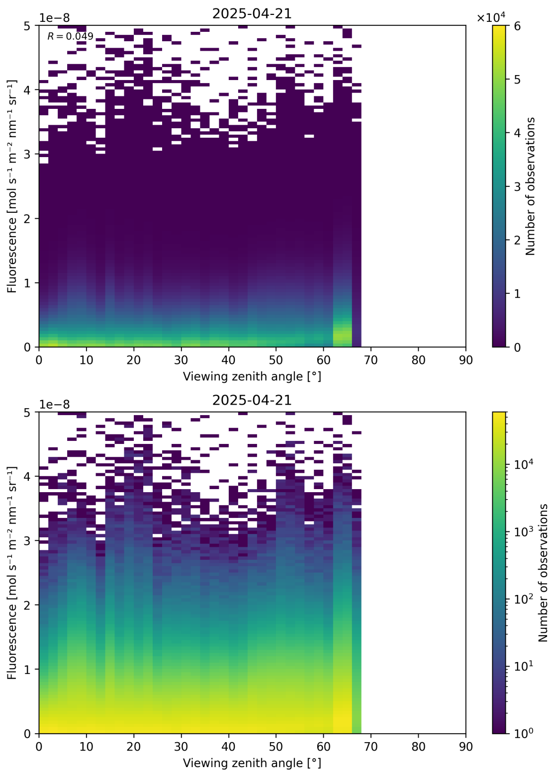
Figure 122: Scatter density plot of “Viewing zenith angle” against “Fluorescence” for 2025-04-20 to 2025-04-22.
