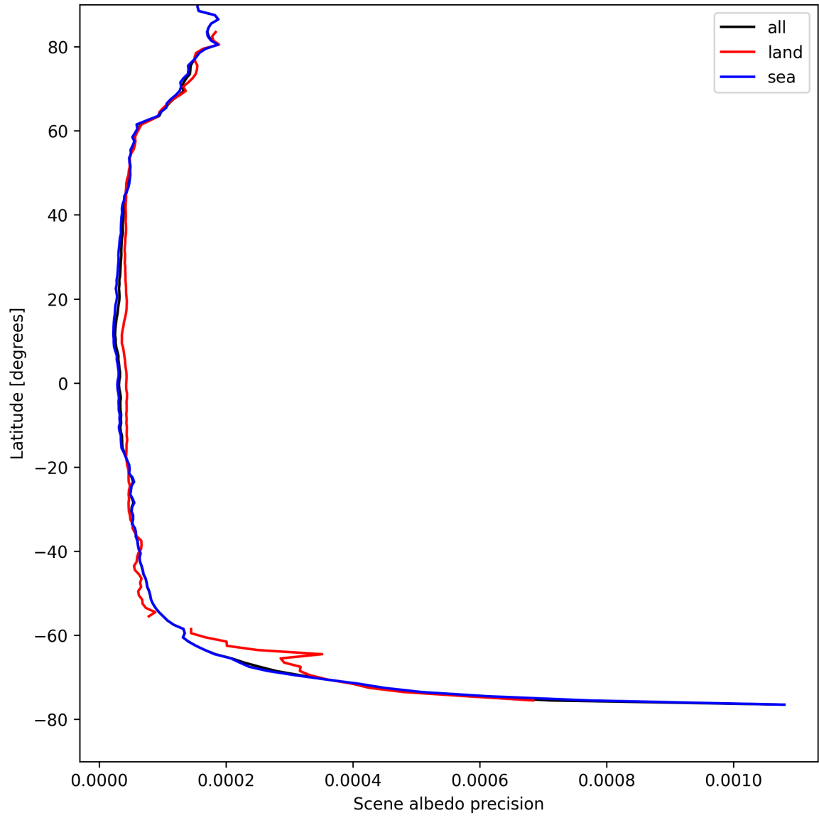
Figure 18: Zonal average of “Scene albedo precision” for 2025-04-20 to 2025-04-22.
