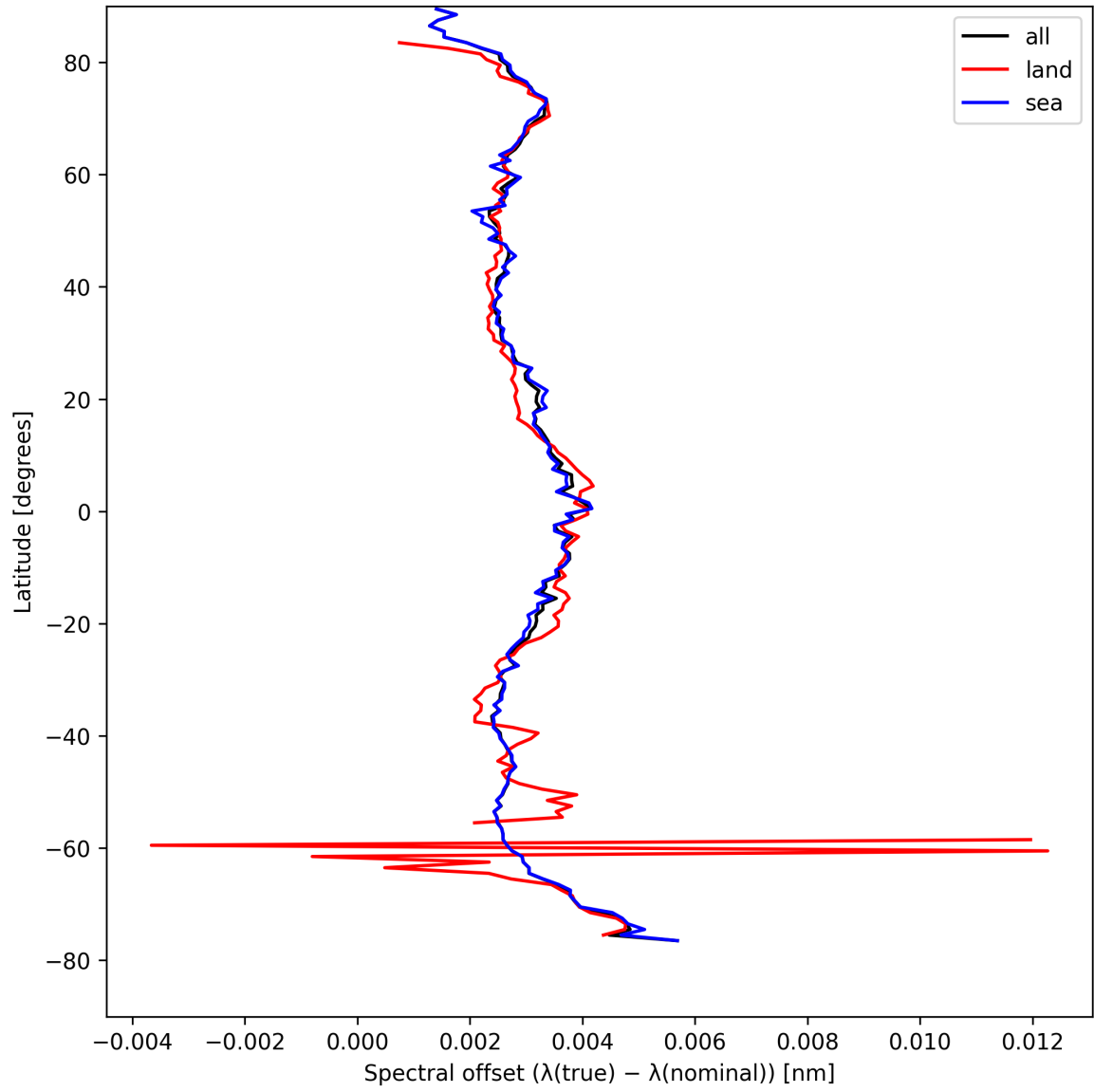
Figure 28: Zonal average of “Spectral offset ( \lambda_{\text{true}} - \lambda_{\text{nominal}} )” for 2025-04-20 to 2025-04-22.
