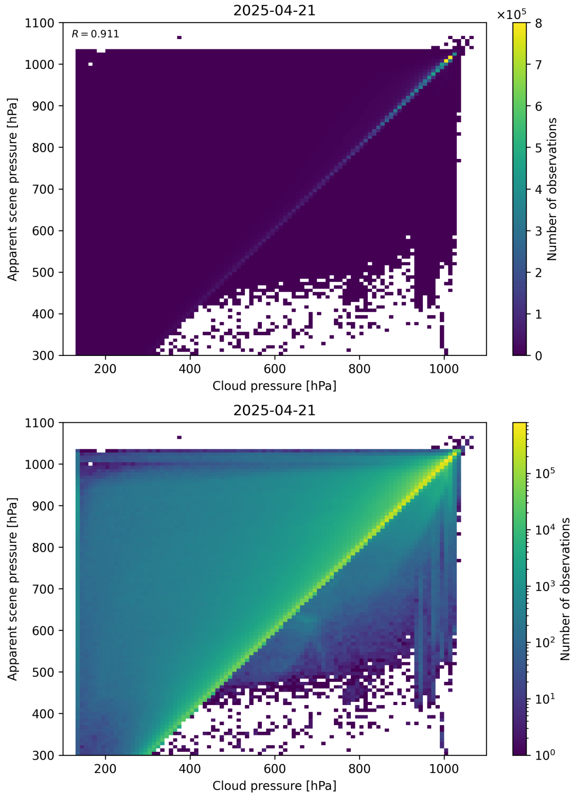
Figure 77: Scatter density plot of “Cloud pressure” against “Apparent scene pressure” for 2025-04-20 to 2025-04-22.
