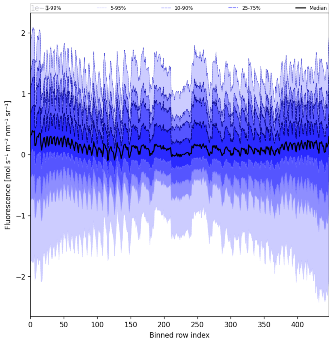
Figure 57: Along track statistics of “Fluorescence” for 2025-04-20 to 2025-04-22
