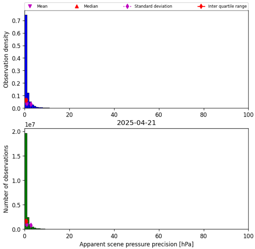
Figure 37: Histogram of “Apparent scene pressure precision” for 2025-04-20 to 2025-04-22
