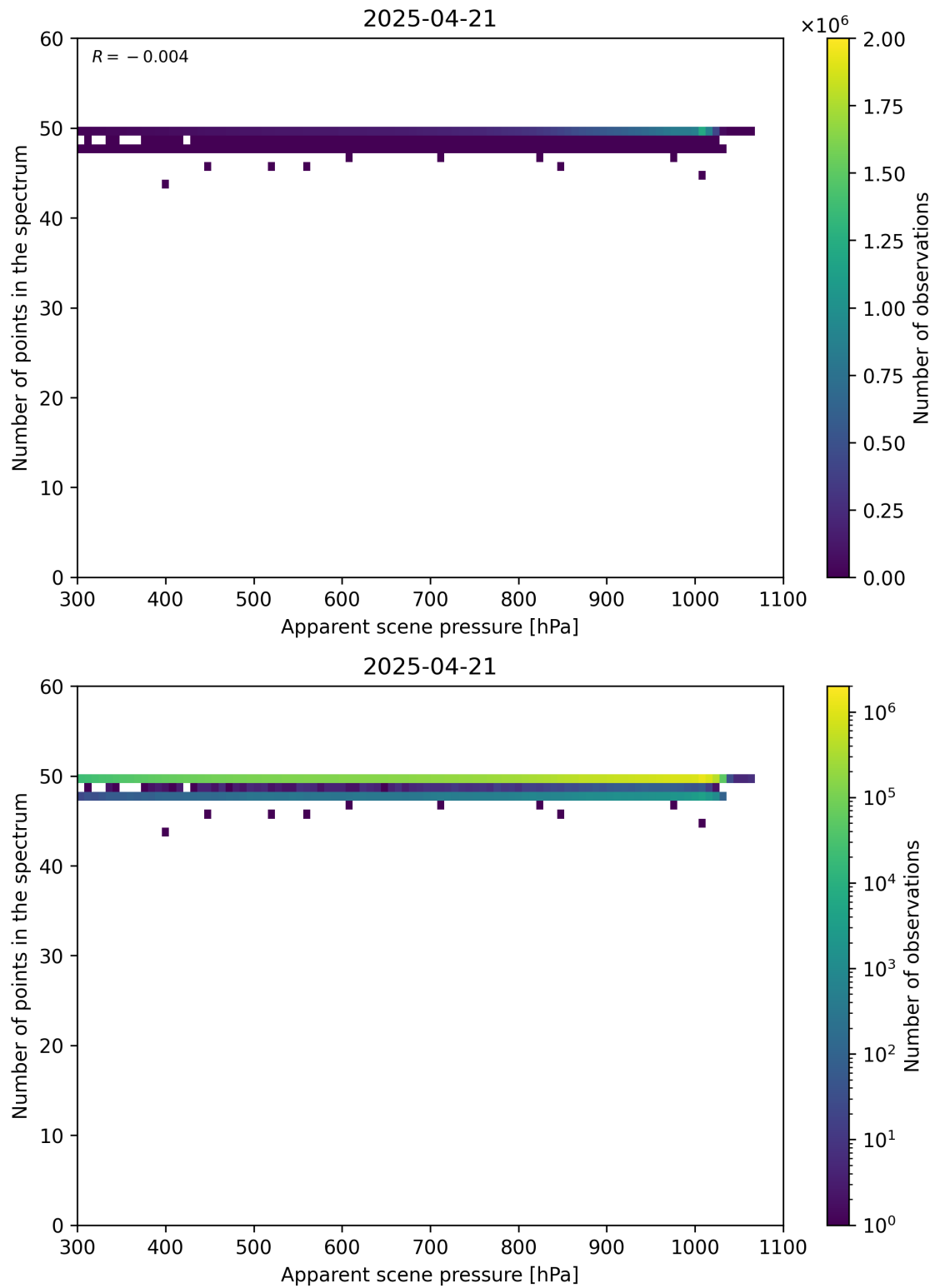
Figure 66: Scatter density plot of “Apparent scene pressure” against “Number of points in the spectrum” for 2025-04-20 to 2025-04-22.
