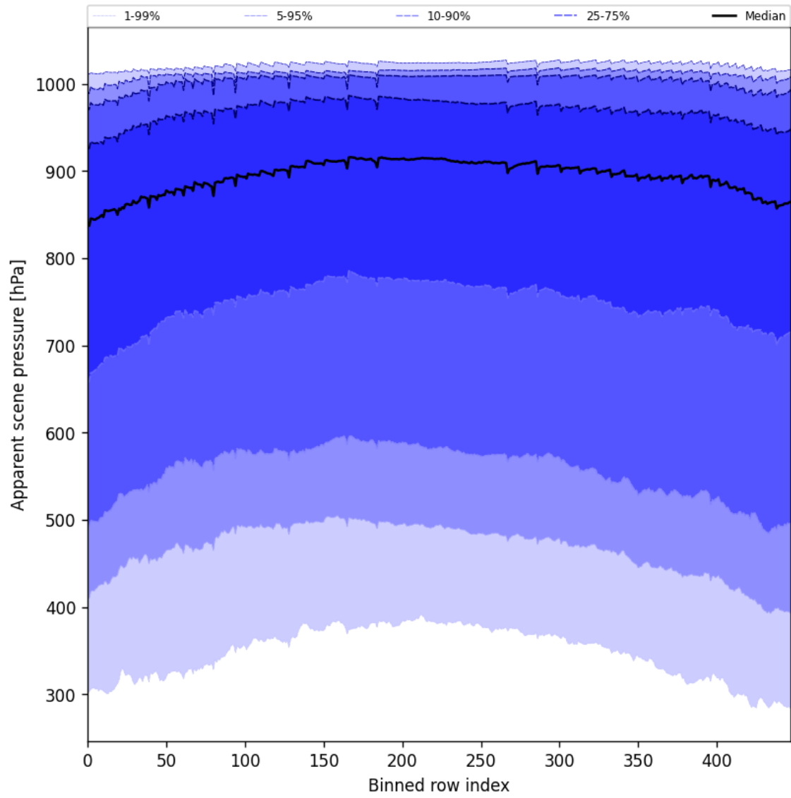
Figure 53: Along track statistics of “Apparent scene pressure” for 2025-04-20 to 2025-04-22
