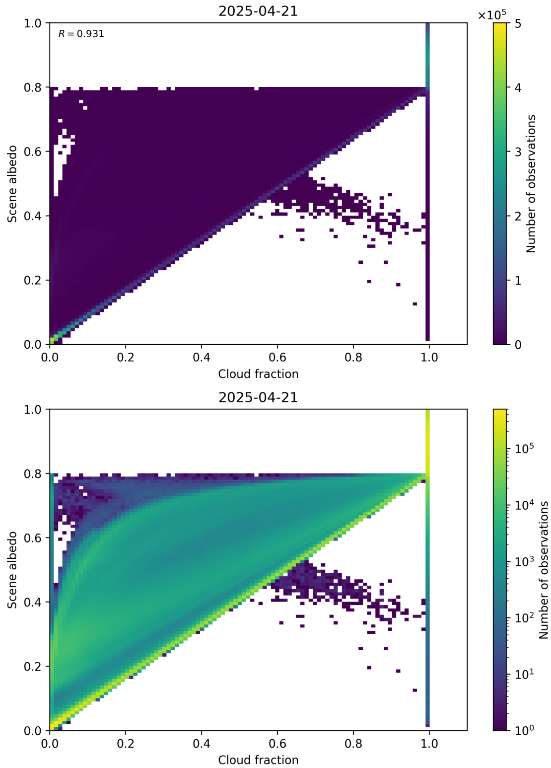
Figure 75: Scatter density plot of “Cloud fraction” against “Scene albedo” for 2025-04-20 to 2025-04-22.
