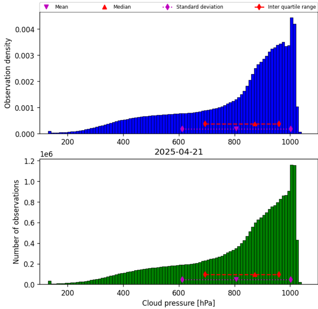
Figure 30: Histogram of “Cloud pressure” for 2025-04-20 to 2025-04-22
