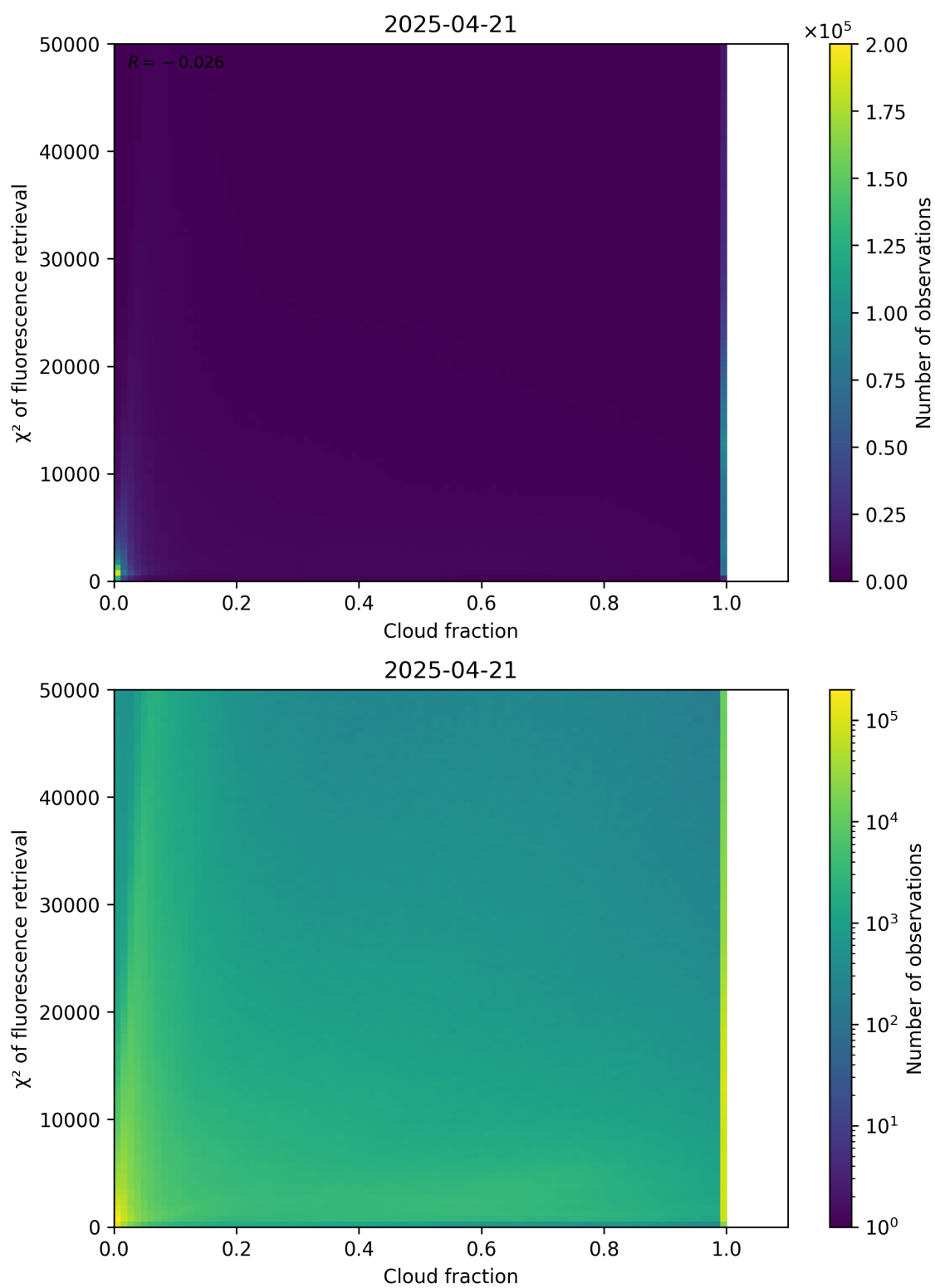
Figure 71: Scatter density plot of “Cloud fraction” against “ \chi^2 of fluorescence retrieval” for 2025-04-20 to 2025-04-22.
