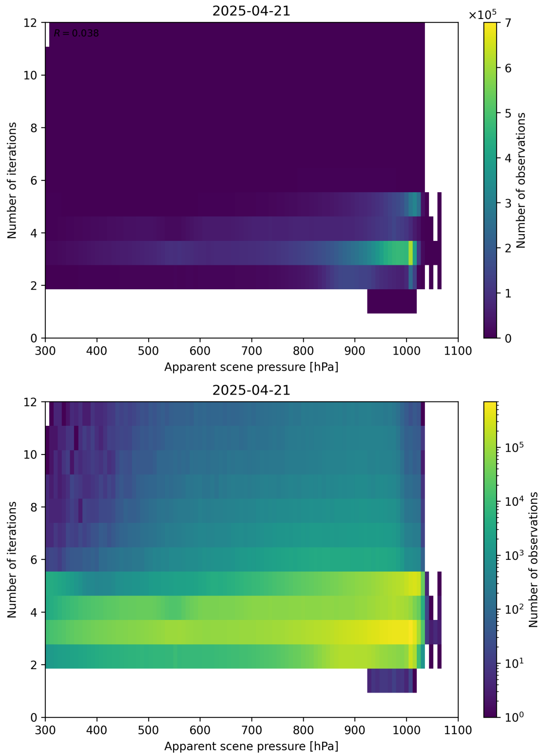
Figure 65: Scatter density plot of “Apparent scene pressure” against “Number of iterations” for 2025-04-20 to 2025-04-22.
