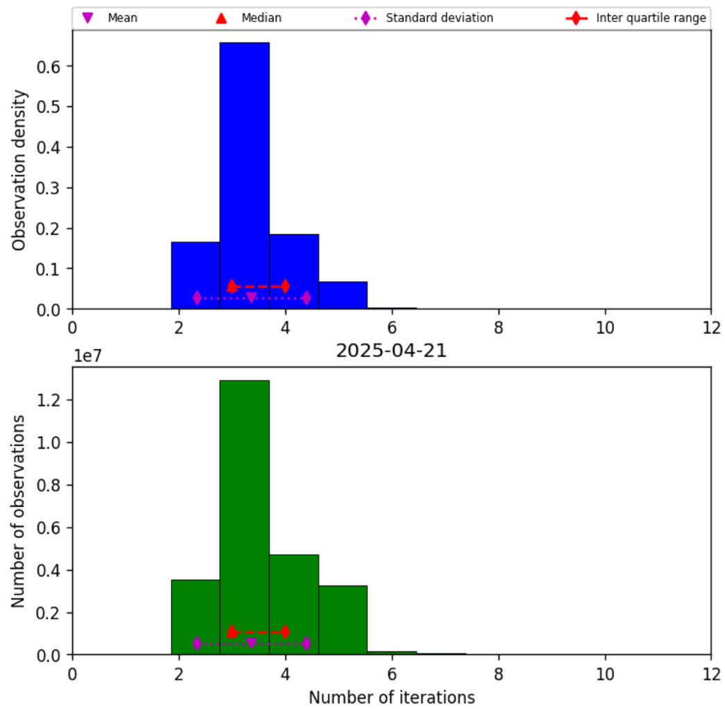
Figure 39: Histogram of “Number of iterations” for 2025-04-20 to 2025-04-22
