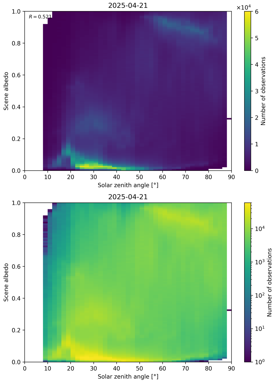
Figure 116: Scatter density plot of “Solar zenith angle” against “Scene albedo” for 2025-04-20 to 2025-04-22.
