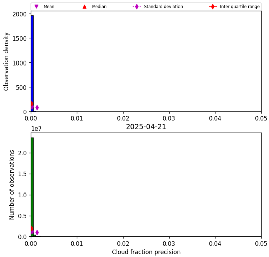
Figure 33: Histogram of “Cloud fraction precision” for 2025-04-20 to 2025-04-22
