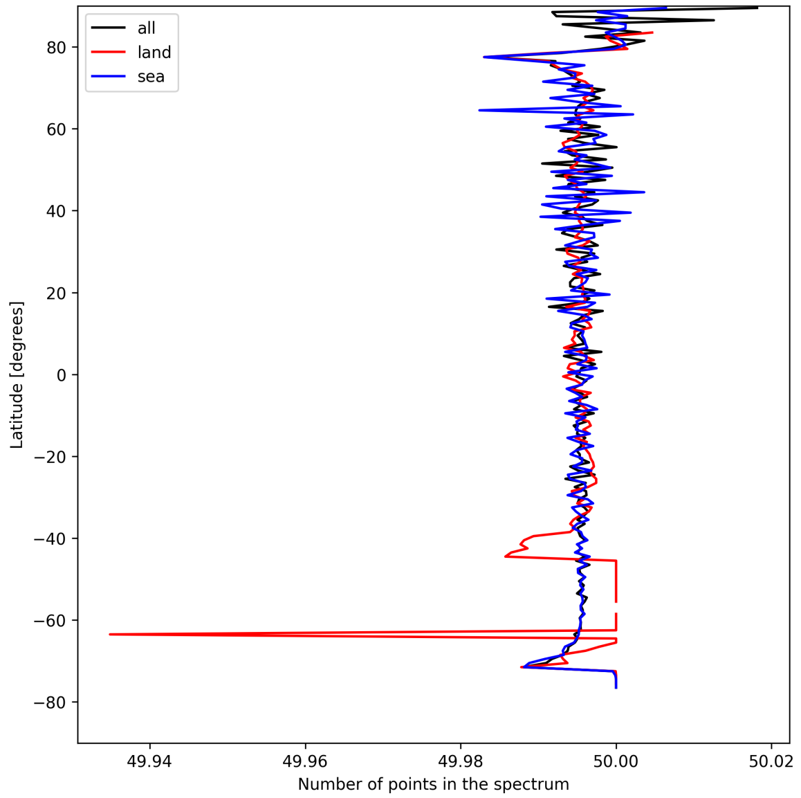
Figure 27: Zonal average of “Number of points in the spectrum” for 2025-04-20 to 2025-04-22.
