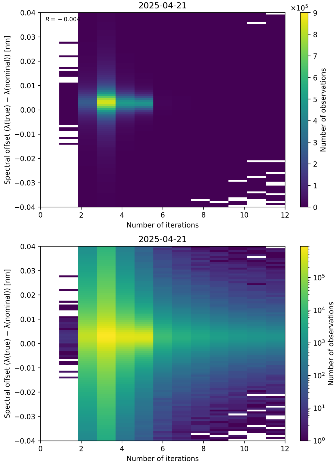
Figure 100: Scatter density plot of “Number of iterations” against “Spectral offset ( \lambda_{\text{true}} - \lambda_{\text{nominal}} )” for 2025-04-20 to 2025-04-22.
