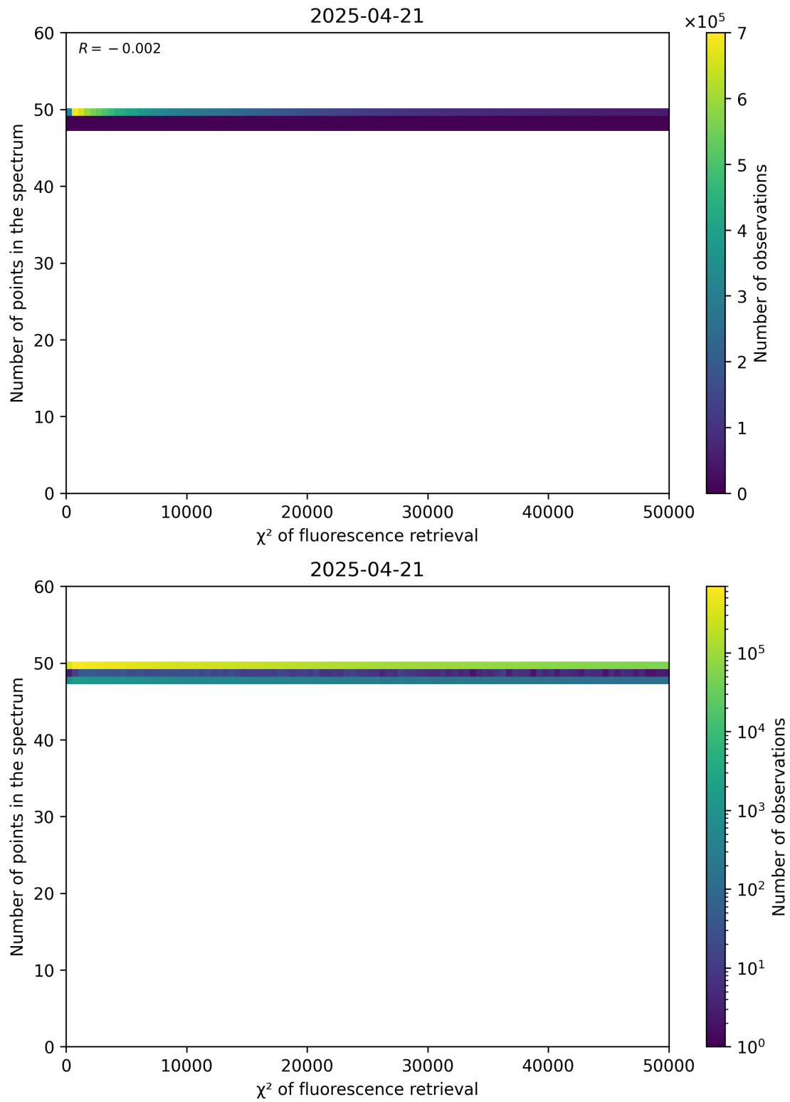
Figure 68: Scatter density plot of " \chi^2 of fluorescence retrieval" against "Number of points in the spectrum" for 2025-04-20 to 2025-04-22.
