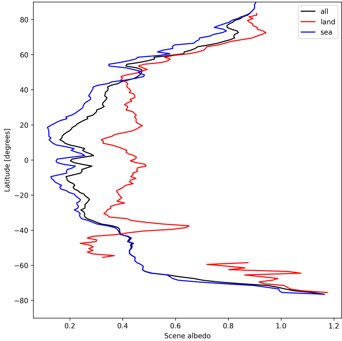
Figure 17: Zonal average of “Scene albedo” for 2025-04-20 to 2025-04-22.
