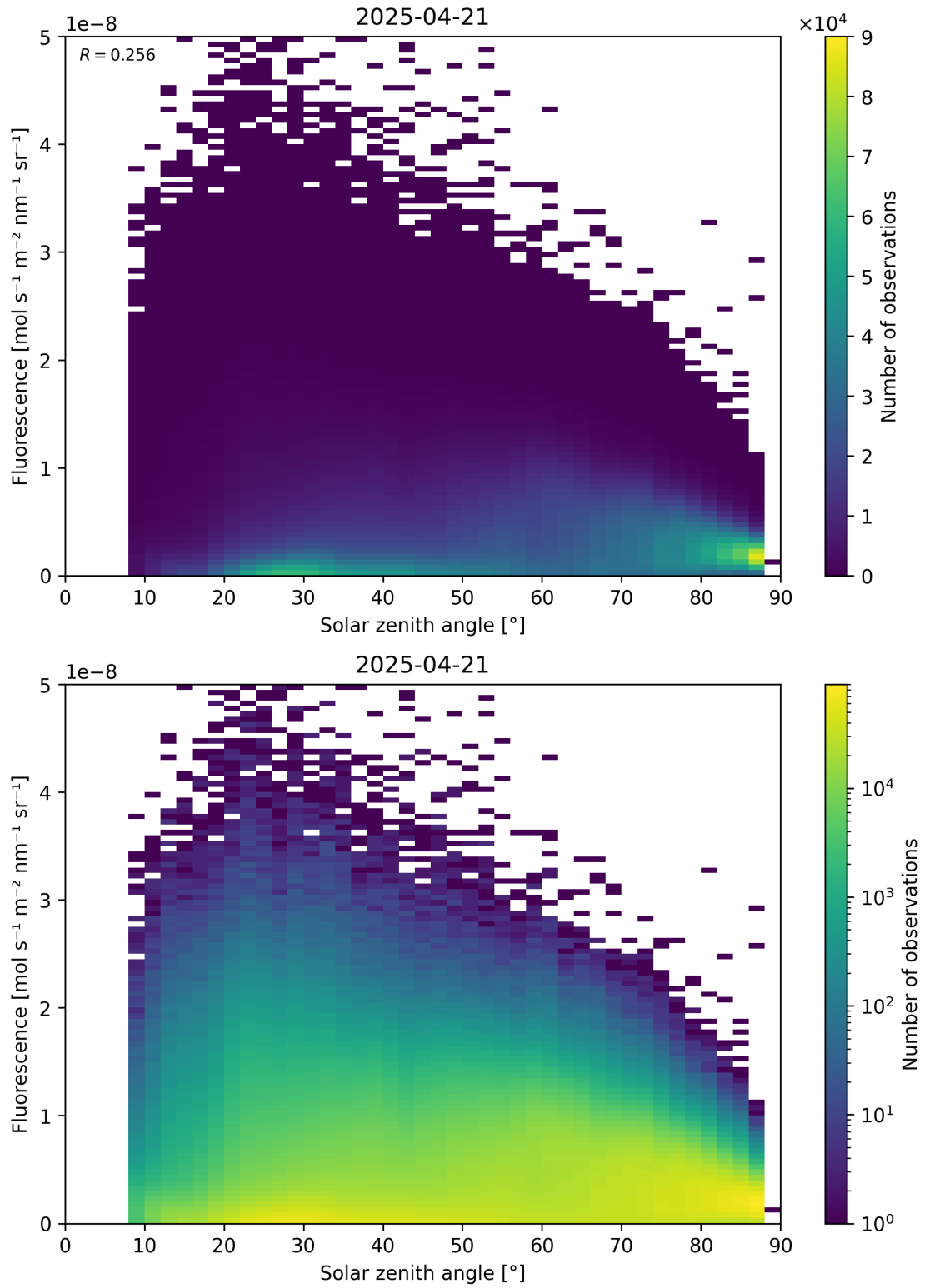
Figure 112: Scatter density plot of “Solar zenith angle” against “Fluorescence” for 2025-04-20 to 2025-04-22.
