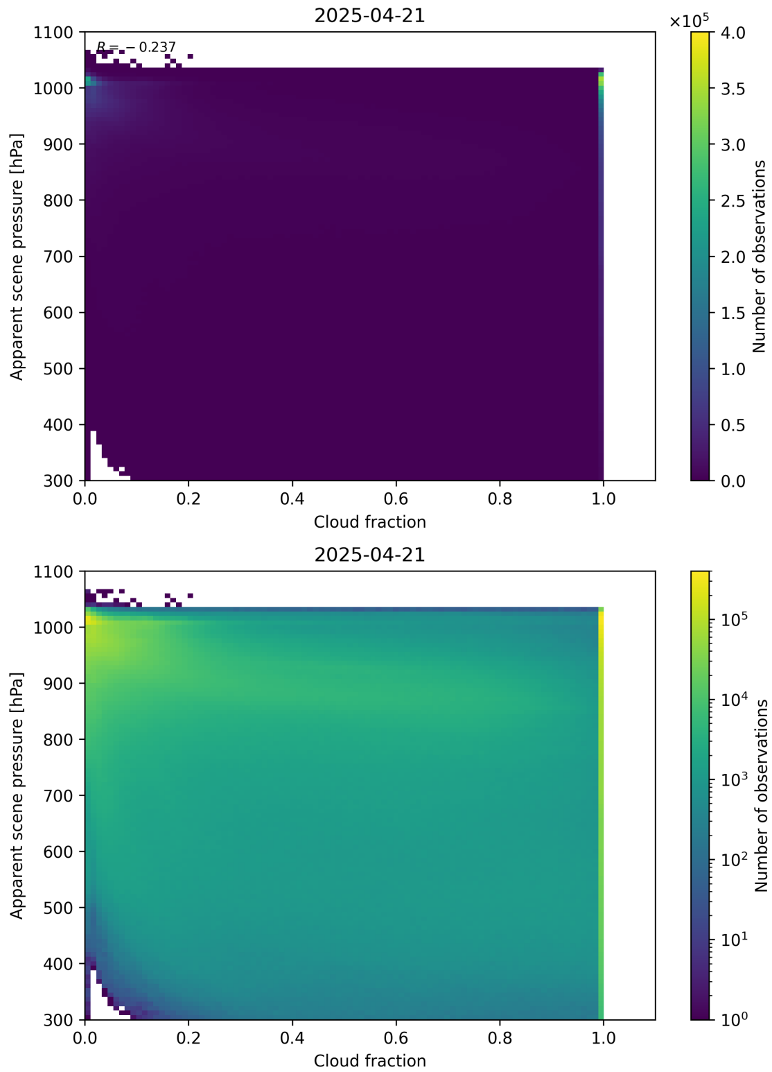
Figure 70: Scatter density plot of “Cloud fraction” against “Apparent scene pressure” for 2025-04-20 to 2025-04-22.
