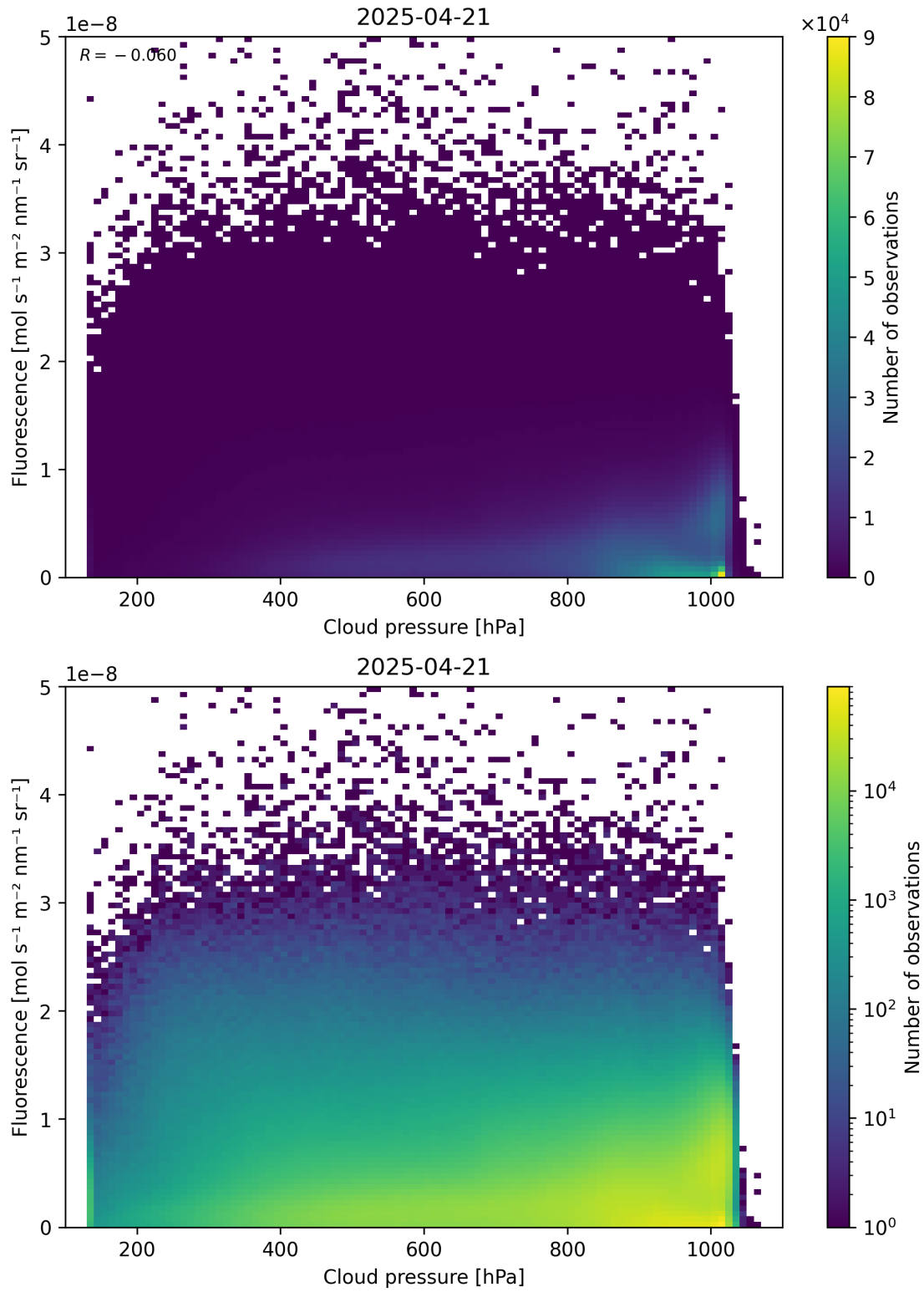
Figure 80: Scatter density plot of “Cloud pressure” against “Fluorescence” for 2025-04-20 to 2025-04-22.
