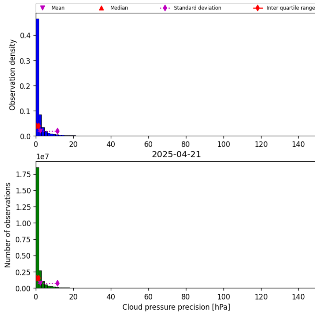
Figure 31: Histogram of “Cloud pressure precision” for 2025-04-20 to 2025-04-22
