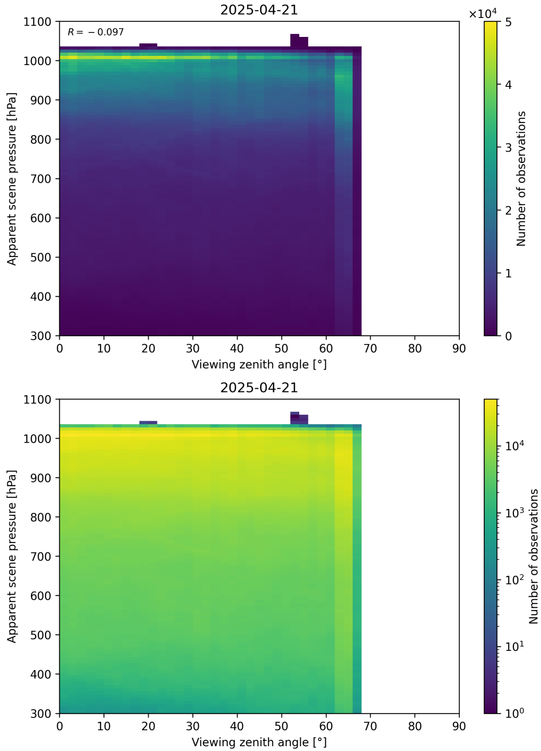
Figure 118: Scatter density plot of “Viewing zenith angle” against “Apparent scene pressure” for 2025-04-20 to 2025-04-22.
