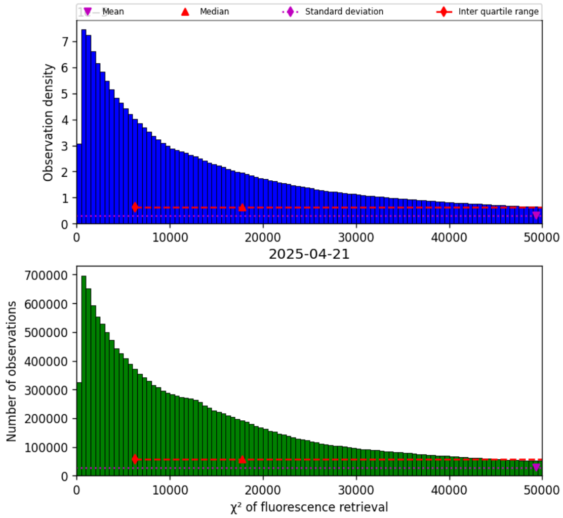
Figure 42: Histogram of “ \chi^2 of fluorescence retrieval” for 2025-04-20 to 2025-04-22
