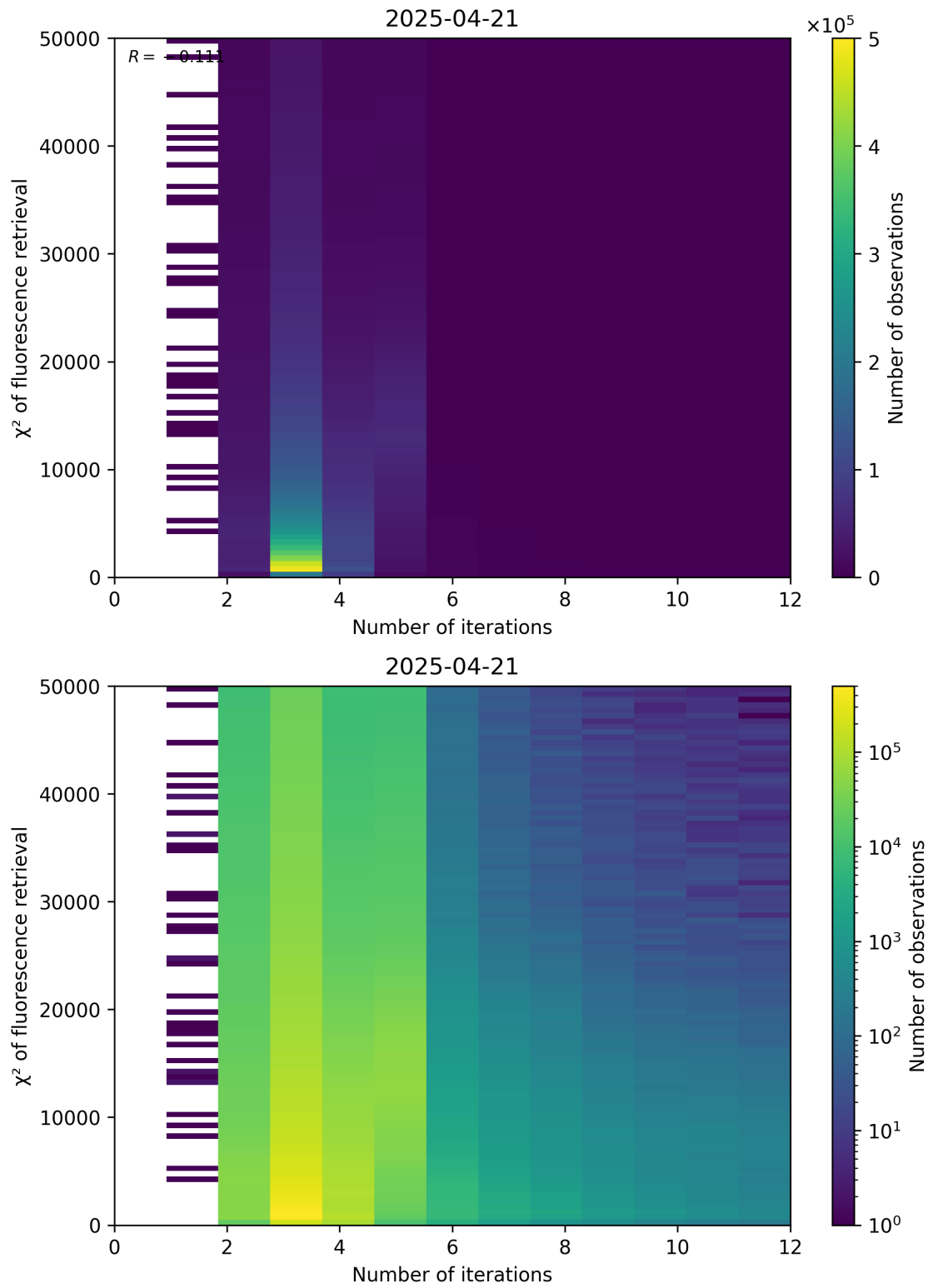
Figure 97: Scatter density plot of “Number of iterations” against “ \chi^2 of fluorescence retrieval” for 2025-04-20 to 2025-04-22.
