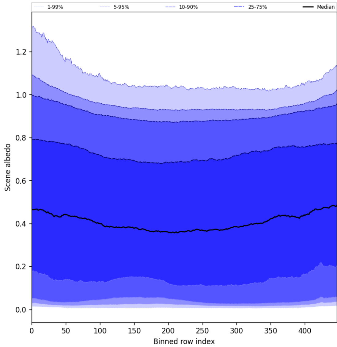
Figure 51: Along track statistics of “Scene albedo” for 2025-04-20 to 2025-04-22
