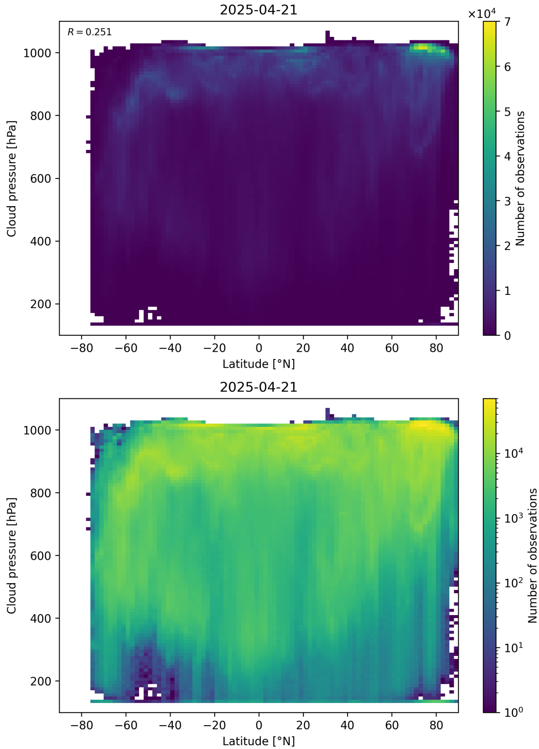
Figure 91: Scatter density plot of “Latitude” against “Cloud pressure” for 2025-04-20 to 2025-04-22.
