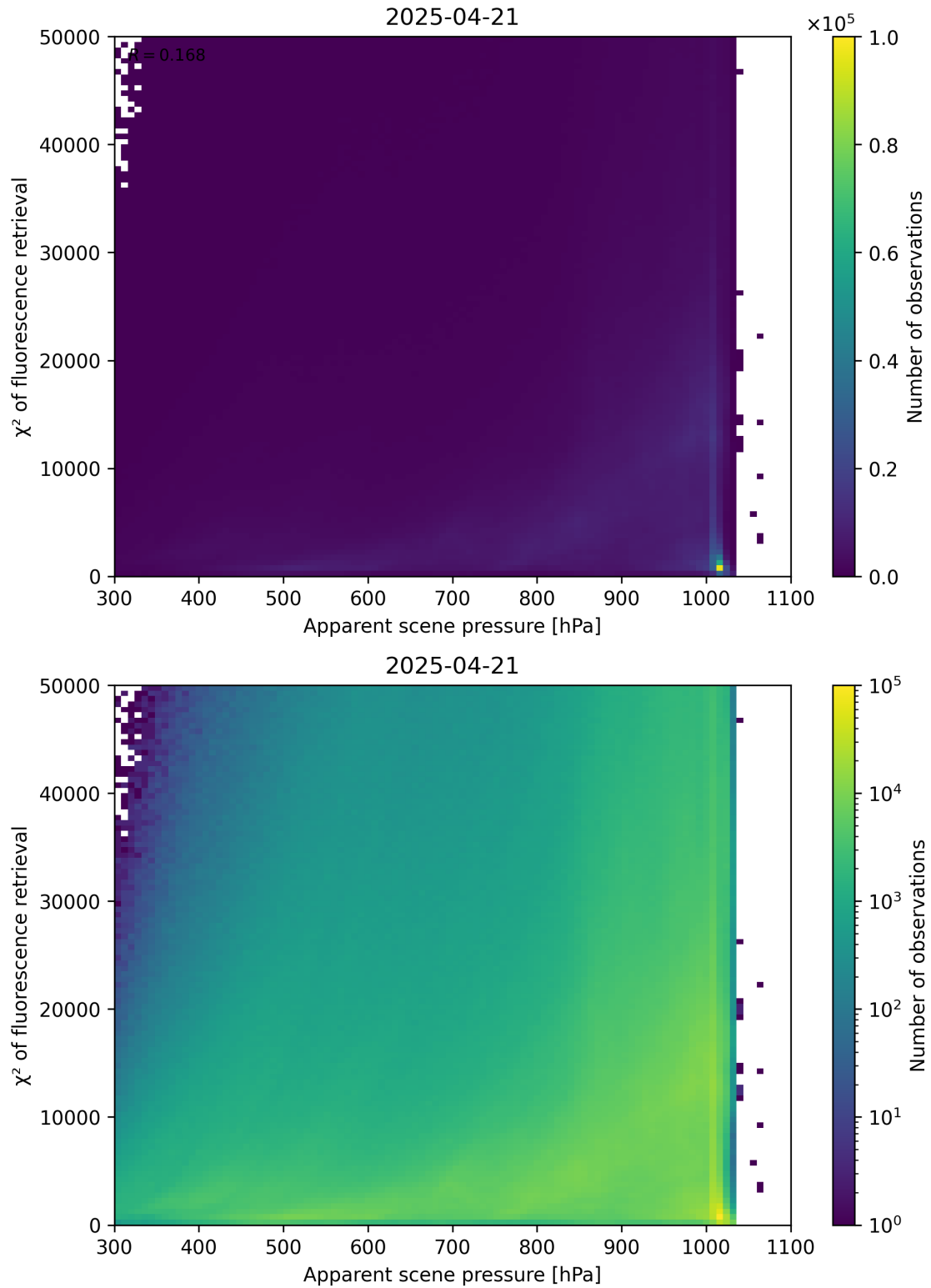
Figure 63: Scatter density plot of “Apparent scene pressure” against “ \chi^2 of fluorescence retrieval” for 2025-04-20 to 2025-04-22.
