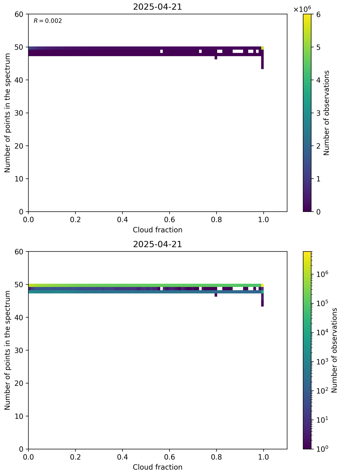
Figure 74: Scatter density plot of “Cloud fraction” against “Number of points in the spectrum” for 2025-04-20 to 2025-04-22.
