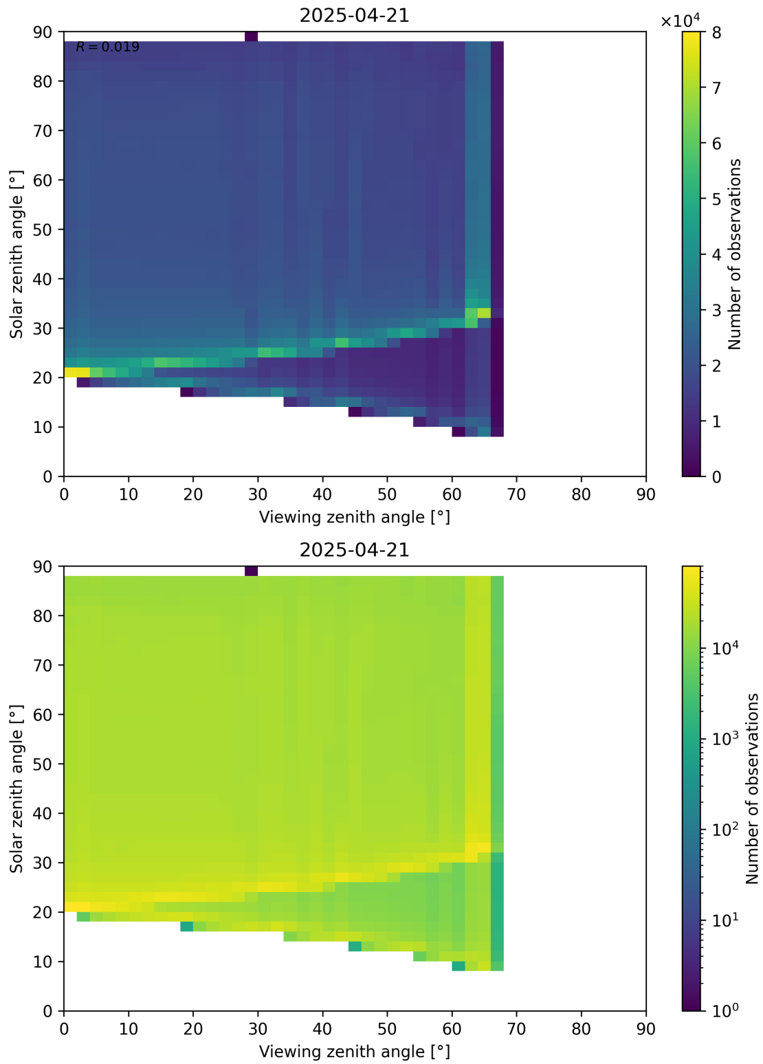
Figure 127: Scatter density plot of “Viewing zenith angle” against “Solar zenith angle” for 2025-04-20 to 2025-04-22.
