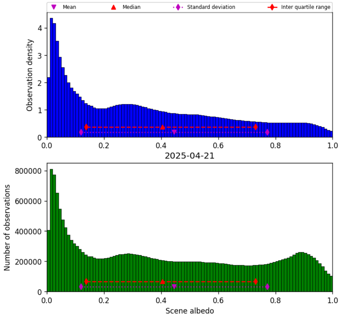
Figure 34: Histogram of “Scene albedo” for 2025-04-20 to 2025-04-22
