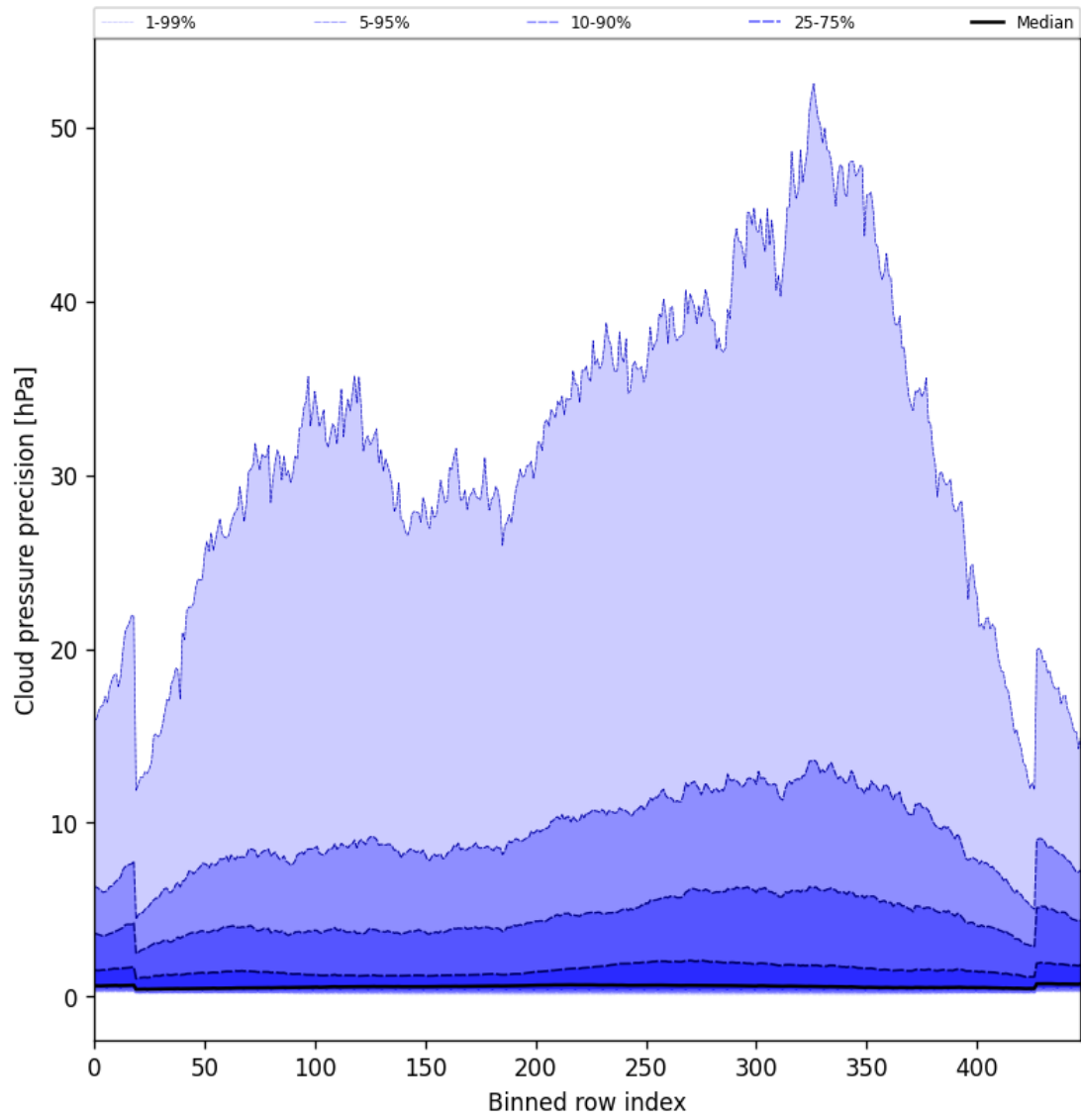
Figure 48: Along track statistics of “Cloud pressure precision” for 2025-04-20 to 2025-04-22
