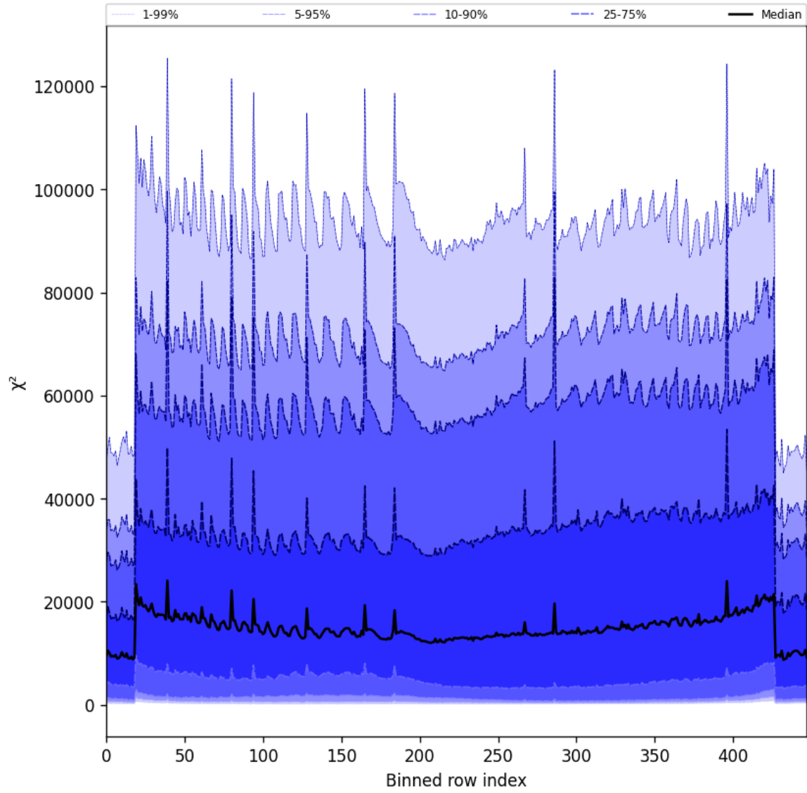
Figure 55: Along track statistics of “ \chi^2 ” for 2025-04-20 to 2025-04-22
