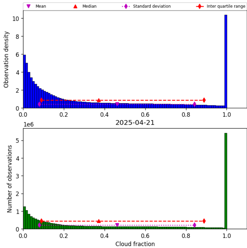
Figure 32: Histogram of “Cloud fraction” for 2025-04-20 to 2025-04-22
