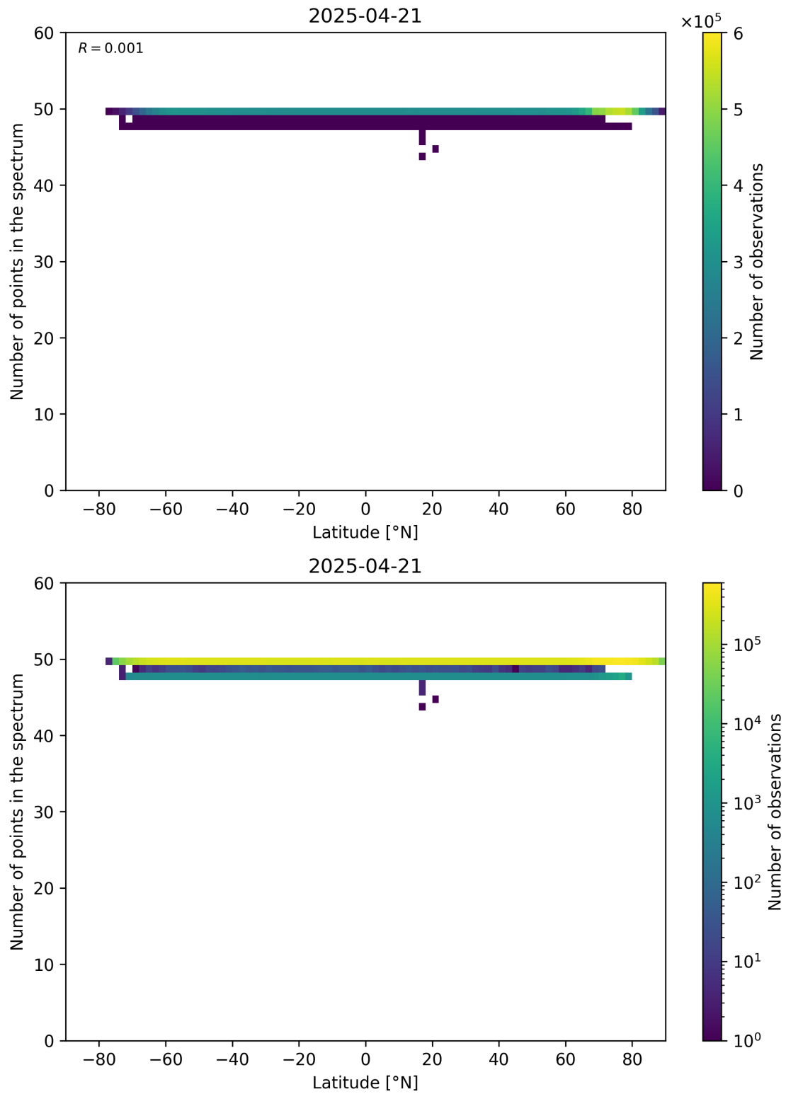
Figure 94: Scatter density plot of “Latitude” against “Number of points in the spectrum” for 2025-04-20 to 2025-04-22.
