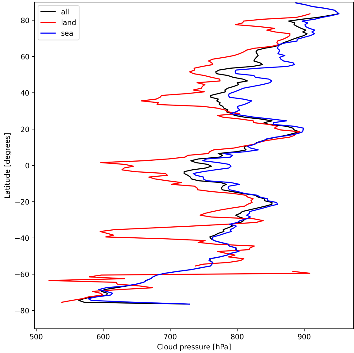
Figure 13: Zonal average of “Cloud pressure” for 2025-04-20 to 2025-04-22.
