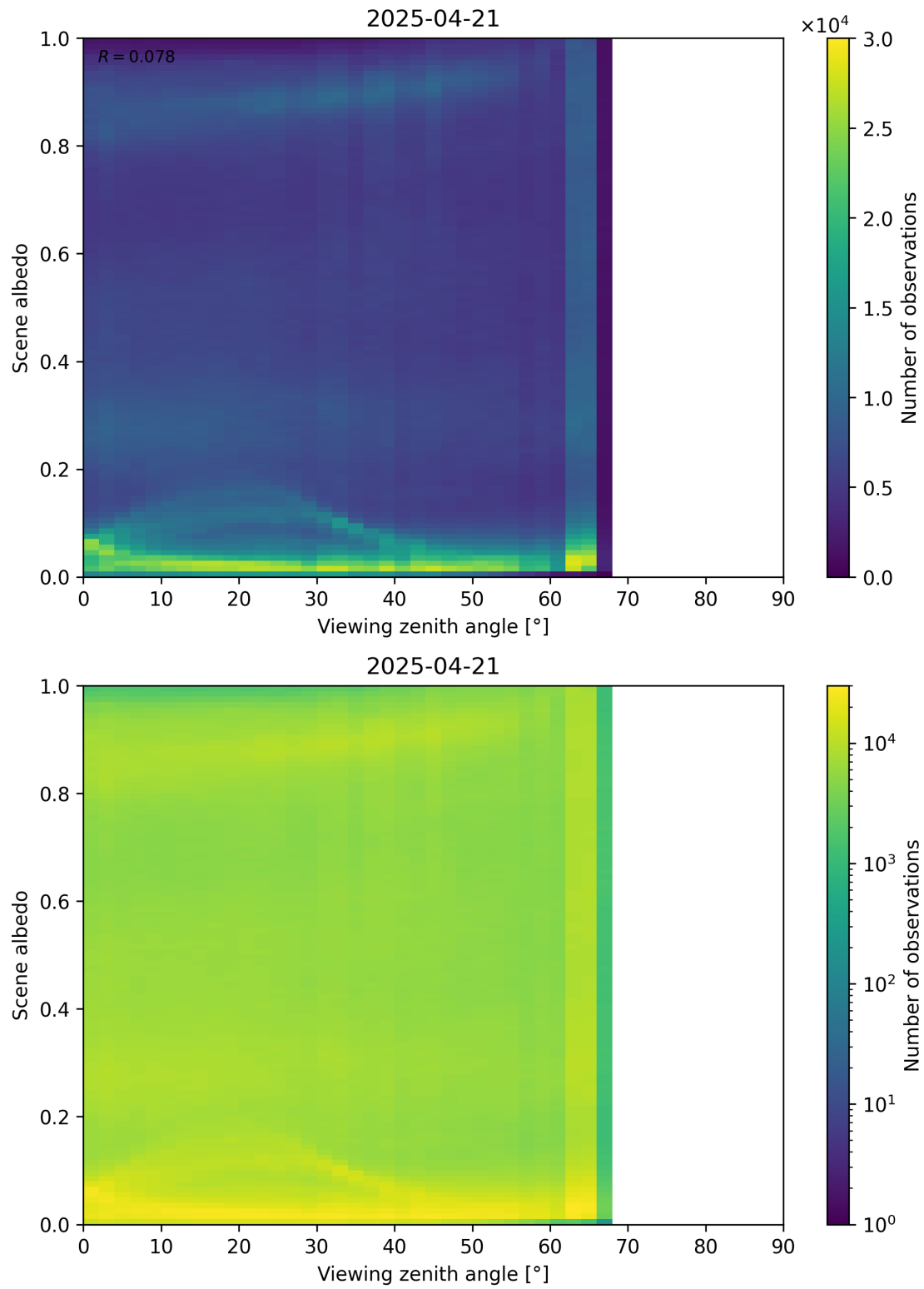
Figure 126: Scatter density plot of “Viewing zenith angle” against “Scene albedo” for 2025-04-20 to 2025-04-22.
