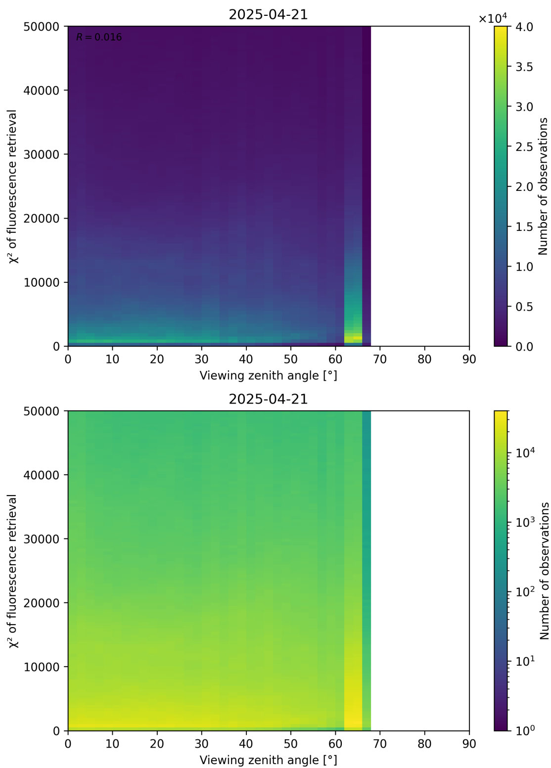
Figure 119: Scatter density plot of “Viewing zenith angle” against “ \chi^2 of fluorescence retrieval” for 2025-04-20 to 2025-04-22.
