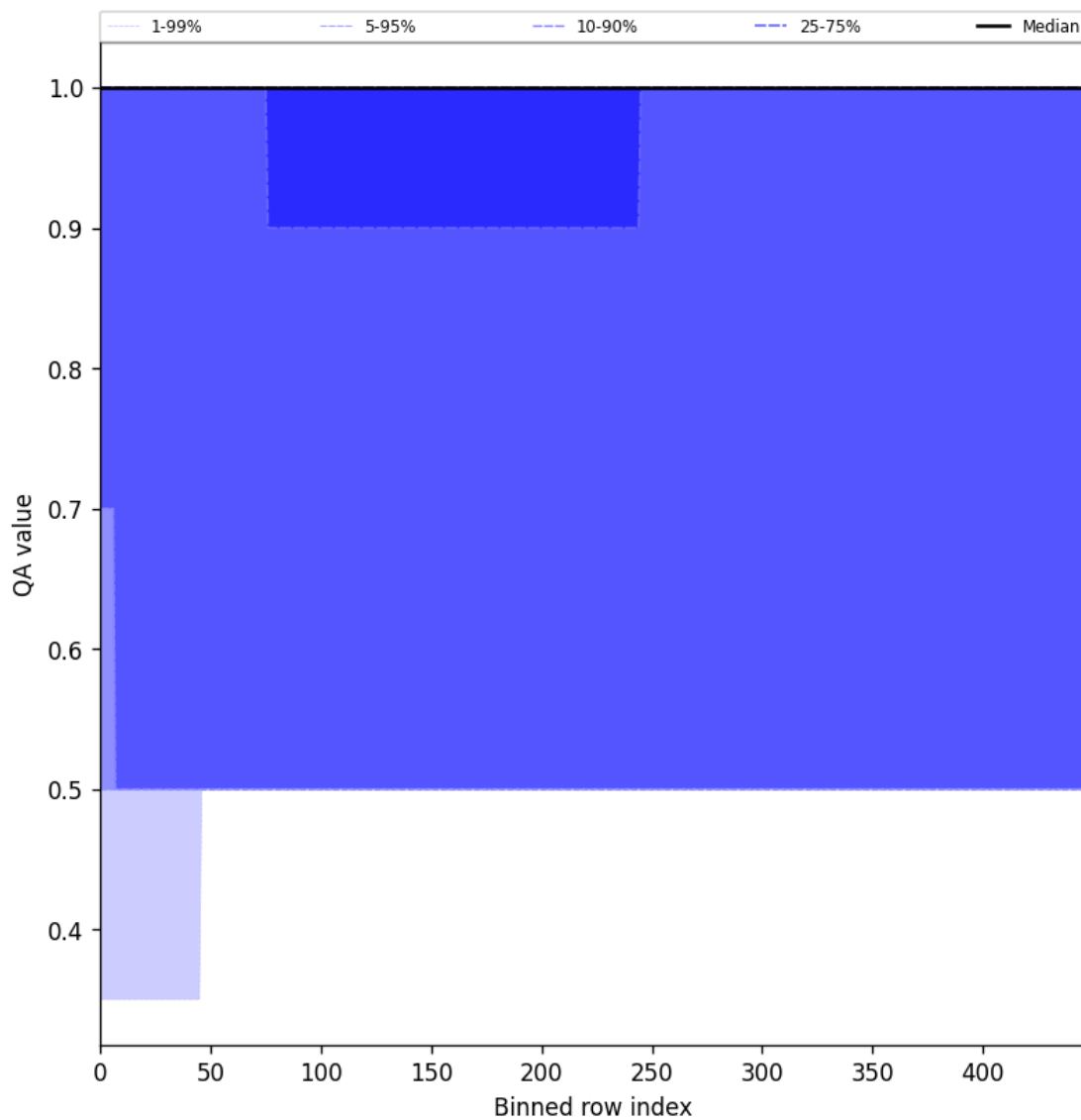
Figure 46: Along track statistics of “QA value” for 2025-04-20 to 2025-04-22
