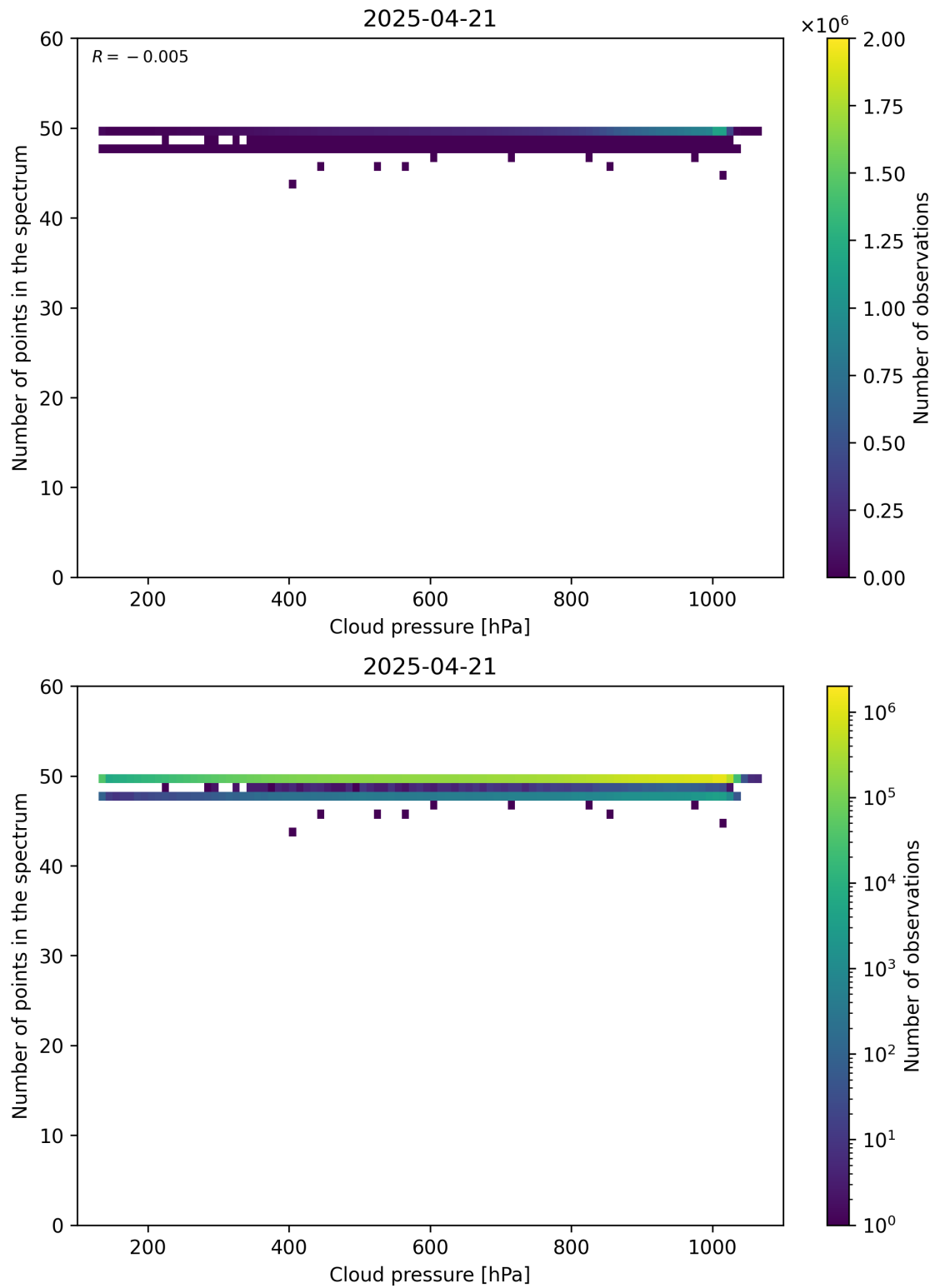
Figure 82: Scatter density plot of “Cloud pressure” against “Number of points in the spectrum” for 2025-04-20 to 2025-04-22.
