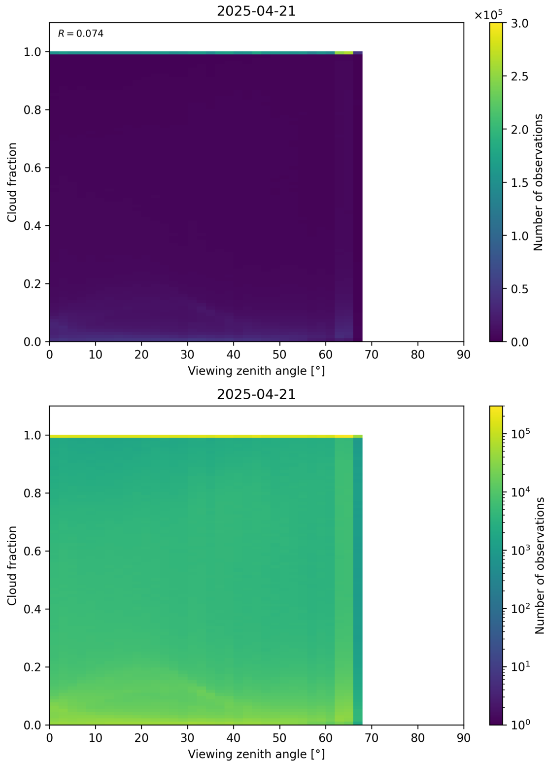
Figure 120: Scatter density plot of “Viewing zenith angle” against “Cloud fraction” for 2025-04-20 to 2025-04-22.
