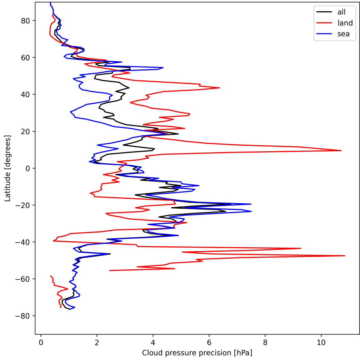
Figure 14: Zonal average of "Cloud pressure precision" for 2025-04-20 to 2025-04-22.
