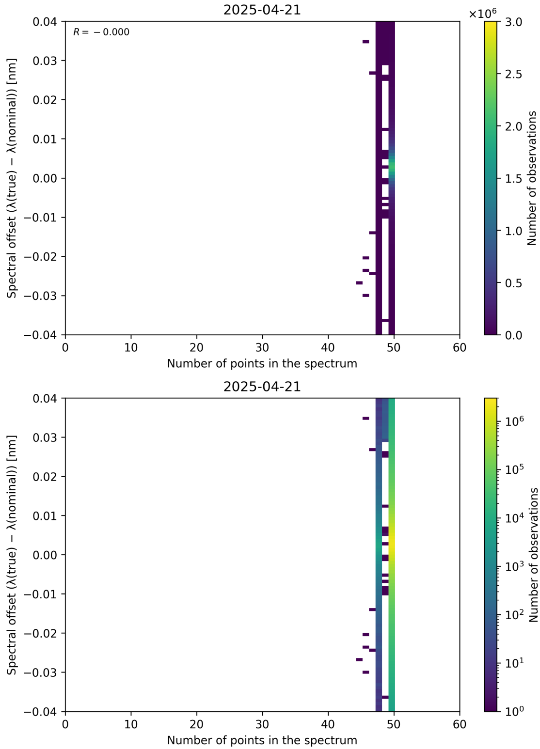
Figure 101: Scatter density plot of “Number of points in the spectrum” against “Spectral offset ( \lambda_{\text{true}} - \lambda_{\text{nominal}} )” for 2025-04-20 to 2025-04-22.
