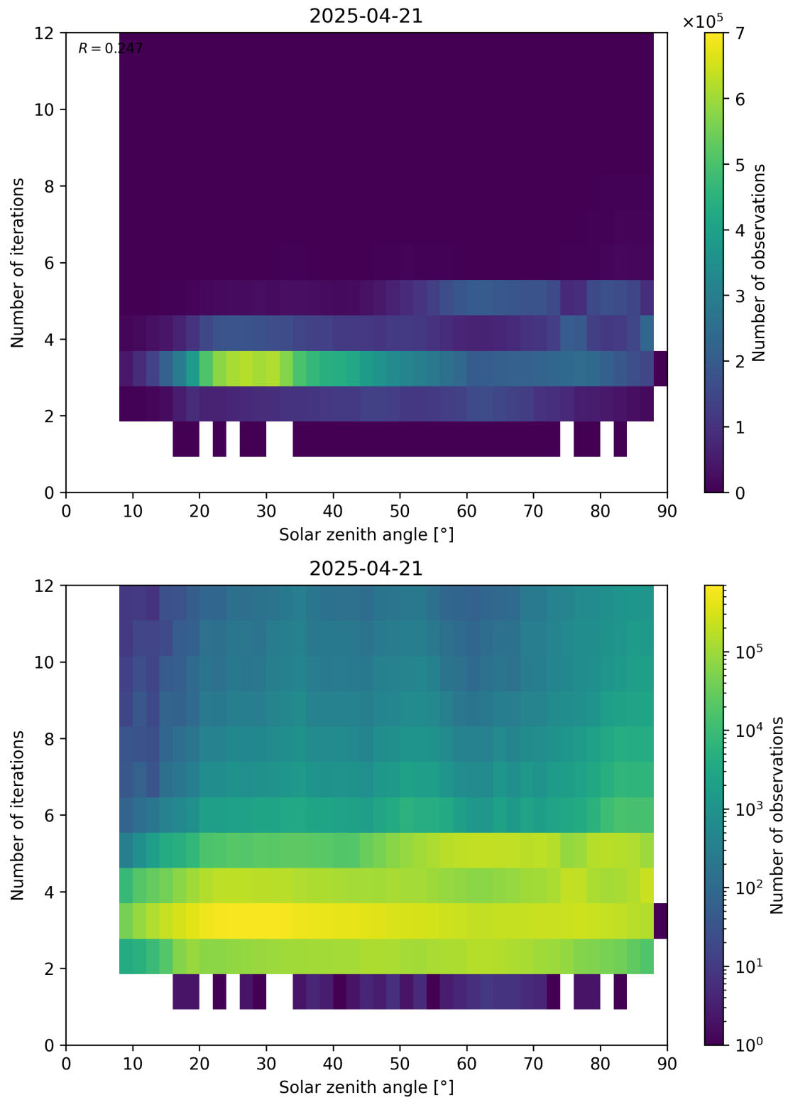
Figure 114: Scatter density plot of “Solar zenith angle” against “Number of iterations” for 2025-04-20 to 2025-04-22.
