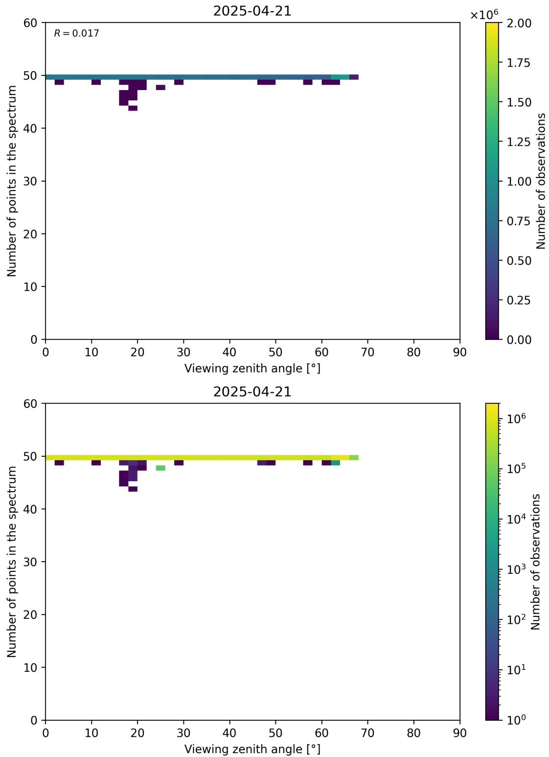
Figure 125: Scatter density plot of “Viewing zenith angle” against “Number of points in the spectrum” for 2025-04-20 to 2025-04-22.
