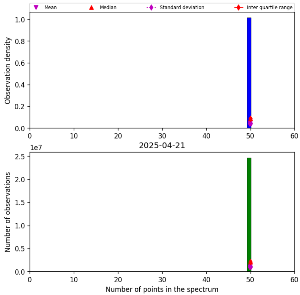
Figure 44: Histogram of “Number of points in the spectrum” for 2025-04-20 to 2025-04-22
