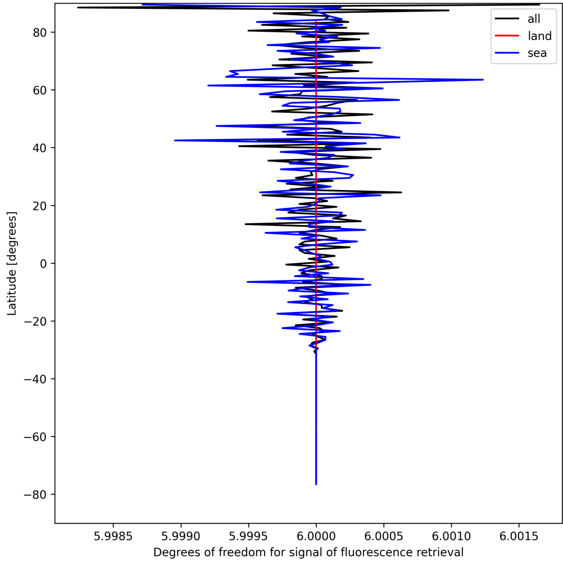
Figure 26: Zonal average of “Degrees of freedom for signal of fluorescence retrieval” for 2025-04-20 to 2025-04-22.
