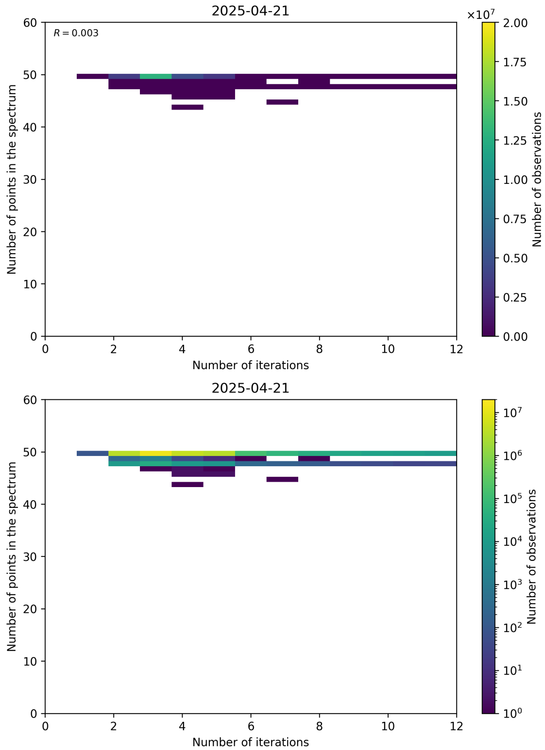
Figure 99: Scatter density plot of “Number of iterations” against “Number of points in the spectrum” for 2025-04-20 to 2025-04-22.
