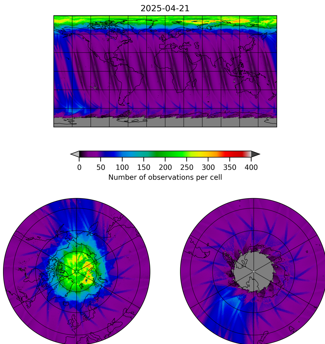
Figure 11: Map of the number of observations for 2025-04-20 to 2025-04-22
