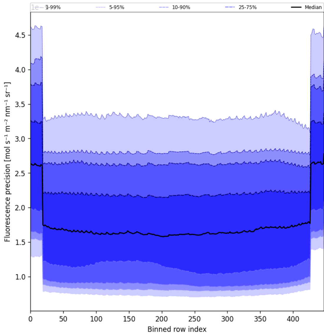
Figure 58: Along track statistics of “Fluorescence precision” for 2025-04-20 to 2025-04-22
