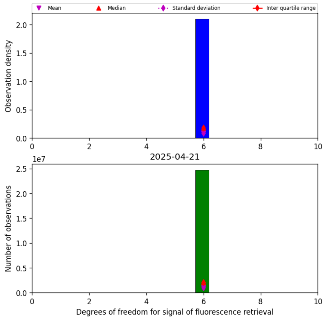
Figure 43: Histogram of "Degrees of freedom for signal of fluorescence retrieval" for 2025-04-20 to 2025-04-22
