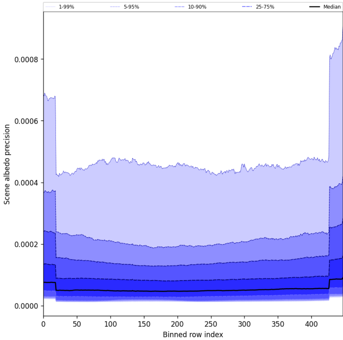
Figure 52: Along track statistics of “Scene albedo precision” for 2025-04-20 to 2025-04-22
