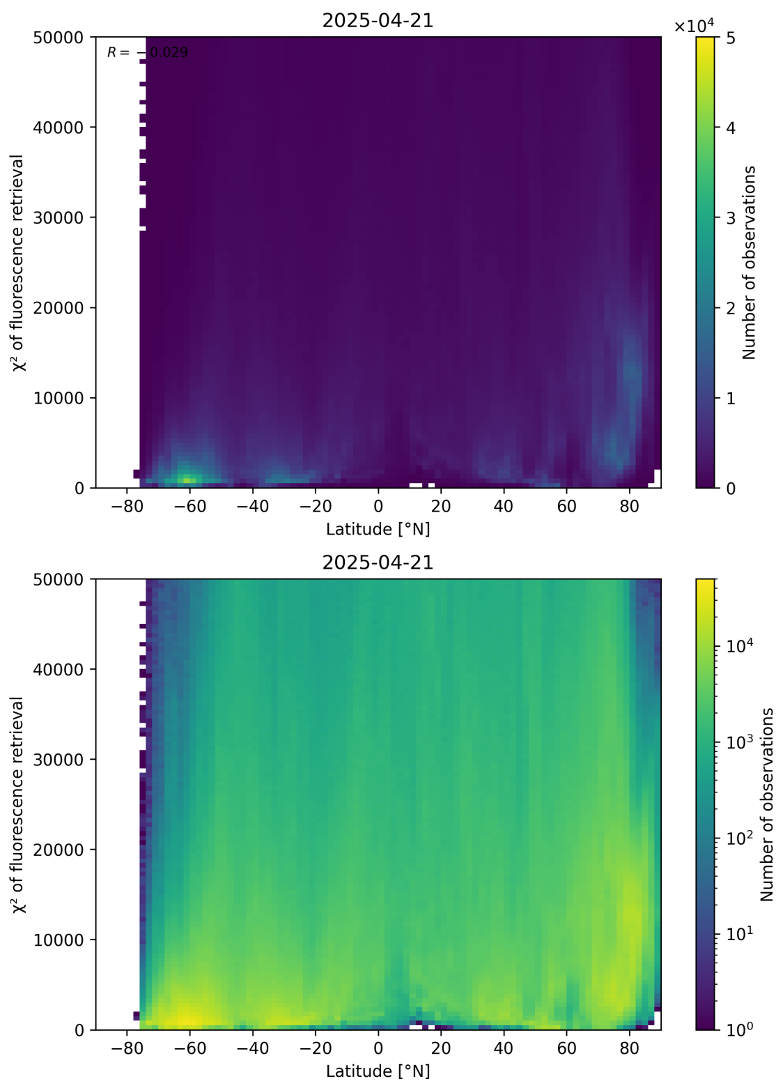
Figure 89: Scatter density plot of “Latitude” against “ \chi^2 of fluorescence retrieval” for 2025-04-20 to 2025-04-22.
