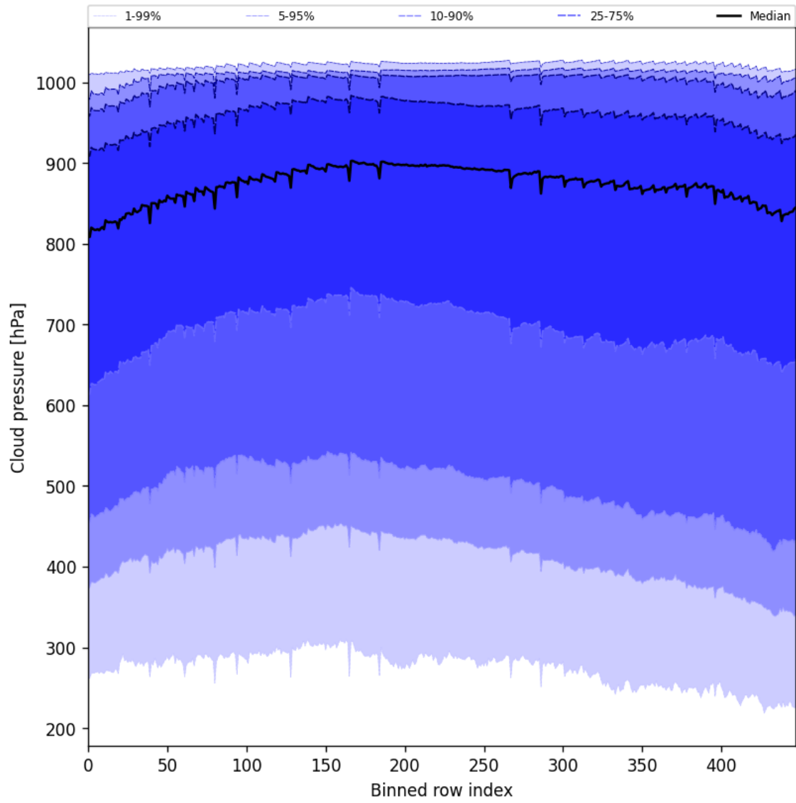
Figure 47: Along track statistics of “Cloud pressure” for 2025-04-20 to 2025-04-22
