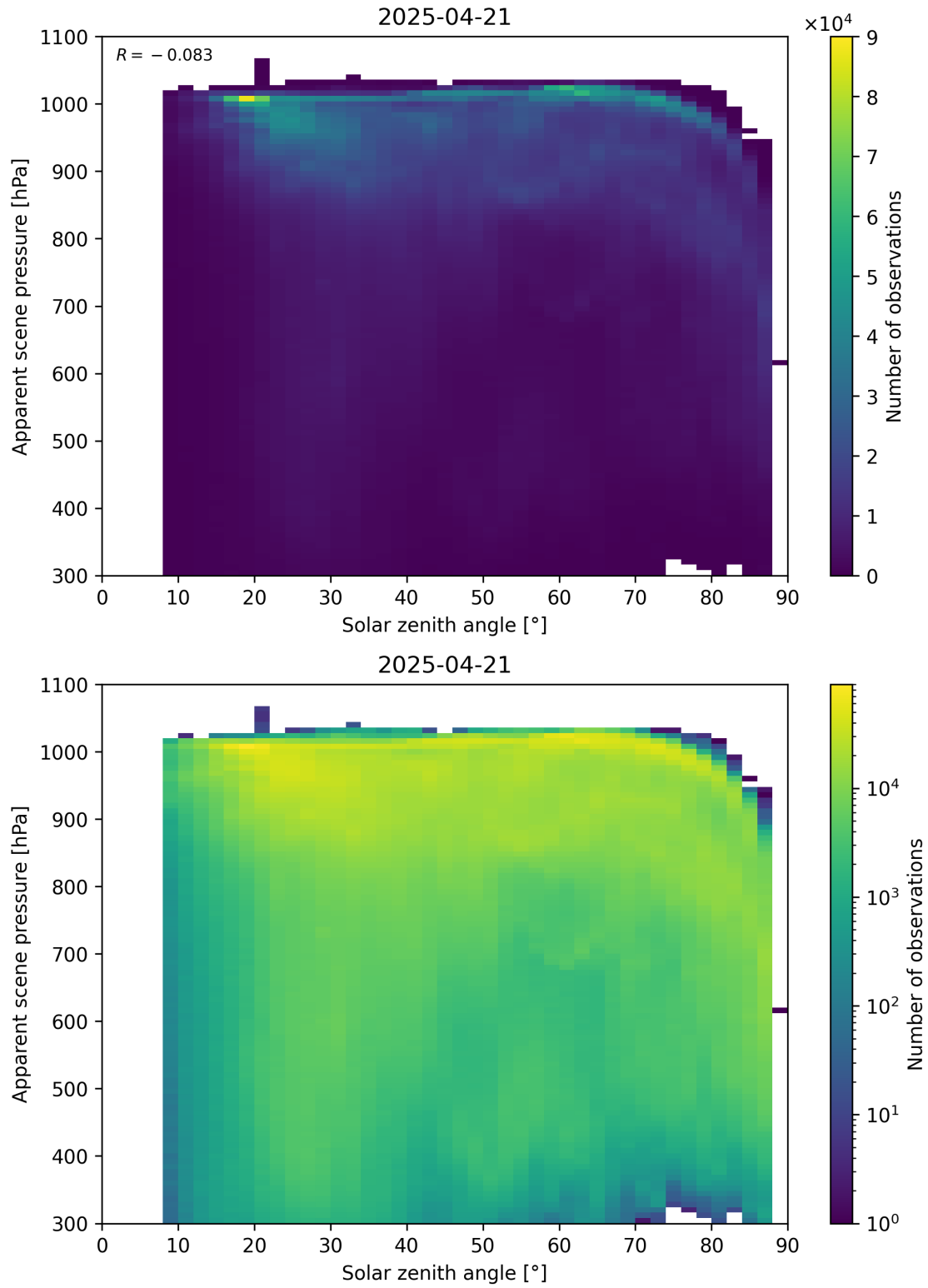
Figure 108: Scatter density plot of “Solar zenith angle” against “Apparent scene pressure” for 2025-04-20 to 2025-04-22.
