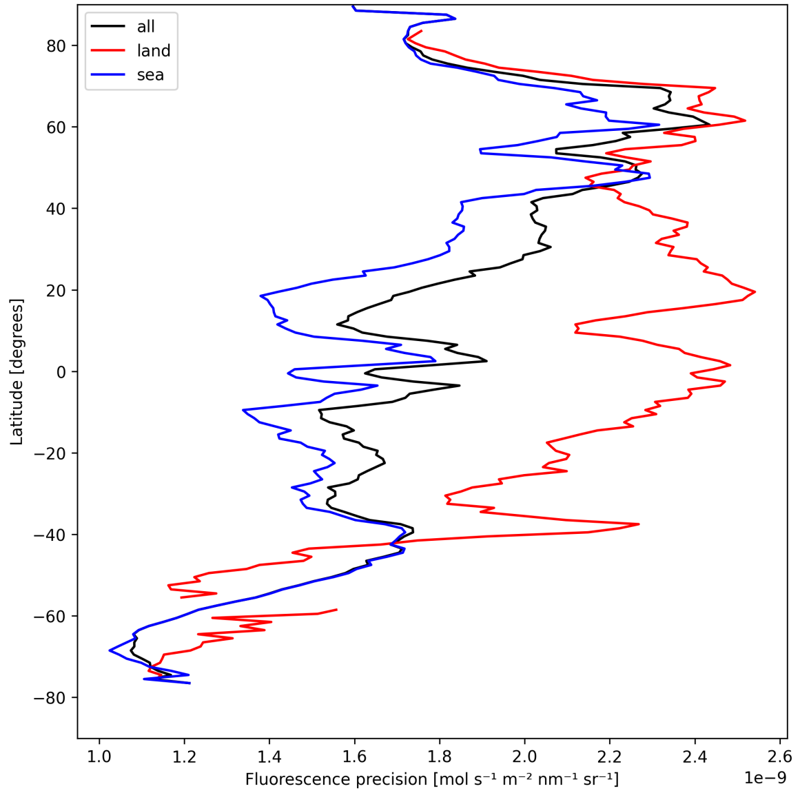
Figure 24: Zonal average of “Fluorescence precision” for 2025-04-20 to 2025-04-22.
