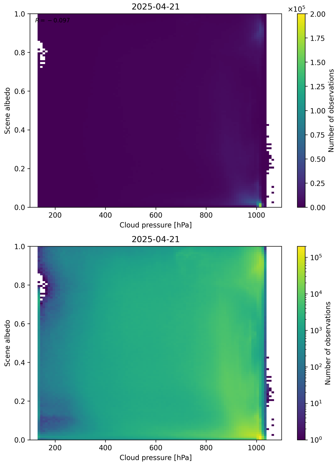
Figure 83: Scatter density plot of “Cloud pressure” against “Scene albedo” for 2025-04-20 to 2025-04-22.
