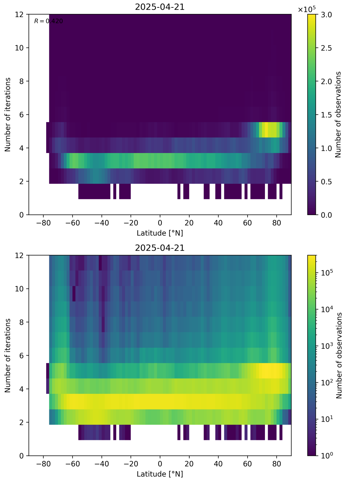
Figure 93: Scatter density plot of “Latitude” against “Number of iterations” for 2025-04-20 to 2025-04-22.
