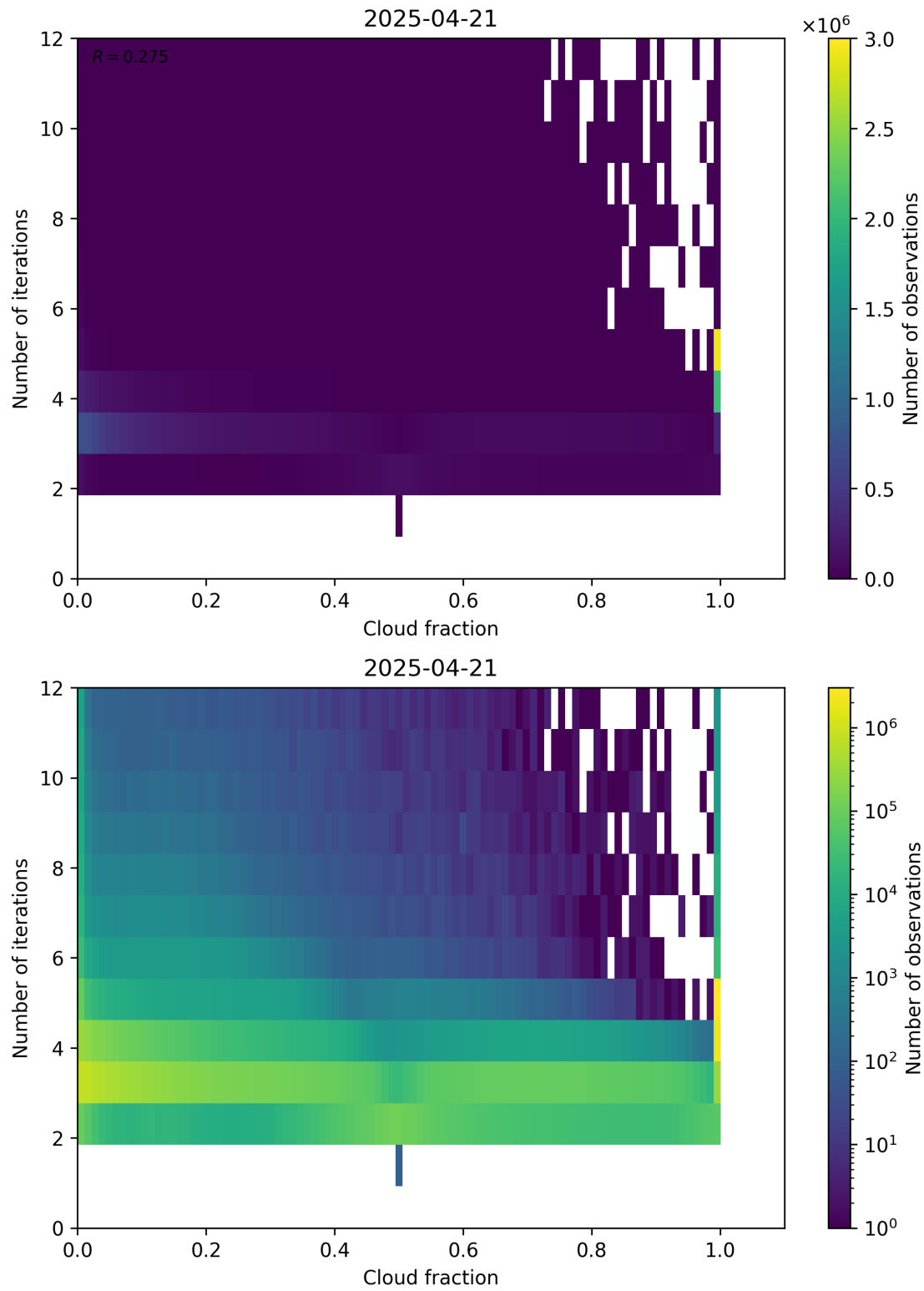
Figure 73: Scatter density plot of “Cloud fraction” against “Number of iterations” for 2025-04-20 to 2025-04-22.
