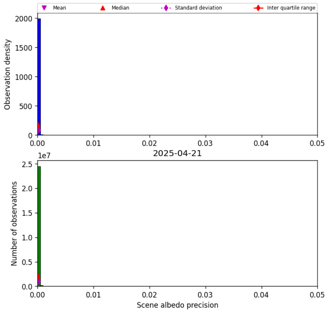
Figure 35: Histogram of “Scene albedo precision” for 2025-04-20 to 2025-04-22
