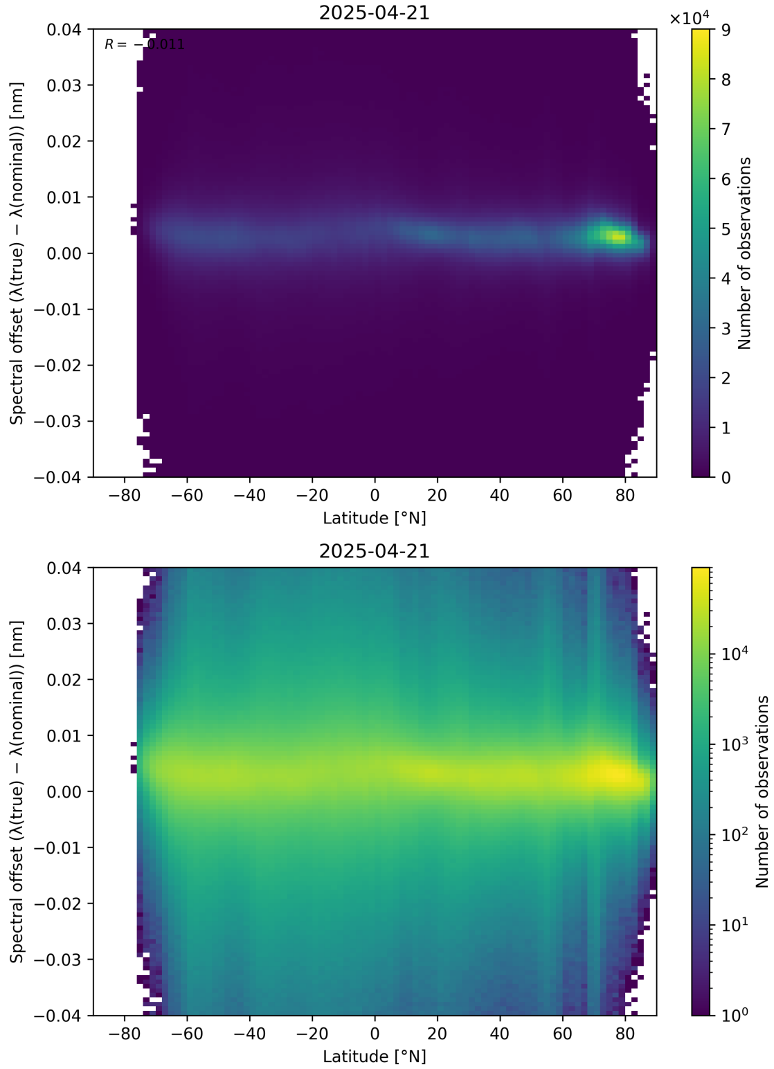
Figure 96: Scatter density plot of “Latitude” against “Spectral offset ( \lambda_{\text{true}} - \lambda_{\text{nominal}} )” for 2025-04-20 to 2025-04-22.
