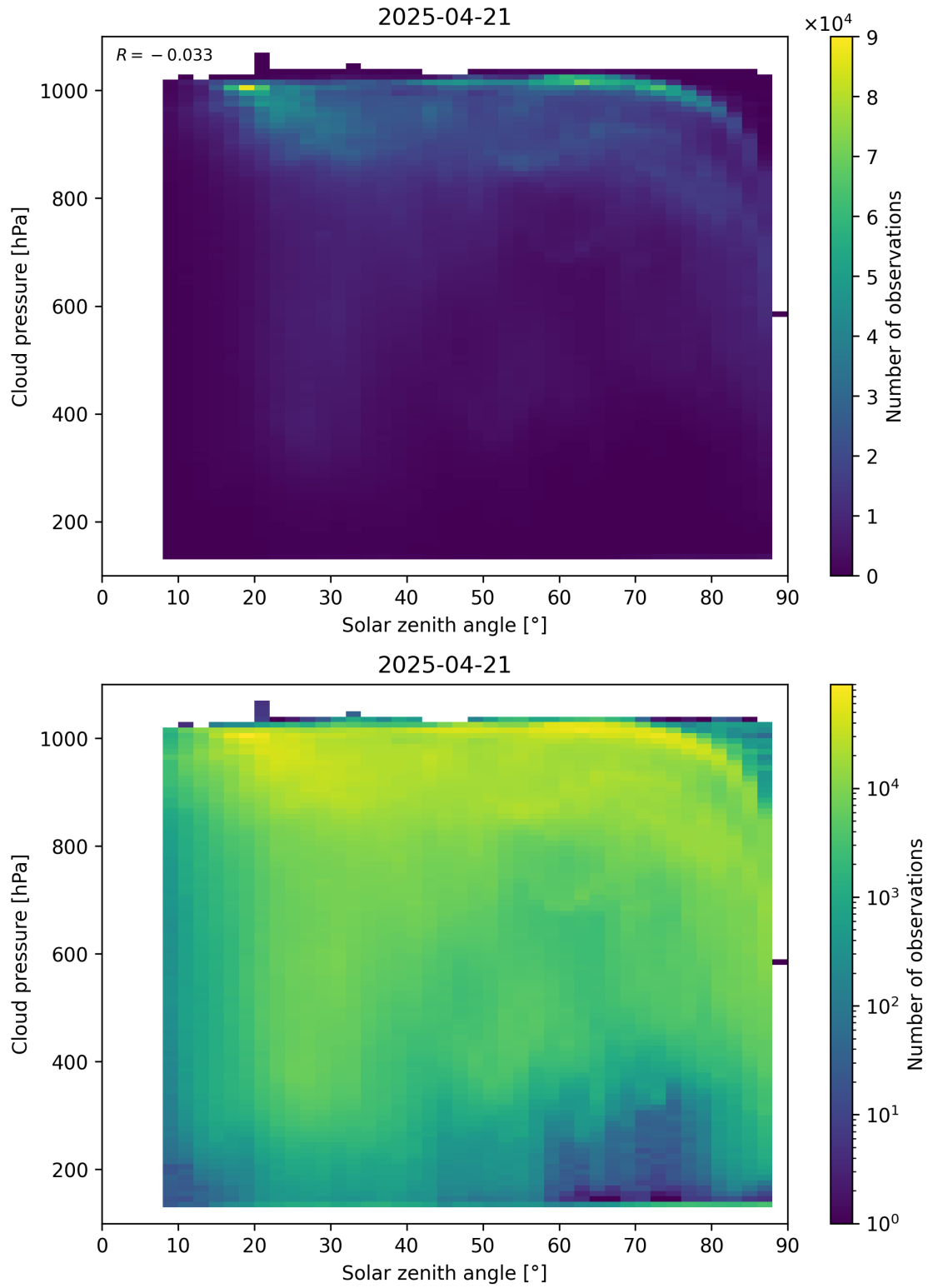
Figure 111: Scatter density plot of “Solar zenith angle” against “Cloud pressure” for 2025-04-20 to 2025-04-22.
