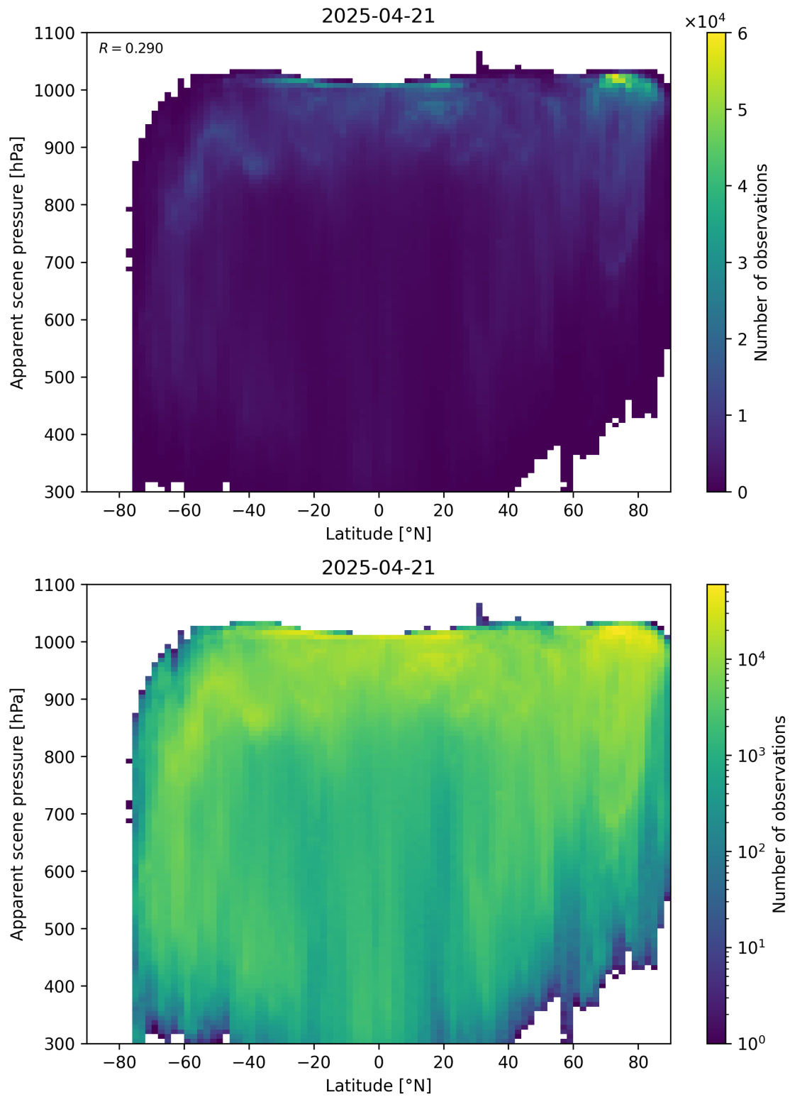
Figure 88: Scatter density plot of “Latitude” against “Apparent scene pressure” for 2025-04-20 to 2025-04-22.
