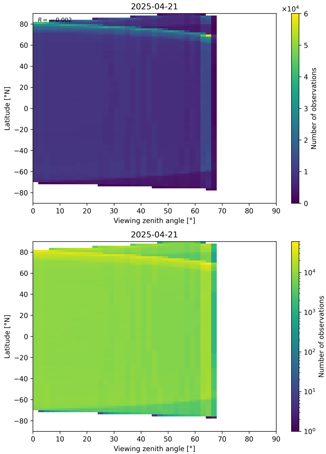
Figure 123: Scatter density plot of “Viewing zenith angle” against “Latitude” for 2025-04-20 to 2025-04-22.
