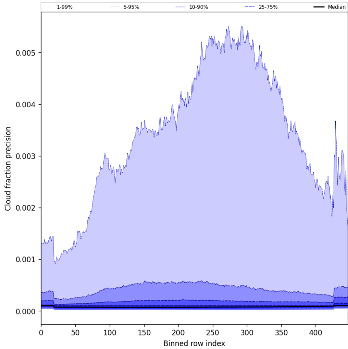
Figure 50: Along track statistics of “Cloud fraction precision” for 2025-04-20 to 2025-04-22
