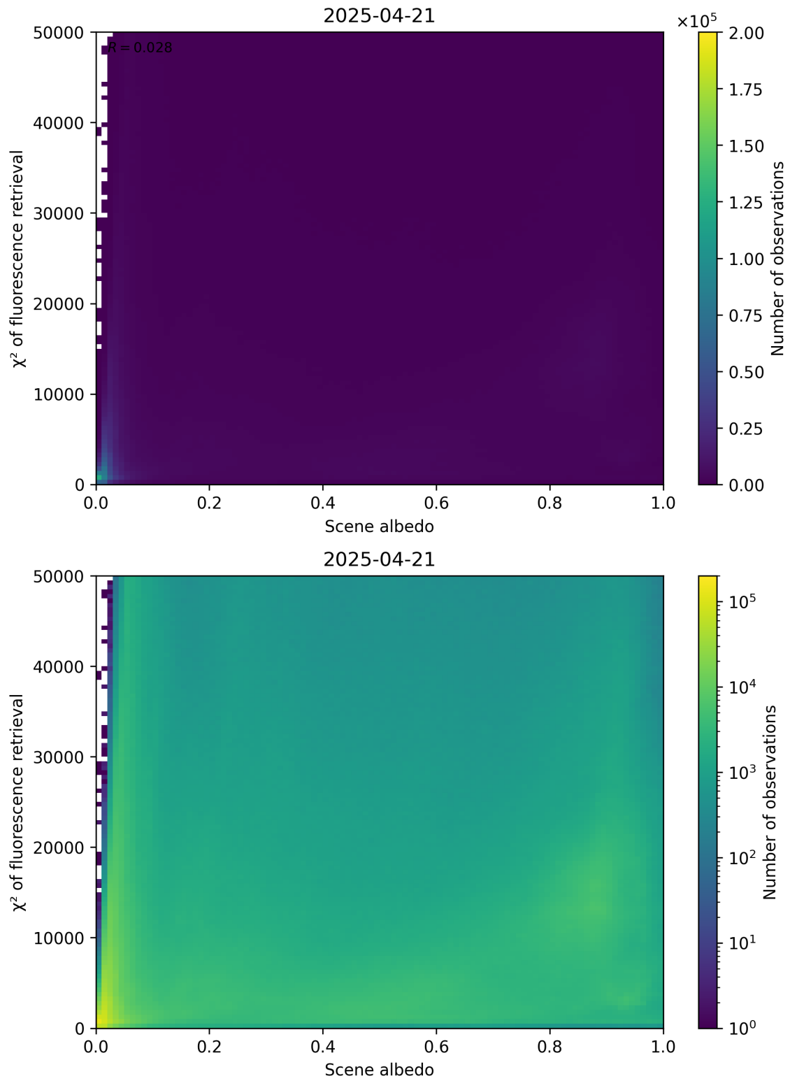
Figure 103: Scatter density plot of “Scene albedo” against “ \chi^2 of fluorescence retrieval” for 2025-04-20 to 2025-04-22.
