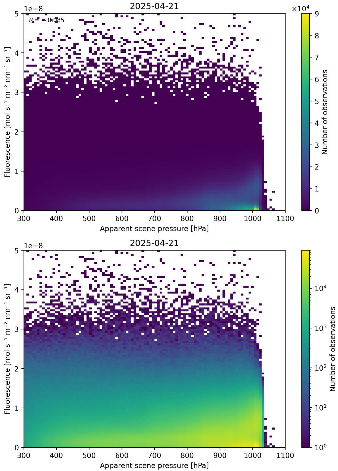
Figure 64: Scatter density plot of “Apparent scene pressure” against “Fluorescence” for 2025-04-20 to 2025-04-22.
