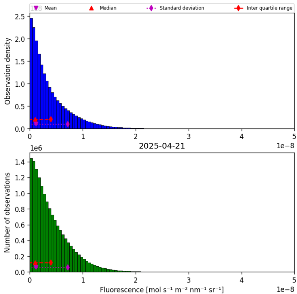
Figure 40: Histogram of “Fluorescence” for 2025-04-20 to 2025-04-22
