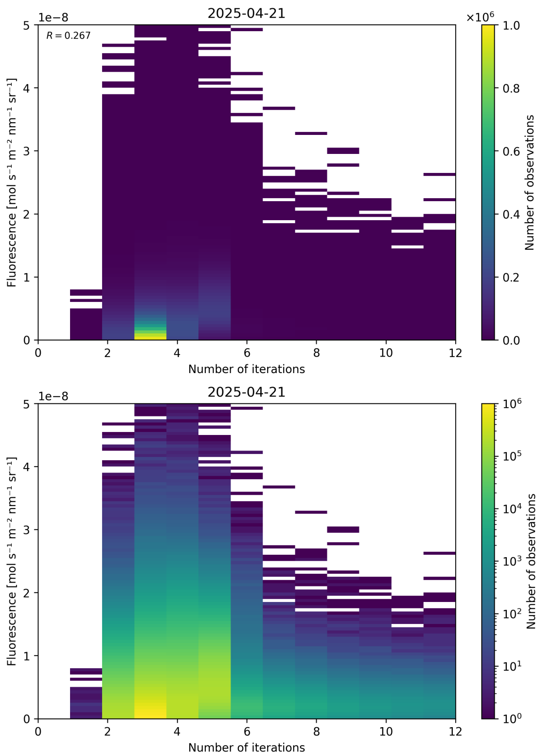
Figure 98: Scatter density plot of “Number of iterations” against “Fluorescence” for 2025-04-20 to 2025-04-22.
