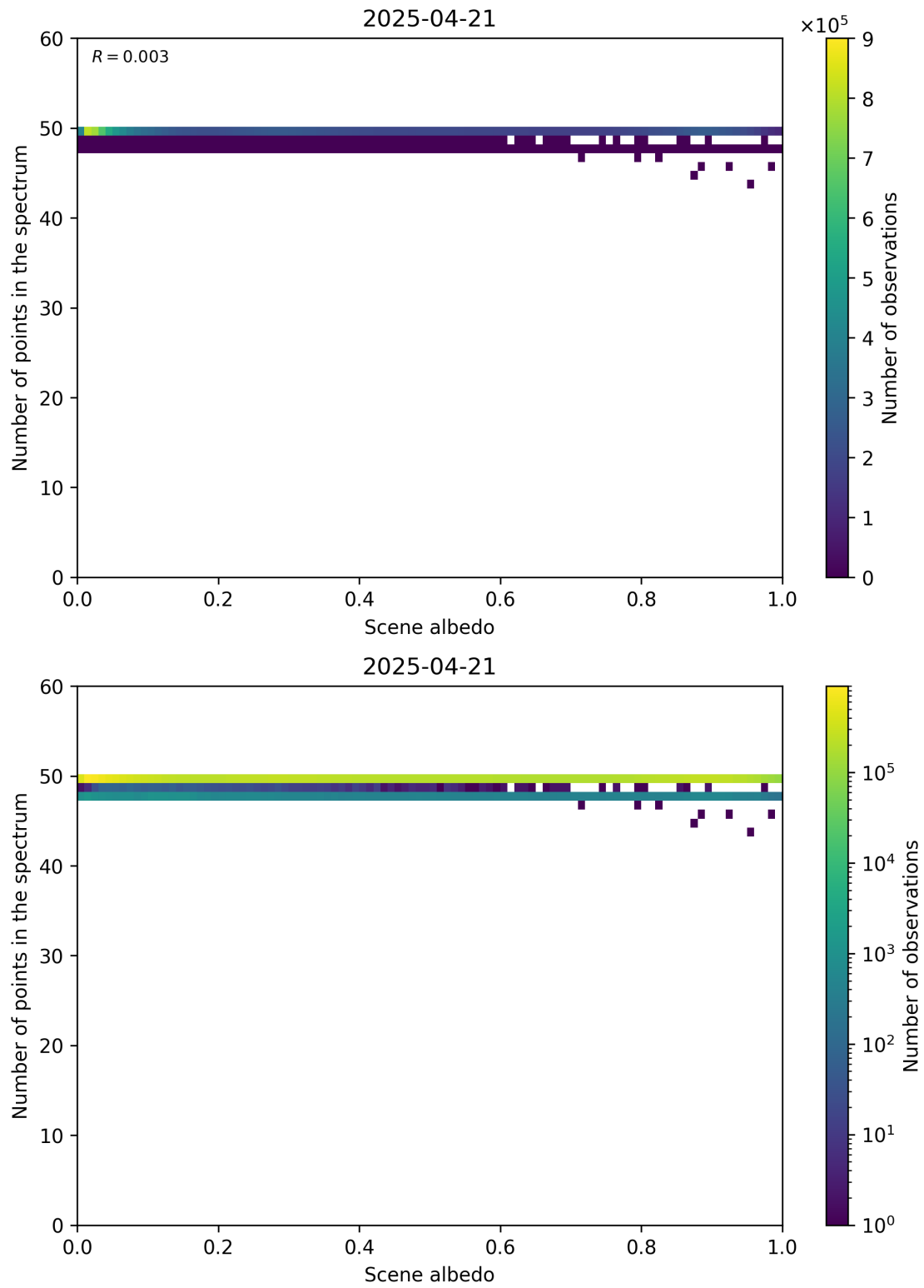
Figure 106: Scatter density plot of “Scene albedo” against “Number of points in the spectrum” for 2025-04-20 to 2025-04-22.
