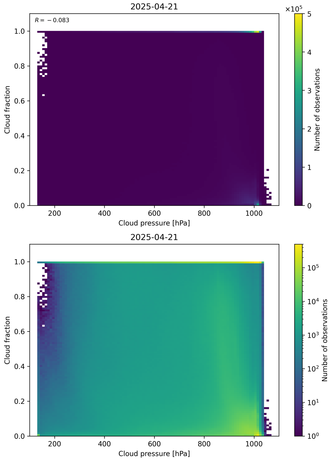
Figure 79: Scatter density plot of “Cloud pressure” against “Cloud fraction” for 2025-04-20 to 2025-04-22.
