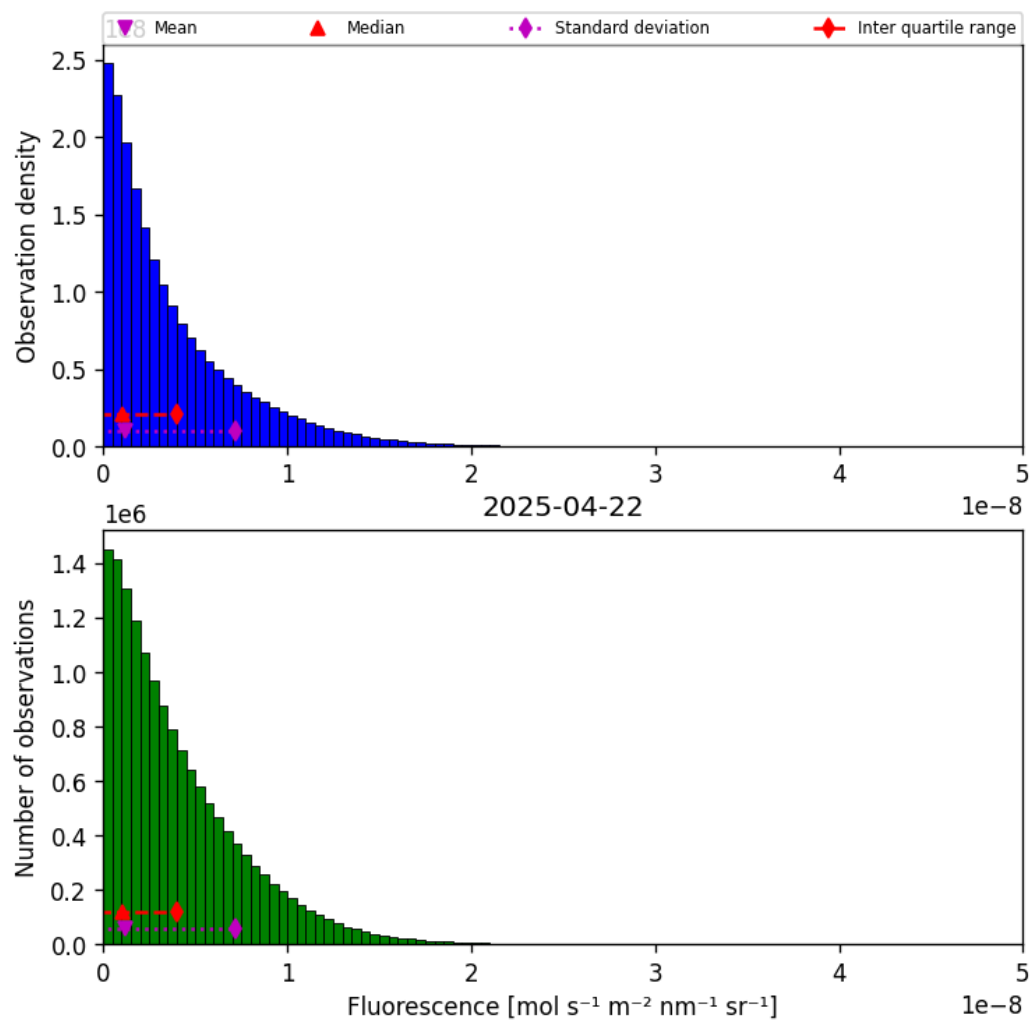
Figure 40: Histogram of “Fluorescence” for 2025-04-21 to 2025-04-23
