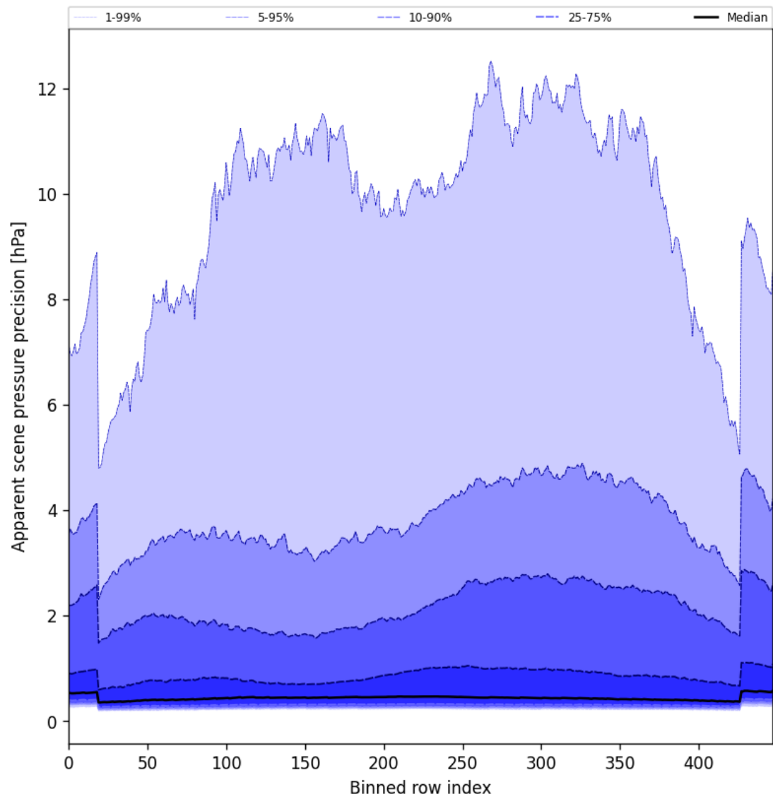
Figure 54: Along track statistics of “Apparent scene pressure precision” for 2025-04-21 to 2025-04-23
