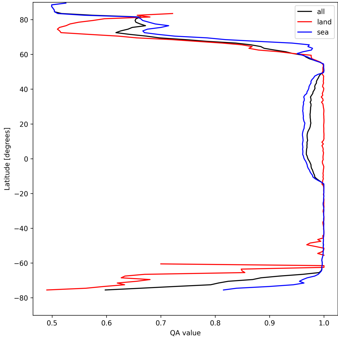
Figure 12: Zonal average of “QA value” for 2025-04-21 to 2025-04-23.
