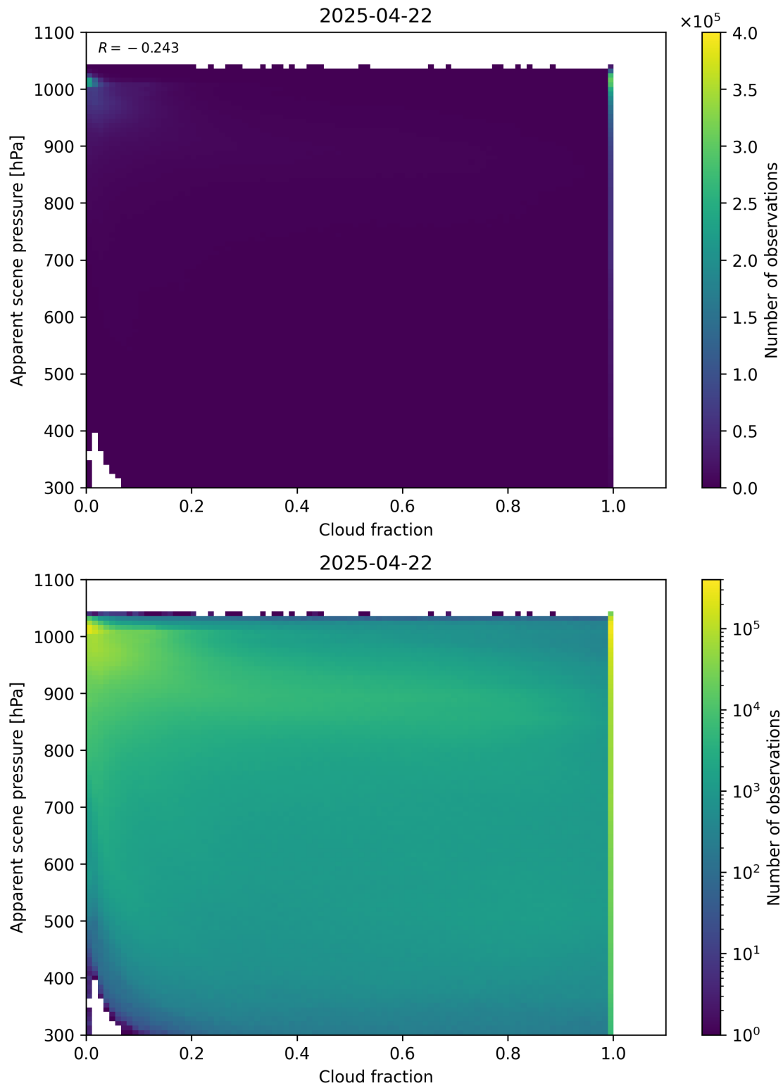
Figure 70: Scatter density plot of “Cloud fraction” against “Apparent scene pressure” for 2025-04-21 to 2025-04-23.
