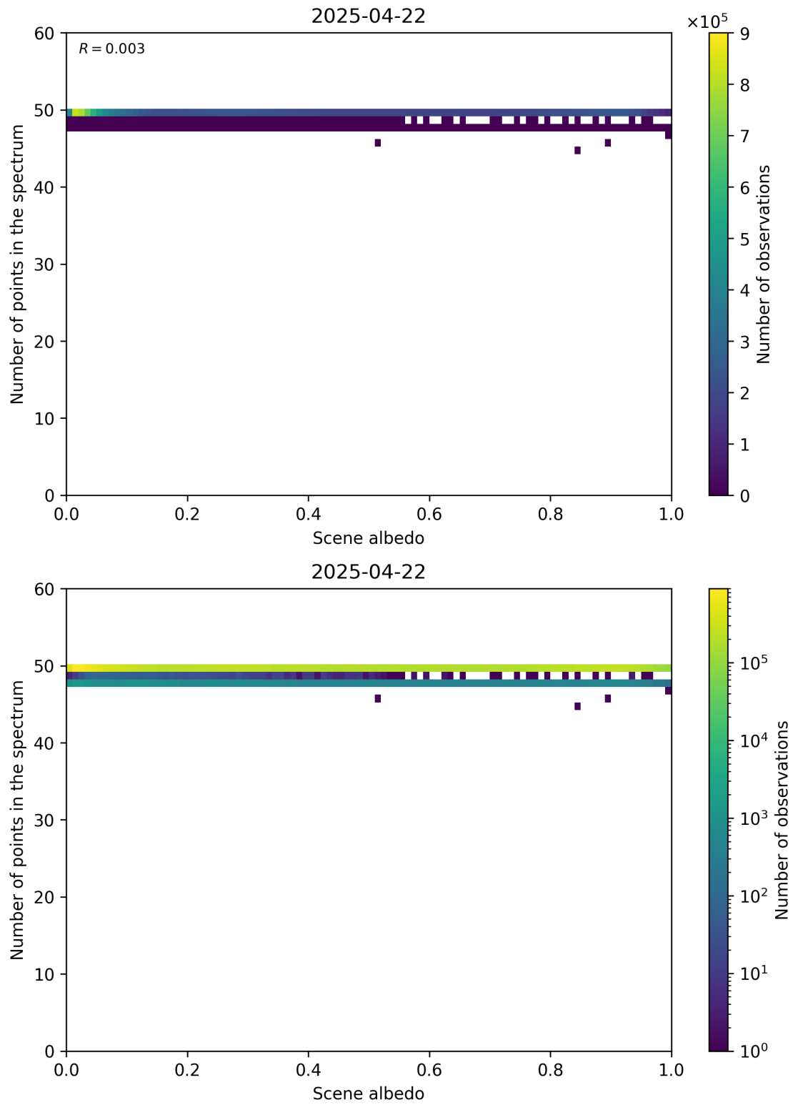
Figure 106: Scatter density plot of “Scene albedo” against “Number of points in the spectrum” for 2025-04-21 to 2025-04-23.
