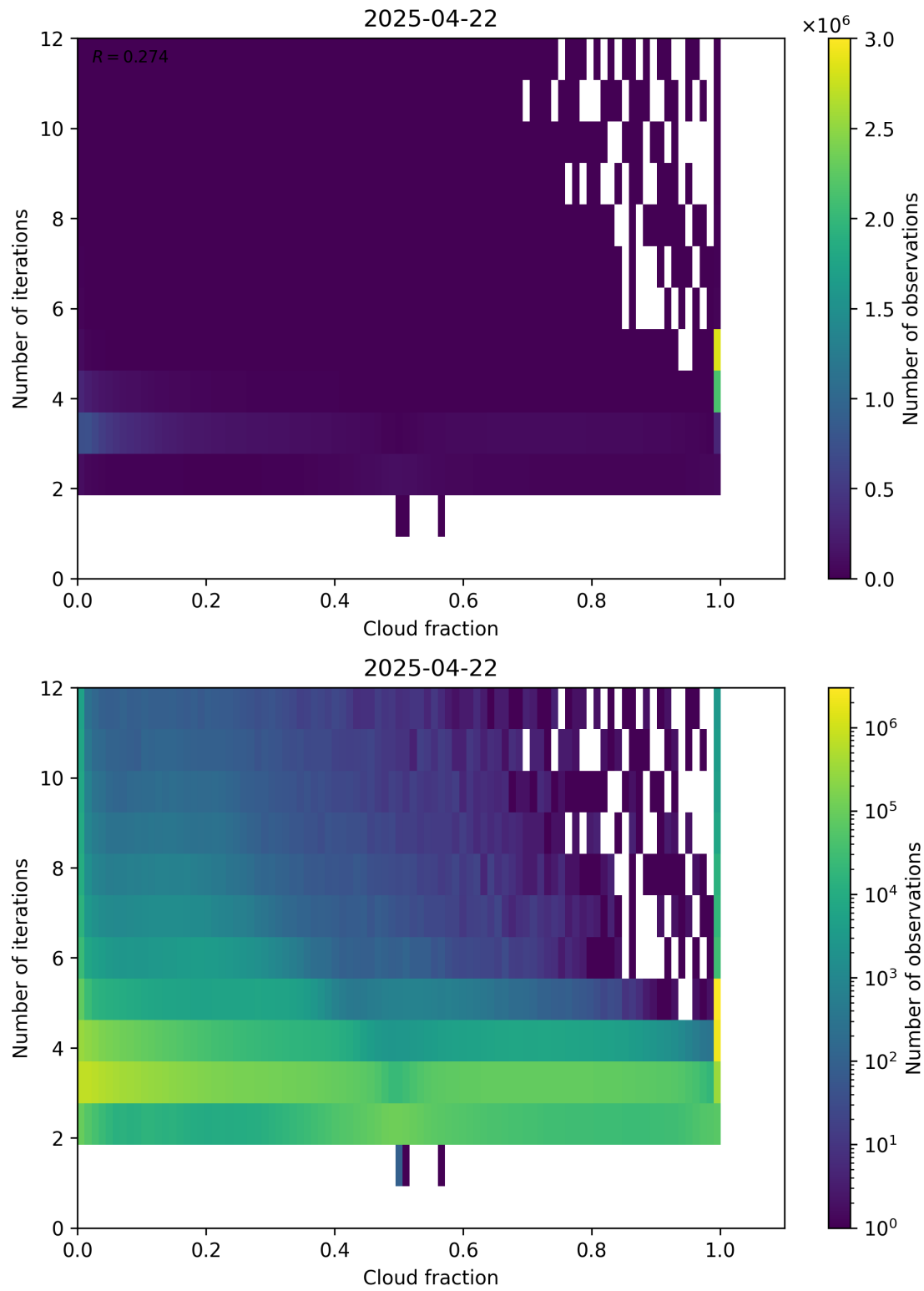
Figure 73: Scatter density plot of “Cloud fraction” against “Number of iterations” for 2025-04-21 to 2025-04-23.
