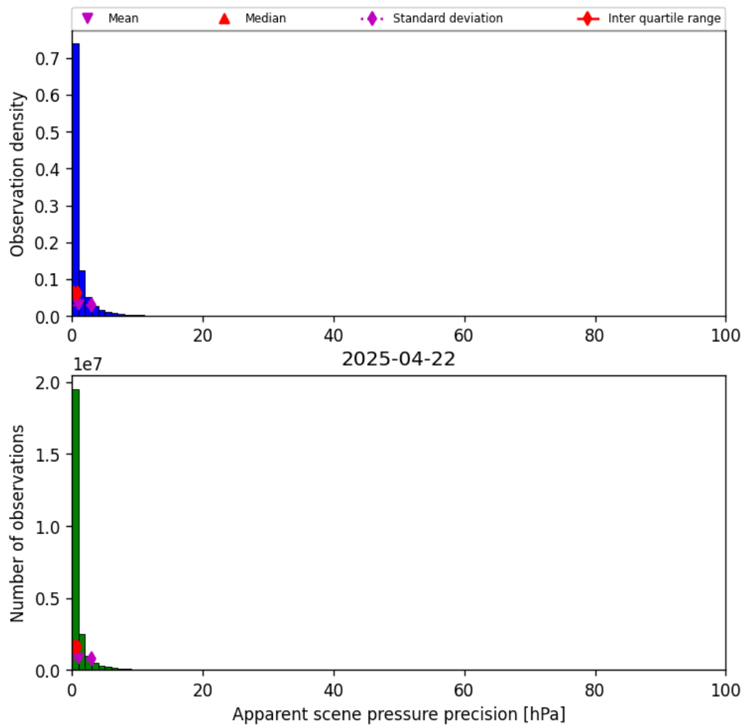
Figure 37: Histogram of “Apparent scene pressure precision” for 2025-04-21 to 2025-04-23
