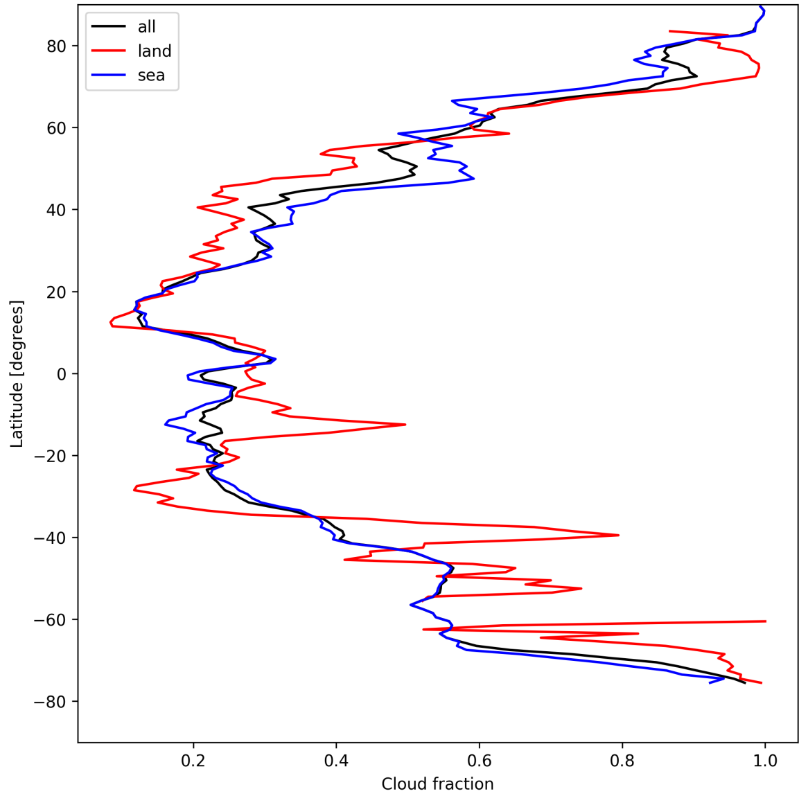
Figure 15: Zonal average of “Cloud fraction” for 2025-04-21 to 2025-04-23.
