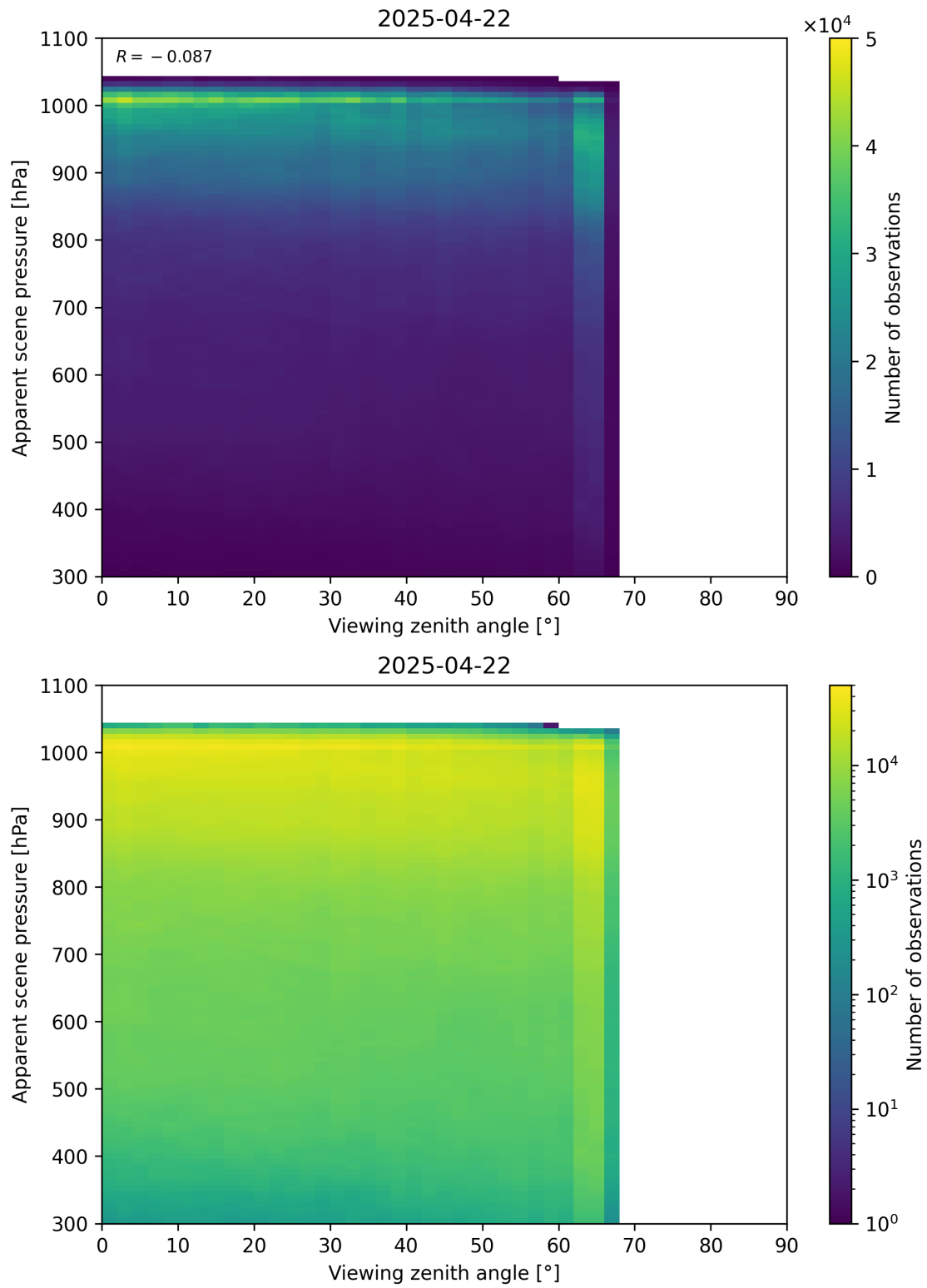
Figure 118: Scatter density plot of “Viewing zenith angle” against “Apparent scene pressure” for 2025-04-21 to 2025-04-23.
