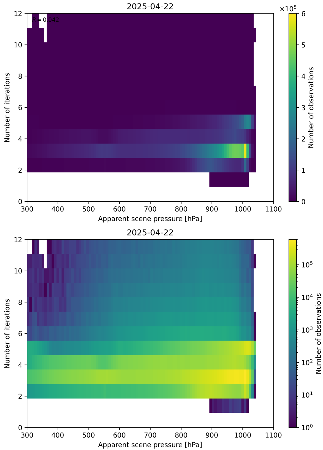
Figure 65: Scatter density plot of “Apparent scene pressure” against “Number of iterations” for 2025-04-21 to 2025-04-23.
