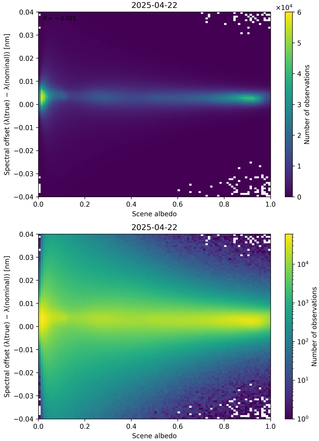
Figure 107: Scatter density plot of “Scene albedo” against “Spectral offset ( \lambda_{\text{true}} - \lambda_{\text{nominal}} )” for 2025-04-21 to 2025-04-23.
