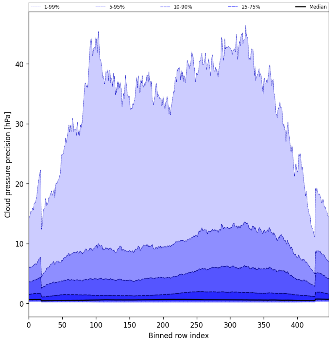
Figure 48: Along track statistics of “Cloud pressure precision” for 2025-04-21 to 2025-04-23
