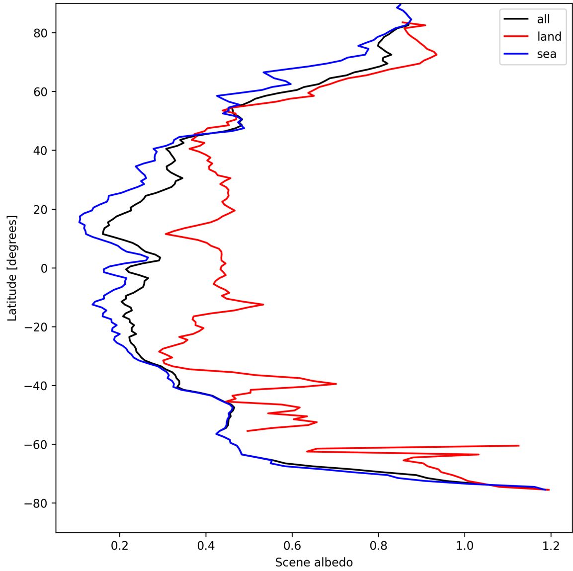
Figure 17: Zonal average of “Scene albedo” for 2025-04-21 to 2025-04-23.
