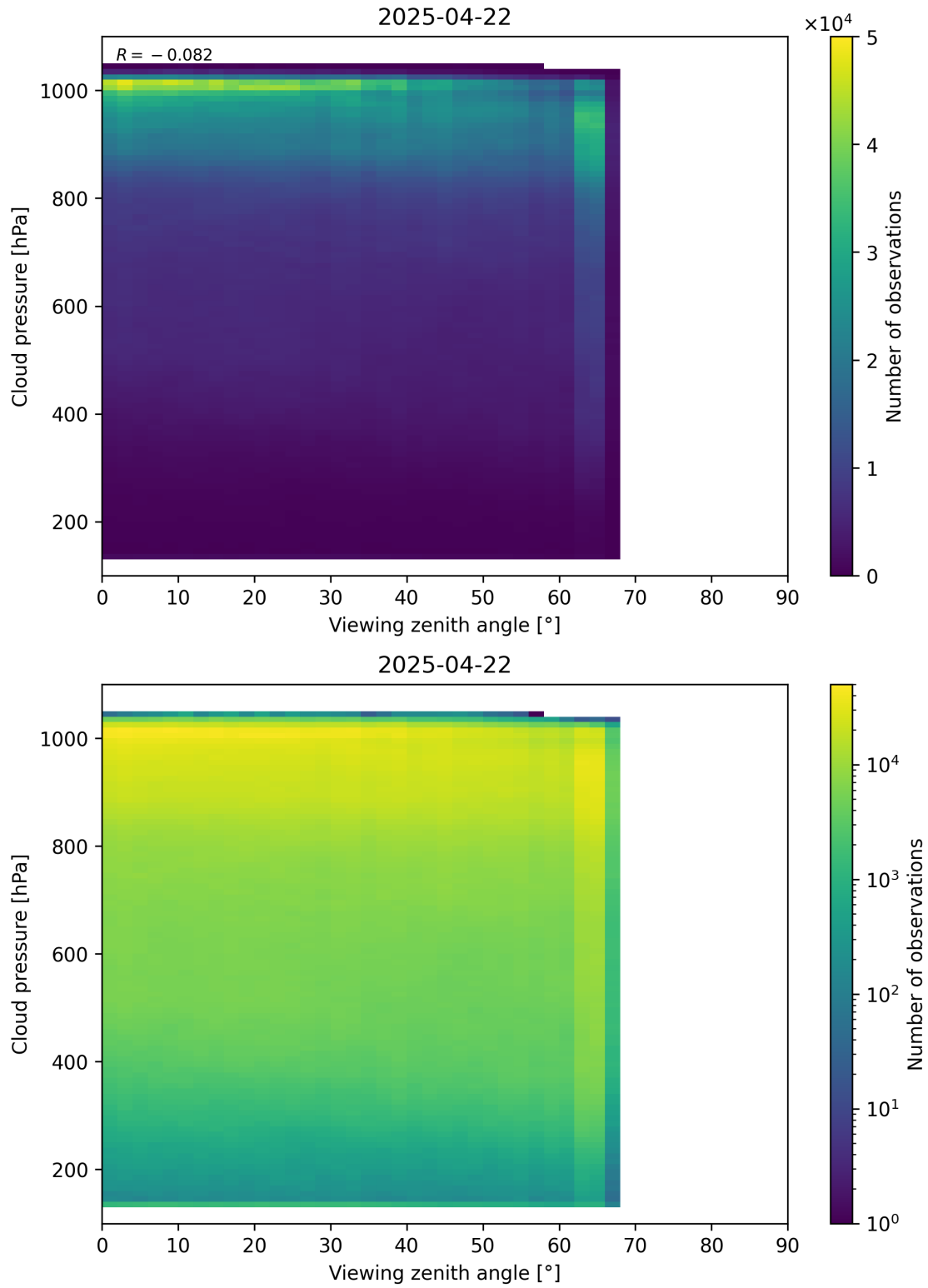
Figure 121: Scatter density plot of “Viewing zenith angle” against “Cloud pressure” for 2025-04-21 to 2025-04-23.
