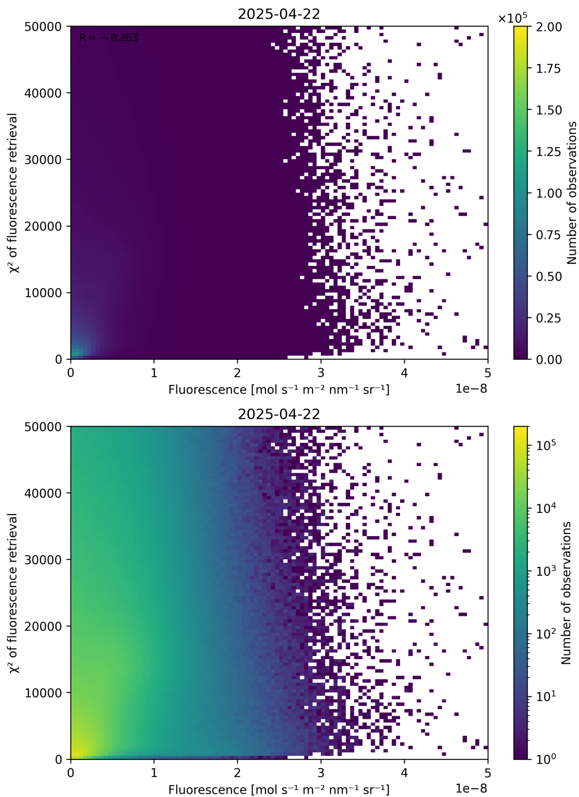
Figure 85: Scatter density plot of “Fluorescence” against “ \chi^2 of fluorescence retrieval” for 2025-04-21 to 2025-04-23.
