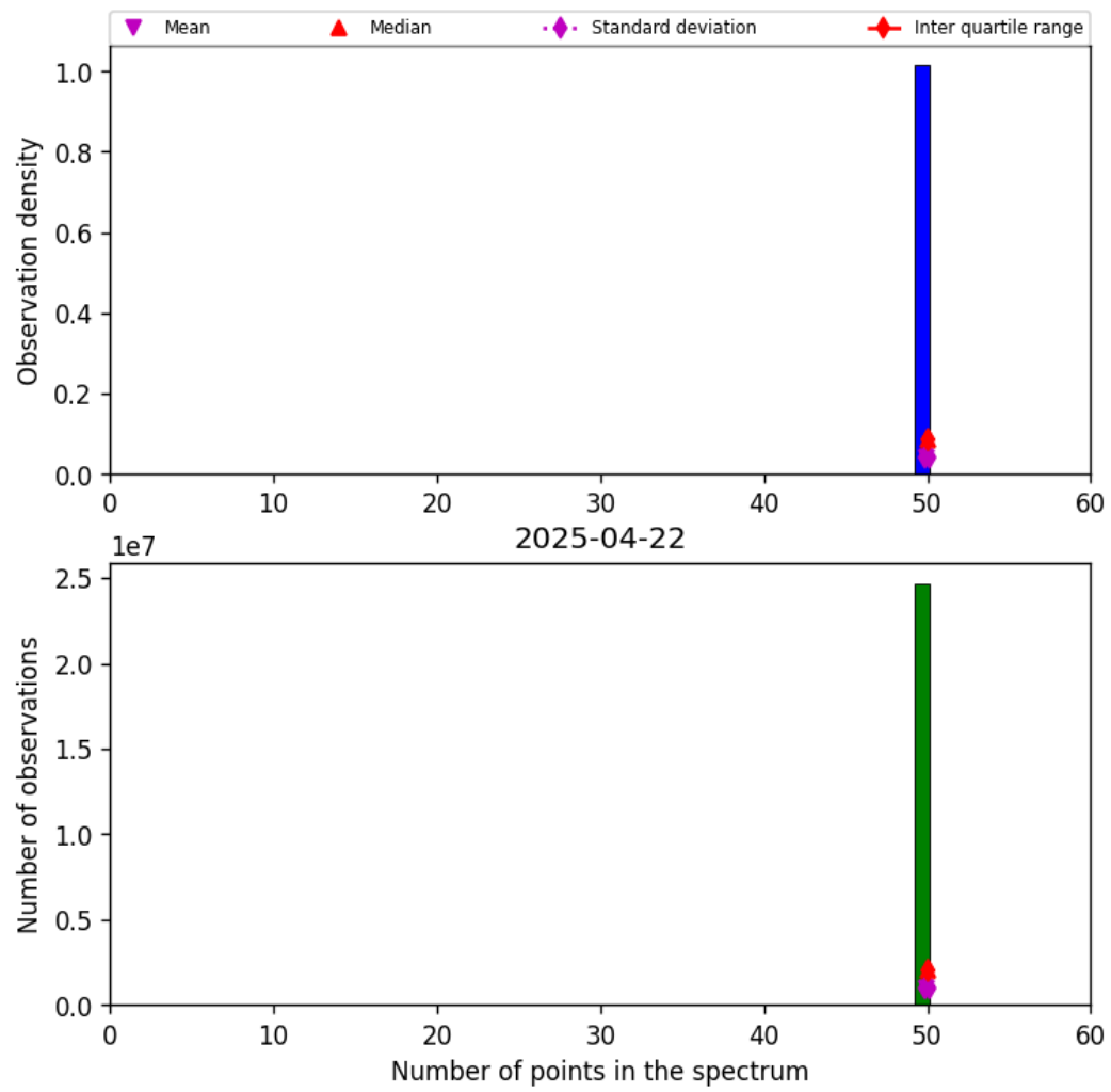
Figure 44: Histogram of “Number of points in the spectrum” for 2025-04-21 to 2025-04-23
