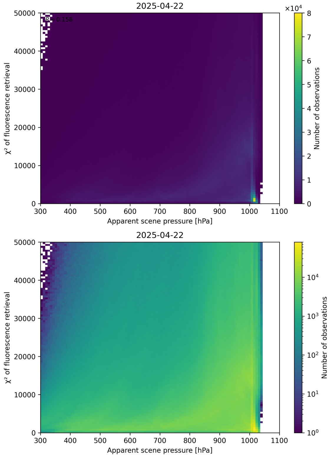
Figure 63: Scatter density plot of “Apparent scene pressure” against “ \chi^2 of fluorescence retrieval” for 2025-04-21 to 2025-04-23.
