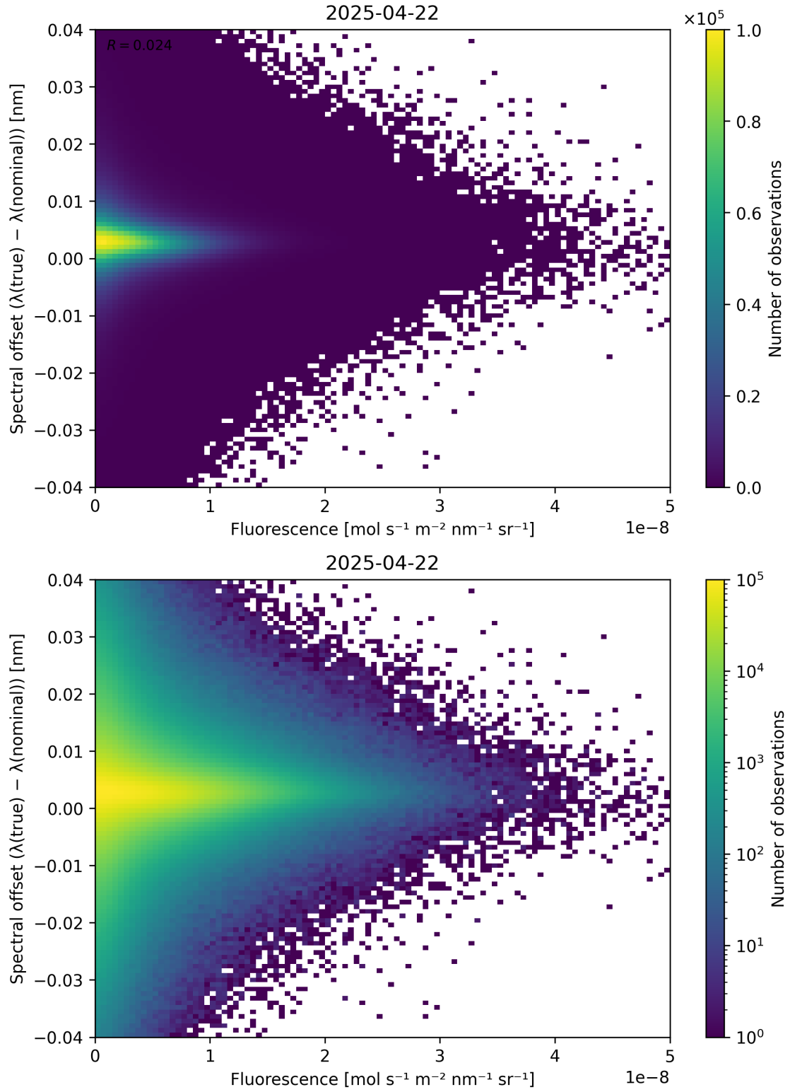
Figure 87: Scatter density plot of “Fluorescence” against “Spectral offset ( \lambda_{\text{true}} - \lambda_{\text{nominal}} )” for 2025-04-21 to 2025-04-23.
