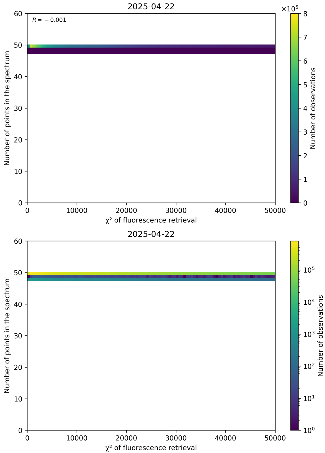
Figure 68: Scatter density plot of " \chi^2 of fluorescence retrieval" against "Number of points in the spectrum" for 2025-04-21 to 2025-04-23.
