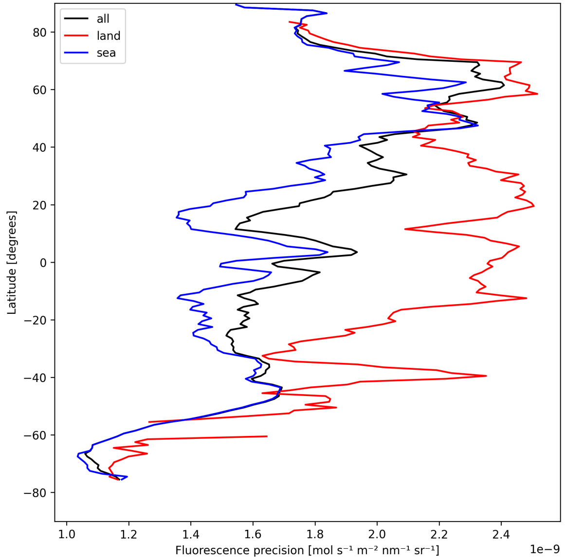
Figure 24: Zonal average of “Fluorescence precision” for 2025-04-21 to 2025-04-23.
