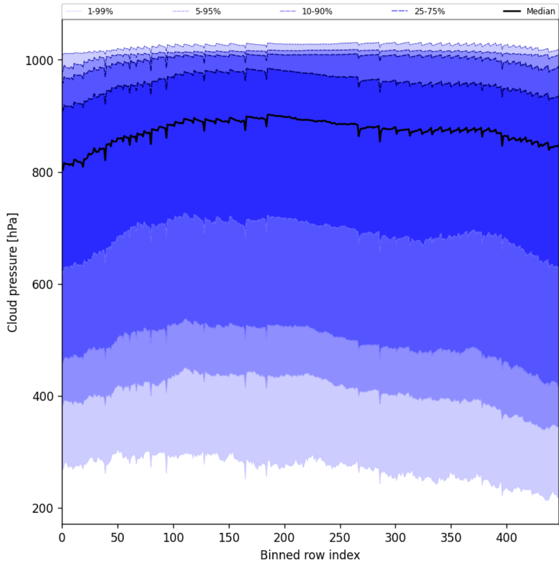
Figure 47: Along track statistics of “Cloud pressure” for 2025-04-21 to 2025-04-23
