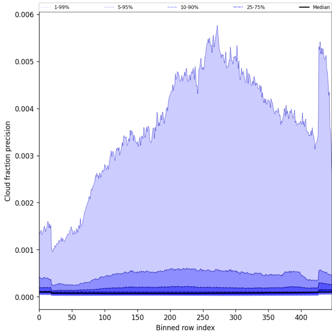
Figure 50: Along track statistics of “Cloud fraction precision” for 2025-04-21 to 2025-04-23
