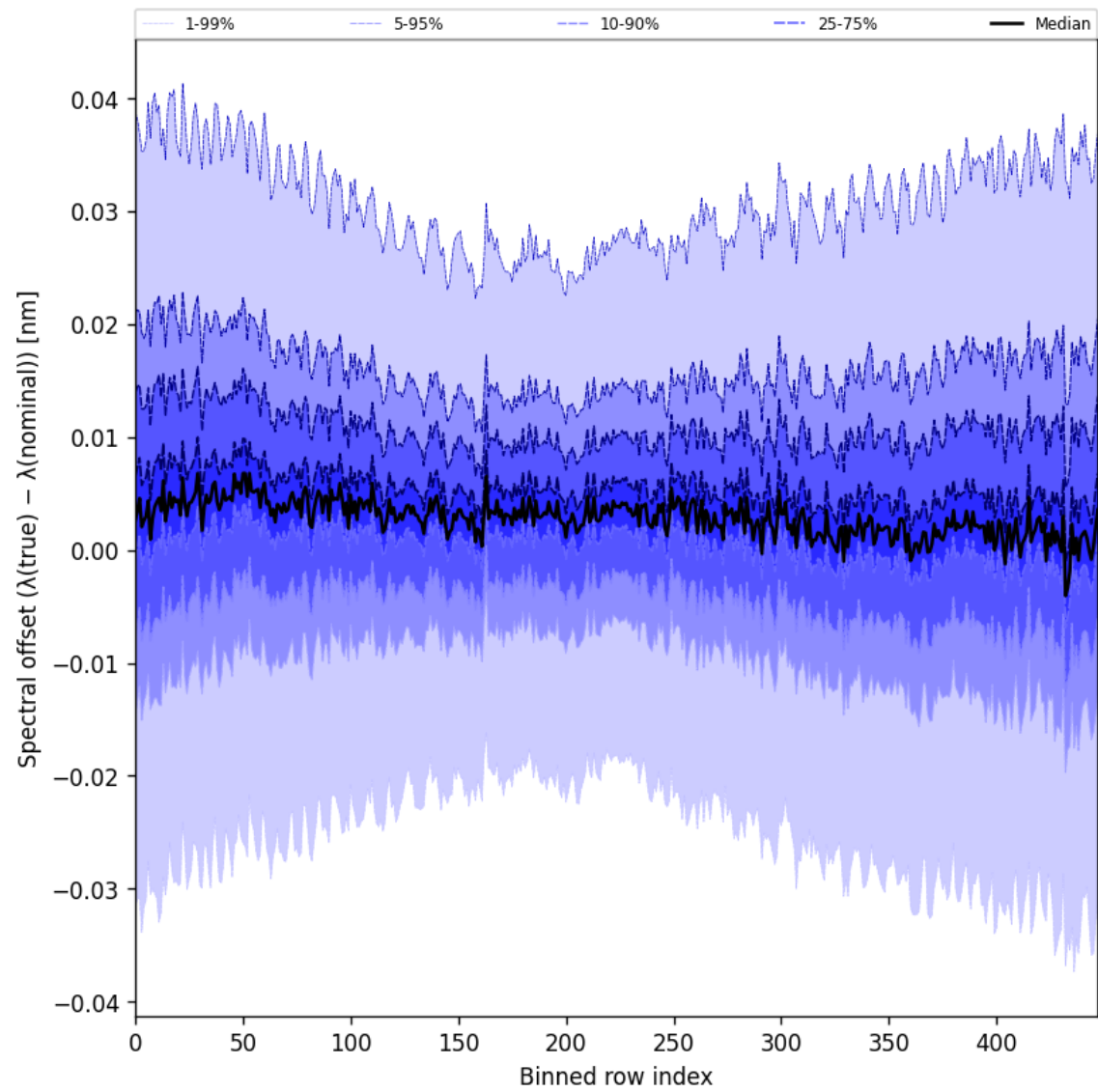
Figure 62: Along track statistics of “Spectral offset ( \lambda_{\text{true}} - \lambda_{\text{nominal}} )” for 2025-04-21 to 2025-04-23
