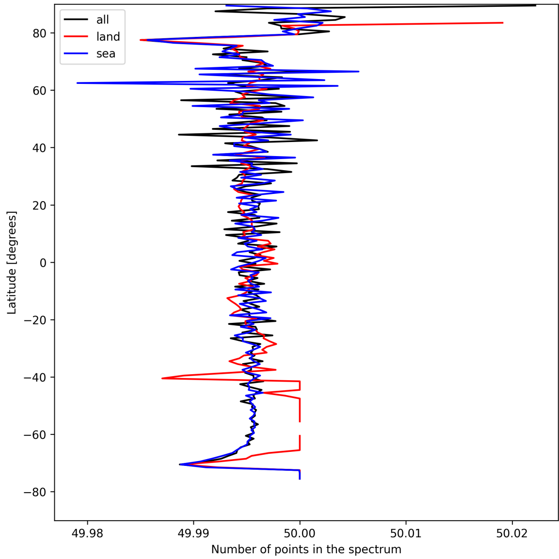
Figure 27: Zonal average of “Number of points in the spectrum” for 2025-04-21 to 2025-04-23.
