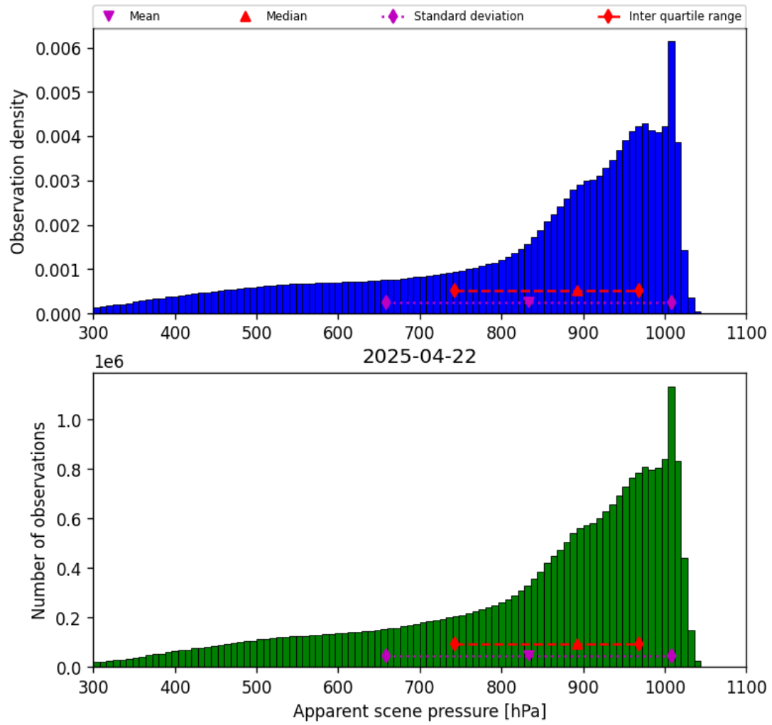
Figure 36: Histogram of “Apparent scene pressure” for 2025-04-21 to 2025-04-23
