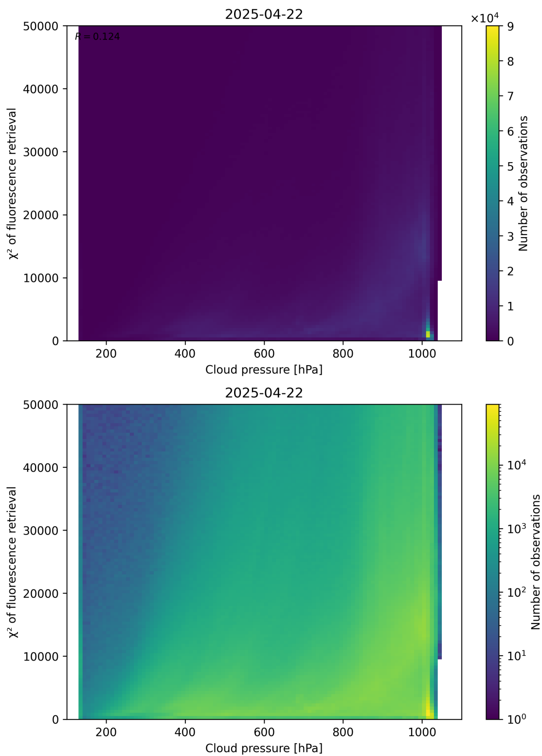
Figure 78: Scatter density plot of “Cloud pressure” against “ \chi^2 of fluorescence retrieval” for 2025-04-21 to 2025-04-23.
