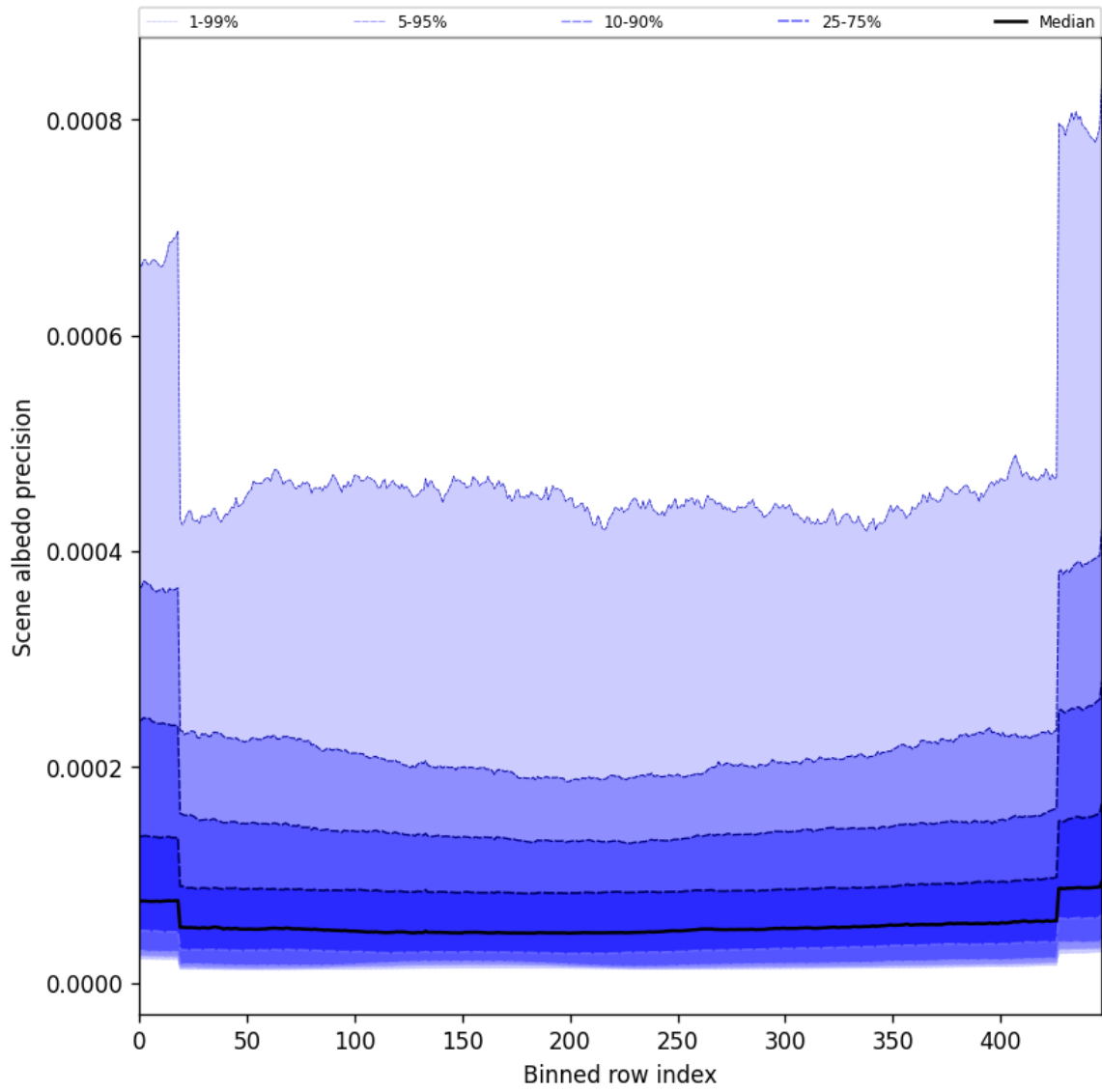
Figure 52: Along track statistics of “Scene albedo precision” for 2025-04-21 to 2025-04-23
