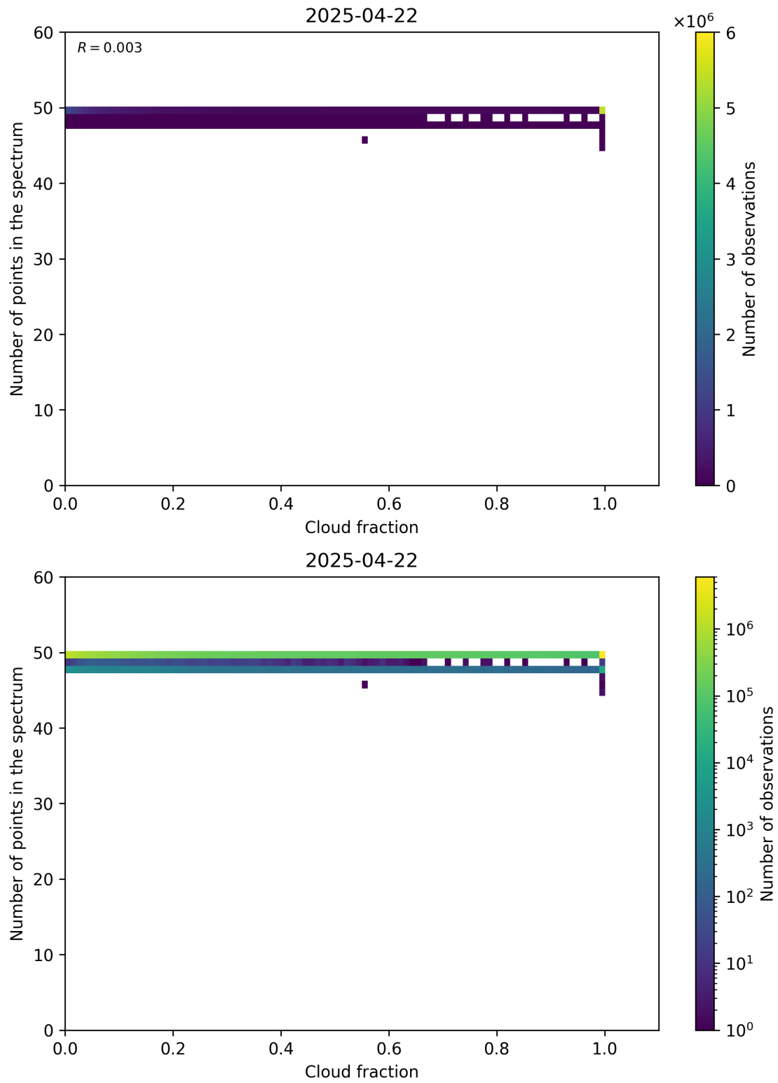
Figure 74: Scatter density plot of “Cloud fraction” against “Number of points in the spectrum” for 2025-04-21 to 2025-04-23.
