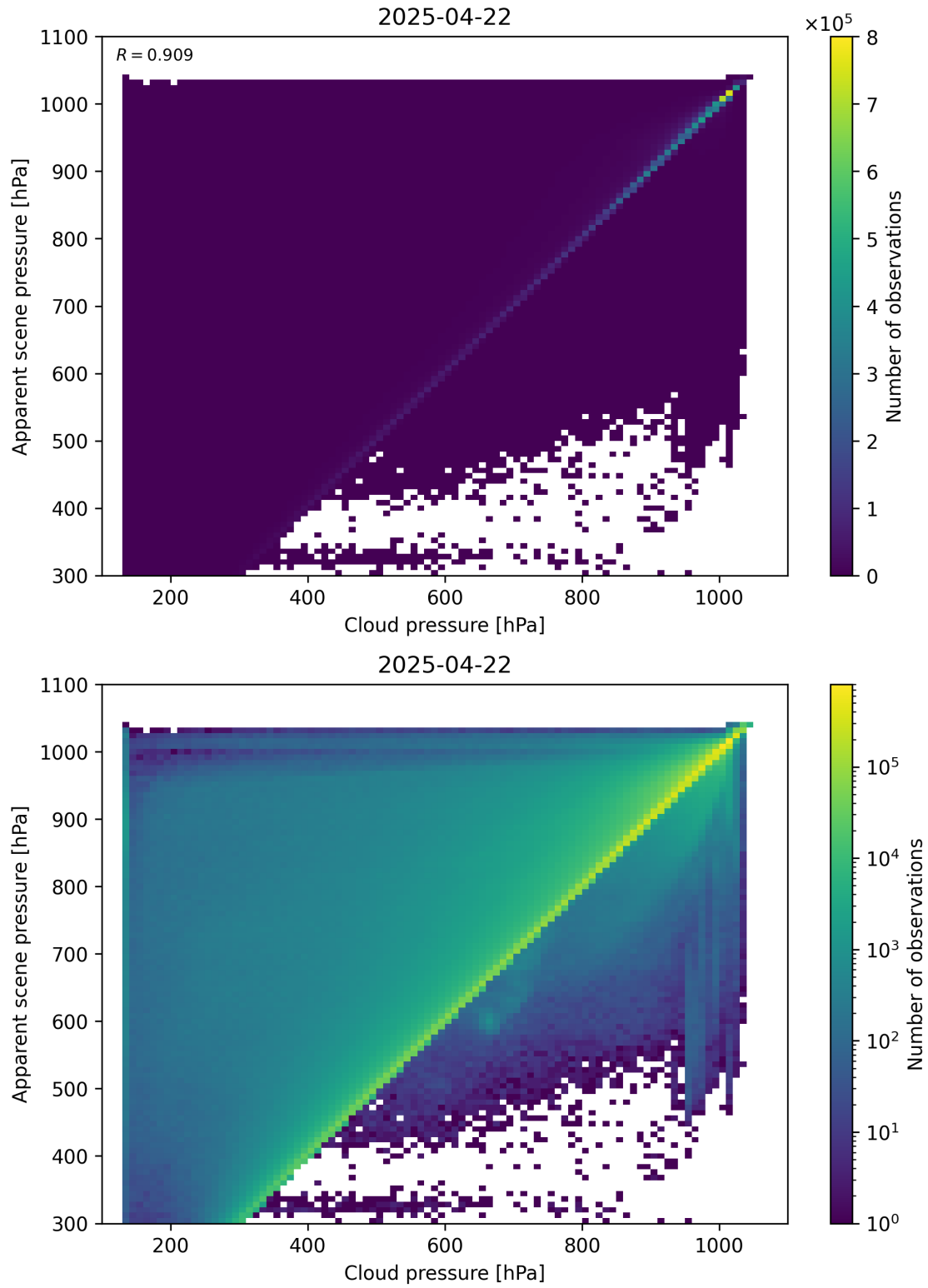
Figure 77: Scatter density plot of “Cloud pressure” against “Apparent scene pressure” for 2025-04-21 to 2025-04-23.
