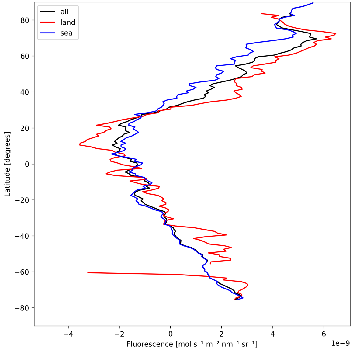
Figure 23: Zonal average of “Fluorescence” for 2025-04-21 to 2025-04-23.
