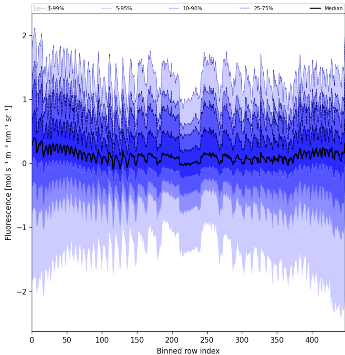
Figure 57: Along track statistics of “Fluorescence” for 2025-04-21 to 2025-04-23
