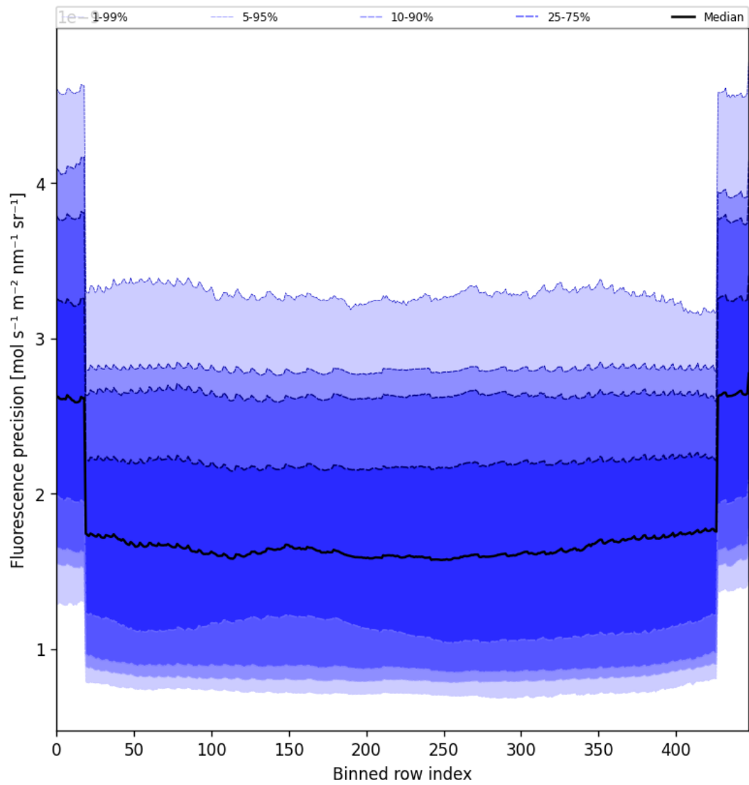
Figure 58: Along track statistics of “Fluorescence precision” for 2025-04-21 to 2025-04-23
