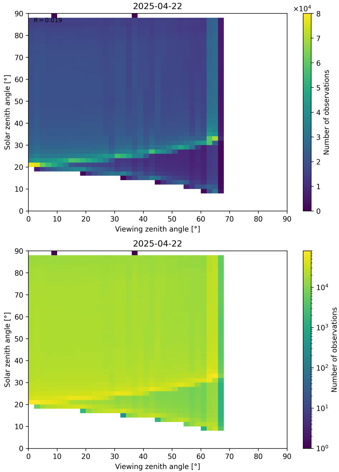
Figure 127: Scatter density plot of “Viewing zenith angle” against “Solar zenith angle” for 2025-04-21 to 2025-04-23.
