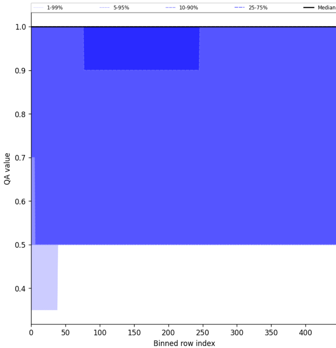
Figure 46: Along track statistics of “QA value” for 2025-04-21 to 2025-04-23
