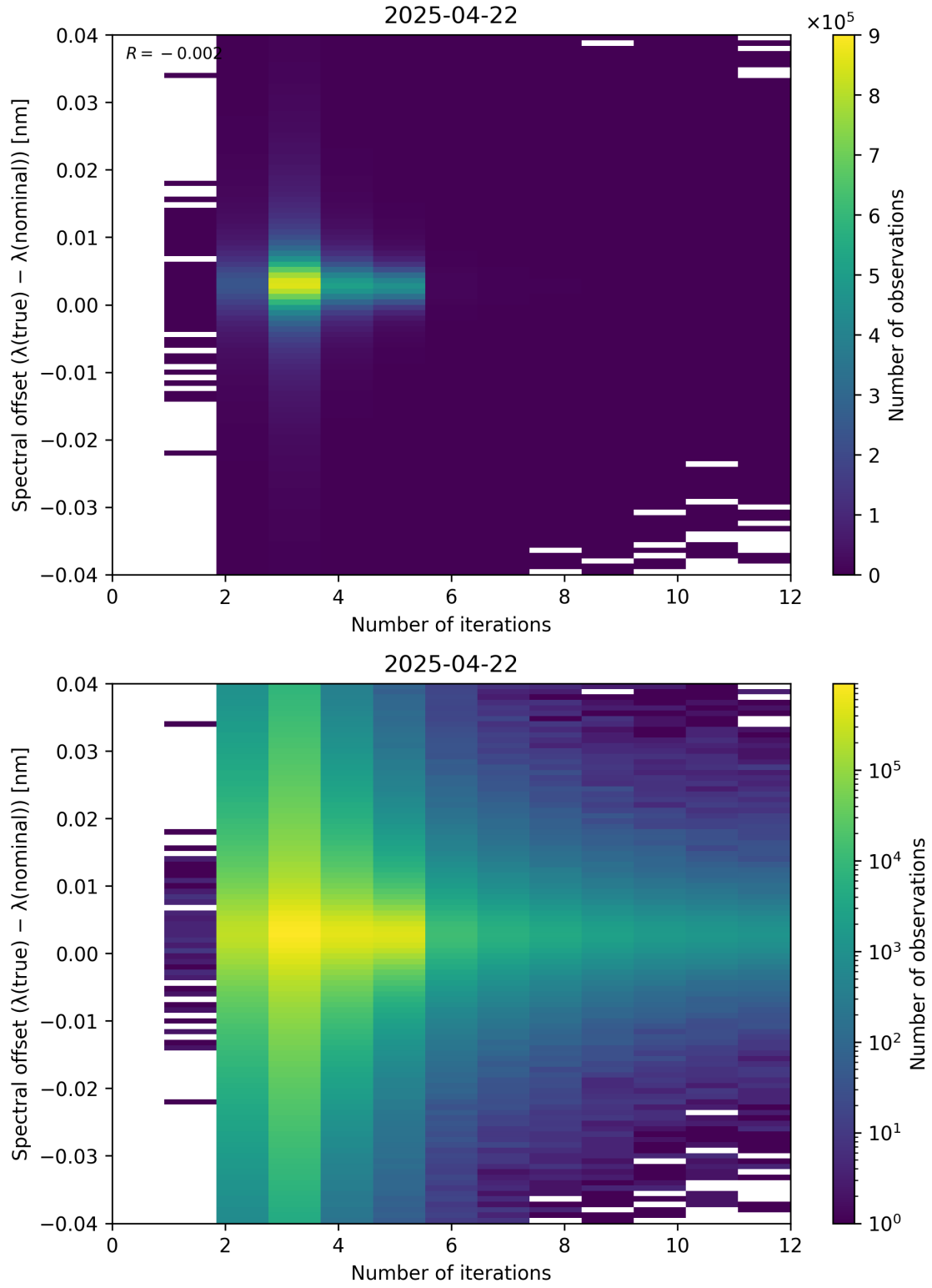
Figure 100: Scatter density plot of “Number of iterations” against “Spectral offset ( \lambda_{\text{true}} - \lambda_{\text{nominal}} )” for 2025-04-21 to 2025-04-23.
