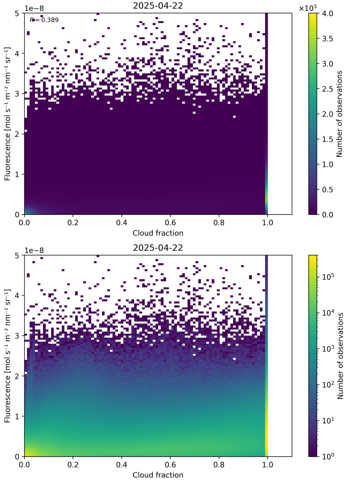
Figure 72: Scatter density plot of “Cloud fraction” against “Fluorescence” for 2025-04-21 to 2025-04-23.
