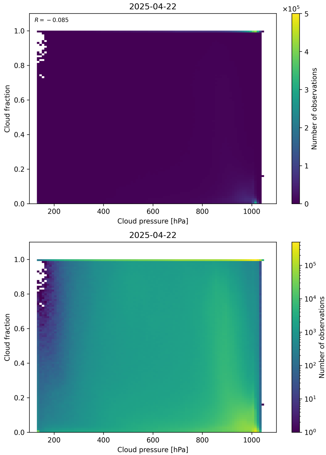
Figure 79: Scatter density plot of “Cloud pressure” against “Cloud fraction” for 2025-04-21 to 2025-04-23.
