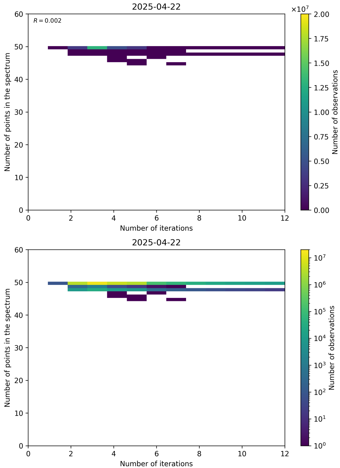
Figure 99: Scatter density plot of “Number of iterations” against “Number of points in the spectrum” for 2025-04-21 to 2025-04-23.
