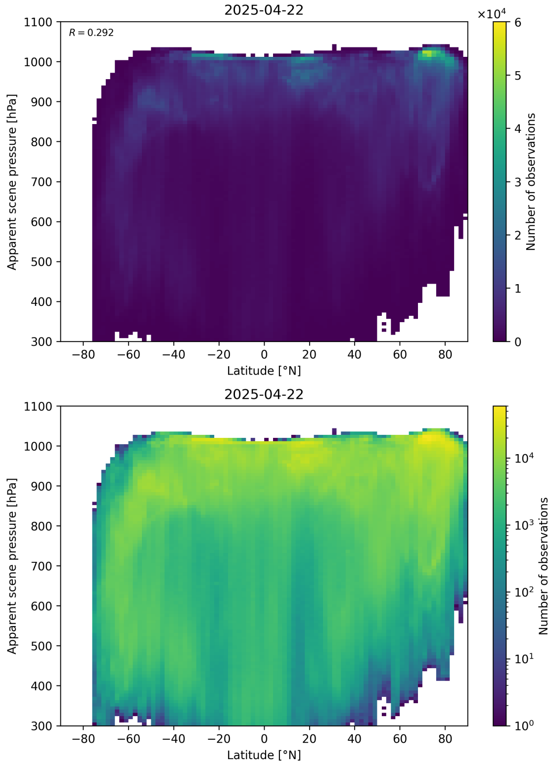
Figure 88: Scatter density plot of “Latitude” against “Apparent scene pressure” for 2025-04-21 to 2025-04-23.
