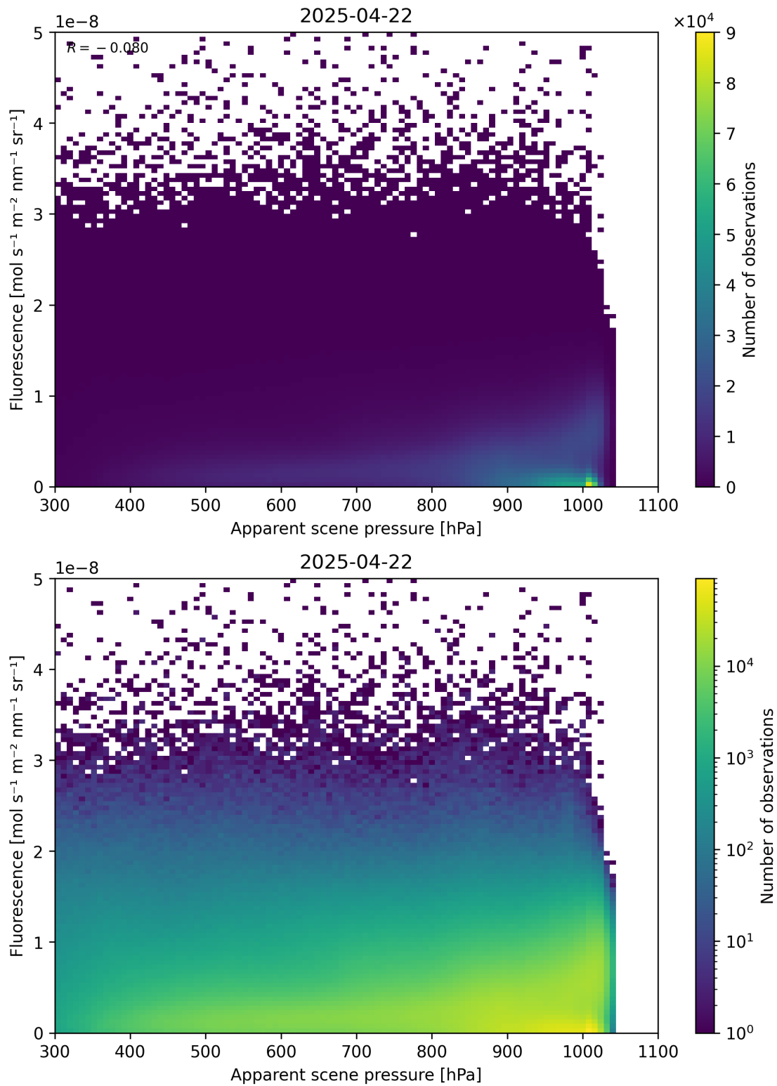
Figure 64: Scatter density plot of “Apparent scene pressure” against “Fluorescence” for 2025-04-21 to 2025-04-23.
