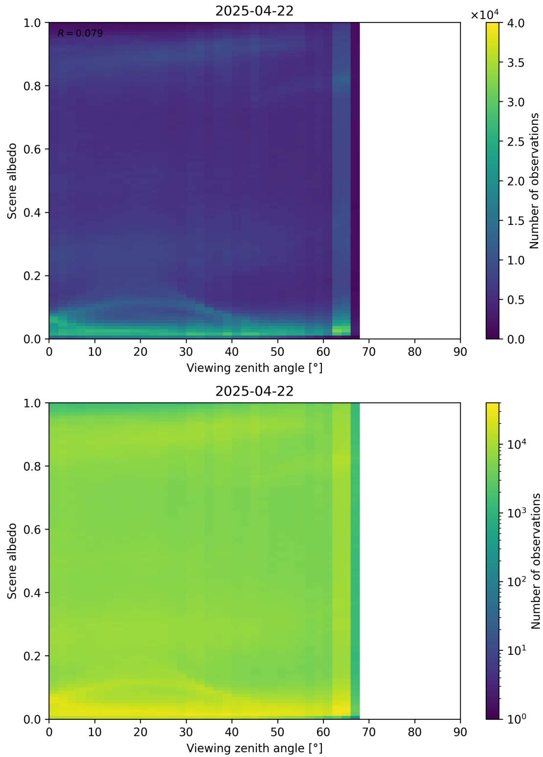
Figure 126: Scatter density plot of “Viewing zenith angle” against “Scene albedo” for 2025-04-21 to 2025-04-23.
