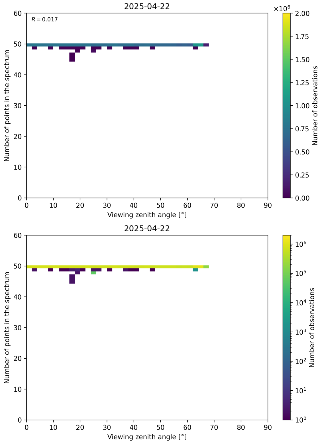
Figure 125: Scatter density plot of “Viewing zenith angle” against “Number of points in the spectrum” for 2025-04-21 to 2025-04-23.
