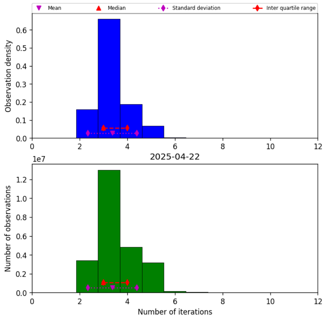
Figure 39: Histogram of “Number of iterations” for 2025-04-21 to 2025-04-23
