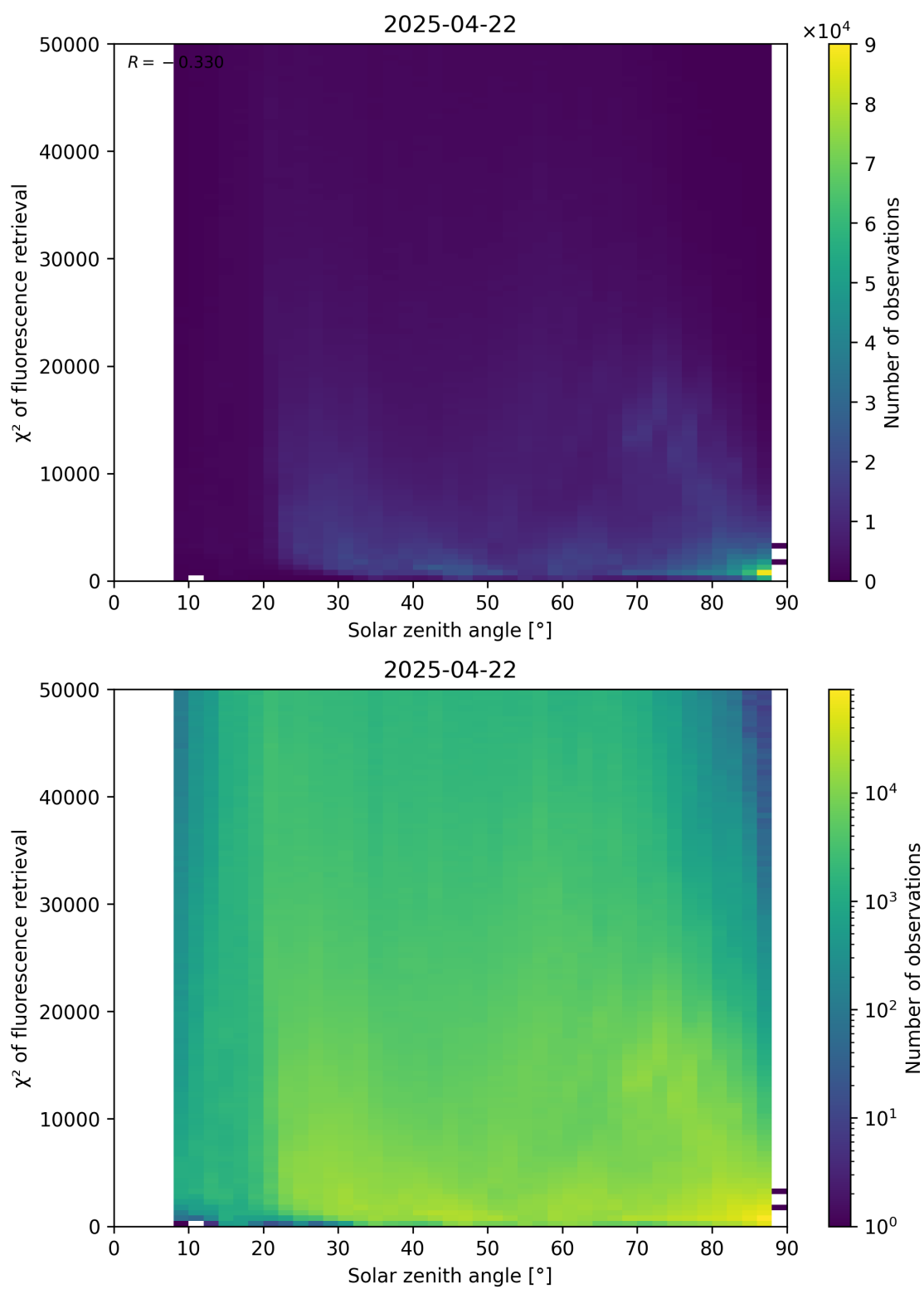
Figure 109: Scatter density plot of “Solar zenith angle” against “ \chi^2 of fluorescence retrieval” for 2025-04-21 to 2025-04-23.
