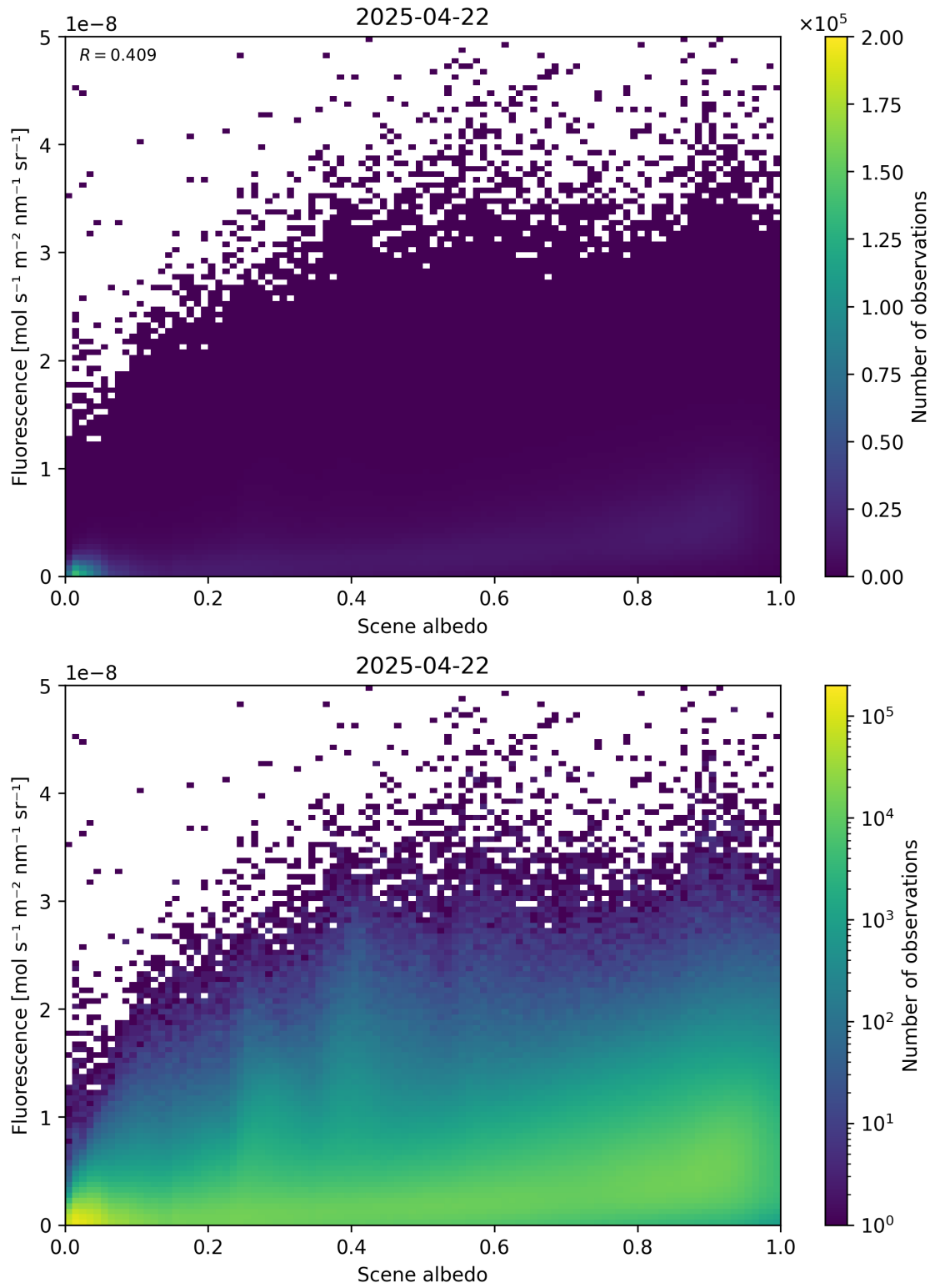
Figure 104: Scatter density plot of “Scene albedo” against “Fluorescence” for 2025-04-21 to 2025-04-23.
