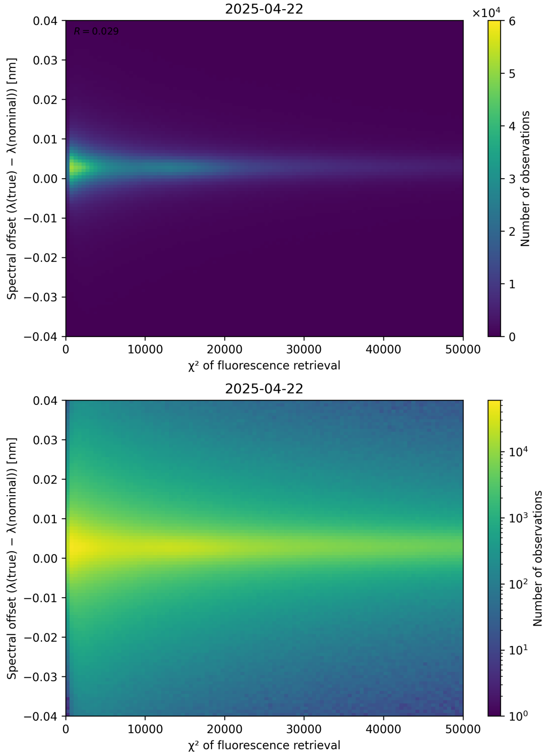
Figure 69: Scatter density plot of “ \chi^2 of fluorescence retrieval” against “Spectral offset ( \lambda_{\text{true}} - \lambda_{\text{nominal}} )” for 2025-04-21 to 2025-04-23.
