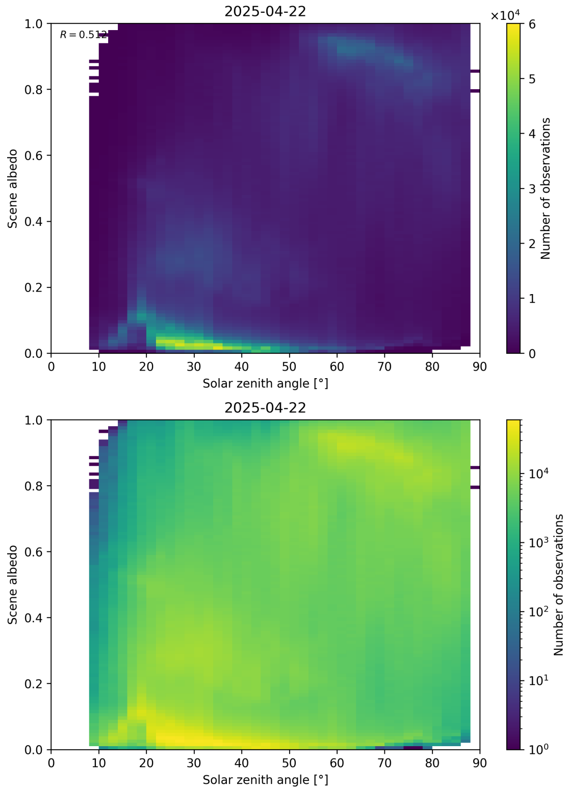
Figure 116: Scatter density plot of “Solar zenith angle” against “Scene albedo” for 2025-04-21 to 2025-04-23.
