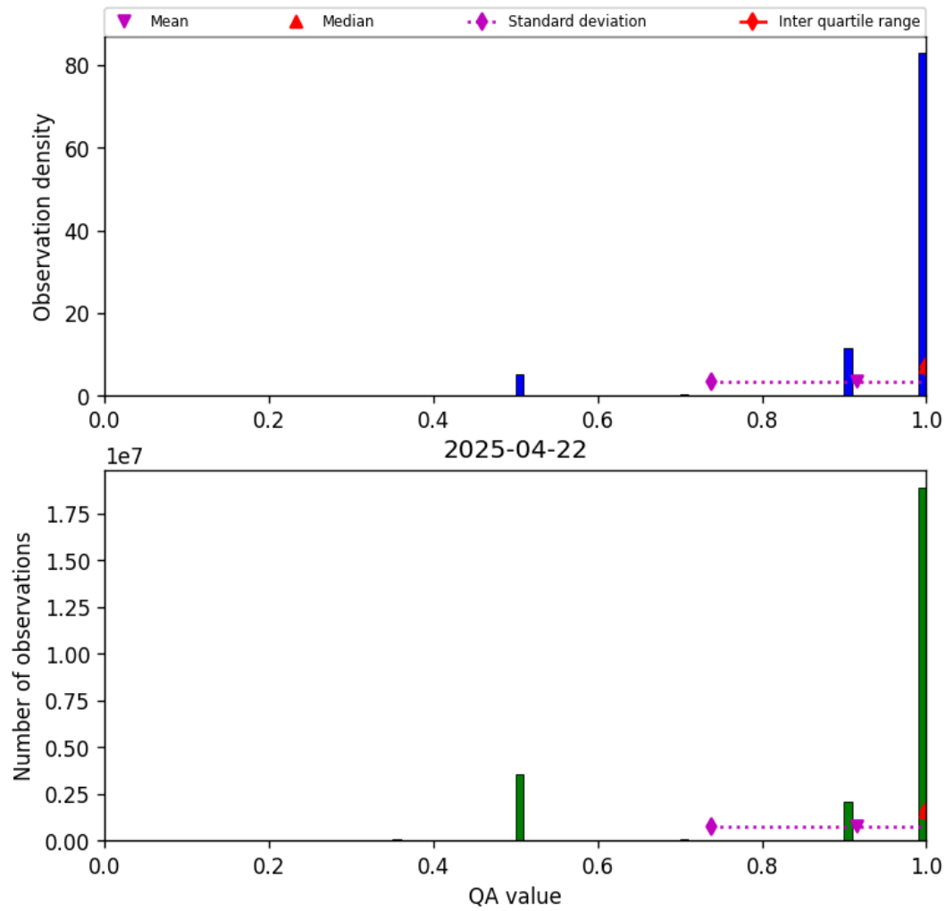
Figure 29: Histogram of “QA value” for 2025-04-21 to 2025-04-23
