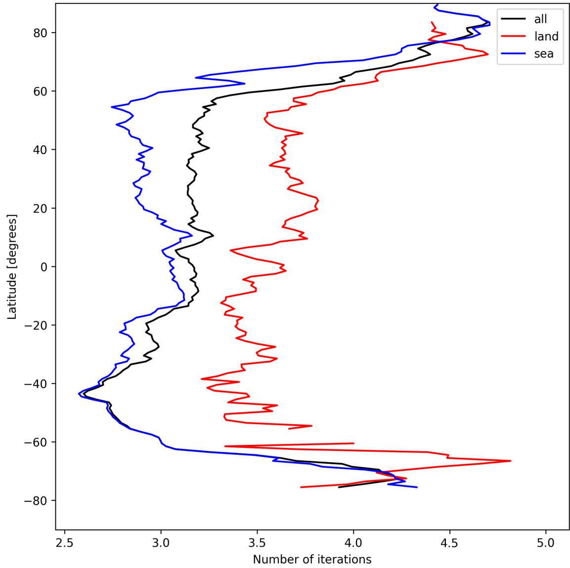
Figure 22: Zonal average of “Number of iterations” for 2025-04-21 to 2025-04-23.
