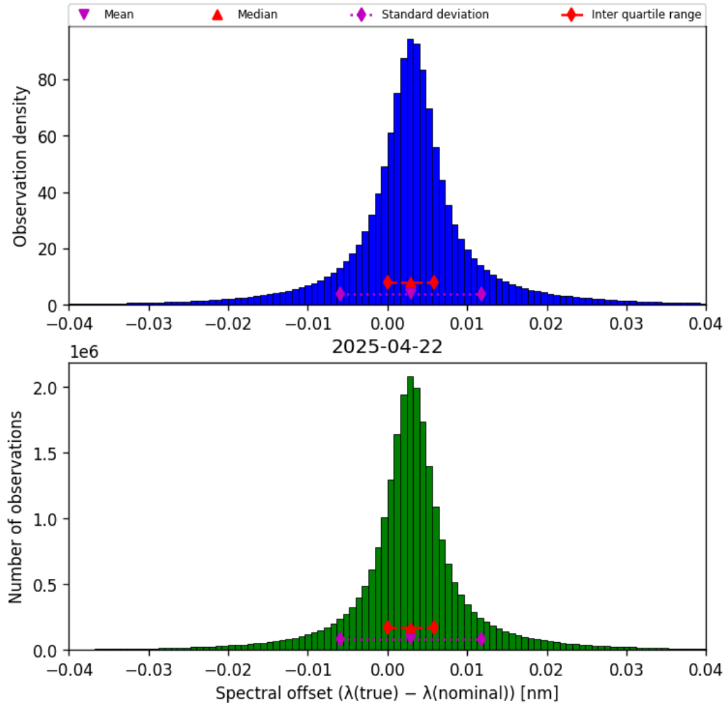
Figure 45: Histogram of “Spectral offset ( \lambda_{\text{true}} - \lambda_{\text{nominal}} )” for 2025-04-21 to 2025-04-23
