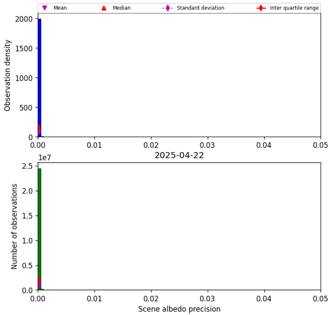
Figure 35: Histogram of “Scene albedo precision” for 2025-04-21 to 2025-04-23
