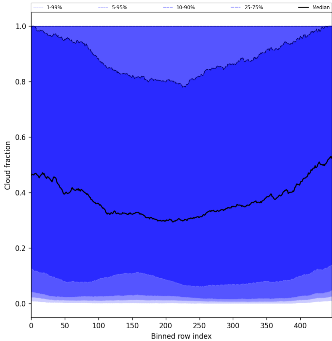
Figure 49: Along track statistics of “Cloud fraction” for 2025-04-21 to 2025-04-23
