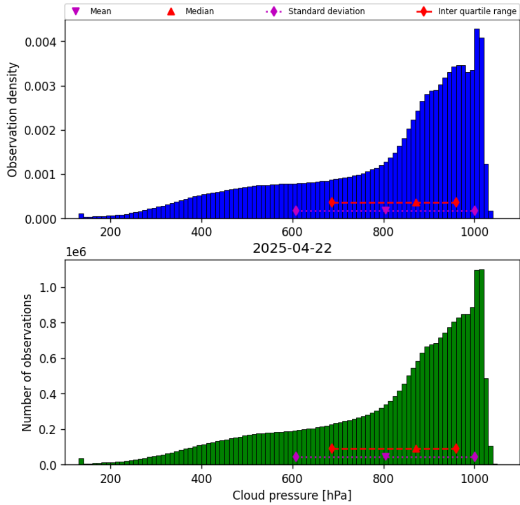
Figure 30: Histogram of “Cloud pressure” for 2025-04-21 to 2025-04-23
