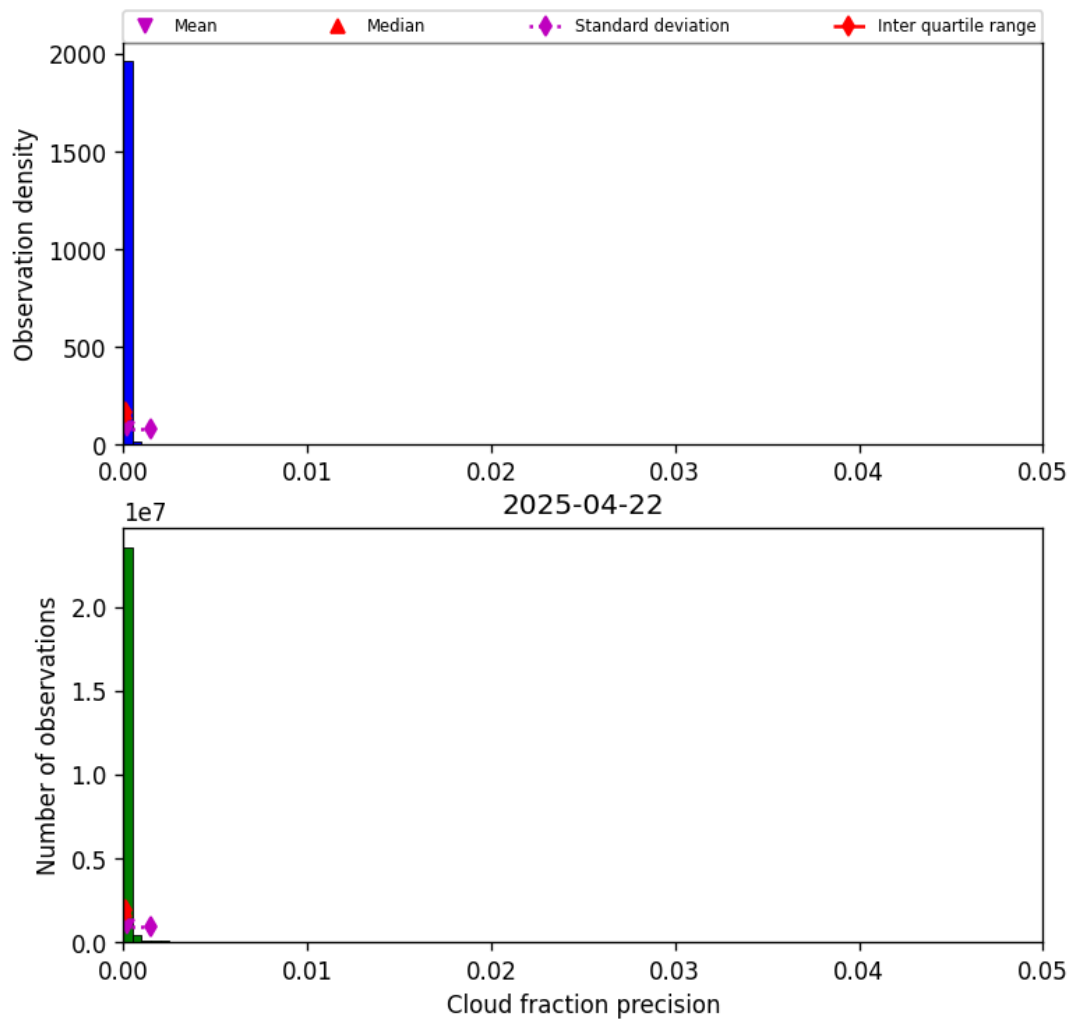
Figure 33: Histogram of “Cloud fraction precision” for 2025-04-21 to 2025-04-23
