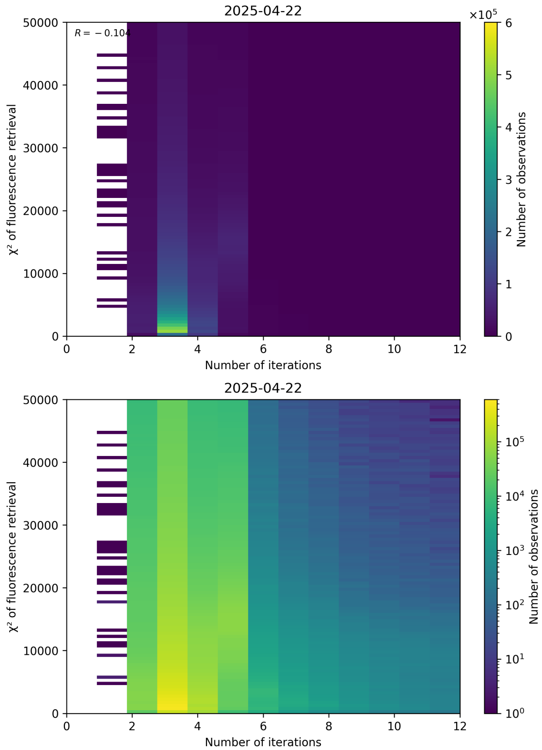
Figure 97: Scatter density plot of “Number of iterations” against “ \chi^2 of fluorescence retrieval” for 2025-04-21 to 2025-04-23.
