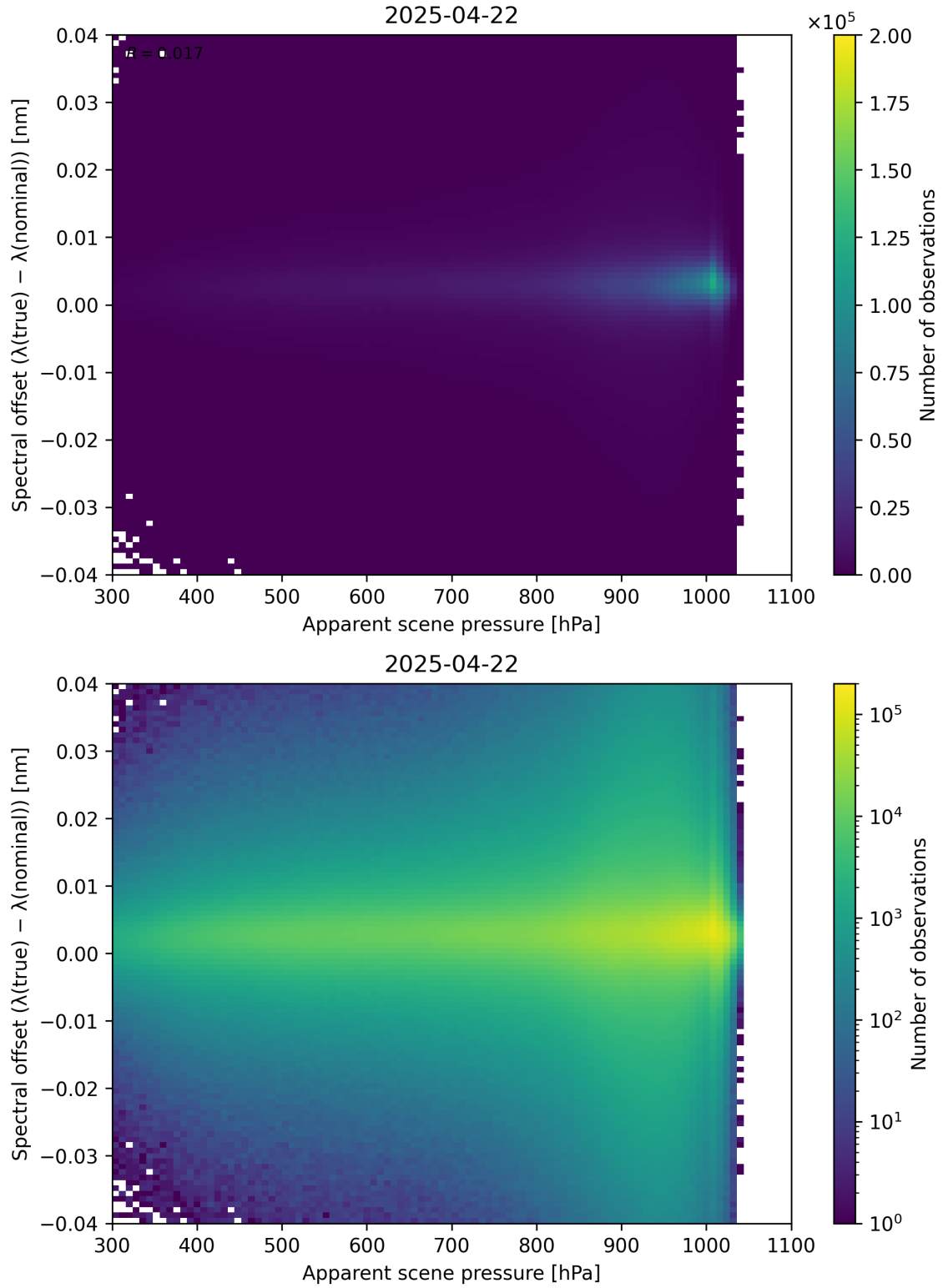
Figure 67: Scatter density plot of “Apparent scene pressure” against “Spectral offset ( \lambda_{\text{true}} - \lambda_{\text{nominal}} )” for 2025-04-21 to 2025-04-23.
