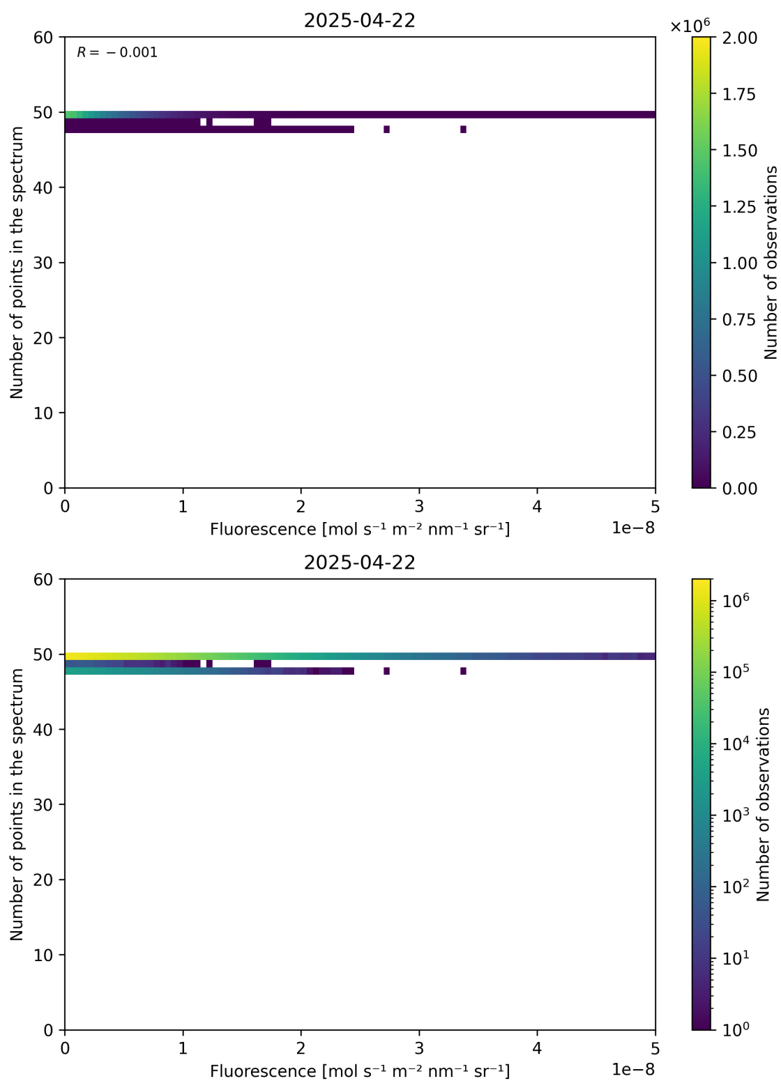
Figure 86: Scatter density plot of “Fluorescence” against “Number of points in the spectrum” for 2025-04-21 to 2025-04-23.
