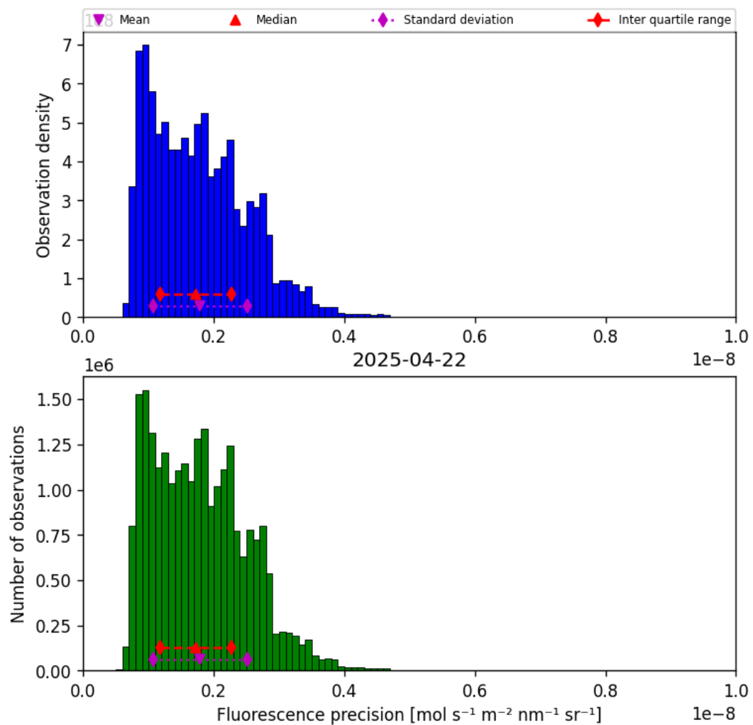
Figure 41: Histogram of “Fluorescence precision” for 2025-04-21 to 2025-04-23
