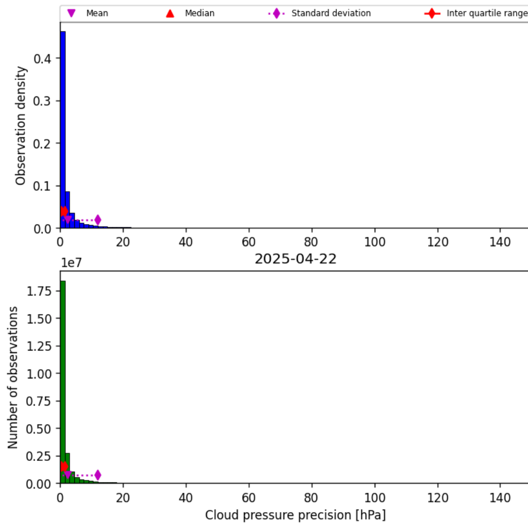
Figure 31: Histogram of “Cloud pressure precision” for 2025-04-21 to 2025-04-23
