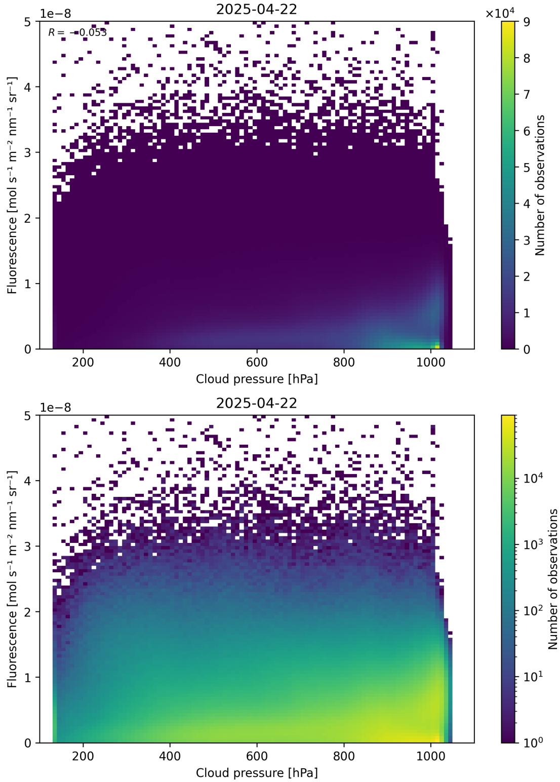
Figure 80: Scatter density plot of “Cloud pressure” against “Fluorescence” for 2025-04-21 to 2025-04-23.
