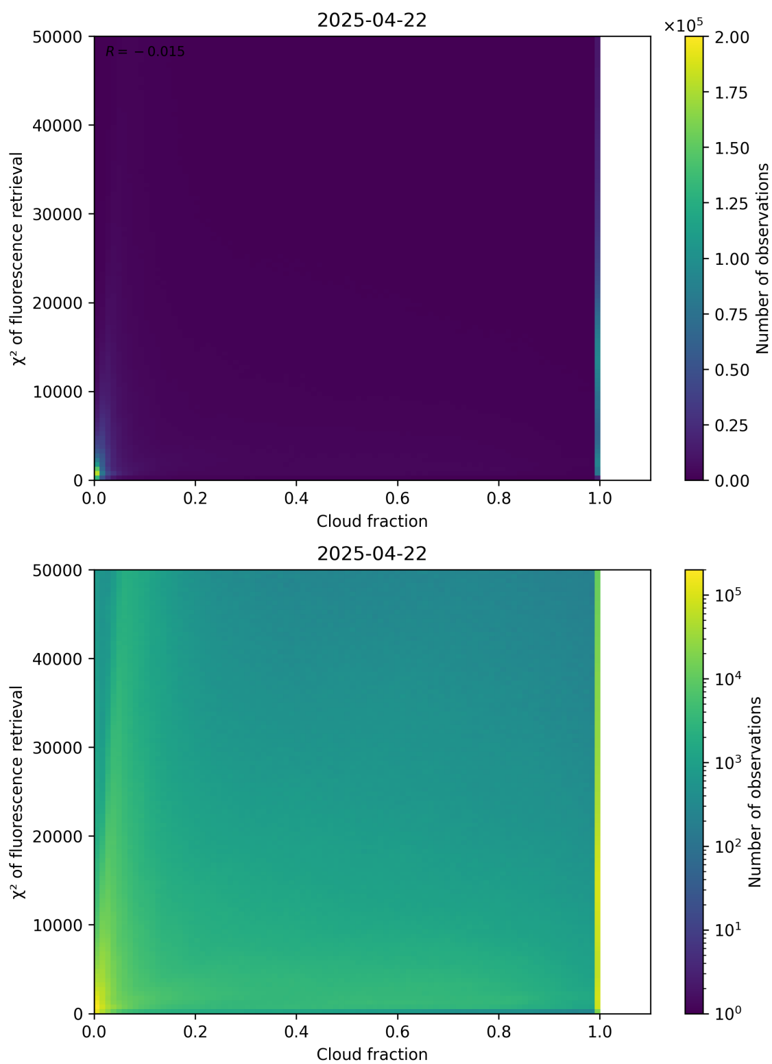
Figure 71: Scatter density plot of “Cloud fraction” against “ \chi^2 of fluorescence retrieval” for 2025-04-21 to 2025-04-23.
