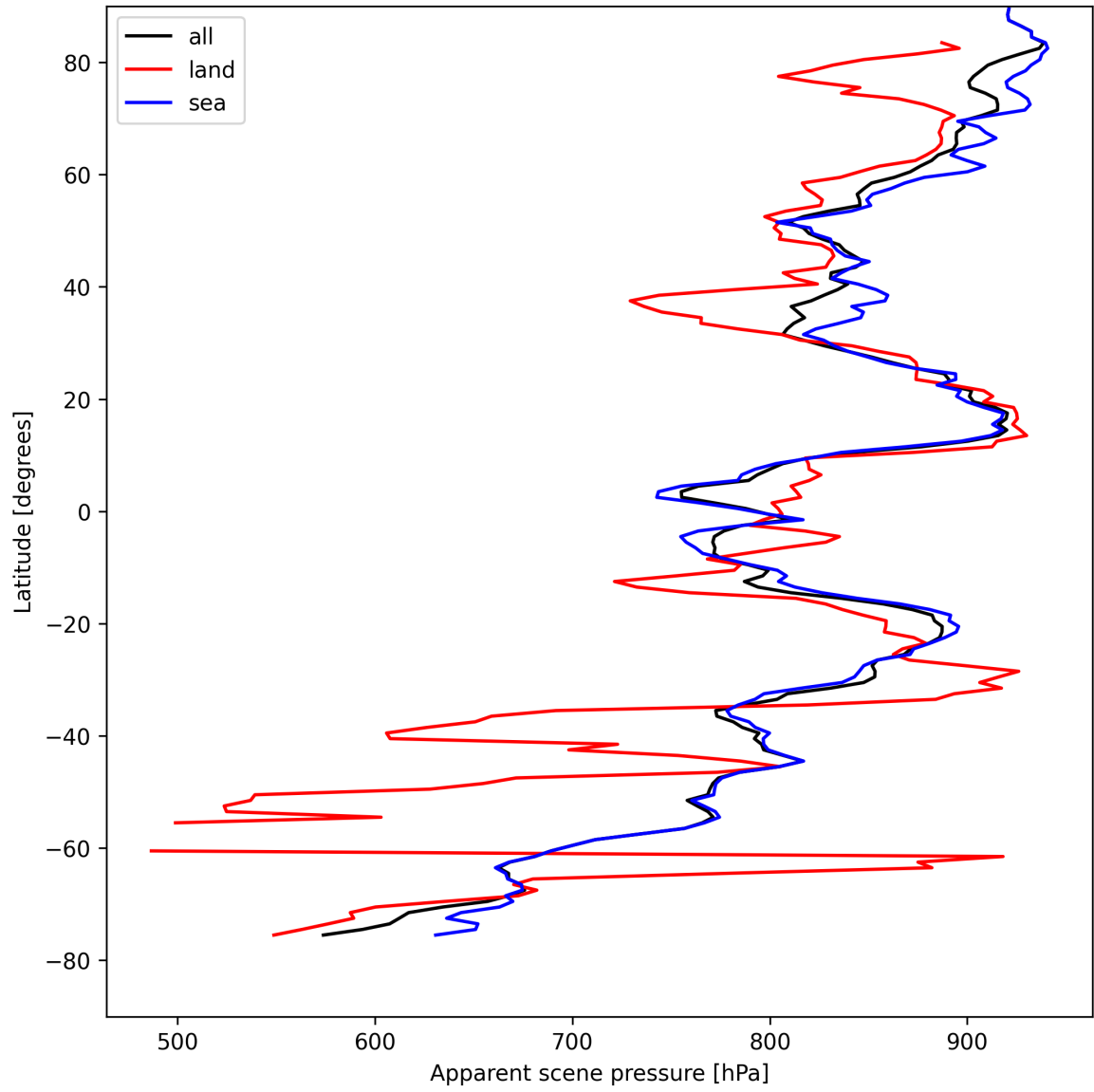
Figure 19: Zonal average of “Apparent scene pressure” for 2025-04-21 to 2025-04-23.
