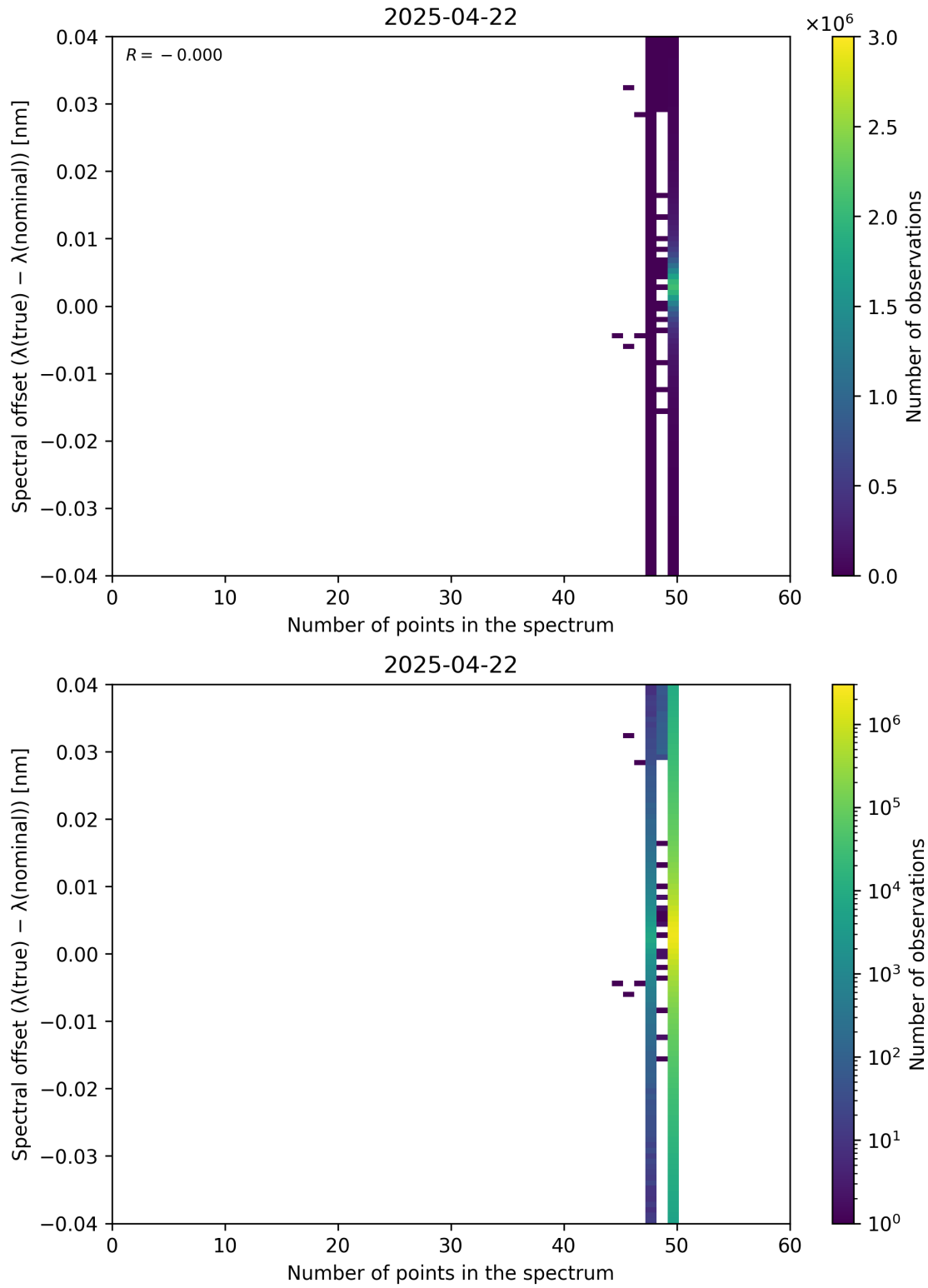
Figure 101: Scatter density plot of “Number of points in the spectrum” against “Spectral offset ( \lambda_{\text{true}} - \lambda_{\text{nominal}} )” for 2025-04-21 to 2025-04-23.
