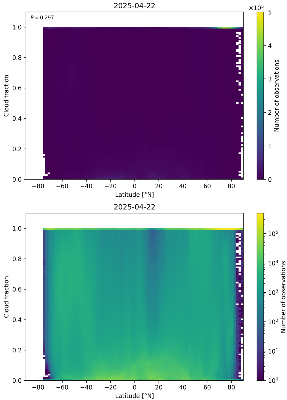
Figure 90: Scatter density plot of “Latitude” against “Cloud fraction” for 2025-04-21 to 2025-04-23.
