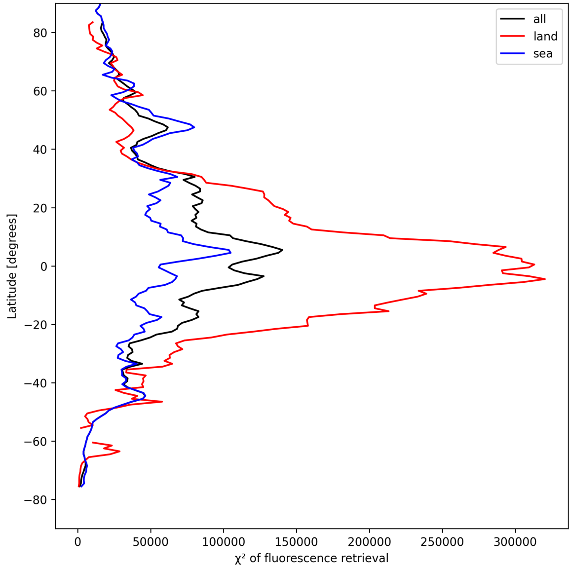
Figure 25: Zonal average of “ \chi^2 of fluorescence retrieval” for 2025-04-21 to 2025-04-23.
