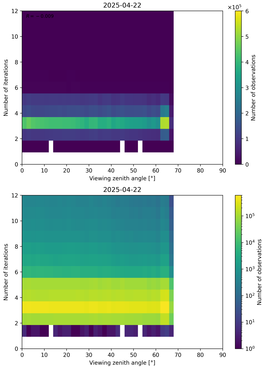
Figure 124: Scatter density plot of “Viewing zenith angle” against “Number of iterations” for 2025-04-21 to 2025-04-23.
