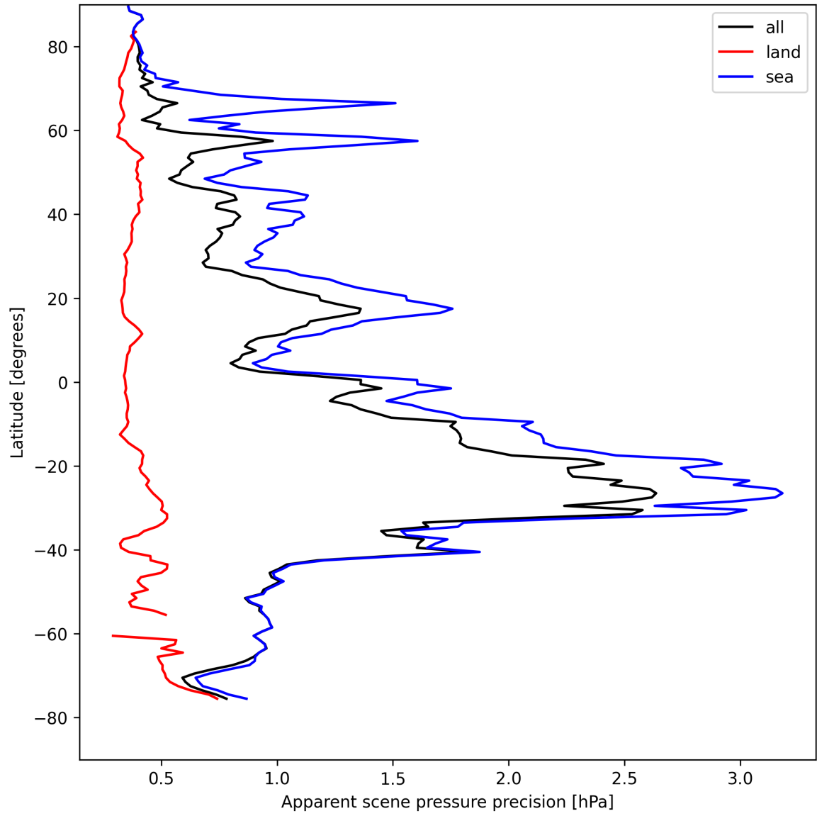
Figure 20: Zonal average of “Apparent scene pressure precision” for 2025-04-21 to 2025-04-23.
