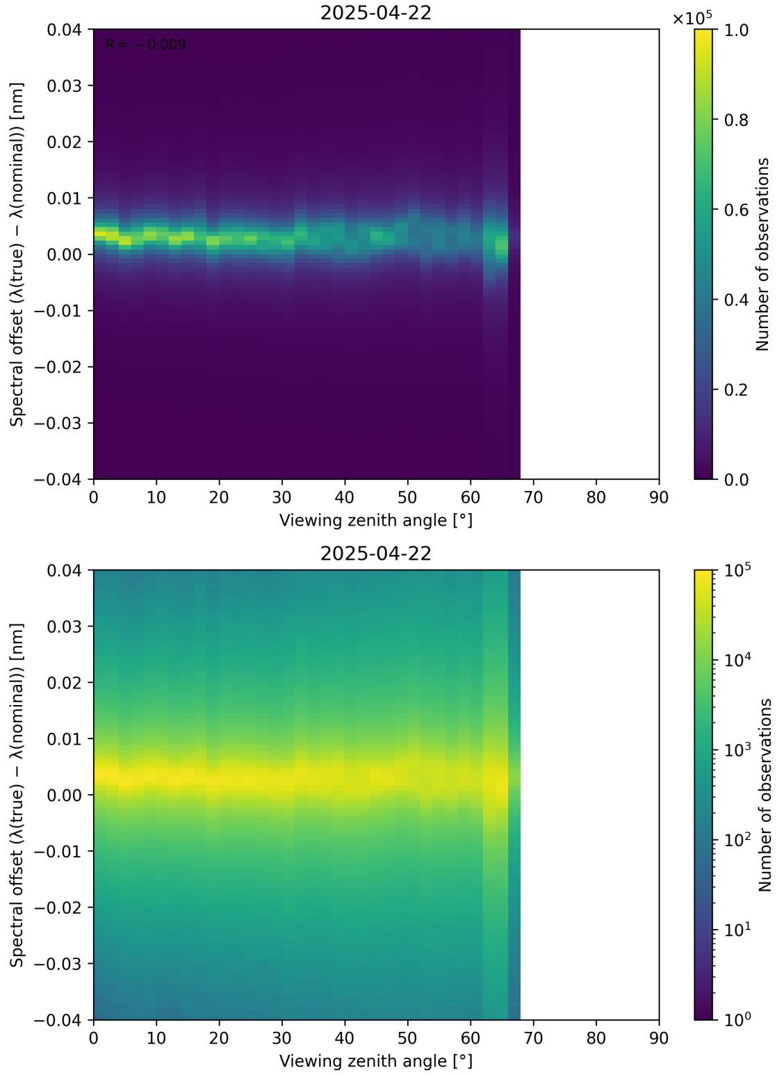
Figure 128: Scatter density plot of “Viewing zenith angle” against “Spectral offset ( \lambda_{\text{true}} - \lambda_{\text{nominal}} )” for 2025-04-21 to 2025-04-23.
