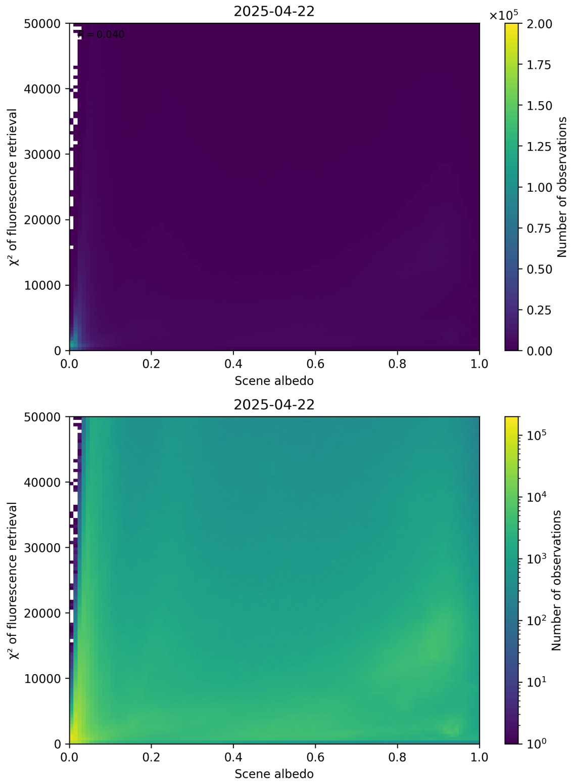
Figure 103: Scatter density plot of “Scene albedo” against “ \chi^2 of fluorescence retrieval” for 2025-04-21 to 2025-04-23.
