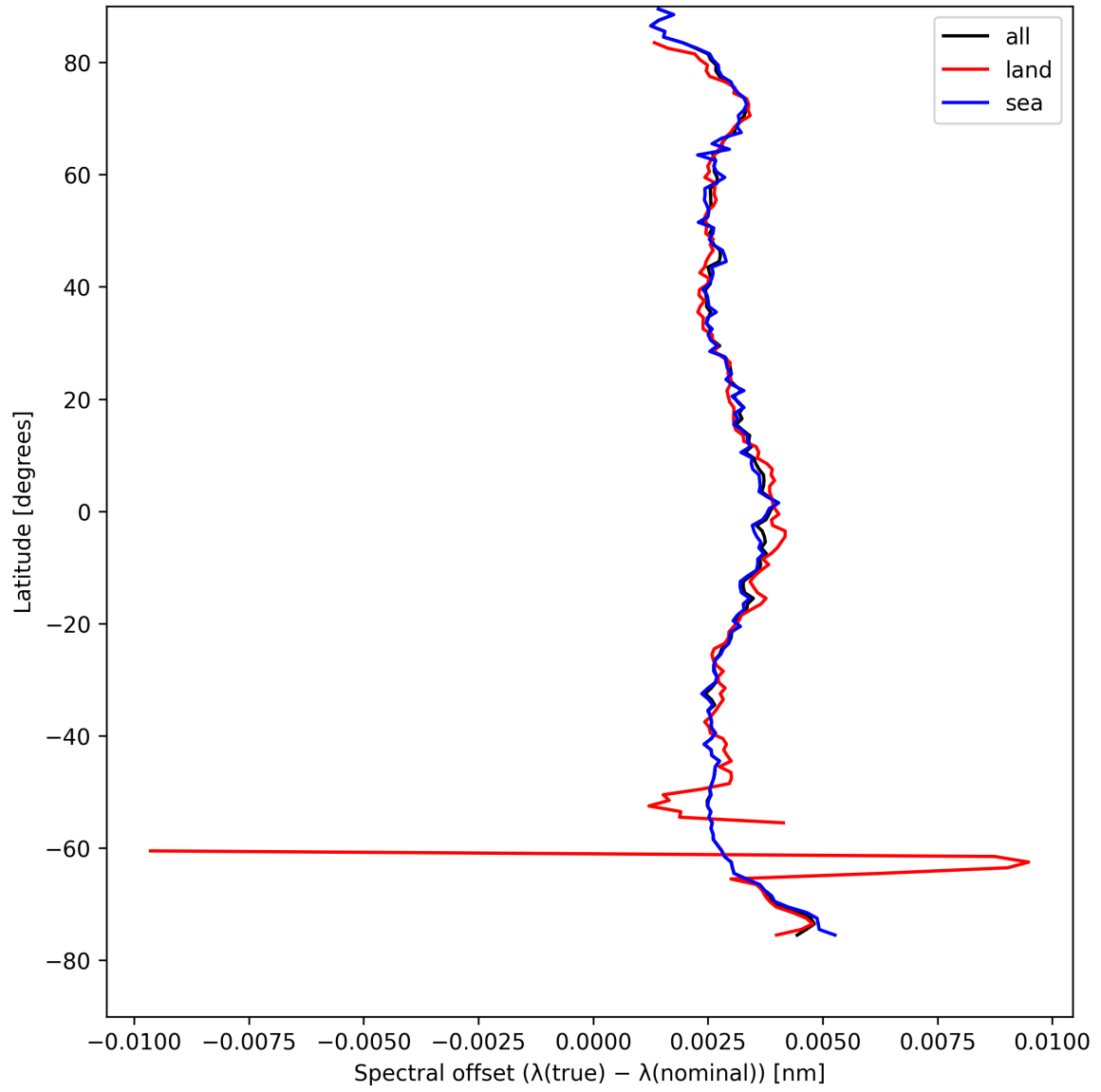
Figure 28: Zonal average of “Spectral offset ( \lambda_{\text{true}} - \lambda_{\text{nominal}} )” for 2025-04-21 to 2025-04-23.
