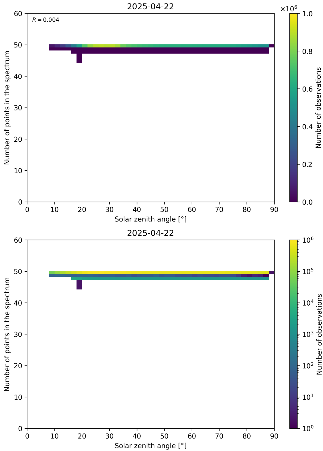
Figure 115: Scatter density plot of “Solar zenith angle” against “Number of points in the spectrum” for 2025-04-21 to 2025-04-23.
