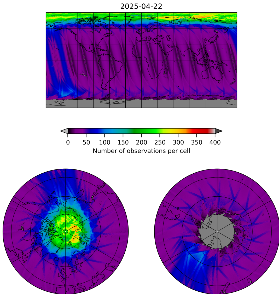
Figure 11: Map of the number of observations for 2025-04-21 to 2025-04-23
