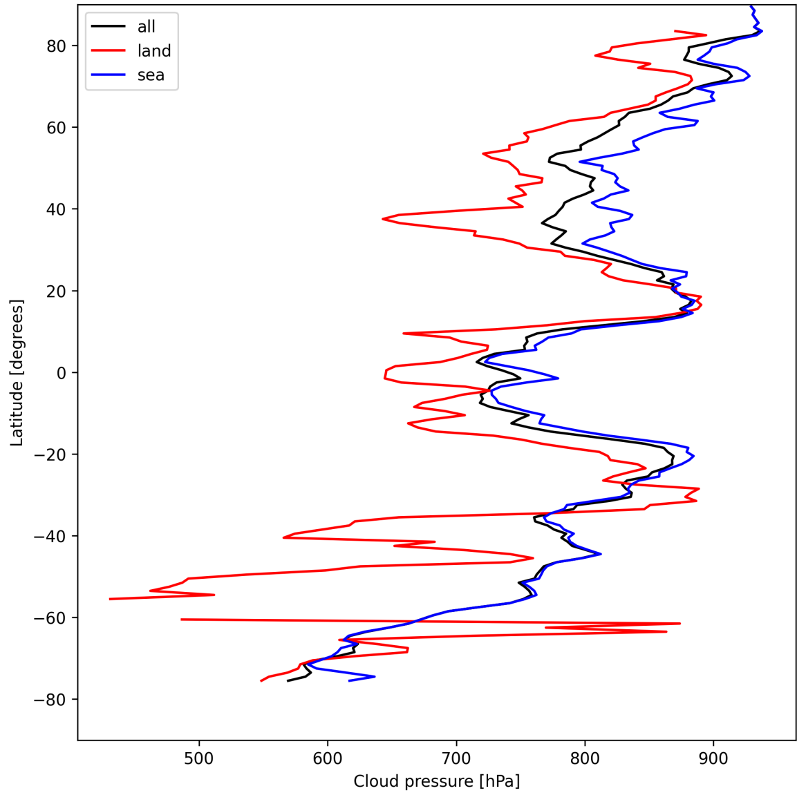
Figure 13: Zonal average of “Cloud pressure” for 2025-04-21 to 2025-04-23.
