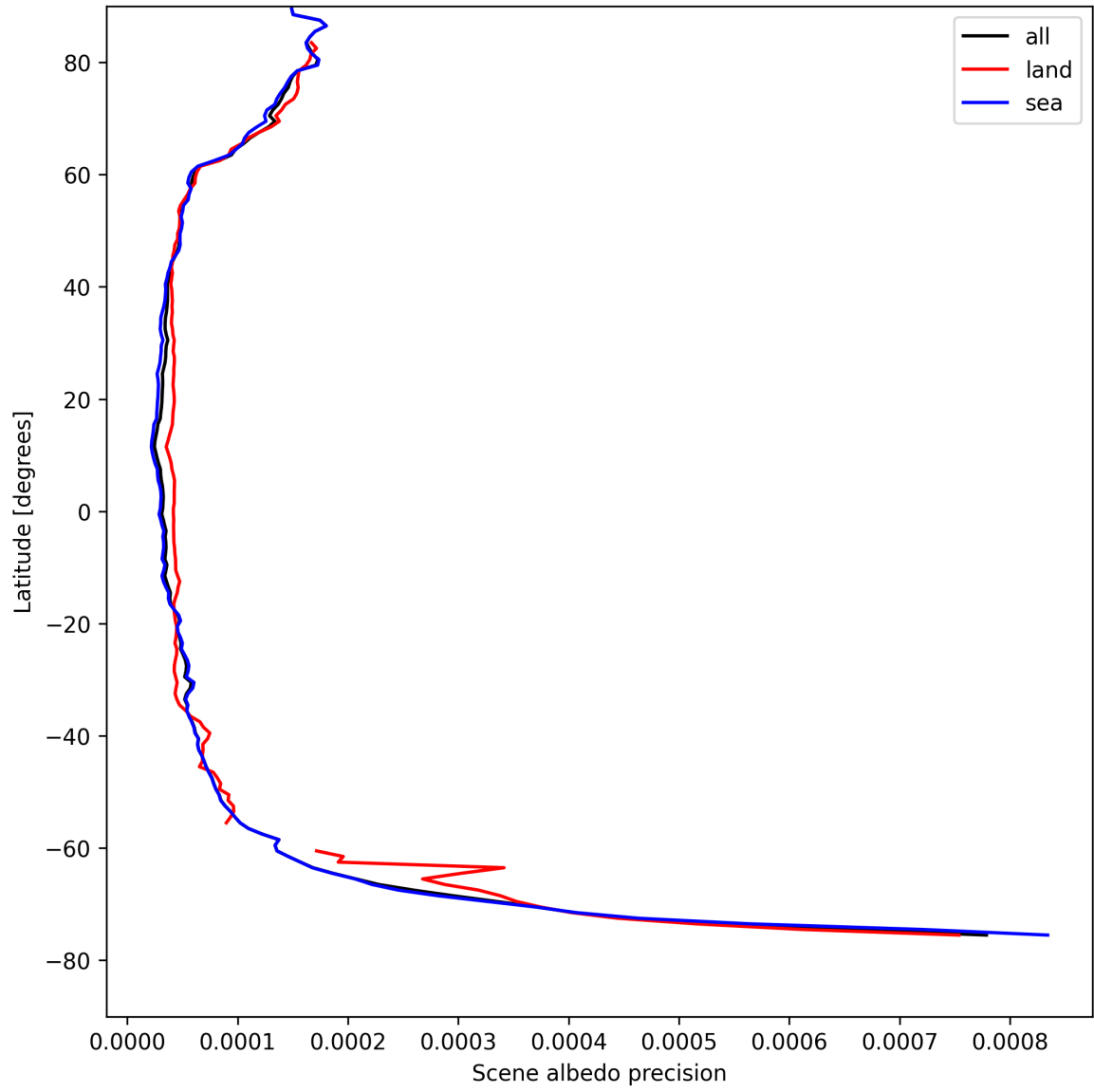
Figure 18: Zonal average of “Scene albedo precision” for 2025-04-21 to 2025-04-23.
