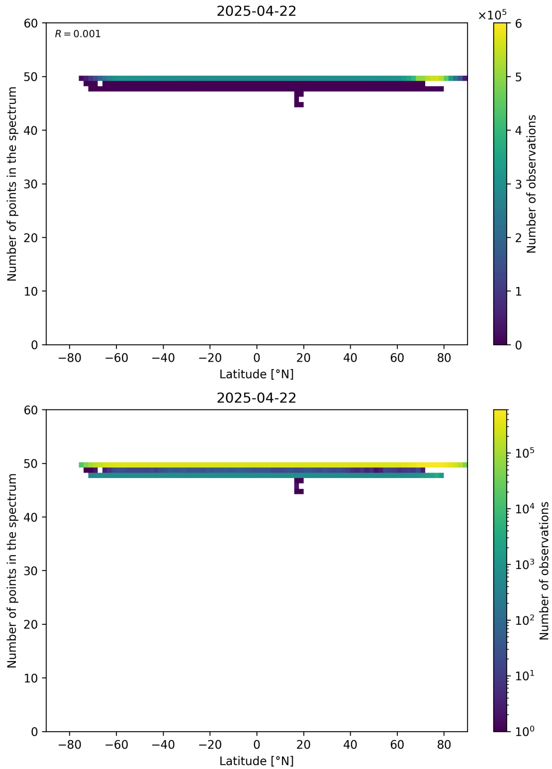
Figure 94: Scatter density plot of “Latitude” against “Number of points in the spectrum” for 2025-04-21 to 2025-04-23.
