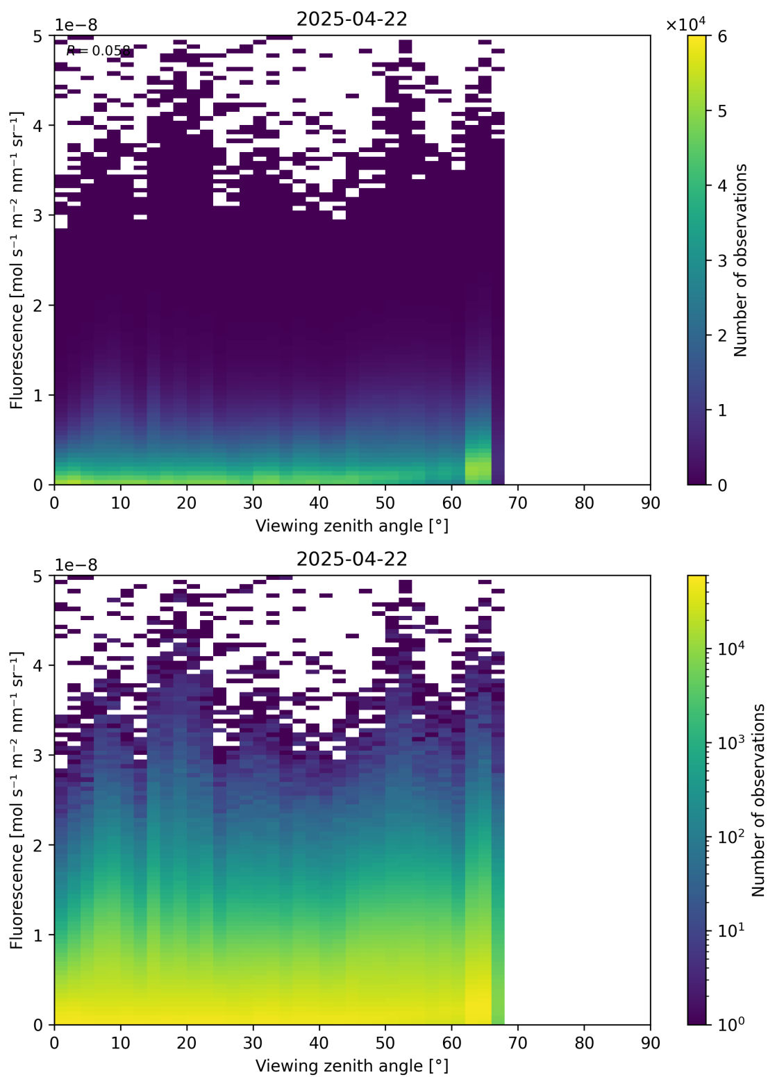
Figure 122: Scatter density plot of “Viewing zenith angle” against “Fluorescence” for 2025-04-21 to 2025-04-23.
