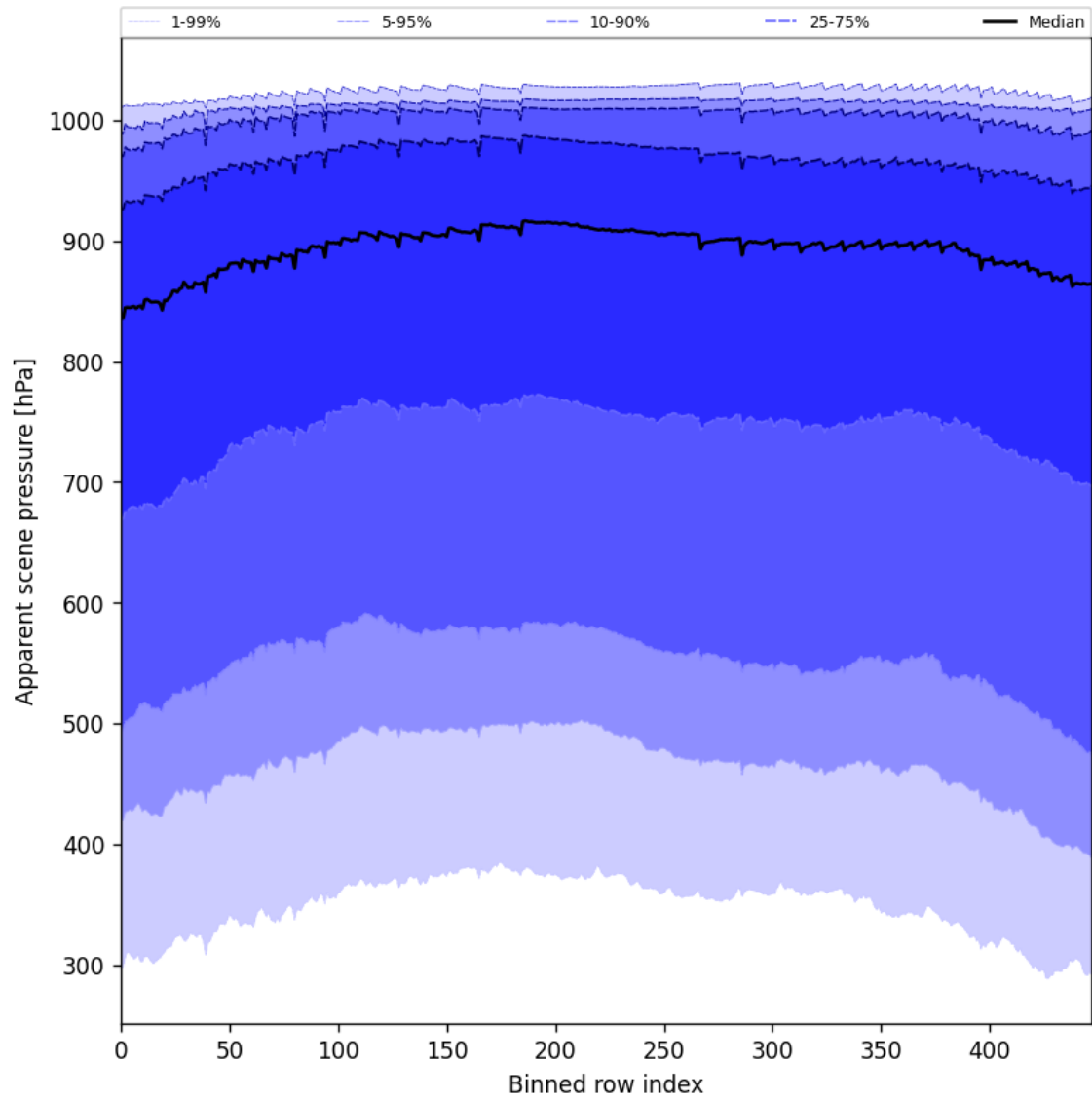
Figure 53: Along track statistics of “Apparent scene pressure” for 2025-04-21 to 2025-04-23
