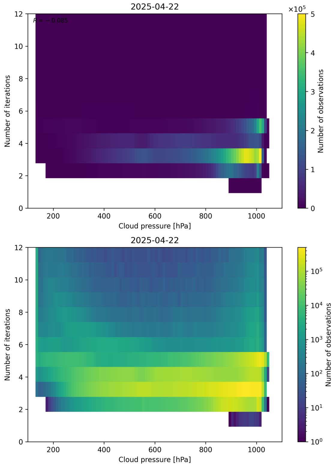
Figure 81: Scatter density plot of “Cloud pressure” against “Number of iterations” for 2025-04-21 to 2025-04-23.
