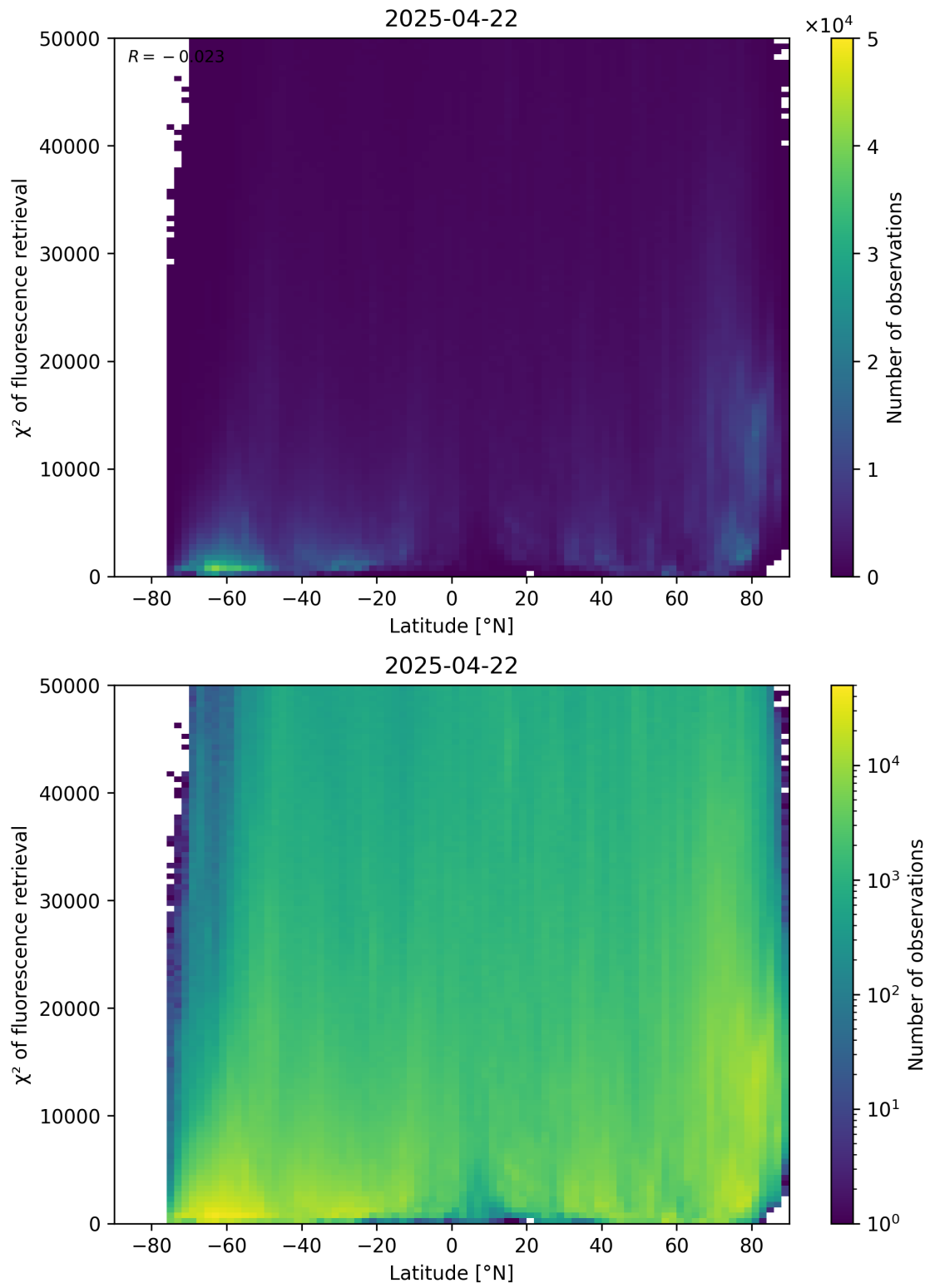
Figure 89: Scatter density plot of “Latitude” against “ \chi^2 of fluorescence retrieval” for 2025-04-21 to 2025-04-23.
