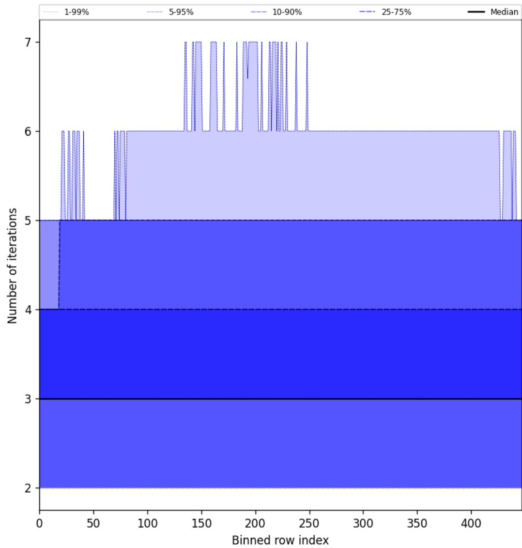
Figure 56: Along track statistics of “Number of iterations” for 2025-04-21 to 2025-04-23
