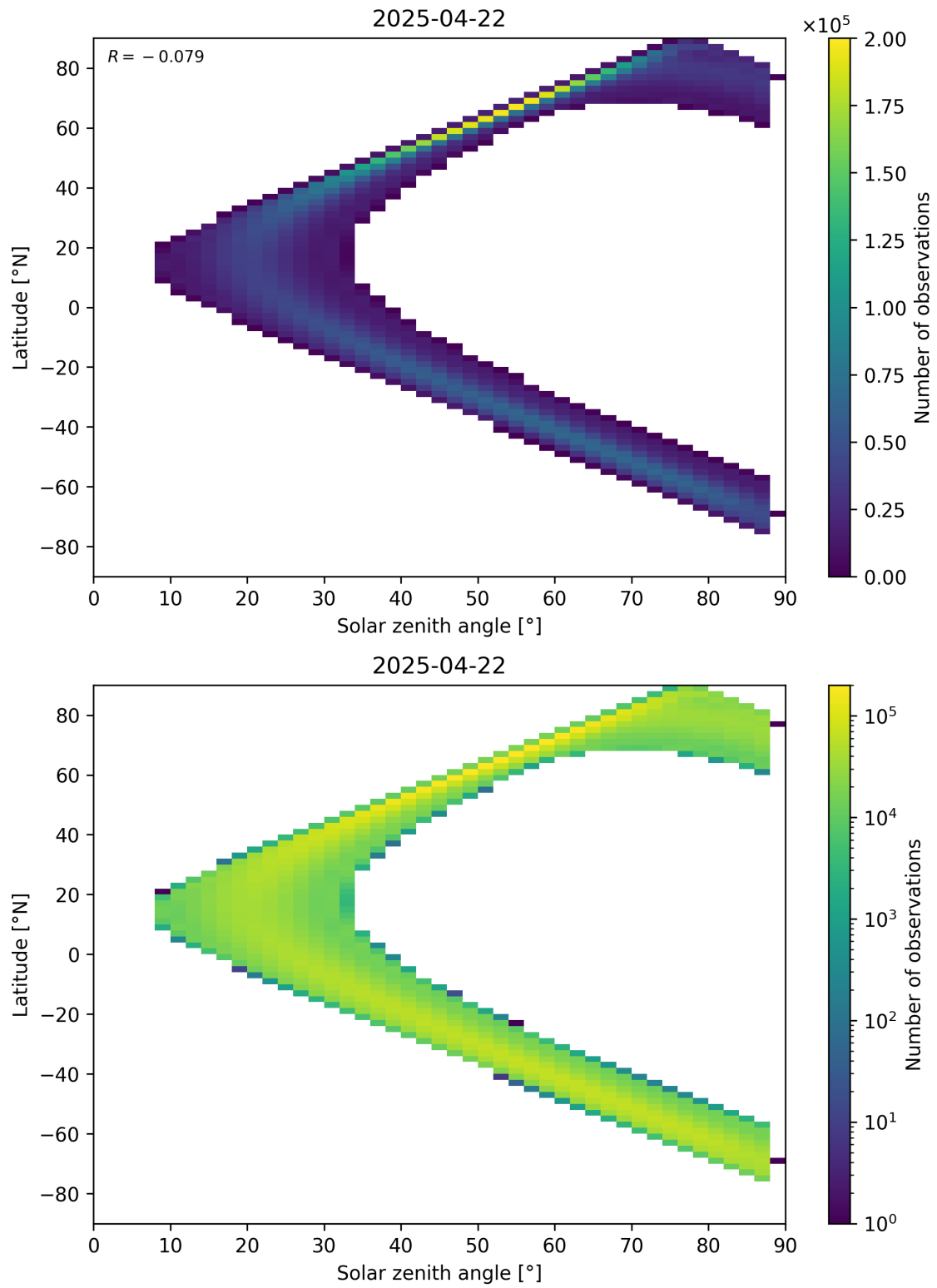
Figure 113: Scatter density plot of “Solar zenith angle” against “Latitude” for 2025-04-21 to 2025-04-23.
