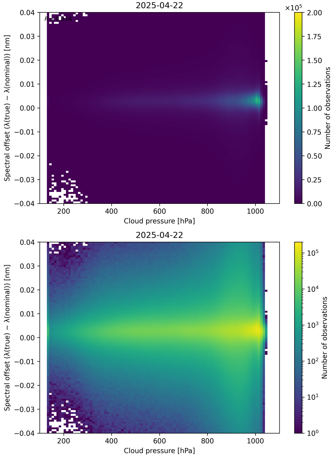
Figure 84: Scatter density plot of “Cloud pressure” against “Spectral offset ( \lambda_{\text{true}} - \lambda_{\text{nominal}} )” for 2025-04-21 to 2025-04-23.
