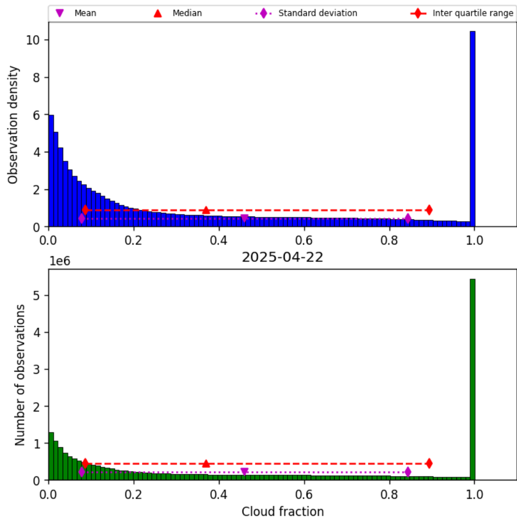
Figure 32: Histogram of “Cloud fraction” for 2025-04-21 to 2025-04-23
