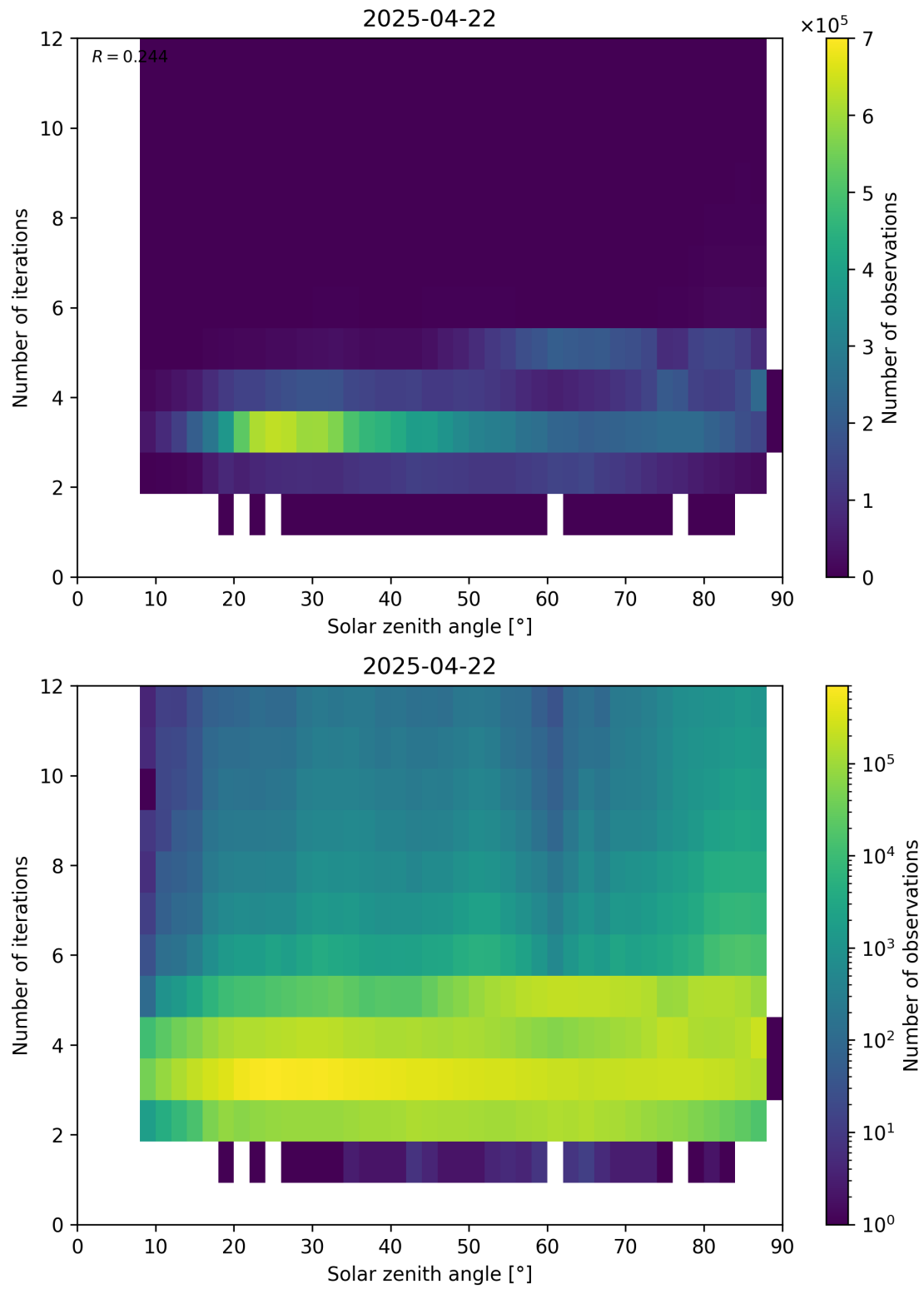
Figure 114: Scatter density plot of “Solar zenith angle” against “Number of iterations” for 2025-04-21 to 2025-04-23.
