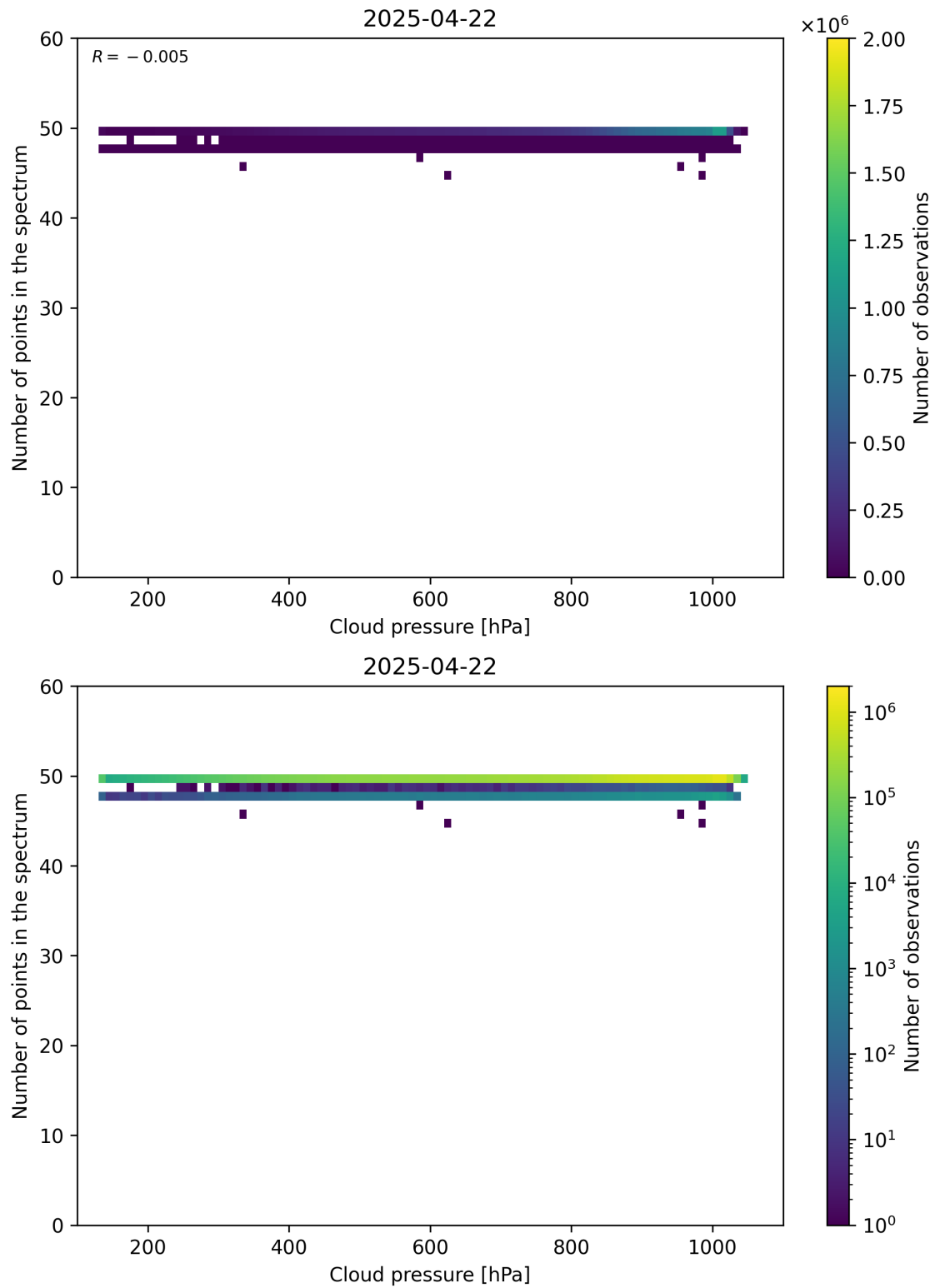
Figure 82: Scatter density plot of “Cloud pressure” against “Number of points in the spectrum” for 2025-04-21 to 2025-04-23.
