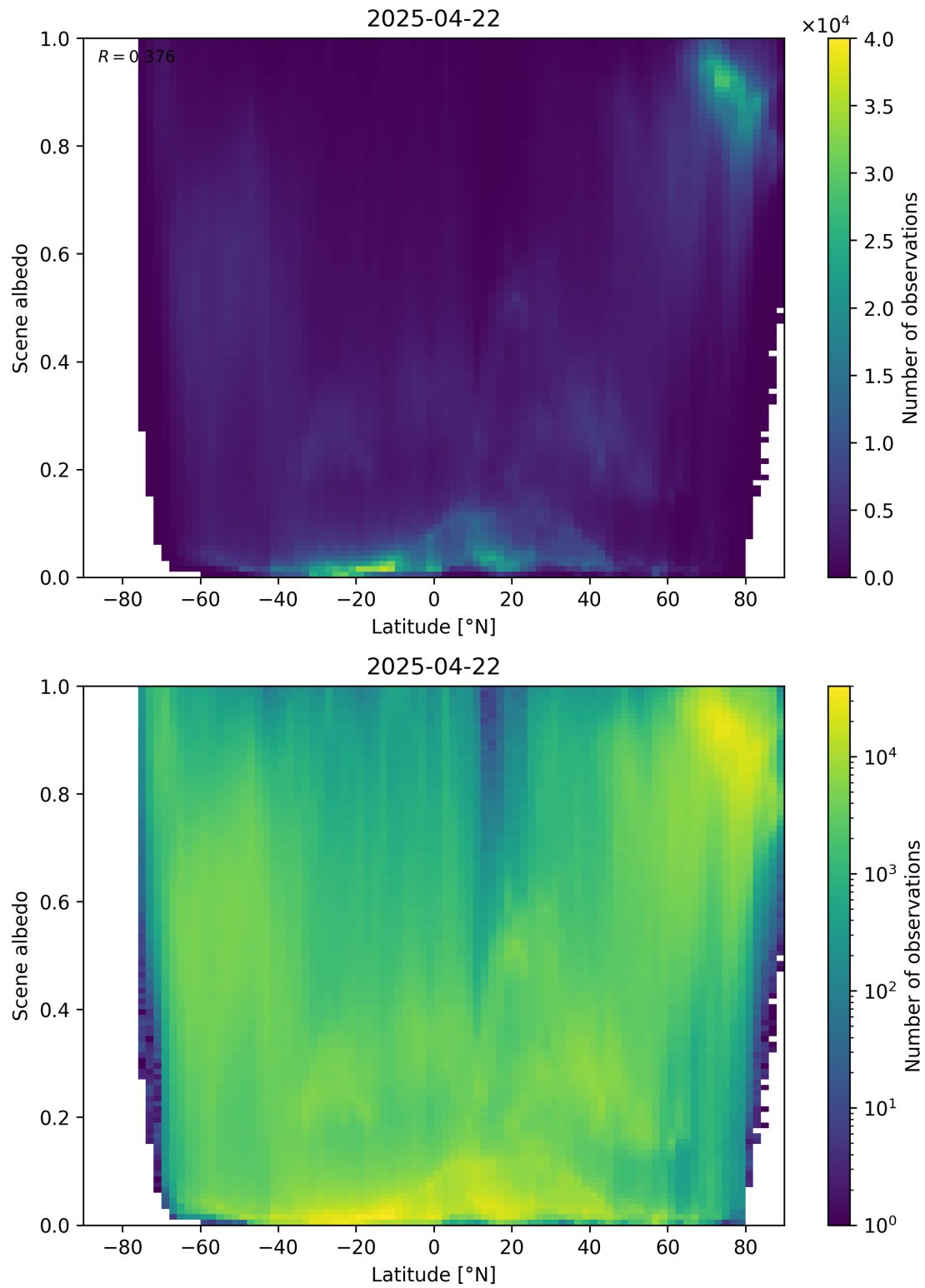
Figure 95: Scatter density plot of “Latitude” against “Scene albedo” for 2025-04-21 to 2025-04-23.
