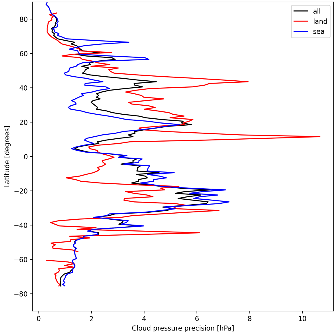
Figure 14: Zonal average of "Cloud pressure precision" for 2025-04-21 to 2025-04-23.
