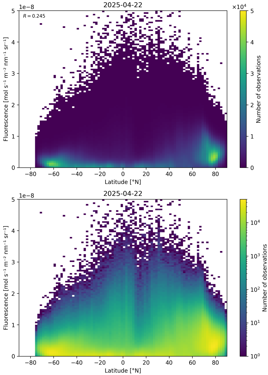
Figure 92: Scatter density plot of “Latitude” against “Fluorescence” for 2025-04-21 to 2025-04-23.
