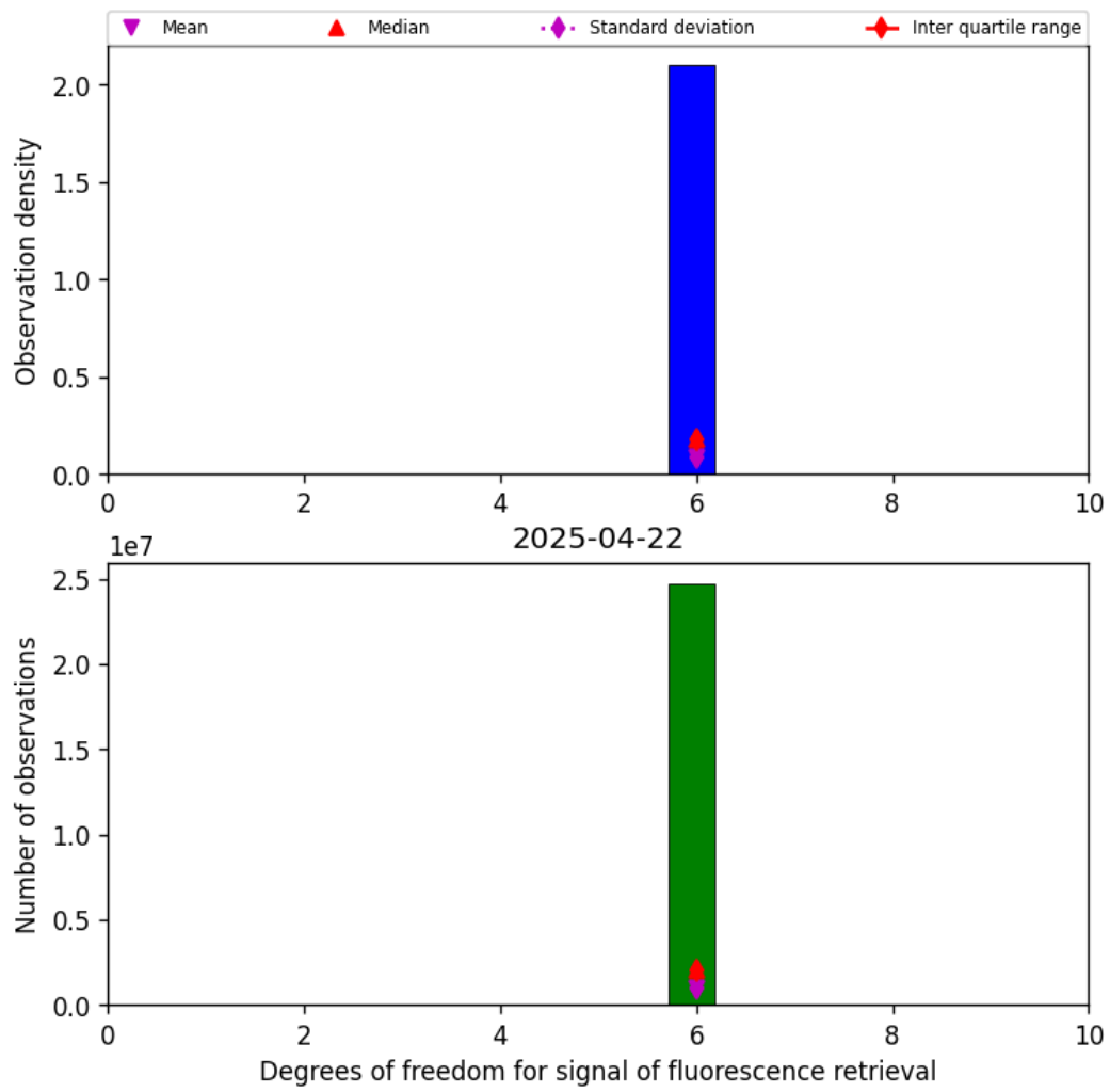
Figure 43: Histogram of "Degrees of freedom for signal of fluorescence retrieval" for 2025-04-21 to 2025-04-23
