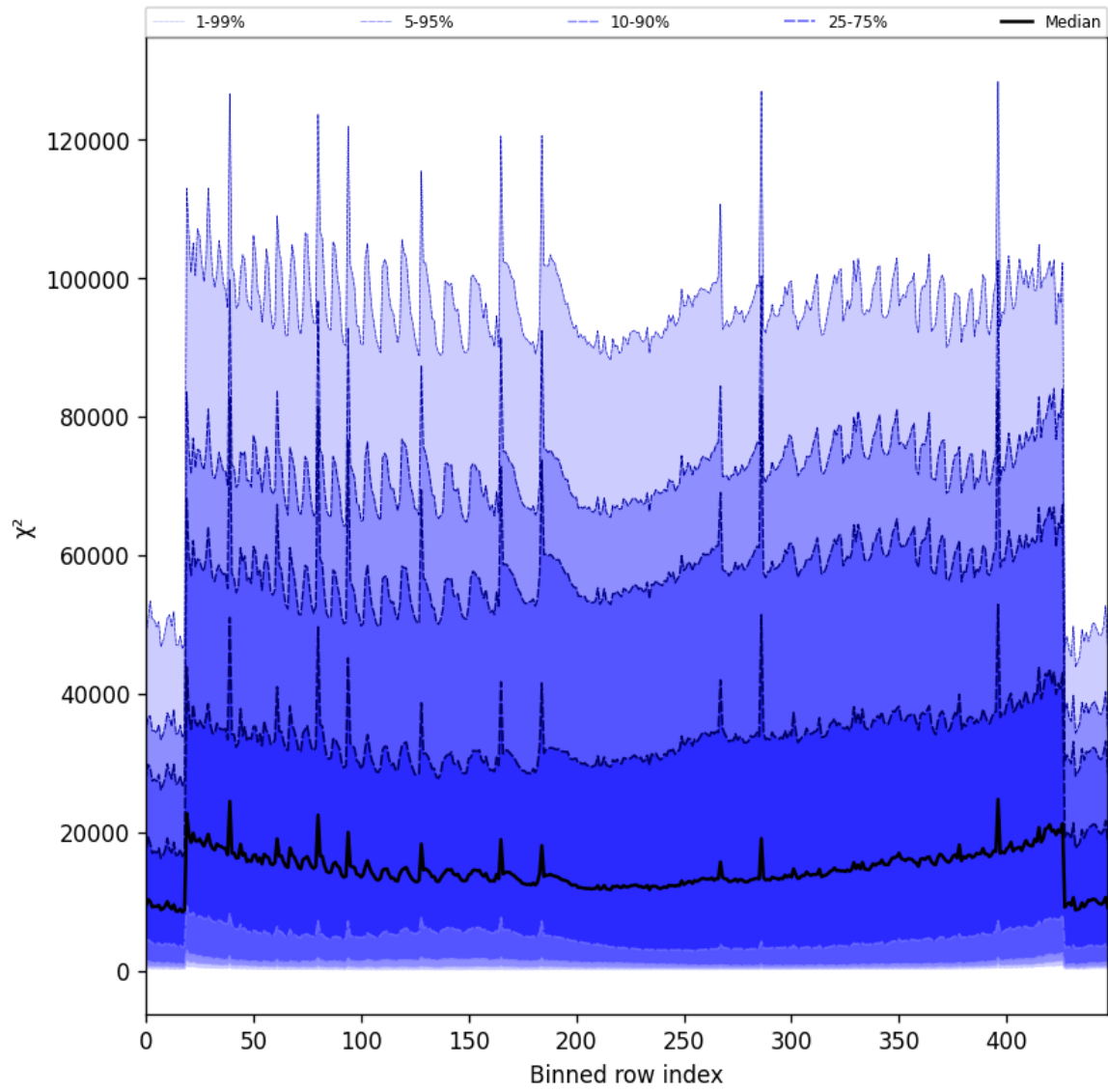
Figure 55: Along track statistics of “ \chi^2 ” for 2025-04-21 to 2025-04-23
