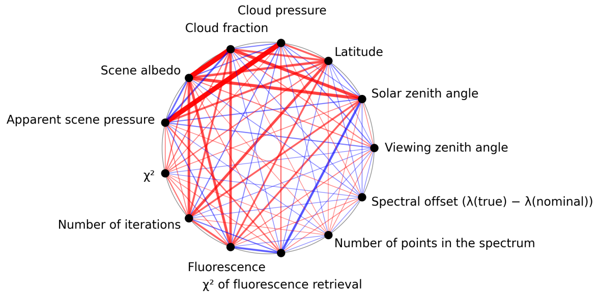
Figure 1: Map of correlation graph for 2025-04-21 to 2025-04-23.
