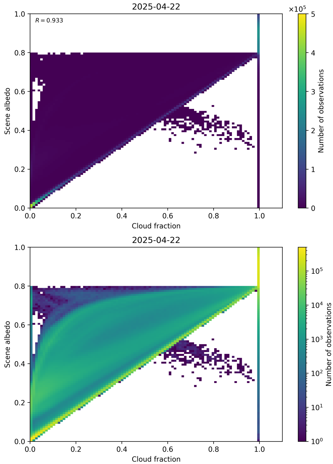
Figure 75: Scatter density plot of “Cloud fraction” against “Scene albedo” for 2025-04-21 to 2025-04-23.
