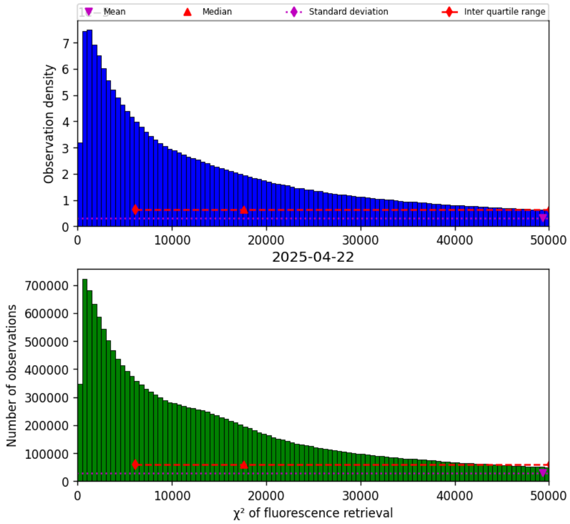
Figure 42: Histogram of “ \chi^2 of fluorescence retrieval” for 2025-04-21 to 2025-04-23
