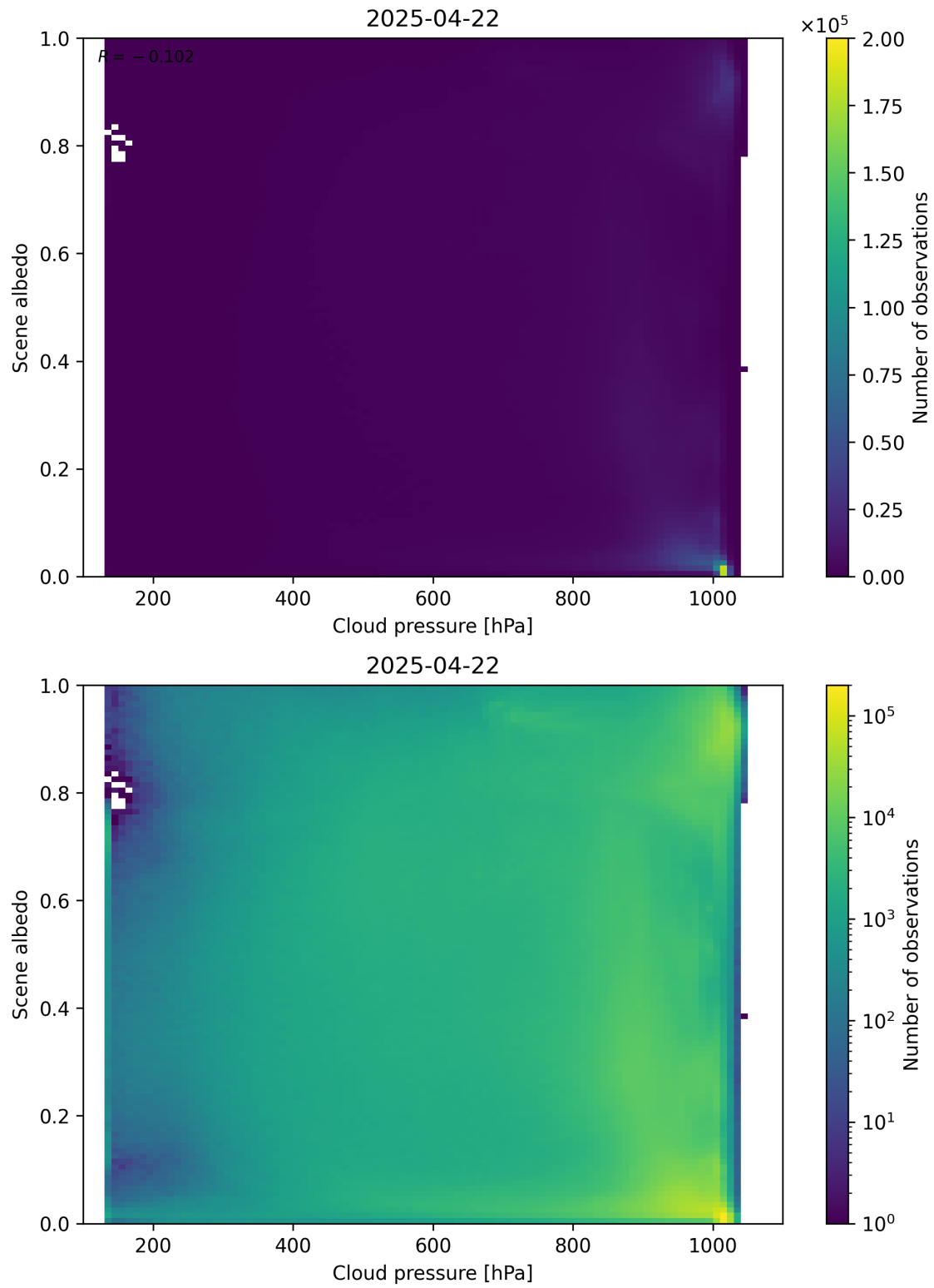
Figure 83: Scatter density plot of “Cloud pressure” against “Scene albedo” for 2025-04-21 to 2025-04-23.
