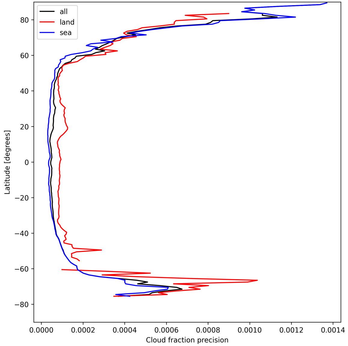
Figure 16: Zonal average of “Cloud fraction precision” for 2025-04-21 to 2025-04-23.
