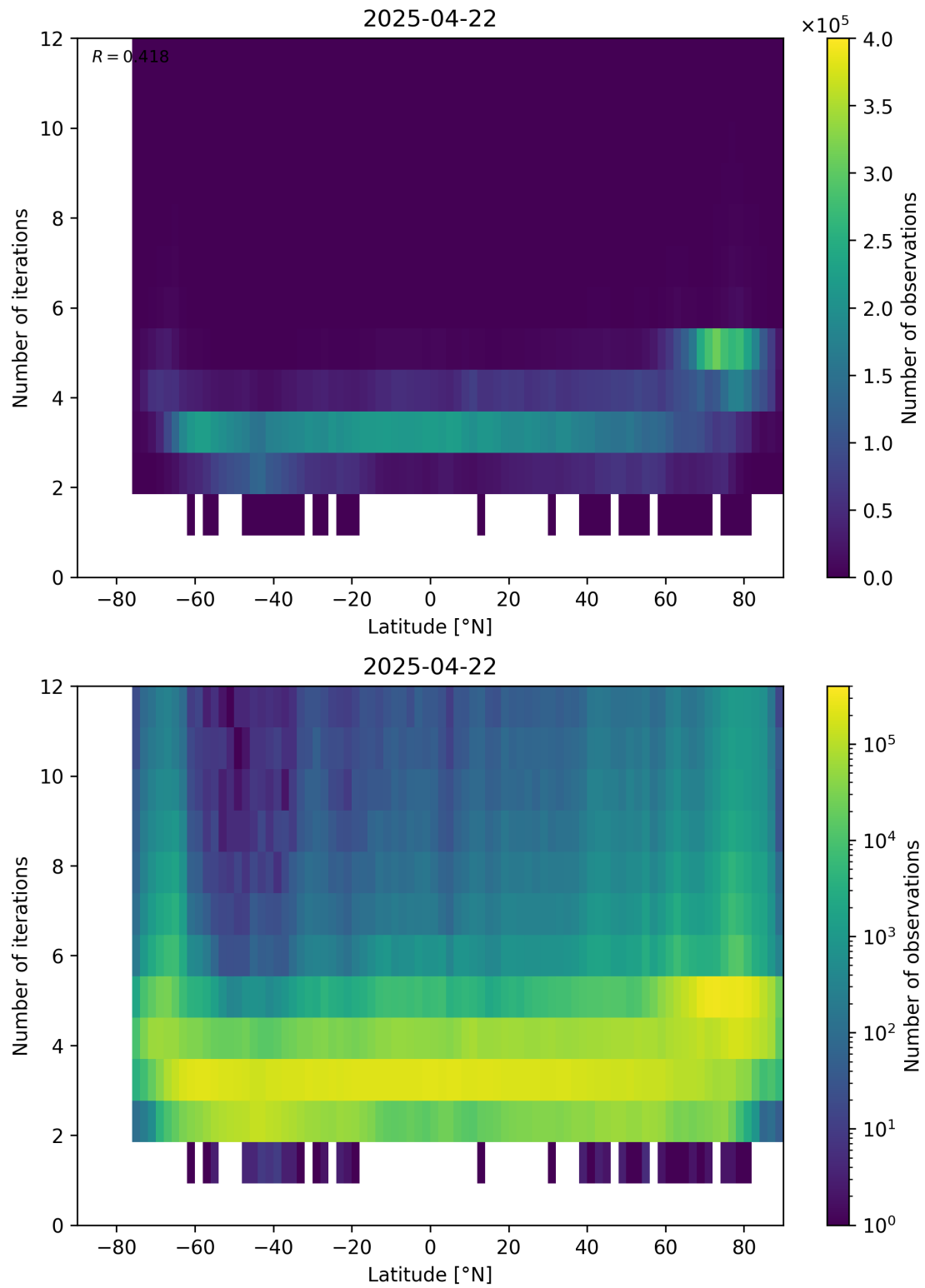
Figure 93: Scatter density plot of “Latitude” against “Number of iterations” for 2025-04-21 to 2025-04-23.
