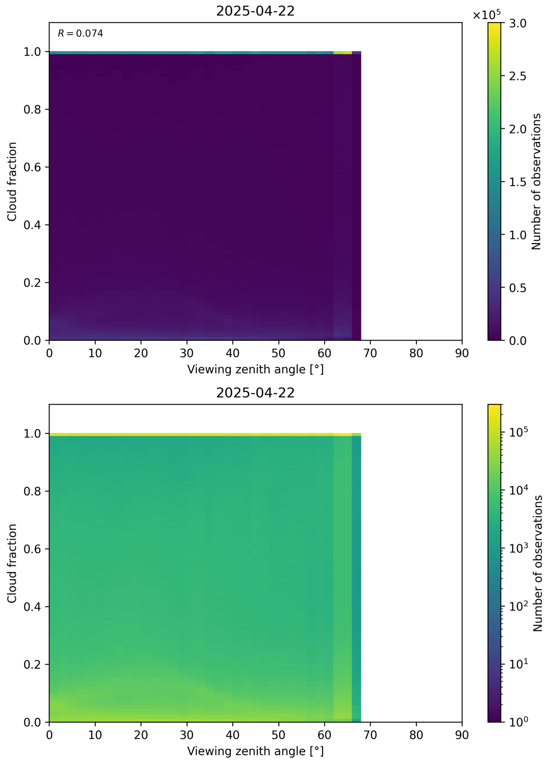
Figure 120: Scatter density plot of “Viewing zenith angle” against “Cloud fraction” for 2025-04-21 to 2025-04-23.
