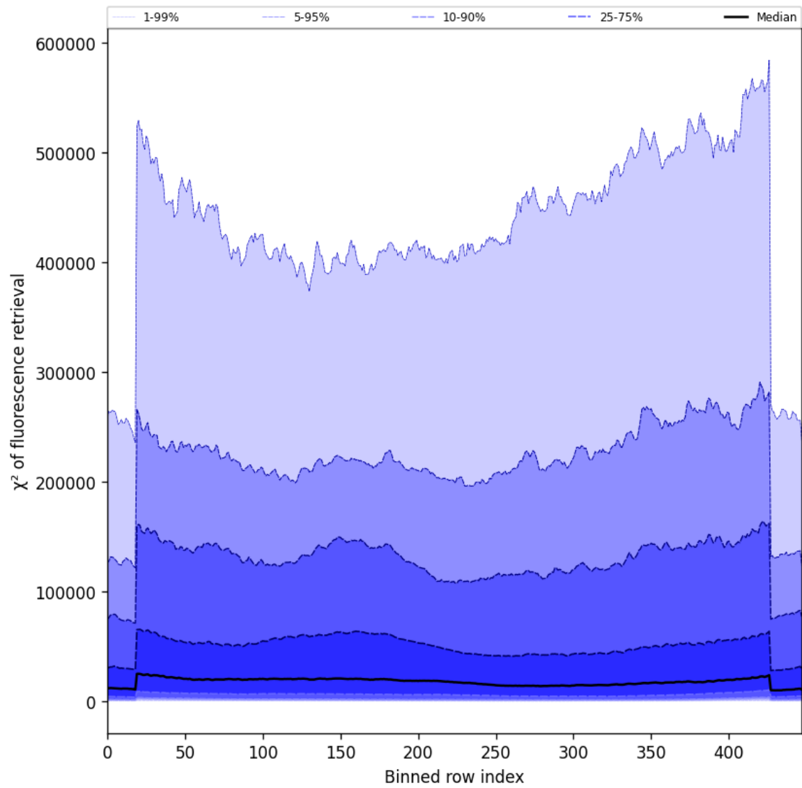
Figure 59: Along track statistics of “ \chi^2 of fluorescence retrieval” for 2025-04-21 to 2025-04-23
