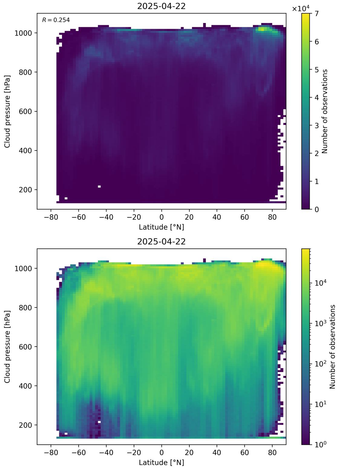
Figure 91: Scatter density plot of “Latitude” against “Cloud pressure” for 2025-04-21 to 2025-04-23.
