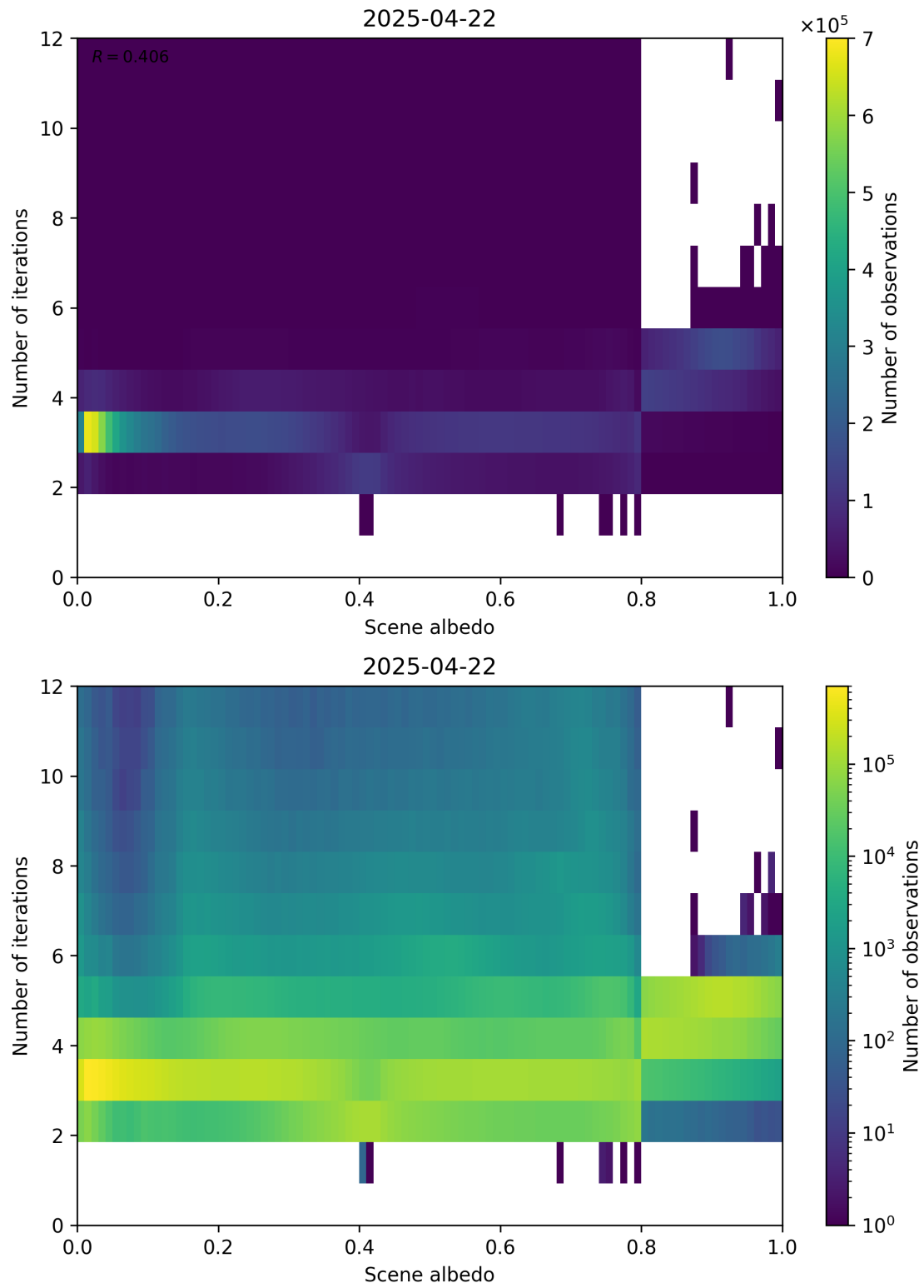
Figure 105: Scatter density plot of “Scene albedo” against “Number of iterations” for 2025-04-21 to 2025-04-23.
