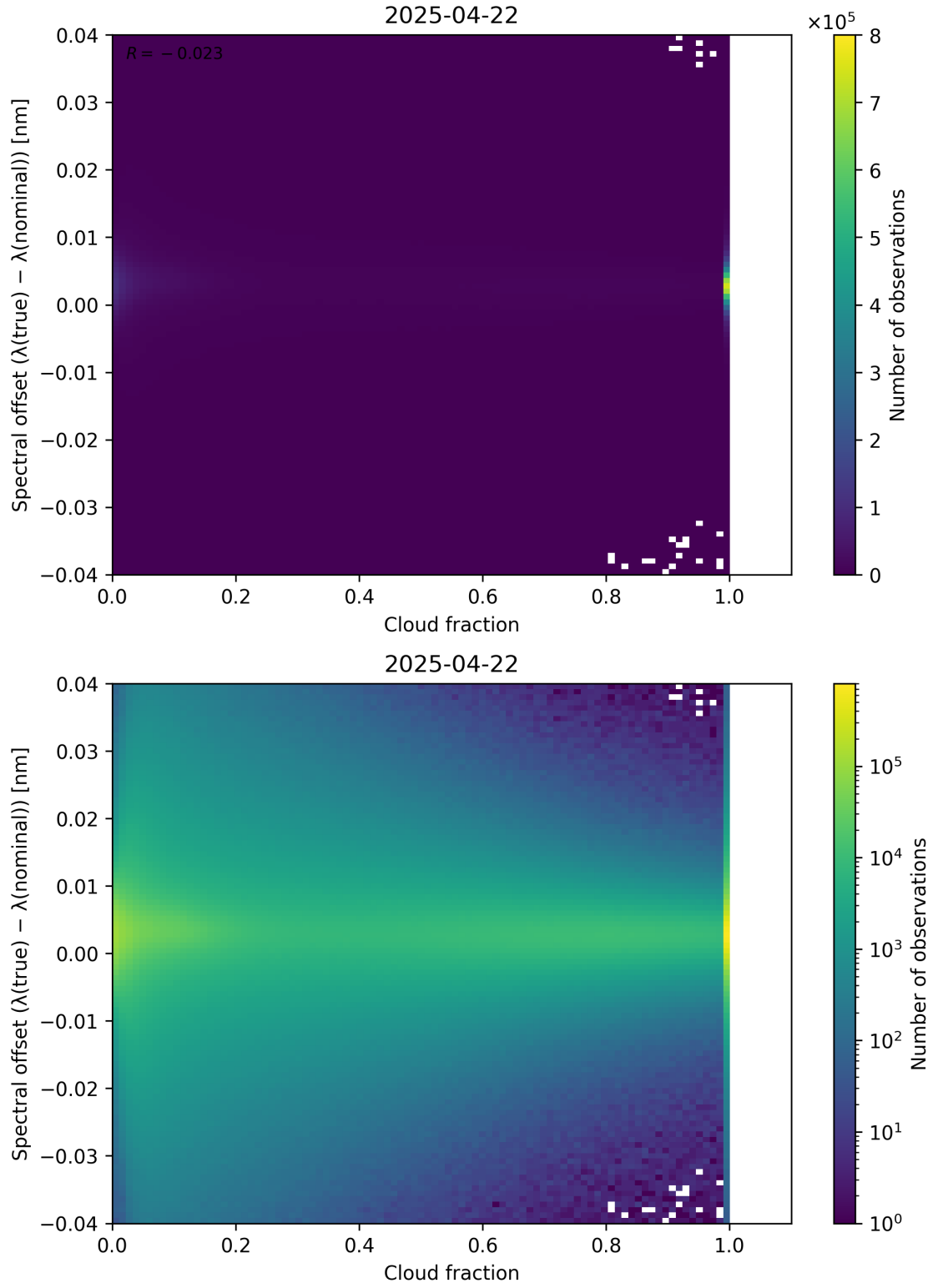
Figure 76: Scatter density plot of “Cloud fraction” against “Spectral offset ( \lambda_{\text{true}} - \lambda_{\text{nominal}} )” for 2025-04-21 to 2025-04-23.
