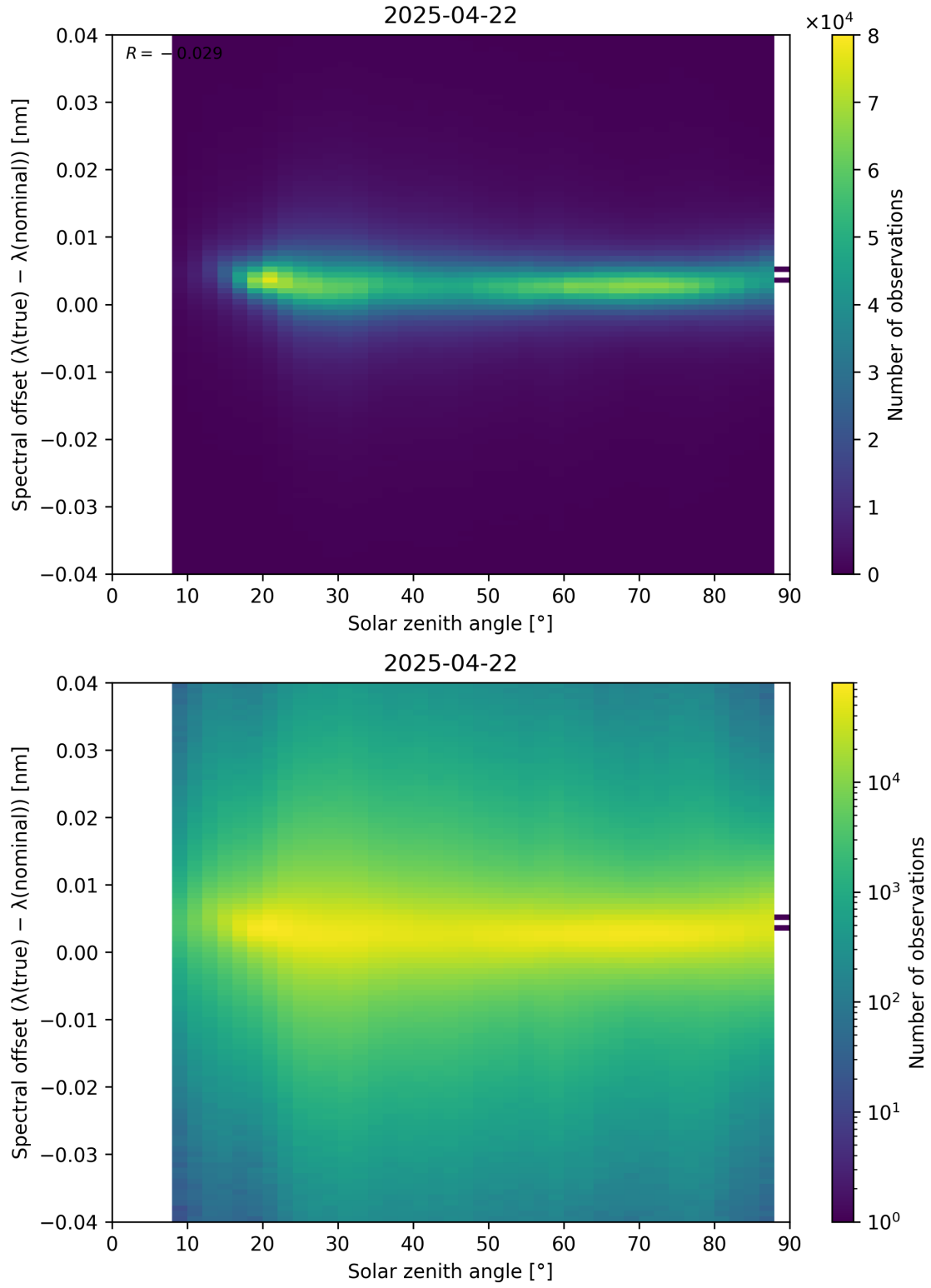
Figure 117: Scatter density plot of “Solar zenith angle” against “Spectral offset ( \lambda_{\text{true}} - \lambda_{\text{nominal}} )” for 2025-04-21 to 2025-04-23.
