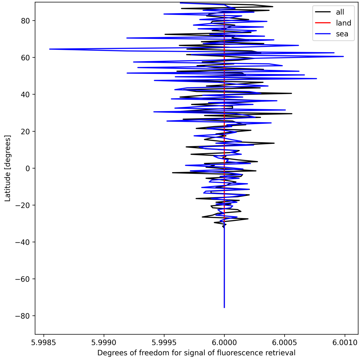
Figure 26: Zonal average of “Degrees of freedom for signal of fluorescence retrieval” for 2025-04-21 to 2025-04-23.
