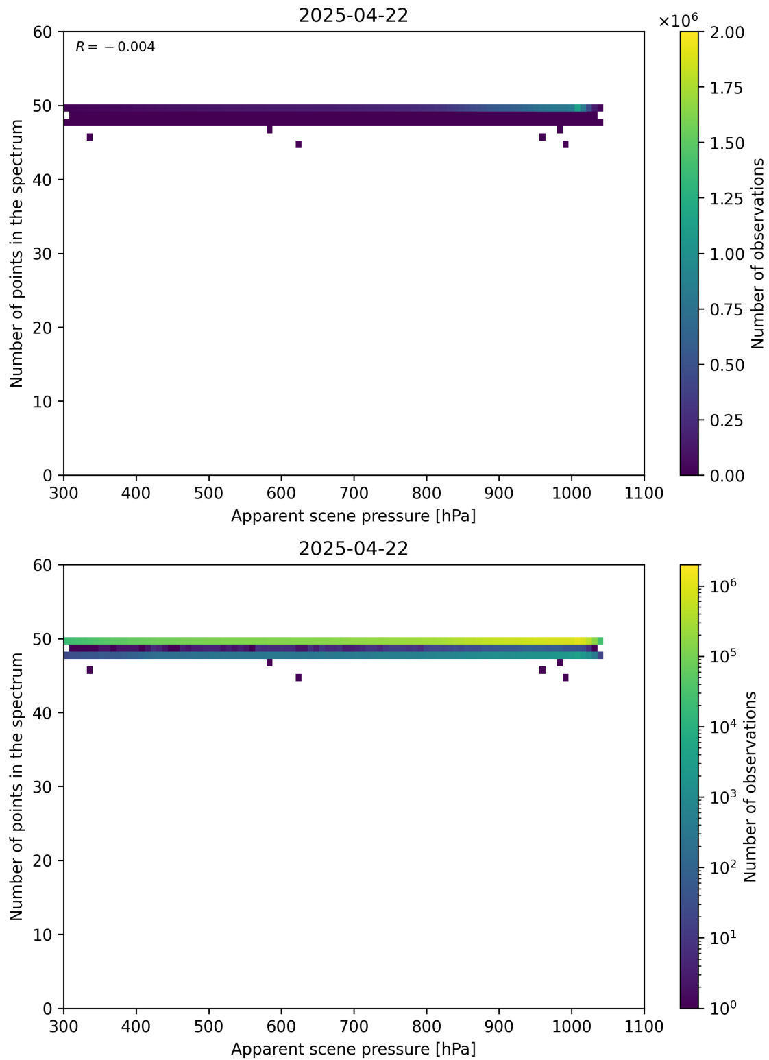
Figure 66: Scatter density plot of “Apparent scene pressure” against “Number of points in the spectrum” for 2025-04-21 to 2025-04-23.
