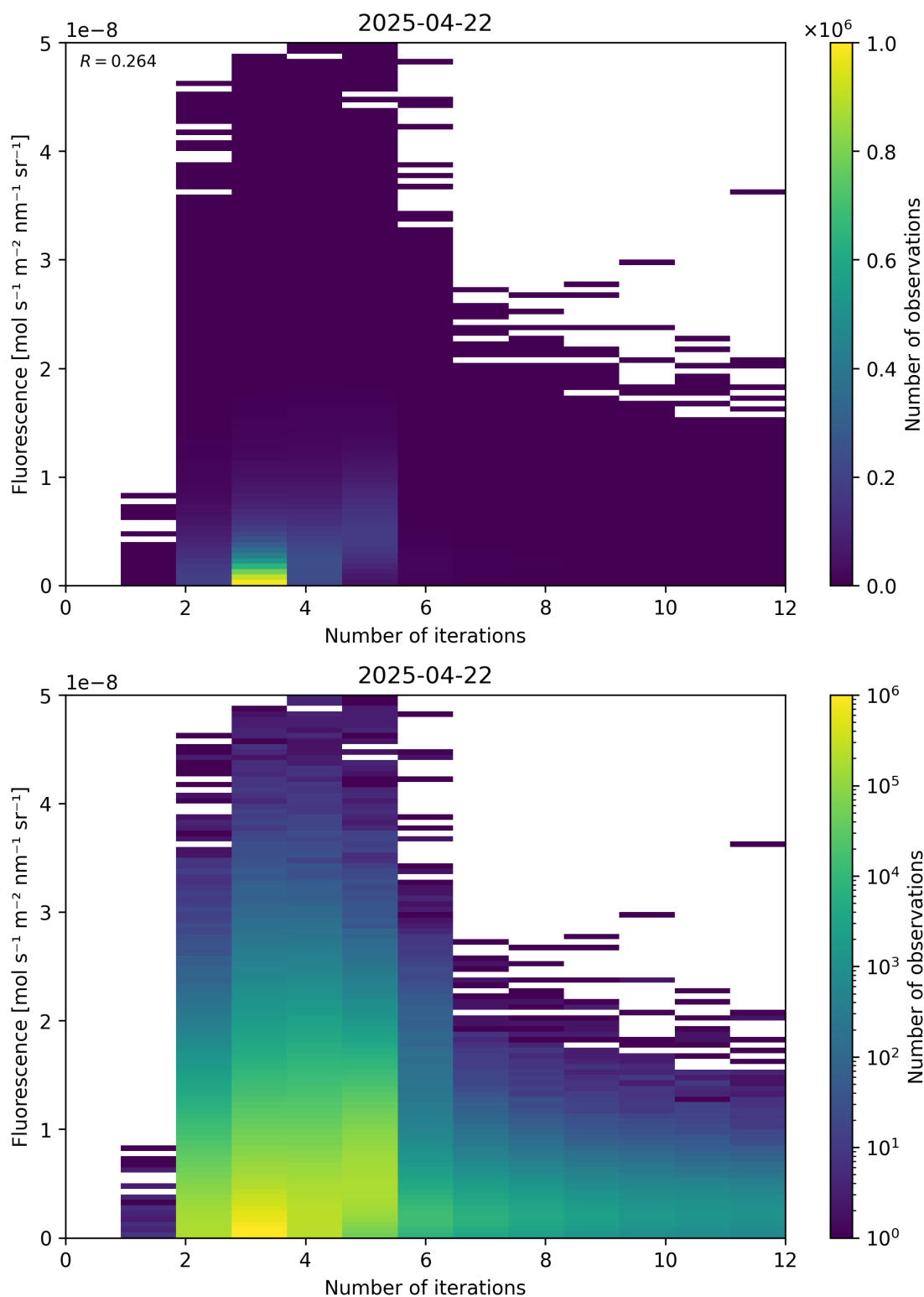
Figure 98: Scatter density plot of “Number of iterations” against “Fluorescence” for 2025-04-21 to 2025-04-23.
