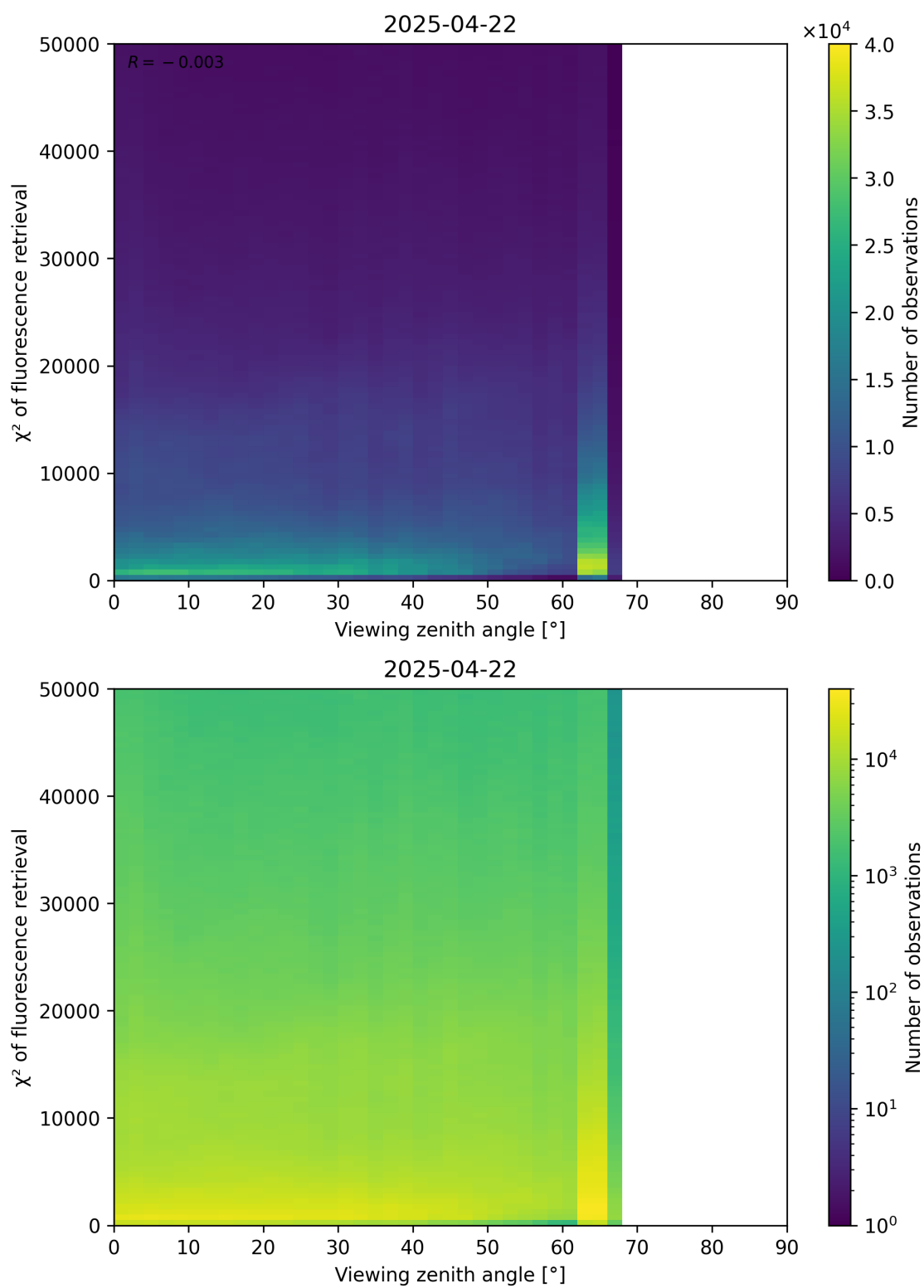
Figure 119: Scatter density plot of “Viewing zenith angle” against “ \chi^2 of fluorescence retrieval” for 2025-04-21 to 2025-04-23.
