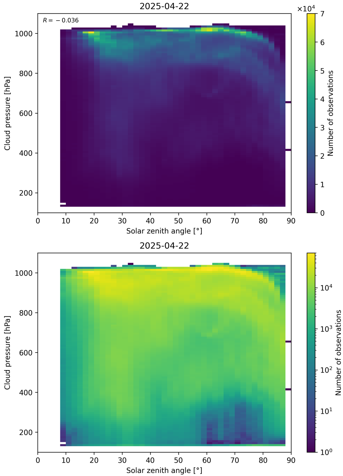
Figure 111: Scatter density plot of “Solar zenith angle” against “Cloud pressure” for 2025-04-21 to 2025-04-23.
