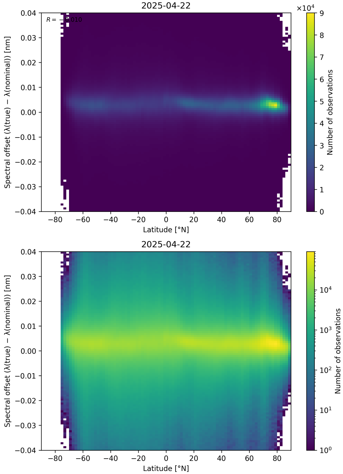
Figure 96: Scatter density plot of “Latitude” against “Spectral offset ( \lambda_{\text{true}} - \lambda_{\text{nominal}} )” for 2025-04-21 to 2025-04-23.
