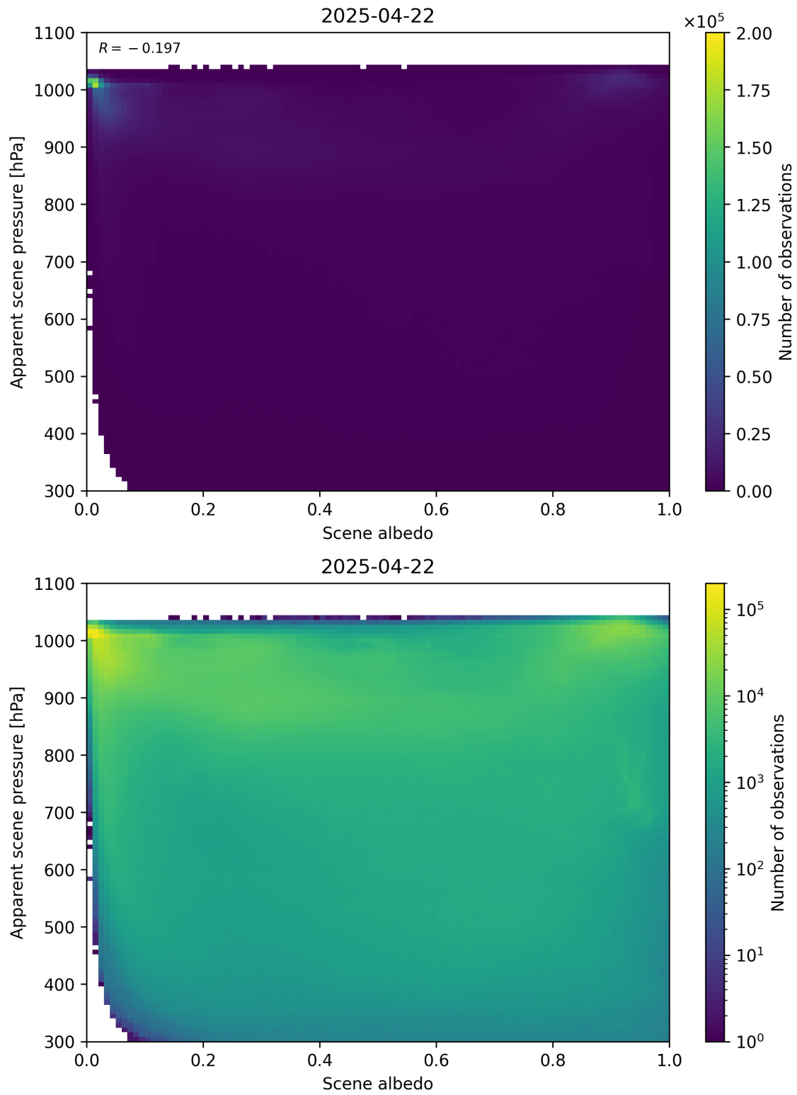
Figure 102: Scatter density plot of “Scene albedo” against “Apparent scene pressure” for 2025-04-21 to 2025-04-23.
