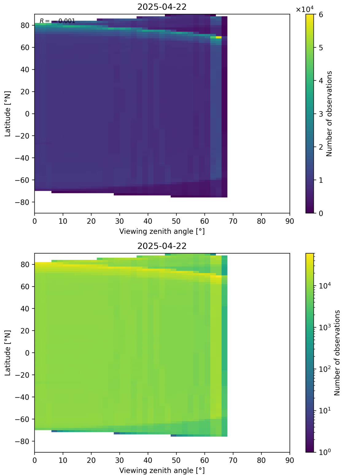
Figure 123: Scatter density plot of “Viewing zenith angle” against “Latitude” for 2025-04-21 to 2025-04-23.
