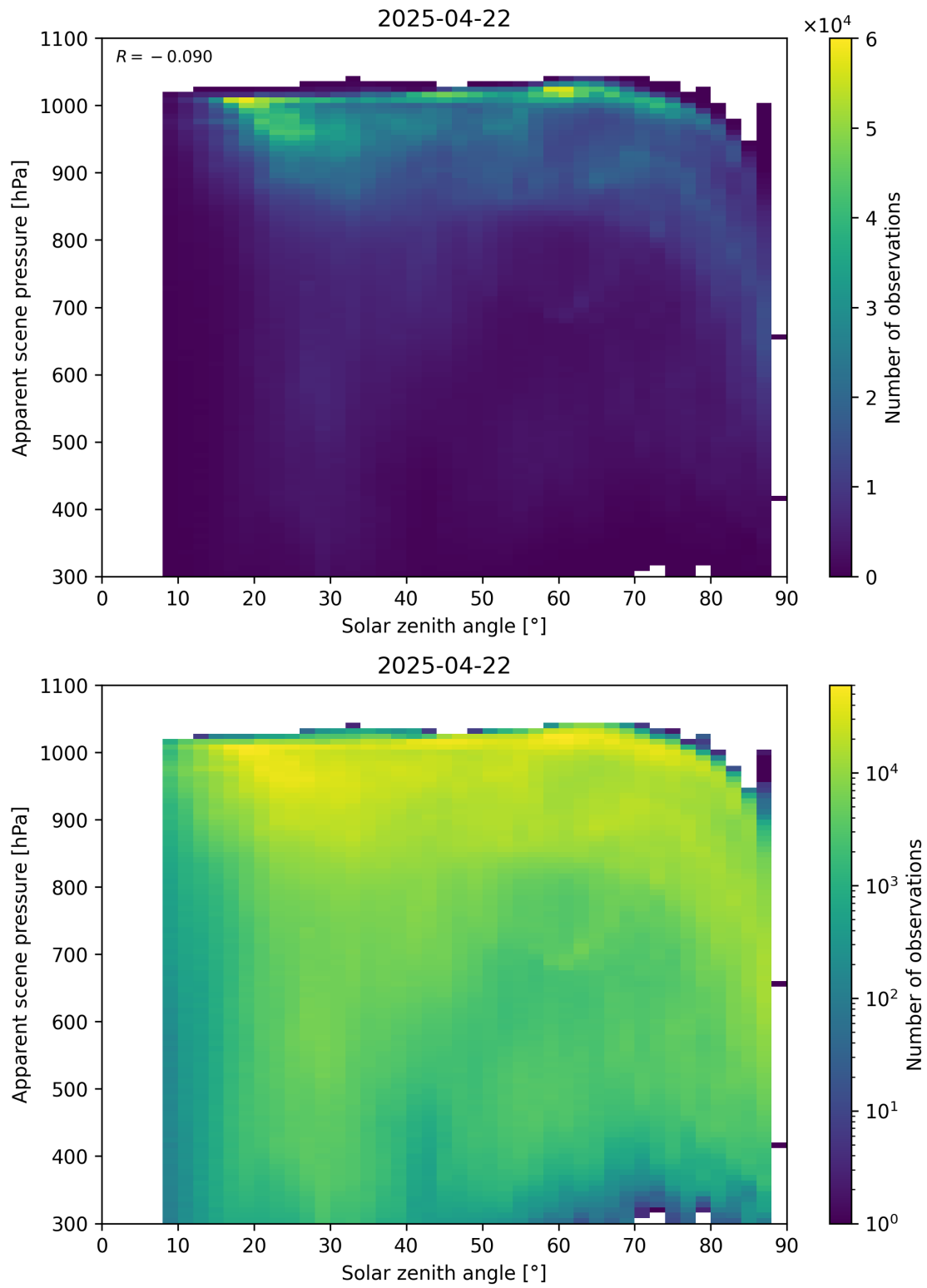
Figure 108: Scatter density plot of “Solar zenith angle” against “Apparent scene pressure” for 2025-04-21 to 2025-04-23.
