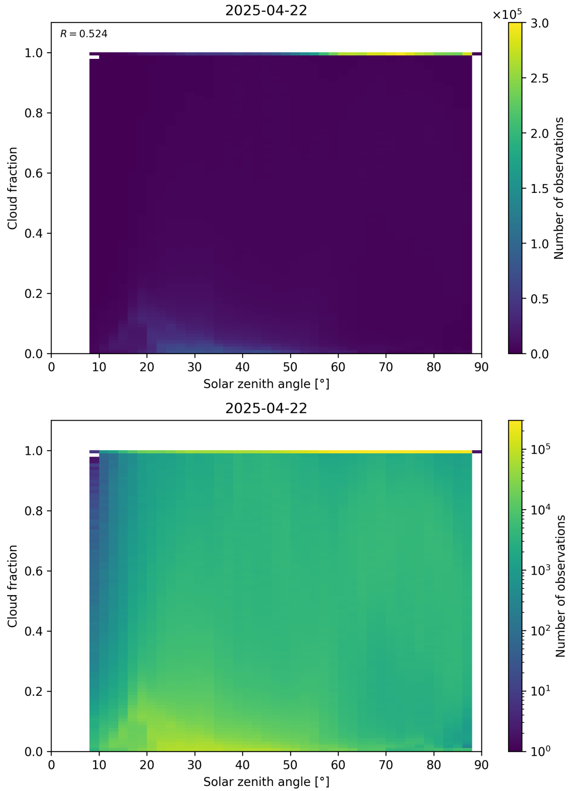
Figure 110: Scatter density plot of “Solar zenith angle” against “Cloud fraction” for 2025-04-21 to 2025-04-23.
