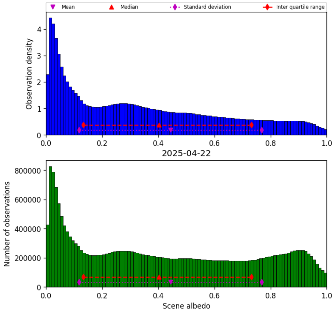
Figure 34: Histogram of “Scene albedo” for 2025-04-21 to 2025-04-23
