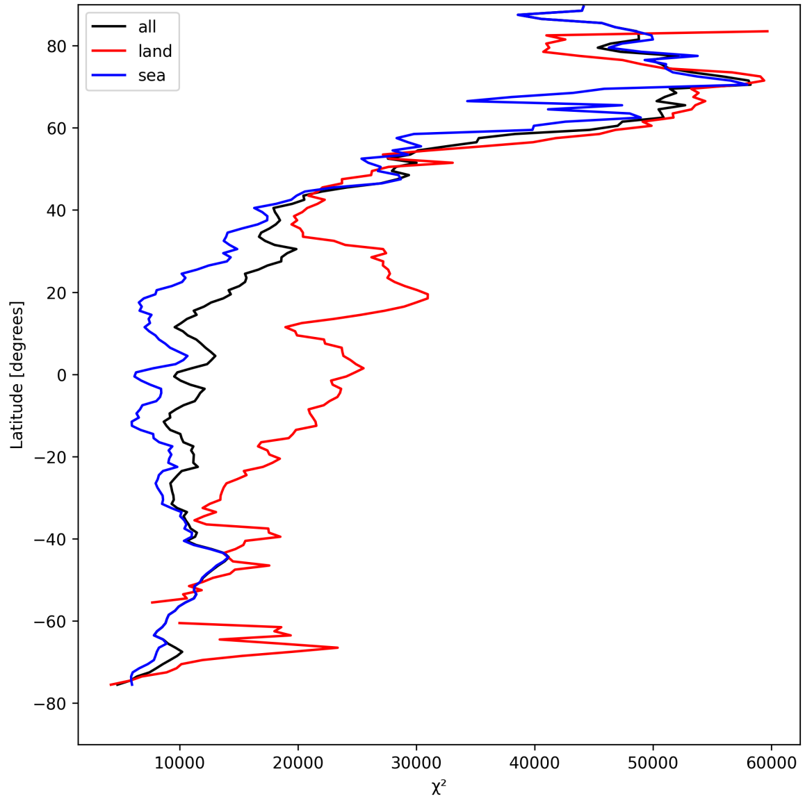
Figure 21: Zonal average of “ \chi^2 ” for 2025-04-21 to 2025-04-23.
