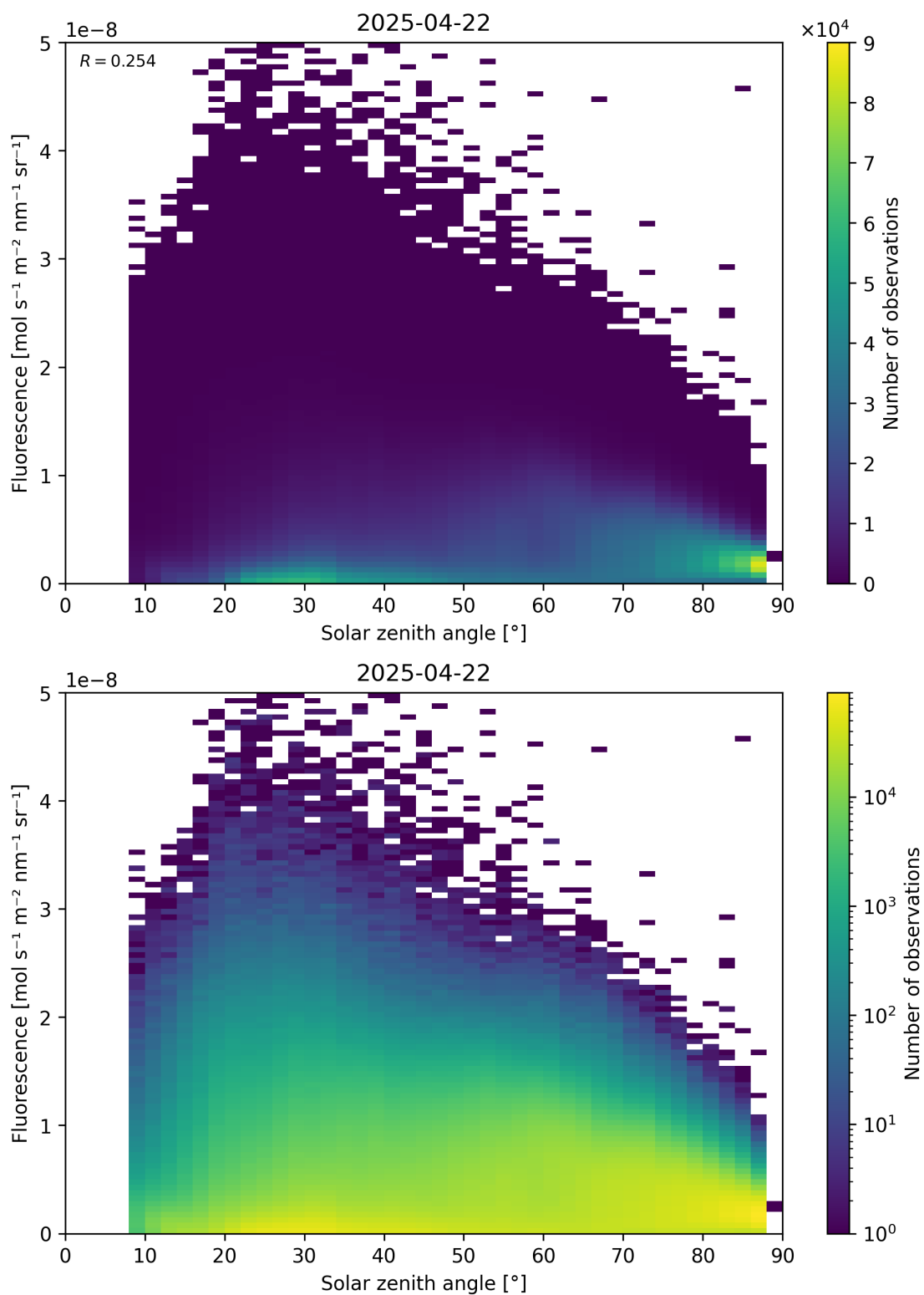
Figure 112: Scatter density plot of “Solar zenith angle” against “Fluorescence” for 2025-04-21 to 2025-04-23.
