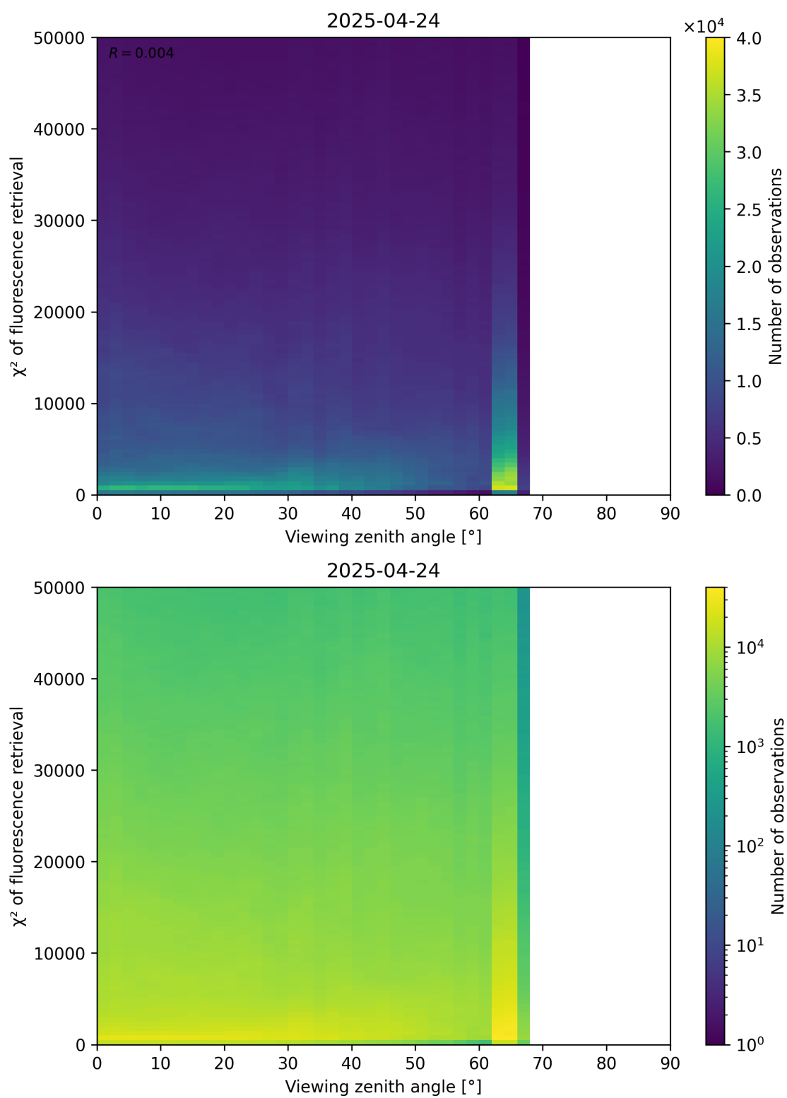
Figure 119: Scatter density plot of “Viewing zenith angle” against “ \chi^2 of fluorescence retrieval” for 2025-04-24 to 2025-04-25.
