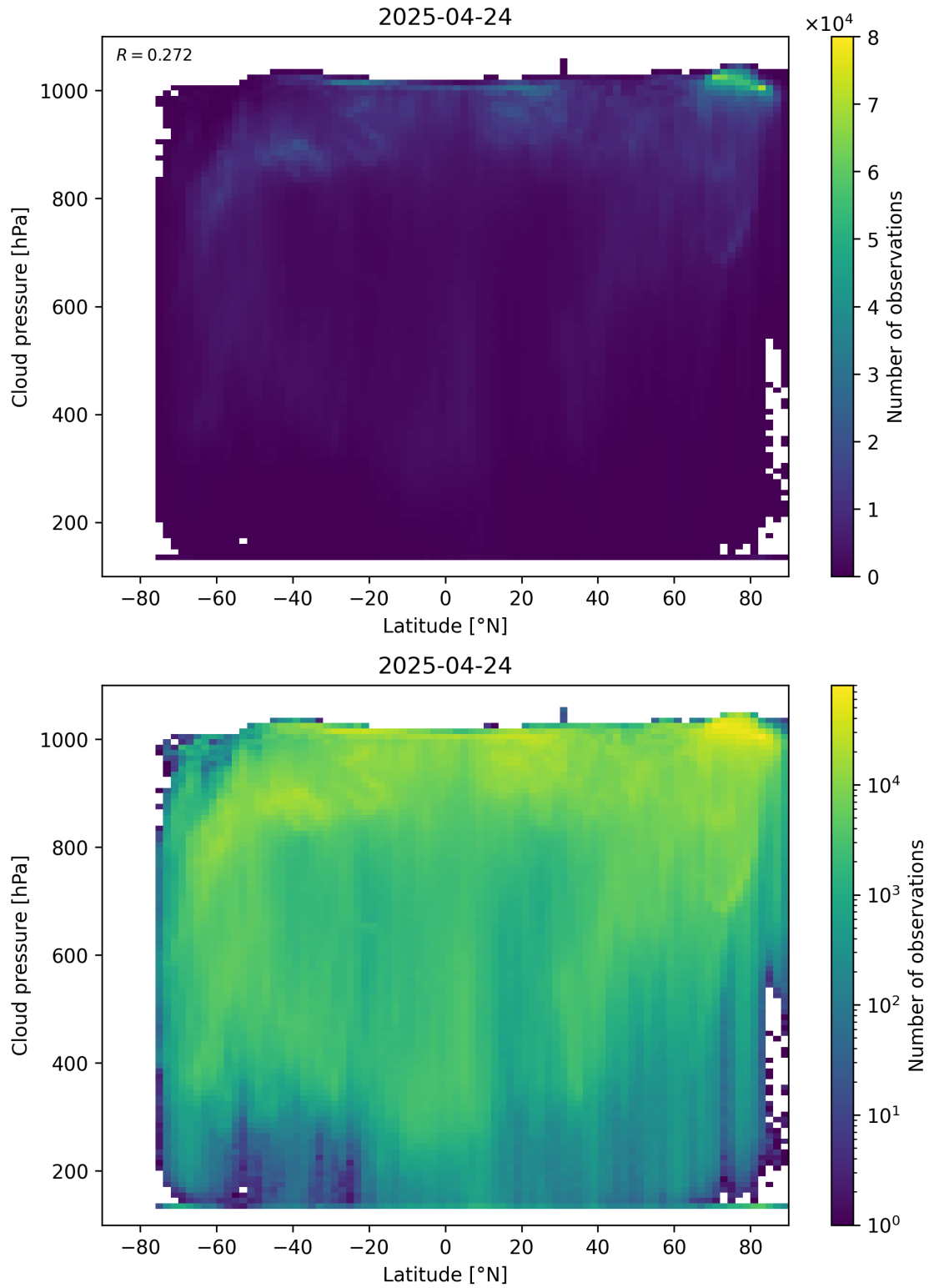
Figure 91: Scatter density plot of “Latitude” against “Cloud pressure” for 2025-04-24 to 2025-04-25.
