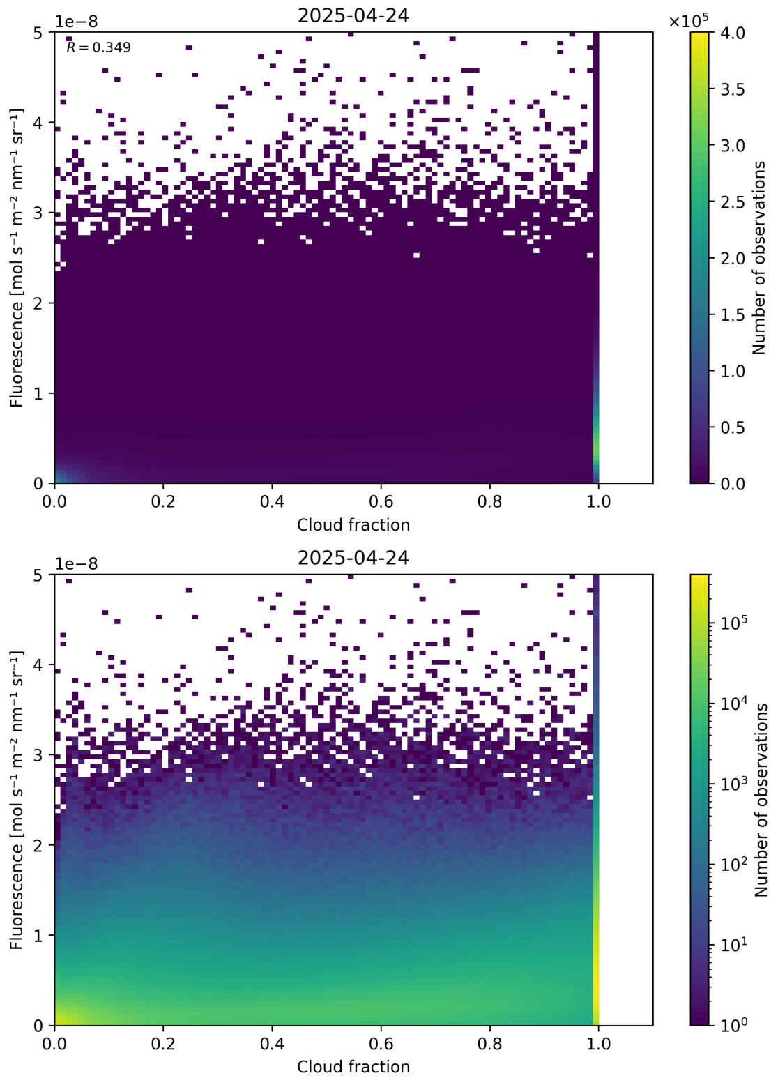
Figure 72: Scatter density plot of “Cloud fraction” against “Fluorescence” for 2025-04-24 to 2025-04-25.
