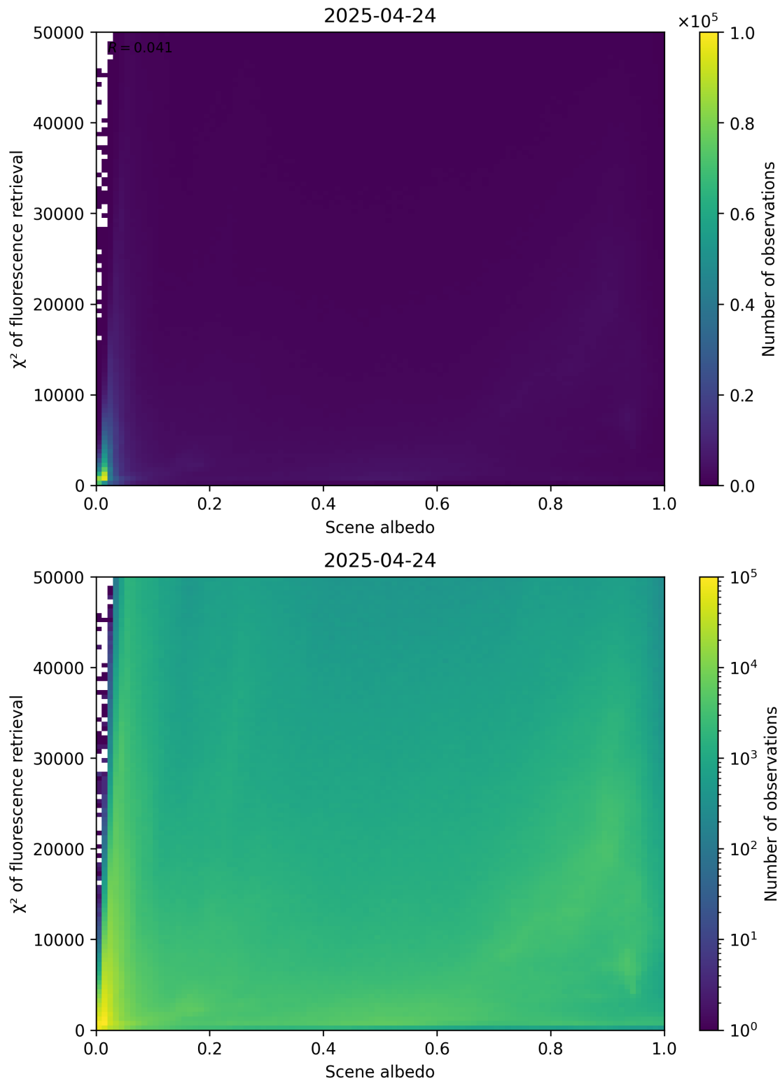
Figure 103: Scatter density plot of “Scene albedo” against “ \chi^2 of fluorescence retrieval” for 2025-04-24 to 2025-04-25.
