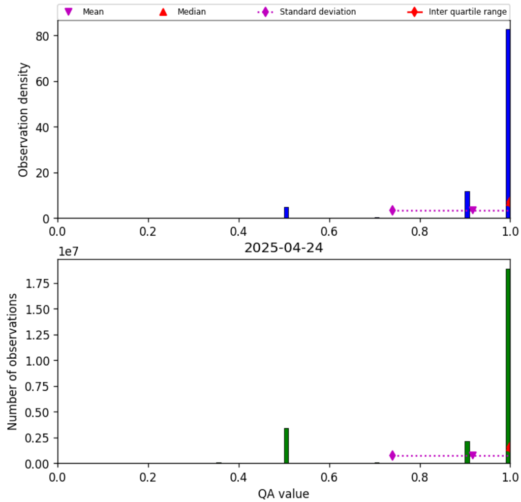
Figure 29: Histogram of “QA value” for 2025-04-24 to 2025-04-25
