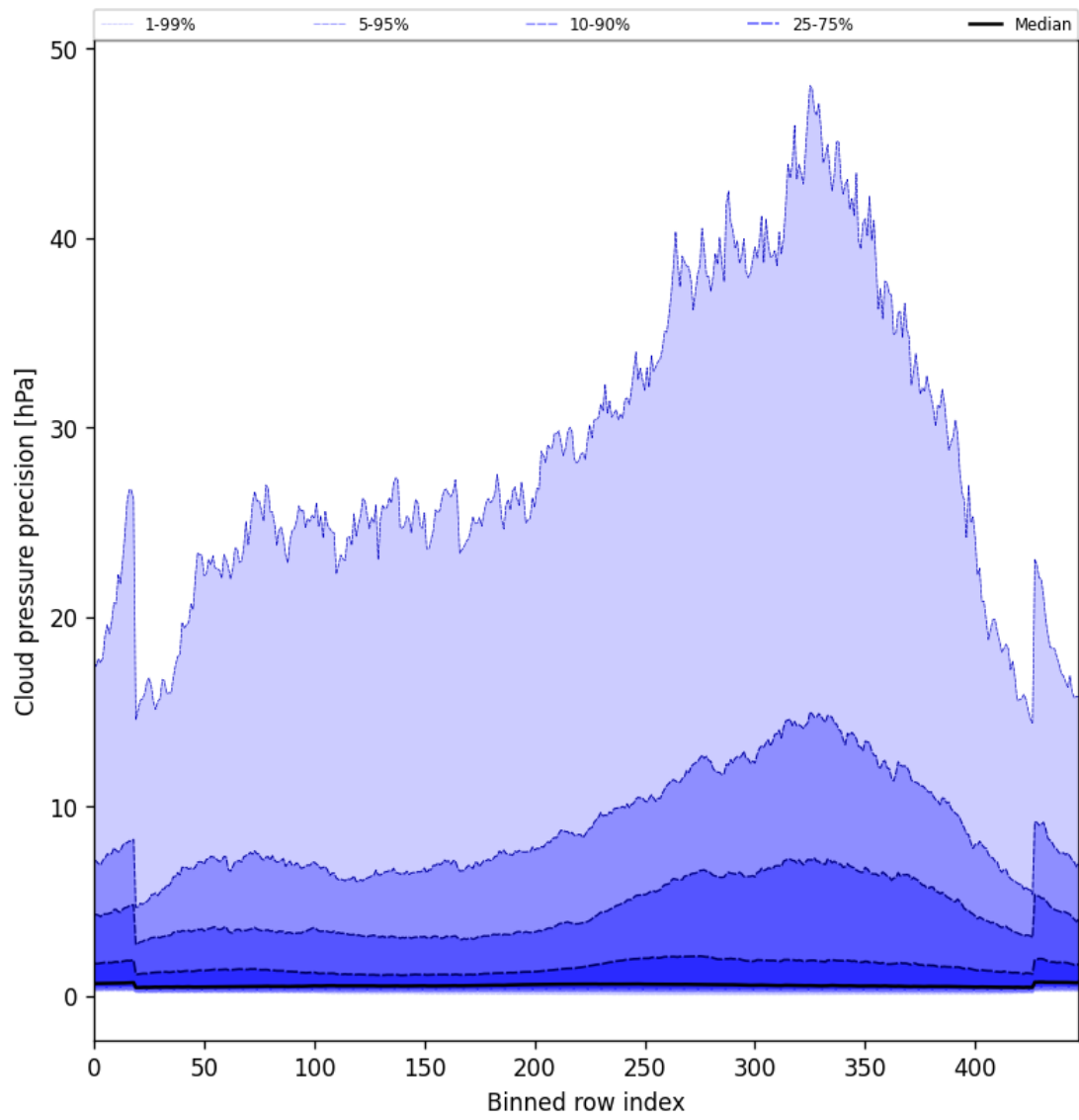
Figure 48: Along track statistics of “Cloud pressure precision” for 2025-04-24 to 2025-04-25
