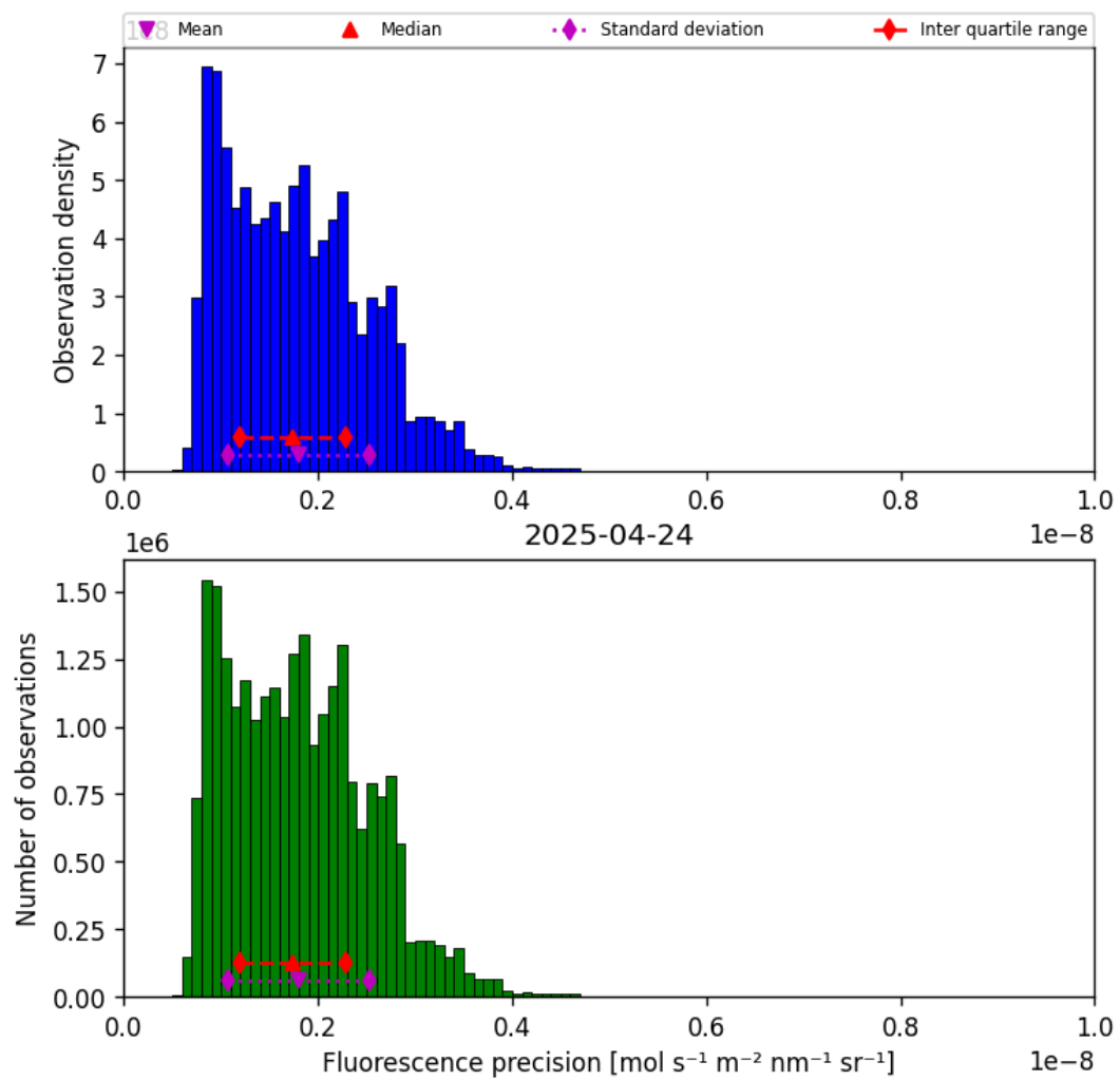
Figure 41: Histogram of “Fluorescence precision” for 2025-04-24 to 2025-04-25
