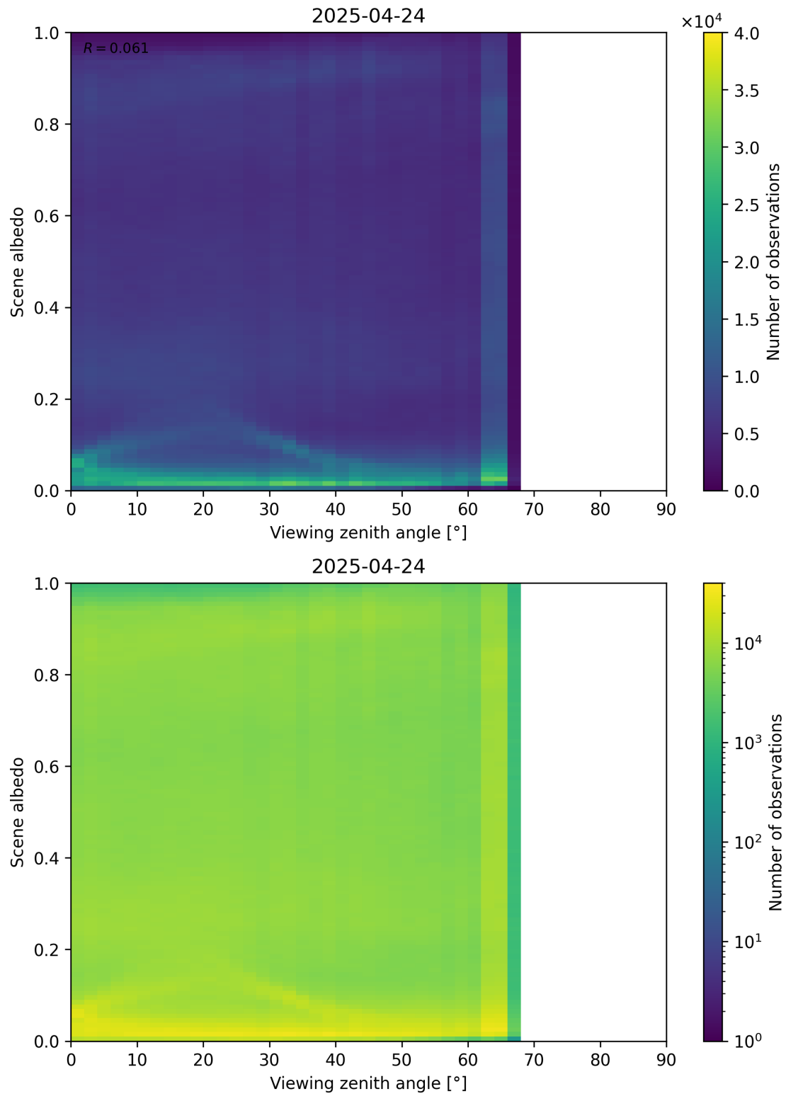
Figure 126: Scatter density plot of “Viewing zenith angle” against “Scene albedo” for 2025-04-24 to 2025-04-25.
