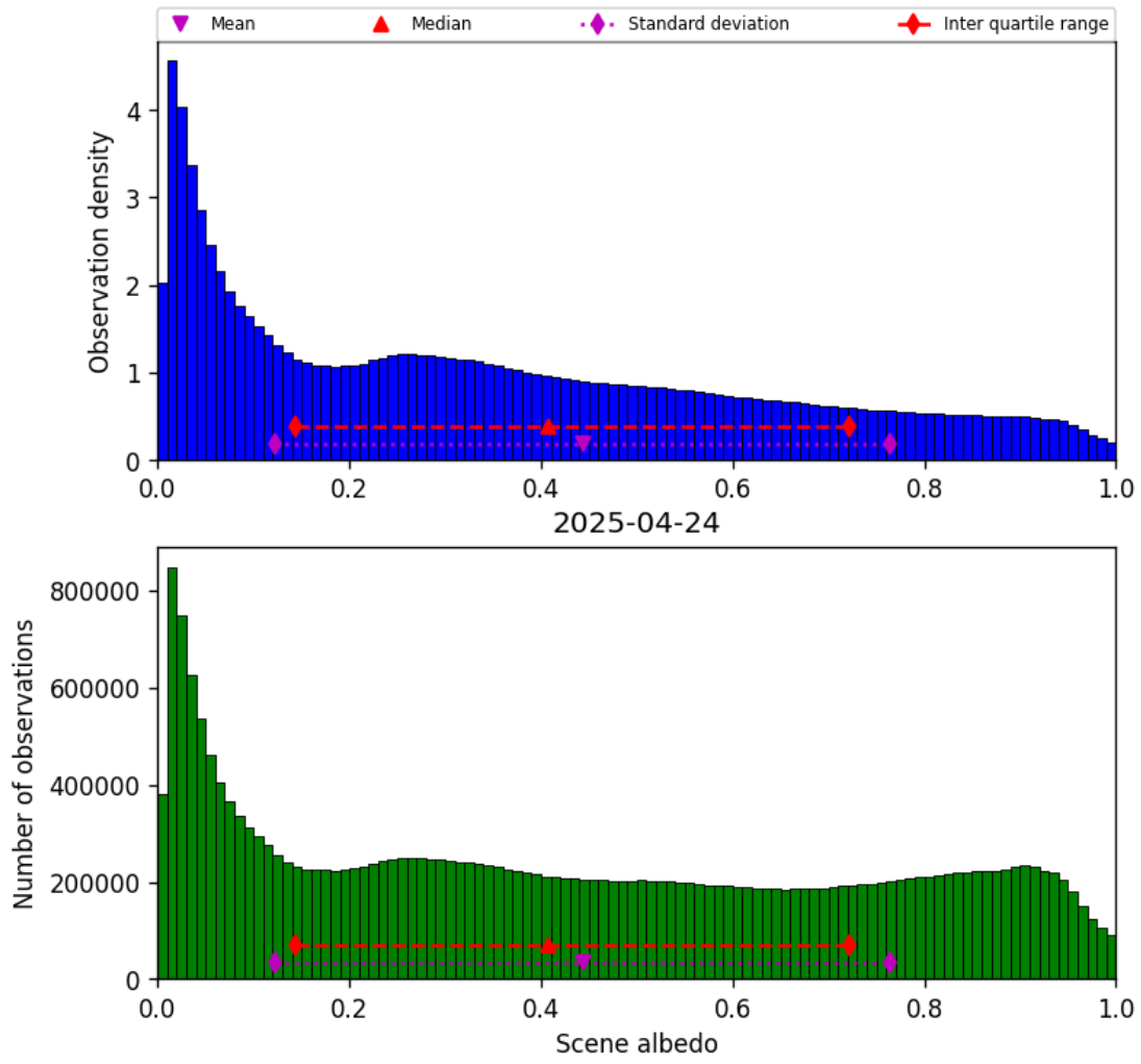
Figure 34: Histogram of “Scene albedo” for 2025-04-24 to 2025-04-25
