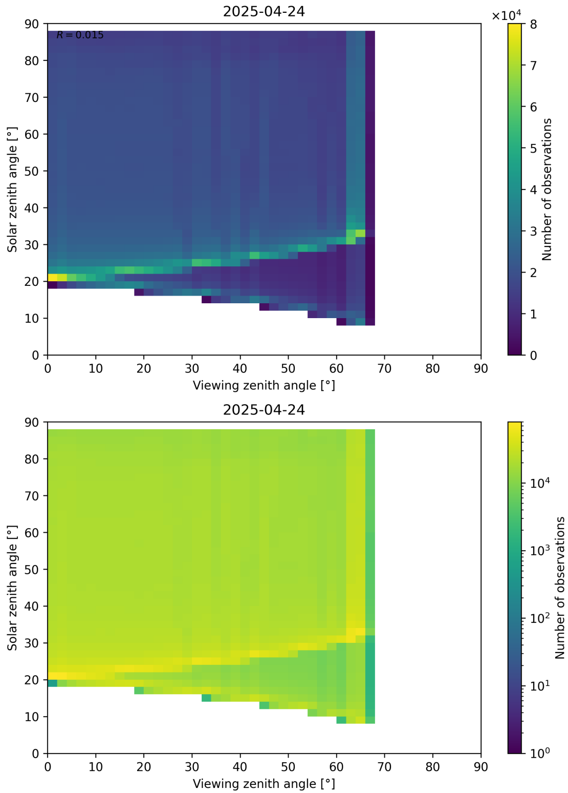
Figure 127: Scatter density plot of “Viewing zenith angle” against “Solar zenith angle” for 2025-04-24 to 2025-04-25.
