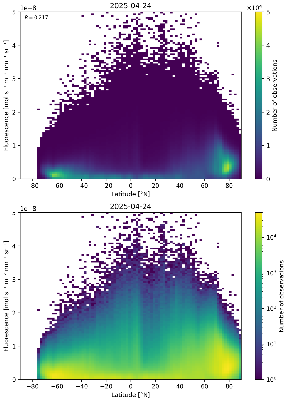
Figure 92: Scatter density plot of “Latitude” against “Fluorescence” for 2025-04-24 to 2025-04-25.
