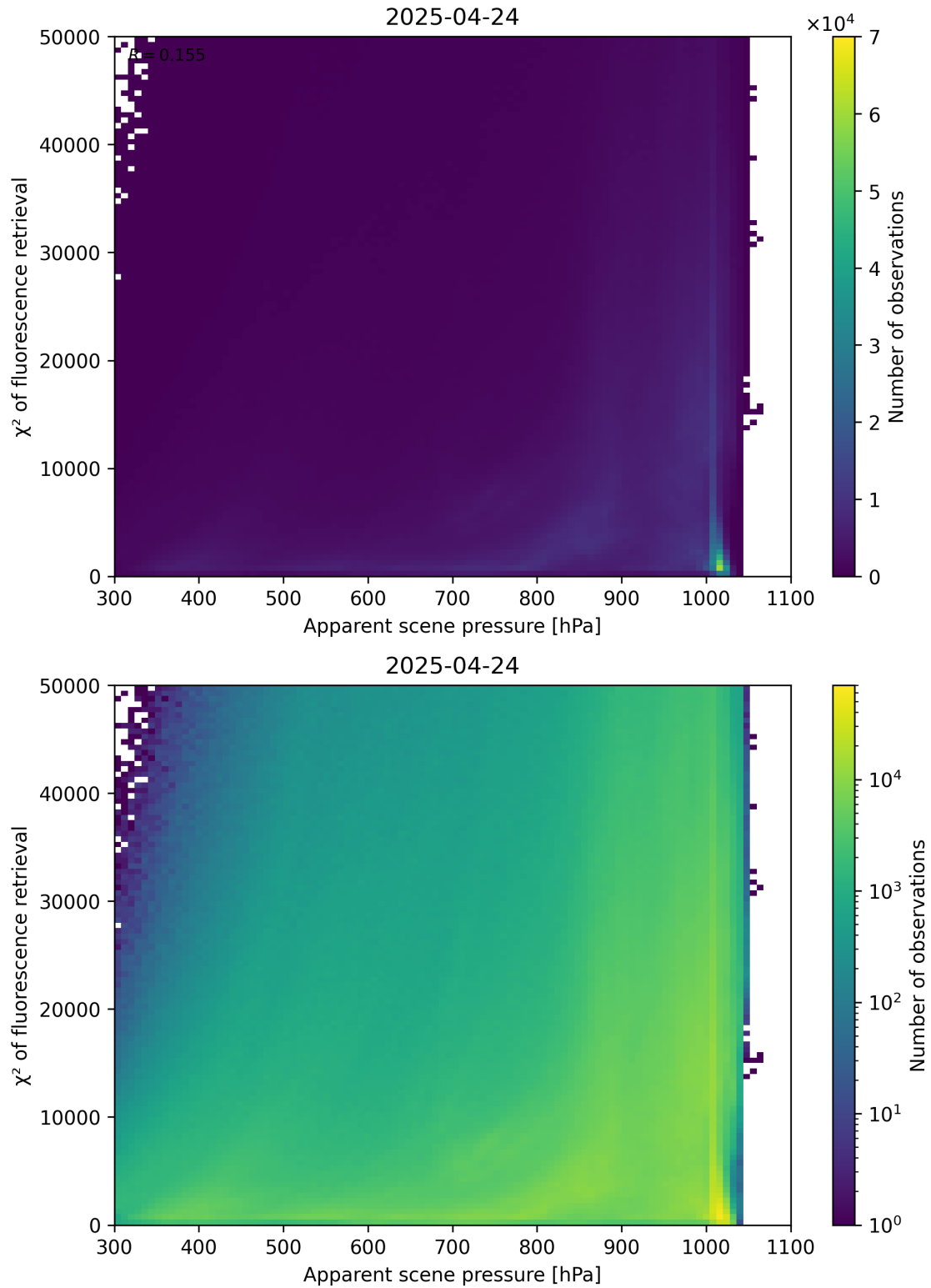
Figure 63: Scatter density plot of “Apparent scene pressure” against “ \chi^2 of fluorescence retrieval” for 2025-04-24 to 2025-04-25.
