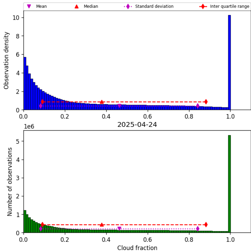
Figure 32: Histogram of “Cloud fraction” for 2025-04-24 to 2025-04-25
