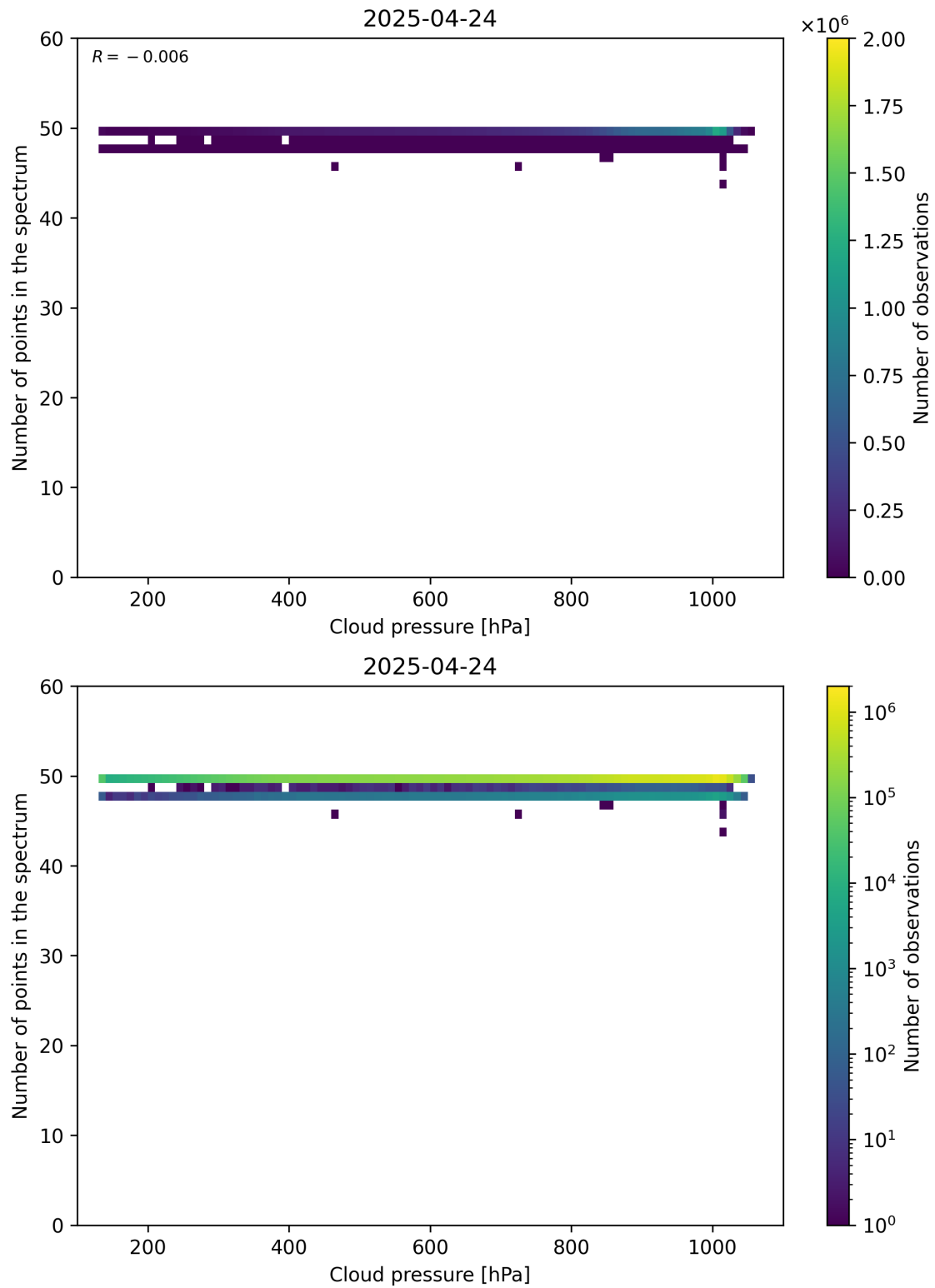
Figure 82: Scatter density plot of “Cloud pressure” against “Number of points in the spectrum” for 2025-04-24 to 2025-04-25.
