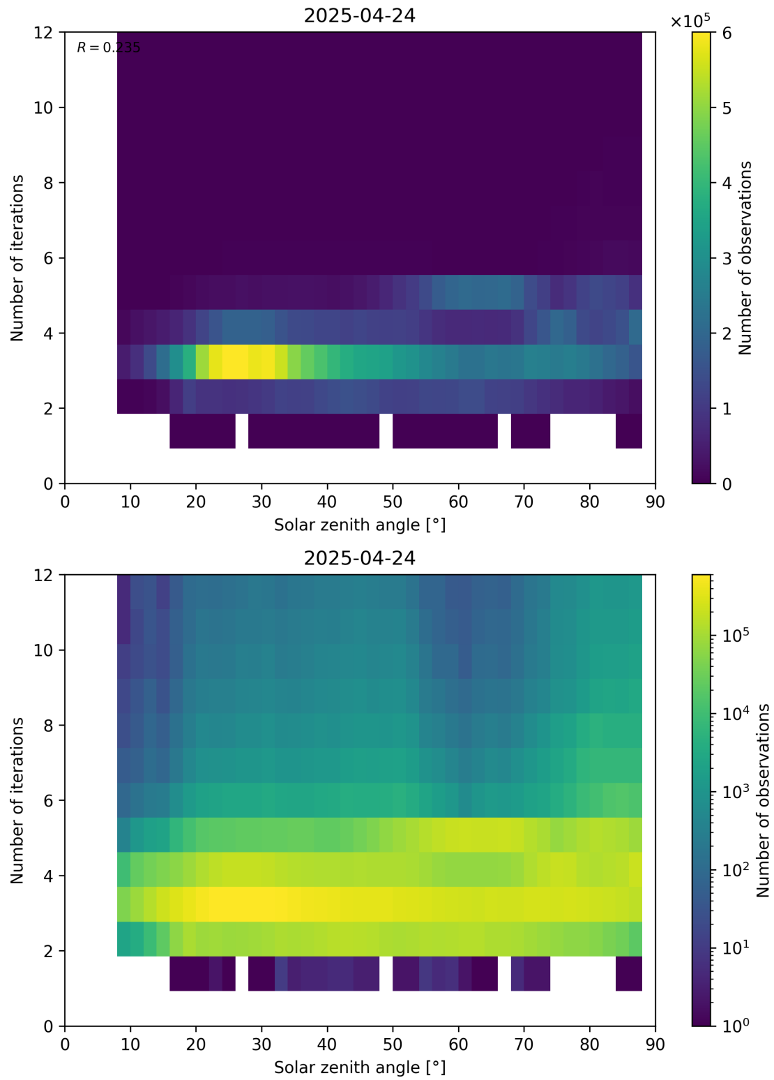
Figure 114: Scatter density plot of “Solar zenith angle” against “Number of iterations” for 2025-04-24 to 2025-04-25.
