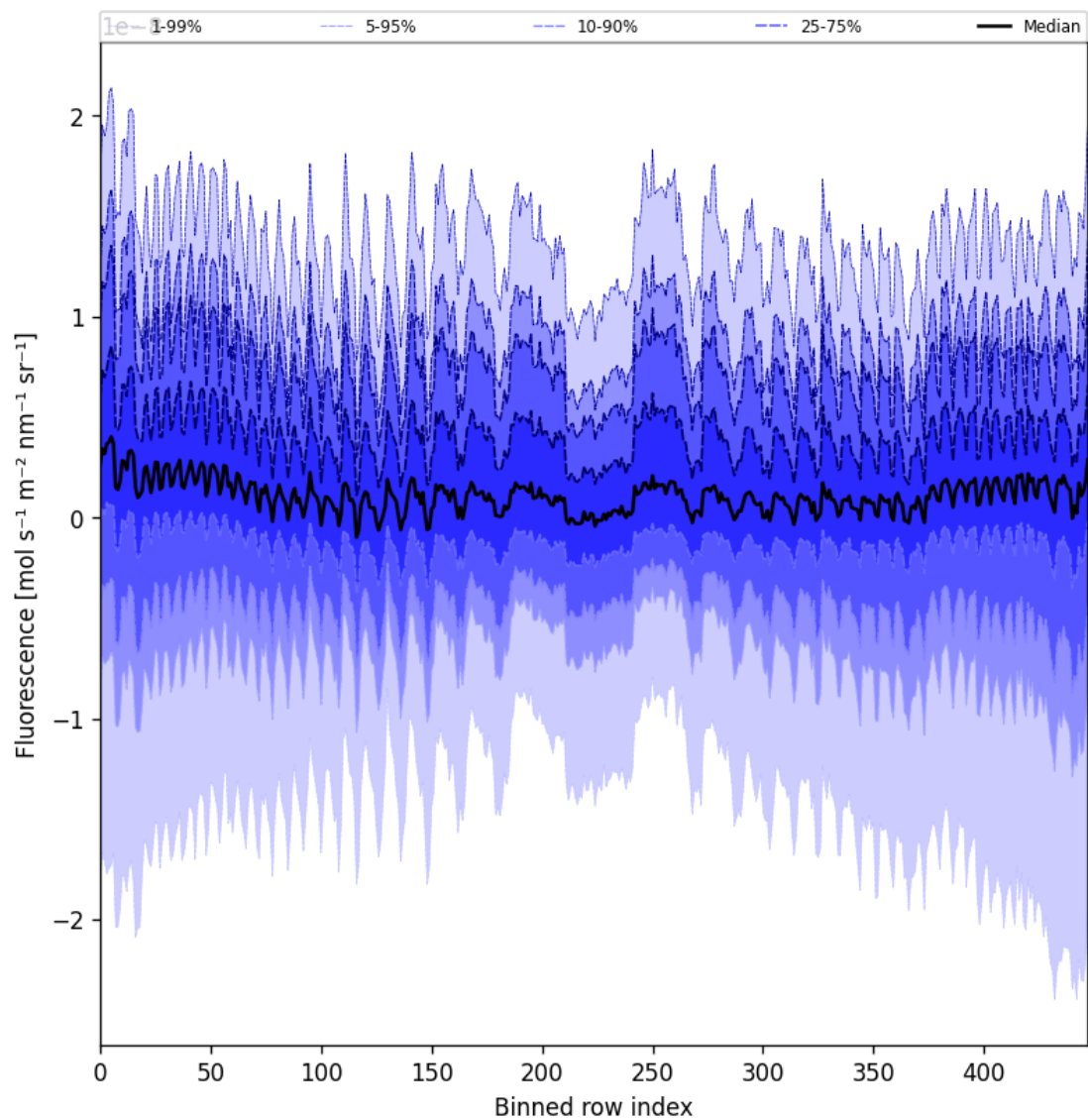
Figure 57: Along track statistics of “Fluorescence” for 2025-04-24 to 2025-04-25
