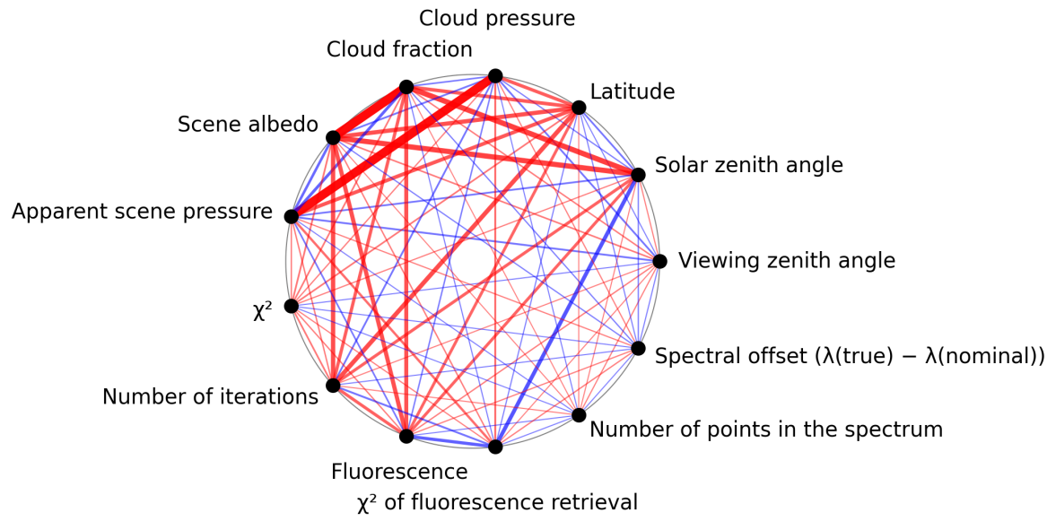
Figure 1: Map of correlation graph for 2025-04-24 to 2025-04-25.
