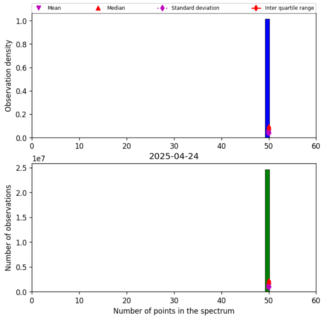
Figure 44: Histogram of “Number of points in the spectrum” for 2025-04-24 to 2025-04-25
