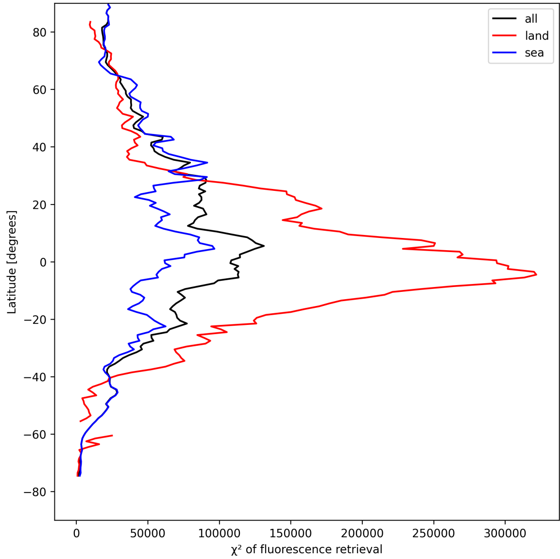
Figure 25: Zonal average of “ \chi^2 of fluorescence retrieval” for 2025-04-24 to 2025-04-25.
