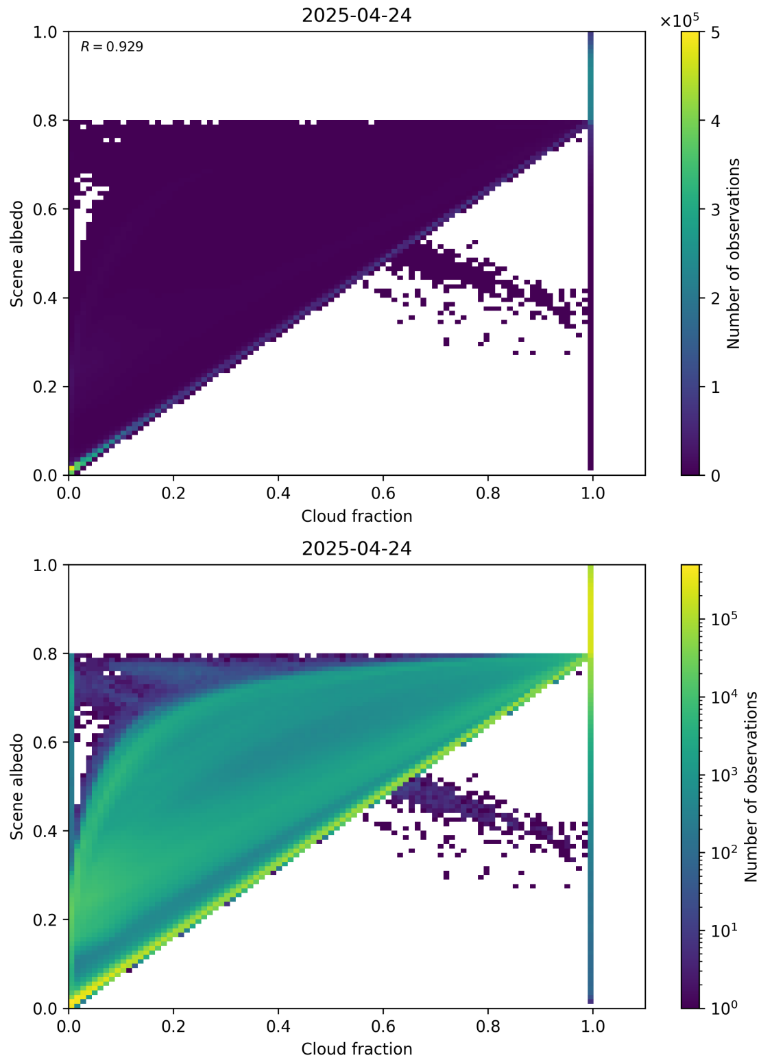
Figure 75: Scatter density plot of “Cloud fraction” against “Scene albedo” for 2025-04-24 to 2025-04-25.
