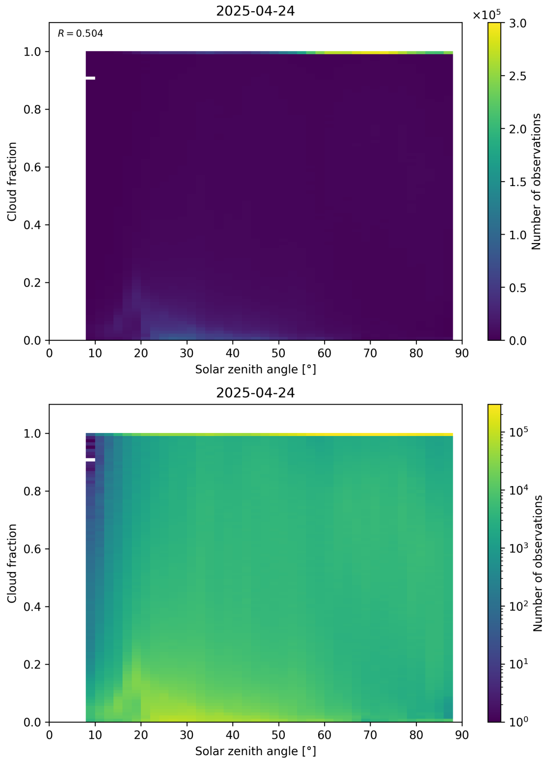
Figure 110: Scatter density plot of “Solar zenith angle” against “Cloud fraction” for 2025-04-24 to 2025-04-25.
