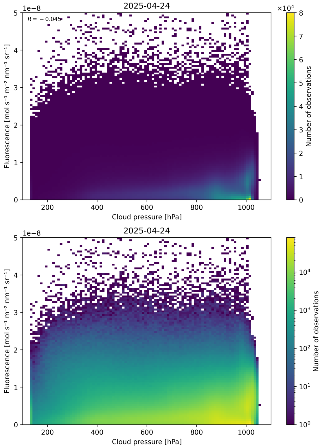
Figure 80: Scatter density plot of “Cloud pressure” against “Fluorescence” for 2025-04-24 to 2025-04-25.
