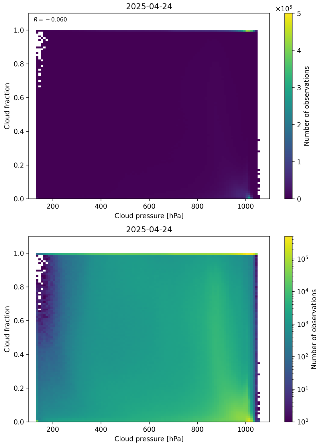
Figure 79: Scatter density plot of “Cloud pressure” against “Cloud fraction” for 2025-04-24 to 2025-04-25.
