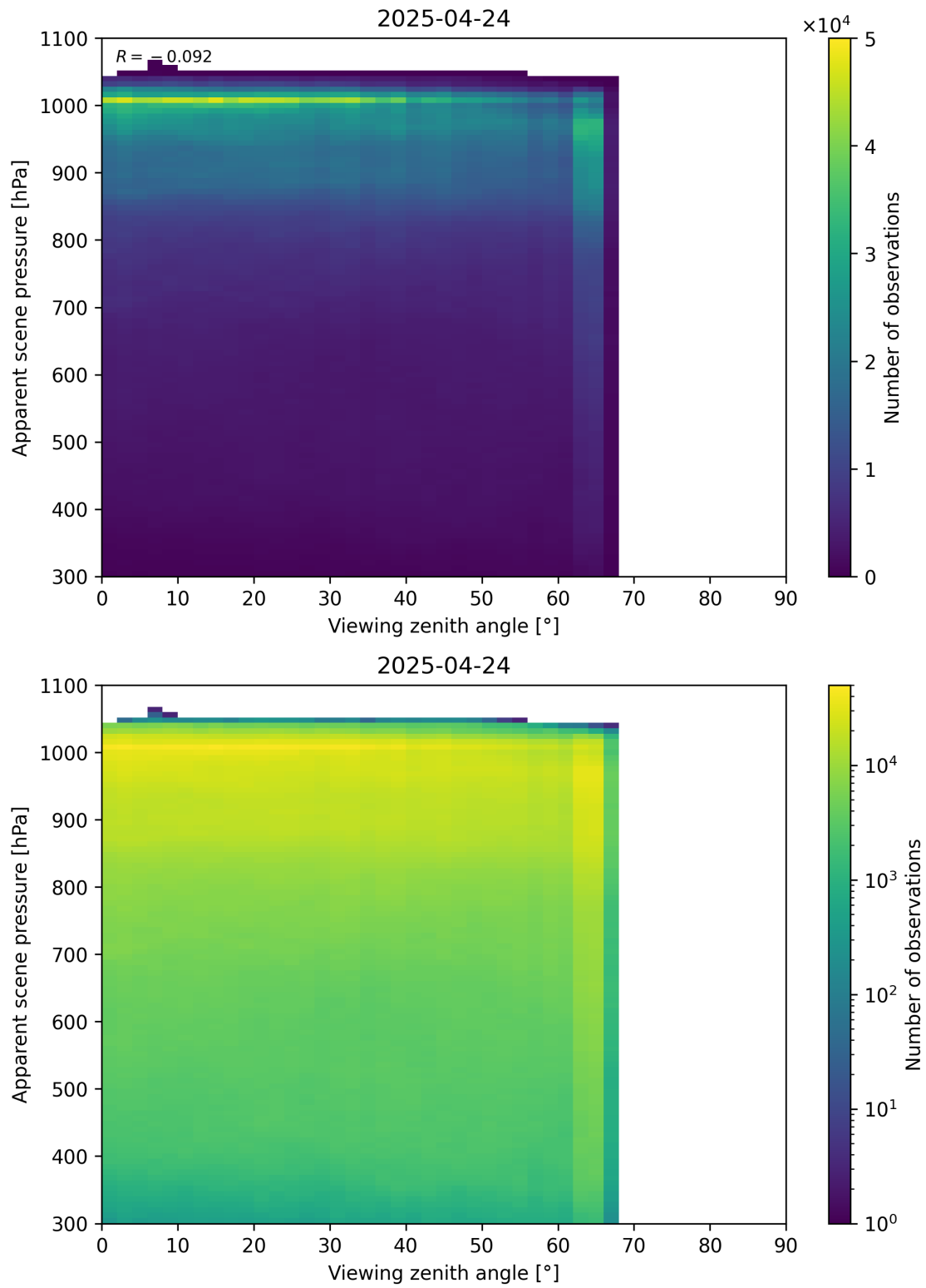
Figure 118: Scatter density plot of “Viewing zenith angle” against “Apparent scene pressure” for 2025-04-24 to 2025-04-25.
