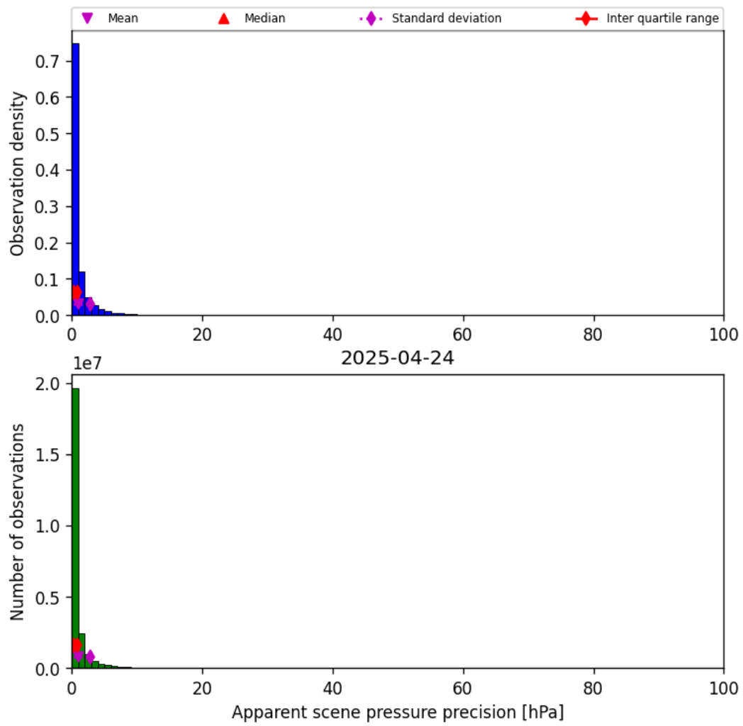
Figure 37: Histogram of “Apparent scene pressure precision” for 2025-04-24 to 2025-04-25
