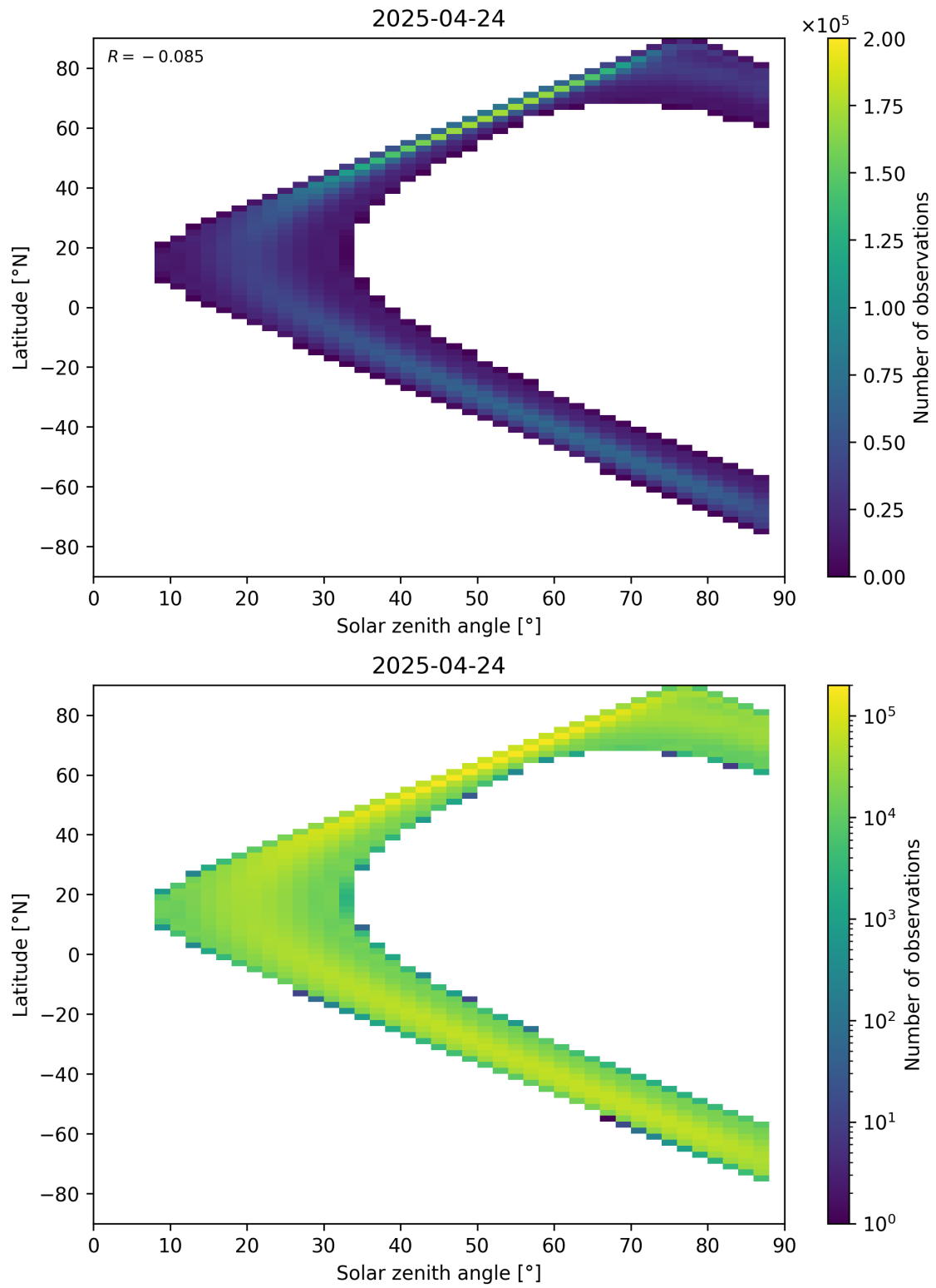
Figure 113: Scatter density plot of “Solar zenith angle” against “Latitude” for 2025-04-24 to 2025-04-25.
