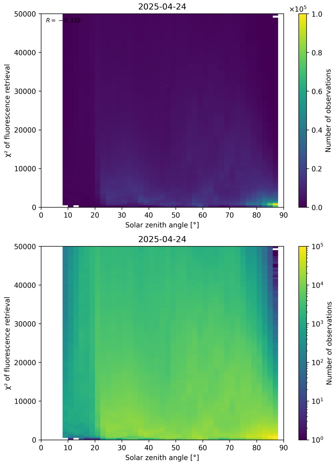
Figure 109: Scatter density plot of “Solar zenith angle” against “ \chi^2 of fluorescence retrieval” for 2025-04-24 to 2025-04-25.
