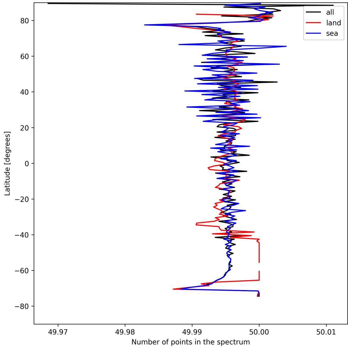
Figure 27: Zonal average of “Number of points in the spectrum” for 2025-04-24 to 2025-04-25.
