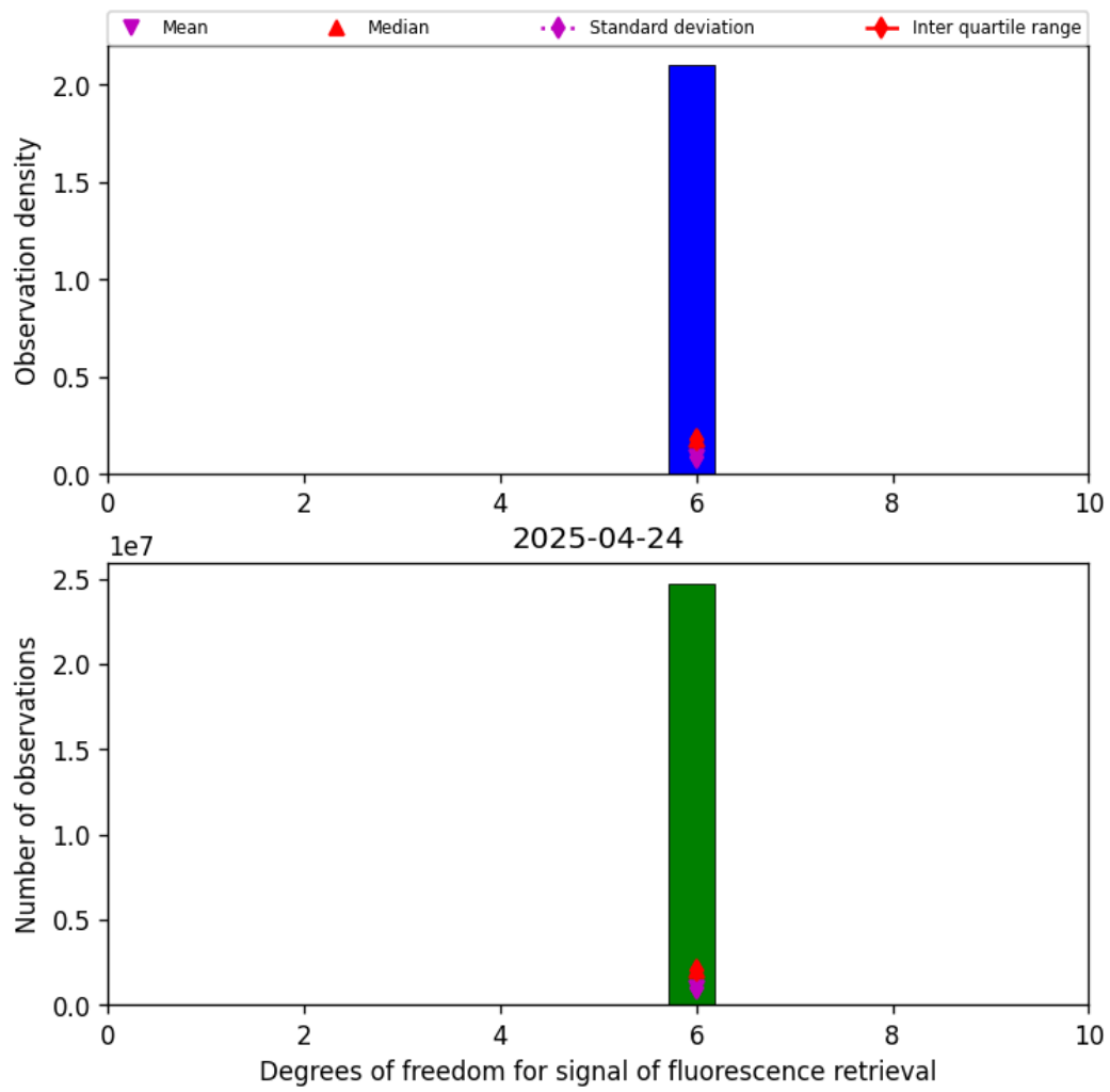
Figure 43: Histogram of “Degrees of freedom for signal of fluorescence retrieval” for 2025-04-24 to 2025-04-25
