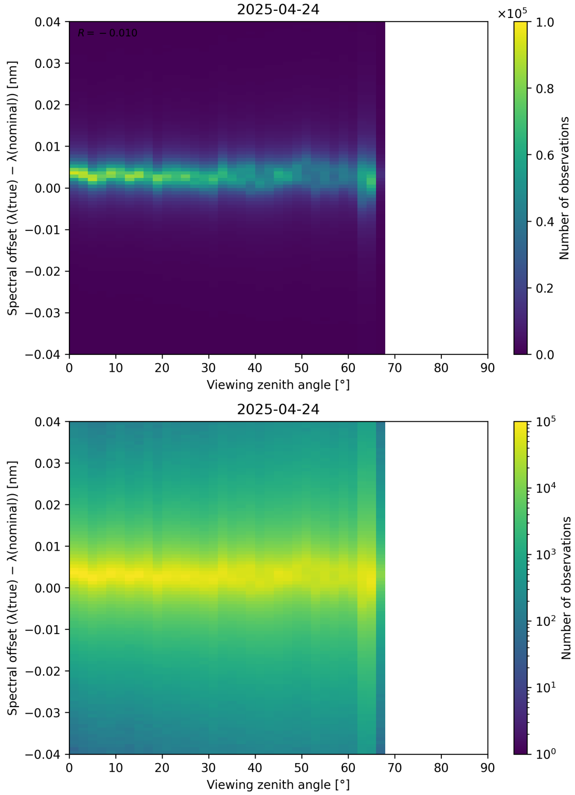
Figure 128: Scatter density plot of “Viewing zenith angle” against “Spectral offset ( \lambda_{\text{true}} - \lambda_{\text{nominal}} )” for 2025-04-24 to 2025-04-25.
