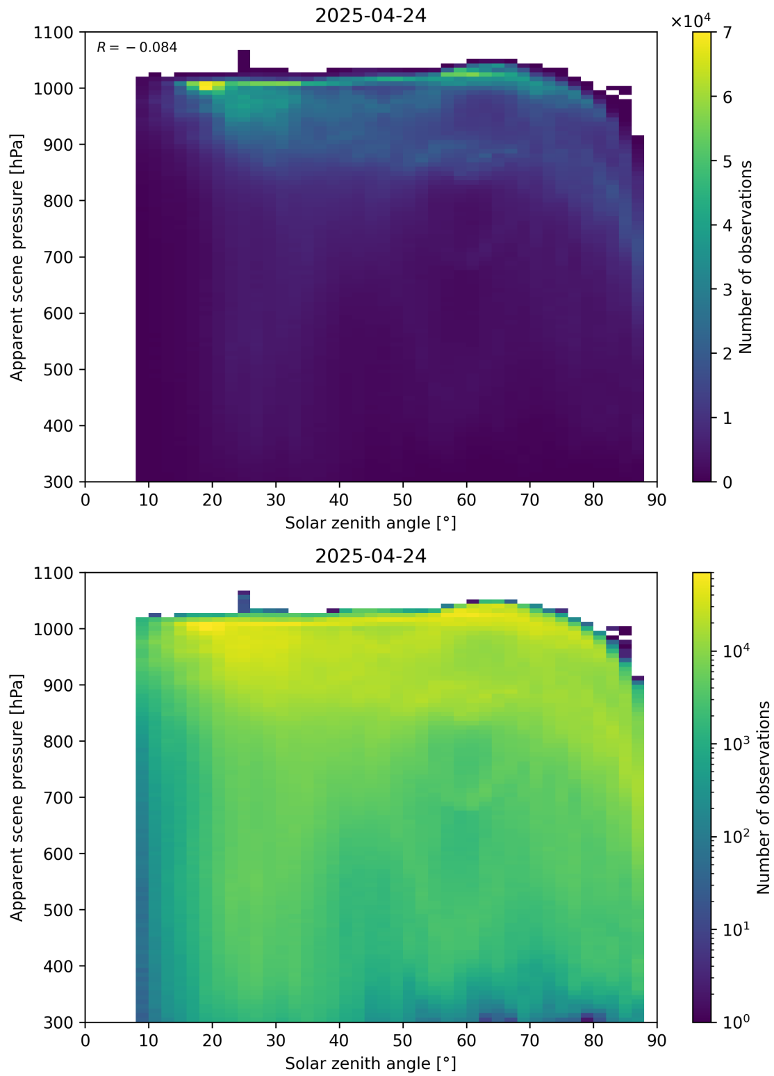
Figure 108: Scatter density plot of “Solar zenith angle” against “Apparent scene pressure” for 2025-04-24 to 2025-04-25.
