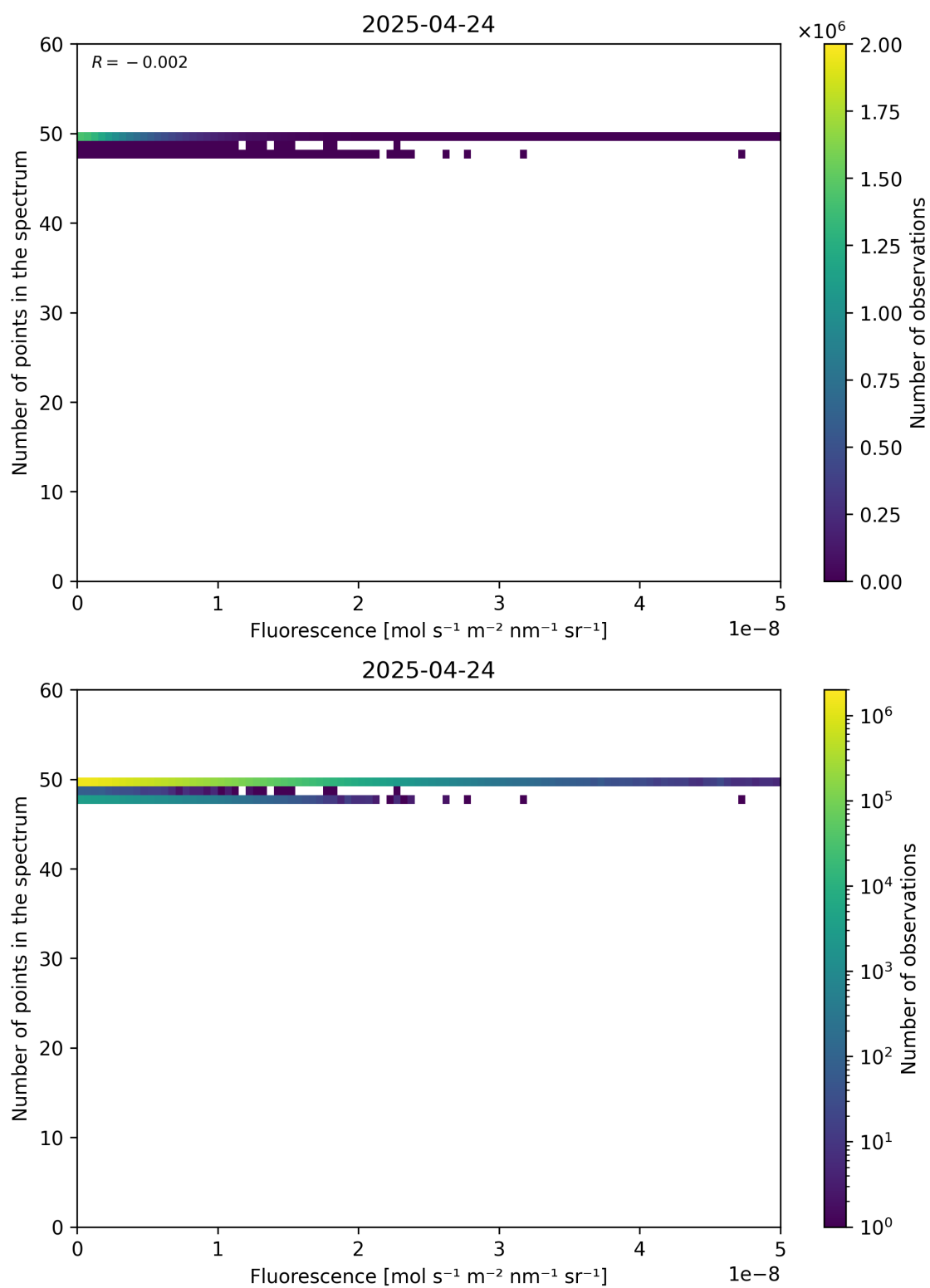
Figure 86: Scatter density plot of “Fluorescence” against “Number of points in the spectrum” for 2025-04-24 to 2025-04-25.
