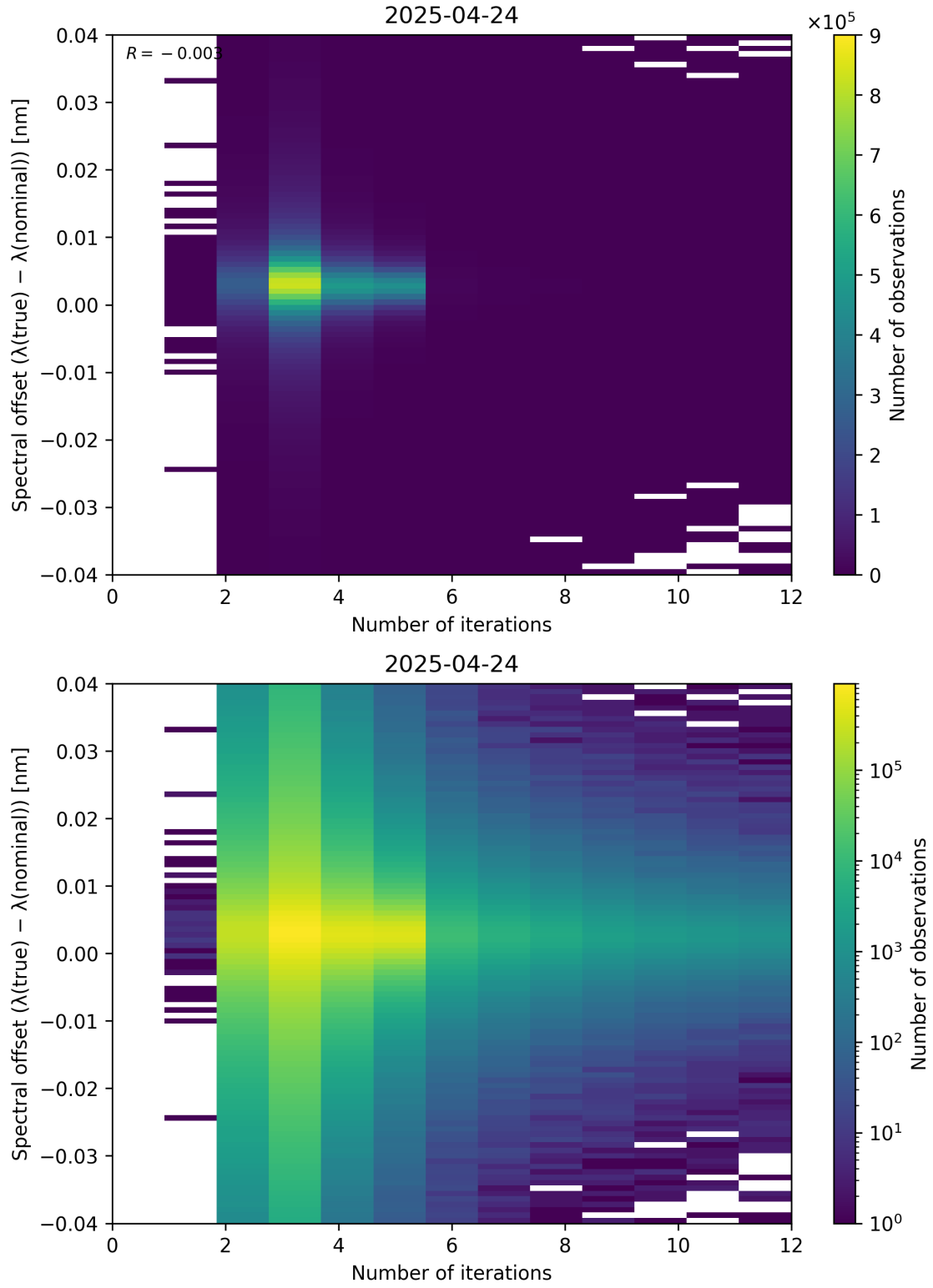
Figure 100: Scatter density plot of “Number of iterations” against “Spectral offset ( \lambda_{\text{true}} - \lambda_{\text{nominal}} )” for 2025-04-24 to 2025-04-25.
