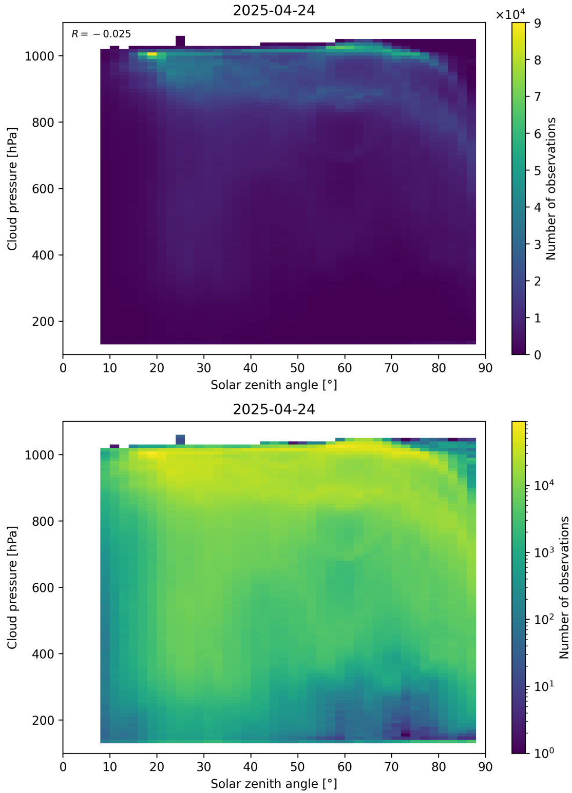
Figure 111: Scatter density plot of “Solar zenith angle” against “Cloud pressure” for 2025-04-24 to 2025-04-25.
