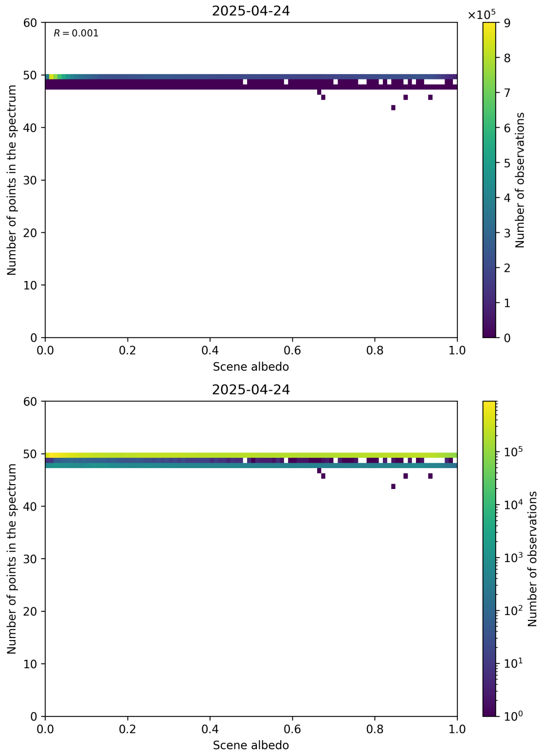
Figure 106: Scatter density plot of “Scene albedo” against “Number of points in the spectrum” for 2025-04-24 to 2025-04-25.
