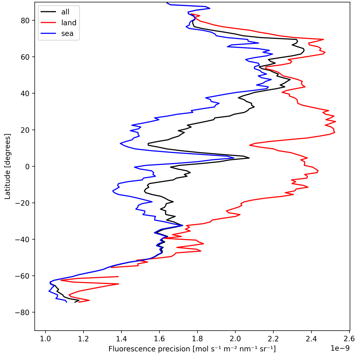
Figure 24: Zonal average of “Fluorescence precision” for 2025-04-24 to 2025-04-25.
