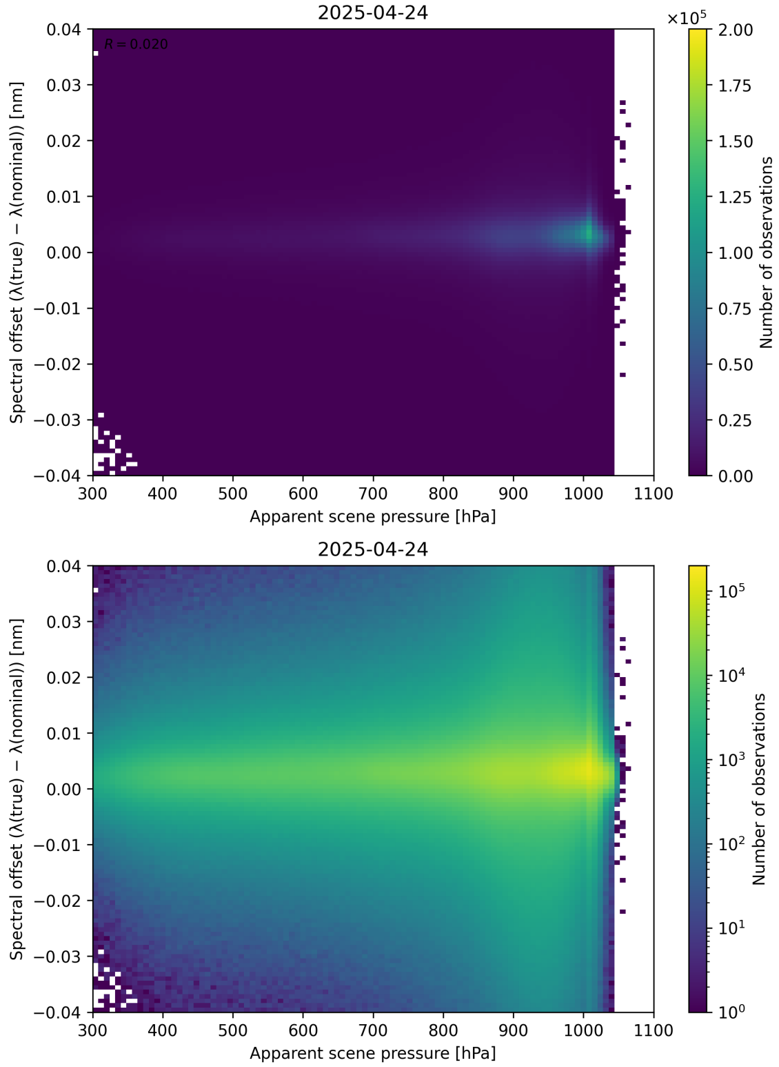
Figure 67: Scatter density plot of “Apparent scene pressure” against “Spectral offset ( \lambda_{\text{true}} - \lambda_{\text{nominal}} )” for 2025-04-24 to 2025-04-25.
