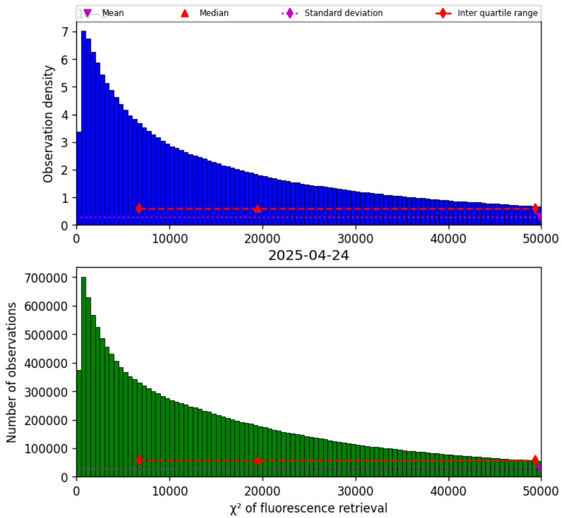
Figure 42: Histogram of “ \chi^2 of fluorescence retrieval” for 2025-04-24 to 2025-04-25
