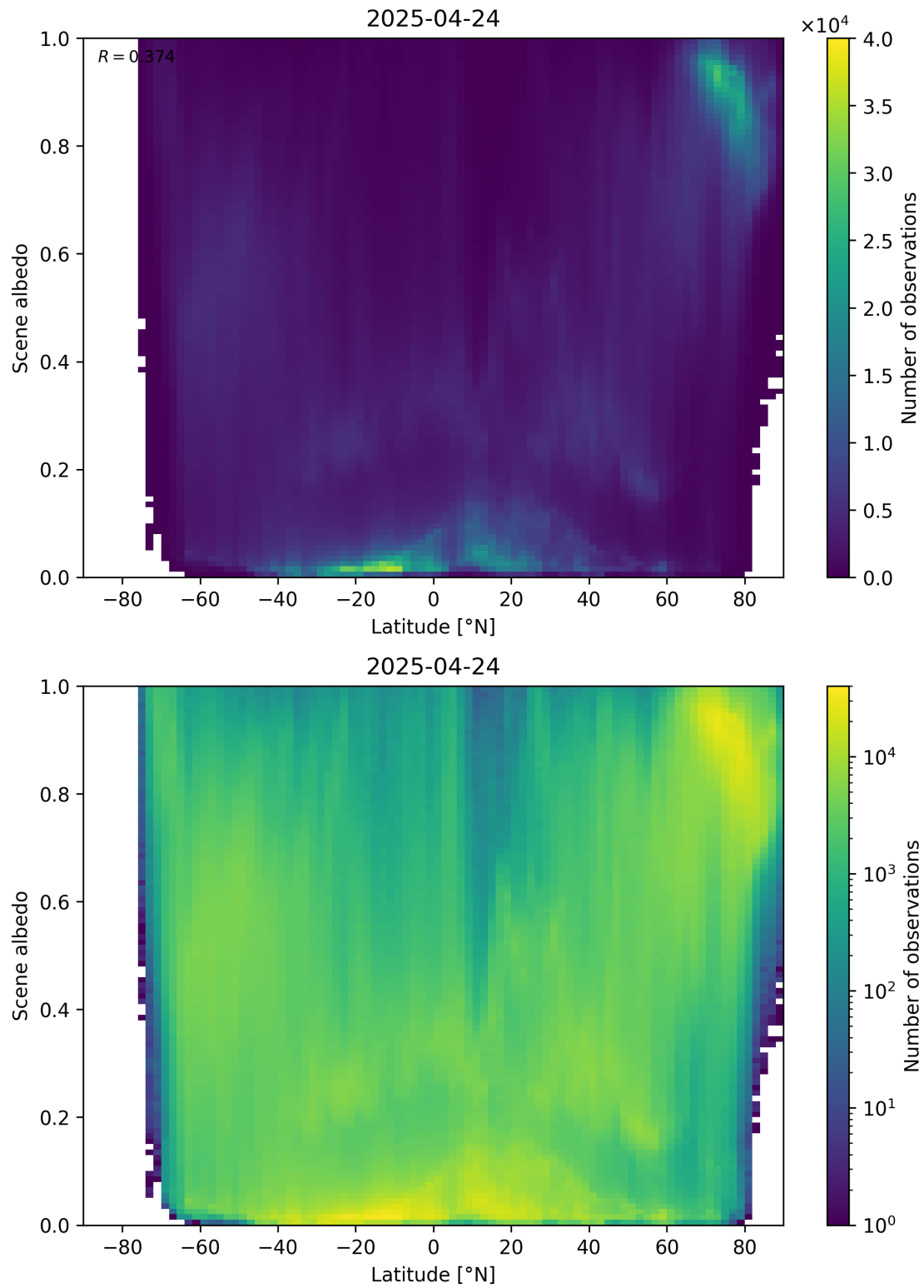
Figure 95: Scatter density plot of “Latitude” against “Scene albedo” for 2025-04-24 to 2025-04-25.
