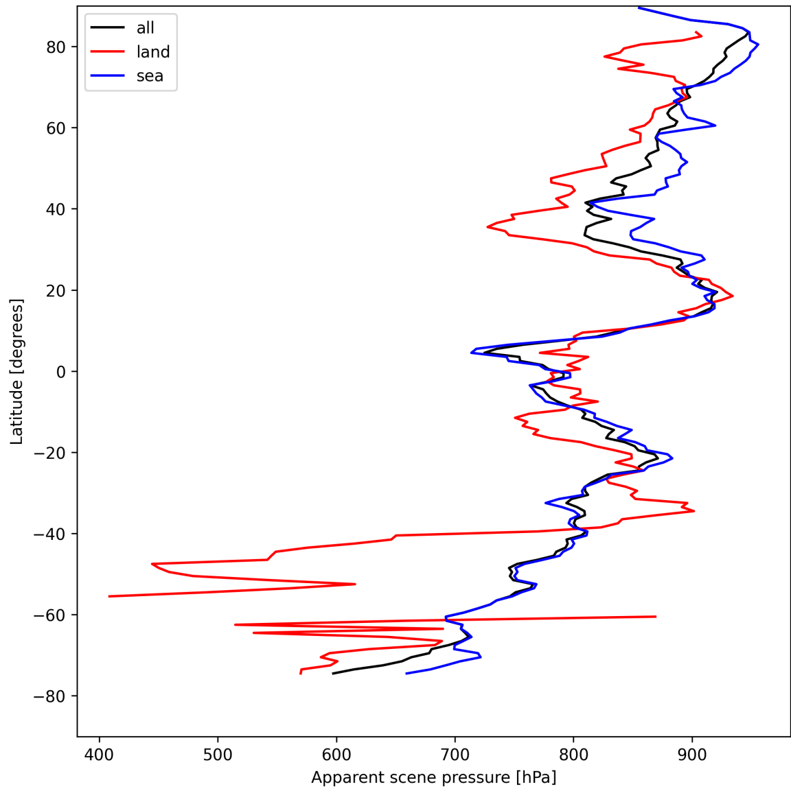
Figure 19: Zonal average of “Apparent scene pressure” for 2025-04-24 to 2025-04-25.
