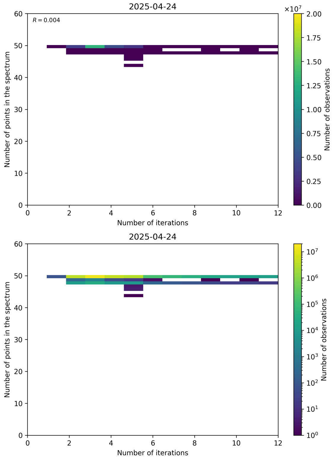
Figure 99: Scatter density plot of “Number of iterations” against “Number of points in the spectrum” for 2025-04-24 to 2025-04-25.
