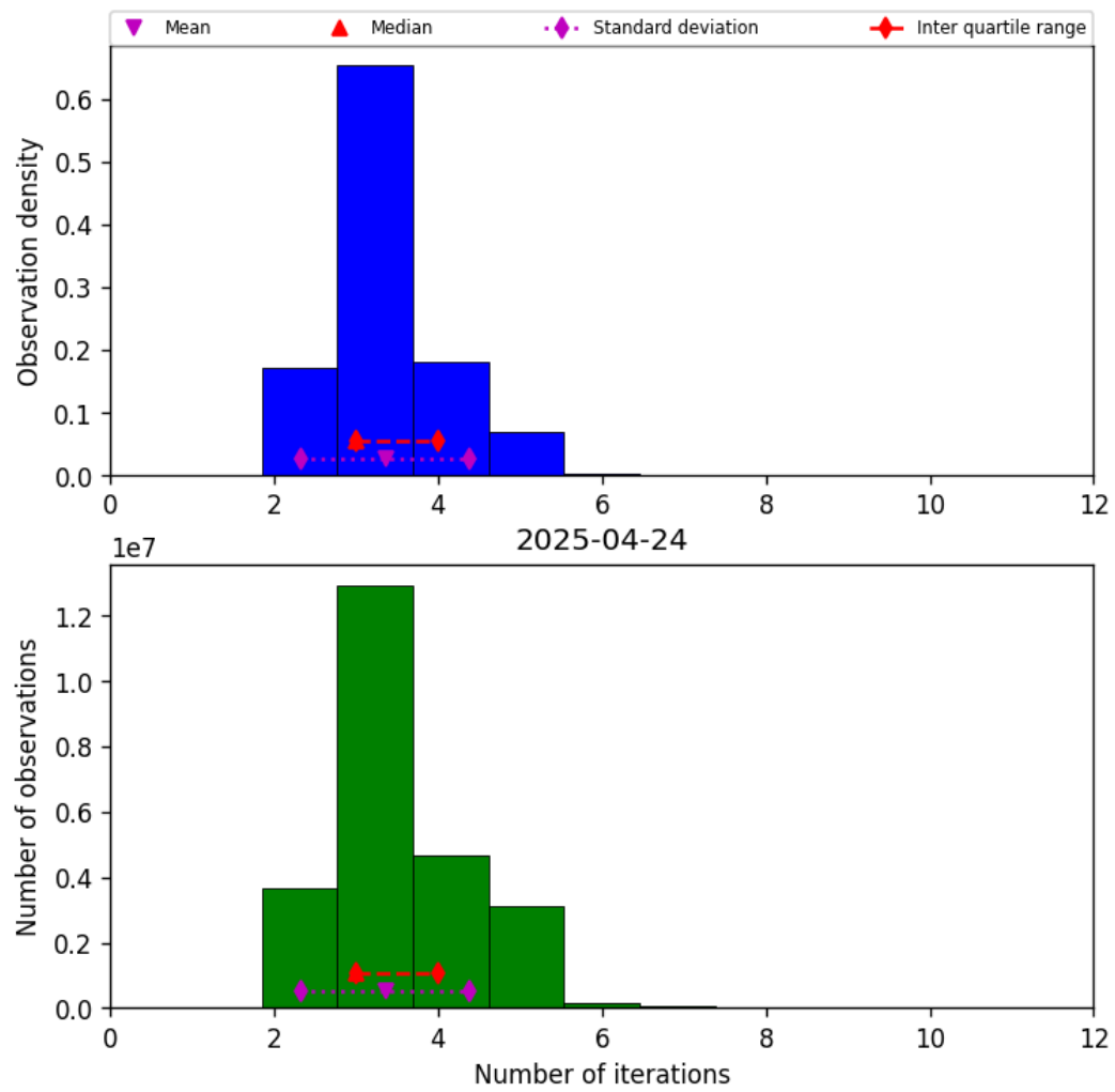
Figure 39: Histogram of “Number of iterations” for 2025-04-24 to 2025-04-25
