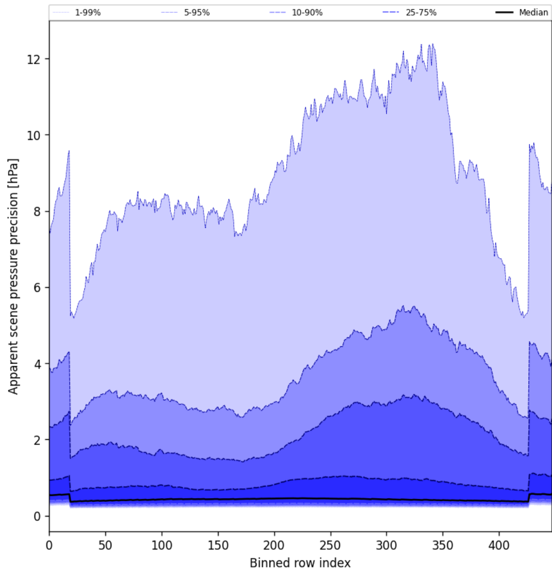
Figure 54: Along track statistics of “Apparent scene pressure precision” for 2025-04-24 to 2025-04-25
