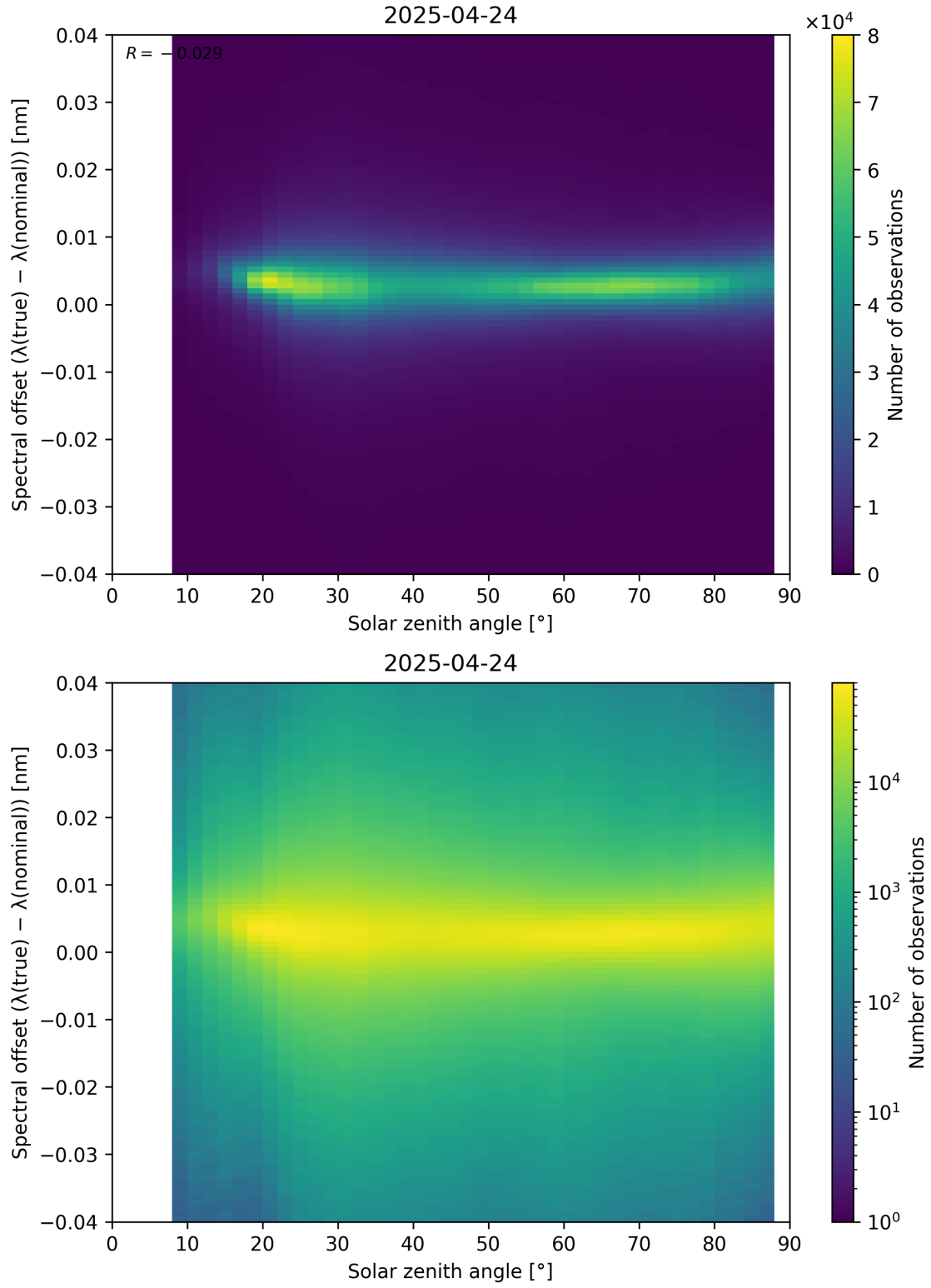
Figure 117: Scatter density plot of “Solar zenith angle” against “Spectral offset ( \lambda_{\text{true}} - \lambda_{\text{nominal}} )” for 2025-04-24 to 2025-04-25.
