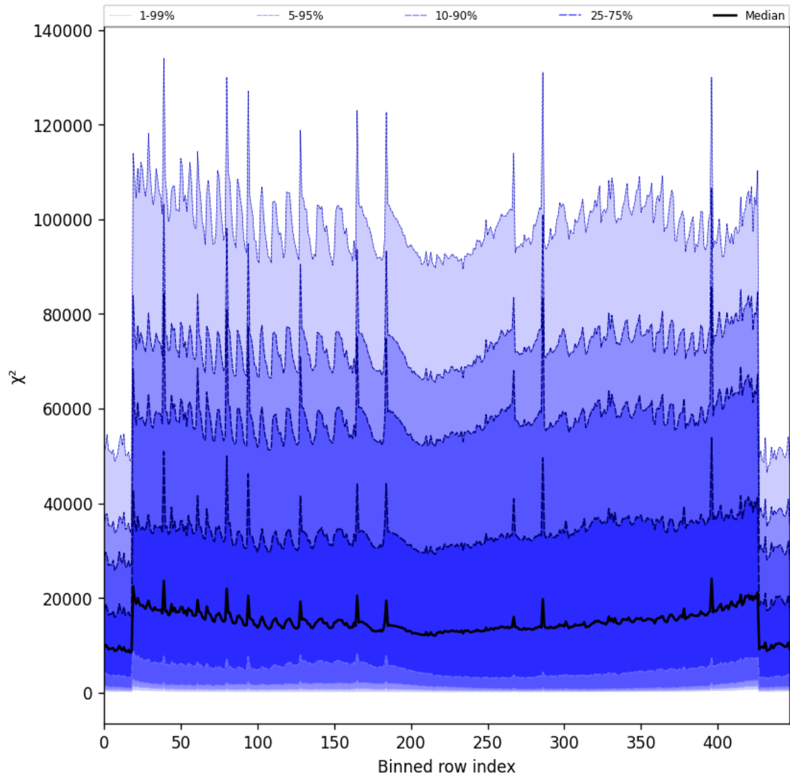
Figure 55: Along track statistics of “ \chi^2 ” for 2025-04-24 to 2025-04-25
