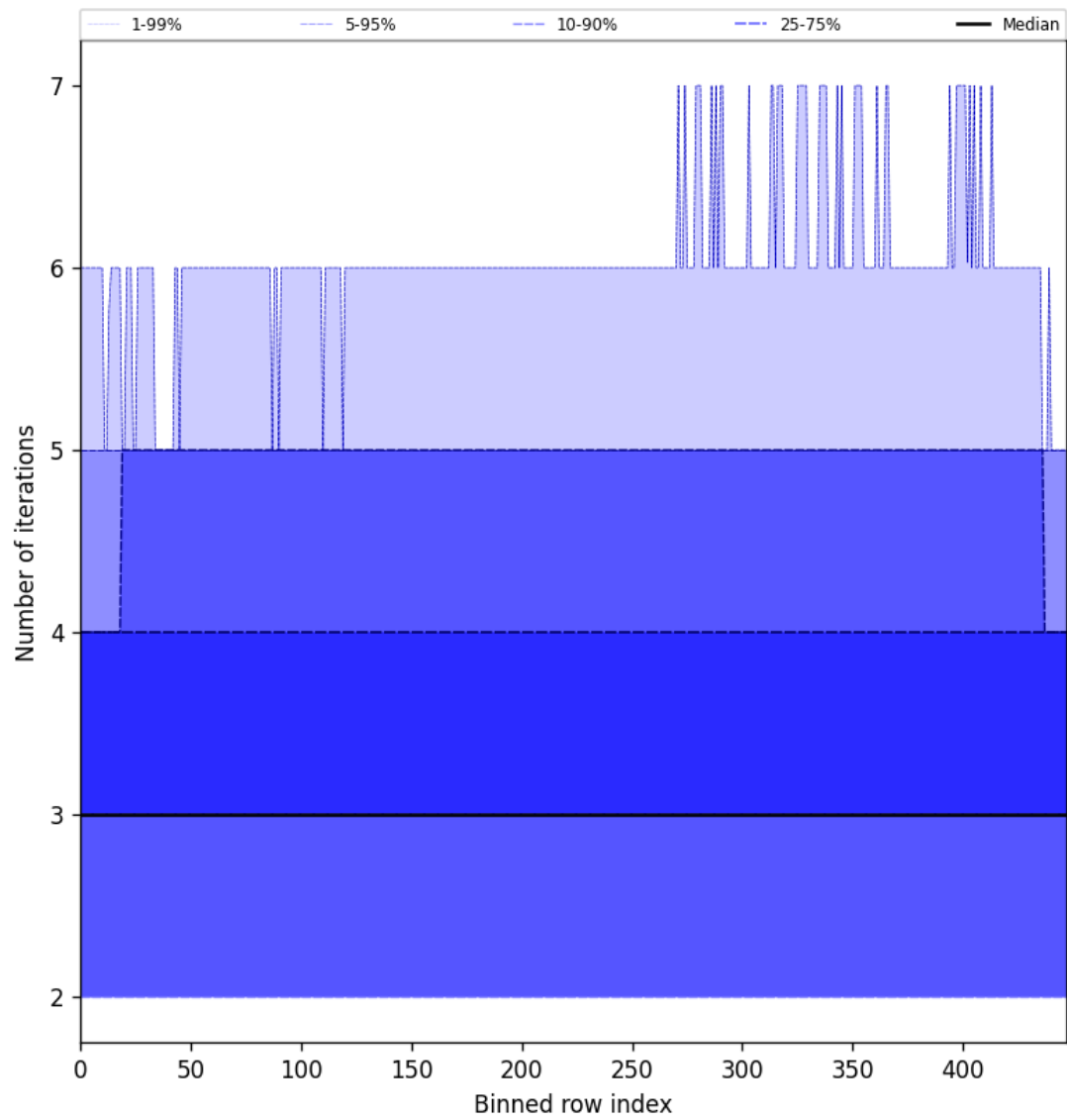
Figure 56: Along track statistics of “Number of iterations” for 2025-04-24 to 2025-04-25
