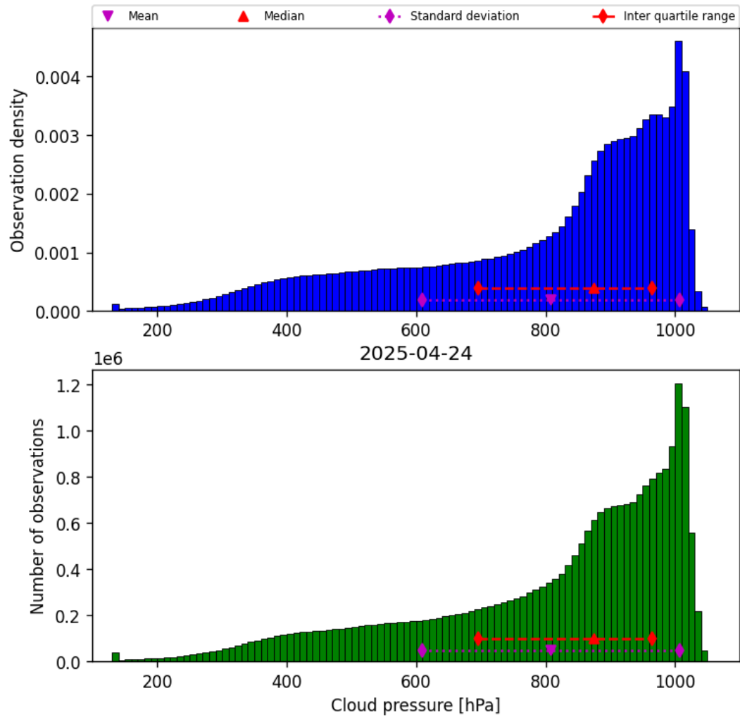
Figure 30: Histogram of “Cloud pressure” for 2025-04-24 to 2025-04-25
