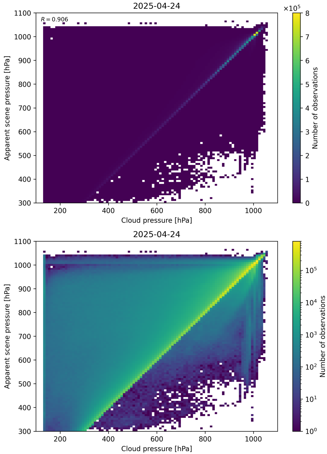
Figure 77: Scatter density plot of “Cloud pressure” against “Apparent scene pressure” for 2025-04-24 to 2025-04-25.
