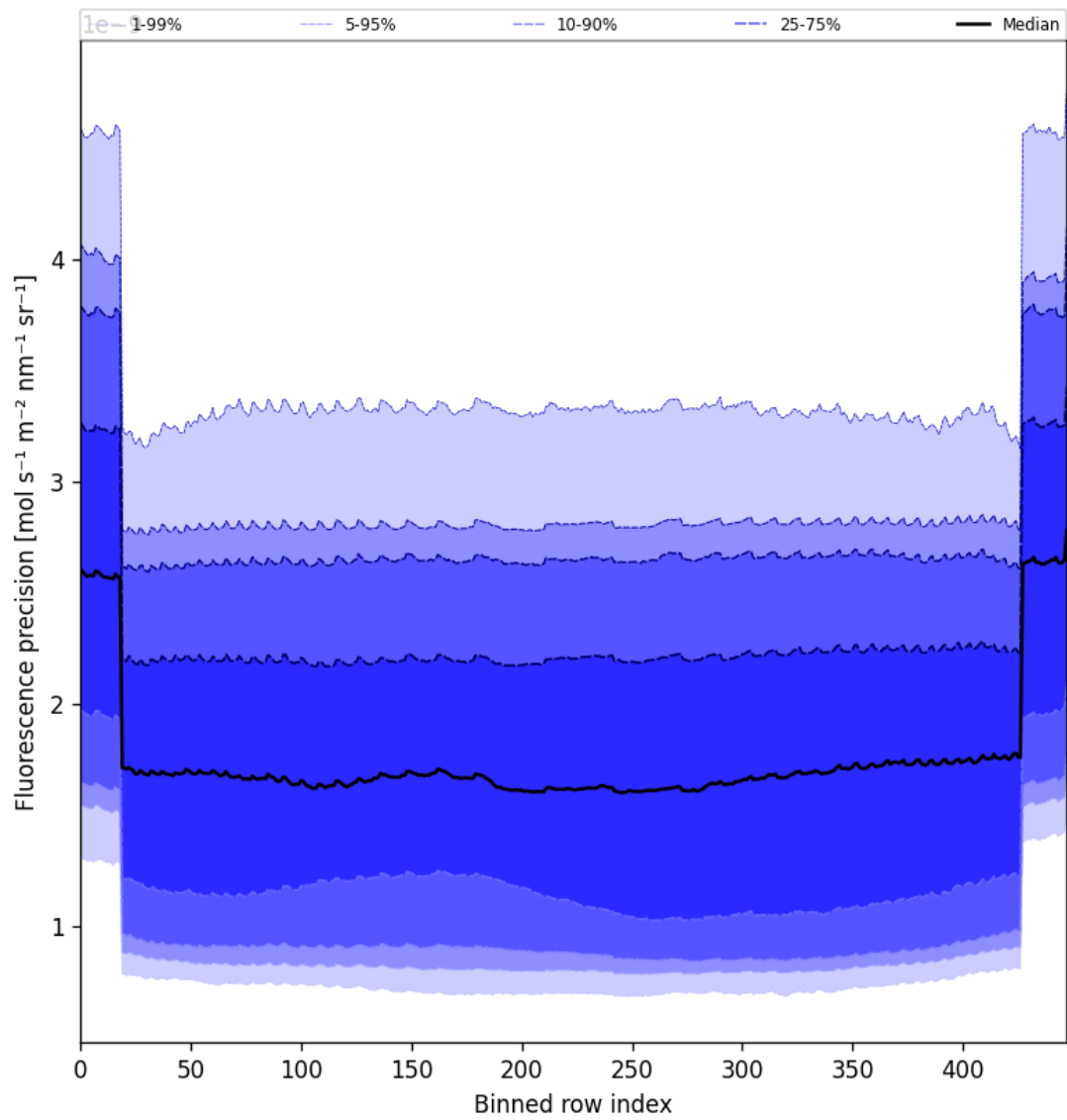
Figure 58: Along track statistics of “Fluorescence precision” for 2025-04-24 to 2025-04-25
