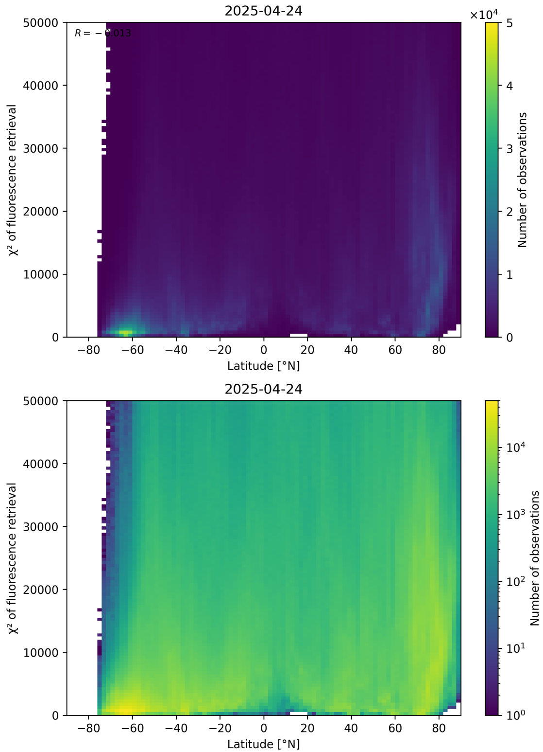
Figure 89: Scatter density plot of “Latitude” against “ \chi^2 of fluorescence retrieval” for 2025-04-24 to 2025-04-25.
