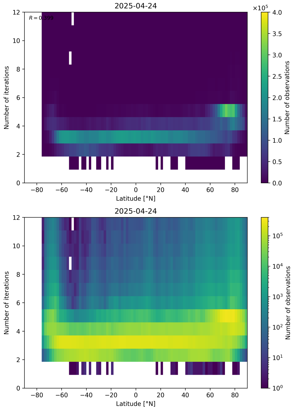
Figure 93: Scatter density plot of “Latitude” against “Number of iterations” for 2025-04-24 to 2025-04-25.
