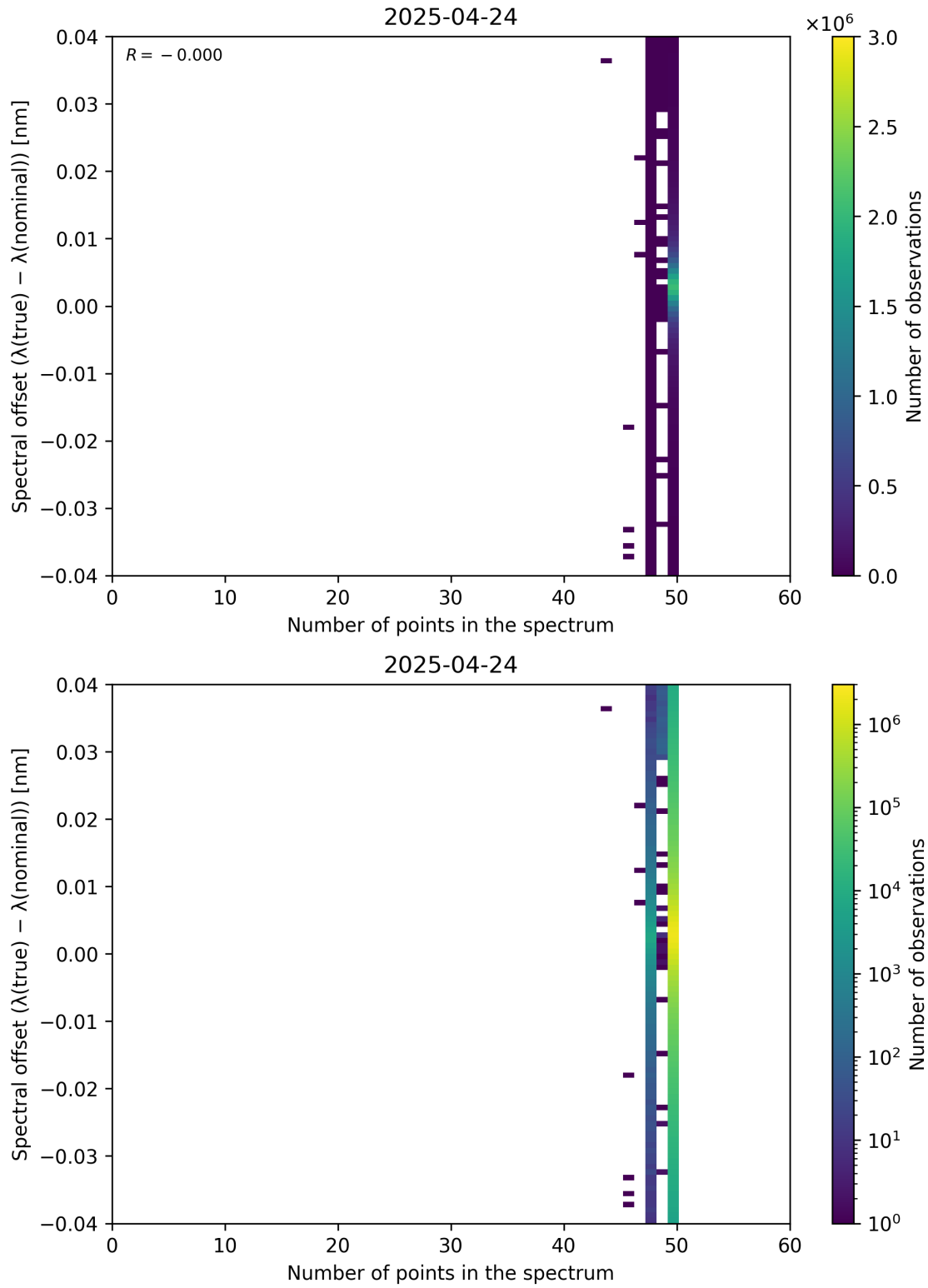
Figure 101: Scatter density plot of “Number of points in the spectrum” against “Spectral offset ( \lambda_{\text{true}} - \lambda_{\text{nominal}} )” for 2025-04-24 to 2025-04-25.
