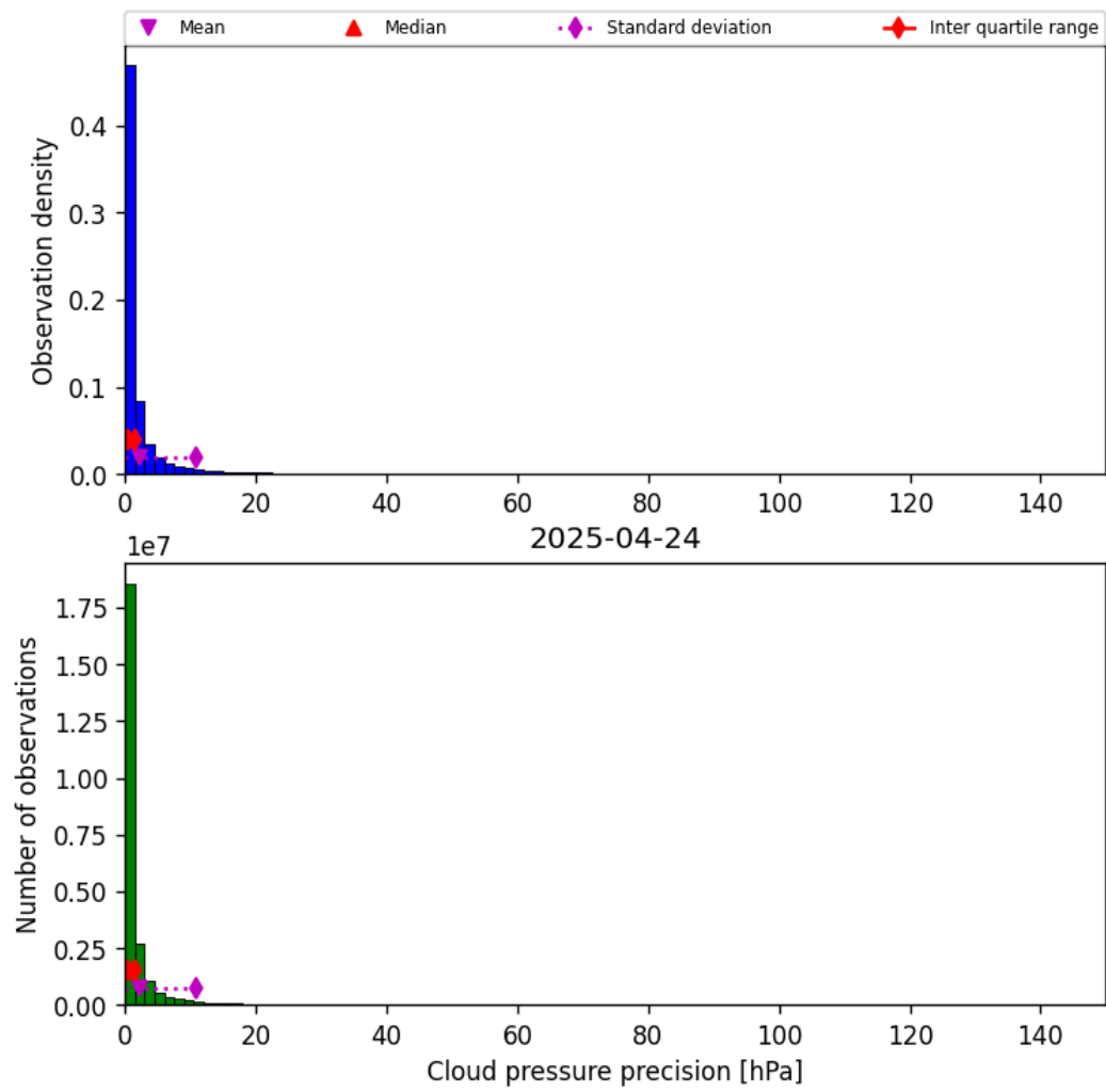
Figure 31: Histogram of “Cloud pressure precision” for 2025-04-24 to 2025-04-25
