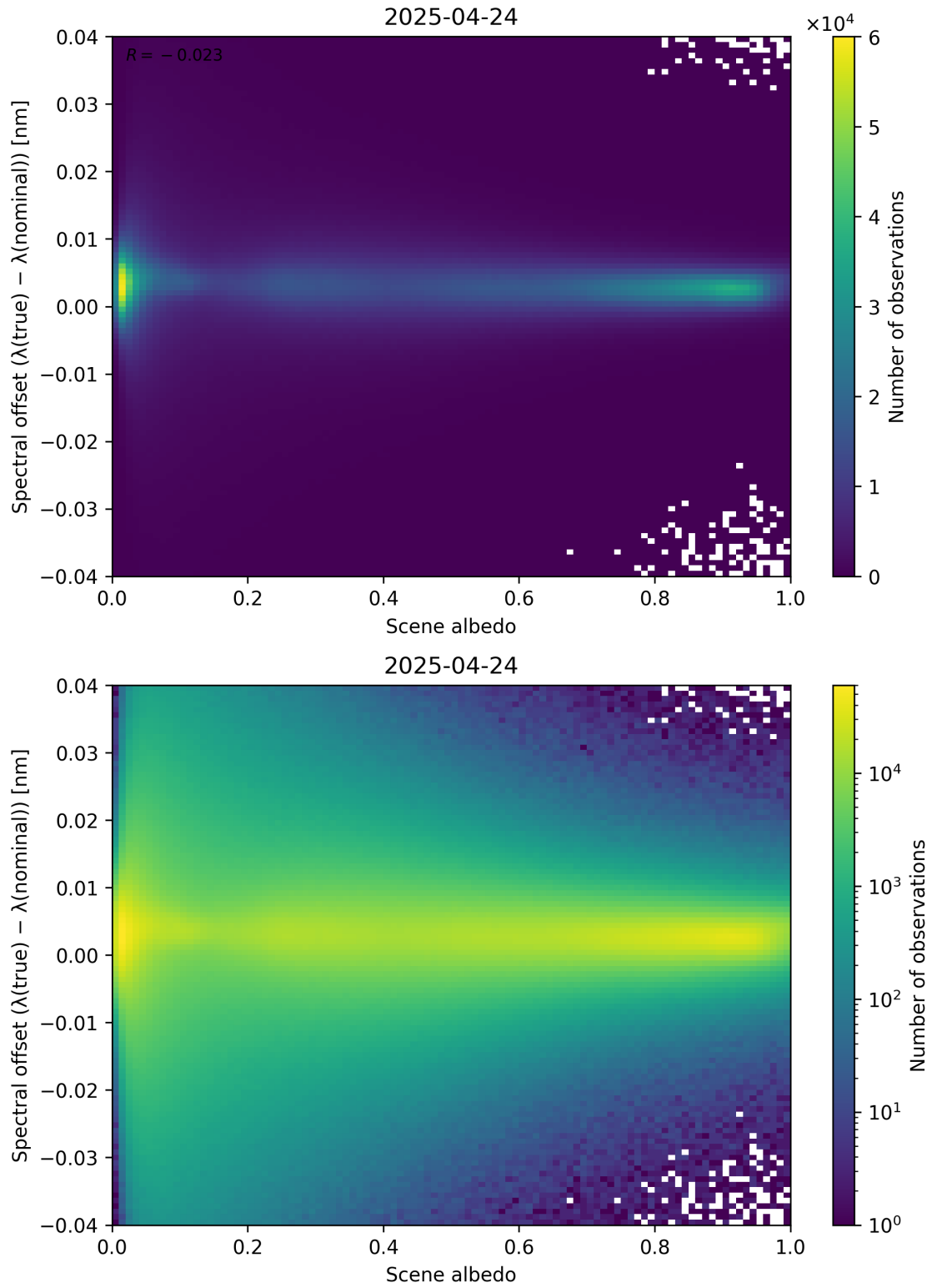
Figure 107: Scatter density plot of “Scene albedo” against “Spectral offset ( \lambda_{\text{true}} - \lambda_{\text{nominal}} )” for 2025-04-24 to 2025-04-25.
