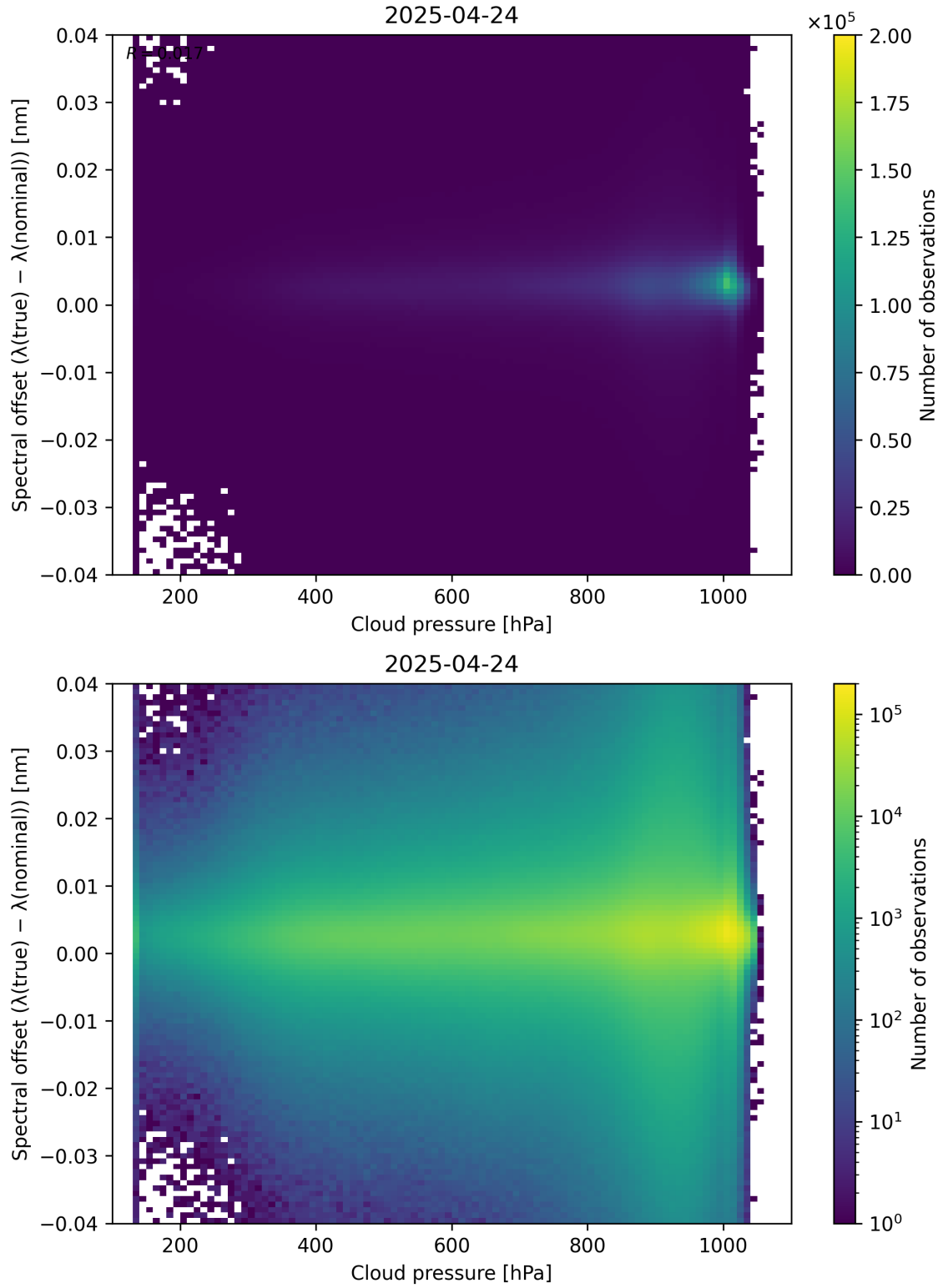
Figure 84: Scatter density plot of “Cloud pressure” against “Spectral offset ( \lambda_{\text{true}} - \lambda_{\text{nominal}} )” for 2025-04-24 to 2025-04-25.
