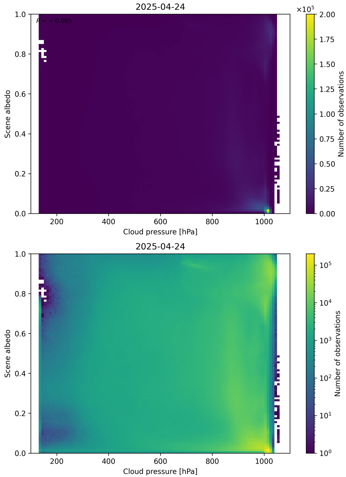
Figure 83: Scatter density plot of “Cloud pressure” against “Scene albedo” for 2025-04-24 to 2025-04-25.
