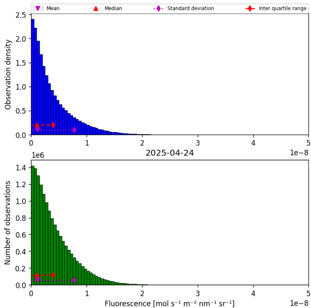
Figure 40: Histogram of “Fluorescence” for 2025-04-24 to 2025-04-25
