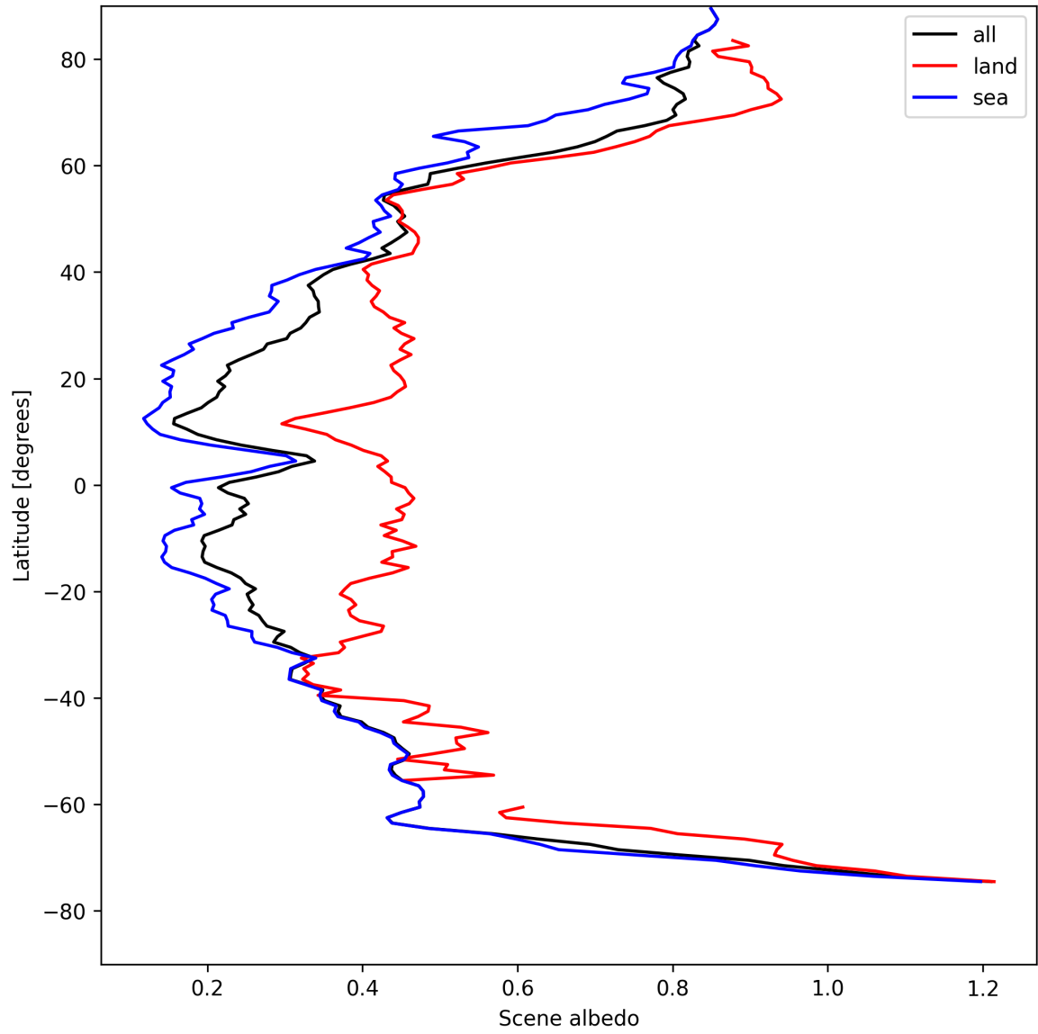
Figure 17: Zonal average of “Scene albedo” for 2025-04-24 to 2025-04-25.
