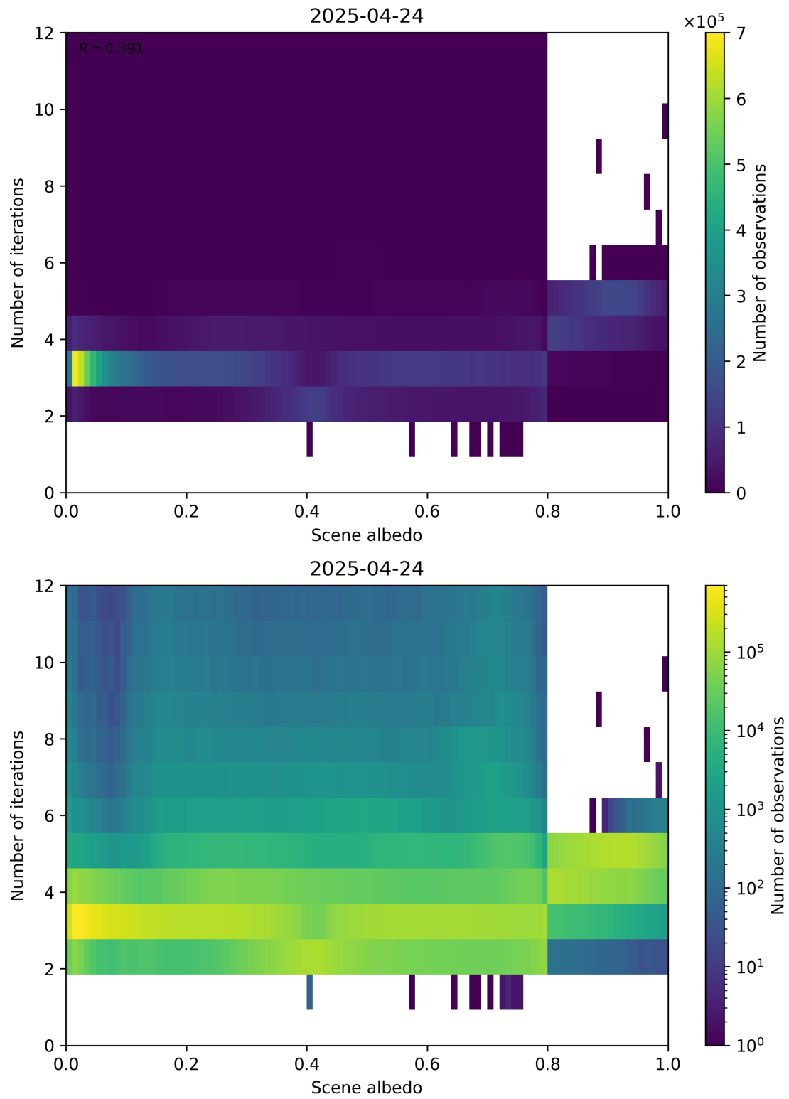
Figure 105: Scatter density plot of “Scene albedo” against “Number of iterations” for 2025-04-24 to 2025-04-25.
