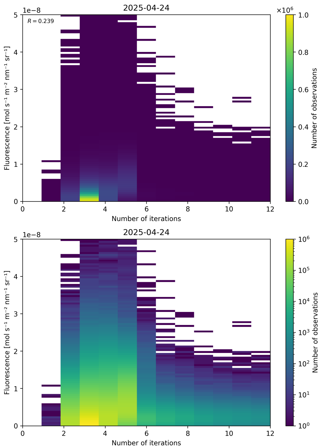
Figure 98: Scatter density plot of “Number of iterations” against “Fluorescence” for 2025-04-24 to 2025-04-25.
