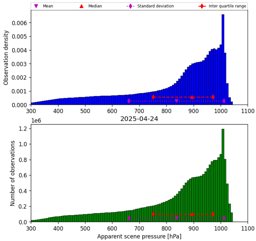
Figure 36: Histogram of “Apparent scene pressure” for 2025-04-24 to 2025-04-25
