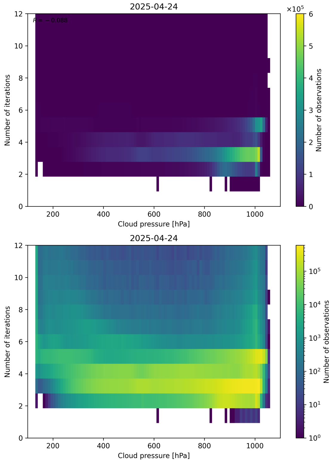
Figure 81: Scatter density plot of “Cloud pressure” against “Number of iterations” for 2025-04-24 to 2025-04-25.
