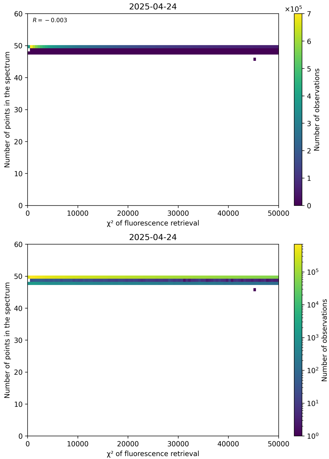
Figure 68: Scatter density plot of “ \chi^2 of fluorescence retrieval” against “Number of points in the spectrum” for 2025-04-24 to 2025-04-25.
