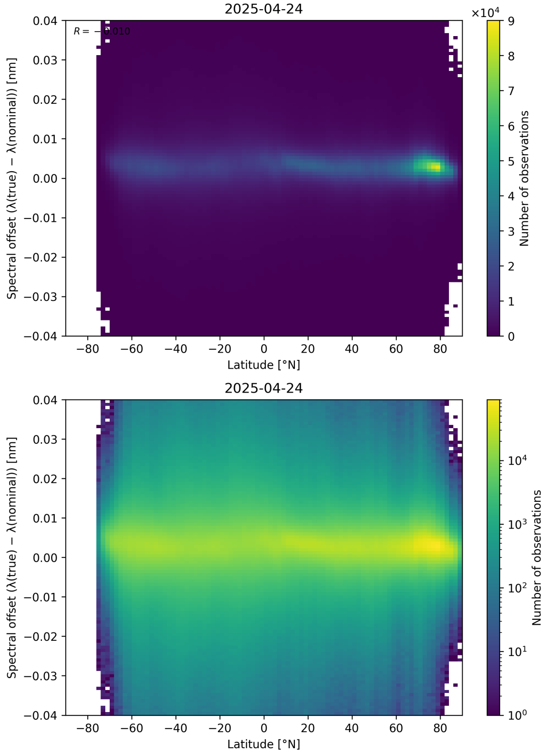
Figure 96: Scatter density plot of “Latitude” against “Spectral offset ( \lambda_{\text{true}} - \lambda_{\text{nominal}} )” for 2025-04-24 to 2025-04-25.
