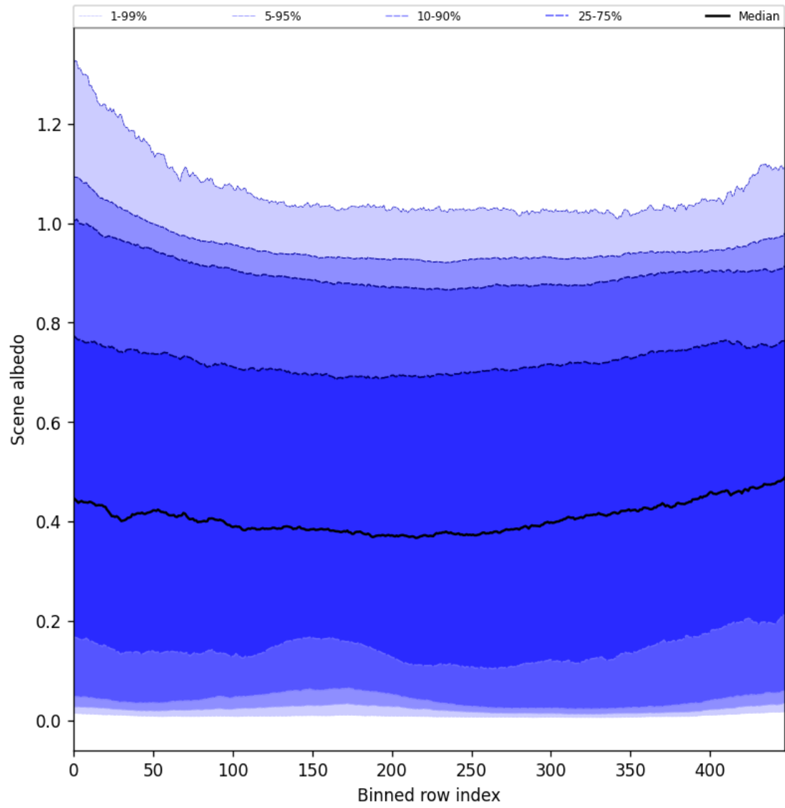
Figure 51: Along track statistics of “Scene albedo” for 2025-04-24 to 2025-04-25
