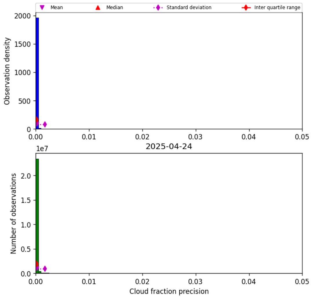
Figure 33: Histogram of “Cloud fraction precision” for 2025-04-24 to 2025-04-25
