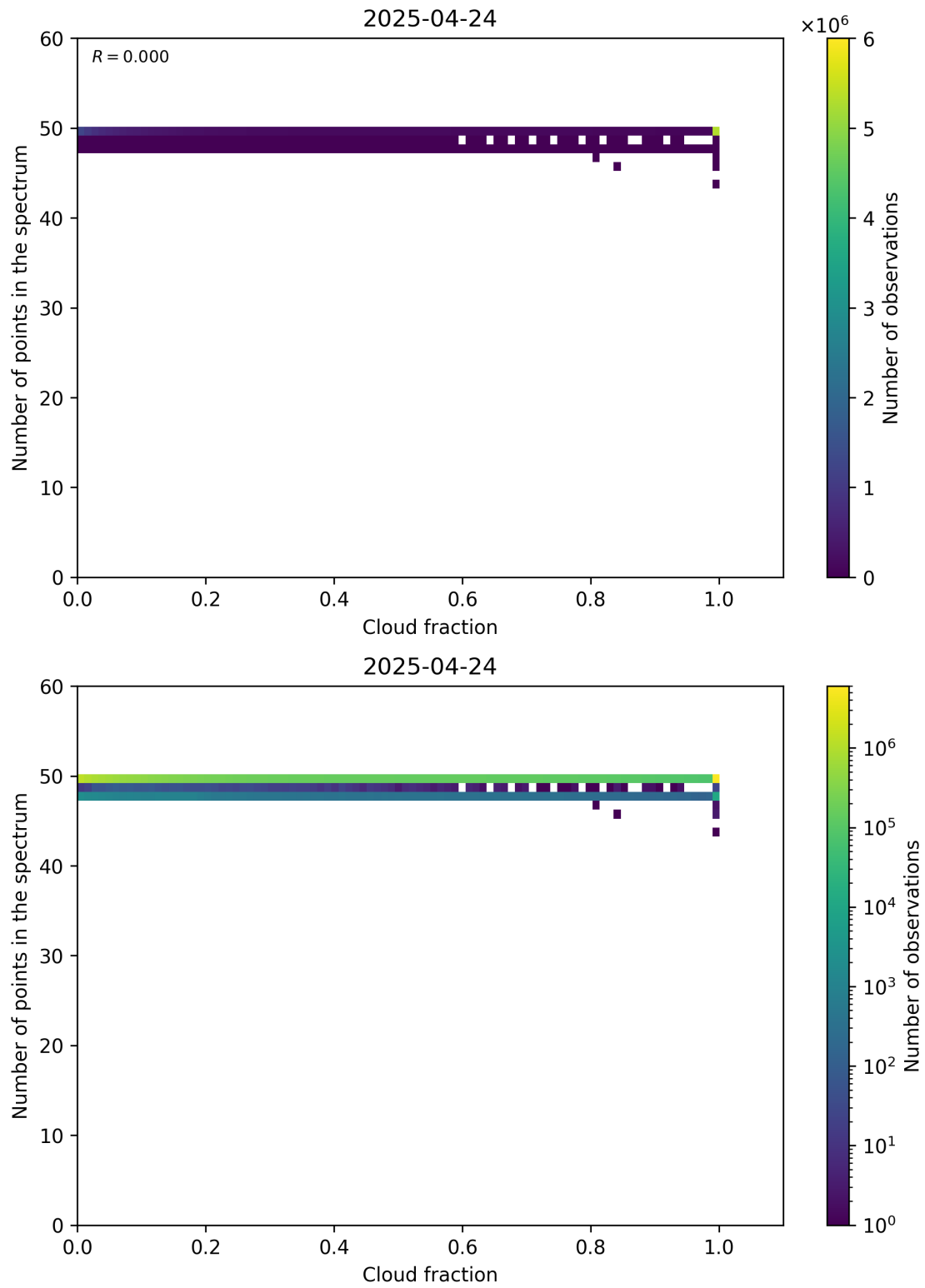
Figure 74: Scatter density plot of “Cloud fraction” against “Number of points in the spectrum” for 2025-04-24 to 2025-04-25.
