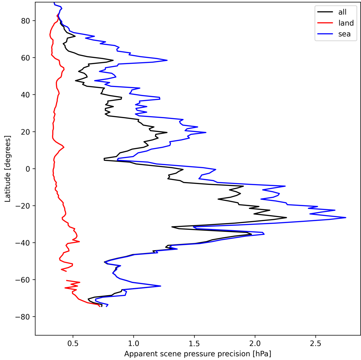
Figure 20: Zonal average of “Apparent scene pressure precision” for 2025-04-24 to 2025-04-25.
