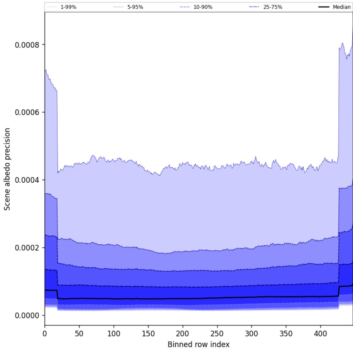
Figure 52: Along track statistics of “Scene albedo precision” for 2025-04-24 to 2025-04-25
