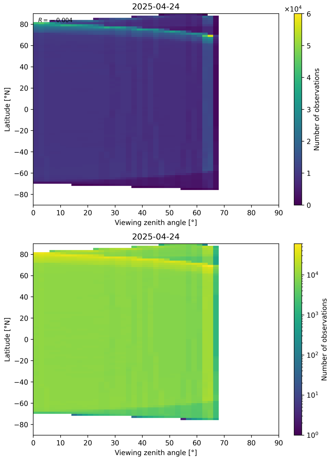
Figure 123: Scatter density plot of “Viewing zenith angle” against “Latitude” for 2025-04-24 to 2025-04-25.
