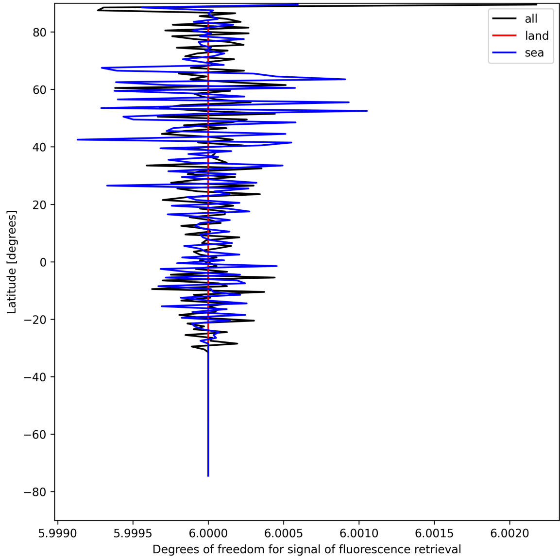
Figure 26: Zonal average of “Degrees of freedom for signal of fluorescence retrieval” for 2025-04-24 to 2025-04-25.
