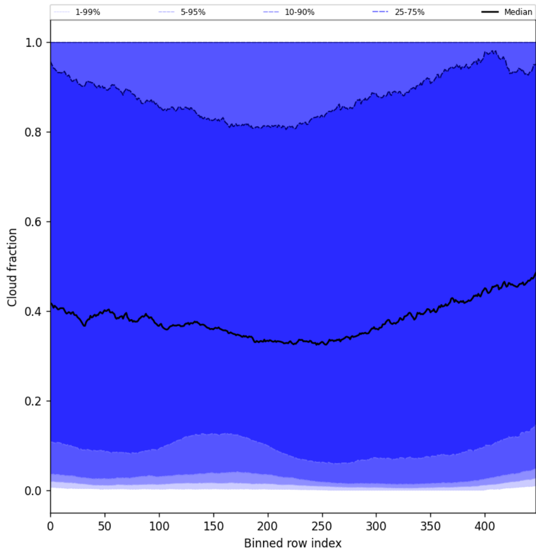
Figure 49: Along track statistics of “Cloud fraction” for 2025-04-24 to 2025-04-25
