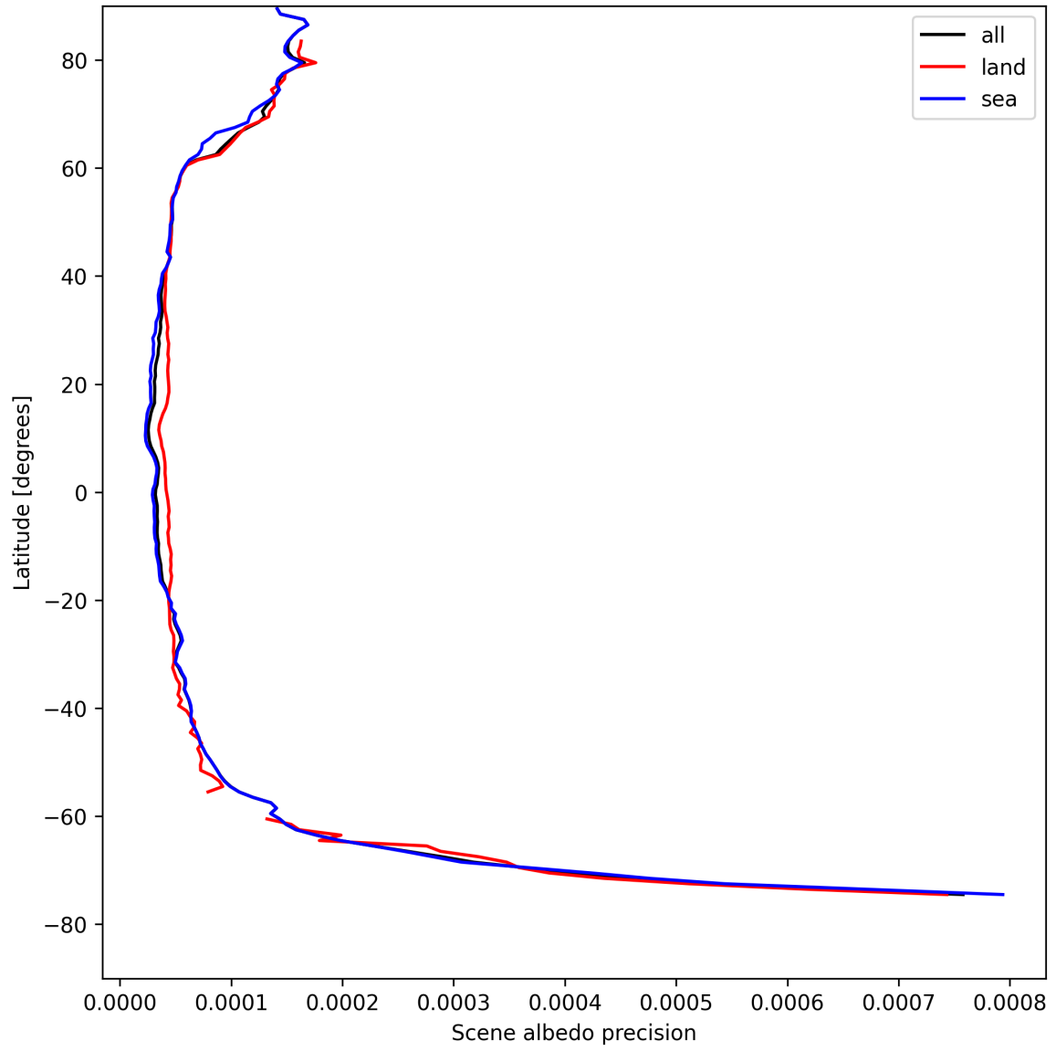
Figure 18: Zonal average of “Scene albedo precision” for 2025-04-24 to 2025-04-25.
