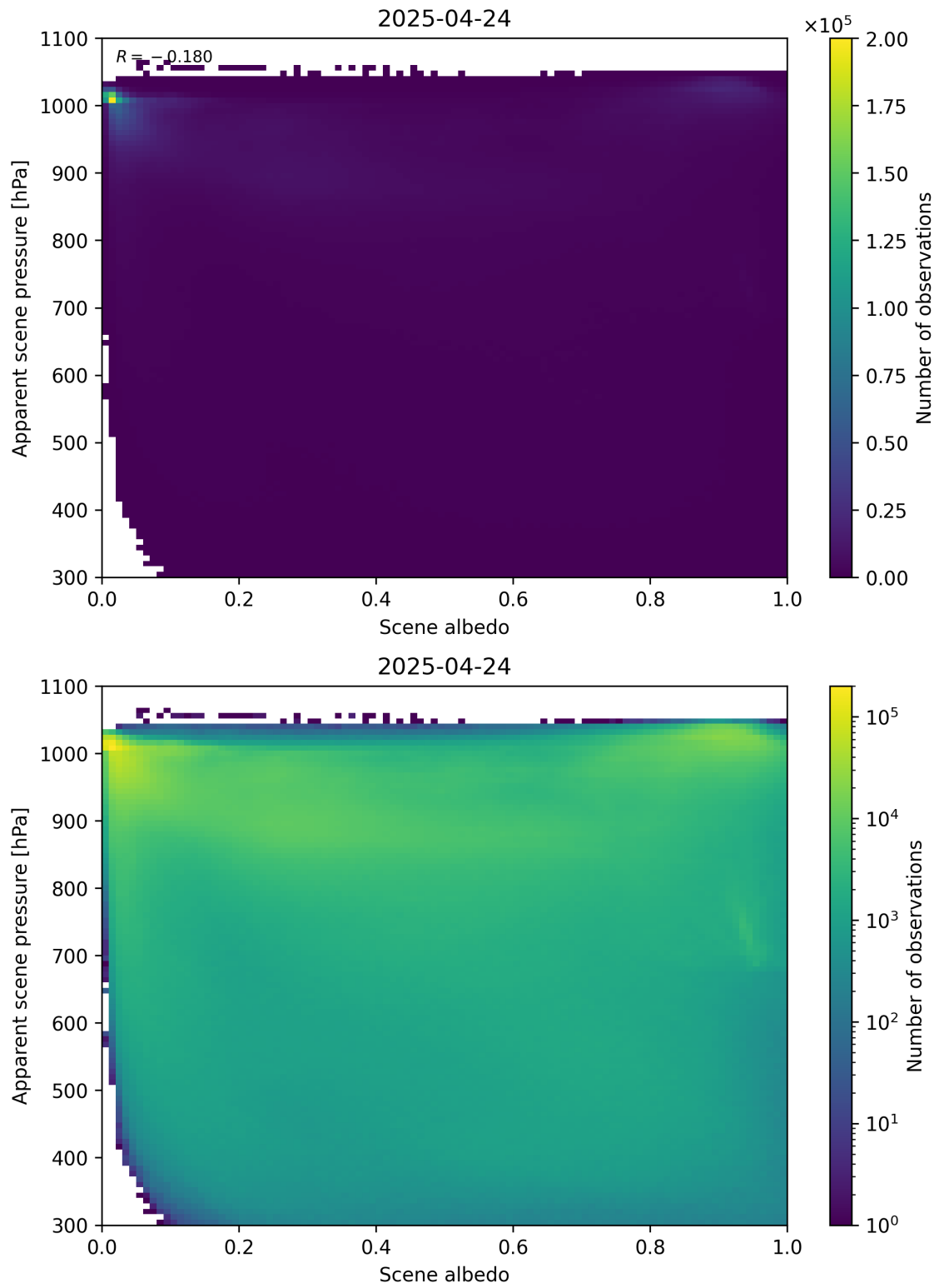
Figure 102: Scatter density plot of “Scene albedo” against “Apparent scene pressure” for 2025-04-24 to 2025-04-25.
