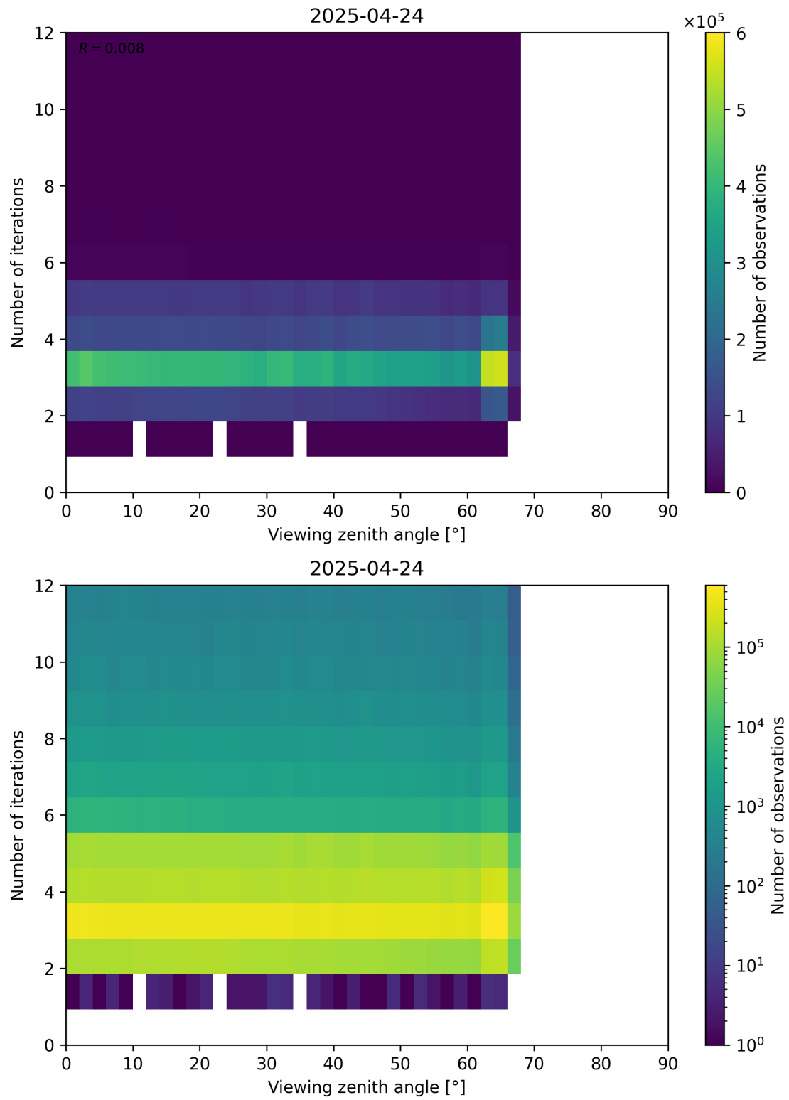
Figure 124: Scatter density plot of “Viewing zenith angle” against “Number of iterations” for 2025-04-24 to 2025-04-25.
