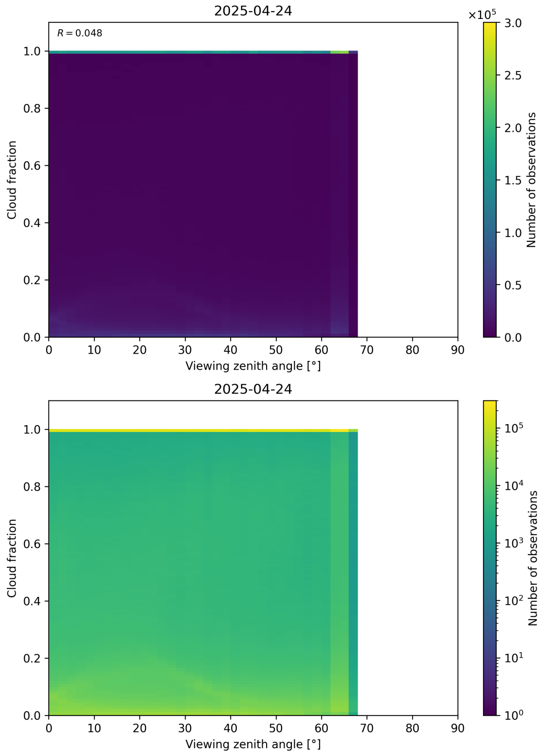
Figure 120: Scatter density plot of “Viewing zenith angle” against “Cloud fraction” for 2025-04-24 to 2025-04-25.
