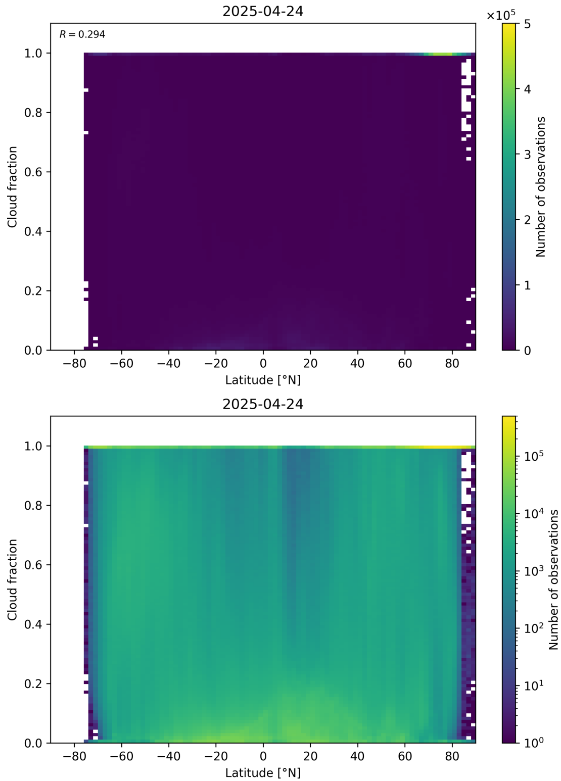
Figure 90: Scatter density plot of “Latitude” against “Cloud fraction” for 2025-04-24 to 2025-04-25.
