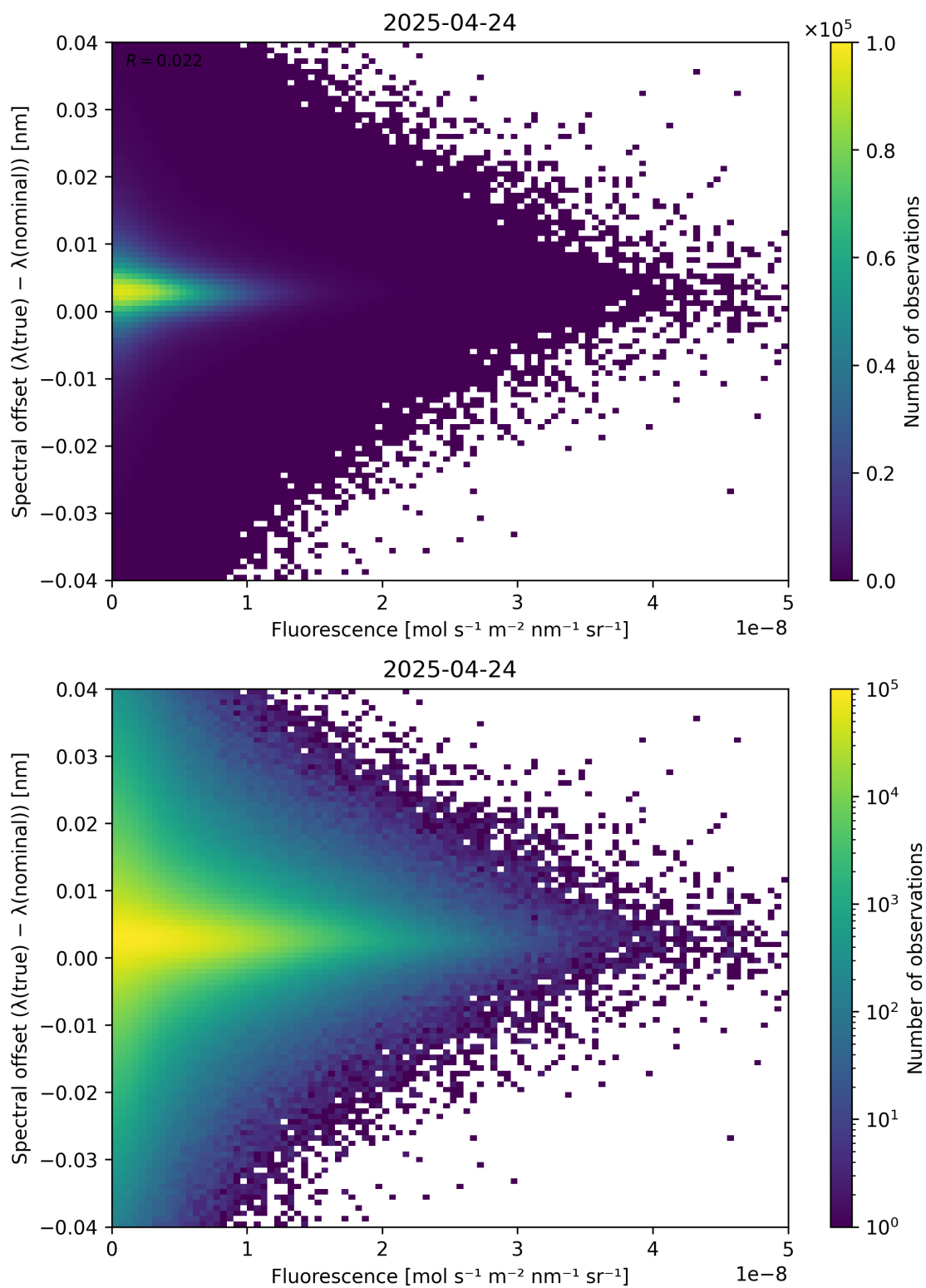
Figure 87: Scatter density plot of “Fluorescence” against “Spectral offset ( \lambda_{\text{true}} - \lambda_{\text{nominal}} )” for 2025-04-24 to 2025-04-25.
