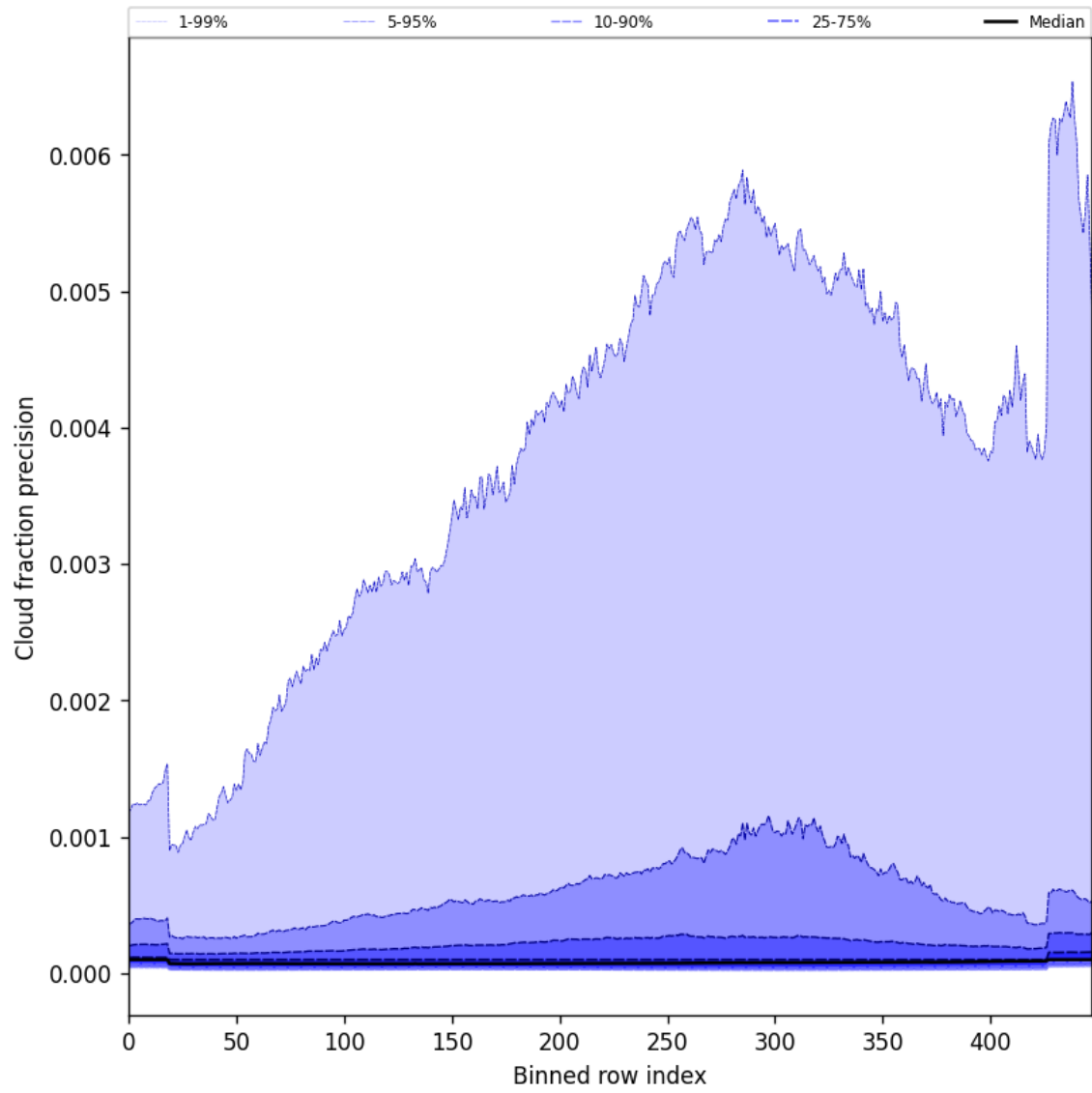
Figure 50: Along track statistics of “Cloud fraction precision” for 2025-04-24 to 2025-04-25
