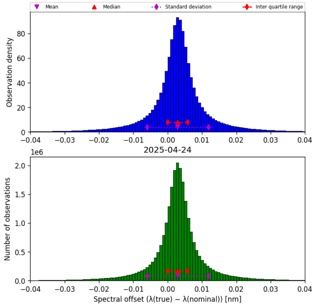
Figure 45: Histogram of “Spectral offset ( \lambda_{\text{true}} - \lambda_{\text{nominal}} )” for 2025-04-24 to 2025-04-25
