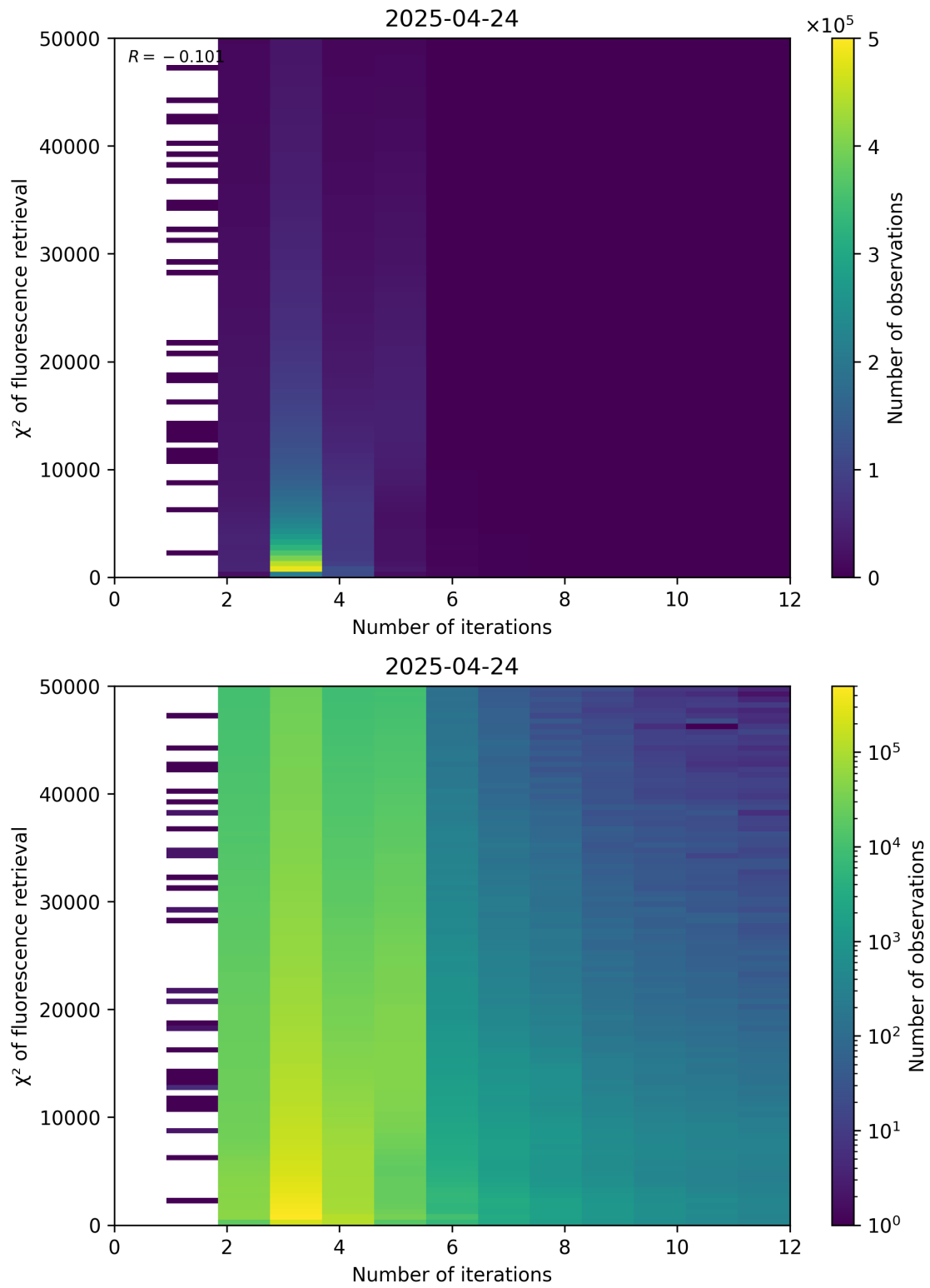
Figure 97: Scatter density plot of “Number of iterations” against “ \chi^2 of fluorescence retrieval” for 2025-04-24 to 2025-04-25.
