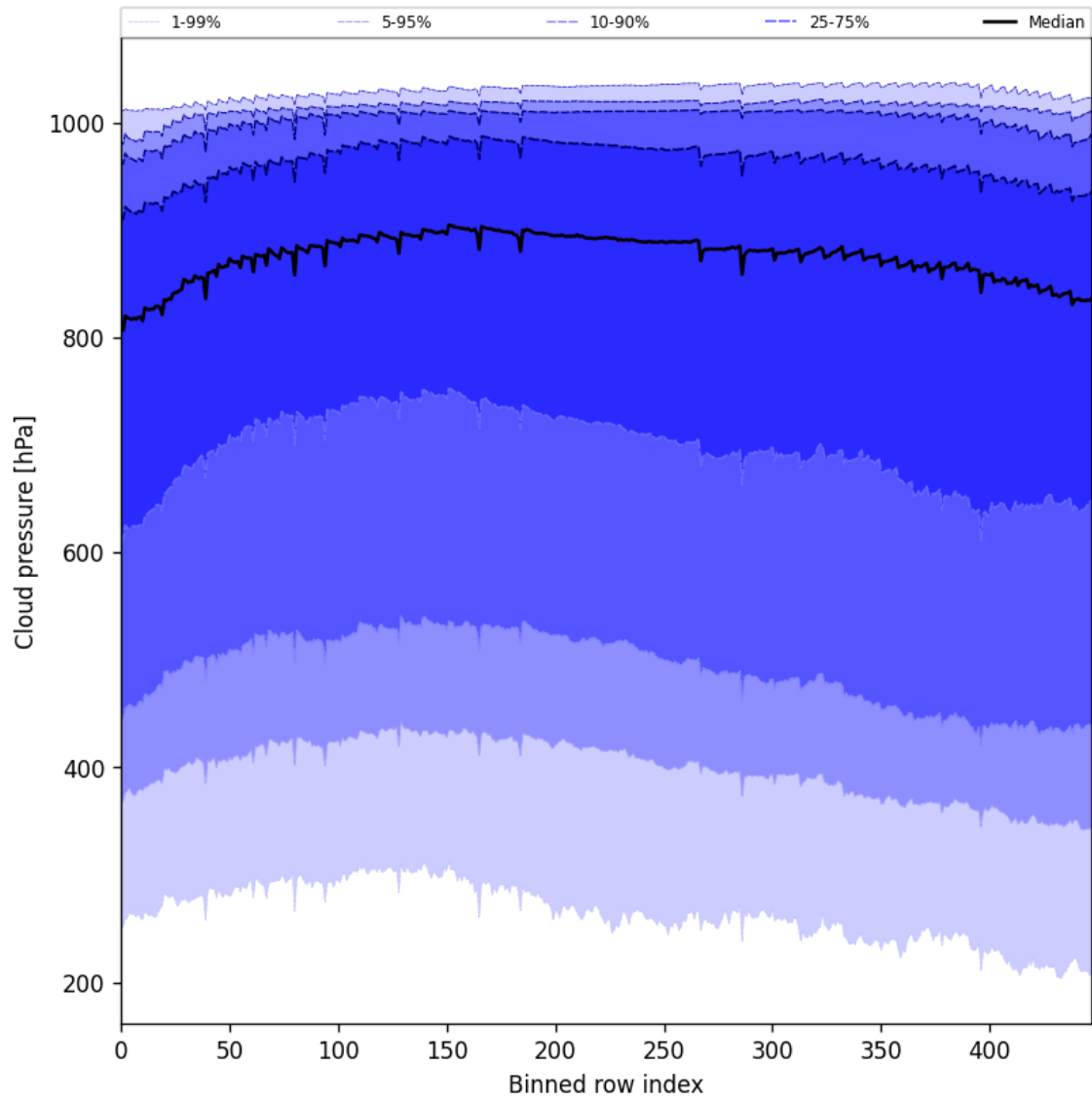
Figure 47: Along track statistics of “Cloud pressure” for 2025-04-24 to 2025-04-25
