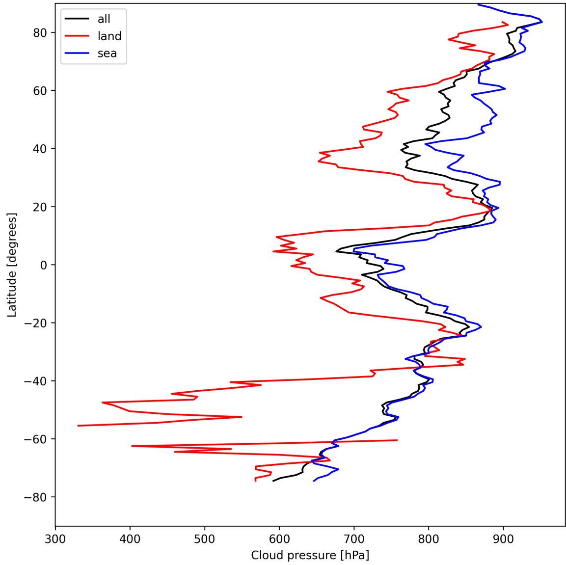
Figure 13: Zonal average of “Cloud pressure” for 2025-04-24 to 2025-04-25.
