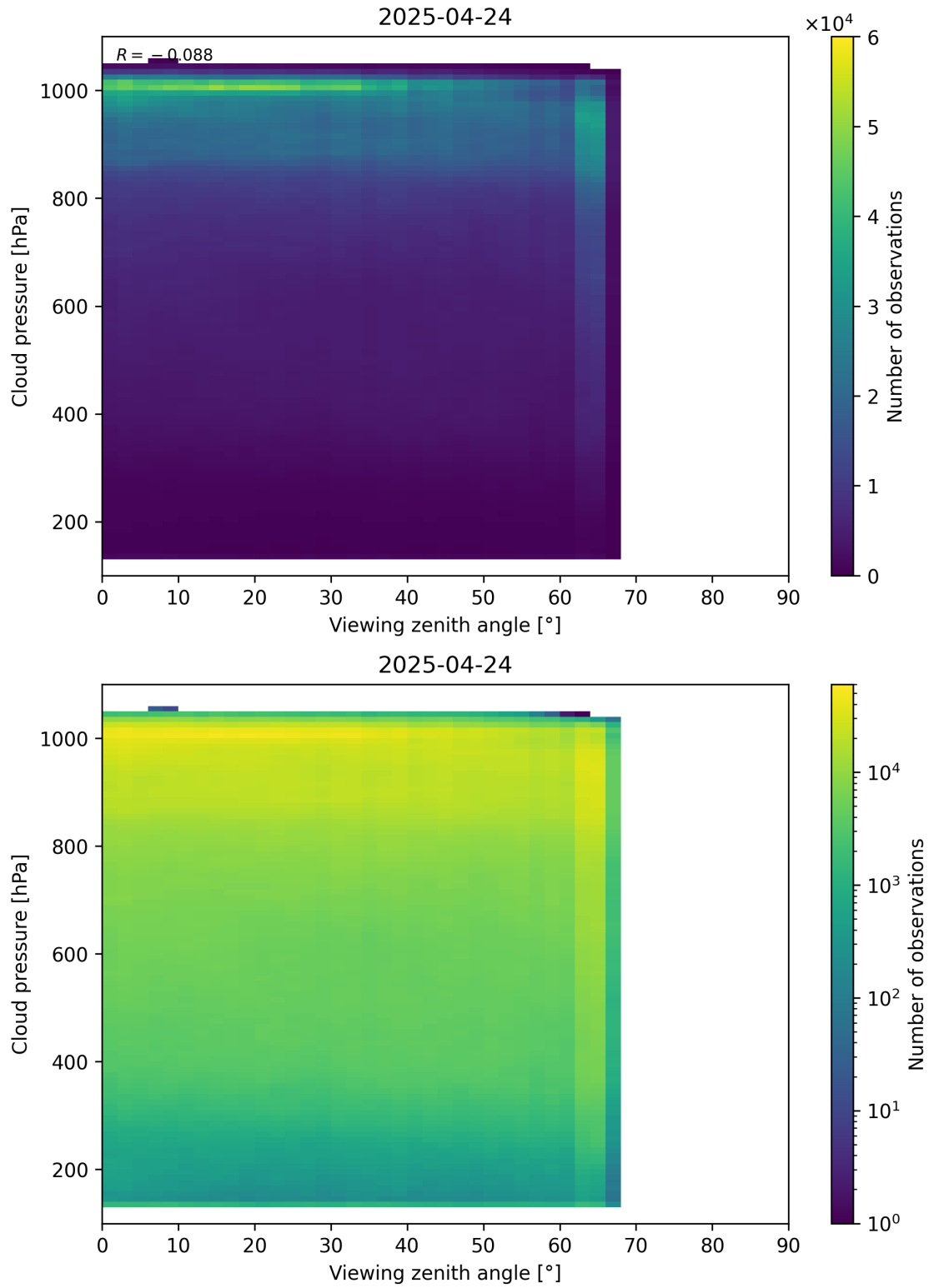
Figure 121: Scatter density plot of “Viewing zenith angle” against “Cloud pressure” for 2025-04-24 to 2025-04-25.
