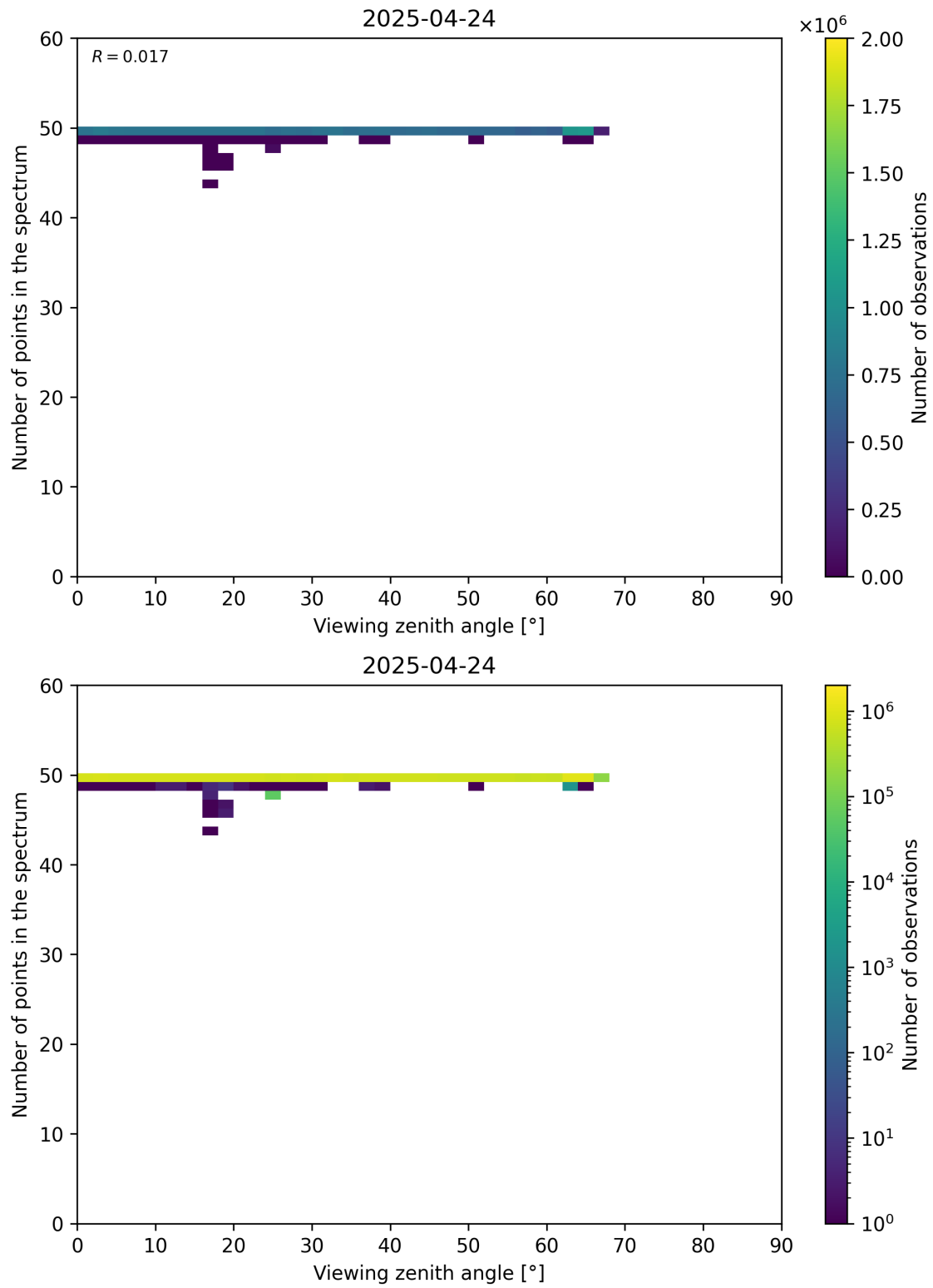
Figure 125: Scatter density plot of “Viewing zenith angle” against “Number of points in the spectrum” for 2025-04-24 to 2025-04-25.
