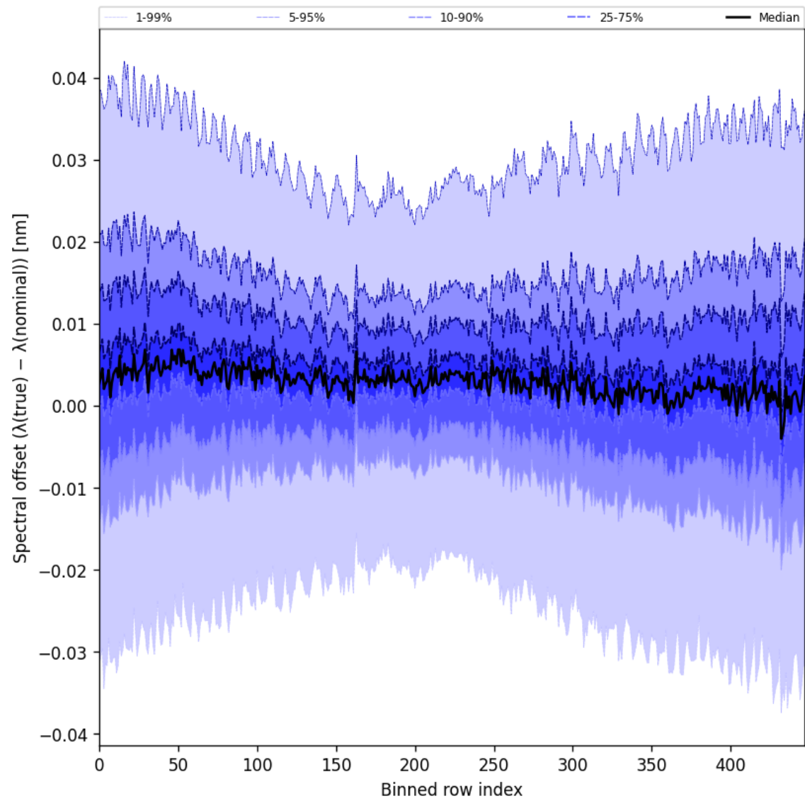
Figure 62: Along track statistics of “Spectral offset ( \lambda_{\text{true}} - \lambda_{\text{nominal}} )” for 2025-04-24 to 2025-04-25
