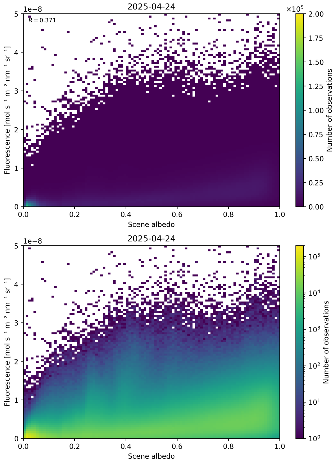
Figure 104: Scatter density plot of “Scene albedo” against “Fluorescence” for 2025-04-24 to 2025-04-25.
