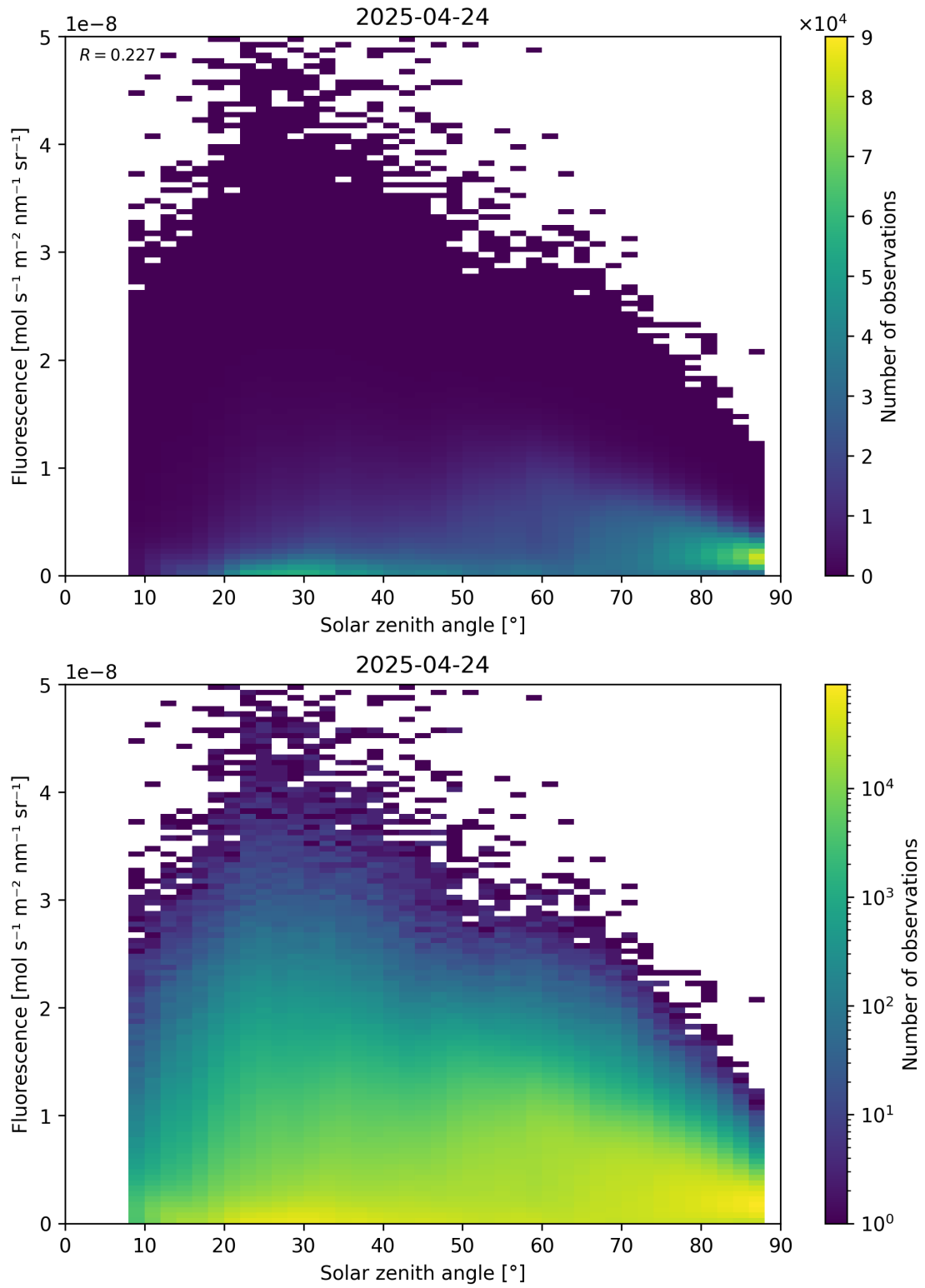
Figure 112: Scatter density plot of “Solar zenith angle” against “Fluorescence” for 2025-04-24 to 2025-04-25.
