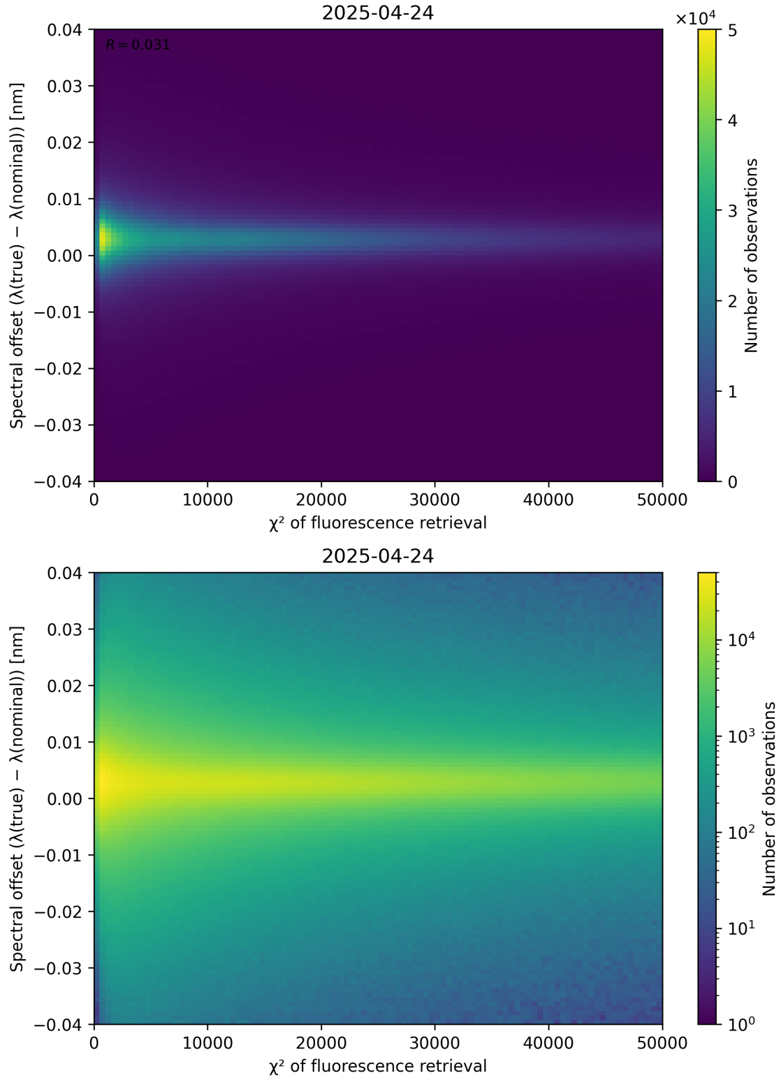
Figure 69: Scatter density plot of “ \chi^2 of fluorescence retrieval” against “Spectral offset ( \lambda_{\text{true}} - \lambda_{\text{nominal}} )” for 2025-04-24 to 2025-04-25.
