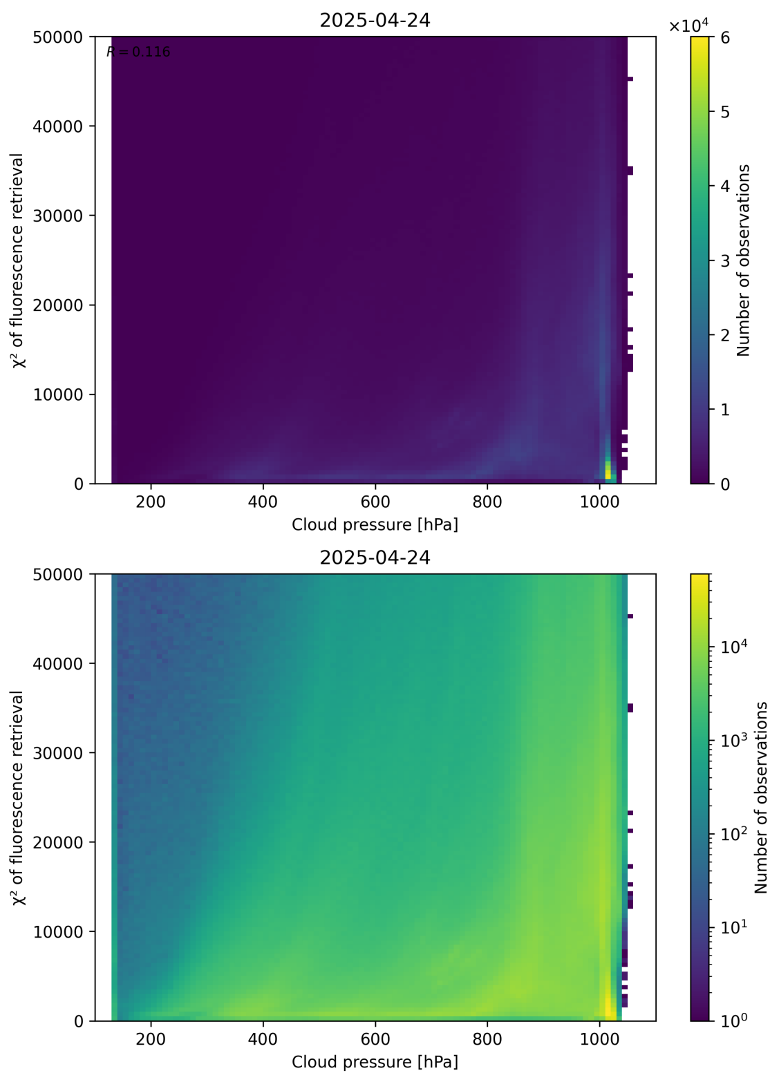
Figure 78: Scatter density plot of “Cloud pressure” against “ \chi^2 of fluorescence retrieval” for 2025-04-24 to 2025-04-25.
