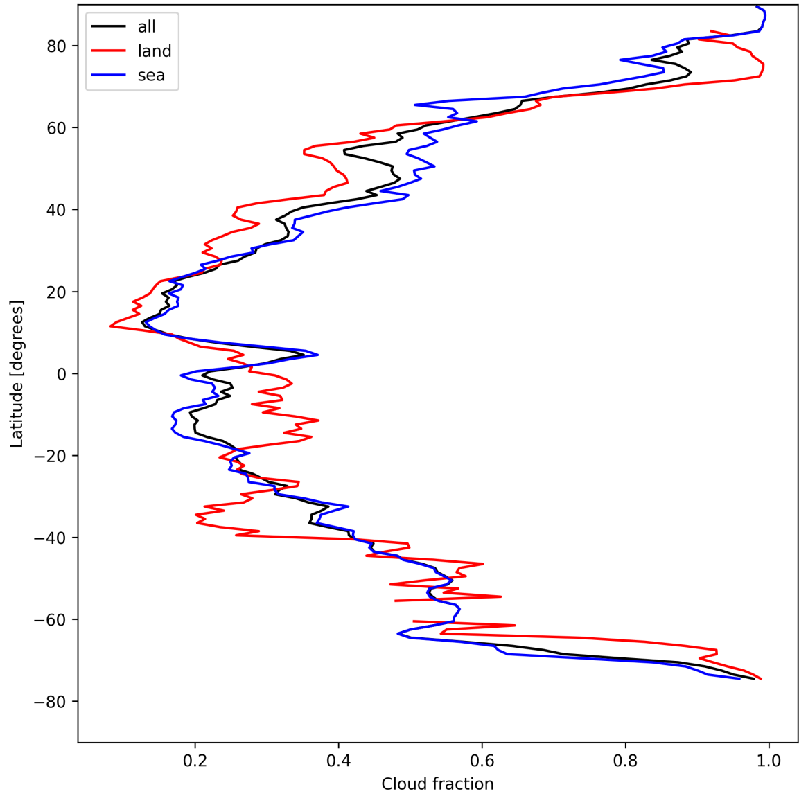
Figure 15: Zonal average of “Cloud fraction” for 2025-04-24 to 2025-04-25.
