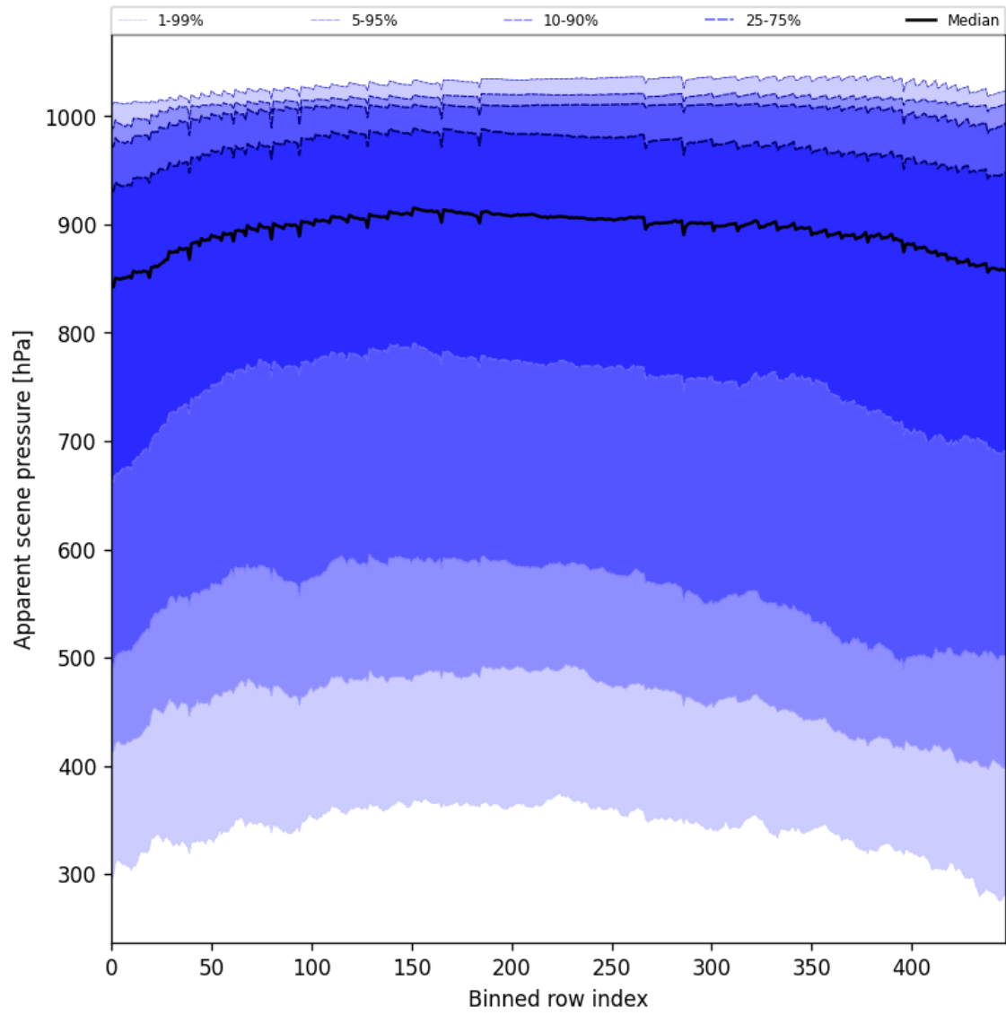
Figure 53: Along track statistics of “Apparent scene pressure” for 2025-04-24 to 2025-04-25
