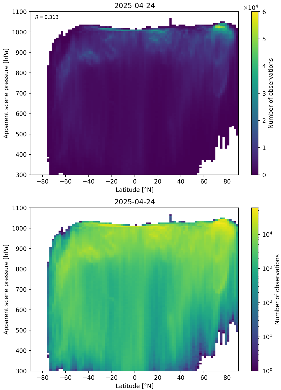
Figure 88: Scatter density plot of “Latitude” against “Apparent scene pressure” for 2025-04-24 to 2025-04-25.
