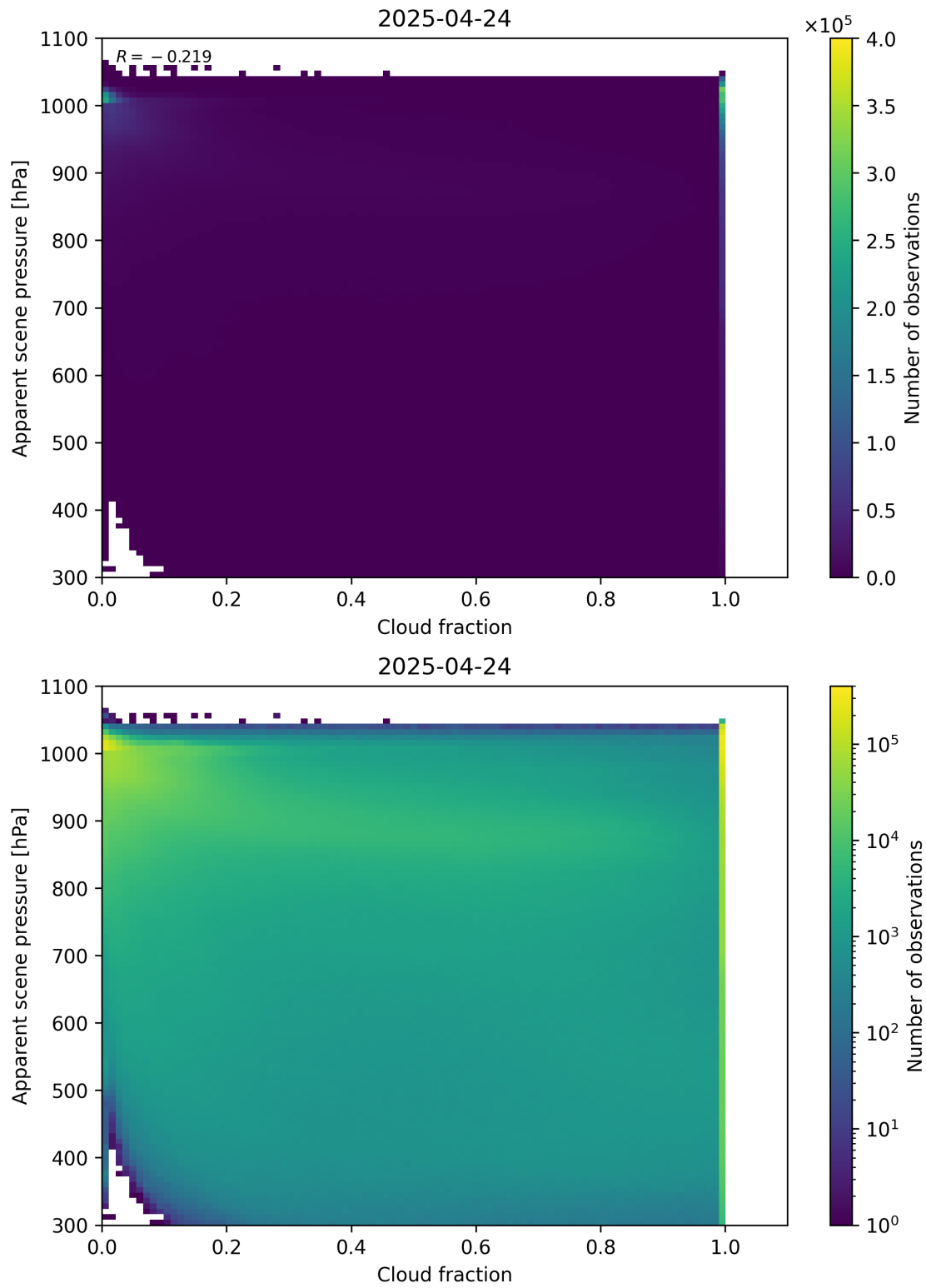
Figure 70: Scatter density plot of “Cloud fraction” against “Apparent scene pressure” for 2025-04-24 to 2025-04-25.
