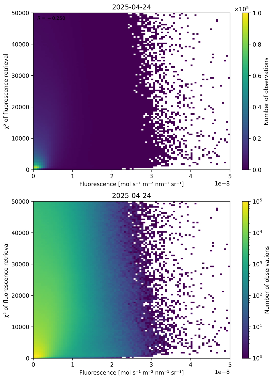
Figure 85: Scatter density plot of “Fluorescence” against “ \chi^2 of fluorescence retrieval” for 2025-04-24 to 2025-04-25.
