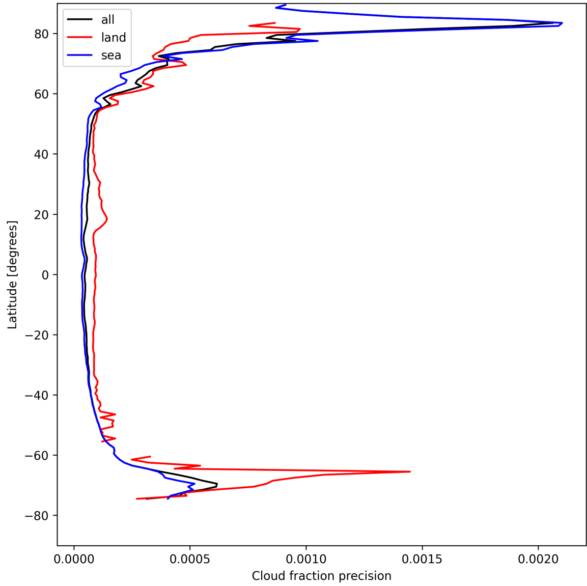
Figure 16: Zonal average of “Cloud fraction precision” for 2025-04-24 to 2025-04-25.
