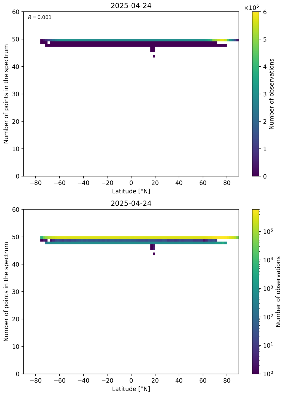
Figure 94: Scatter density plot of “Latitude” against “Number of points in the spectrum” for 2025-04-24 to 2025-04-25.
