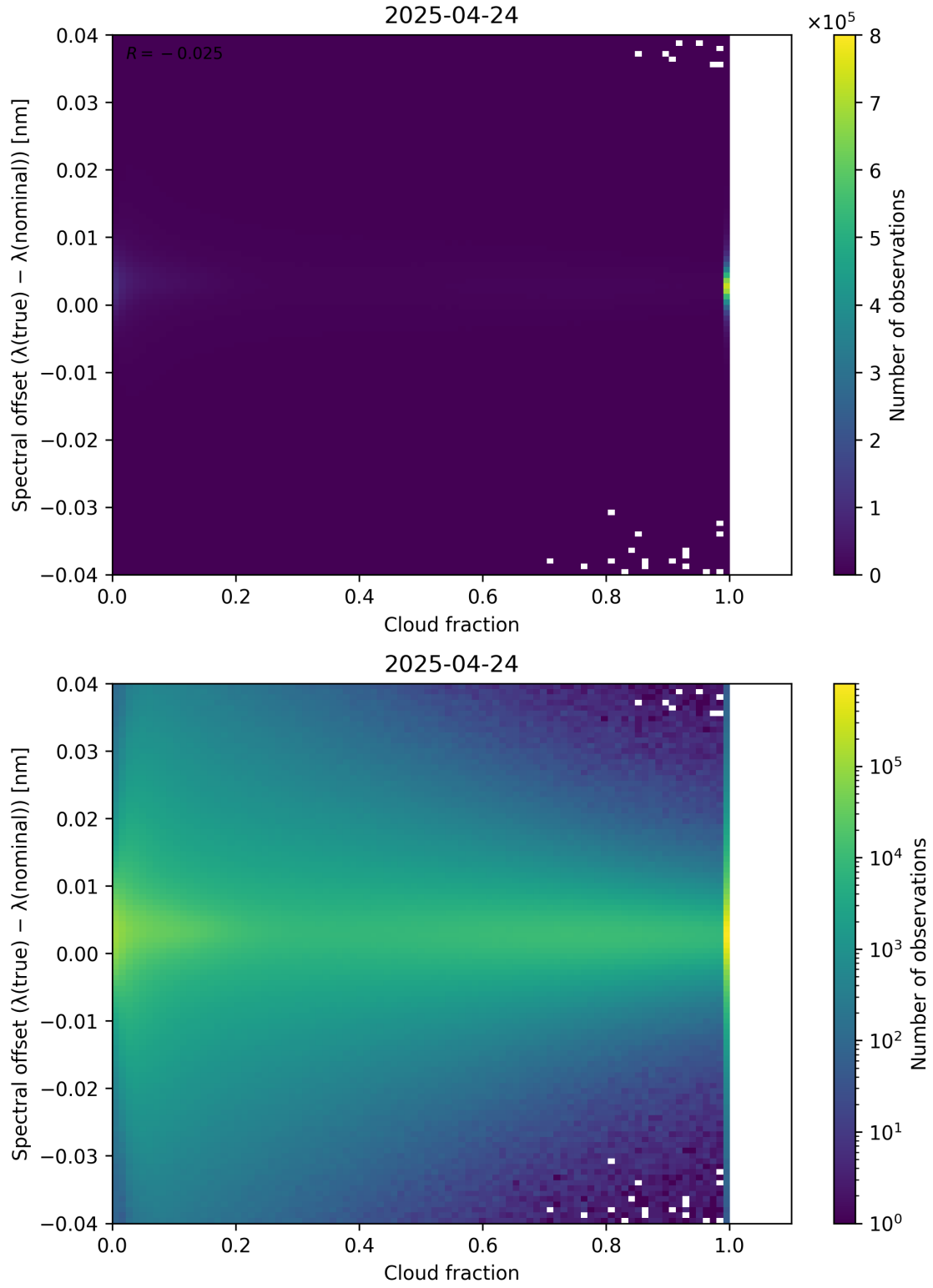
Figure 76: Scatter density plot of “Cloud fraction” against “Spectral offset ( \lambda_{\text{true}} - \lambda_{\text{nominal}} )” for 2025-04-24 to 2025-04-25.
