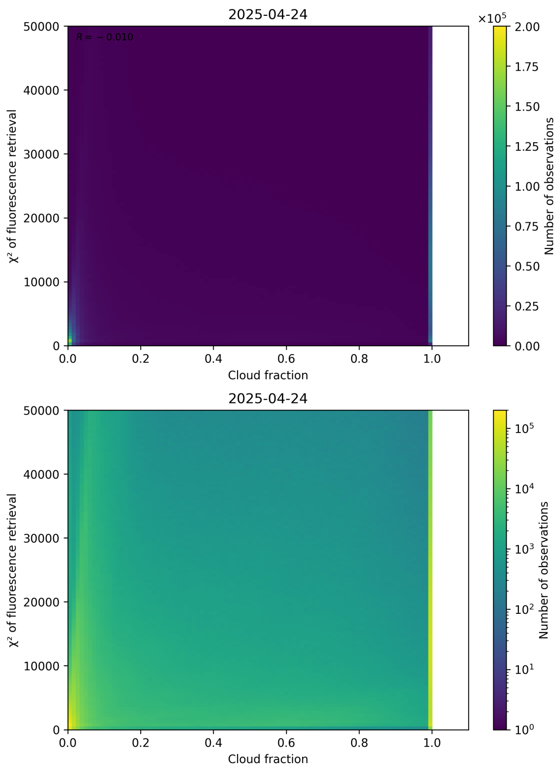
Figure 71: Scatter density plot of “Cloud fraction” against “ \chi^2 of fluorescence retrieval” for 2025-04-24 to 2025-04-25.
