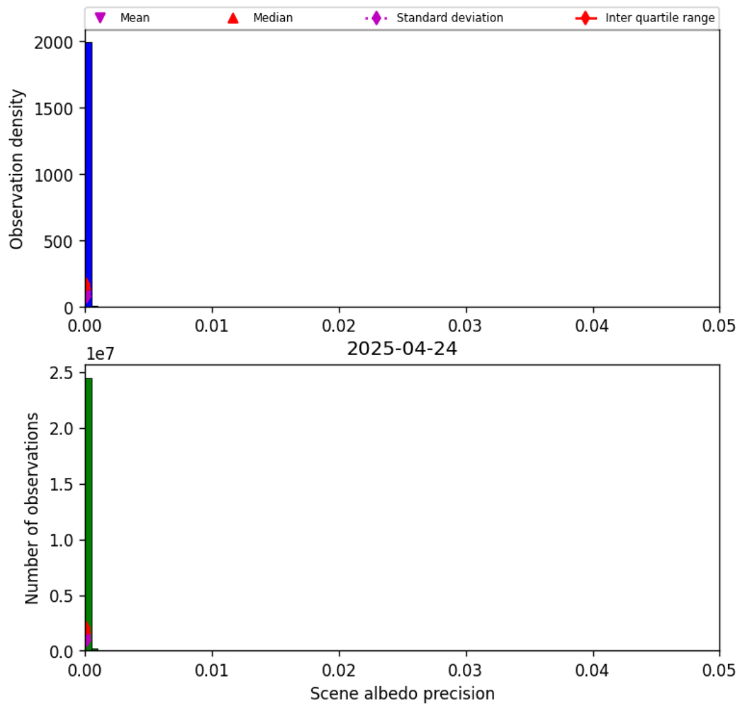
Figure 35: Histogram of “Scene albedo precision” for 2025-04-24 to 2025-04-25
