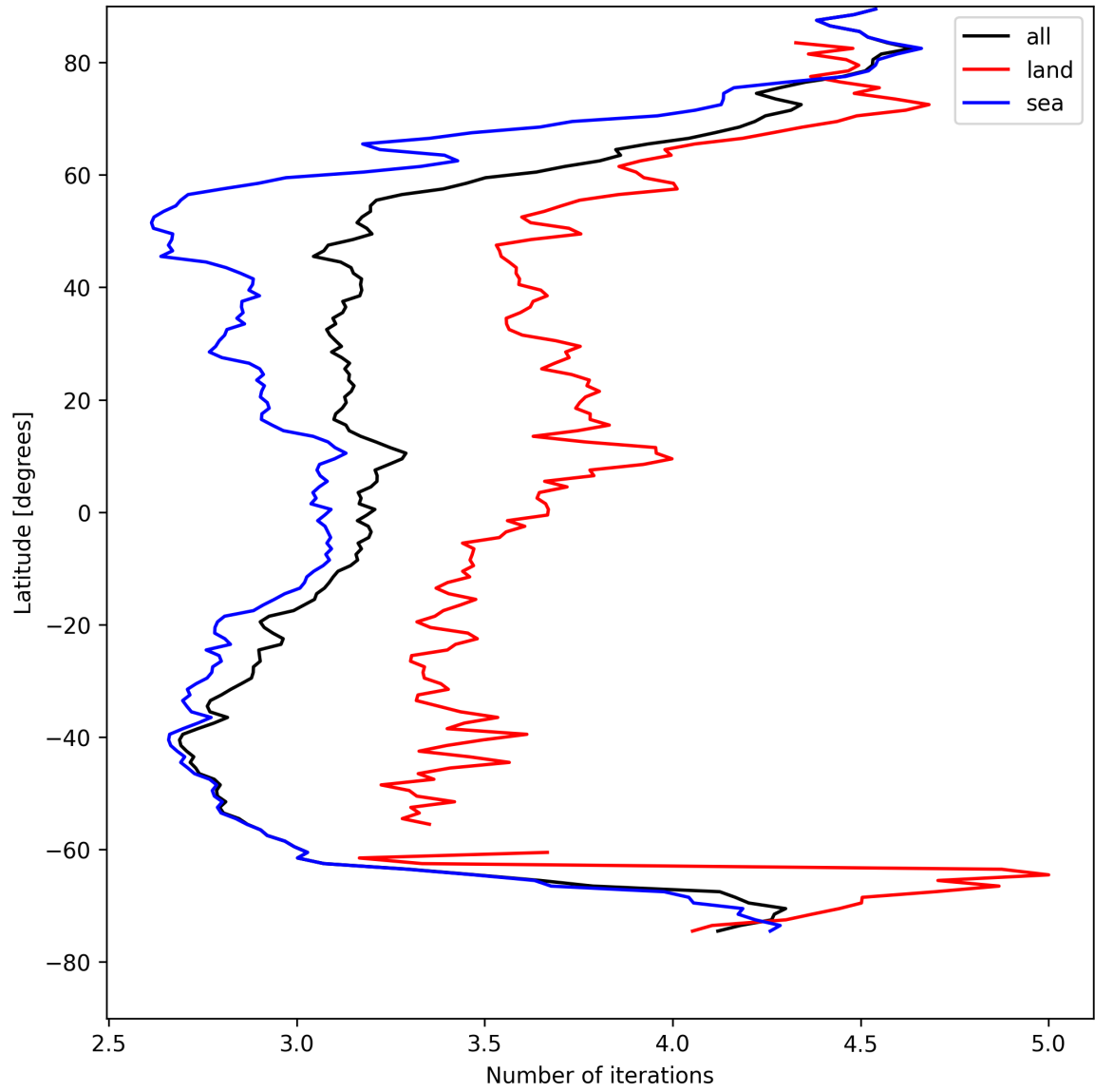
Figure 22: Zonal average of “Number of iterations” for 2025-04-24 to 2025-04-25.
