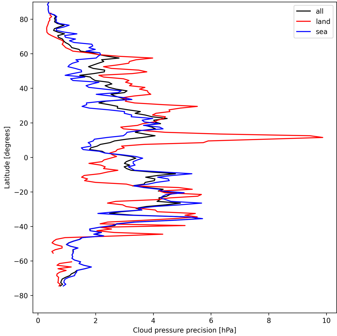
Figure 14: Zonal average of “Cloud pressure precision” for 2025-04-24 to 2025-04-25.
