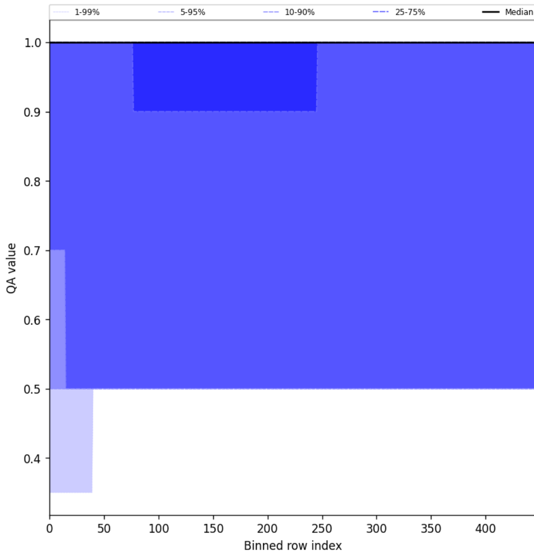
Figure 46: Along track statistics of “QA value” for 2025-04-24 to 2025-04-25
