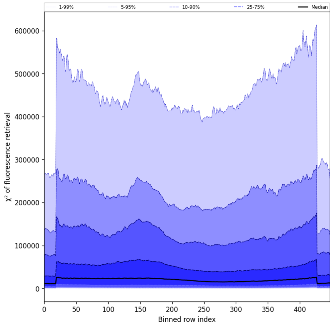
Figure 59: Along track statistics of “ \chi^2 of fluorescence retrieval” for 2025-04-24 to 2025-04-25
