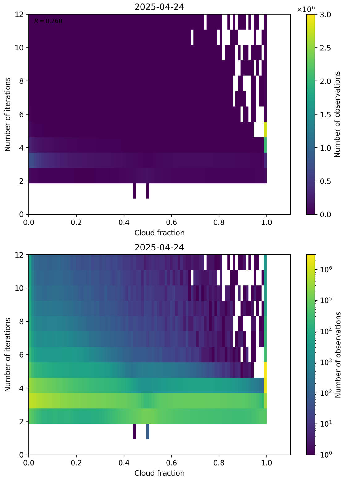
Figure 73: Scatter density plot of “Cloud fraction” against “Number of iterations” for 2025-04-24 to 2025-04-25.
