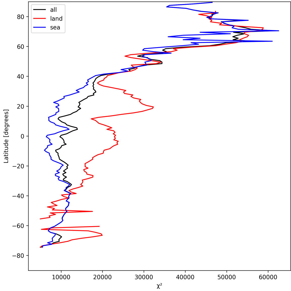
Figure 21: Zonal average of “ \chi^2 ” for 2025-04-24 to 2025-04-25.
