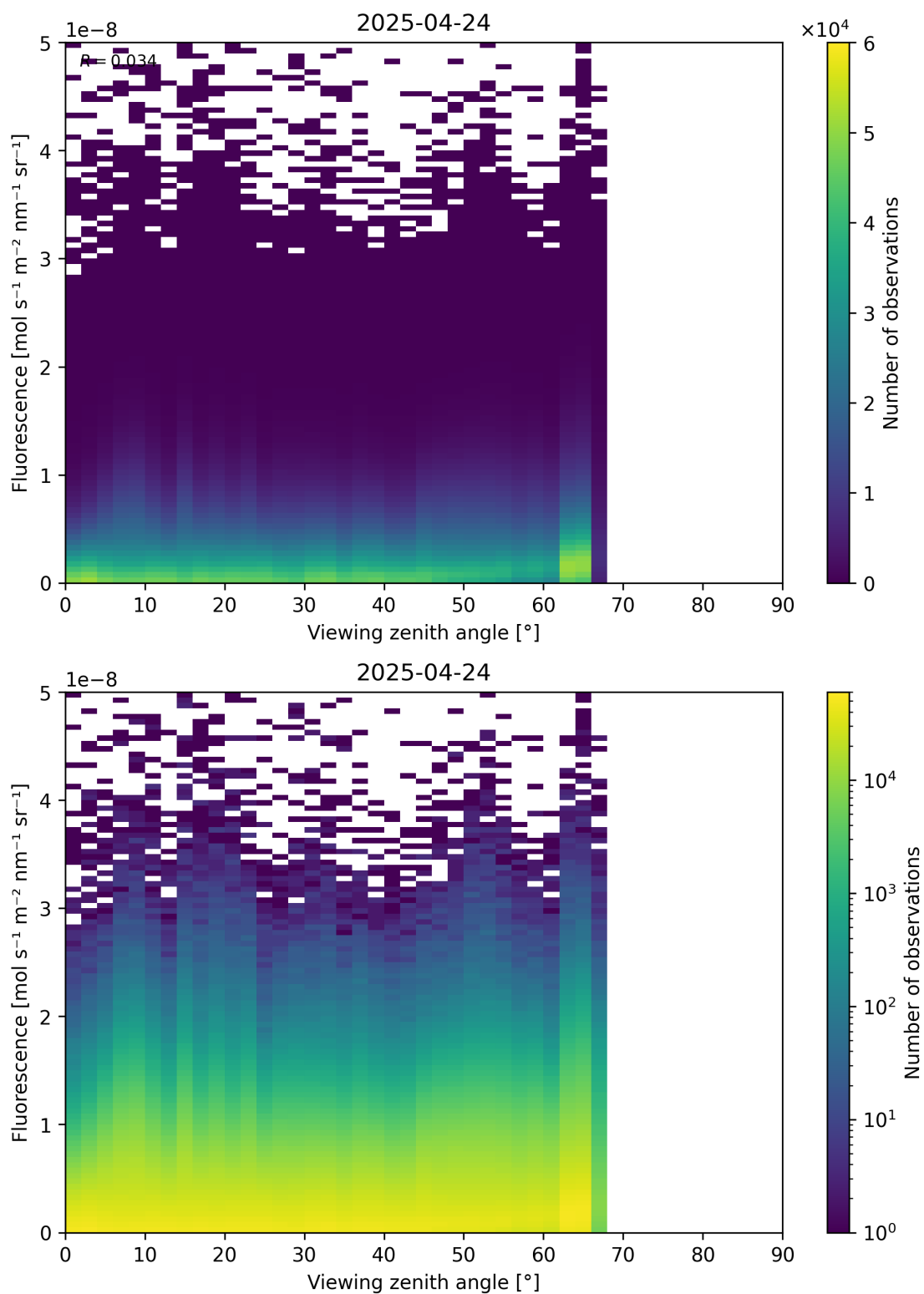
Figure 122: Scatter density plot of “Viewing zenith angle” against “Fluorescence” for 2025-04-24 to 2025-04-25.
