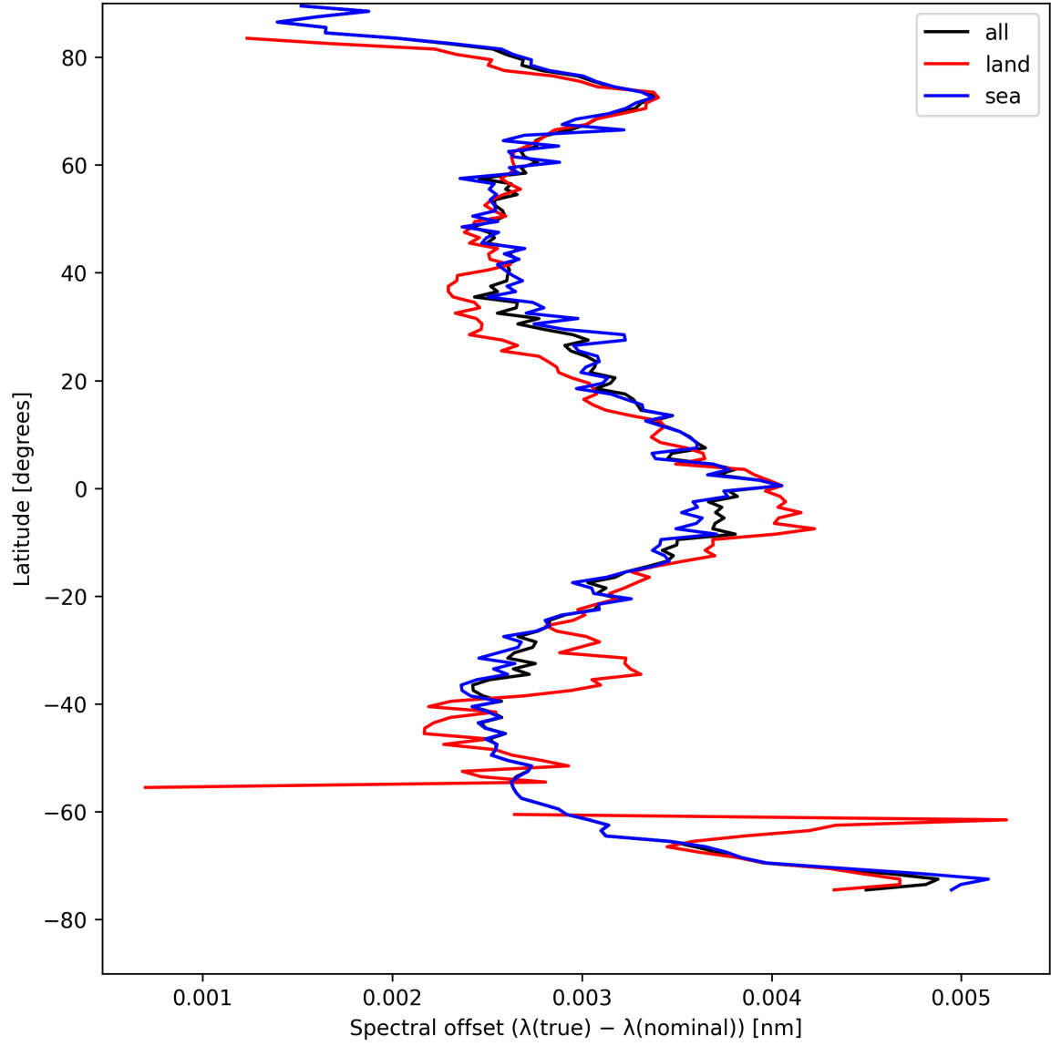
Figure 28: Zonal average of “Spectral offset ( \lambda_{\text{true}} - \lambda_{\text{nominal}} )” for 2025-04-24 to 2025-04-25.
