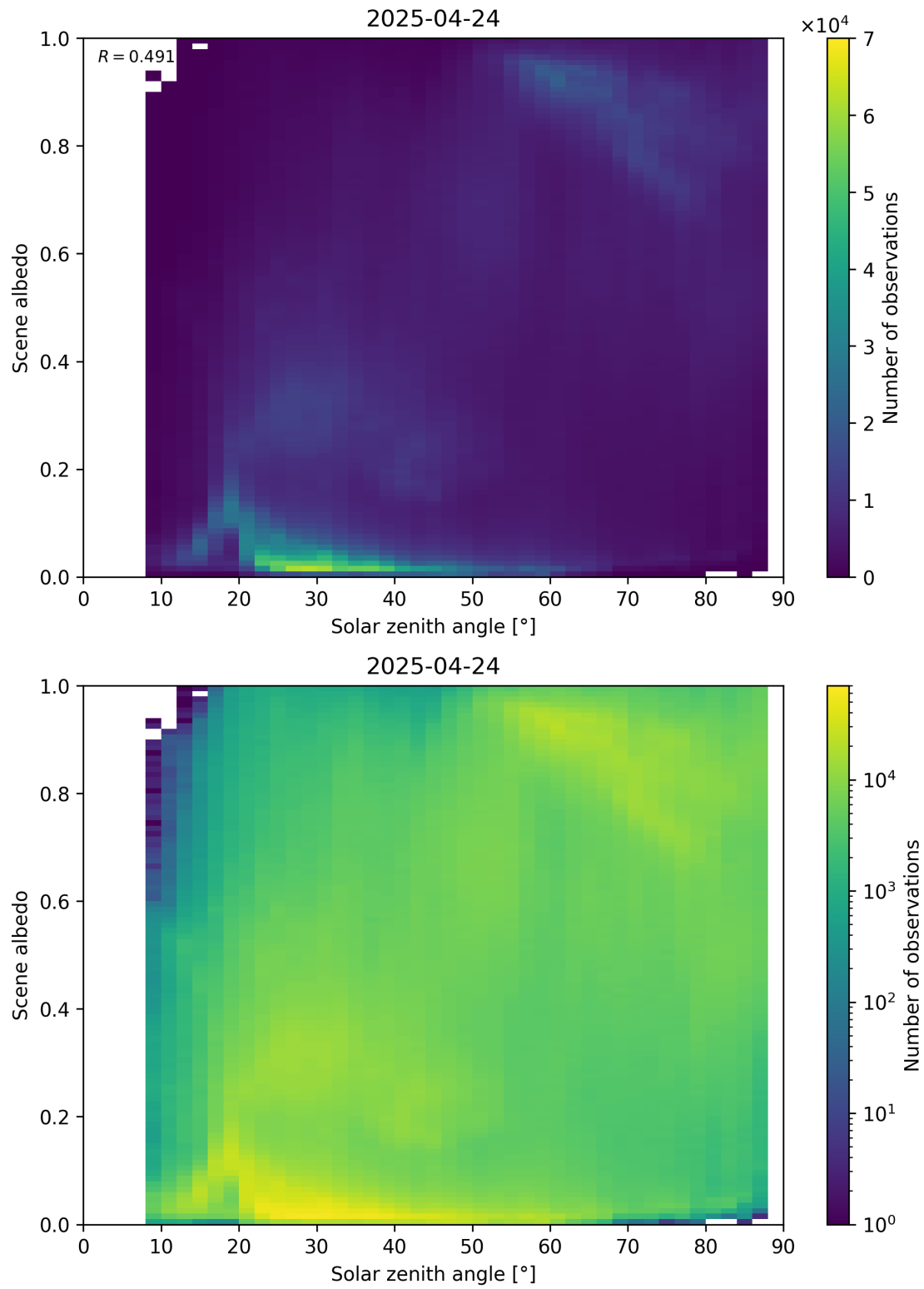
Figure 116: Scatter density plot of “Solar zenith angle” against “Scene albedo” for 2025-04-24 to 2025-04-25.
