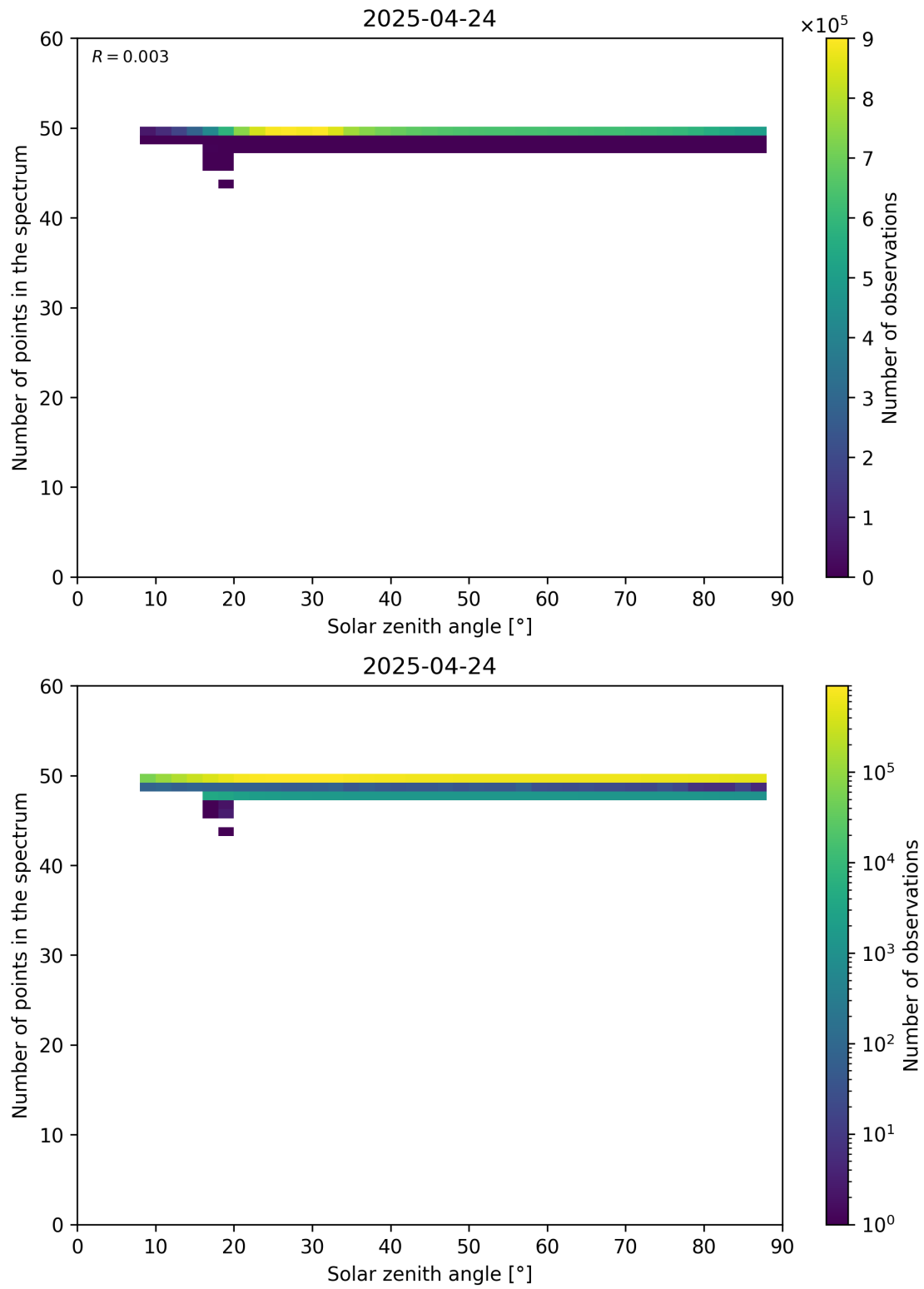
Figure 115: Scatter density plot of “Solar zenith angle” against “Number of points in the spectrum” for 2025-04-24 to 2025-04-25.
