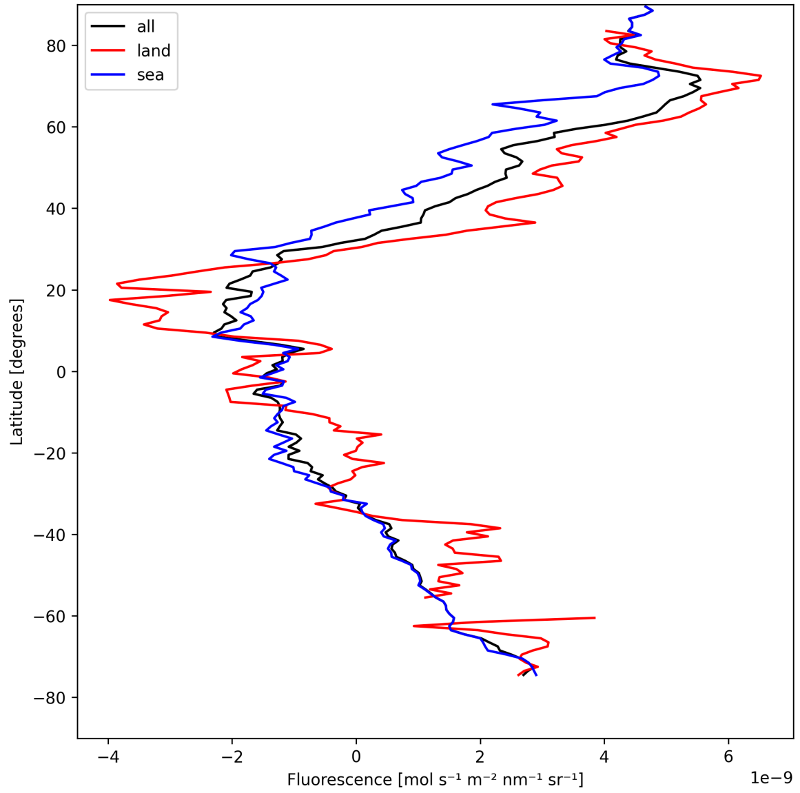
Figure 23: Zonal average of “Fluorescence” for 2025-04-24 to 2025-04-25.
