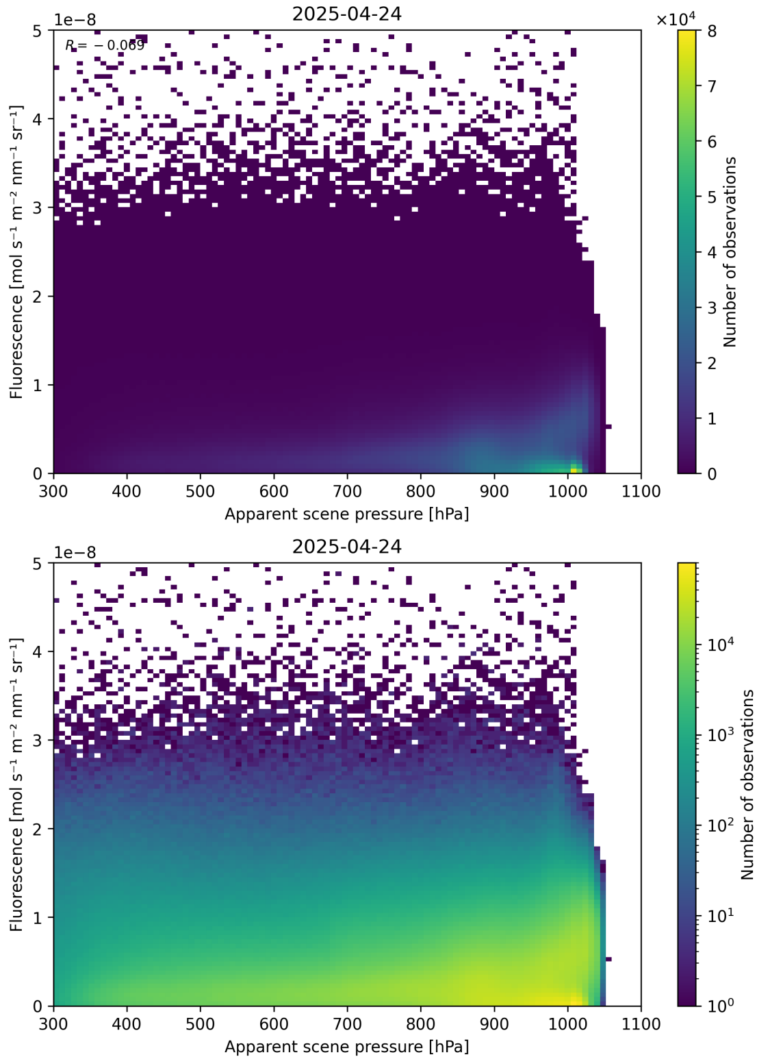
Figure 64: Scatter density plot of “Apparent scene pressure” against “Fluorescence” for 2025-04-24 to 2025-04-25.
