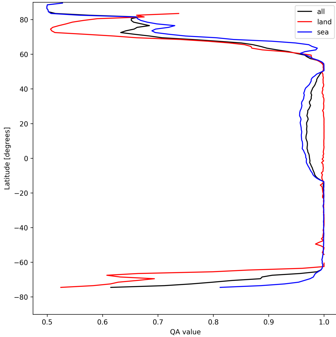
Figure 12: Zonal average of “QA value” for 2025-04-24 to 2025-04-25.
