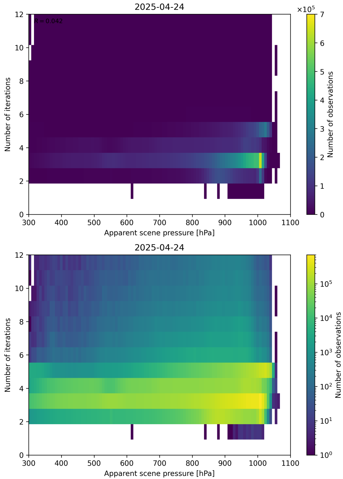
Figure 65: Scatter density plot of “Apparent scene pressure” against “Number of iterations” for 2025-04-24 to 2025-04-25.
