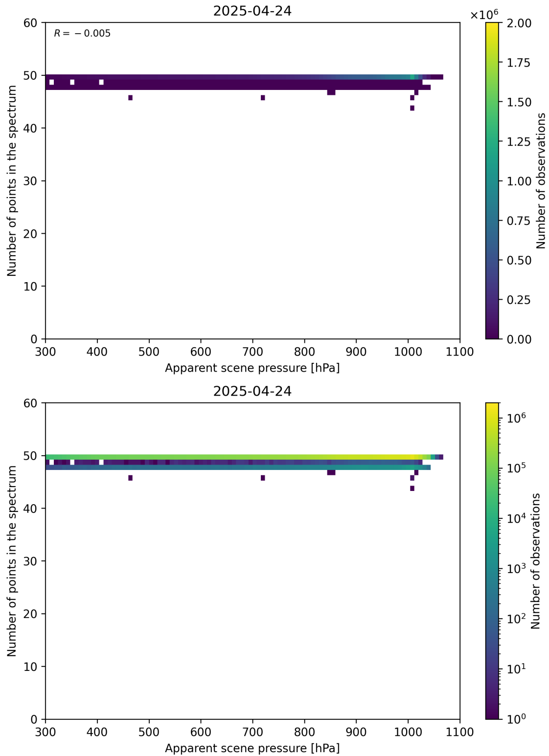
Figure 66: Scatter density plot of “Apparent scene pressure” against “Number of points in the spectrum” for 2025-04-24 to 2025-04-25.
