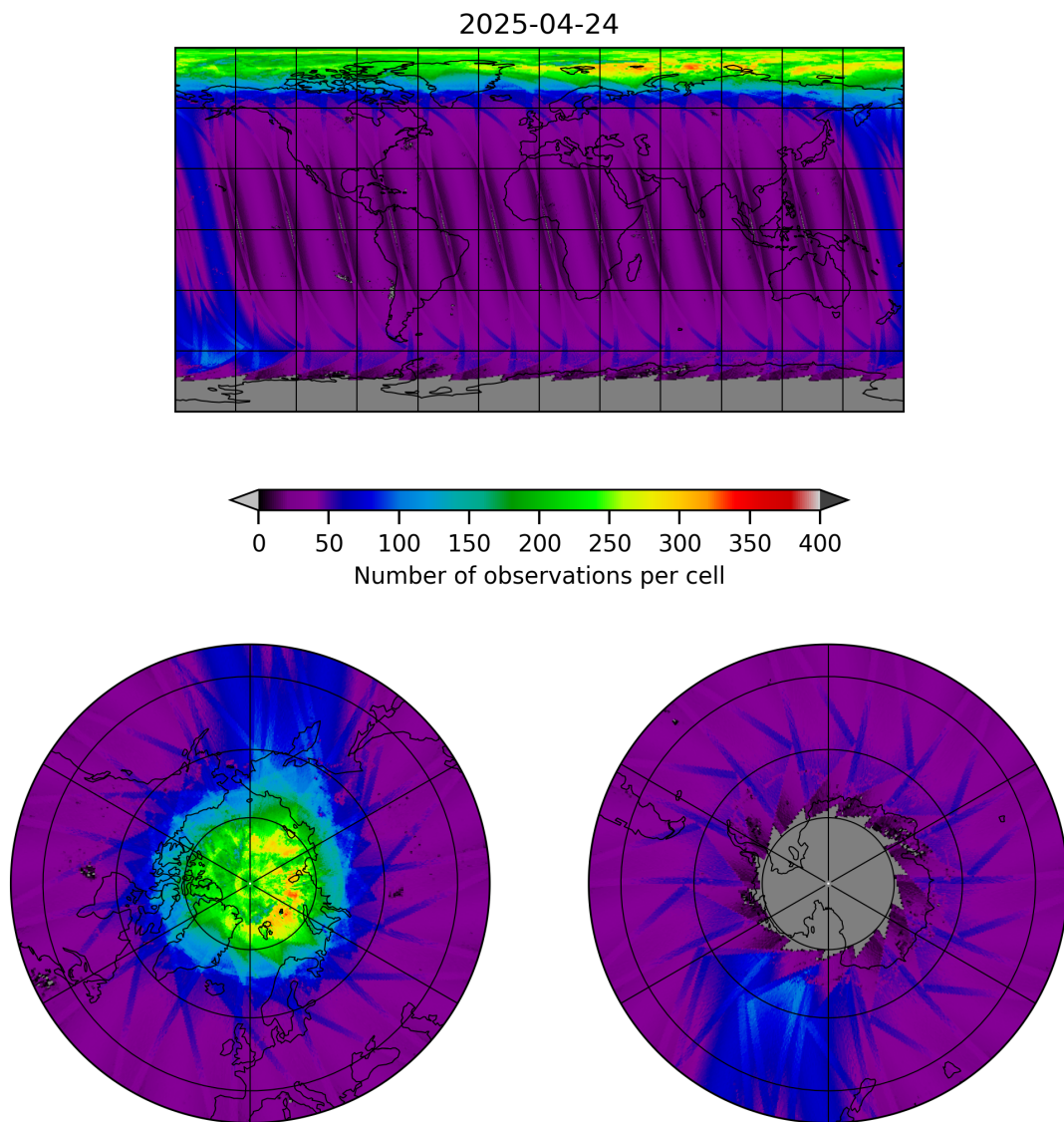
Figure 11: Map of the number of observations for 2025-04-24 to 2025-04-25
