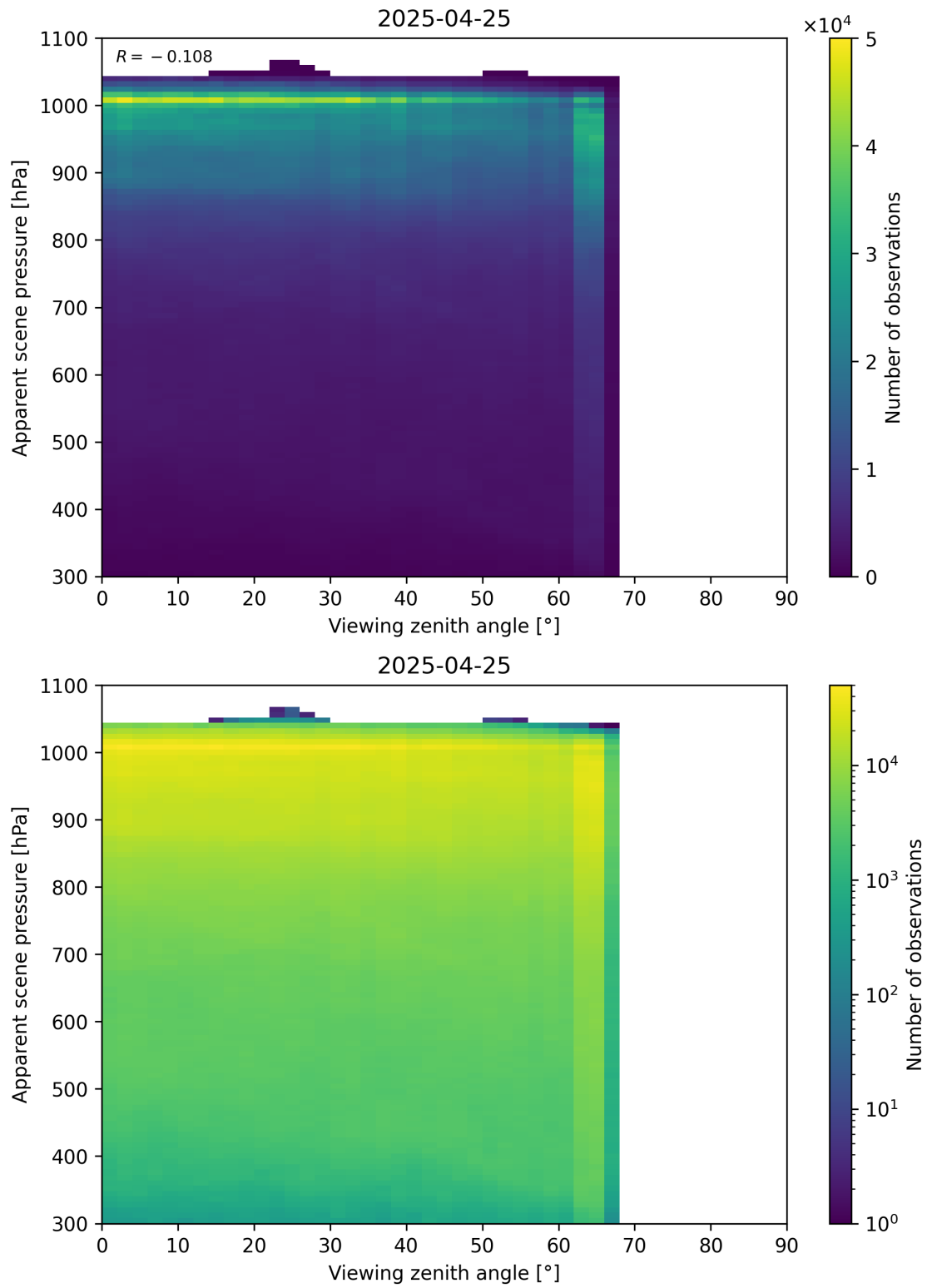
Figure 118: Scatter density plot of “Viewing zenith angle” against “Apparent scene pressure” for 2025-04-24 to 2025-04-26.
