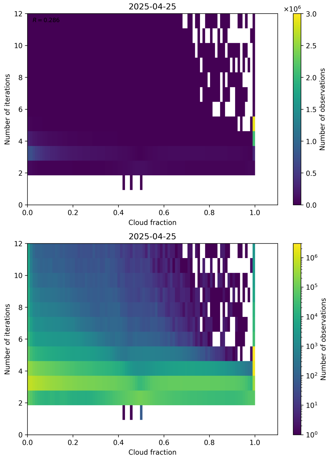
Figure 73: Scatter density plot of “Cloud fraction” against “Number of iterations” for 2025-04-24 to 2025-04-26.
