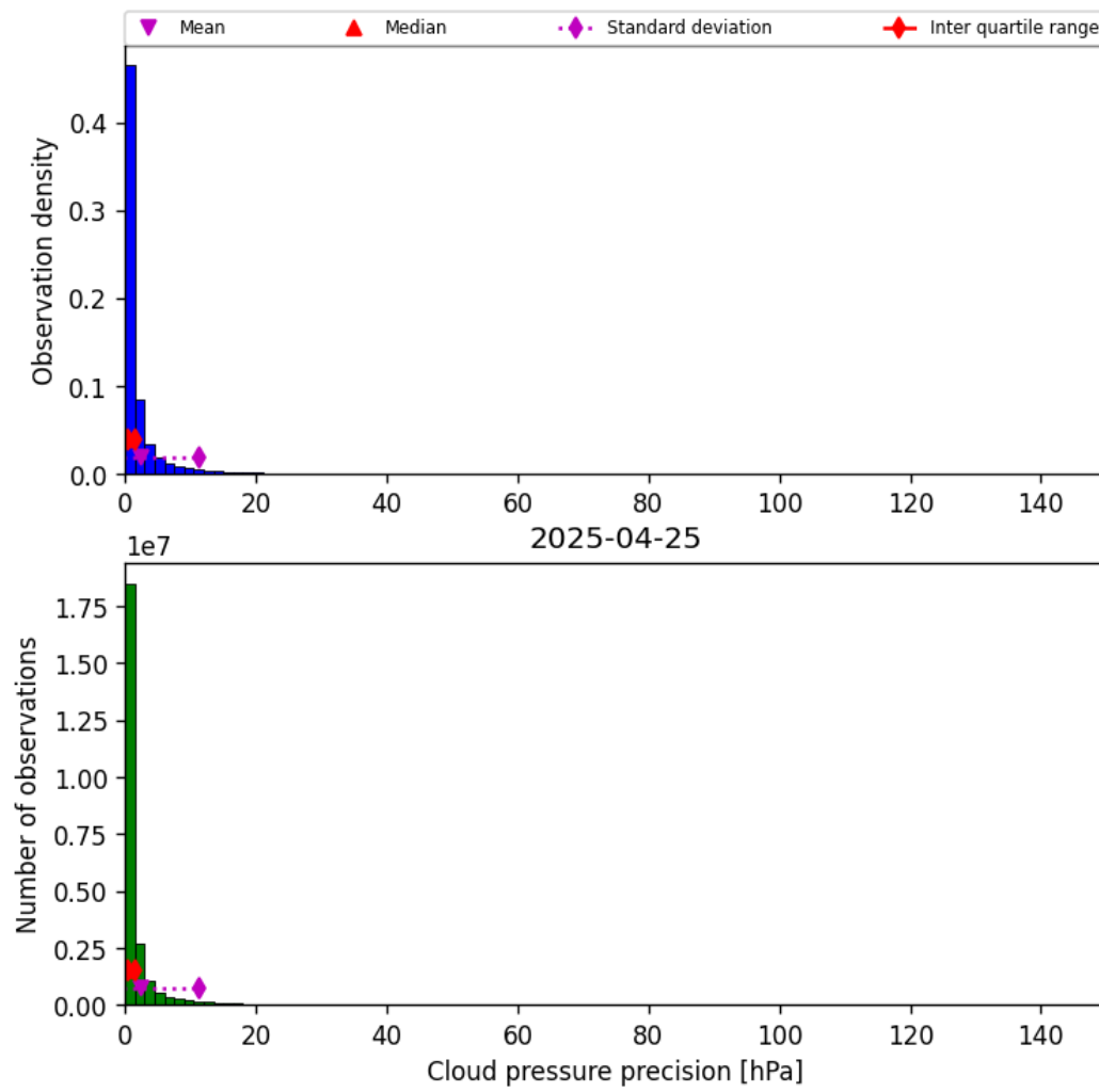
Figure 31: Histogram of “Cloud pressure precision” for 2025-04-24 to 2025-04-26
