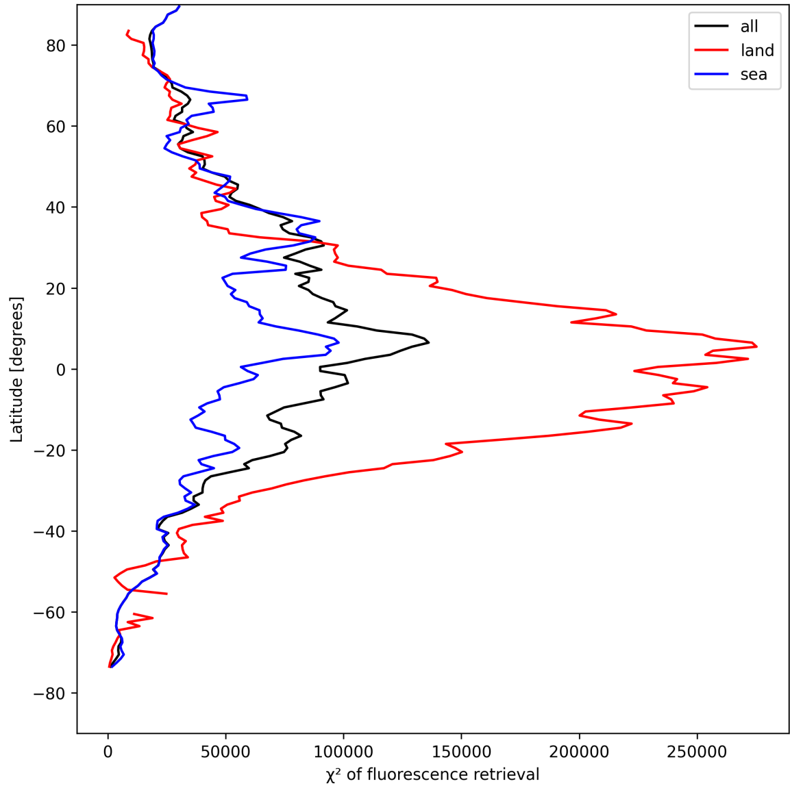
Figure 25: Zonal average of “ \chi^2 of fluorescence retrieval” for 2025-04-26 to 2025-04-28.
