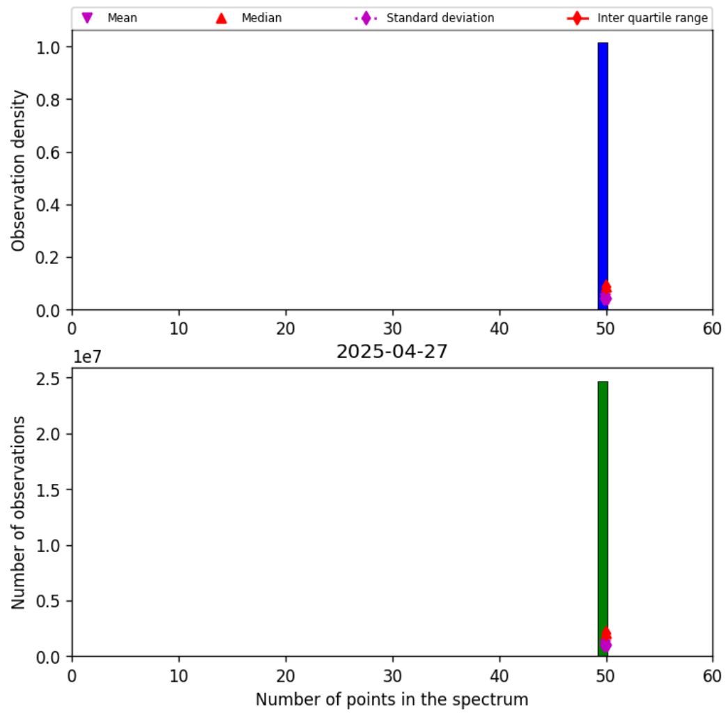
Figure 44: Histogram of “Number of points in the spectrum” for 2025-04-26 to 2025-04-28
