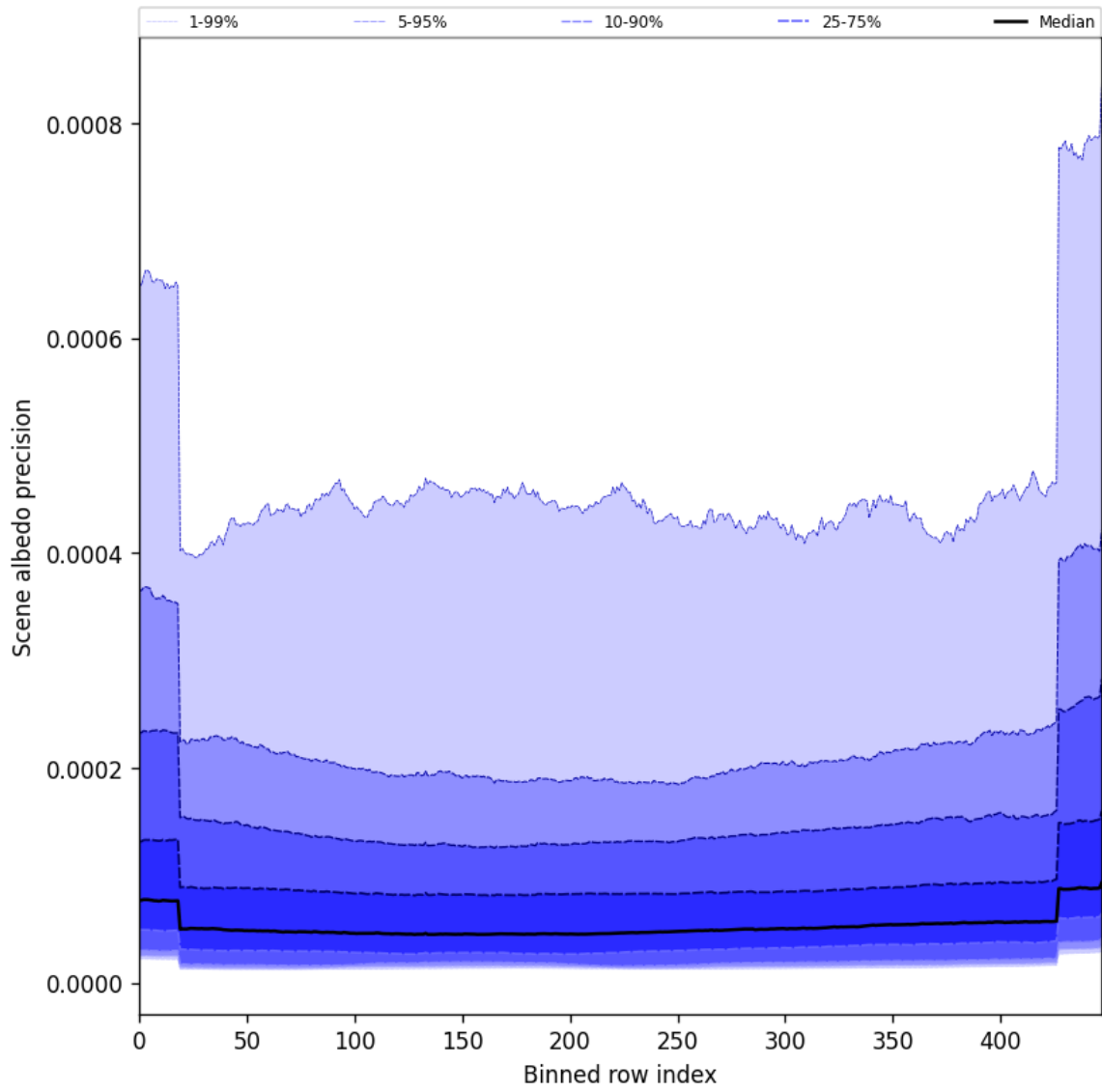
Figure 52: Along track statistics of “Scene albedo precision” for 2025-04-26 to 2025-04-28
