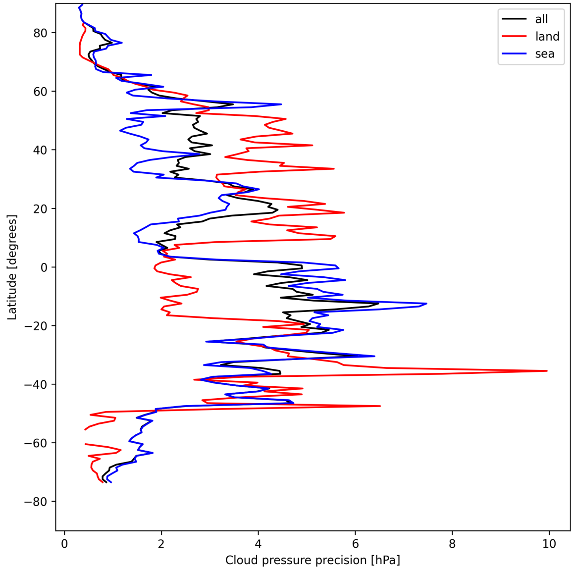
Figure 14: Zonal average of “Cloud pressure precision” for 2025-04-26 to 2025-04-28.
