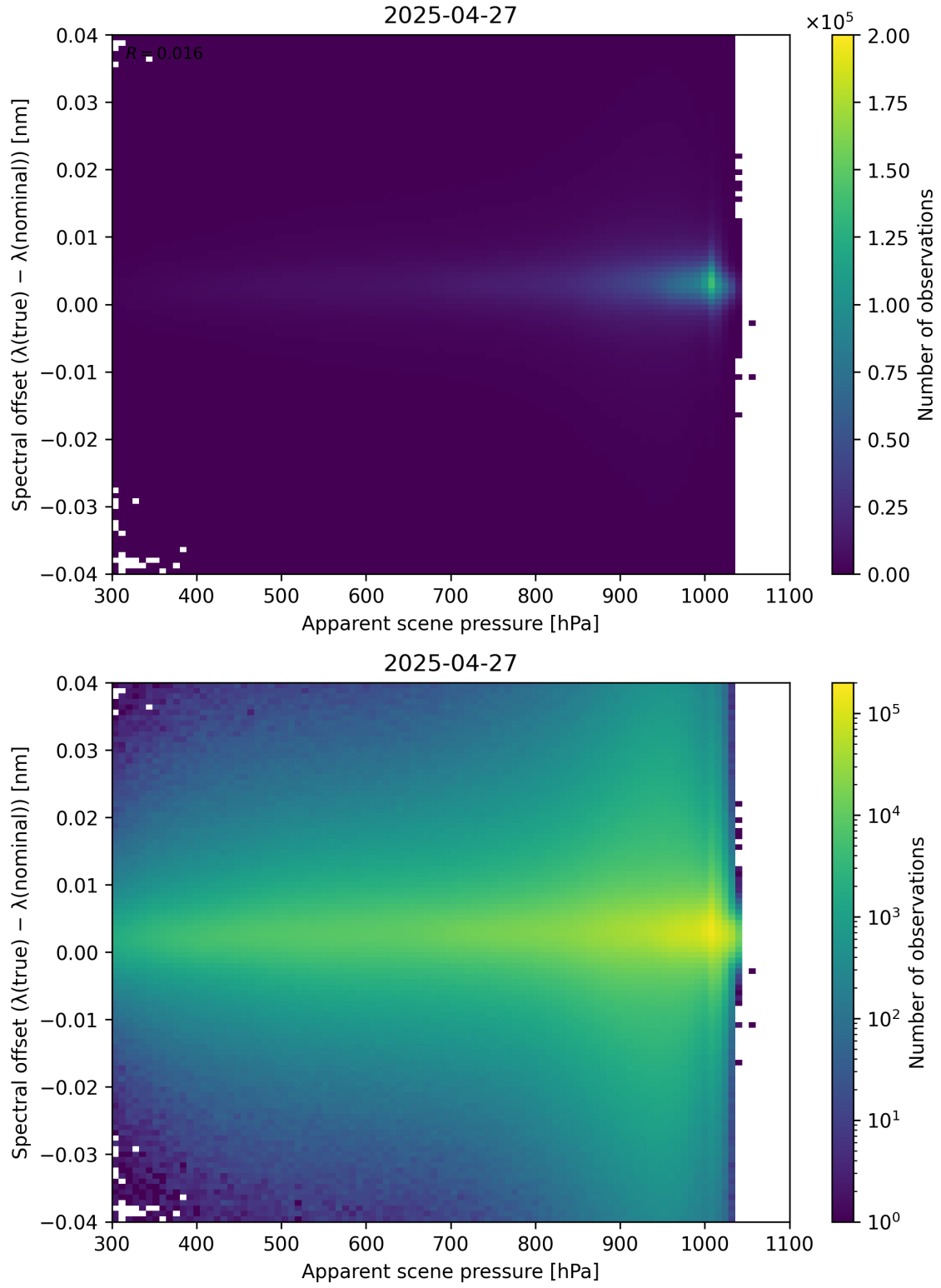
Figure 67: Scatter density plot of “Apparent scene pressure” against “Spectral offset ( \lambda_{\text{true}} - \lambda_{\text{nominal}} )” for 2025-04-26 to 2025-04-28.
