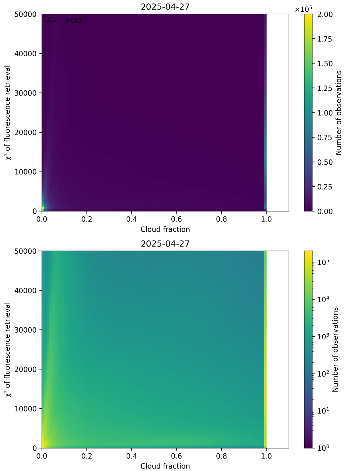
Figure 71: Scatter density plot of “Cloud fraction” against “ \chi^2 of fluorescence retrieval” for 2025-04-26 to 2025-04-28.
