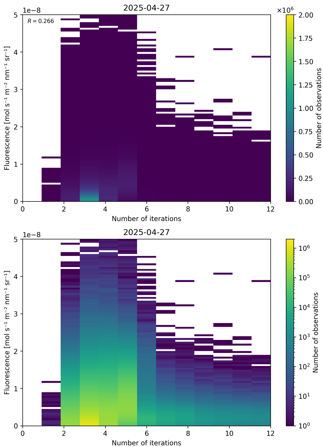
Figure 98: Scatter density plot of “Number of iterations” against “Fluorescence” for 2025-04-26 to 2025-04-28.
