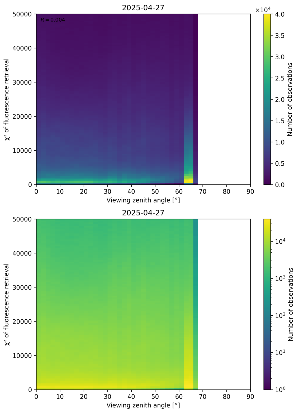
Figure 119: Scatter density plot of “Viewing zenith angle” against “ \chi^2 of fluorescence retrieval” for 2025-04-26 to 2025-04-28.
