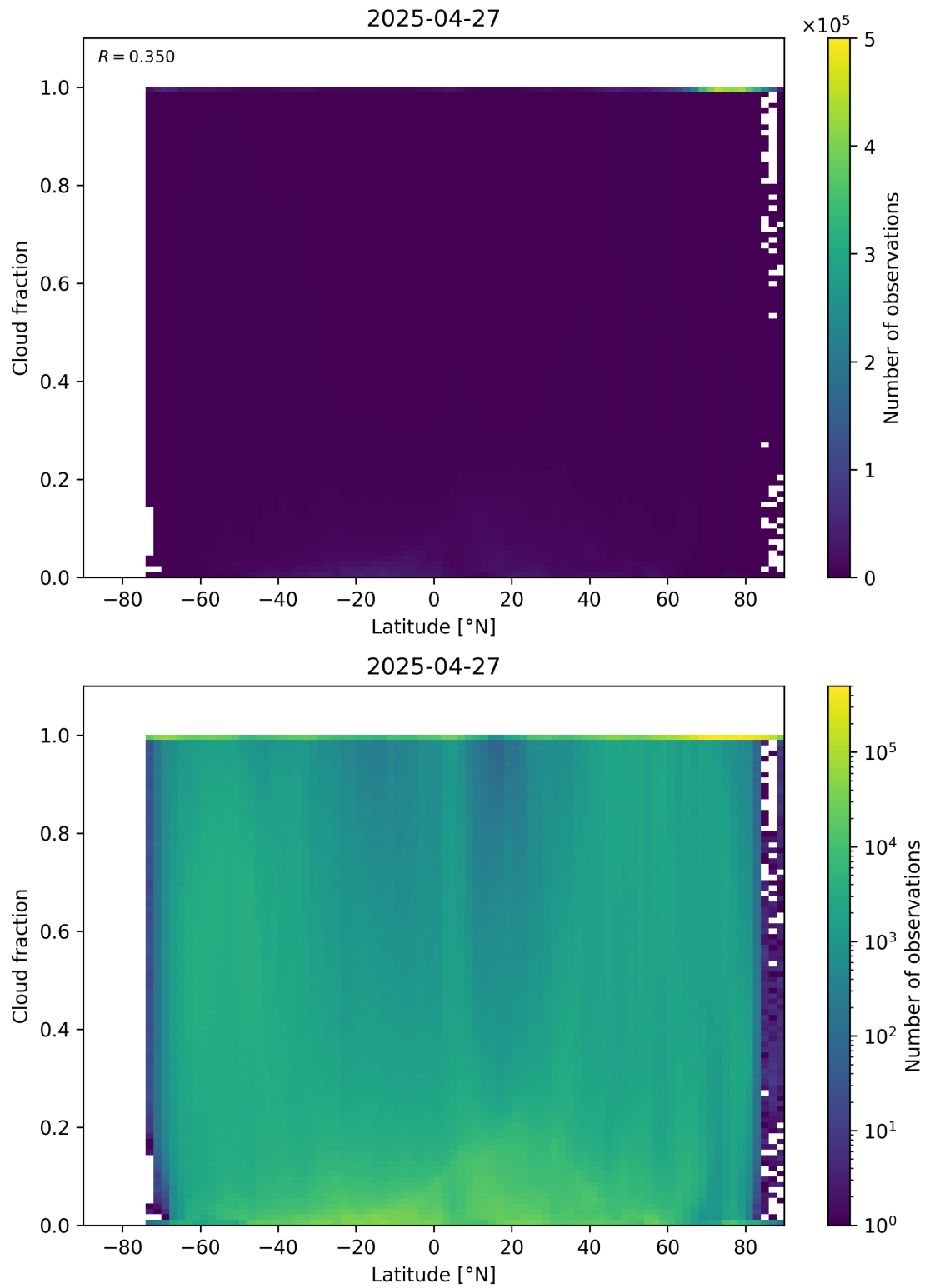
Figure 90: Scatter density plot of “Latitude” against “Cloud fraction” for 2025-04-26 to 2025-04-28.
