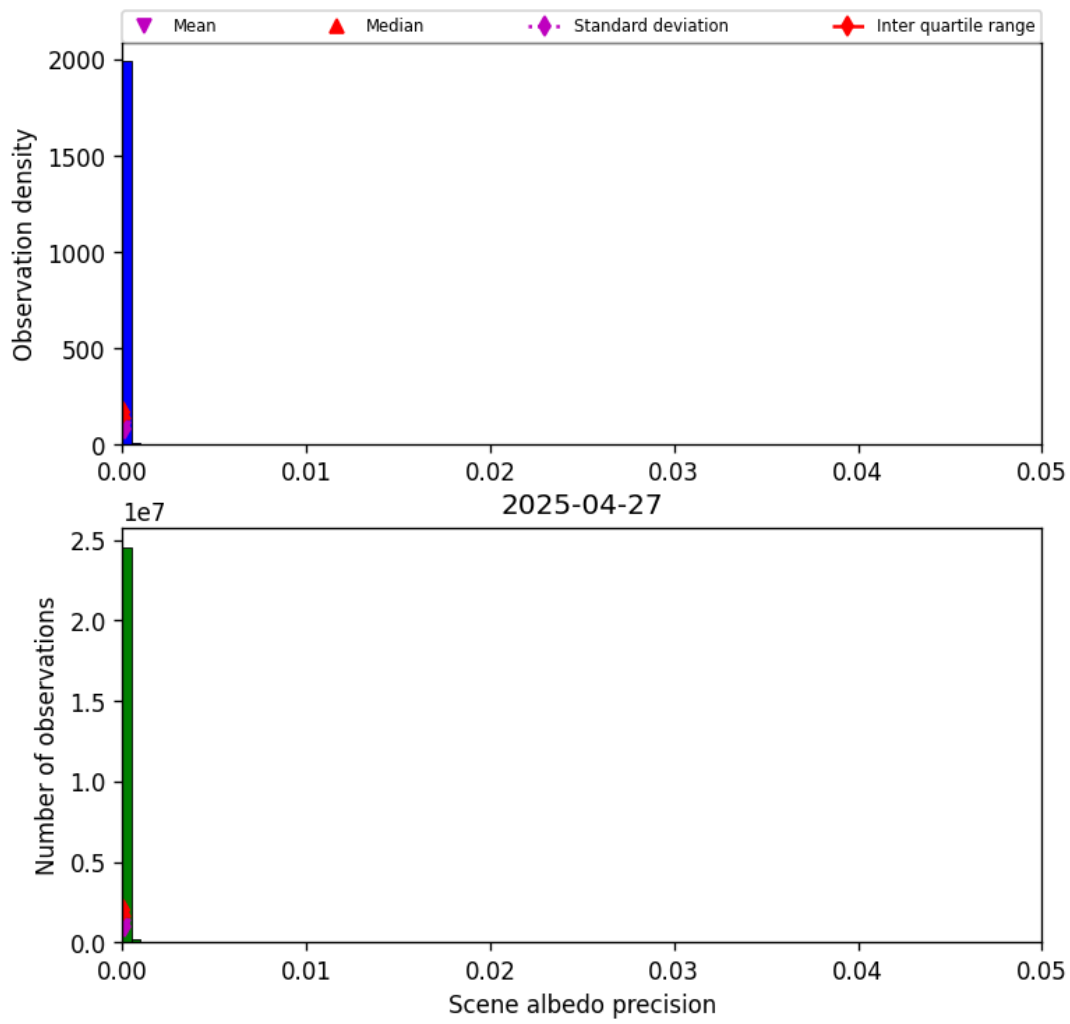
Figure 35: Histogram of “Scene albedo precision” for 2025-04-26 to 2025-04-28
