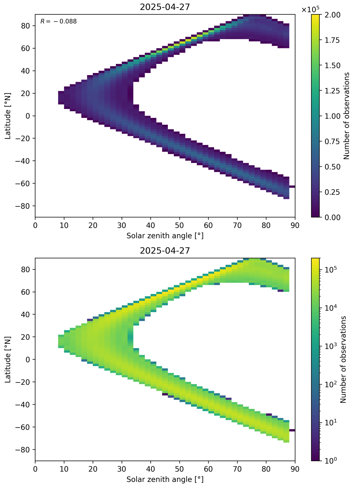
Figure 113: Scatter density plot of “Solar zenith angle” against “Latitude” for 2025-04-26 to 2025-04-28.
