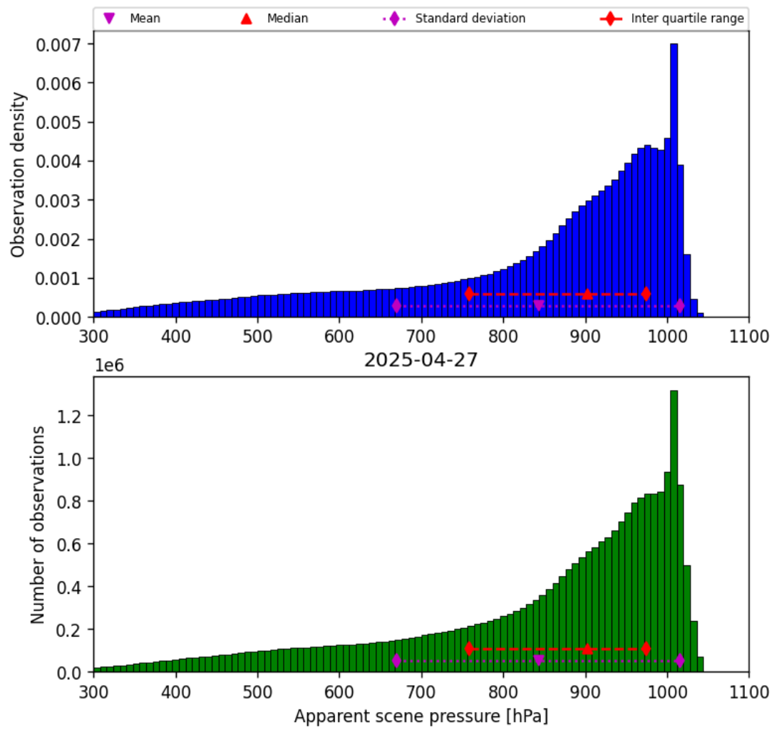
Figure 36: Histogram of “Apparent scene pressure” for 2025-04-26 to 2025-04-28
