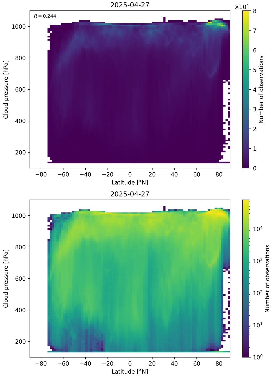
Figure 91: Scatter density plot of “Latitude” against “Cloud pressure” for 2025-04-26 to 2025-04-28.
