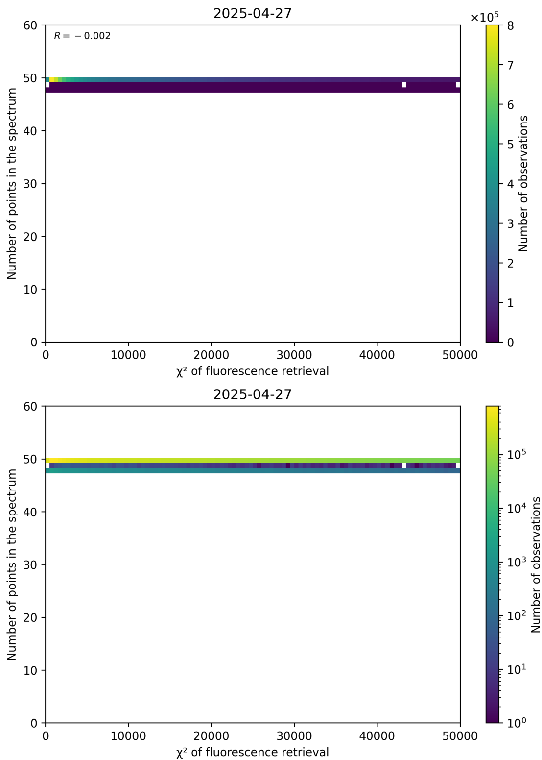
Figure 68: Scatter density plot of " \chi^2 of fluorescence retrieval" against "Number of points in the spectrum" for 2025-04-26 to 2025-04-28.
