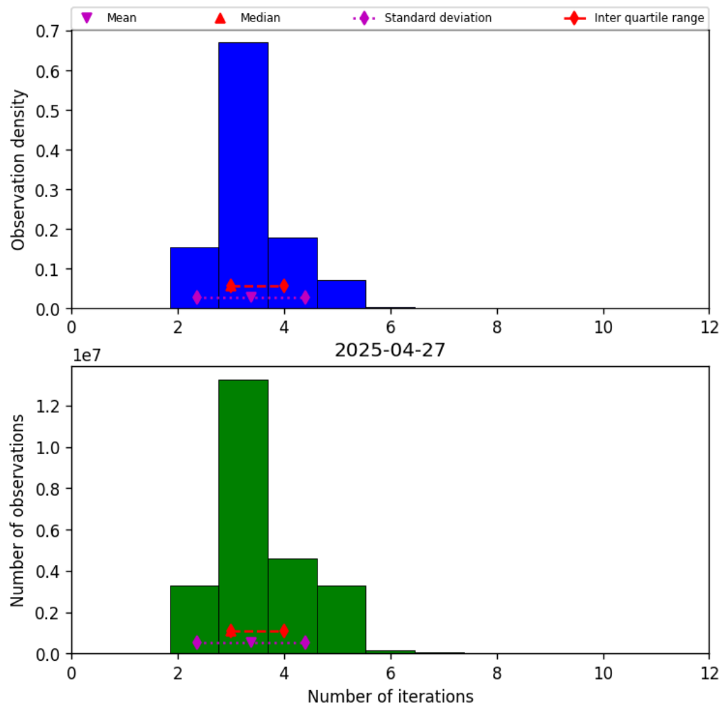
Figure 39: Histogram of “Number of iterations” for 2025-04-26 to 2025-04-28
