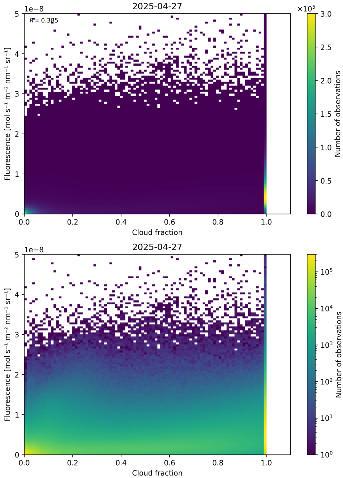
Figure 72: Scatter density plot of “Cloud fraction” against “Fluorescence” for 2025-04-26 to 2025-04-28.
