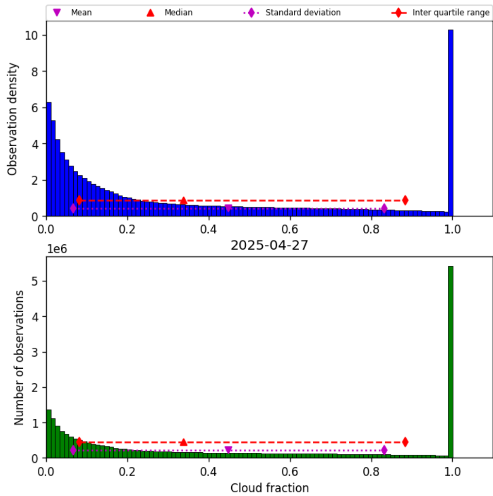
Figure 32: Histogram of “Cloud fraction” for 2025-04-26 to 2025-04-28
