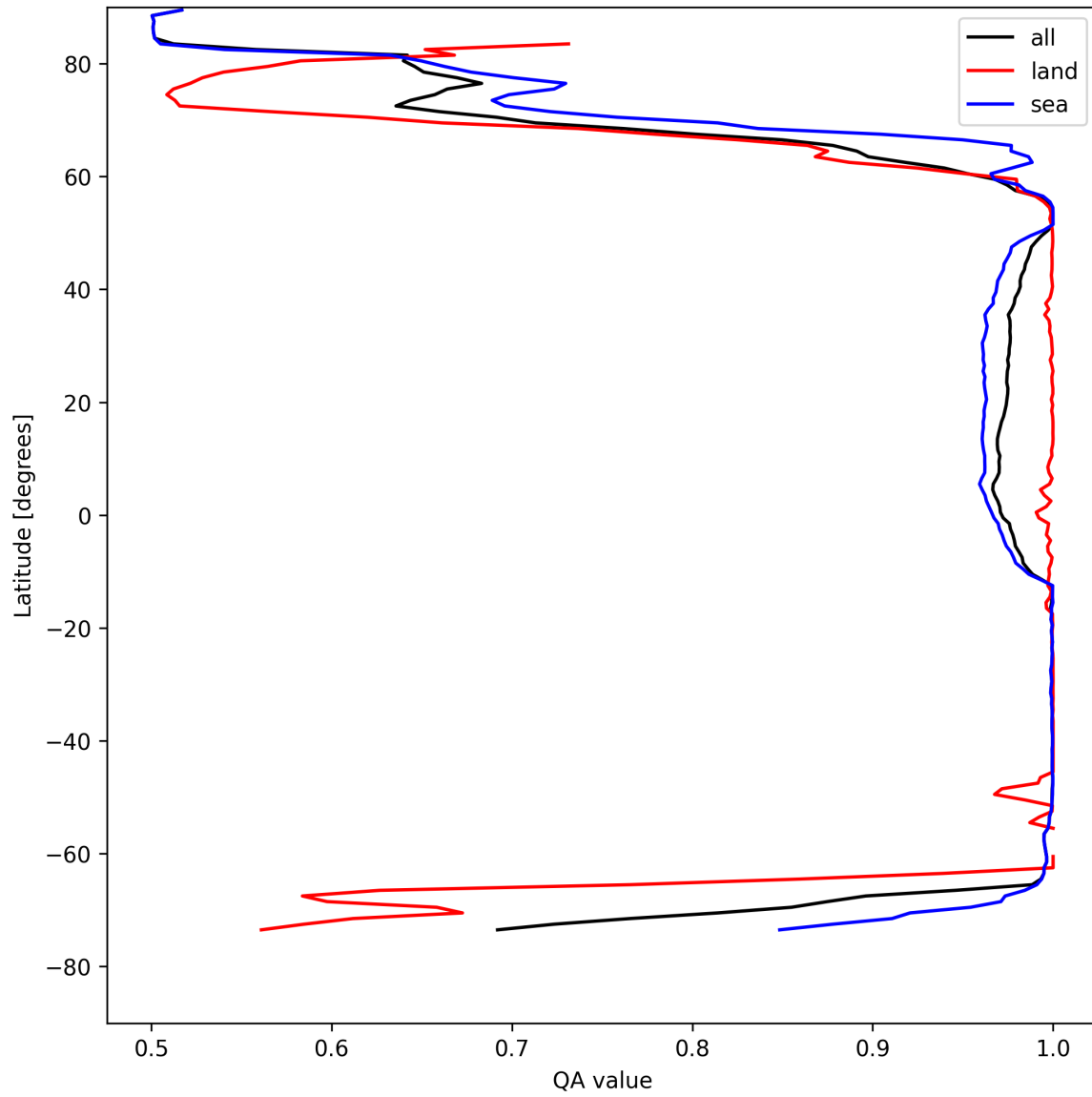
Figure 12: Zonal average of “QA value” for 2025-04-26 to 2025-04-28.
