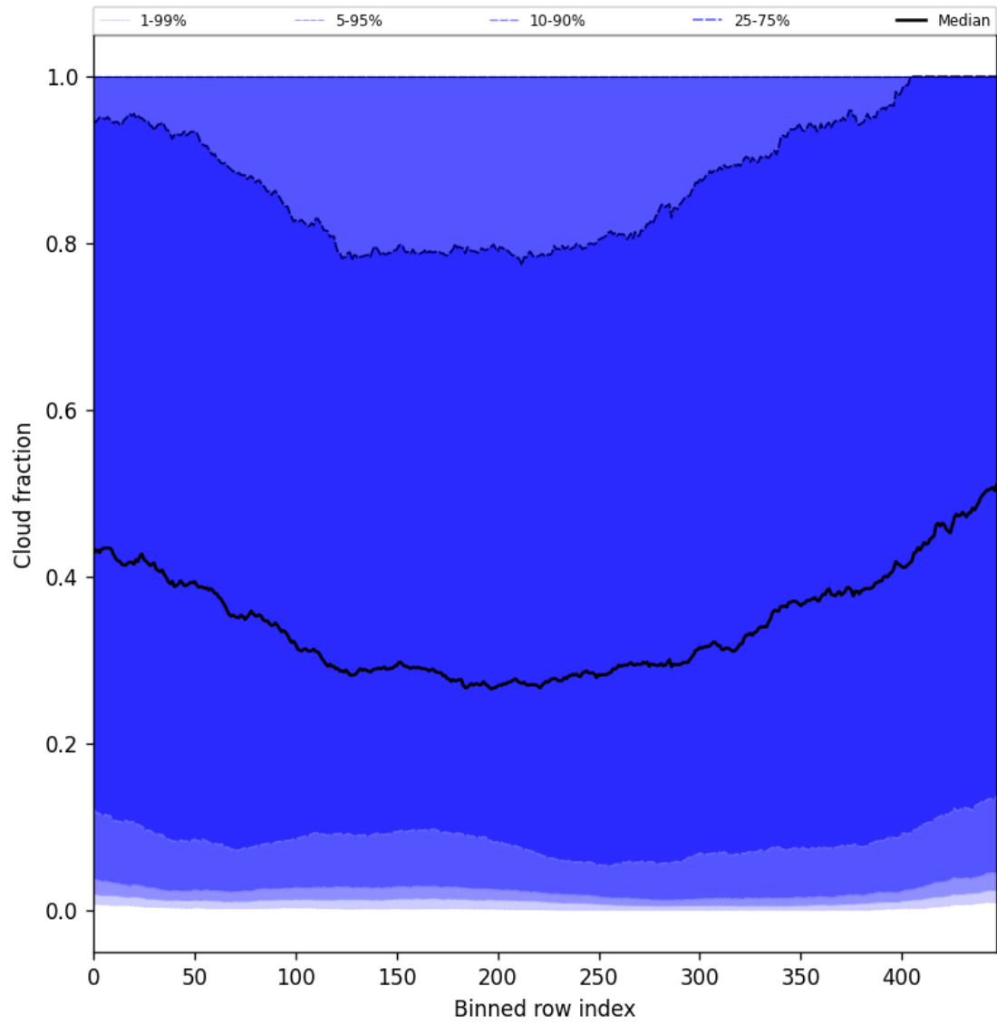
Figure 49: Along track statistics of “Cloud fraction” for 2025-04-26 to 2025-04-28
