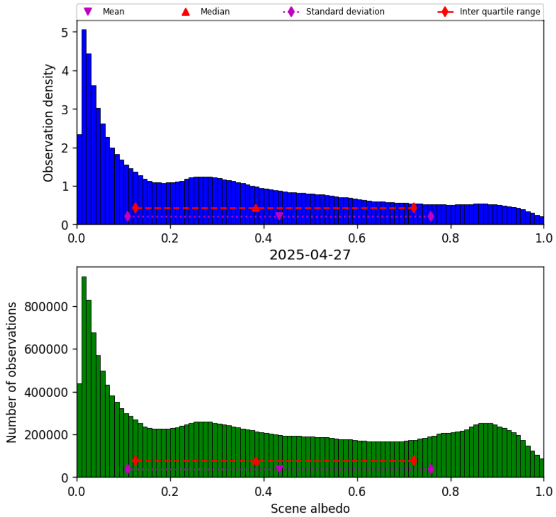
Figure 34: Histogram of “Scene albedo” for 2025-04-26 to 2025-04-28
