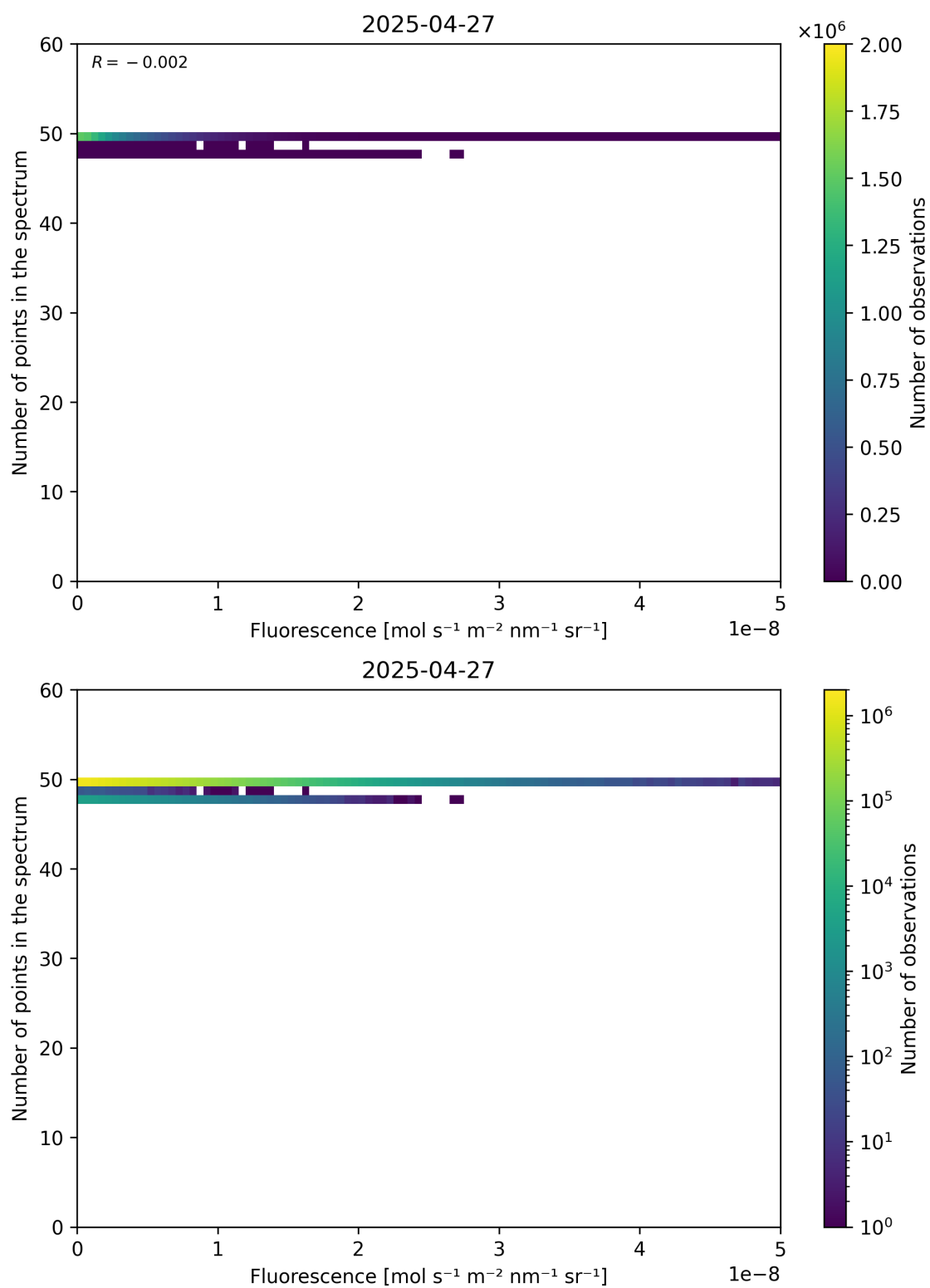
Figure 86: Scatter density plot of “Fluorescence” against “Number of points in the spectrum” for 2025-04-26 to 2025-04-28.
