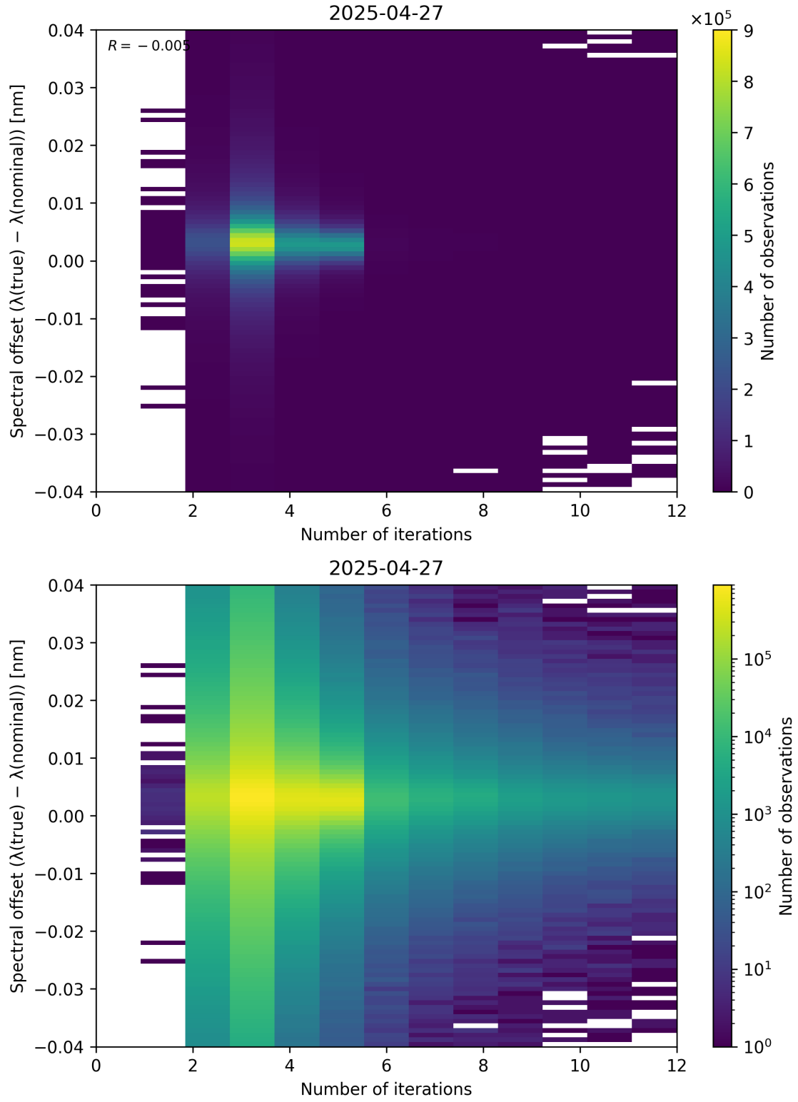
Figure 100: Scatter density plot of “Number of iterations” against “Spectral offset ( \lambda_{\text{true}} - \lambda_{\text{nominal}} )” for 2025-04-26 to 2025-04-28.
