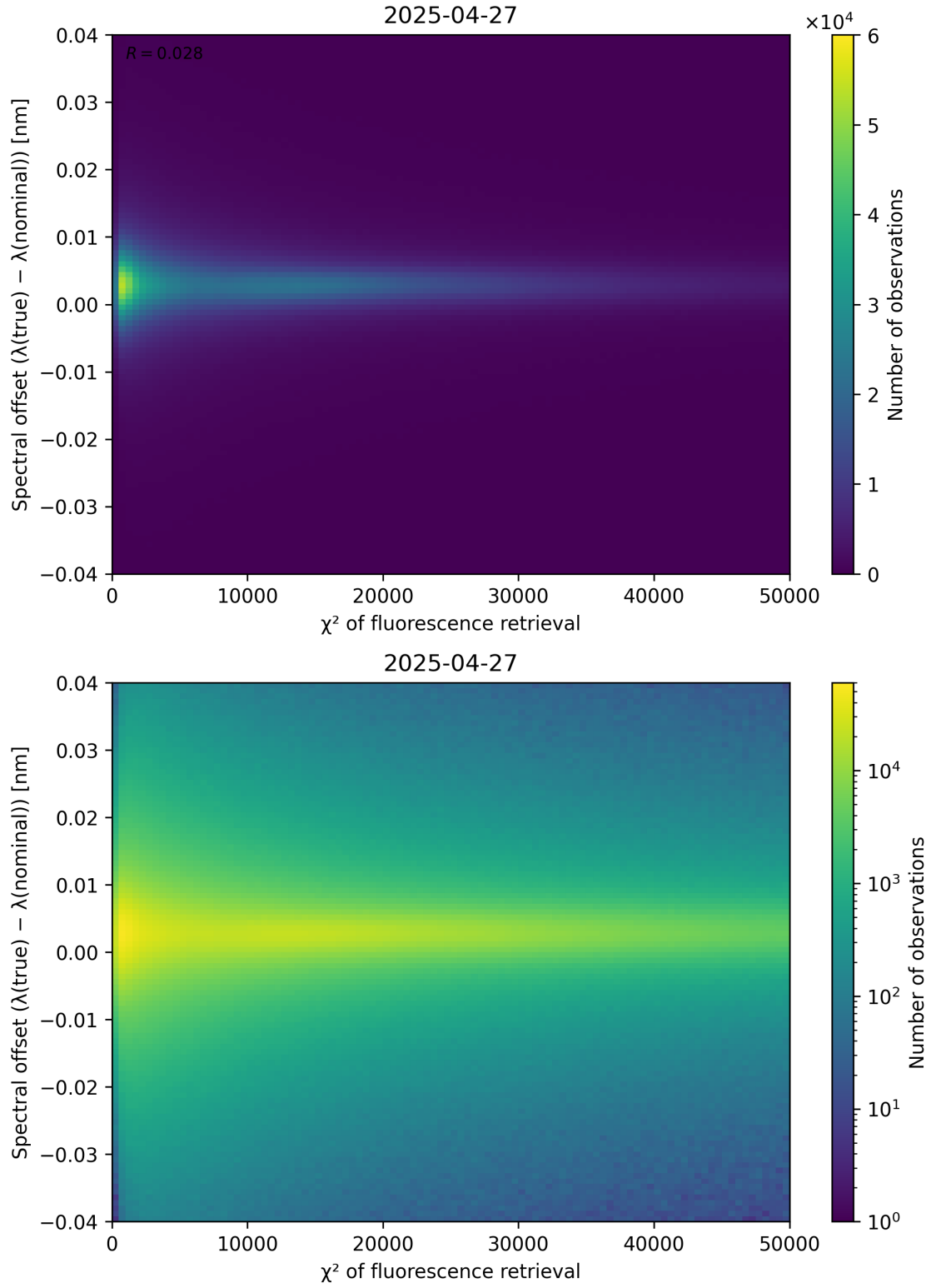
Figure 69: Scatter density plot of “ \chi^2 of fluorescence retrieval” against “Spectral offset ( \lambda_{\text{true}} - \lambda_{\text{nominal}} )” for 2025-04-26 to 2025-04-28.
