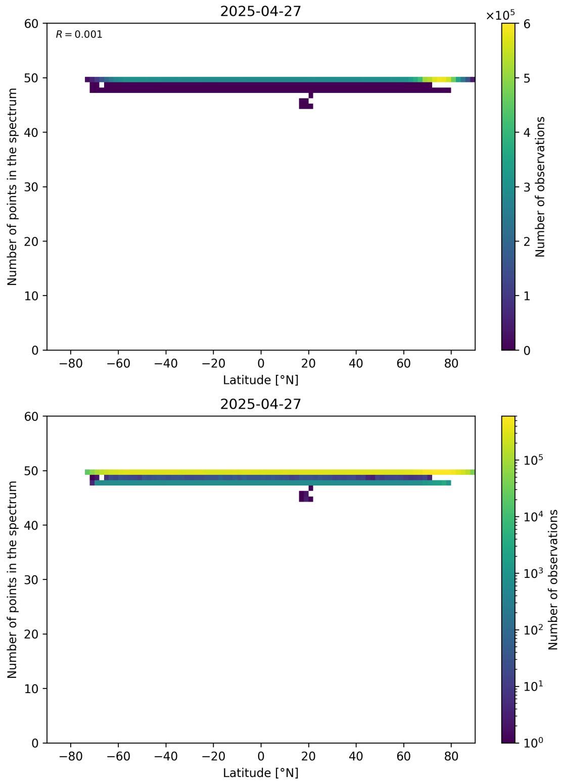
Figure 94: Scatter density plot of “Latitude” against “Number of points in the spectrum” for 2025-04-26 to 2025-04-28.
