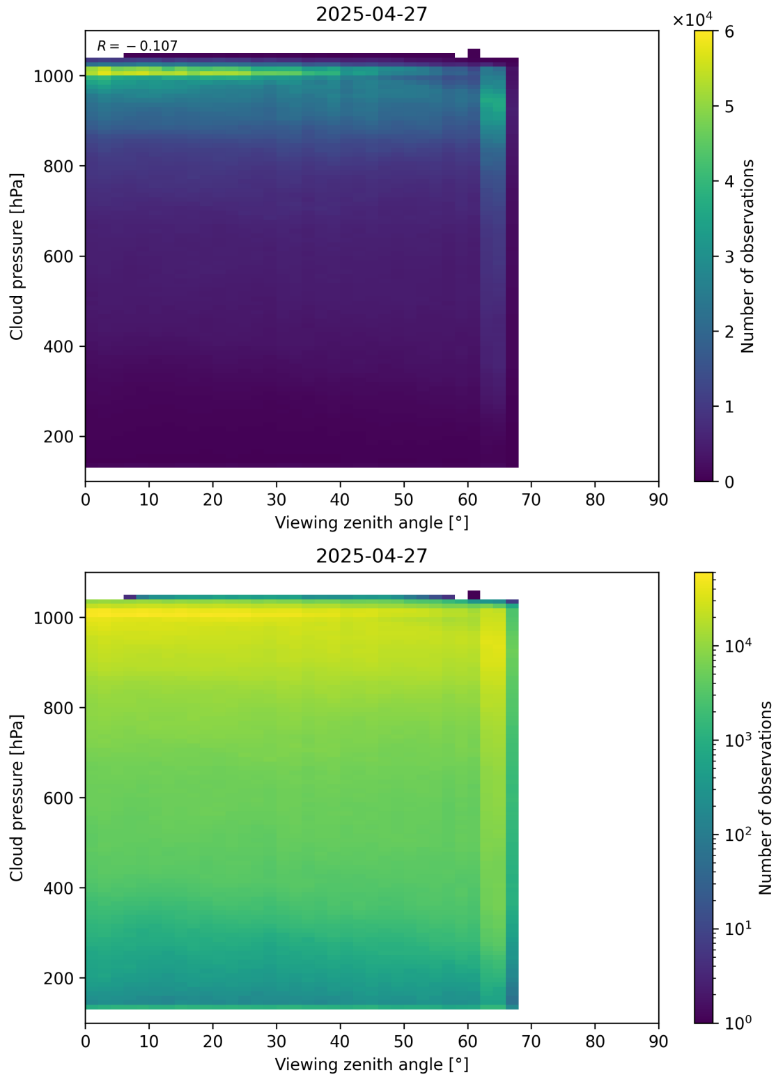
Figure 121: Scatter density plot of “Viewing zenith angle” against “Cloud pressure” for 2025-04-26 to 2025-04-28.
