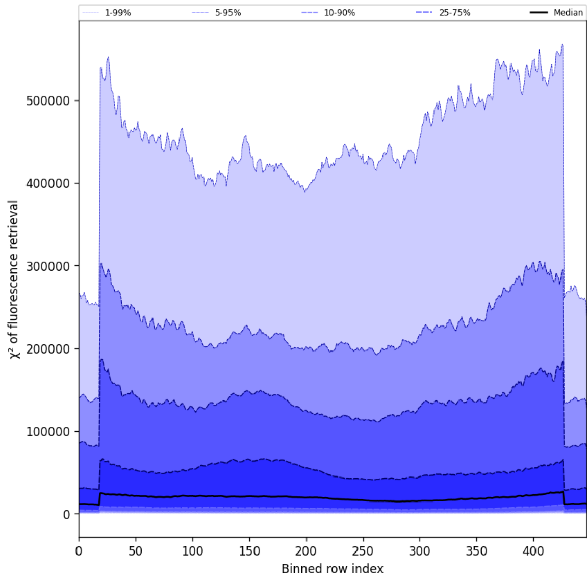
Figure 59: Along track statistics of “ \chi^2 of fluorescence retrieval” for 2025-04-26 to 2025-04-28
