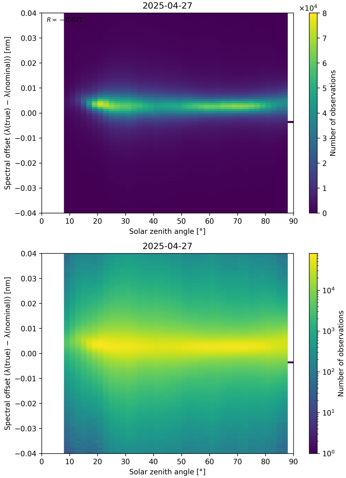
Figure 117: Scatter density plot of “Solar zenith angle” against “Spectral offset ( \lambda_{\text{true}} - \lambda_{\text{nominal}} )” for 2025-04-26 to 2025-04-28.
