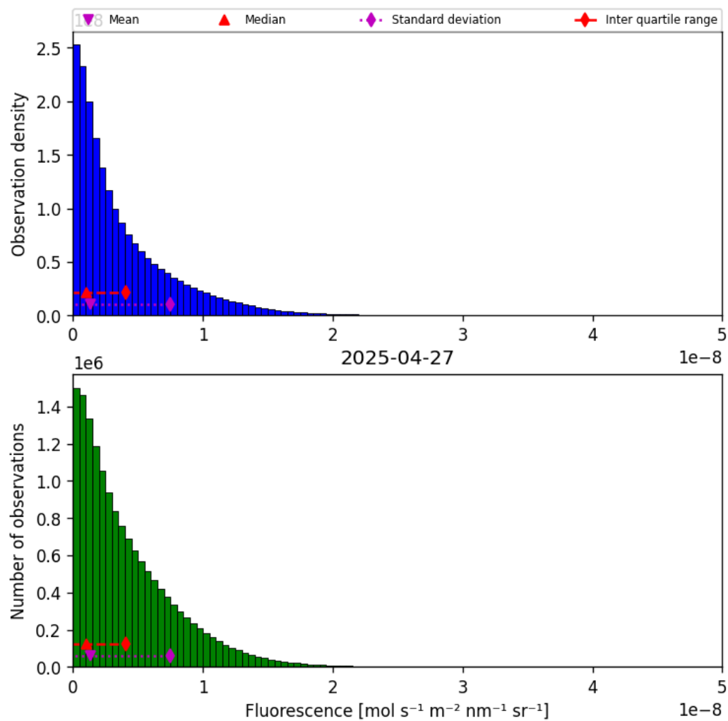
Figure 40: Histogram of “Fluorescence” for 2025-04-26 to 2025-04-28
