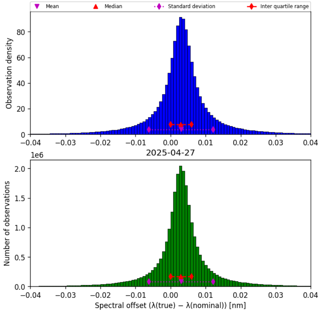
Figure 45: Histogram of “Spectral offset ( \lambda_{\text{true}} - \lambda_{\text{nominal}} )” for 2025-04-26 to 2025-04-28
