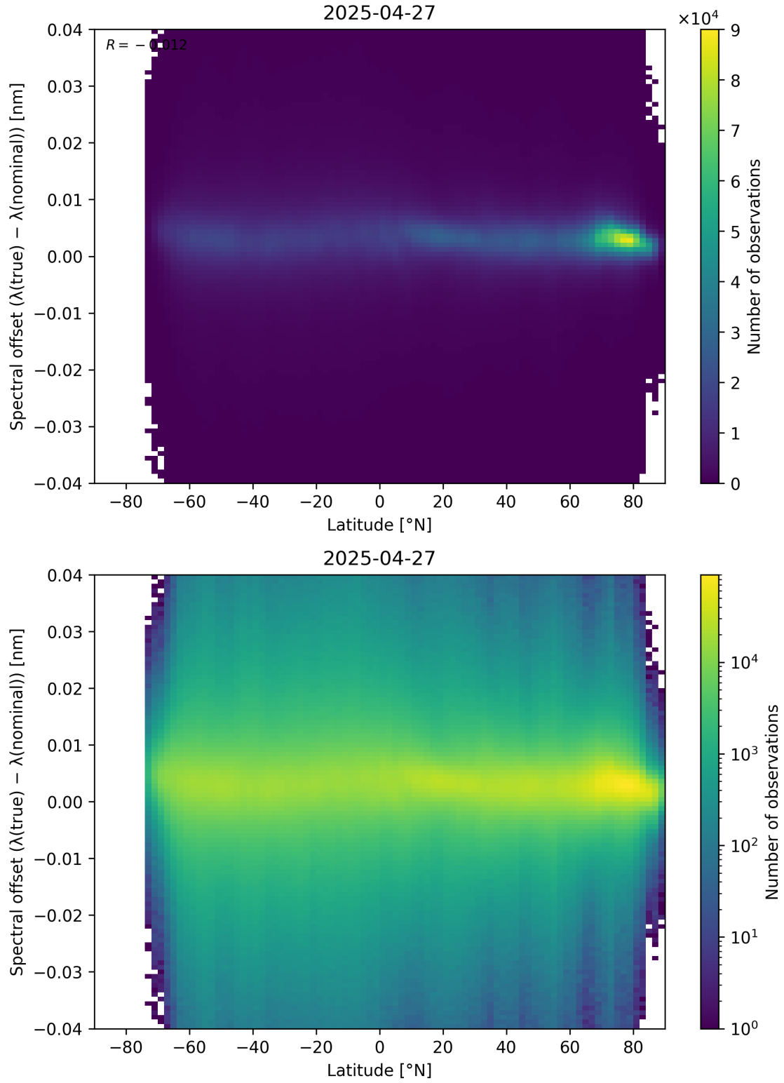
Figure 96: Scatter density plot of “Latitude” against “Spectral offset ( \lambda_{\text{true}} - \lambda_{\text{nominal}} )” for 2025-04-26 to 2025-04-28.
