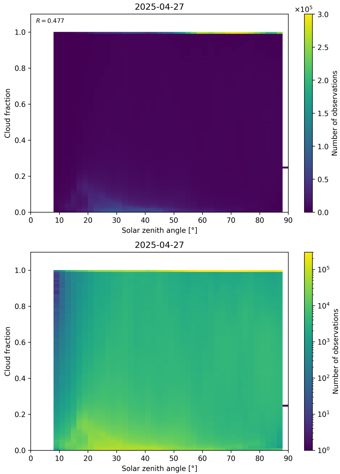
Figure 110: Scatter density plot of “Solar zenith angle” against “Cloud fraction” for 2025-04-26 to 2025-04-28.
