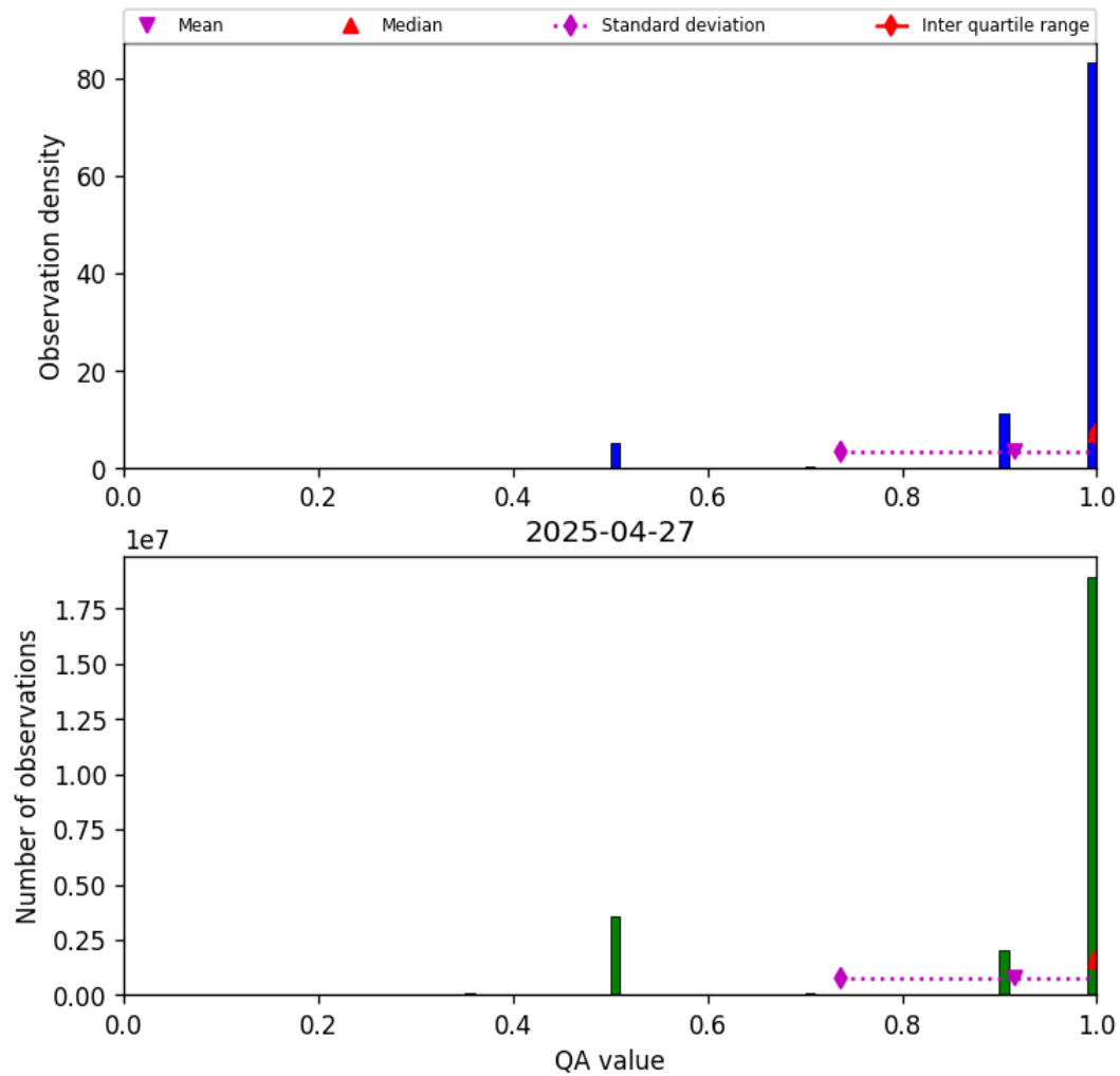
Figure 29: Histogram of “QA value” for 2025-04-26 to 2025-04-28
