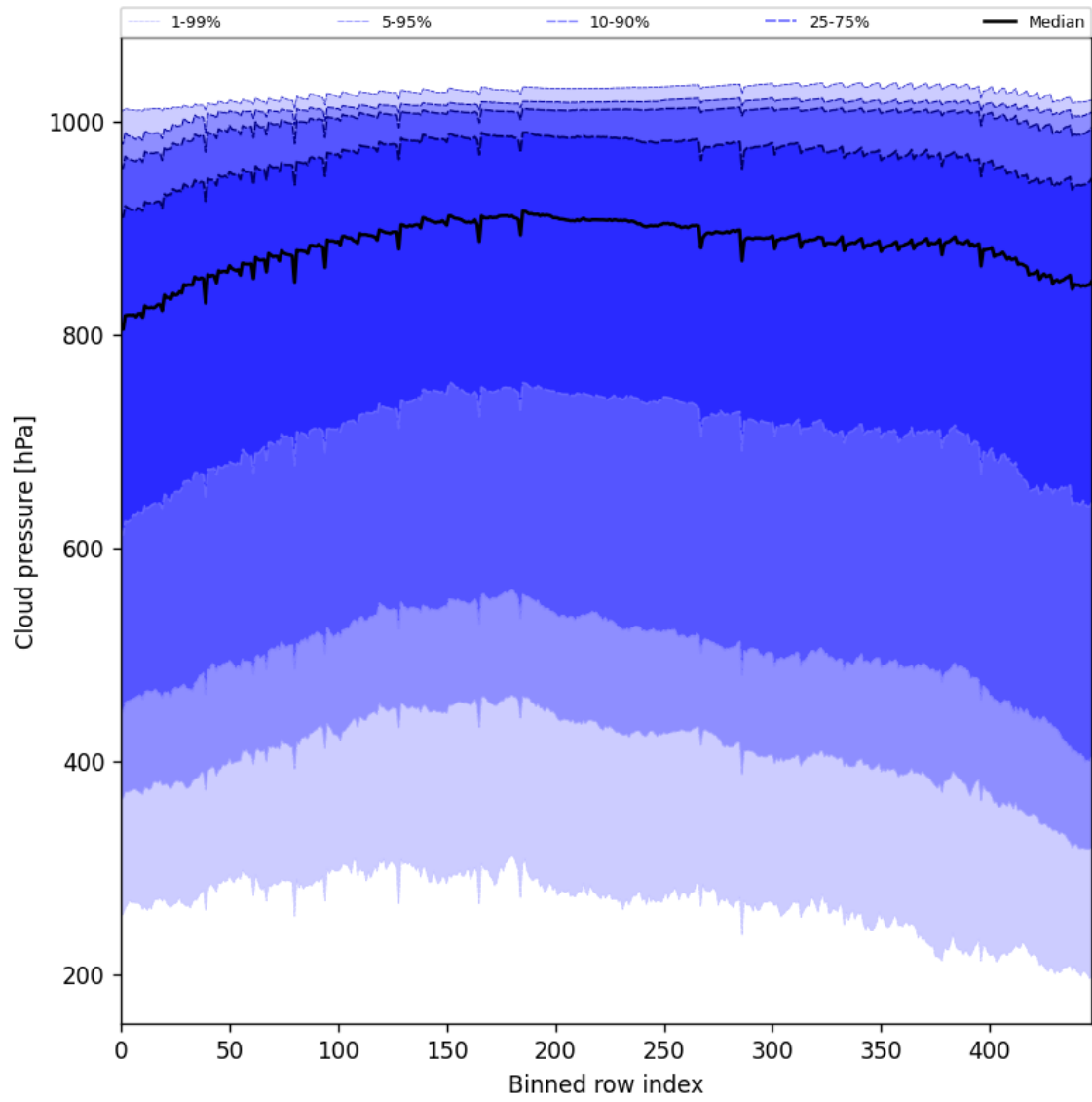
Figure 47: Along track statistics of “Cloud pressure” for 2025-04-26 to 2025-04-28
