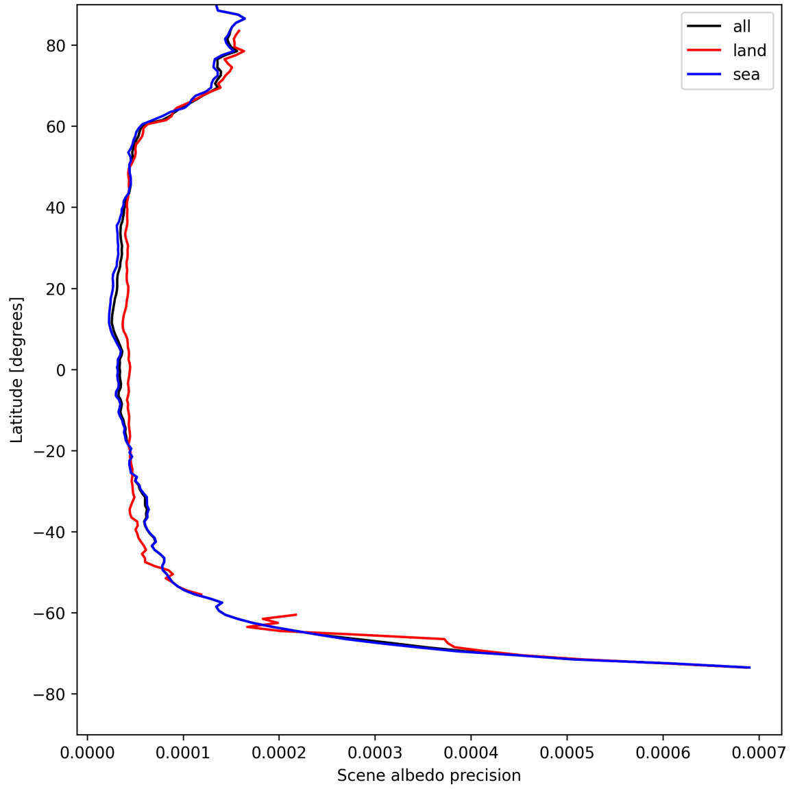
Figure 18: Zonal average of “Scene albedo precision” for 2025-04-26 to 2025-04-28.
