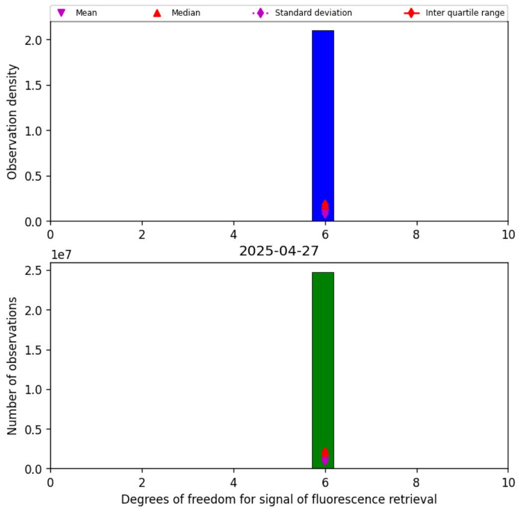
Figure 43: Histogram of "Degrees of freedom for signal of fluorescence retrieval" for 2025-04-26 to 2025-04-28
