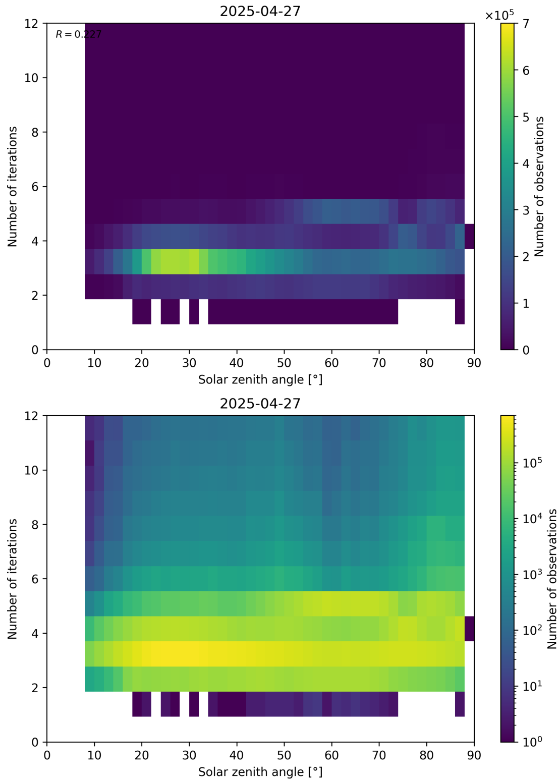
Figure 114: Scatter density plot of “Solar zenith angle” against “Number of iterations” for 2025-04-26 to 2025-04-28.
