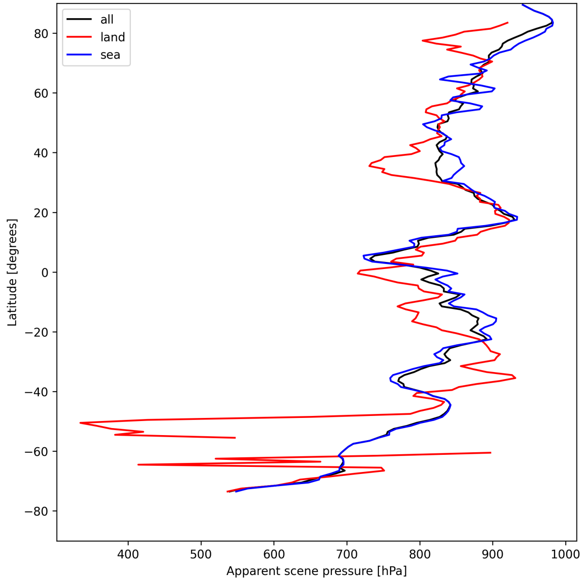
Figure 19: Zonal average of “Apparent scene pressure” for 2025-04-26 to 2025-04-28.
