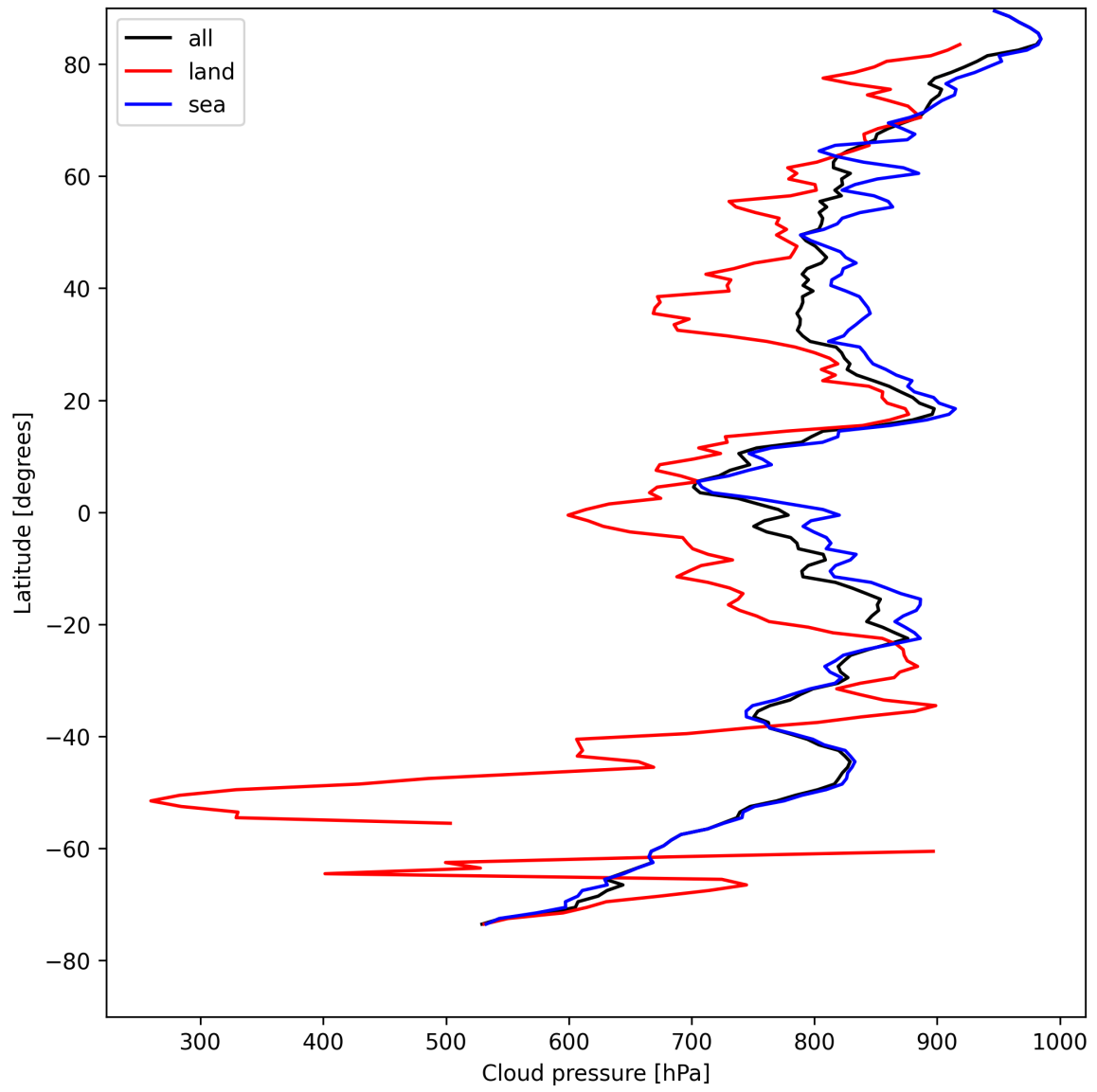
Figure 13: Zonal average of “Cloud pressure” for 2025-04-26 to 2025-04-28.
