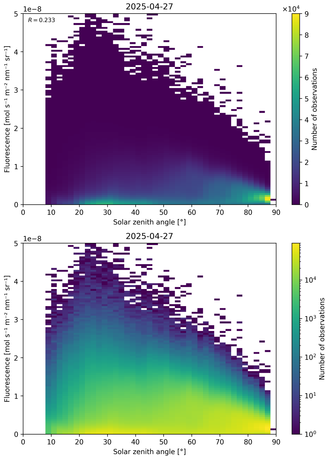
Figure 112: Scatter density plot of “Solar zenith angle” against “Fluorescence” for 2025-04-26 to 2025-04-28.
