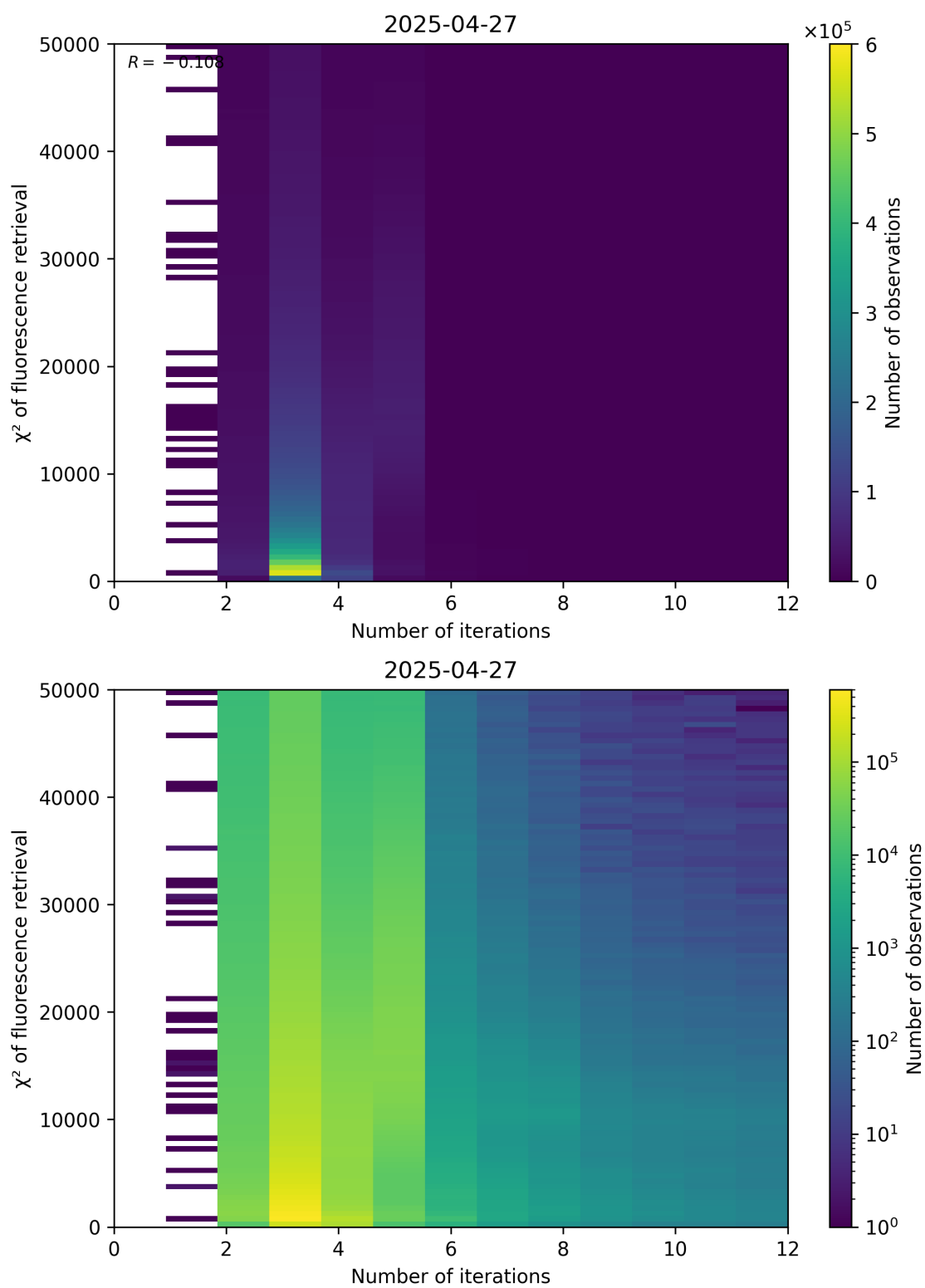
Figure 97: Scatter density plot of “Number of iterations” against “ \chi^2 of fluorescence retrieval” for 2025-04-26 to 2025-04-28.
