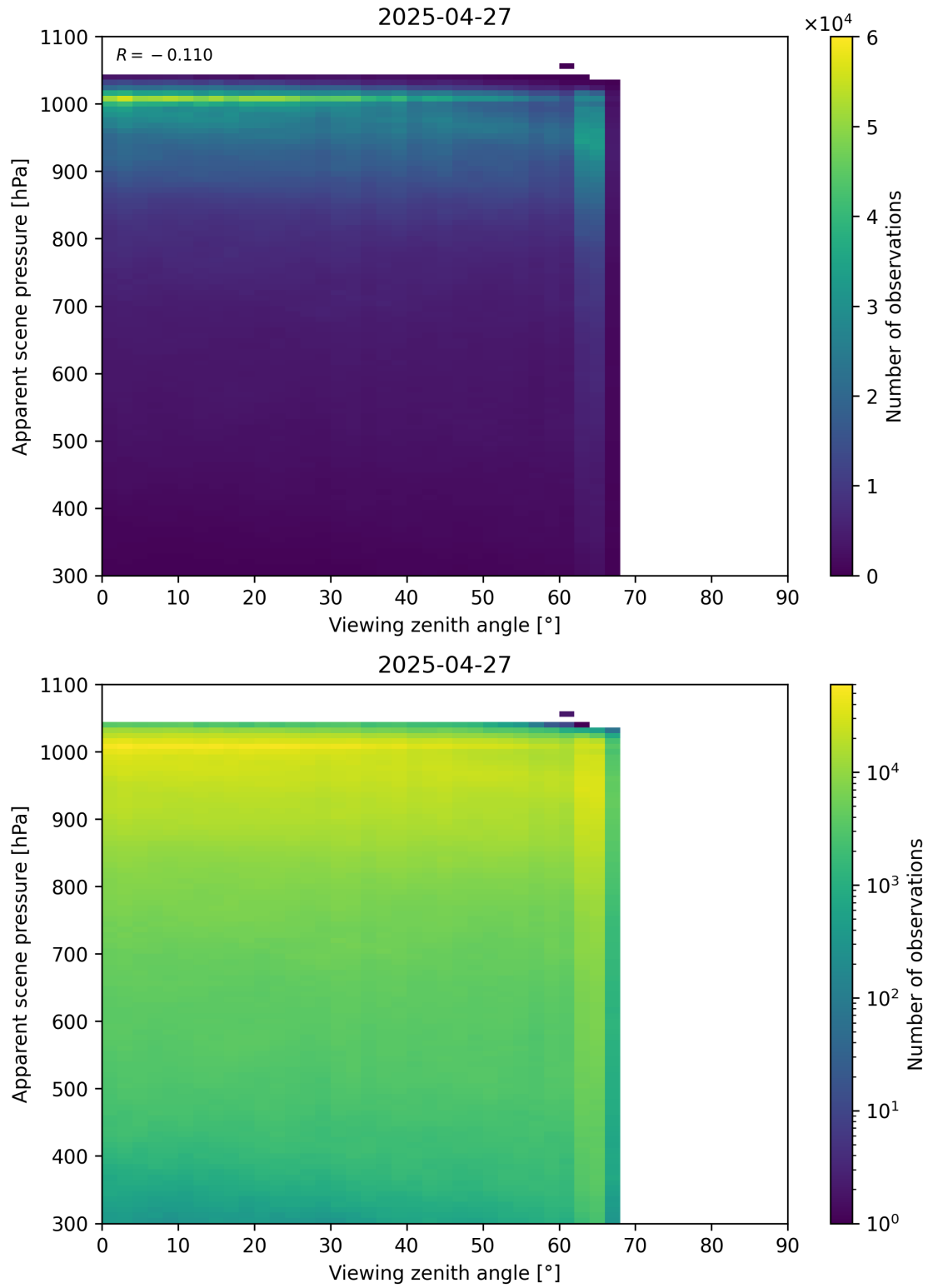
Figure 118: Scatter density plot of “Viewing zenith angle” against “Apparent scene pressure” for 2025-04-26 to 2025-04-28.
