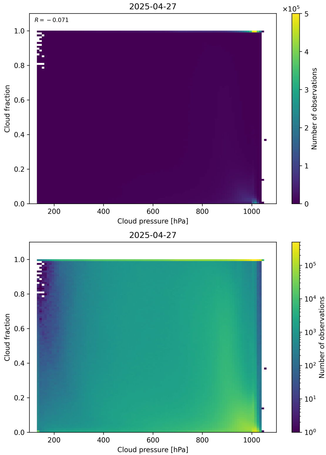
Figure 79: Scatter density plot of “Cloud pressure” against “Cloud fraction” for 2025-04-26 to 2025-04-28.
