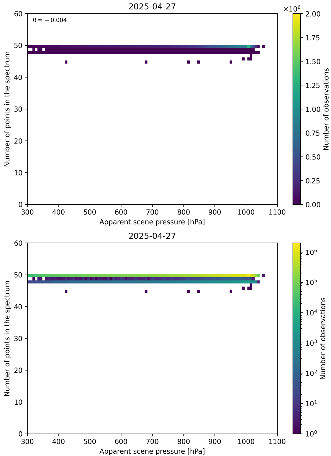
Figure 66: Scatter density plot of “Apparent scene pressure” against “Number of points in the spectrum” for 2025-04-26 to 2025-04-28.
