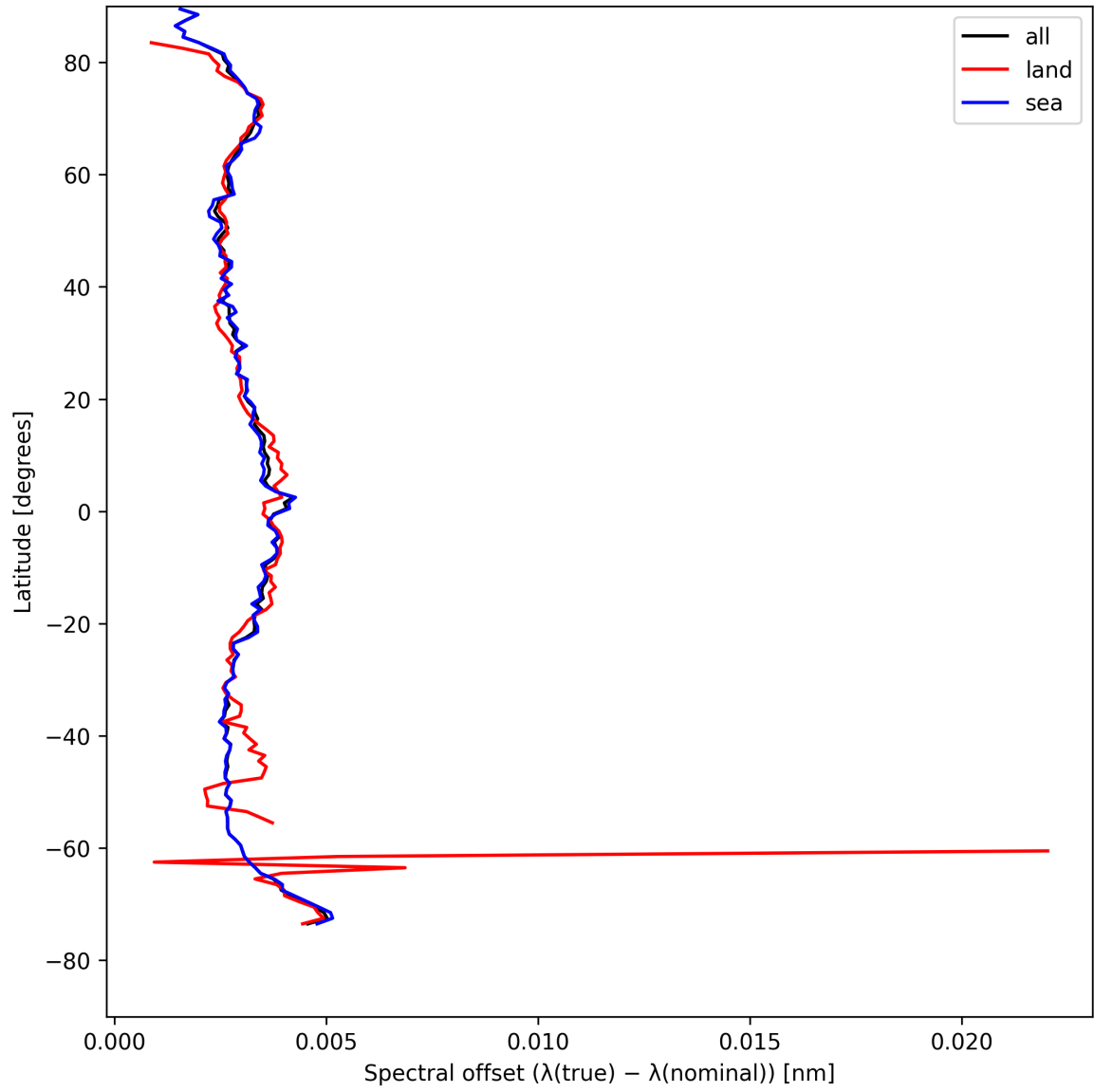
Figure 28: Zonal average of “Spectral offset ( \lambda_{\text{true}} - \lambda_{\text{nominal}} )” for 2025-04-26 to 2025-04-28.
