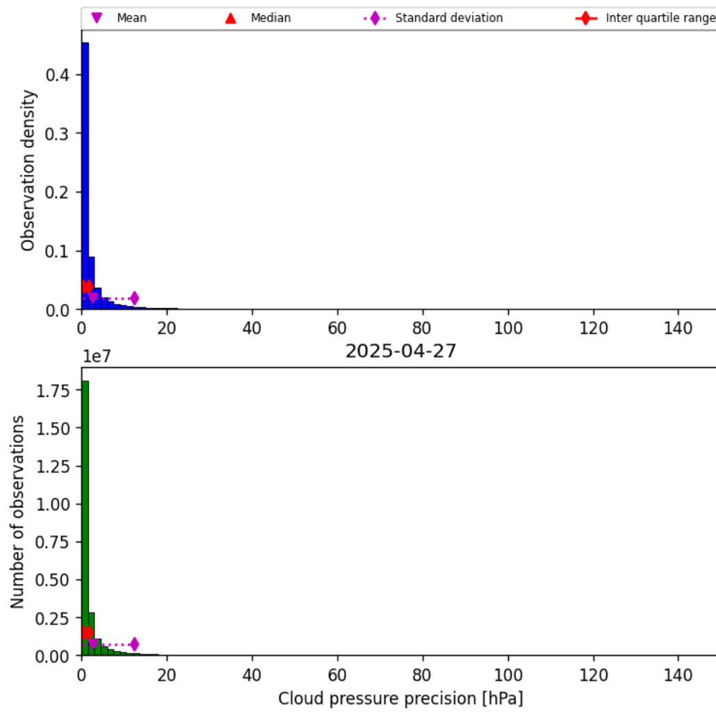
Figure 31: Histogram of “Cloud pressure precision” for 2025-04-26 to 2025-04-28
