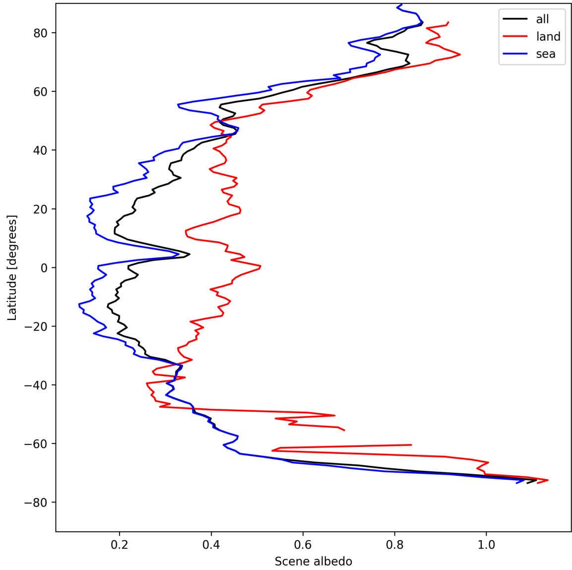
Figure 17: Zonal average of “Scene albedo” for 2025-04-26 to 2025-04-28.
