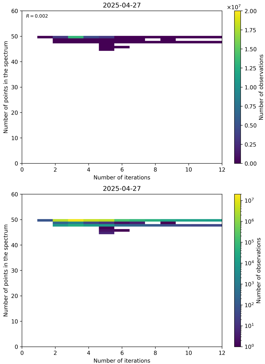
Figure 99: Scatter density plot of “Number of iterations” against “Number of points in the spectrum” for 2025-04-26 to 2025-04-28.
