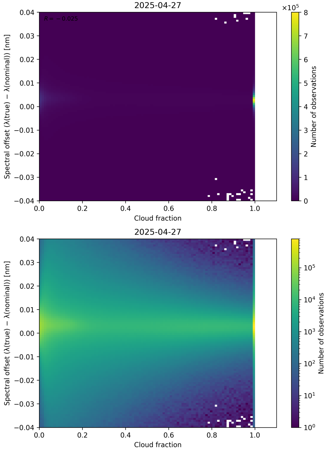
Figure 76: Scatter density plot of “Cloud fraction” against “Spectral offset ( \lambda_{\text{true}} - \lambda_{\text{nominal}} )” for 2025-04-26 to 2025-04-28.
