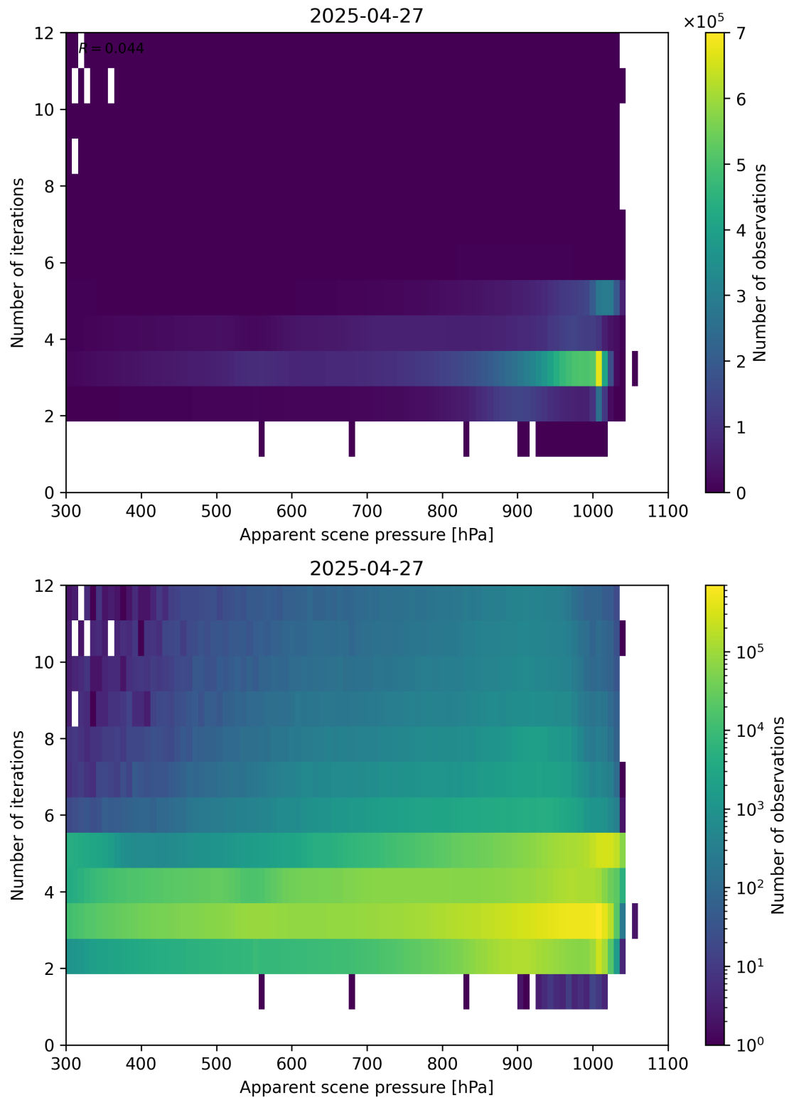
Figure 65: Scatter density plot of “Apparent scene pressure” against “Number of iterations” for 2025-04-26 to 2025-04-28.
