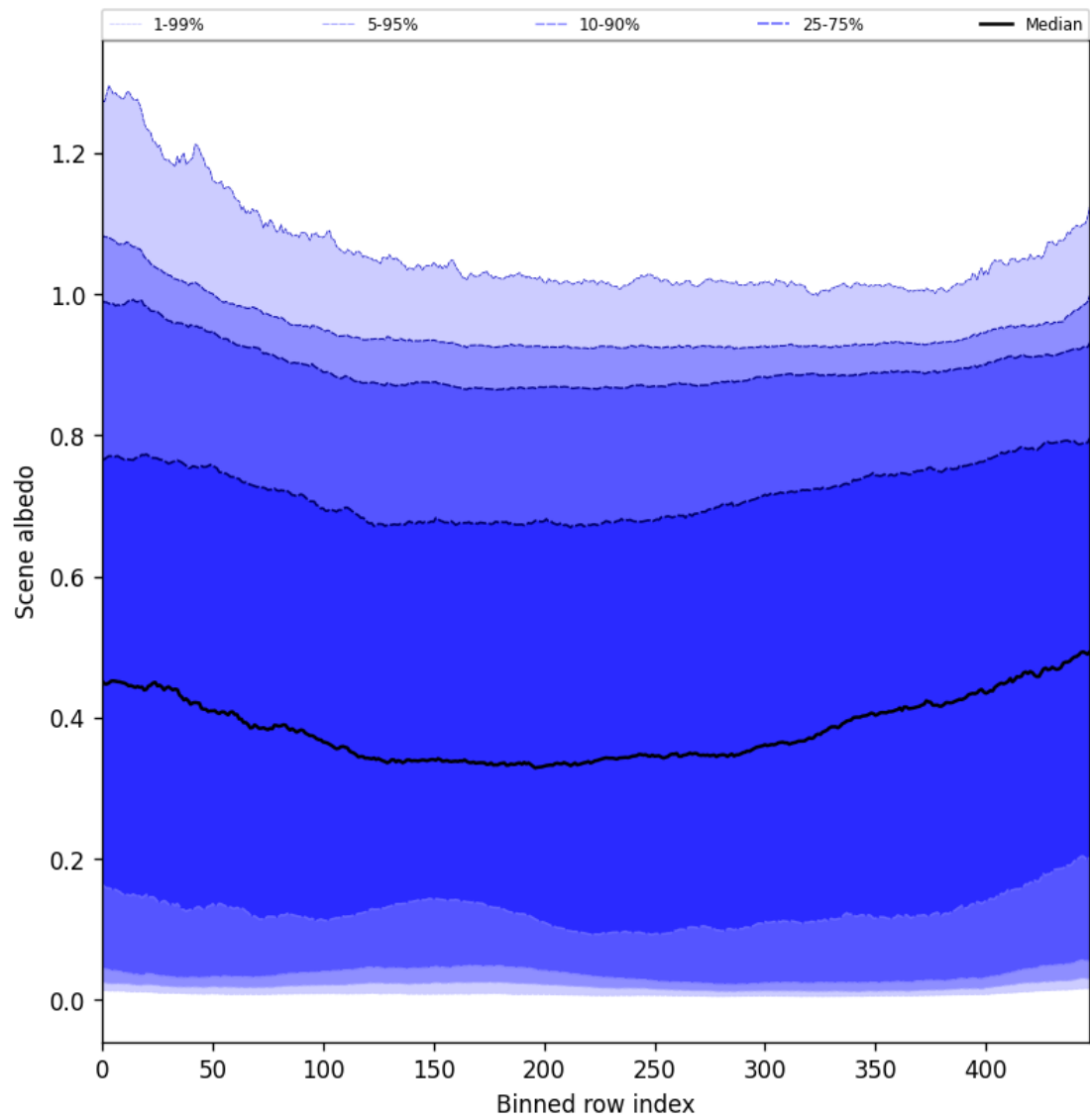
Figure 51: Along track statistics of “Scene albedo” for 2025-04-26 to 2025-04-28
