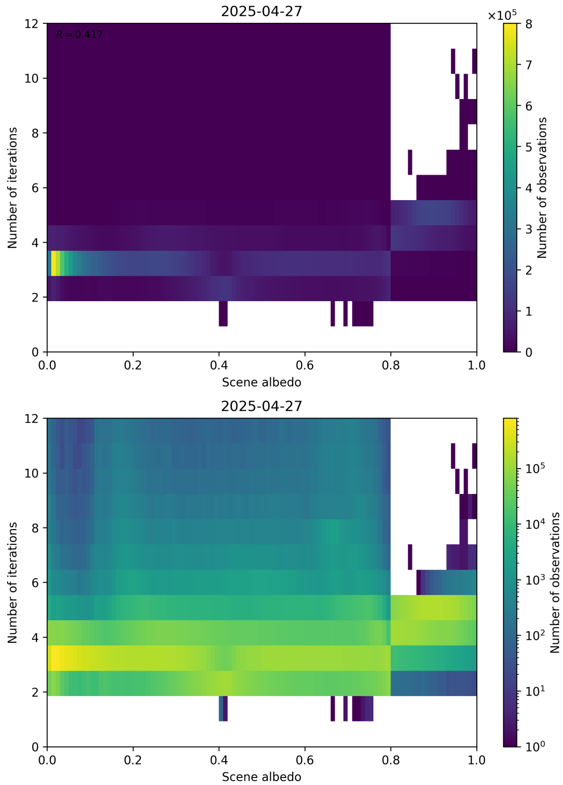
Figure 105: Scatter density plot of “Scene albedo” against “Number of iterations” for 2025-04-26 to 2025-04-28.
