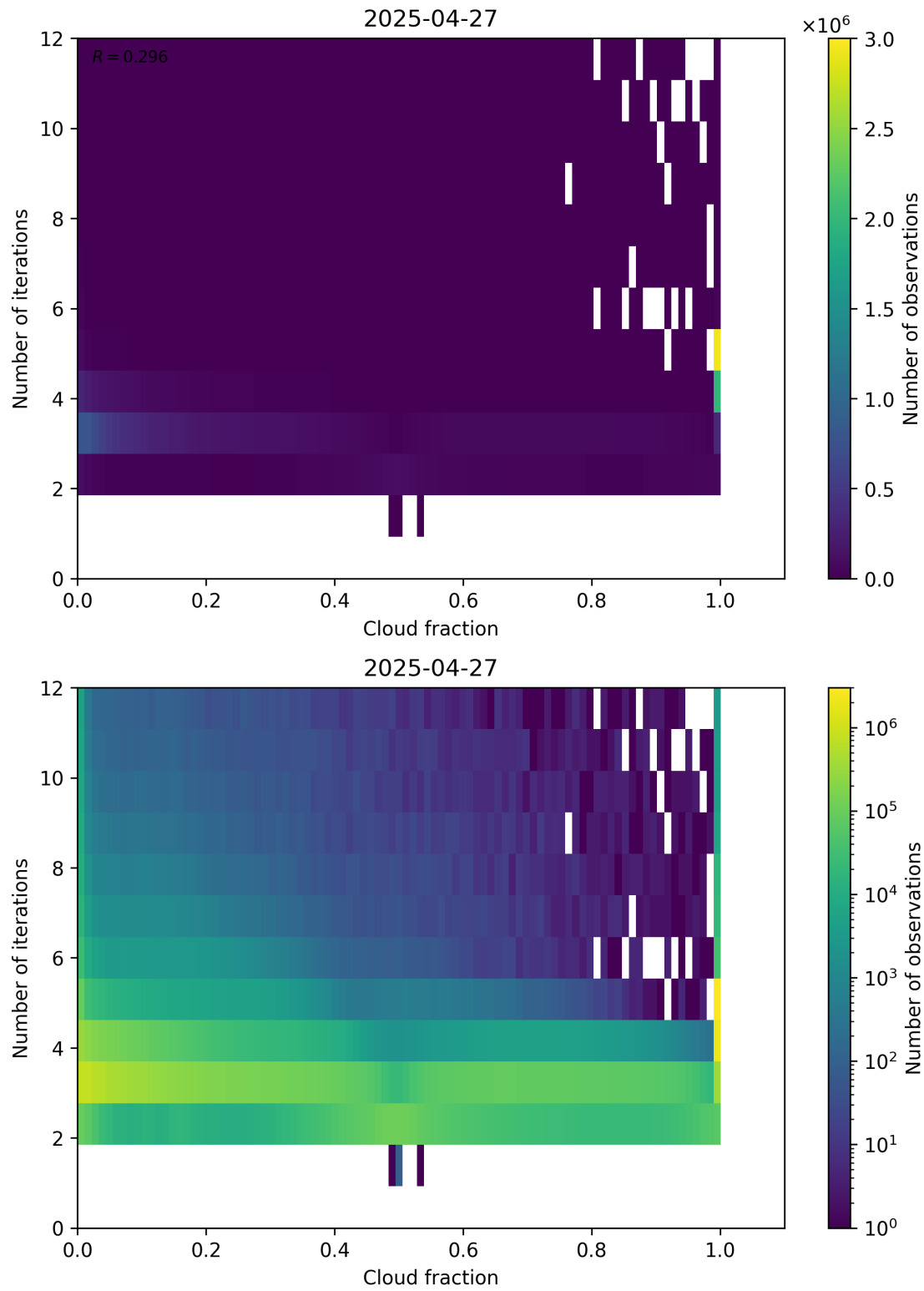
Figure 73: Scatter density plot of “Cloud fraction” against “Number of iterations” for 2025-04-26 to 2025-04-28.
