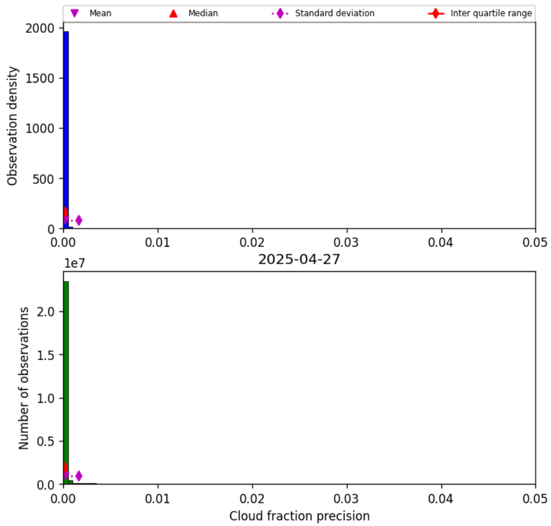
Figure 33: Histogram of “Cloud fraction precision” for 2025-04-26 to 2025-04-28
