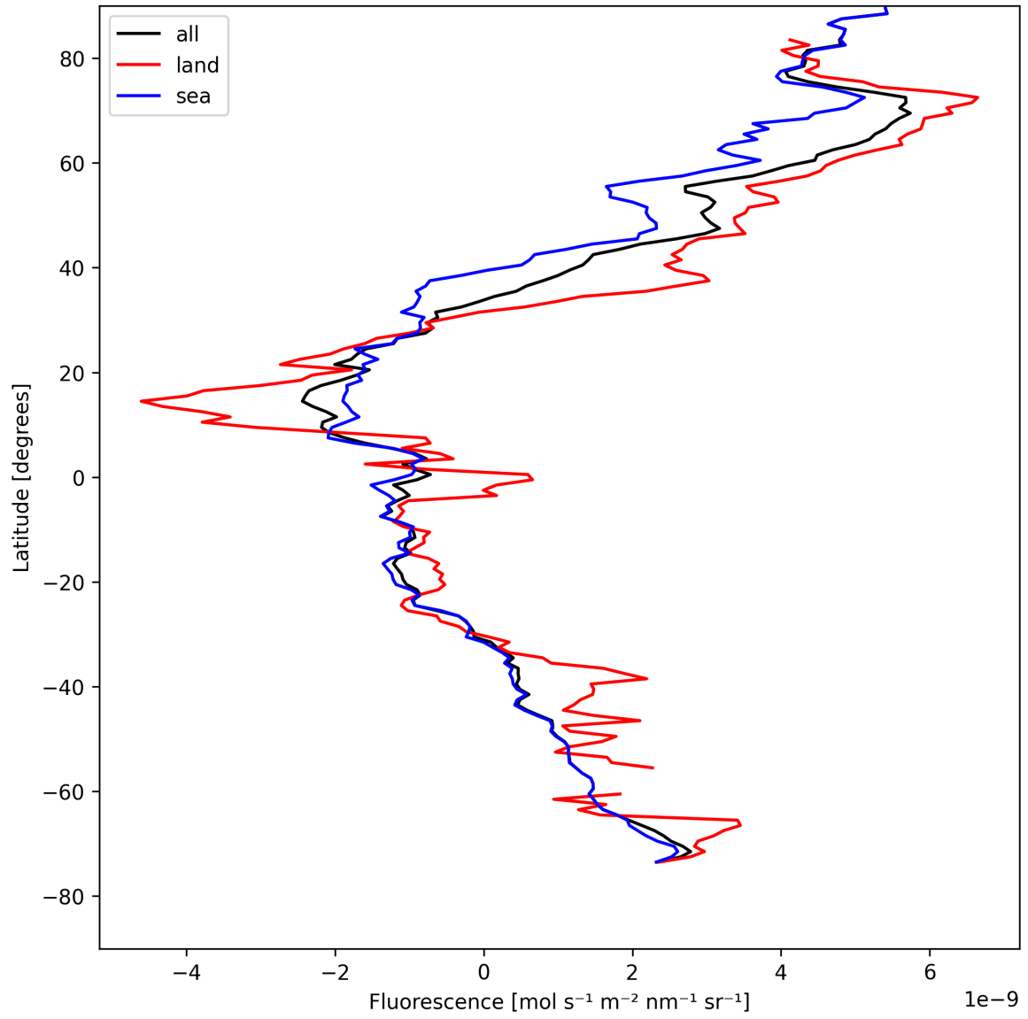
Figure 23: Zonal average of “Fluorescence” for 2025-04-26 to 2025-04-28.
