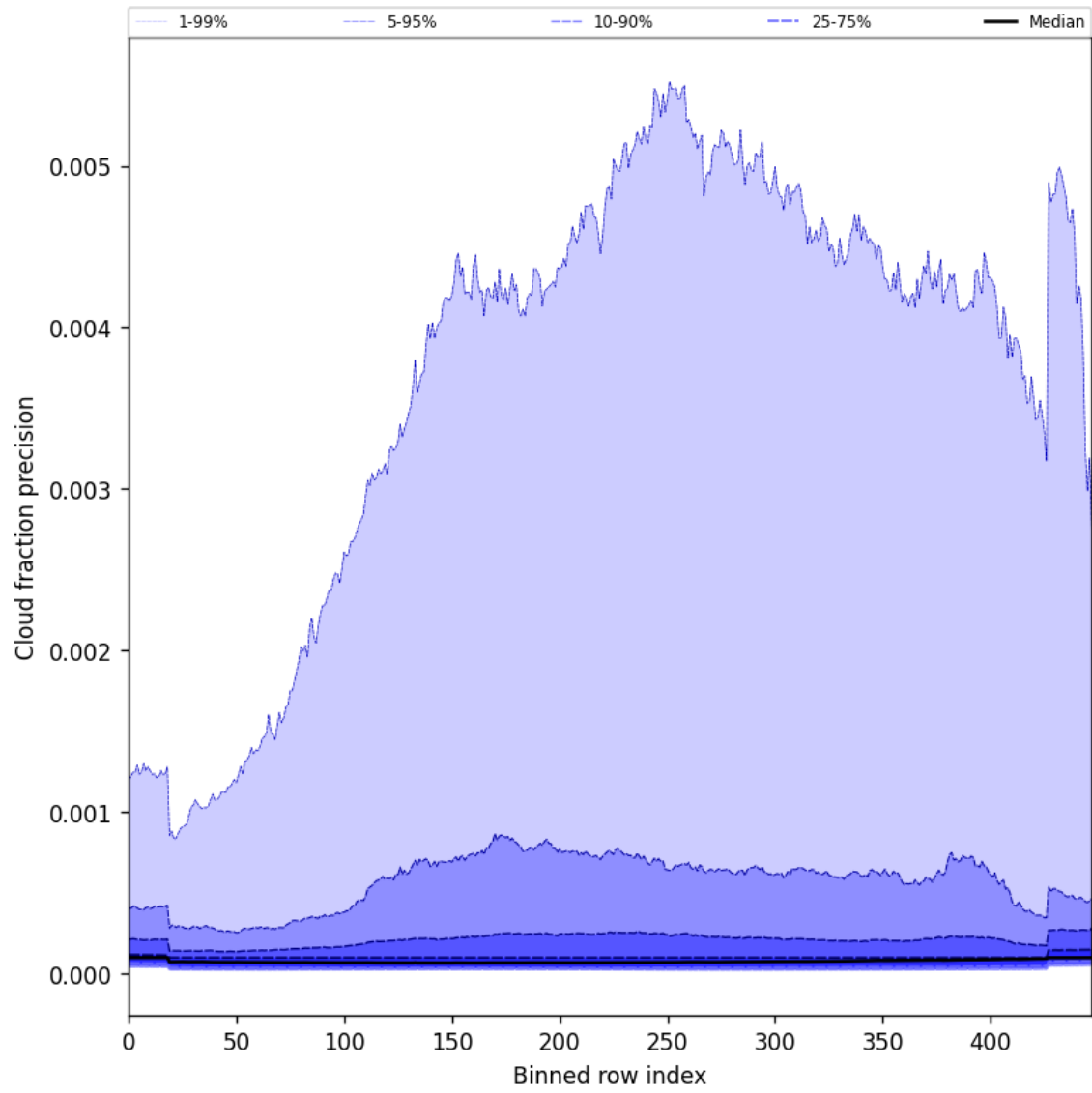
Figure 50: Along track statistics of “Cloud fraction precision” for 2025-04-26 to 2025-04-28
