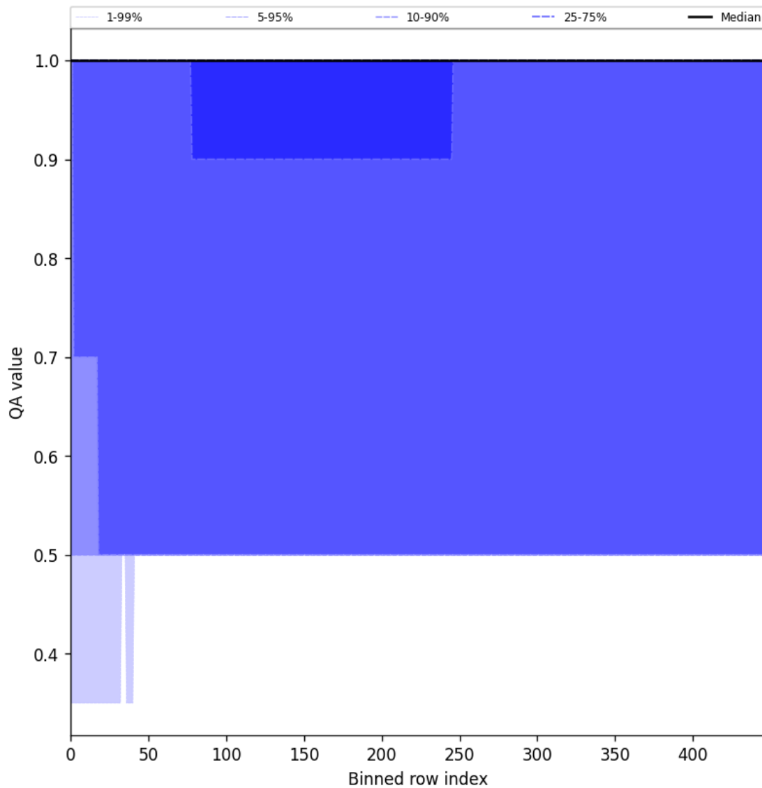
Figure 46: Along track statistics of “QA value” for 2025-04-26 to 2025-04-28
