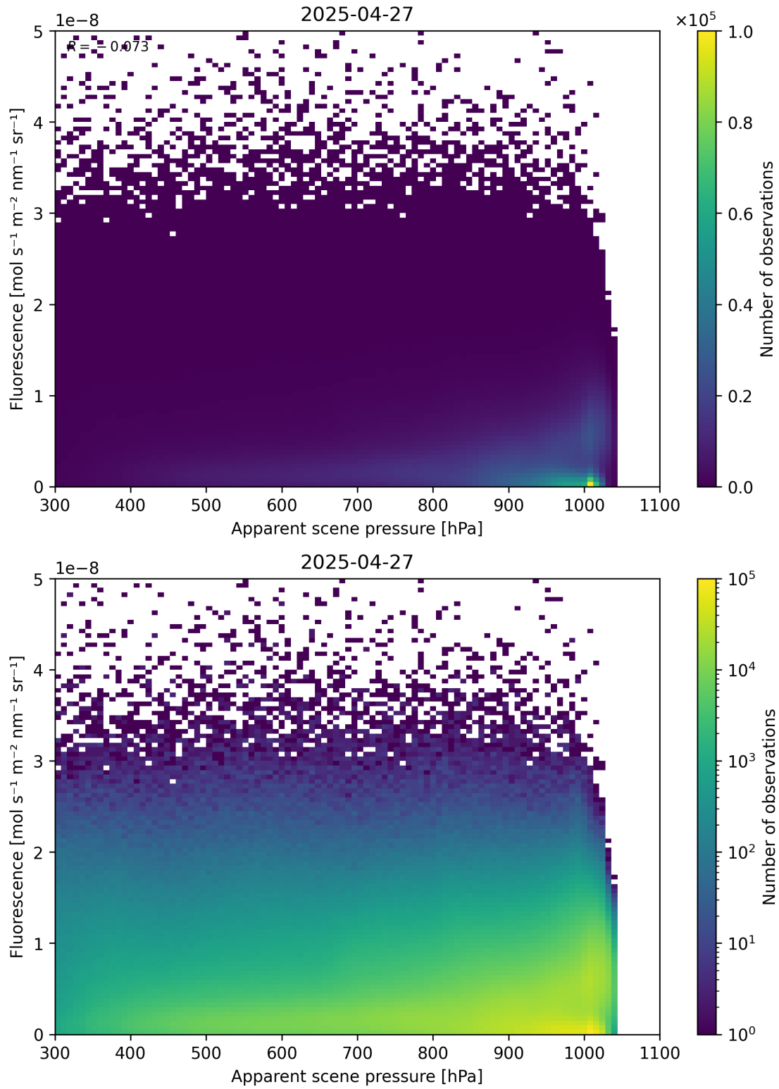
Figure 64: Scatter density plot of “Apparent scene pressure” against “Fluorescence” for 2025-04-26 to 2025-04-28.
