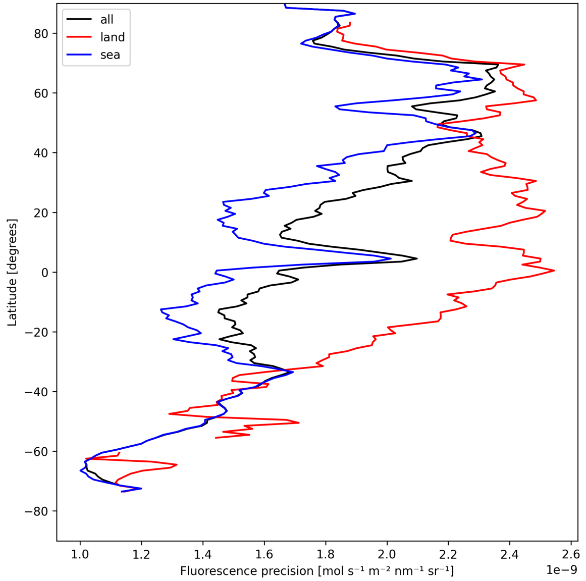
Figure 24: Zonal average of "Fluorescence precision" for 2025-04-26 to 2025-04-28.
