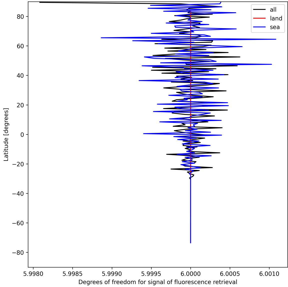
Figure 26: Zonal average of “Degrees of freedom for signal of fluorescence retrieval” for 2025-04-26 to 2025-04-28.
