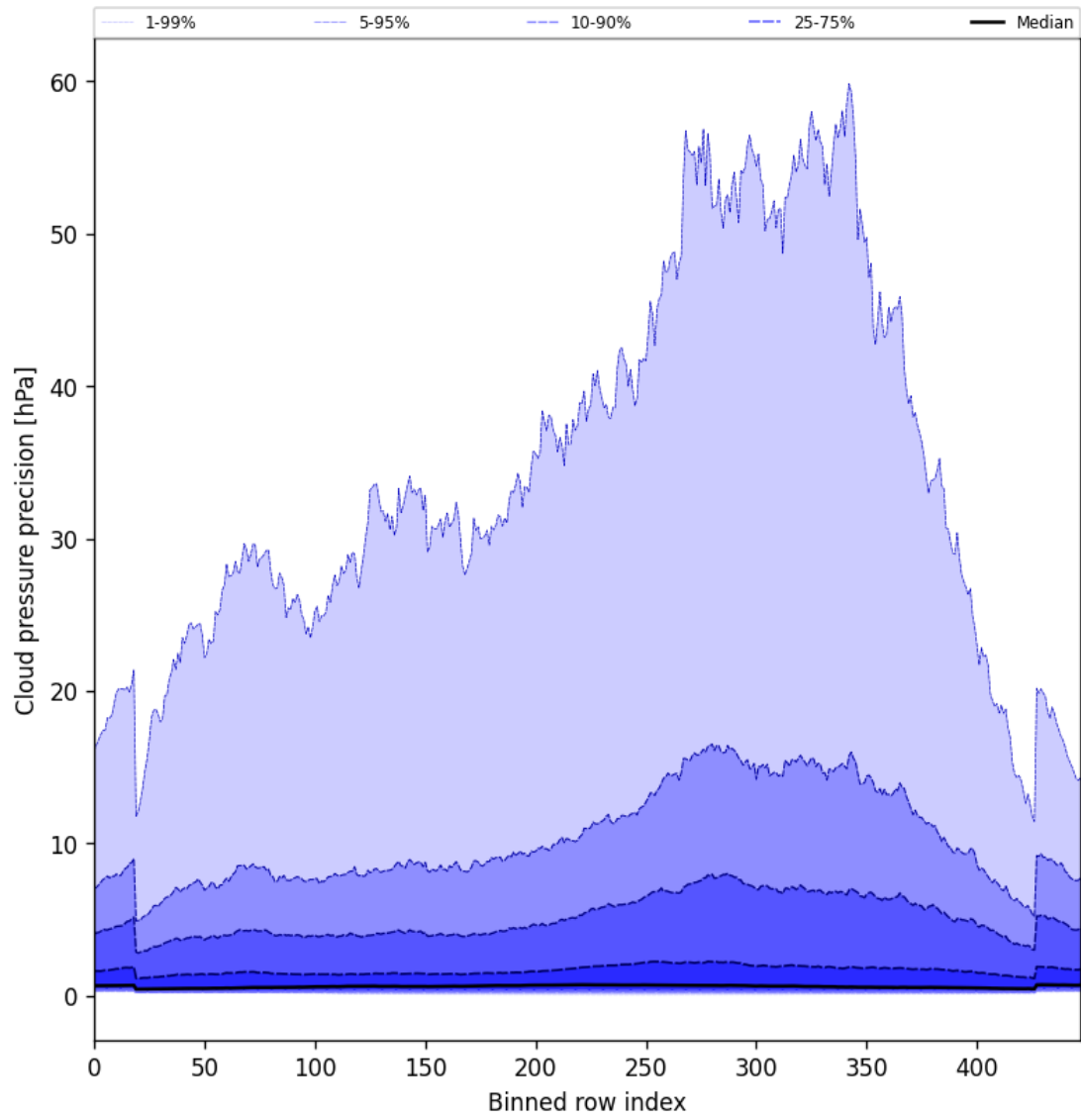
Figure 48: Along track statistics of “Cloud pressure precision” for 2025-04-26 to 2025-04-28
