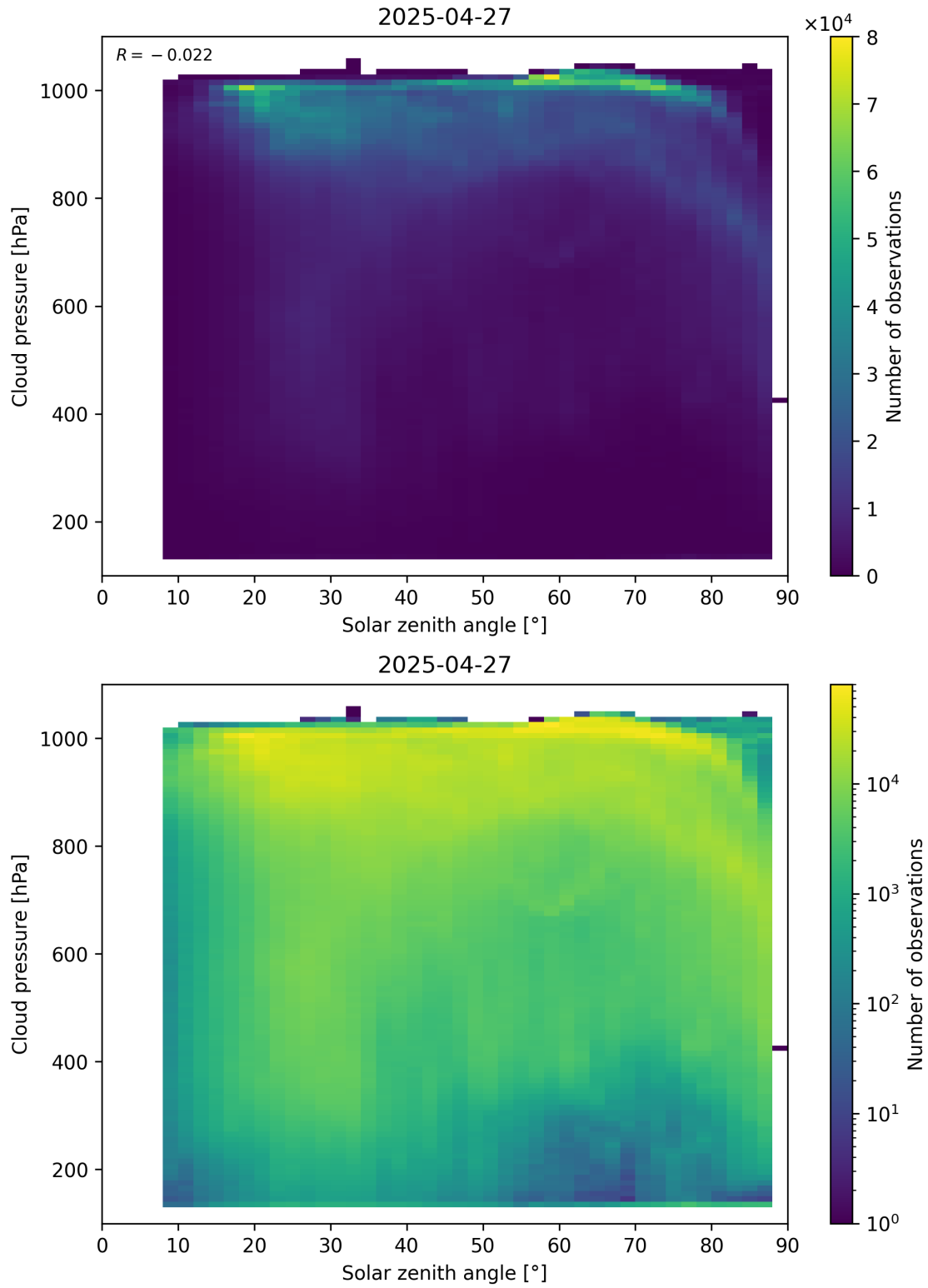
Figure 111: Scatter density plot of “Solar zenith angle” against “Cloud pressure” for 2025-04-26 to 2025-04-28.
