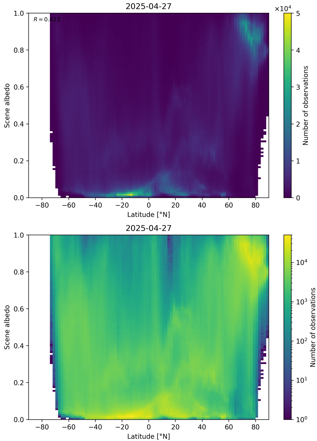
Figure 95: Scatter density plot of “Latitude” against “Scene albedo” for 2025-04-26 to 2025-04-28.
