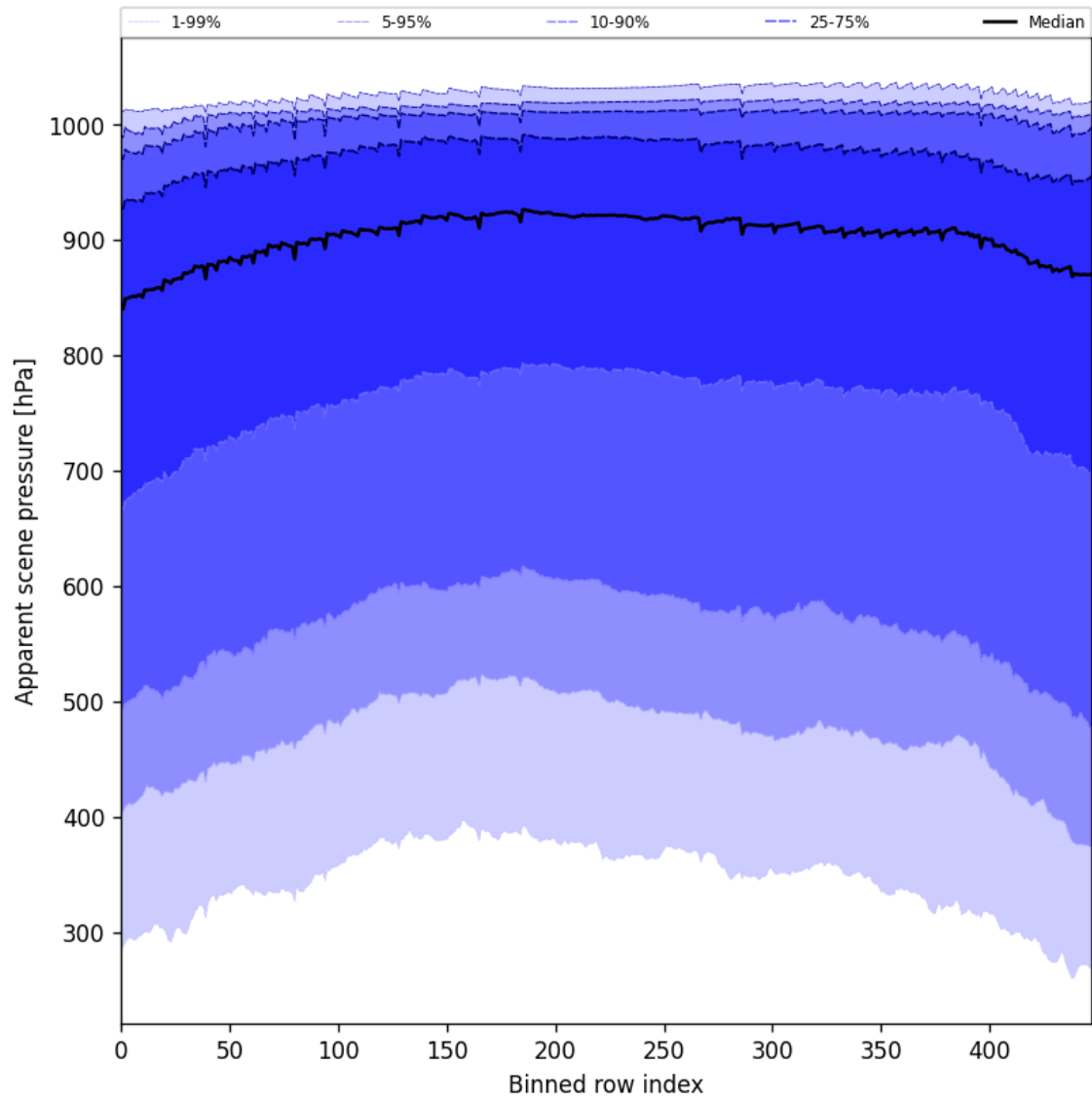
Figure 53: Along track statistics of “Apparent scene pressure” for 2025-04-26 to 2025-04-28
