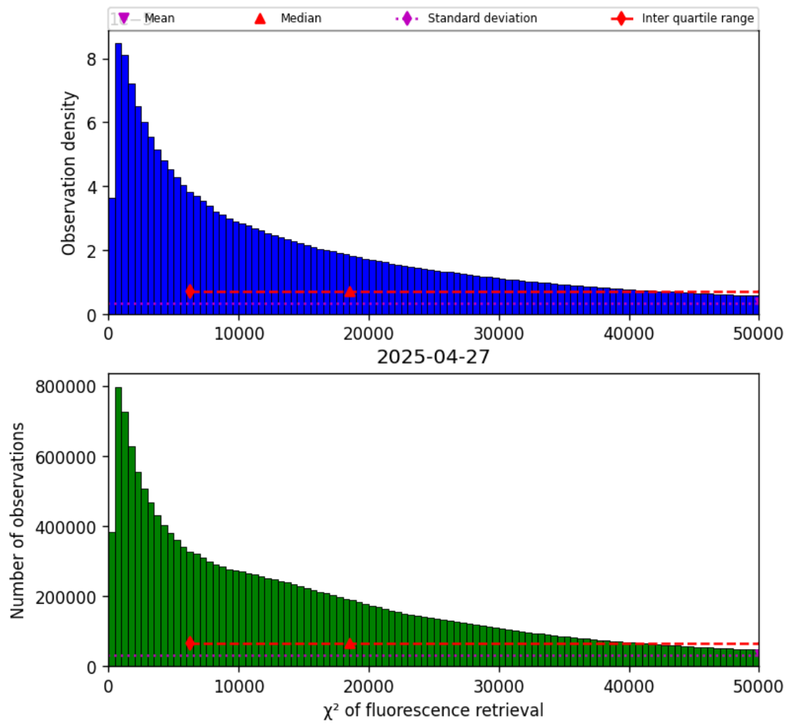
Figure 42: Histogram of “ \chi^2 of fluorescence retrieval” for 2025-04-26 to 2025-04-28
