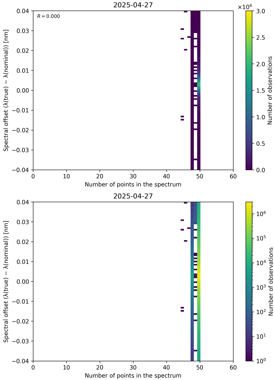
Figure 101: Scatter density plot of “Number of points in the spectrum” against “Spectral offset ( \lambda_{\text{true}} - \lambda_{\text{nominal}} )” for 2025-04-26 to 2025-04-28.
