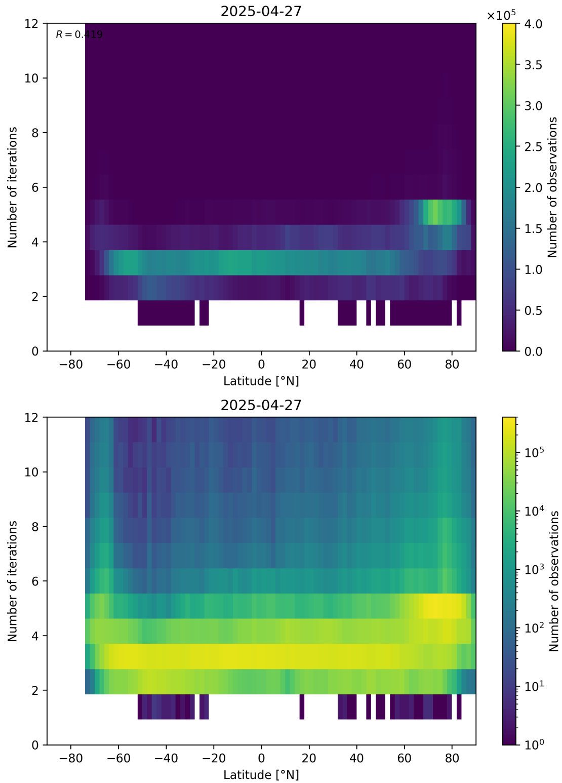
Figure 93: Scatter density plot of “Latitude” against “Number of iterations” for 2025-04-26 to 2025-04-28.
