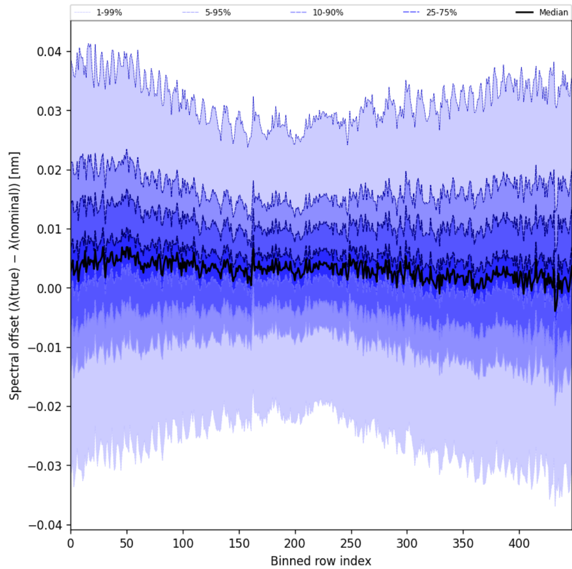
Figure 62: Along track statistics of “Spectral offset ( \lambda_{\text{true}} - \lambda_{\text{nominal}} )” for 2025-04-26 to 2025-04-28
