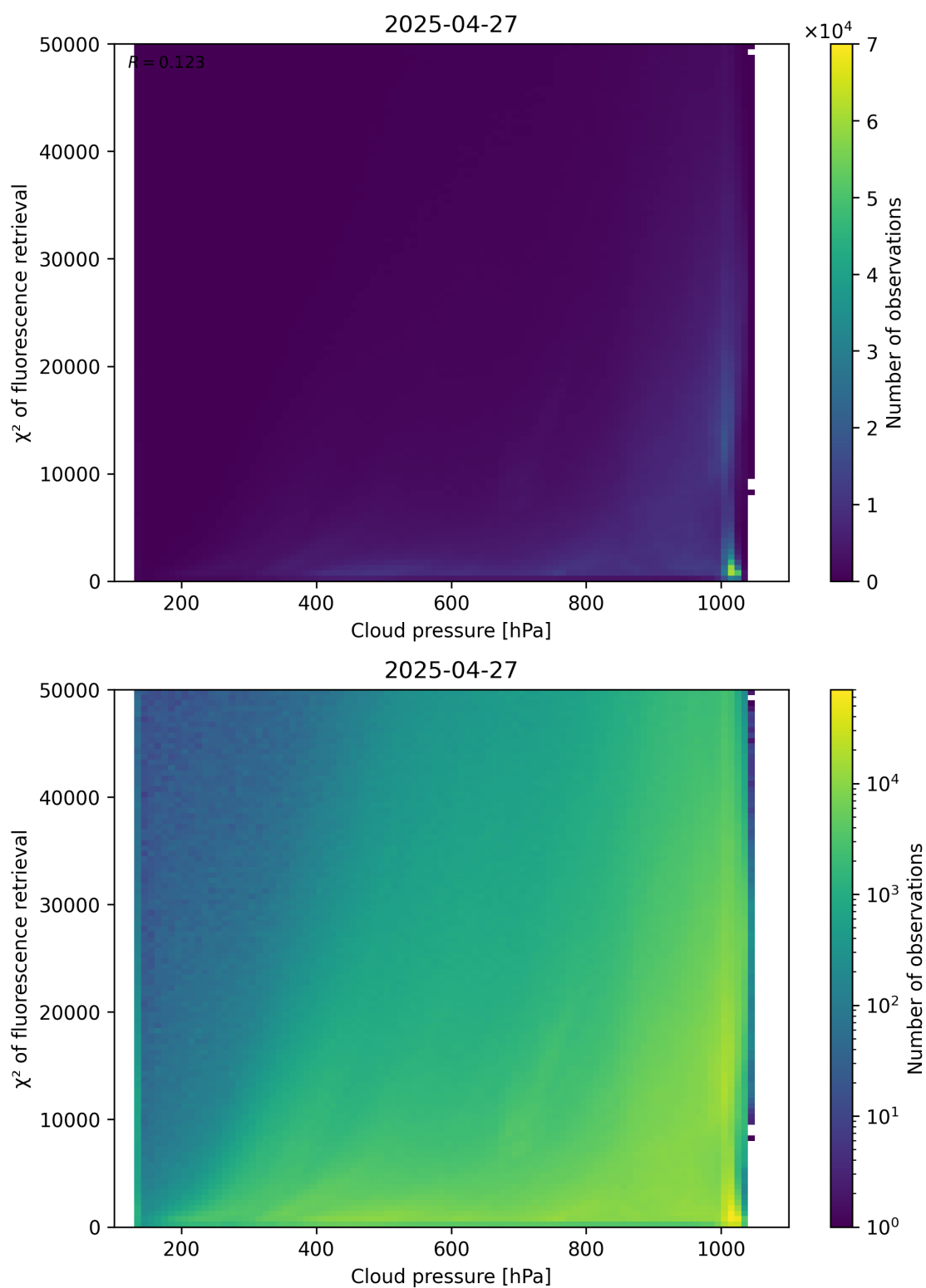
Figure 78: Scatter density plot of “Cloud pressure” against “ \chi^2 of fluorescence retrieval” for 2025-04-26 to 2025-04-28.
