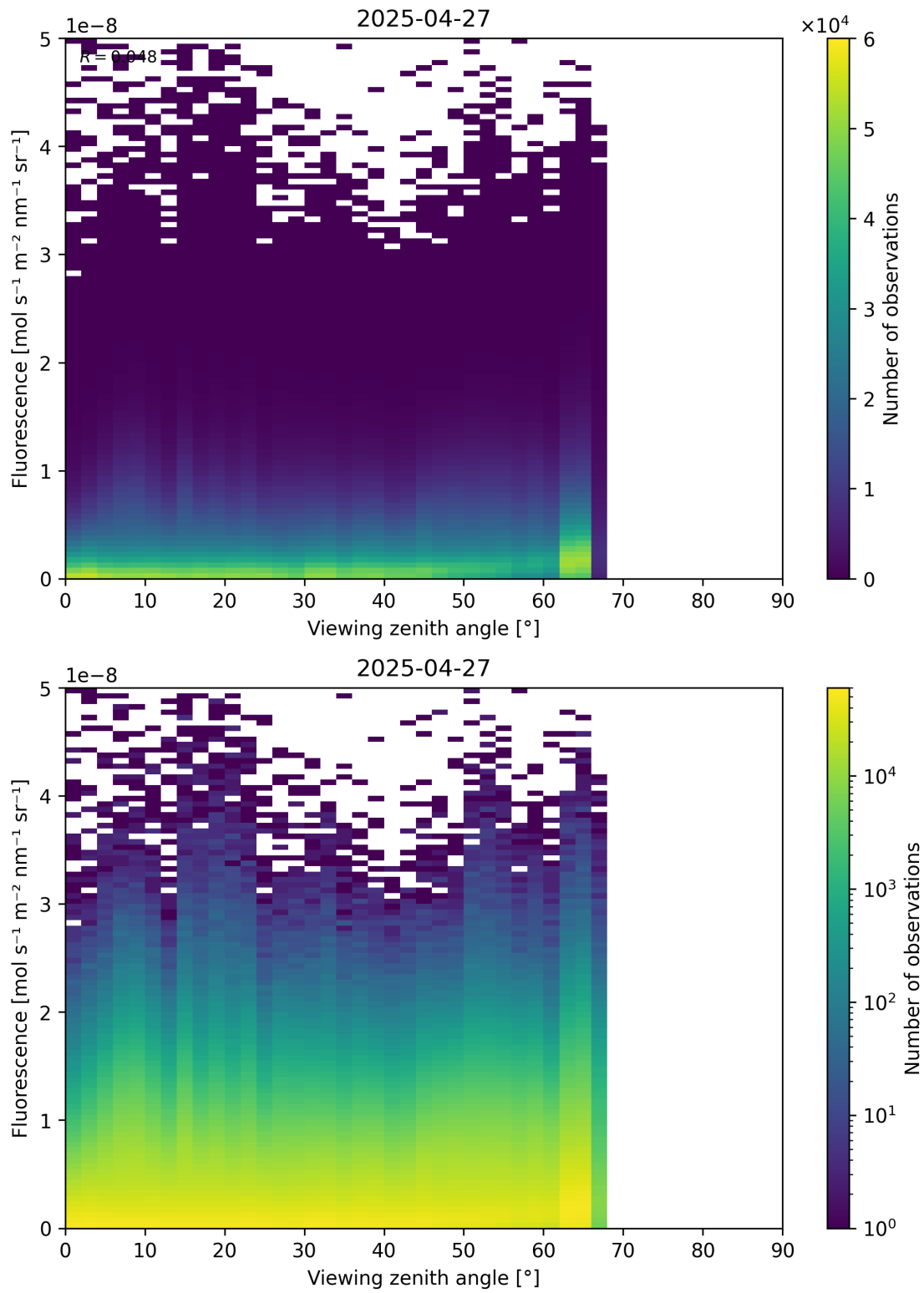
Figure 122: Scatter density plot of “Viewing zenith angle” against “Fluorescence” for 2025-04-26 to 2025-04-28.
