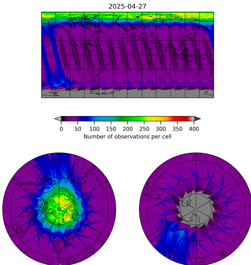
Figure 11: Map of the number of observations for 2025-04-26 to 2025-04-28
