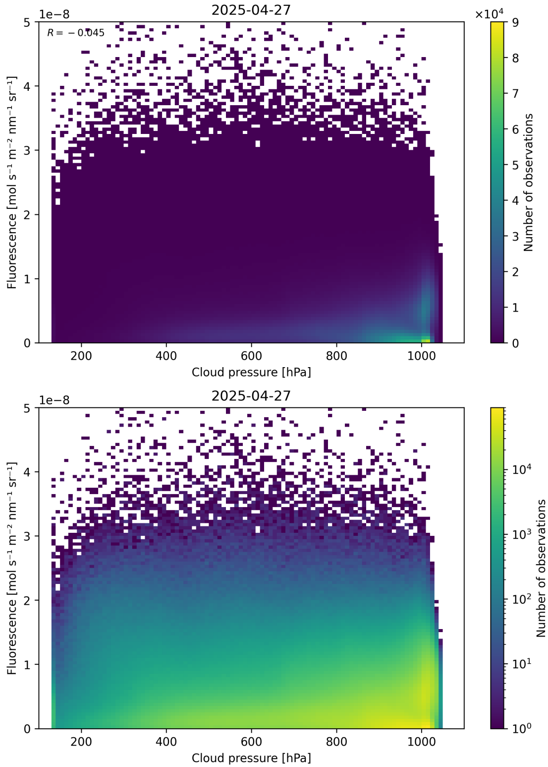
Figure 80: Scatter density plot of “Cloud pressure” against “Fluorescence” for 2025-04-26 to 2025-04-28.
