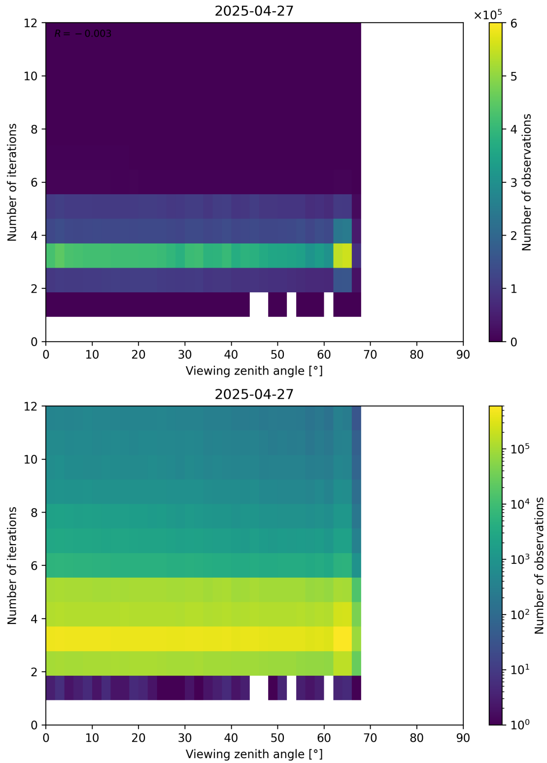
Figure 124: Scatter density plot of “Viewing zenith angle” against “Number of iterations” for 2025-04-26 to 2025-04-28.
