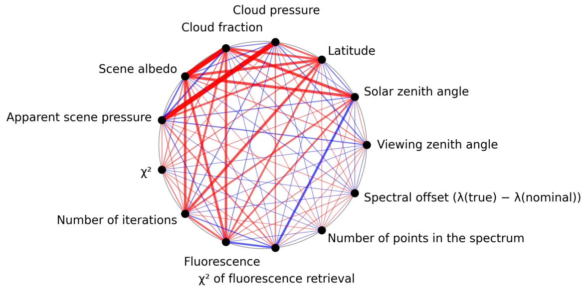
Figure 1: Map of correlation graph for 2025-04-26 to 2025-04-28.
