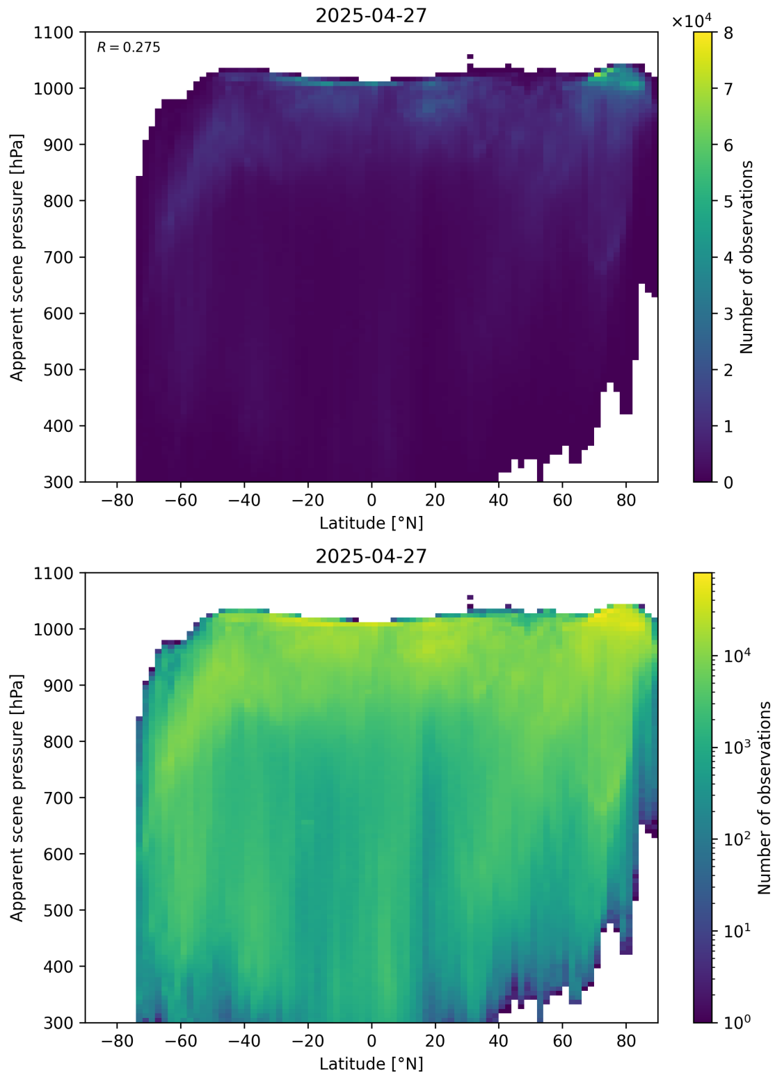
Figure 88: Scatter density plot of “Latitude” against “Apparent scene pressure” for 2025-04-26 to 2025-04-28.
