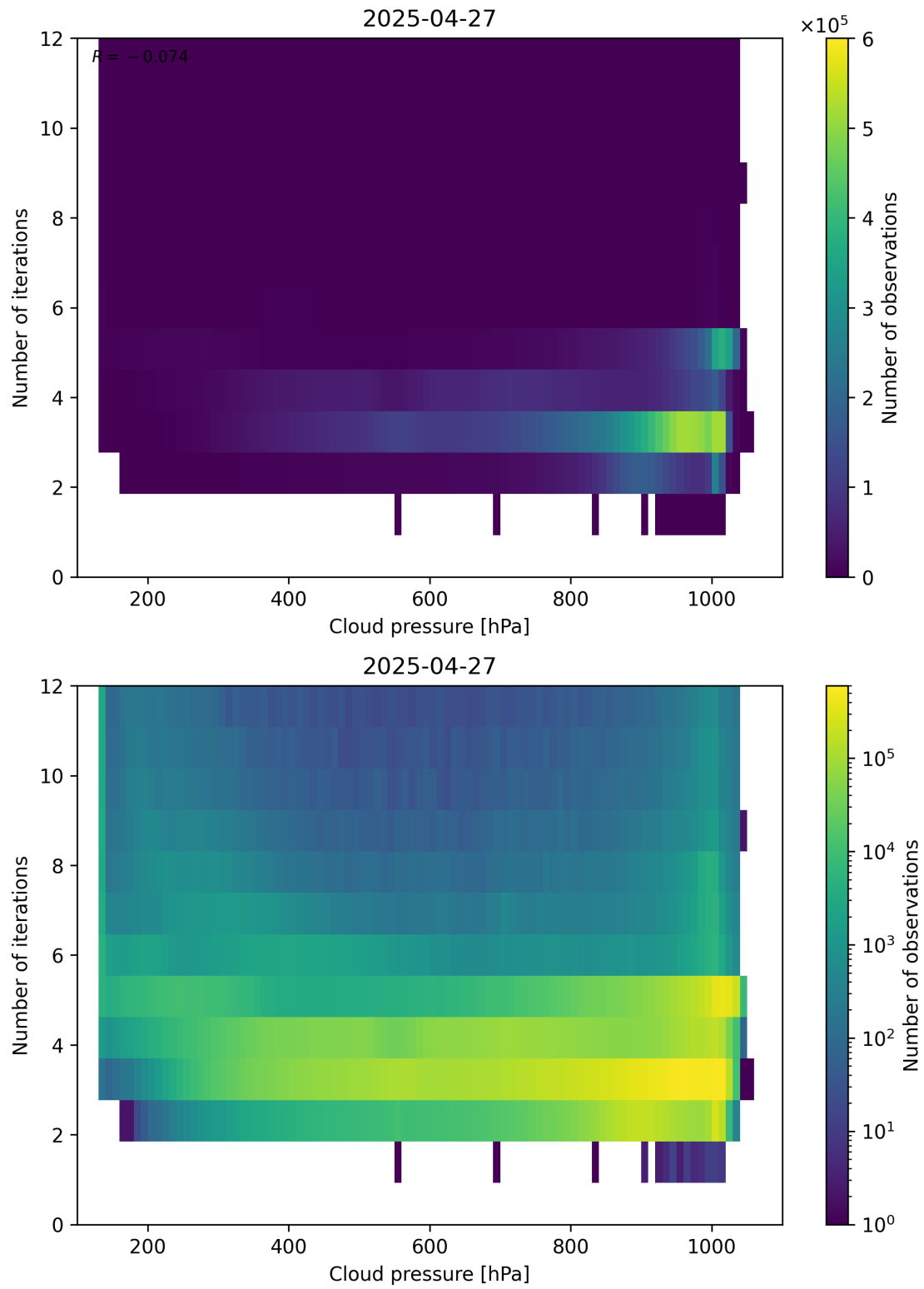
Figure 81: Scatter density plot of “Cloud pressure” against “Number of iterations” for 2025-04-26 to 2025-04-28.
