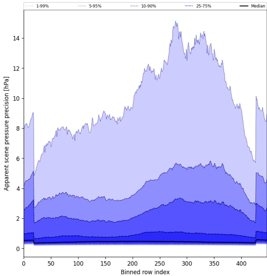
Figure 54: Along track statistics of “Apparent scene pressure precision” for 2025-04-26 to 2025-04-28
