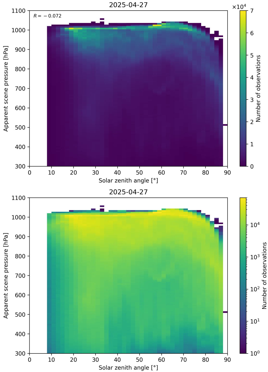
Figure 108: Scatter density plot of “Solar zenith angle” against “Apparent scene pressure” for 2025-04-26 to 2025-04-28.
