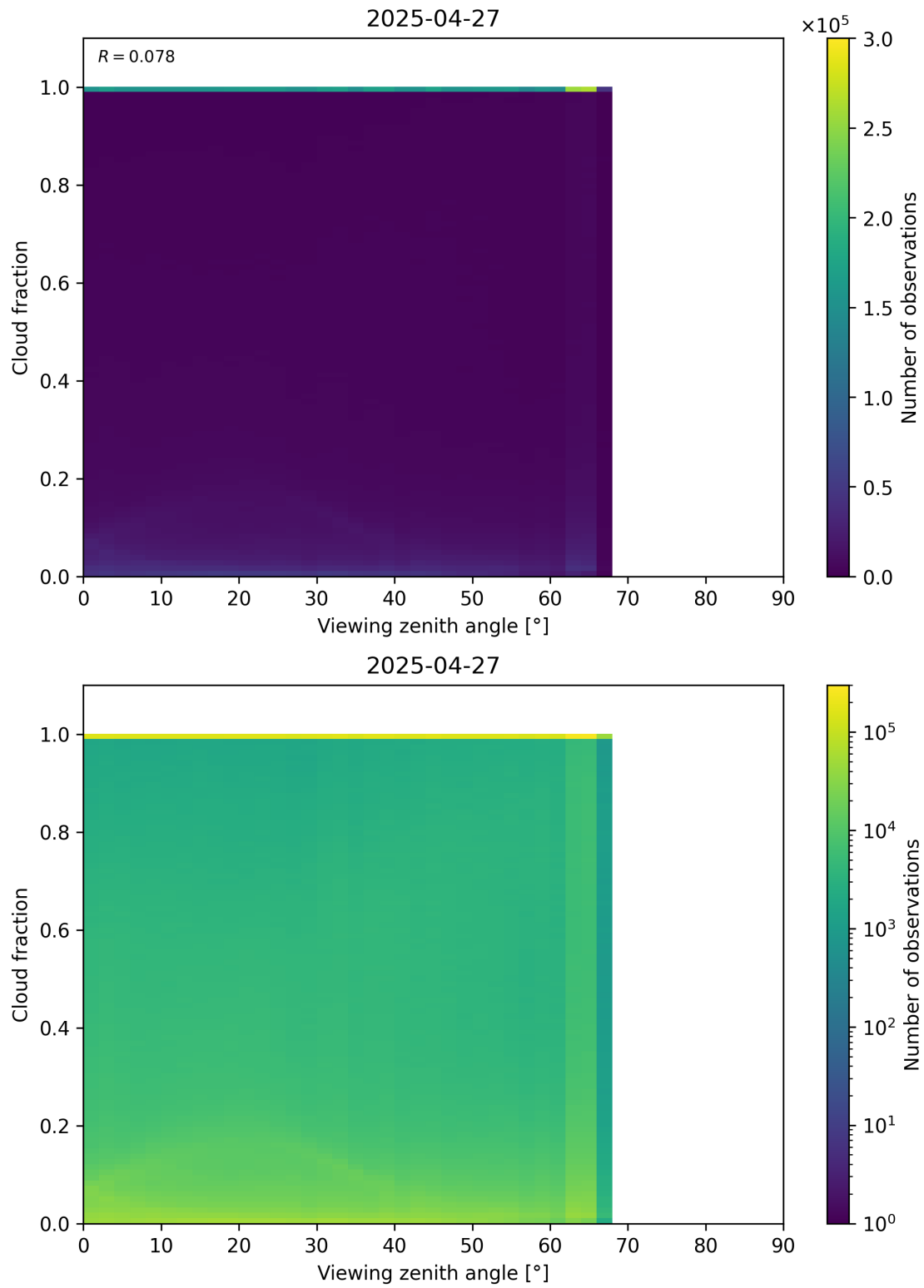
Figure 120: Scatter density plot of “Viewing zenith angle” against “Cloud fraction” for 2025-04-26 to 2025-04-28.
