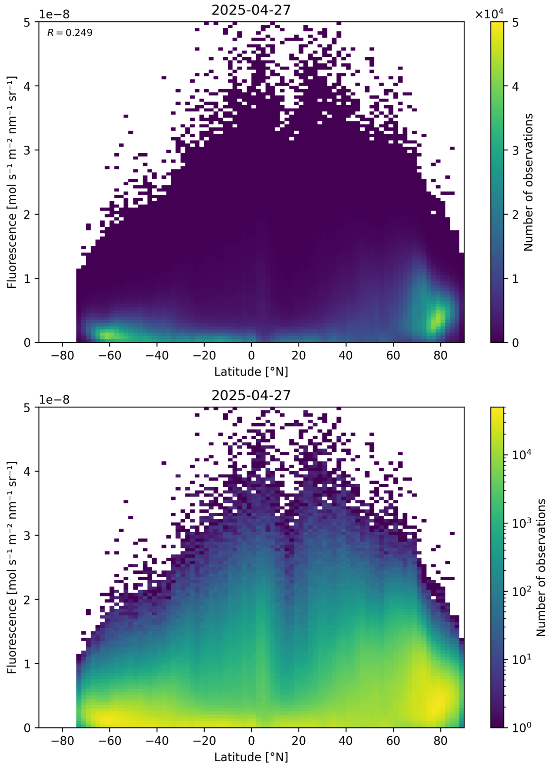
Figure 92: Scatter density plot of “Latitude” against “Fluorescence” for 2025-04-26 to 2025-04-28.
