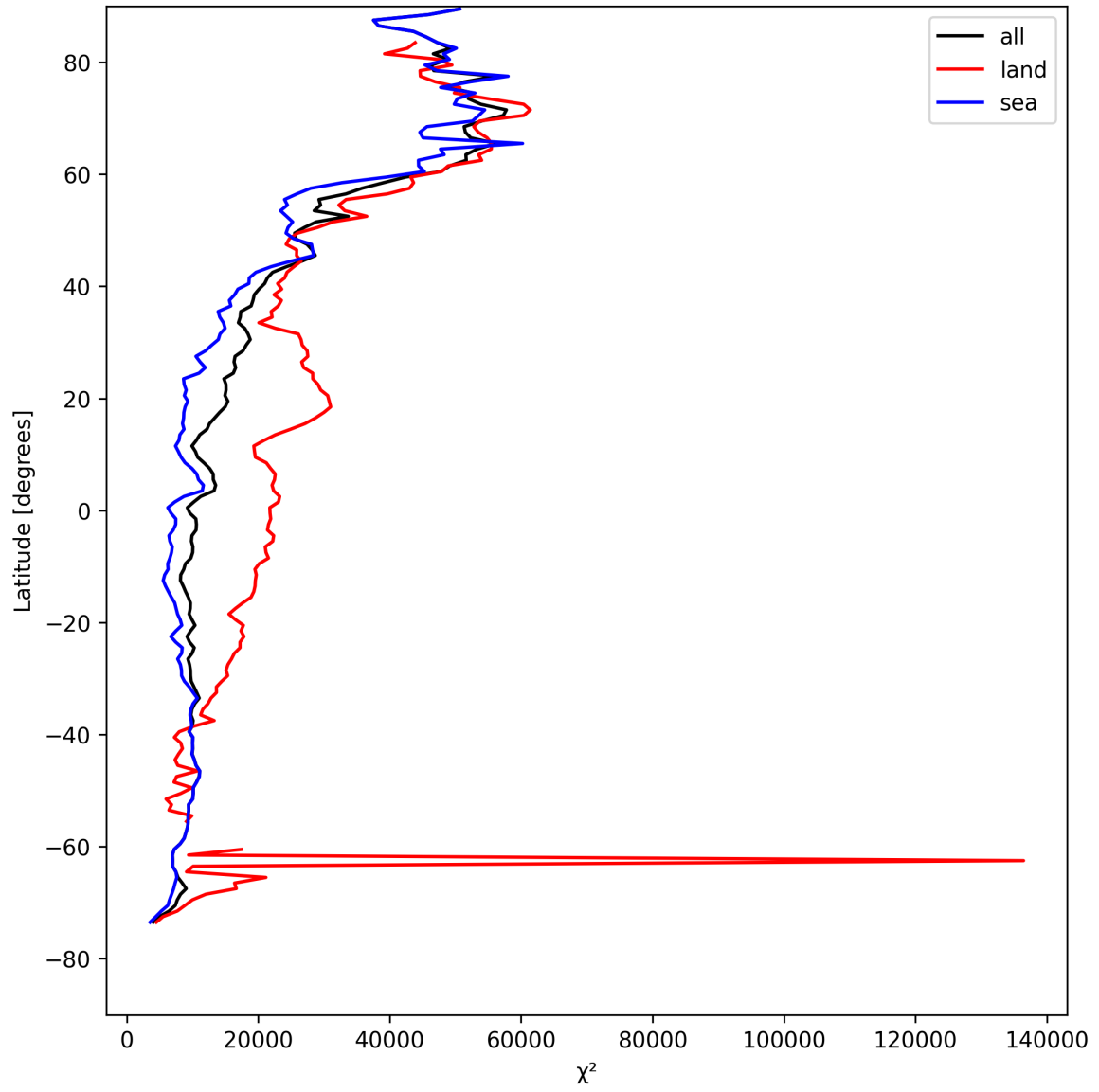
Figure 21: Zonal average of “ \chi^2 ” for 2025-04-26 to 2025-04-28.
