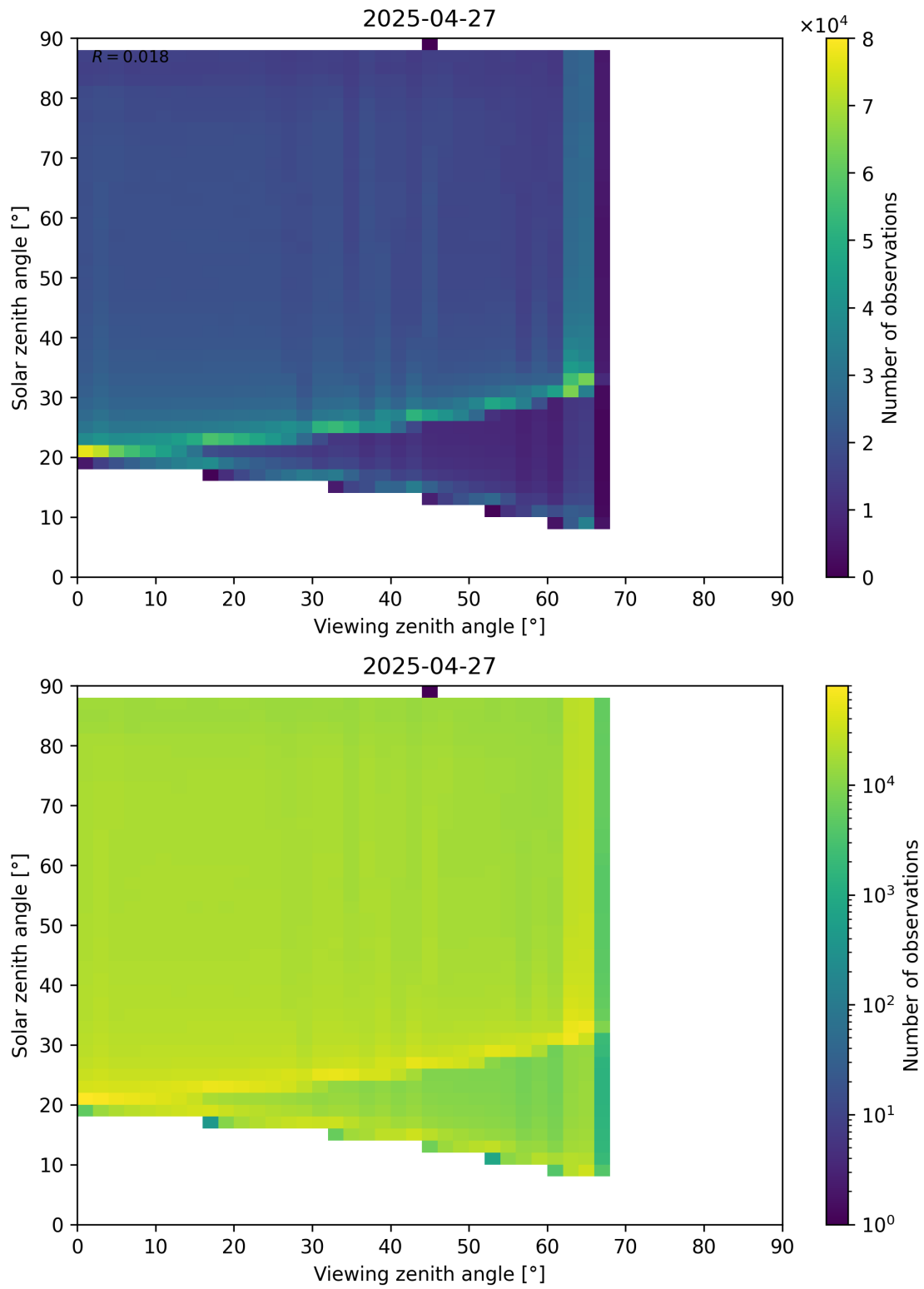
Figure 127: Scatter density plot of “Viewing zenith angle” against “Solar zenith angle” for 2025-04-26 to 2025-04-28.
