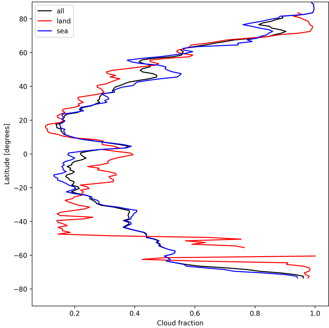
Figure 15: Zonal average of “Cloud fraction” for 2025-04-26 to 2025-04-28.
