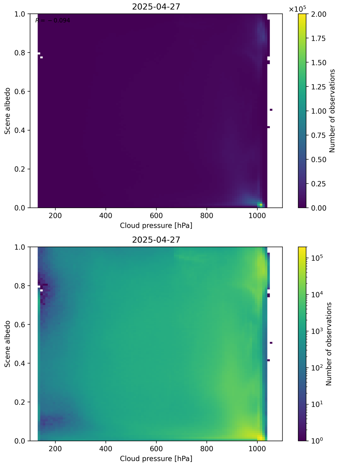
Figure 83: Scatter density plot of “Cloud pressure” against “Scene albedo” for 2025-04-26 to 2025-04-28.
