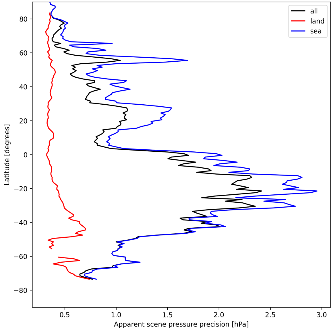
Figure 20: Zonal average of “Apparent scene pressure precision” for 2025-04-26 to 2025-04-28.
