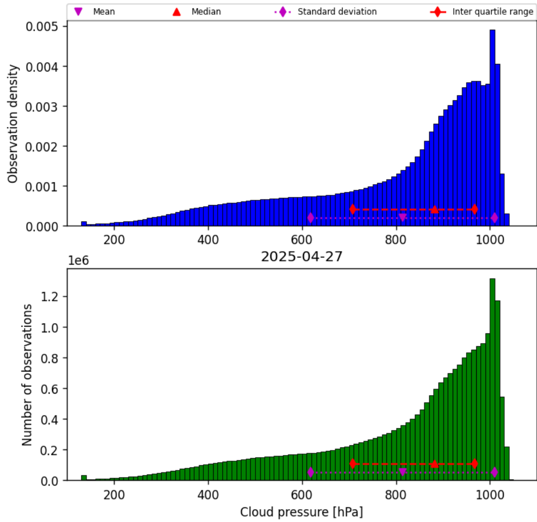
Figure 30: Histogram of “Cloud pressure” for 2025-04-26 to 2025-04-28
