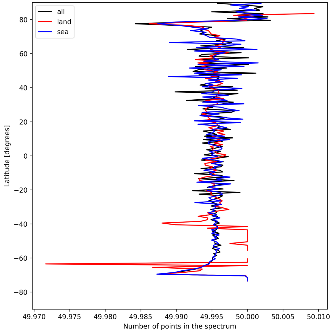
Figure 27: Zonal average of “Number of points in the spectrum” for 2025-04-26 to 2025-04-28.
