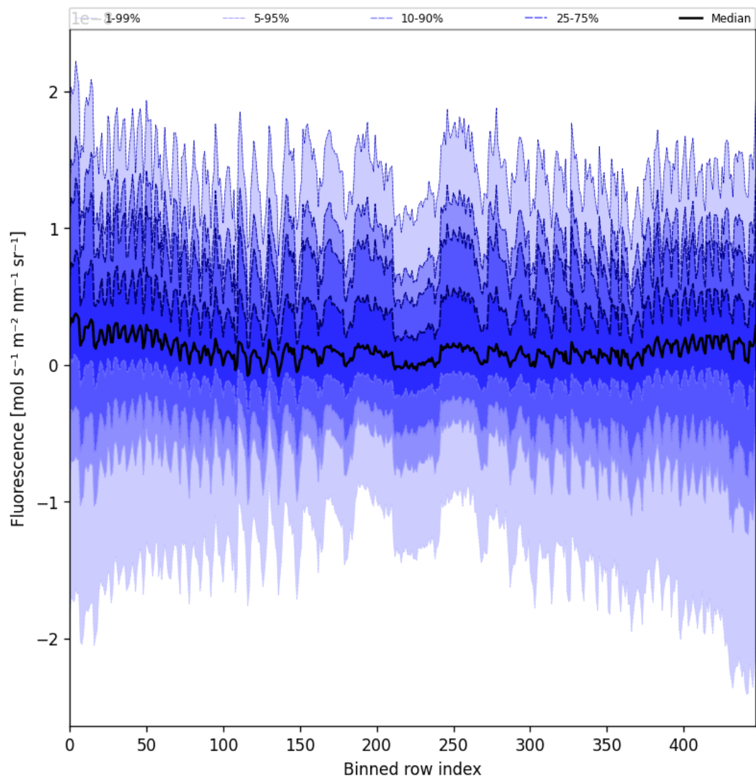
Figure 57: Along track statistics of “Fluorescence” for 2025-04-26 to 2025-04-28
