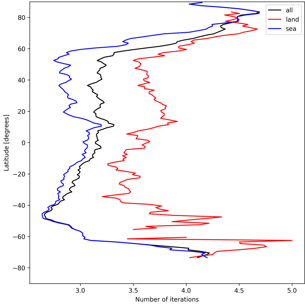
Figure 22: Zonal average of “Number of iterations” for 2025-04-26 to 2025-04-28.
