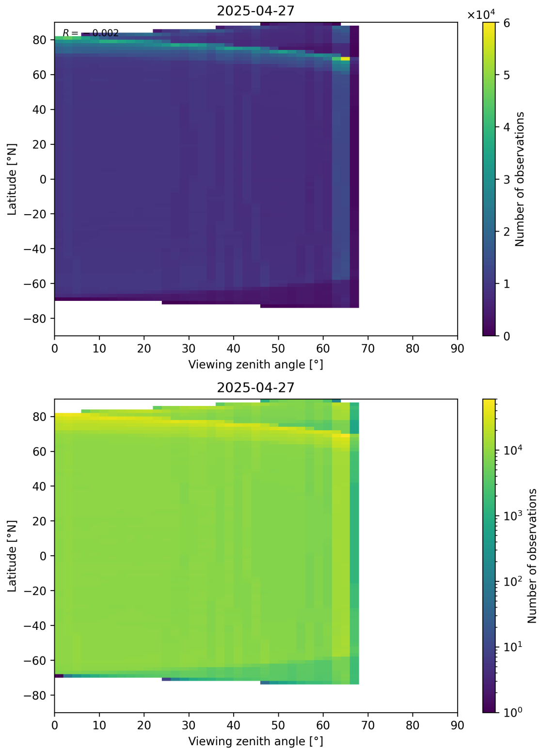
Figure 123: Scatter density plot of “Viewing zenith angle” against “Latitude” for 2025-04-26 to 2025-04-28.
