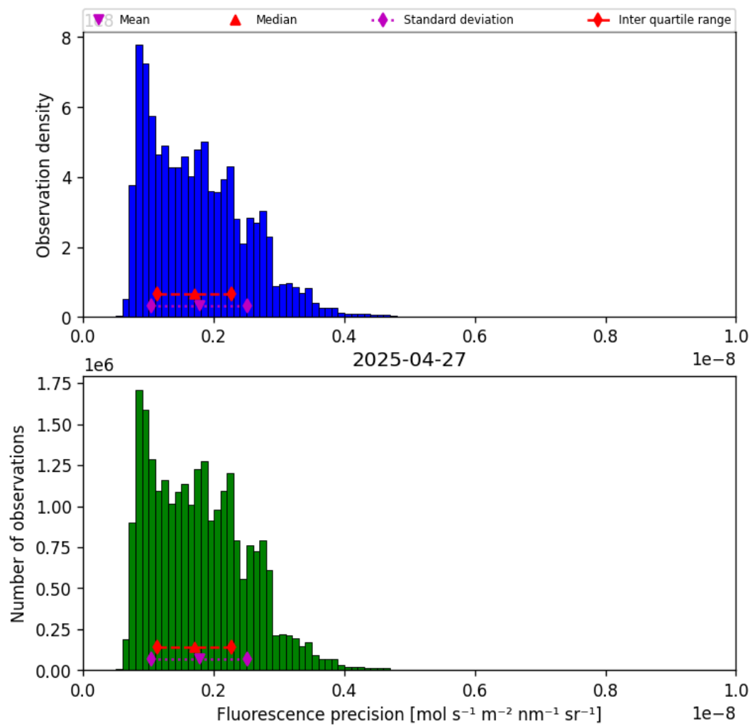
Figure 41: Histogram of “Fluorescence precision” for 2025-04-26 to 2025-04-28
