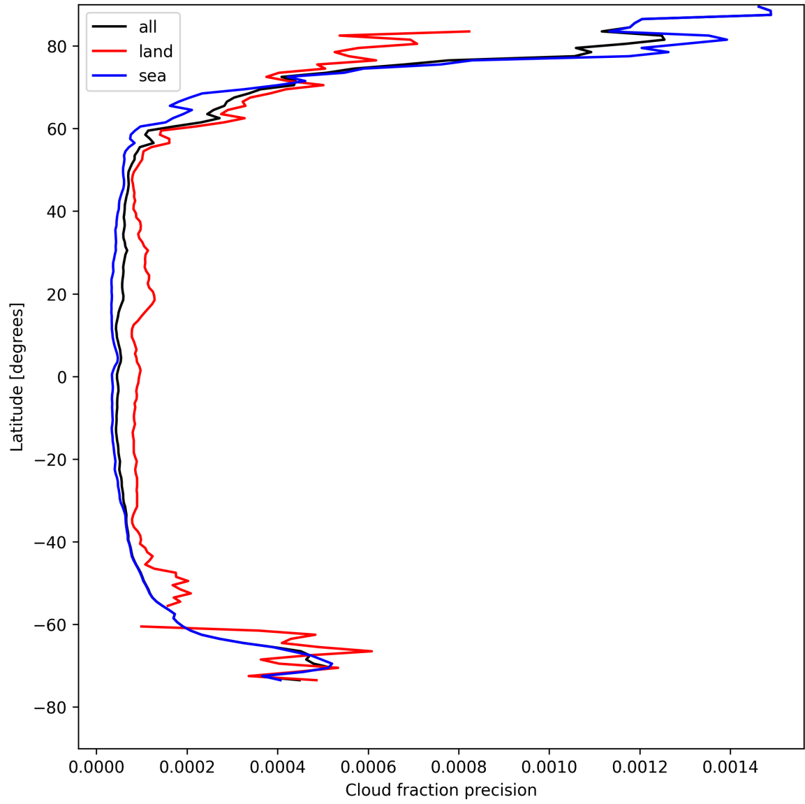
Figure 16: Zonal average of “Cloud fraction precision” for 2025-04-26 to 2025-04-28.
