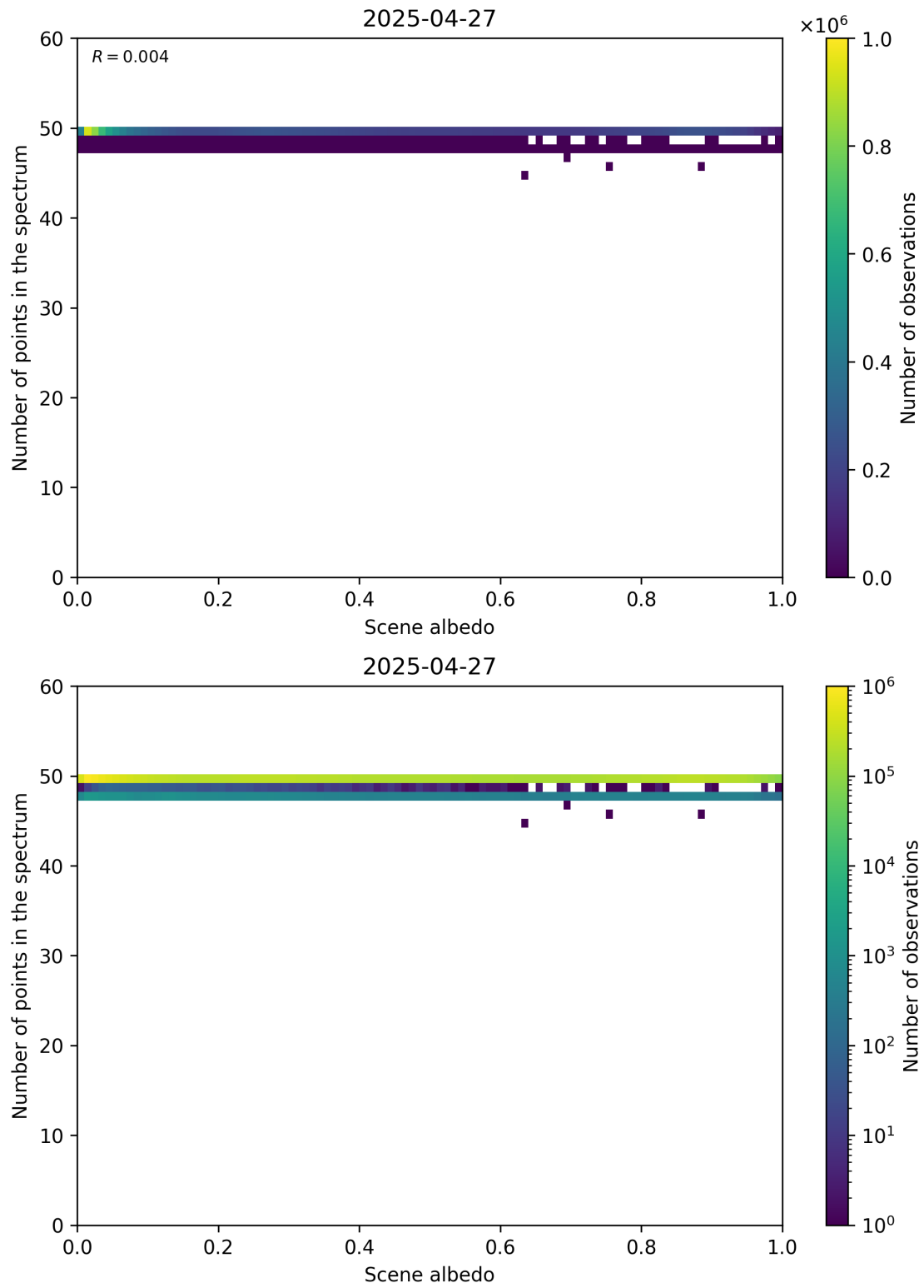
Figure 106: Scatter density plot of “Scene albedo” against “Number of points in the spectrum” for 2025-04-26 to 2025-04-28.
