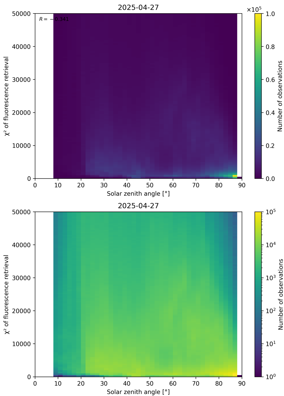
Figure 109: Scatter density plot of “Solar zenith angle” against “ \chi^2 of fluorescence retrieval” for 2025-04-26 to 2025-04-28.
