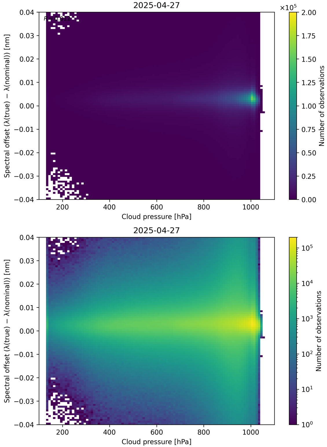
Figure 84: Scatter density plot of “Cloud pressure” against “Spectral offset ( \lambda_{\text{true}} - \lambda_{\text{nominal}} )” for 2025-04-26 to 2025-04-28.
