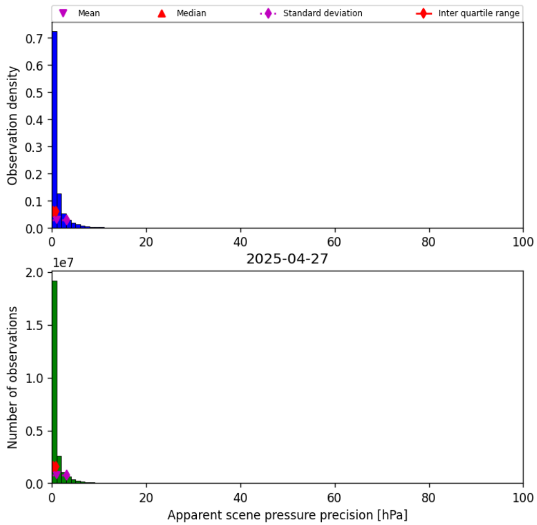
Figure 37: Histogram of “Apparent scene pressure precision” for 2025-04-26 to 2025-04-28
