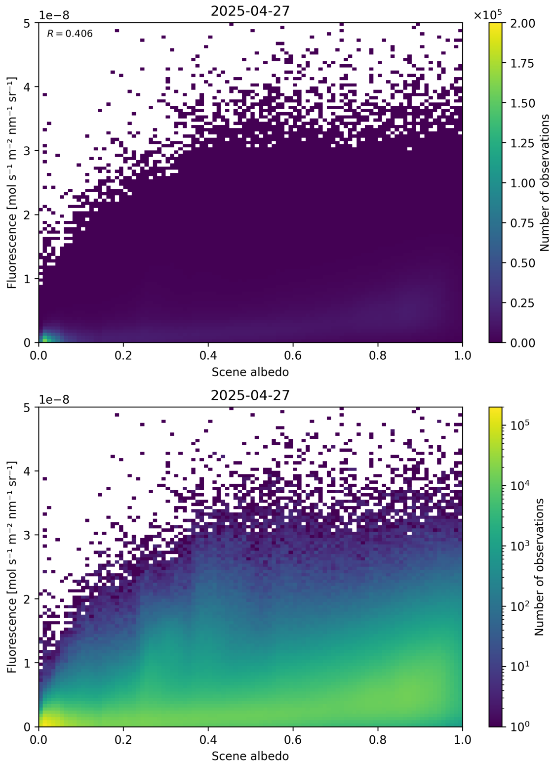
Figure 104: Scatter density plot of “Scene albedo” against “Fluorescence” for 2025-04-26 to 2025-04-28.
