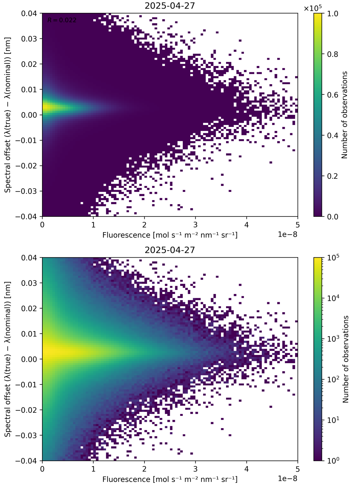
Figure 87: Scatter density plot of “Fluorescence” against “Spectral offset ( \lambda_{\text{true}} - \lambda_{\text{nominal}} )” for 2025-04-26 to 2025-04-28.
