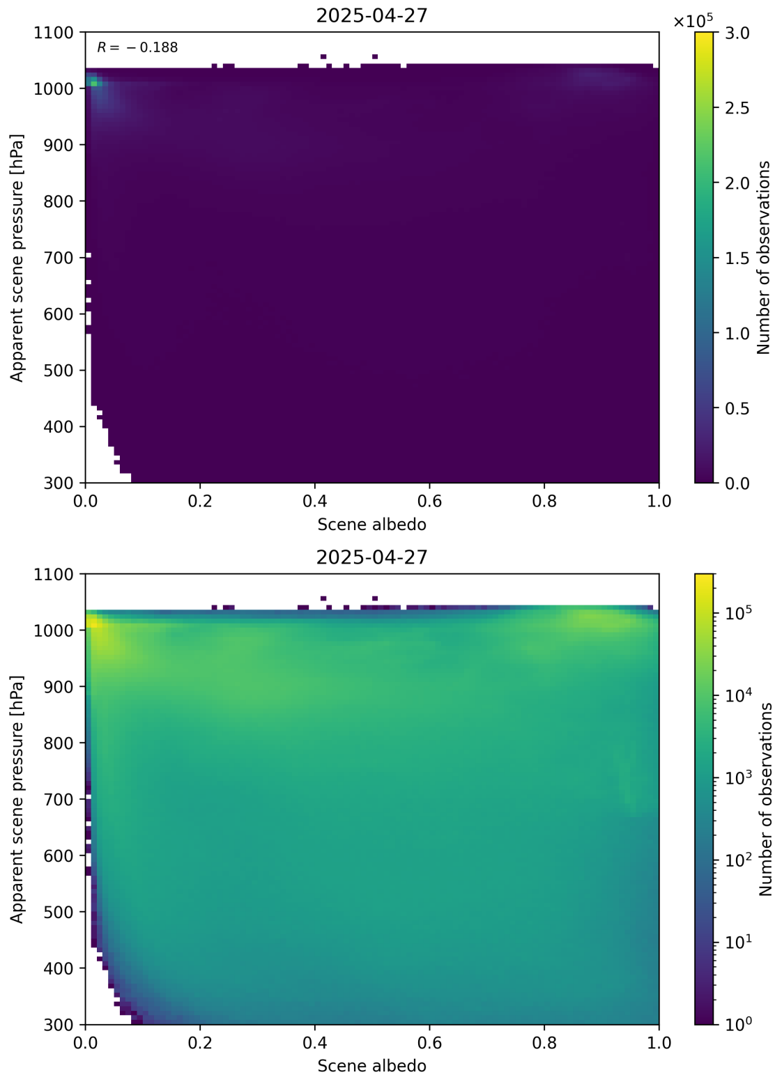
Figure 102: Scatter density plot of “Scene albedo” against “Apparent scene pressure” for 2025-04-26 to 2025-04-28.
