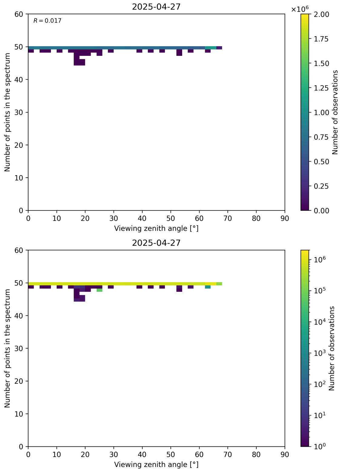
Figure 125: Scatter density plot of “Viewing zenith angle” against “Number of points in the spectrum” for 2025-04-26 to 2025-04-28.
