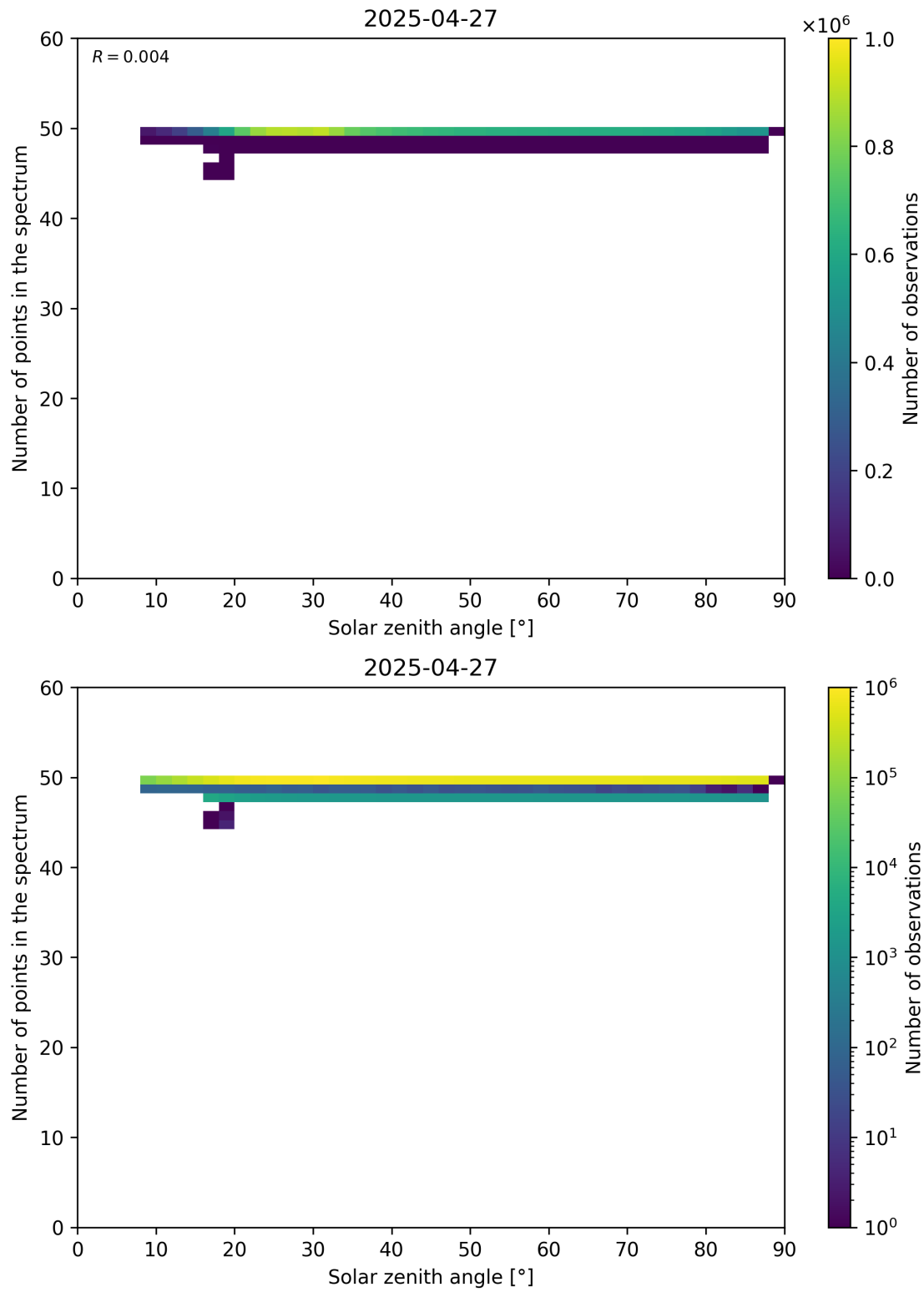
Figure 115: Scatter density plot of “Solar zenith angle” against “Number of points in the spectrum” for 2025-04-26 to 2025-04-28.
