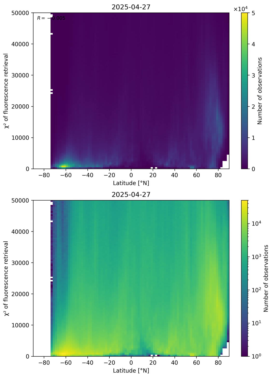
Figure 89: Scatter density plot of “Latitude” against “ \chi^2 of fluorescence retrieval” for 2025-04-26 to 2025-04-28.
