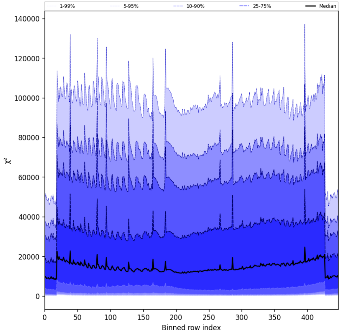
Figure 55: Along track statistics of “ \chi^2 ” for 2025-04-26 to 2025-04-28
