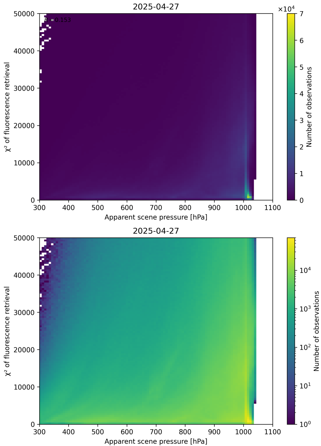
Figure 63: Scatter density plot of “Apparent scene pressure” against “ \chi^2 of fluorescence retrieval” for 2025-04-26 to 2025-04-28.
