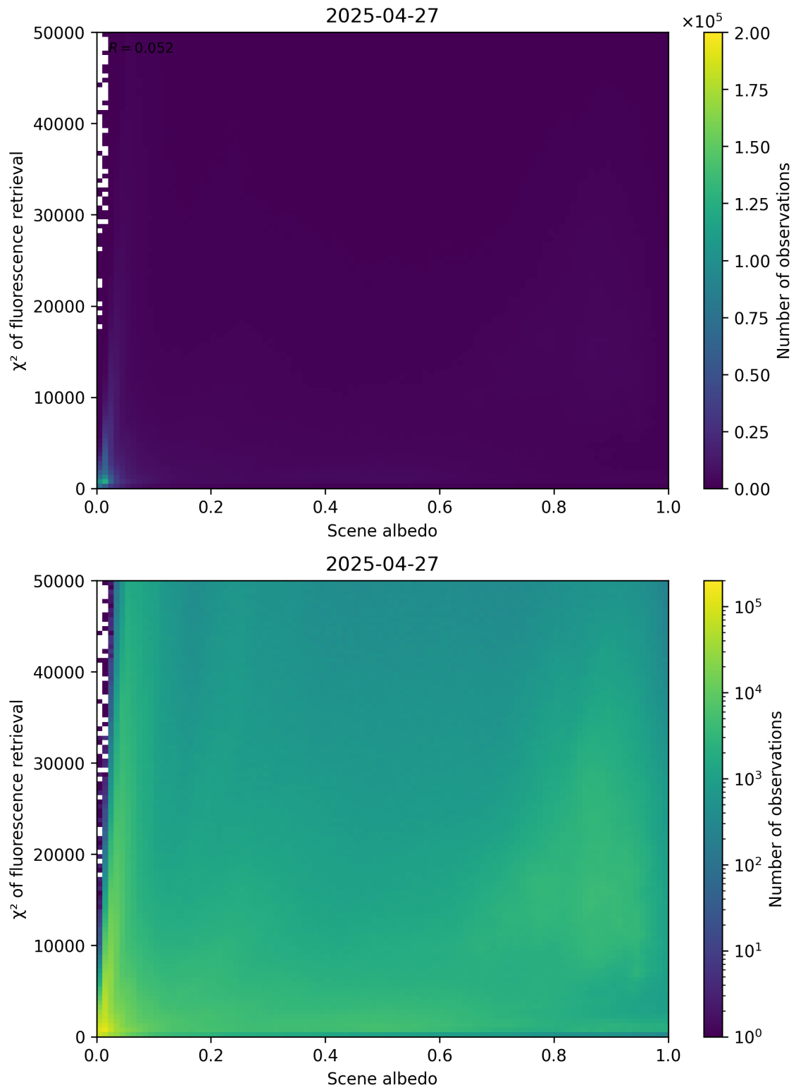
Figure 103: Scatter density plot of “Scene albedo” against “ \chi^2 of fluorescence retrieval” for 2025-04-26 to 2025-04-28.
