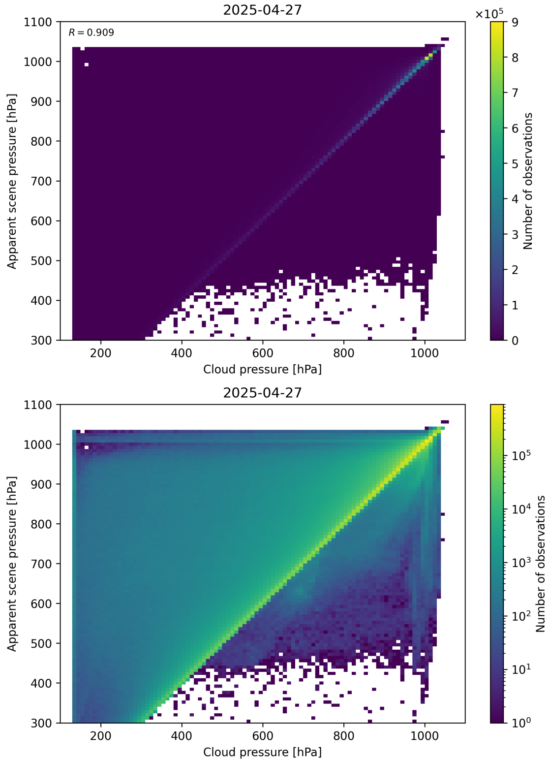
Figure 77: Scatter density plot of “Cloud pressure” against “Apparent scene pressure” for 2025-04-26 to 2025-04-28.
