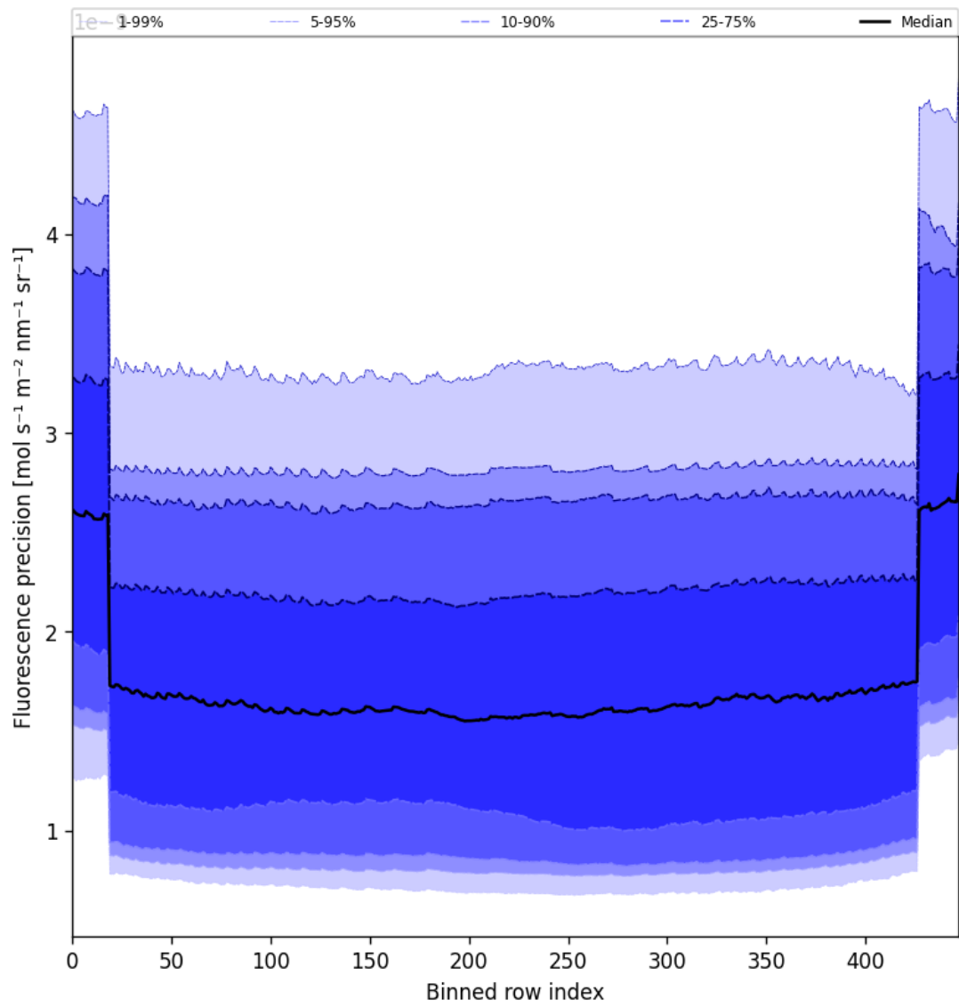
Figure 58: Along track statistics of “Fluorescence precision” for 2025-04-26 to 2025-04-28
