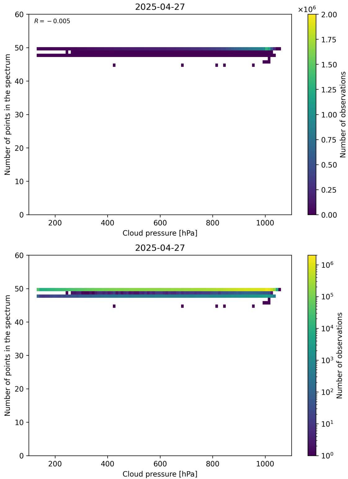
Figure 82: Scatter density plot of “Cloud pressure” against “Number of points in the spectrum” for 2025-04-26 to 2025-04-28.
