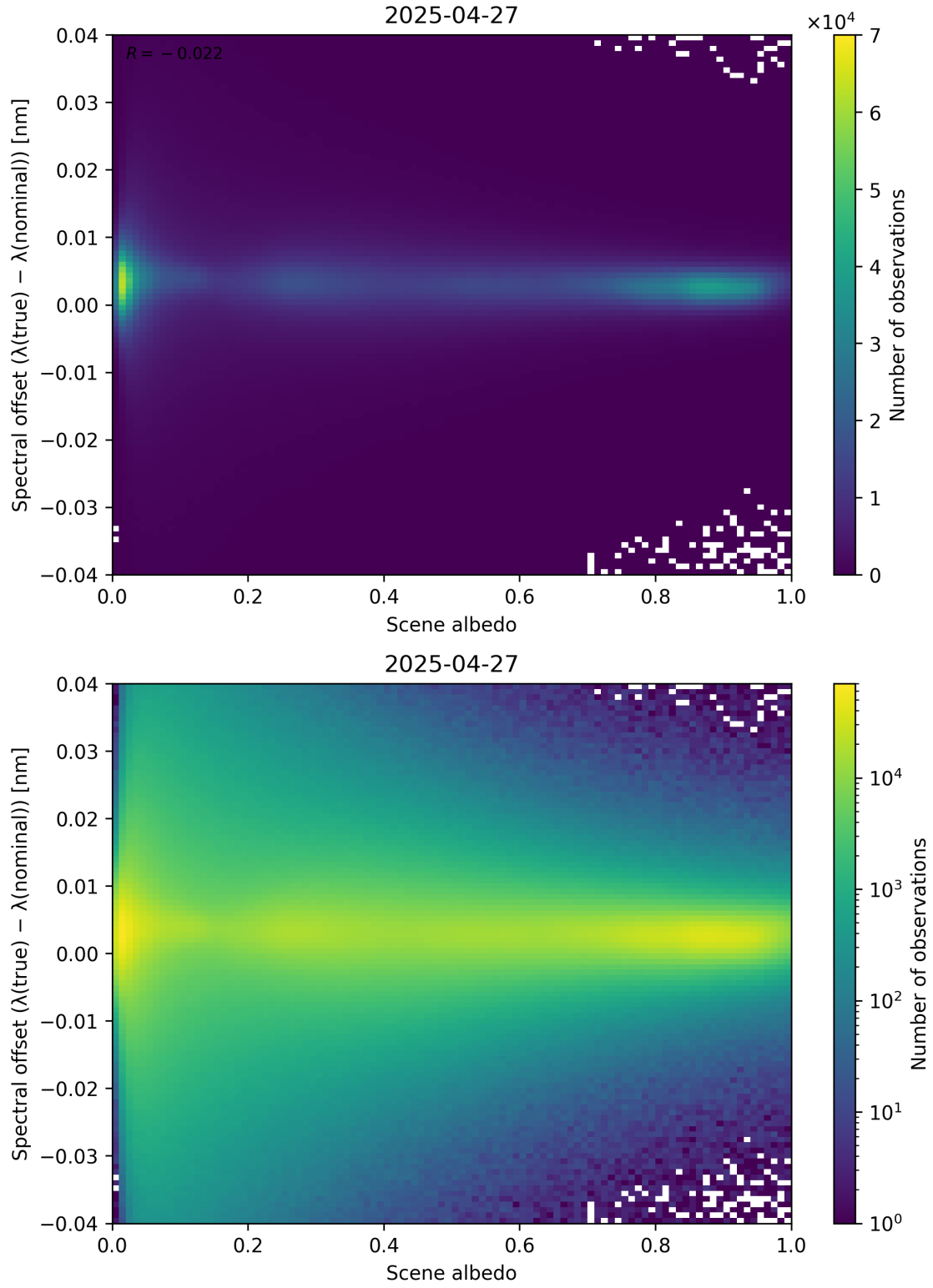
Figure 107: Scatter density plot of “Scene albedo” against “Spectral offset ( \lambda_{\text{true}} - \lambda_{\text{nominal}} )” for 2025-04-26 to 2025-04-28.
