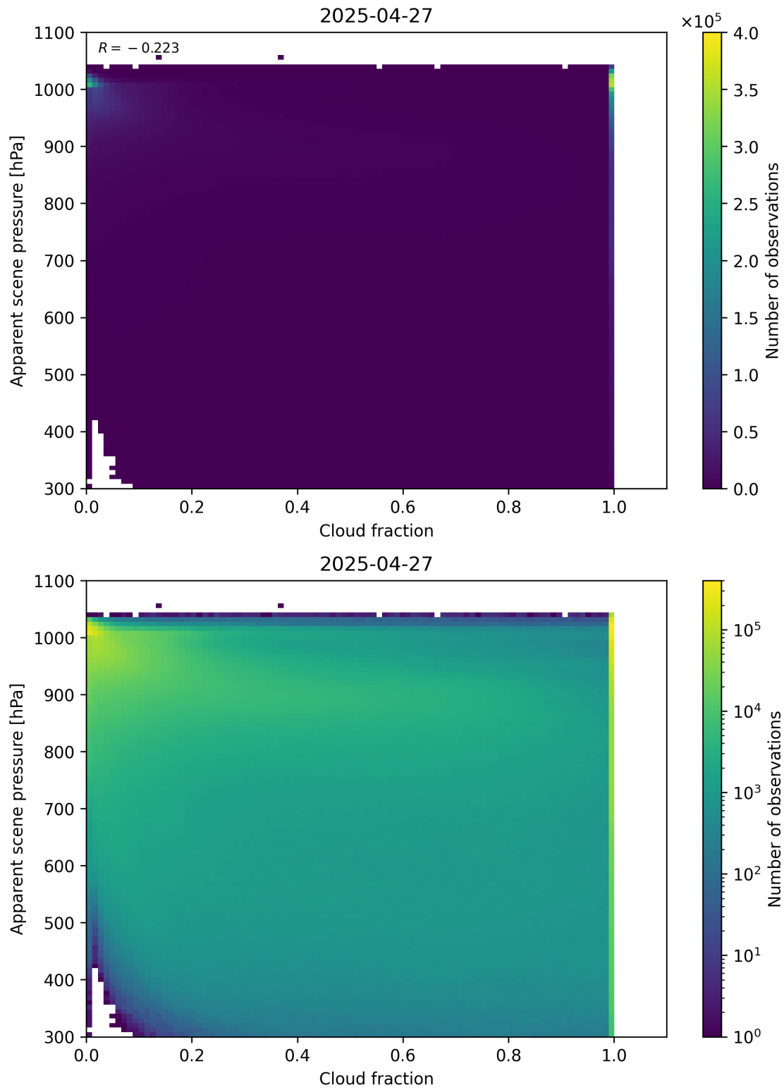
Figure 70: Scatter density plot of “Cloud fraction” against “Apparent scene pressure” for 2025-04-26 to 2025-04-28.
