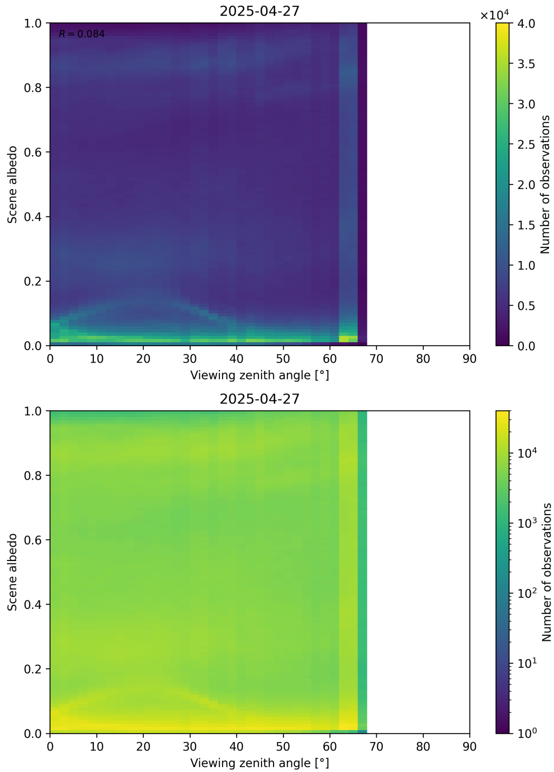
Figure 126: Scatter density plot of “Viewing zenith angle” against “Scene albedo” for 2025-04-26 to 2025-04-28.
