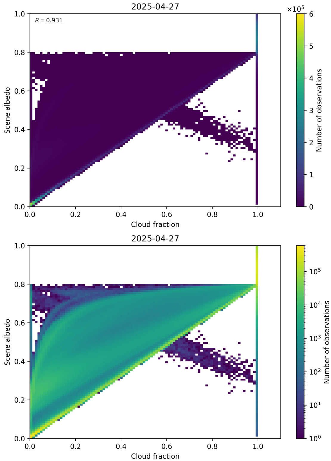
Figure 75: Scatter density plot of “Cloud fraction” against “Scene albedo” for 2025-04-26 to 2025-04-28.
