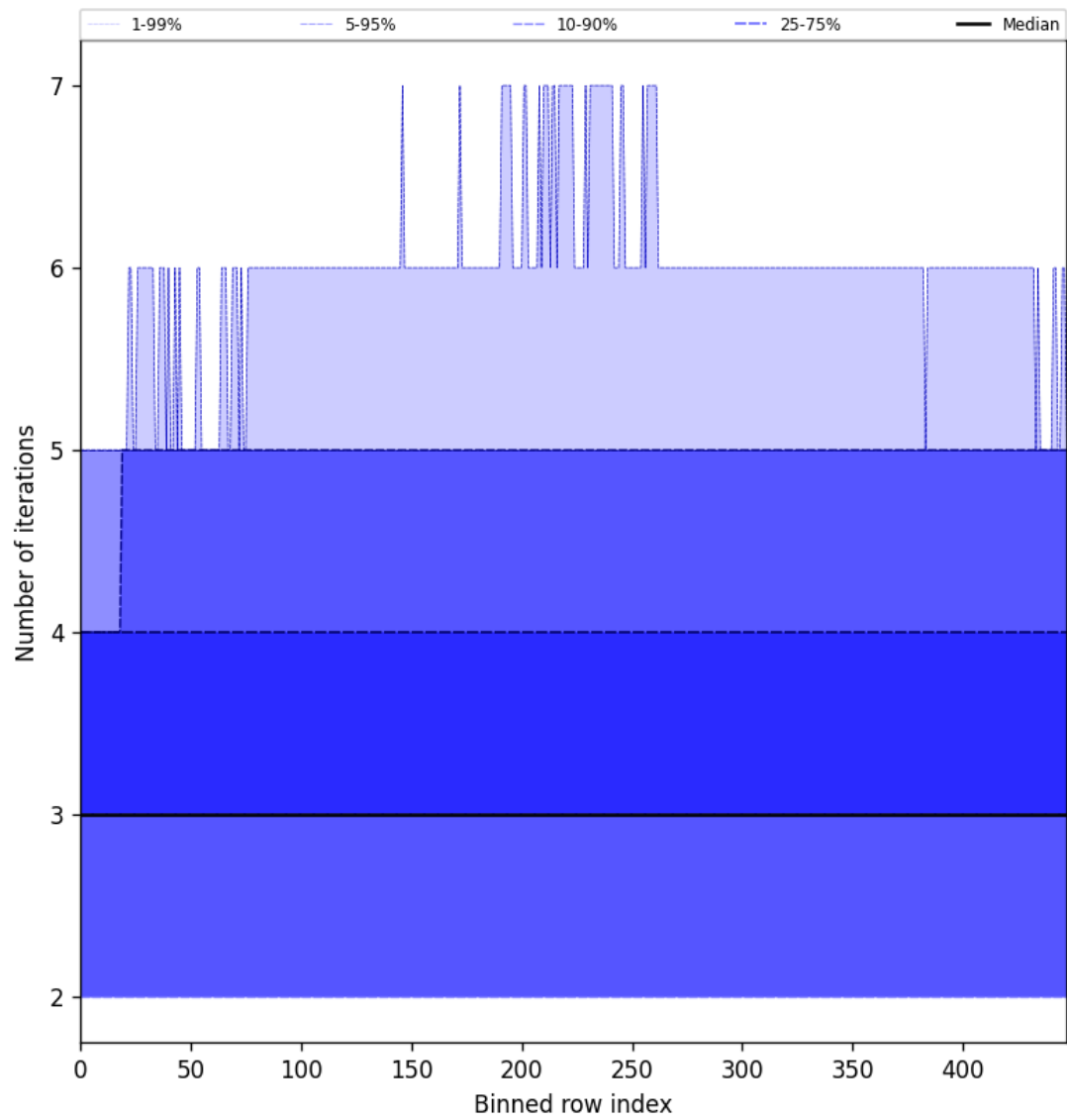
Figure 56: Along track statistics of “Number of iterations” for 2025-04-26 to 2025-04-28
