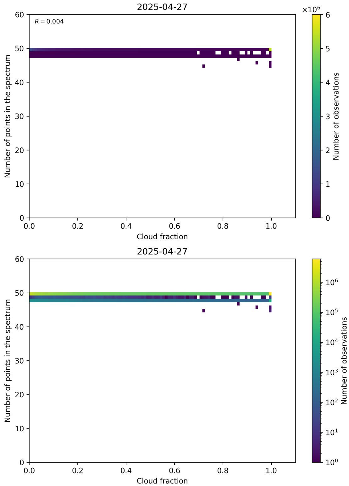
Figure 74: Scatter density plot of “Cloud fraction” against “Number of points in the spectrum” for 2025-04-26 to 2025-04-28.
