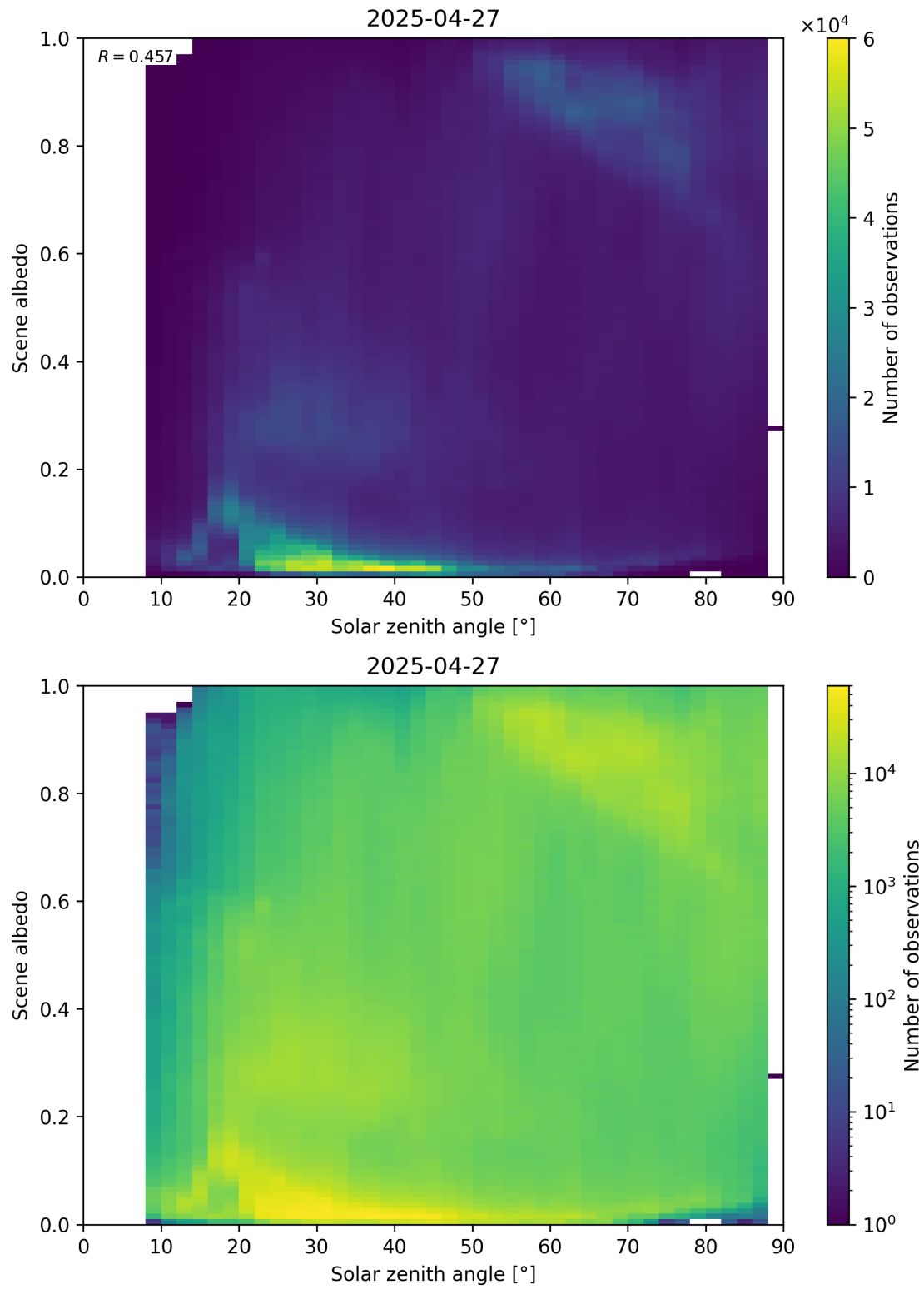
Figure 116: Scatter density plot of “Solar zenith angle” against “Scene albedo” for 2025-04-26 to 2025-04-28.
