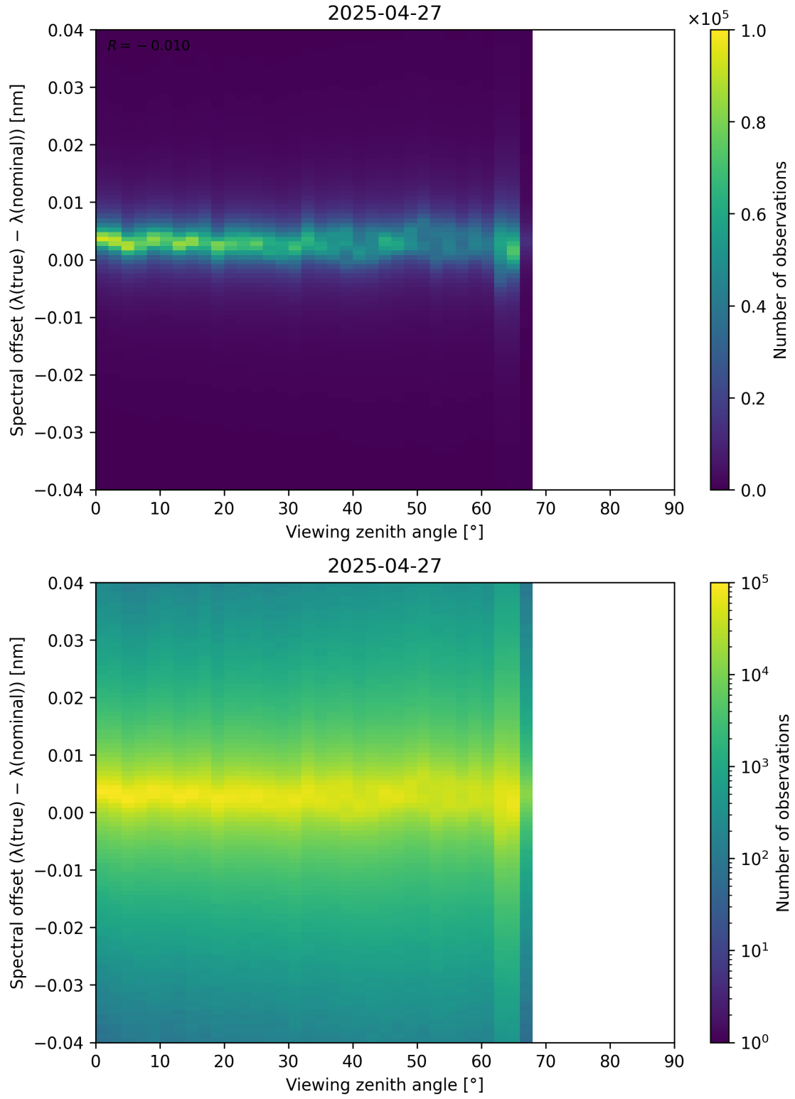
Figure 128: Scatter density plot of “Viewing zenith angle” against “Spectral offset ( \lambda_{\text{true}} - \lambda_{\text{nominal}} )” for 2025-04-26 to 2025-04-28.
