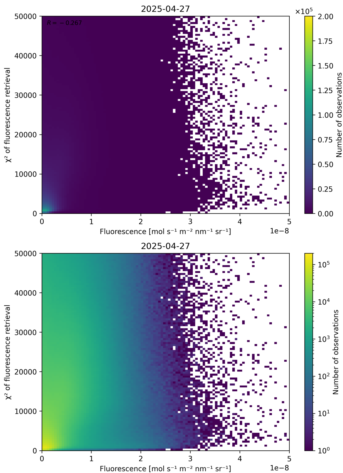
Figure 85: Scatter density plot of “Fluorescence” against “ \chi^2 of fluorescence retrieval” for 2025-04-26 to 2025-04-28.
