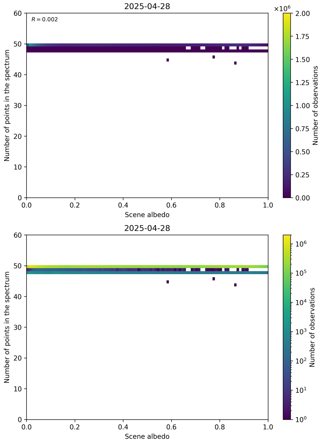
Figure 106: Scatter density plot of “Scene albedo” against “Number of points in the spectrum” for 2025-04-27 to 2025-04-29.
