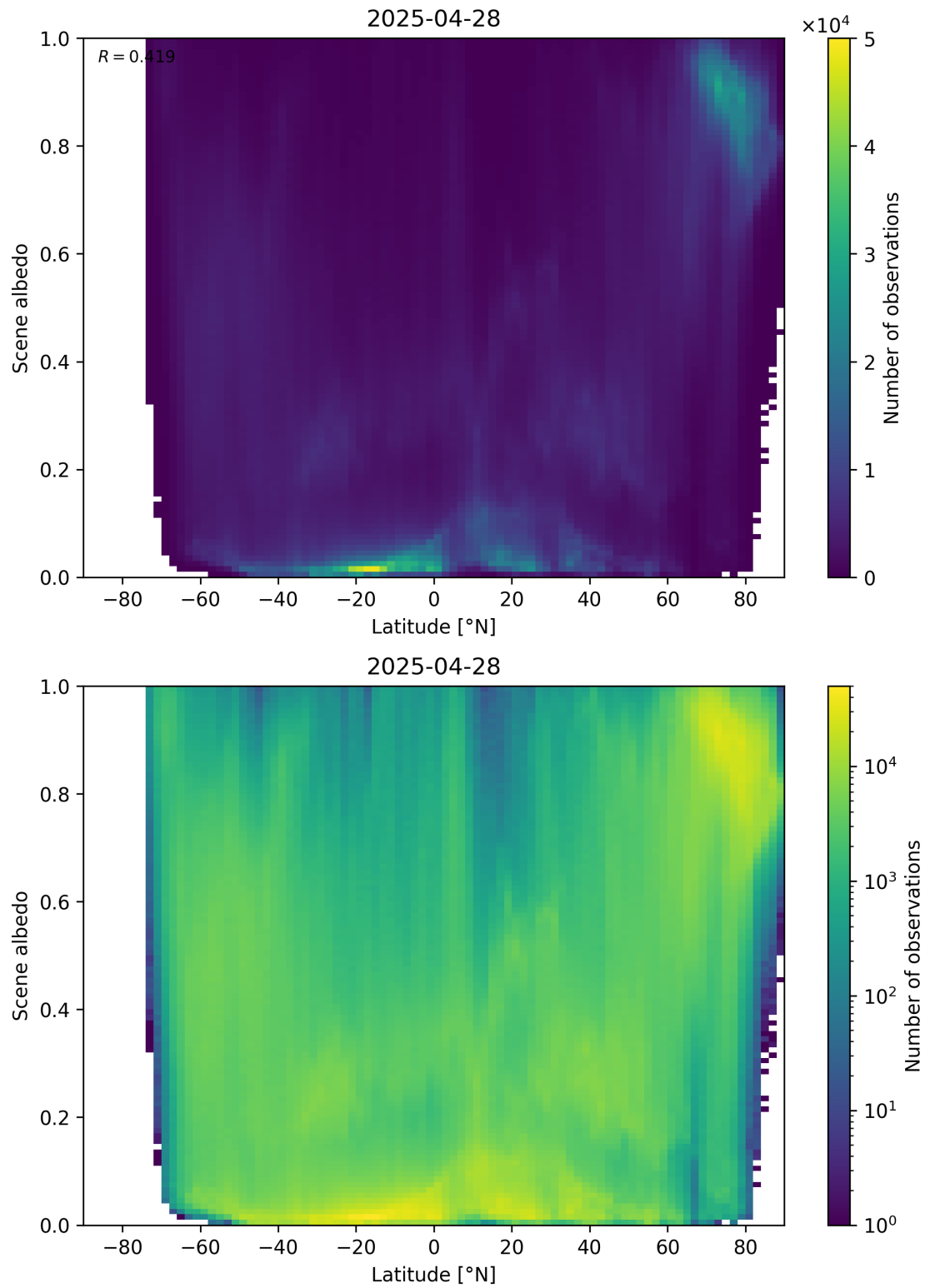
Figure 95: Scatter density plot of “Latitude” against “Scene albedo” for 2025-04-27 to 2025-04-29.
