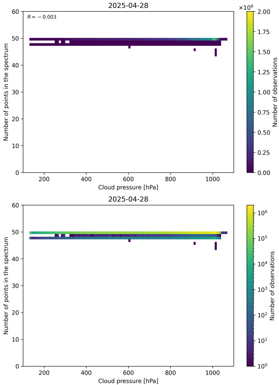
Figure 82: Scatter density plot of “Cloud pressure” against “Number of points in the spectrum” for 2025-04-27 to 2025-04-29.
