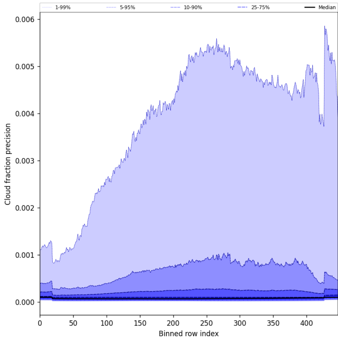
Figure 50: Along track statistics of “Cloud fraction precision” for 2025-04-27 to 2025-04-29
