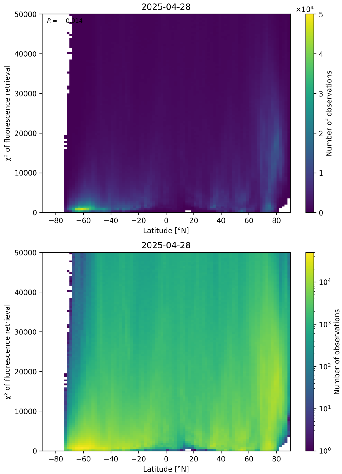
Figure 89: Scatter density plot of “Latitude” against “ \chi^2 of fluorescence retrieval” for 2025-04-27 to 2025-04-29.
