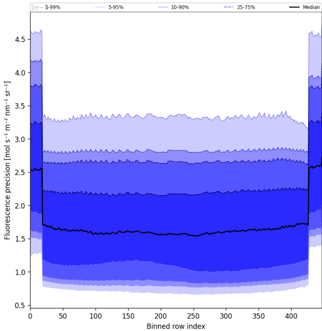
Figure 58: Along track statistics of “Fluorescence precision” for 2025-04-27 to 2025-04-29
