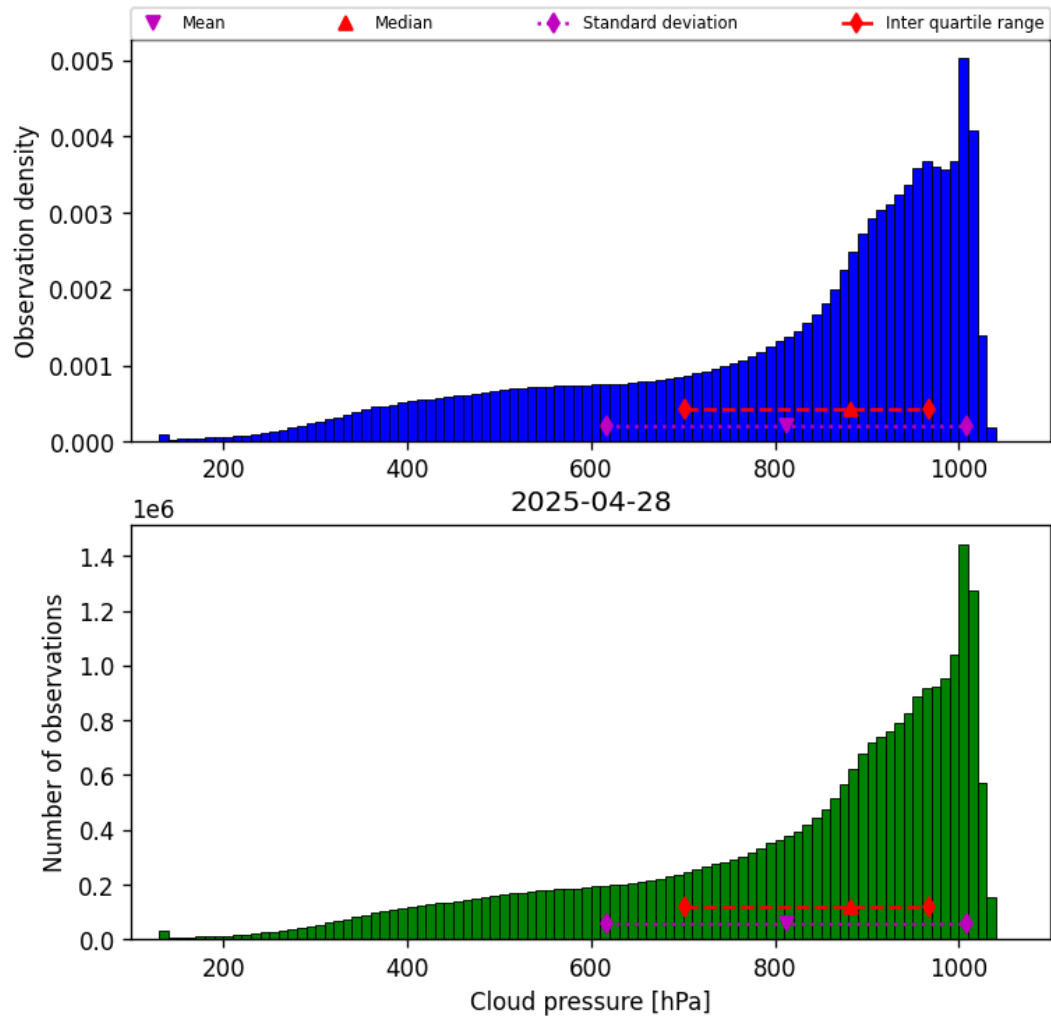
Figure 30: Histogram of “Cloud pressure” for 2025-04-27 to 2025-04-29
