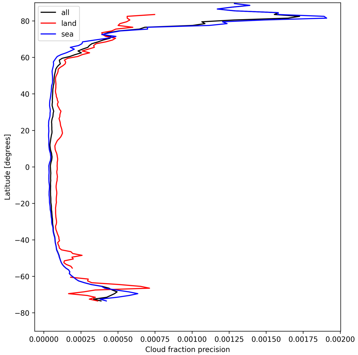
Figure 16: Zonal average of “Cloud fraction precision” for 2025-04-27 to 2025-04-29.
