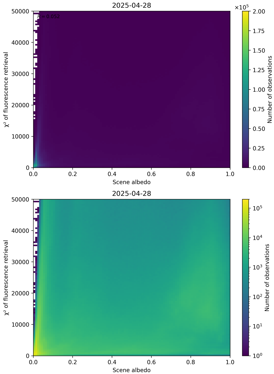
Figure 103: Scatter density plot of “Scene albedo” against “ \chi^2 of fluorescence retrieval” for 2025-04-27 to 2025-04-29.
