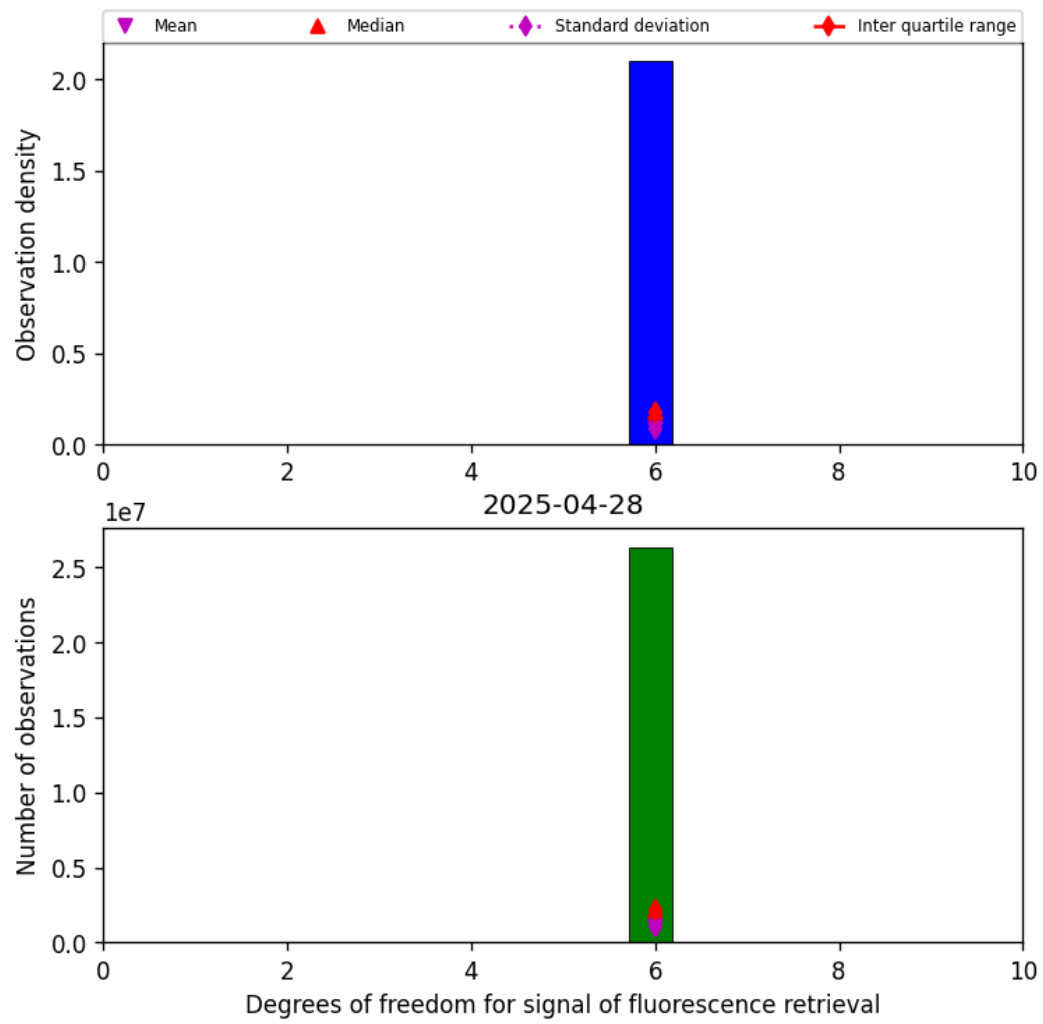
Figure 43: Histogram of "Degrees of freedom for signal of fluorescence retrieval" for 2025-04-27 to 2025-04-29
