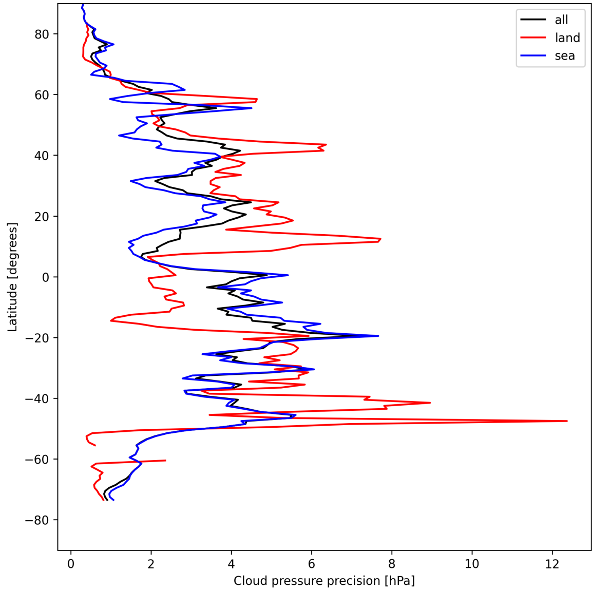
Figure 14: Zonal average of “Cloud pressure precision” for 2025-04-27 to 2025-04-29.
