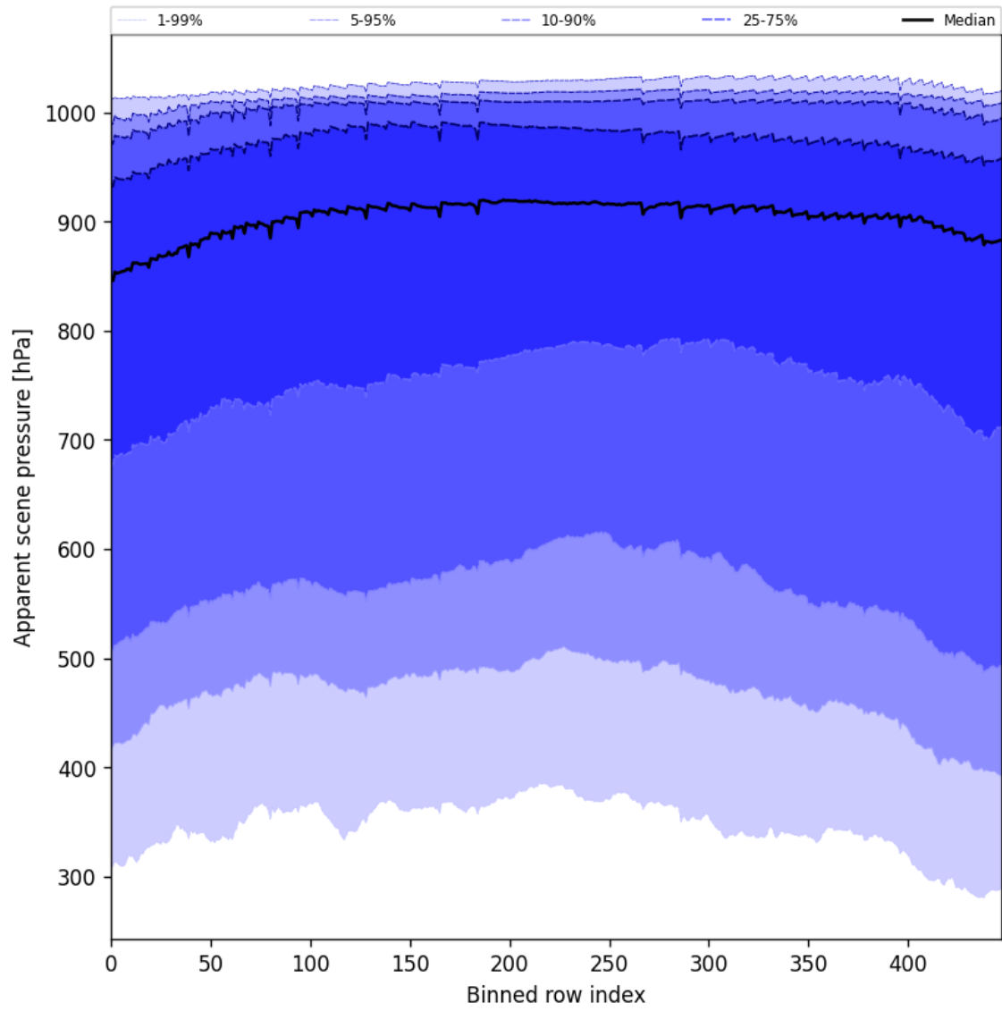
Figure 53: Along track statistics of “Apparent scene pressure” for 2025-04-27 to 2025-04-29
