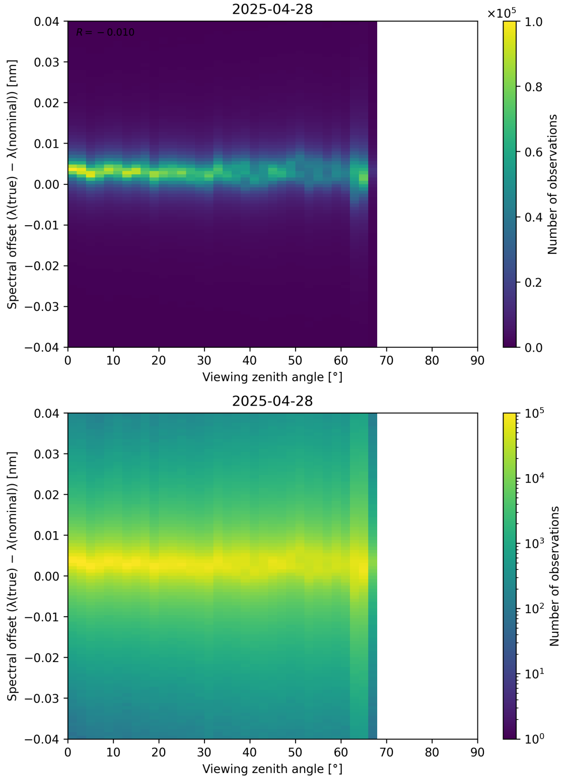
Figure 128: Scatter density plot of “Viewing zenith angle” against “Spectral offset ( \lambda_{\text{true}} - \lambda_{\text{nominal}} )” for 2025-04-27 to 2025-04-29.
