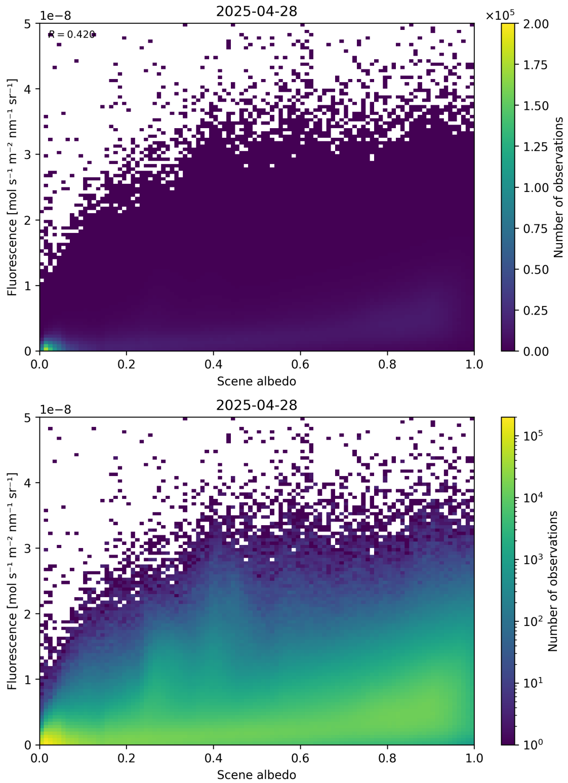
Figure 104: Scatter density plot of “Scene albedo” against “Fluorescence” for 2025-04-27 to 2025-04-29.
