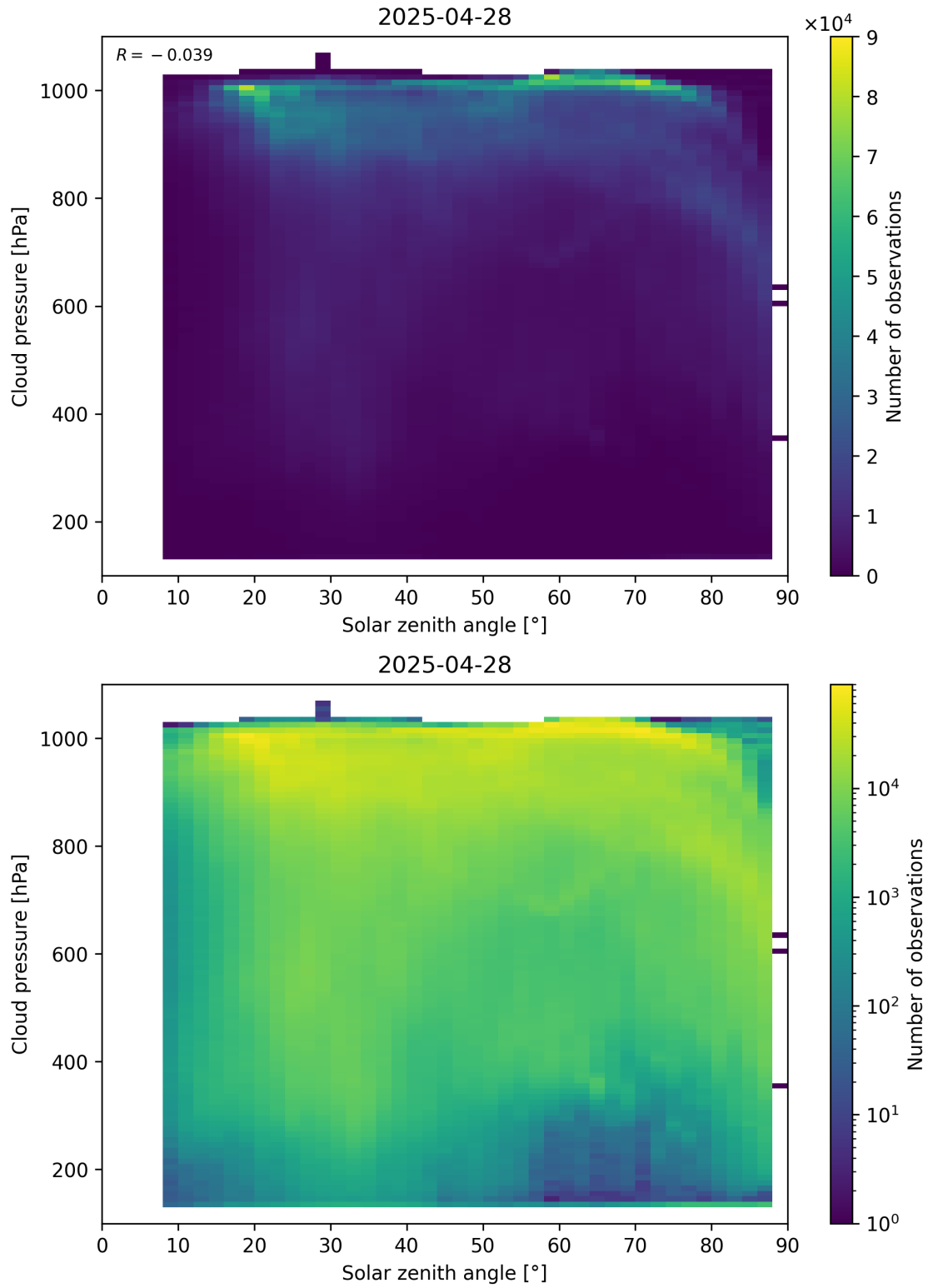
Figure 111: Scatter density plot of “Solar zenith angle” against “Cloud pressure” for 2025-04-27 to 2025-04-29.
