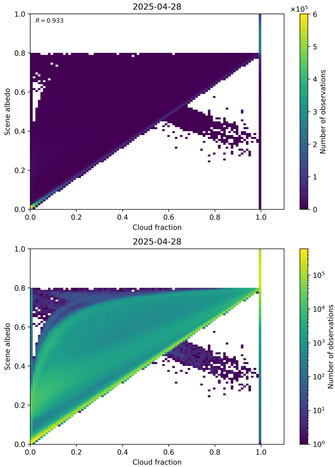
Figure 75: Scatter density plot of “Cloud fraction” against “Scene albedo” for 2025-04-27 to 2025-04-29.
