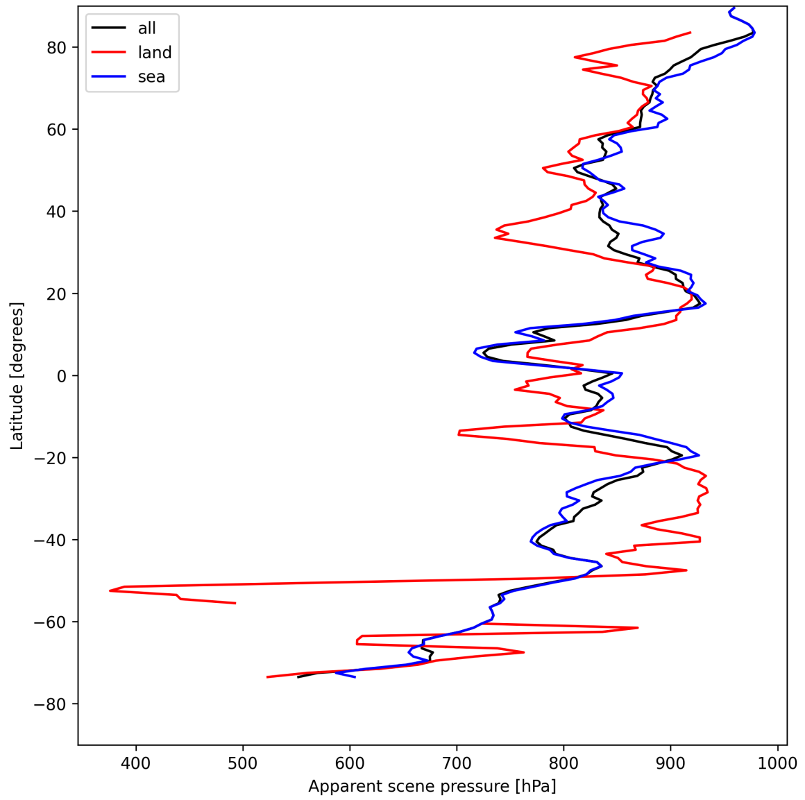
Figure 19: Zonal average of “Apparent scene pressure” for 2025-04-27 to 2025-04-29.
