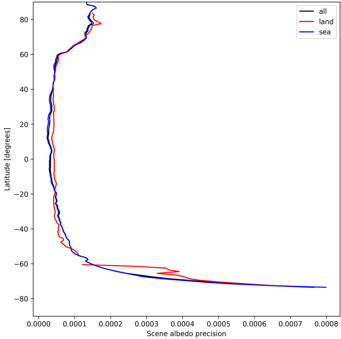
Figure 18: Zonal average of “Scene albedo precision” for 2025-04-27 to 2025-04-29.
