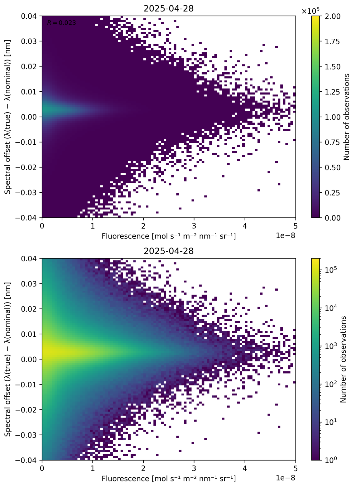
Figure 87: Scatter density plot of “Fluorescence” against “Spectral offset ( \lambda_{\text{true}} - \lambda_{\text{nominal}} )” for 2025-04-27 to 2025-04-29.
