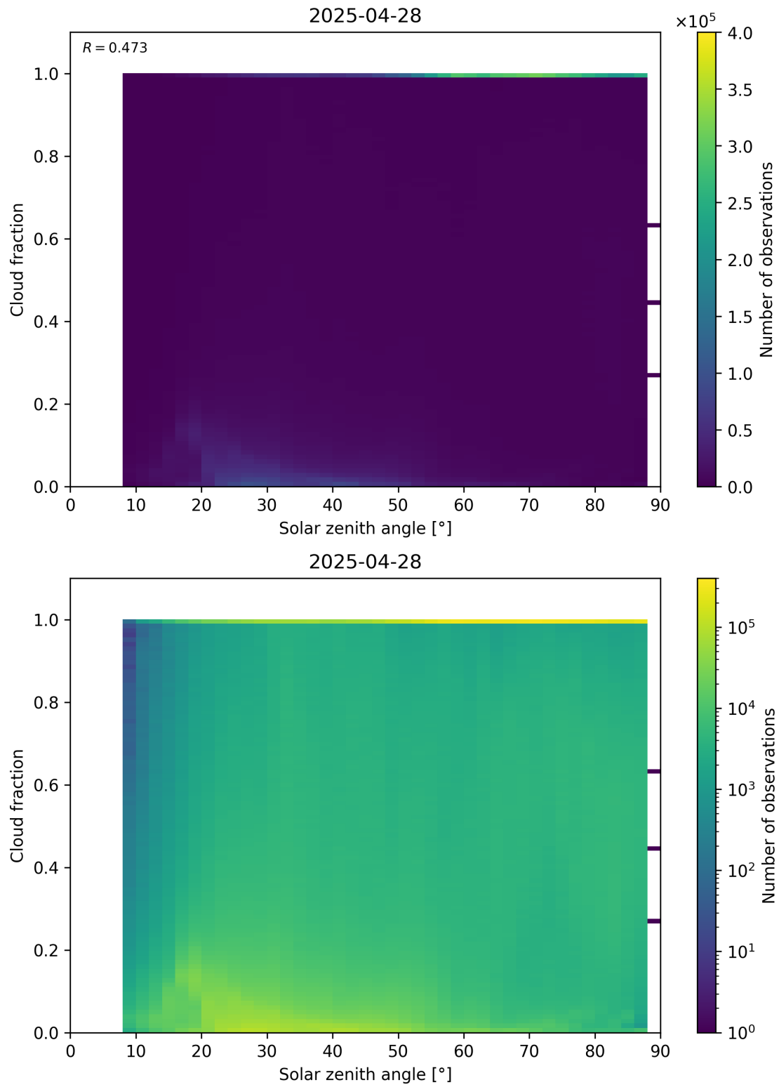
Figure 110: Scatter density plot of “Solar zenith angle” against “Cloud fraction” for 2025-04-27 to 2025-04-29.
