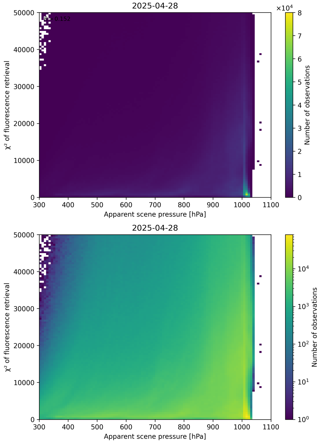
Figure 63: Scatter density plot of “Apparent scene pressure” against “ \chi^2 of fluorescence retrieval” for 2025-04-27 to 2025-04-29.
