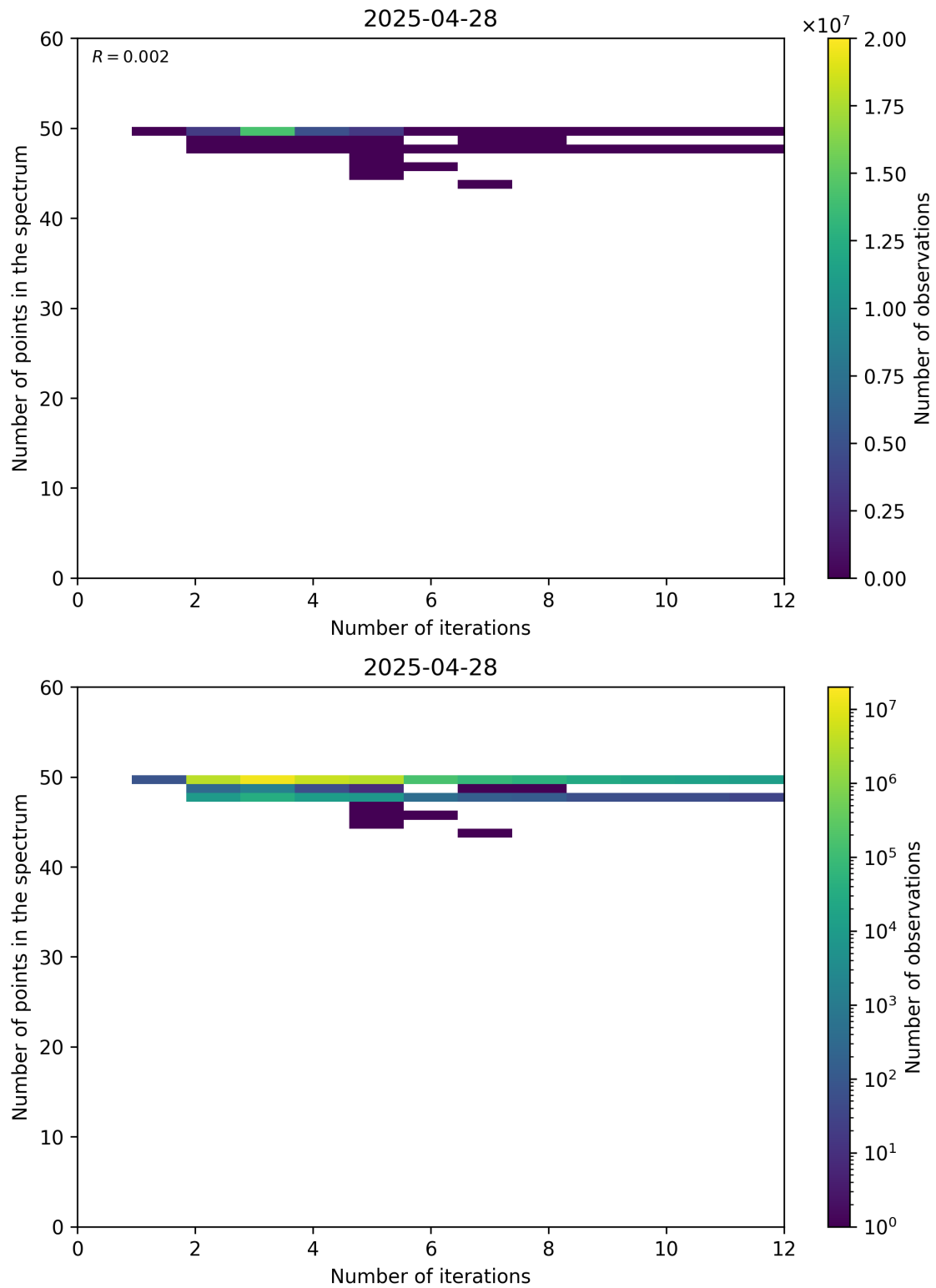
Figure 99: Scatter density plot of “Number of iterations” against “Number of points in the spectrum” for 2025-04-27 to 2025-04-29.
