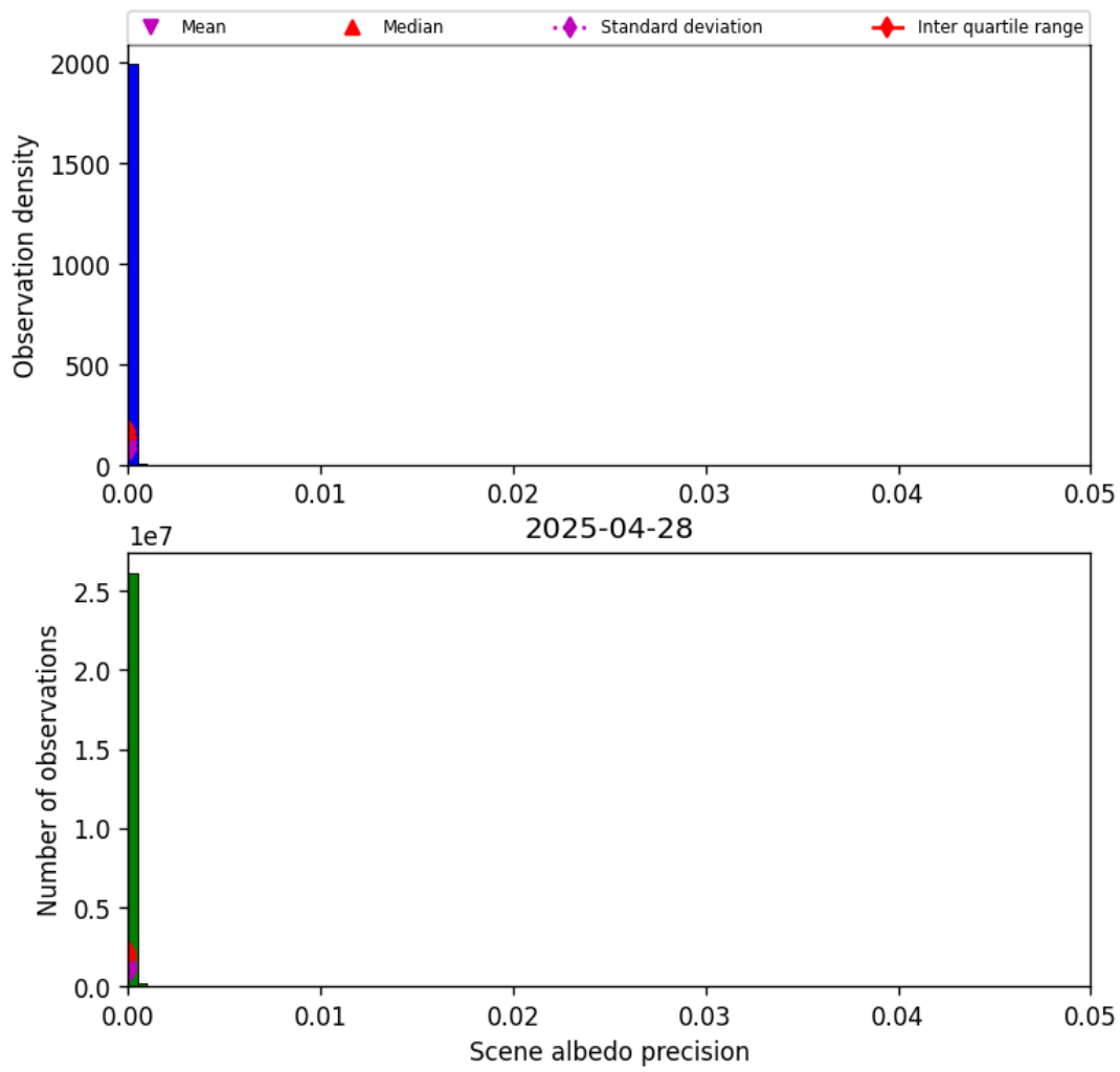
Figure 35: Histogram of “Scene albedo precision” for 2025-04-27 to 2025-04-29
