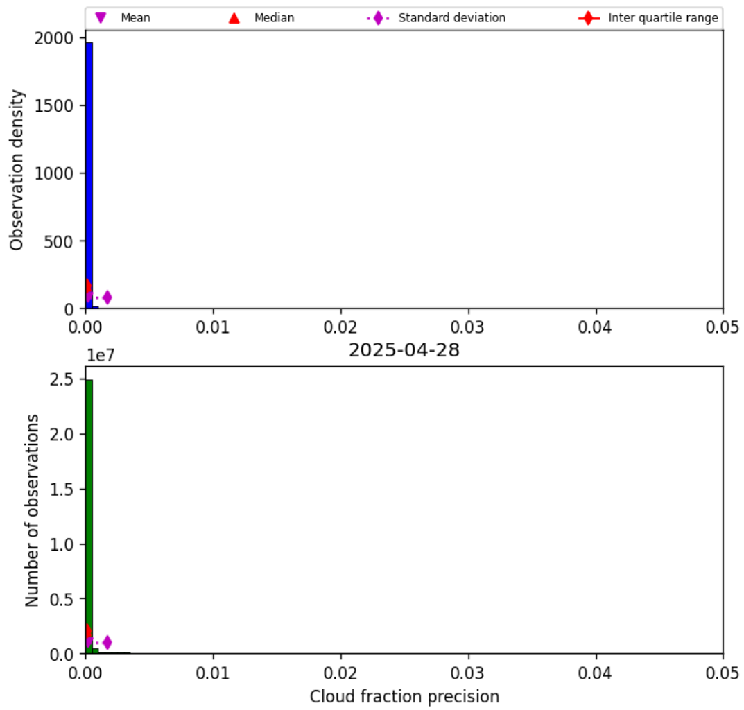
Figure 33: Histogram of “Cloud fraction precision” for 2025-04-27 to 2025-04-29
