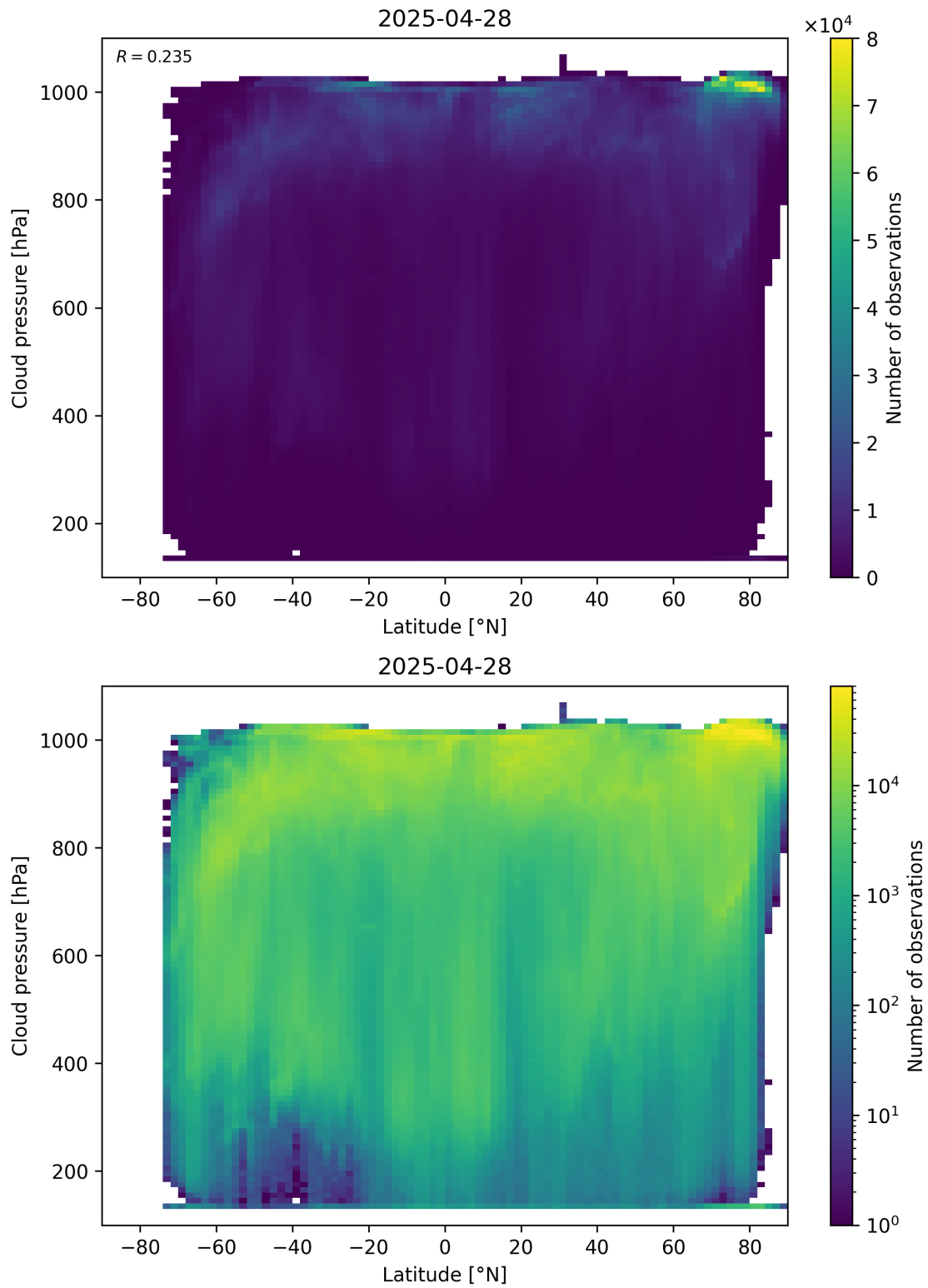
Figure 91: Scatter density plot of “Latitude” against “Cloud pressure” for 2025-04-27 to 2025-04-29.
