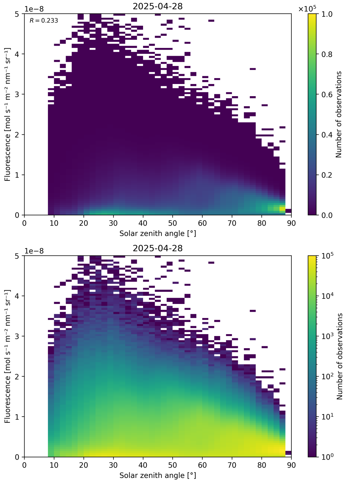
Figure 112: Scatter density plot of “Solar zenith angle” against “Fluorescence” for 2025-04-27 to 2025-04-29.
