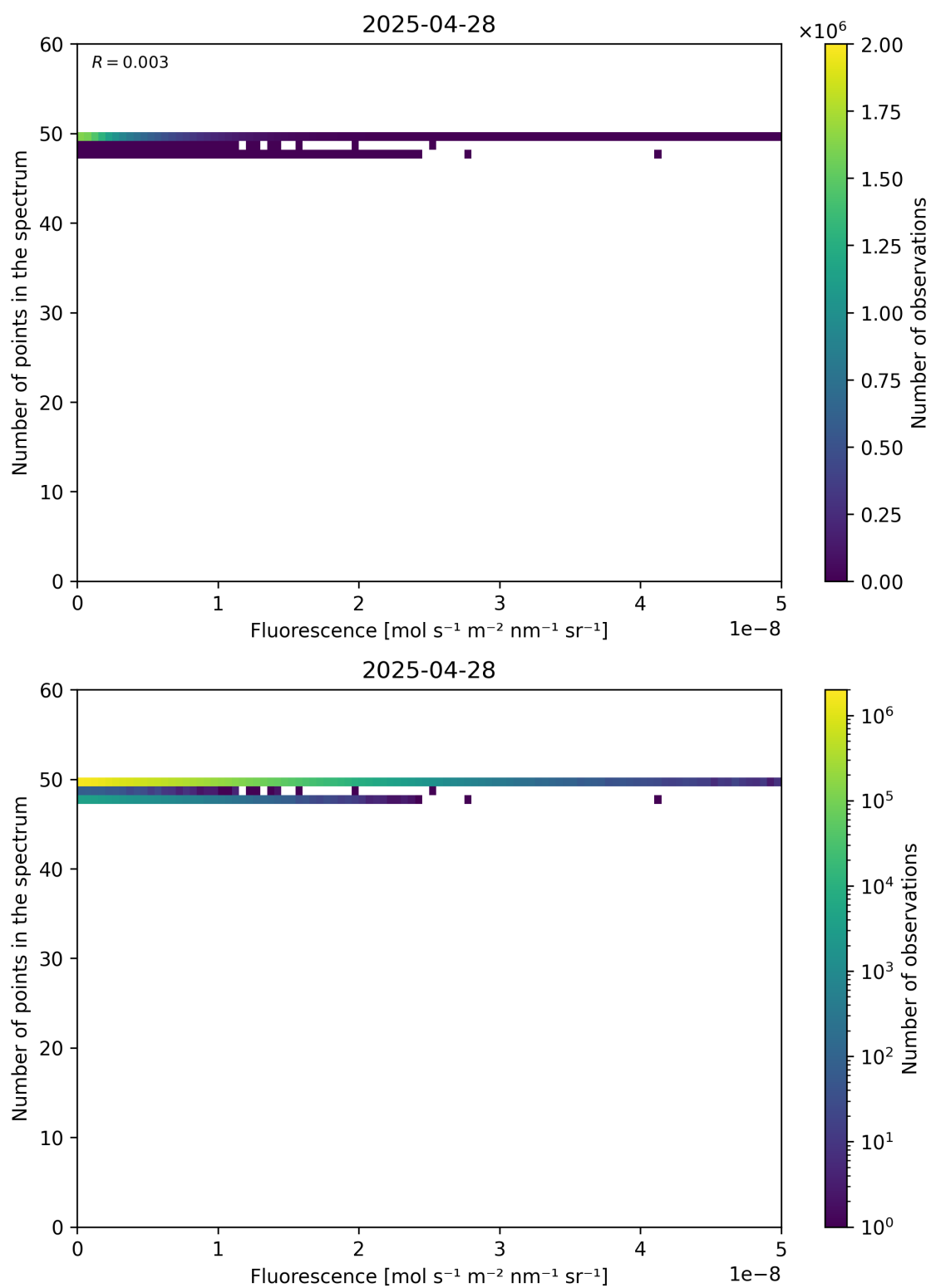
Figure 86: Scatter density plot of “Fluorescence” against “Number of points in the spectrum” for 2025-04-27 to 2025-04-29.
