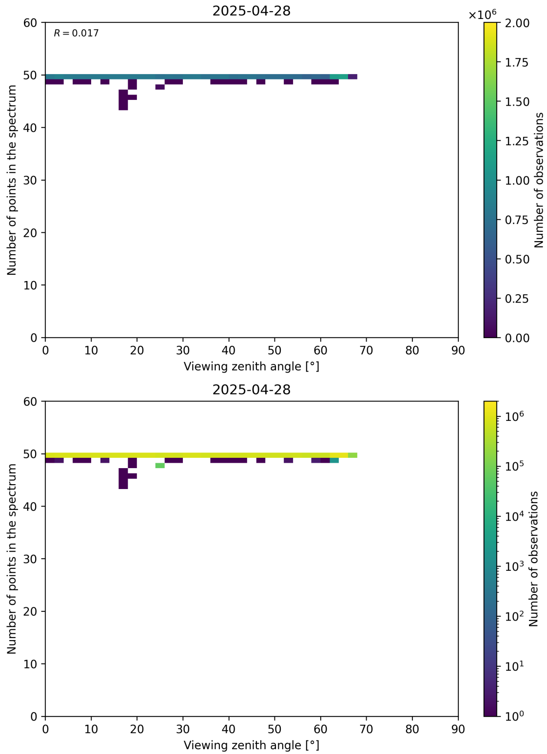
Figure 125: Scatter density plot of “Viewing zenith angle” against “Number of points in the spectrum” for 2025-04-27 to 2025-04-29.
