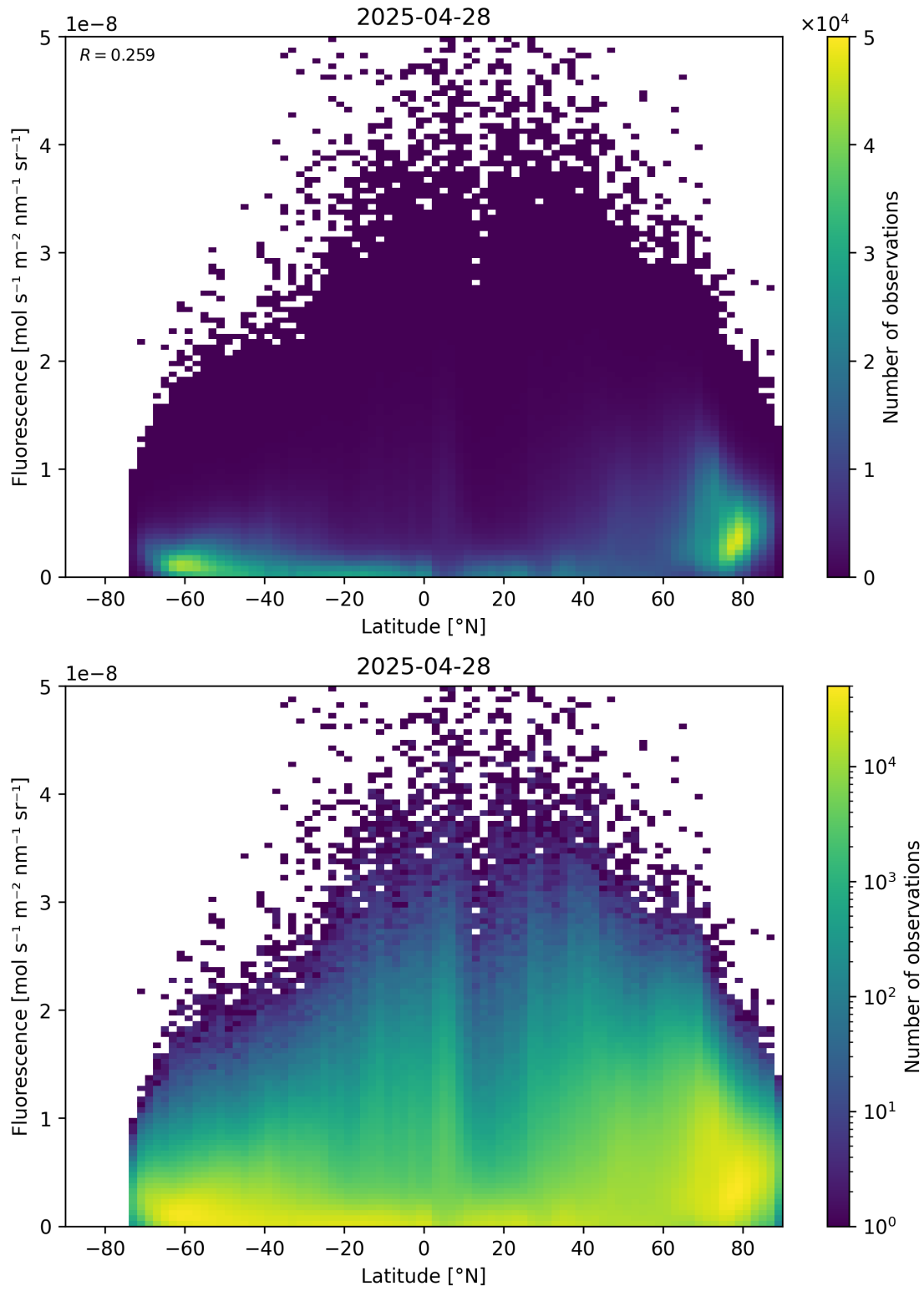
Figure 92: Scatter density plot of “Latitude” against “Fluorescence” for 2025-04-27 to 2025-04-29.
