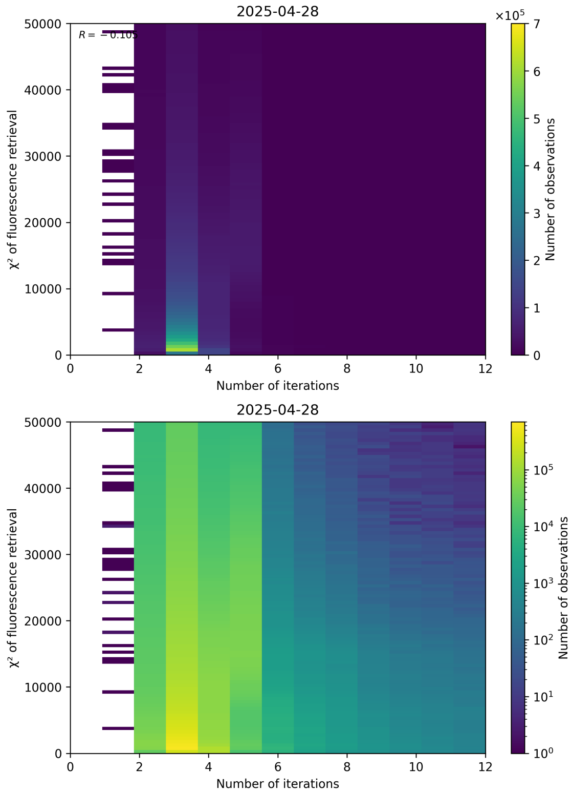
Figure 97: Scatter density plot of “Number of iterations” against “ \chi^2 of fluorescence retrieval” for 2025-04-27 to 2025-04-29.
