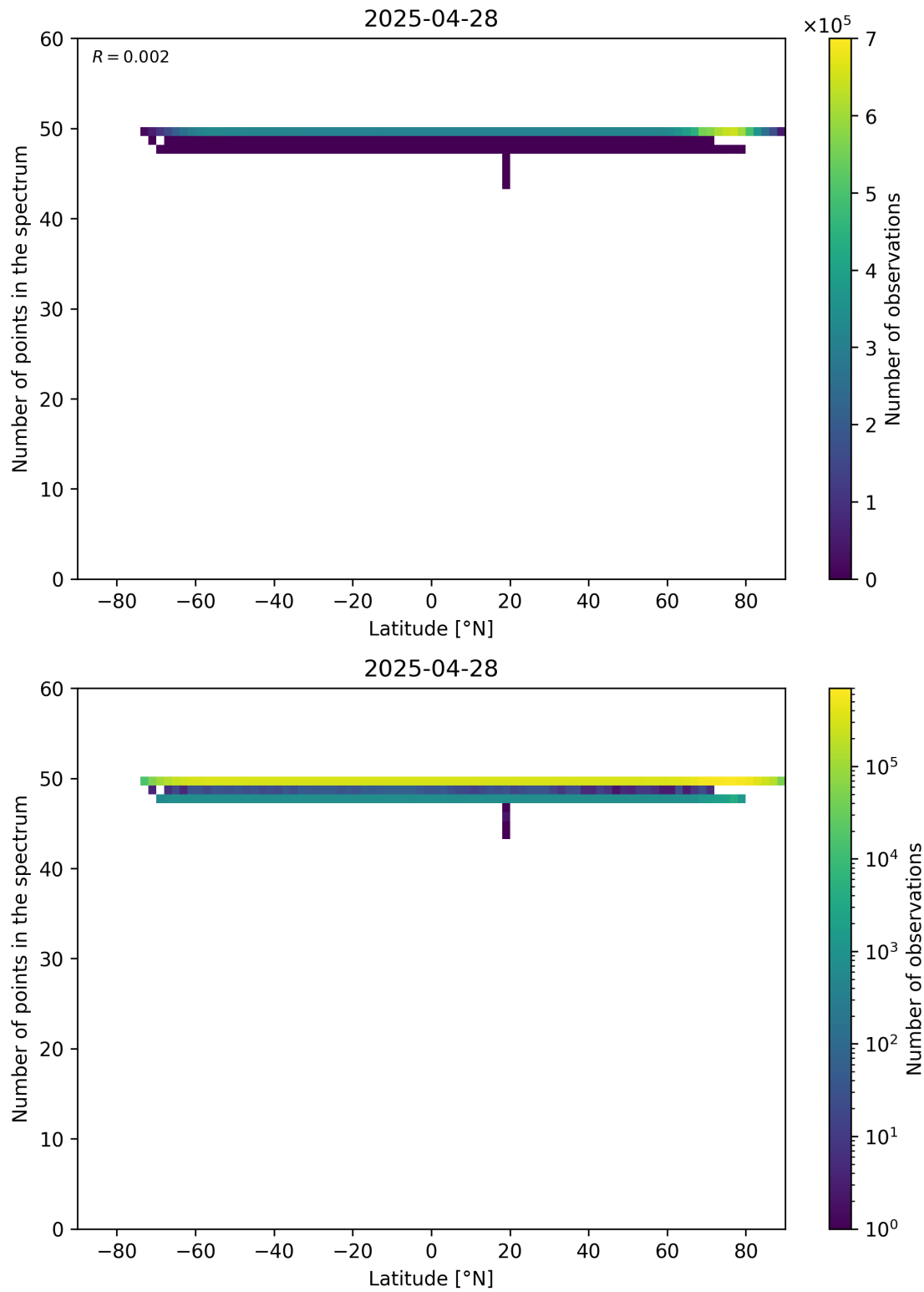
Figure 94: Scatter density plot of “Latitude” against “Number of points in the spectrum” for 2025-04-27 to 2025-04-29.
