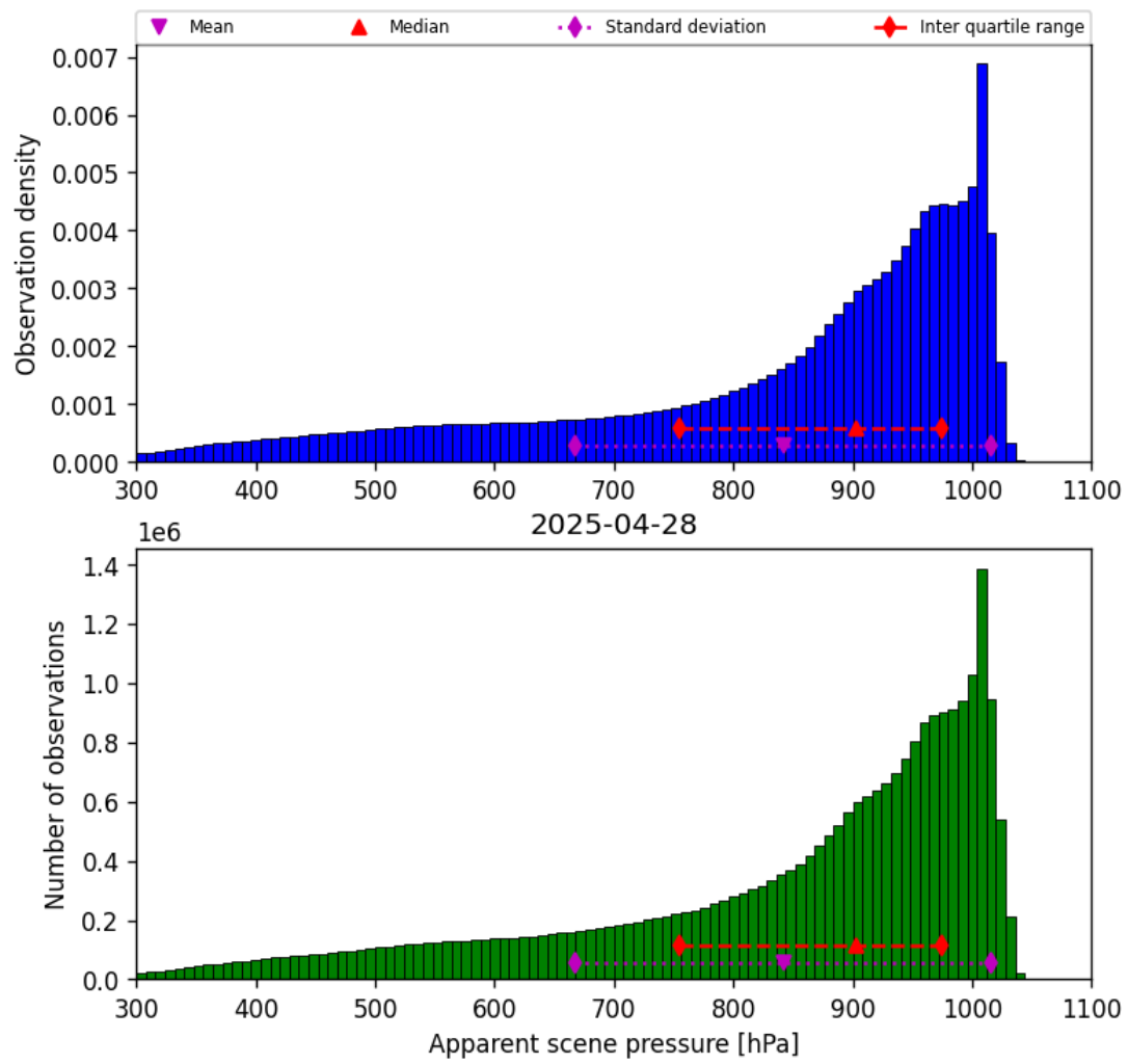
Figure 36: Histogram of “Apparent scene pressure” for 2025-04-27 to 2025-04-29
