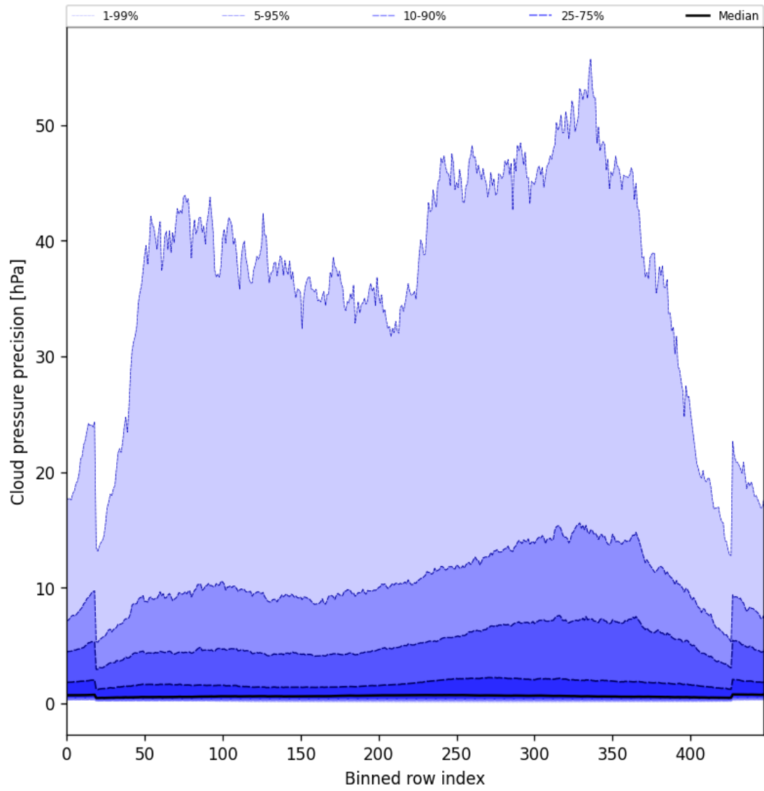
Figure 48: Along track statistics of “Cloud pressure precision” for 2025-04-27 to 2025-04-29
