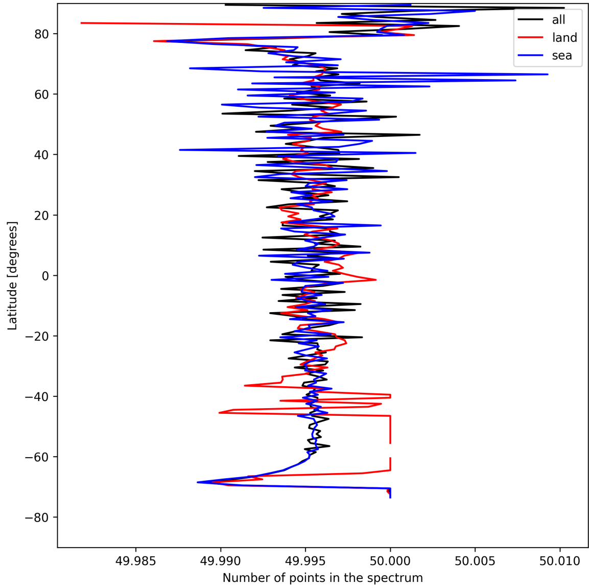
Figure 27: Zonal average of “Number of points in the spectrum” for 2025-04-27 to 2025-04-29.
