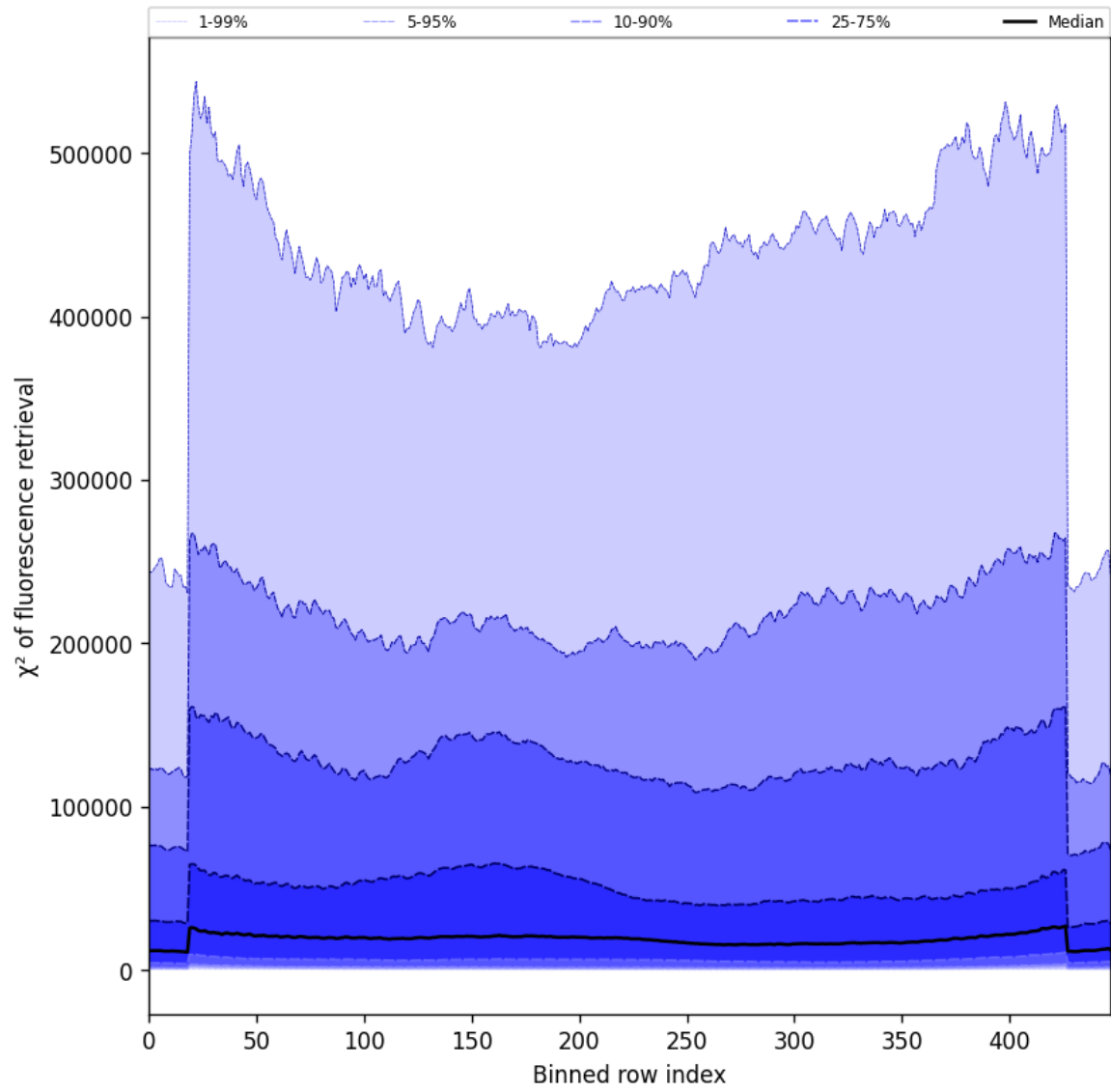
Figure 59: Along track statistics of “ \chi^2 of fluorescence retrieval” for 2025-04-27 to 2025-04-29
