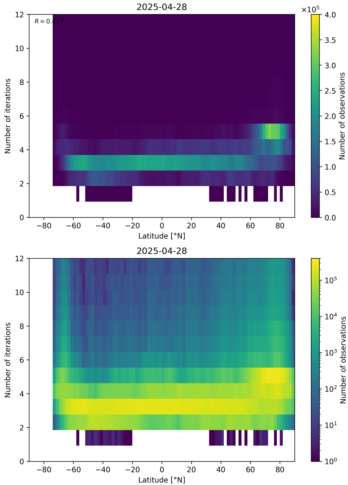
Figure 93: Scatter density plot of “Latitude” against “Number of iterations” for 2025-04-27 to 2025-04-29.
