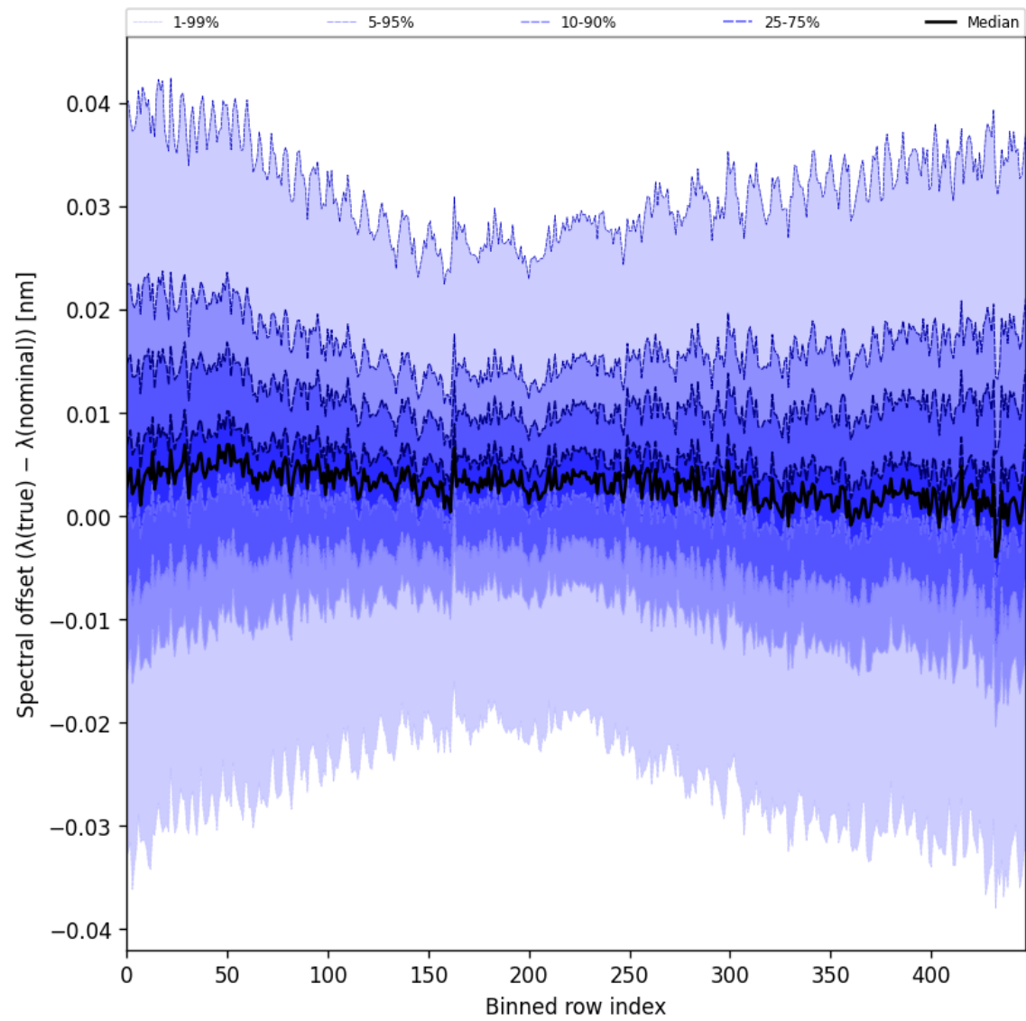
Figure 62: Along track statistics of “Spectral offset ( \lambda_{\text{true}} - \lambda_{\text{nominal}} )” for 2025-04-27 to 2025-04-29
