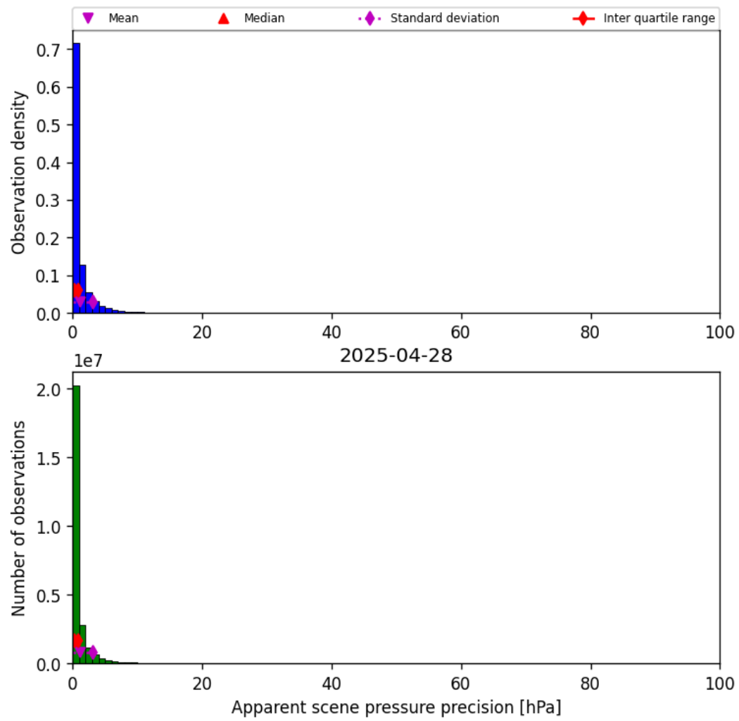
Figure 37: Histogram of “Apparent scene pressure precision” for 2025-04-27 to 2025-04-29
