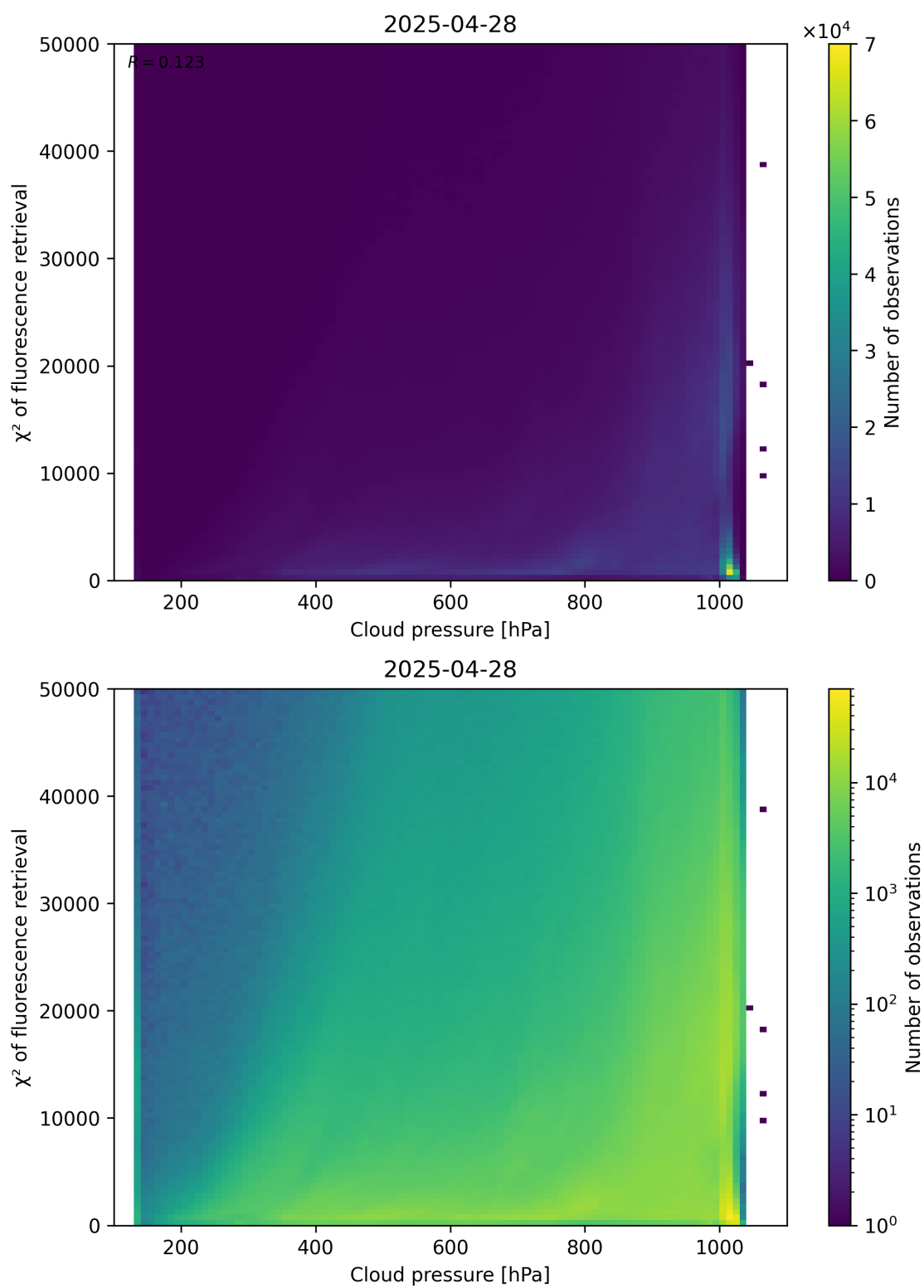
Figure 78: Scatter density plot of “Cloud pressure” against “ \chi^2 of fluorescence retrieval” for 2025-04-27 to 2025-04-29.
