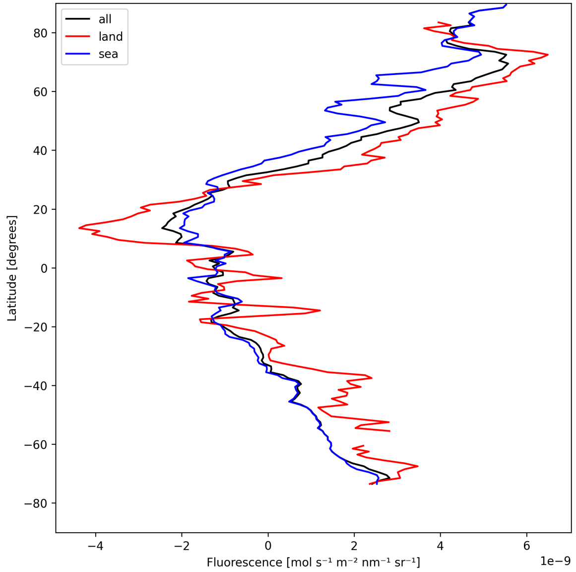
Figure 23: Zonal average of “Fluorescence” for 2025-04-27 to 2025-04-29.
