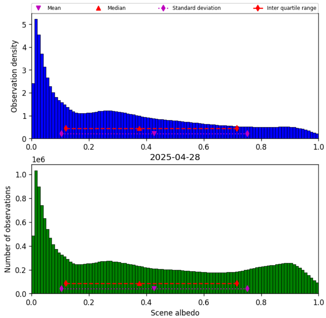
Figure 34: Histogram of “Scene albedo” for 2025-04-27 to 2025-04-29
