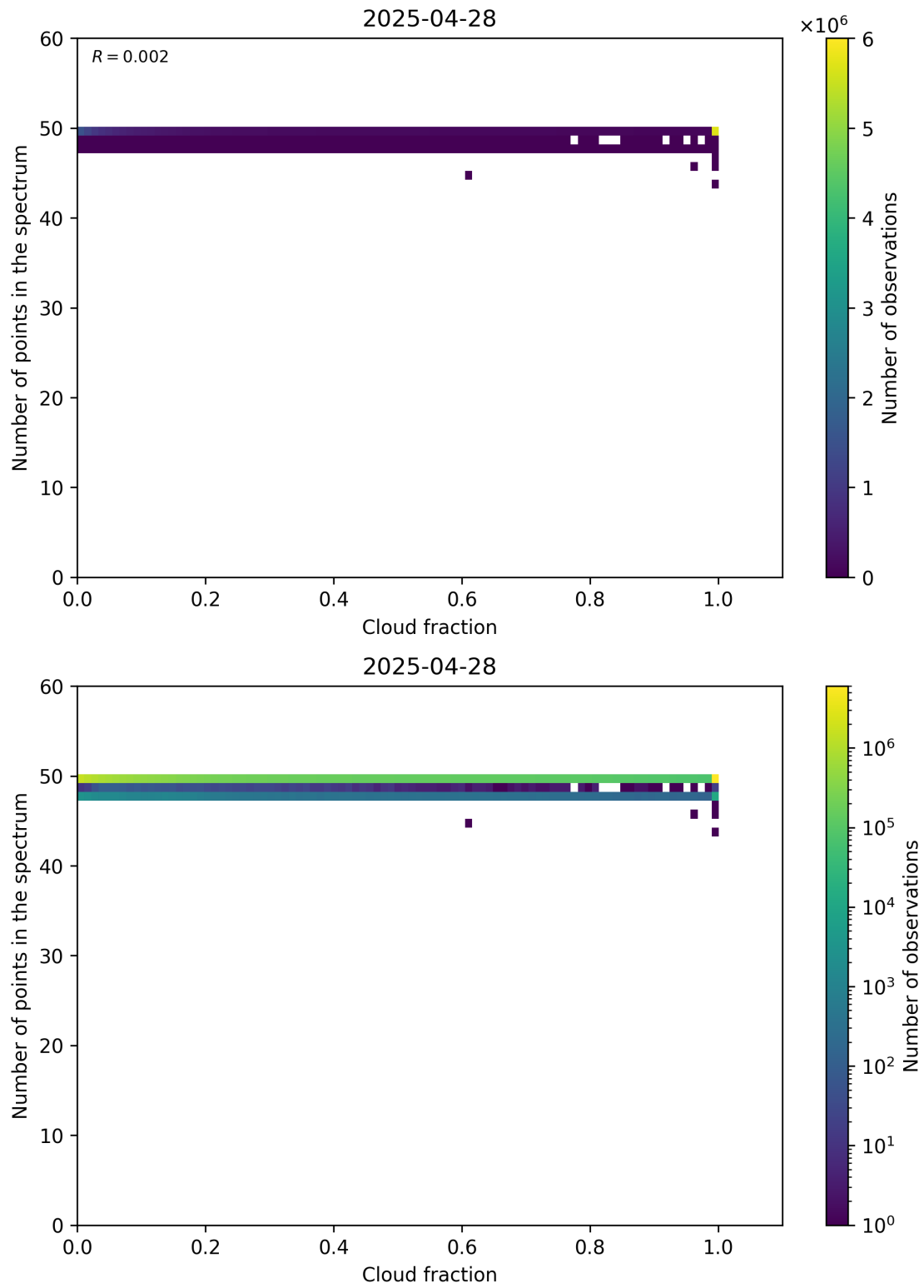
Figure 74: Scatter density plot of “Cloud fraction” against “Number of points in the spectrum” for 2025-04-27 to 2025-04-29.
