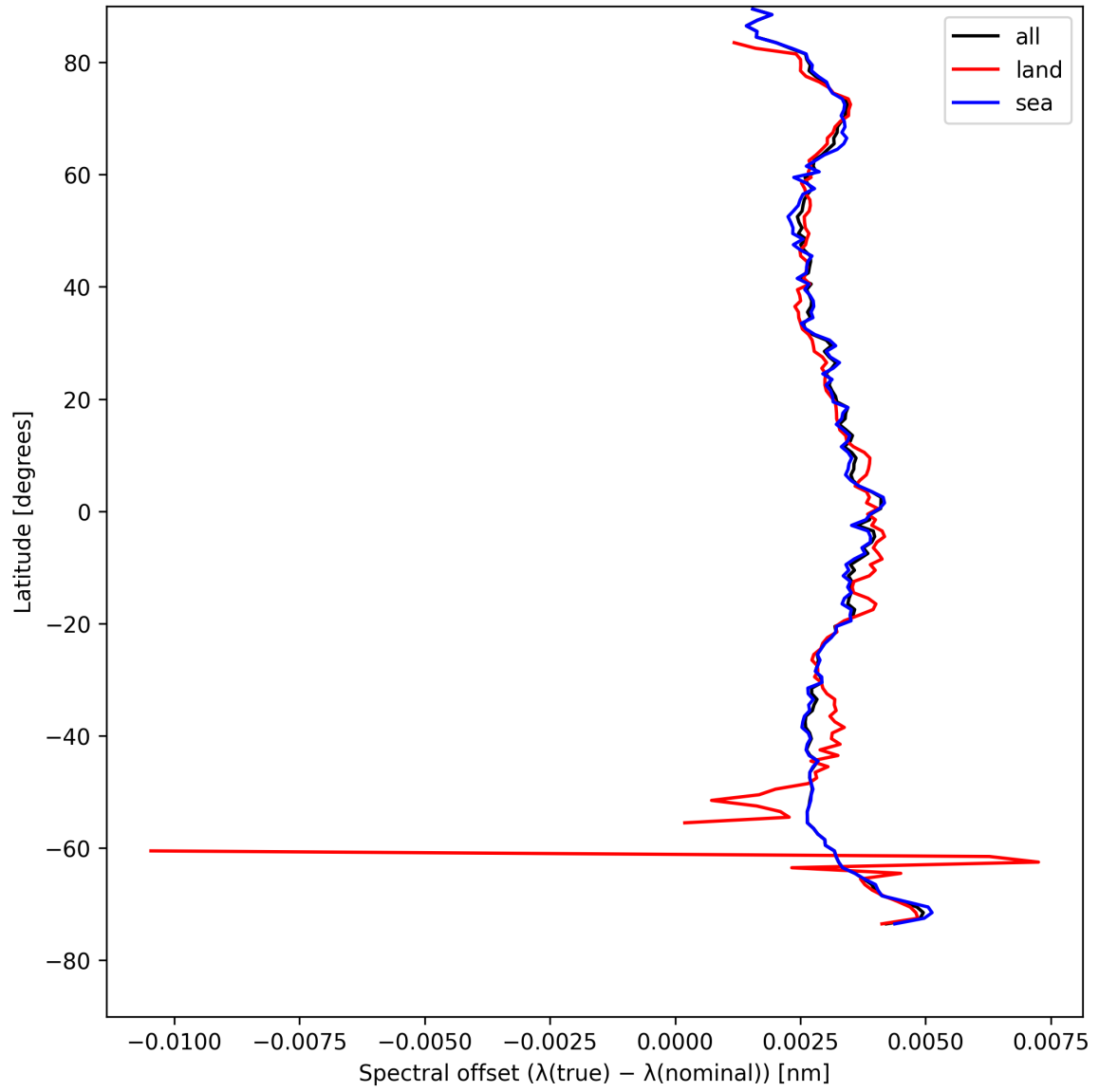
Figure 28: Zonal average of “Spectral offset ( \lambda_{\text{true}} - \lambda_{\text{nominal}} )” for 2025-04-27 to 2025-04-29.
