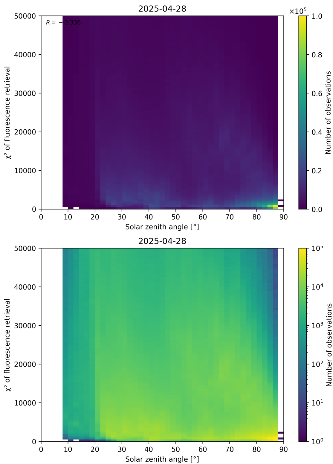
Figure 109: Scatter density plot of “Solar zenith angle” against “ \chi^2 of fluorescence retrieval” for 2025-04-27 to 2025-04-29.
