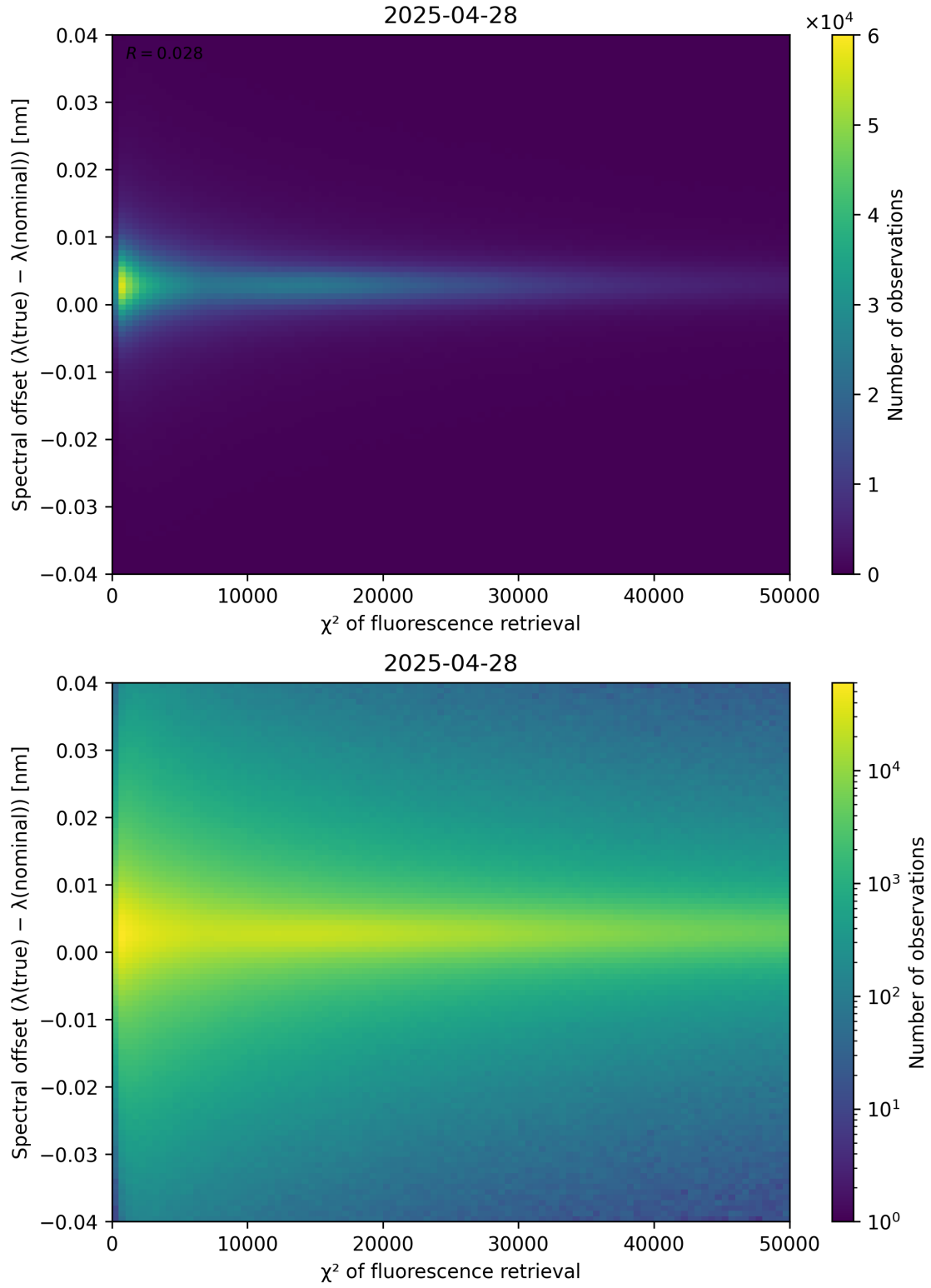
Figure 69: Scatter density plot of “ \chi^2 of fluorescence retrieval” against “Spectral offset ( \lambda_{\text{true}} - \lambda_{\text{nominal}} )” for 2025-04-27 to 2025-04-29.
