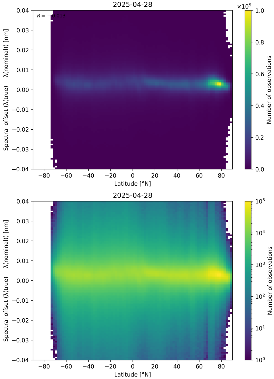
Figure 96: Scatter density plot of “Latitude” against “Spectral offset ( \lambda_{\text{true}} - \lambda_{\text{nominal}} )” for 2025-04-27 to 2025-04-29.
