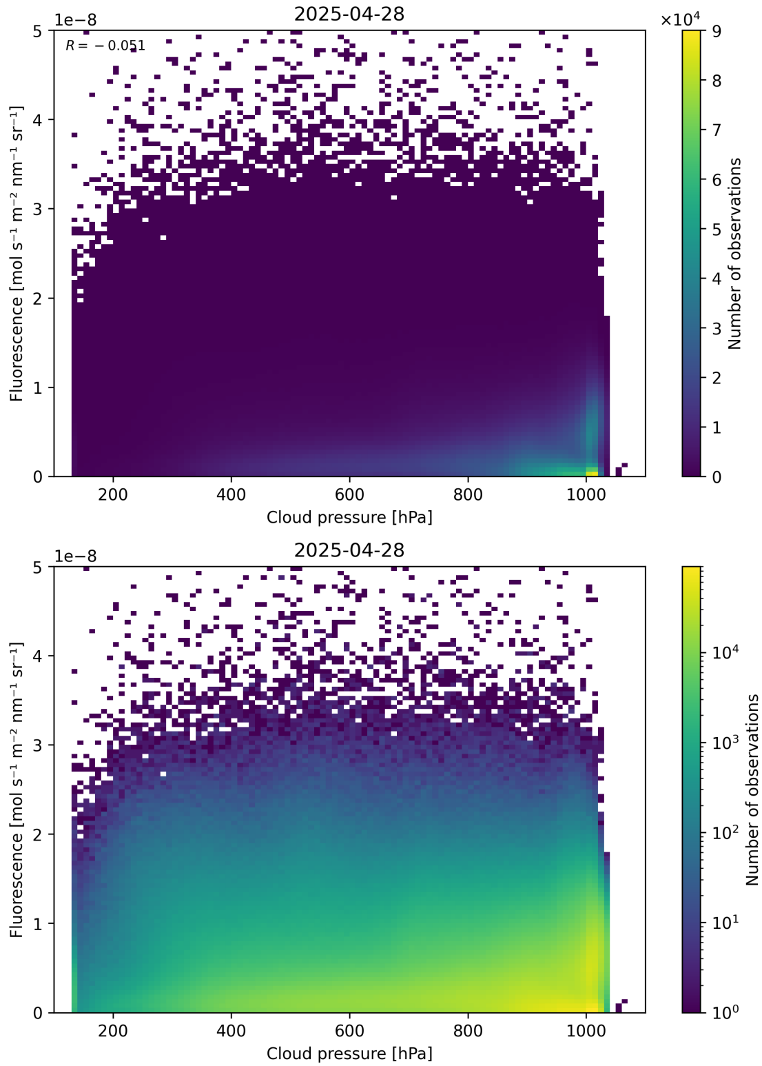
Figure 80: Scatter density plot of “Cloud pressure” against “Fluorescence” for 2025-04-27 to 2025-04-29.
