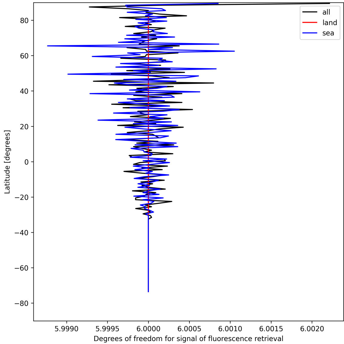
Figure 26: Zonal average of “Degrees of freedom for signal of fluorescence retrieval” for 2025-04-27 to 2025-04-29.
