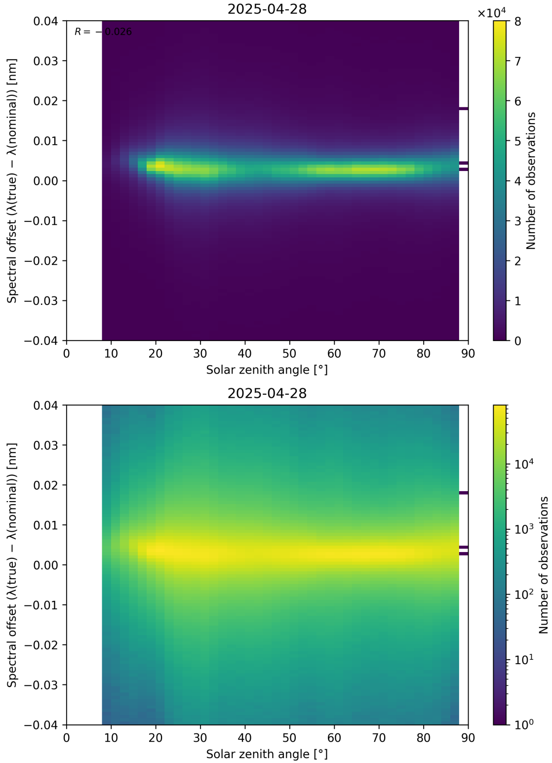
Figure 117: Scatter density plot of “Solar zenith angle” against “Spectral offset ( \lambda_{\text{true}} - \lambda_{\text{nominal}} )” for 2025-04-27 to 2025-04-29.
