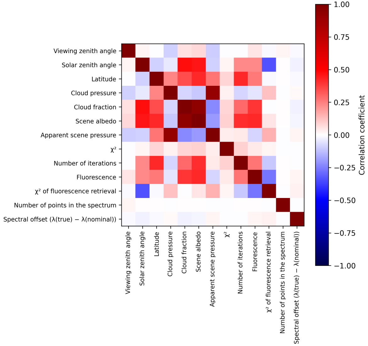
Figure 2: Map of correlation matrix for 2025-04-27 to 2025-04-29.
