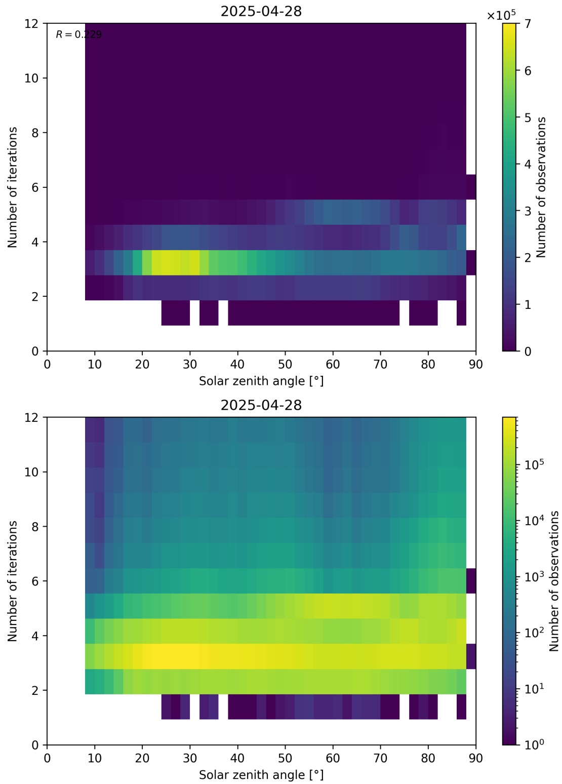
Figure 114: Scatter density plot of “Solar zenith angle” against “Number of iterations” for 2025-04-27 to 2025-04-29.
