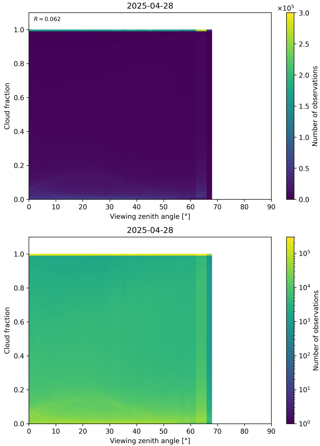
Figure 120: Scatter density plot of “Viewing zenith angle” against “Cloud fraction” for 2025-04-27 to 2025-04-29.
