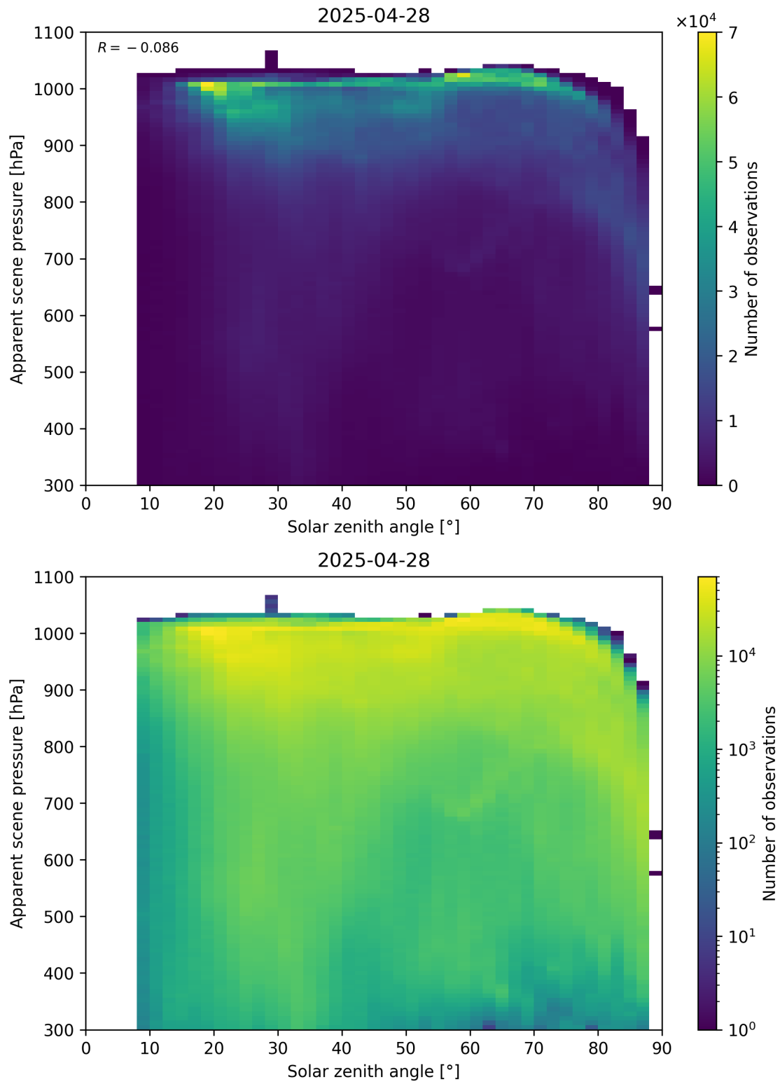
Figure 108: Scatter density plot of “Solar zenith angle” against “Apparent scene pressure” for 2025-04-27 to 2025-04-29.
