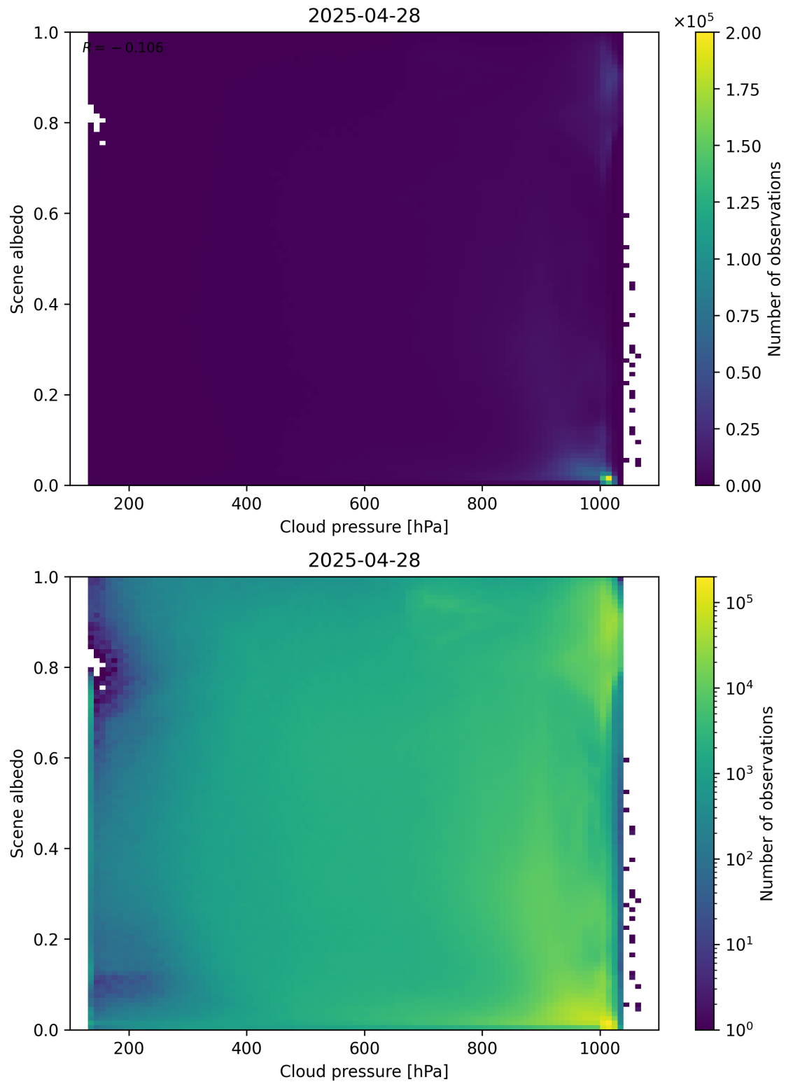
Figure 83: Scatter density plot of “Cloud pressure” against “Scene albedo” for 2025-04-27 to 2025-04-29.
