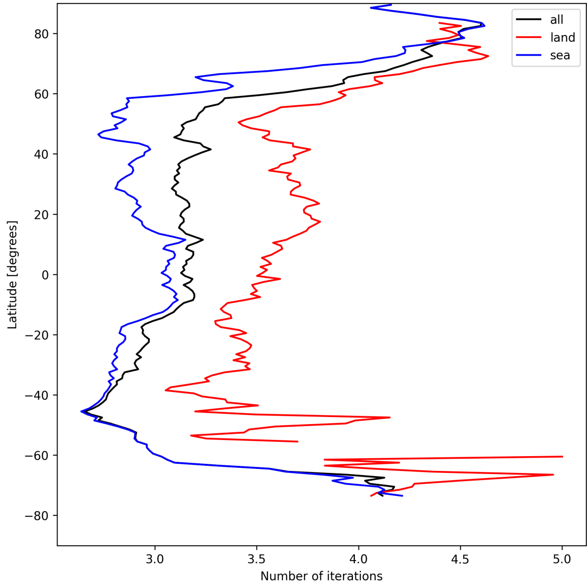
Figure 22: Zonal average of “Number of iterations” for 2025-04-27 to 2025-04-29.
