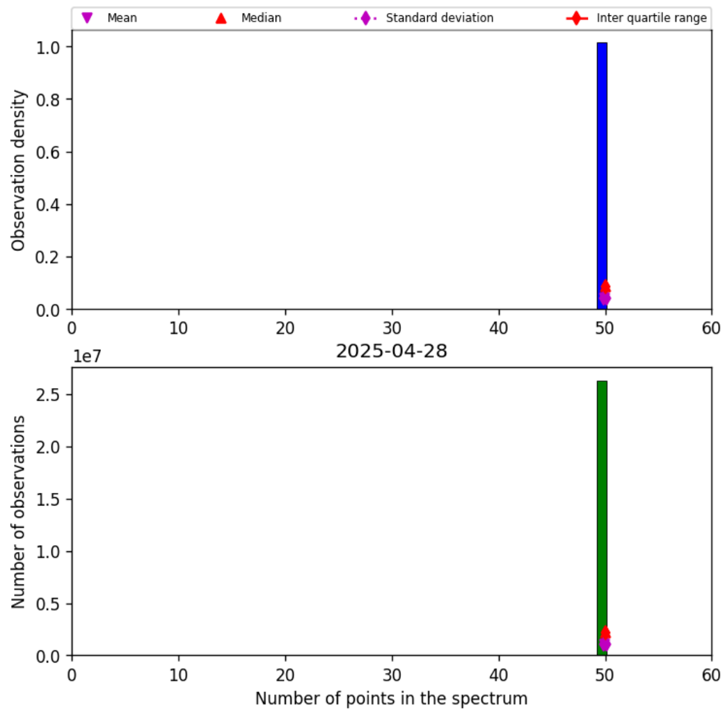
Figure 44: Histogram of “Number of points in the spectrum” for 2025-04-27 to 2025-04-29
