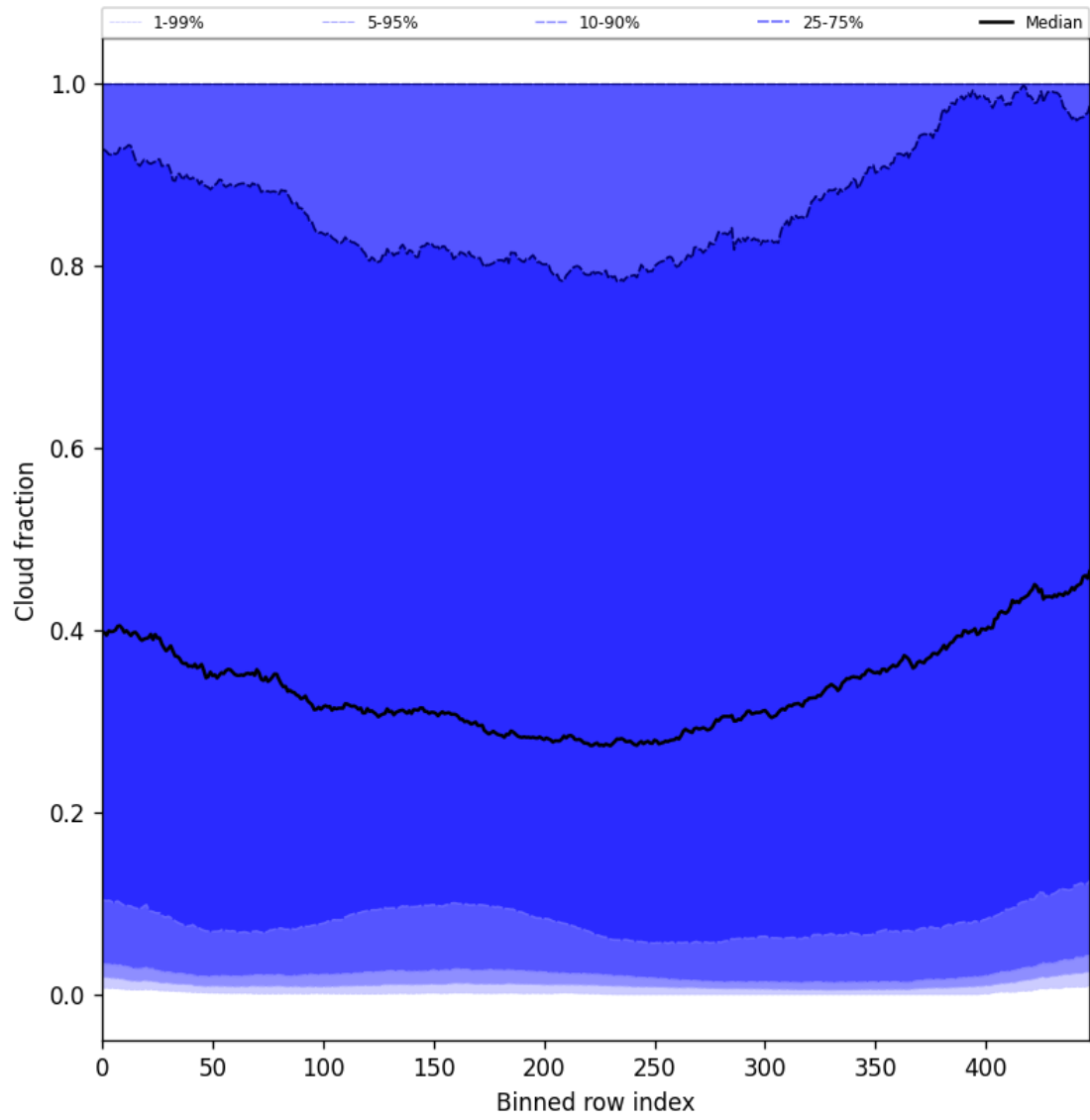
Figure 49: Along track statistics of “Cloud fraction” for 2025-04-27 to 2025-04-29
