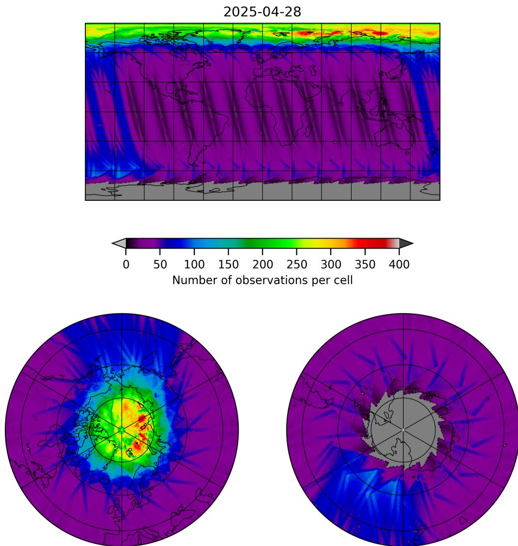
Figure 11: Map of the number of observations for 2025-04-27 to 2025-04-29
