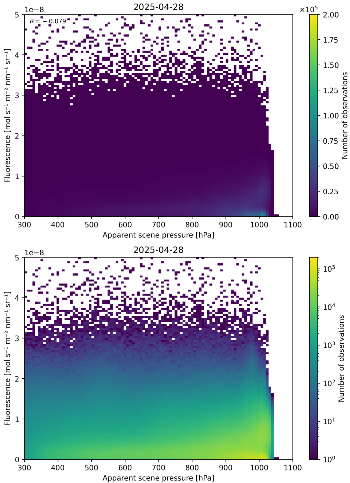
Figure 64: Scatter density plot of “Apparent scene pressure” against “Fluorescence” for 2025-04-27 to 2025-04-29.
