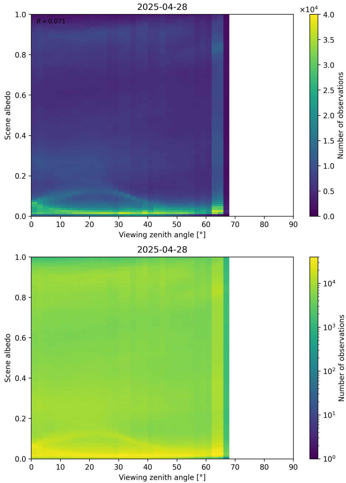
Figure 126: Scatter density plot of “Viewing zenith angle” against “Scene albedo” for 2025-04-27 to 2025-04-29.
