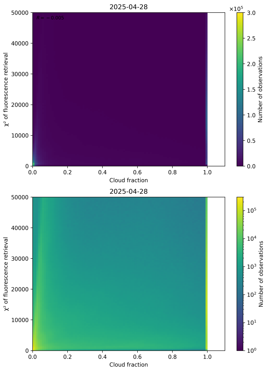
Figure 71: Scatter density plot of “Cloud fraction” against “ \chi^2 of fluorescence retrieval” for 2025-04-27 to 2025-04-29.
