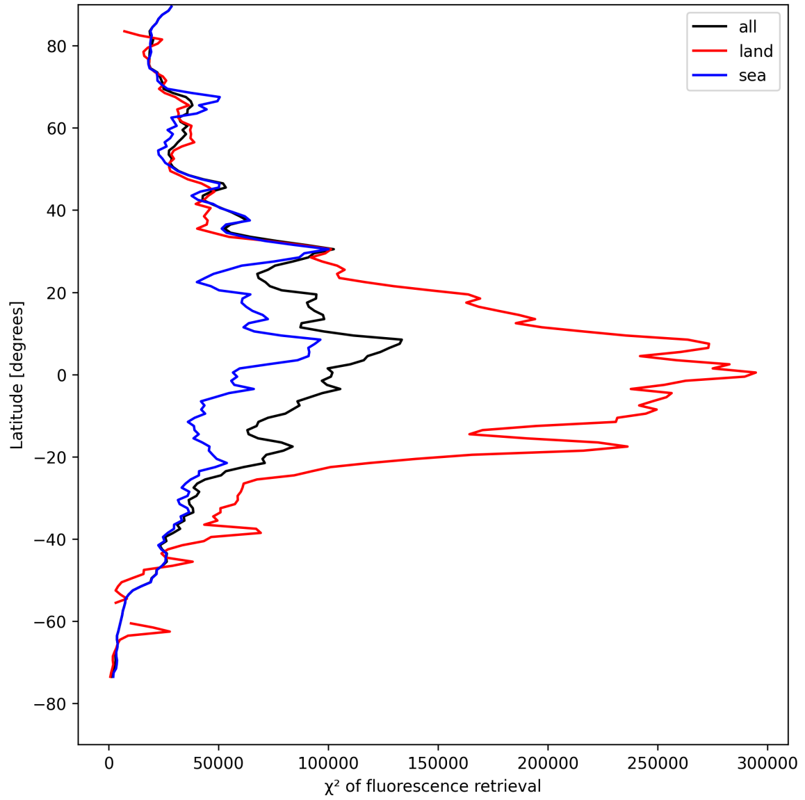
Figure 25: Zonal average of “ \chi^2 of fluorescence retrieval” for 2025-04-27 to 2025-04-29.
