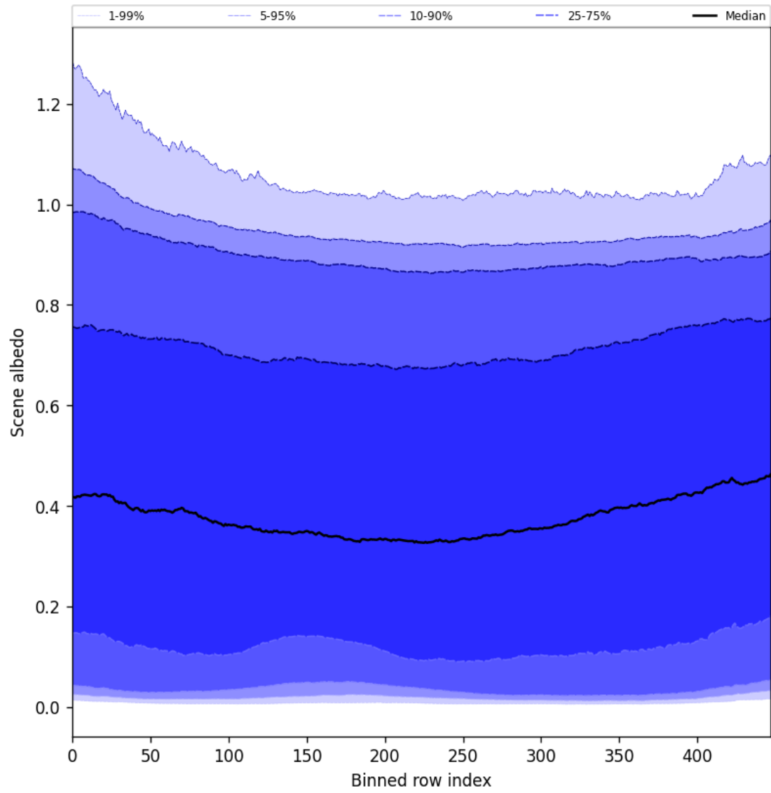
Figure 51: Along track statistics of “Scene albedo” for 2025-04-27 to 2025-04-29
