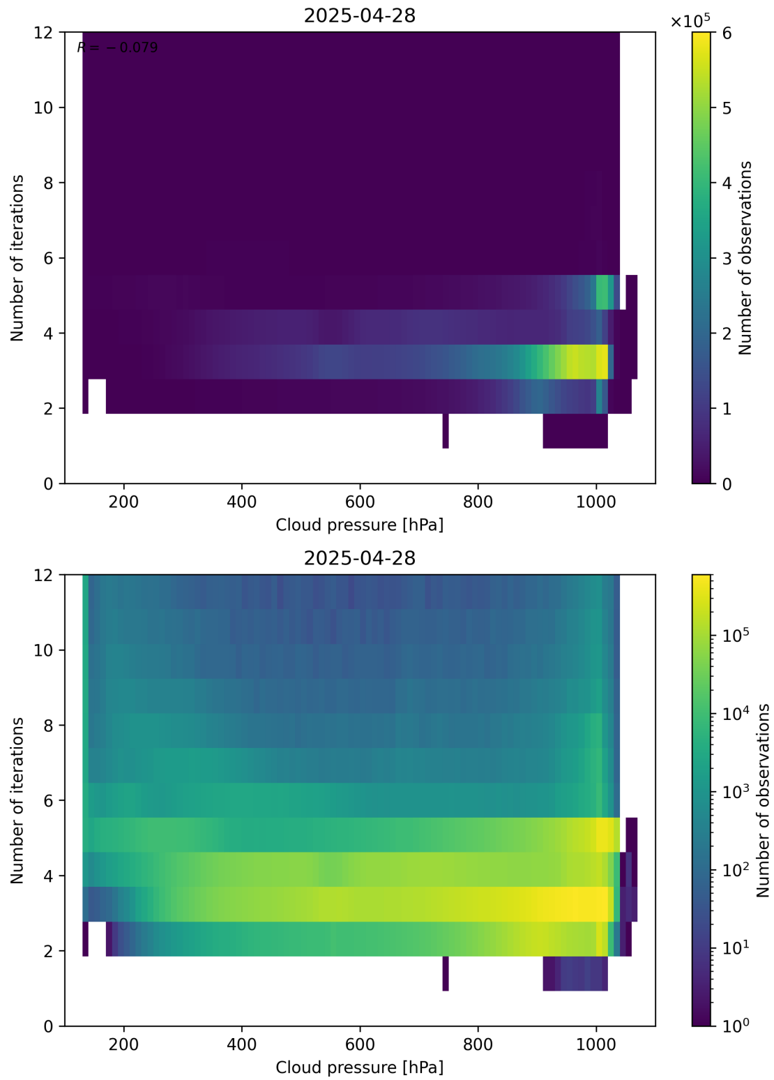
Figure 81: Scatter density plot of “Cloud pressure” against “Number of iterations” for 2025-04-27 to 2025-04-29.
