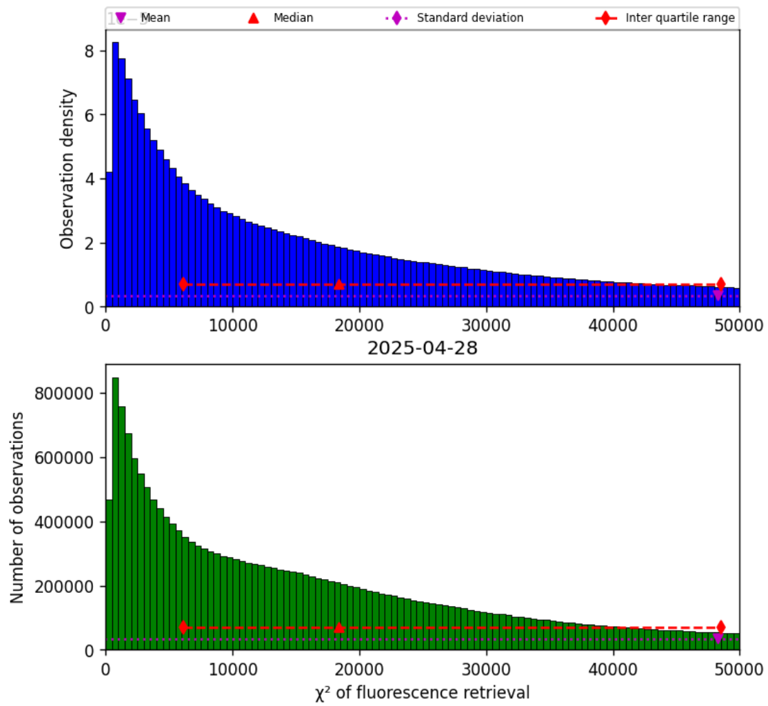
Figure 42: Histogram of “ \chi^2 of fluorescence retrieval” for 2025-04-27 to 2025-04-29
