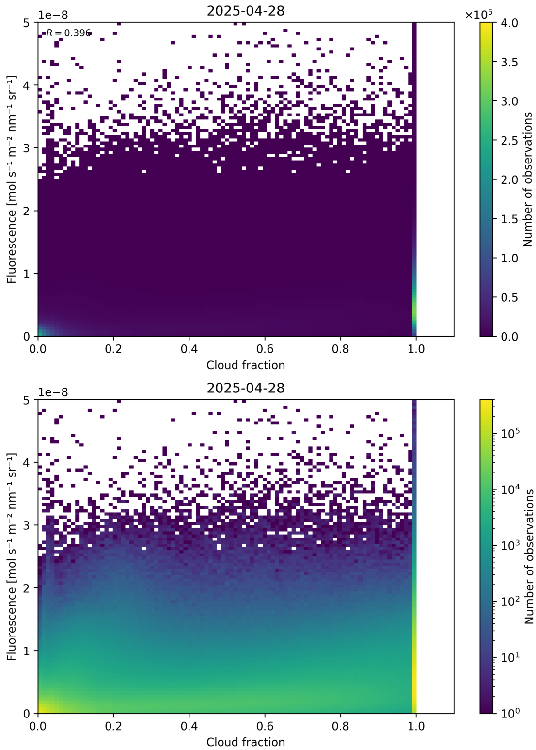
Figure 72: Scatter density plot of “Cloud fraction” against “Fluorescence” for 2025-04-27 to 2025-04-29.
