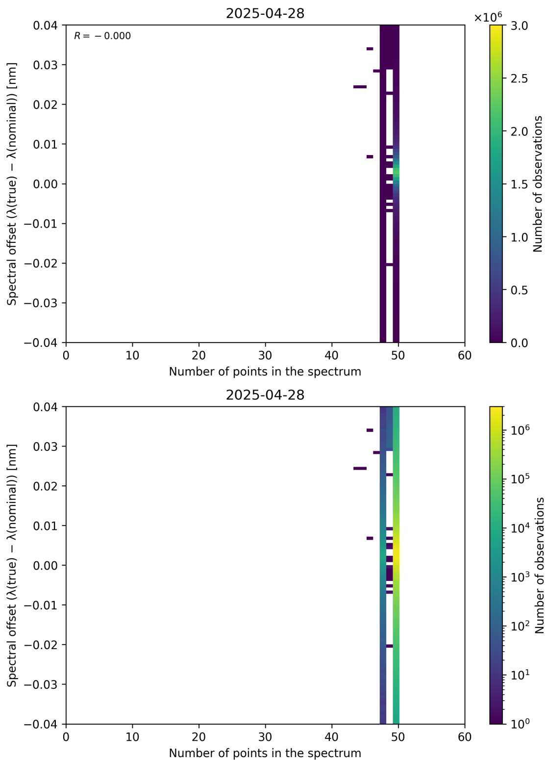
Figure 101: Scatter density plot of “Number of points in the spectrum” against “Spectral offset ( \lambda_{\text{true}} - \lambda_{\text{nominal}} )” for 2025-04-27 to 2025-04-29.
