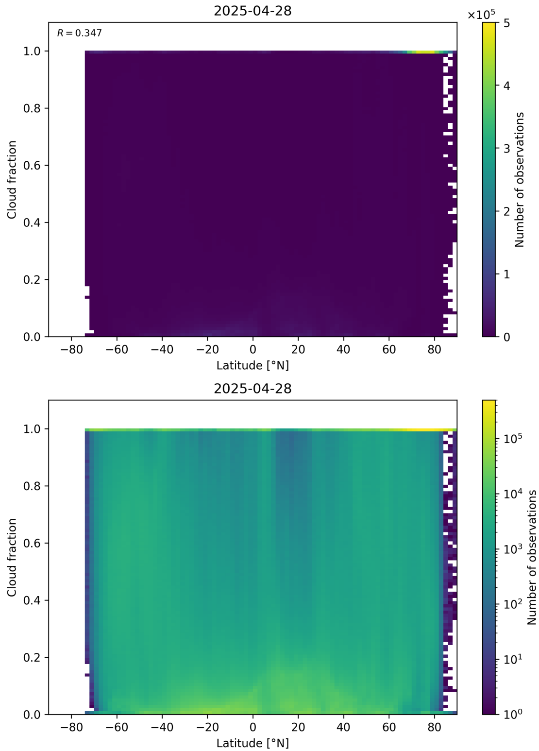
Figure 90: Scatter density plot of “Latitude” against “Cloud fraction” for 2025-04-27 to 2025-04-29.
