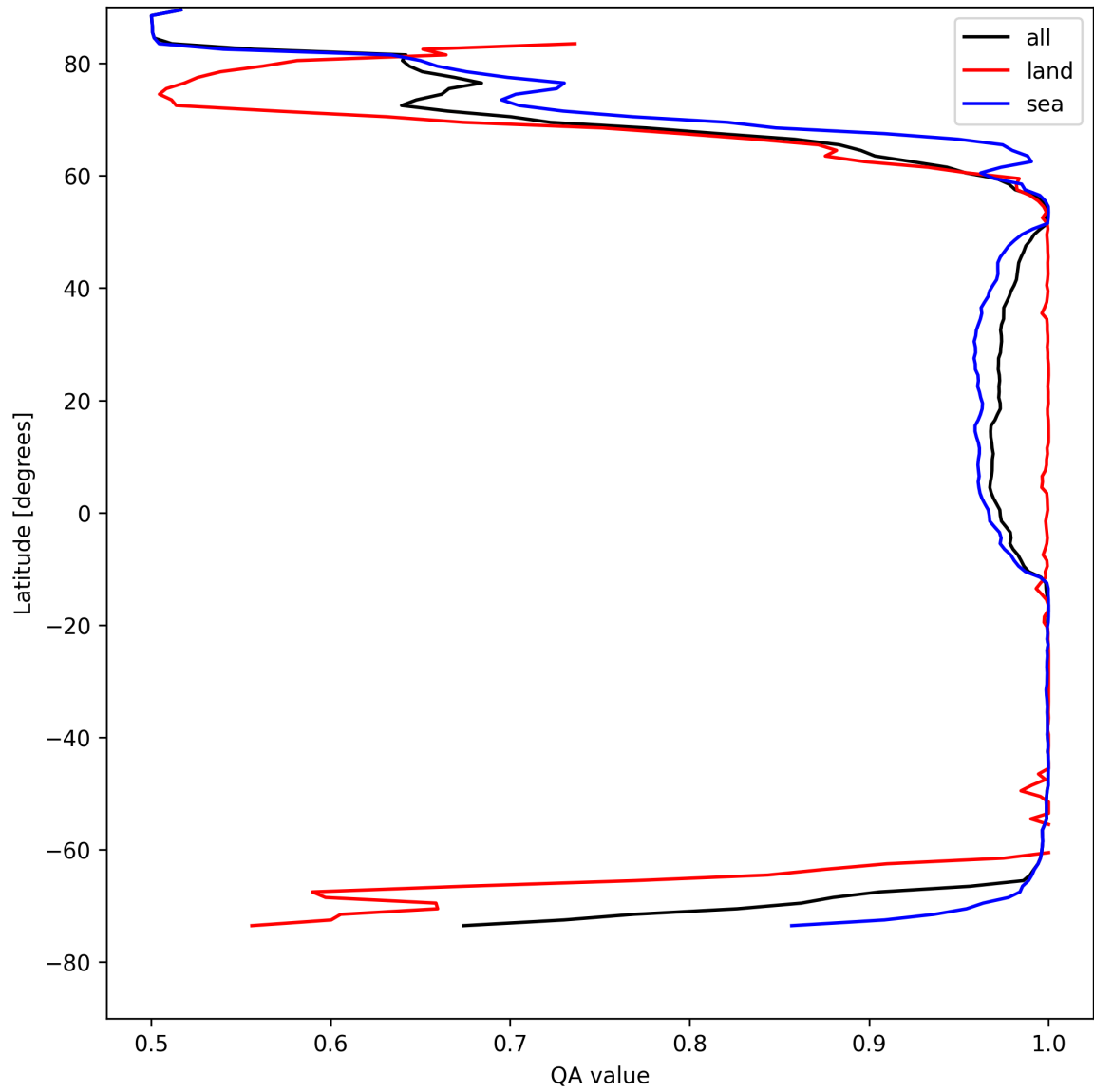
Figure 12: Zonal average of “QA value” for 2025-04-27 to 2025-04-29.
