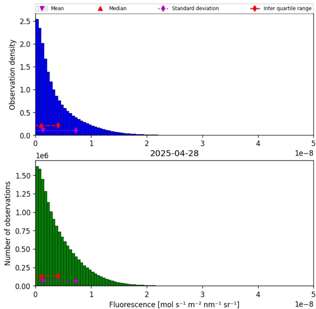
Figure 40: Histogram of “Fluorescence” for 2025-04-27 to 2025-04-29
