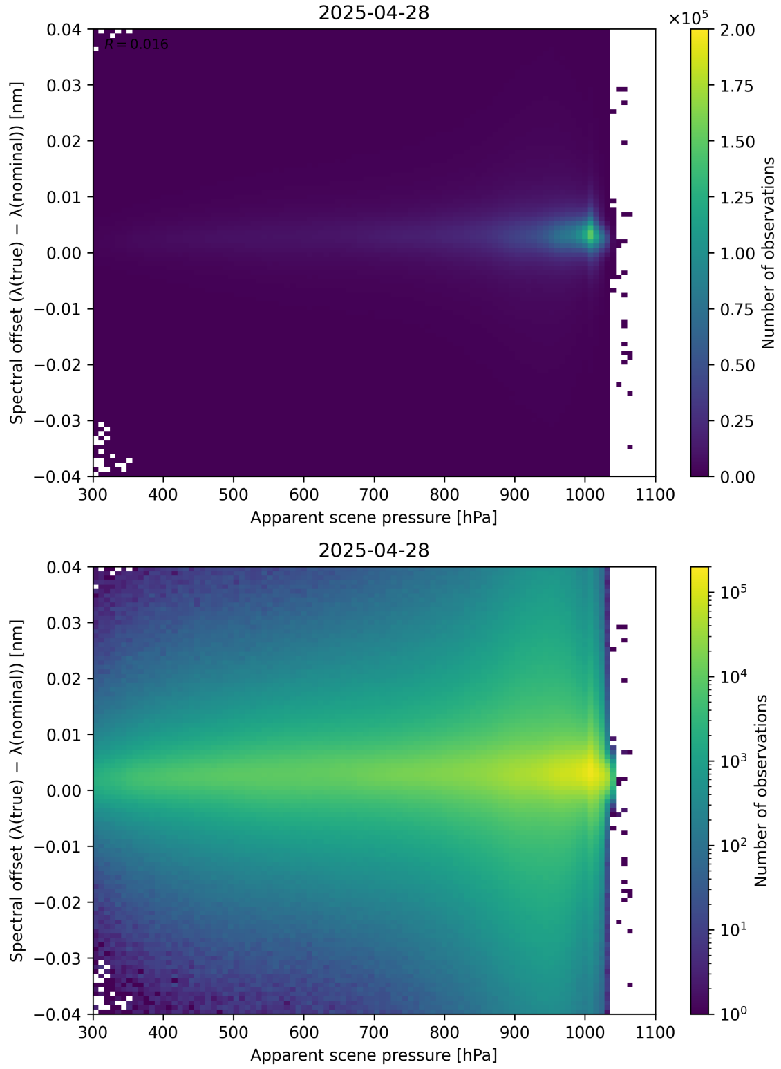
Figure 67: Scatter density plot of “Apparent scene pressure” against “Spectral offset ( \lambda_{\text{true}} - \lambda_{\text{nominal}} )” for 2025-04-27 to 2025-04-29.
