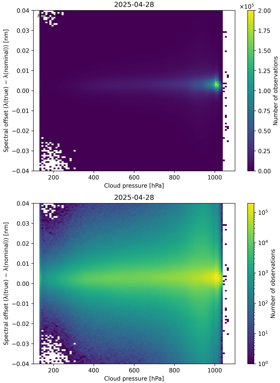
Figure 84: Scatter density plot of “Cloud pressure” against “Spectral offset ( \lambda_{\text{true}} - \lambda_{\text{nominal}} )” for 2025-04-27 to 2025-04-29.
