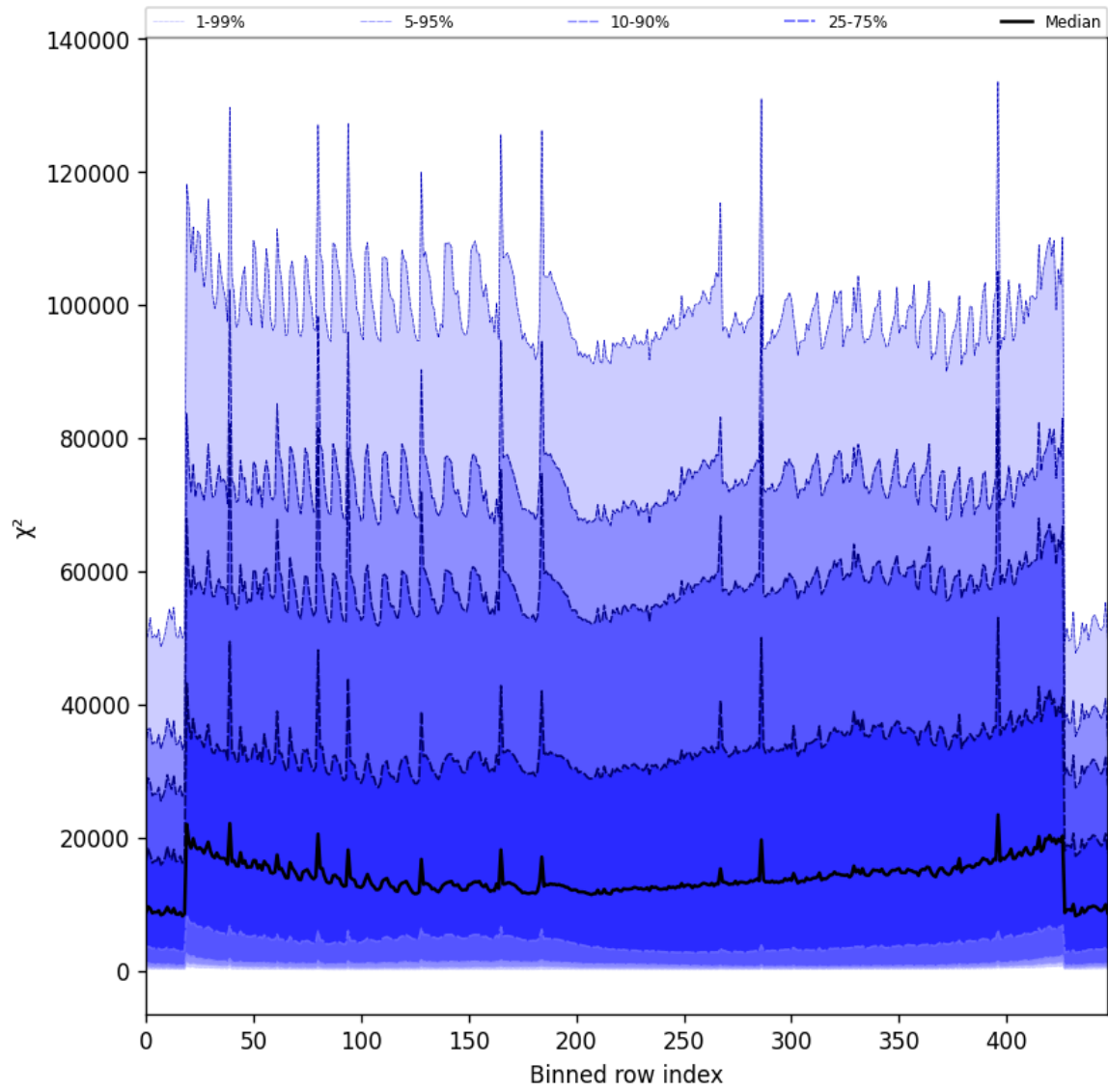
Figure 55: Along track statistics of “ \chi^2 ” for 2025-04-27 to 2025-04-29
