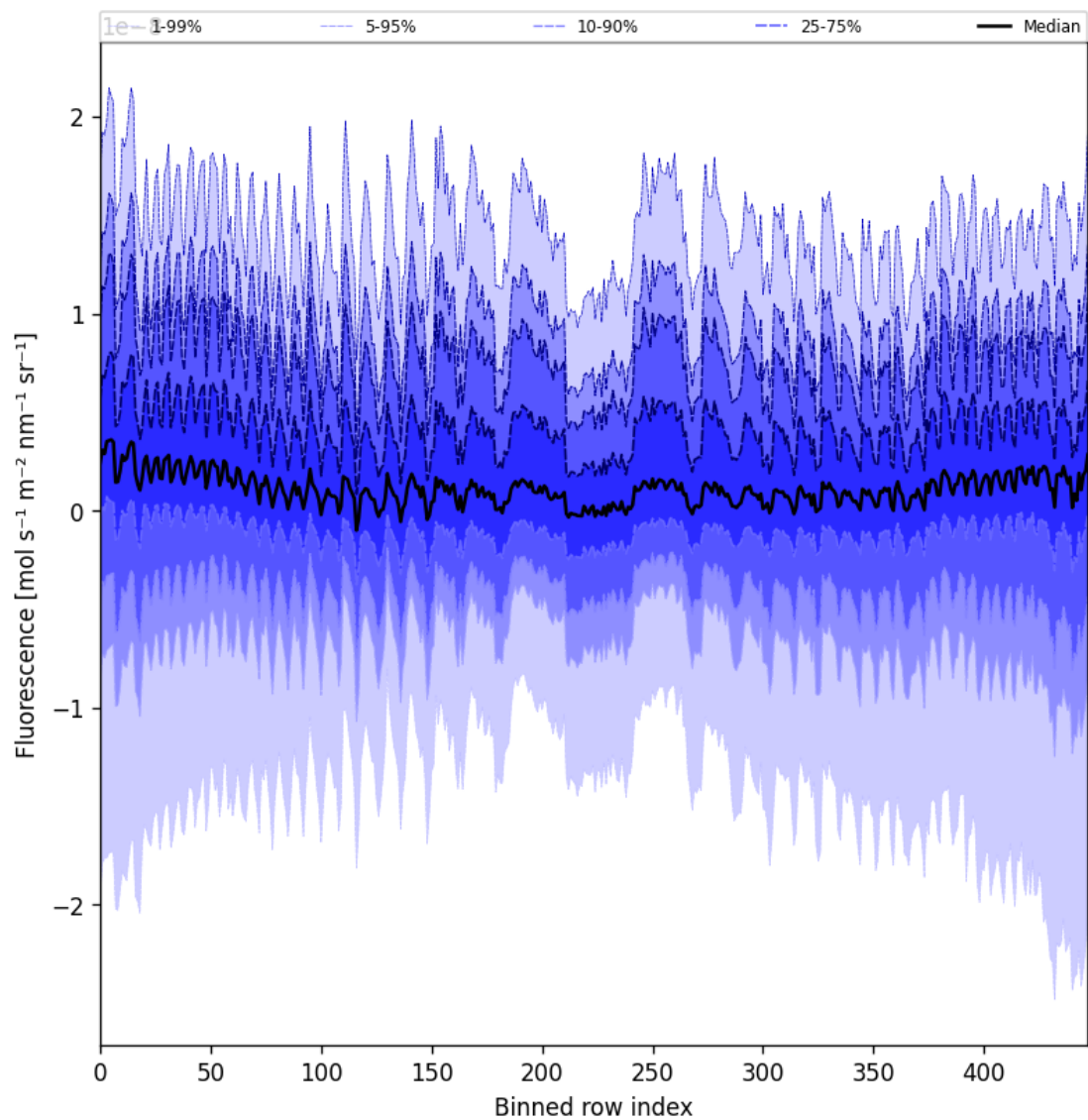
Figure 57: Along track statistics of “Fluorescence” for 2025-04-27 to 2025-04-29
