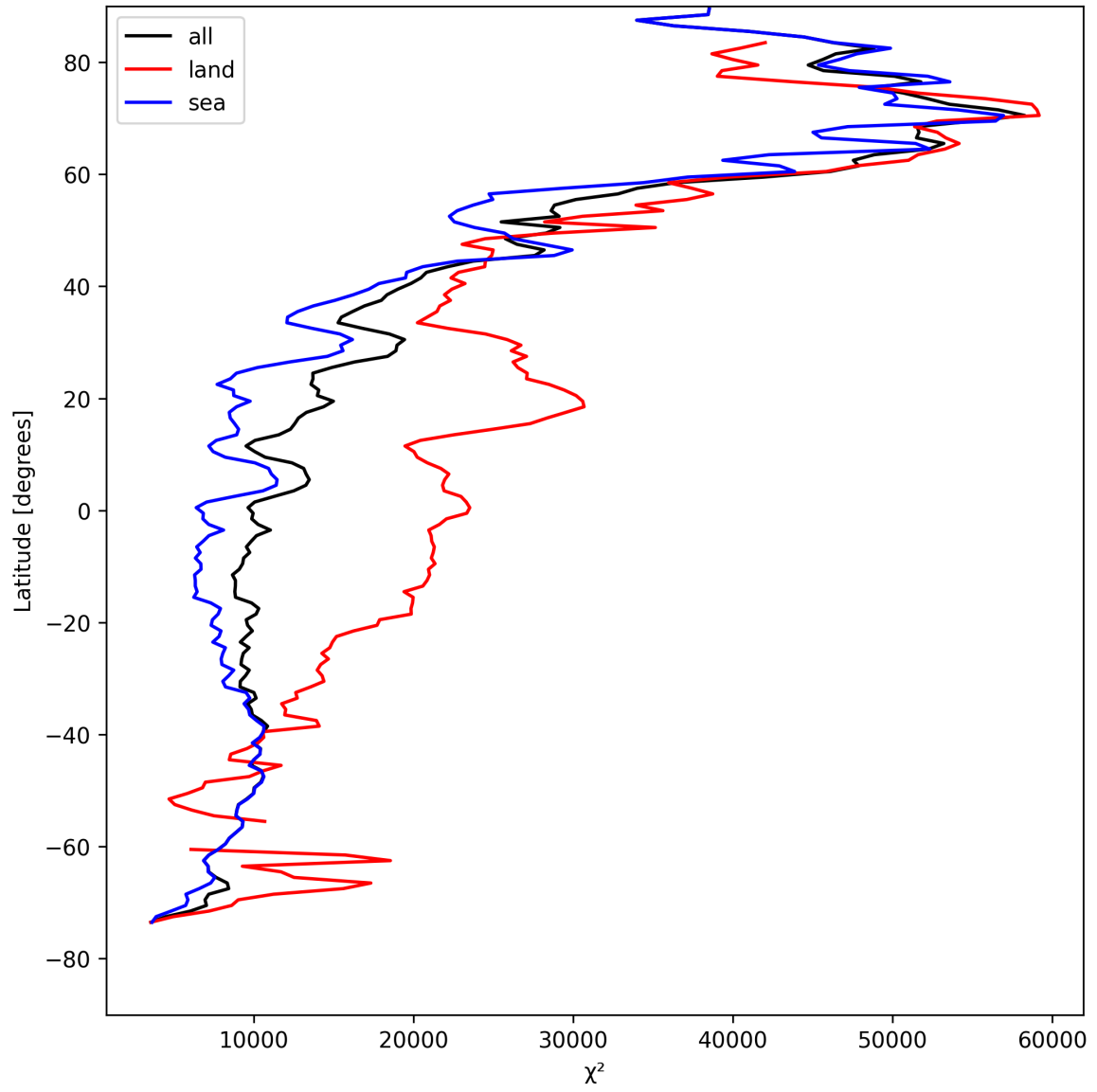
Figure 21: Zonal average of “ \chi^2 ” for 2025-04-27 to 2025-04-29.
