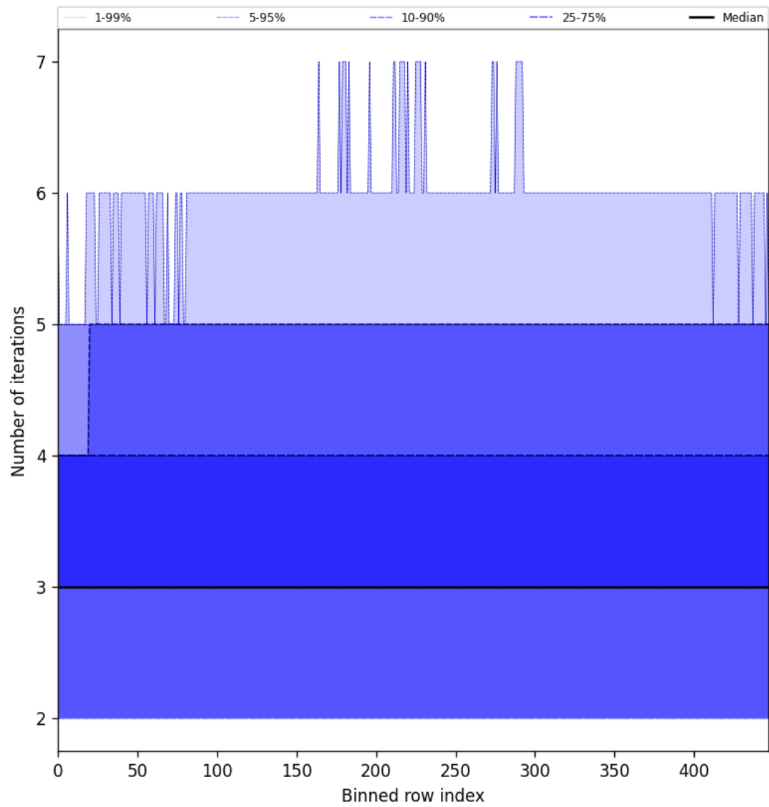
Figure 56: Along track statistics of “Number of iterations” for 2025-04-27 to 2025-04-29
