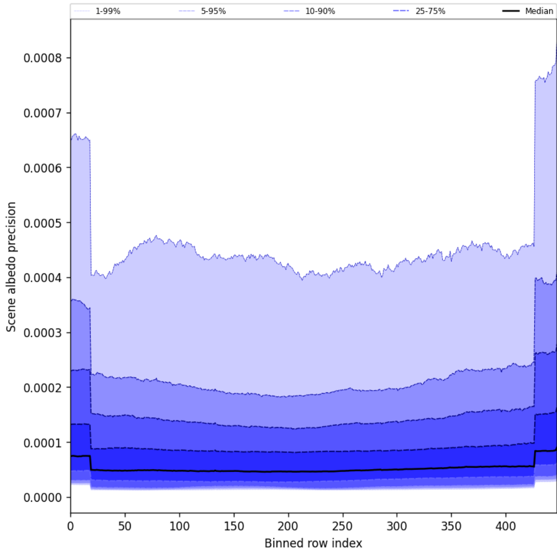
Figure 52: Along track statistics of “Scene albedo precision” for 2025-04-27 to 2025-04-29
