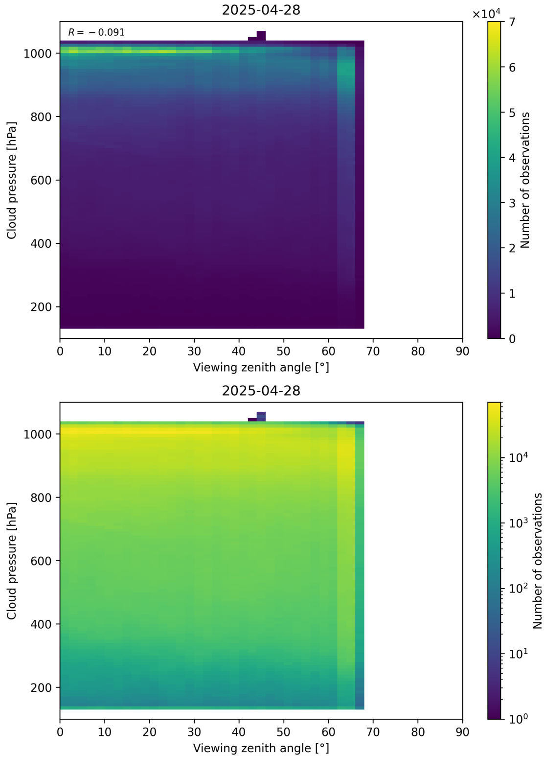
Figure 121: Scatter density plot of “Viewing zenith angle” against “Cloud pressure” for 2025-04-27 to 2025-04-29.
