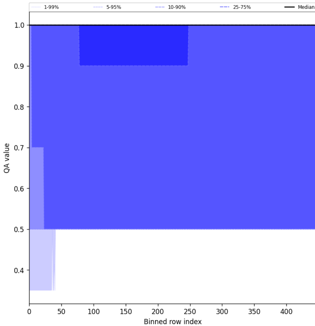
Figure 46: Along track statistics of “QA value” for 2025-04-27 to 2025-04-29
