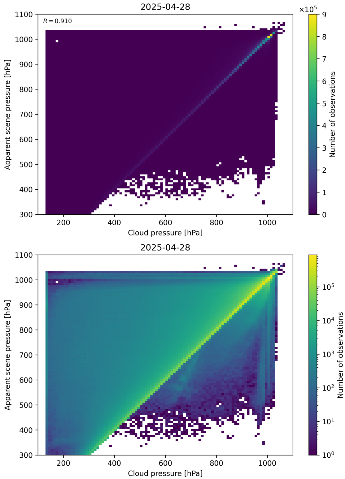
Figure 77: Scatter density plot of “Cloud pressure” against “Apparent scene pressure” for 2025-04-27 to 2025-04-29.
