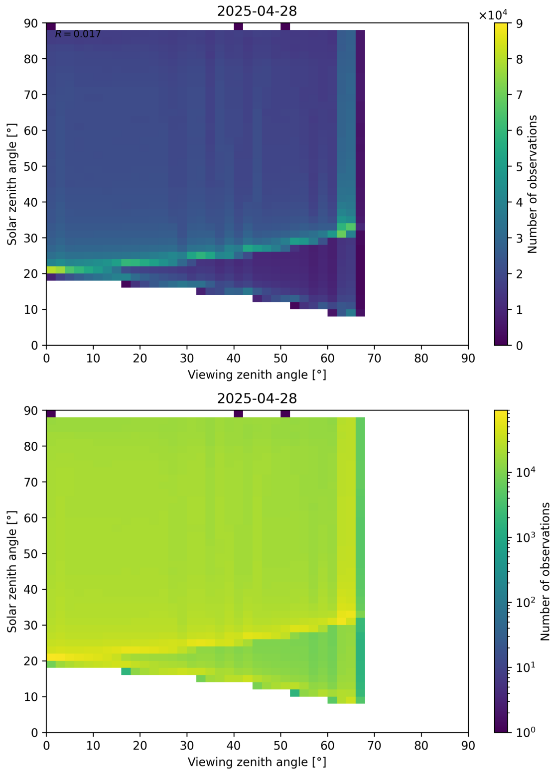
Figure 127: Scatter density plot of “Viewing zenith angle” against “Solar zenith angle” for 2025-04-27 to 2025-04-29.
