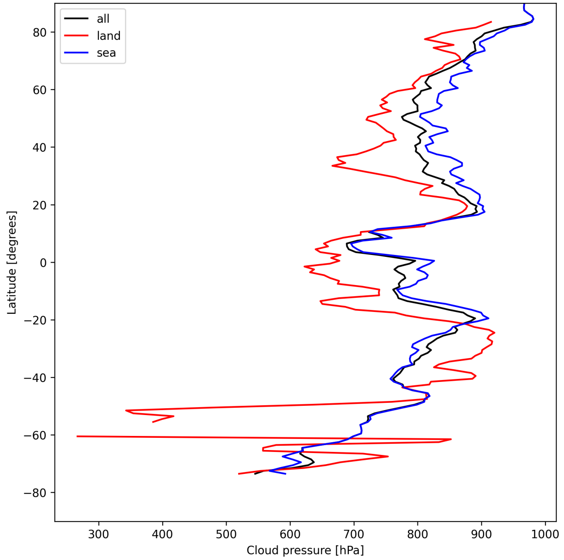
Figure 13: Zonal average of “Cloud pressure” for 2025-04-27 to 2025-04-29.
