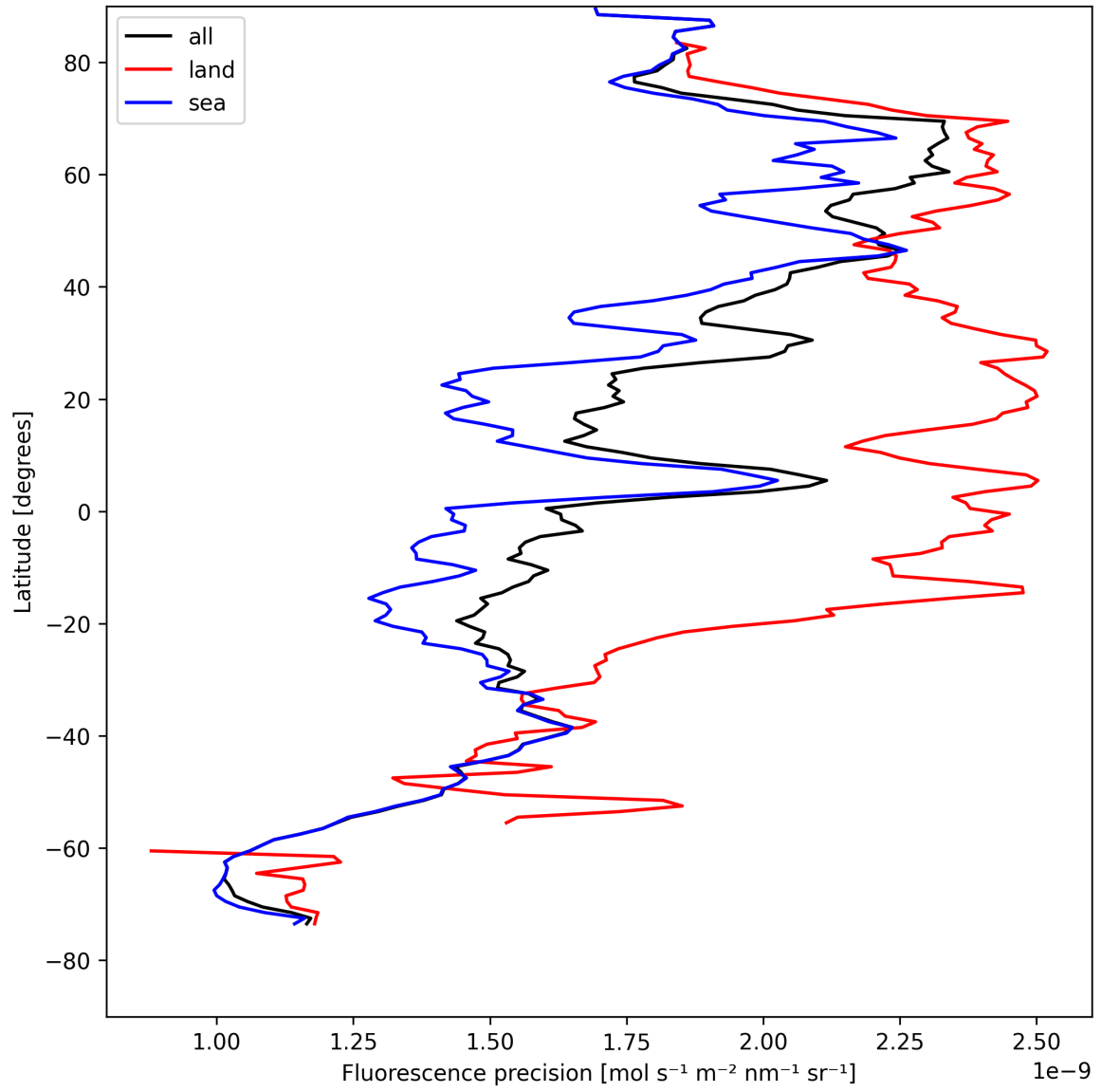
Figure 24: Zonal average of “Fluorescence precision” for 2025-04-27 to 2025-04-29.
