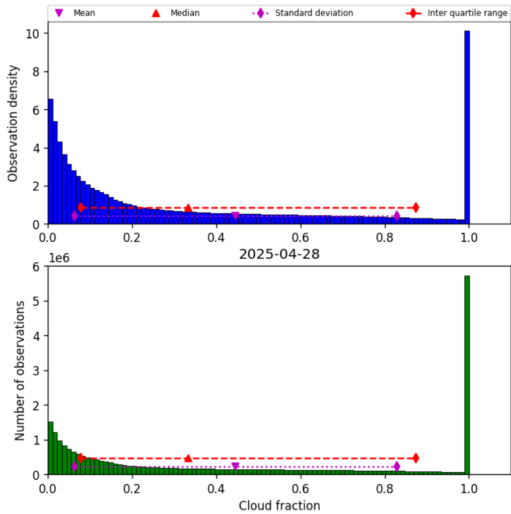
Figure 32: Histogram of “Cloud fraction” for 2025-04-27 to 2025-04-29
