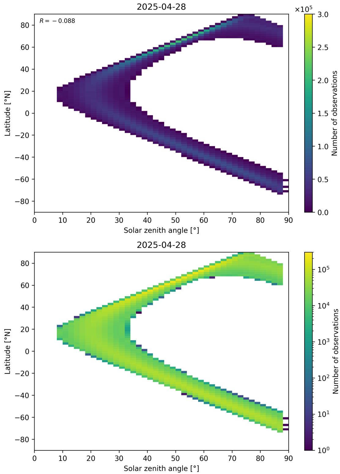
Figure 113: Scatter density plot of “Solar zenith angle” against “Latitude” for 2025-04-27 to 2025-04-29.
