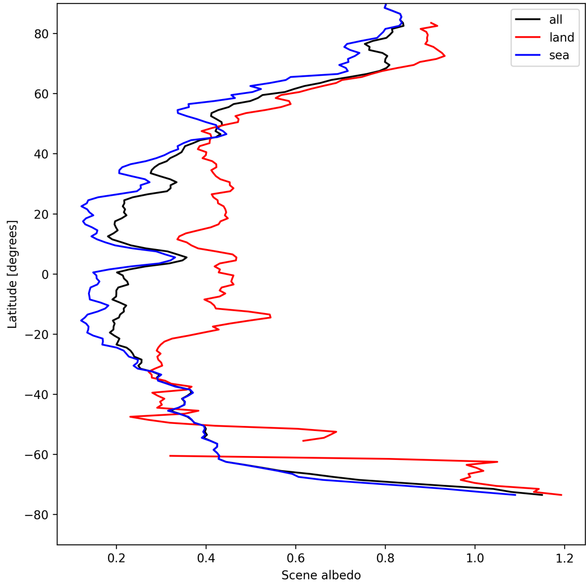
Figure 17: Zonal average of “Scene albedo” for 2025-04-27 to 2025-04-29.
