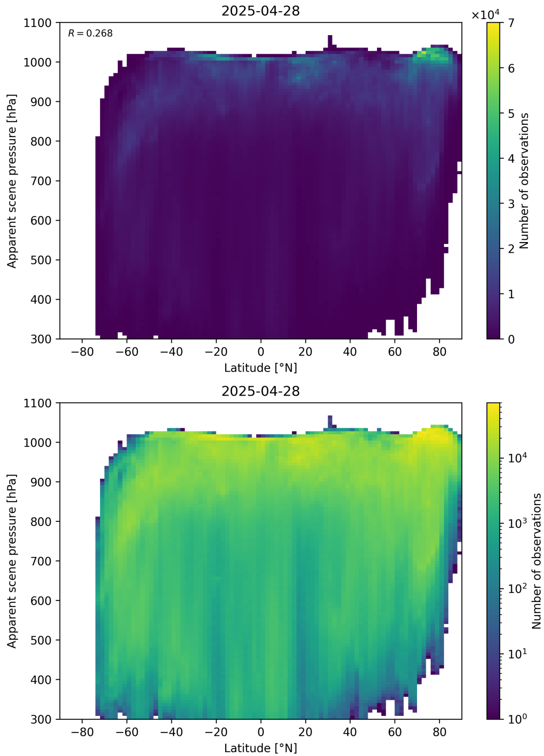
Figure 88: Scatter density plot of “Latitude” against “Apparent scene pressure” for 2025-04-27 to 2025-04-29.
