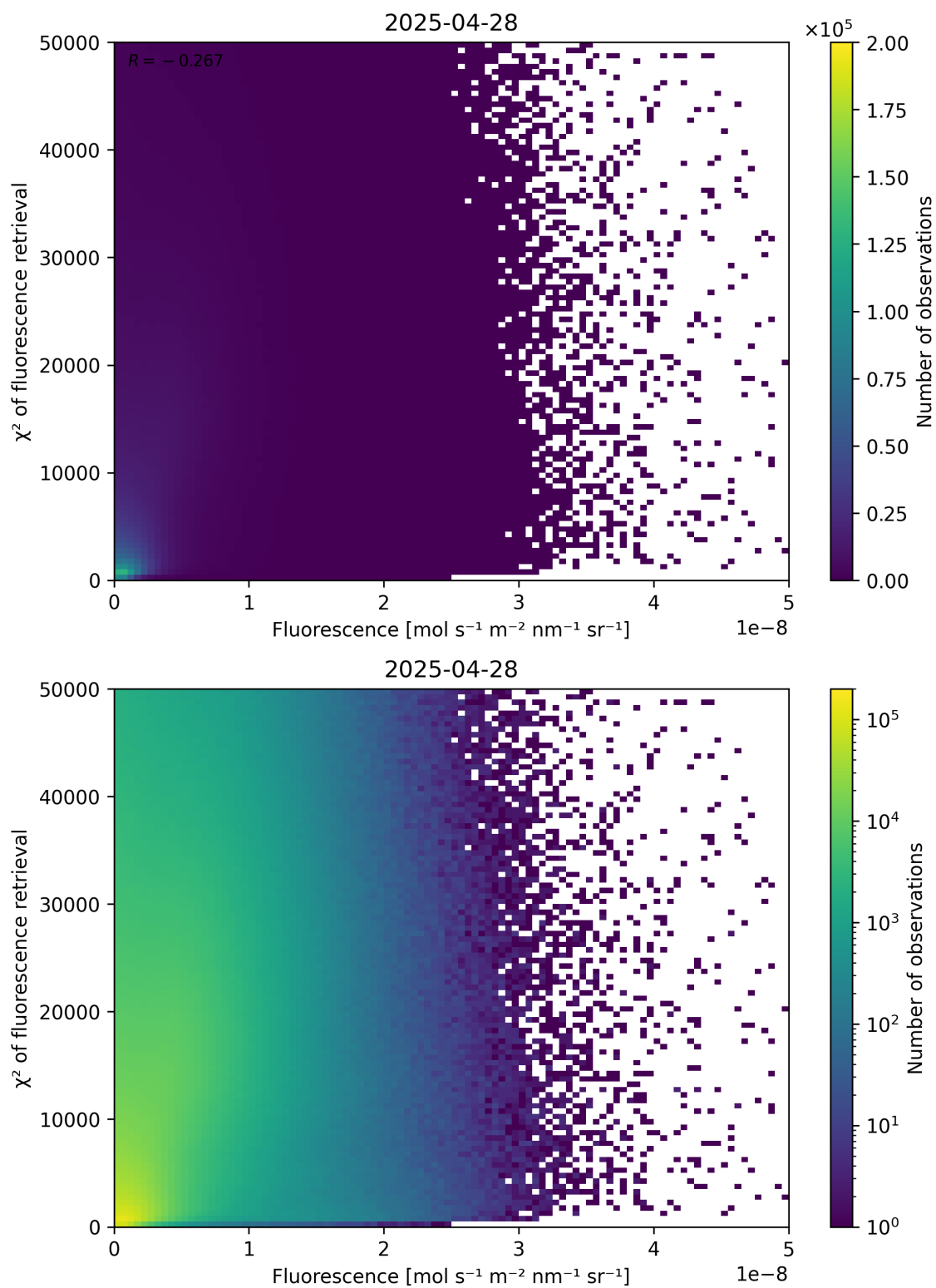
Figure 85: Scatter density plot of “Fluorescence” against “ \chi^2 of fluorescence retrieval” for 2025-04-27 to 2025-04-29.
