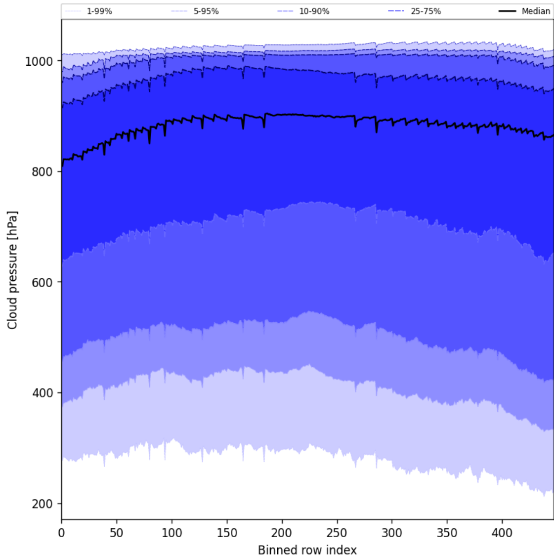
Figure 47: Along track statistics of “Cloud pressure” for 2025-04-27 to 2025-04-29
