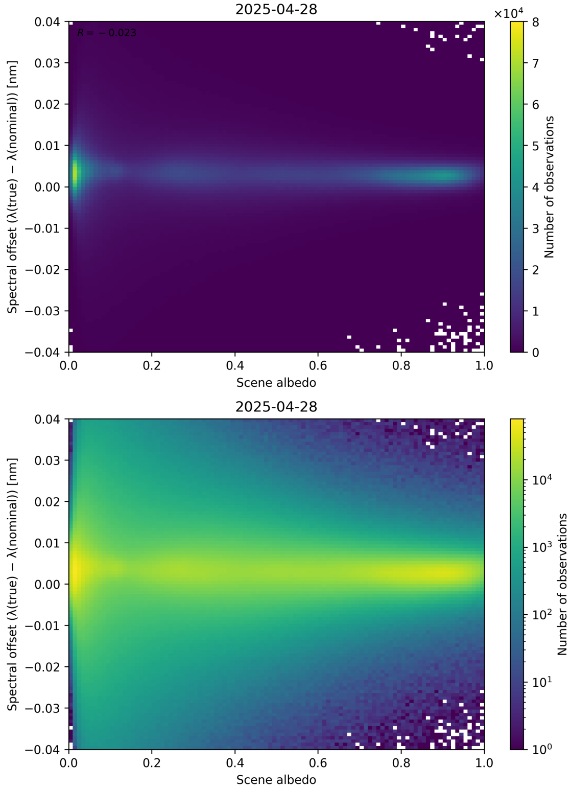
Figure 107: Scatter density plot of “Scene albedo” against “Spectral offset ( \lambda_{\text{true}} - \lambda_{\text{nominal}} )” for 2025-04-27 to 2025-04-29.
