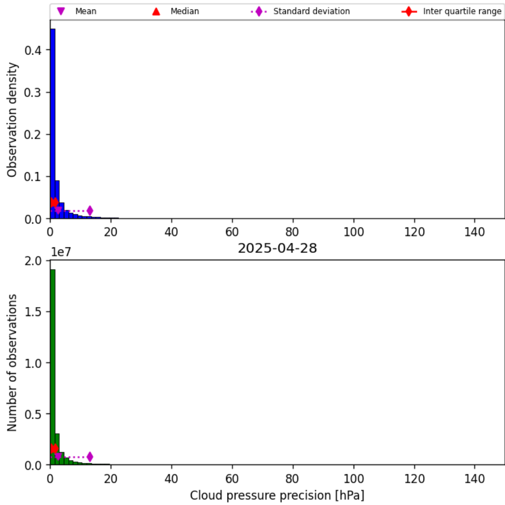
Figure 31: Histogram of “Cloud pressure precision” for 2025-04-27 to 2025-04-29
