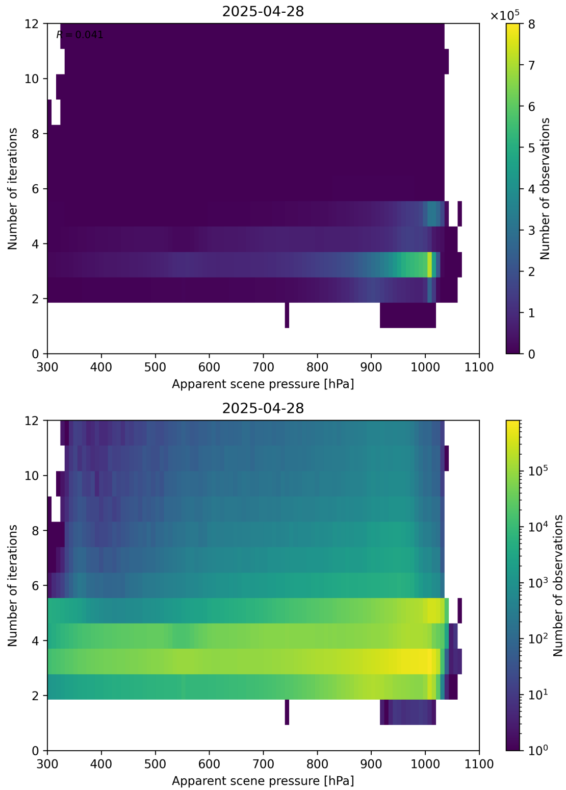
Figure 65: Scatter density plot of “Apparent scene pressure” against “Number of iterations” for 2025-04-27 to 2025-04-29.
