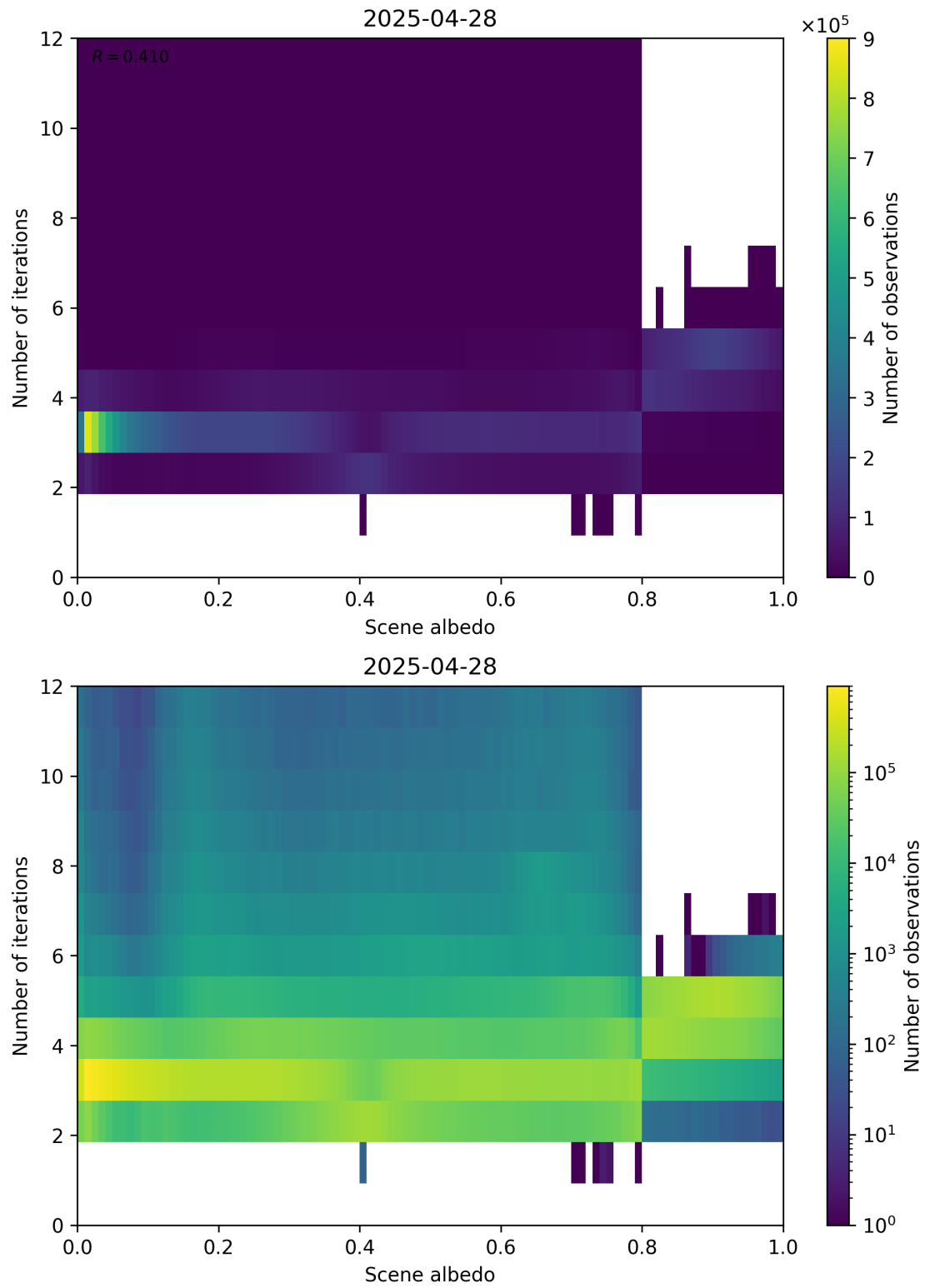
Figure 105: Scatter density plot of “Scene albedo” against “Number of iterations” for 2025-04-27 to 2025-04-29.
