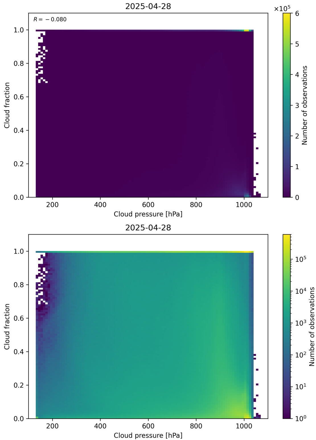
Figure 79: Scatter density plot of “Cloud pressure” against “Cloud fraction” for 2025-04-27 to 2025-04-29.
