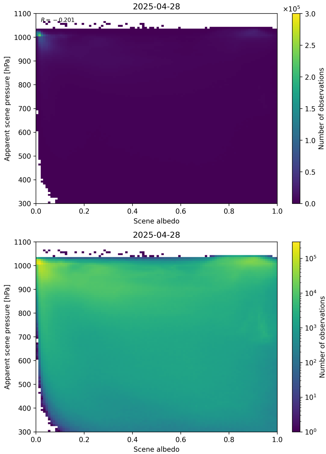
Figure 102: Scatter density plot of “Scene albedo” against “Apparent scene pressure” for 2025-04-27 to 2025-04-29.
