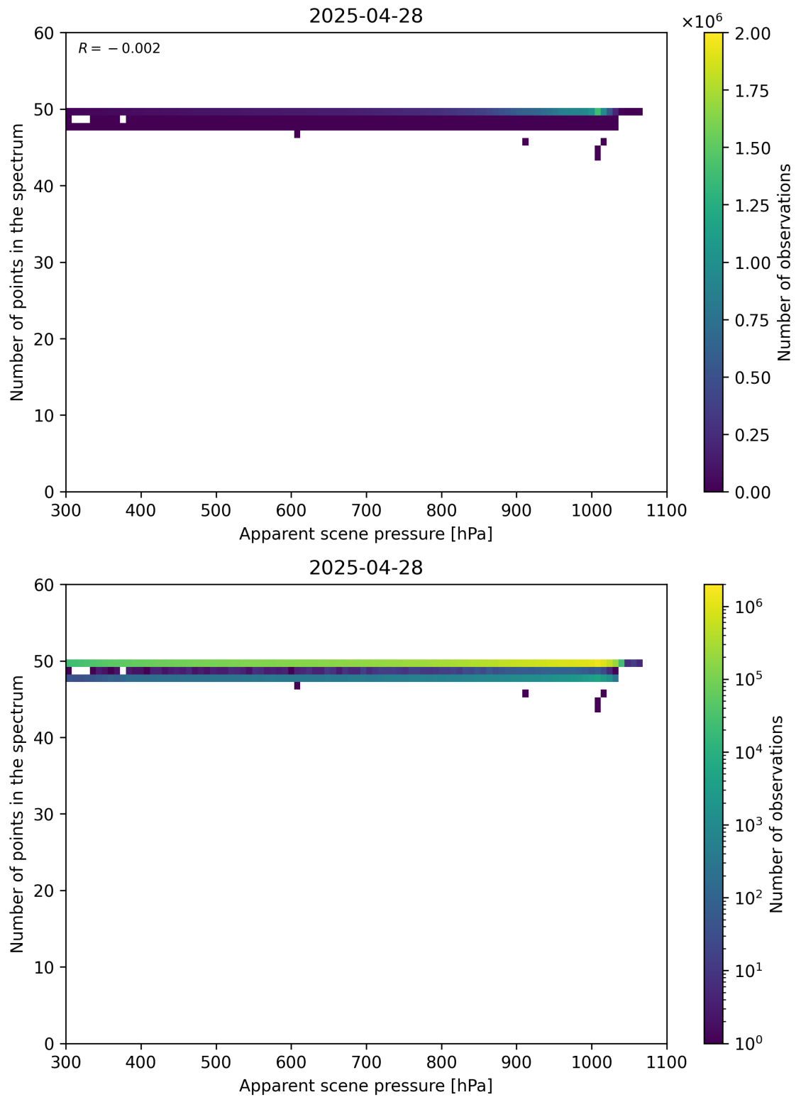
Figure 66: Scatter density plot of “Apparent scene pressure” against “Number of points in the spectrum” for 2025-04-27 to 2025-04-29.
