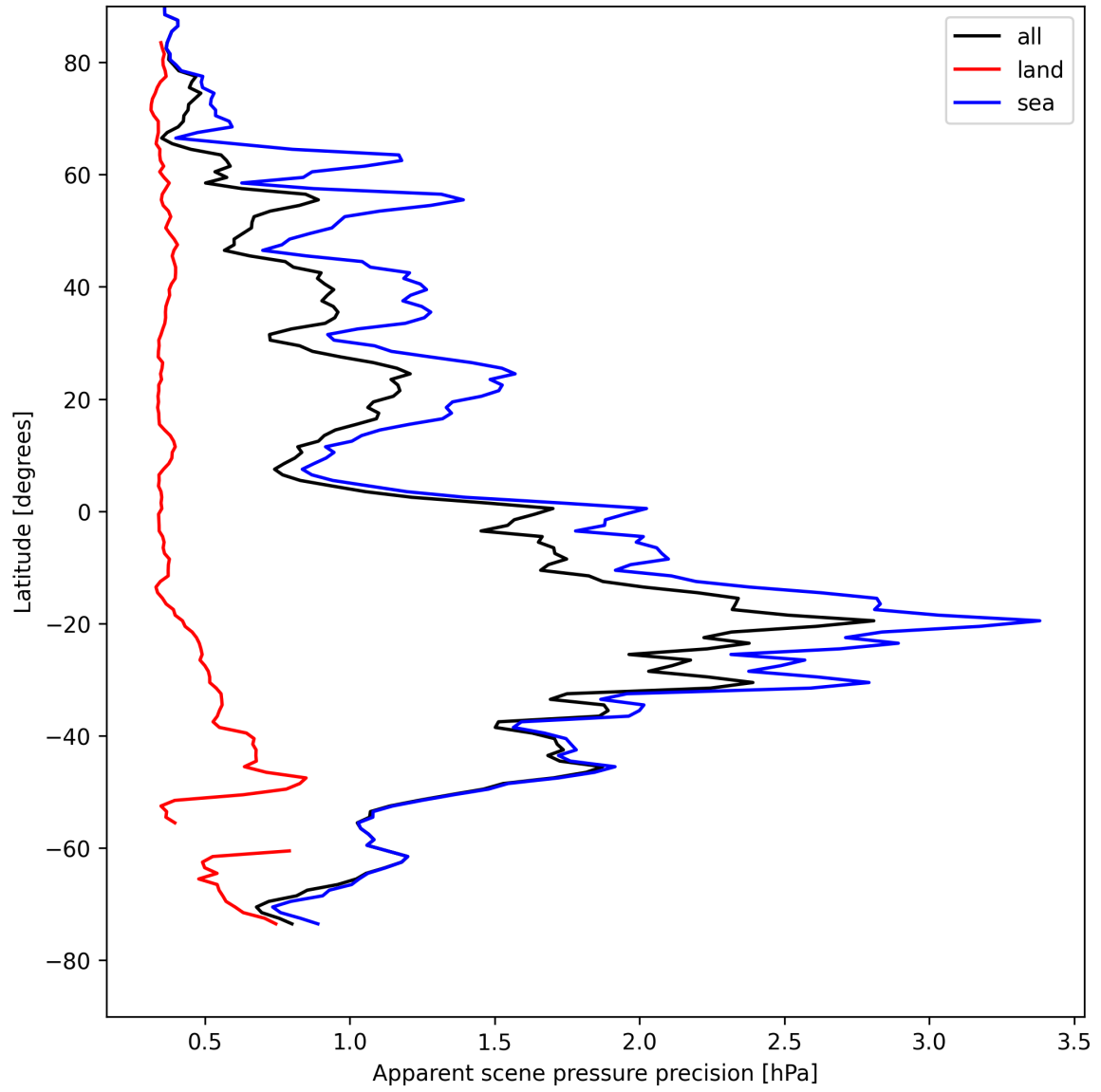
Figure 20: Zonal average of “Apparent scene pressure precision” for 2025-04-27 to 2025-04-29.
