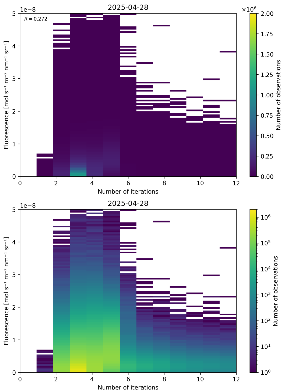
Figure 98: Scatter density plot of “Number of iterations” against “Fluorescence” for 2025-04-27 to 2025-04-29.
