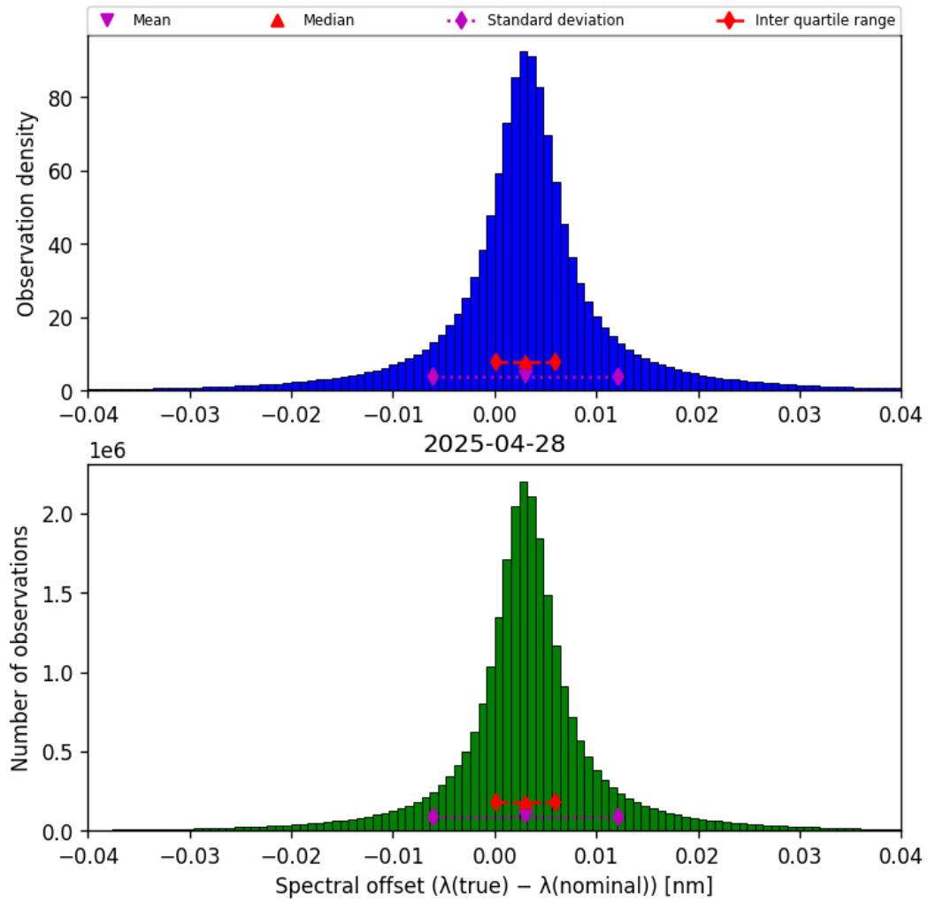
Figure 45: Histogram of “Spectral offset ( \lambda_{\text{true}} - \lambda_{\text{nominal}} )” for 2025-04-27 to 2025-04-29
