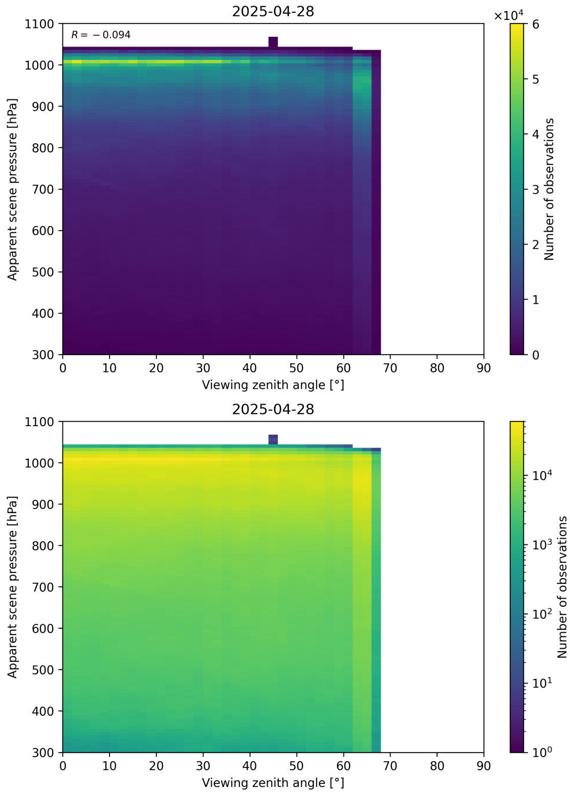
Figure 118: Scatter density plot of “Viewing zenith angle” against “Apparent scene pressure” for 2025-04-27 to 2025-04-29.
