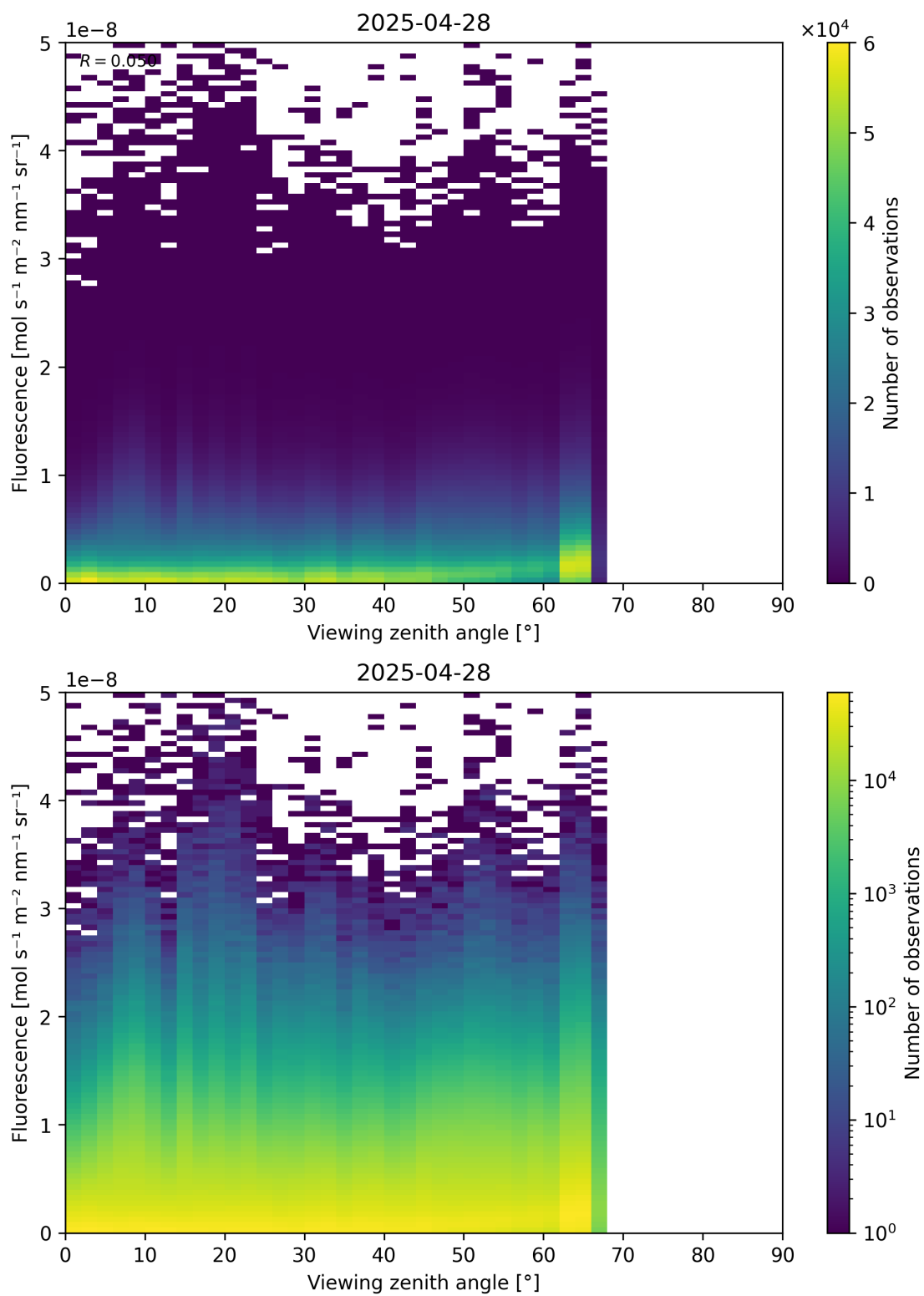
Figure 122: Scatter density plot of “Viewing zenith angle” against “Fluorescence” for 2025-04-27 to 2025-04-29.
