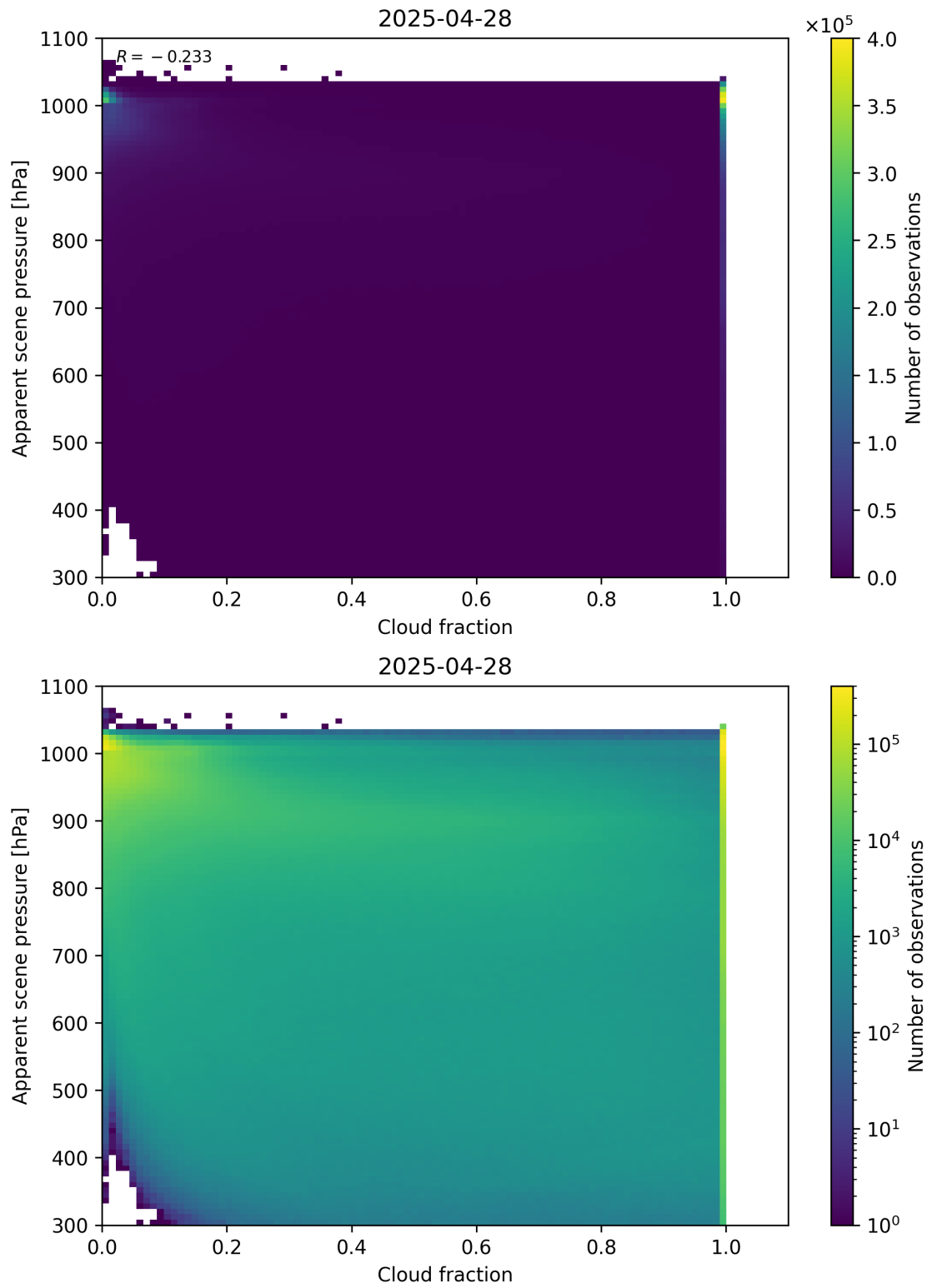
Figure 70: Scatter density plot of “Cloud fraction” against “Apparent scene pressure” for 2025-04-27 to 2025-04-29.
