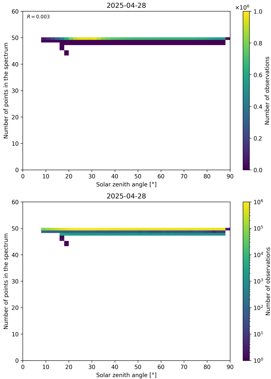
Figure 115: Scatter density plot of “Solar zenith angle” against “Number of points in the spectrum” for 2025-04-27 to 2025-04-29.
