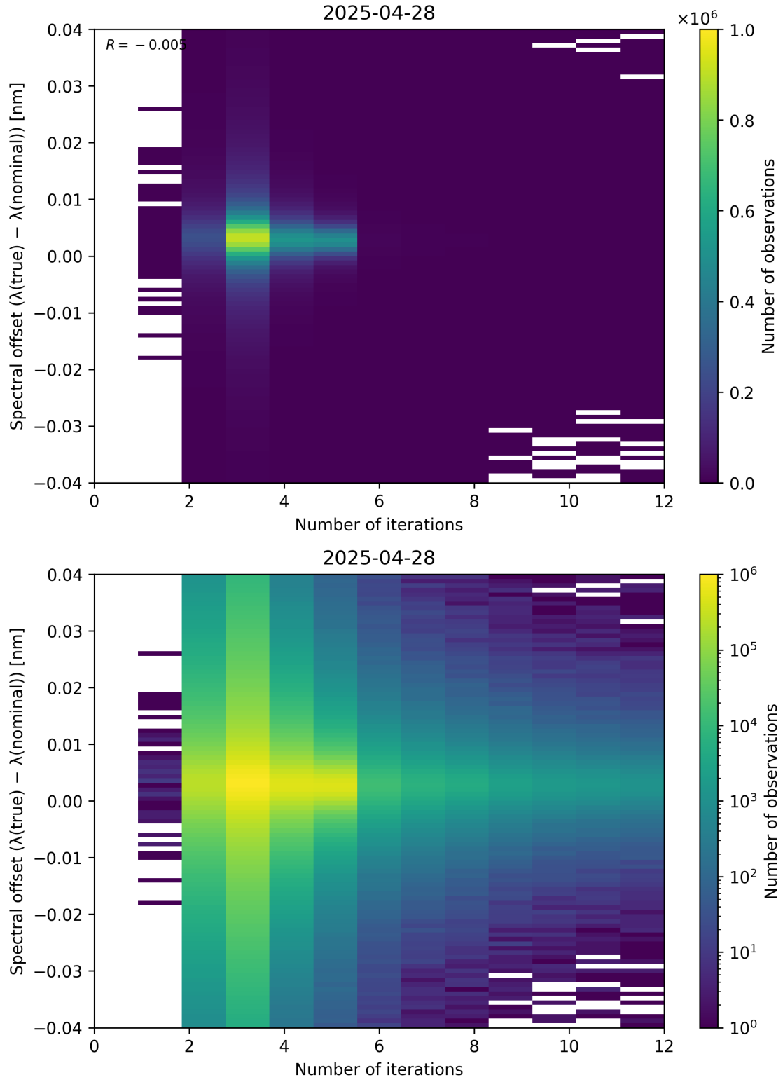
Figure 100: Scatter density plot of “Number of iterations” against “Spectral offset ( \lambda_{\text{true}} - \lambda_{\text{nominal}} )” for 2025-04-27 to 2025-04-29.
