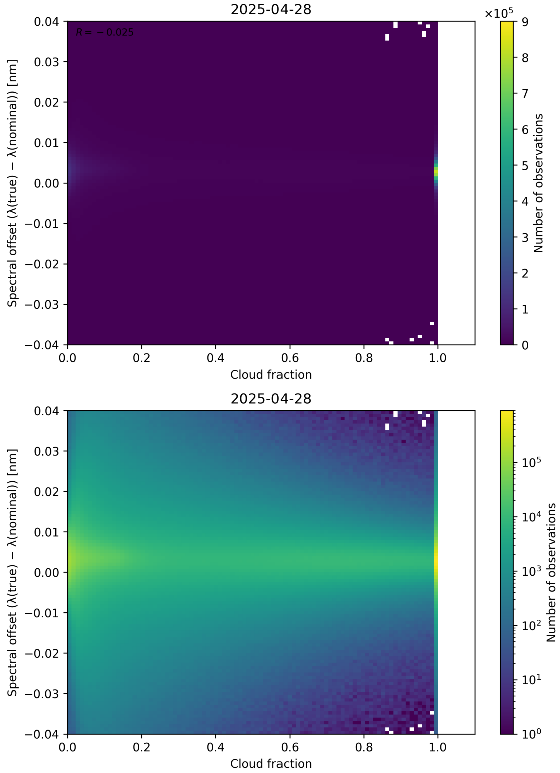
Figure 76: Scatter density plot of “Cloud fraction” against “Spectral offset ( \lambda_{\text{true}} - \lambda_{\text{nominal}} )” for 2025-04-27 to 2025-04-29.
