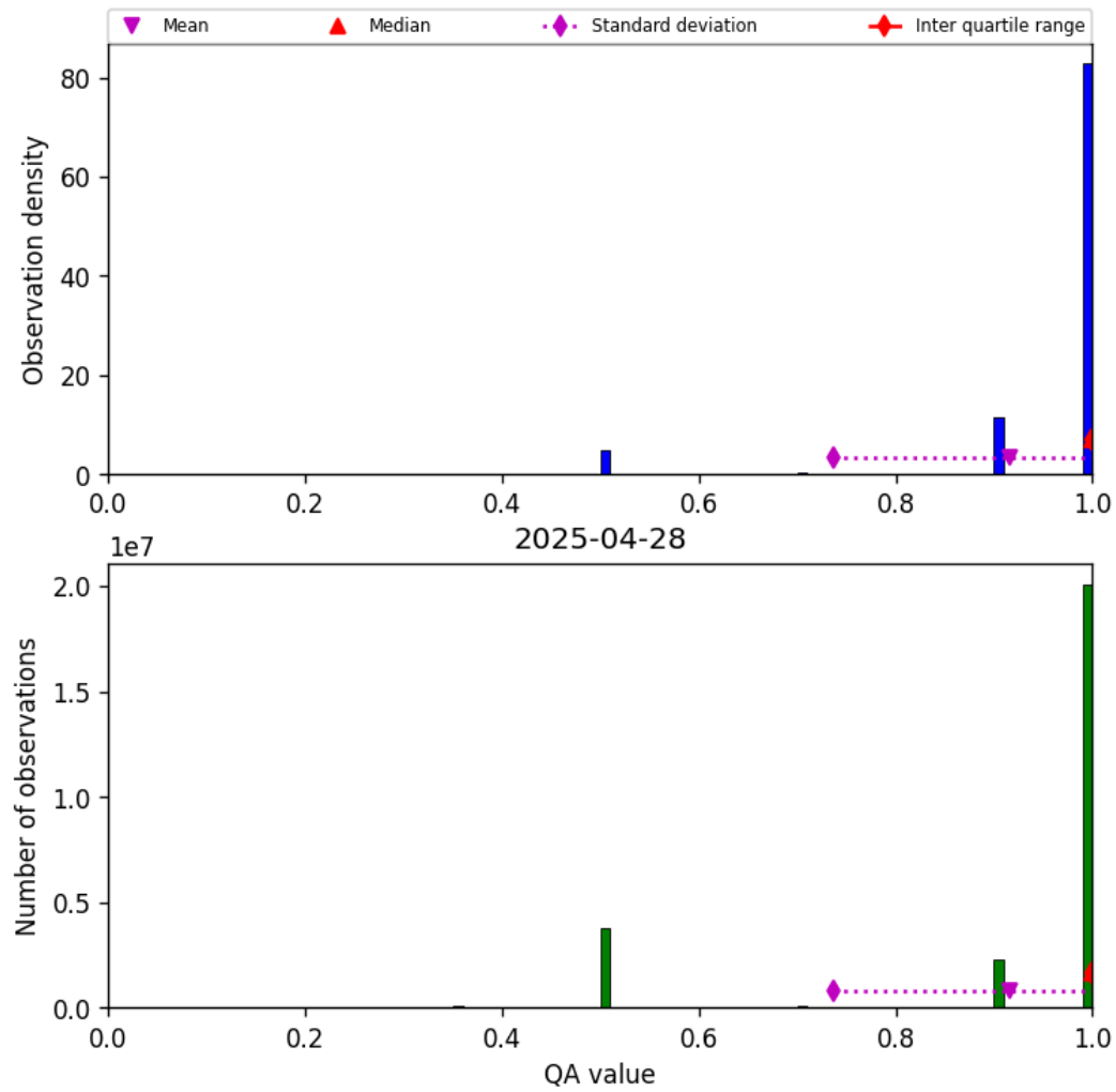
Figure 29: Histogram of “QA value” for 2025-04-27 to 2025-04-29
