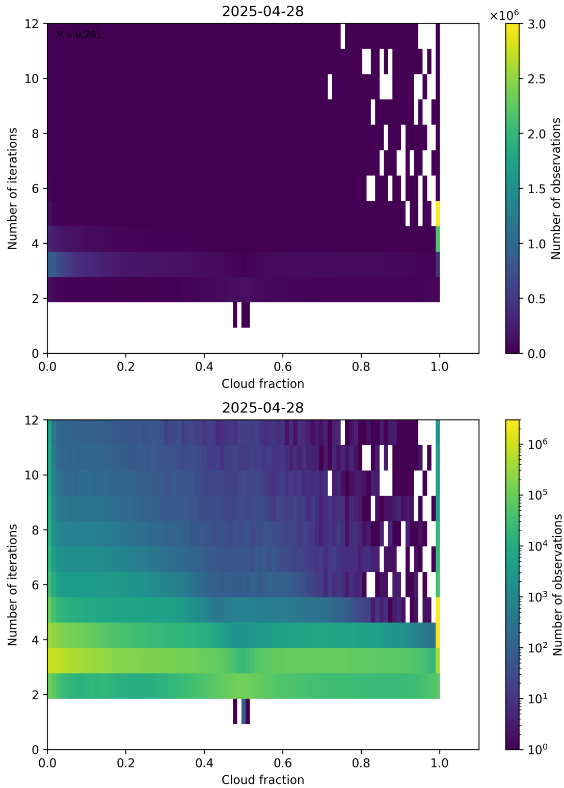
Figure 73: Scatter density plot of “Cloud fraction” against “Number of iterations” for 2025-04-27 to 2025-04-29.
