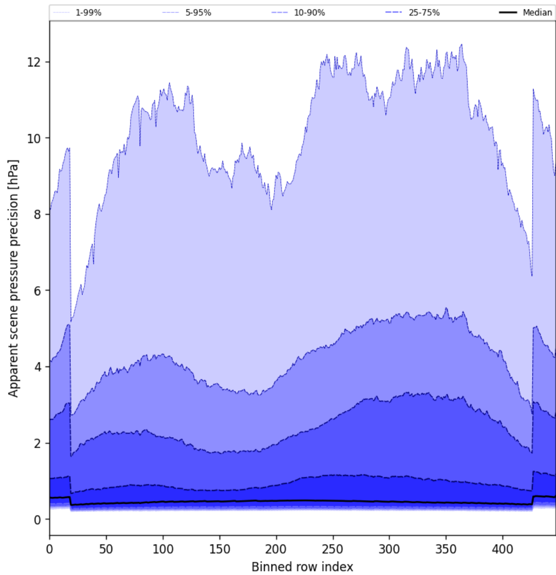
Figure 54: Along track statistics of “Apparent scene pressure precision” for 2025-04-27 to 2025-04-29
