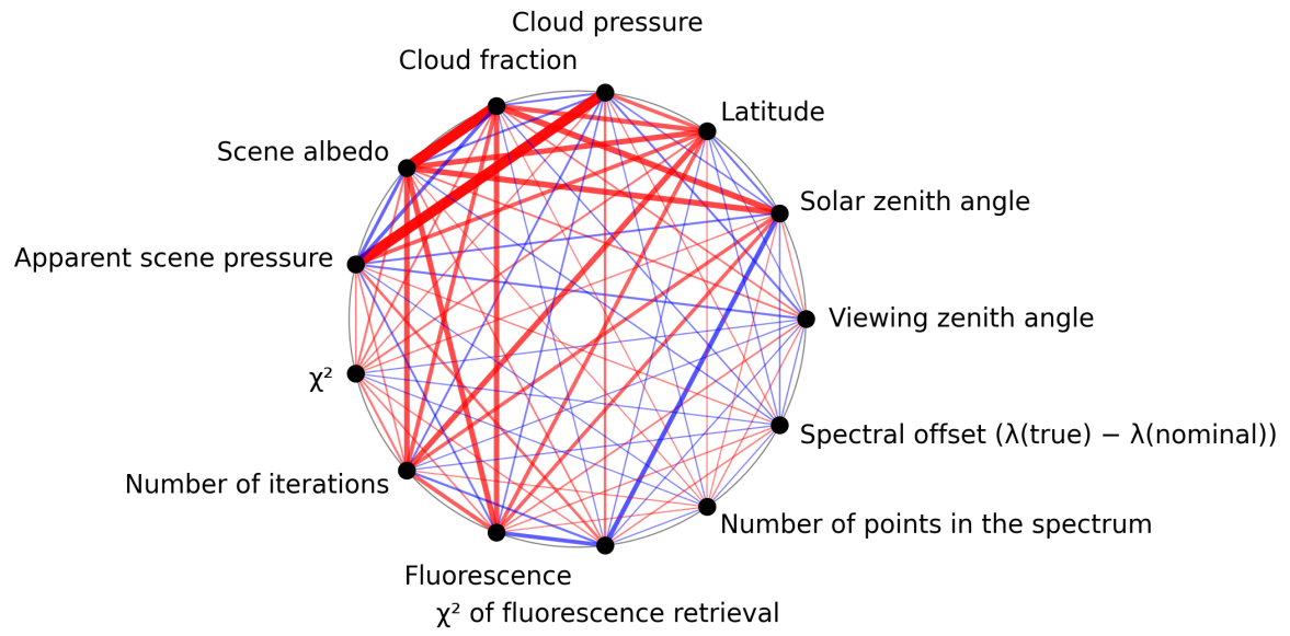
Figure 1: Map of correlation graph for 2025-04-27 to 2025-04-29.
