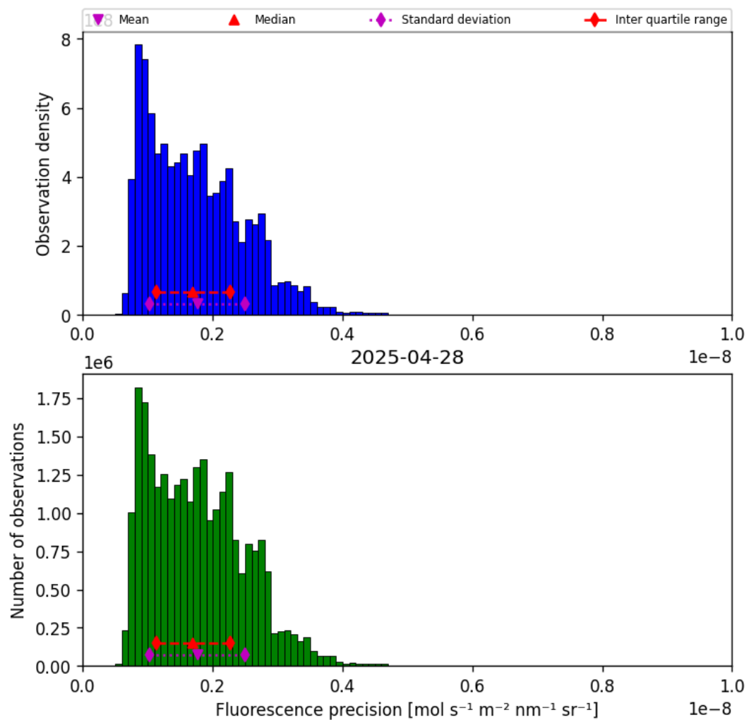
Figure 41: Histogram of “Fluorescence precision” for 2025-04-27 to 2025-04-29
