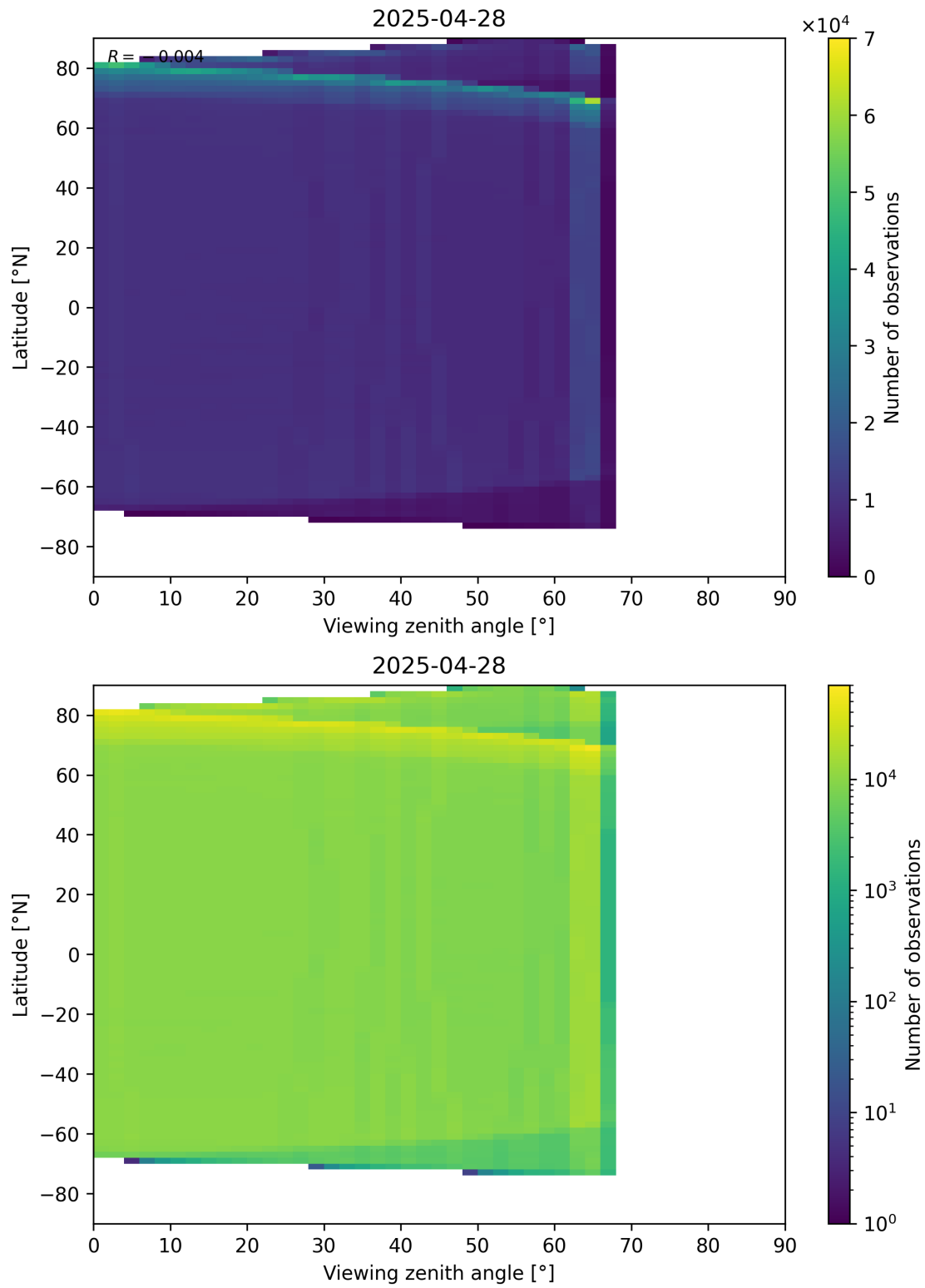
Figure 123: Scatter density plot of “Viewing zenith angle” against “Latitude” for 2025-04-27 to 2025-04-29.
