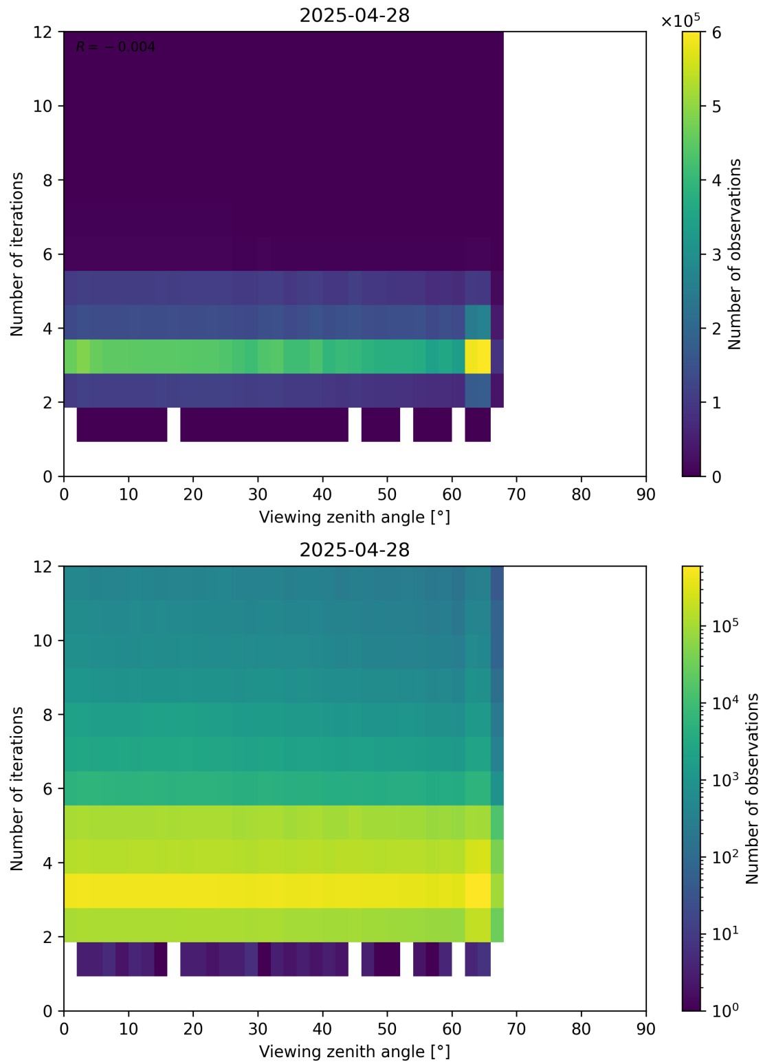
Figure 124: Scatter density plot of “Viewing zenith angle” against “Number of iterations” for 2025-04-27 to 2025-04-29.
