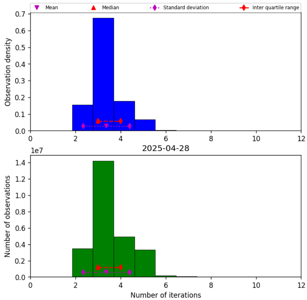
Figure 39: Histogram of “Number of iterations” for 2025-04-27 to 2025-04-29
