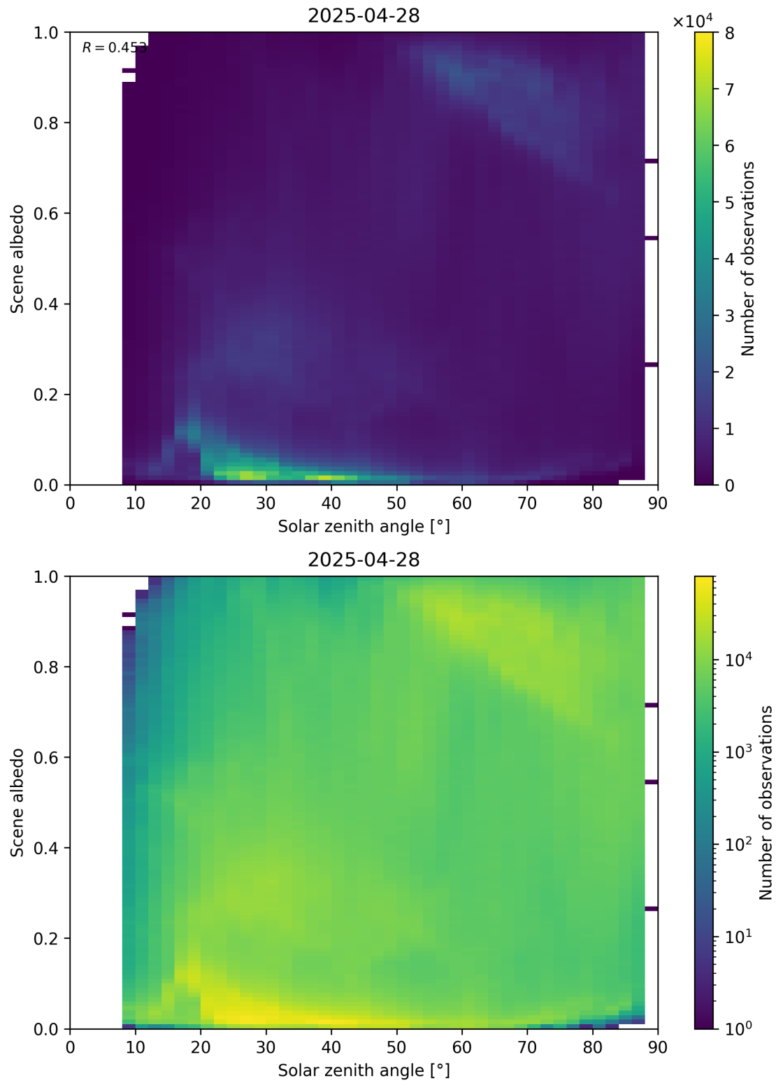
Figure 116: Scatter density plot of “Solar zenith angle” against “Scene albedo” for 2025-04-27 to 2025-04-29.
