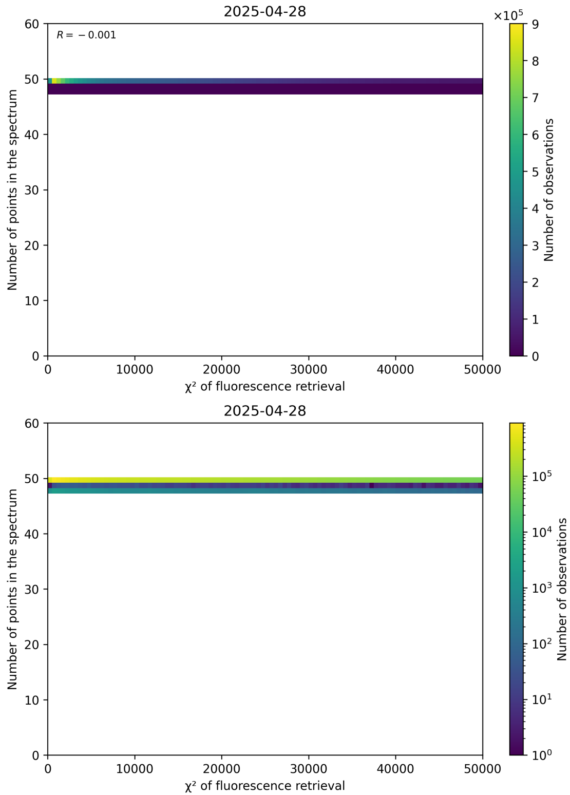
Figure 68: Scatter density plot of “ \chi^2 of fluorescence retrieval” against “Number of points in the spectrum” for 2025-04-27 to 2025-04-29.
