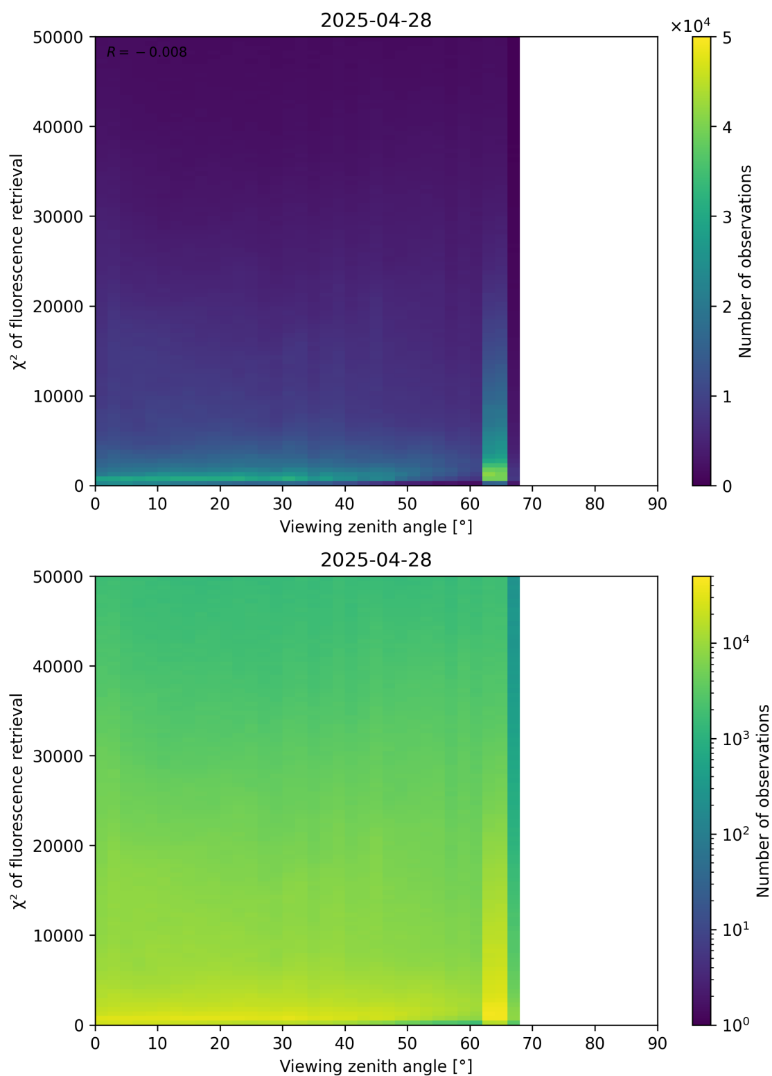
Figure 119: Scatter density plot of “Viewing zenith angle” against “ \chi^2 of fluorescence retrieval” for 2025-04-27 to 2025-04-29.
