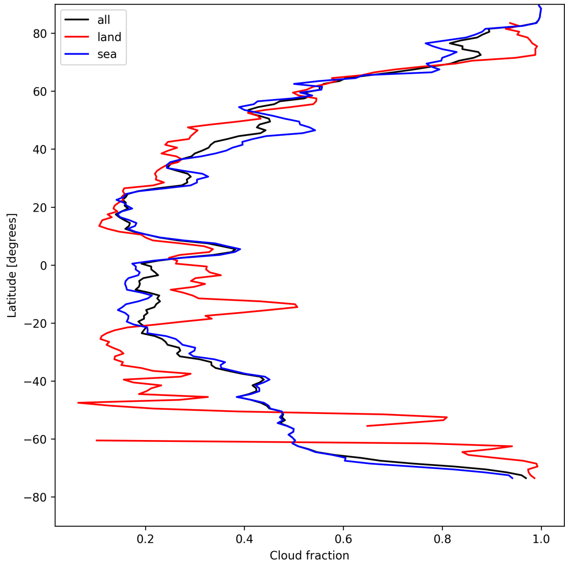
Figure 15: Zonal average of “Cloud fraction” for 2025-04-27 to 2025-04-29.
