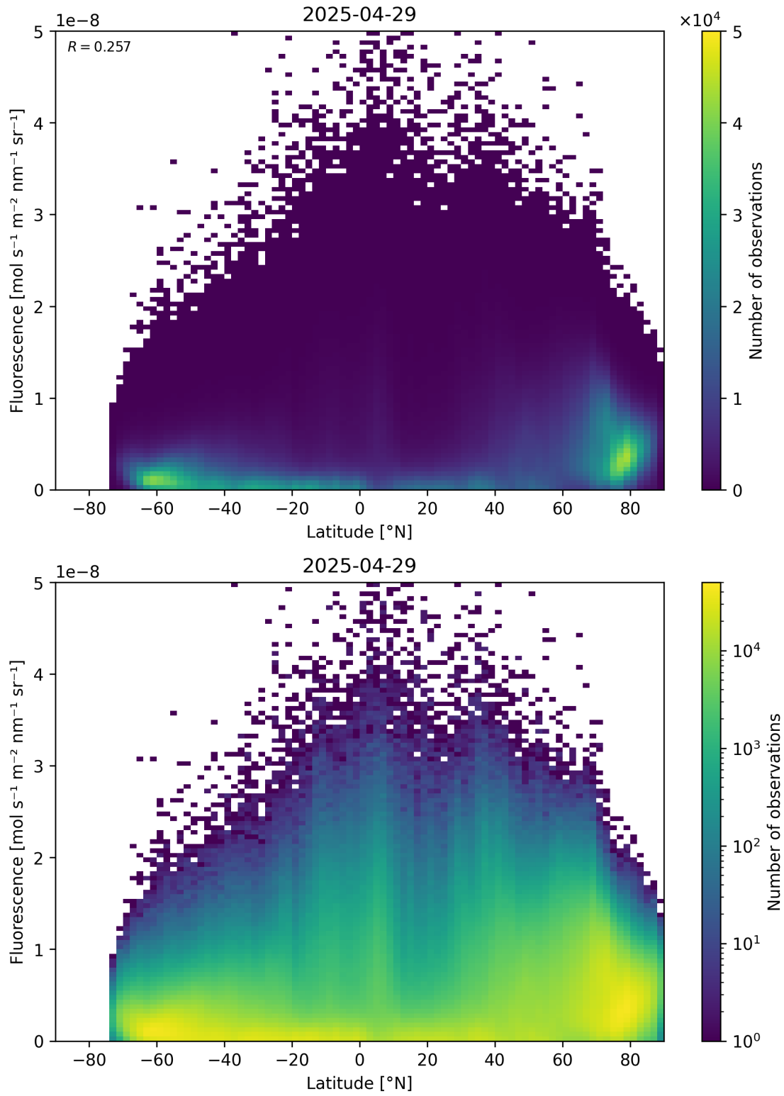
Figure 92: Scatter density plot of “Latitude” against “Fluorescence” for 2025-04-29 to 2025-04-30.
