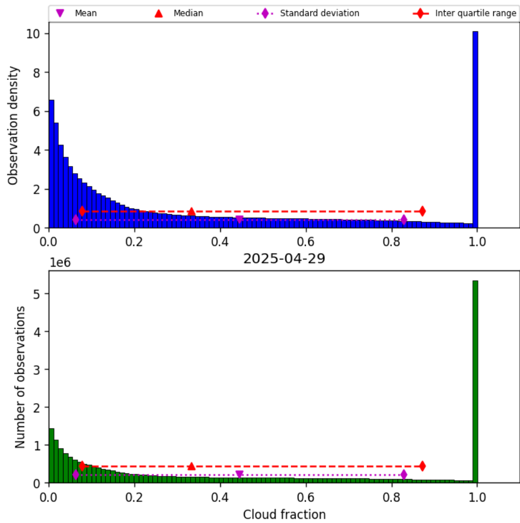
Figure 32: Histogram of “Cloud fraction” for 2025-04-29 to 2025-04-30
