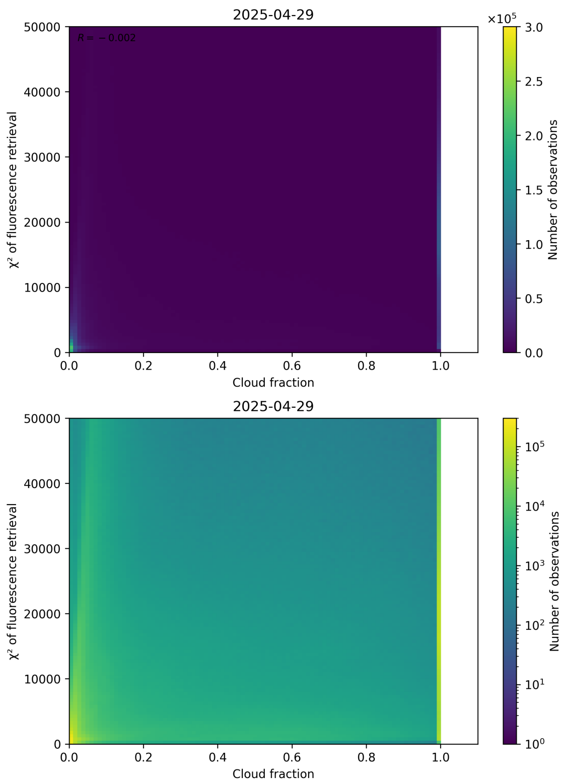
Figure 71: Scatter density plot of “Cloud fraction” against “ \chi^2 of fluorescence retrieval” for 2025-04-29 to 2025-04-30.
