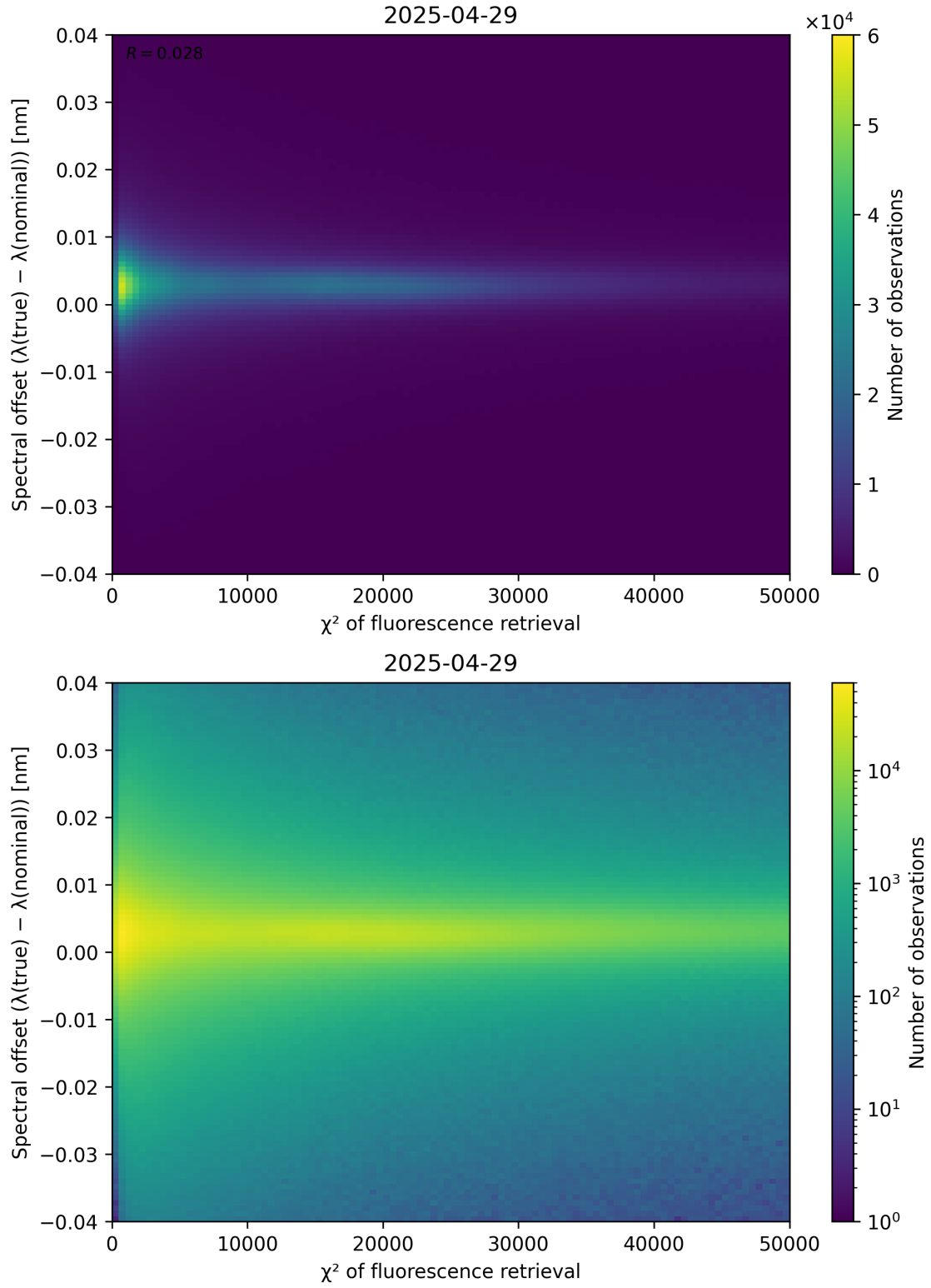
Figure 69: Scatter density plot of “ \chi^2 of fluorescence retrieval” against “Spectral offset ( \lambda_{\text{true}} - \lambda_{\text{nominal}} )” for 2025-04-29 to 2025-04-30.
