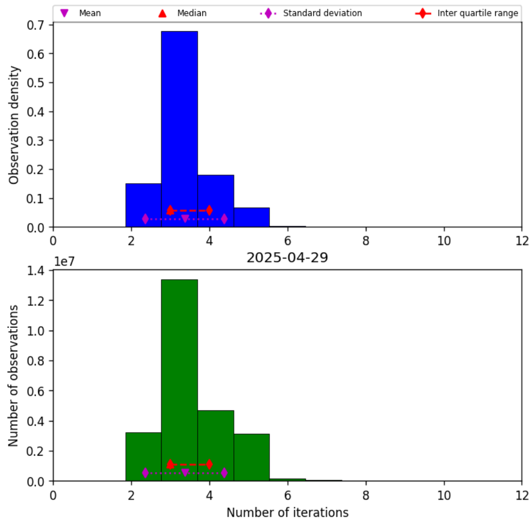
Figure 39: Histogram of “Number of iterations” for 2025-04-29 to 2025-04-30
