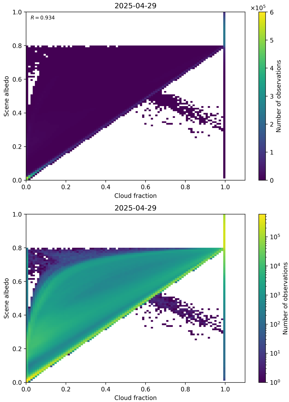
Figure 75: Scatter density plot of “Cloud fraction” against “Scene albedo” for 2025-04-29 to 2025-04-30.
