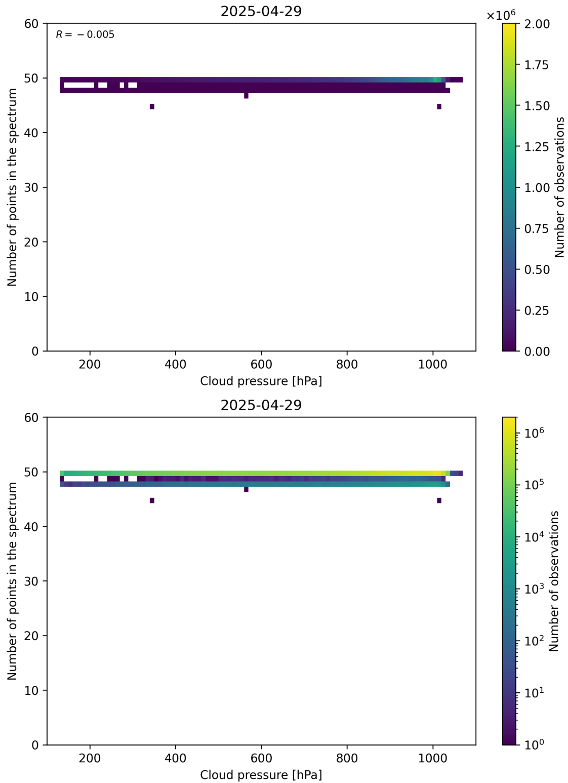
Figure 82: Scatter density plot of “Cloud pressure” against “Number of points in the spectrum” for 2025-04-29 to 2025-04-30.
