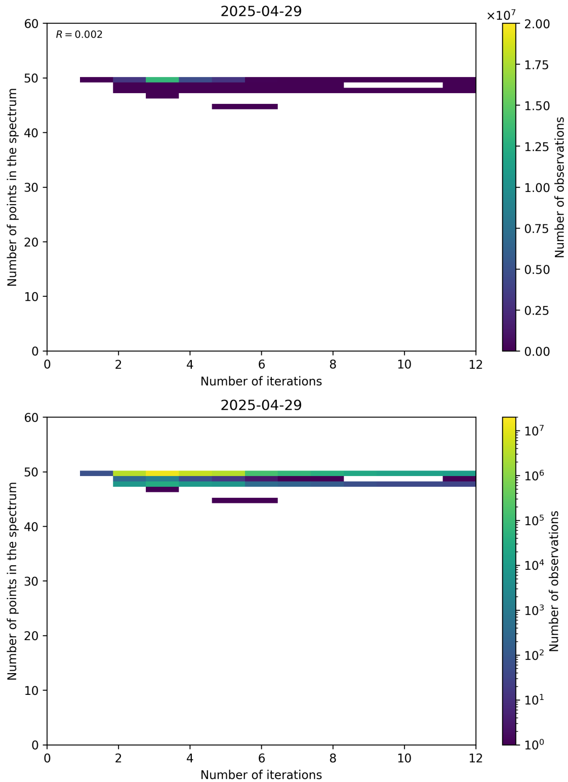
Figure 99: Scatter density plot of “Number of iterations” against “Number of points in the spectrum” for 2025-04-29 to 2025-04-30.
