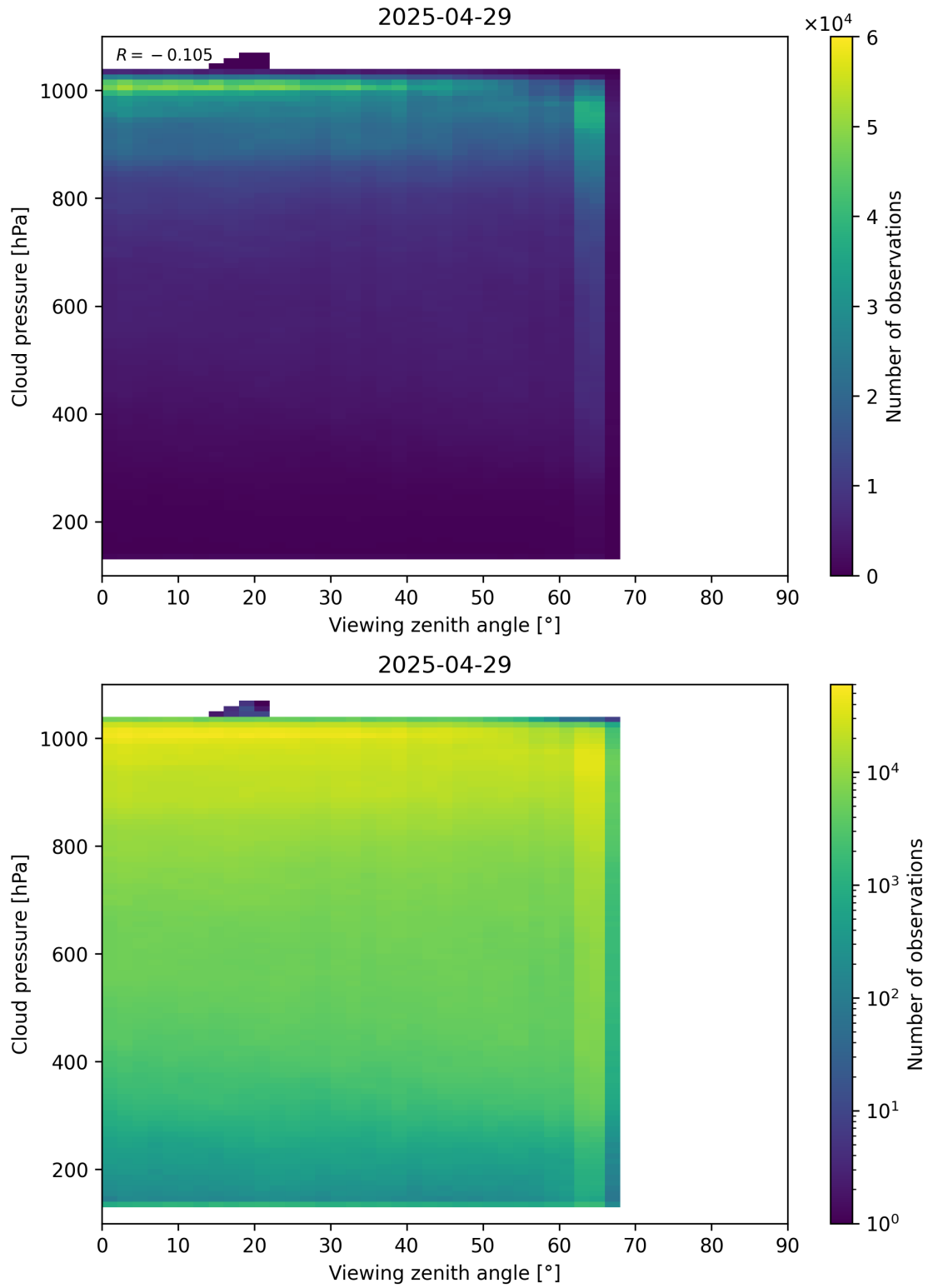
Figure 121: Scatter density plot of “Viewing zenith angle” against “Cloud pressure” for 2025-04-29 to 2025-04-30.
