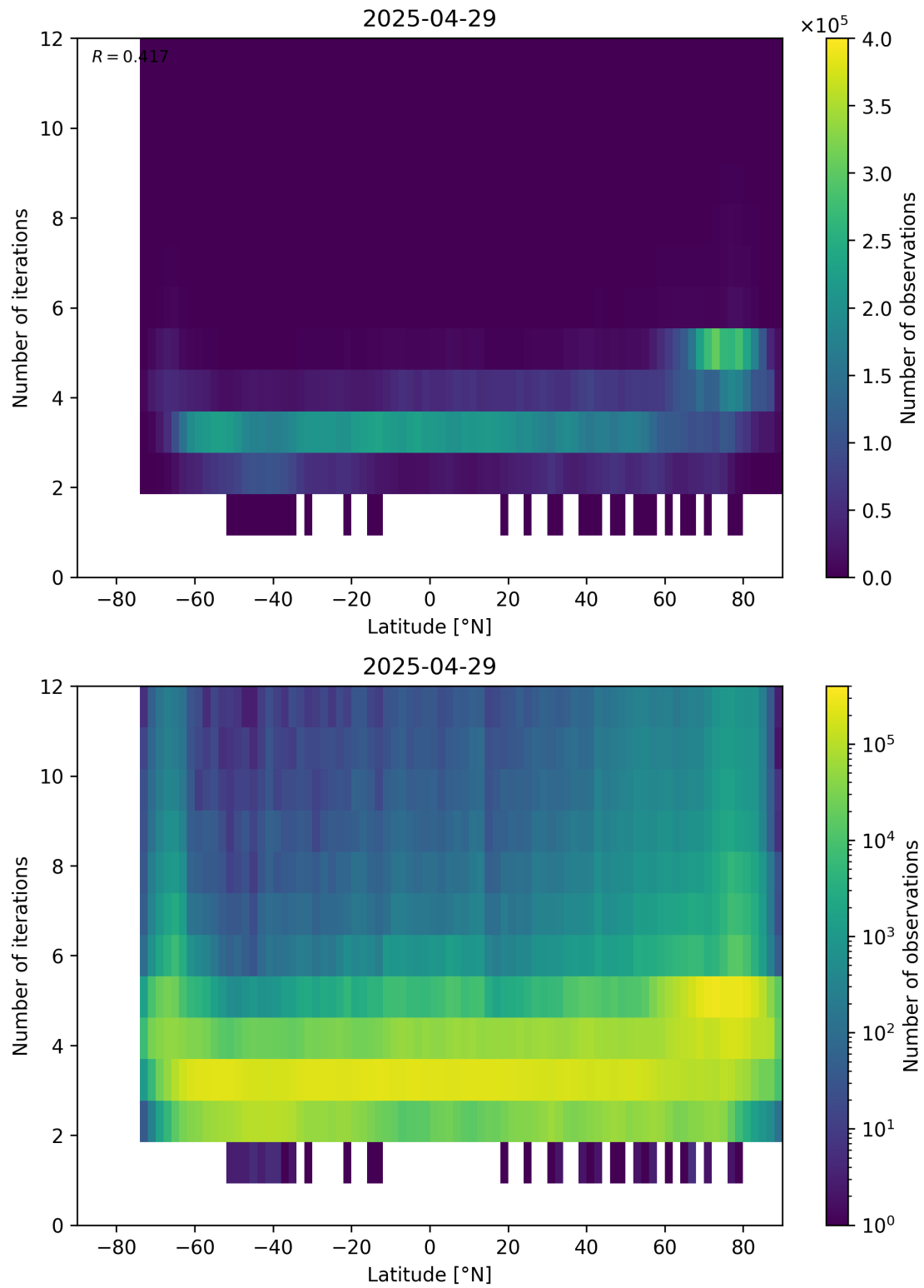
Figure 93: Scatter density plot of “Latitude” against “Number of iterations” for 2025-04-29 to 2025-04-30.
