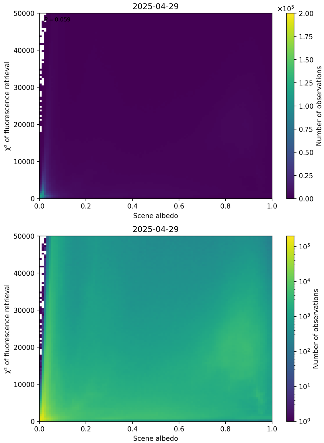
Figure 103: Scatter density plot of “Scene albedo” against “ \chi^2 of fluorescence retrieval” for 2025-04-29 to 2025-04-30.
