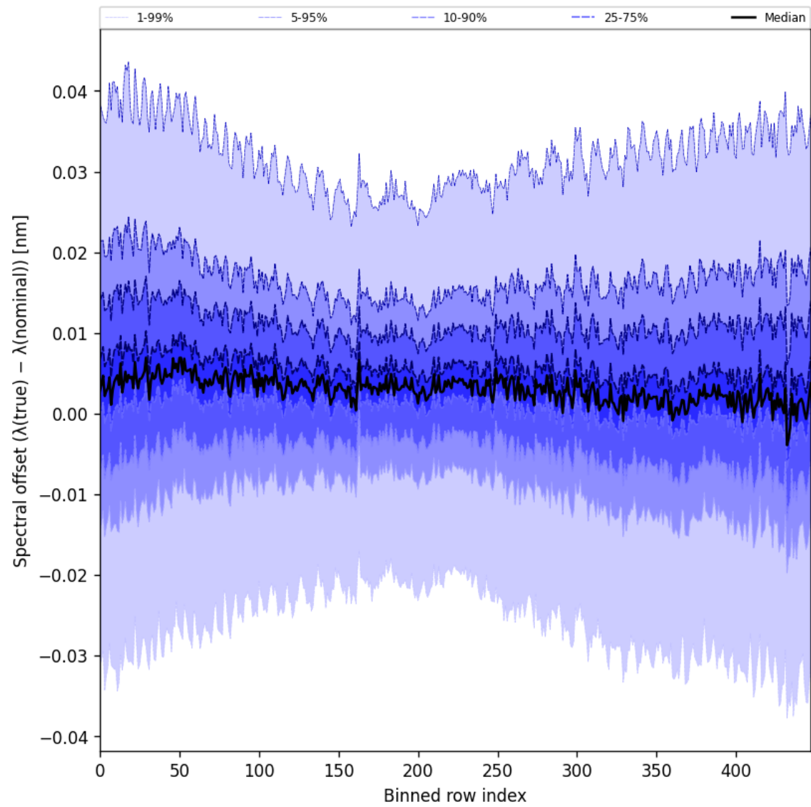
Figure 62: Along track statistics of “Spectral offset ( \lambda_{\text{true}} - \lambda_{\text{nominal}} )” for 2025-04-29 to 2025-04-30
