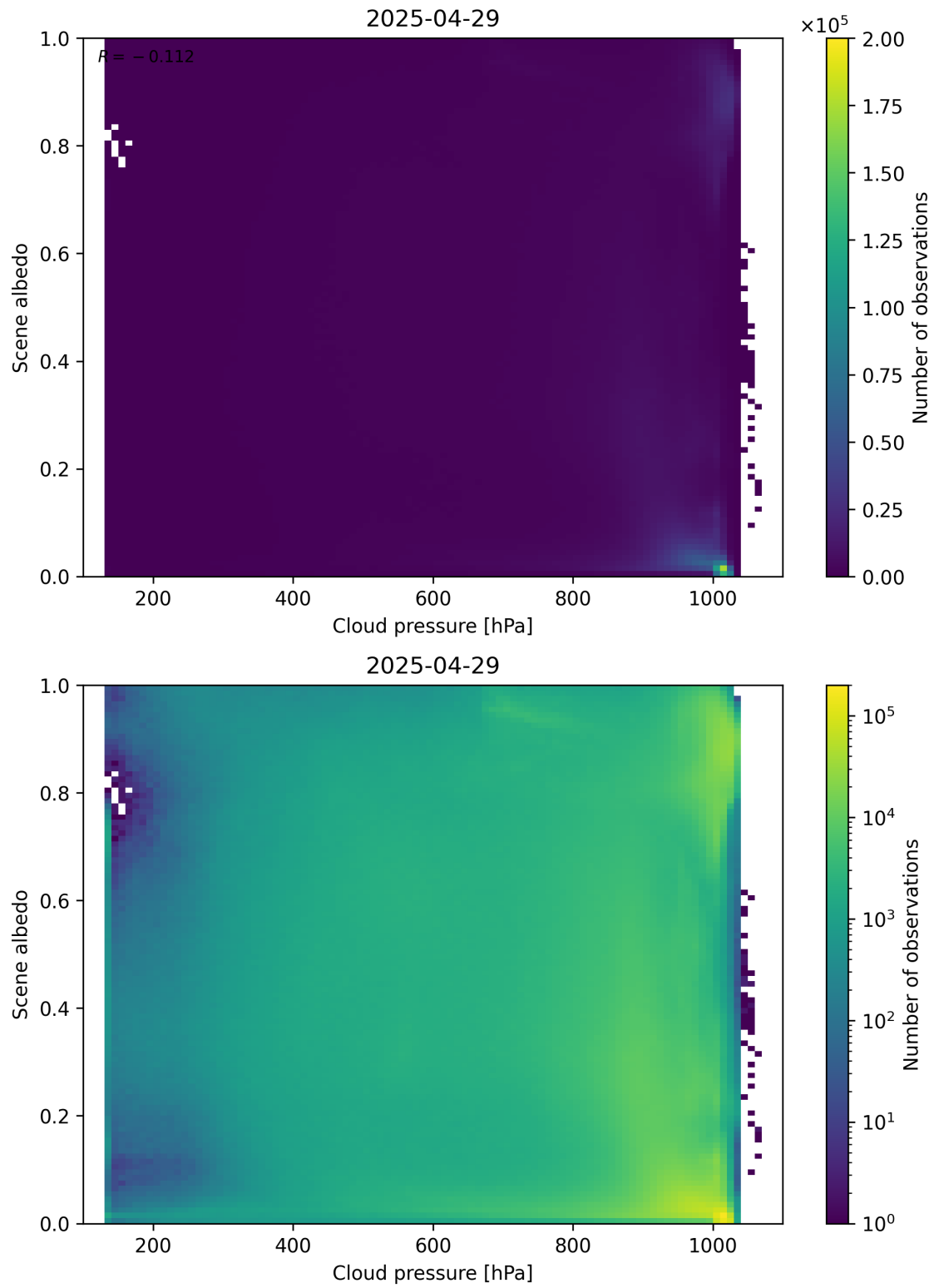
Figure 83: Scatter density plot of “Cloud pressure” against “Scene albedo” for 2025-04-29 to 2025-04-30.
