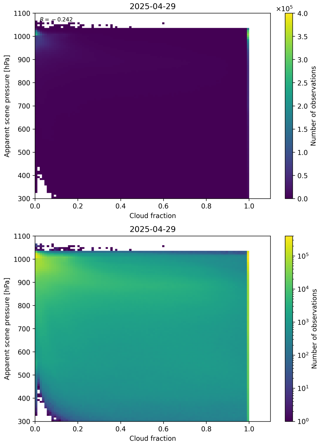
Figure 70: Scatter density plot of “Cloud fraction” against “Apparent scene pressure” for 2025-04-29 to 2025-04-30.
