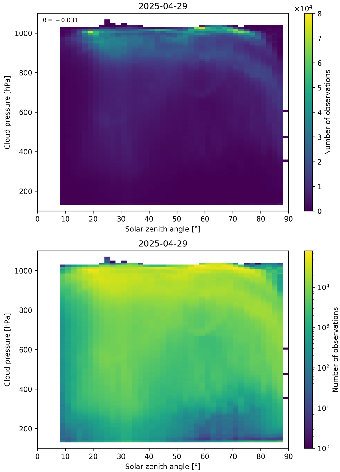
Figure 111: Scatter density plot of “Solar zenith angle” against “Cloud pressure” for 2025-04-29 to 2025-04-30.
