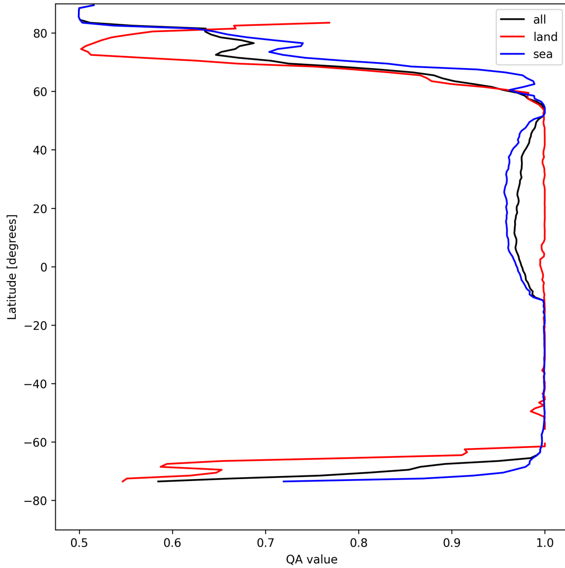
Figure 12: Zonal average of “QA value” for 2025-04-29 to 2025-04-30.
