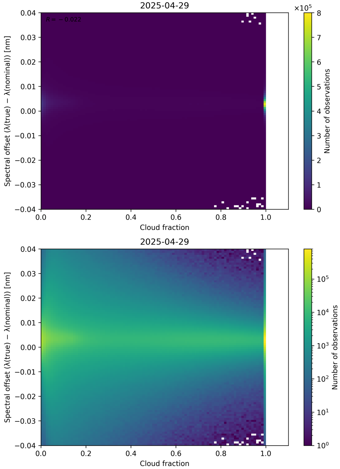
Figure 76: Scatter density plot of “Cloud fraction” against “Spectral offset ( \lambda_{\text{true}} - \lambda_{\text{nominal}} )” for 2025-04-29 to 2025-04-30.
