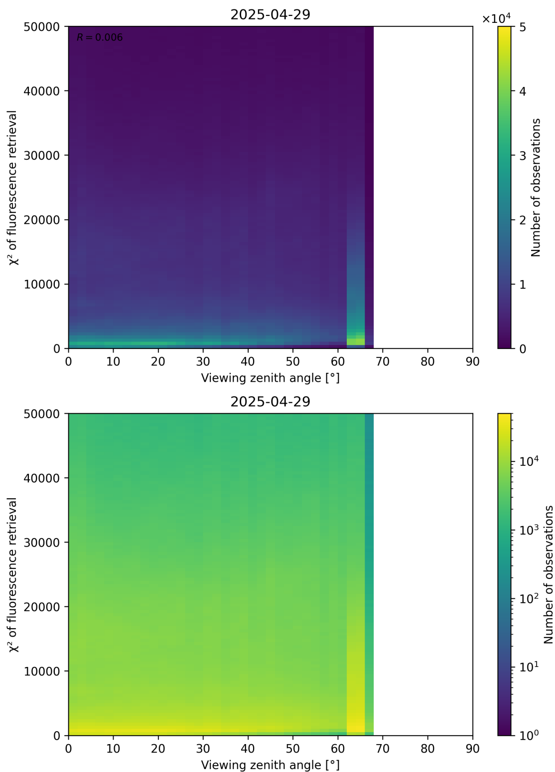
Figure 119: Scatter density plot of “Viewing zenith angle” against “ \chi^2 of fluorescence retrieval” for 2025-04-29 to 2025-04-30.
