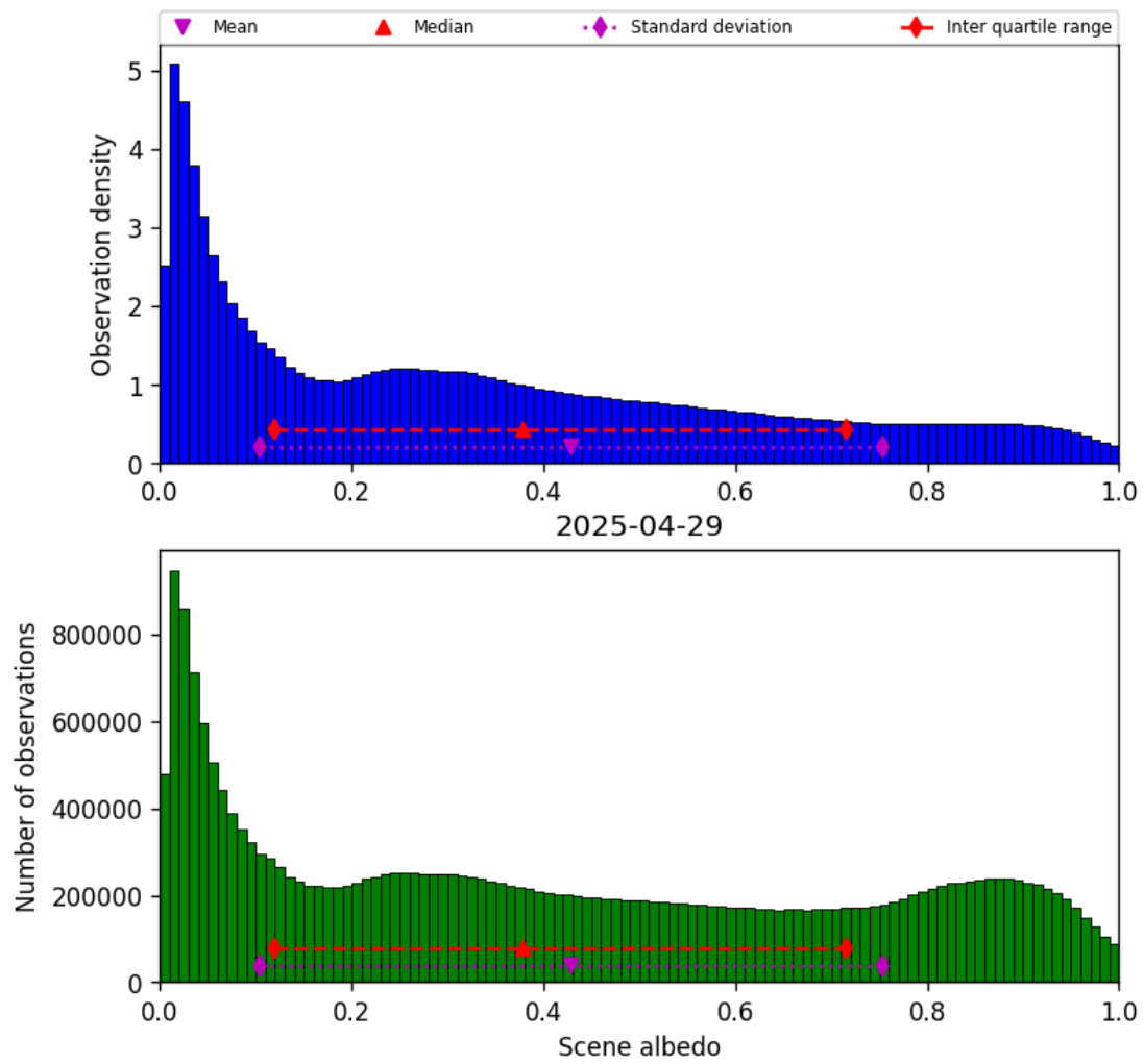
Figure 34: Histogram of “Scene albedo” for 2025-04-29 to 2025-04-30
