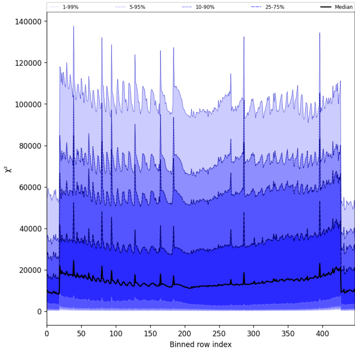
Figure 55: Along track statistics of “ \chi^2 ” for 2025-04-29 to 2025-04-30
