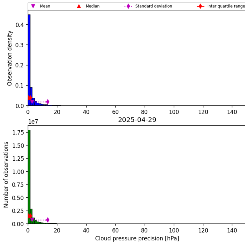
Figure 31: Histogram of “Cloud pressure precision” for 2025-04-29 to 2025-04-30
