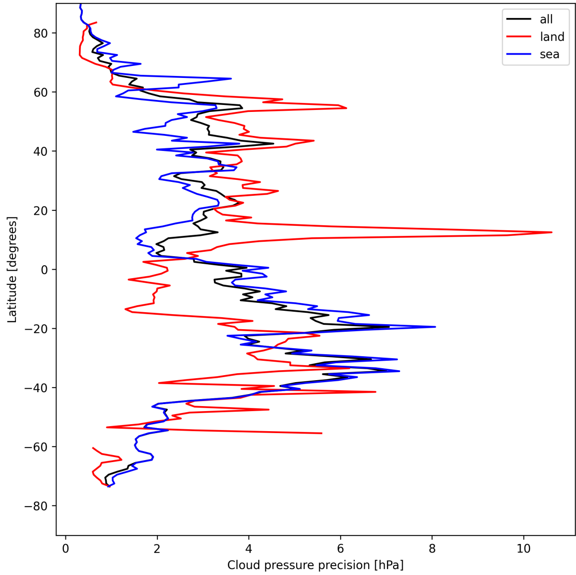
Figure 14: Zonal average of “Cloud pressure precision” for 2025-04-29 to 2025-04-30.
