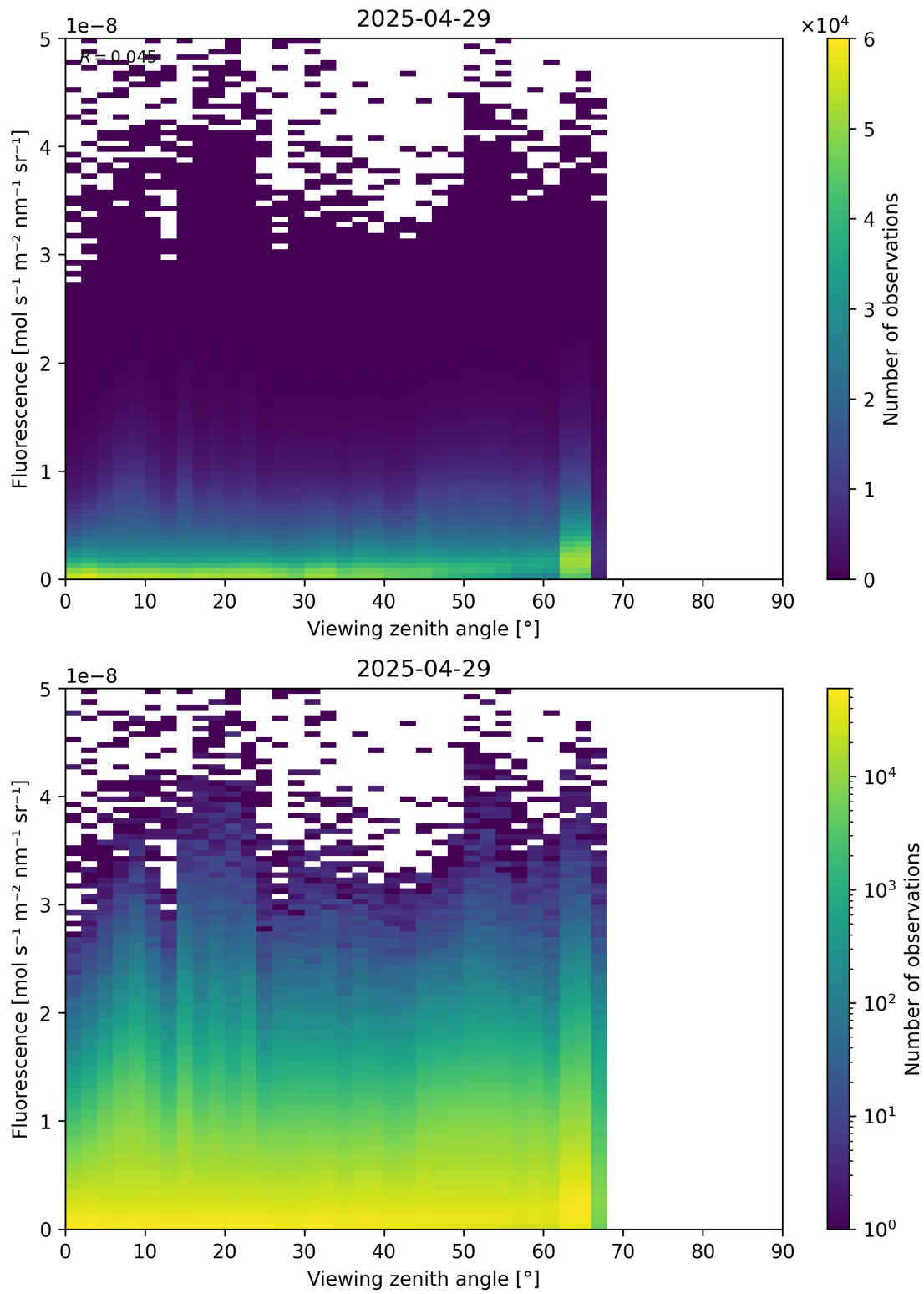
Figure 122: Scatter density plot of “Viewing zenith angle” against “Fluorescence” for 2025-04-29 to 2025-04-30.
