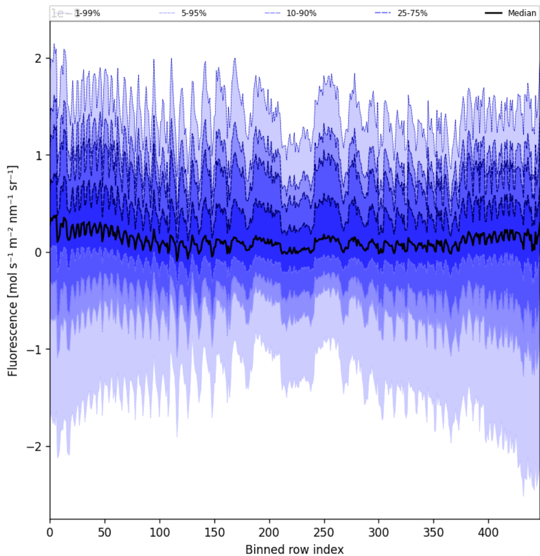
Figure 57: Along track statistics of “Fluorescence” for 2025-04-29 to 2025-04-30
