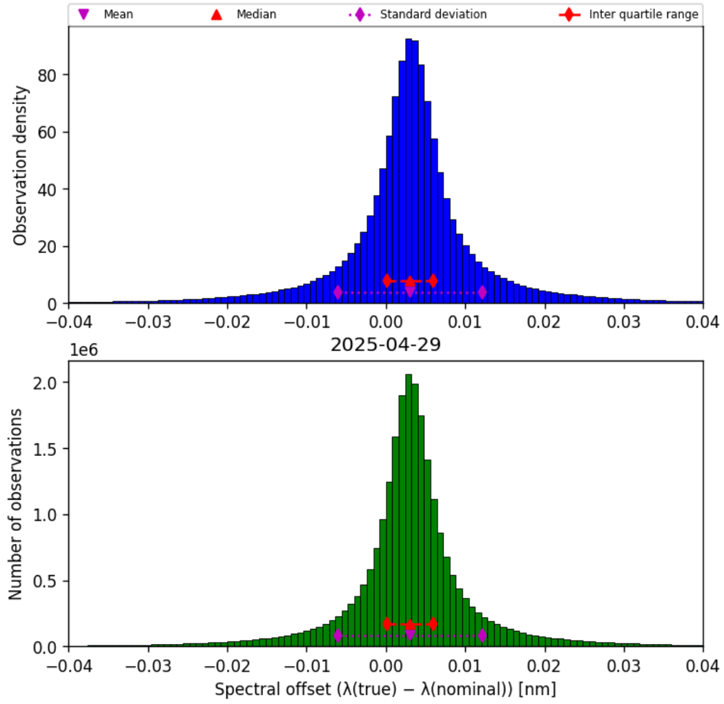
Figure 45: Histogram of “Spectral offset ( \lambda_{\text{true}} - \lambda_{\text{nominal}} )” for 2025-04-29 to 2025-04-30
