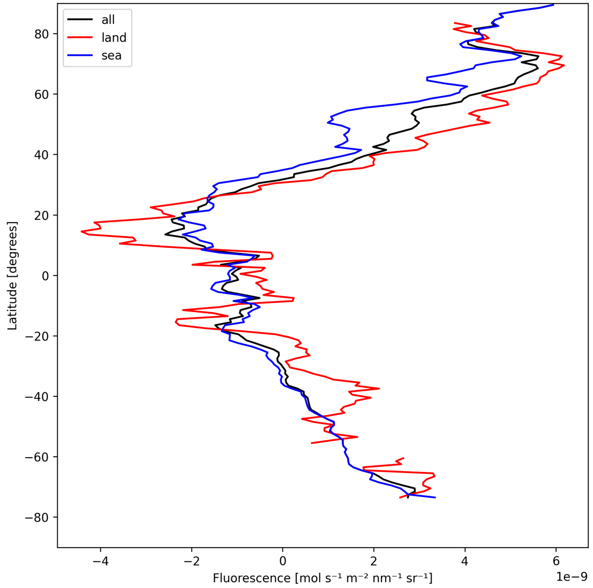
Figure 23: Zonal average of “Fluorescence” for 2025-04-29 to 2025-04-30.
