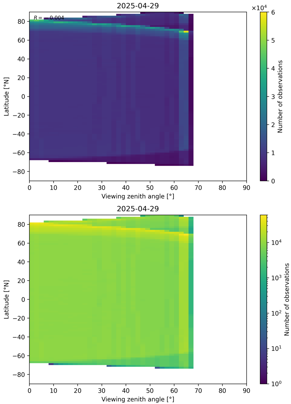
Figure 123: Scatter density plot of “Viewing zenith angle” against “Latitude” for 2025-04-29 to 2025-04-30.
