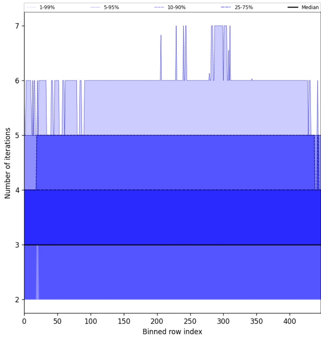
Figure 56: Along track statistics of “Number of iterations” for 2025-04-29 to 2025-04-30
