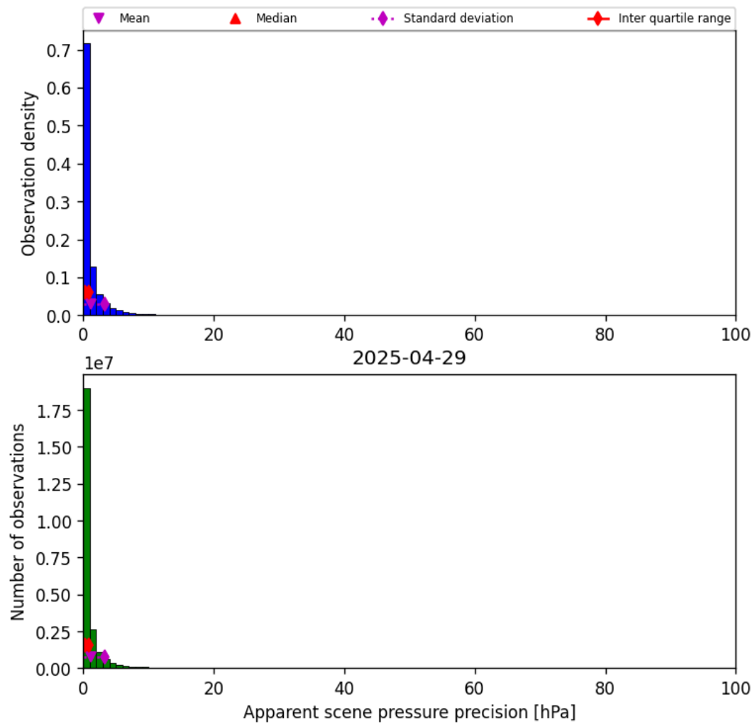
Figure 37: Histogram of “Apparent scene pressure precision” for 2025-04-29 to 2025-04-30
