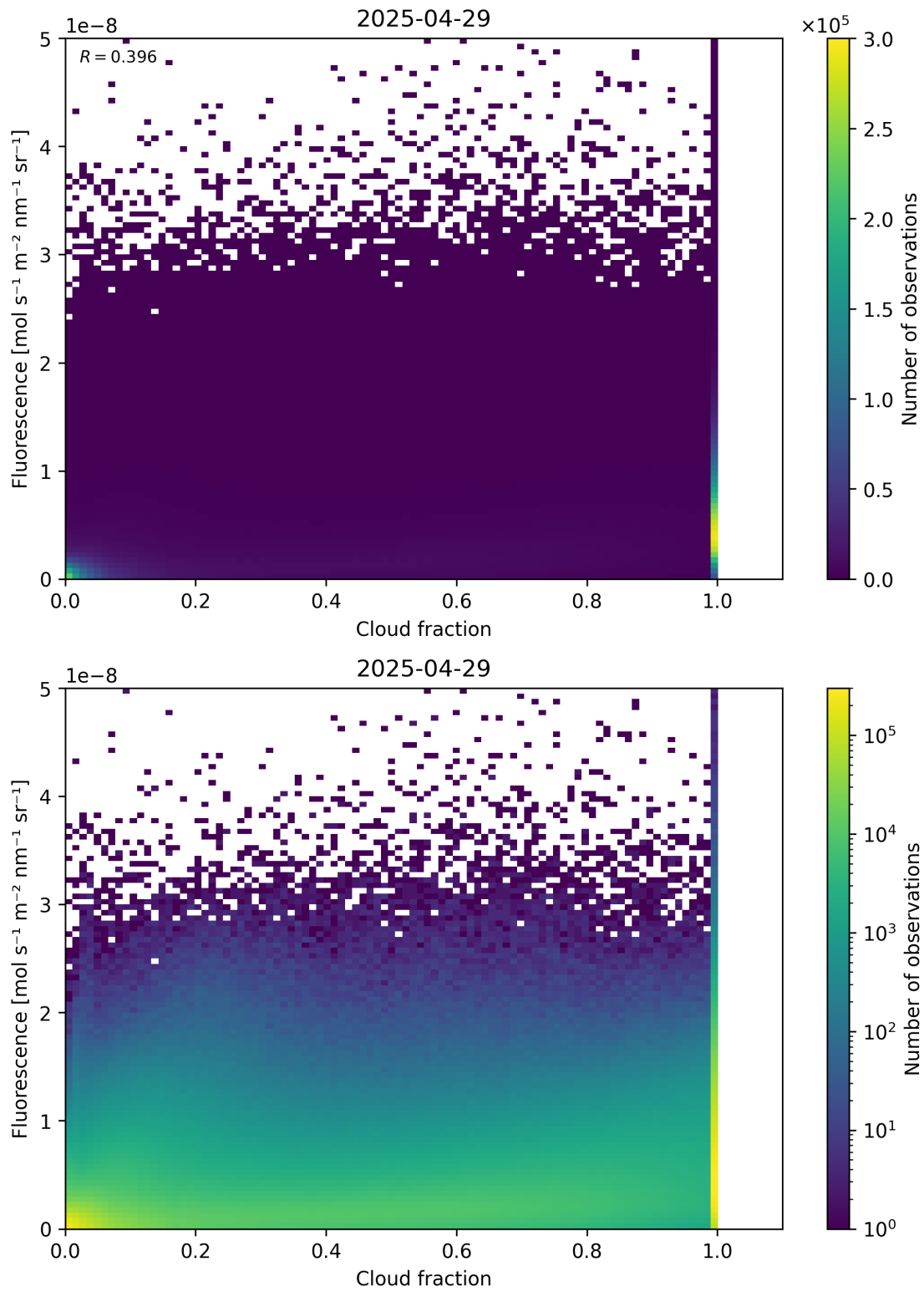
Figure 72: Scatter density plot of “Cloud fraction” against “Fluorescence” for 2025-04-29 to 2025-04-30.
