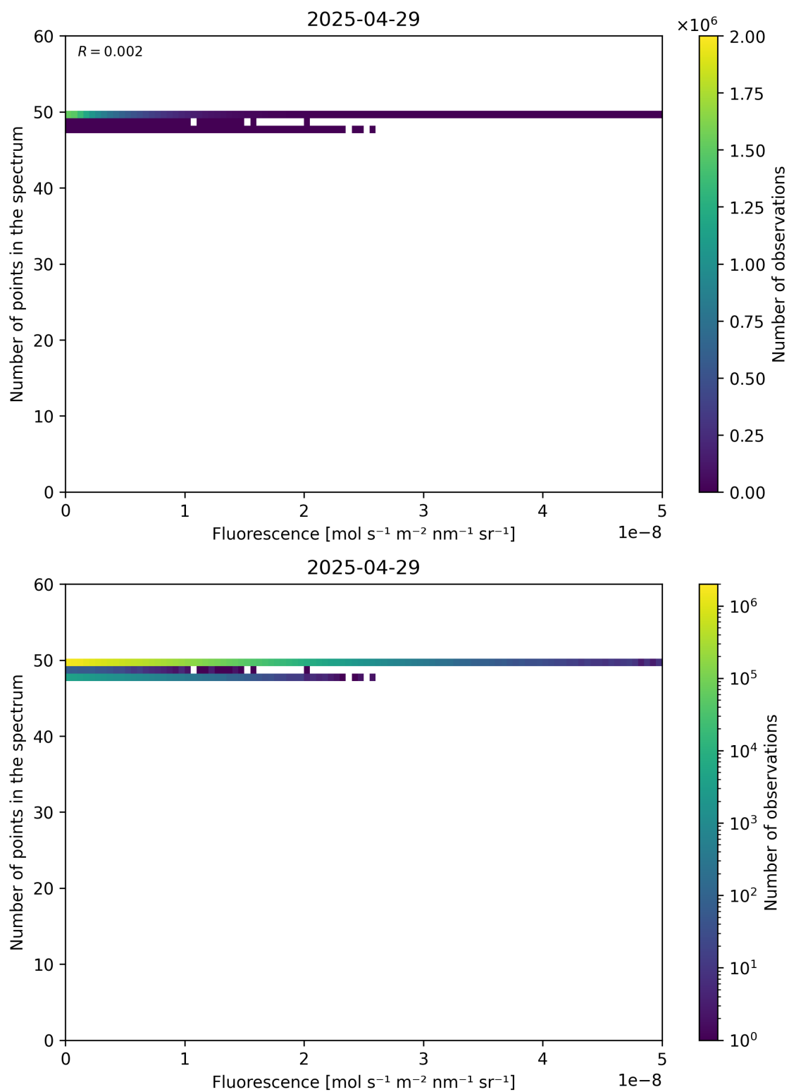
Figure 86: Scatter density plot of “Fluorescence” against “Number of points in the spectrum” for 2025-04-29 to 2025-04-30.
