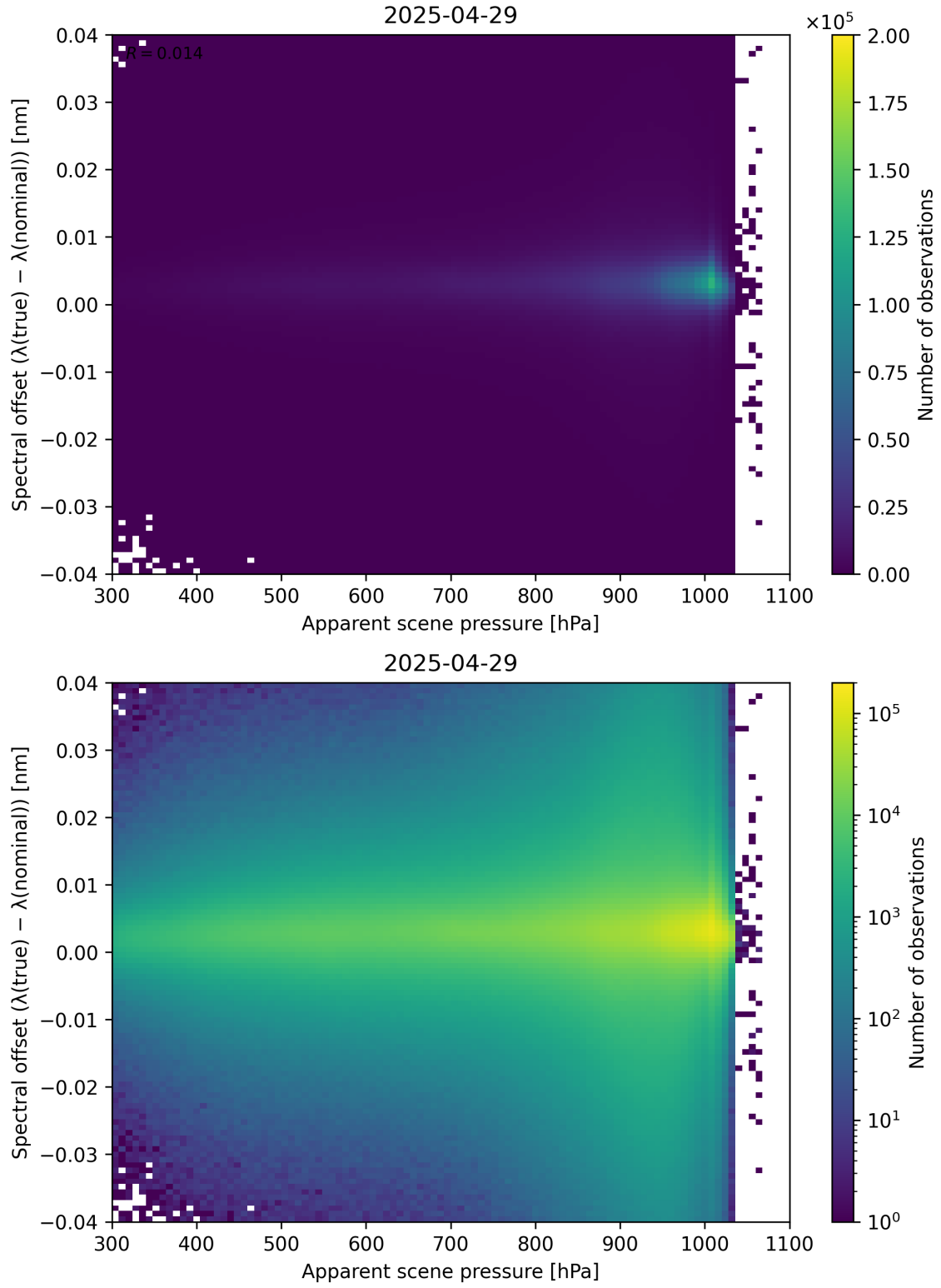
Figure 67: Scatter density plot of “Apparent scene pressure” against “Spectral offset ( \lambda_{\text{true}} - \lambda_{\text{nominal}} )” for 2025-04-29 to 2025-04-30.
