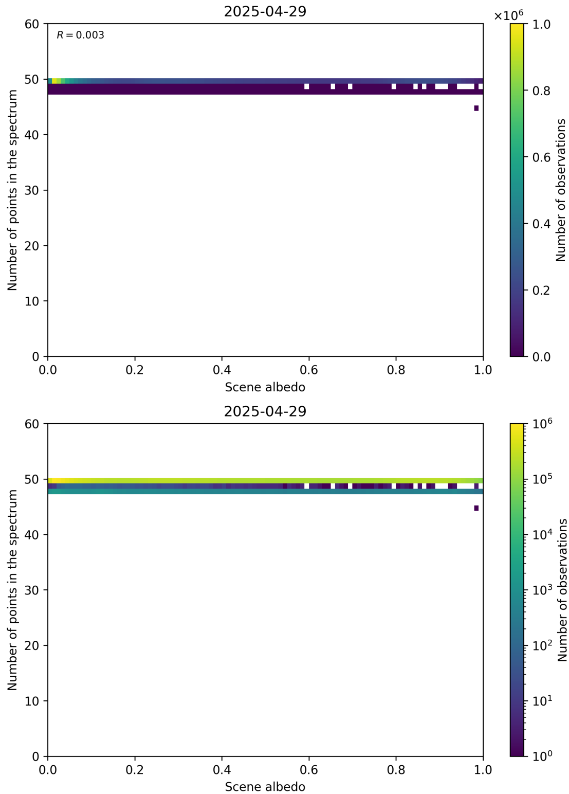
Figure 106: Scatter density plot of “Scene albedo” against “Number of points in the spectrum” for 2025-04-29 to 2025-04-30.
