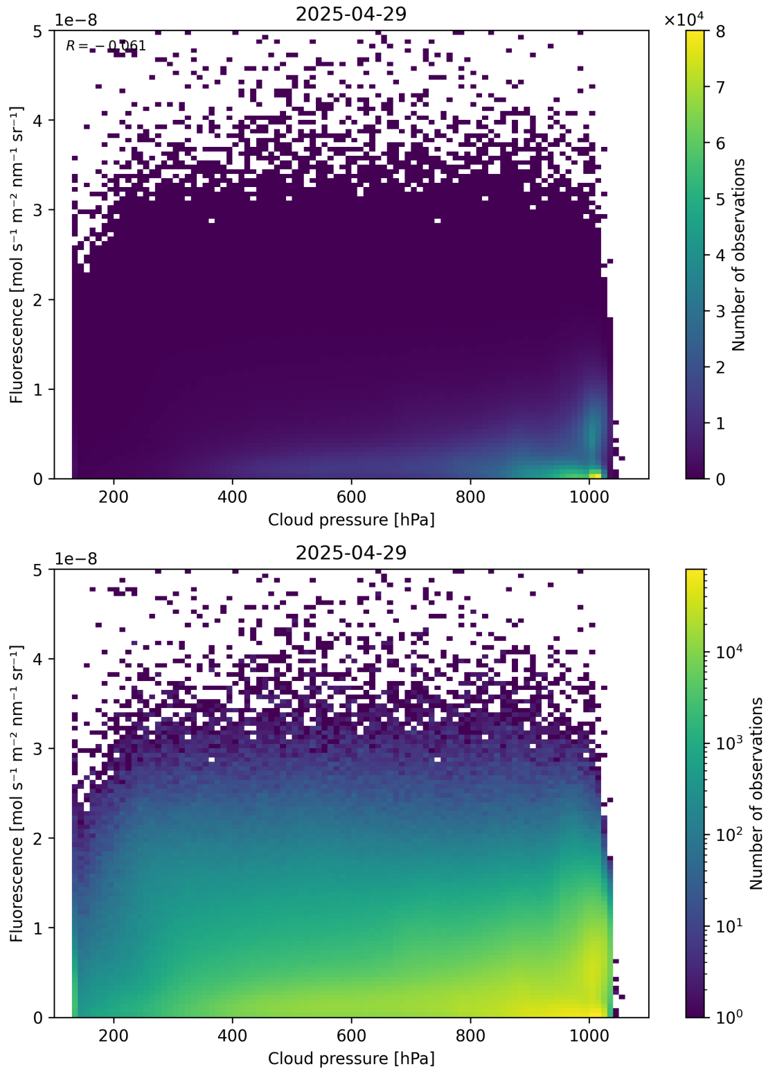
Figure 80: Scatter density plot of “Cloud pressure” against “Fluorescence” for 2025-04-29 to 2025-04-30.
