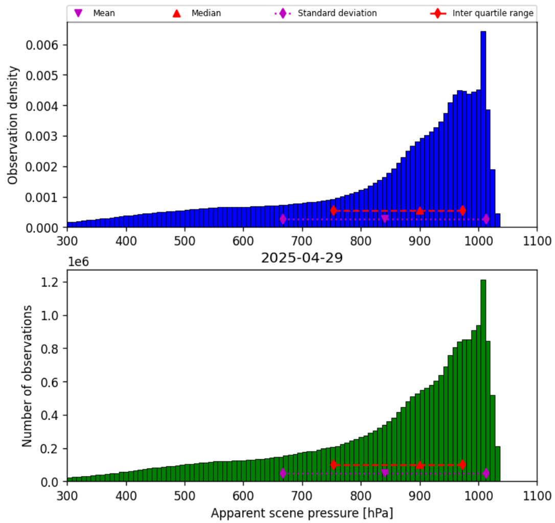
Figure 36: Histogram of “Apparent scene pressure” for 2025-04-29 to 2025-04-30
