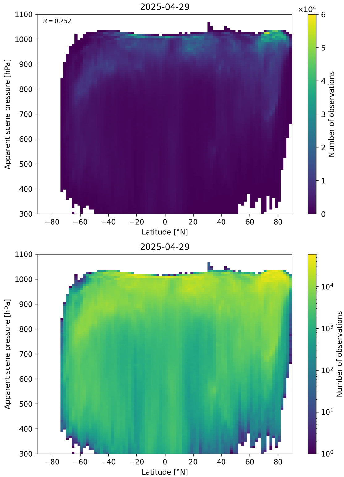
Figure 88: Scatter density plot of “Latitude” against “Apparent scene pressure” for 2025-04-29 to 2025-04-30.
