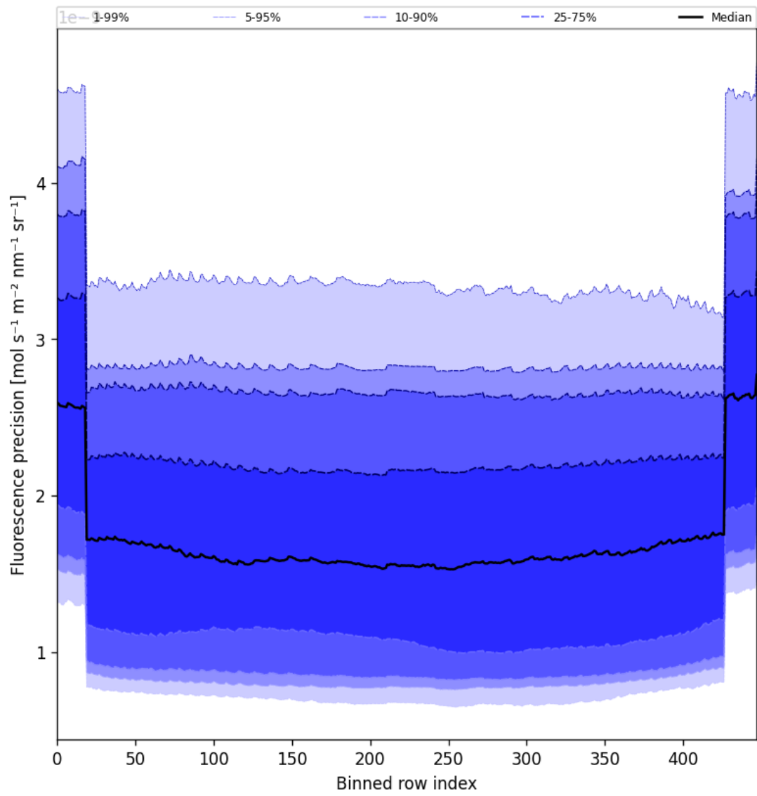
Figure 58: Along track statistics of “Fluorescence precision” for 2025-04-29 to 2025-04-30
