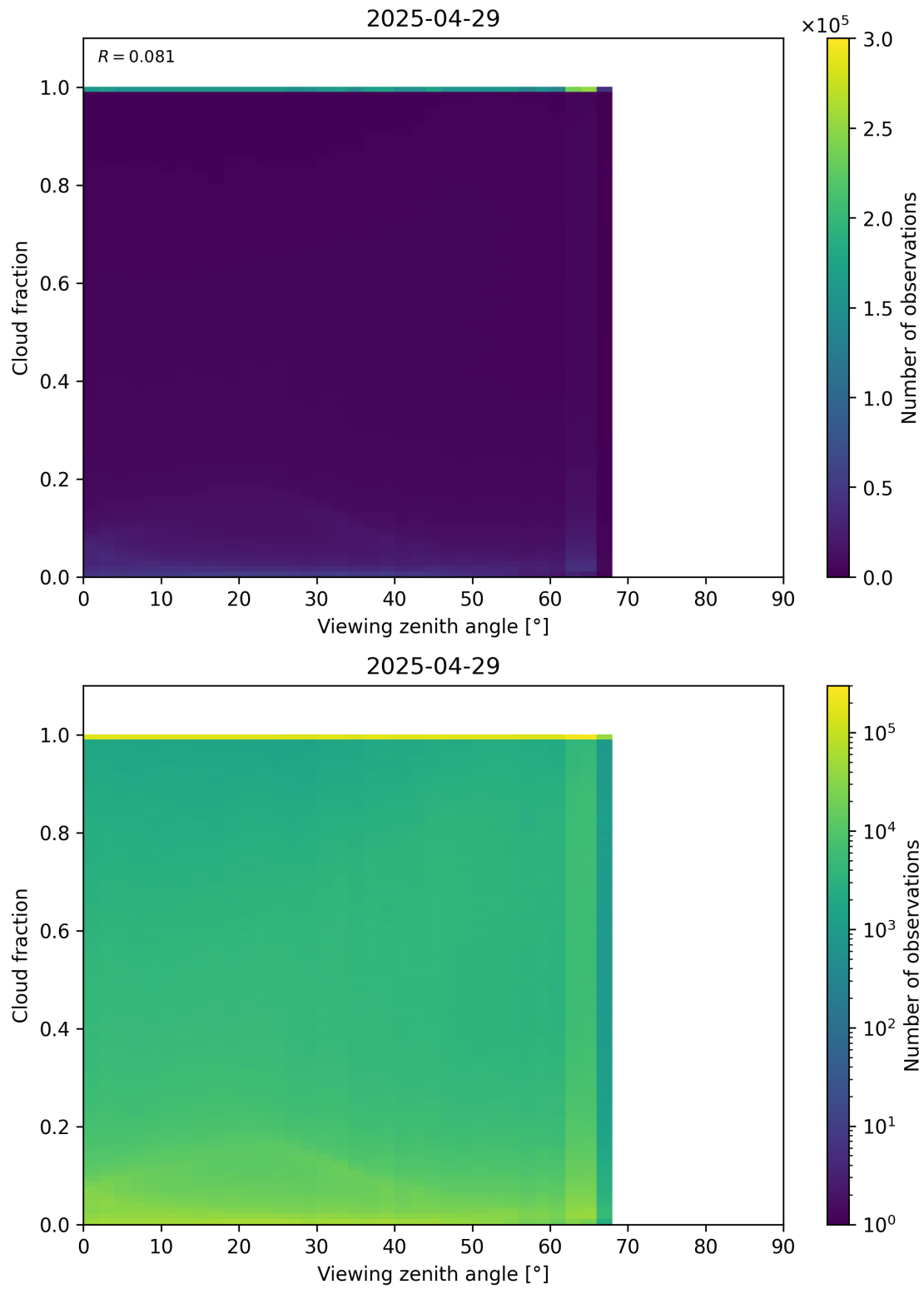
Figure 120: Scatter density plot of “Viewing zenith angle” against “Cloud fraction” for 2025-04-29 to 2025-04-30.
