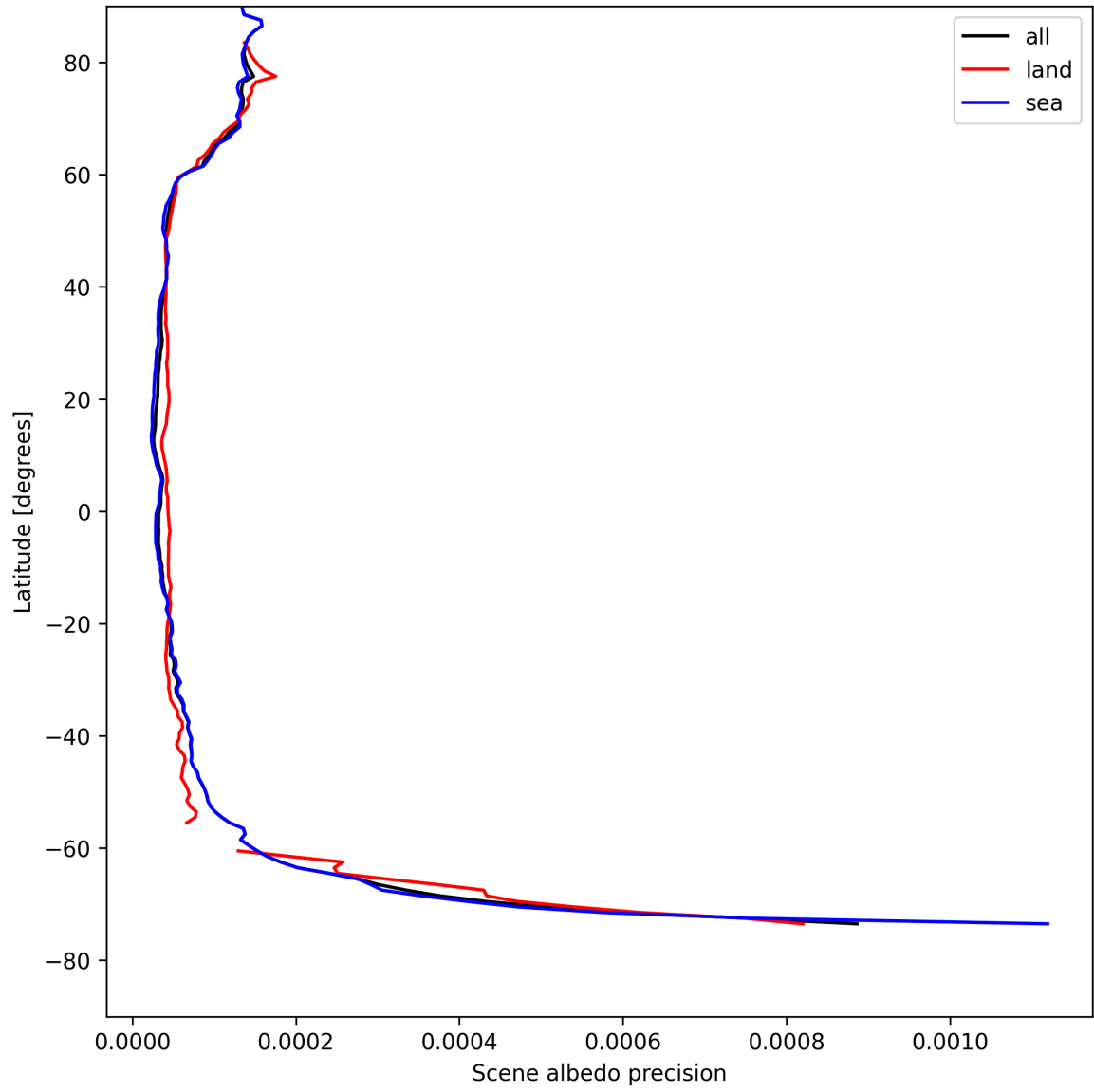
Figure 18: Zonal average of “Scene albedo precision” for 2025-04-29 to 2025-04-30.
