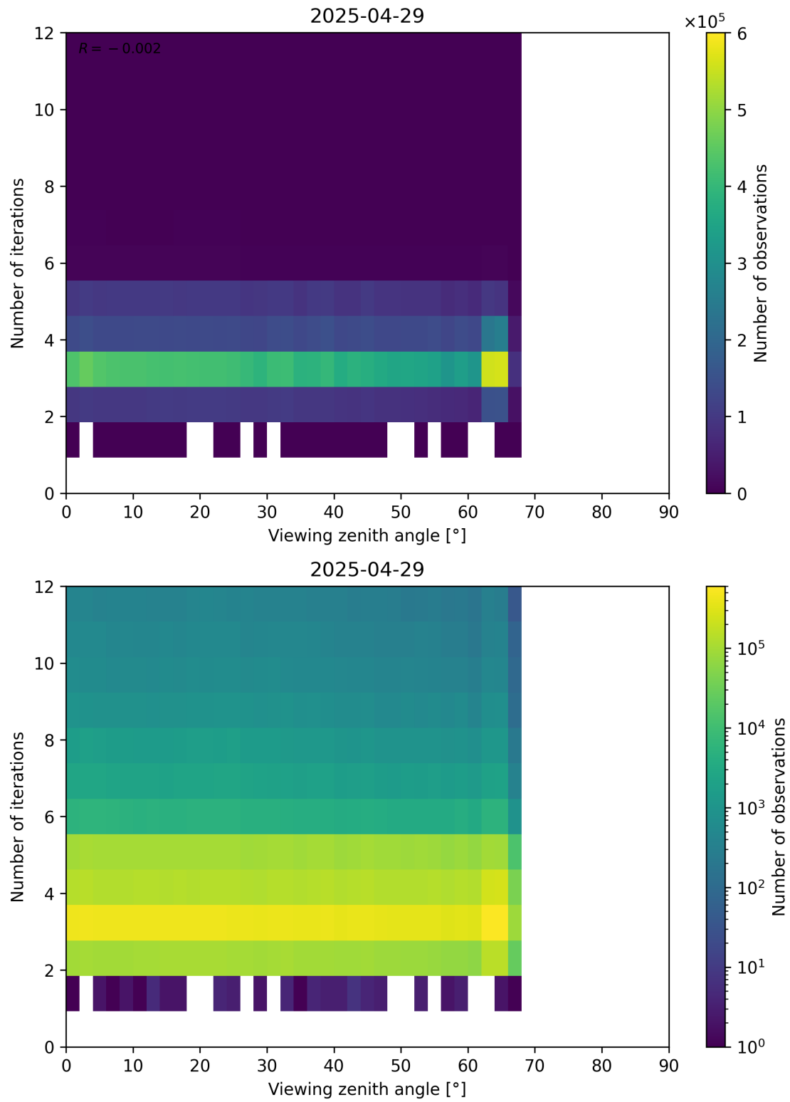
Figure 124: Scatter density plot of “Viewing zenith angle” against “Number of iterations” for 2025-04-29 to 2025-04-30.
