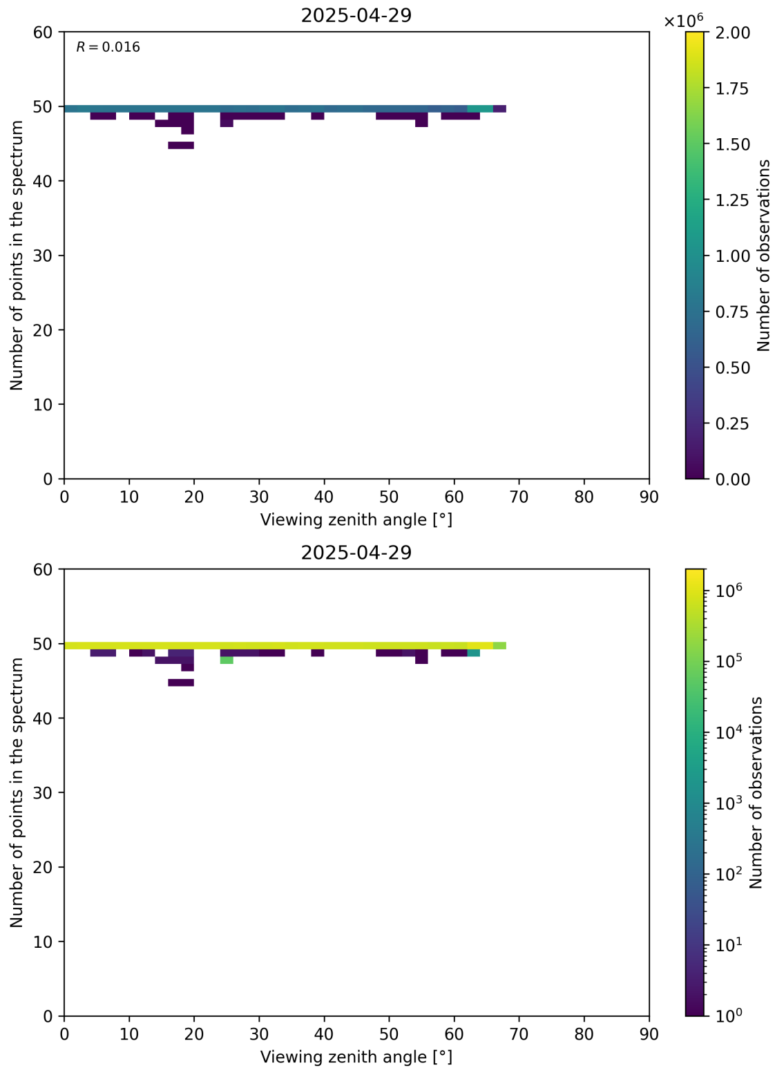
Figure 125: Scatter density plot of “Viewing zenith angle” against “Number of points in the spectrum” for 2025-04-29 to 2025-04-30.
