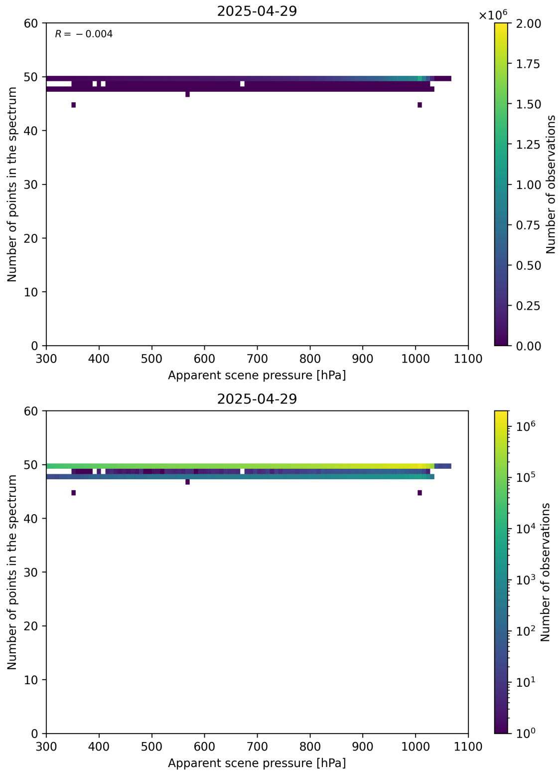
Figure 66: Scatter density plot of “Apparent scene pressure” against “Number of points in the spectrum” for 2025-04-29 to 2025-04-30.
