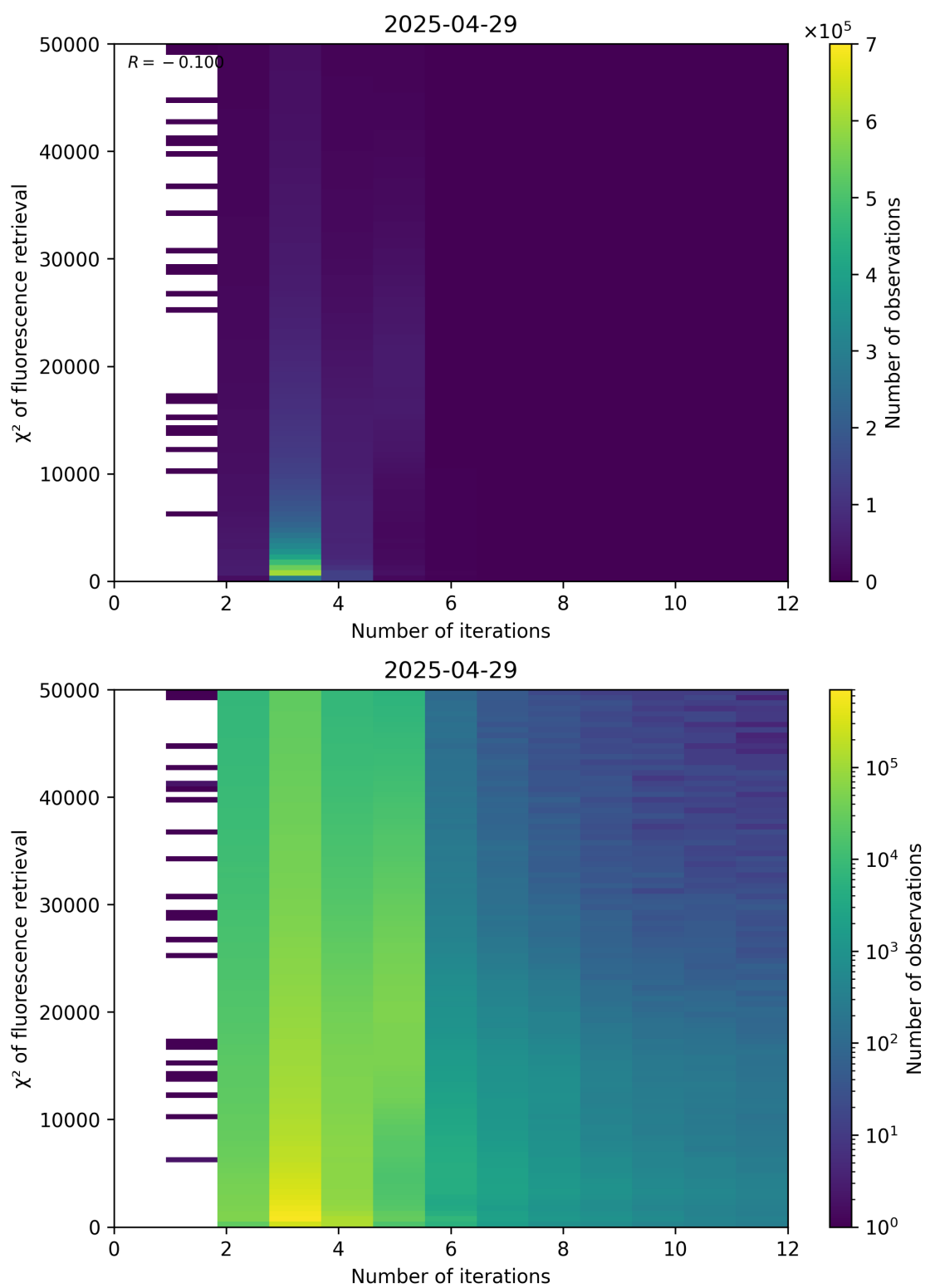
Figure 97: Scatter density plot of “Number of iterations” against “ \chi^2 of fluorescence retrieval” for 2025-04-29 to 2025-04-30.
