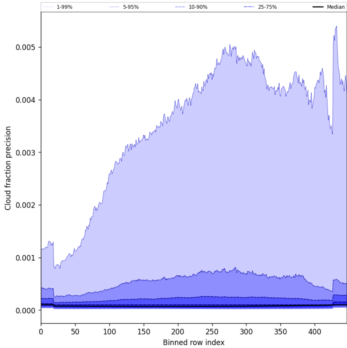
Figure 50: Along track statistics of “Cloud fraction precision” for 2025-04-29 to 2025-04-30
