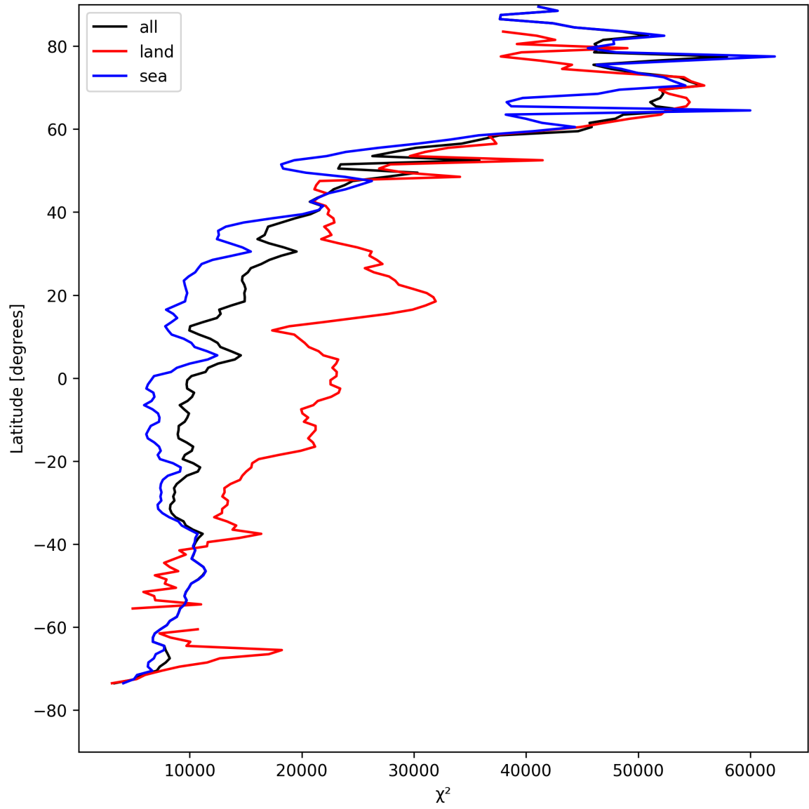
Figure 21: Zonal average of “ \chi^2 ” for 2025-04-29 to 2025-04-30.
