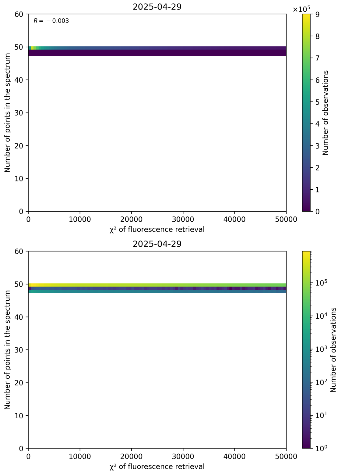
Figure 68: Scatter density plot of “ \chi^2 of fluorescence retrieval” against “Number of points in the spectrum” for 2025-04-29 to 2025-04-30.
