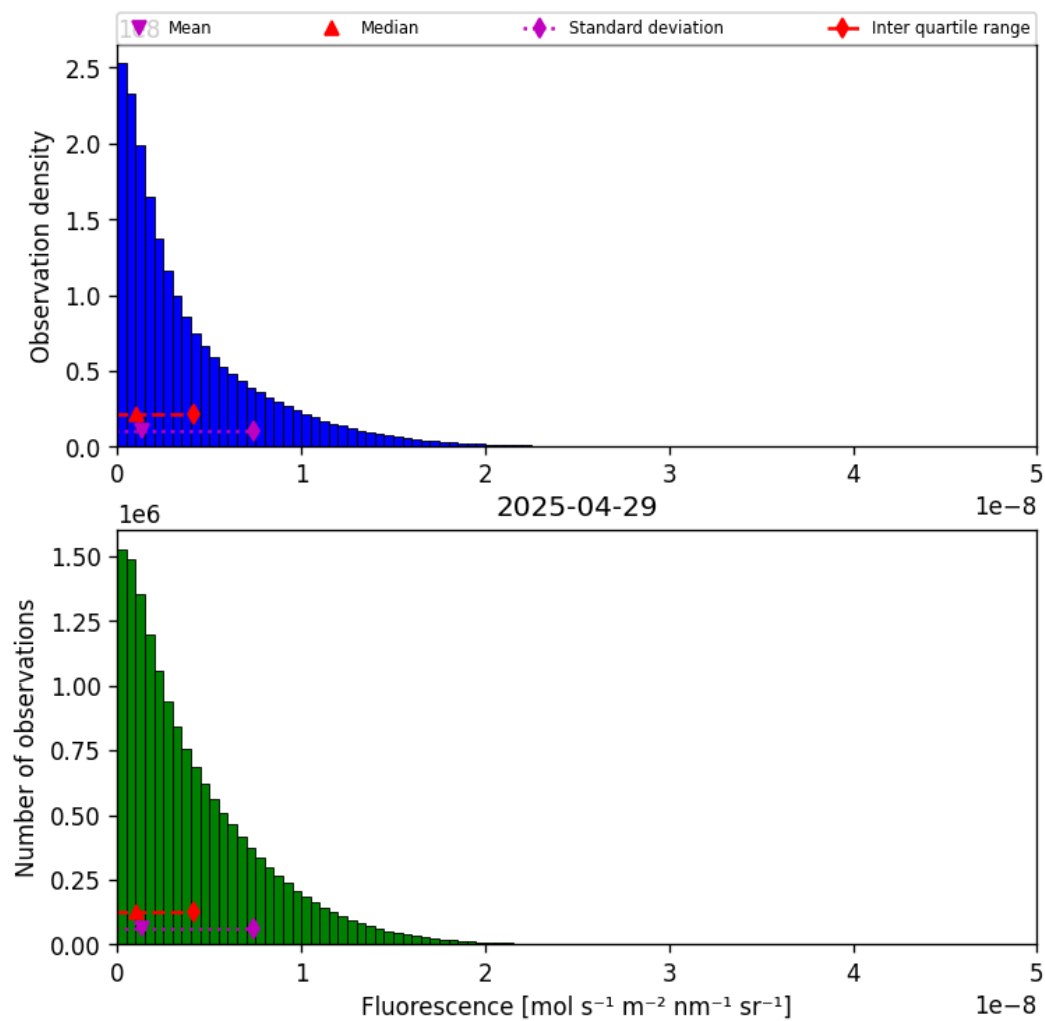
Figure 40: Histogram of “Fluorescence” for 2025-04-29 to 2025-04-30
