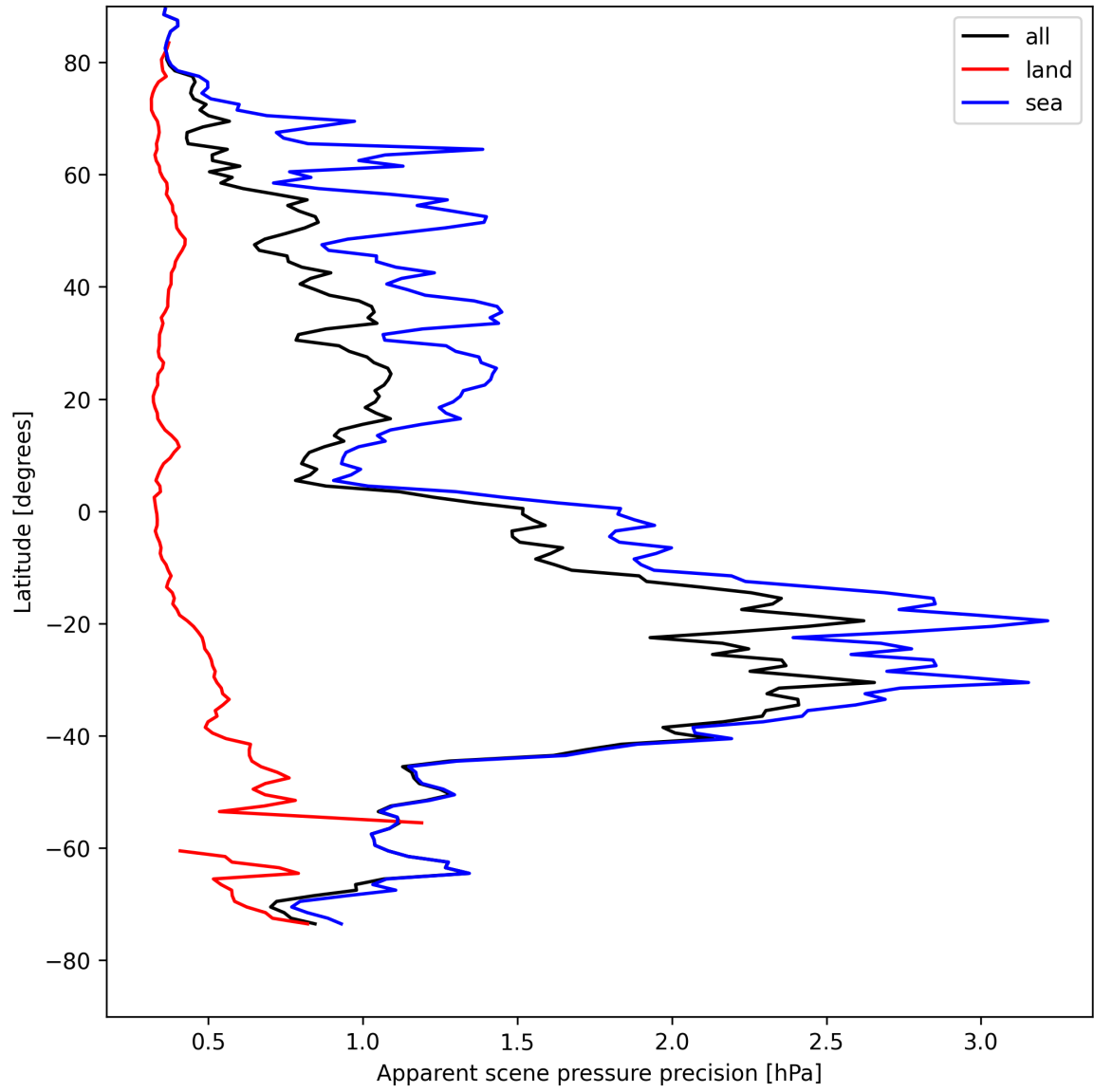
Figure 20: Zonal average of “Apparent scene pressure precision” for 2025-04-29 to 2025-04-30.
