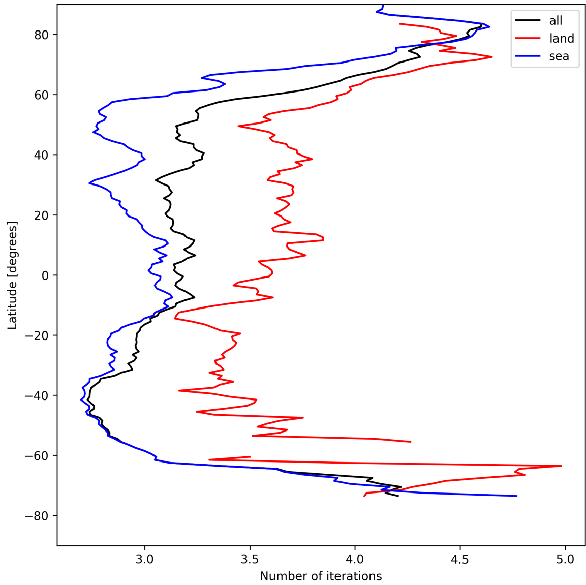
Figure 22: Zonal average of “Number of iterations” for 2025-04-29 to 2025-04-30.
