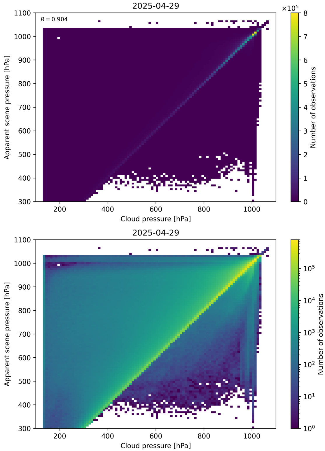
Figure 77: Scatter density plot of “Cloud pressure” against “Apparent scene pressure” for 2025-04-29 to 2025-04-30.
