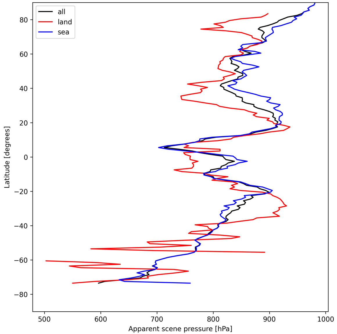
Figure 19: Zonal average of “Apparent scene pressure” for 2025-04-29 to 2025-04-30.
