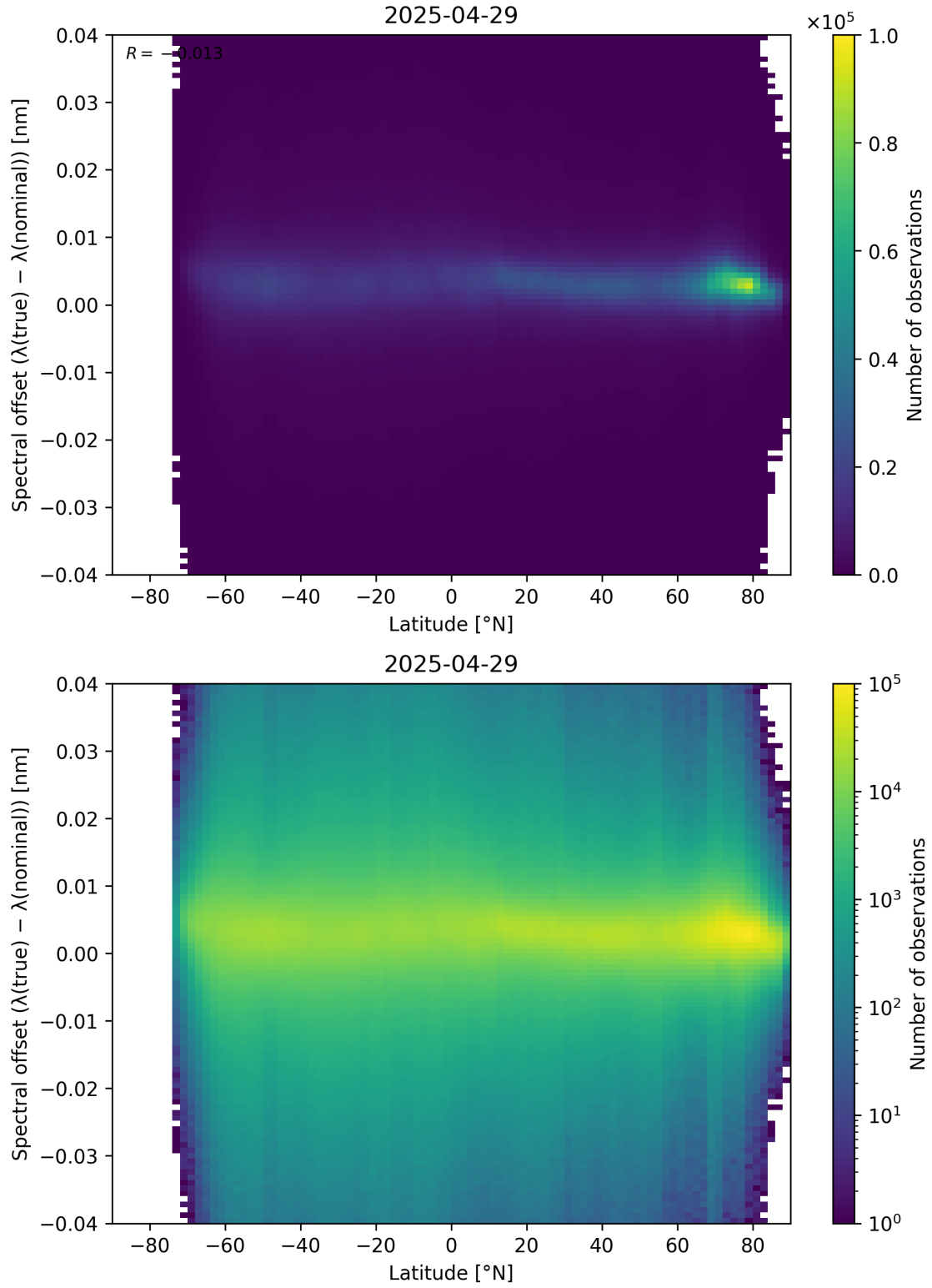
Figure 96: Scatter density plot of “Latitude” against “Spectral offset ( \lambda_{\text{true}} - \lambda_{\text{nominal}} )” for 2025-04-29 to 2025-04-30.
