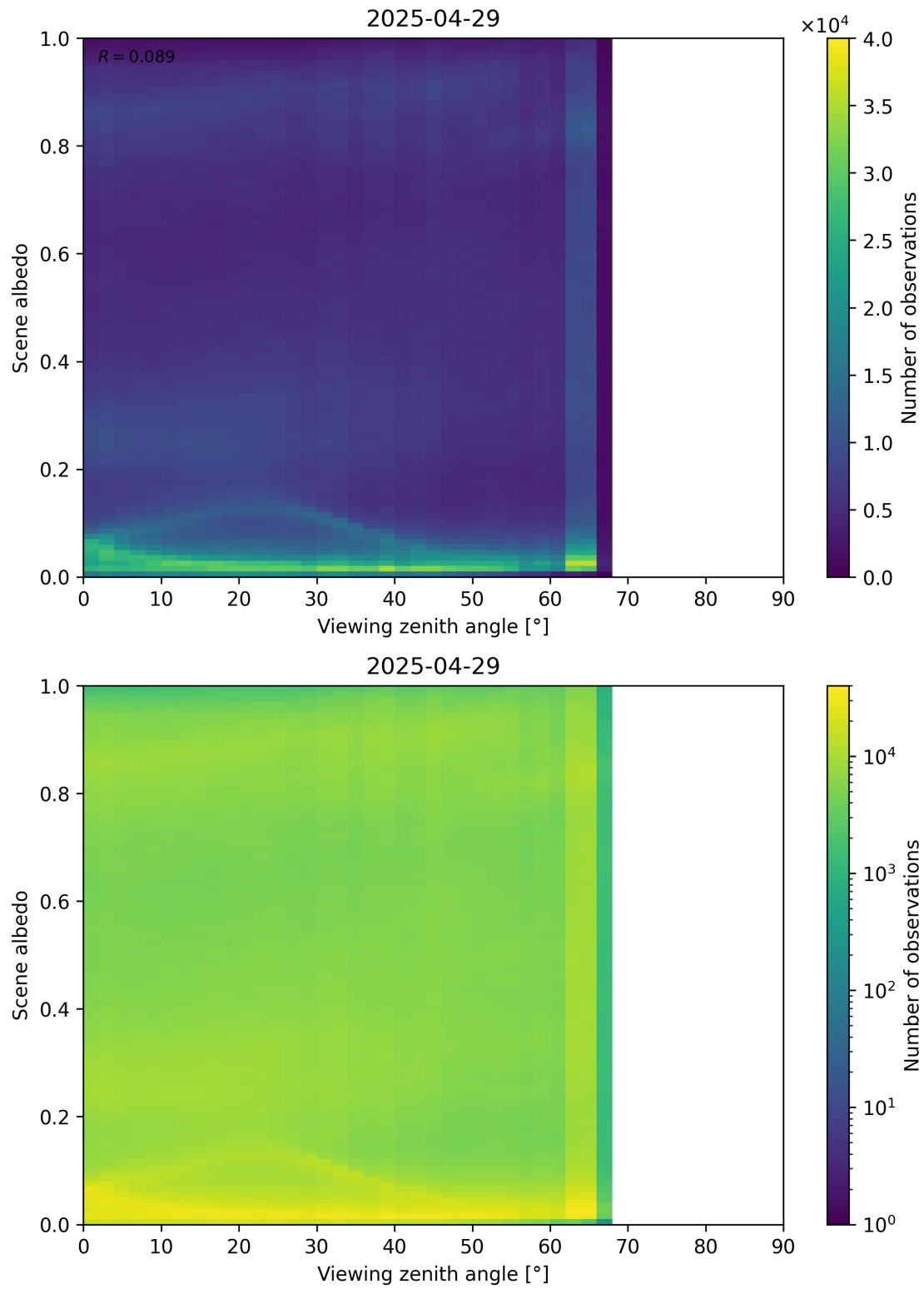
Figure 126: Scatter density plot of “Viewing zenith angle” against “Scene albedo” for 2025-04-29 to 2025-04-30.
