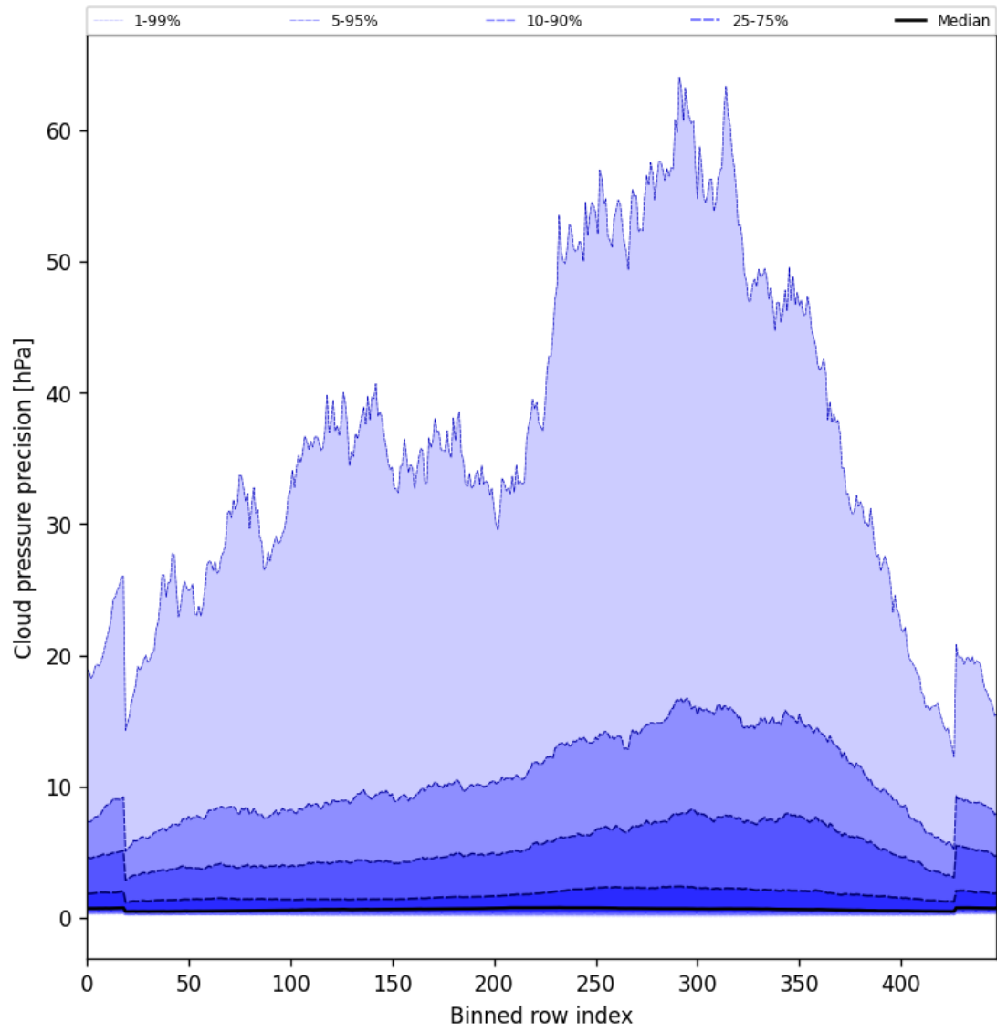
Figure 48: Along track statistics of “Cloud pressure precision” for 2025-04-29 to 2025-04-30
