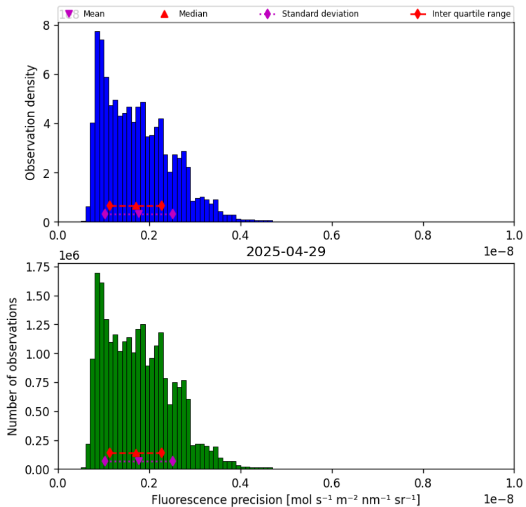
Figure 41: Histogram of “Fluorescence precision” for 2025-04-29 to 2025-04-30
