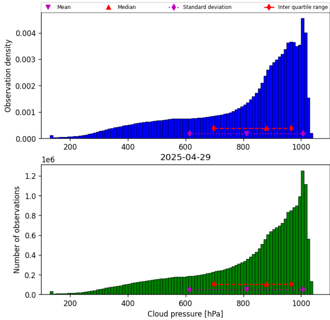
Figure 30: Histogram of “Cloud pressure” for 2025-04-29 to 2025-04-30
