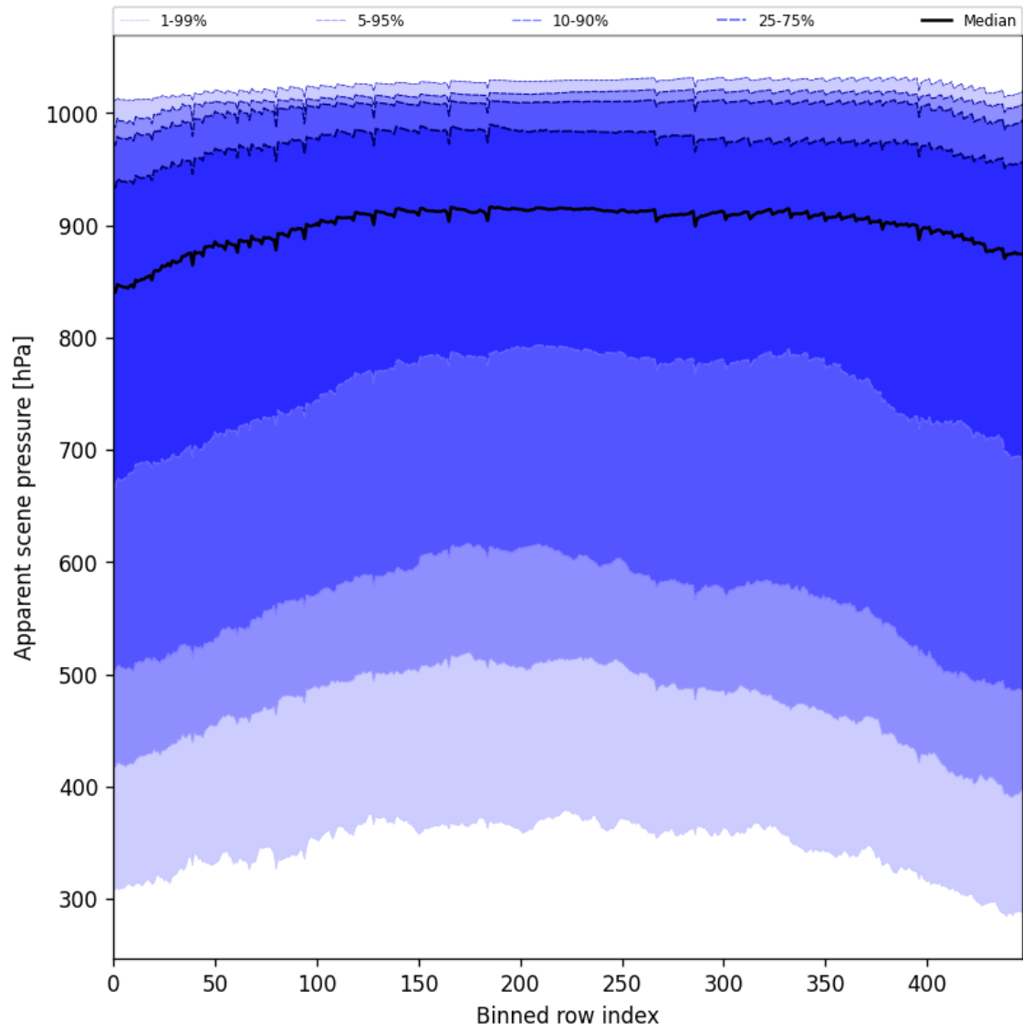
Figure 53: Along track statistics of “Apparent scene pressure” for 2025-04-29 to 2025-04-30
