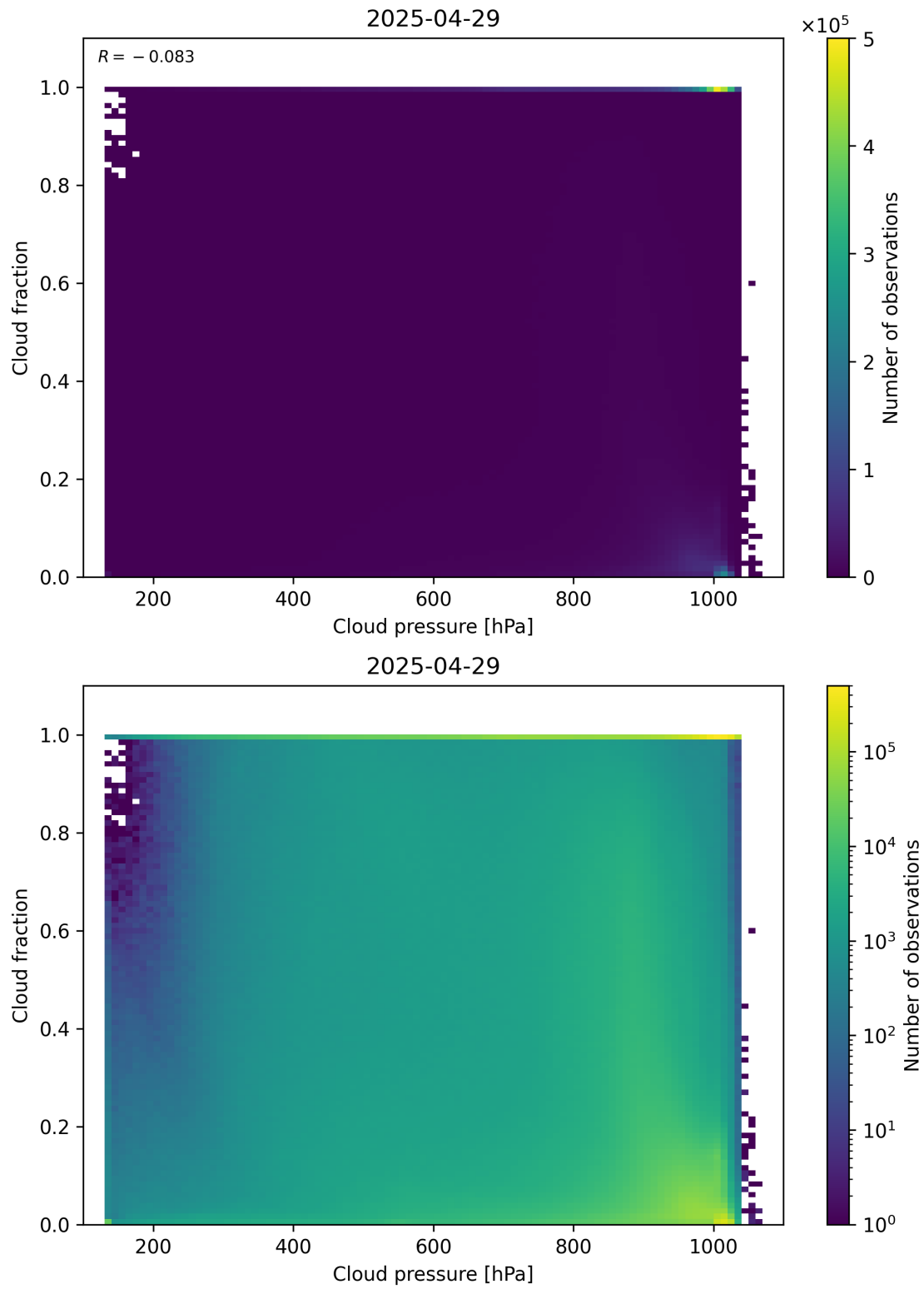
Figure 79: Scatter density plot of “Cloud pressure” against “Cloud fraction” for 2025-04-29 to 2025-04-30.
