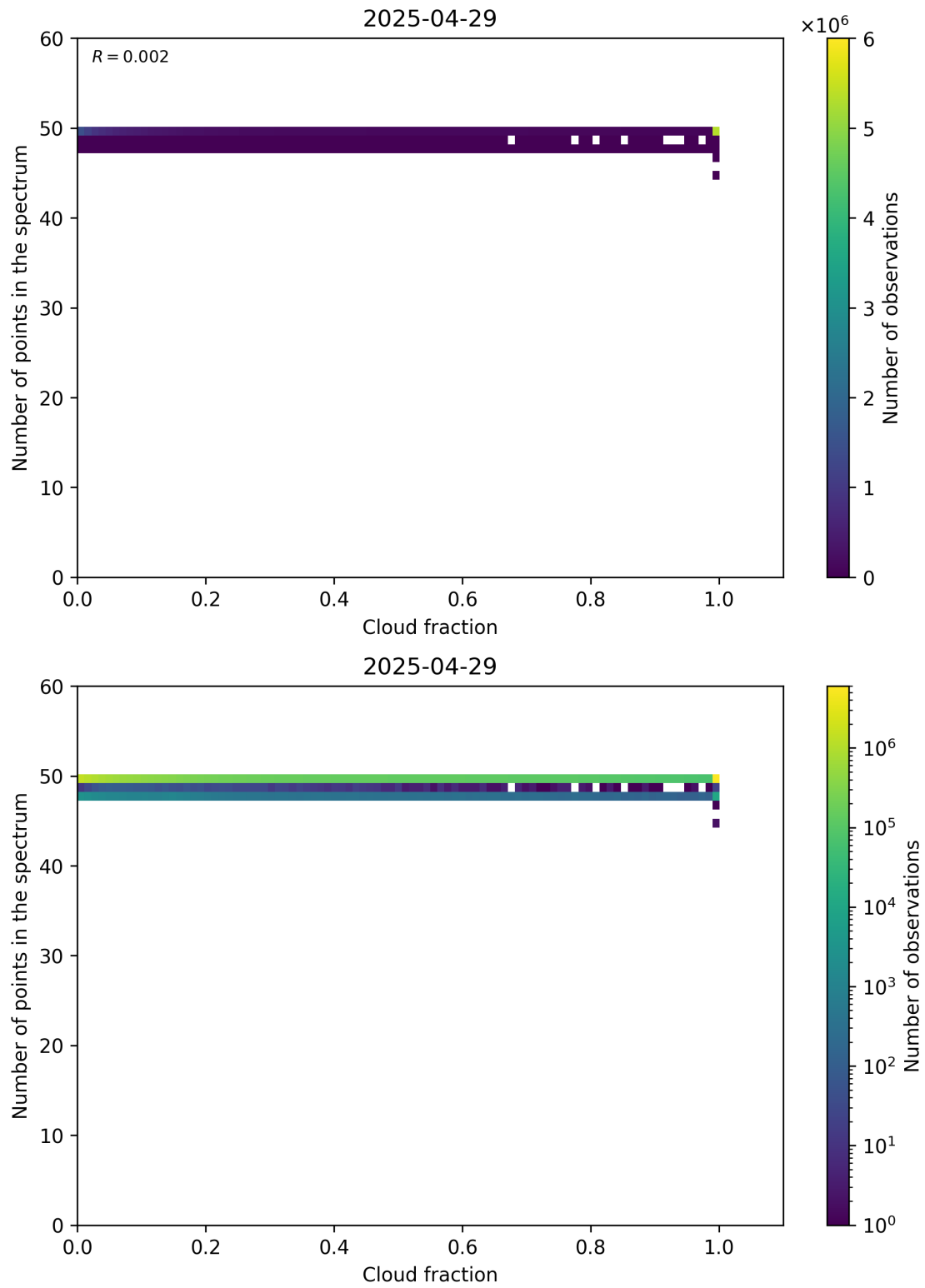
Figure 74: Scatter density plot of “Cloud fraction” against “Number of points in the spectrum” for 2025-04-29 to 2025-04-30.
