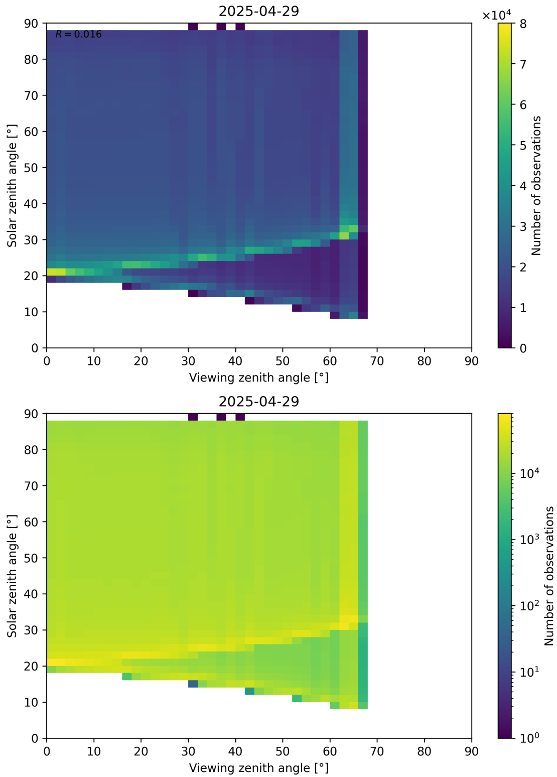
Figure 127: Scatter density plot of “Viewing zenith angle” against “Solar zenith angle” for 2025-04-29 to 2025-04-30.
