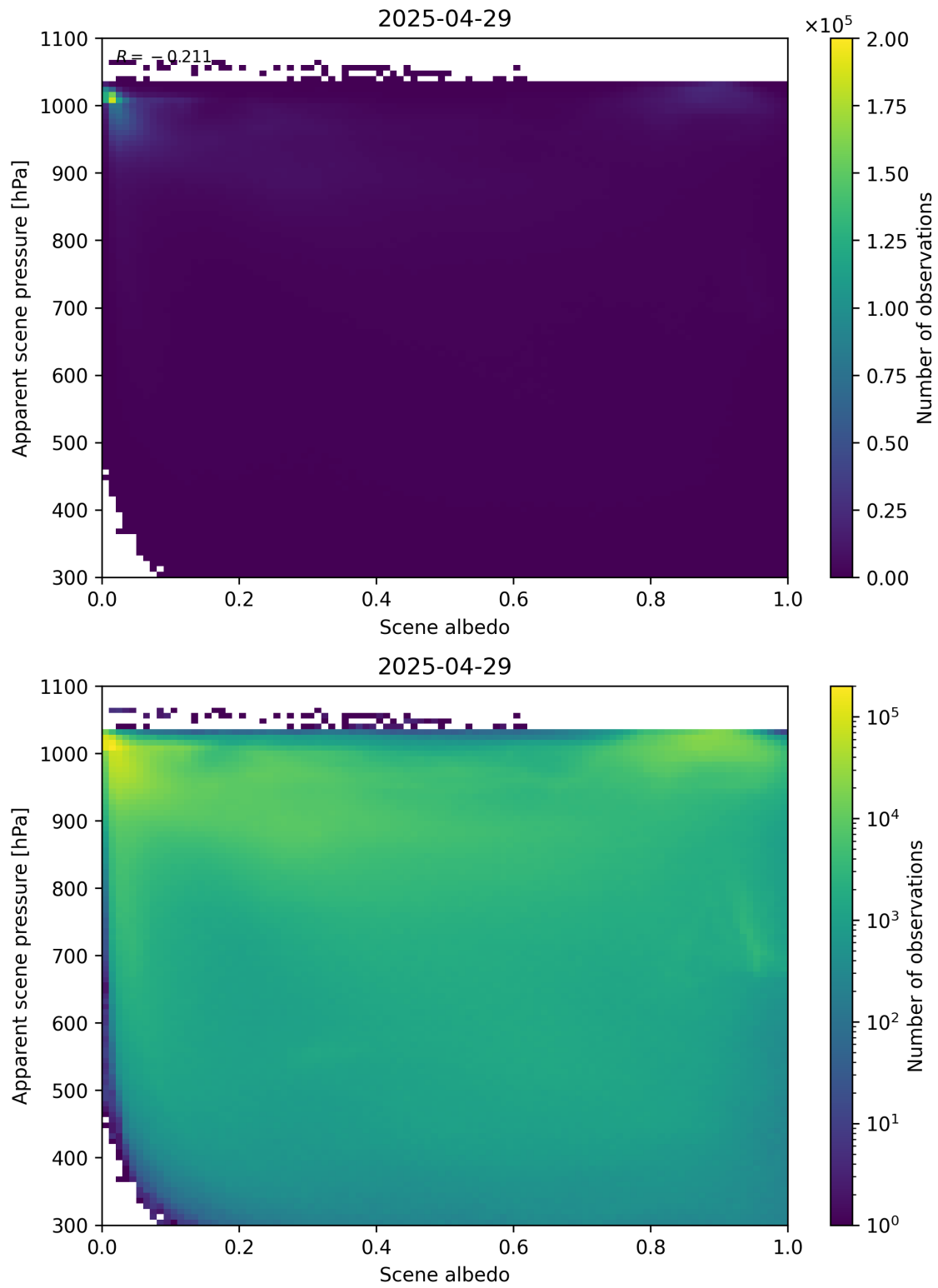
Figure 102: Scatter density plot of “Scene albedo” against “Apparent scene pressure” for 2025-04-29 to 2025-04-30.
