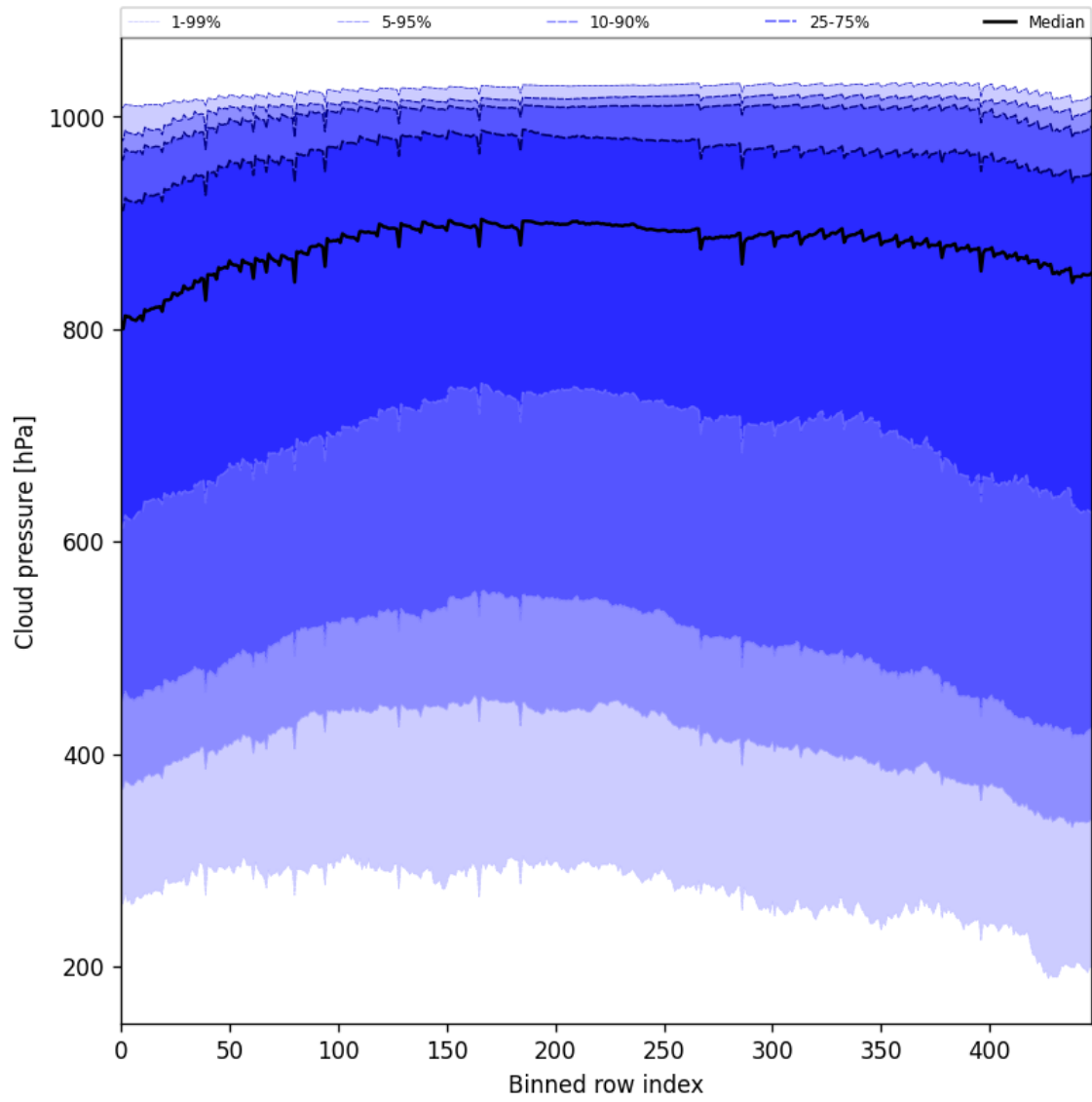
Figure 47: Along track statistics of “Cloud pressure” for 2025-04-29 to 2025-04-30
