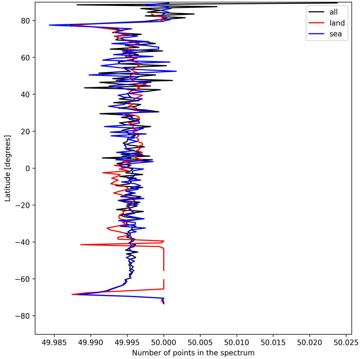
Figure 27: Zonal average of “Number of points in the spectrum” for 2025-04-29 to 2025-04-30.
