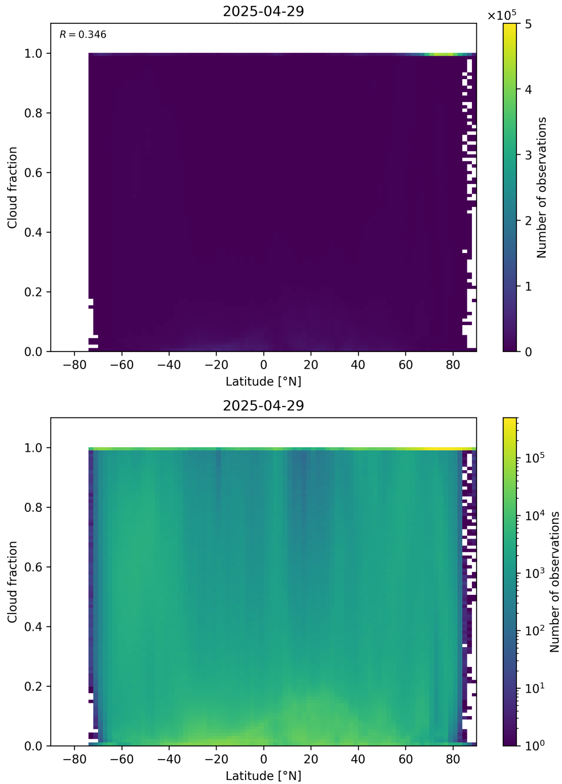
Figure 90: Scatter density plot of “Latitude” against “Cloud fraction” for 2025-04-29 to 2025-04-30.
