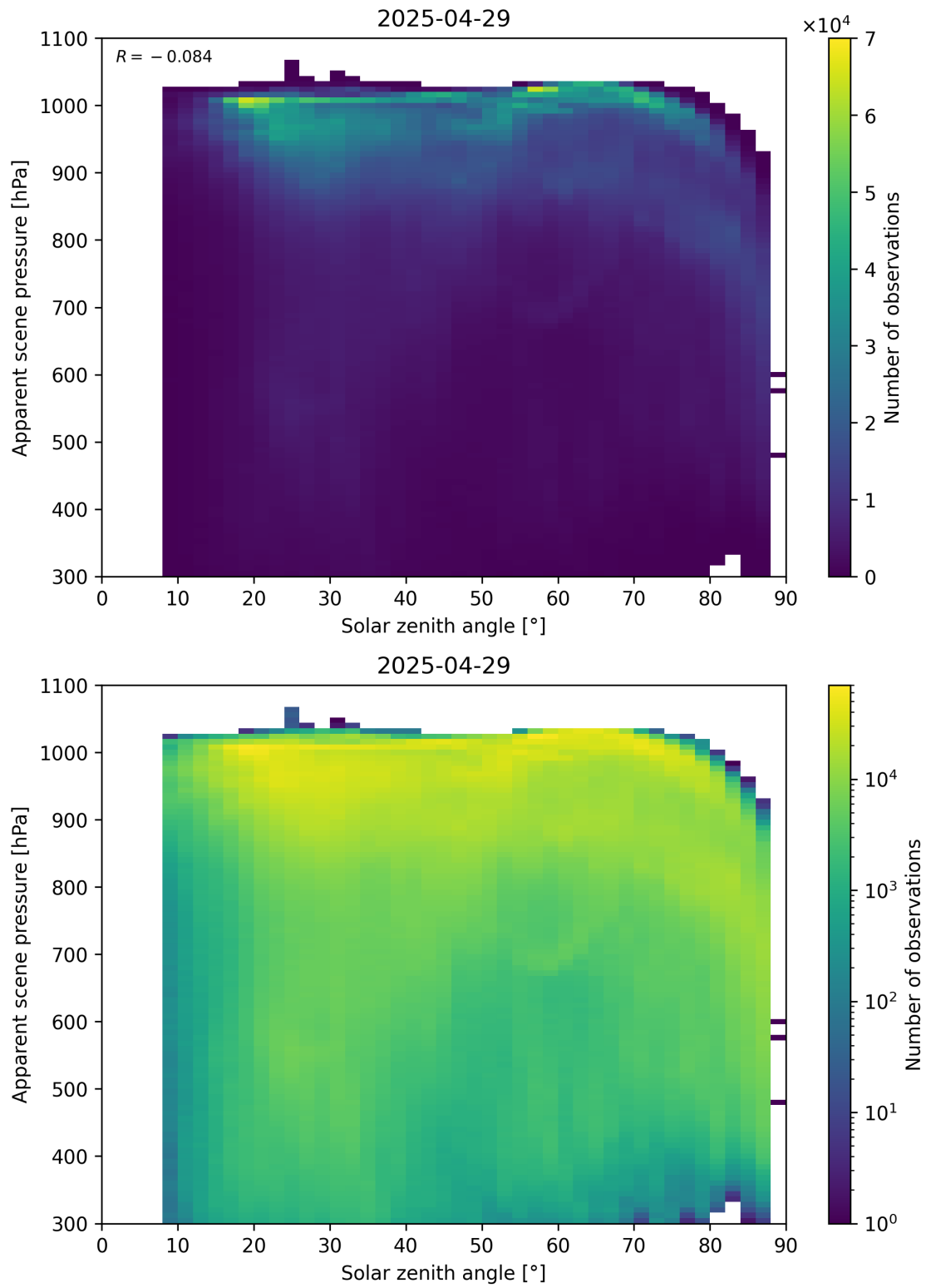
Figure 108: Scatter density plot of “Solar zenith angle” against “Apparent scene pressure” for 2025-04-29 to 2025-04-30.
