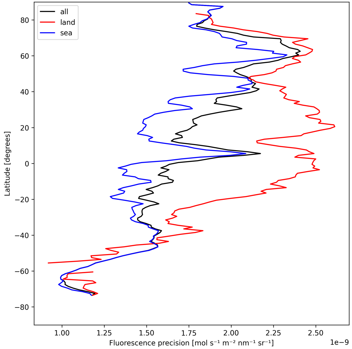
Figure 24: Zonal average of "Fluorescence precision" for 2025-04-29 to 2025-04-30.
