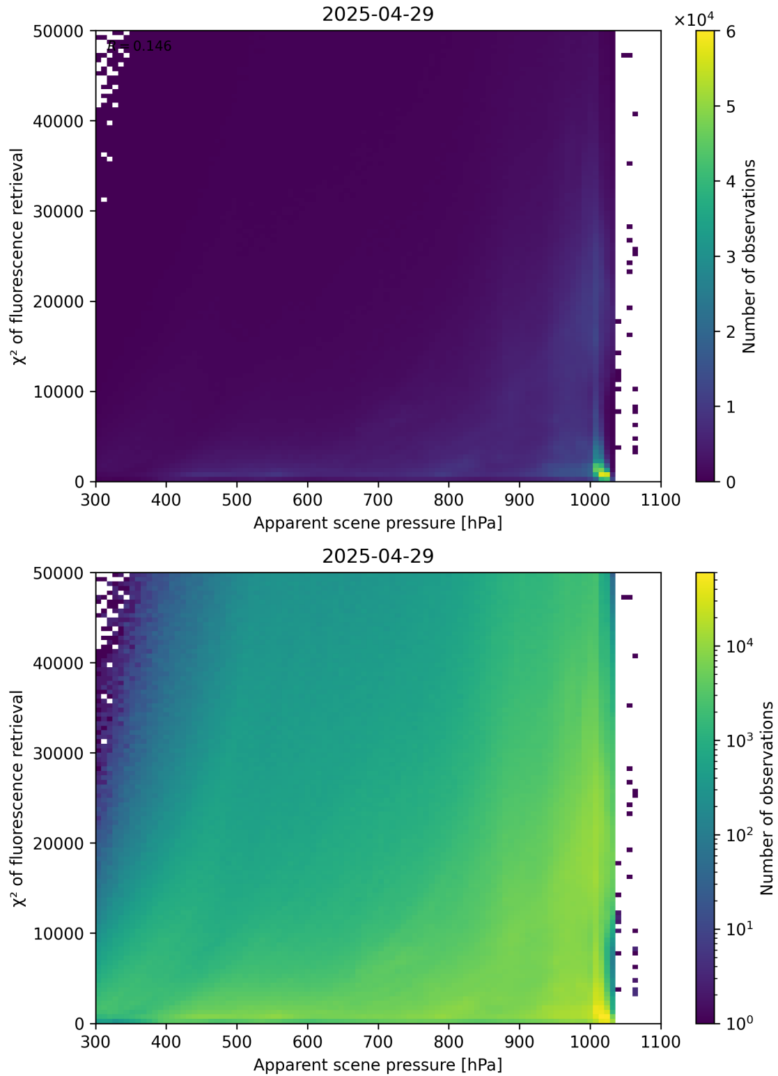
Figure 63: Scatter density plot of “Apparent scene pressure” against “ \chi^2 of fluorescence retrieval” for 2025-04-29 to 2025-04-30.
