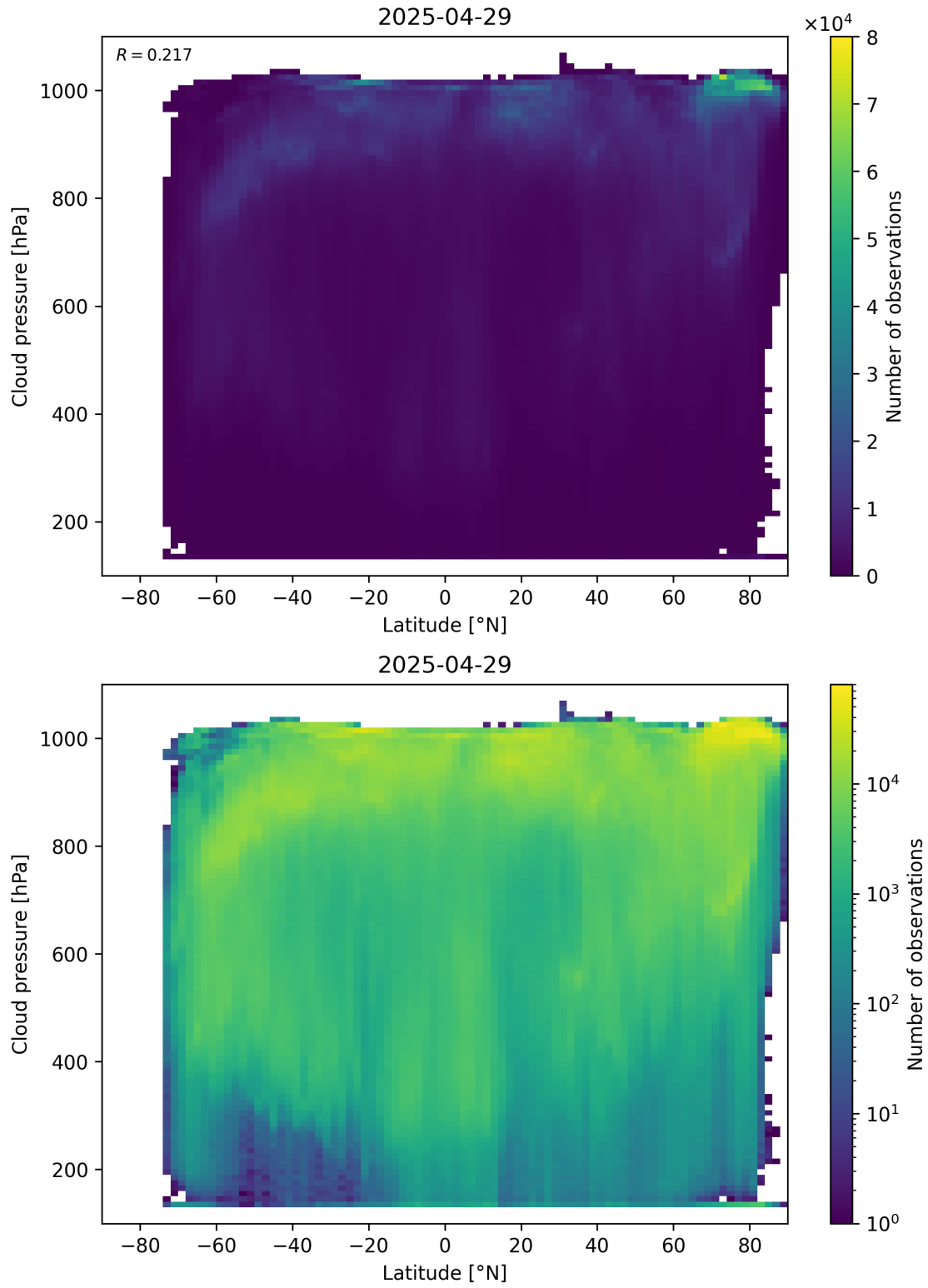
Figure 91: Scatter density plot of “Latitude” against “Cloud pressure” for 2025-04-29 to 2025-04-30.
