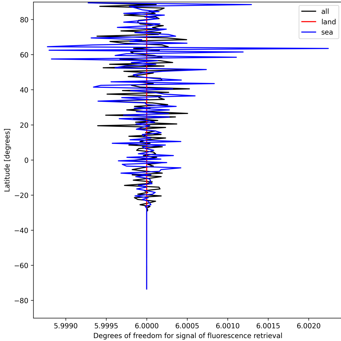
Figure 26: Zonal average of “Degrees of freedom for signal of fluorescence retrieval” for 2025-04-29 to 2025-04-30.
