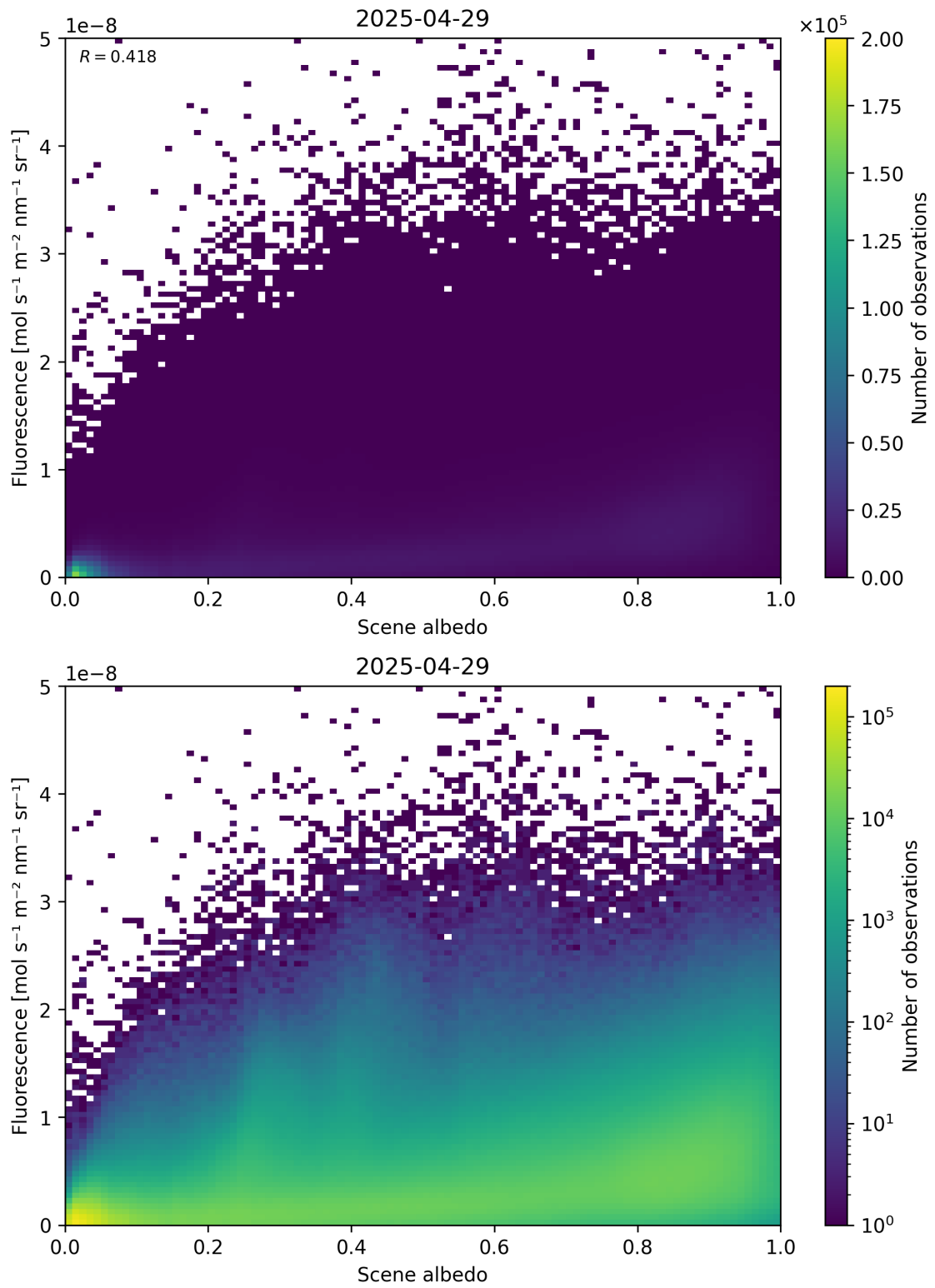
Figure 104: Scatter density plot of “Scene albedo” against “Fluorescence” for 2025-04-29 to 2025-04-30.
