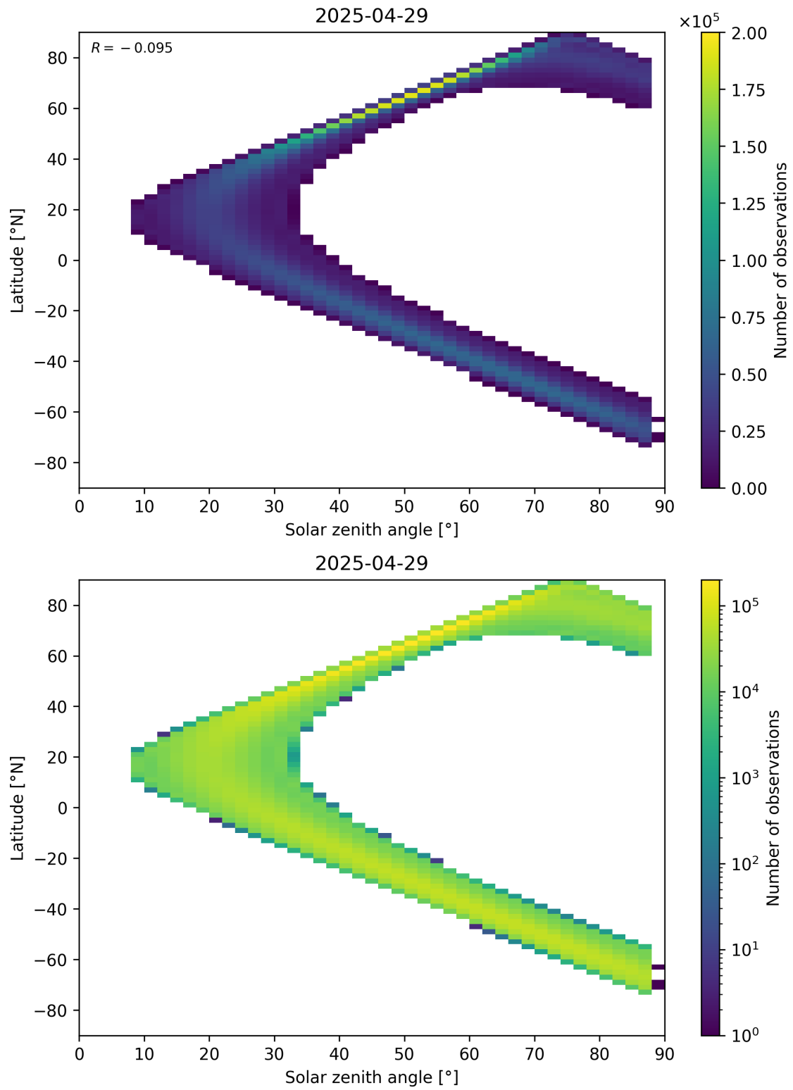
Figure 113: Scatter density plot of “Solar zenith angle” against “Latitude” for 2025-04-29 to 2025-04-30.
