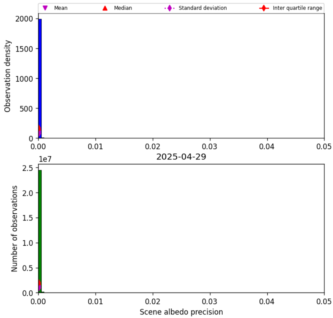
Figure 35: Histogram of “Scene albedo precision” for 2025-04-29 to 2025-04-30
