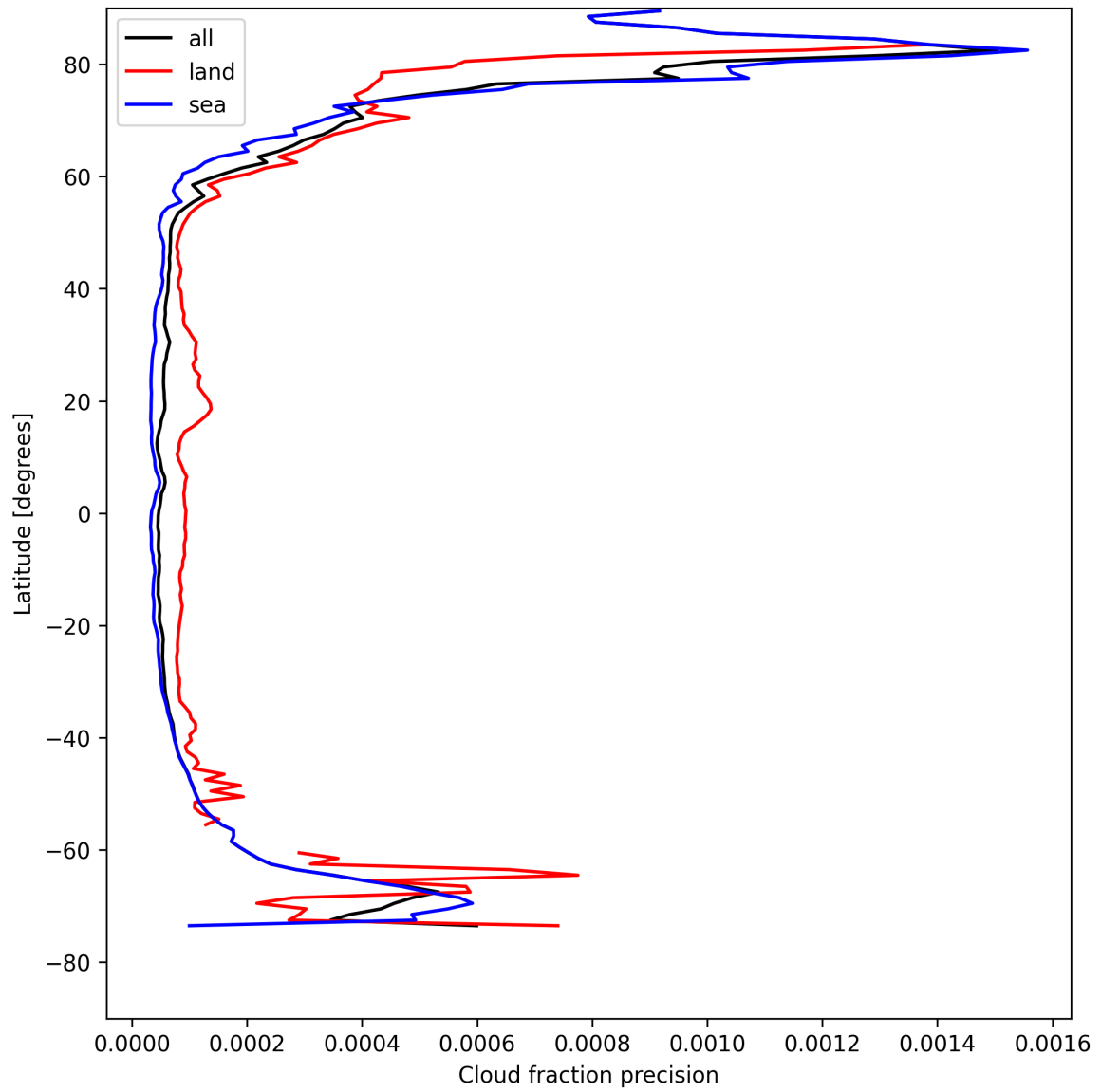
Figure 16: Zonal average of “Cloud fraction precision” for 2025-04-29 to 2025-04-30.
