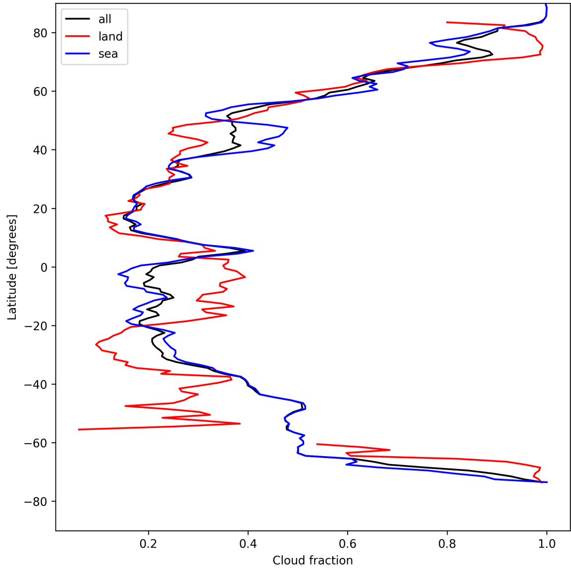
Figure 15: Zonal average of “Cloud fraction” for 2025-04-29 to 2025-04-30.
