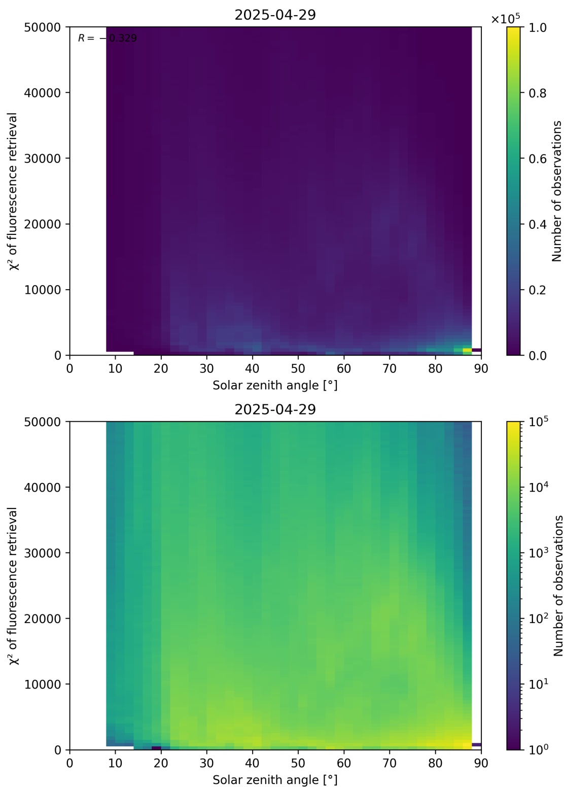
Figure 109: Scatter density plot of “Solar zenith angle” against “ \chi^2 of fluorescence retrieval” for 2025-04-29 to 2025-04-30.
