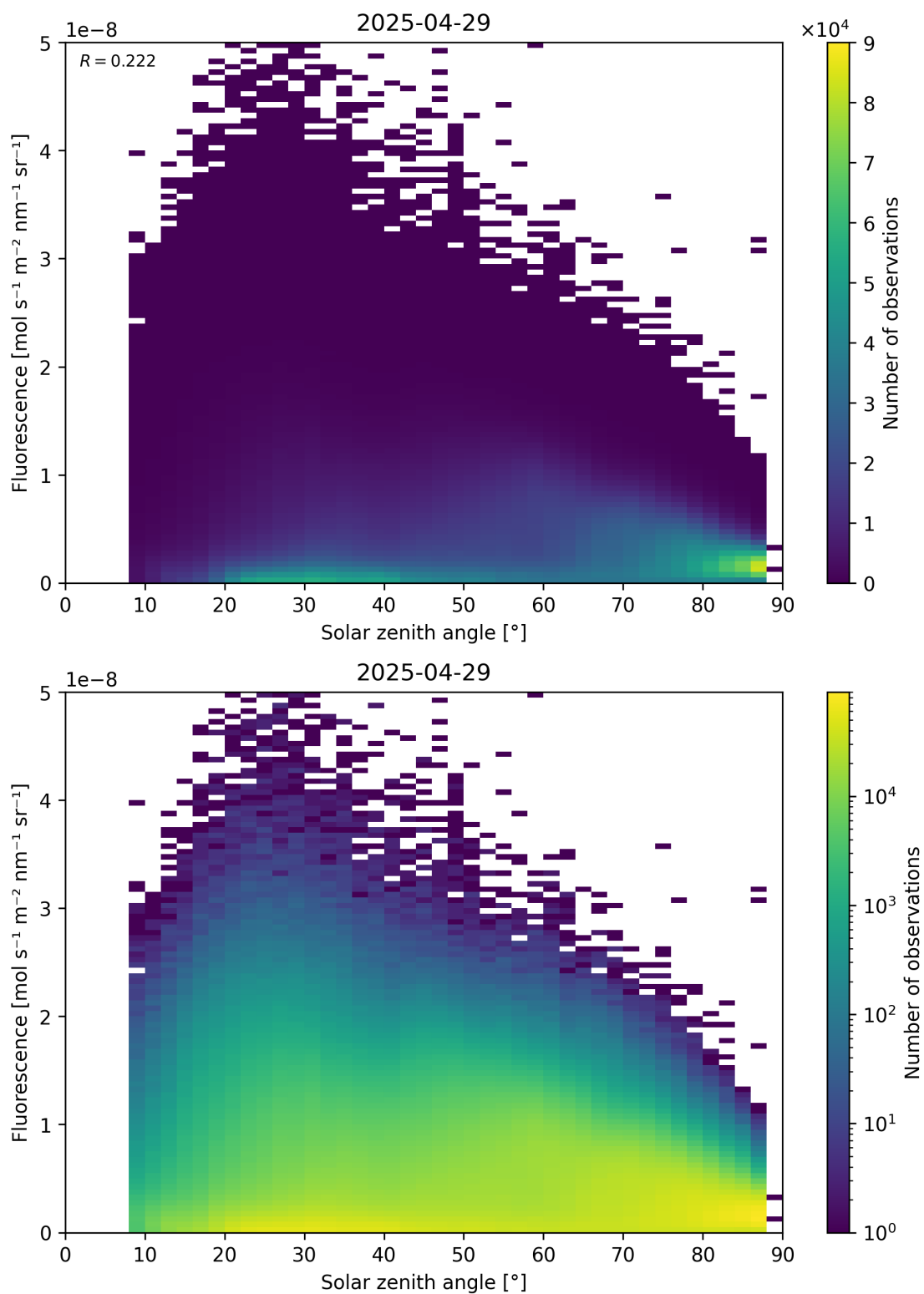
Figure 112: Scatter density plot of “Solar zenith angle” against “Fluorescence” for 2025-04-29 to 2025-04-30.
