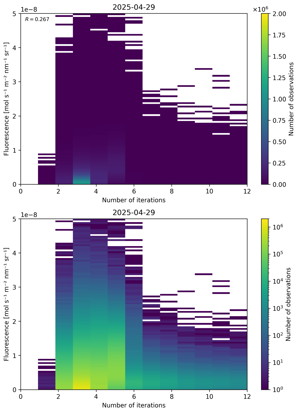
Figure 98: Scatter density plot of “Number of iterations” against “Fluorescence” for 2025-04-29 to 2025-04-30.
