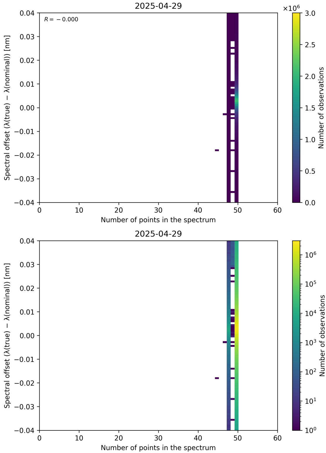
Figure 101: Scatter density plot of “Number of points in the spectrum” against “Spectral offset ( \lambda_{\text{true}} - \lambda_{\text{nominal}} )” for 2025-04-29 to 2025-04-30.
