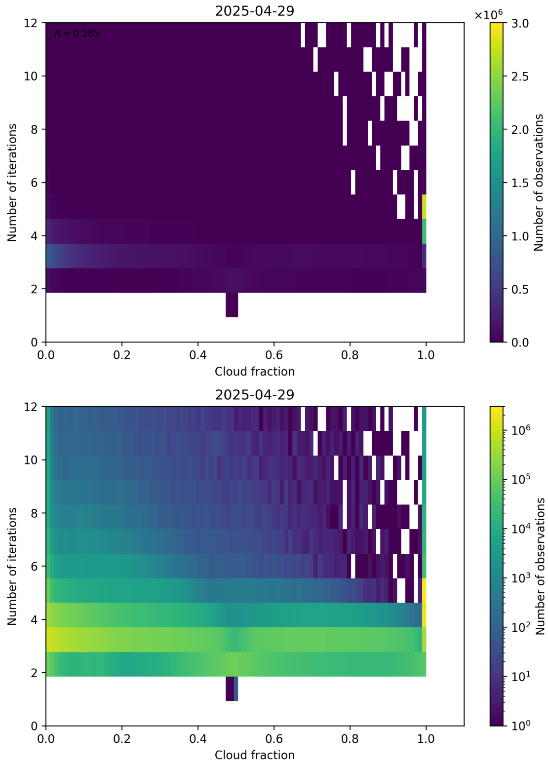
Figure 73: Scatter density plot of “Cloud fraction” against “Number of iterations” for 2025-04-29 to 2025-04-30.
