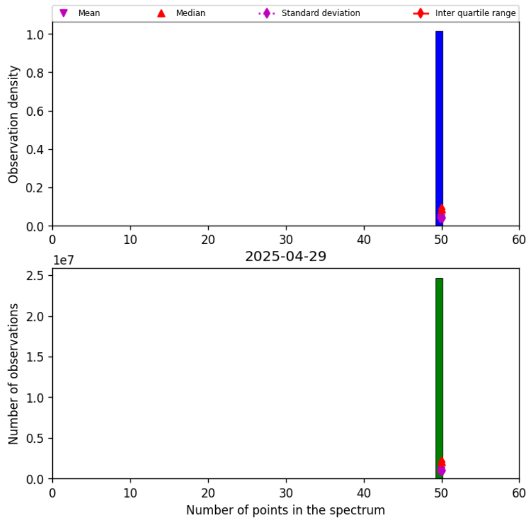
Figure 44: Histogram of “Number of points in the spectrum” for 2025-04-29 to 2025-04-30
