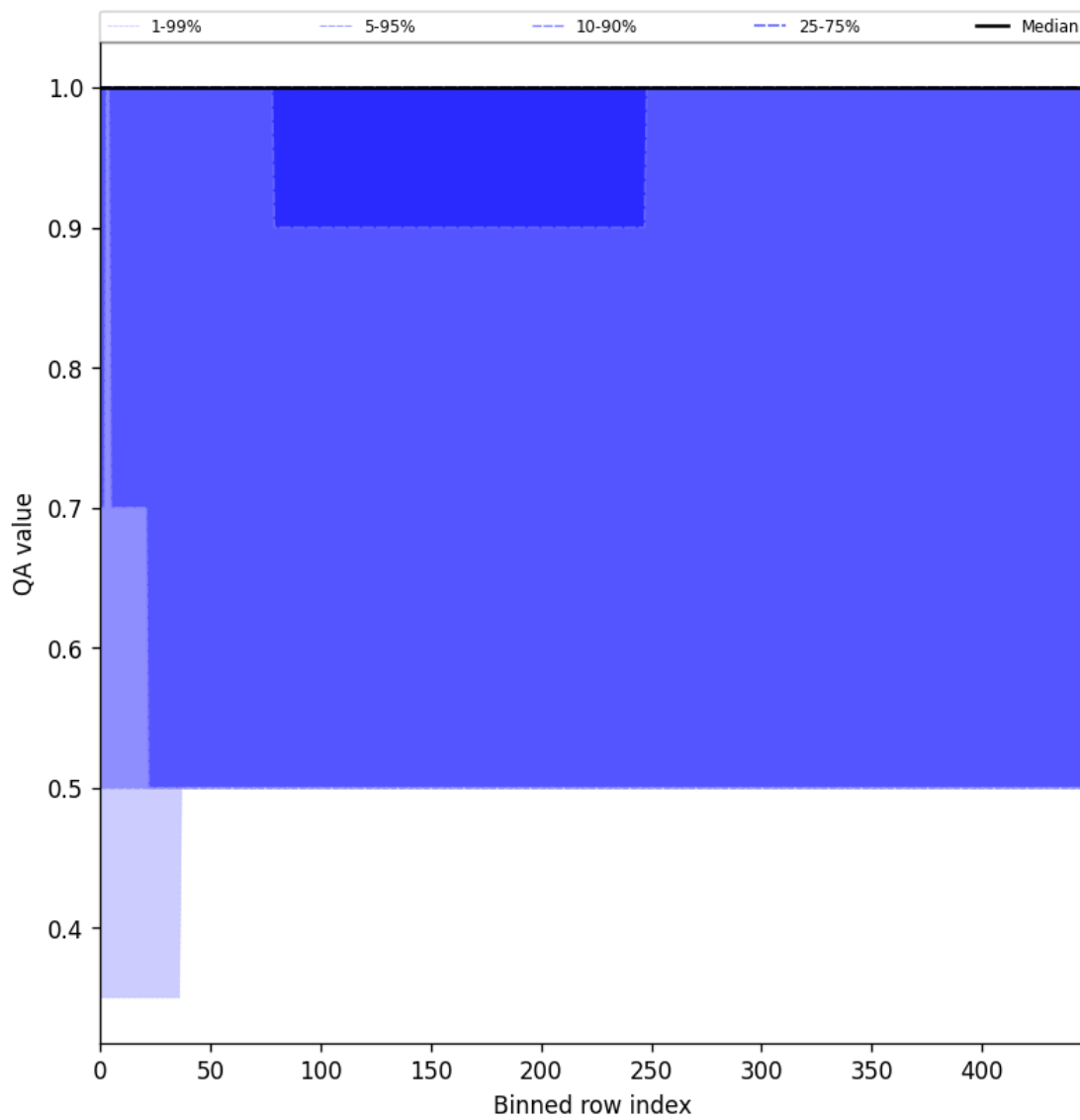
Figure 46: Along track statistics of “QA value” for 2025-04-29 to 2025-04-30
