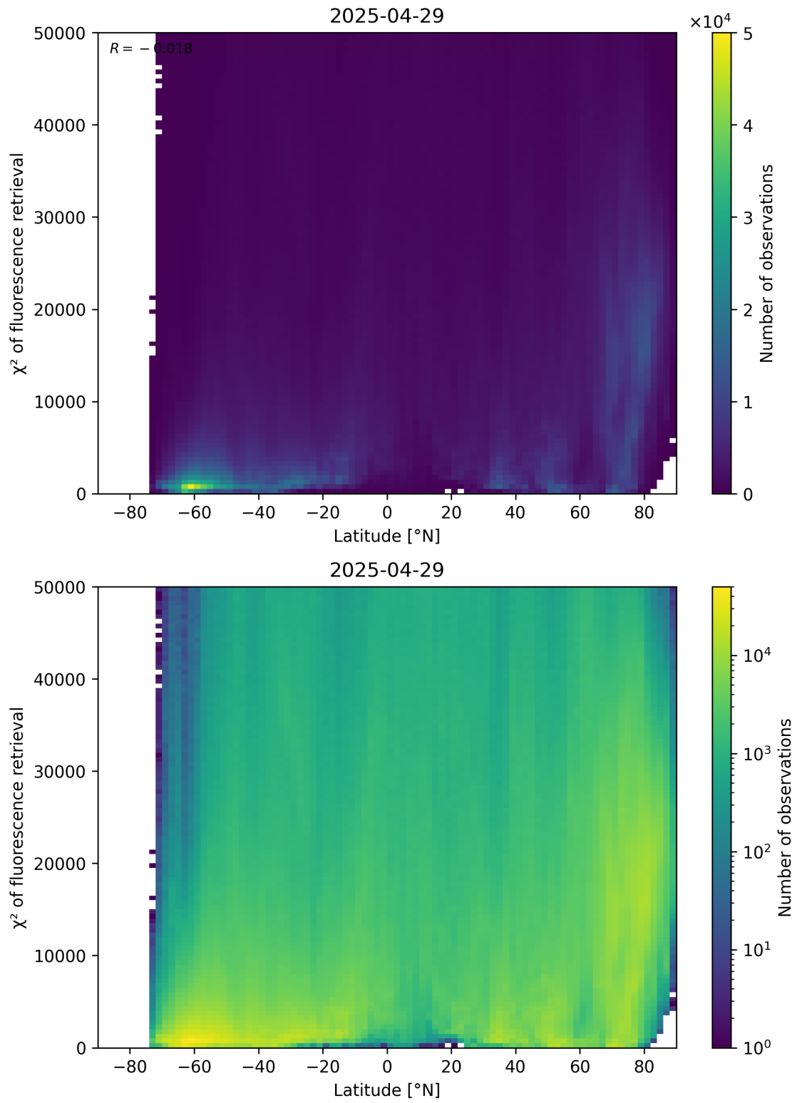
Figure 89: Scatter density plot of “Latitude” against “ \chi^2 of fluorescence retrieval” for 2025-04-29 to 2025-04-30.
