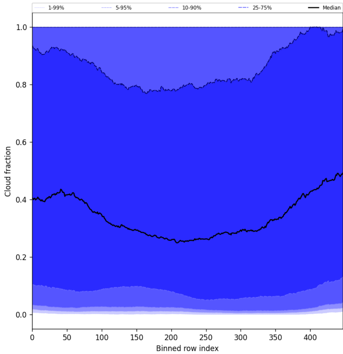
Figure 49: Along track statistics of “Cloud fraction” for 2025-04-29 to 2025-04-30
