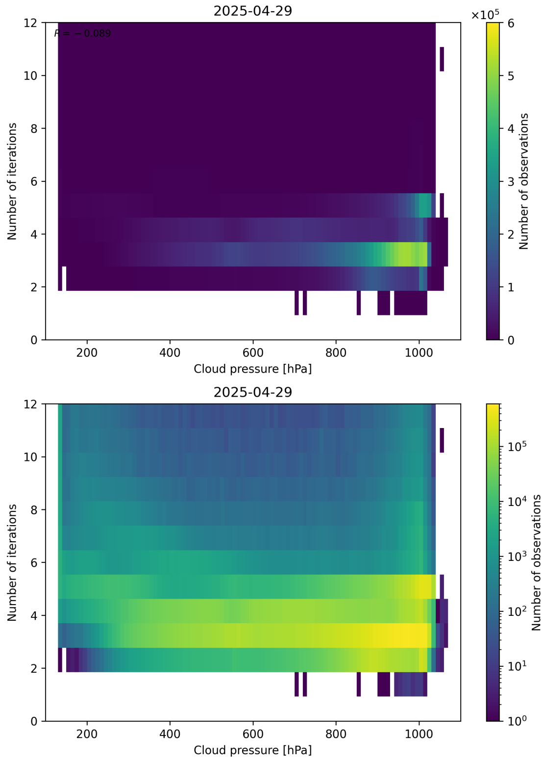
Figure 81: Scatter density plot of “Cloud pressure” against “Number of iterations” for 2025-04-29 to 2025-04-30.
