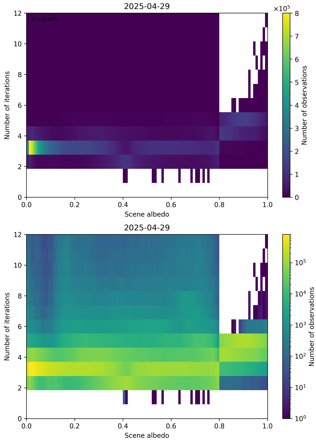
Figure 105: Scatter density plot of “Scene albedo” against “Number of iterations” for 2025-04-29 to 2025-04-30.
