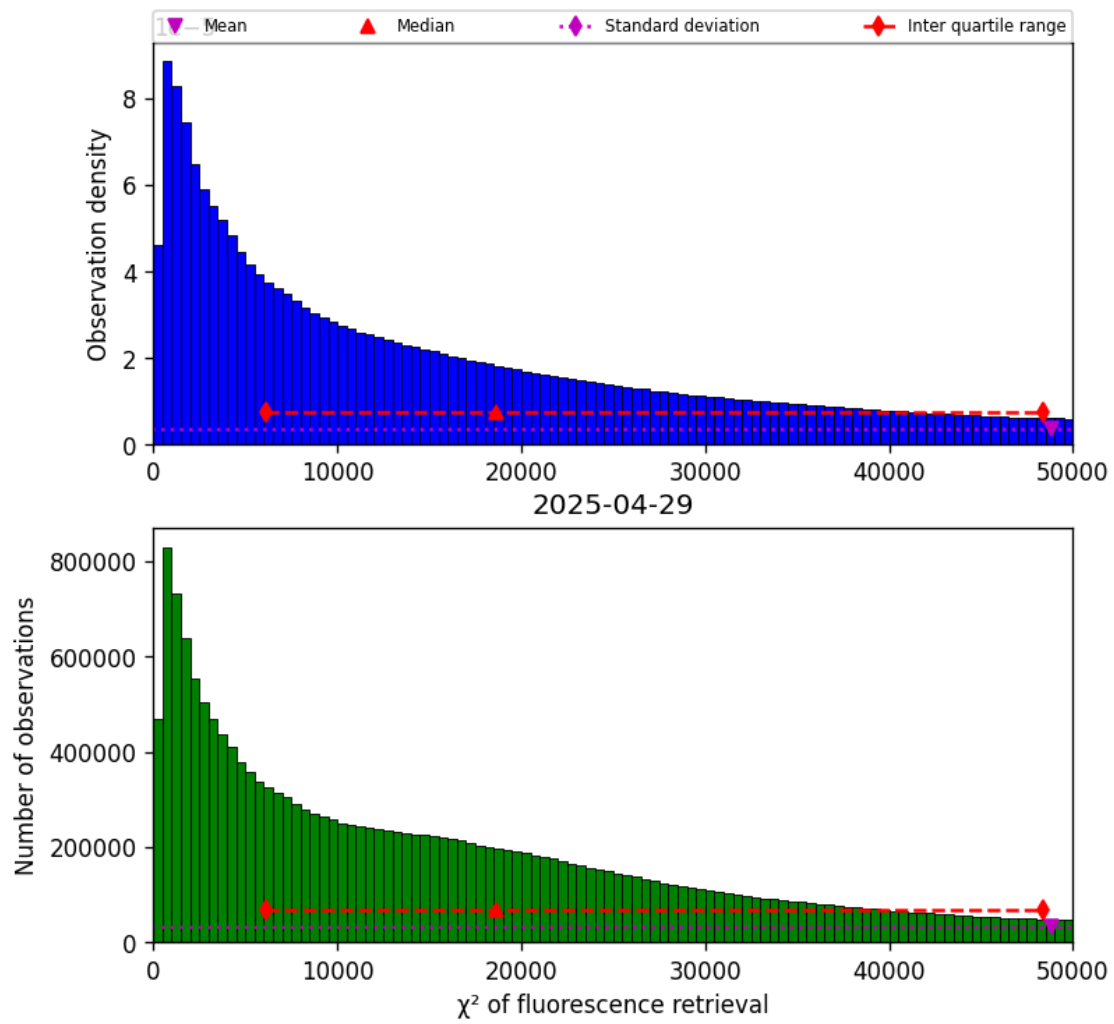
Figure 42: Histogram of “ \chi^2 of fluorescence retrieval” for 2025-04-29 to 2025-04-30
