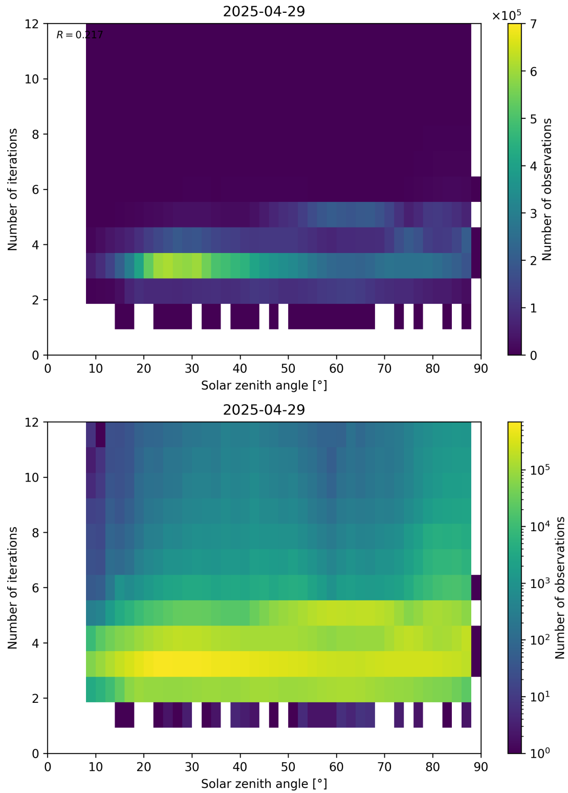
Figure 114: Scatter density plot of “Solar zenith angle” against “Number of iterations” for 2025-04-29 to 2025-04-30.
