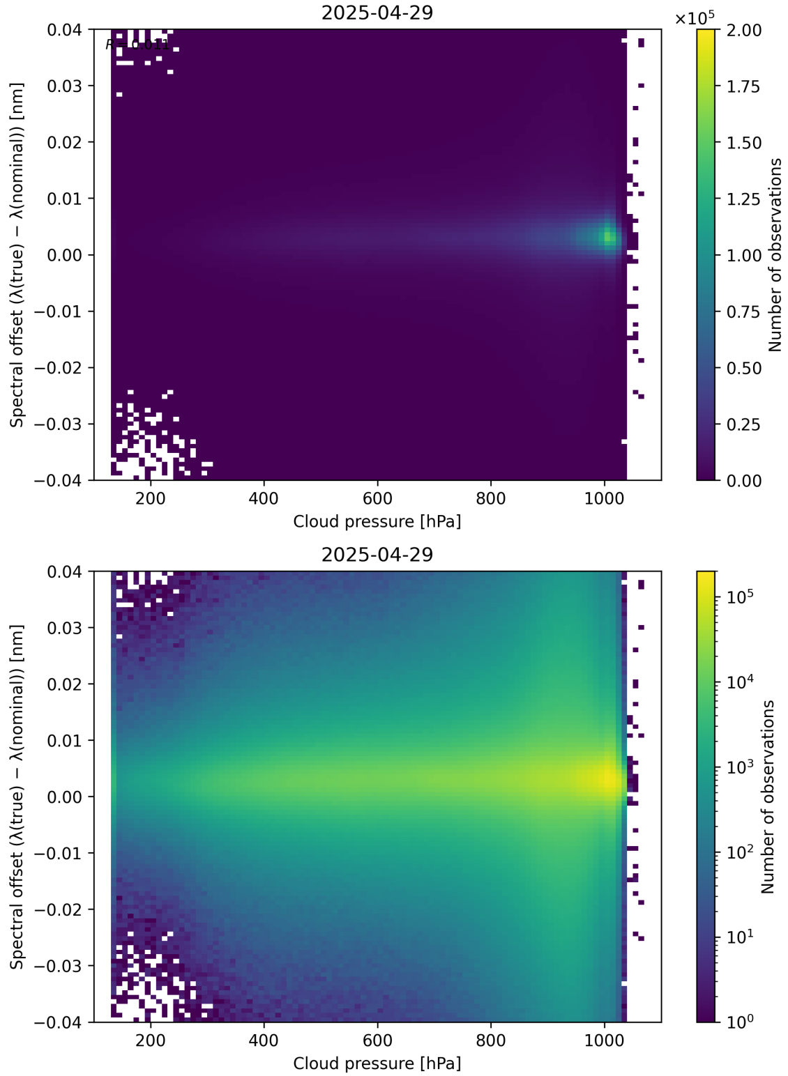
Figure 84: Scatter density plot of “Cloud pressure” against “Spectral offset ( \lambda_{\text{true}} - \lambda_{\text{nominal}} )” for 2025-04-29 to 2025-04-30.
