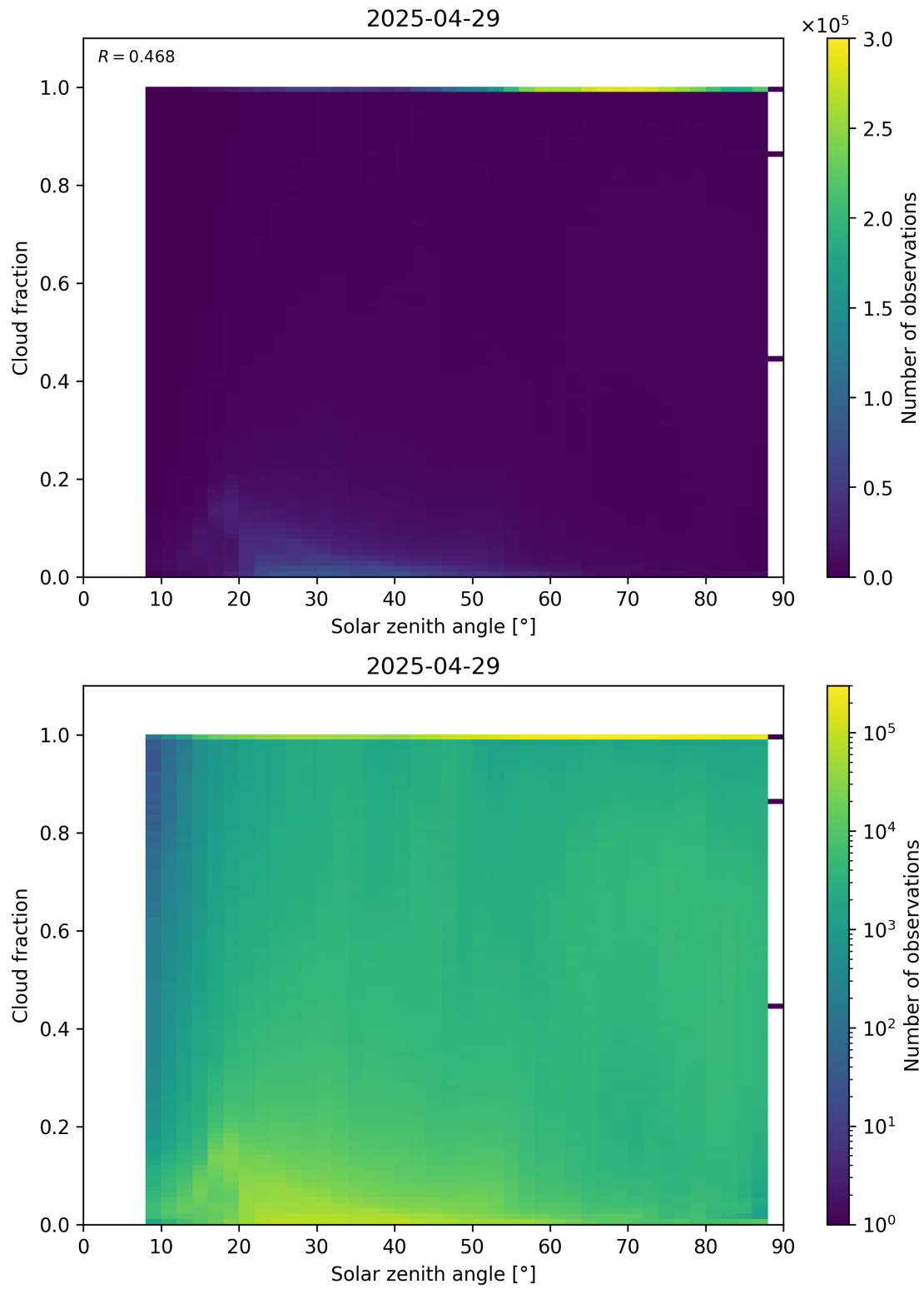
Figure 110: Scatter density plot of “Solar zenith angle” against “Cloud fraction” for 2025-04-29 to 2025-04-30.
