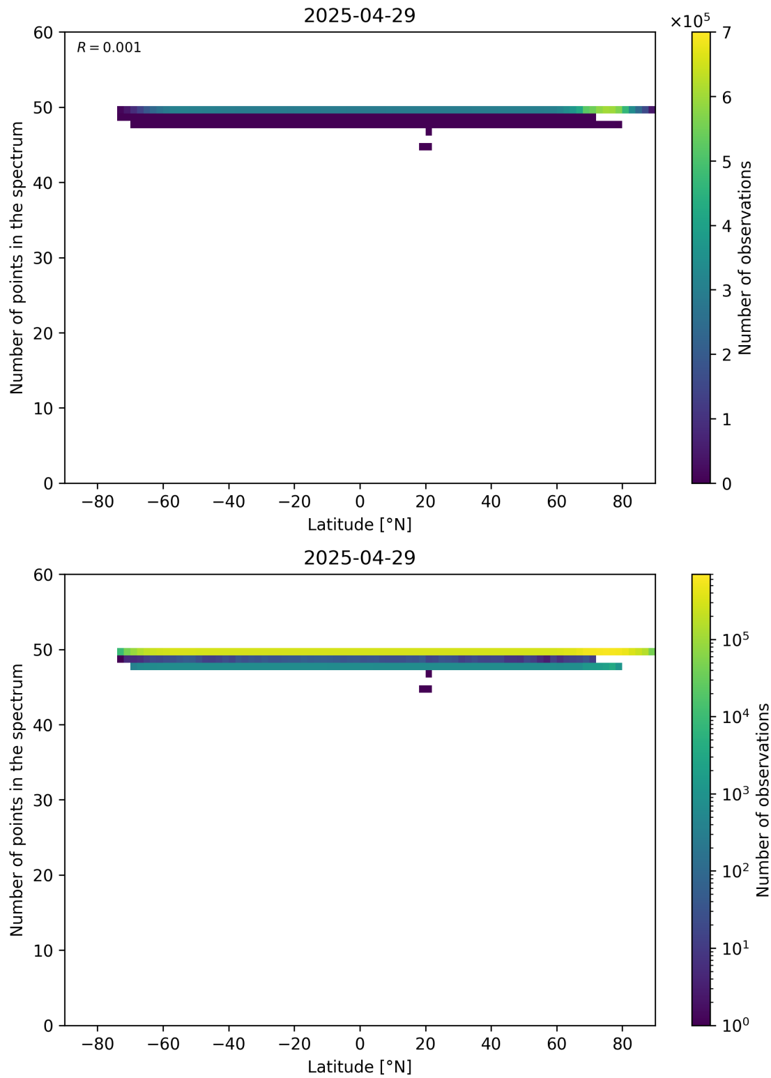
Figure 94: Scatter density plot of “Latitude” against “Number of points in the spectrum” for 2025-04-29 to 2025-04-30.
