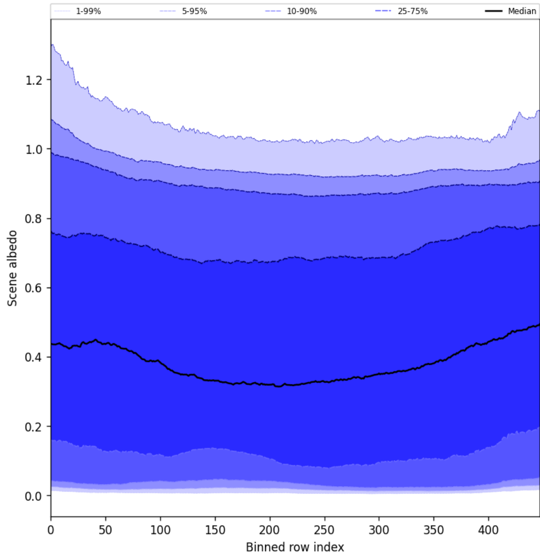
Figure 51: Along track statistics of “Scene albedo” for 2025-04-29 to 2025-04-30
