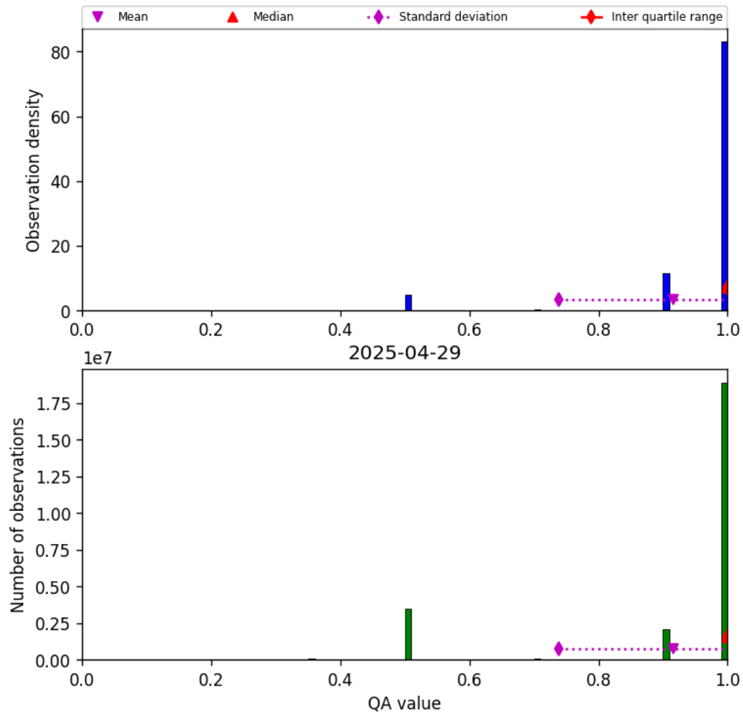
Figure 29: Histogram of “QA value” for 2025-04-29 to 2025-04-30
