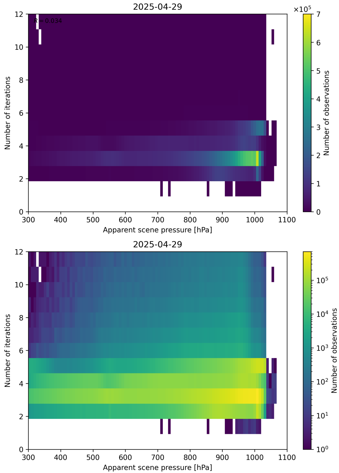
Figure 65: Scatter density plot of “Apparent scene pressure” against “Number of iterations” for 2025-04-29 to 2025-04-30.
