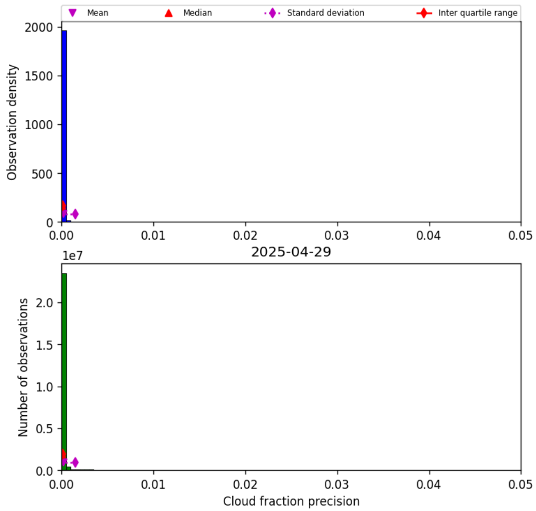
Figure 33: Histogram of “Cloud fraction precision” for 2025-04-29 to 2025-04-30
