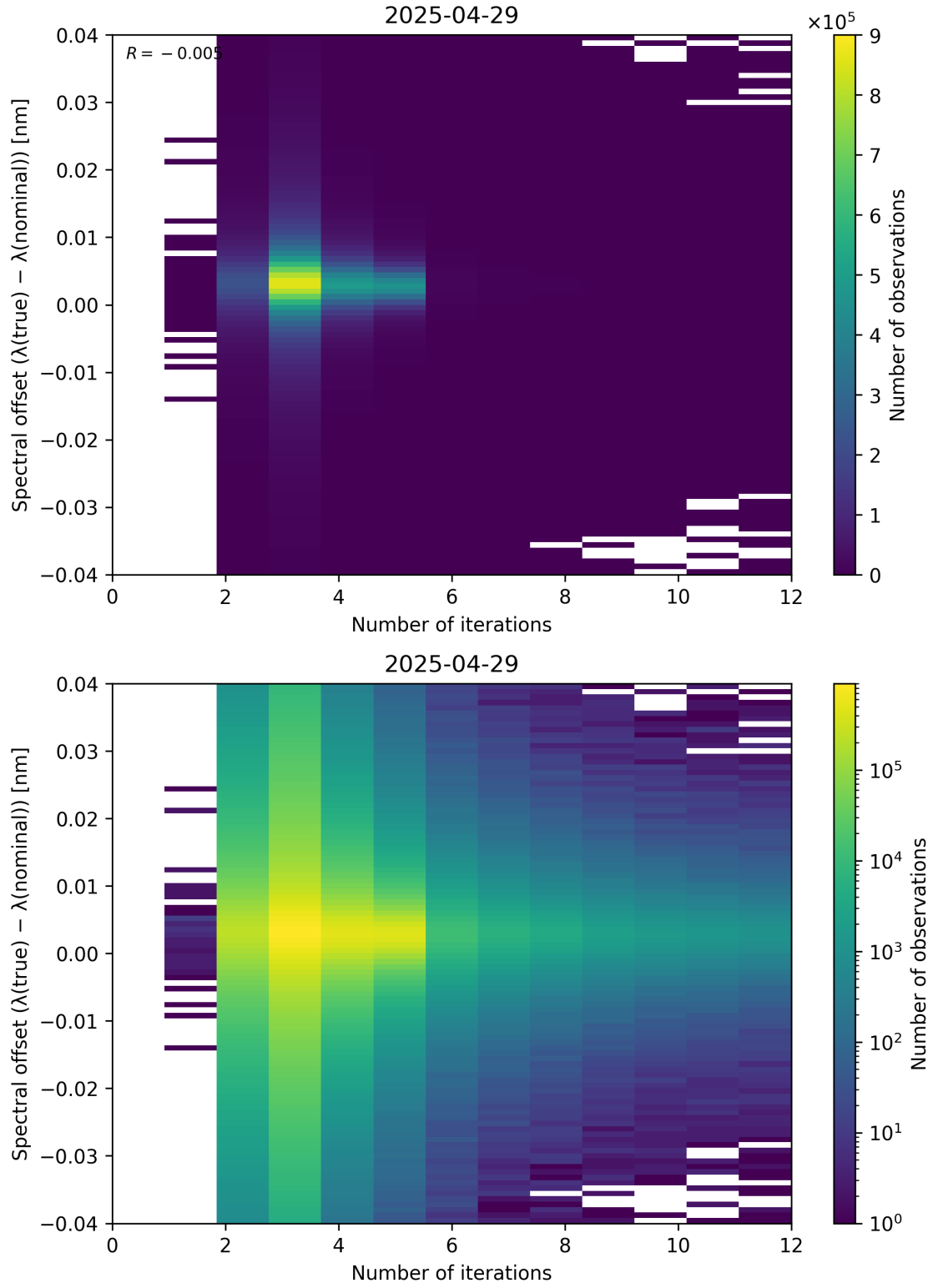
Figure 100: Scatter density plot of “Number of iterations” against “Spectral offset ( \lambda_{\text{true}} - \lambda_{\text{nominal}} )” for 2025-04-29 to 2025-04-30.
