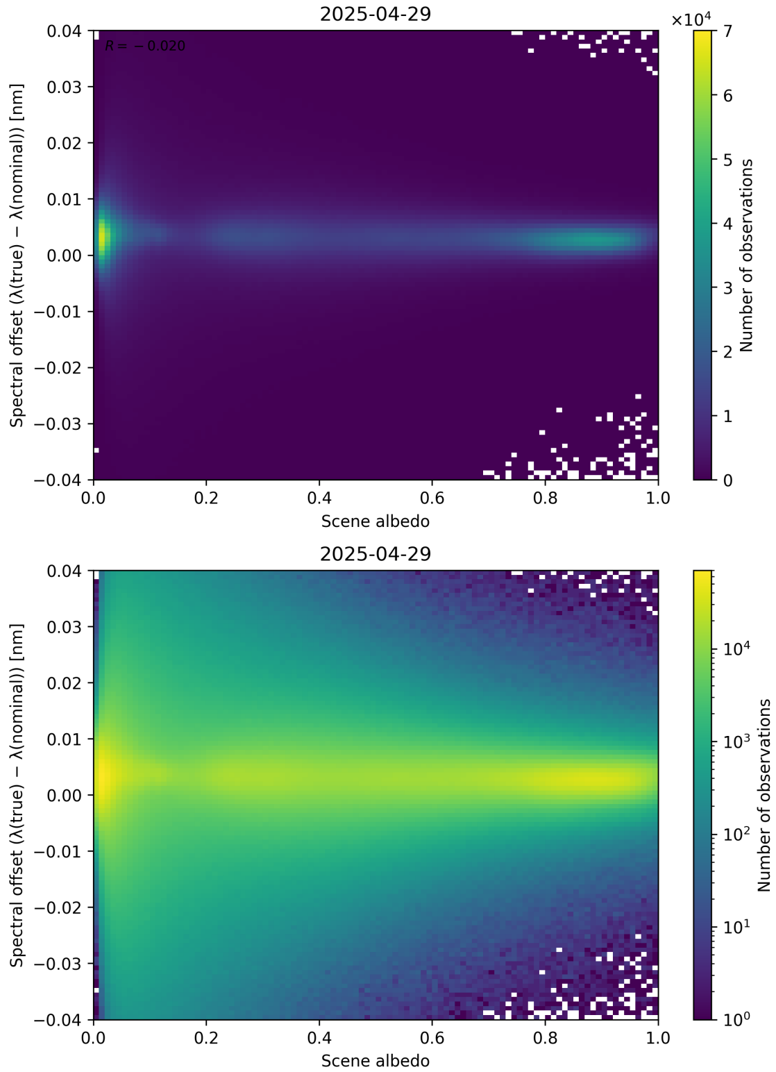
Figure 107: Scatter density plot of “Scene albedo” against “Spectral offset ( \lambda_{\text{true}} - \lambda_{\text{nominal}} )” for 2025-04-29 to 2025-04-30.
