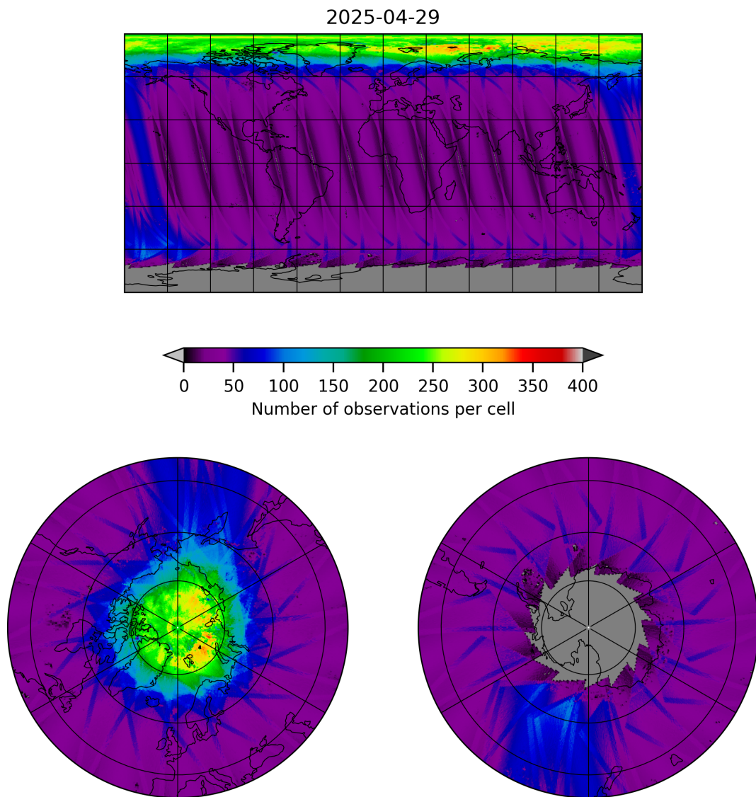
Figure 11: Map of the number of observations for 2025-04-29 to 2025-04-30
