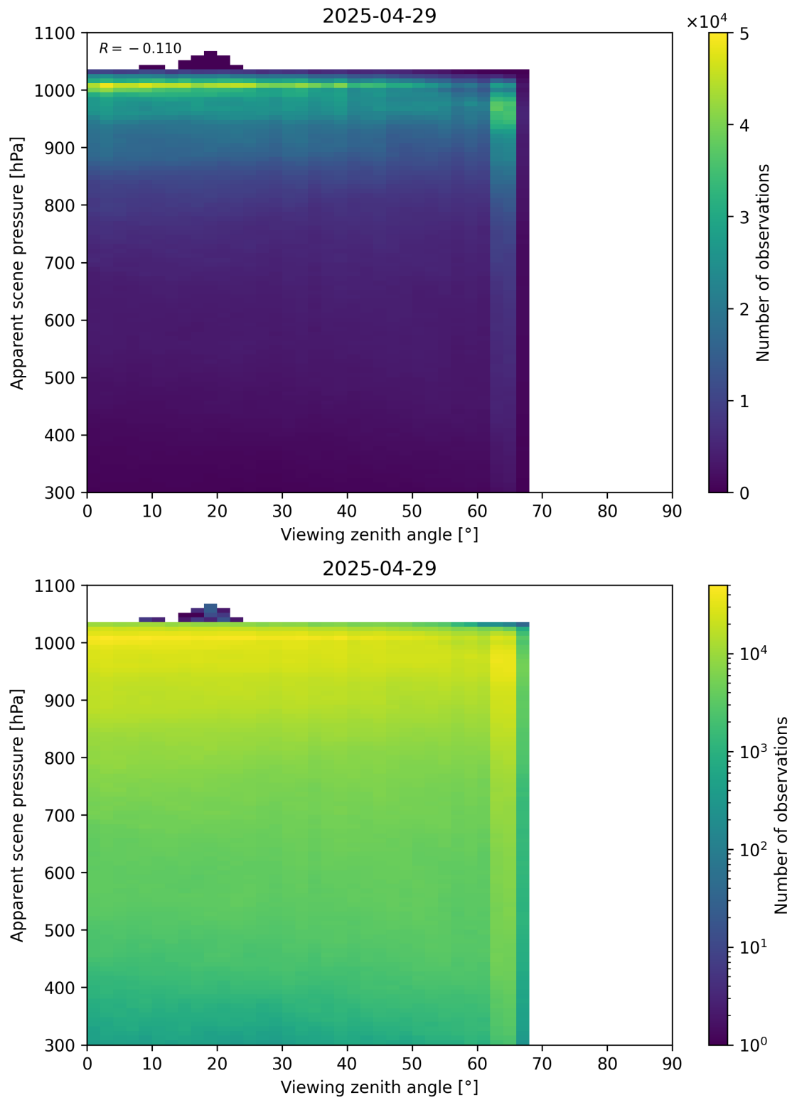
Figure 118: Scatter density plot of “Viewing zenith angle” against “Apparent scene pressure” for 2025-04-29 to 2025-04-30.
