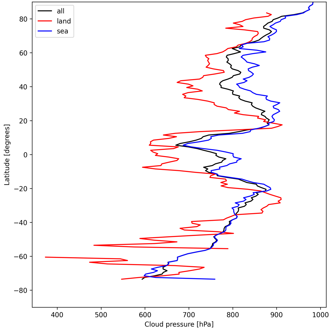
Figure 13: Zonal average of “Cloud pressure” for 2025-04-29 to 2025-04-30.
