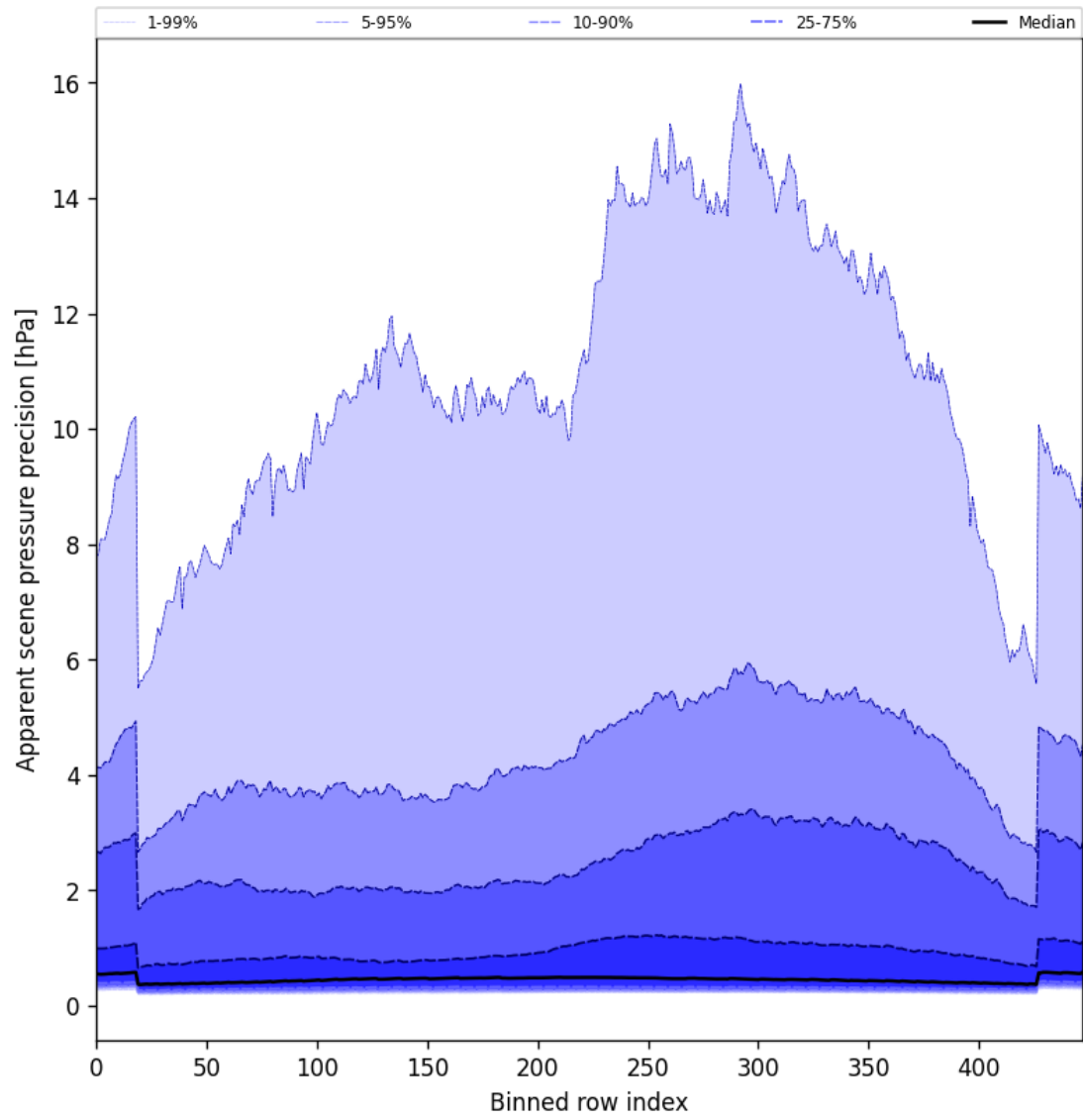
Figure 54: Along track statistics of “Apparent scene pressure precision” for 2025-04-29 to 2025-04-30
