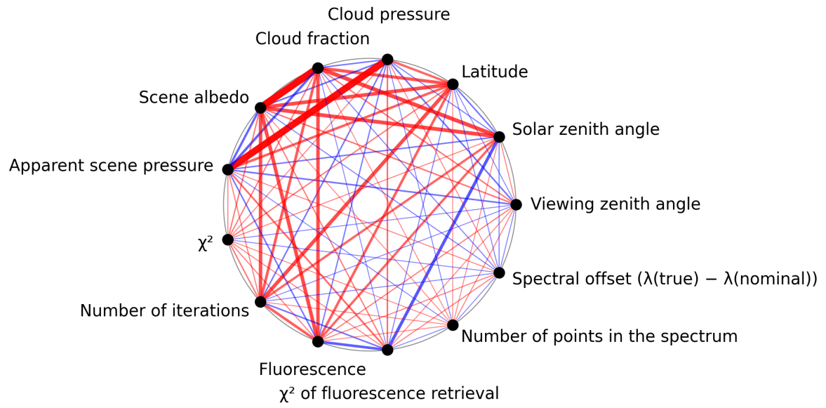
Figure 1: Map of correlation graph for 2025-04-29 to 2025-04-30.
