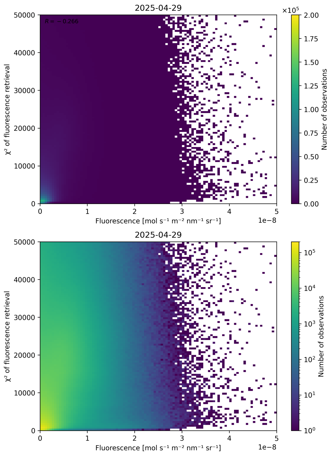
Figure 85: Scatter density plot of “Fluorescence” against “ \chi^2 of fluorescence retrieval” for 2025-04-29 to 2025-04-30.
