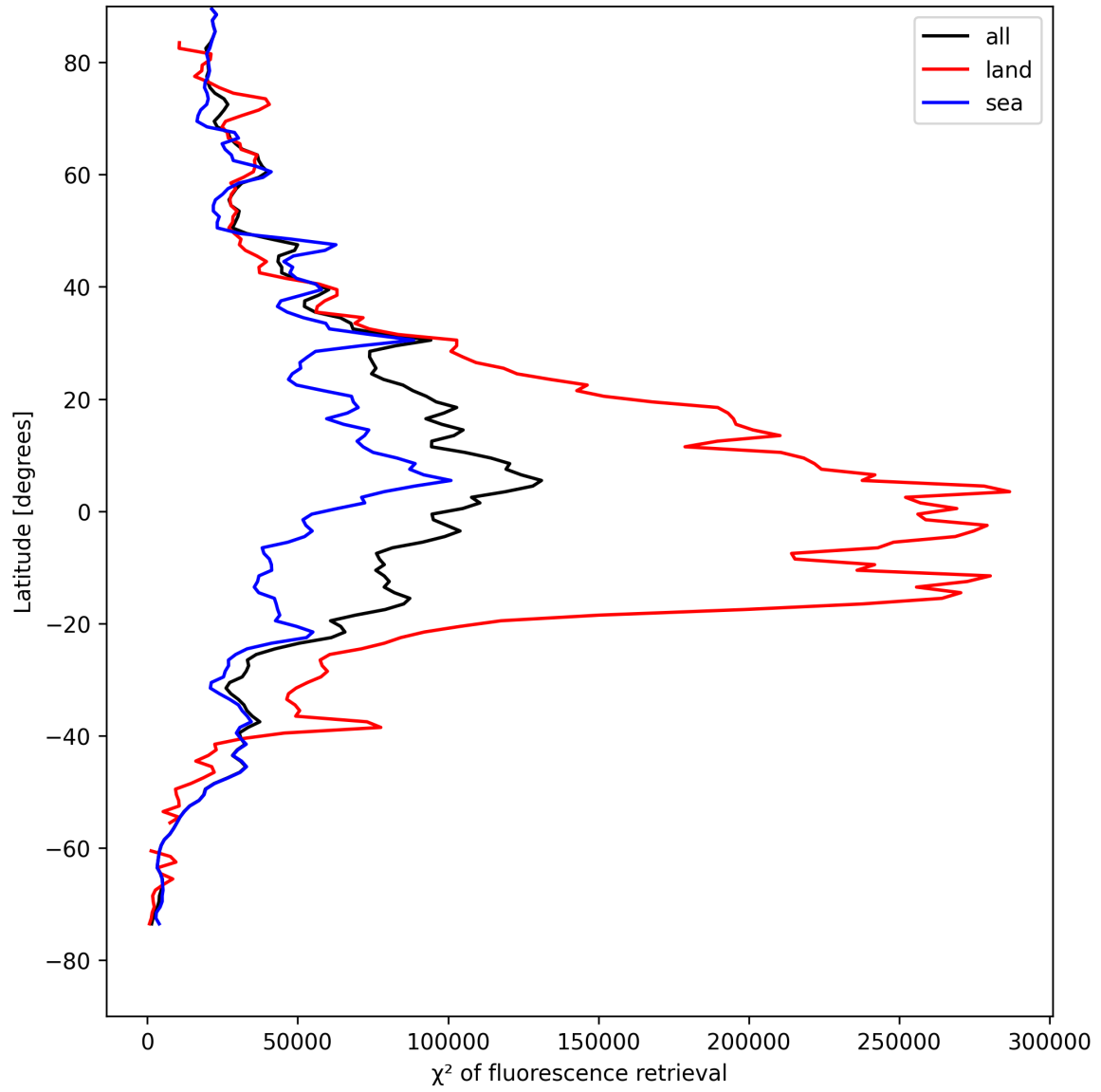
Figure 25: Zonal average of “ \chi^2 of fluorescence retrieval” for 2025-04-29 to 2025-04-30.
