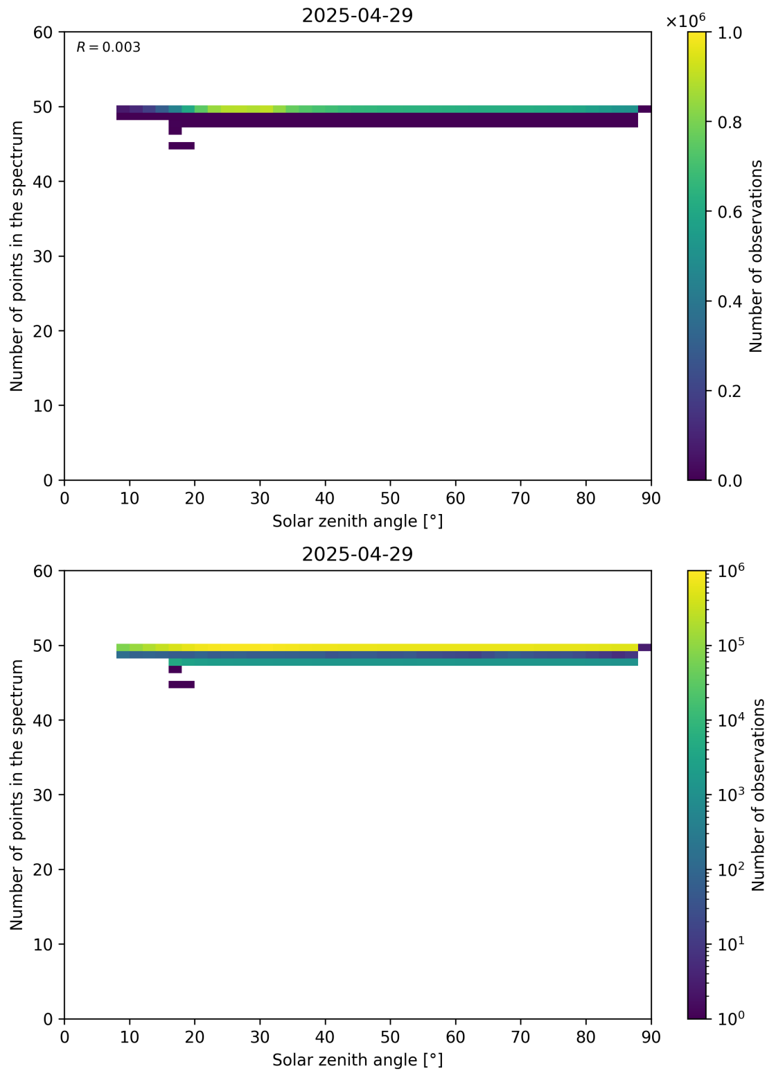
Figure 115: Scatter density plot of “Solar zenith angle” against “Number of points in the spectrum” for 2025-04-29 to 2025-04-30.
