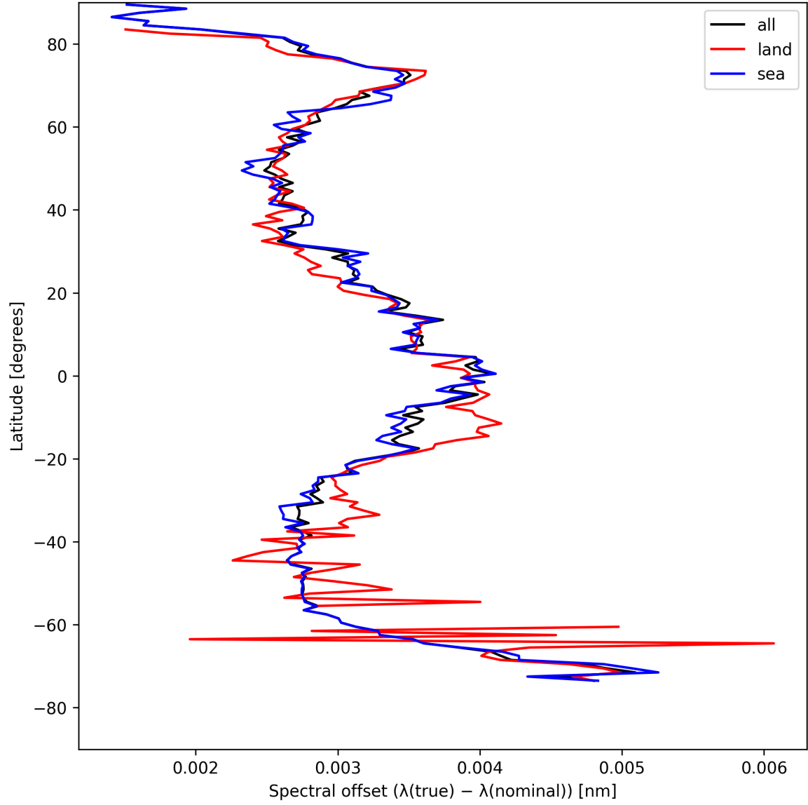
Figure 28: Zonal average of “Spectral offset ( \lambda_{\text{true}} - \lambda_{\text{nominal}} )” for 2025-04-29 to 2025-04-30.
