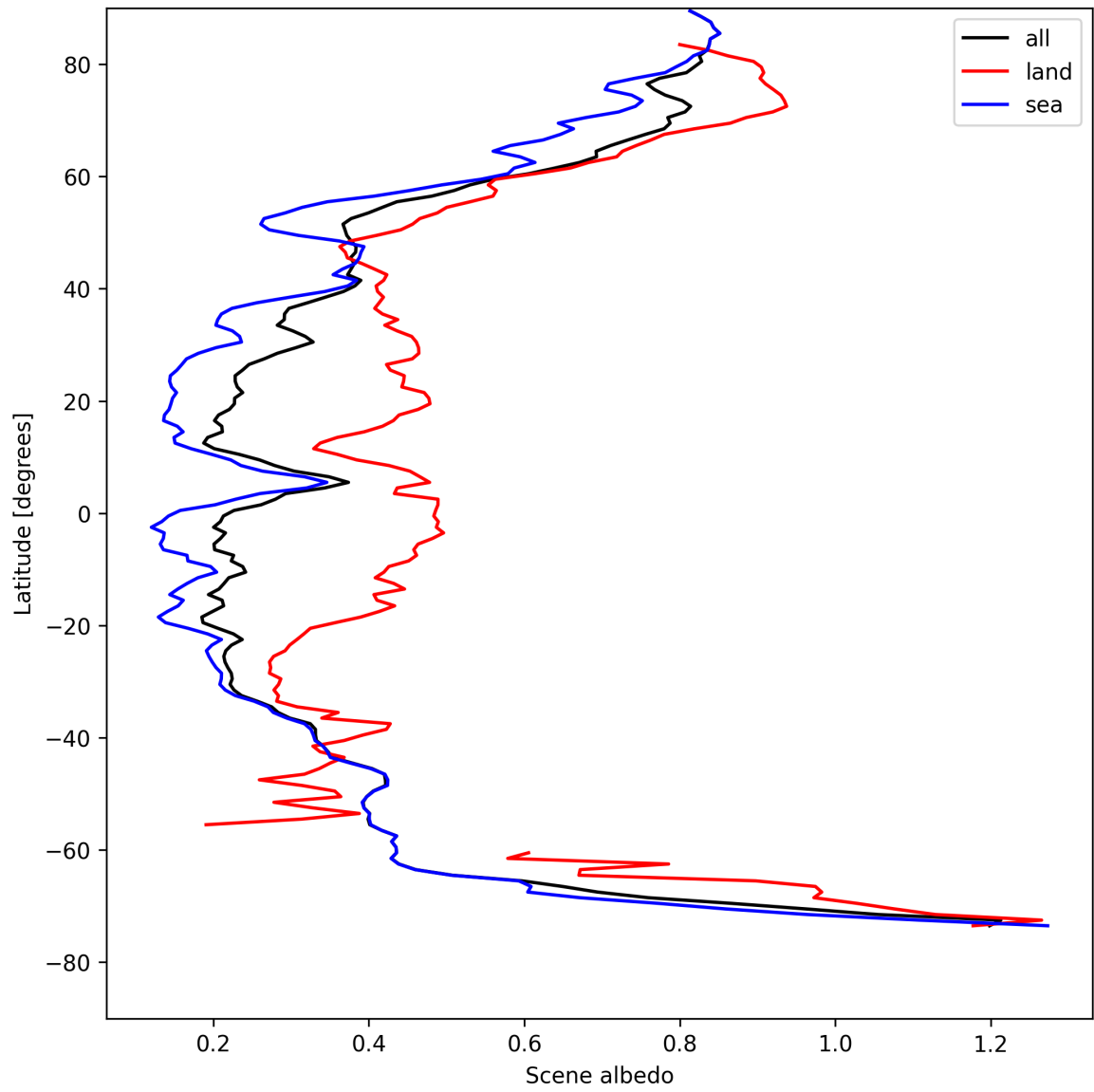
Figure 17: Zonal average of “Scene albedo” for 2025-04-29 to 2025-04-30.
