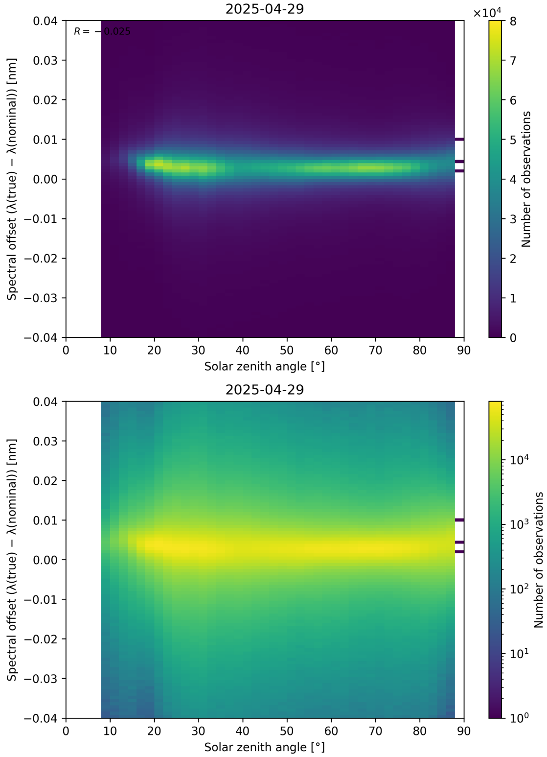
Figure 117: Scatter density plot of “Solar zenith angle” against “Spectral offset ( \lambda_{\text{true}} - \lambda_{\text{nominal}} )” for 2025-04-29 to 2025-04-30.
