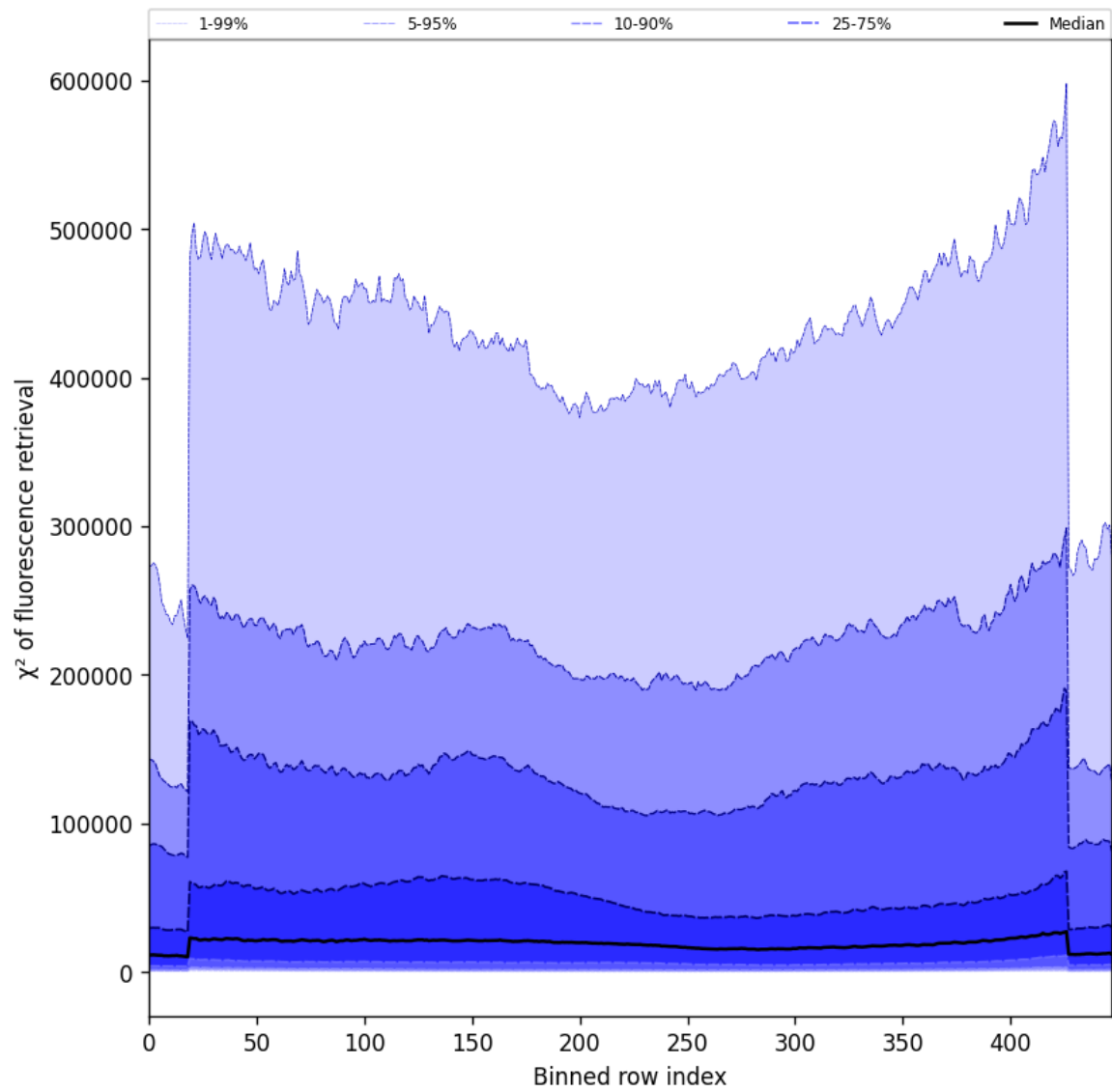
Figure 59: Along track statistics of “ \chi^2 of fluorescence retrieval” for 2025-04-29 to 2025-04-30
