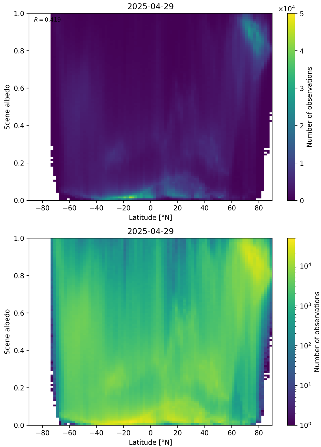
Figure 95: Scatter density plot of “Latitude” against “Scene albedo” for 2025-04-29 to 2025-04-30.
