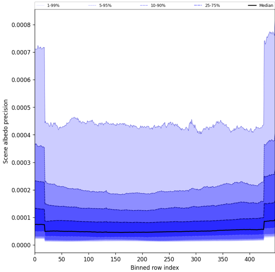
Figure 52: Along track statistics of “Scene albedo precision” for 2025-04-29 to 2025-04-30
