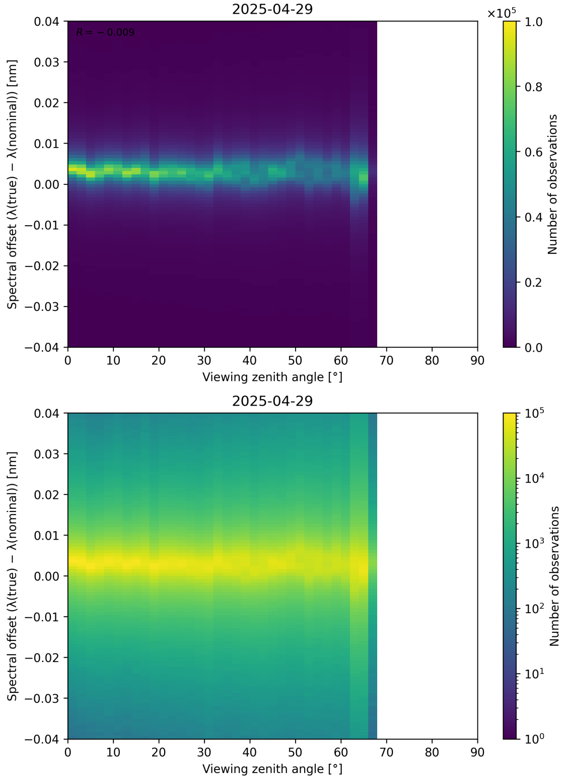
Figure 128: Scatter density plot of “Viewing zenith angle” against “Spectral offset ( \lambda_{\text{true}} - \lambda_{\text{nominal}} )” for 2025-04-29 to 2025-04-30.
