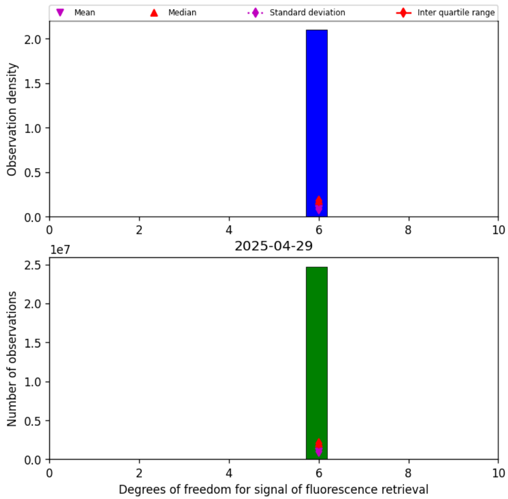
Figure 43: Histogram of “Degrees of freedom for signal of fluorescence retrieval” for 2025-04-29 to 2025-04-30
