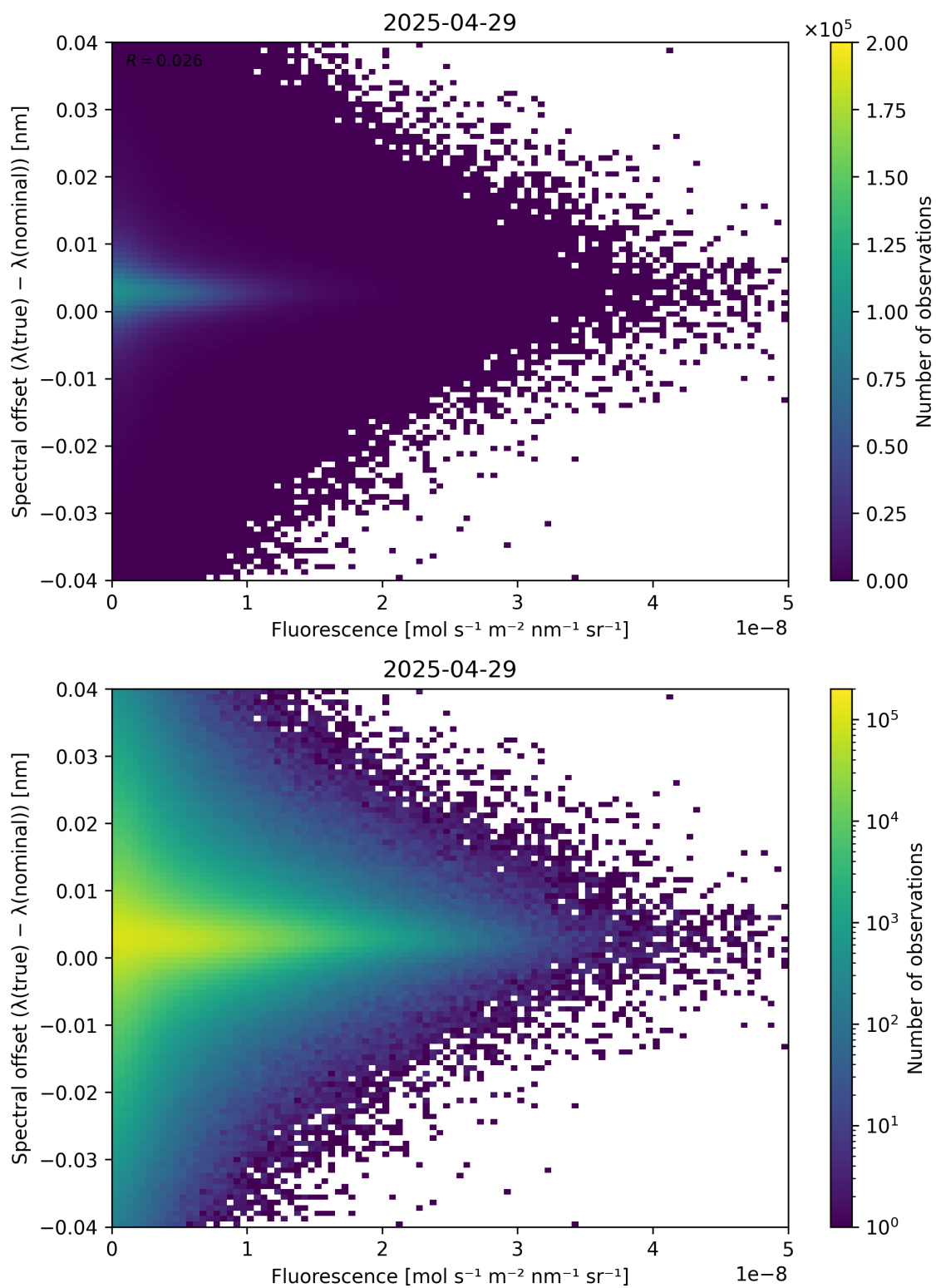
Figure 87: Scatter density plot of “Fluorescence” against “Spectral offset ( \lambda_{\text{true}} - \lambda_{\text{nominal}} )” for 2025-04-29 to 2025-04-30.
