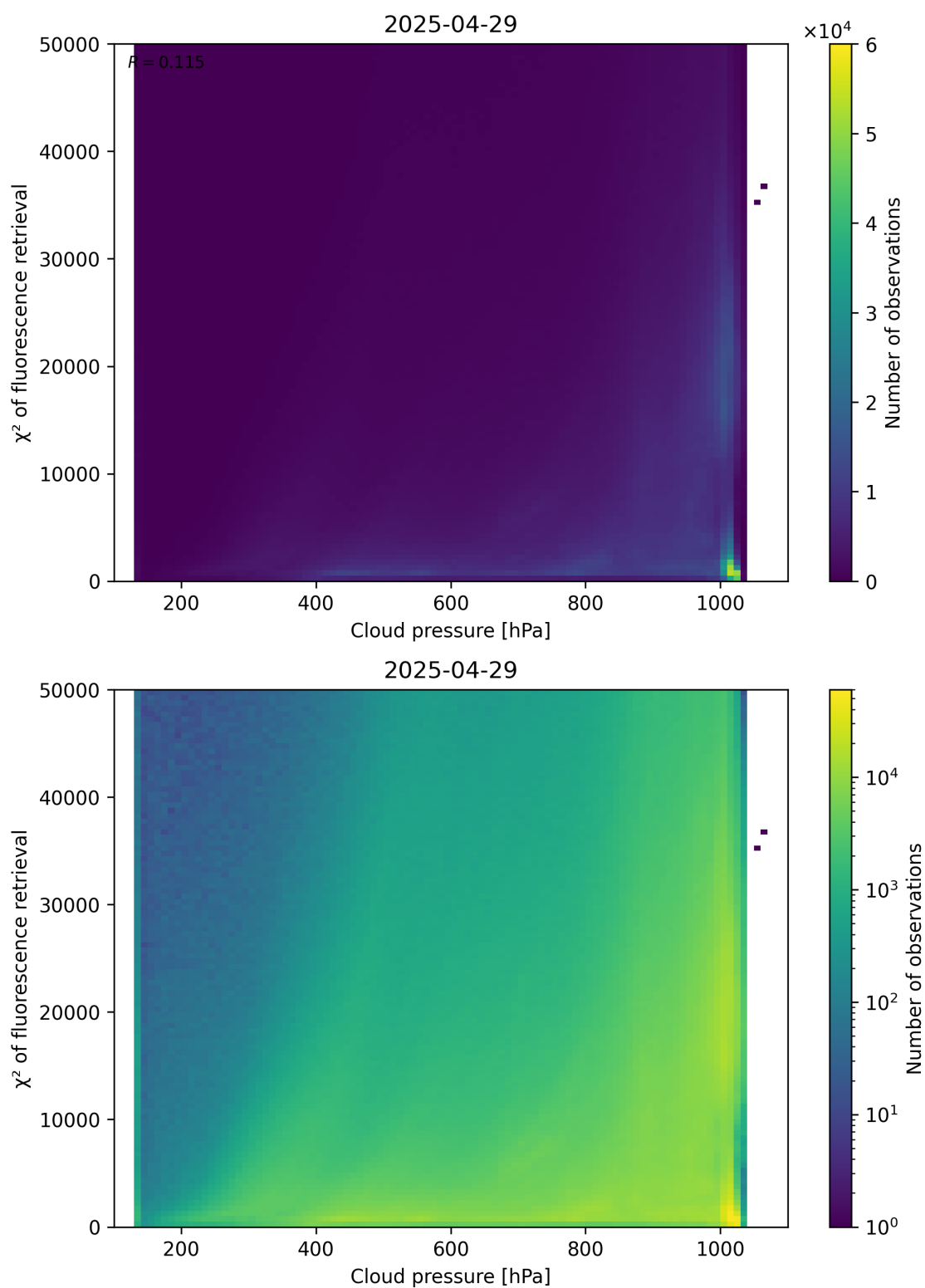
Figure 78: Scatter density plot of “Cloud pressure” against “ \chi^2 of fluorescence retrieval” for 2025-04-29 to 2025-04-30.
