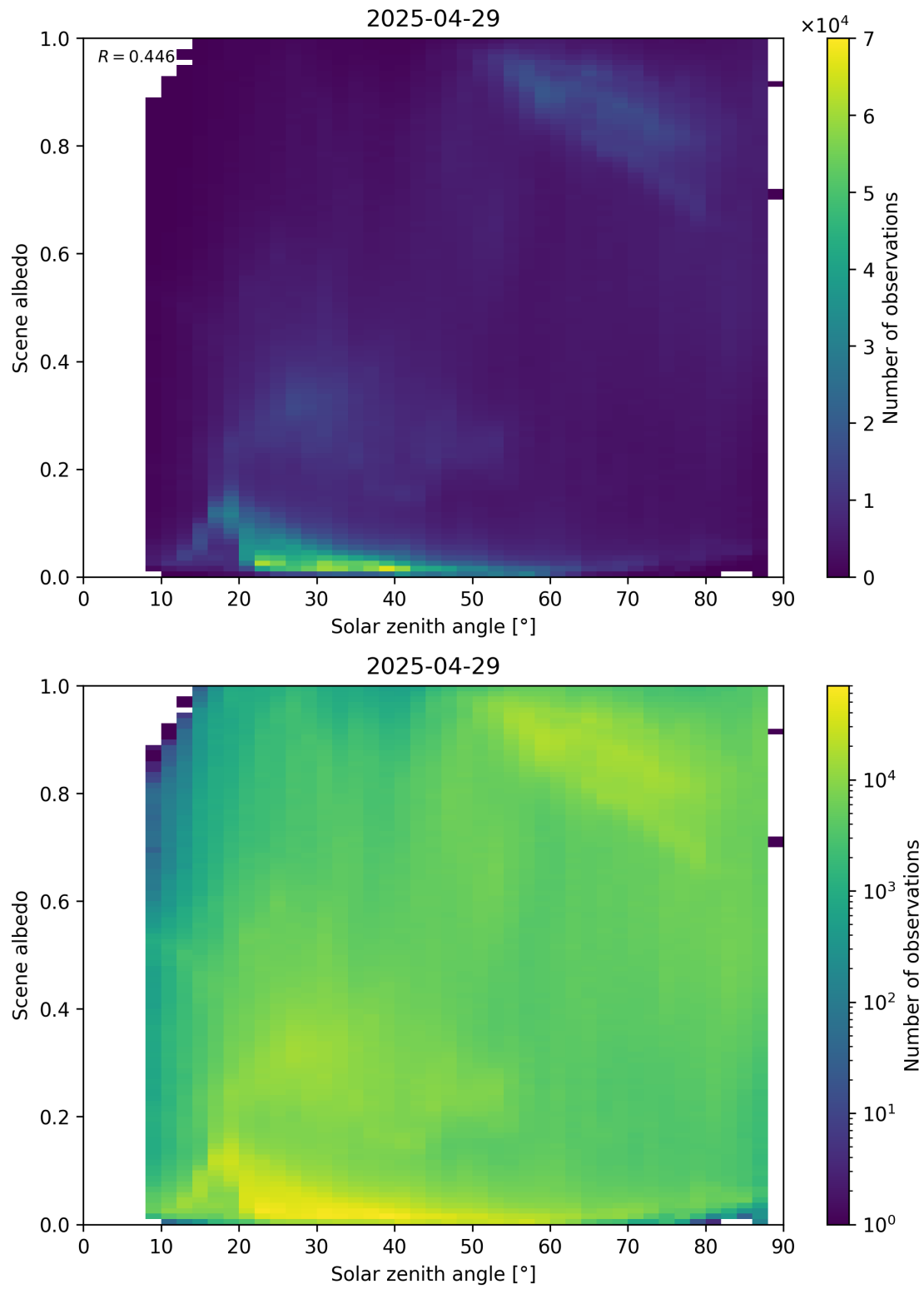
Figure 116: Scatter density plot of “Solar zenith angle” against “Scene albedo” for 2025-04-29 to 2025-04-30.
