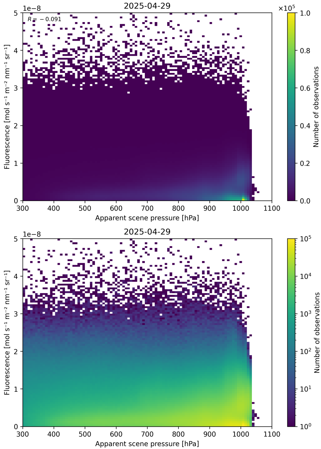
Figure 64: Scatter density plot of “Apparent scene pressure” against “Fluorescence” for 2025-04-29 to 2025-04-30.
