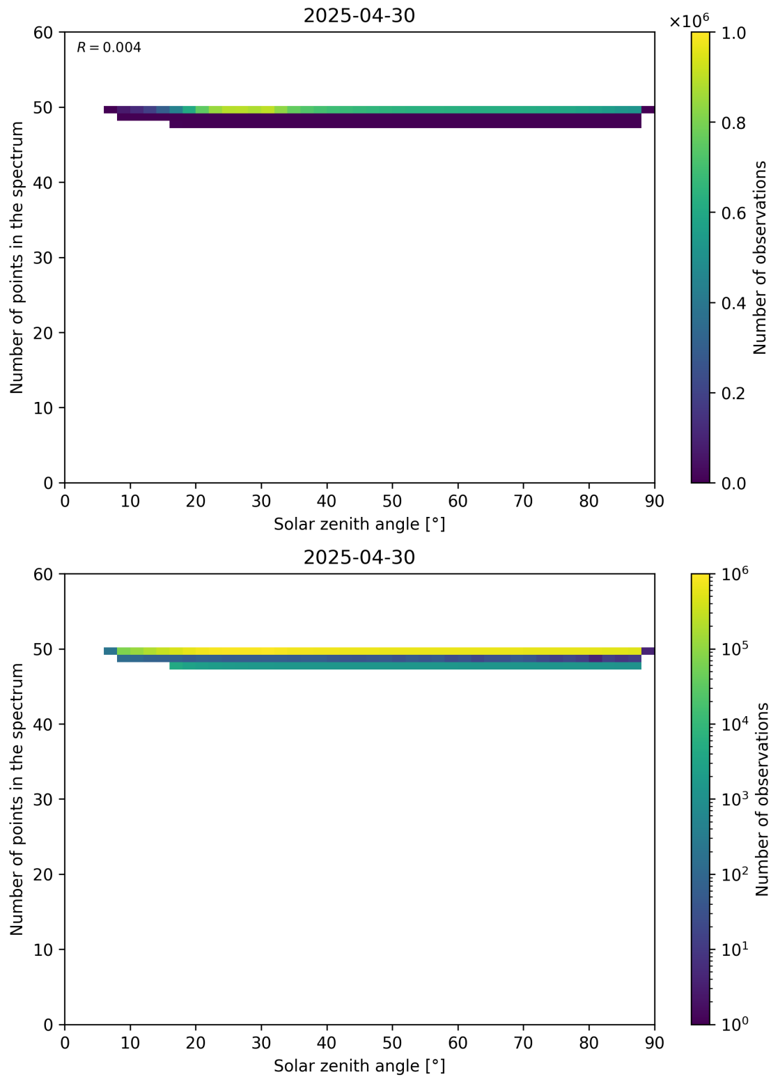
Figure 115: Scatter density plot of “Solar zenith angle” against “Number of points in the spectrum” for 2025-04-29 to 2025-05-01.
