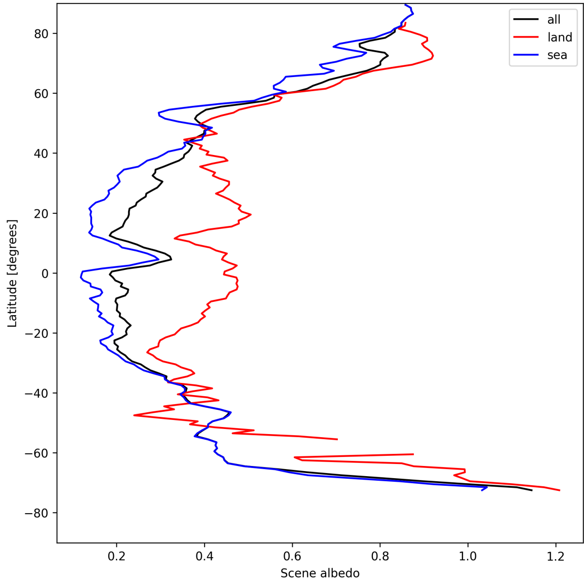
Figure 17: Zonal average of “Scene albedo” for 2025-04-29 to 2025-05-01.
