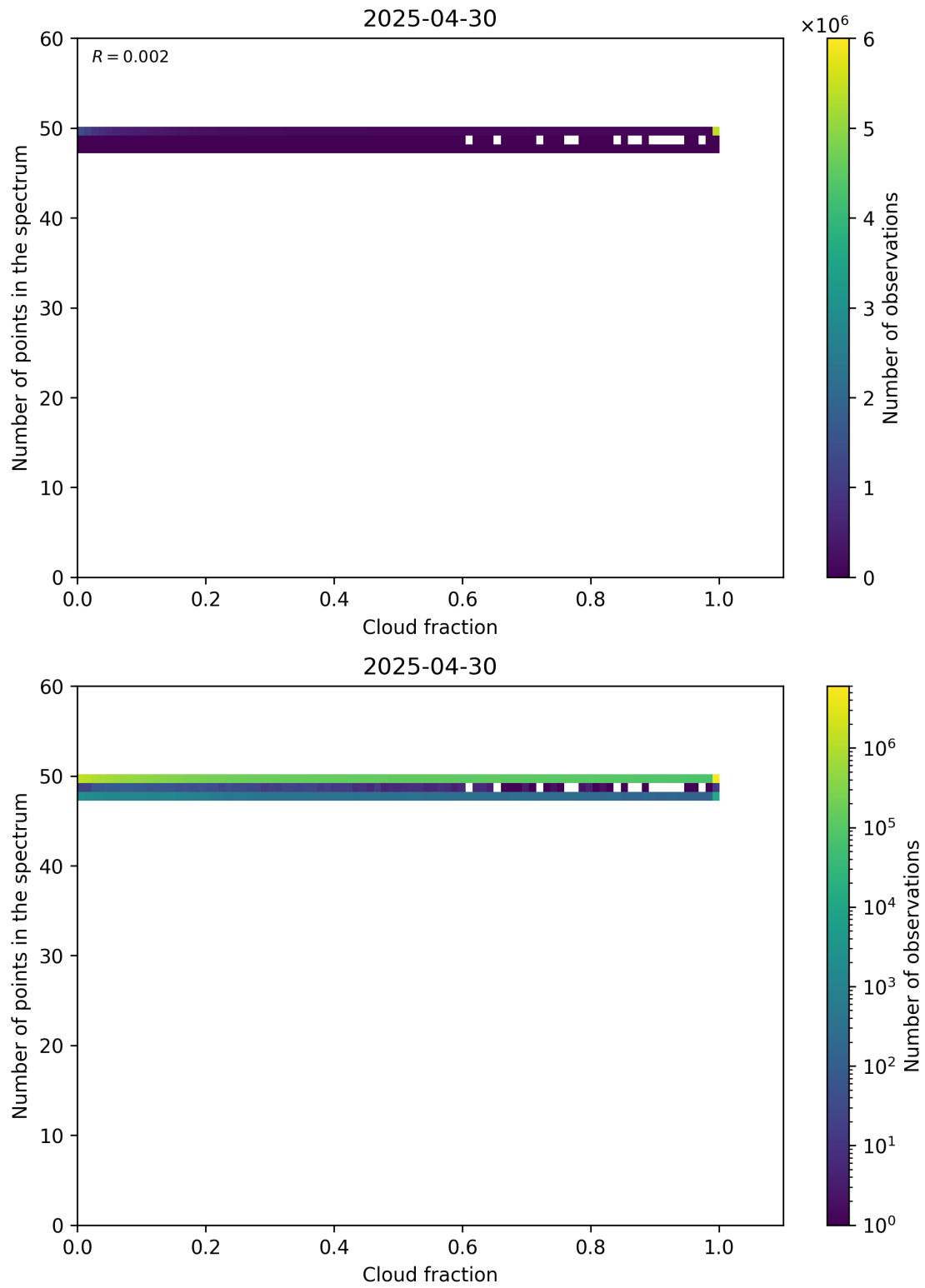
Figure 74: Scatter density plot of “Cloud fraction” against “Number of points in the spectrum” for 2025-04-29 to 2025-05-01.
