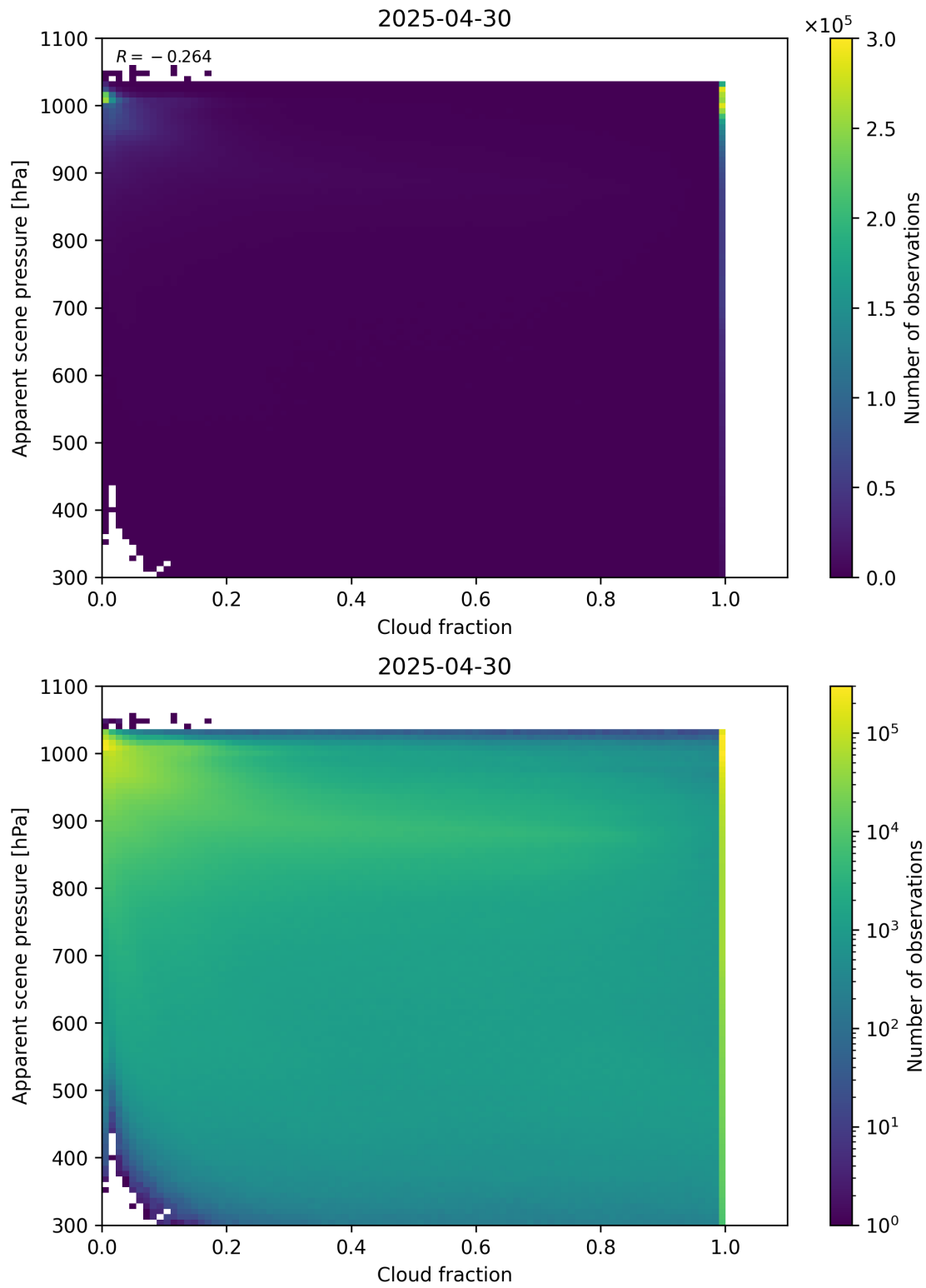
Figure 70: Scatter density plot of “Cloud fraction” against “Apparent scene pressure” for 2025-04-29 to 2025-05-01.
