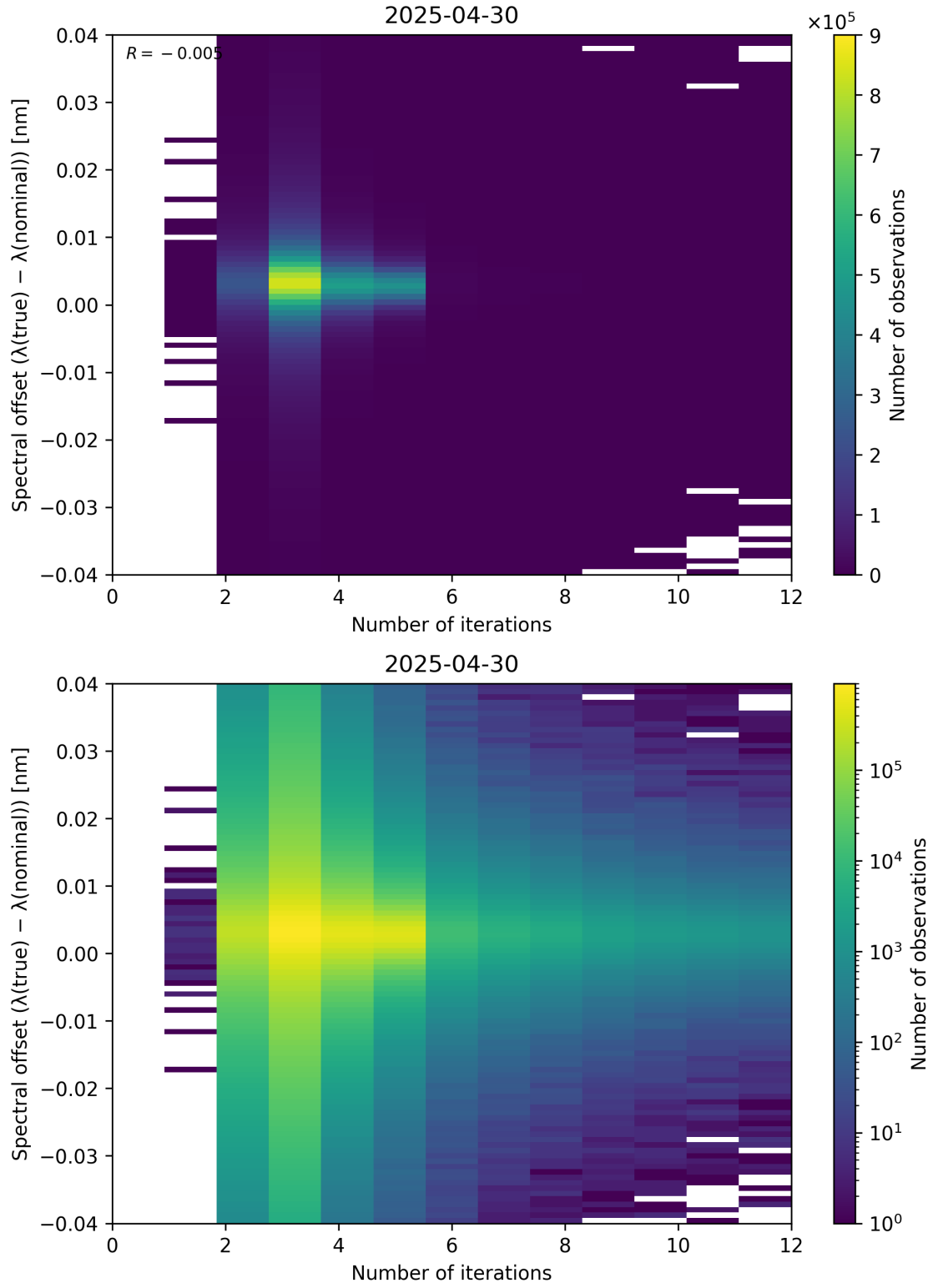
Figure 100: Scatter density plot of “Number of iterations” against “Spectral offset ( \lambda_{\text{true}} - \lambda_{\text{nominal}} )” for 2025-04-29 to 2025-05-01.
