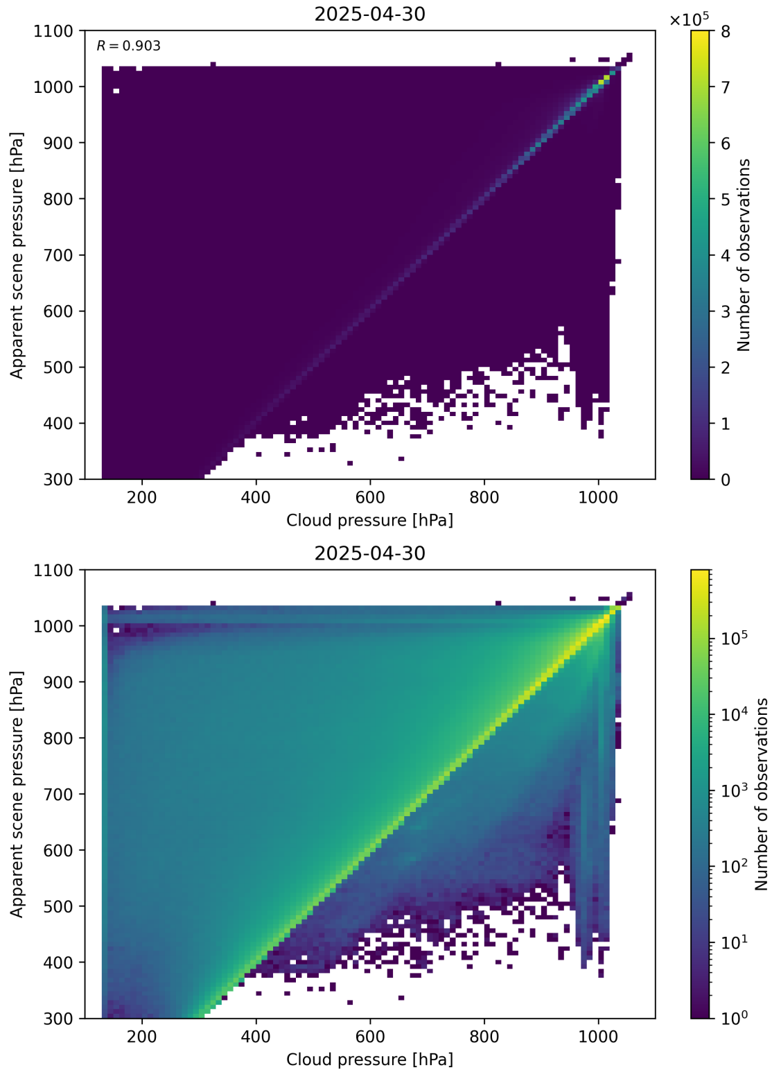
Figure 77: Scatter density plot of “Cloud pressure” against “Apparent scene pressure” for 2025-04-29 to 2025-05-01.
