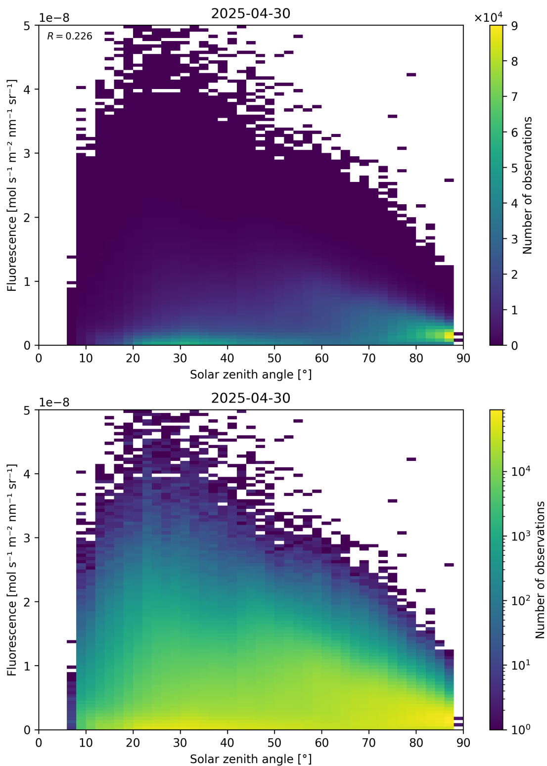
Figure 112: Scatter density plot of “Solar zenith angle” against “Fluorescence” for 2025-04-29 to 2025-05-01.
