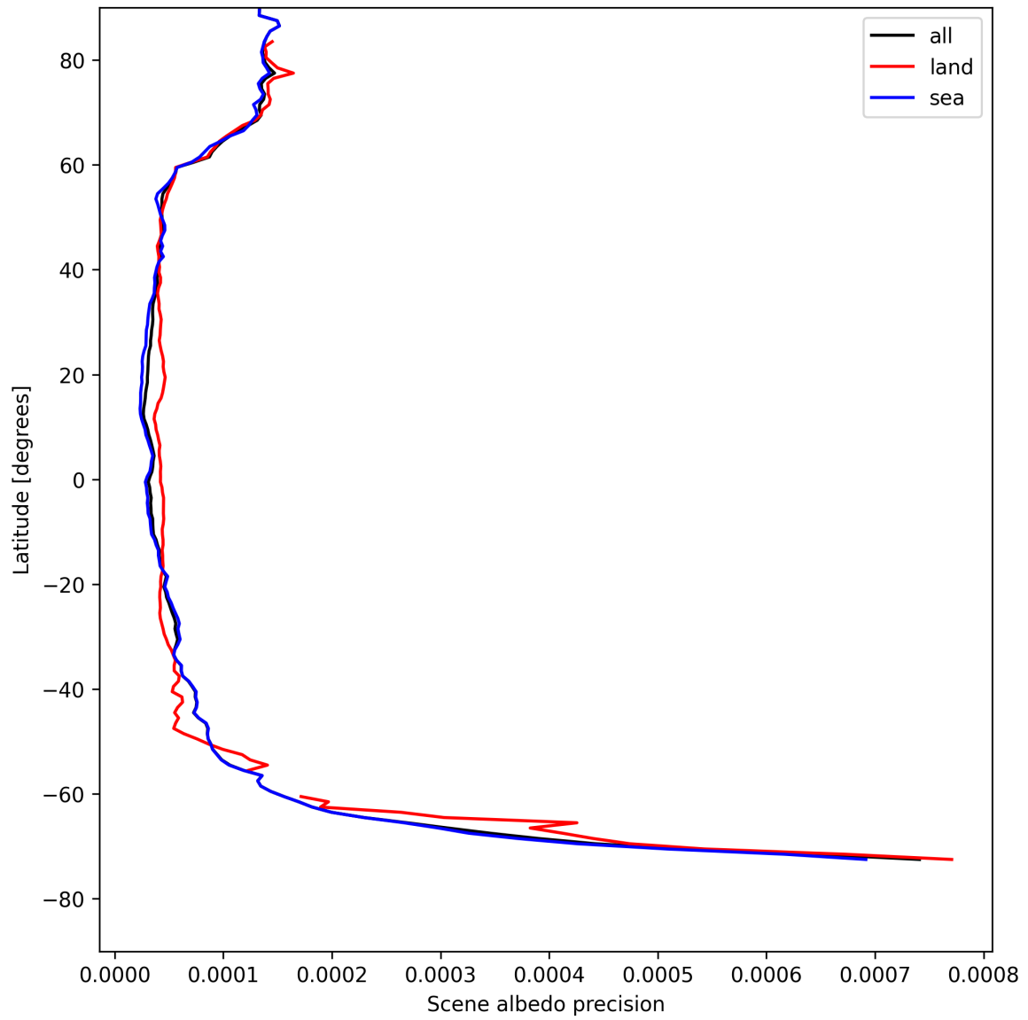
Figure 18: Zonal average of “Scene albedo precision” for 2025-04-29 to 2025-05-01.
