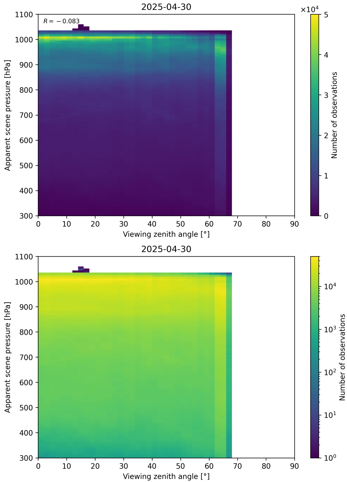
Figure 118: Scatter density plot of “Viewing zenith angle” against “Apparent scene pressure” for 2025-04-29 to 2025-05-01.
