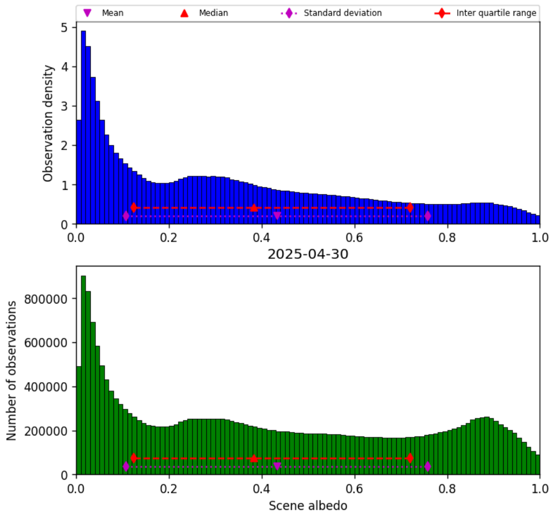
Figure 34: Histogram of “Scene albedo” for 2025-04-29 to 2025-05-01
