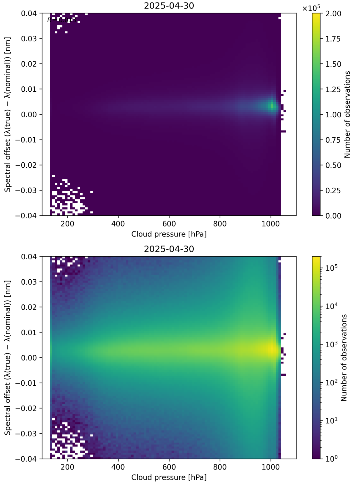
Figure 84: Scatter density plot of “Cloud pressure” against “Spectral offset ( \lambda_{\text{true}} - \lambda_{\text{nominal}} )” for 2025-04-29 to 2025-05-01.
