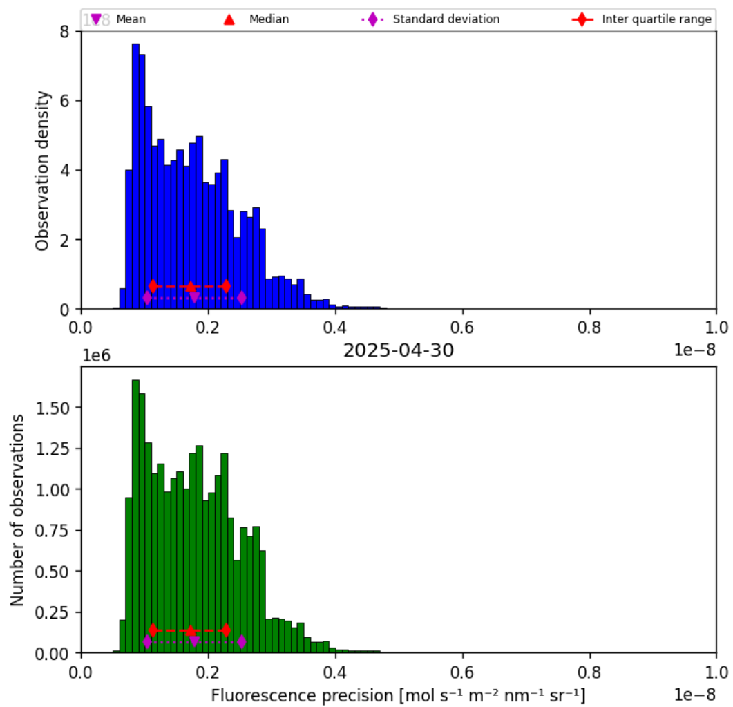
Figure 41: Histogram of “Fluorescence precision” for 2025-04-29 to 2025-05-01
