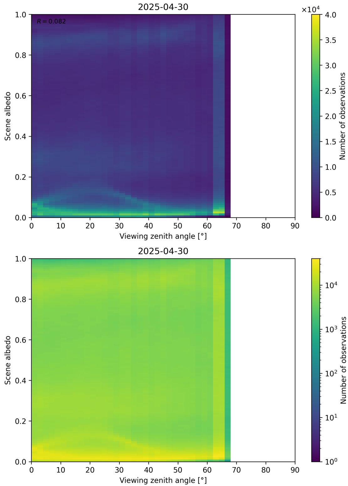
Figure 126: Scatter density plot of “Viewing zenith angle” against “Scene albedo” for 2025-04-29 to 2025-05-01.
