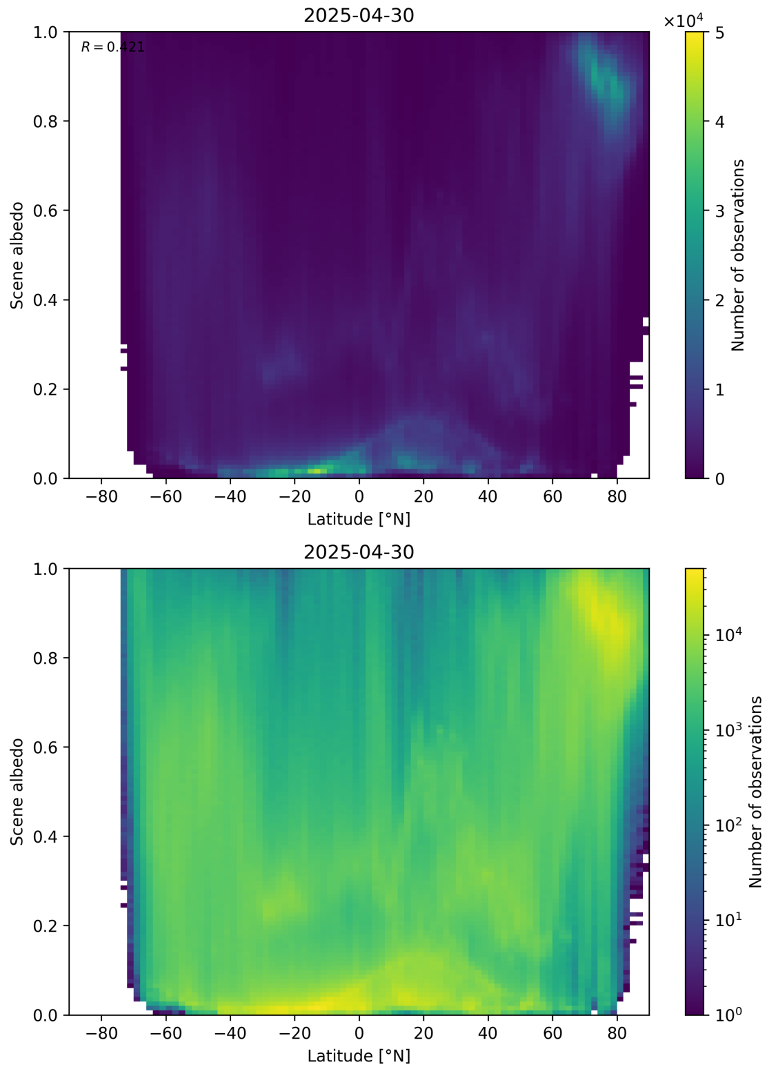
Figure 95: Scatter density plot of “Latitude” against “Scene albedo” for 2025-04-29 to 2025-05-01.
