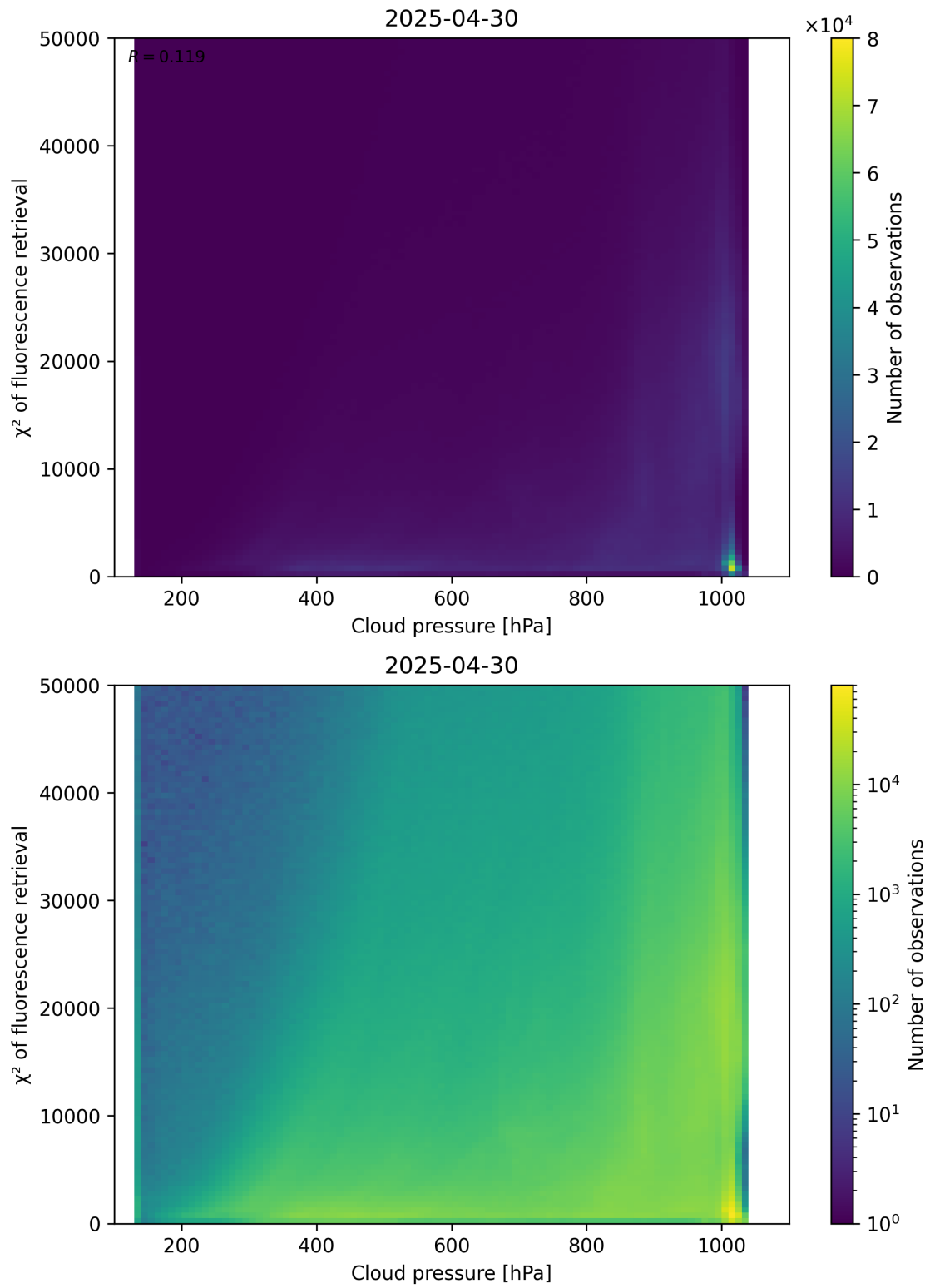
Figure 78: Scatter density plot of “Cloud pressure” against “ \chi^2 of fluorescence retrieval” for 2025-04-29 to 2025-05-01.
