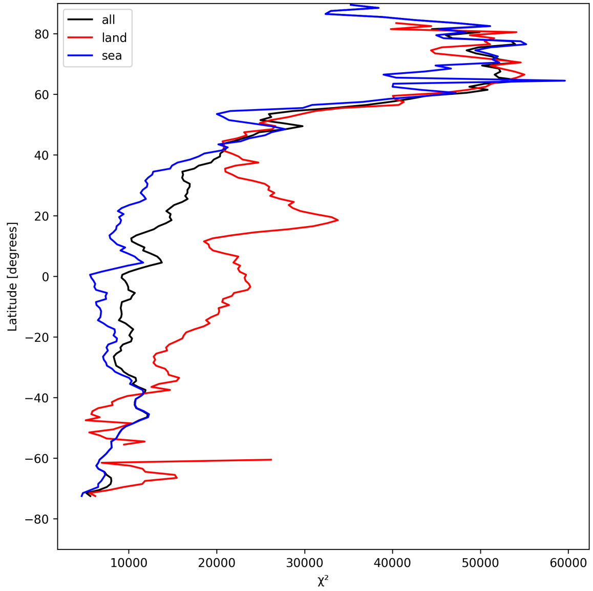
Figure 21: Zonal average of “ \chi^2 ” for 2025-04-29 to 2025-05-01.
