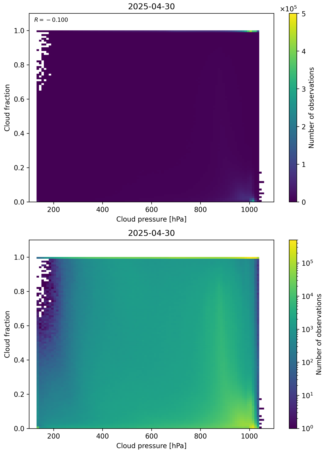
Figure 79: Scatter density plot of “Cloud pressure” against “Cloud fraction” for 2025-04-29 to 2025-05-01.
