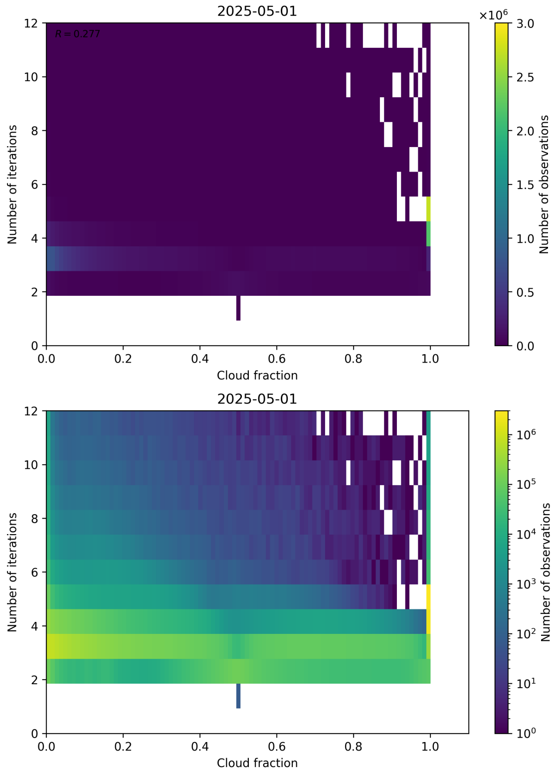
Figure 73: Scatter density plot of “Cloud fraction” against “Number of iterations” for 2025-04-30 to 2025-05-02.
