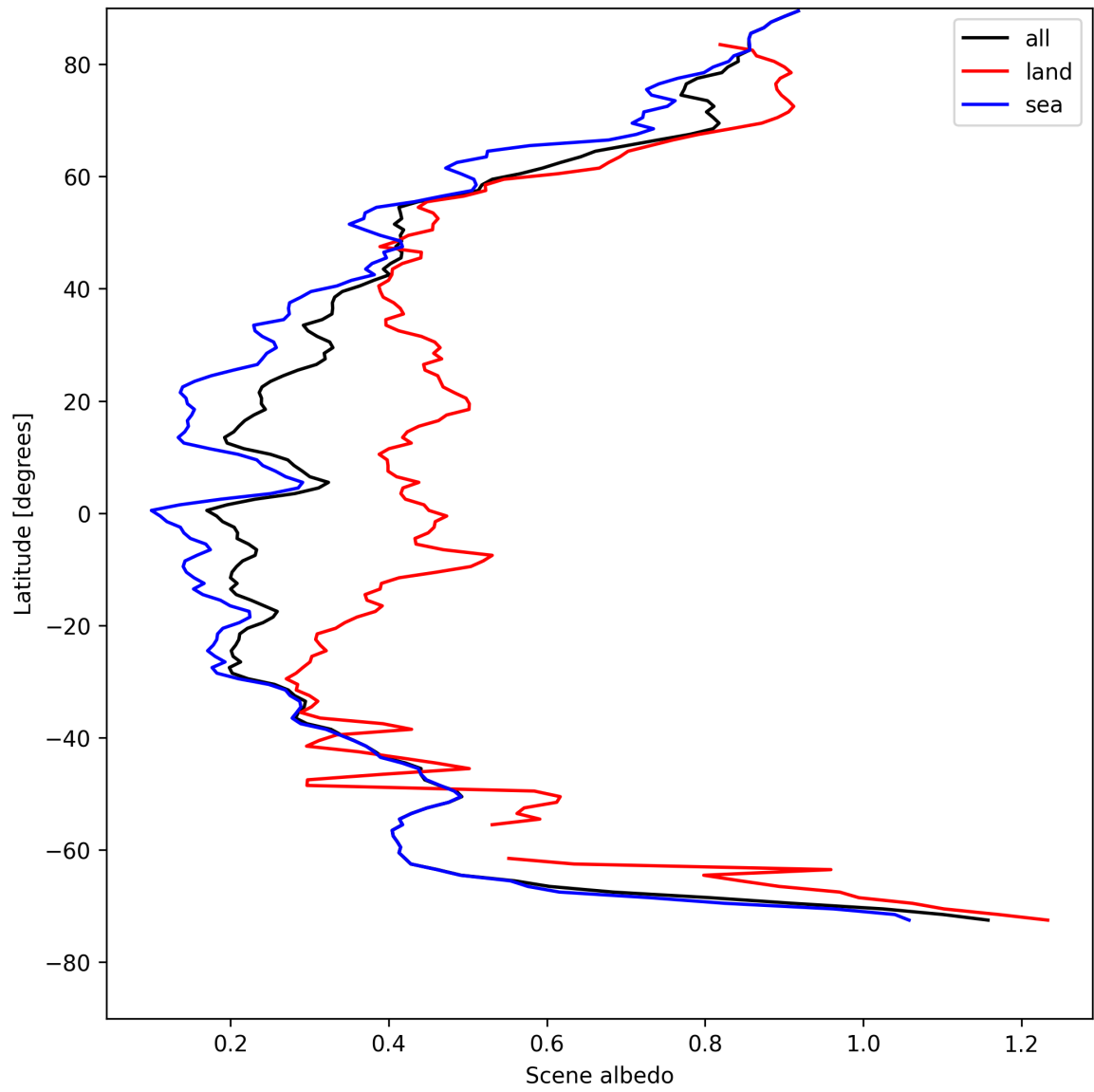
Figure 17: Zonal average of “Scene albedo” for 2025-04-30 to 2025-05-02.
