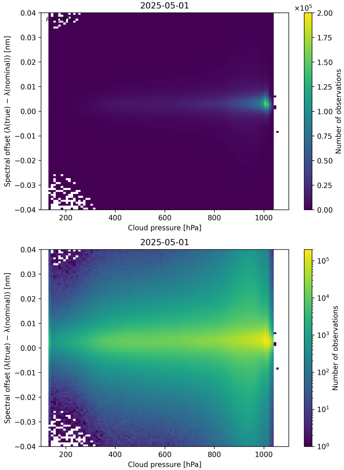
Figure 84: Scatter density plot of “Cloud pressure” against “Spectral offset ( \lambda_{\text{true}} - \lambda_{\text{nominal}} )” for 2025-04-30 to 2025-05-02.
