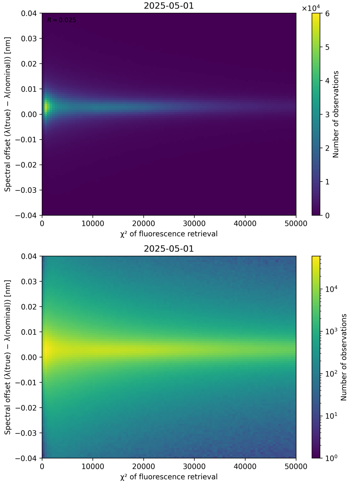
Figure 69: Scatter density plot of “ \chi^2 of fluorescence retrieval” against “Spectral offset ( \lambda_{\text{true}} - \lambda_{\text{nominal}} )” for 2025-04-30 to 2025-05-02.
