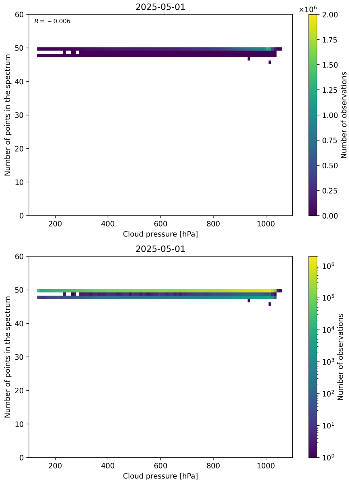
Figure 82: Scatter density plot of “Cloud pressure” against “Number of points in the spectrum” for 2025-04-30 to 2025-05-02.
