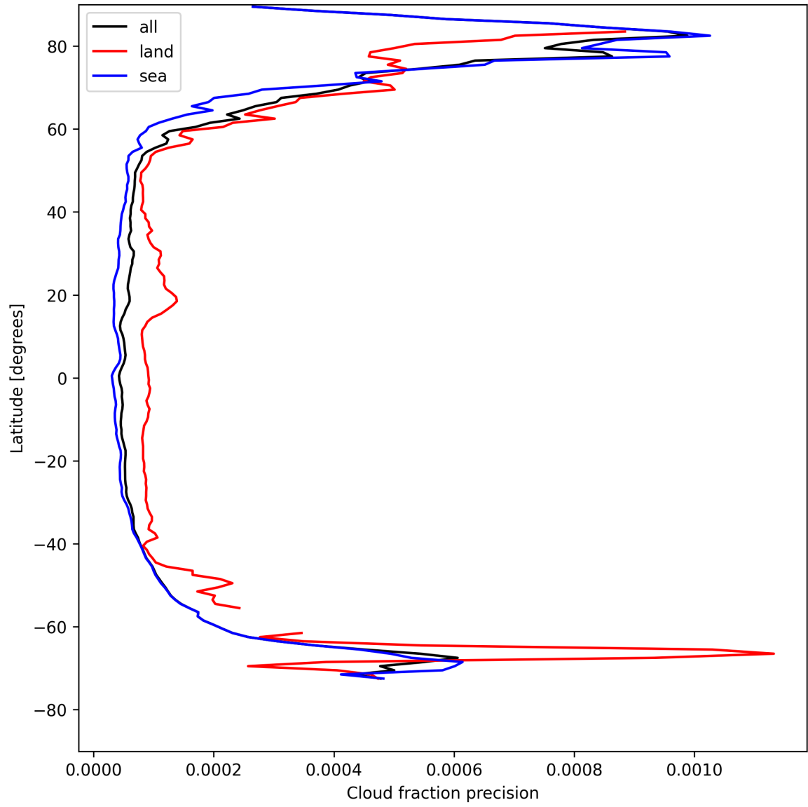
Figure 16: Zonal average of “Cloud fraction precision” for 2025-04-30 to 2025-05-02.
