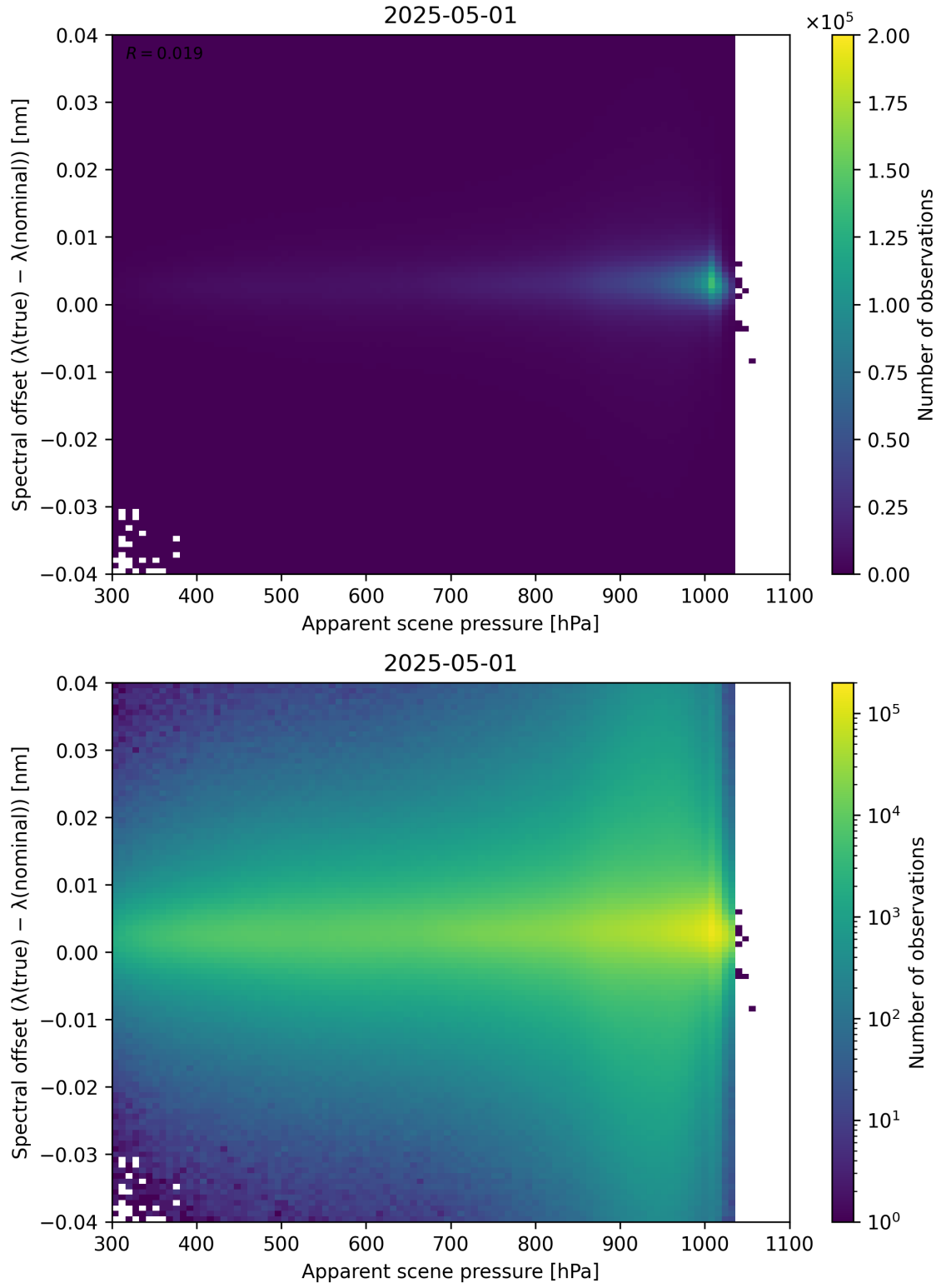
Figure 67: Scatter density plot of “Apparent scene pressure” against “Spectral offset ( \lambda_{\text{true}} - \lambda_{\text{nominal}} )” for 2025-04-30 to 2025-05-02.
