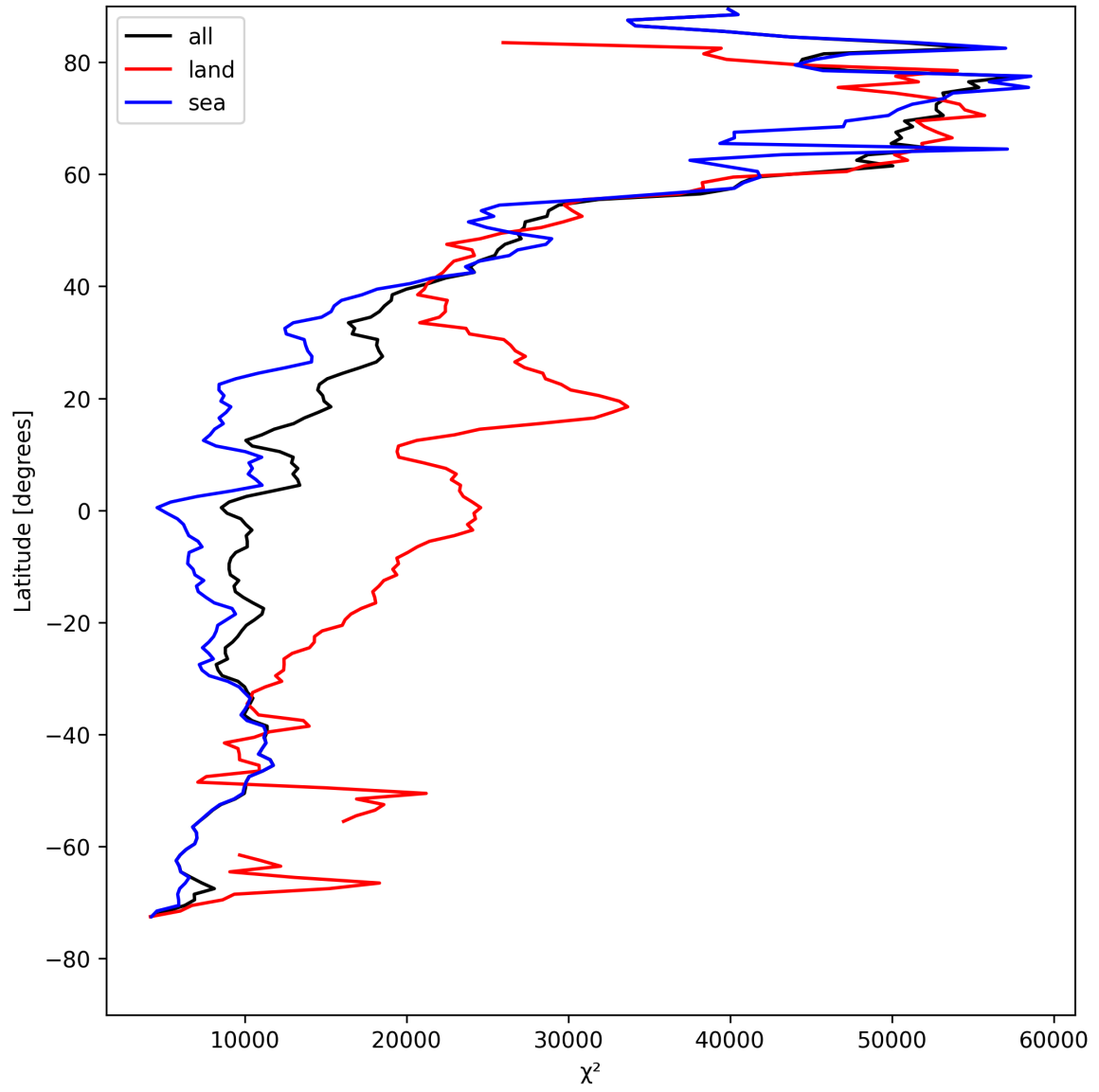
Figure 21: Zonal average of “ \chi^2 ” for 2025-04-30 to 2025-05-02.
