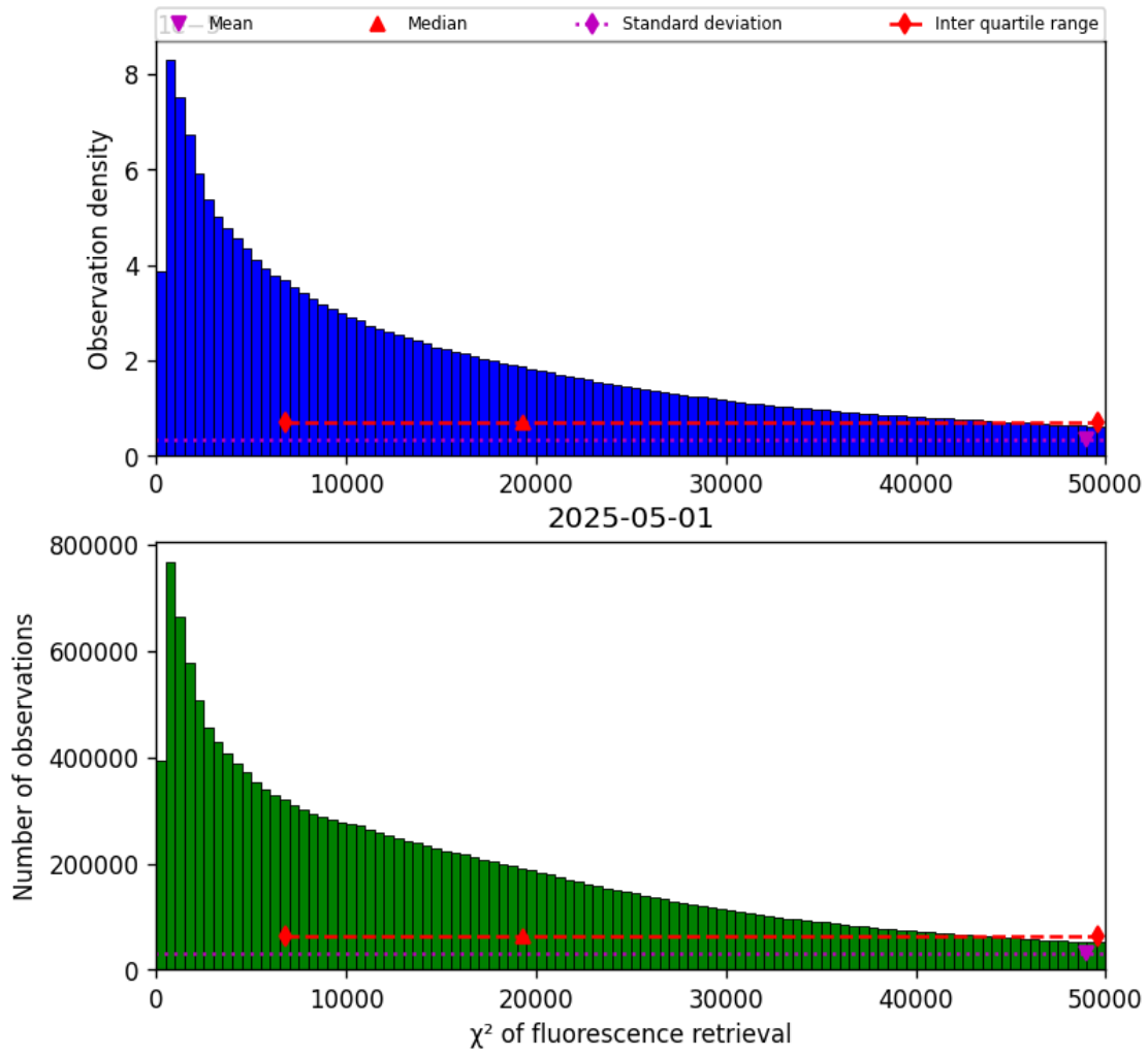
Figure 42: Histogram of “ \chi^2 of fluorescence retrieval” for 2025-04-30 to 2025-05-02
