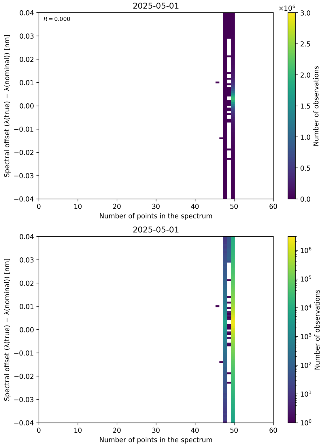
Figure 101: Scatter density plot of “Number of points in the spectrum” against “Spectral offset ( \lambda_{\text{true}} - \lambda_{\text{nominal}} )” for 2025-04-30 to 2025-05-02.
