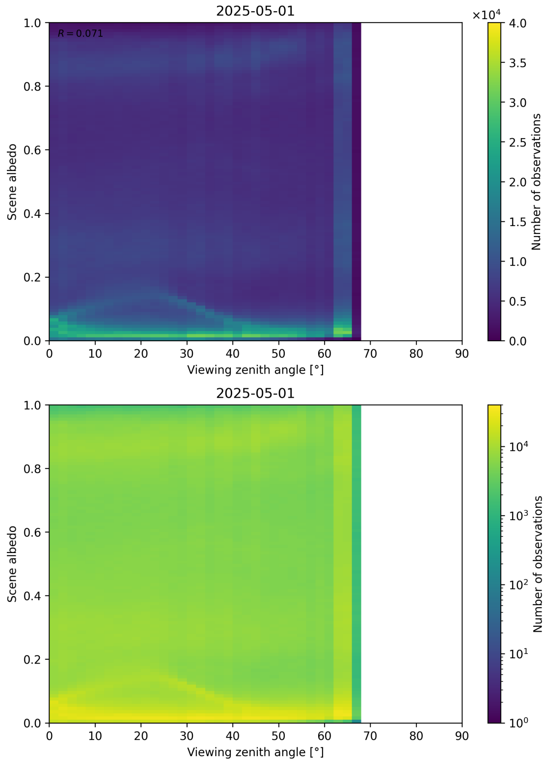
Figure 126: Scatter density plot of “Viewing zenith angle” against “Scene albedo” for 2025-04-30 to 2025-05-02.
