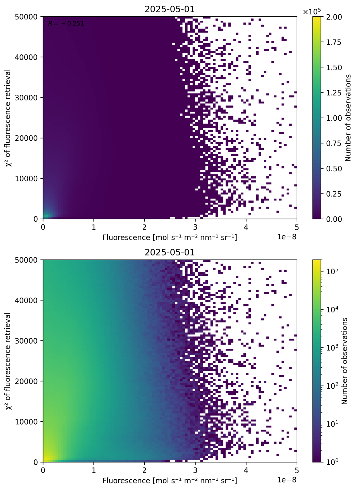
Figure 85: Scatter density plot of “Fluorescence” against “ \chi^2 of fluorescence retrieval” for 2025-04-30 to 2025-05-02.
