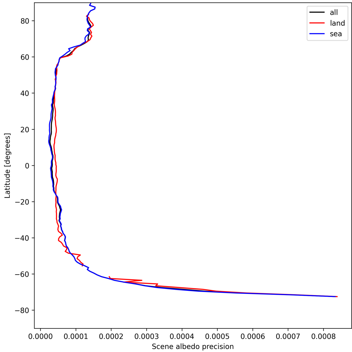
Figure 18: Zonal average of “Scene albedo precision” for 2025-04-30 to 2025-05-02.
