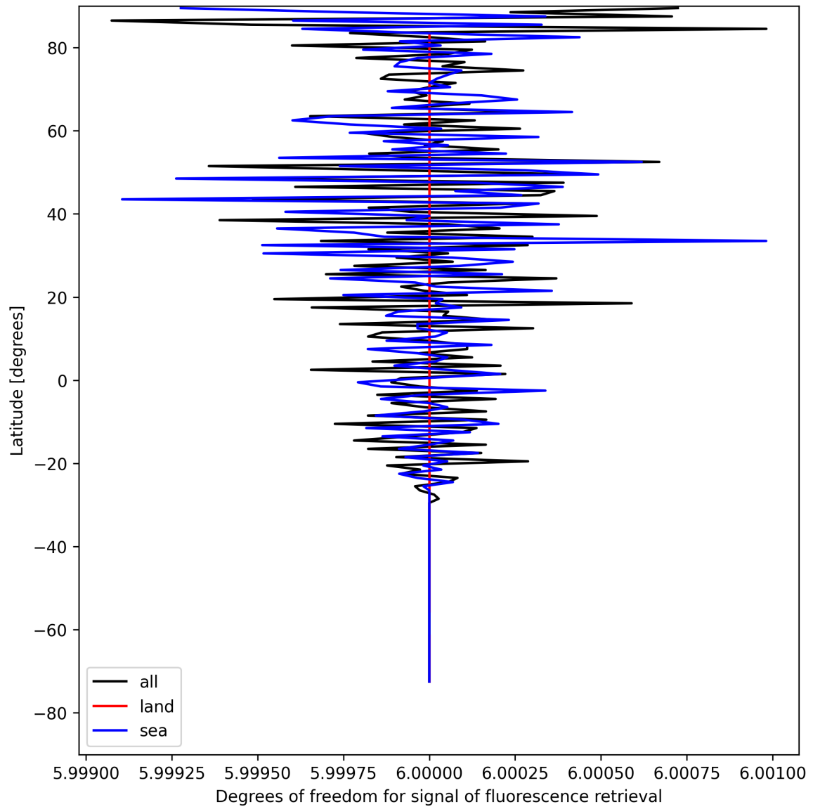
Figure 26: Zonal average of “Degrees of freedom for signal of fluorescence retrieval” for 2025-04-30 to 2025-05-02.
