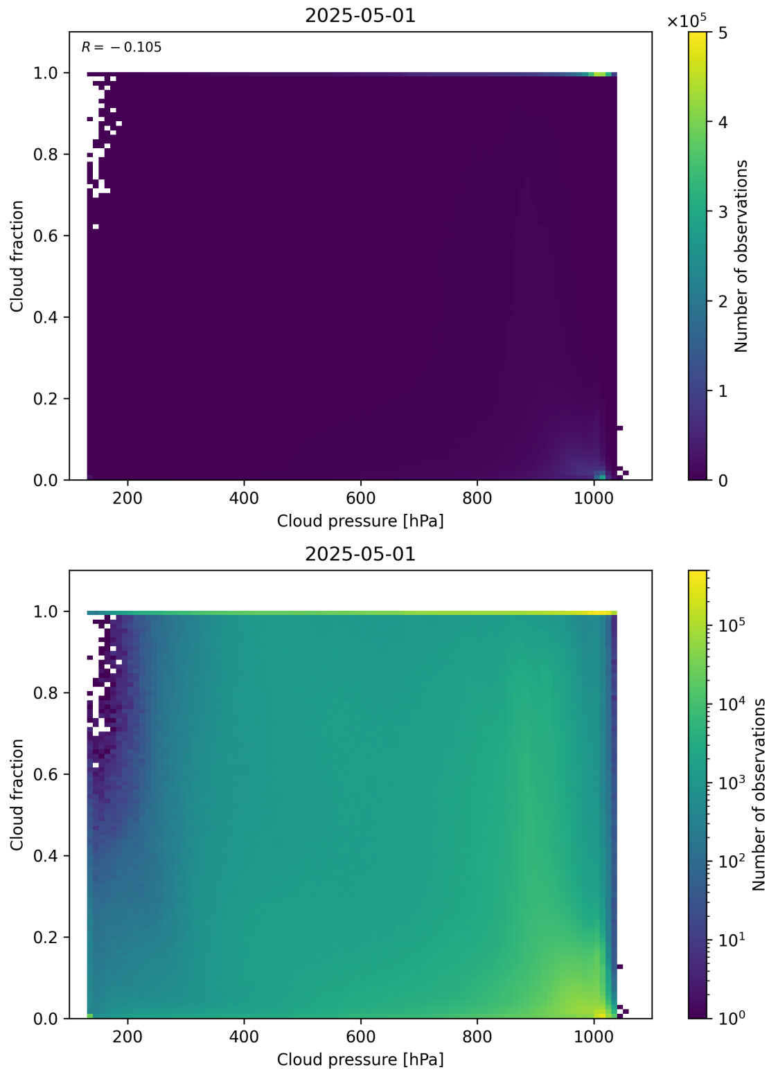
Figure 79: Scatter density plot of “Cloud pressure” against “Cloud fraction” for 2025-04-30 to 2025-05-02.
