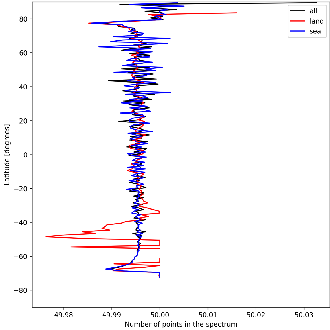
Figure 27: Zonal average of “Number of points in the spectrum” for 2025-04-30 to 2025-05-02.
