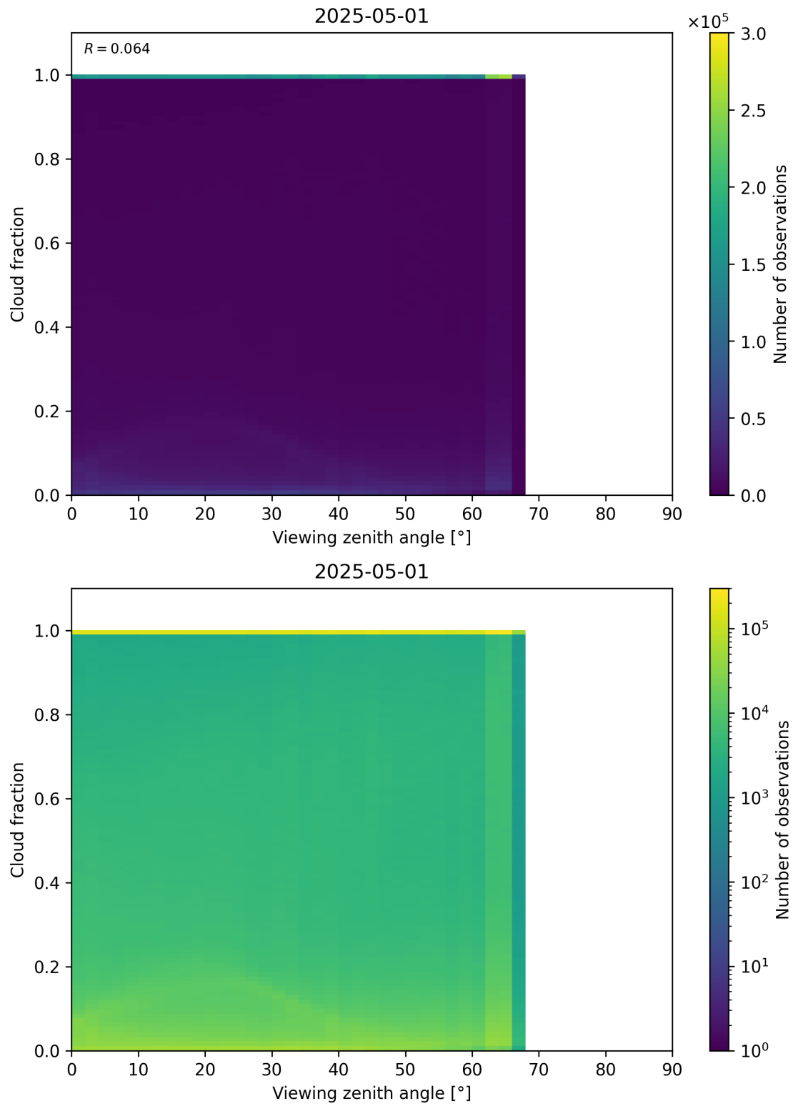
Figure 120: Scatter density plot of “Viewing zenith angle” against “Cloud fraction” for 2025-04-30 to 2025-05-02.
