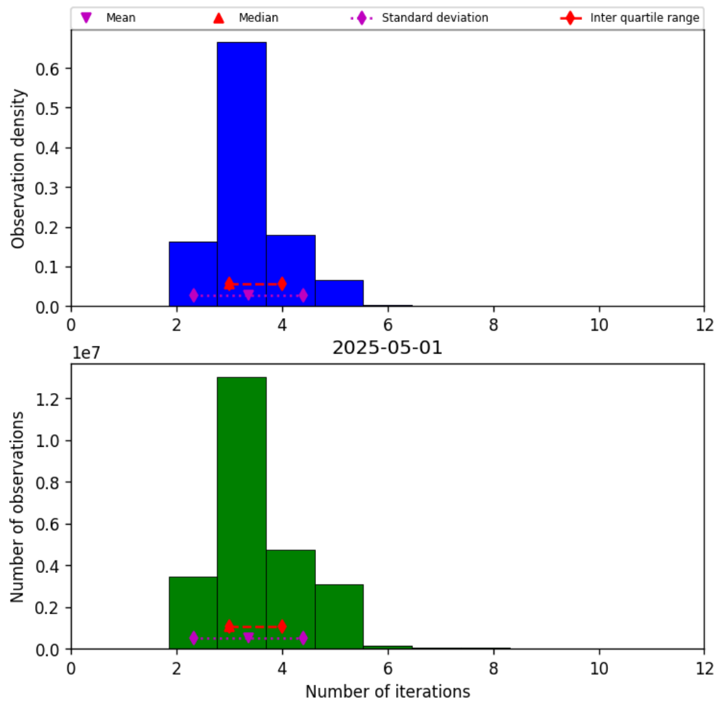
Figure 39: Histogram of “Number of iterations” for 2025-04-30 to 2025-05-02
