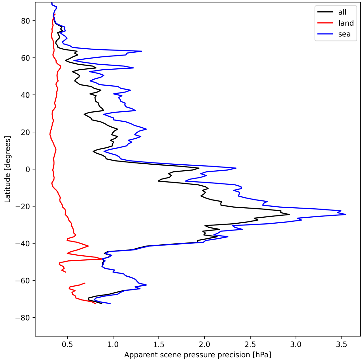
Figure 20: Zonal average of “Apparent scene pressure precision” for 2025-04-30 to 2025-05-02.
