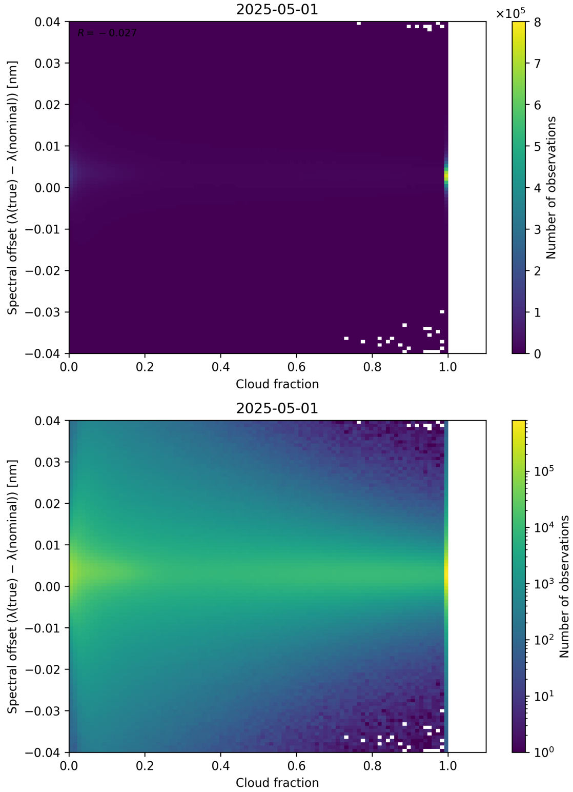
Figure 76: Scatter density plot of “Cloud fraction” against “Spectral offset ( \lambda_{\text{true}} - \lambda_{\text{nominal}} )” for 2025-04-30 to 2025-05-02.
