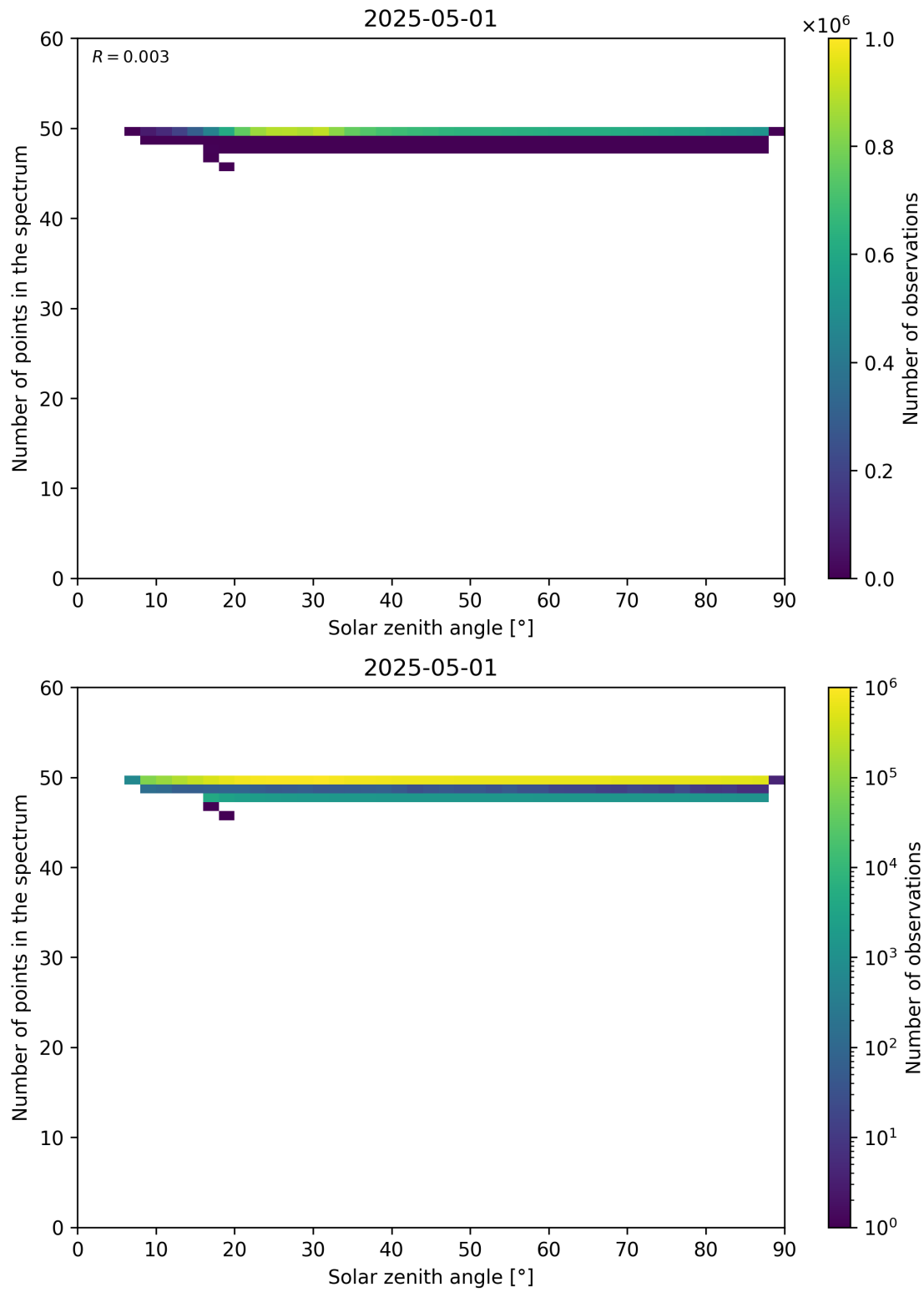
Figure 115: Scatter density plot of “Solar zenith angle” against “Number of points in the spectrum” for 2025-04-30 to 2025-05-02.
