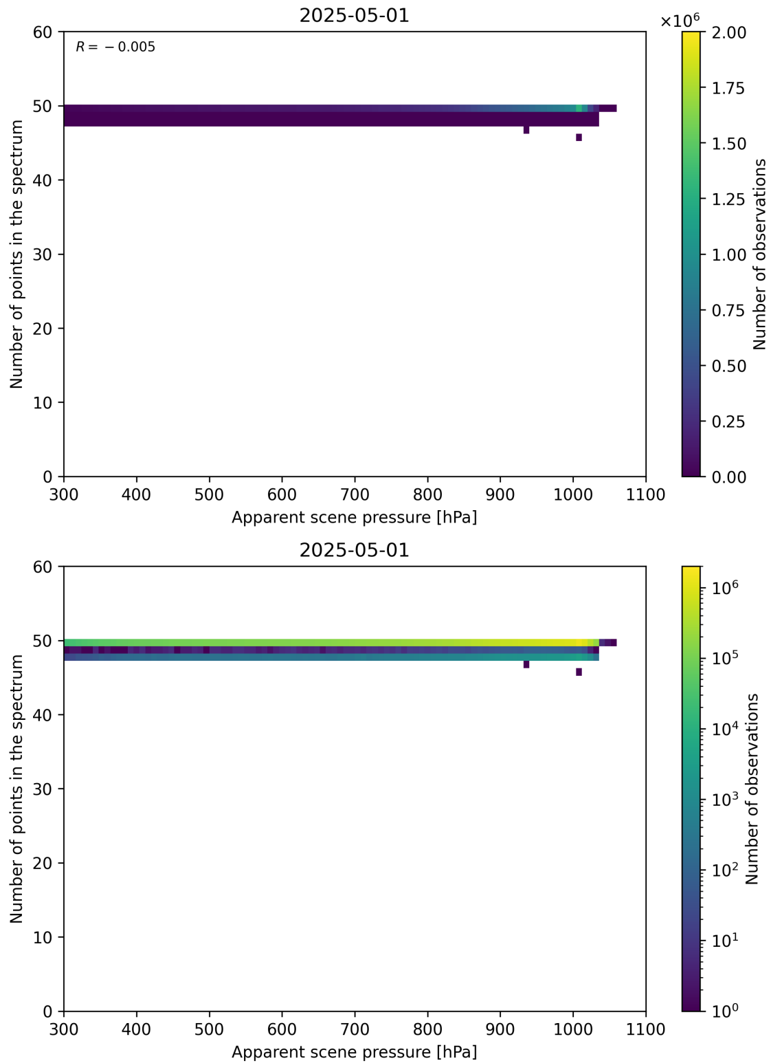
Figure 66: Scatter density plot of “Apparent scene pressure” against “Number of points in the spectrum” for 2025-04-30 to 2025-05-02.
