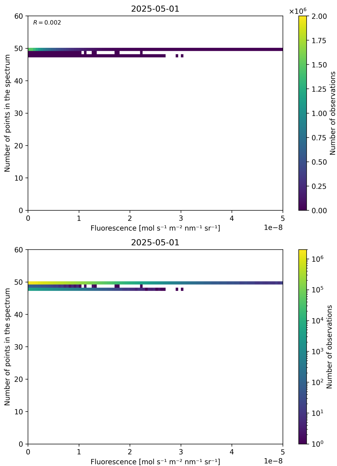
Figure 86: Scatter density plot of “Fluorescence” against “Number of points in the spectrum” for 2025-04-30 to 2025-05-02.
