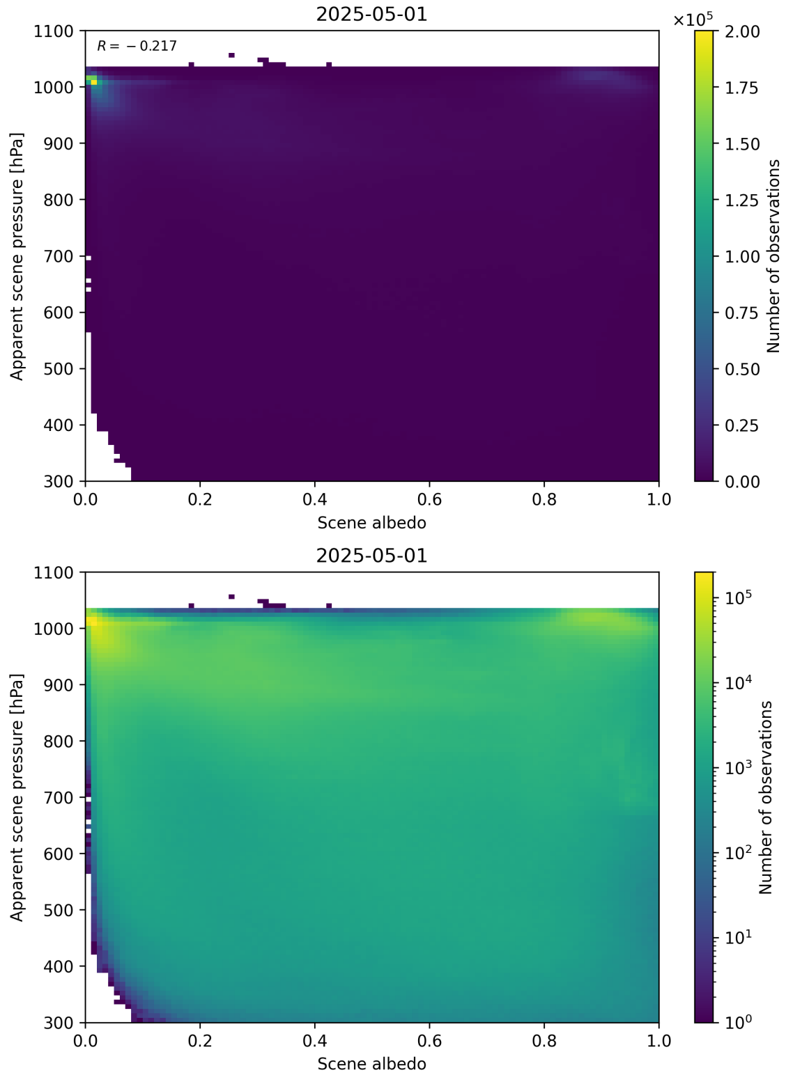
Figure 102: Scatter density plot of “Scene albedo” against “Apparent scene pressure” for 2025-04-30 to 2025-05-02.
