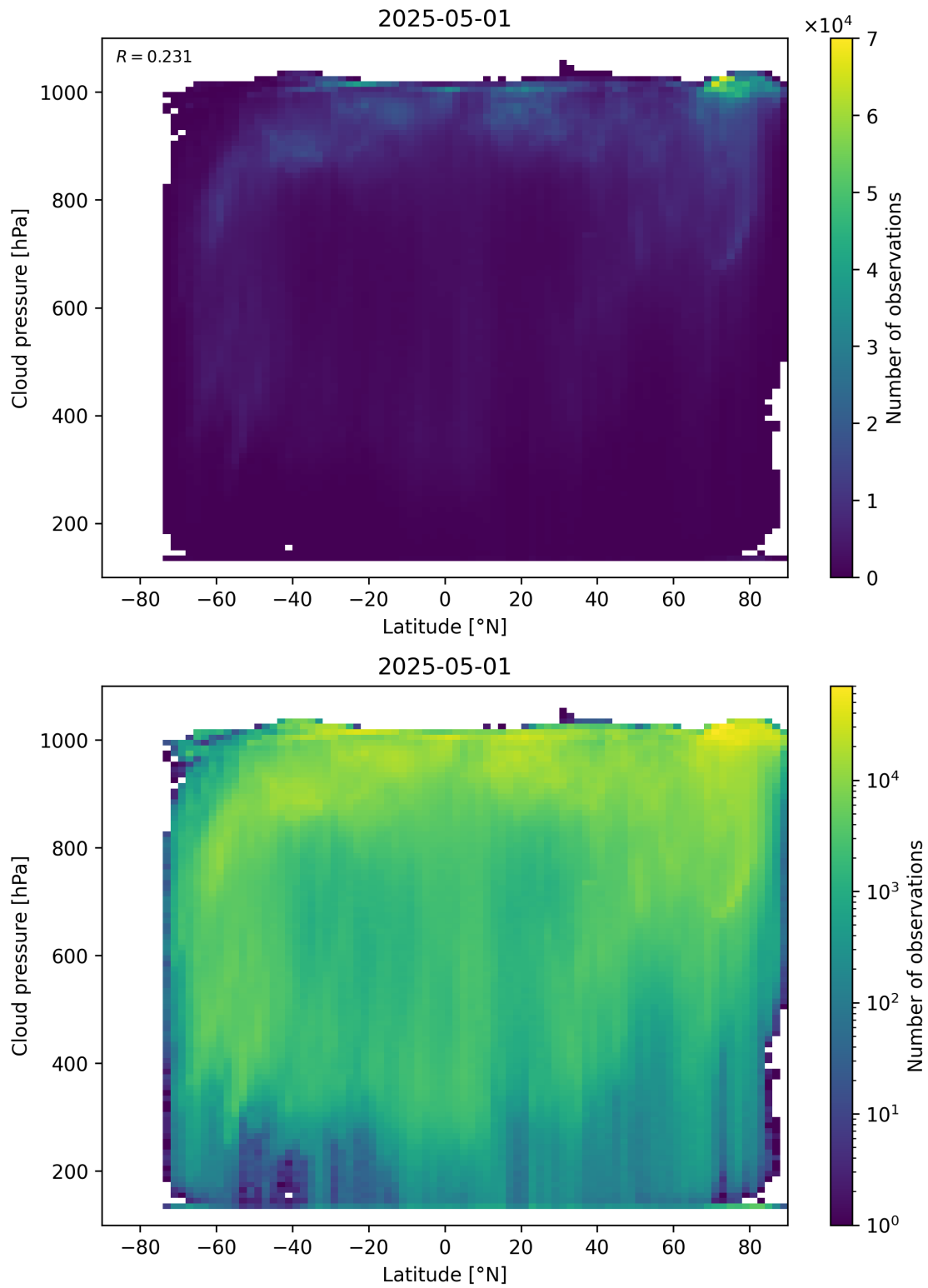
Figure 91: Scatter density plot of “Latitude” against “Cloud pressure” for 2025-04-30 to 2025-05-02.
