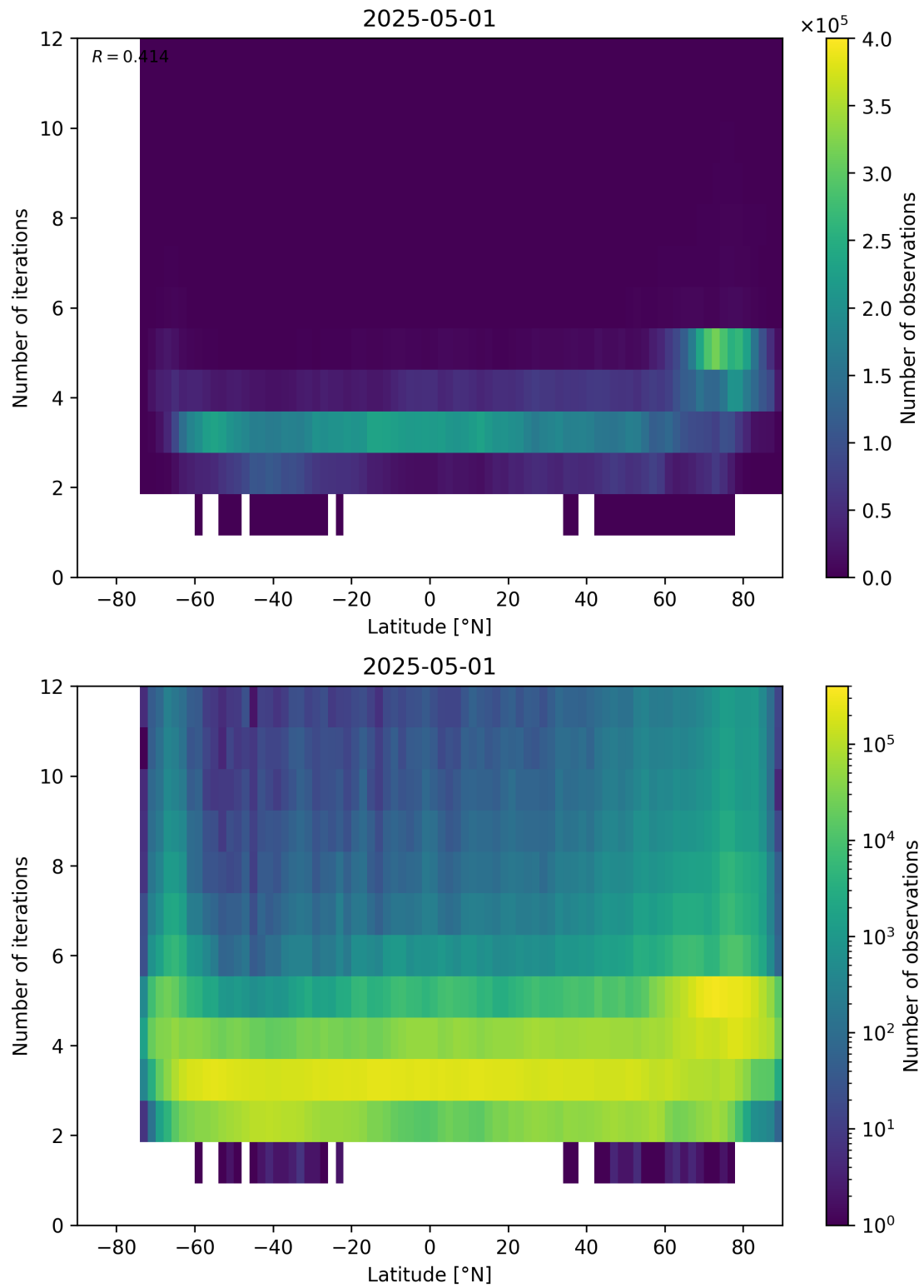
Figure 93: Scatter density plot of “Latitude” against “Number of iterations” for 2025-04-30 to 2025-05-02.
