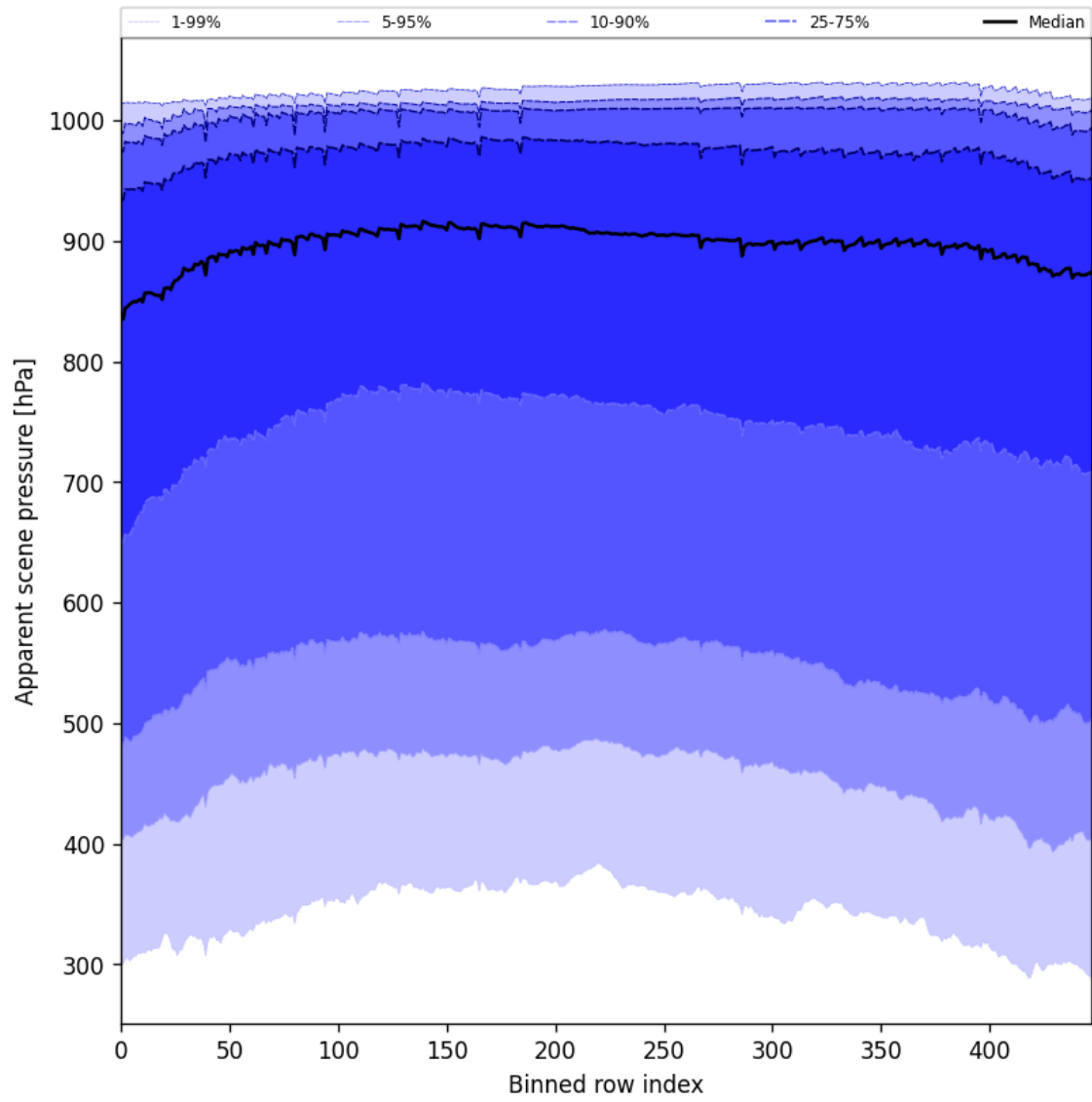
Figure 53: Along track statistics of “Apparent scene pressure” for 2025-04-30 to 2025-05-02
