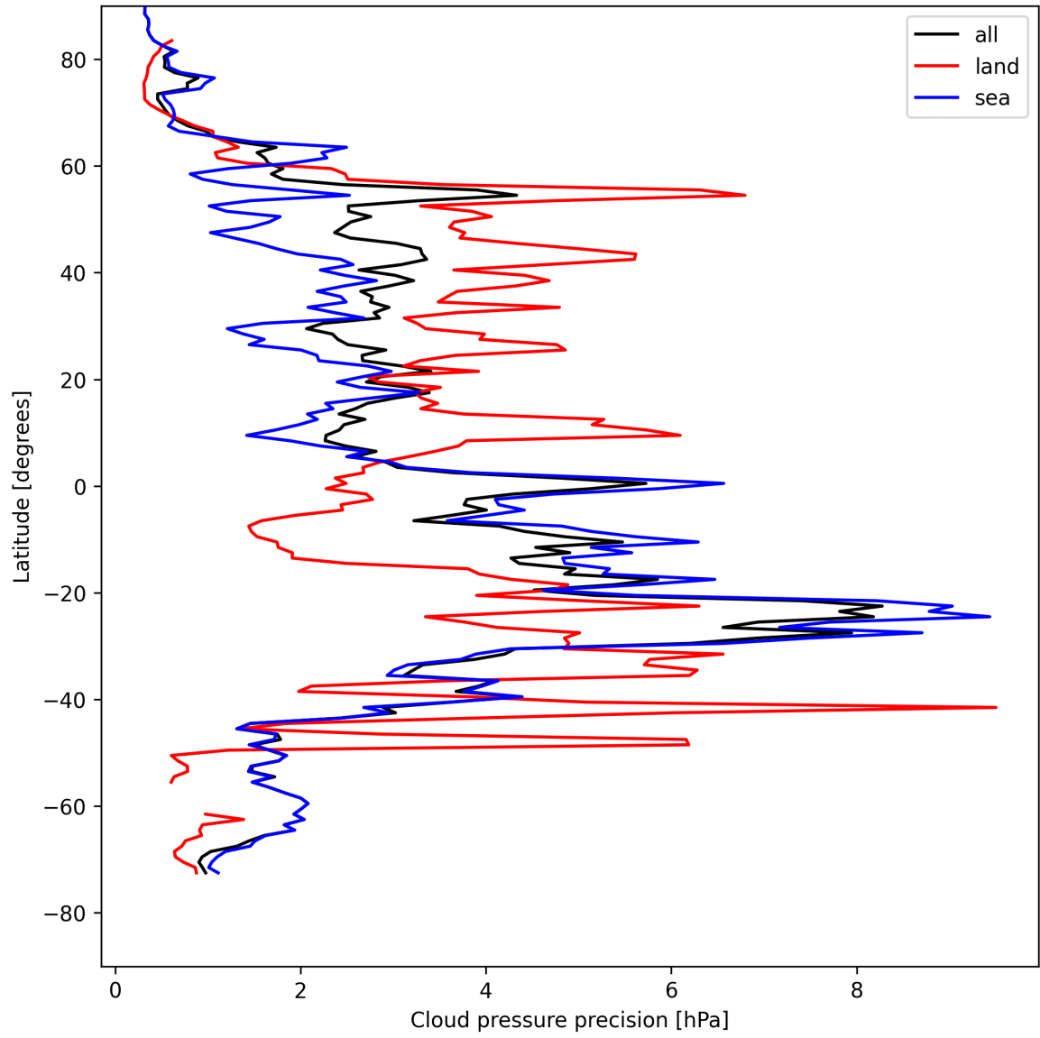
Figure 14: Zonal average of “Cloud pressure precision” for 2025-04-30 to 2025-05-02.
