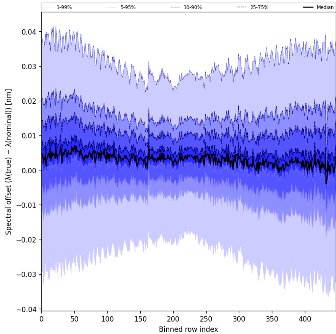
Figure 62: Along track statistics of “Spectral offset ( \lambda_{\text{true}} - \lambda_{\text{nominal}} )” for 2025-04-30 to 2025-05-02
