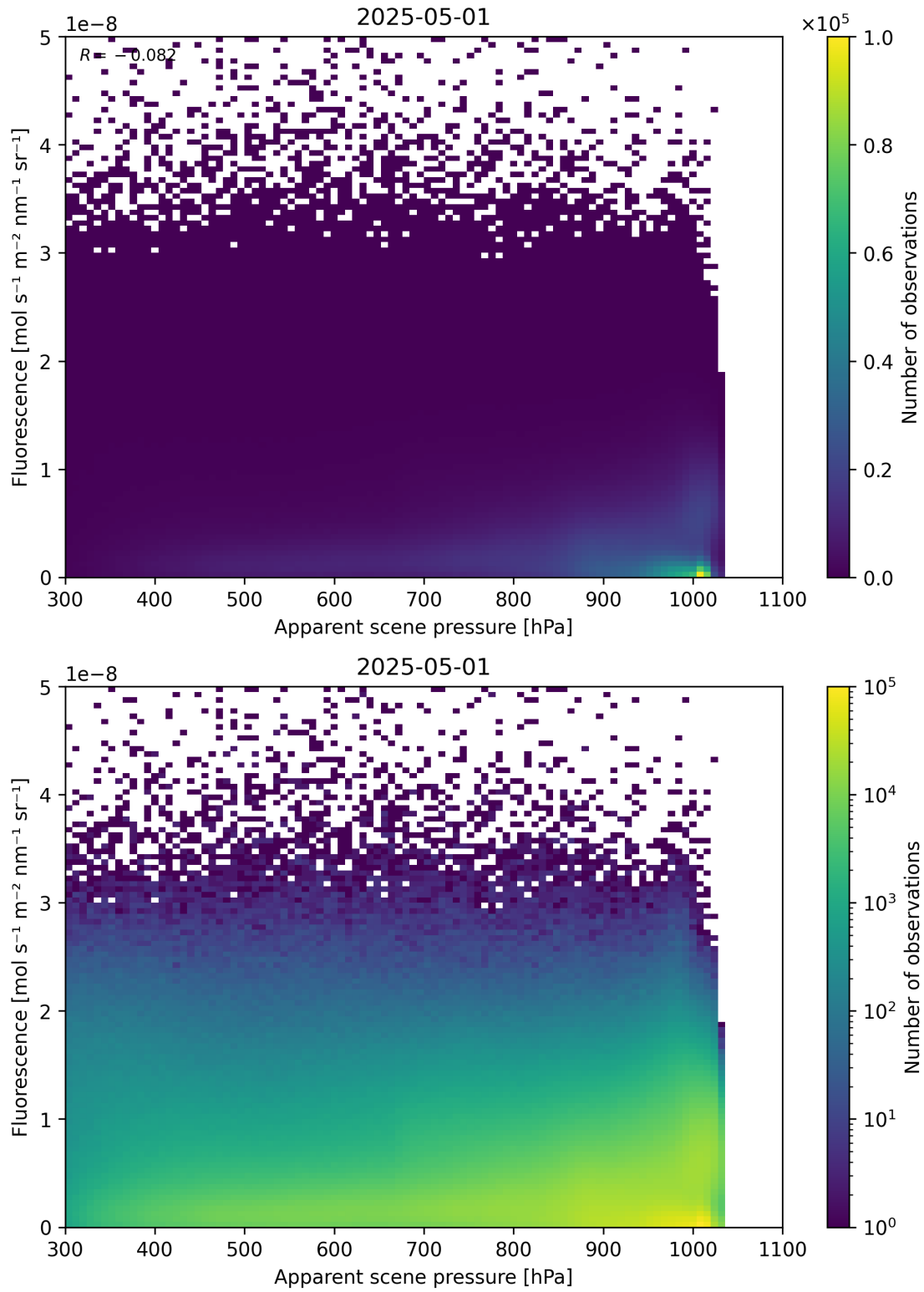
Figure 64: Scatter density plot of “Apparent scene pressure” against “Fluorescence” for 2025-04-30 to 2025-05-02.
