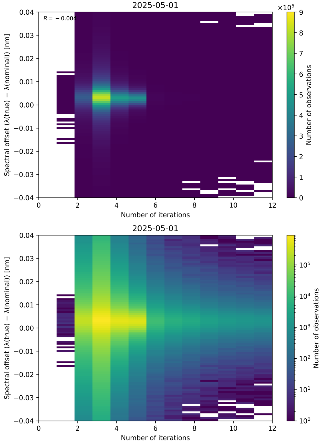
Figure 100: Scatter density plot of “Number of iterations” against “Spectral offset ( \lambda_{\text{true}} - \lambda_{\text{nominal}} )” for 2025-04-30 to 2025-05-02.
