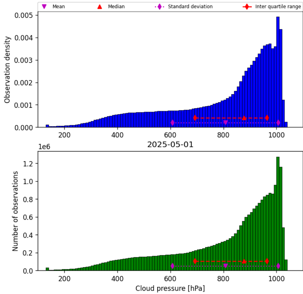
Figure 30: Histogram of “Cloud pressure” for 2025-04-30 to 2025-05-02
