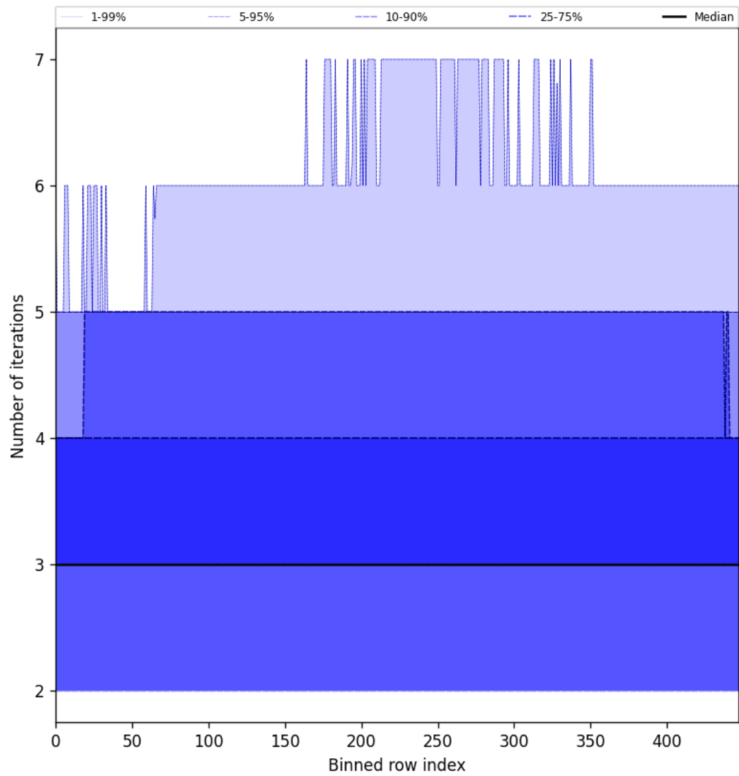
Figure 56: Along track statistics of “Number of iterations” for 2025-04-30 to 2025-05-02
