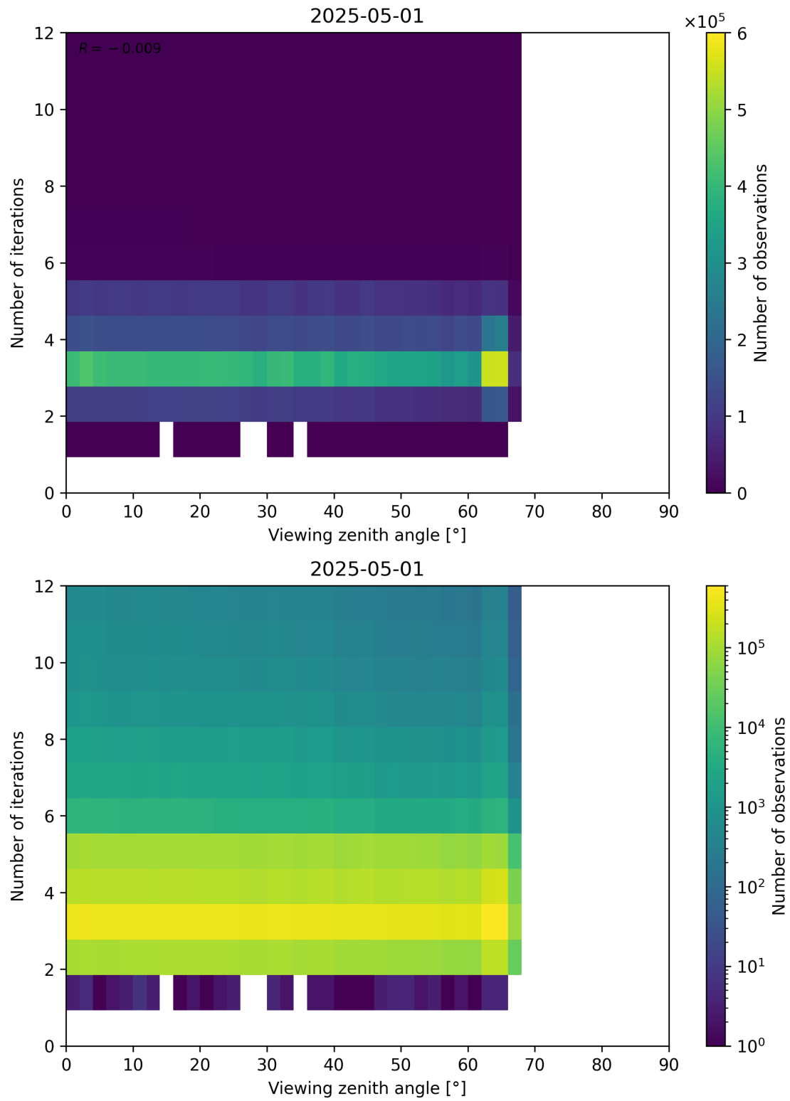
Figure 124: Scatter density plot of “Viewing zenith angle” against “Number of iterations” for 2025-04-30 to 2025-05-02.
