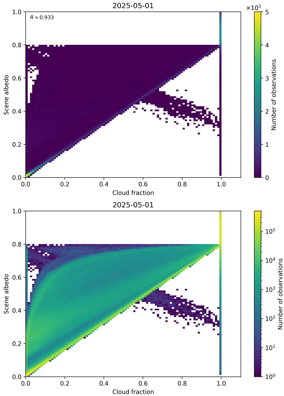
Figure 75: Scatter density plot of “Cloud fraction” against “Scene albedo” for 2025-04-30 to 2025-05-02.
