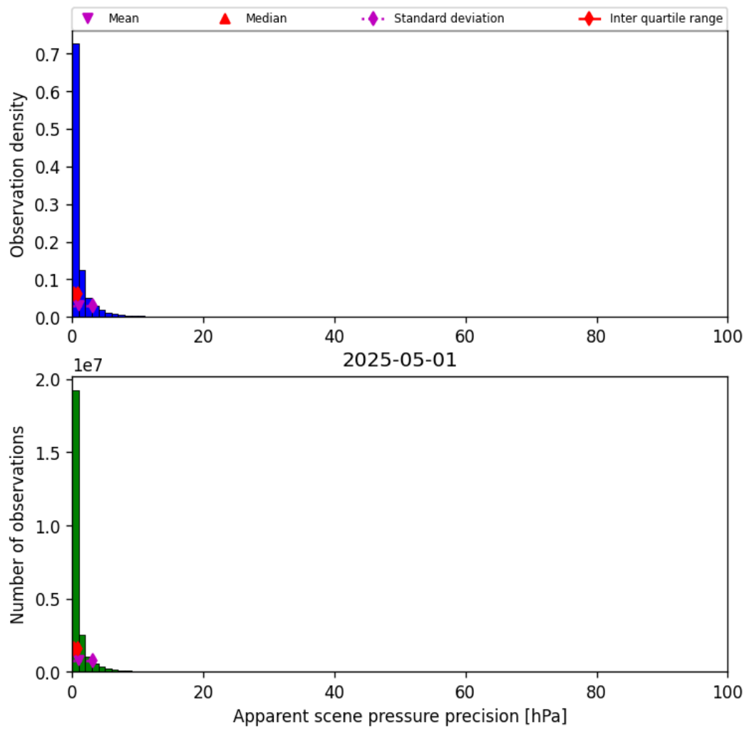
Figure 37: Histogram of “Apparent scene pressure precision” for 2025-04-30 to 2025-05-02
