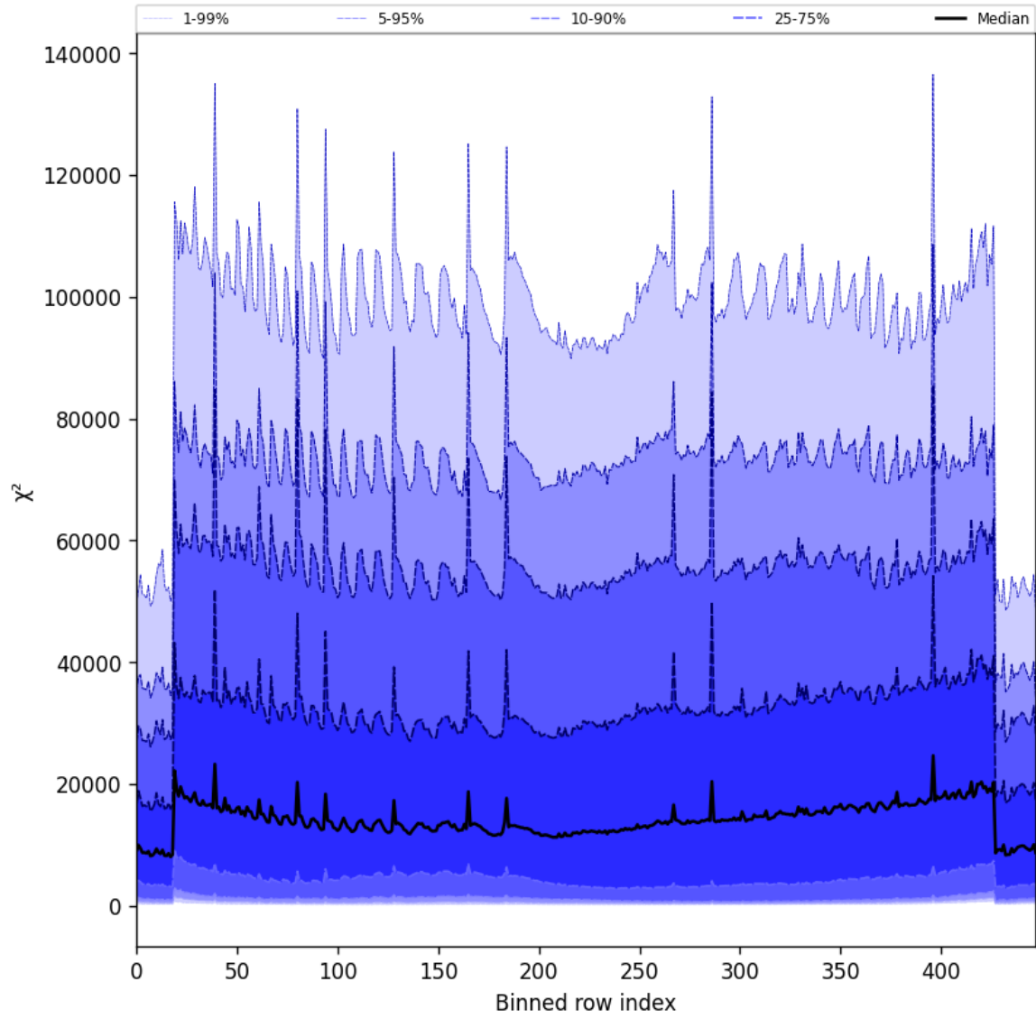
Figure 55: Along track statistics of “ \chi^2 ” for 2025-04-30 to 2025-05-02
