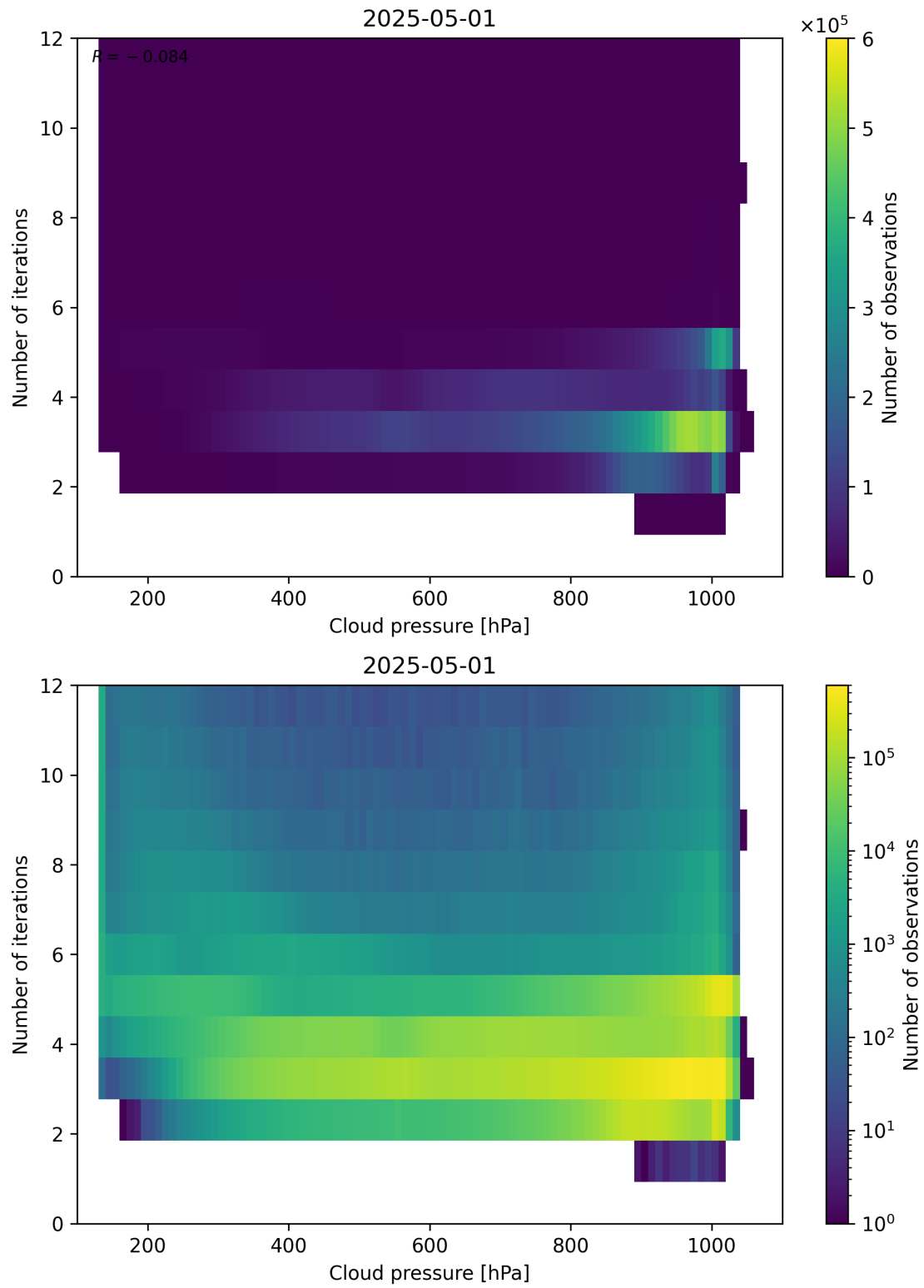
Figure 81: Scatter density plot of “Cloud pressure” against “Number of iterations” for 2025-04-30 to 2025-05-02.
