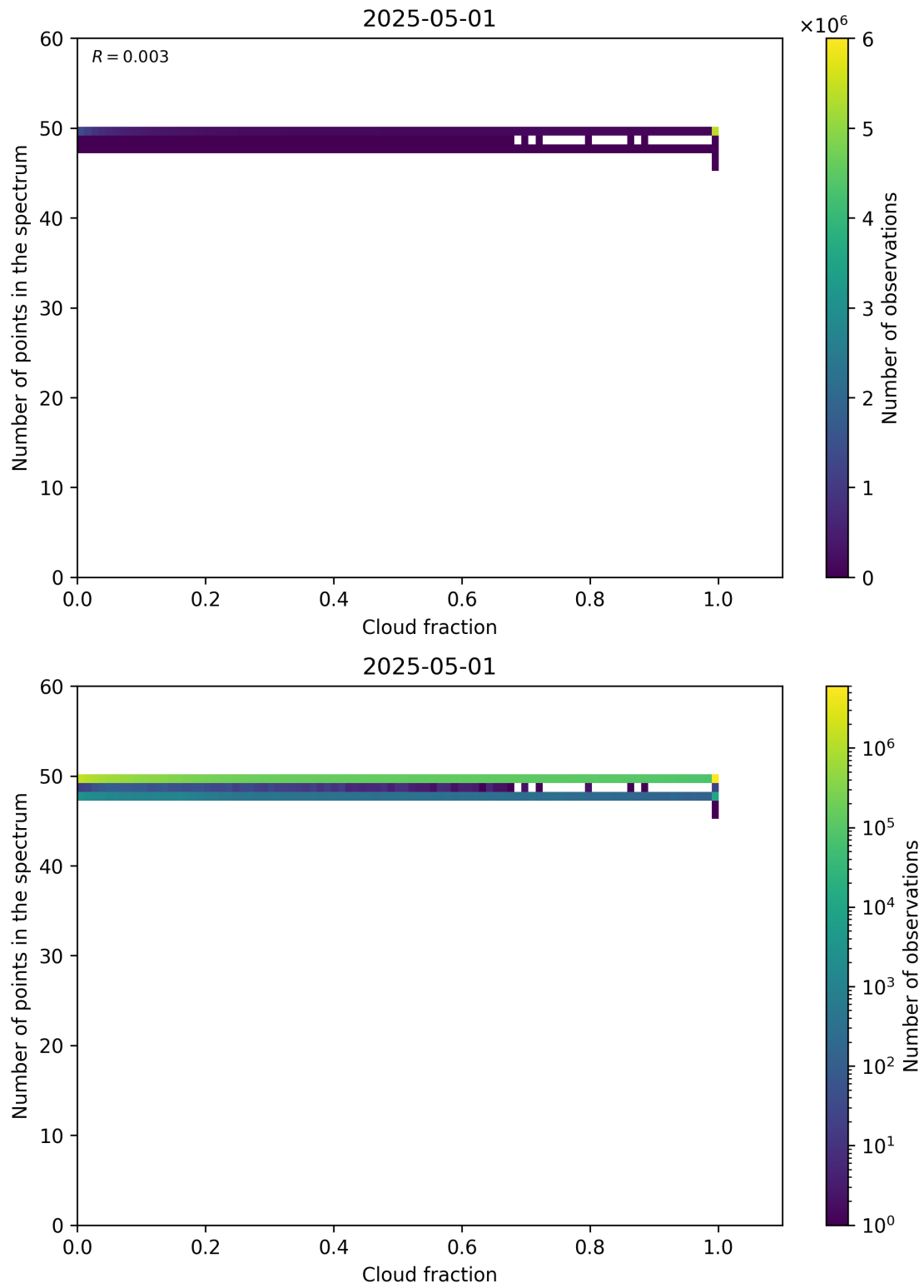
Figure 74: Scatter density plot of “Cloud fraction” against “Number of points in the spectrum” for 2025-04-30 to 2025-05-02.
