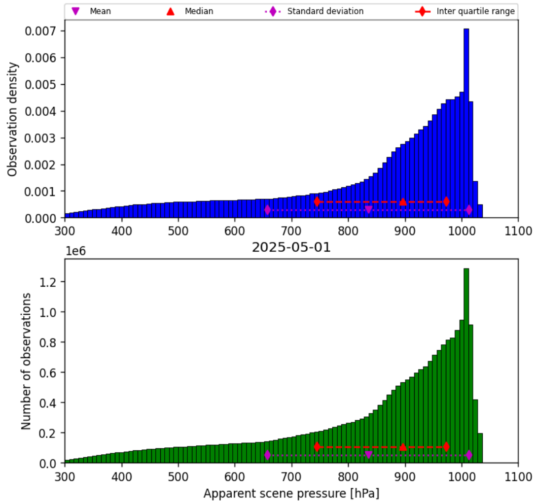
Figure 36: Histogram of “Apparent scene pressure” for 2025-04-30 to 2025-05-02
