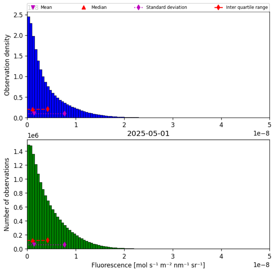
Figure 40: Histogram of “Fluorescence” for 2025-04-30 to 2025-05-02
