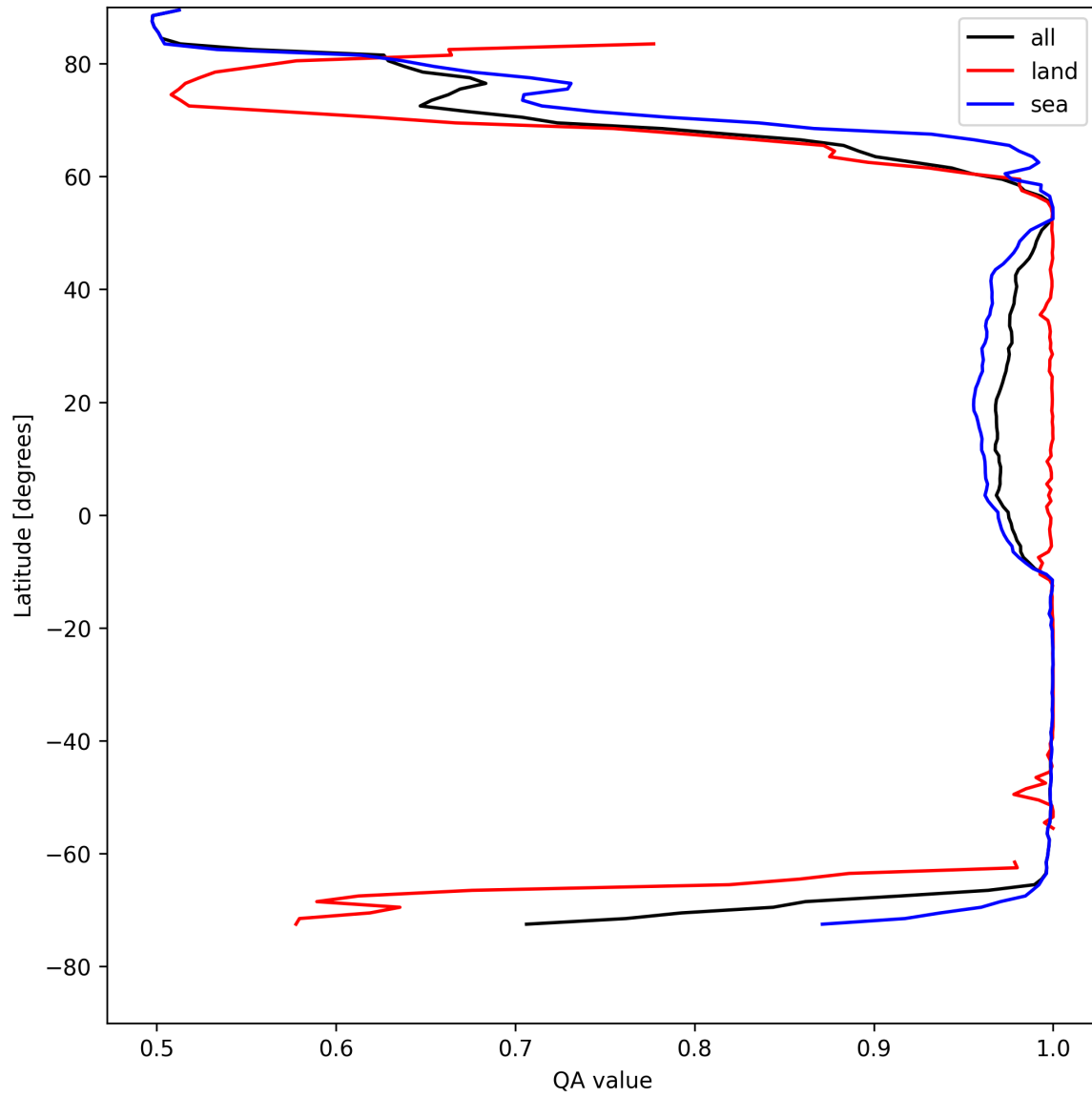
Figure 12: Zonal average of “QA value” for 2025-04-30 to 2025-05-02.
