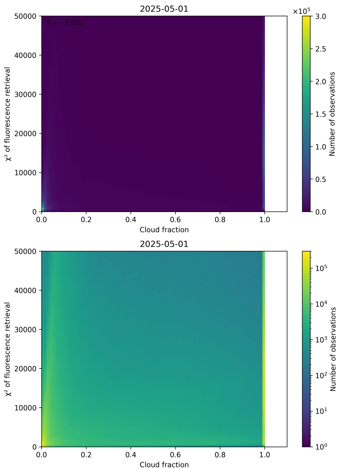
Figure 71: Scatter density plot of “Cloud fraction” against “ \chi^2 of fluorescence retrieval” for 2025-04-30 to 2025-05-02.
