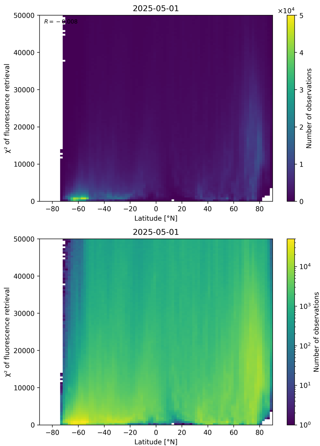
Figure 89: Scatter density plot of “Latitude” against “ \chi^2 of fluorescence retrieval” for 2025-04-30 to 2025-05-02.
