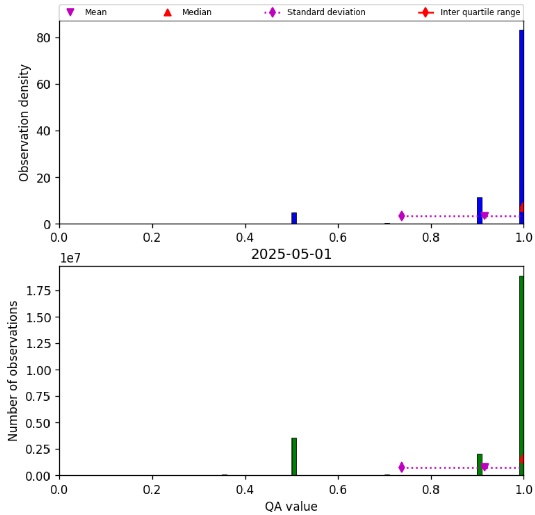
Figure 29: Histogram of “QA value” for 2025-04-30 to 2025-05-02
