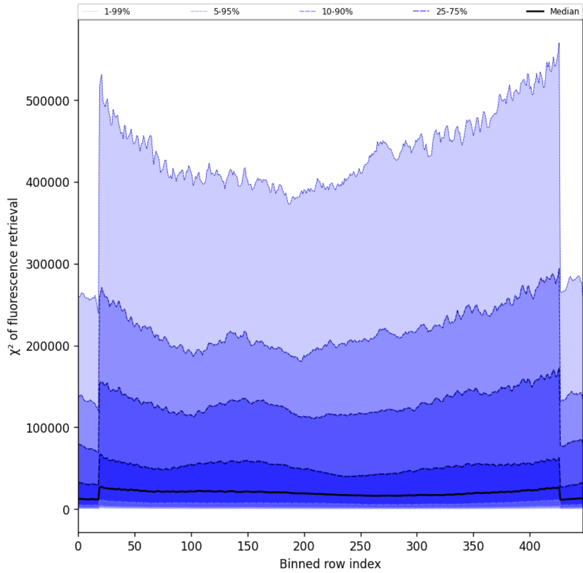
Figure 59: Along track statistics of “ \chi^2 of fluorescence retrieval” for 2025-04-30 to 2025-05-02
