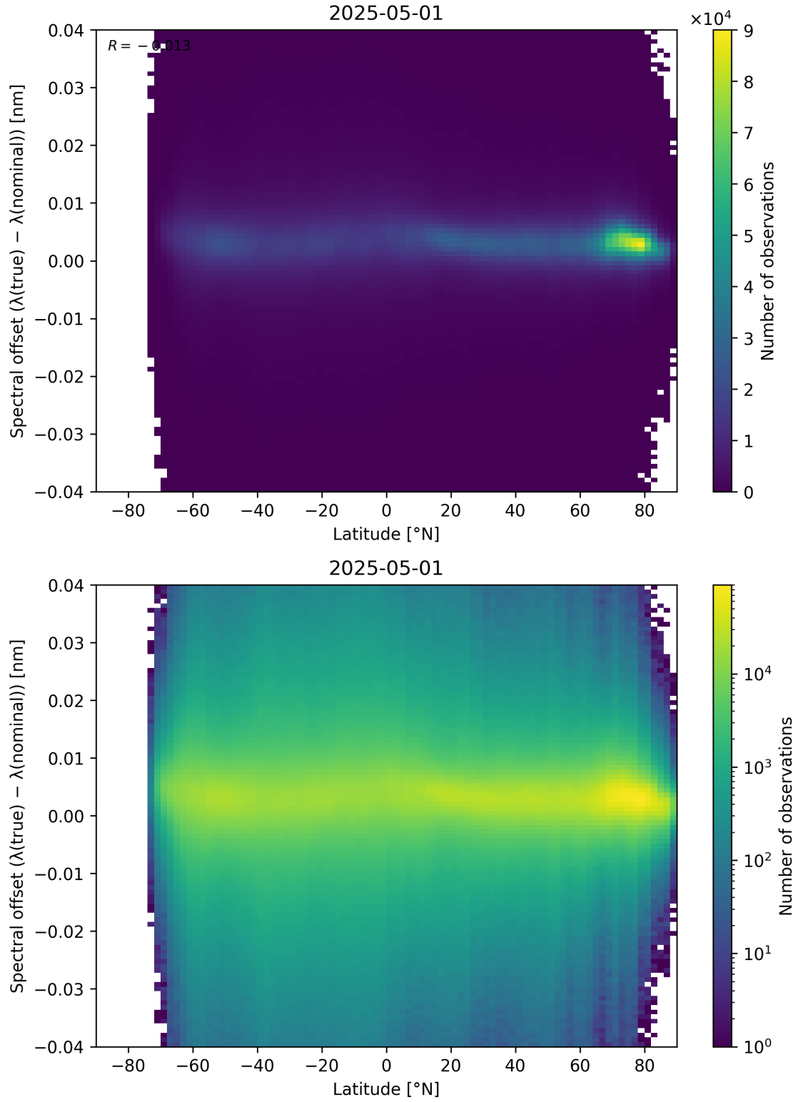
Figure 96: Scatter density plot of “Latitude” against “Spectral offset ( \lambda_{\text{true}} - \lambda_{\text{nominal}} )” for 2025-04-30 to 2025-05-02.
