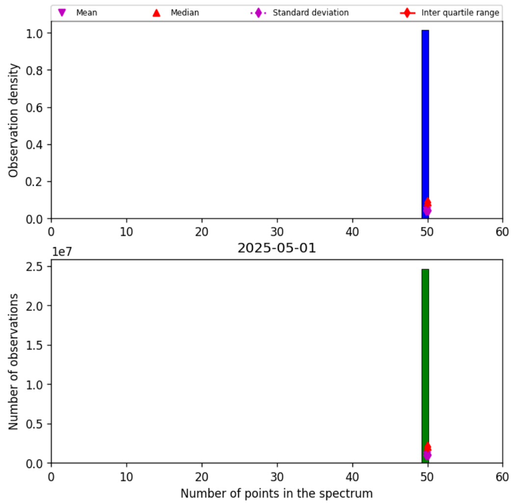
Figure 44: Histogram of "Number of points in the spectrum" for 2025-04-30 to 2025-05-02
