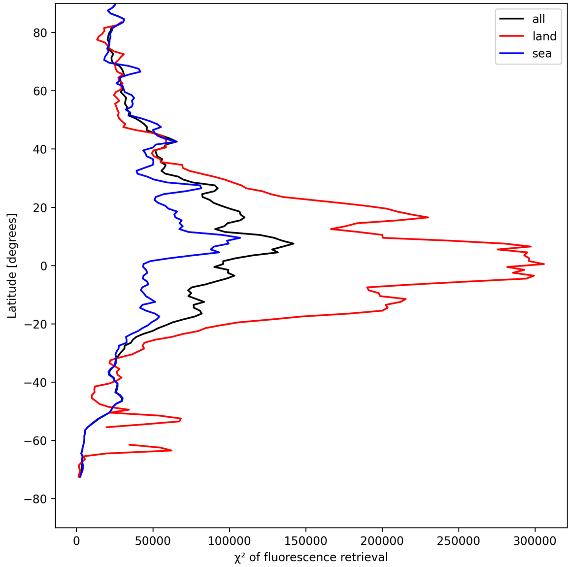
Figure 25: Zonal average of “ \chi^2 of fluorescence retrieval” for 2025-04-30 to 2025-05-02.
