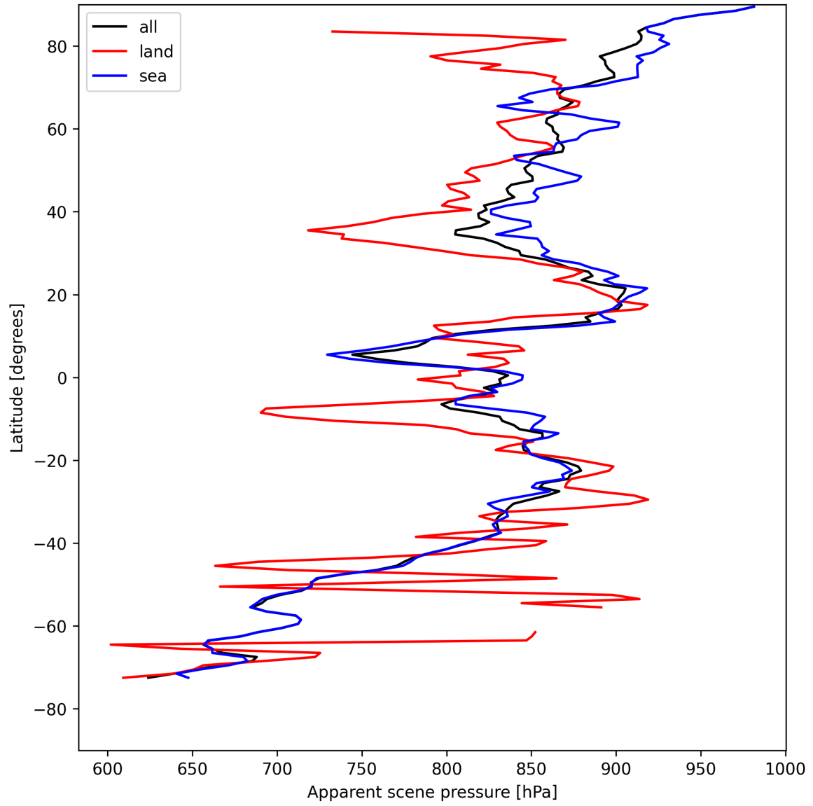
Figure 19: Zonal average of “Apparent scene pressure” for 2025-04-30 to 2025-05-02.
