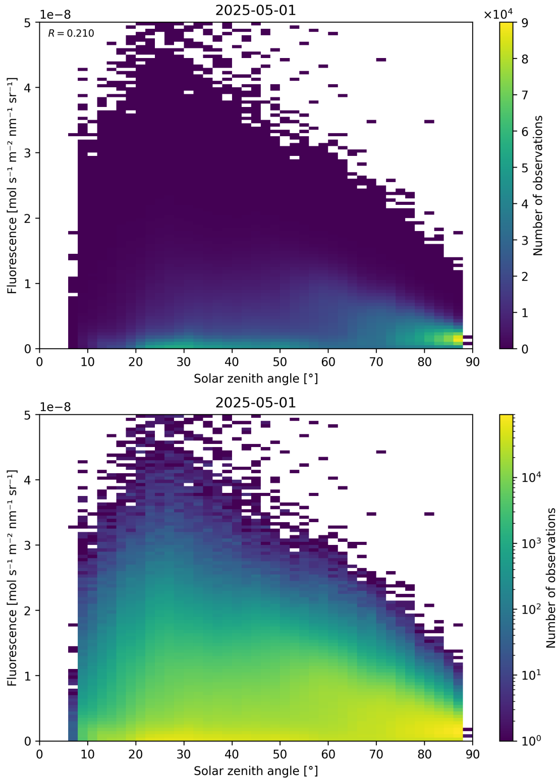
Figure 112: Scatter density plot of “Solar zenith angle” against “Fluorescence” for 2025-04-30 to 2025-05-02.
