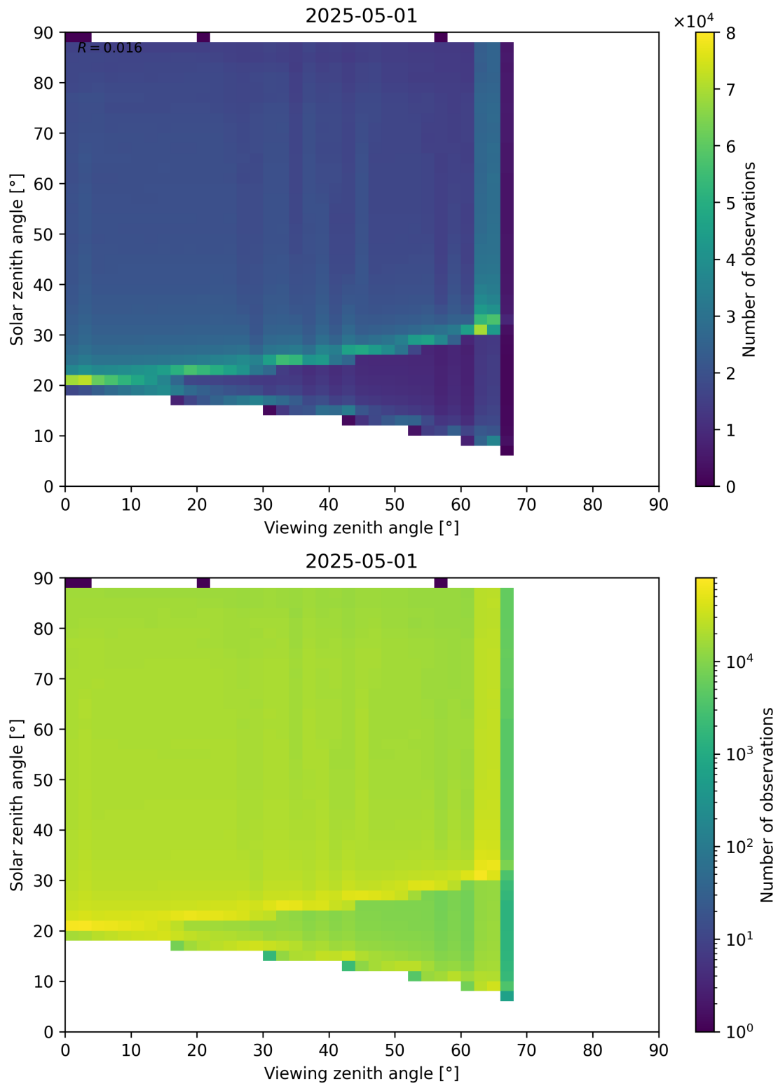
Figure 127: Scatter density plot of “Viewing zenith angle” against “Solar zenith angle” for 2025-04-30 to 2025-05-02.
