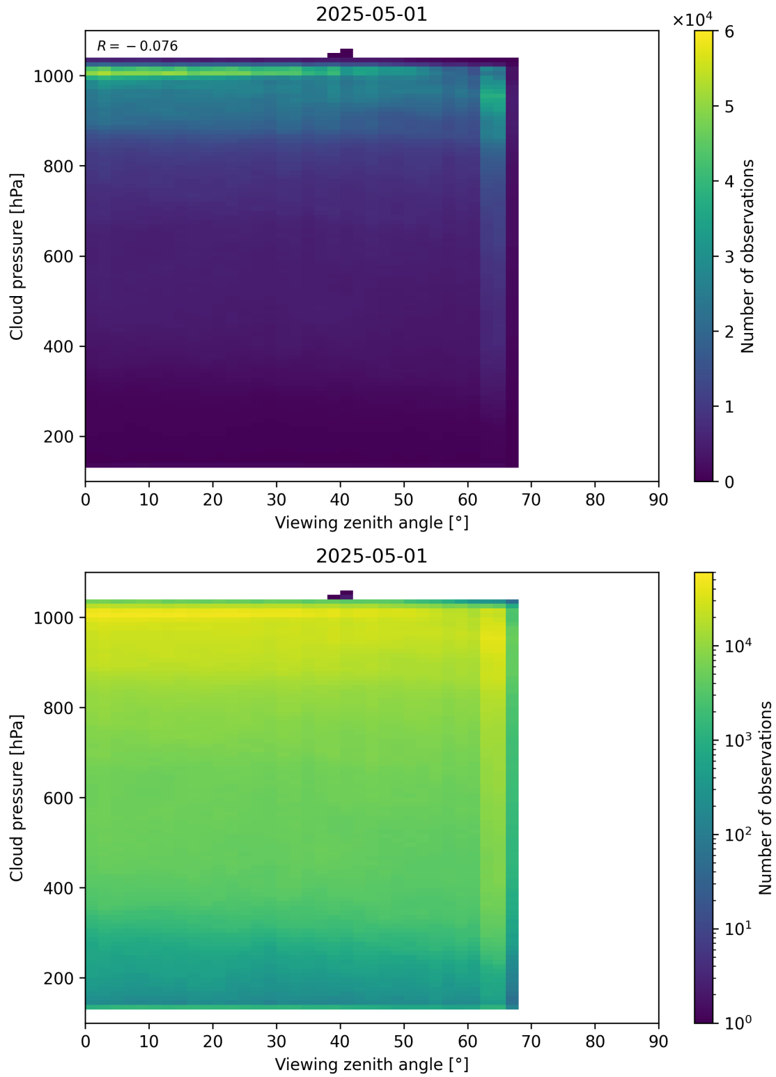
Figure 121: Scatter density plot of “Viewing zenith angle” against “Cloud pressure” for 2025-04-30 to 2025-05-02.
