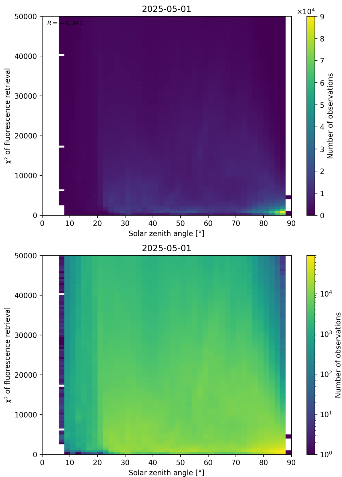
Figure 109: Scatter density plot of “Solar zenith angle” against “ \chi^2 of fluorescence retrieval” for 2025-04-30 to 2025-05-02.
