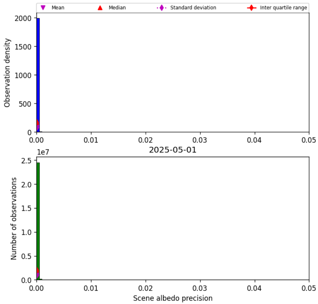
Figure 35: Histogram of “Scene albedo precision” for 2025-04-30 to 2025-05-02
