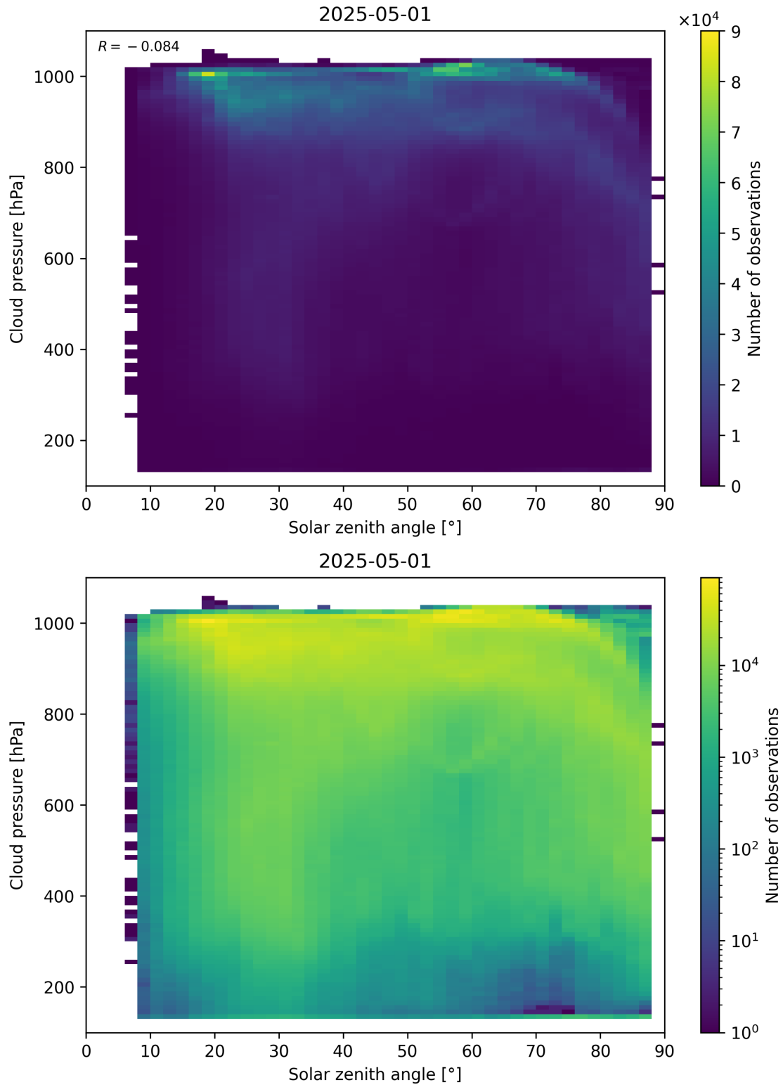
Figure 111: Scatter density plot of “Solar zenith angle” against “Cloud pressure” for 2025-04-30 to 2025-05-02.
