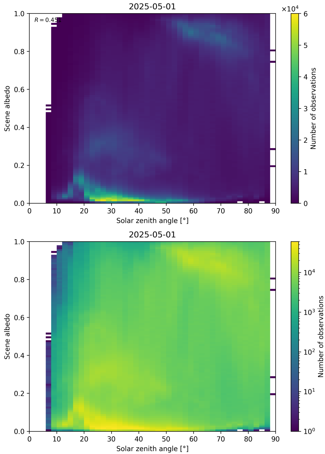
Figure 116: Scatter density plot of “Solar zenith angle” against “Scene albedo” for 2025-04-30 to 2025-05-02.
