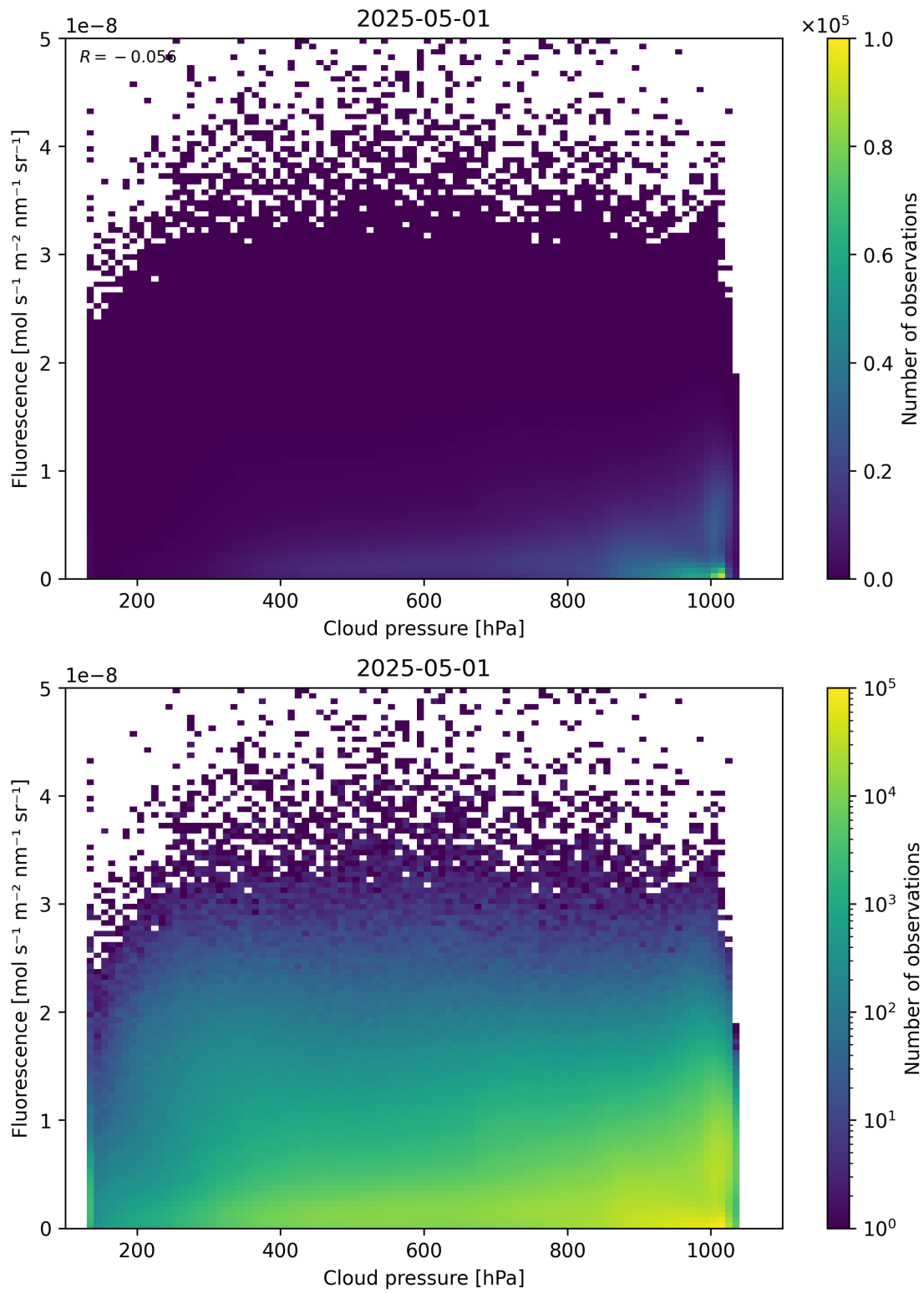
Figure 80: Scatter density plot of “Cloud pressure” against “Fluorescence” for 2025-04-30 to 2025-05-02.
