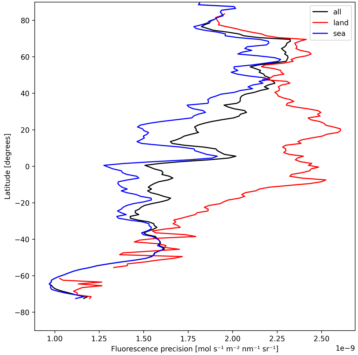
Figure 24: Zonal average of “Fluorescence precision” for 2025-04-30 to 2025-05-02.
