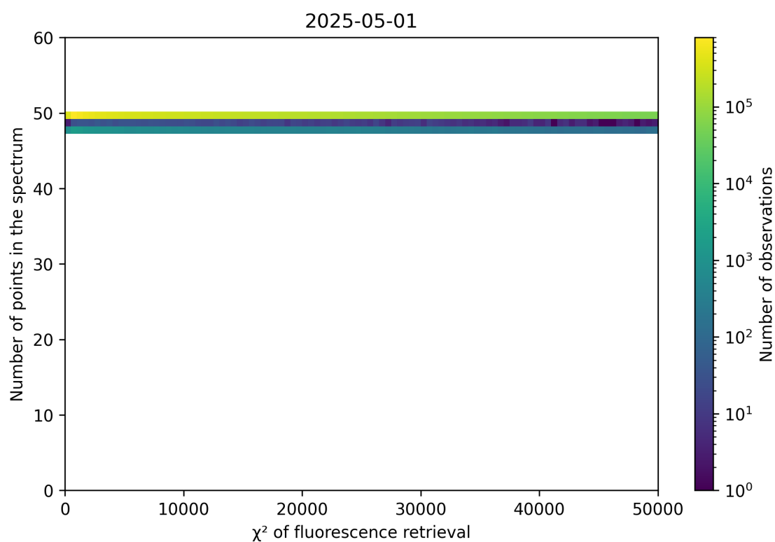
Figure 68: Scatter density plot of “ \chi^2 of fluorescence retrieval” against “Number of points in the spectrum” for 2025-04-30 to 2025-05-02.
