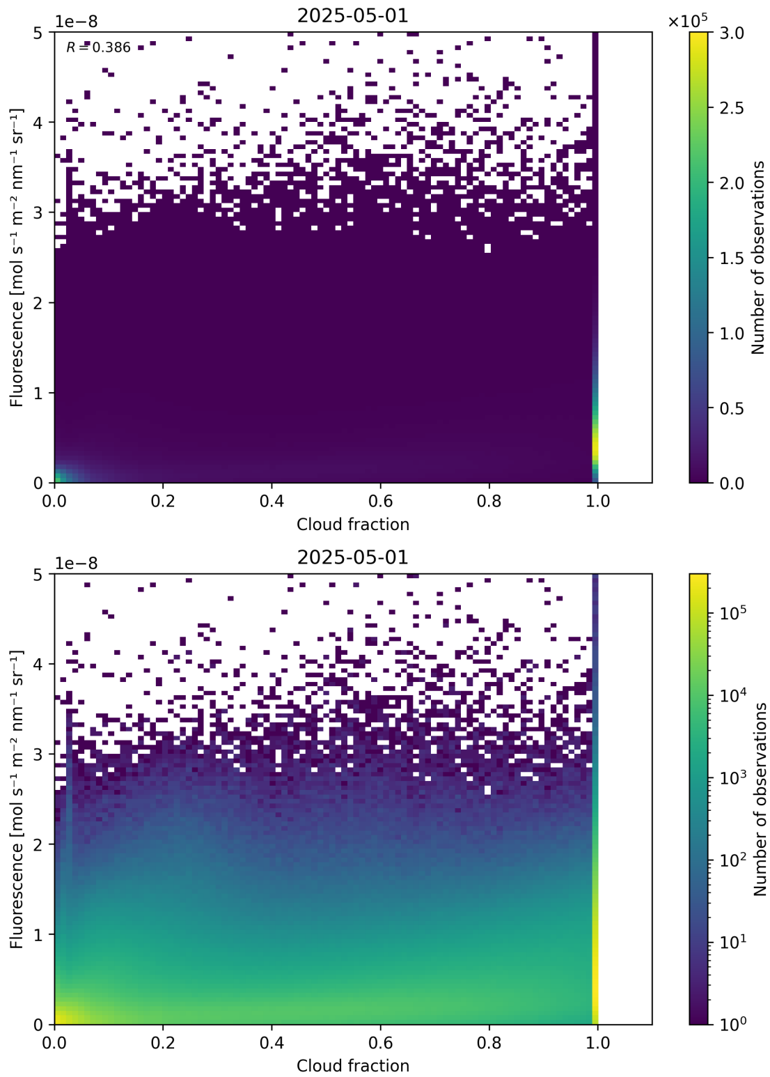
Figure 72: Scatter density plot of “Cloud fraction” against “Fluorescence” for 2025-04-30 to 2025-05-02.
