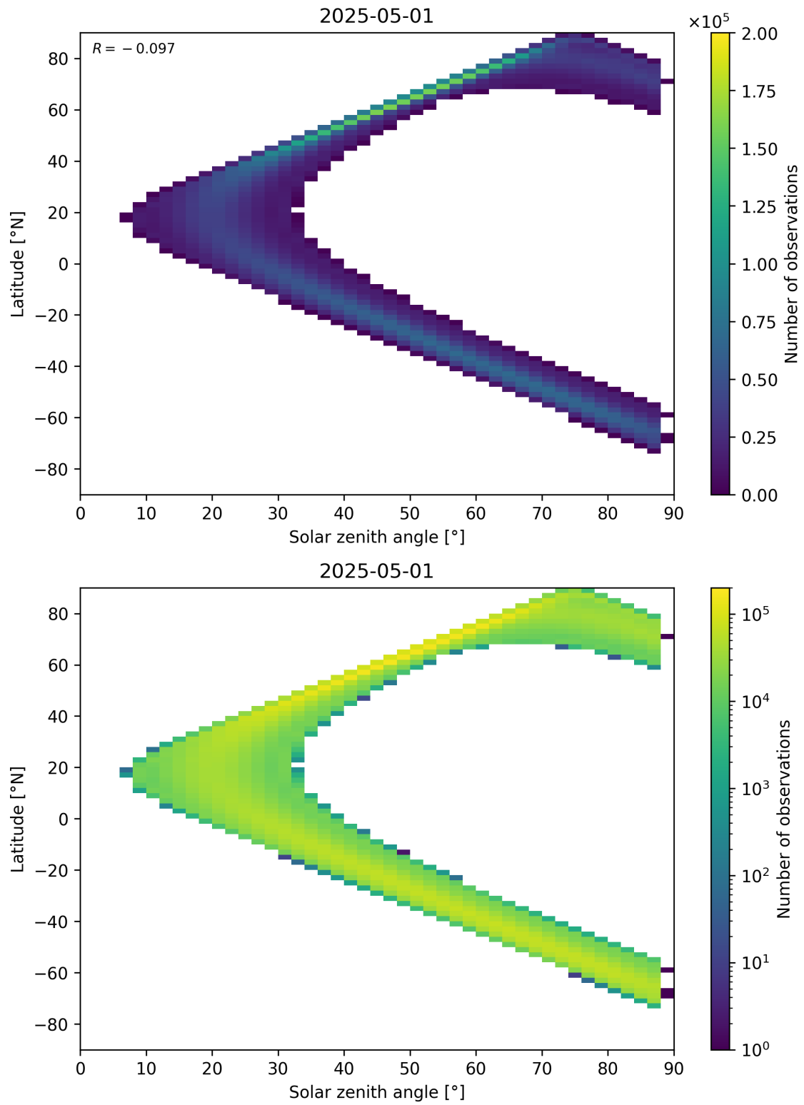
Figure 113: Scatter density plot of “Solar zenith angle” against “Latitude” for 2025-04-30 to 2025-05-02.
