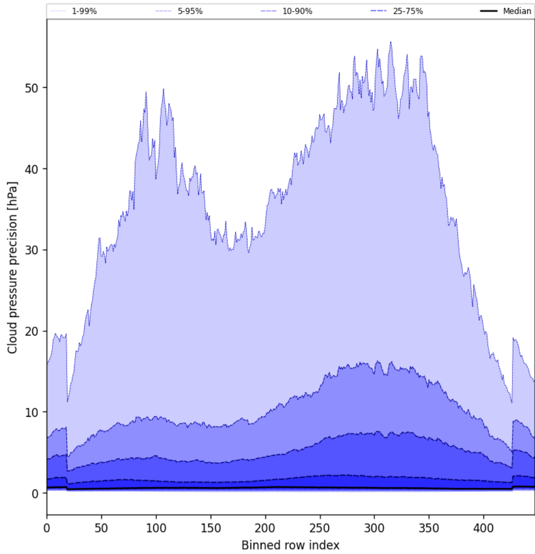
Figure 48: Along track statistics of “Cloud pressure precision” for 2025-04-30 to 2025-05-02
