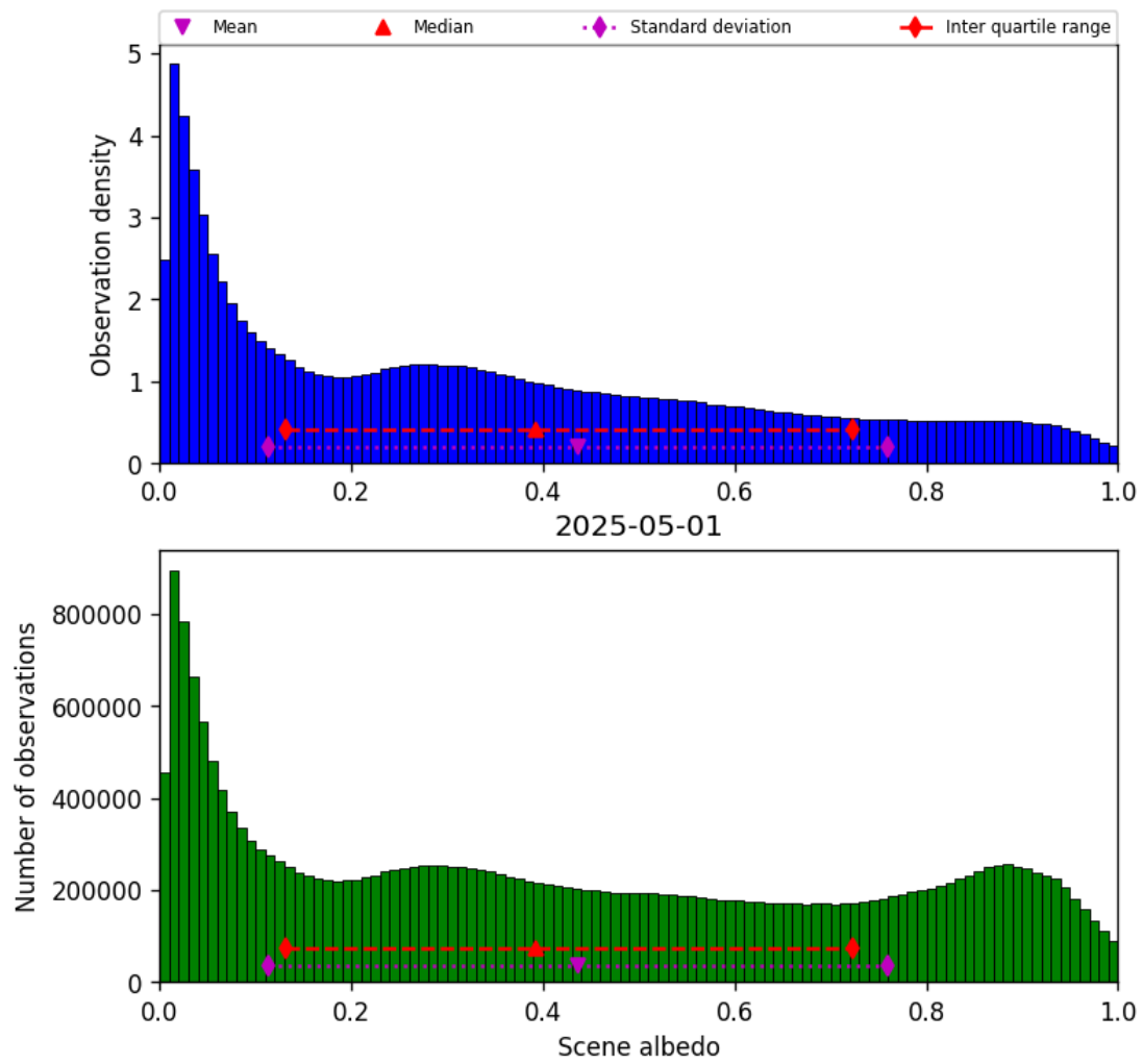
Figure 34: Histogram of “Scene albedo” for 2025-04-30 to 2025-05-02
