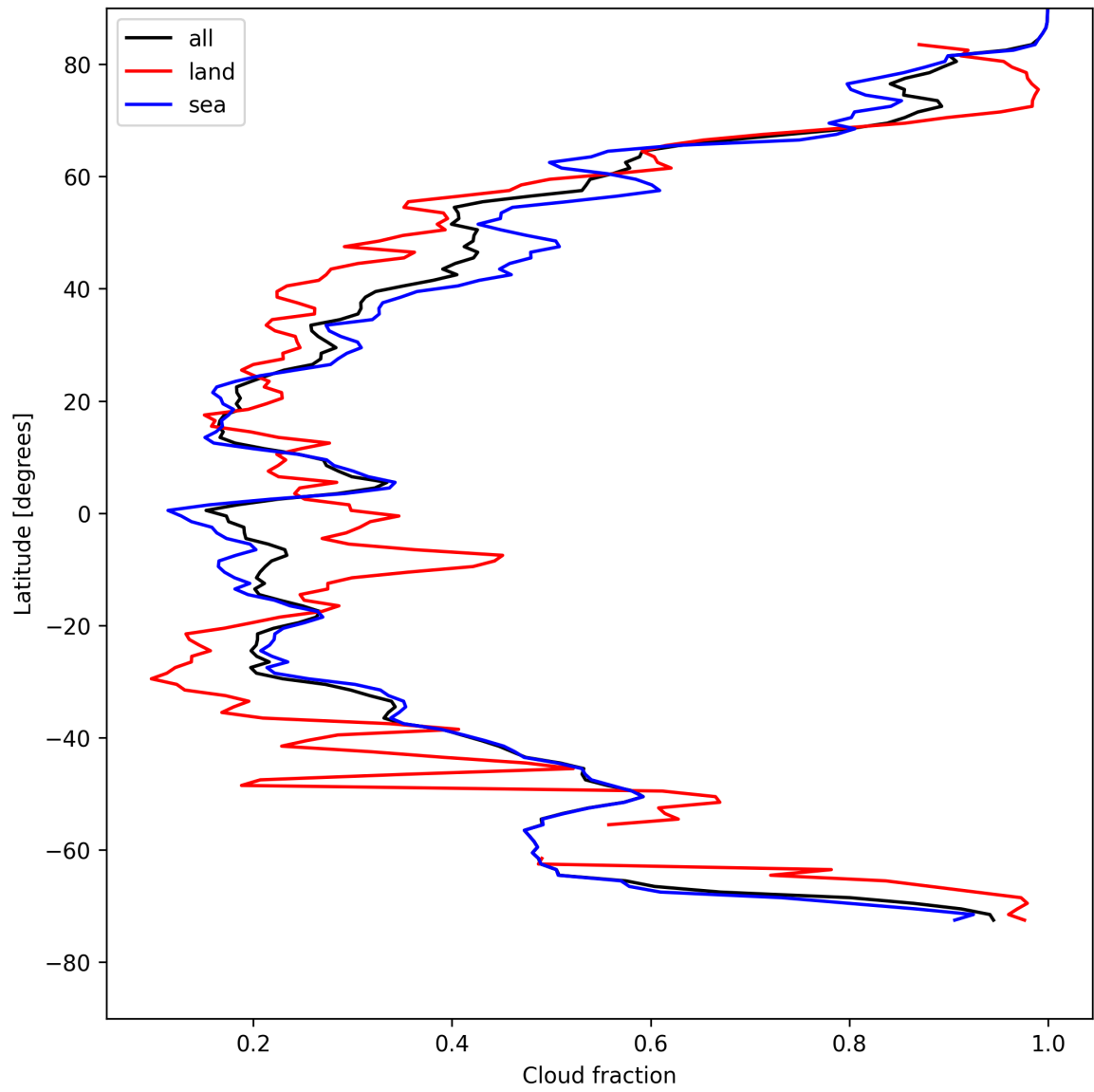
Figure 15: Zonal average of “Cloud fraction” for 2025-04-30 to 2025-05-02.
