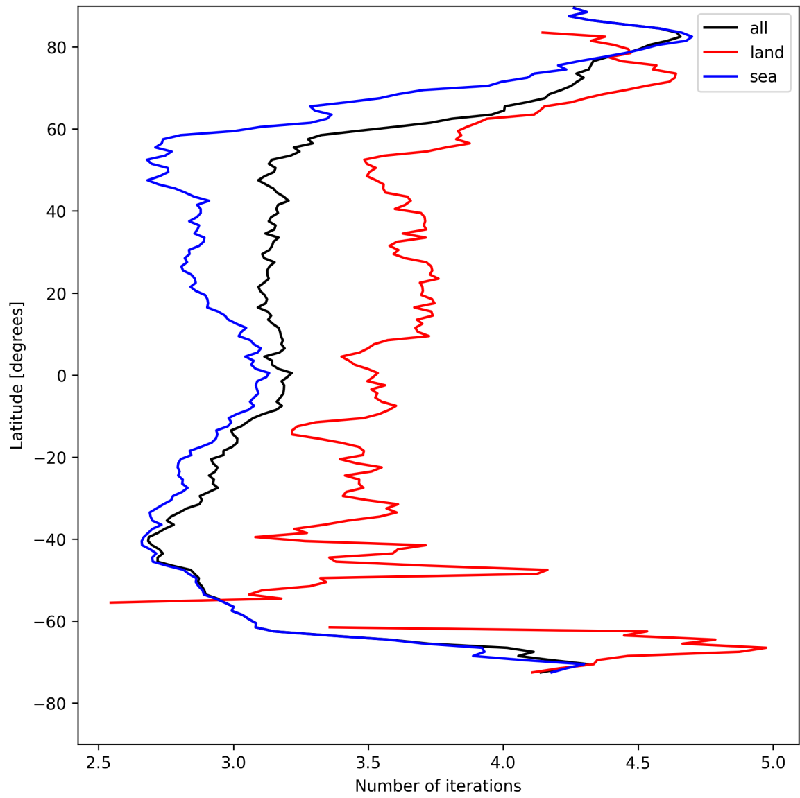
Figure 22: Zonal average of “Number of iterations” for 2025-04-30 to 2025-05-02.
