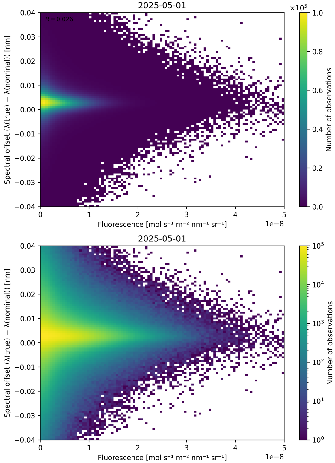
Figure 87: Scatter density plot of “Fluorescence” against “Spectral offset ( \lambda_{\text{true}} - \lambda_{\text{nominal}} )” for 2025-04-30 to 2025-05-02.
