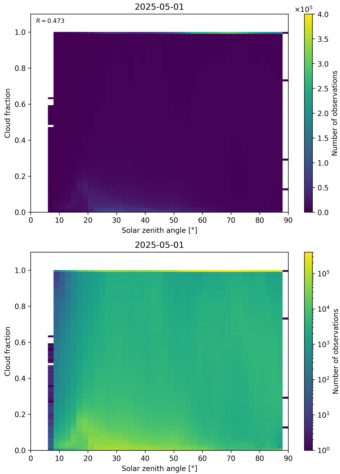
Figure 110: Scatter density plot of “Solar zenith angle” against “Cloud fraction” for 2025-04-30 to 2025-05-02.
