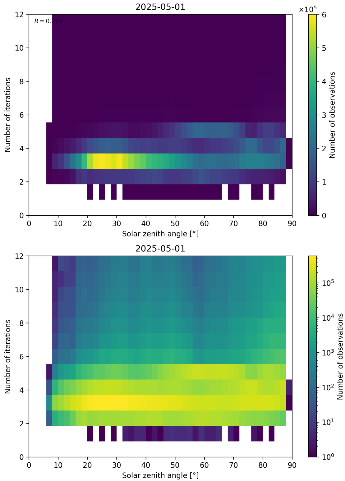
Figure 114: Scatter density plot of “Solar zenith angle” against “Number of iterations” for 2025-04-30 to 2025-05-02.
