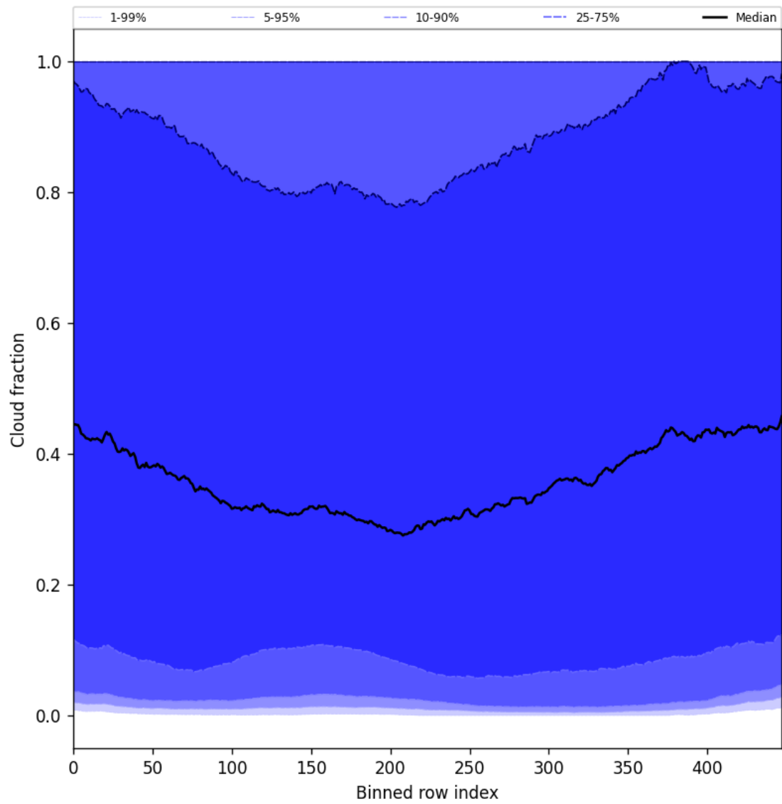
Figure 49: Along track statistics of “Cloud fraction” for 2025-04-30 to 2025-05-02
