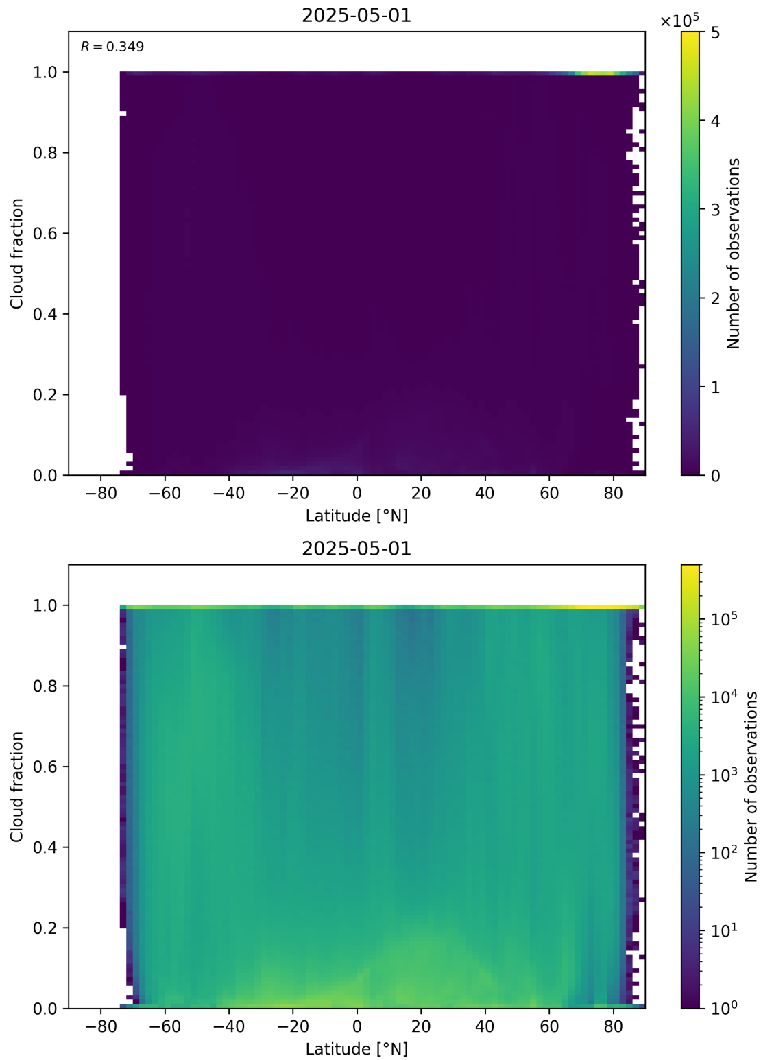
Figure 90: Scatter density plot of “Latitude” against “Cloud fraction” for 2025-04-30 to 2025-05-02.
