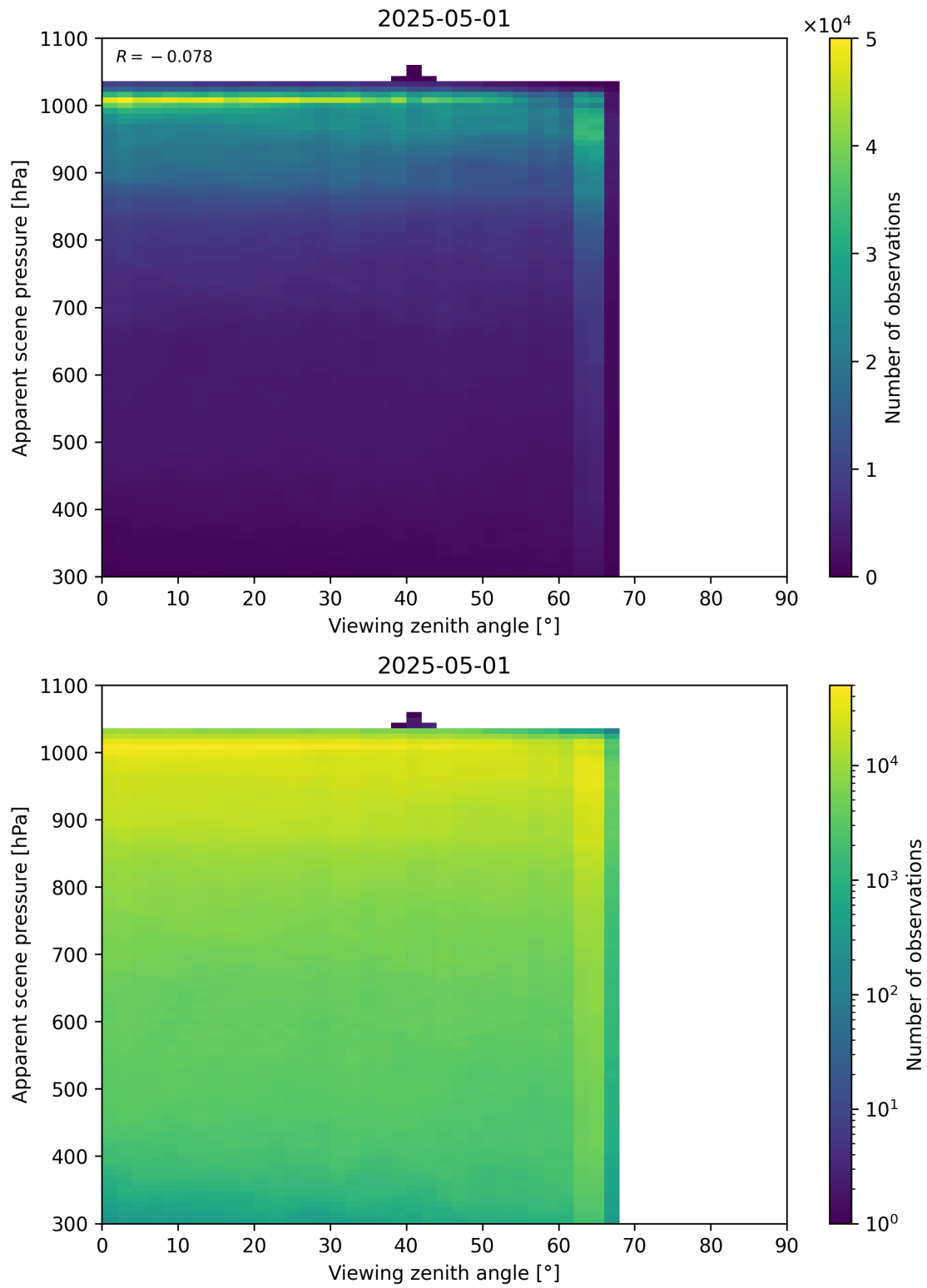
Figure 118: Scatter density plot of “Viewing zenith angle” against “Apparent scene pressure” for 2025-04-30 to 2025-05-02.
