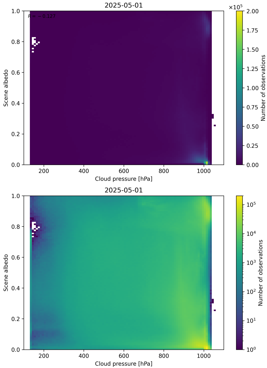
Figure 83: Scatter density plot of “Cloud pressure” against “Scene albedo” for 2025-04-30 to 2025-05-02.
