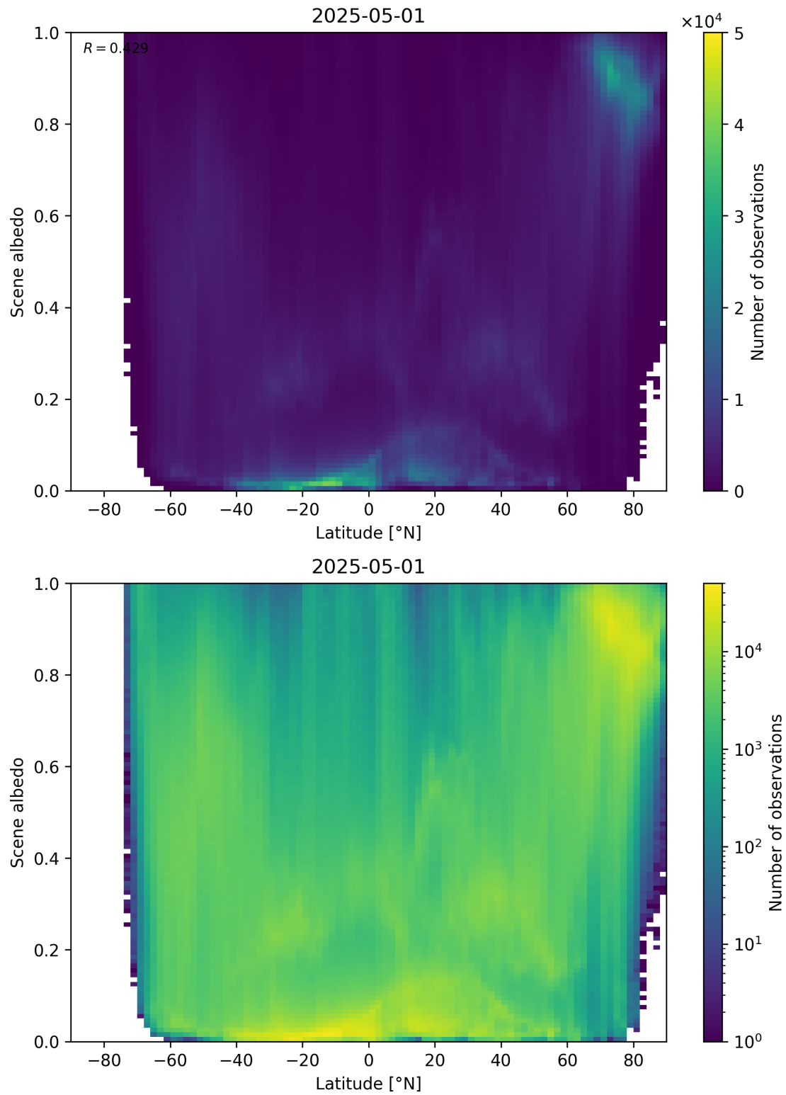
Figure 95: Scatter density plot of “Latitude” against “Scene albedo” for 2025-04-30 to 2025-05-02.
