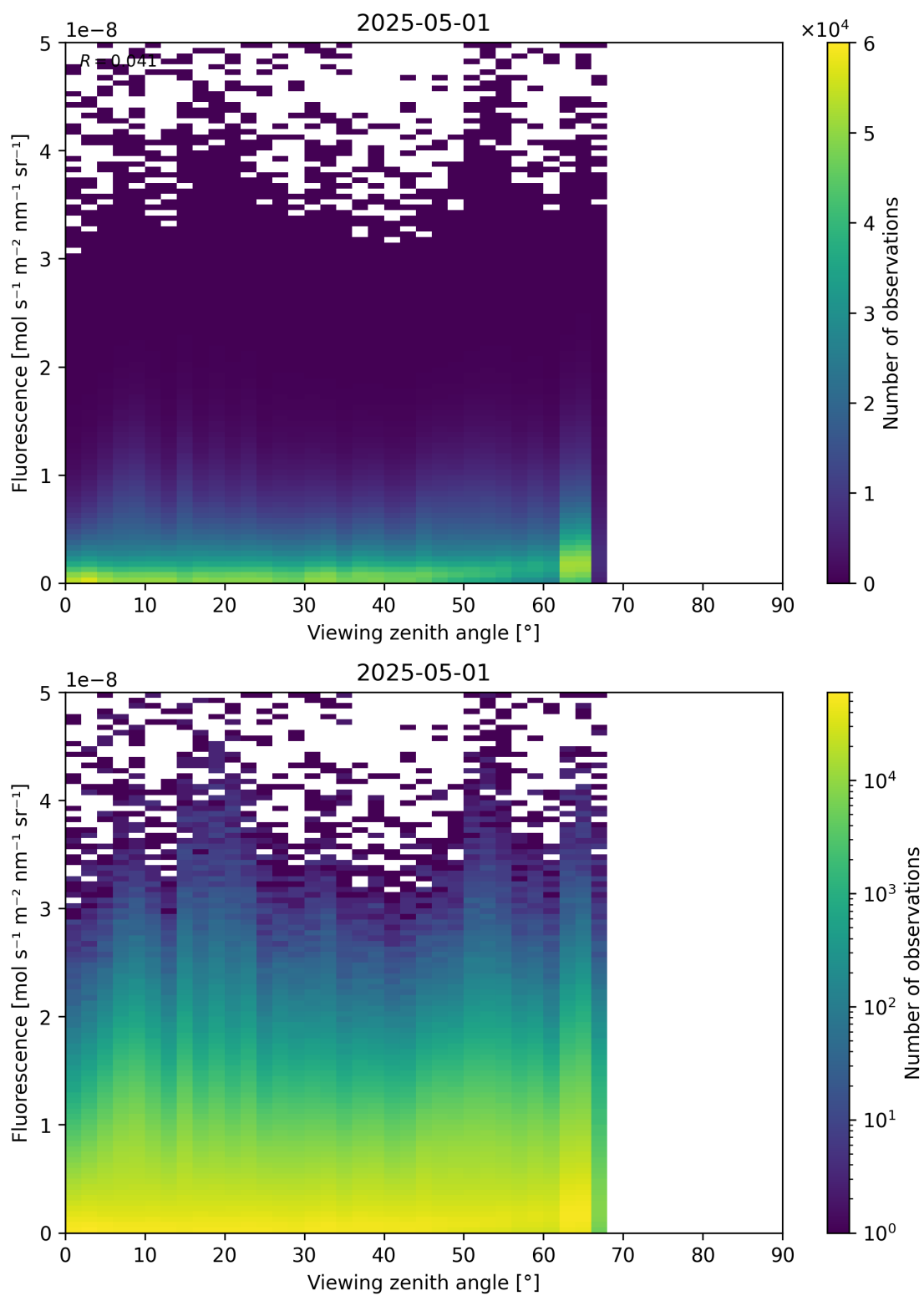
Figure 122: Scatter density plot of “Viewing zenith angle” against “Fluorescence” for 2025-04-30 to 2025-05-02.
