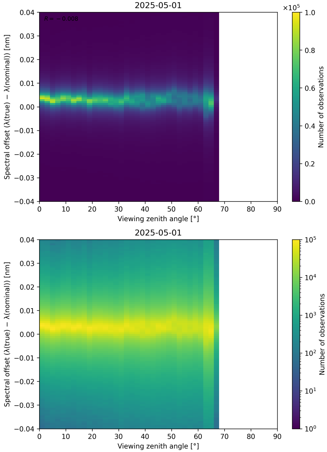
Figure 128: Scatter density plot of “Viewing zenith angle” against “Spectral offset ( \lambda_{\text{true}} - \lambda_{\text{nominal}} )” for 2025-04-30 to 2025-05-02.
