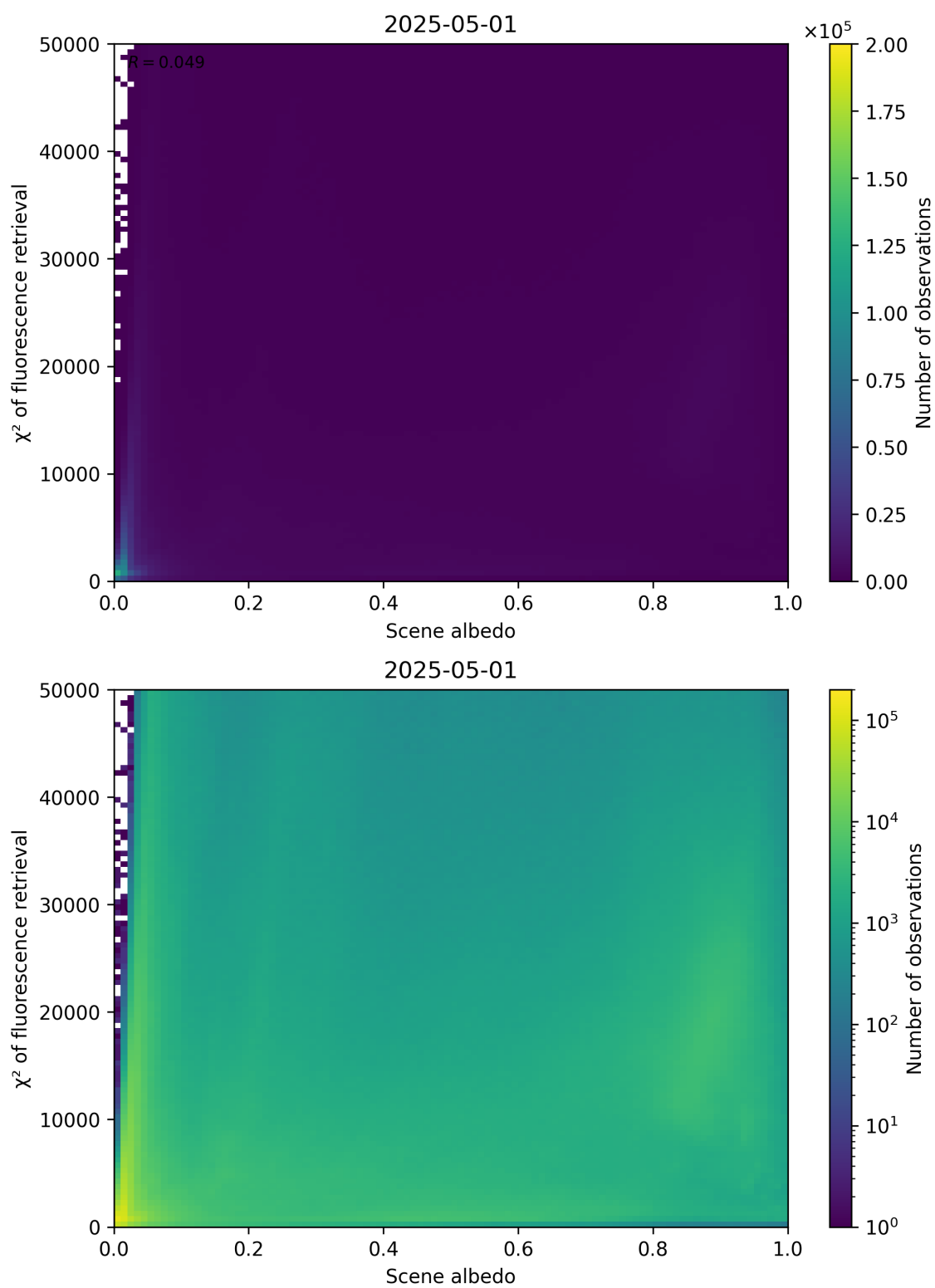
Figure 103: Scatter density plot of “Scene albedo” against “ \chi^2 of fluorescence retrieval” for 2025-04-30 to 2025-05-02.
