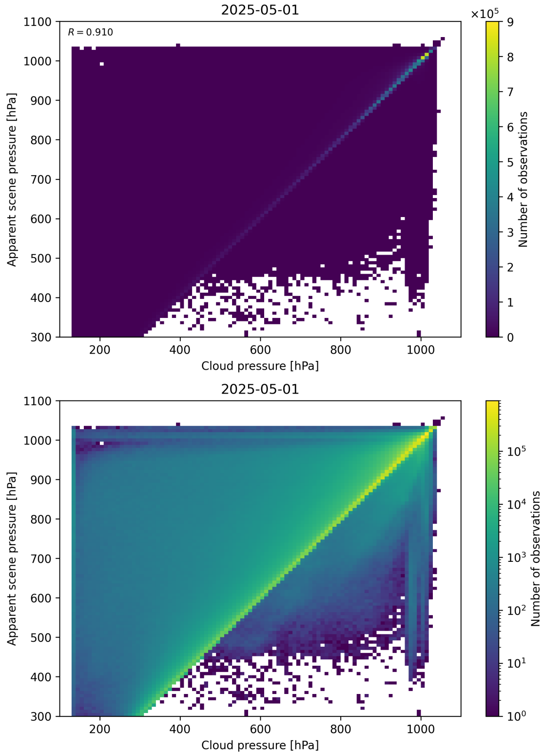
Figure 77: Scatter density plot of “Cloud pressure” against “Apparent scene pressure” for 2025-04-30 to 2025-05-02.
