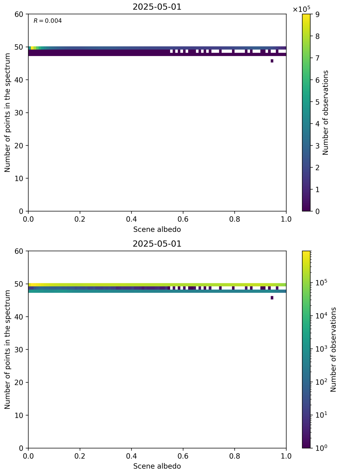
Figure 106: Scatter density plot of “Scene albedo” against “Number of points in the spectrum” for 2025-04-30 to 2025-05-02.
