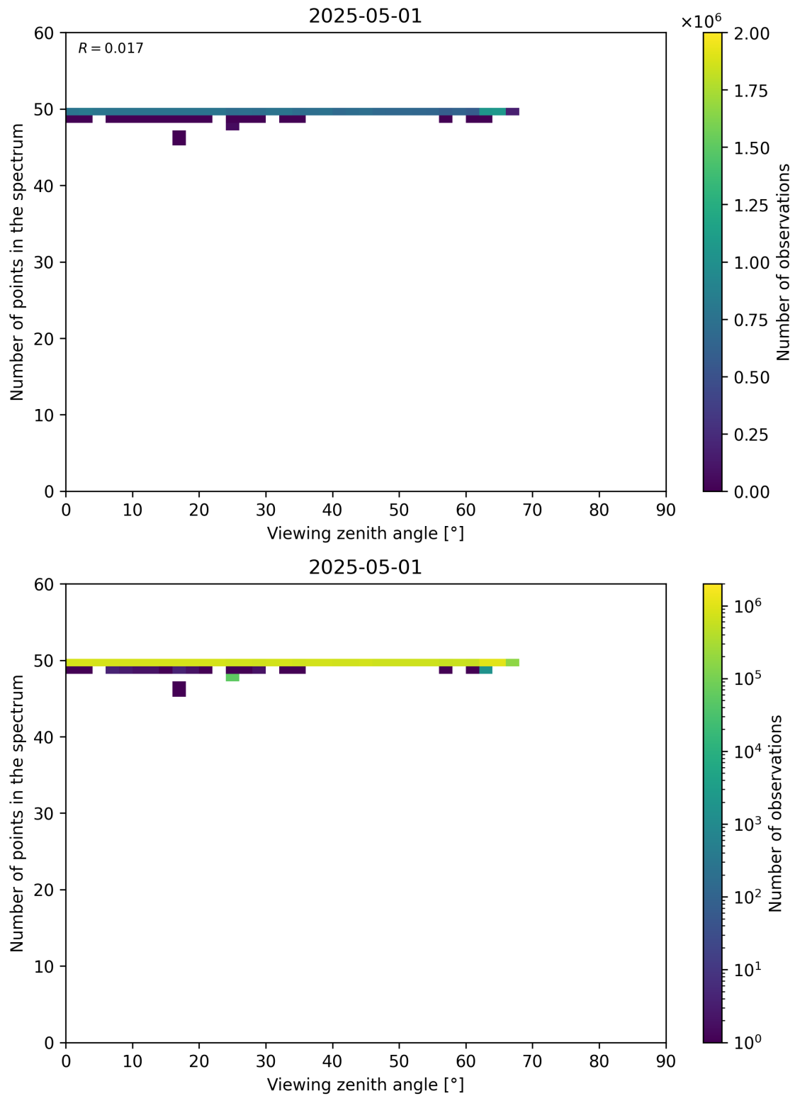
Figure 125: Scatter density plot of “Viewing zenith angle” against “Number of points in the spectrum” for 2025-04-30 to 2025-05-02.
