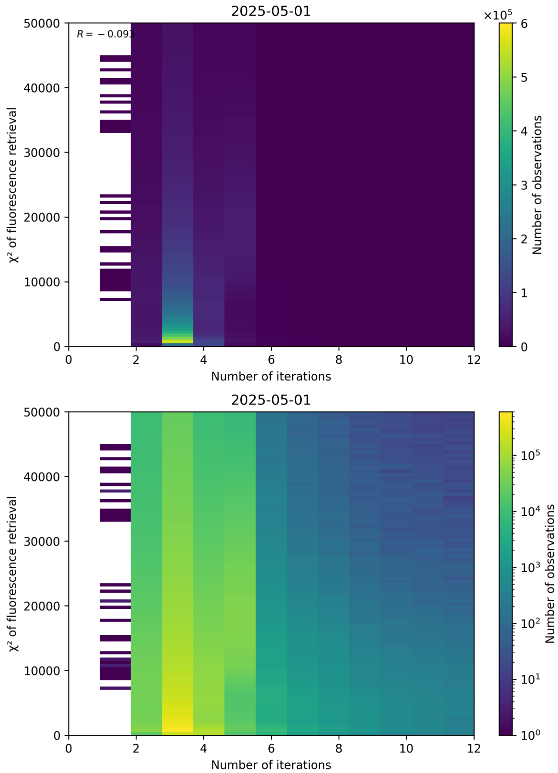
Figure 97: Scatter density plot of “Number of iterations” against “ \chi^2 of fluorescence retrieval” for 2025-04-30 to 2025-05-02.
