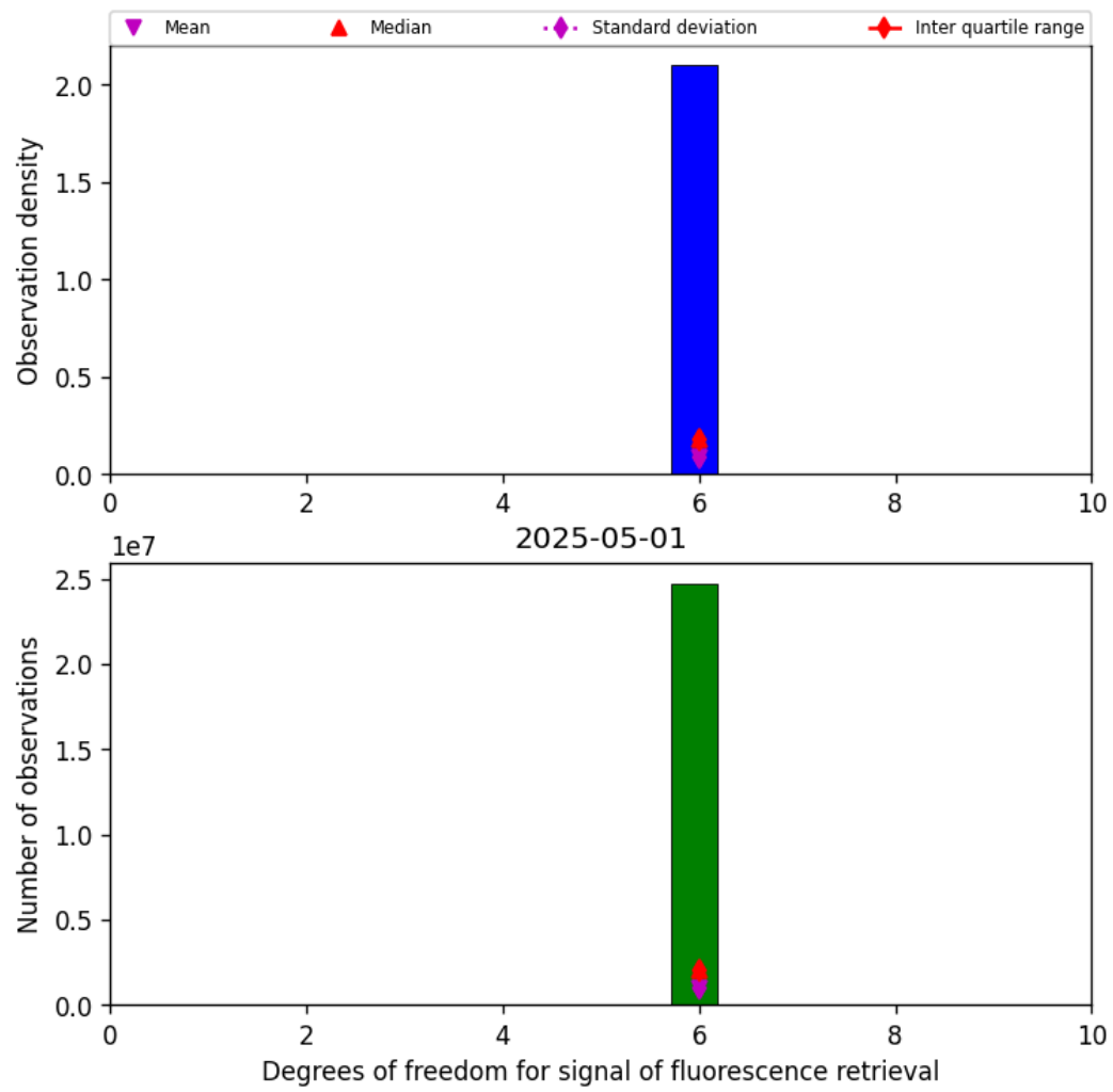
Figure 43: Histogram of “Degrees of freedom for signal of fluorescence retrieval” for 2025-04-30 to 2025-05-02
