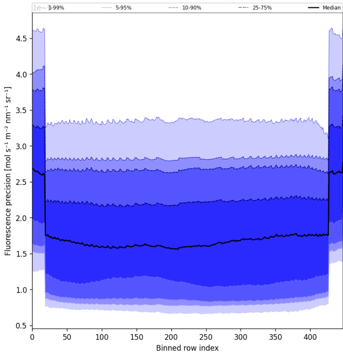
Figure 58: Along track statistics of “Fluorescence precision” for 2025-04-30 to 2025-05-02
