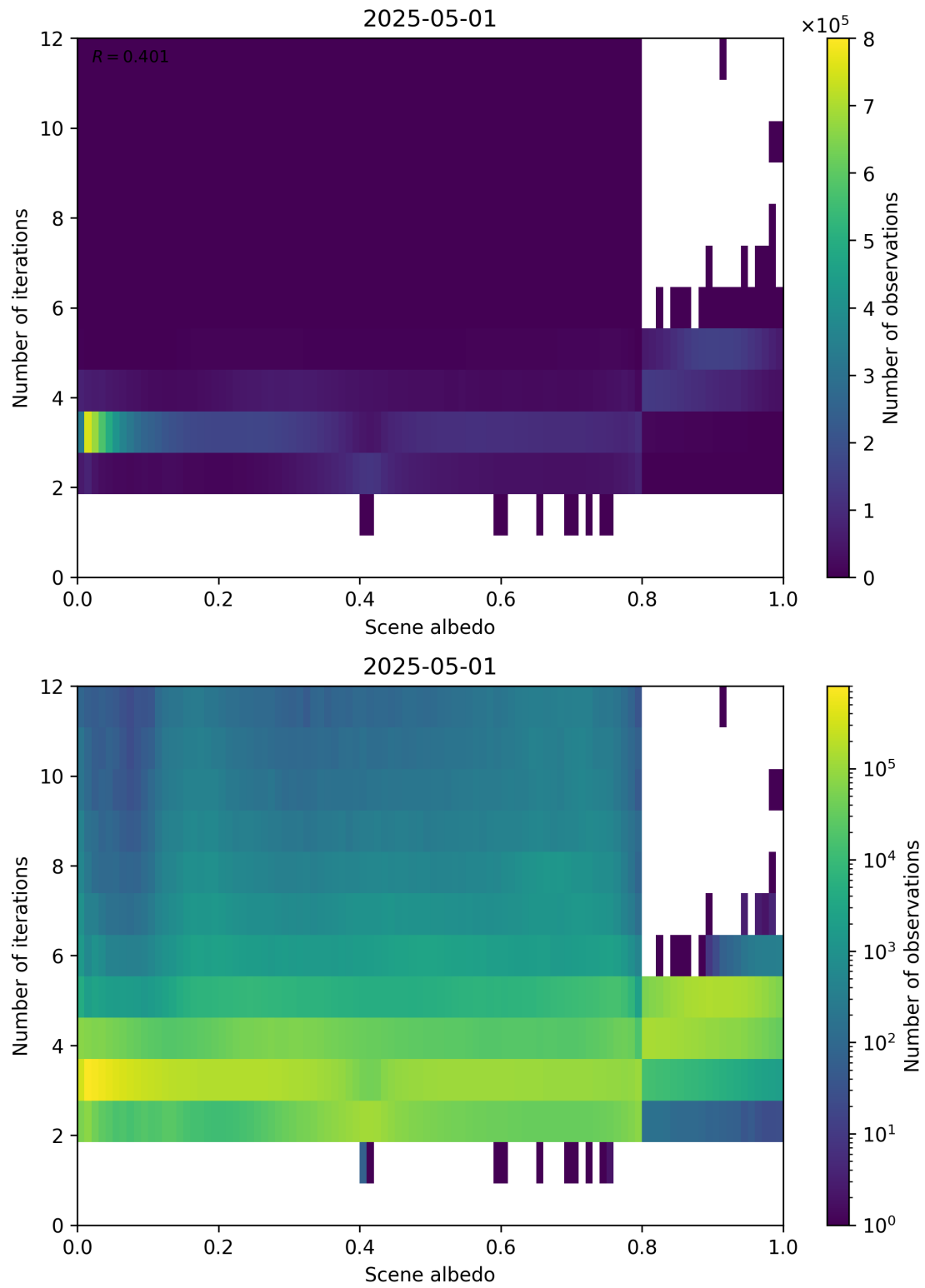
Figure 105: Scatter density plot of “Scene albedo” against “Number of iterations” for 2025-04-30 to 2025-05-02.
