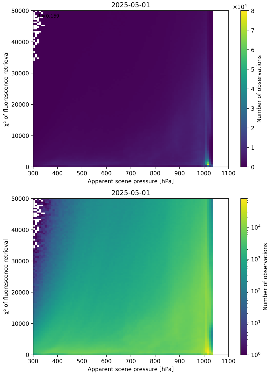
Figure 63: Scatter density plot of “Apparent scene pressure” against “ \chi^2 of fluorescence retrieval” for 2025-04-30 to 2025-05-02.
