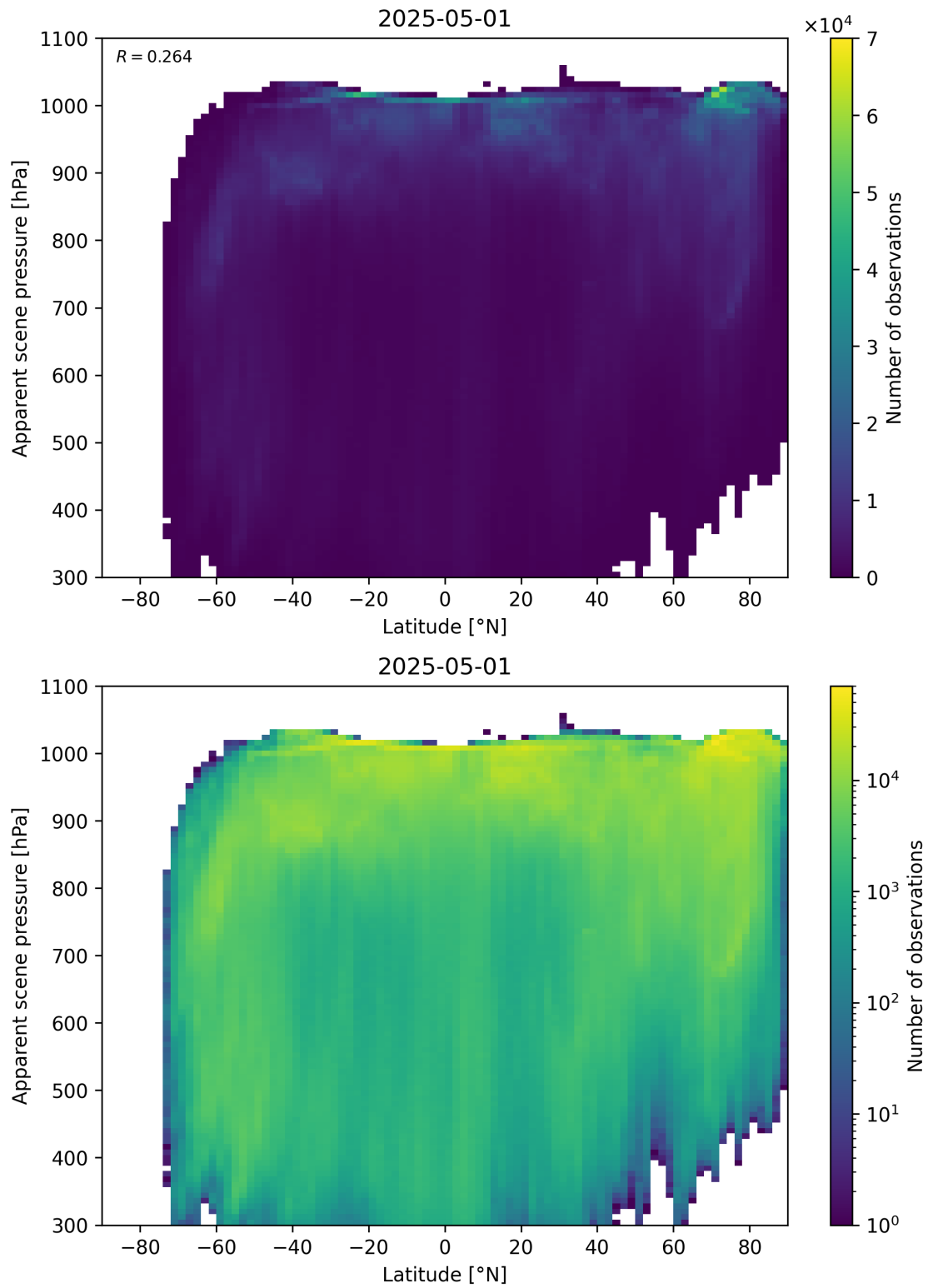
Figure 88: Scatter density plot of “Latitude” against “Apparent scene pressure” for 2025-04-30 to 2025-05-02.
