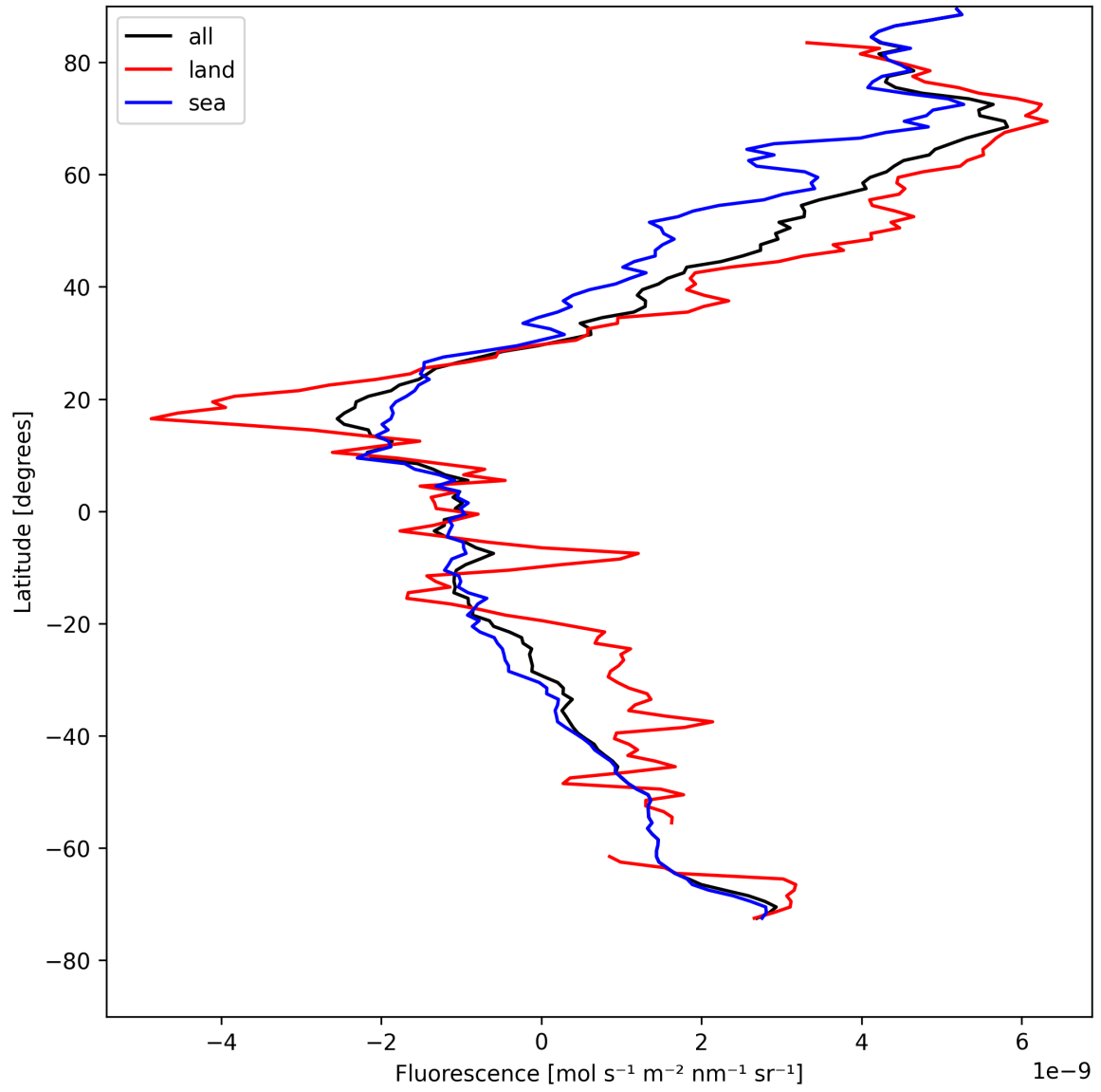
Figure 23: Zonal average of “Fluorescence” for 2025-04-30 to 2025-05-02.
