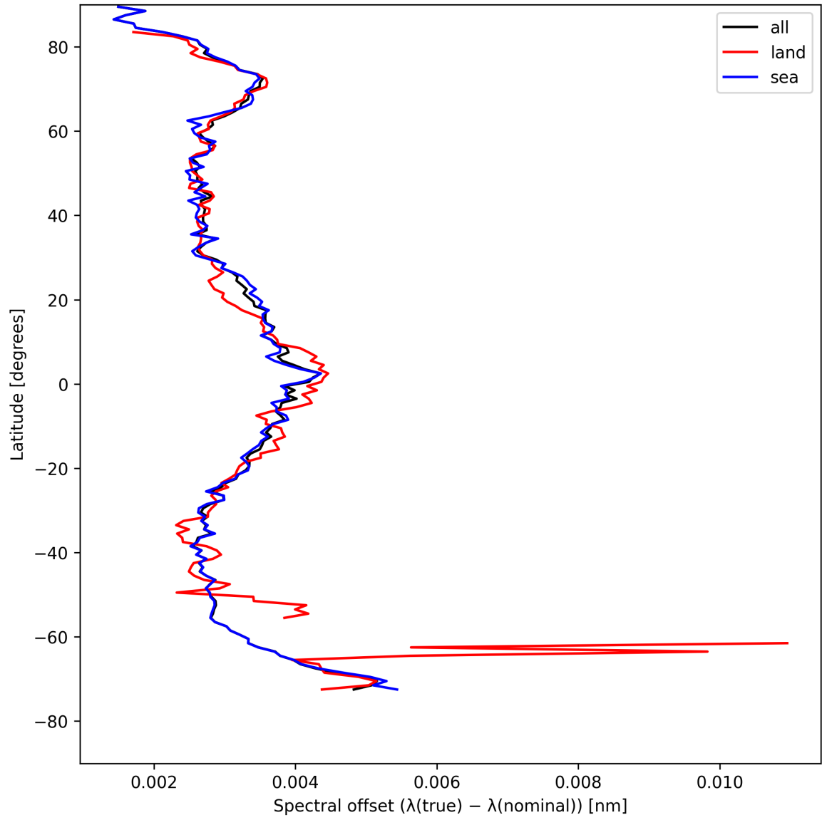
Figure 28: Zonal average of “Spectral offset ( \lambda_{\text{true}} - \lambda_{\text{nominal}} )” for 2025-04-30 to 2025-05-02.
