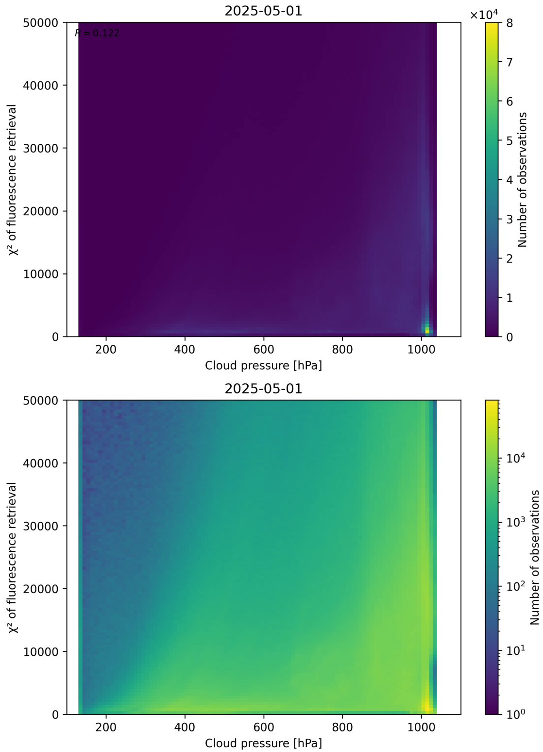
Figure 78: Scatter density plot of “Cloud pressure” against “ \chi^2 of fluorescence retrieval” for 2025-04-30 to 2025-05-02.
