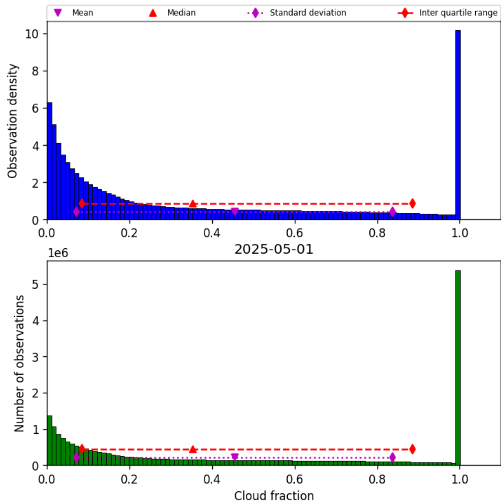
Figure 32: Histogram of “Cloud fraction” for 2025-04-30 to 2025-05-02
