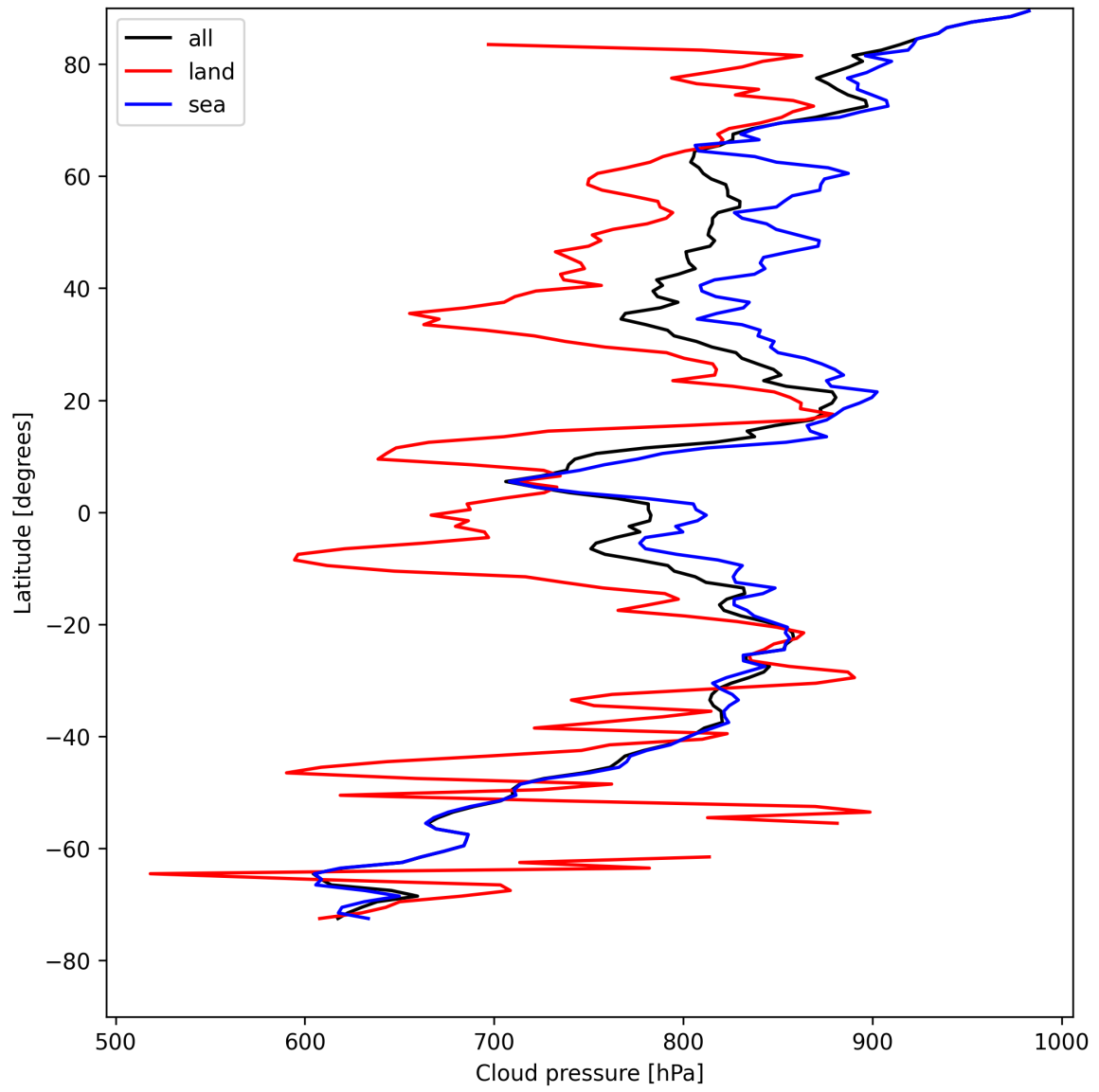
Figure 13: Zonal average of “Cloud pressure” for 2025-04-30 to 2025-05-02.
