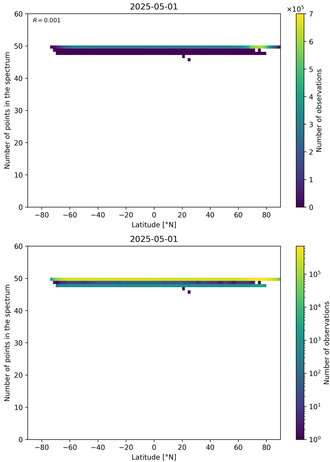
Figure 94: Scatter density plot of “Latitude” against “Number of points in the spectrum” for 2025-04-30 to 2025-05-02.
