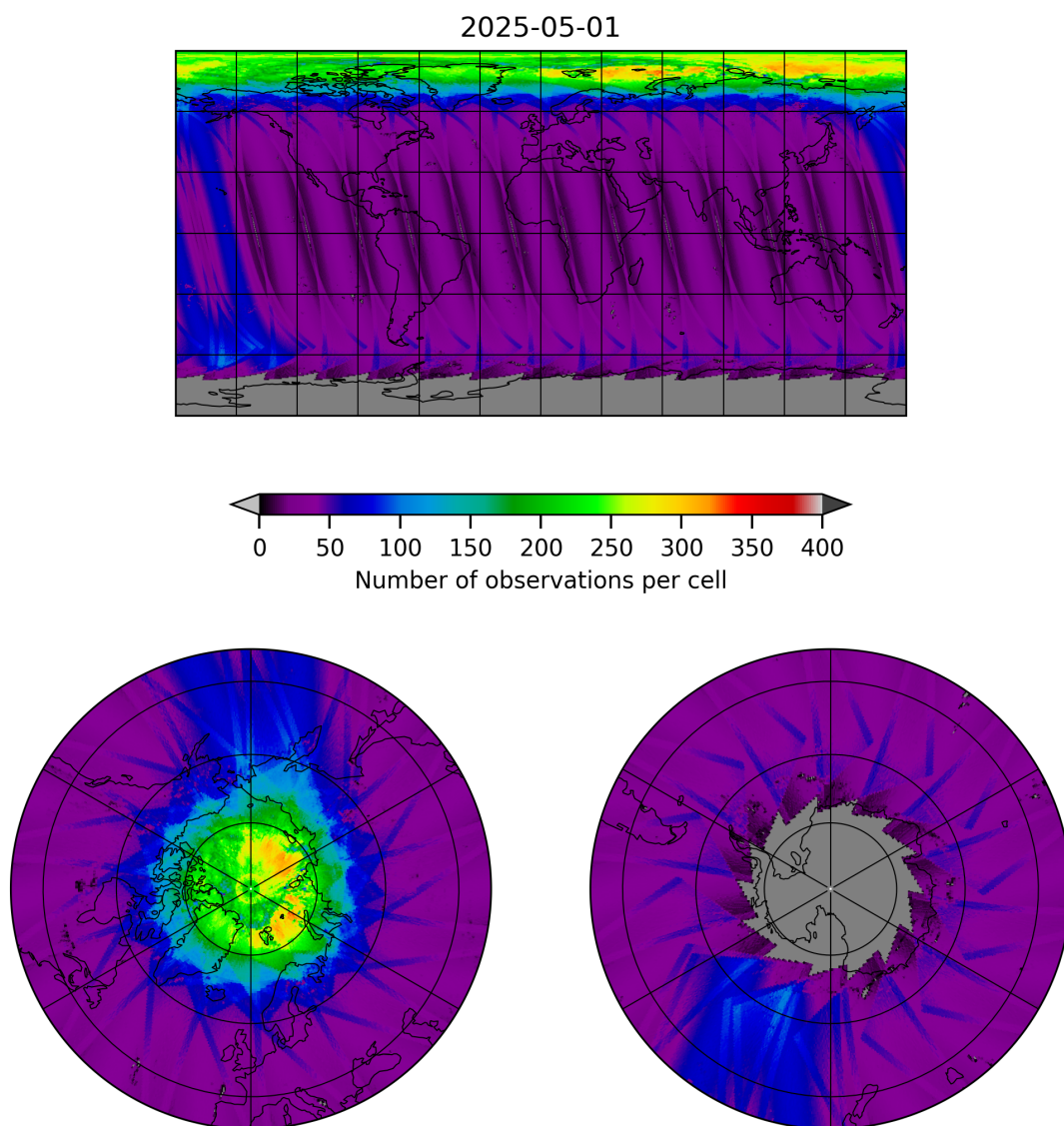
Figure 11: Map of the number of observations for 2025-04-30 to 2025-05-02
