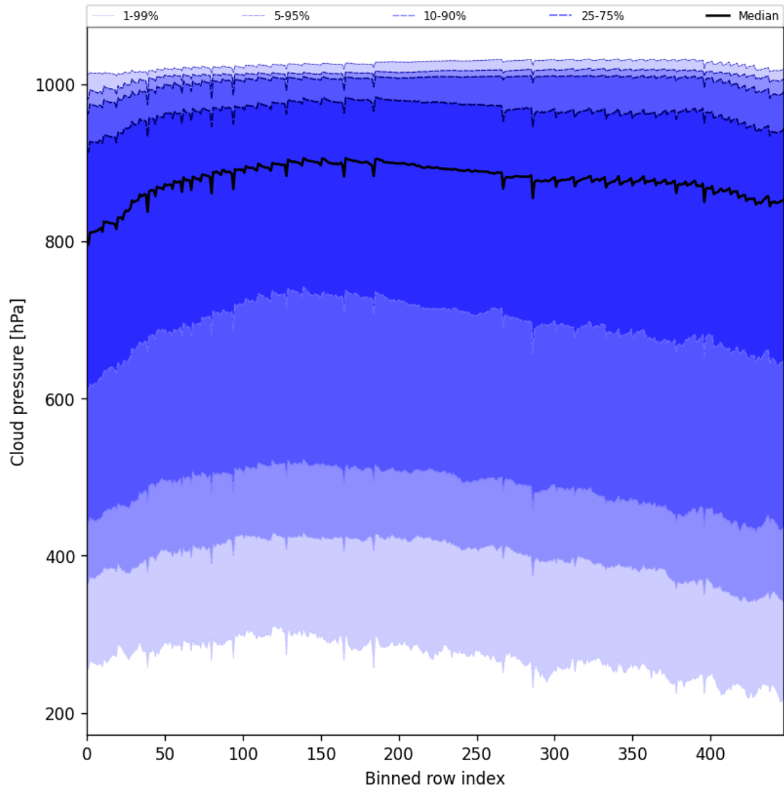
Figure 47: Along track statistics of “Cloud pressure” for 2025-04-30 to 2025-05-02
