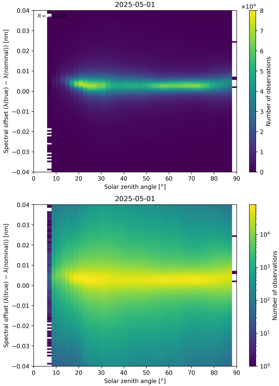
Figure 117: Scatter density plot of “Solar zenith angle” against “Spectral offset ( \lambda_{\text{true}} - \lambda_{\text{nominal}} )” for 2025-04-30 to 2025-05-02.
