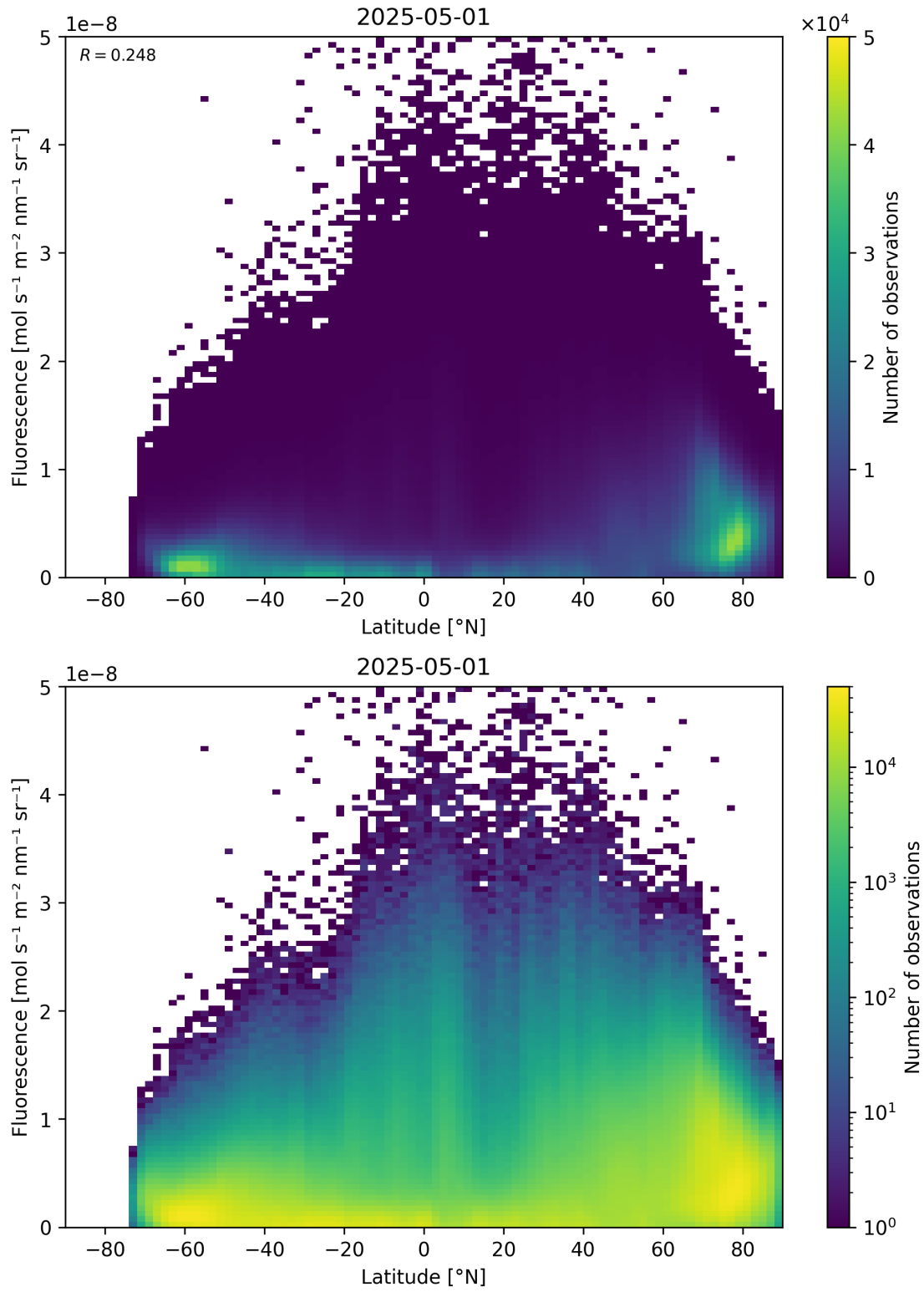
Figure 92: Scatter density plot of “Latitude” against “Fluorescence” for 2025-04-30 to 2025-05-02.
