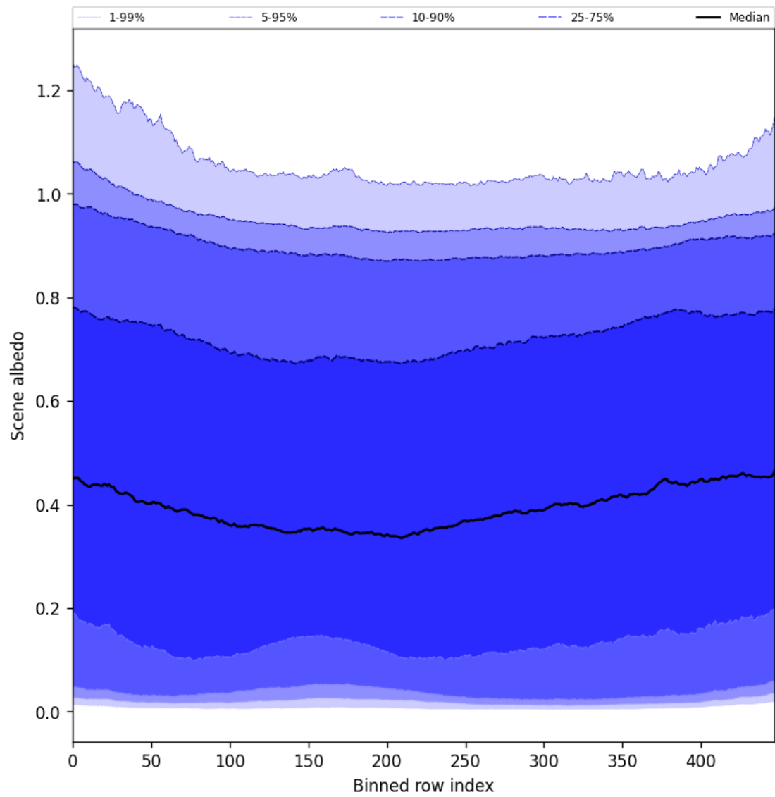
Figure 51: Along track statistics of “Scene albedo” for 2025-04-30 to 2025-05-02
