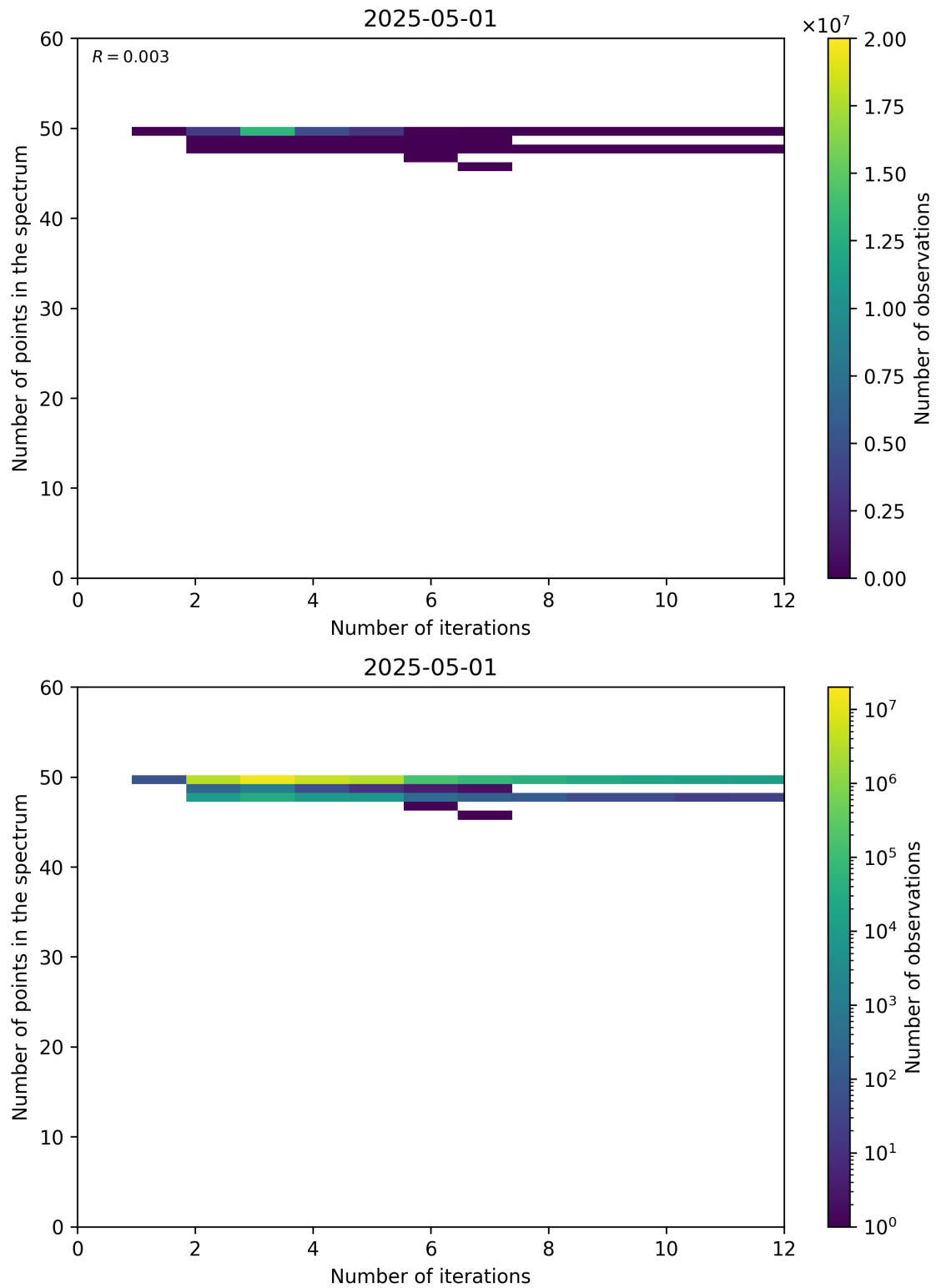
Figure 99: Scatter density plot of “Number of iterations” against “Number of points in the spectrum” for 2025-04-30 to 2025-05-02.
