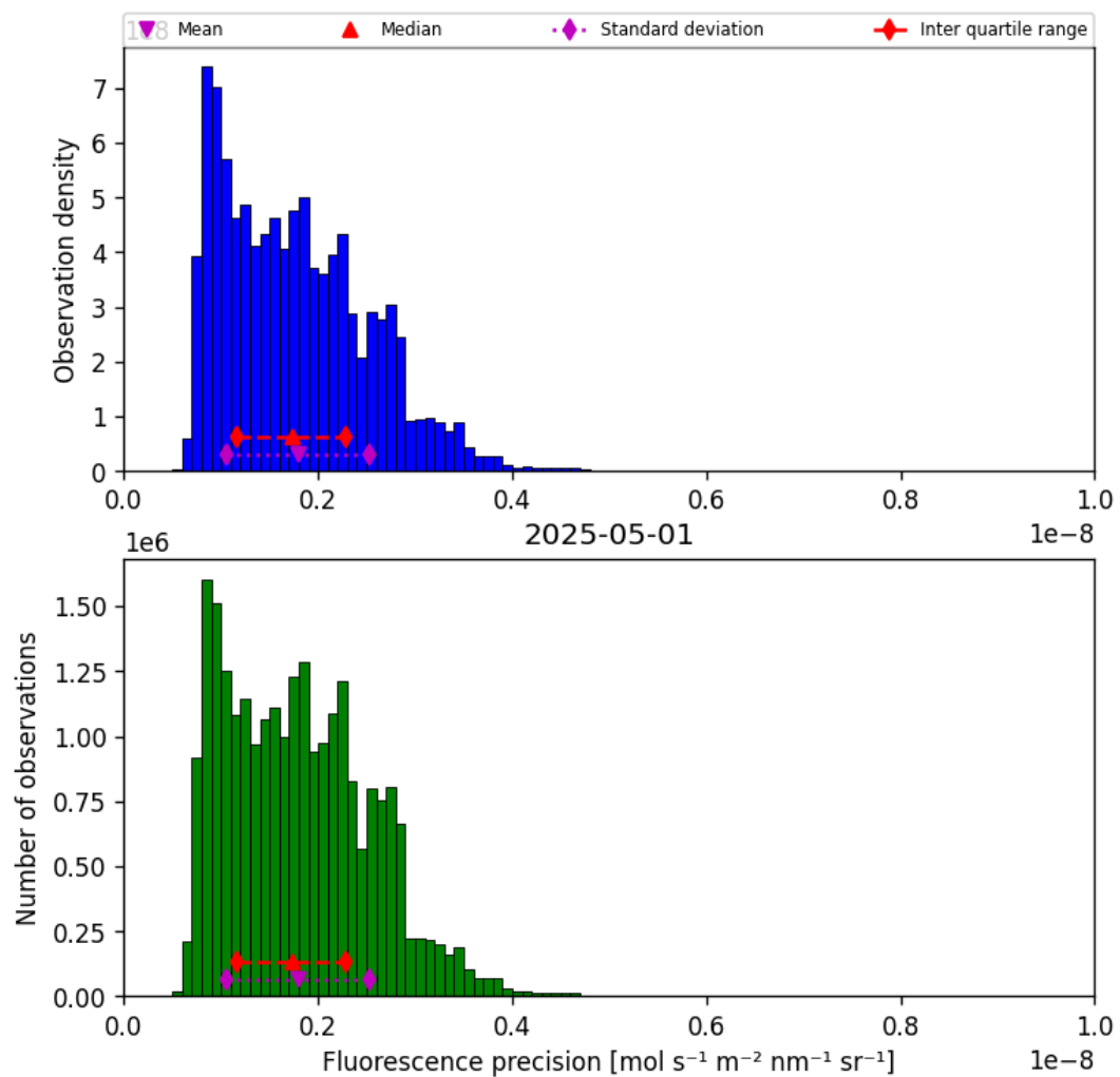
Figure 41: Histogram of “Fluorescence precision” for 2025-04-30 to 2025-05-02
