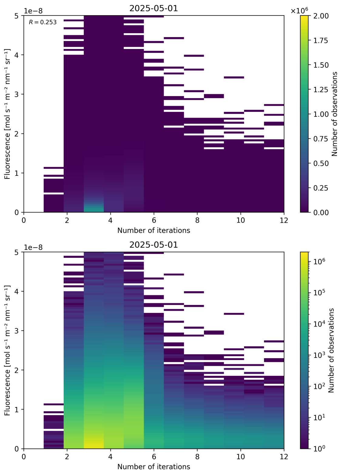
Figure 98: Scatter density plot of “Number of iterations” against “Fluorescence” for 2025-04-30 to 2025-05-02.
