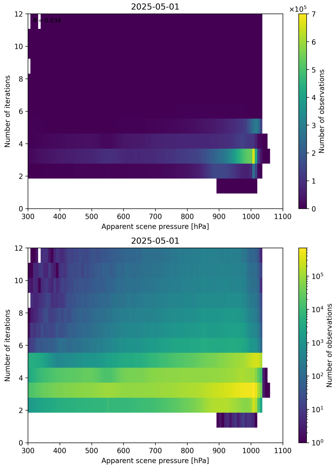
Figure 65: Scatter density plot of “Apparent scene pressure” against “Number of iterations” for 2025-04-30 to 2025-05-02.
