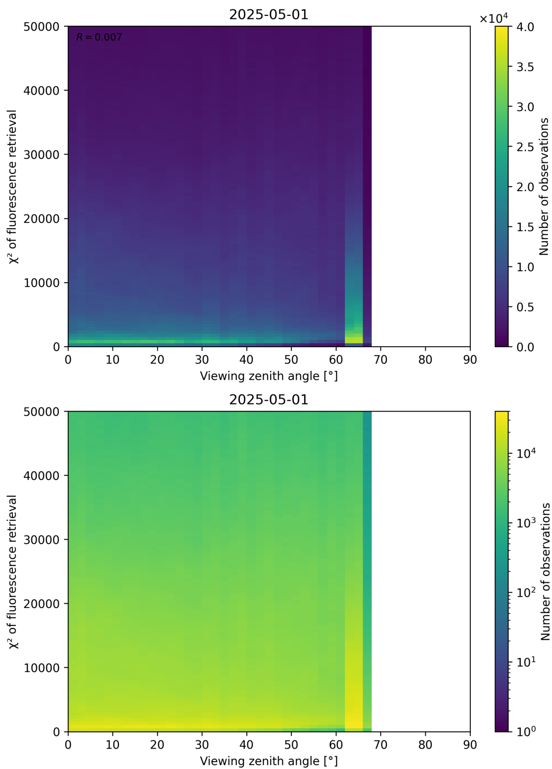
Figure 119: Scatter density plot of “Viewing zenith angle” against “ \chi^2 of fluorescence retrieval” for 2025-04-30 to 2025-05-02.
