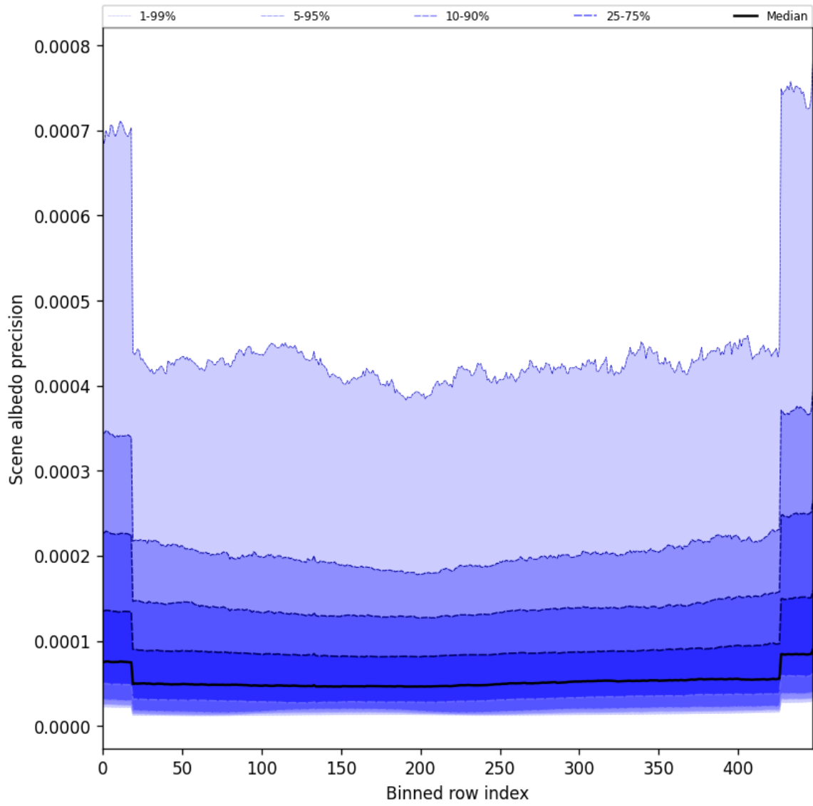
Figure 52: Along track statistics of “Scene albedo precision” for 2025-04-30 to 2025-05-02
