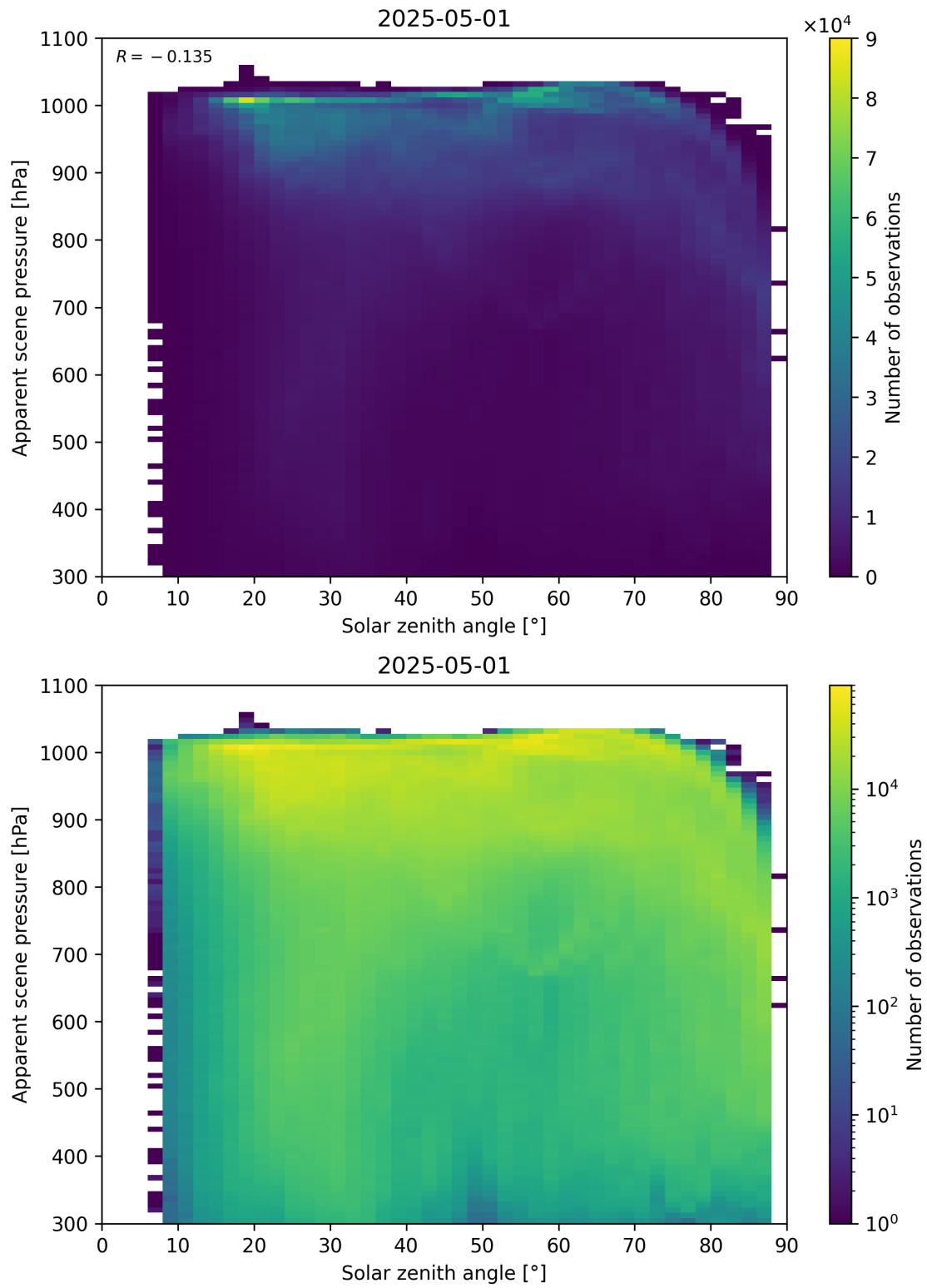
Figure 108: Scatter density plot of “Solar zenith angle” against “Apparent scene pressure” for 2025-04-30 to 2025-05-02.
