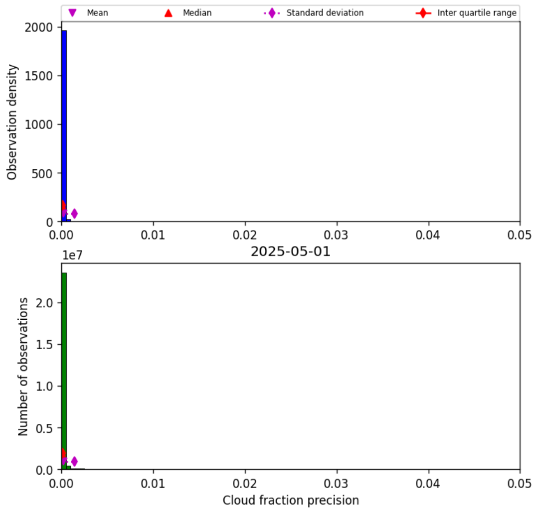
Figure 33: Histogram of “Cloud fraction precision” for 2025-04-30 to 2025-05-02
