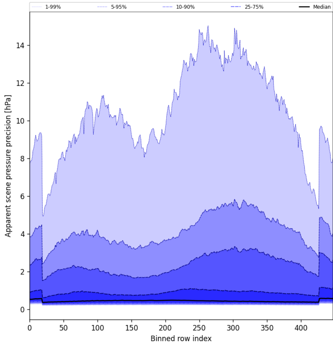
Figure 54: Along track statistics of “Apparent scene pressure precision” for 2025-04-30 to 2025-05-02
