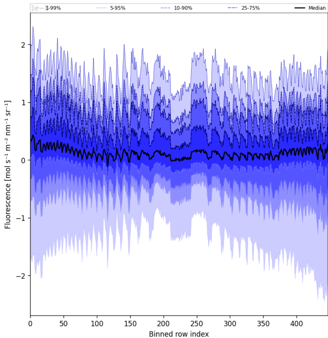
Figure 57: Along track statistics of “Fluorescence” for 2025-04-30 to 2025-05-02
