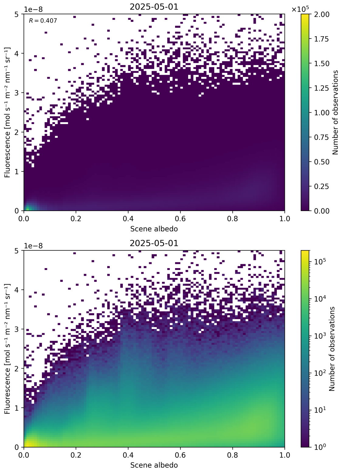
Figure 104: Scatter density plot of “Scene albedo” against “Fluorescence” for 2025-04-30 to 2025-05-02.
