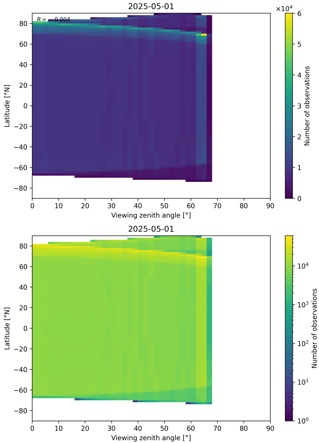
Figure 123: Scatter density plot of “Viewing zenith angle” against “Latitude” for 2025-04-30 to 2025-05-02.
