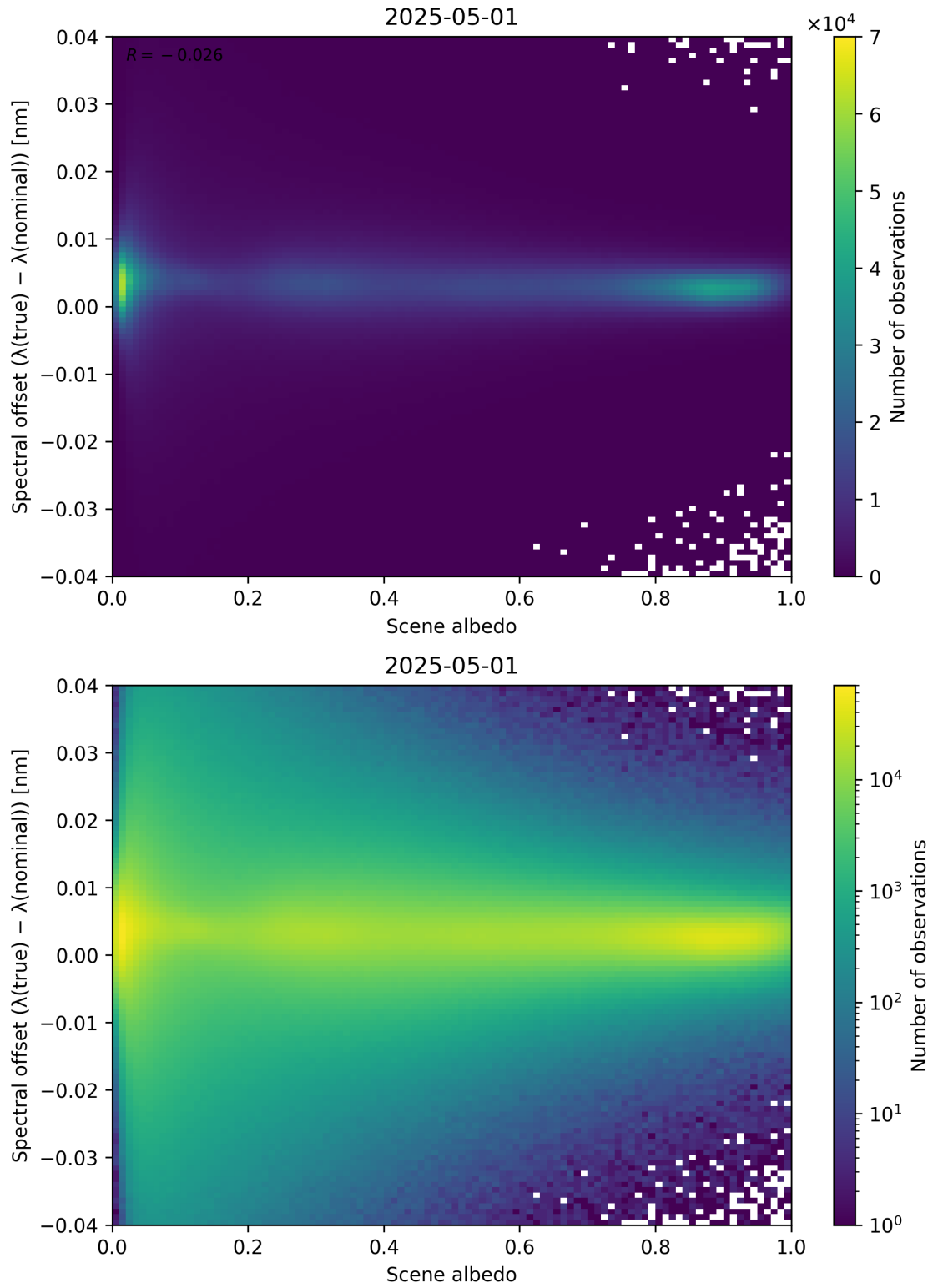
Figure 107: Scatter density plot of “Scene albedo” against “Spectral offset ( \lambda_{\text{true}} - \lambda_{\text{nominal}} )” for 2025-04-30 to 2025-05-02.
