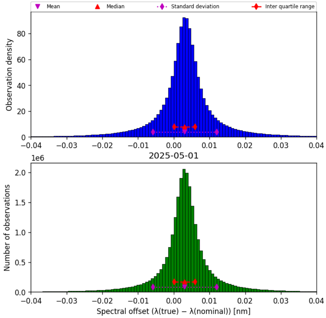
Figure 45: Histogram of “Spectral offset ( \lambda_{\text{true}} - \lambda_{\text{nominal}} )” for 2025-04-30 to 2025-05-02
