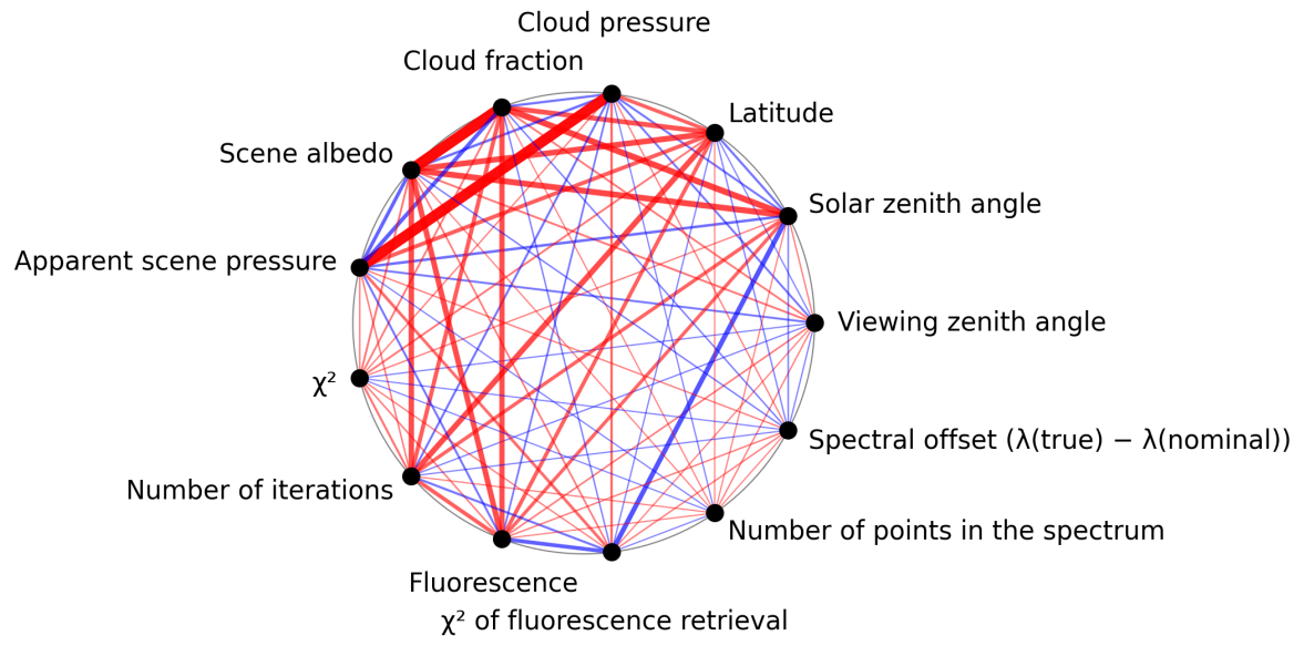
Figure 1: Map of correlation graph for 2025-04-30 to 2025-05-02.
