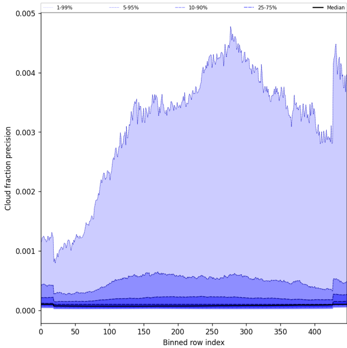
Figure 50: Along track statistics of “Cloud fraction precision” for 2025-04-30 to 2025-05-02
