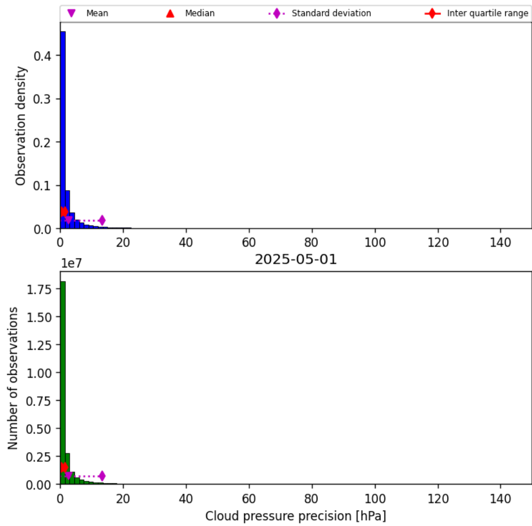
Figure 31: Histogram of “Cloud pressure precision” for 2025-04-30 to 2025-05-02
