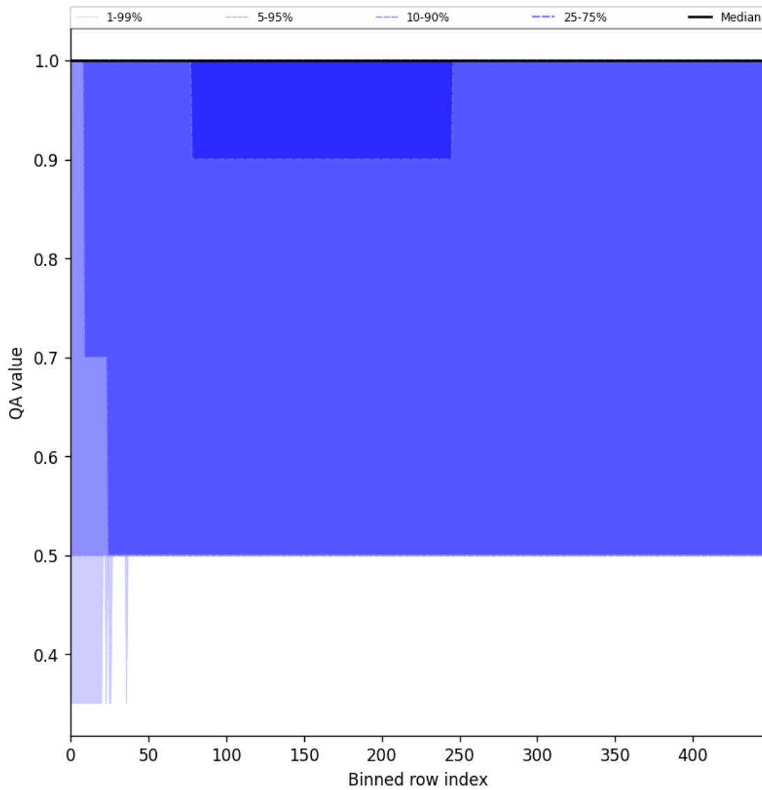
Figure 46: Along track statistics of “QA value” for 2025-04-30 to 2025-05-02
