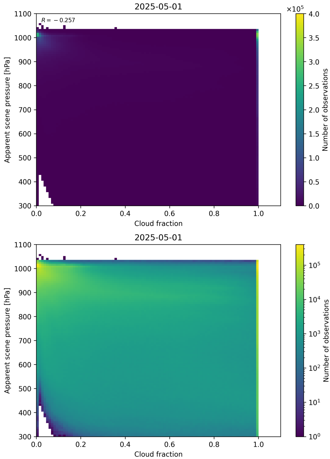
Figure 70: Scatter density plot of “Cloud fraction” against “Apparent scene pressure” for 2025-04-30 to 2025-05-02.
