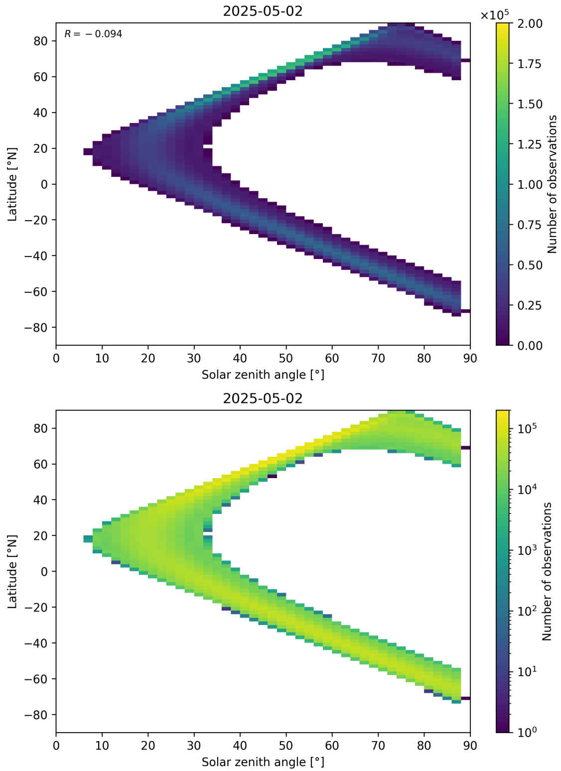
Figure 113: Scatter density plot of “Solar zenith angle” against “Latitude” for 2025-05-01 to 2025-05-03.
