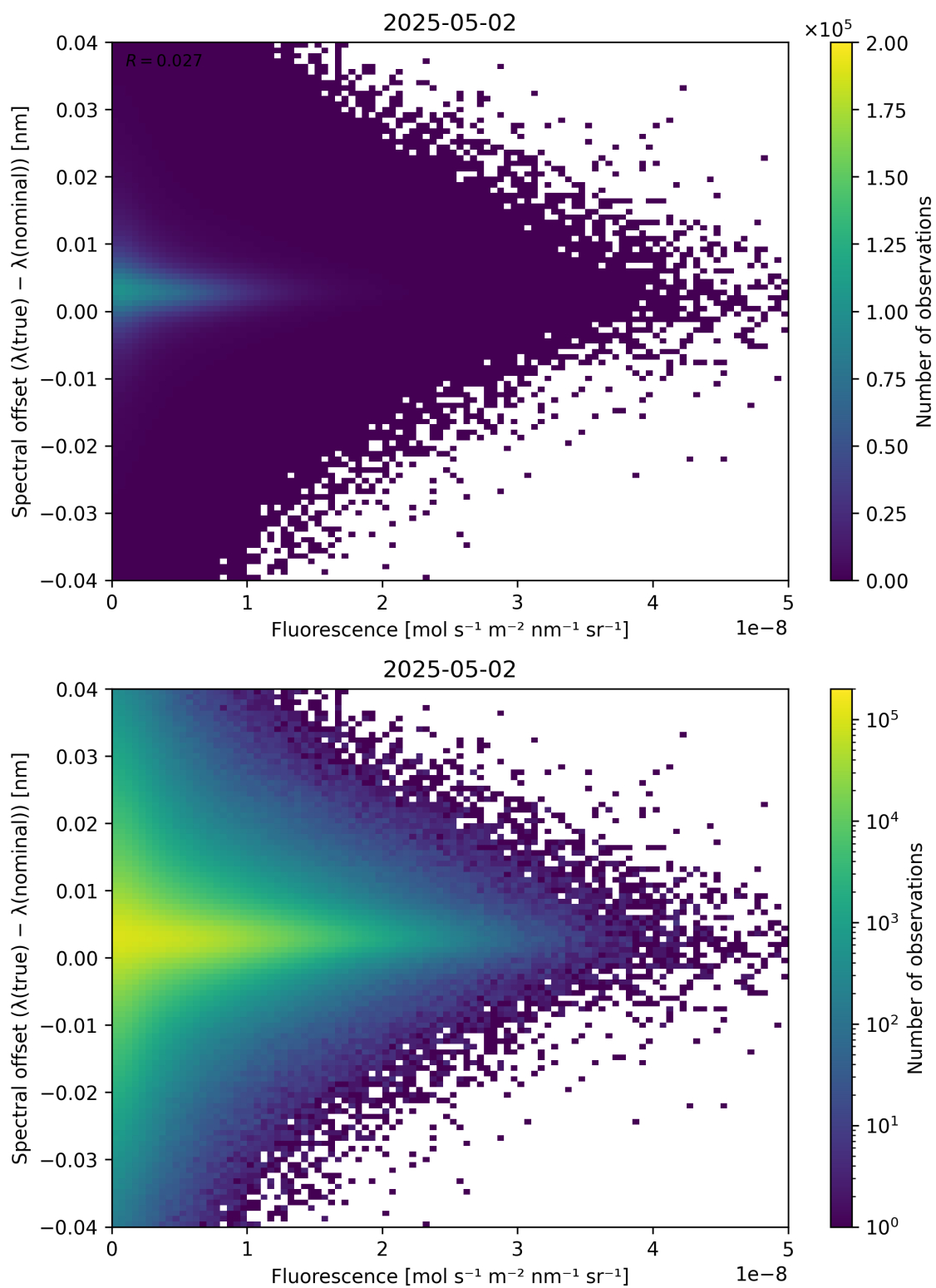
Figure 87: Scatter density plot of “Fluorescence” against “Spectral offset ( \lambda_{\text{true}} - \lambda_{\text{nominal}} )” for 2025-05-01 to 2025-05-03.
