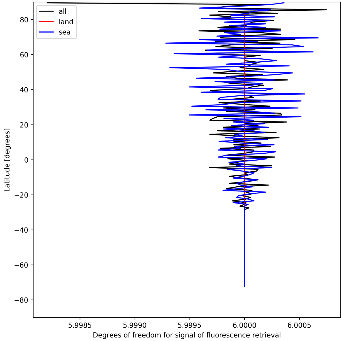
Figure 26: Zonal average of “Degrees of freedom for signal of fluorescence retrieval” for 2025-05-01 to 2025-05-03.
