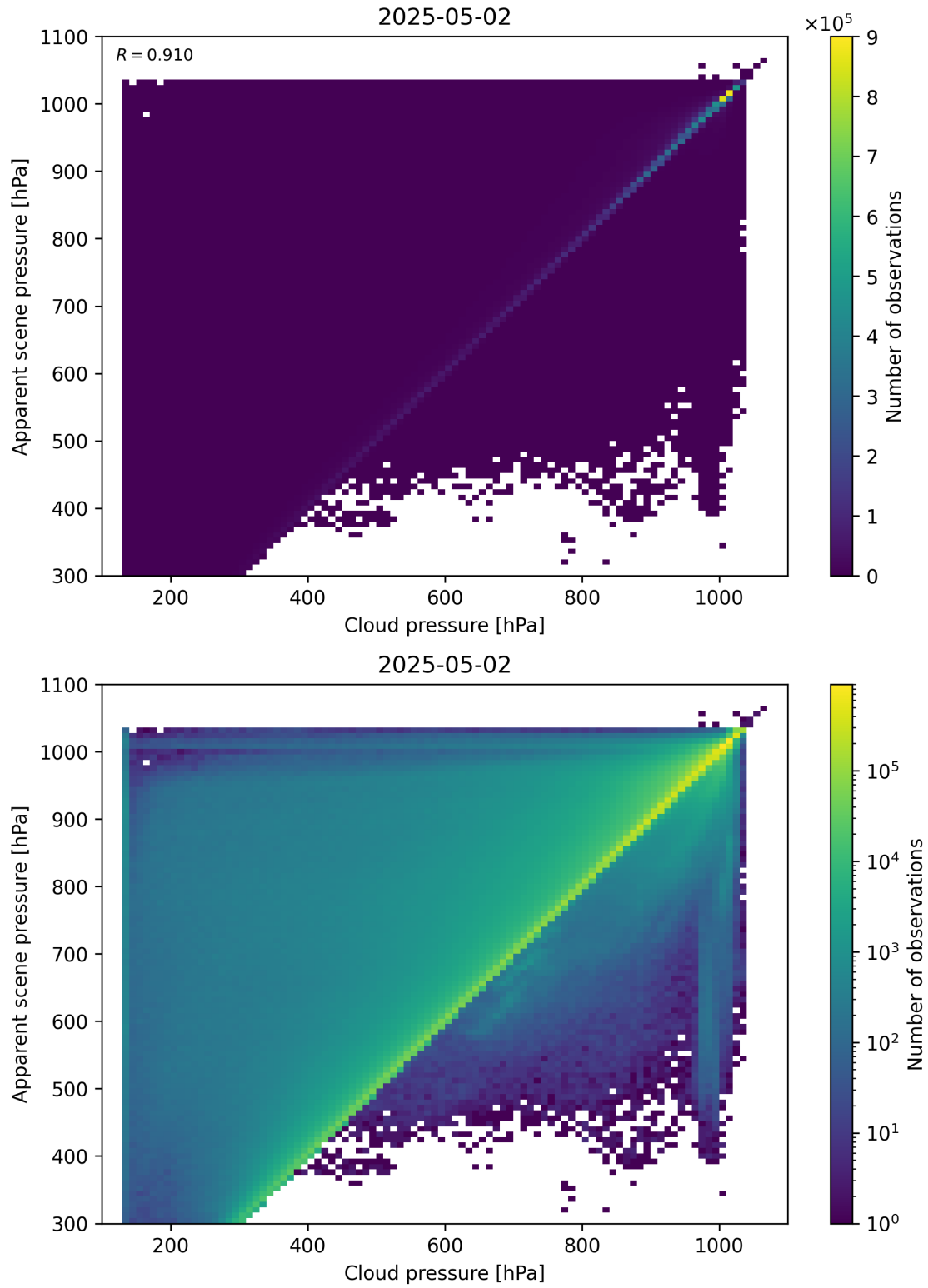
Figure 77: Scatter density plot of “Cloud pressure” against “Apparent scene pressure” for 2025-05-01 to 2025-05-03.
