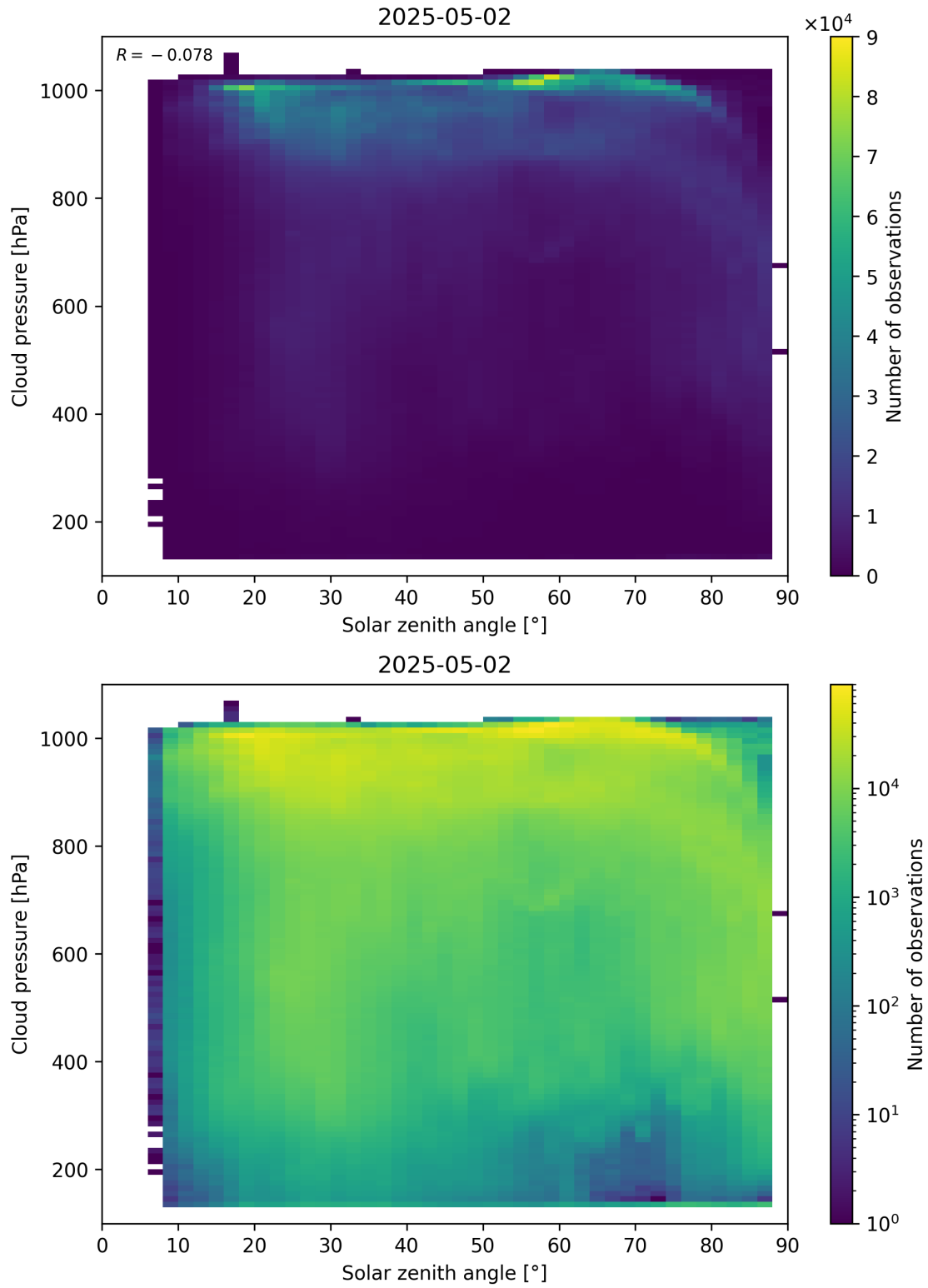
Figure 111: Scatter density plot of “Solar zenith angle” against “Cloud pressure” for 2025-05-01 to 2025-05-03.
