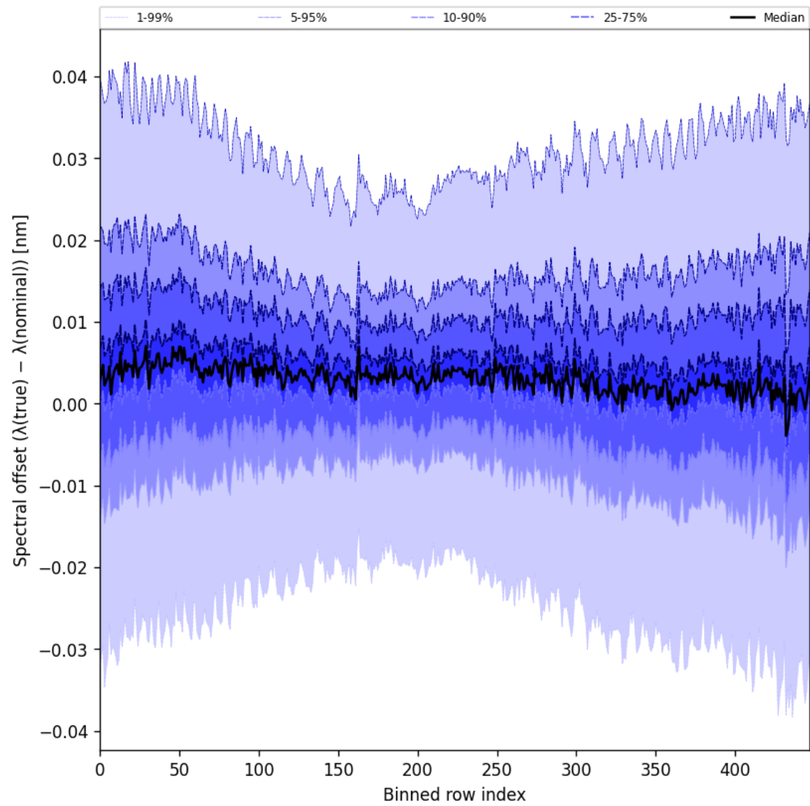
Figure 62: Along track statistics of “Spectral offset ( \lambda_{\text{true}} - \lambda_{\text{nominal}} )” for 2025-05-01 to 2025-05-03
