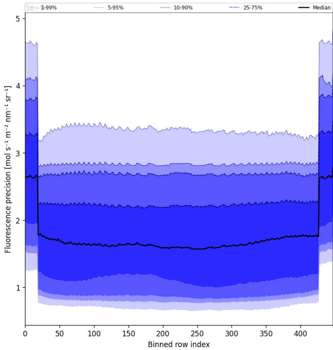
Figure 58: Along track statistics of “Fluorescence precision” for 2025-05-01 to 2025-05-03
