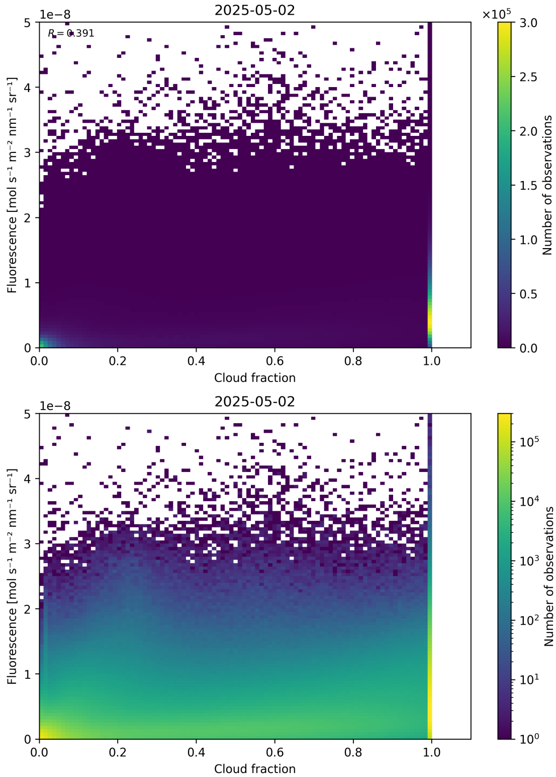
Figure 72: Scatter density plot of “Cloud fraction” against “Fluorescence” for 2025-05-01 to 2025-05-03.
