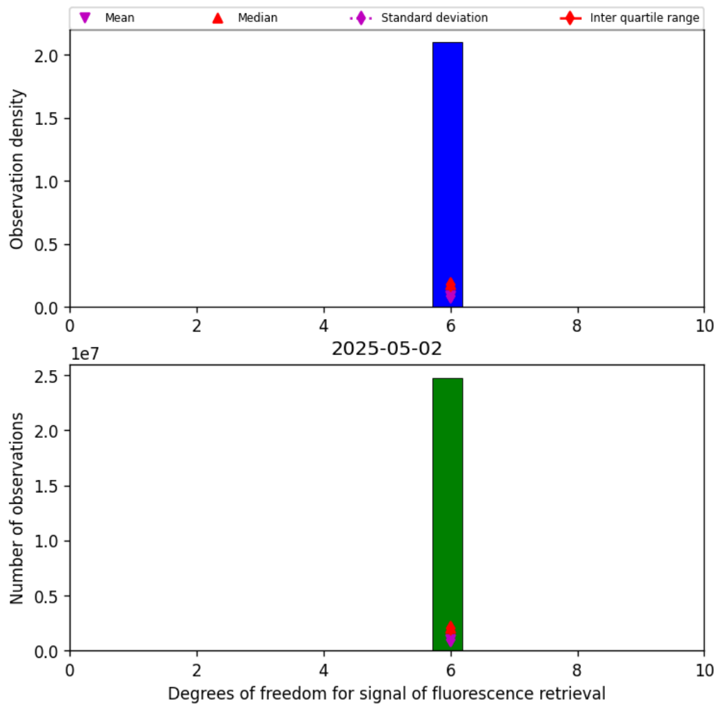
Figure 43: Histogram of "Degrees of freedom for signal of fluorescence retrieval" for 2025-05-01 to 2025-05-03
