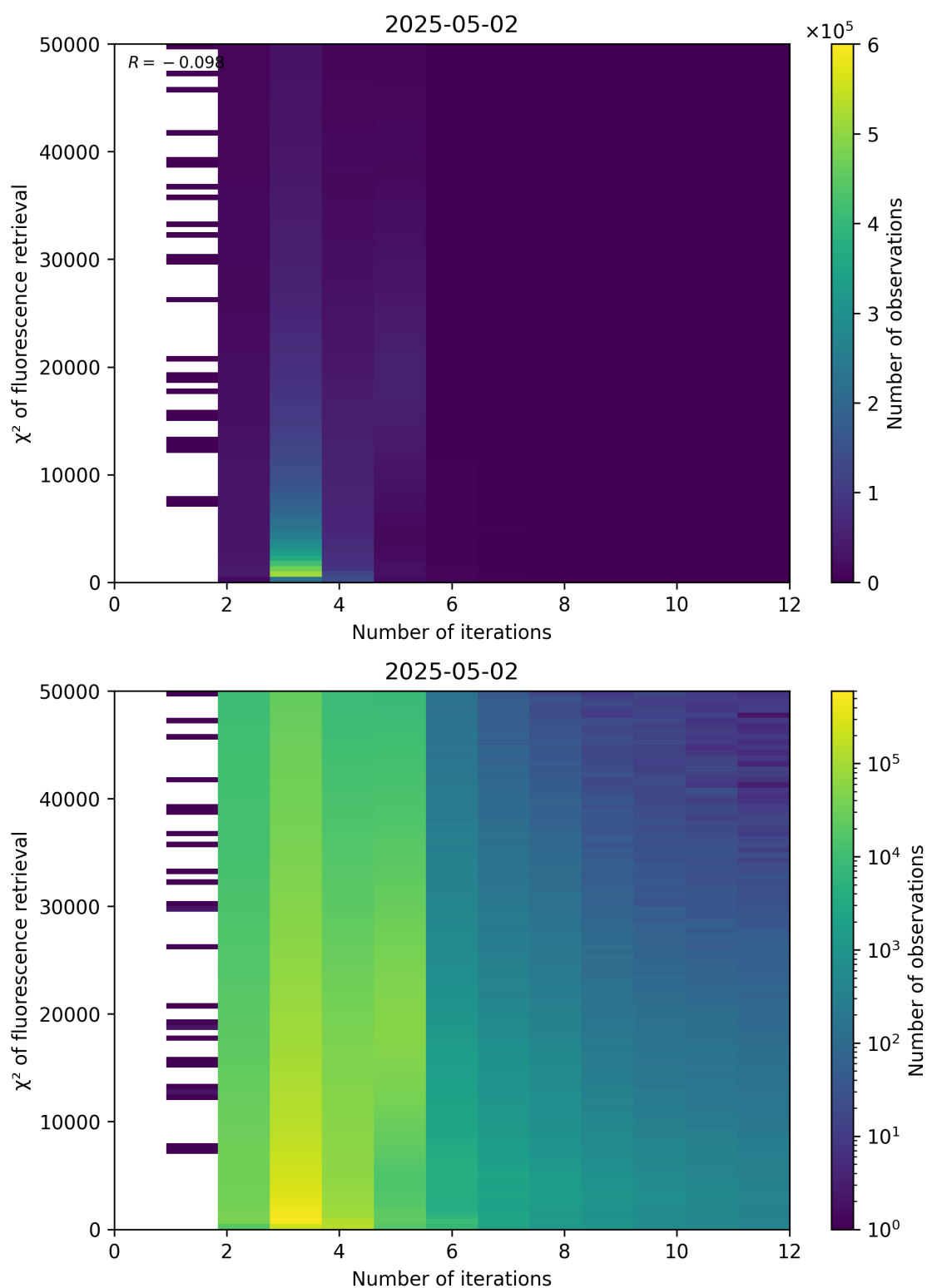
Figure 97: Scatter density plot of “Number of iterations” against “ \chi^2 of fluorescence retrieval” for 2025-05-01 to 2025-05-03.
