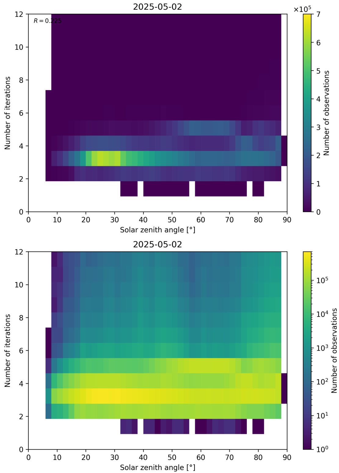
Figure 114: Scatter density plot of “Solar zenith angle” against “Number of iterations” for 2025-05-01 to 2025-05-03.
