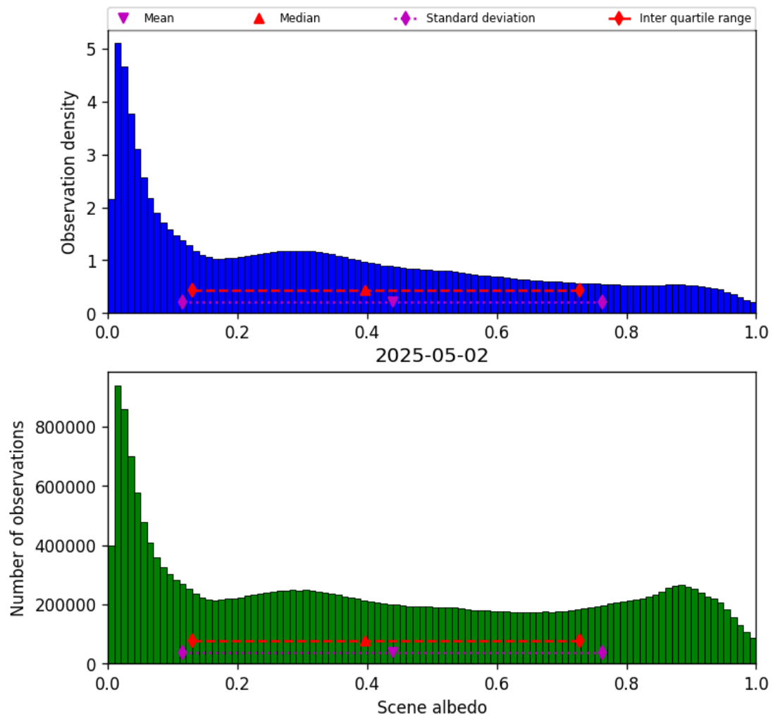
Figure 34: Histogram of “Scene albedo” for 2025-05-01 to 2025-05-03
