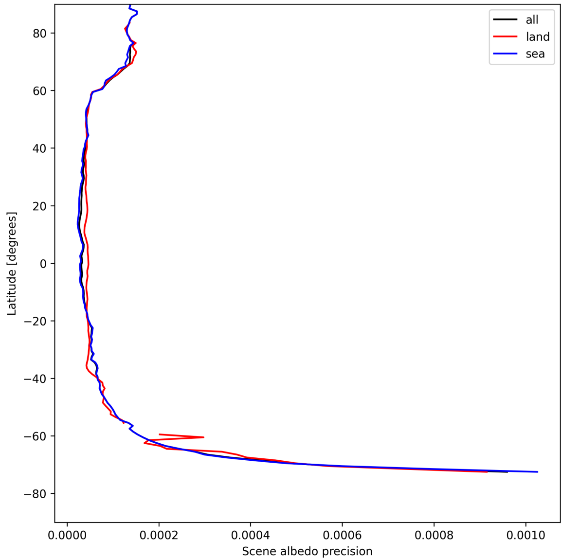
Figure 18: Zonal average of “Scene albedo precision” for 2025-05-01 to 2025-05-03.
