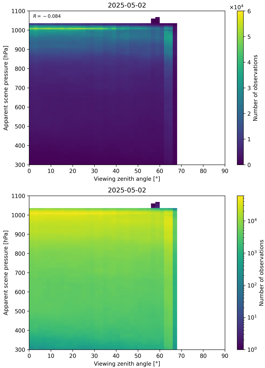
Figure 118: Scatter density plot of “Viewing zenith angle” against “Apparent scene pressure” for 2025-05-01 to 2025-05-03.
