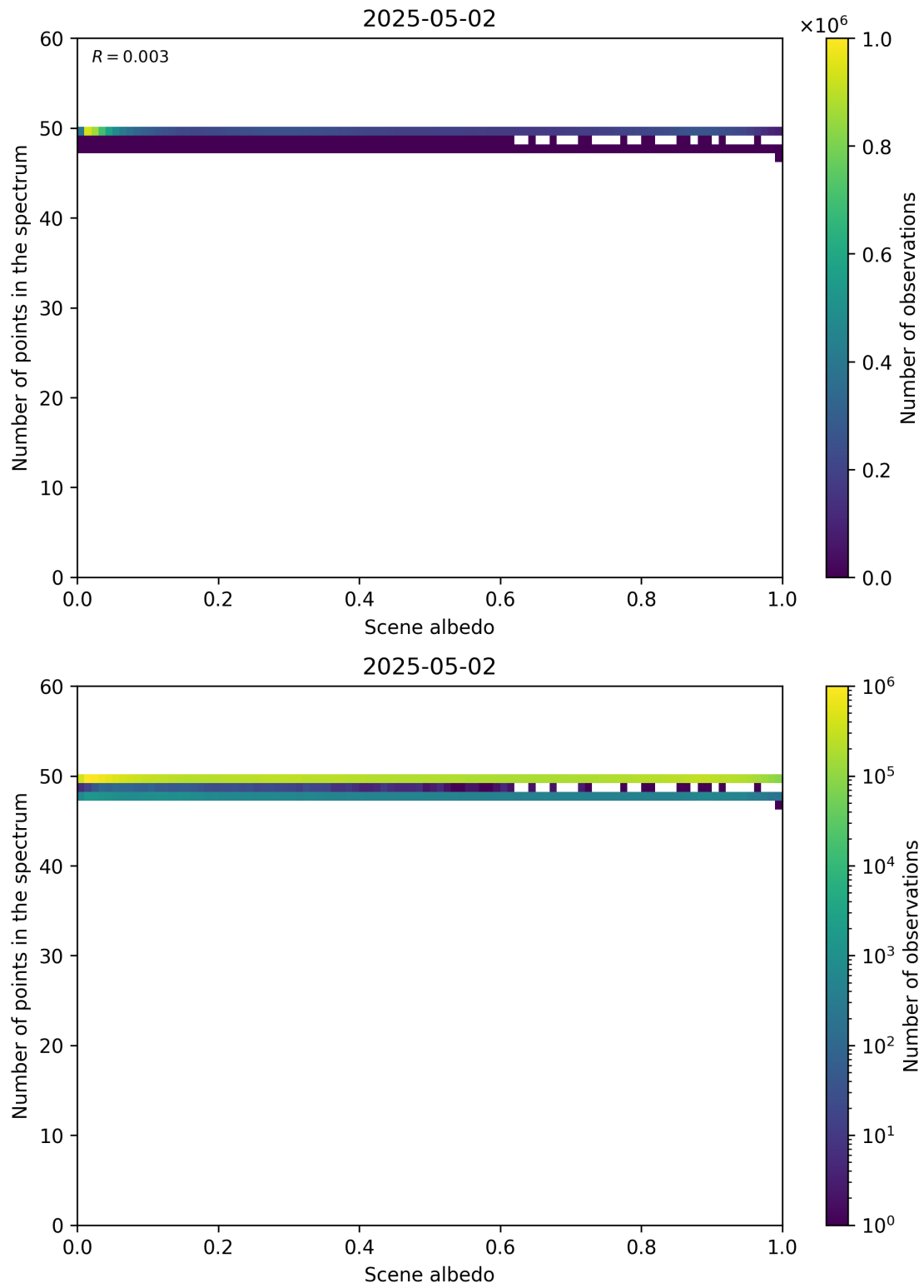
Figure 106: Scatter density plot of “Scene albedo” against “Number of points in the spectrum” for 2025-05-01 to 2025-05-03.
