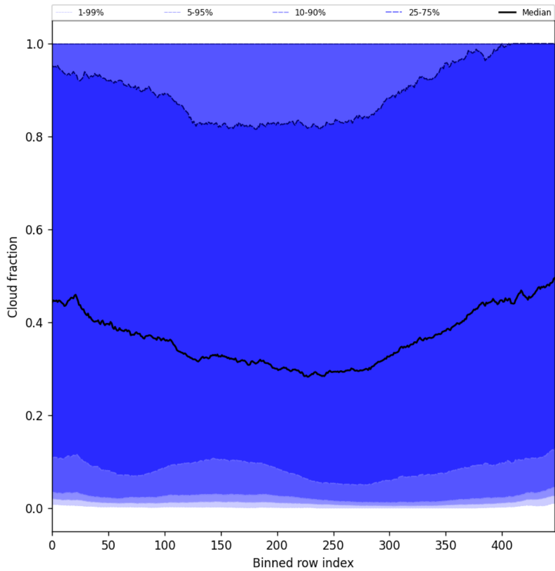
Figure 49: Along track statistics of “Cloud fraction” for 2025-05-01 to 2025-05-03
