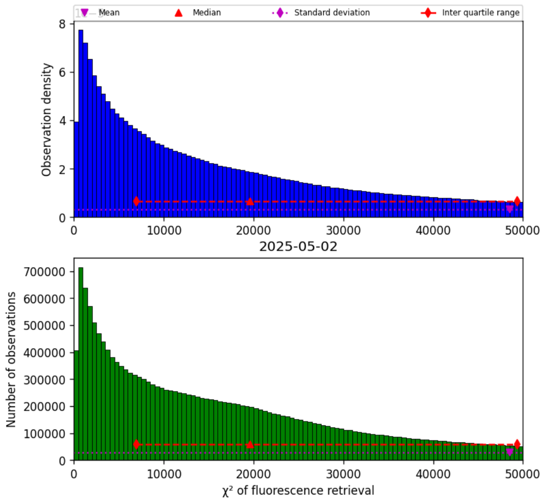
Figure 42: Histogram of “ \chi^2 of fluorescence retrieval” for 2025-05-01 to 2025-05-03
