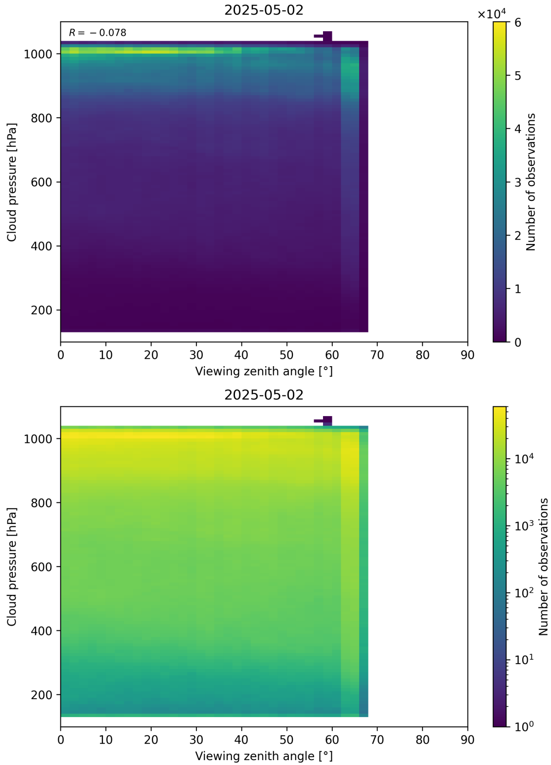
Figure 121: Scatter density plot of “Viewing zenith angle” against “Cloud pressure” for 2025-05-01 to 2025-05-03.
