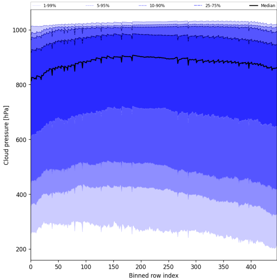
Figure 47: Along track statistics of “Cloud pressure” for 2025-05-01 to 2025-05-03
