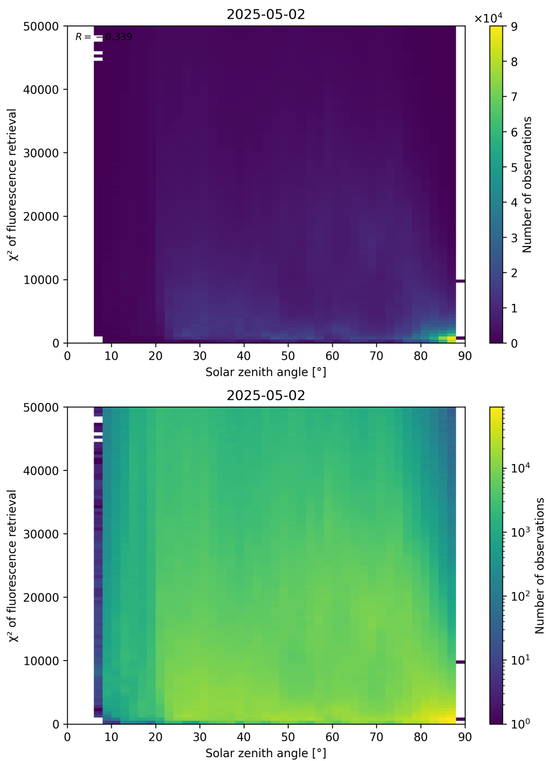
Figure 109: Scatter density plot of “Solar zenith angle” against “ \chi^2 of fluorescence retrieval” for 2025-05-01 to 2025-05-03.
