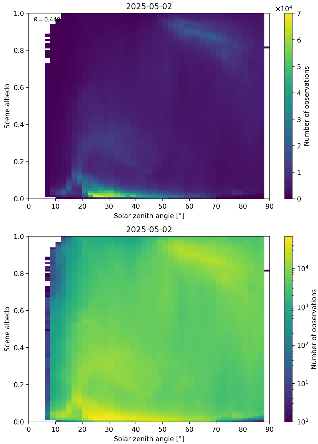
Figure 116: Scatter density plot of “Solar zenith angle” against “Scene albedo” for 2025-05-01 to 2025-05-03.
