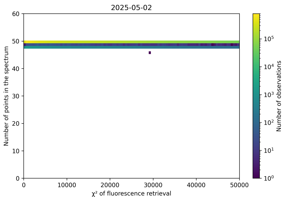
Figure 68: Scatter density plot of “ \chi^2 of fluorescence retrieval” against “Number of points in the spectrum” for 2025-05-01 to 2025-05-03.
