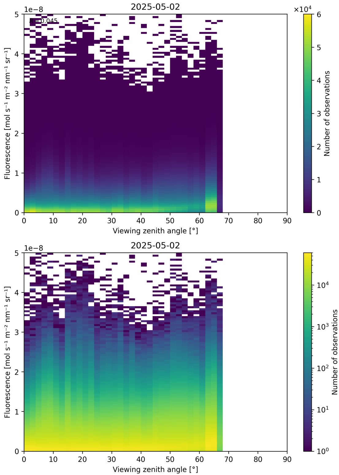
Figure 122: Scatter density plot of “Viewing zenith angle” against “Fluorescence” for 2025-05-01 to 2025-05-03.
