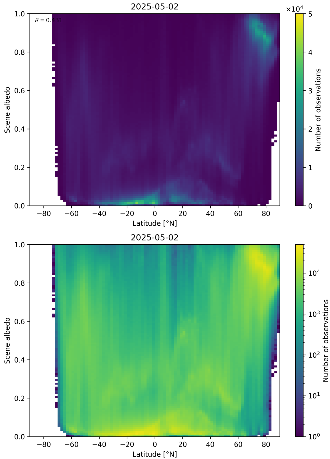
Figure 95: Scatter density plot of “Latitude” against “Scene albedo” for 2025-05-01 to 2025-05-03.
