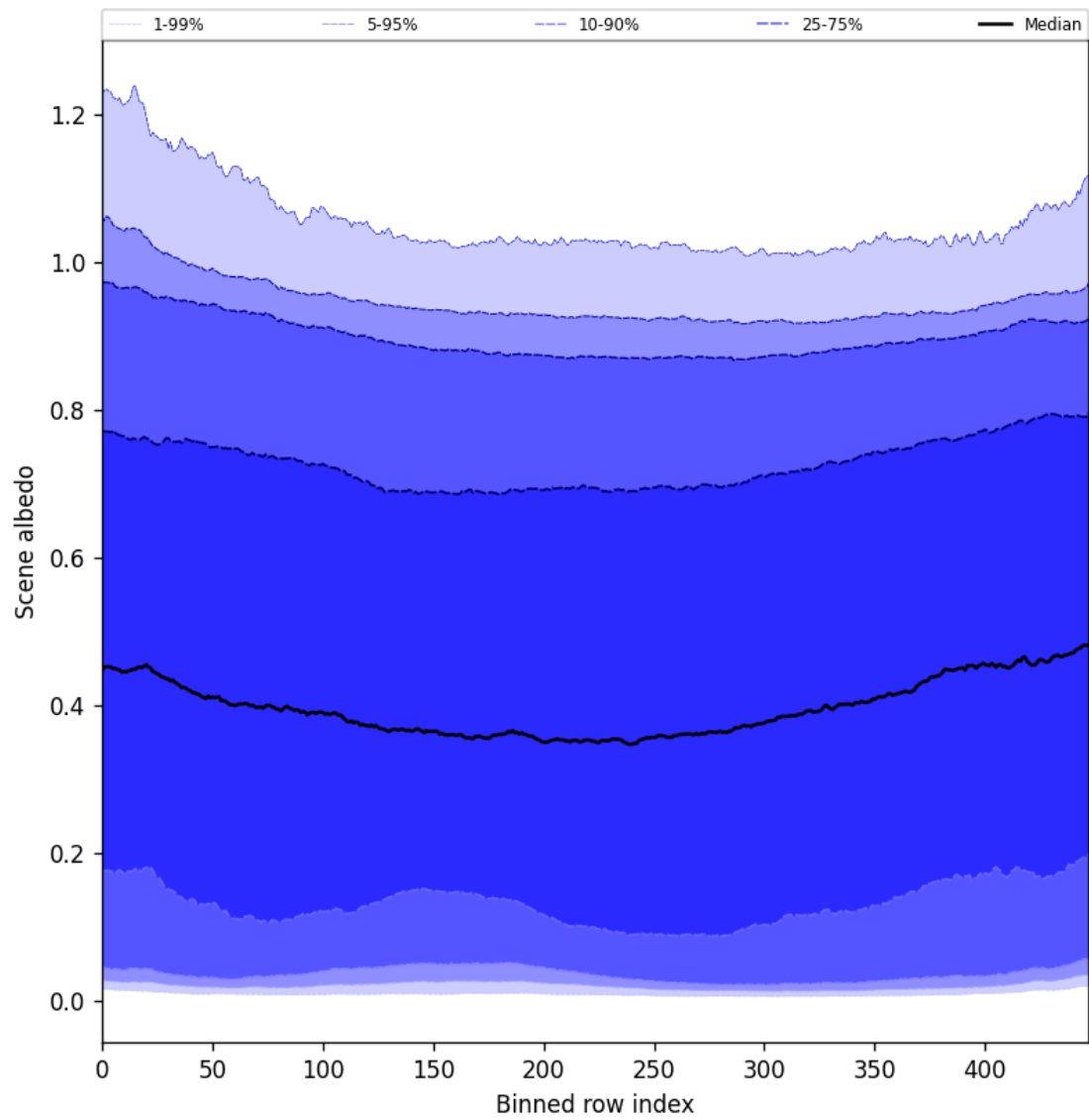
Figure 51: Along track statistics of “Scene albedo” for 2025-05-01 to 2025-05-03
