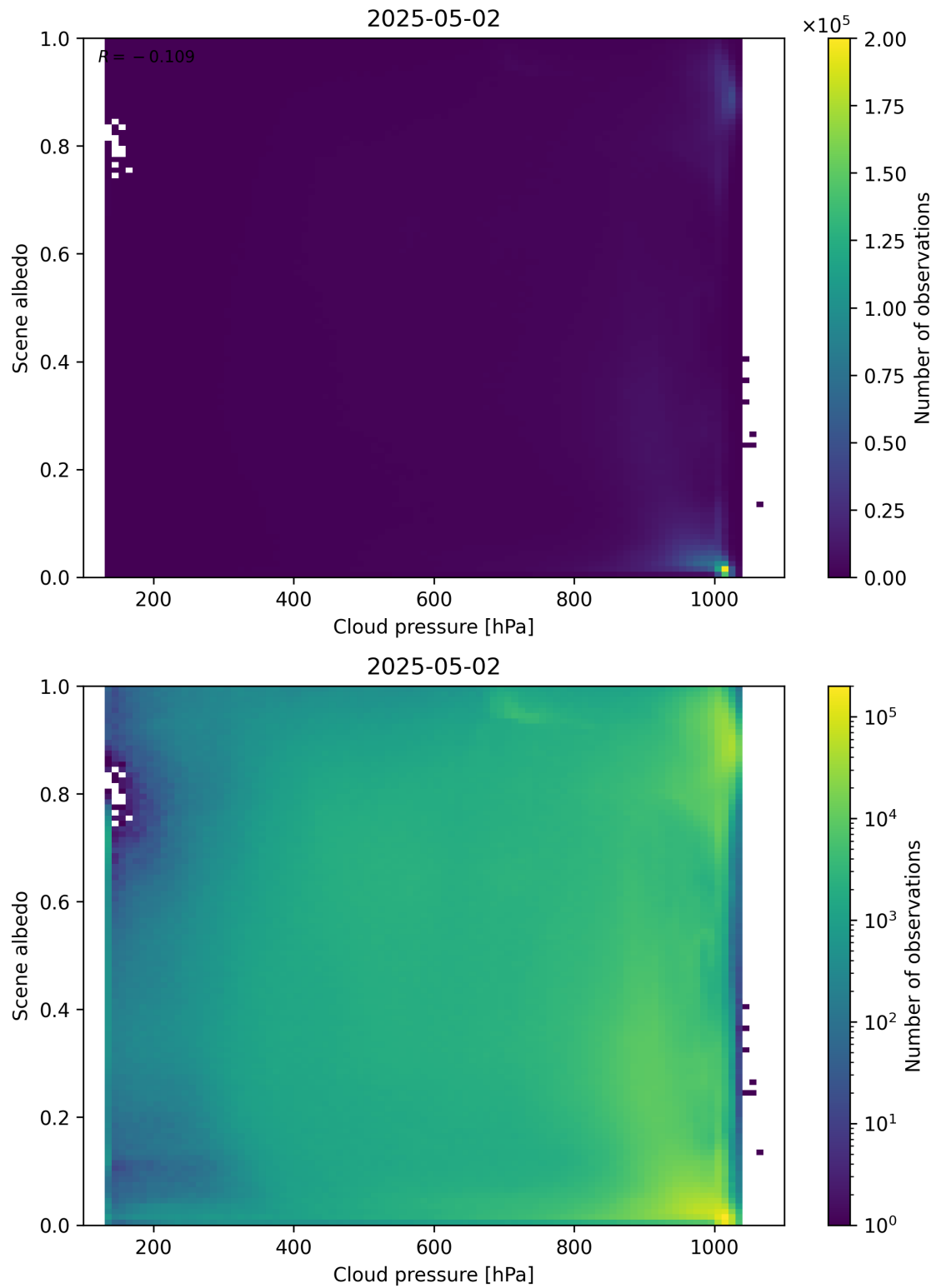
Figure 83: Scatter density plot of “Cloud pressure” against “Scene albedo” for 2025-05-01 to 2025-05-03.
