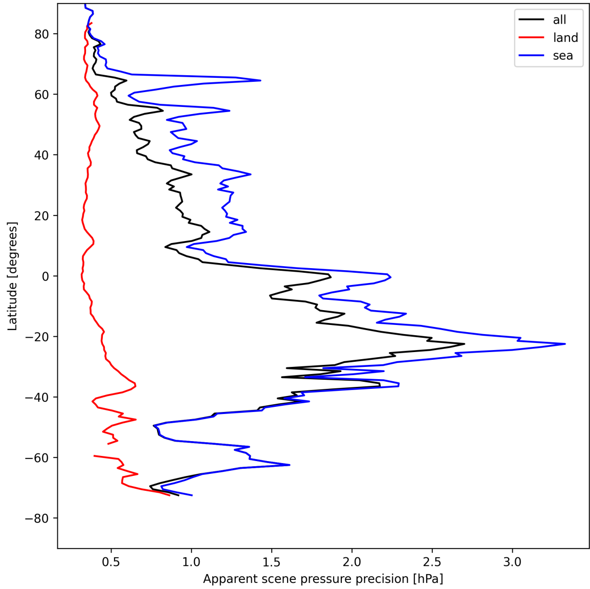
Figure 20: Zonal average of “Apparent scene pressure precision” for 2025-05-01 to 2025-05-03.
