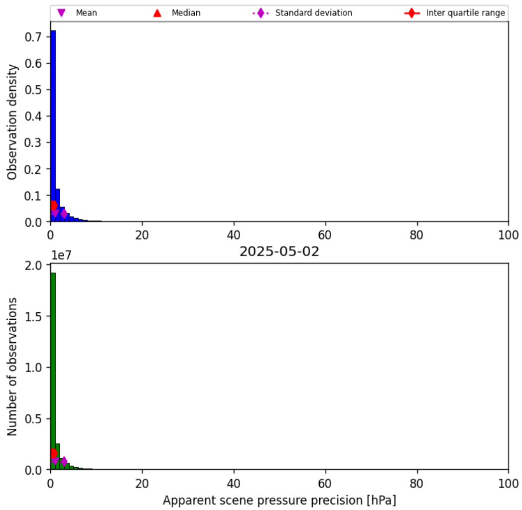
Figure 37: Histogram of “Apparent scene pressure precision” for 2025-05-01 to 2025-05-03
