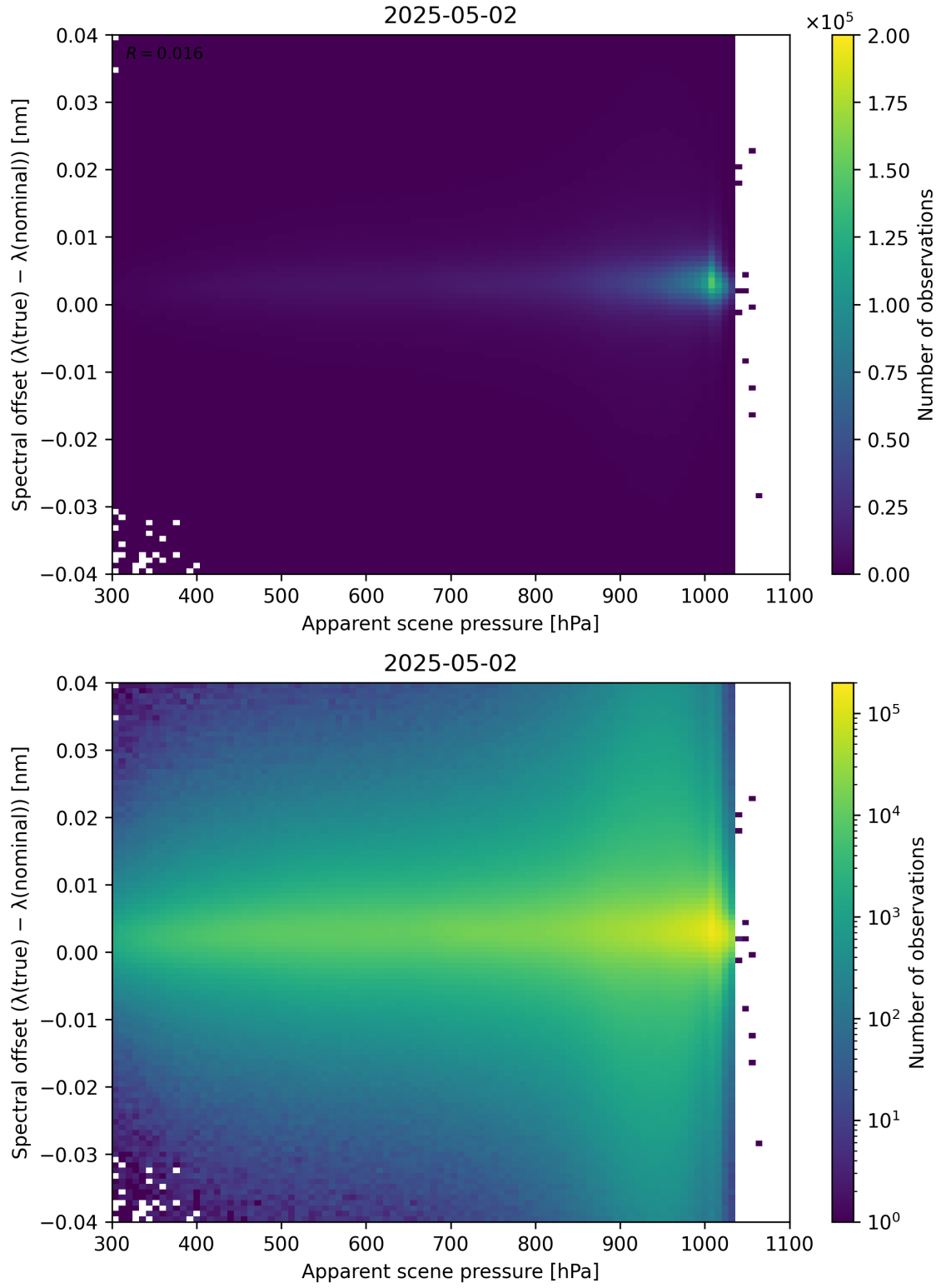
Figure 67: Scatter density plot of “Apparent scene pressure” against “Spectral offset ( \lambda_{\text{true}} - \lambda_{\text{nominal}} )” for 2025-05-01 to 2025-05-03.
