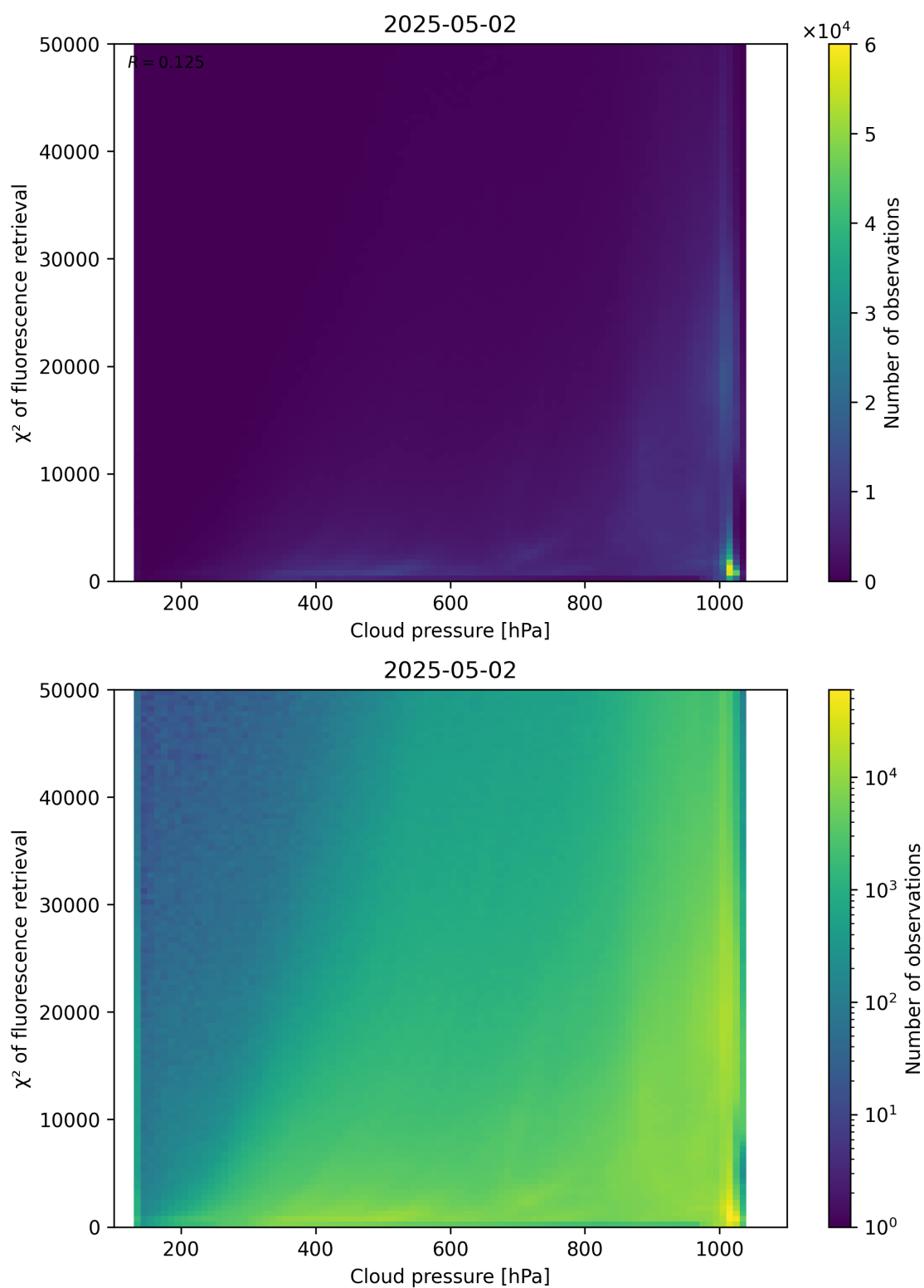
Figure 78: Scatter density plot of “Cloud pressure” against “ \chi^2 of fluorescence retrieval” for 2025-05-01 to 2025-05-03.
