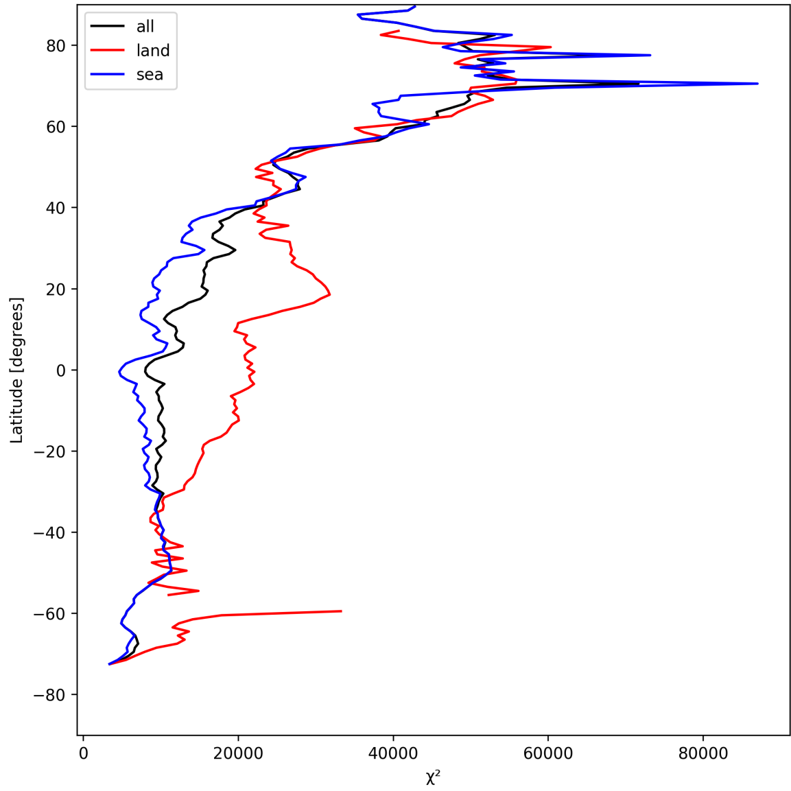
Figure 21: Zonal average of “ \chi^2 ” for 2025-05-01 to 2025-05-03.
