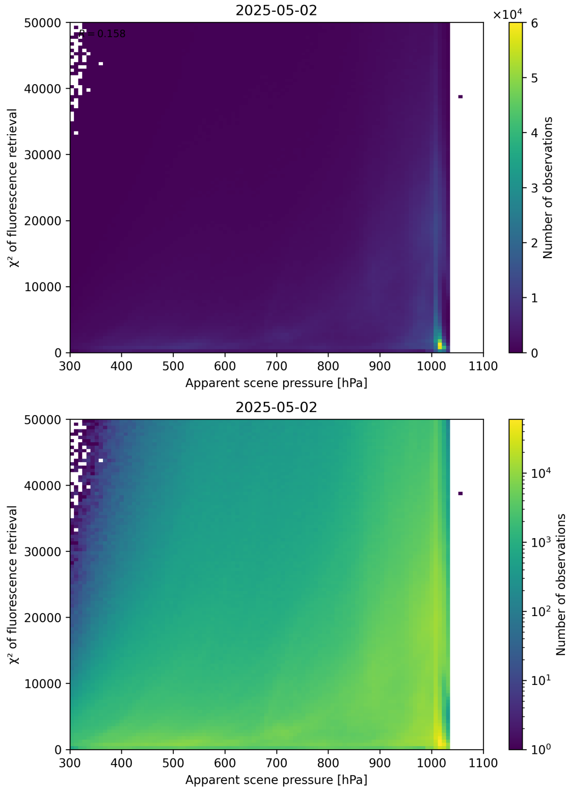
Figure 63: Scatter density plot of “Apparent scene pressure” against “ \chi^2 of fluorescence retrieval” for 2025-05-01 to 2025-05-03.
