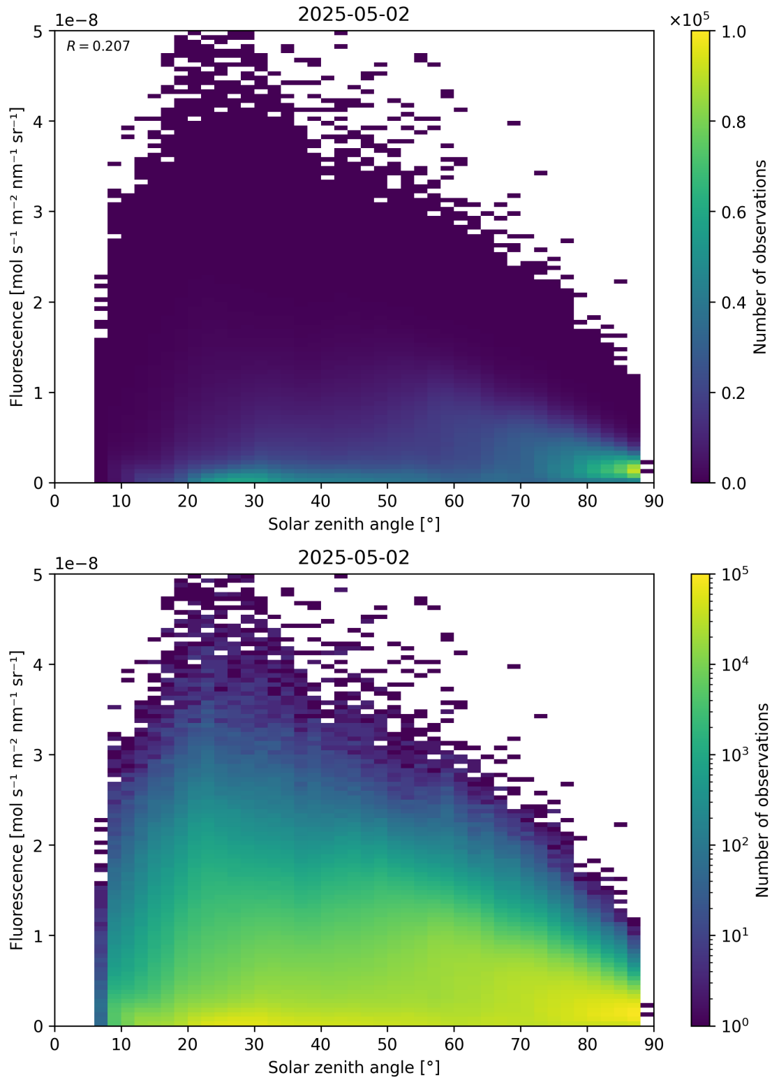
Figure 112: Scatter density plot of “Solar zenith angle” against “Fluorescence” for 2025-05-01 to 2025-05-03.
