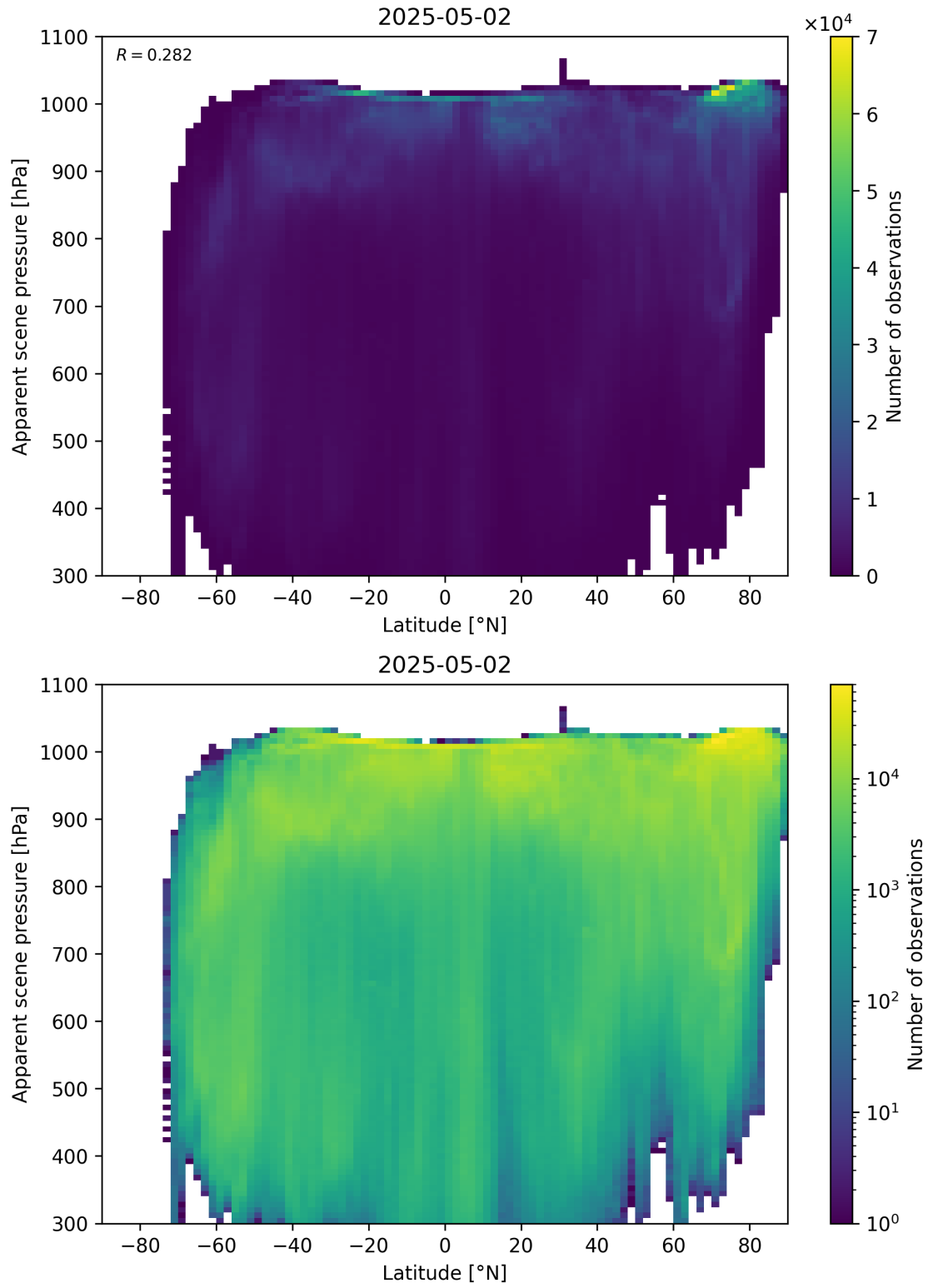
Figure 88: Scatter density plot of “Latitude” against “Apparent scene pressure” for 2025-05-01 to 2025-05-03.
