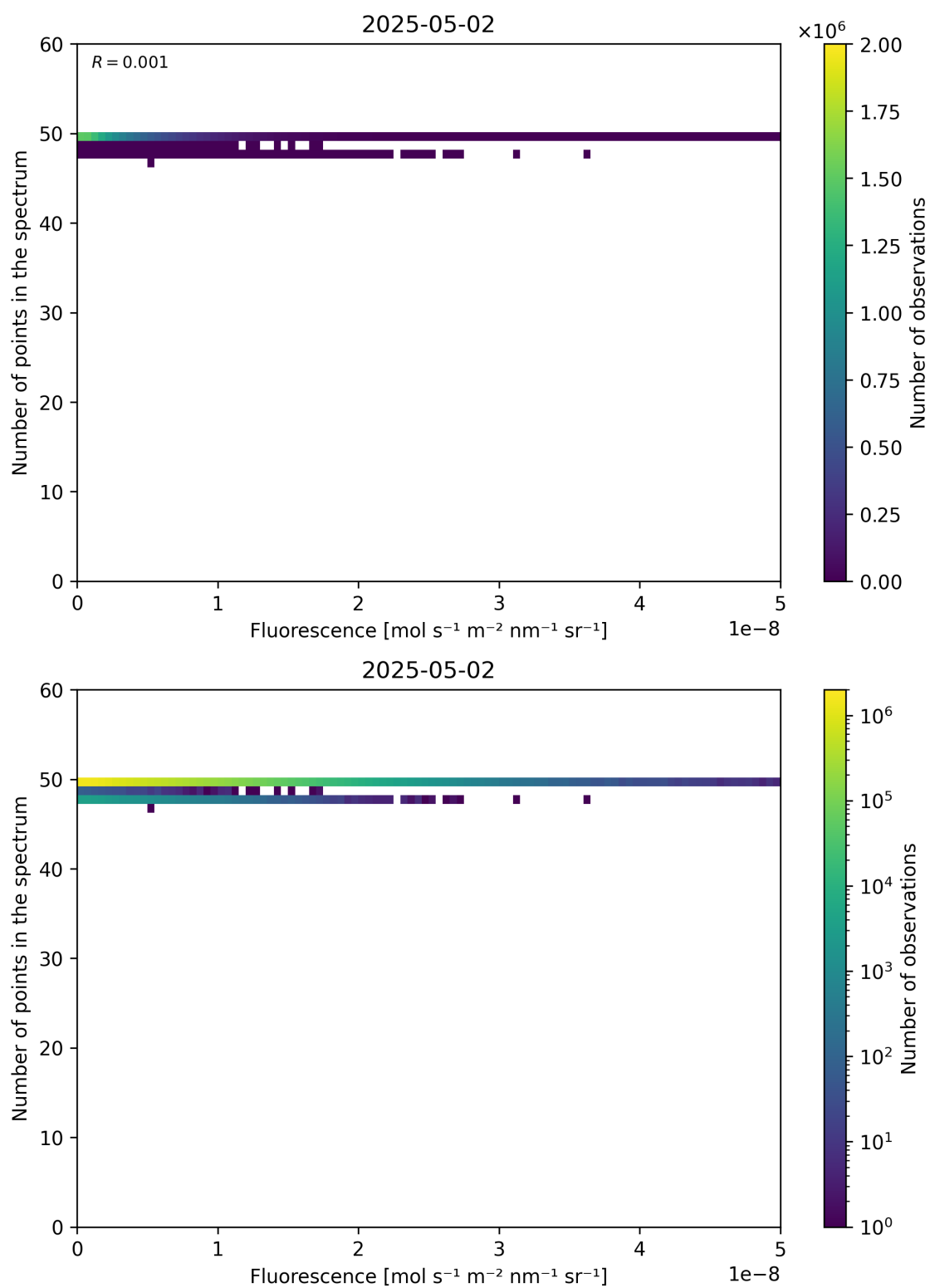
Figure 86: Scatter density plot of “Fluorescence” against “Number of points in the spectrum” for 2025-05-01 to 2025-05-03.
