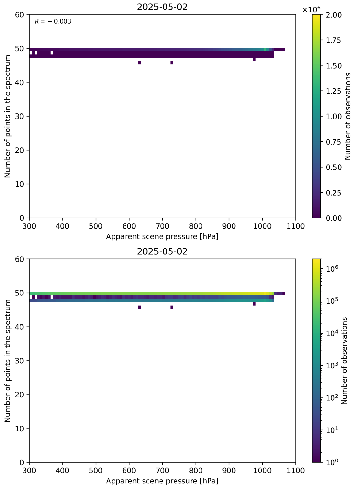
Figure 66: Scatter density plot of “Apparent scene pressure” against “Number of points in the spectrum” for 2025-05-01 to 2025-05-03.
