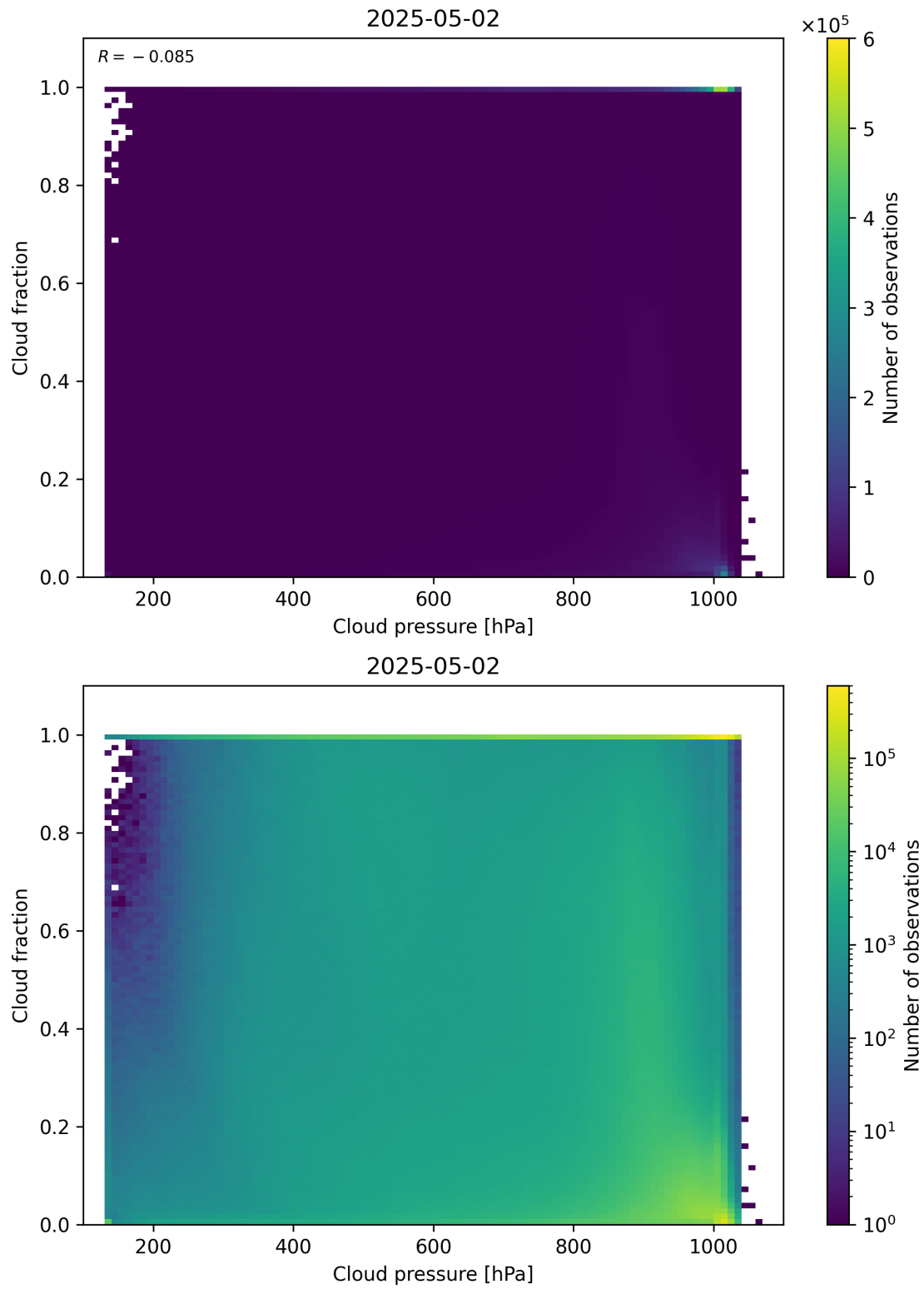
Figure 79: Scatter density plot of “Cloud pressure” against “Cloud fraction” for 2025-05-01 to 2025-05-03.
