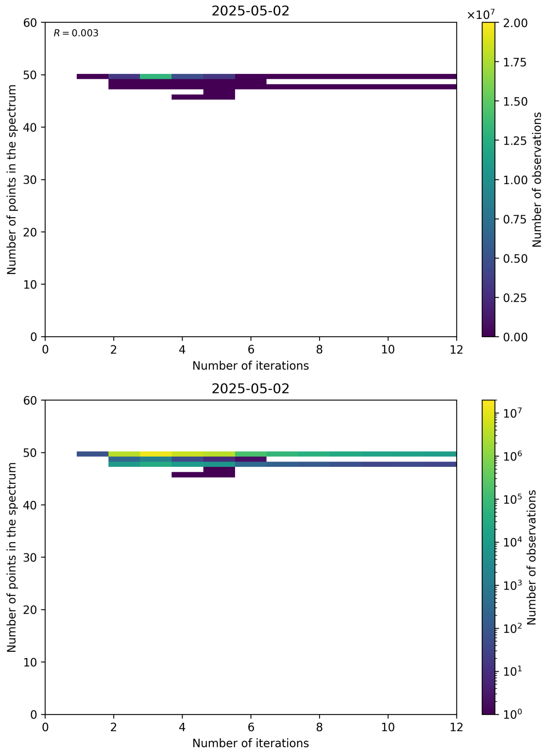
Figure 99: Scatter density plot of “Number of iterations” against “Number of points in the spectrum” for 2025-05-01 to 2025-05-03.
