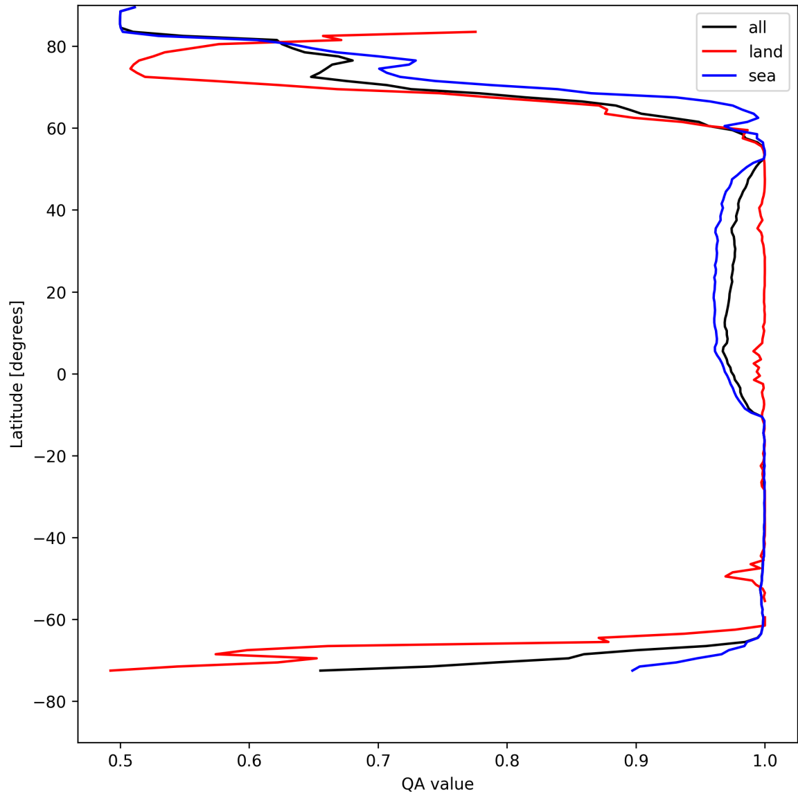
Figure 12: Zonal average of "QA value" for 2025-05-01 to 2025-05-03.
