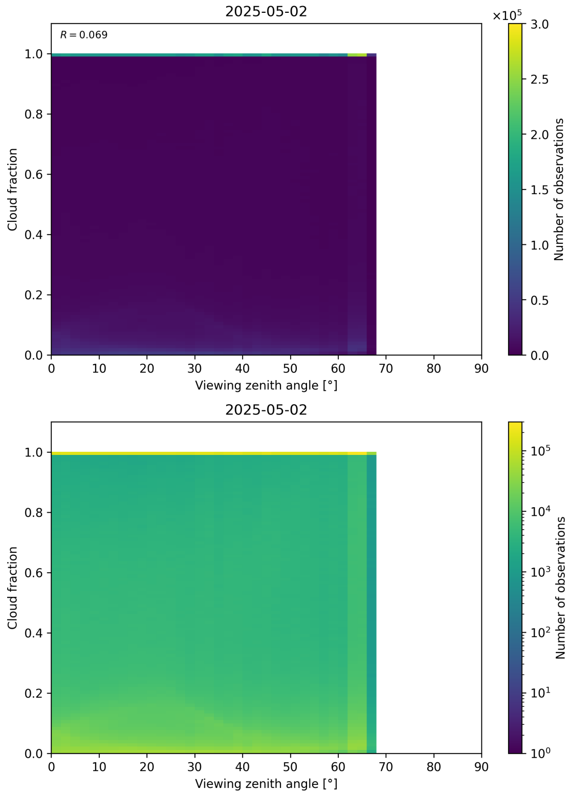
Figure 120: Scatter density plot of “Viewing zenith angle” against “Cloud fraction” for 2025-05-01 to 2025-05-03.
