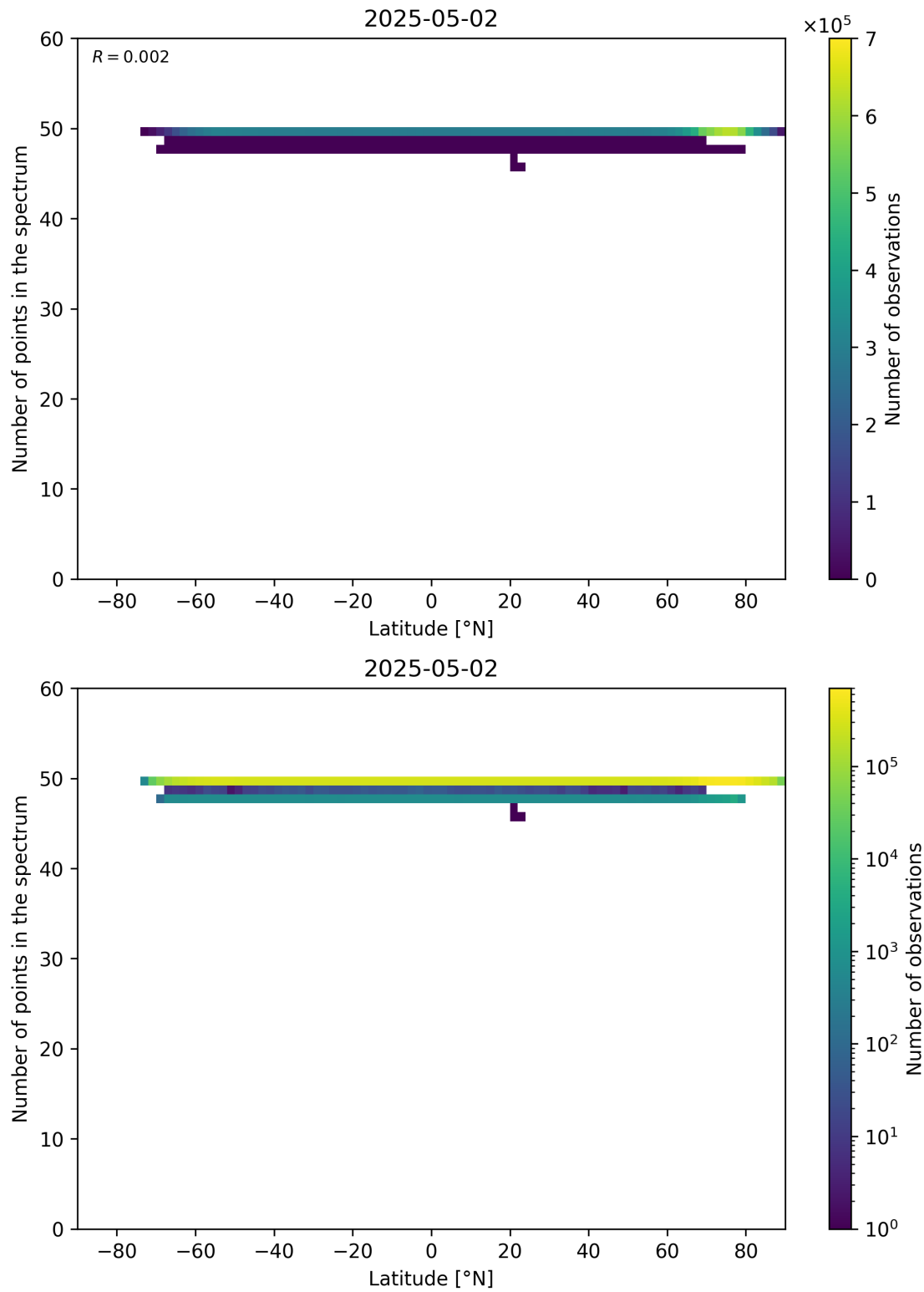
Figure 94: Scatter density plot of “Latitude” against “Number of points in the spectrum” for 2025-05-01 to 2025-05-03.
