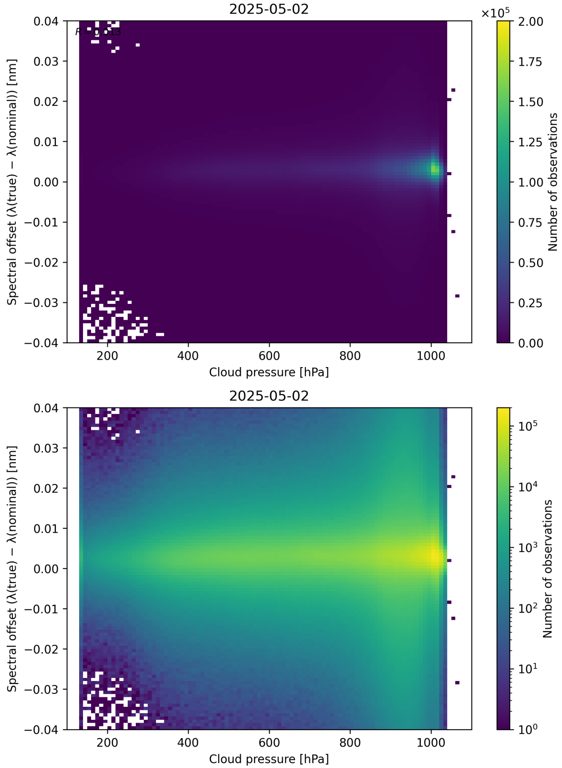
Figure 84: Scatter density plot of “Cloud pressure” against “Spectral offset ( \lambda_{\text{true}} - \lambda_{\text{nominal}} )” for 2025-05-01 to 2025-05-03.
