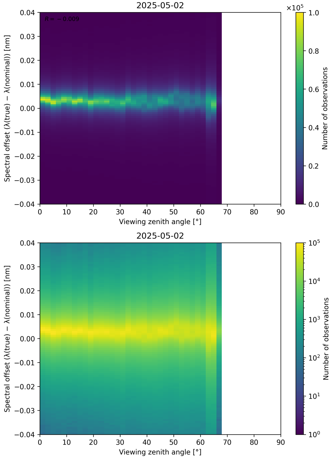
Figure 128: Scatter density plot of “Viewing zenith angle” against “Spectral offset ( \lambda_{\text{true}} - \lambda_{\text{nominal}} )” for 2025-05-01 to 2025-05-03.
