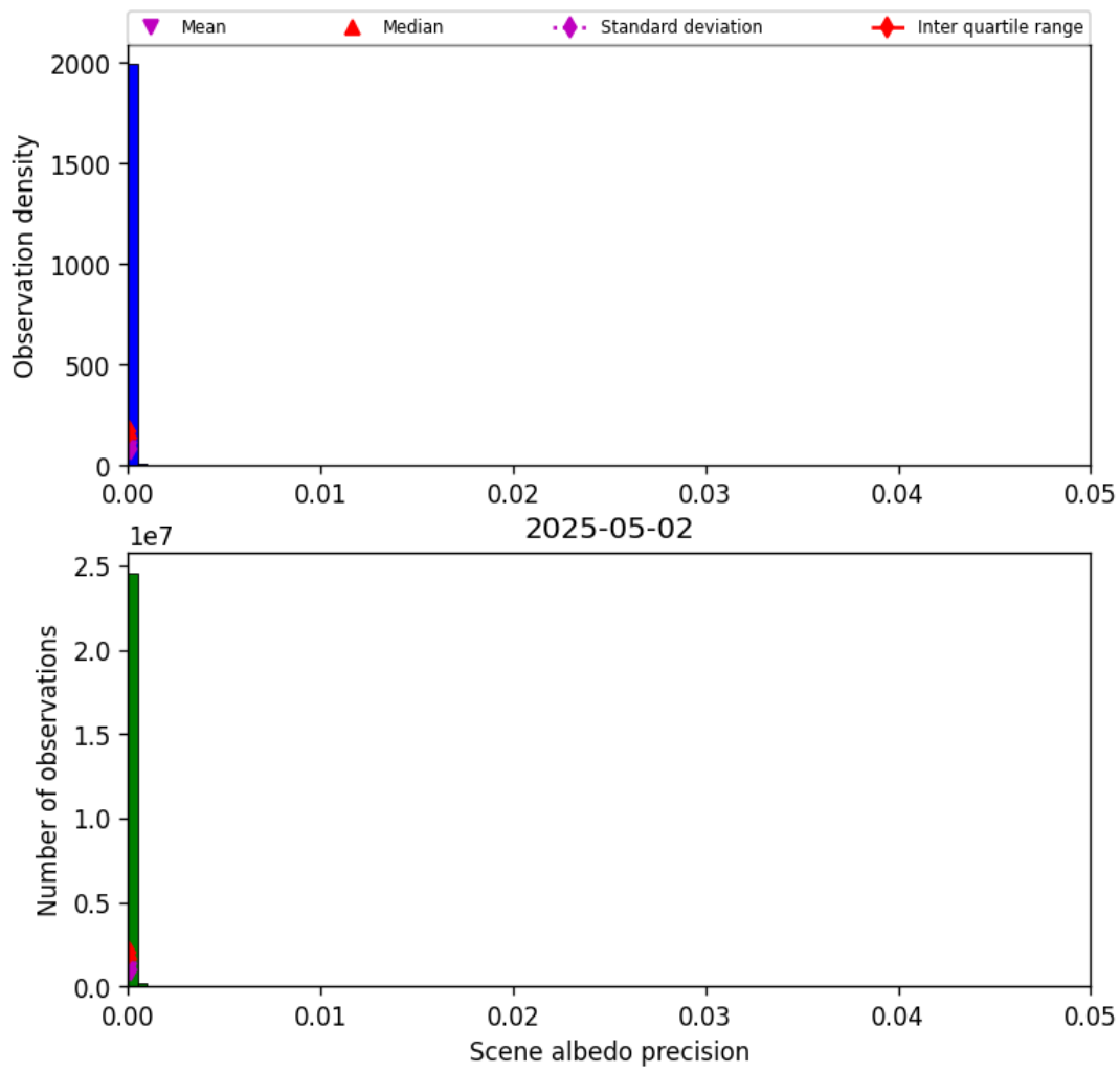
Figure 35: Histogram of “Scene albedo precision” for 2025-05-01 to 2025-05-03
