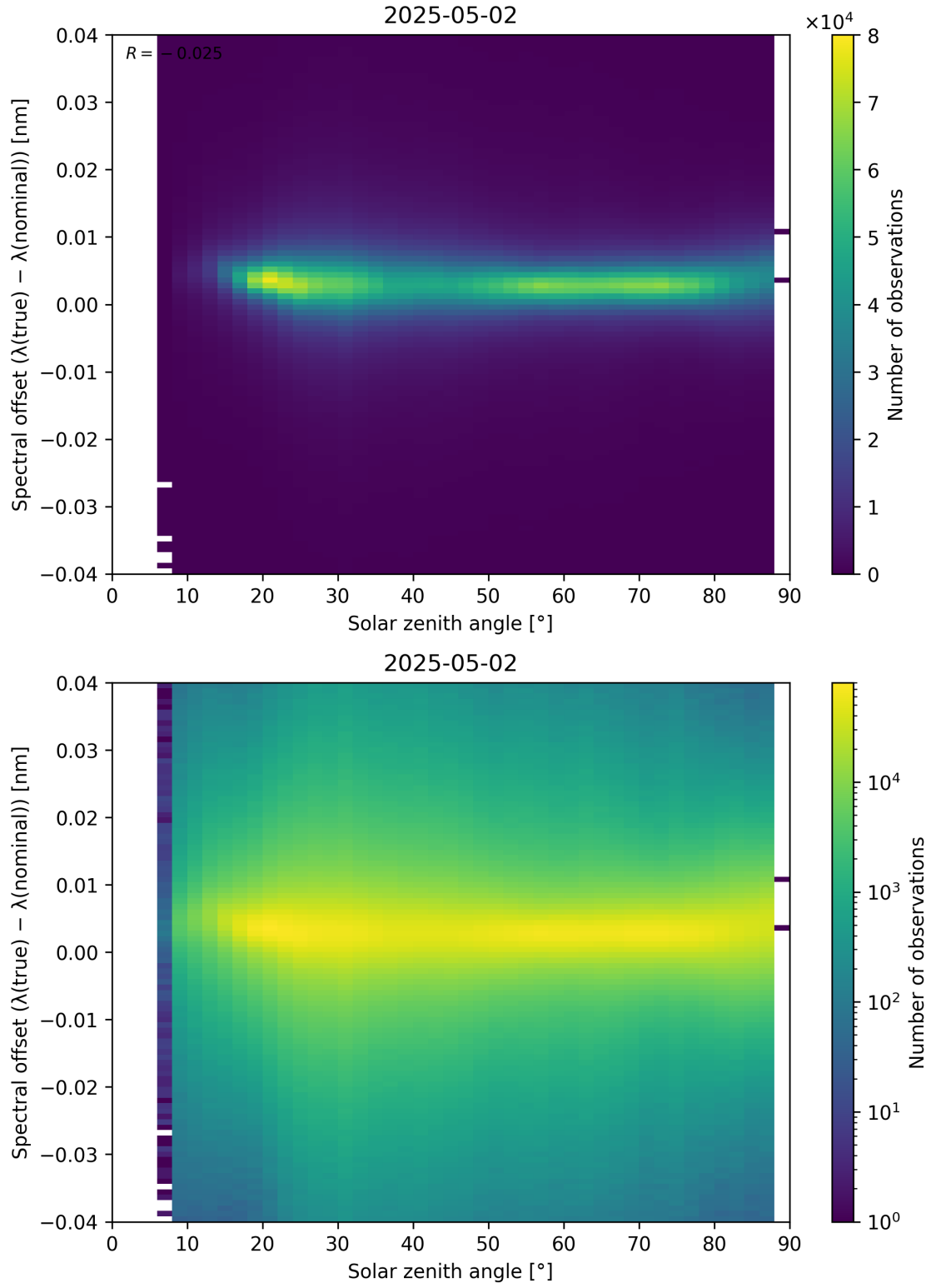
Figure 117: Scatter density plot of “Solar zenith angle” against “Spectral offset ( \lambda_{\text{true}} - \lambda_{\text{nominal}} )” for 2025-05-01 to 2025-05-03.
