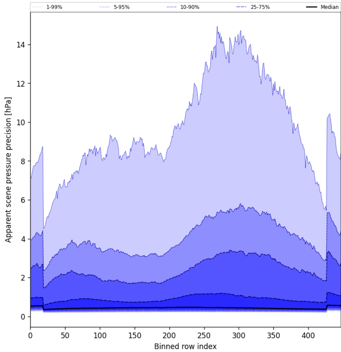
Figure 54: Along track statistics of “Apparent scene pressure precision” for 2025-05-01 to 2025-05-03
