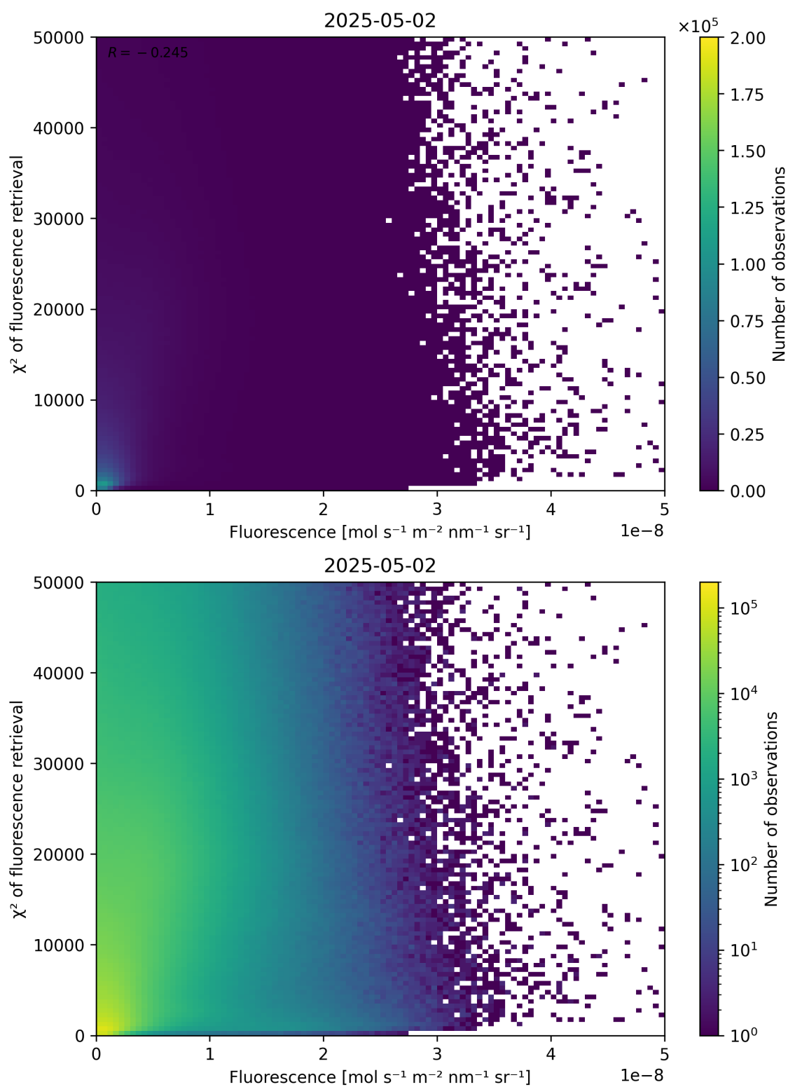
Figure 85: Scatter density plot of “Fluorescence” against “ \chi^2 of fluorescence retrieval” for 2025-05-01 to 2025-05-03.
