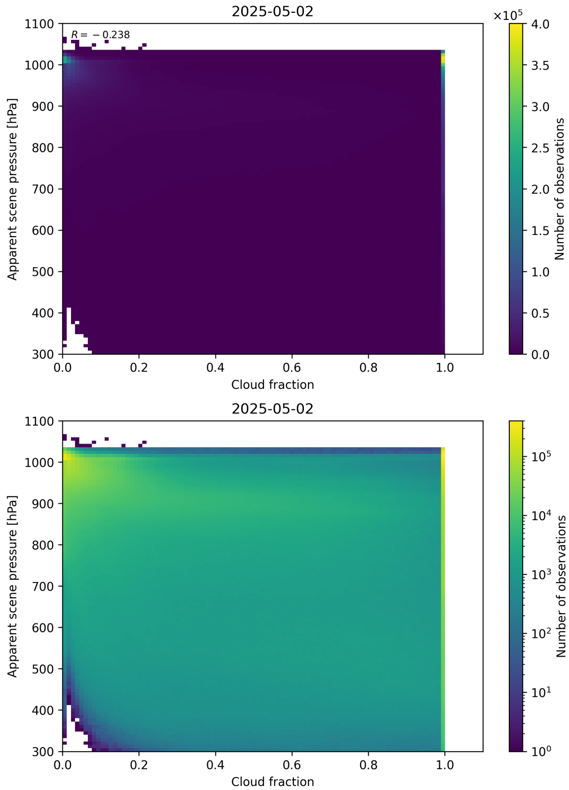
Figure 70: Scatter density plot of “Cloud fraction” against “Apparent scene pressure” for 2025-05-01 to 2025-05-03.
