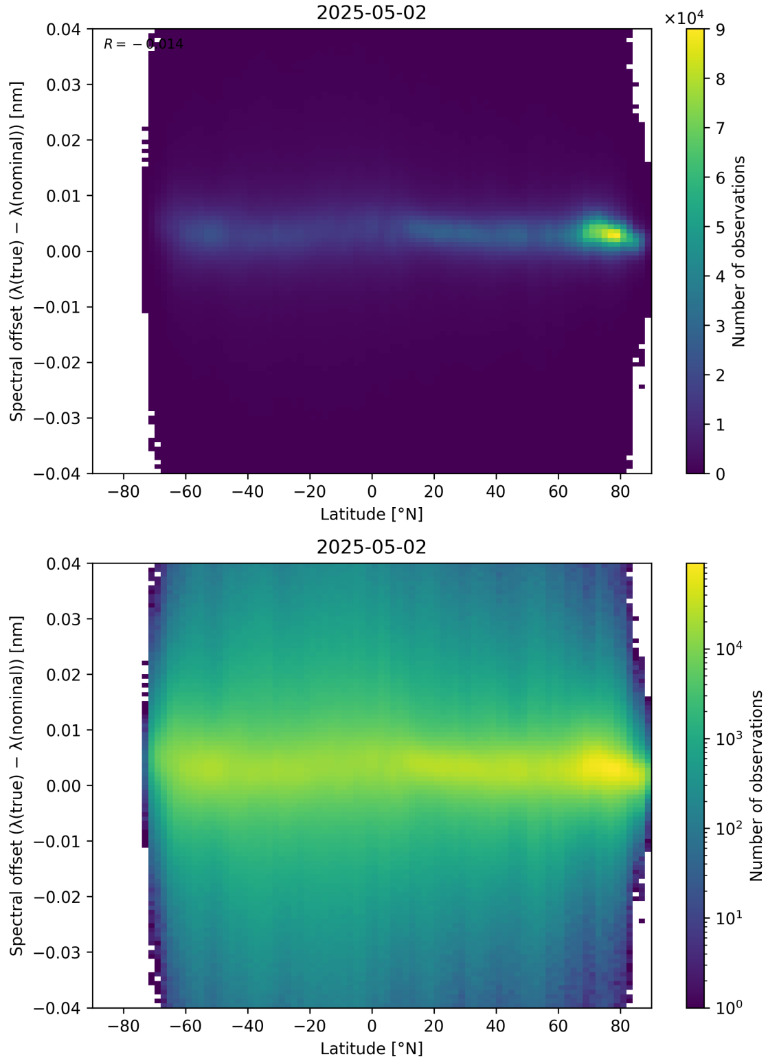
Figure 96: Scatter density plot of “Latitude” against “Spectral offset ( \lambda_{\text{true}} - \lambda_{\text{nominal}} )” for 2025-05-01 to 2025-05-03.
