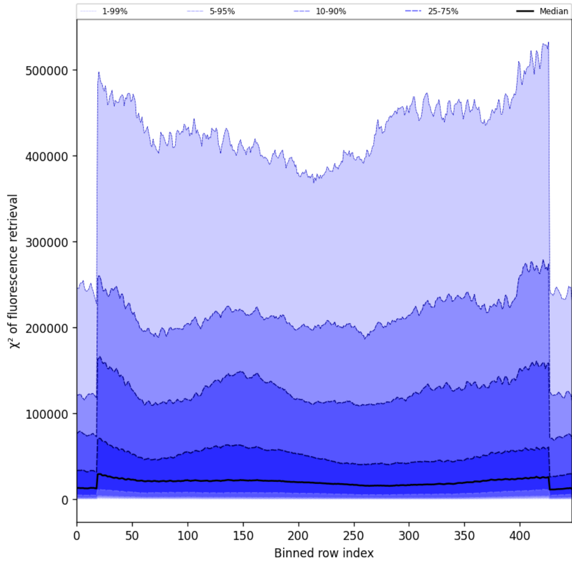
Figure 59: Along track statistics of “ \chi^2 of fluorescence retrieval” for 2025-05-01 to 2025-05-03
