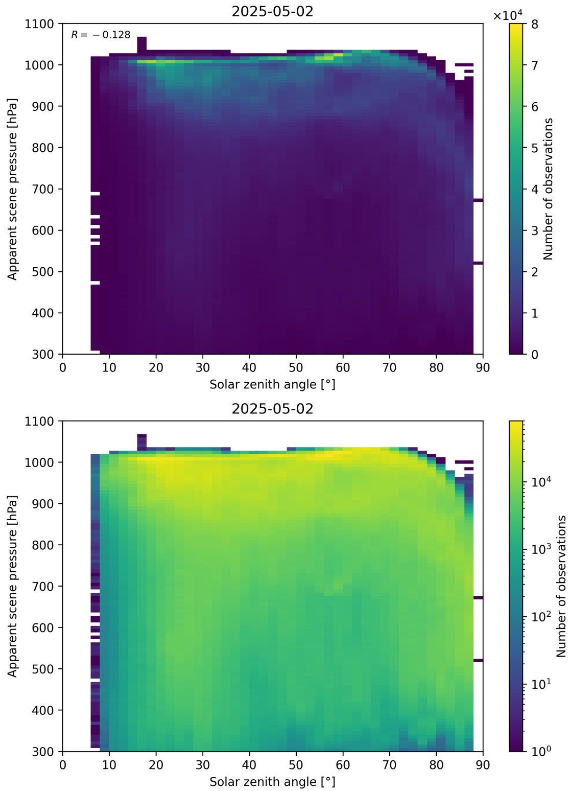
Figure 108: Scatter density plot of “Solar zenith angle” against “Apparent scene pressure” for 2025-05-01 to 2025-05-03.
