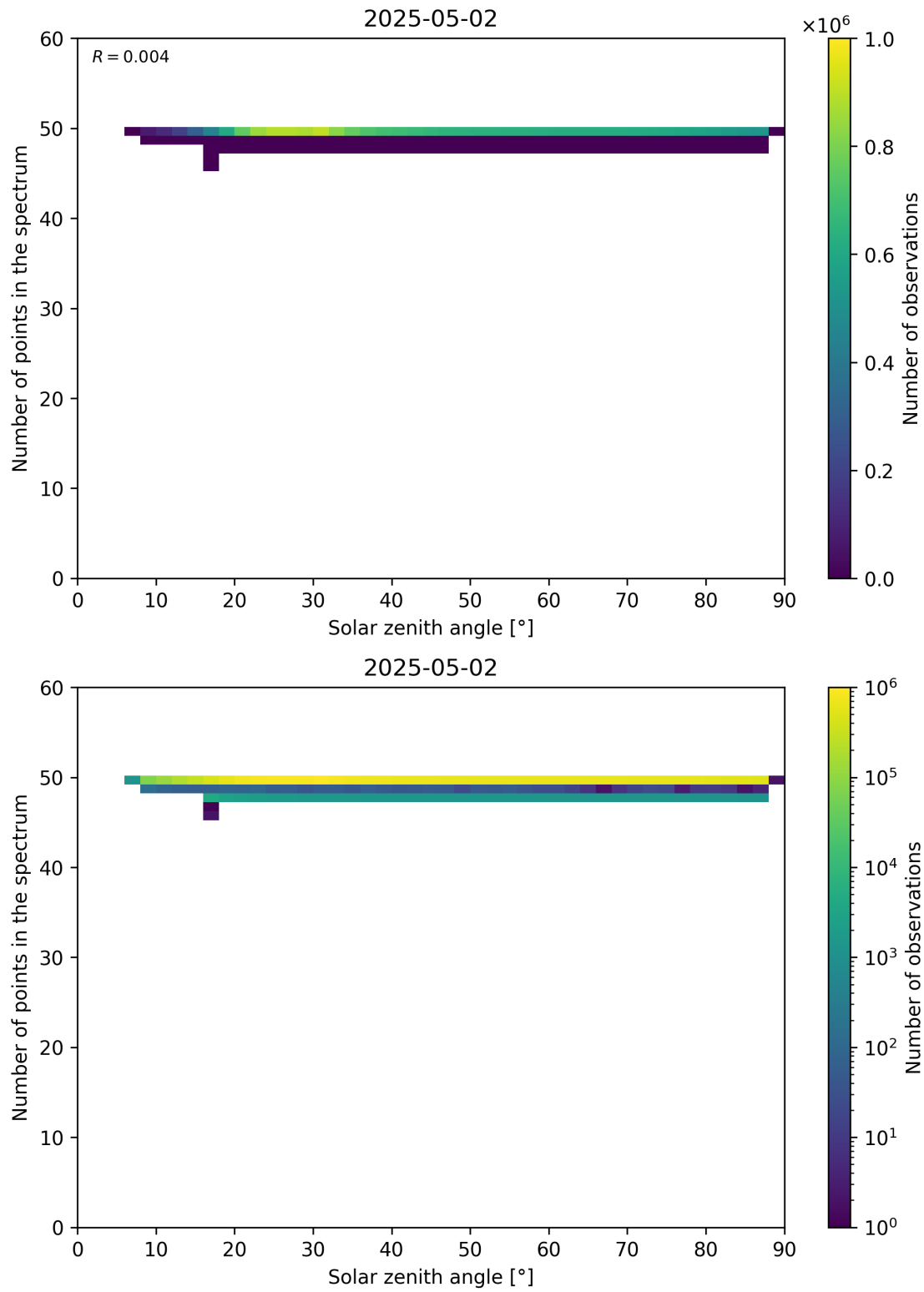
Figure 115: Scatter density plot of “Solar zenith angle” against “Number of points in the spectrum” for 2025-05-01 to 2025-05-03.
