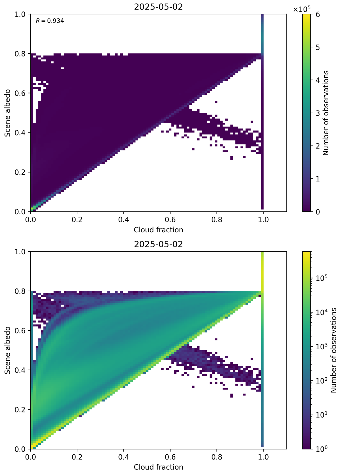
Figure 75: Scatter density plot of “Cloud fraction” against “Scene albedo” for 2025-05-01 to 2025-05-03.
