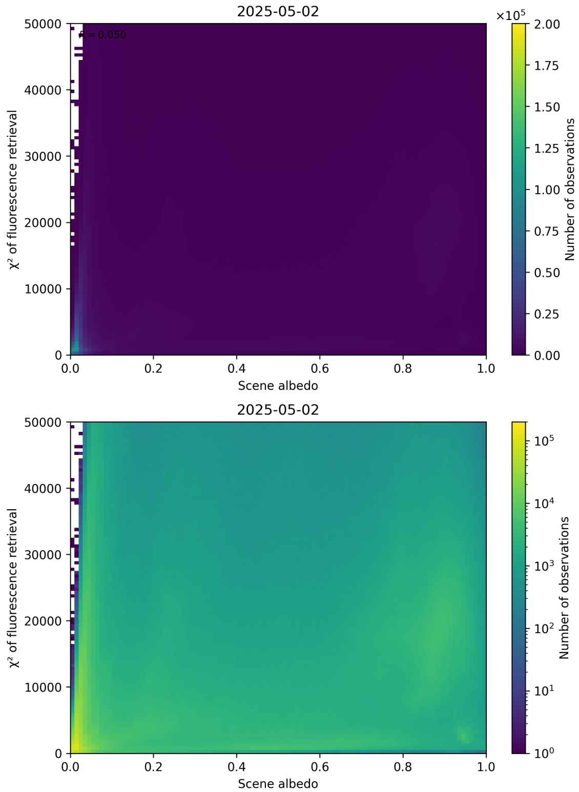
Figure 103: Scatter density plot of “Scene albedo” against “ \chi^2 of fluorescence retrieval” for 2025-05-01 to 2025-05-03.
