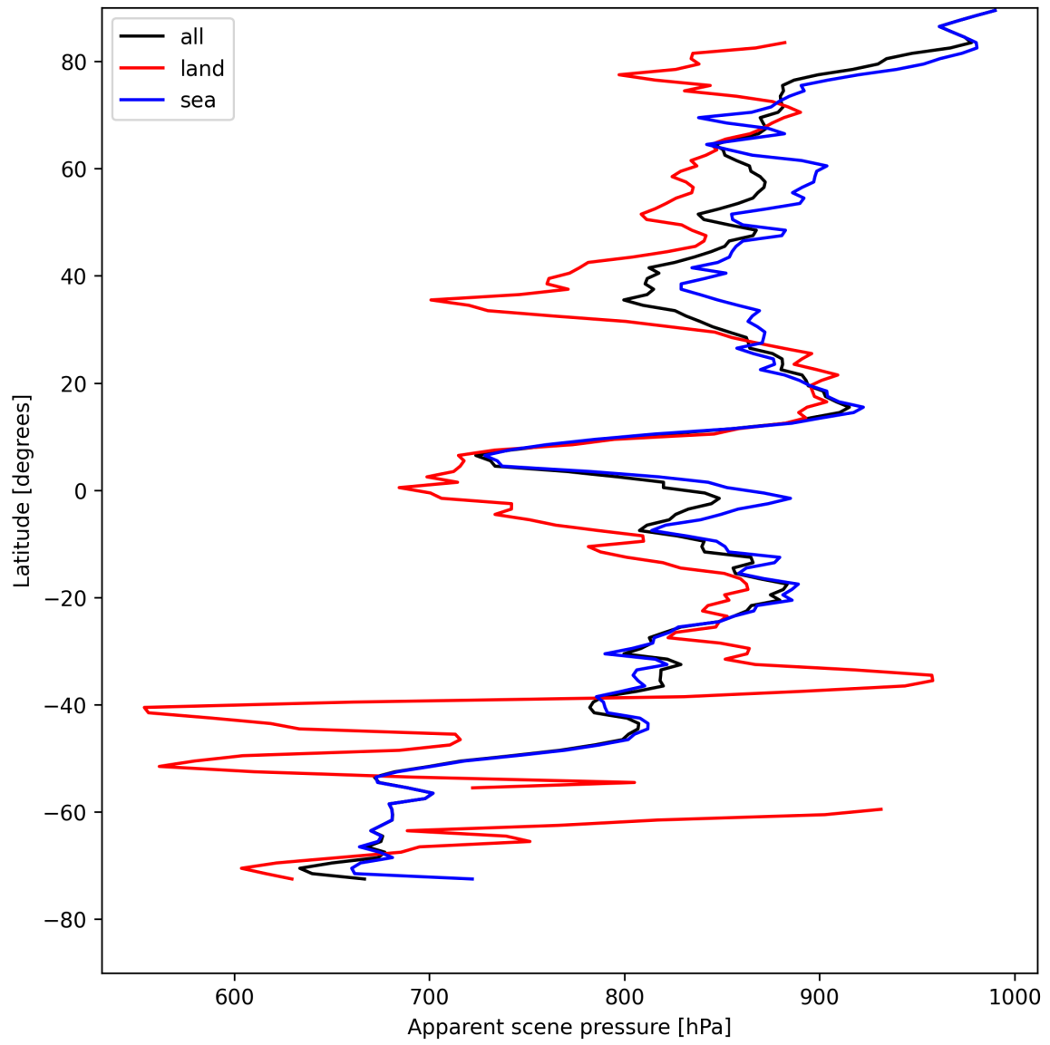
Figure 19: Zonal average of “Apparent scene pressure” for 2025-05-01 to 2025-05-03.
