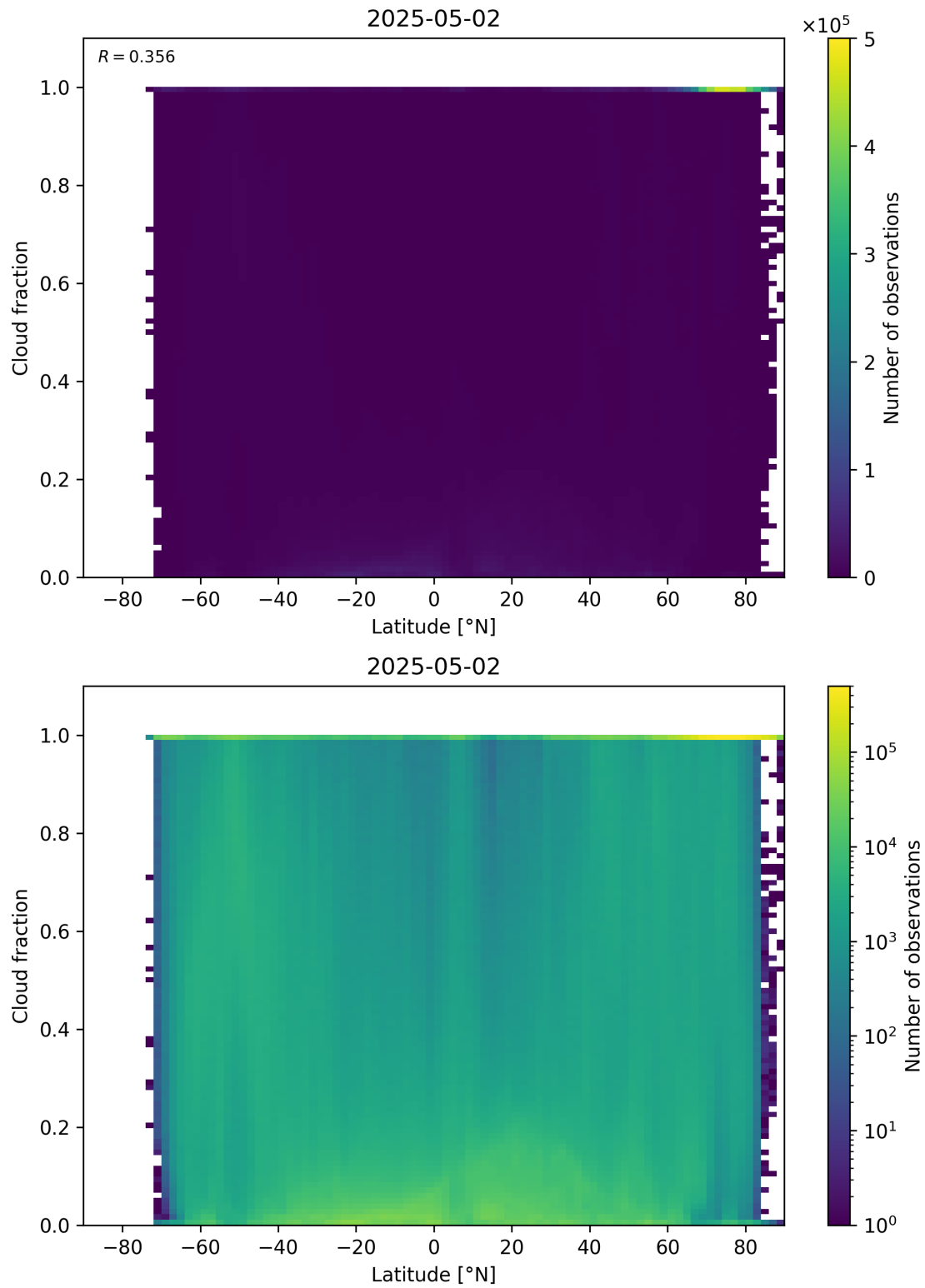
Figure 90: Scatter density plot of “Latitude” against “Cloud fraction” for 2025-05-01 to 2025-05-03.
