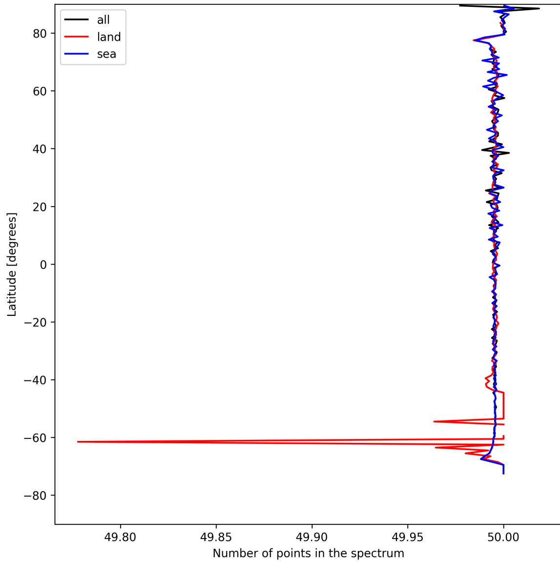
Figure 27: Zonal average of “Number of points in the spectrum” for 2025-05-01 to 2025-05-03.
