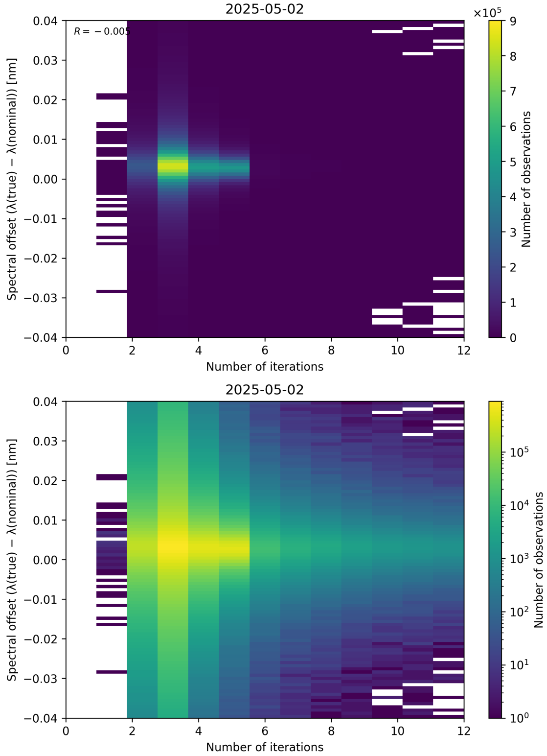
Figure 100: Scatter density plot of “Number of iterations” against “Spectral offset ( \lambda_{\text{true}} - \lambda_{\text{nominal}} )” for 2025-05-01 to 2025-05-03.
