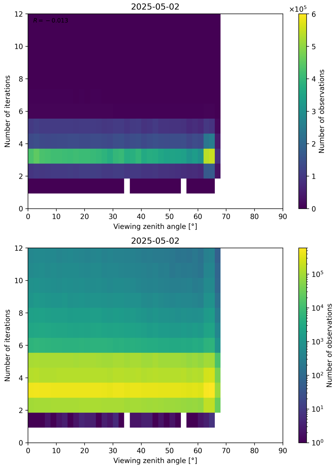
Figure 124: Scatter density plot of “Viewing zenith angle” against “Number of iterations” for 2025-05-01 to 2025-05-03.
