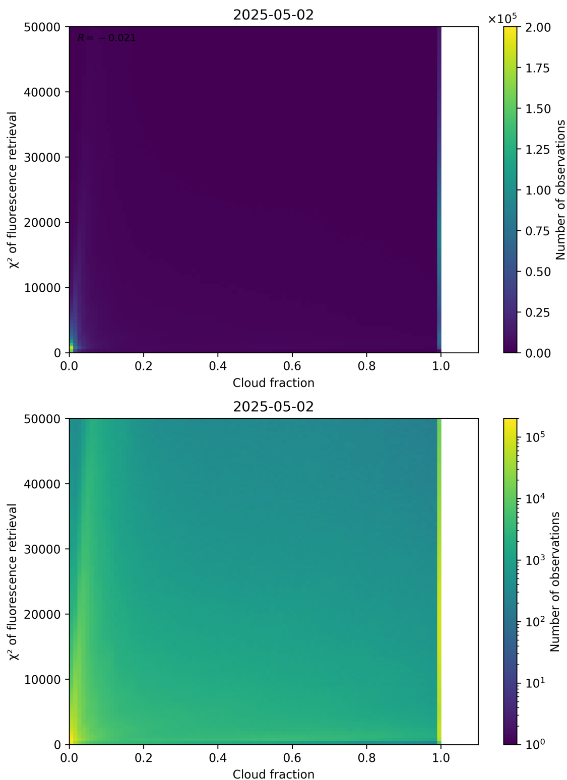
Figure 71: Scatter density plot of “Cloud fraction” against “ \chi^2 of fluorescence retrieval” for 2025-05-01 to 2025-05-03.
