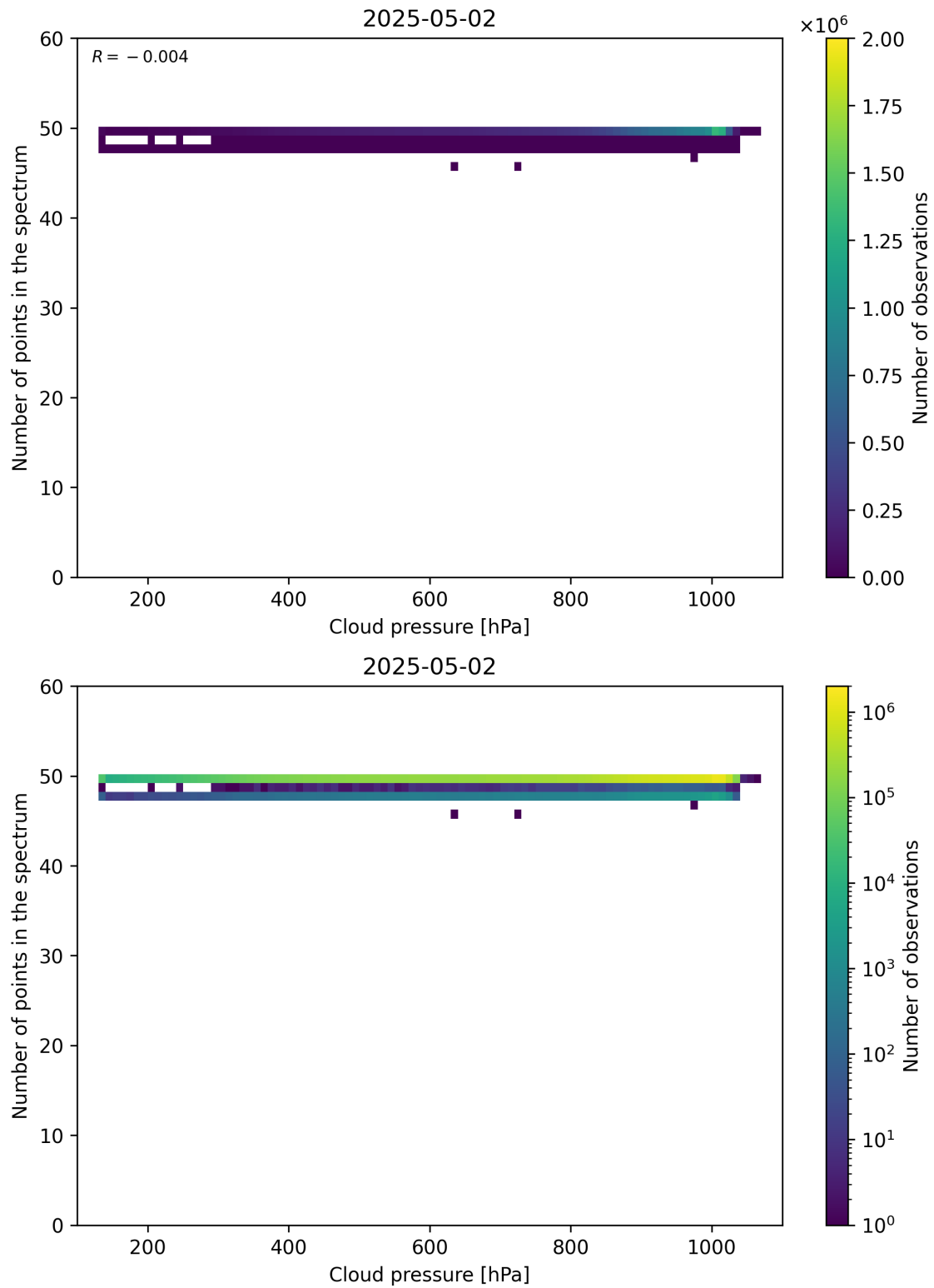
Figure 82: Scatter density plot of “Cloud pressure” against “Number of points in the spectrum” for 2025-05-01 to 2025-05-03.
