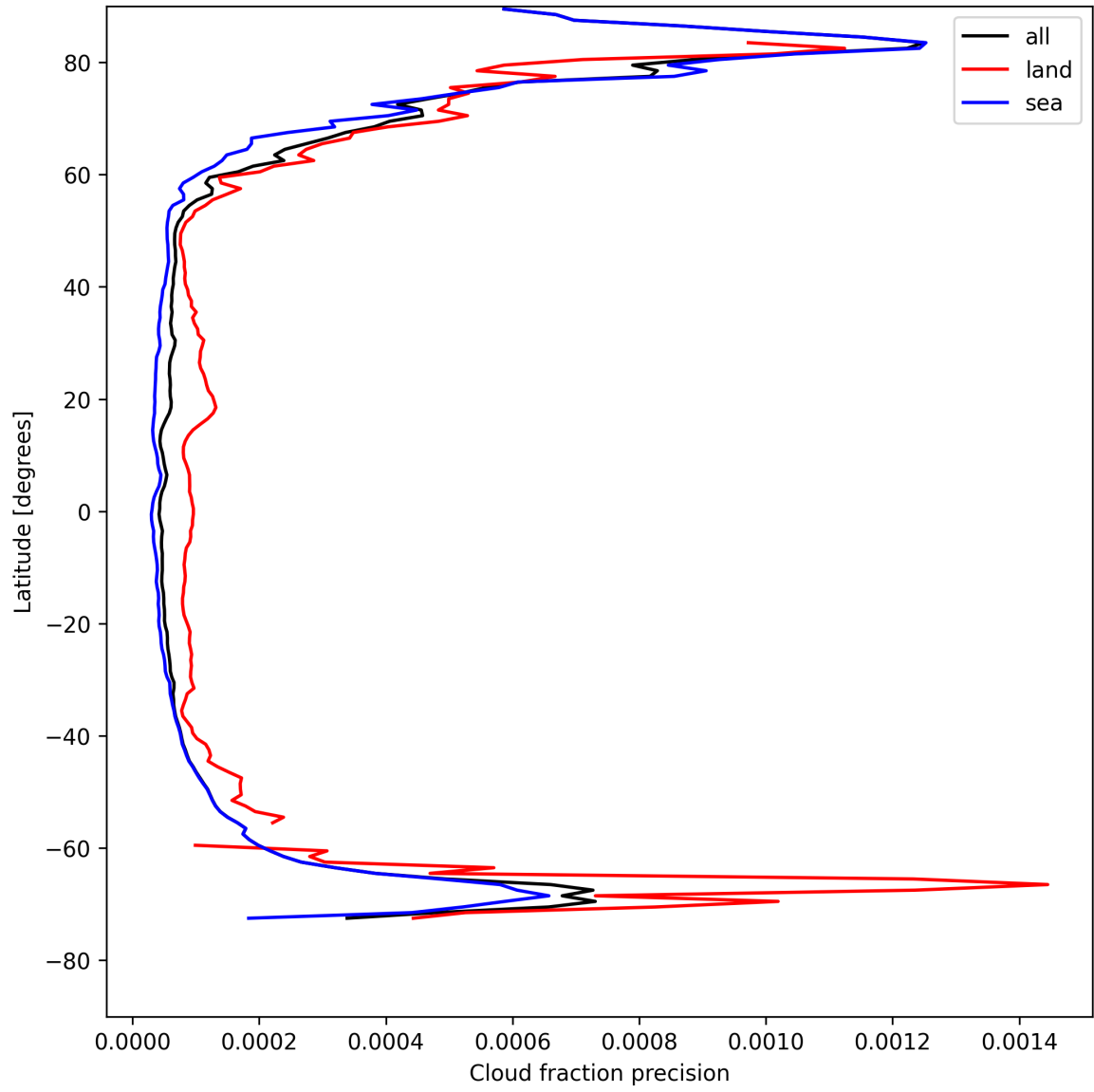
Figure 16: Zonal average of “Cloud fraction precision” for 2025-05-01 to 2025-05-03.
