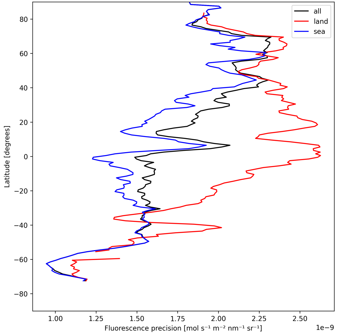
Figure 24: Zonal average of “Fluorescence precision” for 2025-05-01 to 2025-05-03.
