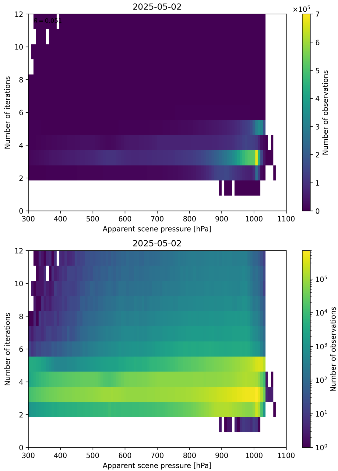
Figure 65: Scatter density plot of “Apparent scene pressure” against “Number of iterations” for 2025-05-01 to 2025-05-03.
