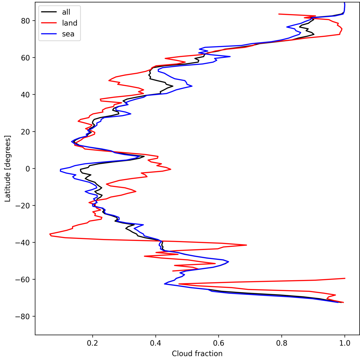
Figure 15: Zonal average of “Cloud fraction” for 2025-05-01 to 2025-05-03.
