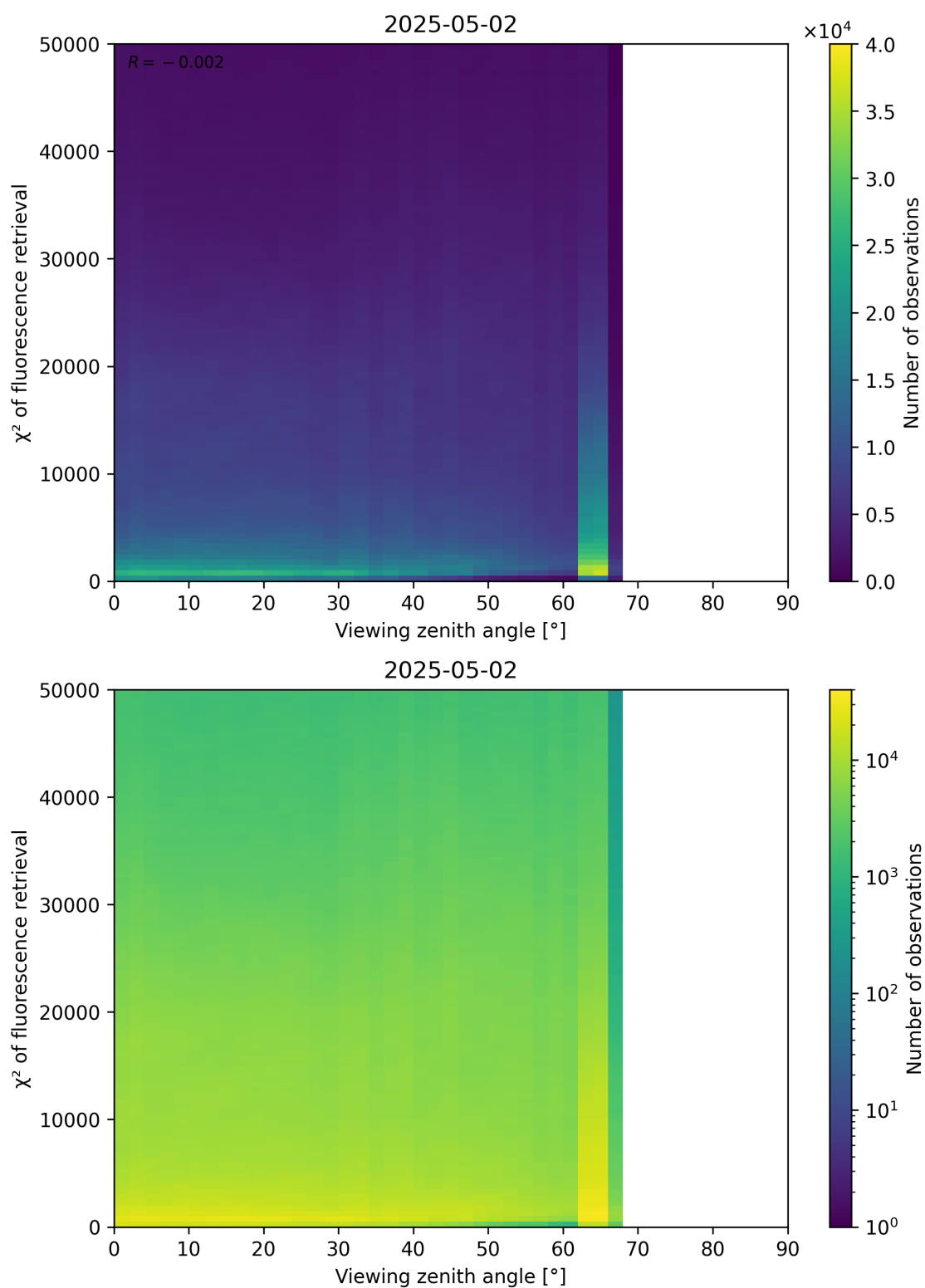
Figure 119: Scatter density plot of “Viewing zenith angle” against “ \chi^2 of fluorescence retrieval” for 2025-05-01 to 2025-05-03.
