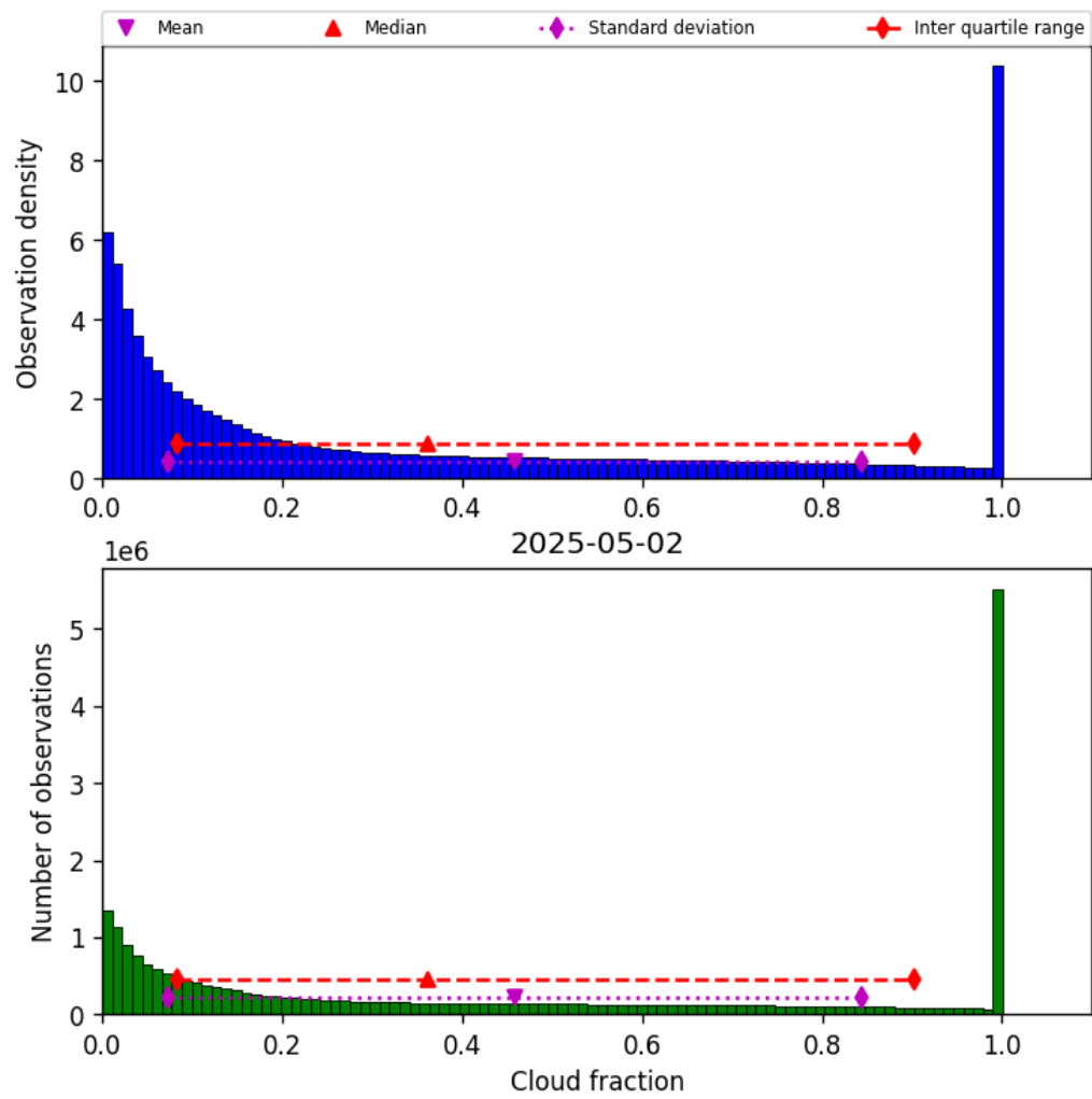
Figure 32: Histogram of “Cloud fraction” for 2025-05-01 to 2025-05-03
