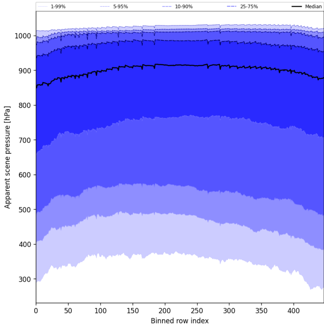
Figure 53: Along track statistics of “Apparent scene pressure” for 2025-05-01 to 2025-05-03
