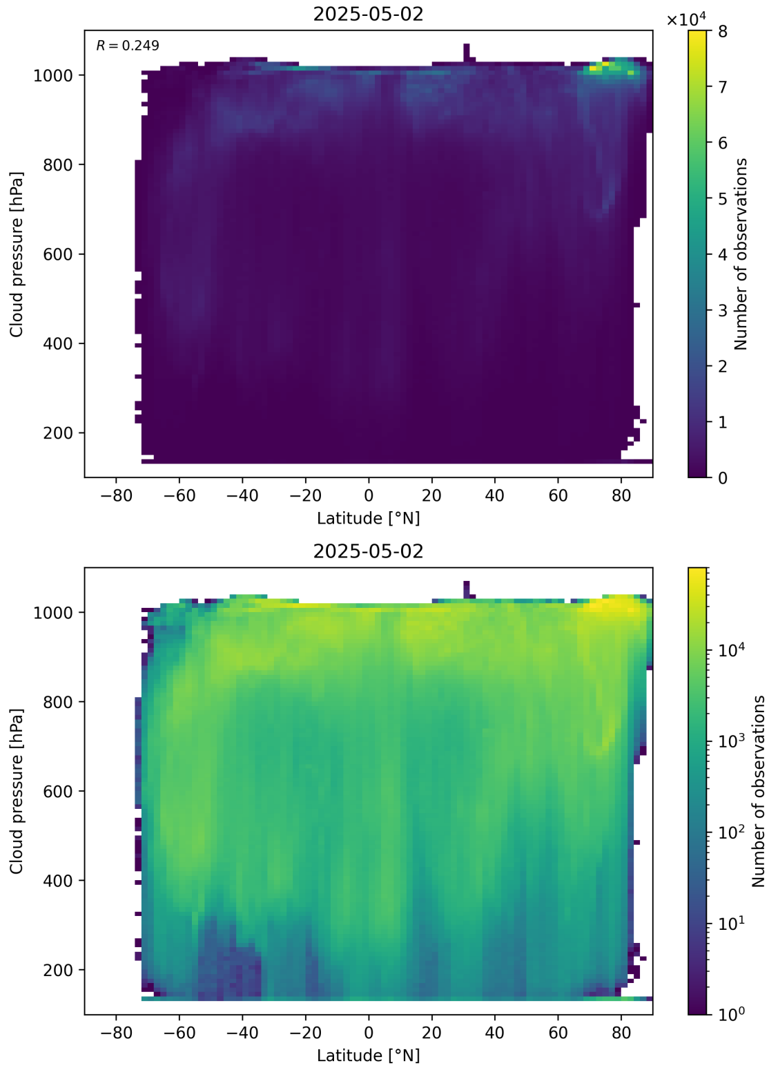
Figure 91: Scatter density plot of “Latitude” against “Cloud pressure” for 2025-05-01 to 2025-05-03.
