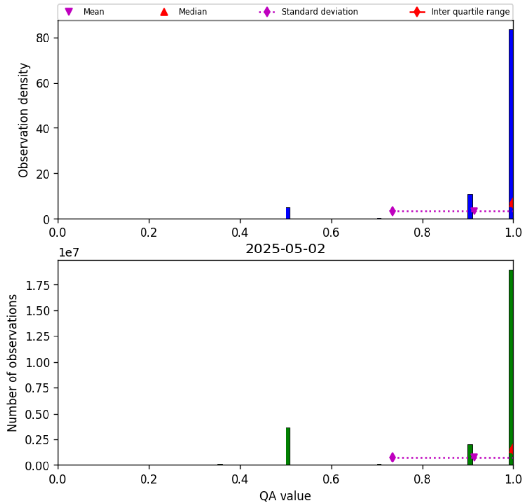
Figure 29: Histogram of “QA value” for 2025-05-01 to 2025-05-03
