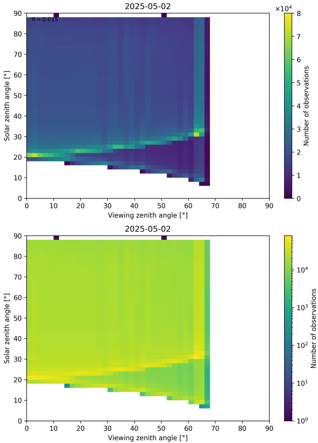
Figure 127: Scatter density plot of “Viewing zenith angle” against “Solar zenith angle” for 2025-05-01 to 2025-05-03.
