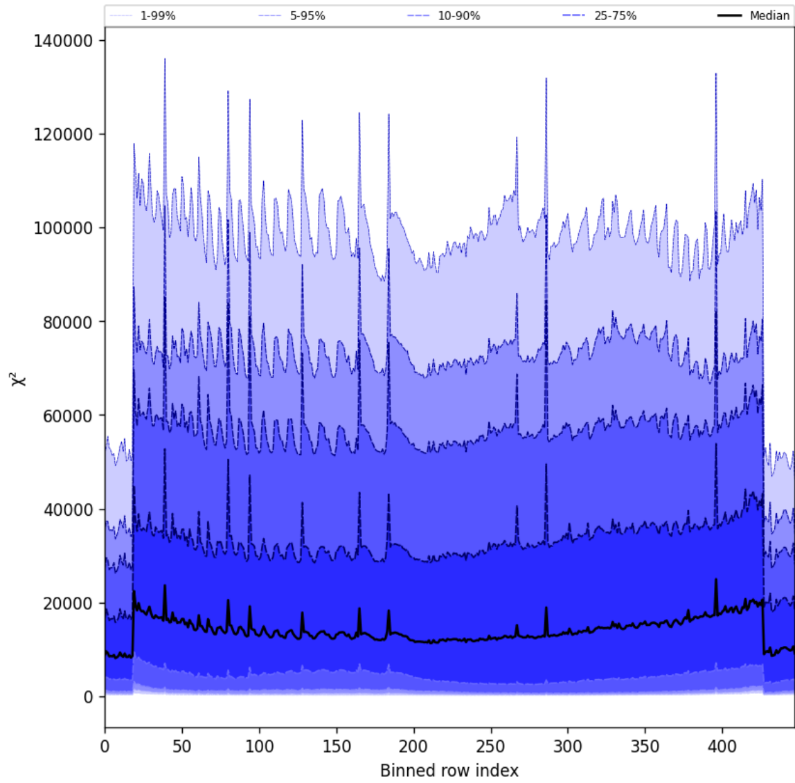
Figure 55: Along track statistics of “ \chi^2 ” for 2025-05-01 to 2025-05-03
