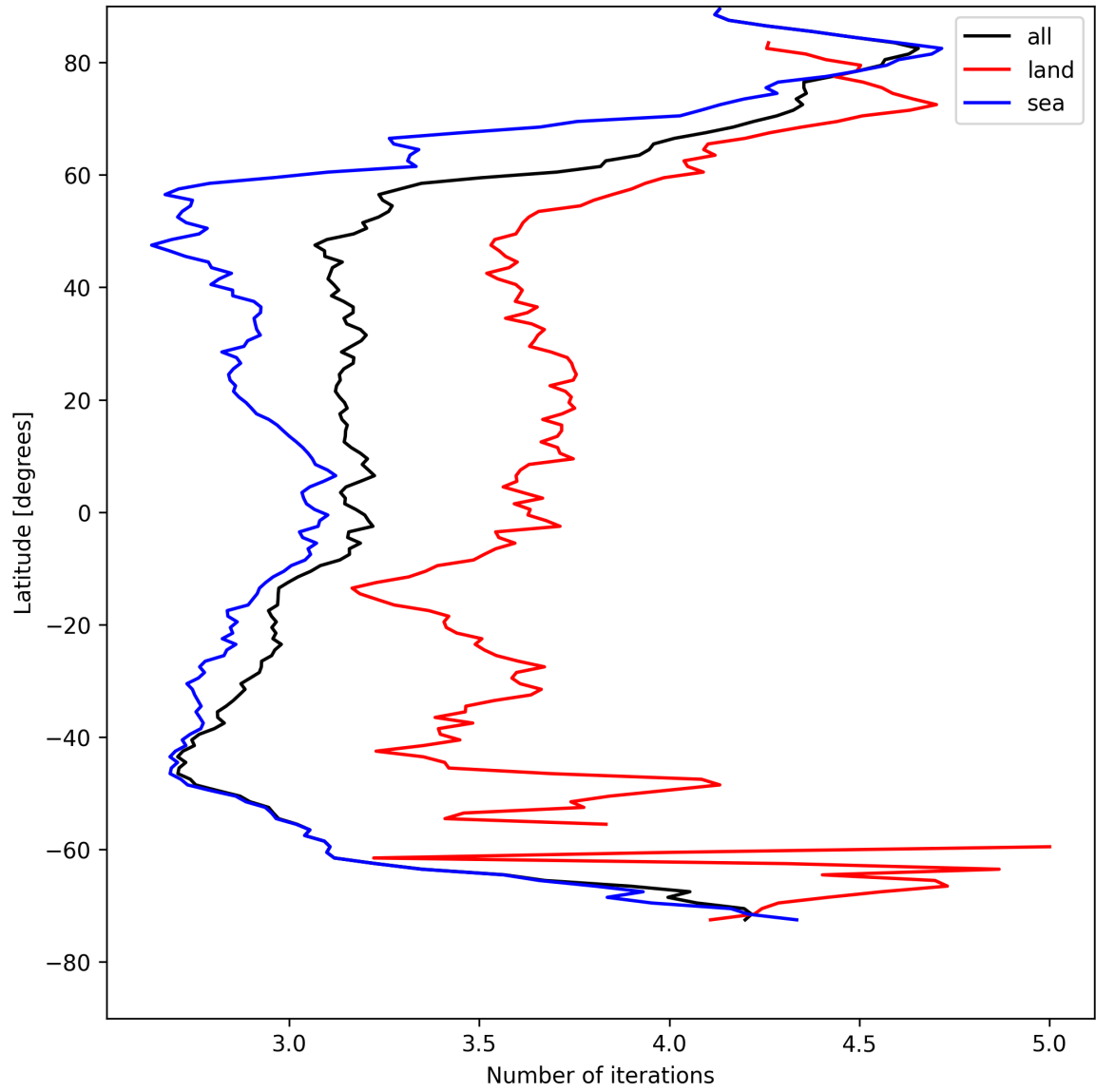
Figure 22: Zonal average of “Number of iterations” for 2025-05-01 to 2025-05-03.
