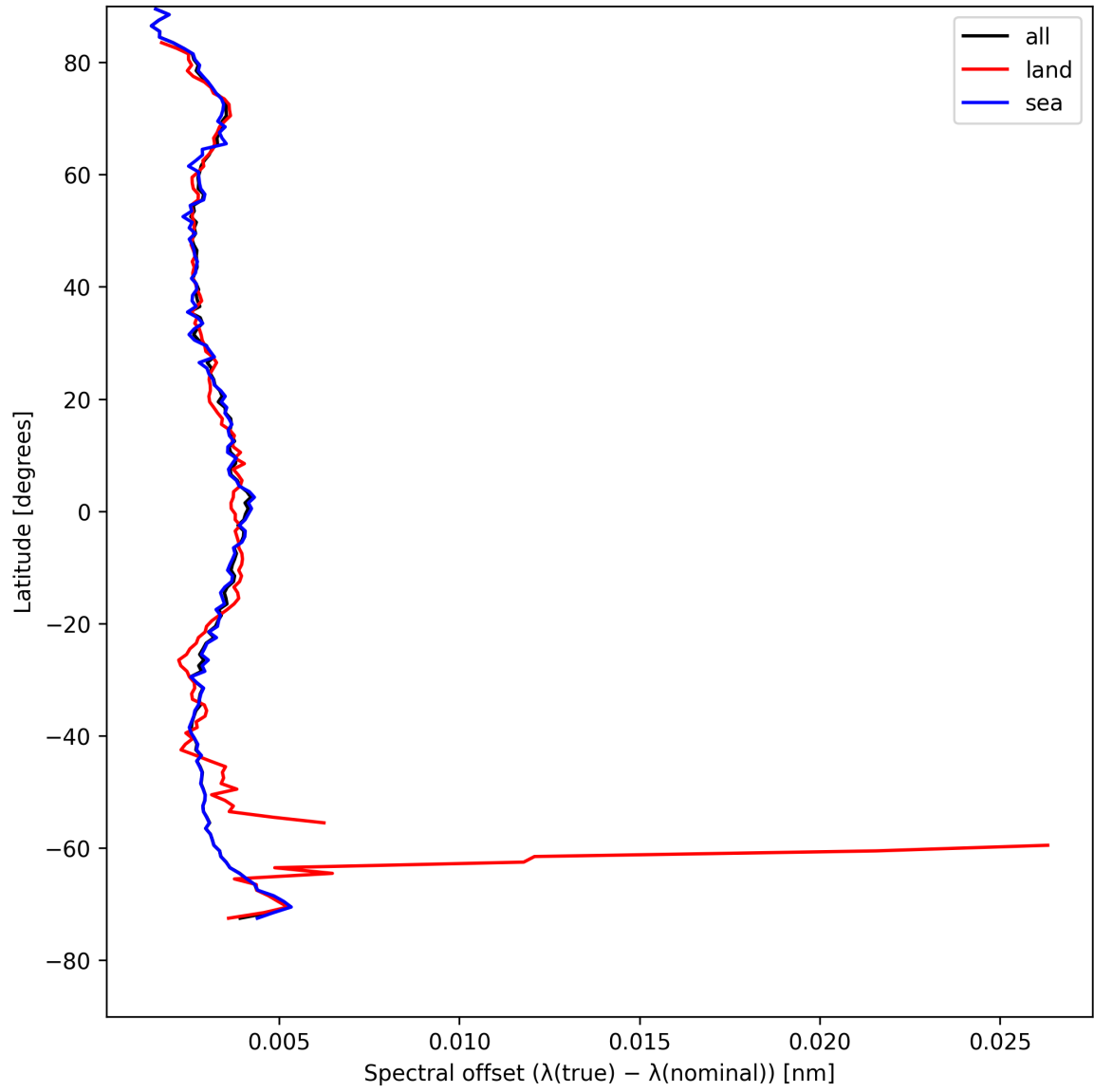
Figure 28: Zonal average of “Spectral offset ( \lambda_{\text{true}} - \lambda_{\text{nominal}} )” for 2025-05-01 to 2025-05-03.
