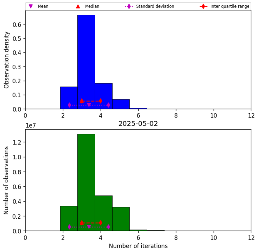
Figure 39: Histogram of “Number of iterations” for 2025-05-01 to 2025-05-03
