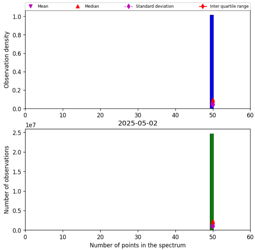
Figure 44: Histogram of “Number of points in the spectrum” for 2025-05-01 to 2025-05-03
