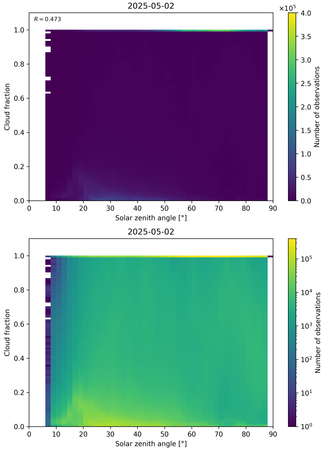
Figure 110: Scatter density plot of “Solar zenith angle” against “Cloud fraction” for 2025-05-01 to 2025-05-03.
