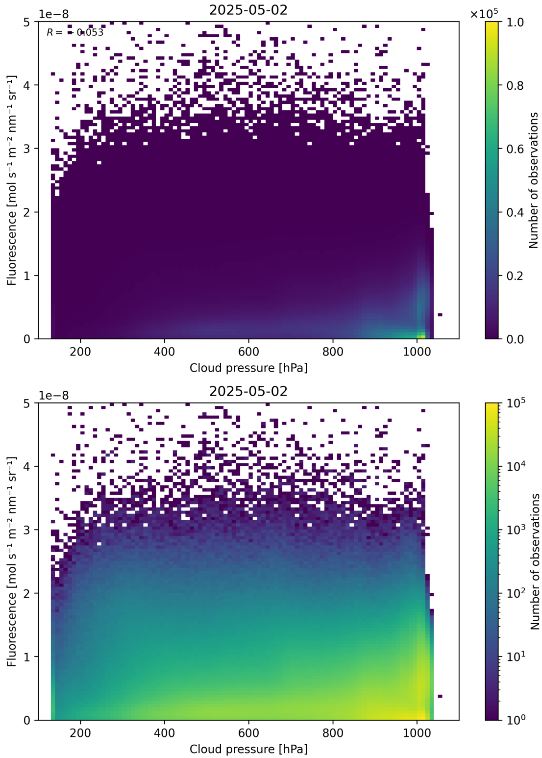
Figure 80: Scatter density plot of “Cloud pressure” against “Fluorescence” for 2025-05-01 to 2025-05-03.
