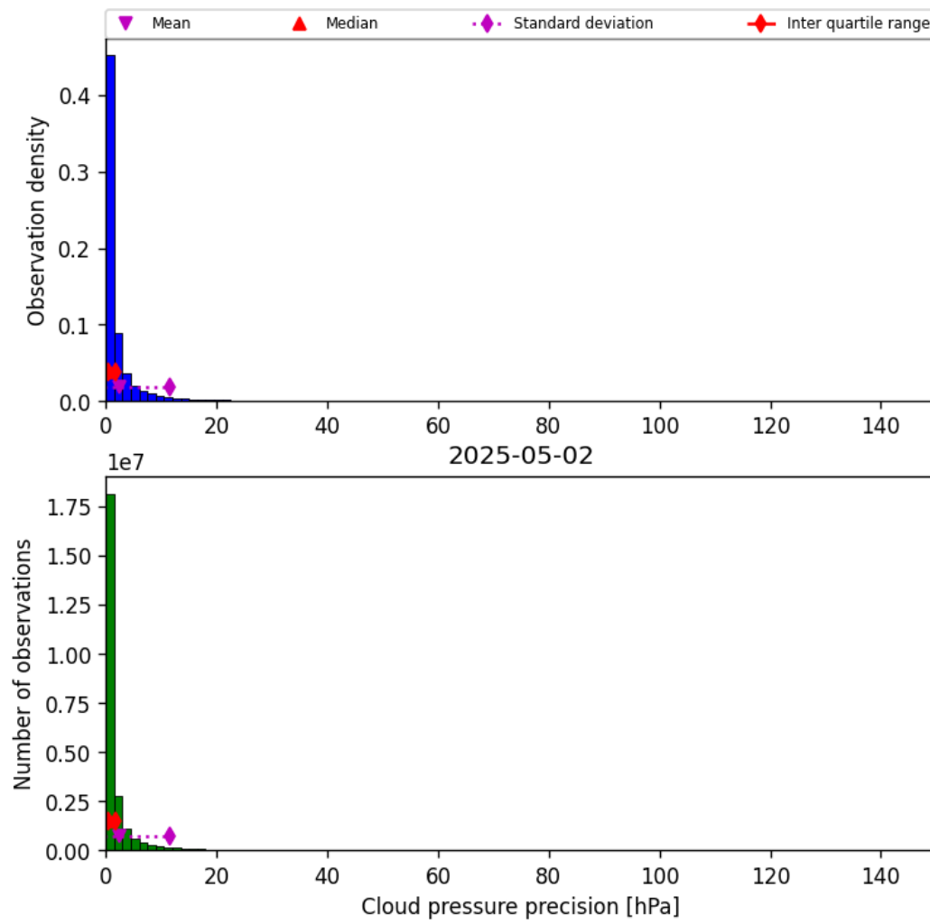
Figure 31: Histogram of “Cloud pressure precision” for 2025-05-01 to 2025-05-03
