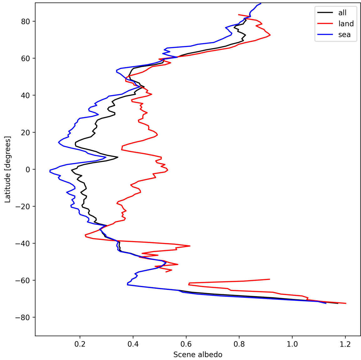
Figure 17: Zonal average of “Scene albedo” for 2025-05-01 to 2025-05-03.
