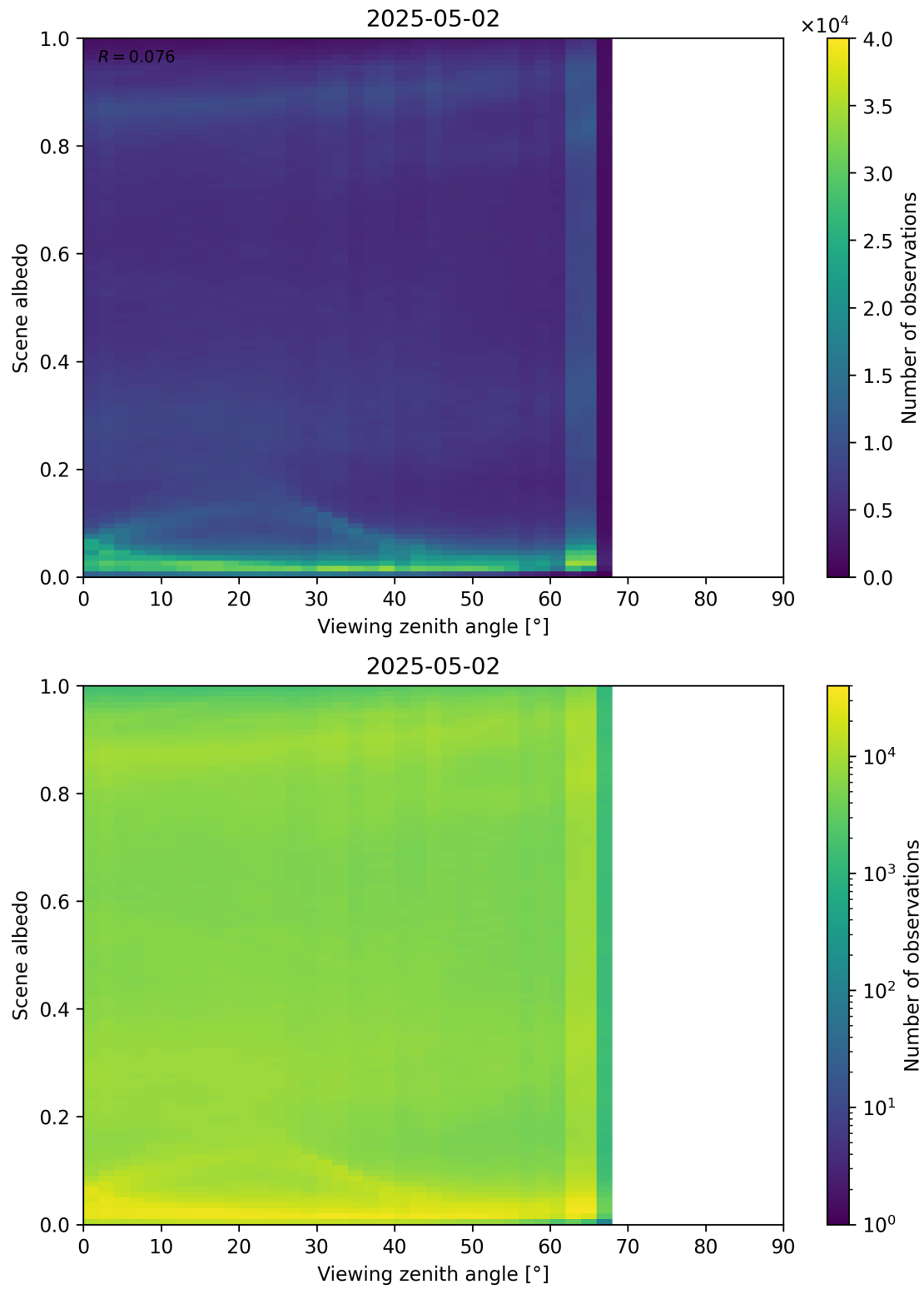
Figure 126: Scatter density plot of “Viewing zenith angle” against “Scene albedo” for 2025-05-01 to 2025-05-03.
