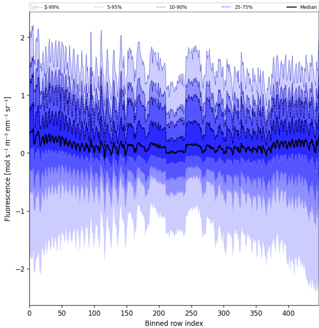
Figure 57: Along track statistics of “Fluorescence” for 2025-05-01 to 2025-05-03
