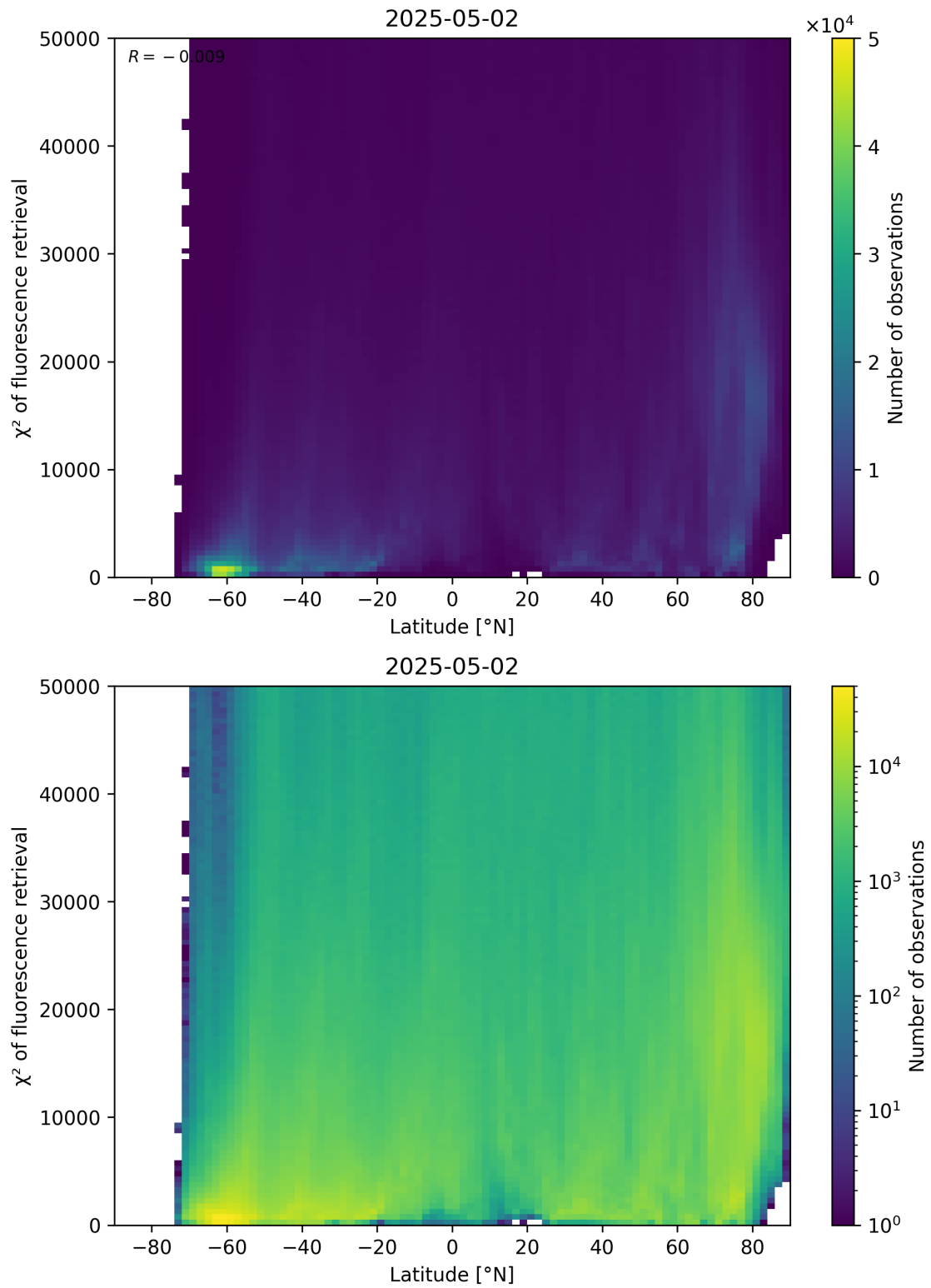
Figure 89: Scatter density plot of “Latitude” against “ \chi^2 of fluorescence retrieval” for 2025-05-01 to 2025-05-03.
