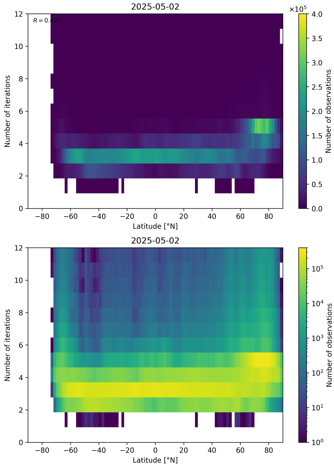
Figure 93: Scatter density plot of “Latitude” against “Number of iterations” for 2025-05-01 to 2025-05-03.
