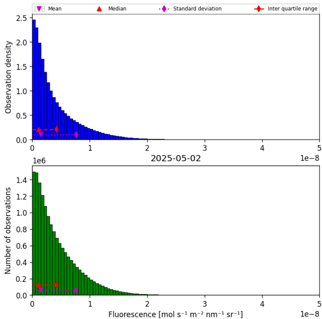
Figure 40: Histogram of “Fluorescence” for 2025-05-01 to 2025-05-03
