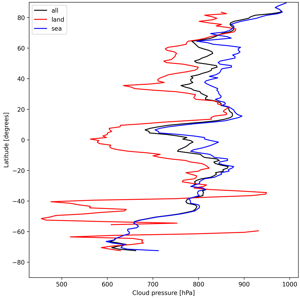
Figure 13: Zonal average of “Cloud pressure” for 2025-05-01 to 2025-05-03.
