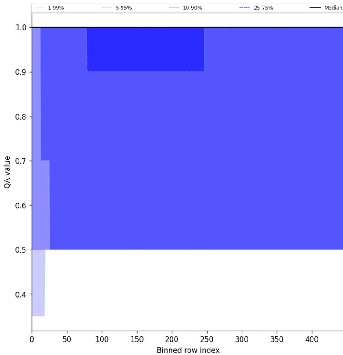
Figure 46: Along track statistics of “QA value” for 2025-05-01 to 2025-05-03
