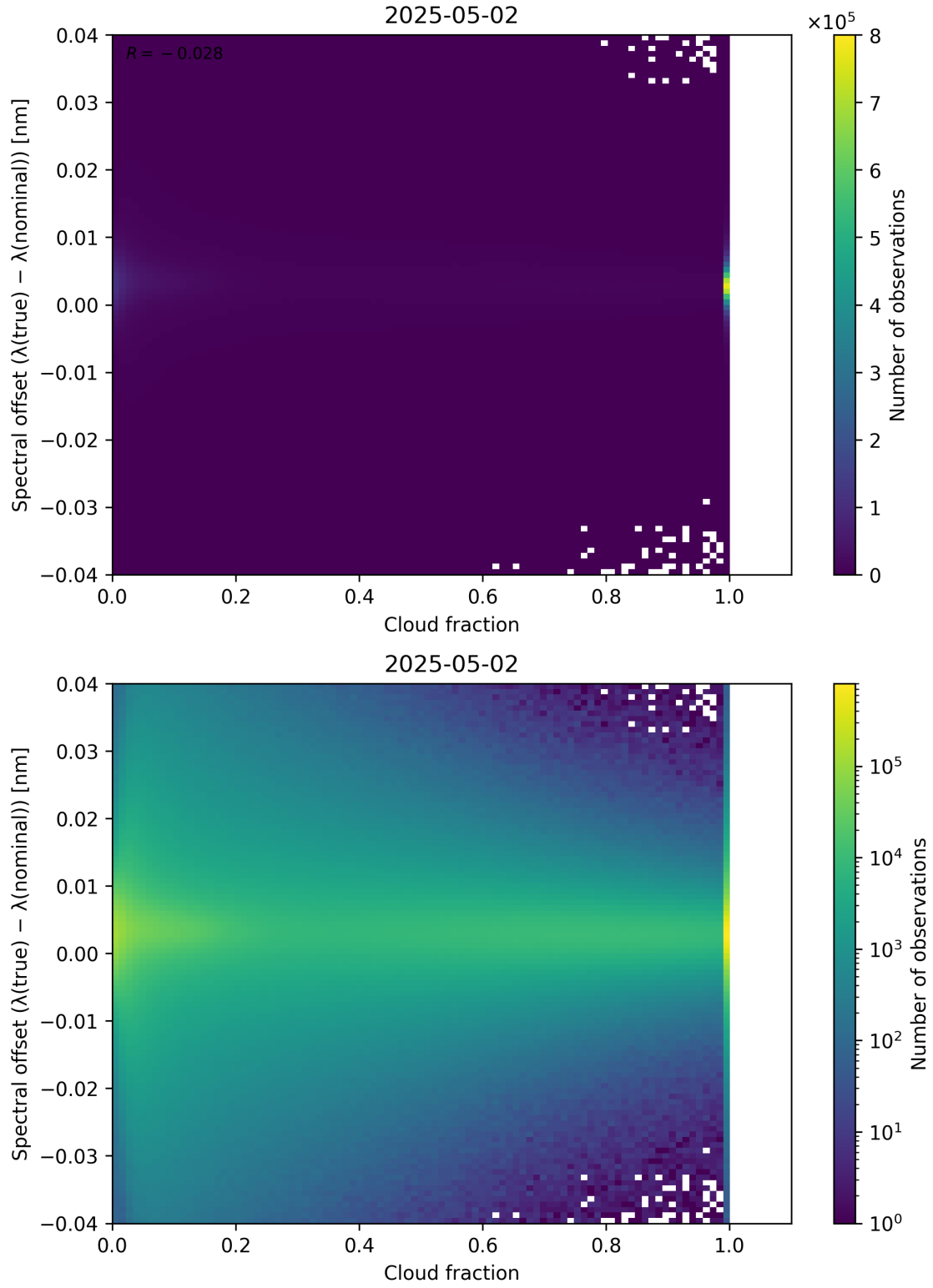
Figure 76: Scatter density plot of “Cloud fraction” against “Spectral offset ( \lambda_{\text{true}} - \lambda_{\text{nominal}} )” for 2025-05-01 to 2025-05-03.
