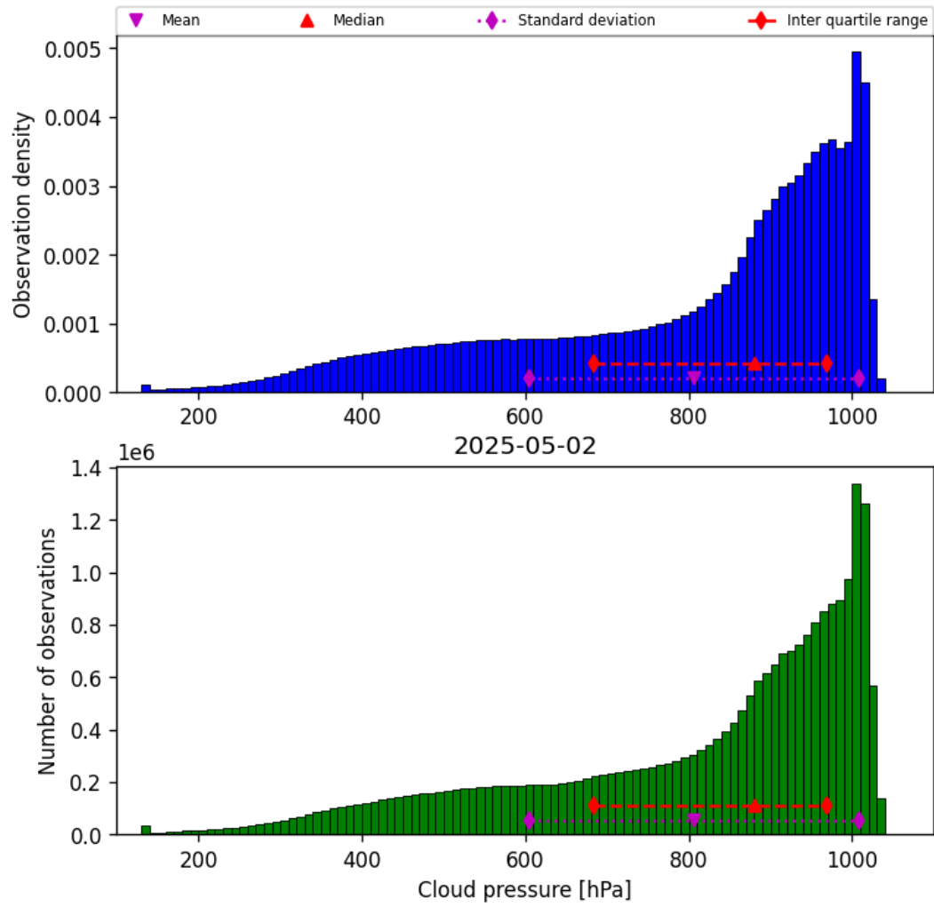
Figure 30: Histogram of “Cloud pressure” for 2025-05-01 to 2025-05-03
