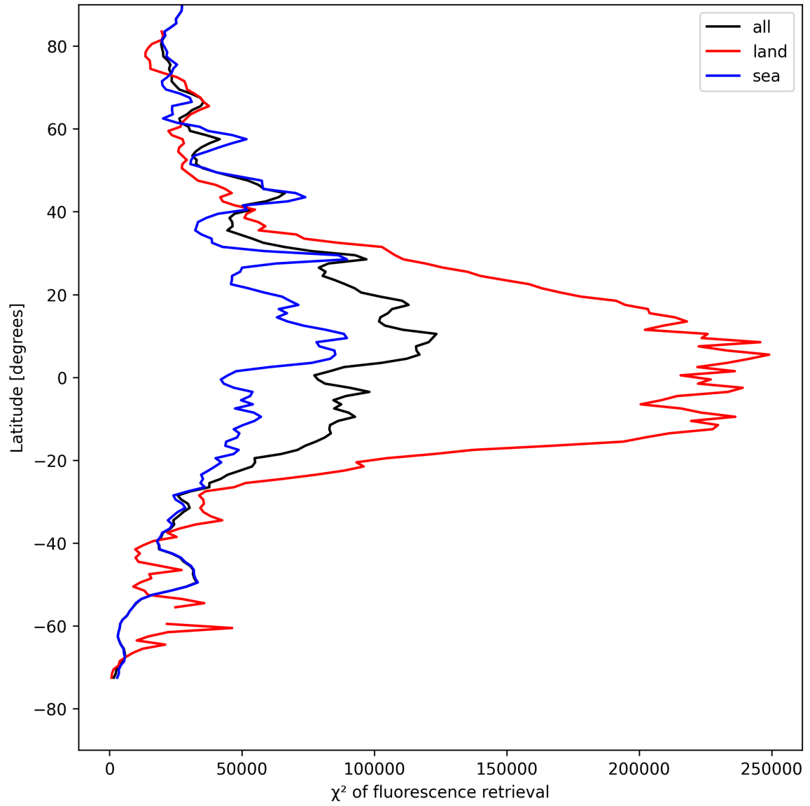
Figure 25: Zonal average of “ \chi^2 of fluorescence retrieval” for 2025-05-01 to 2025-05-03.
