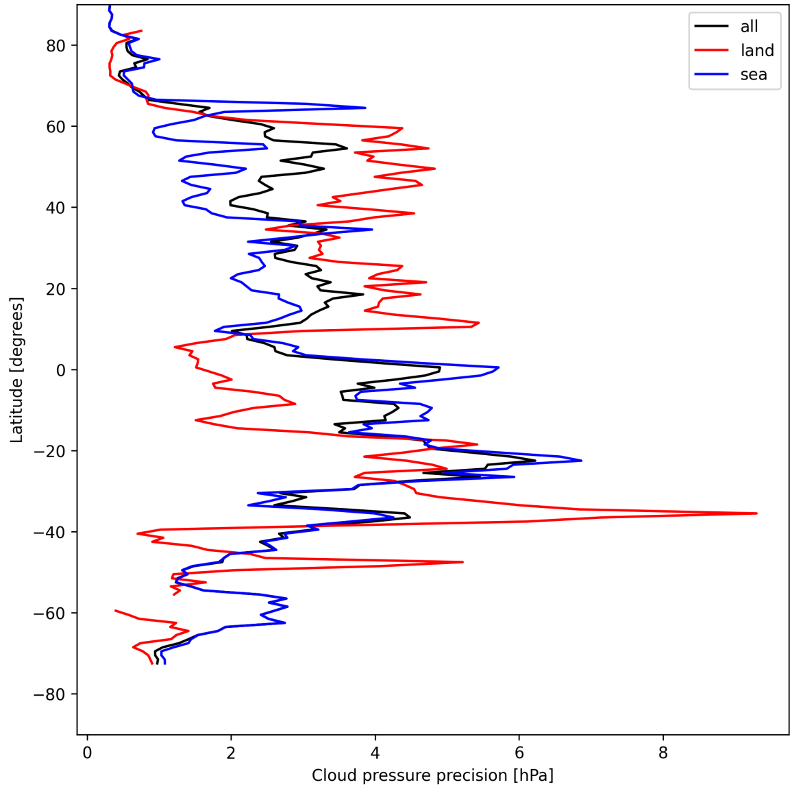
Figure 14: Zonal average of “Cloud pressure precision” for 2025-05-01 to 2025-05-03.
