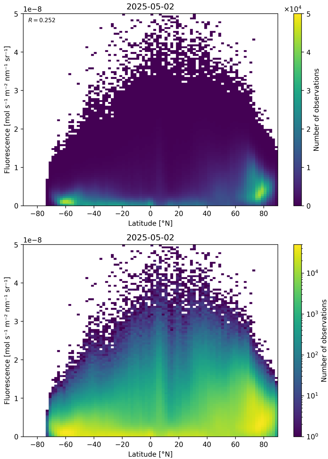
Figure 92: Scatter density plot of “Latitude” against “Fluorescence” for 2025-05-01 to 2025-05-03.
