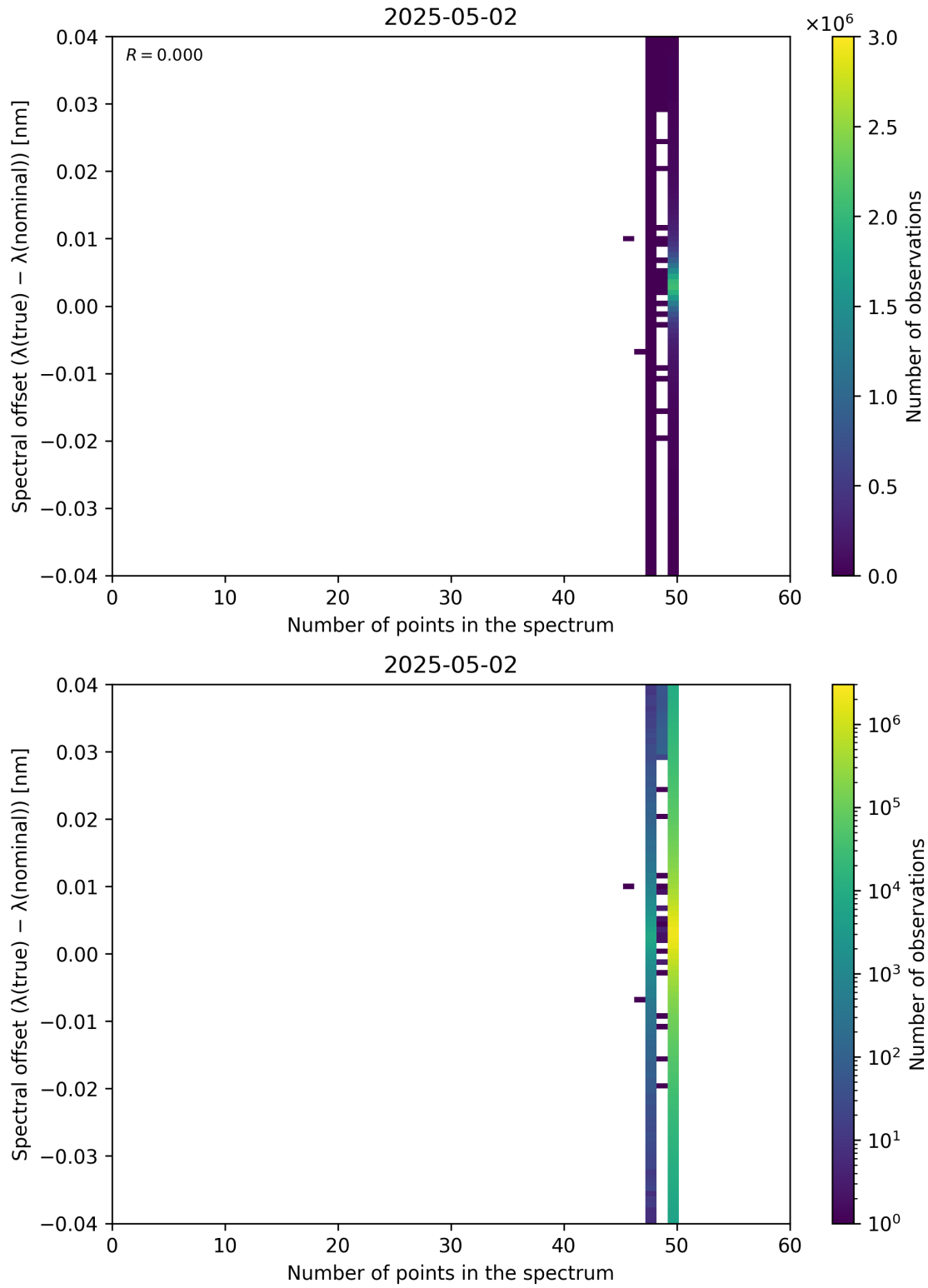
Figure 101: Scatter density plot of “Number of points in the spectrum” against “Spectral offset ( \lambda_{\text{true}} - \lambda_{\text{nominal}} )” for 2025-05-01 to 2025-05-03.
