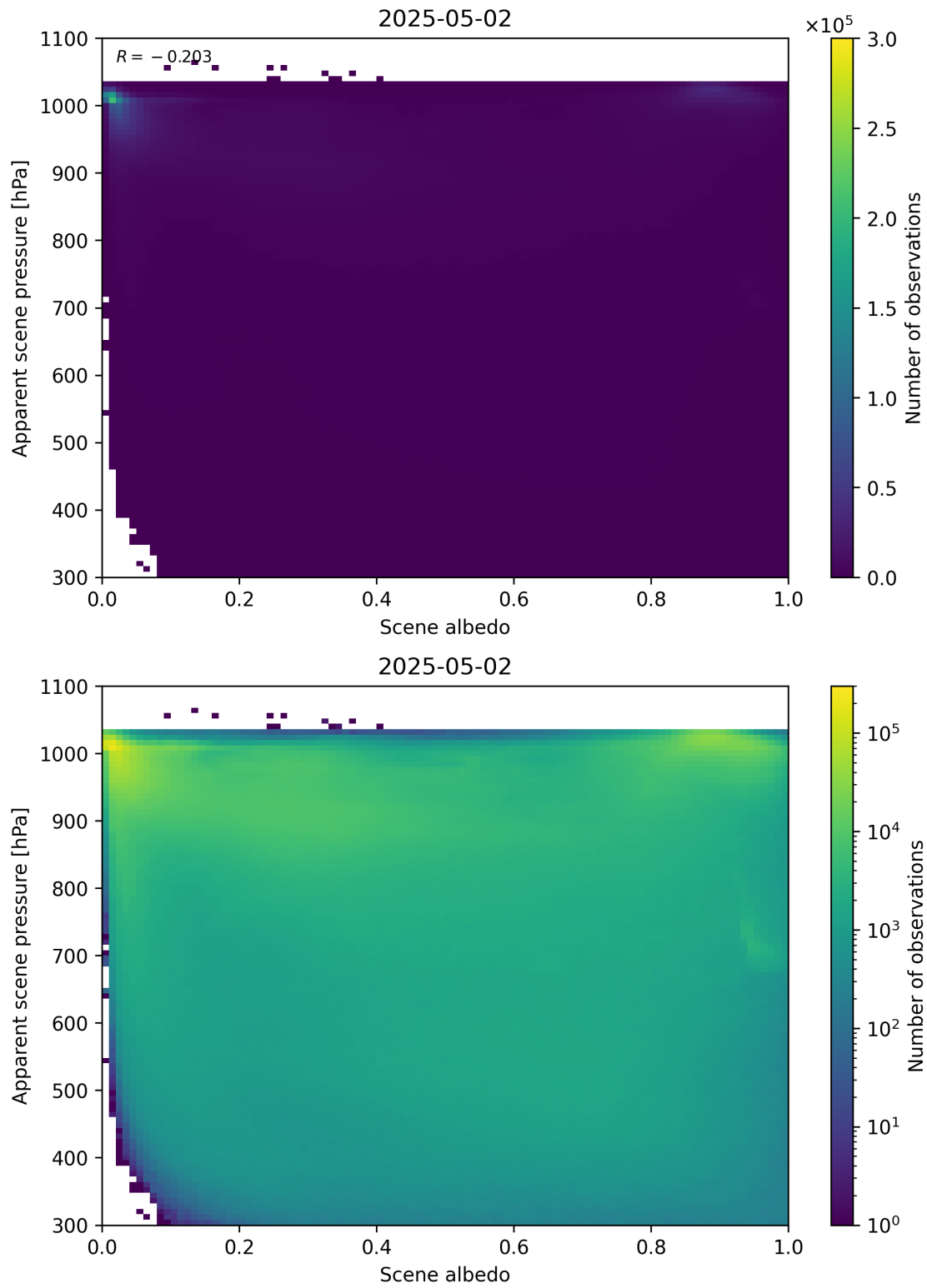
Figure 102: Scatter density plot of “Scene albedo” against “Apparent scene pressure” for 2025-05-01 to 2025-05-03.
