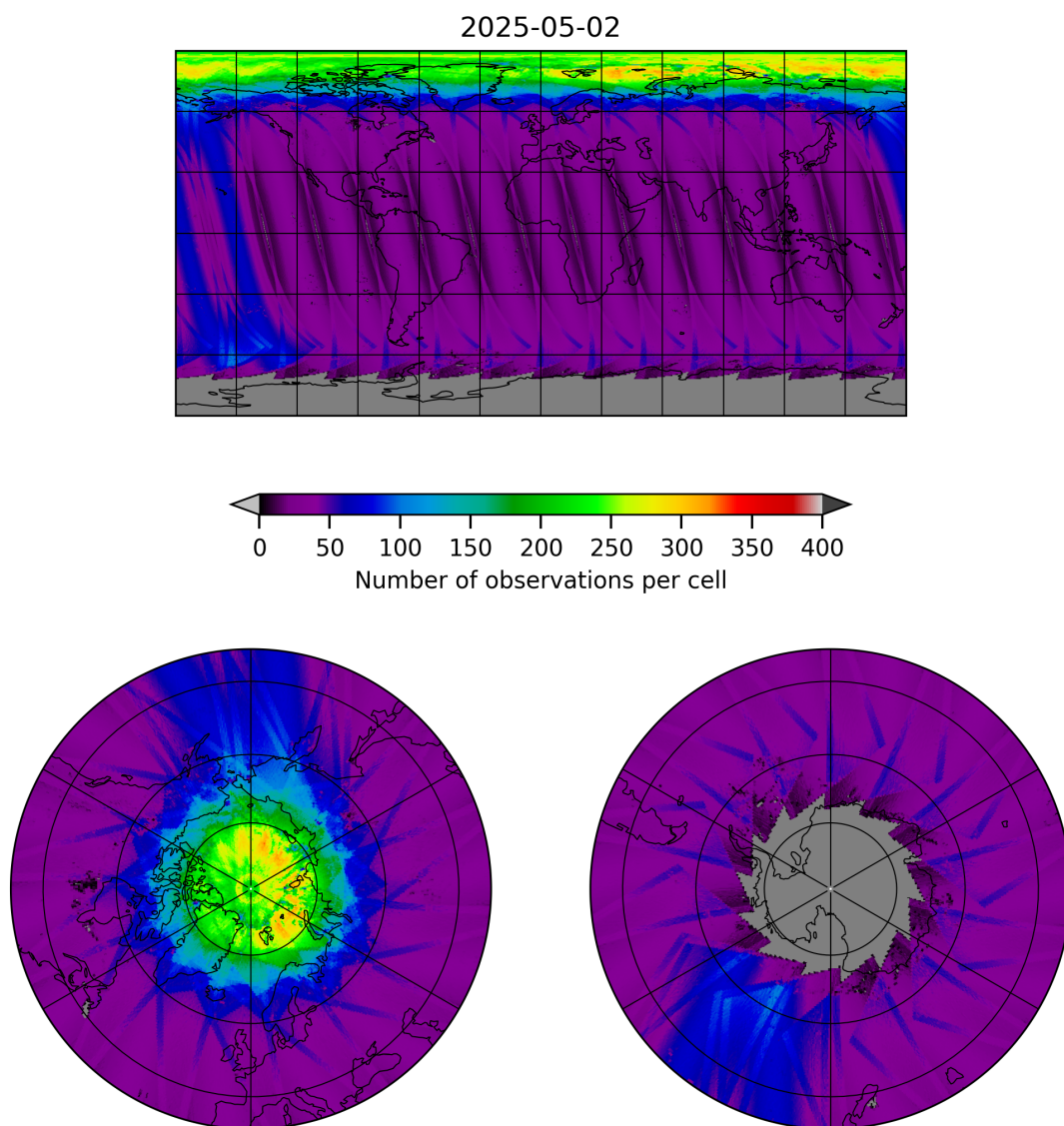
Figure 11: Map of the number of observations for 2025-05-01 to 2025-05-03
