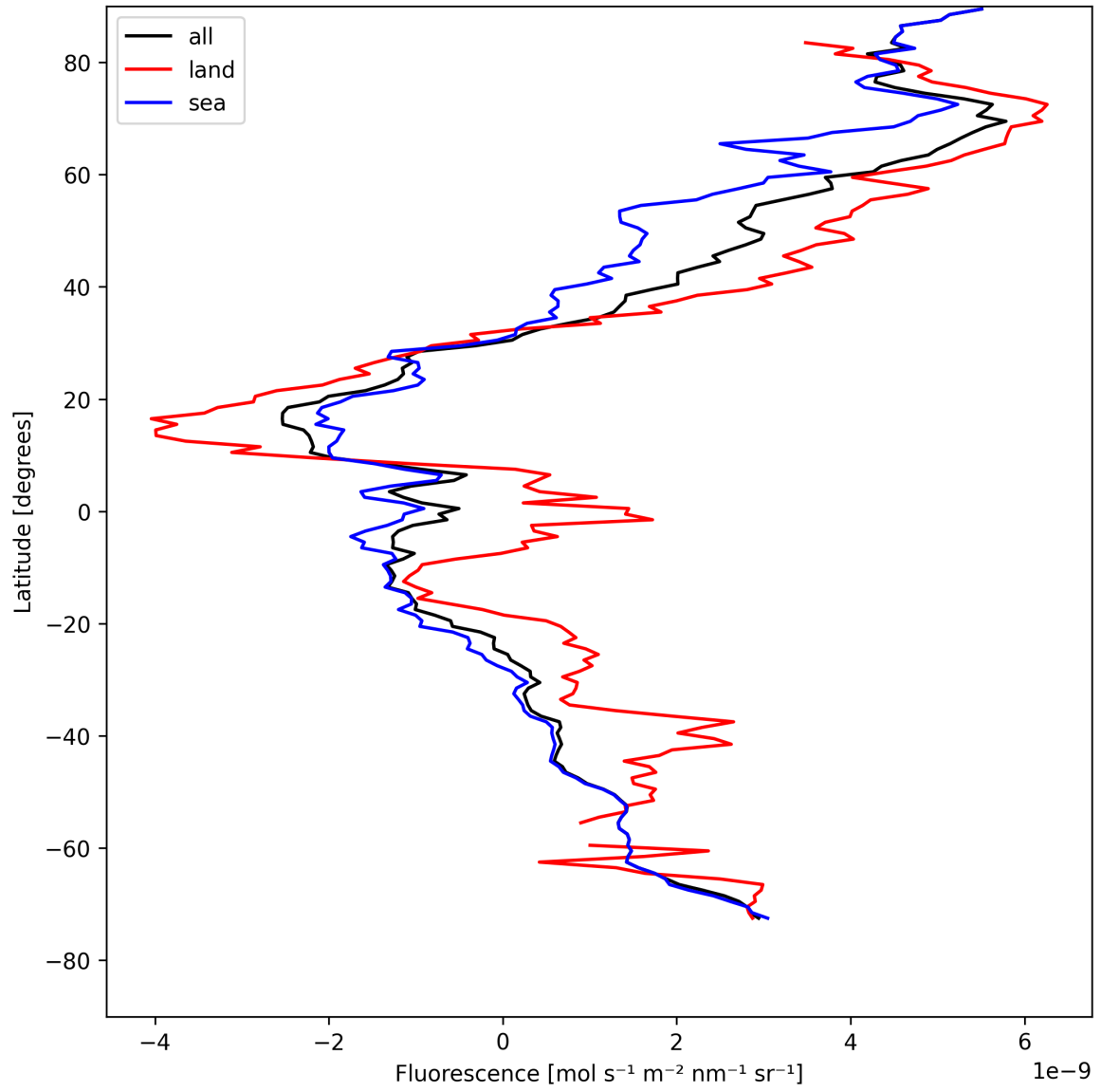
Figure 23: Zonal average of “Fluorescence” for 2025-05-01 to 2025-05-03.
