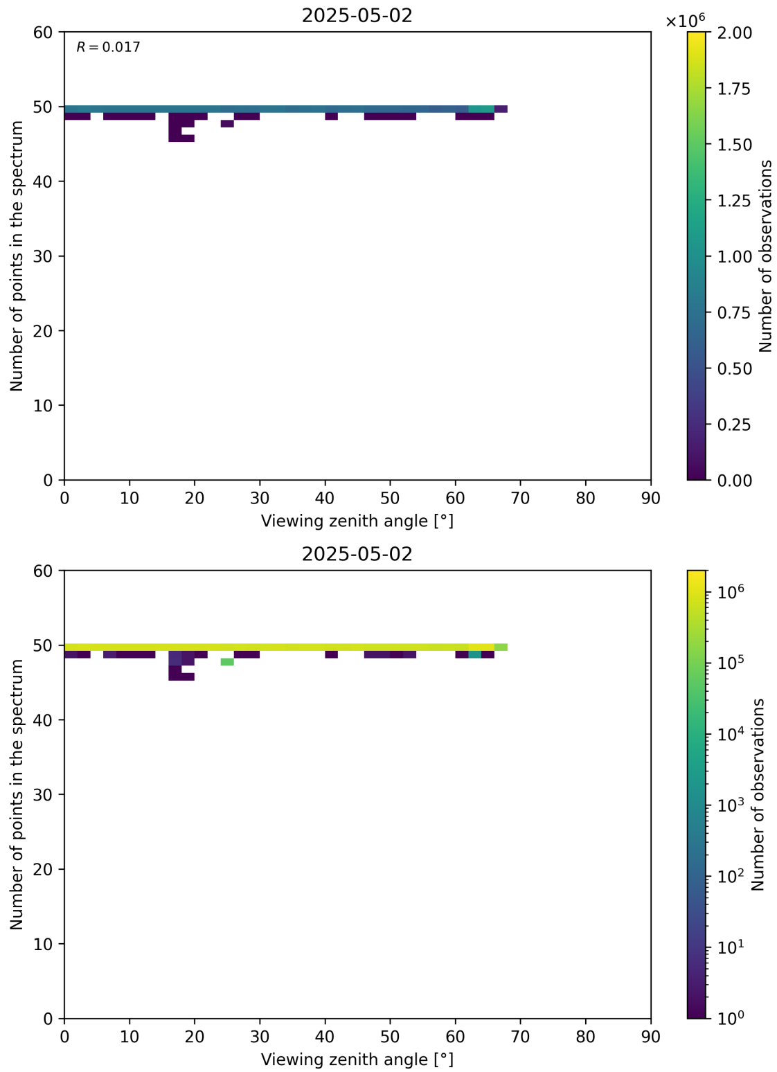
Figure 125: Scatter density plot of “Viewing zenith angle” against “Number of points in the spectrum” for 2025-05-01 to 2025-05-03.
