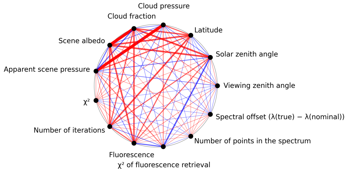
Figure 1: Map of correlation graph for 2025-05-01 to 2025-05-03.
