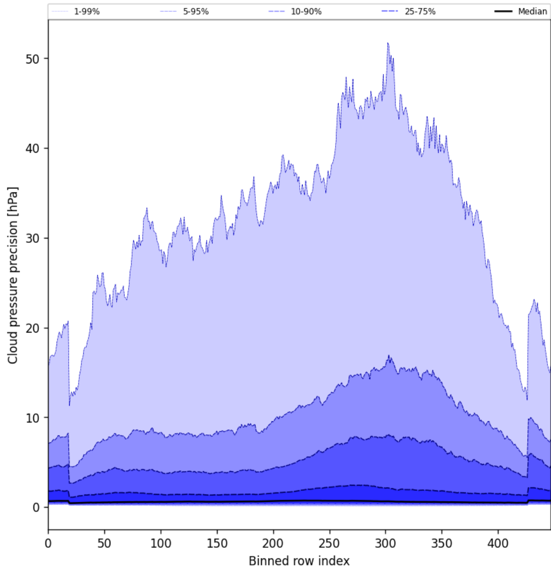
Figure 48: Along track statistics of “Cloud pressure precision” for 2025-05-01 to 2025-05-03
