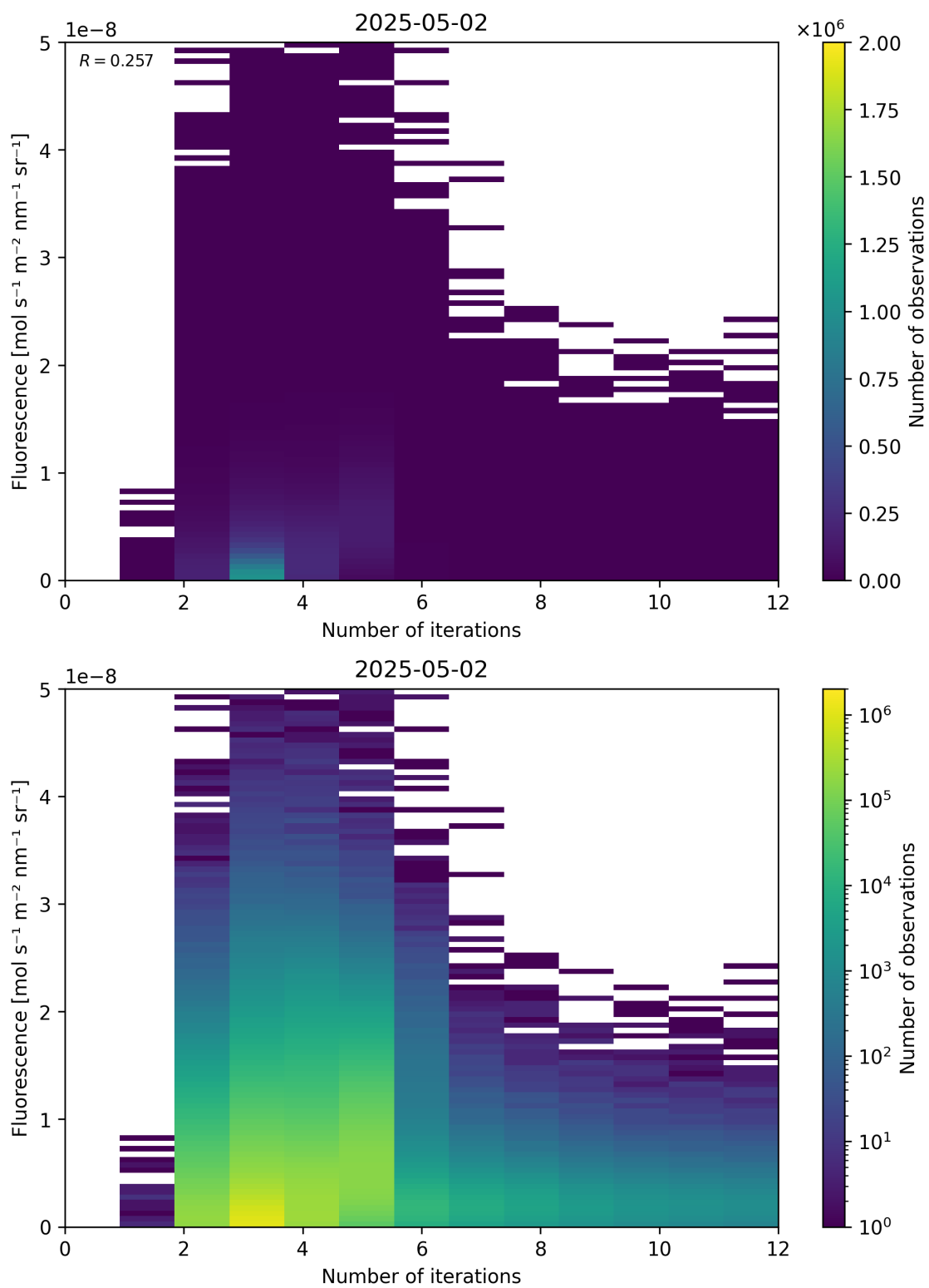
Figure 98: Scatter density plot of “Number of iterations” against “Fluorescence” for 2025-05-01 to 2025-05-03.
