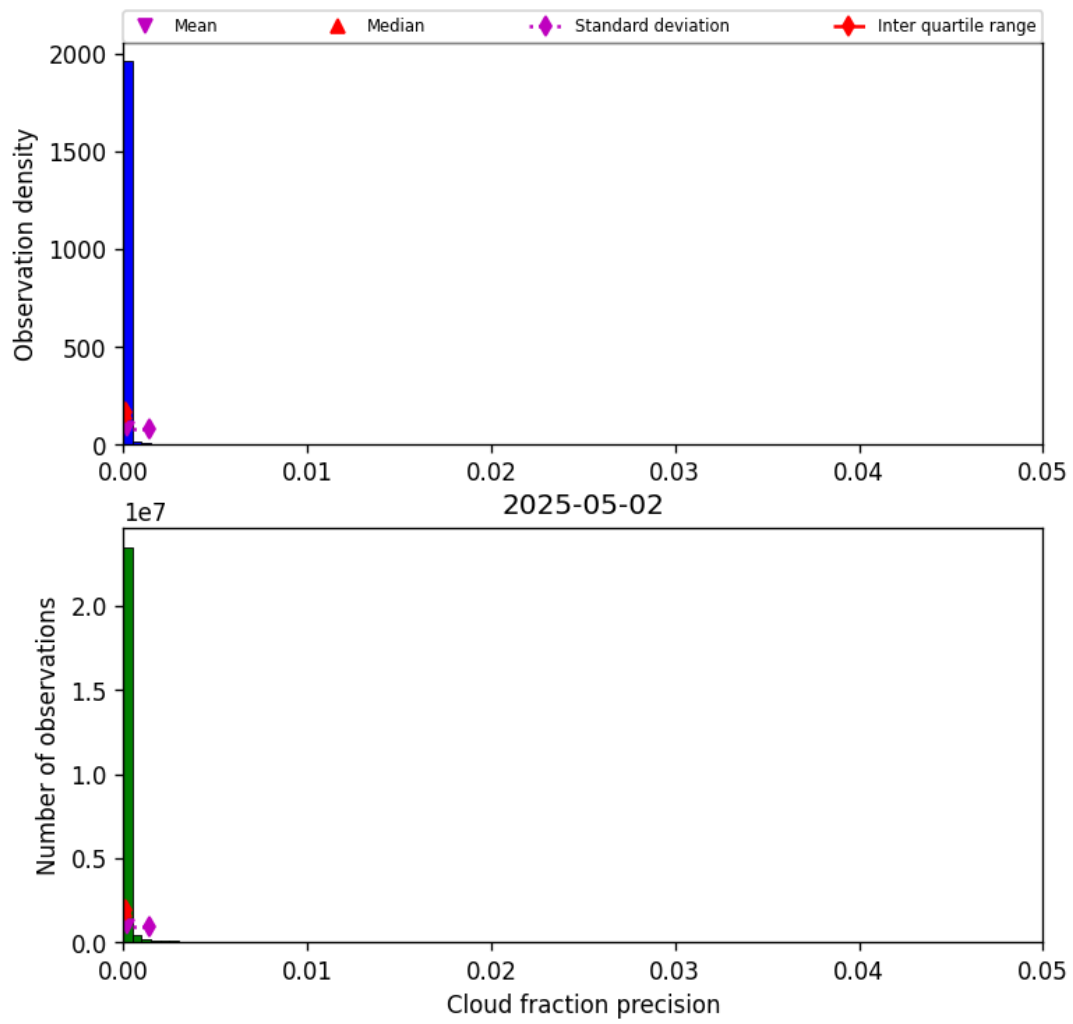
Figure 33: Histogram of “Cloud fraction precision” for 2025-05-01 to 2025-05-03
