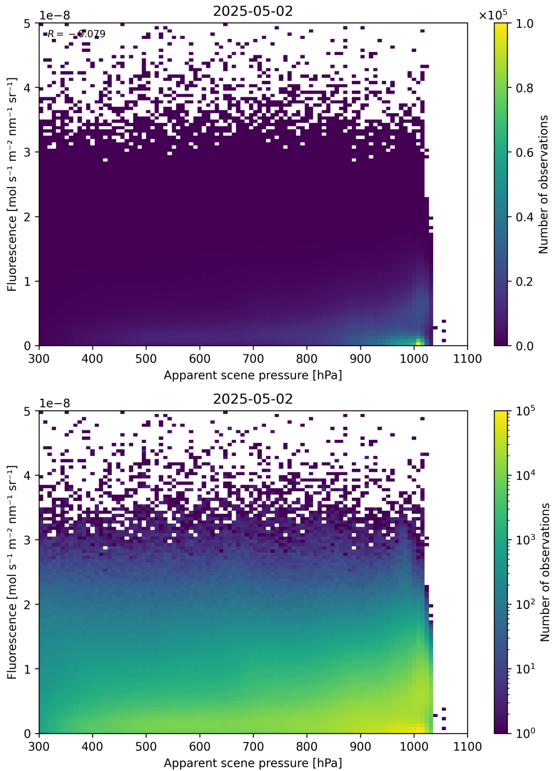
Figure 64: Scatter density plot of “Apparent scene pressure” against “Fluorescence” for 2025-05-01 to 2025-05-03.
