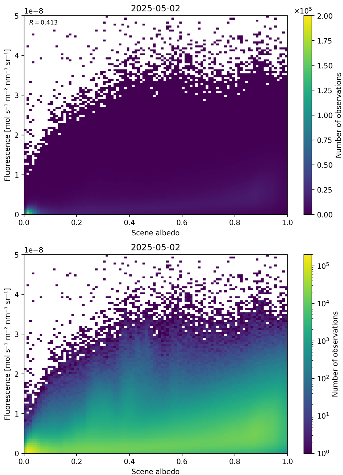
Figure 104: Scatter density plot of “Scene albedo” against “Fluorescence” for 2025-05-01 to 2025-05-03.
