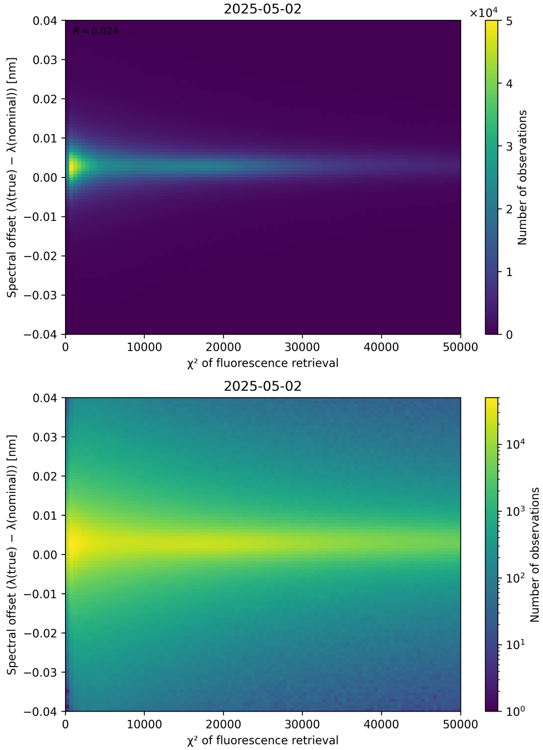
Figure 69: Scatter density plot of “ \chi^2 of fluorescence retrieval” against “Spectral offset ( \lambda_{\text{true}} - \lambda_{\text{nominal}} )” for 2025-05-01 to 2025-05-03.
