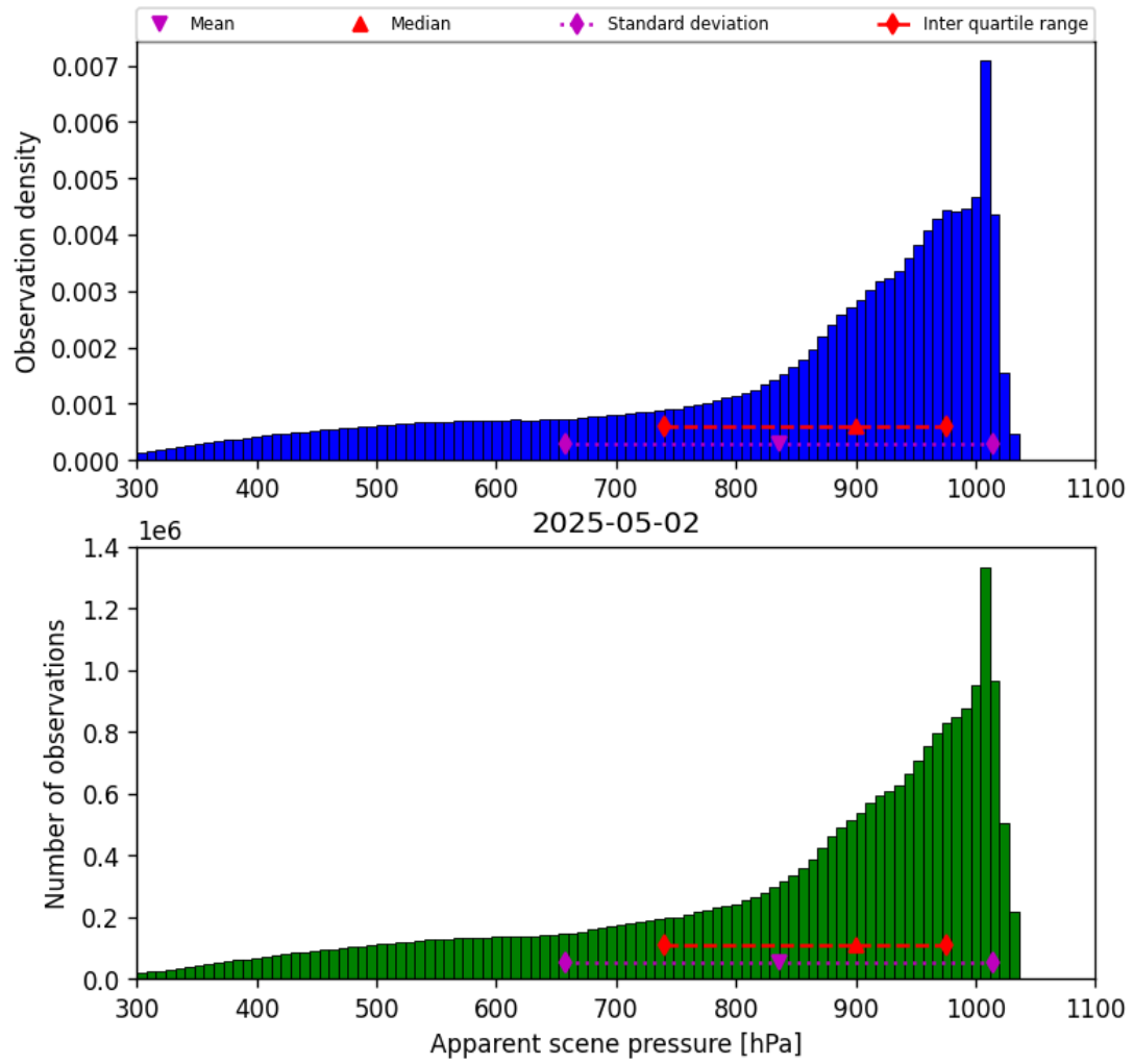
Figure 36: Histogram of “Apparent scene pressure” for 2025-05-01 to 2025-05-03
