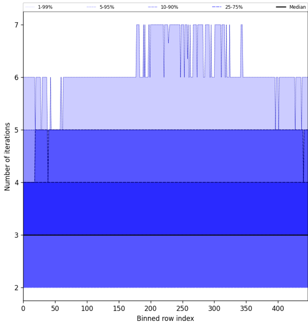
Figure 56: Along track statistics of “Number of iterations” for 2025-05-01 to 2025-05-03
