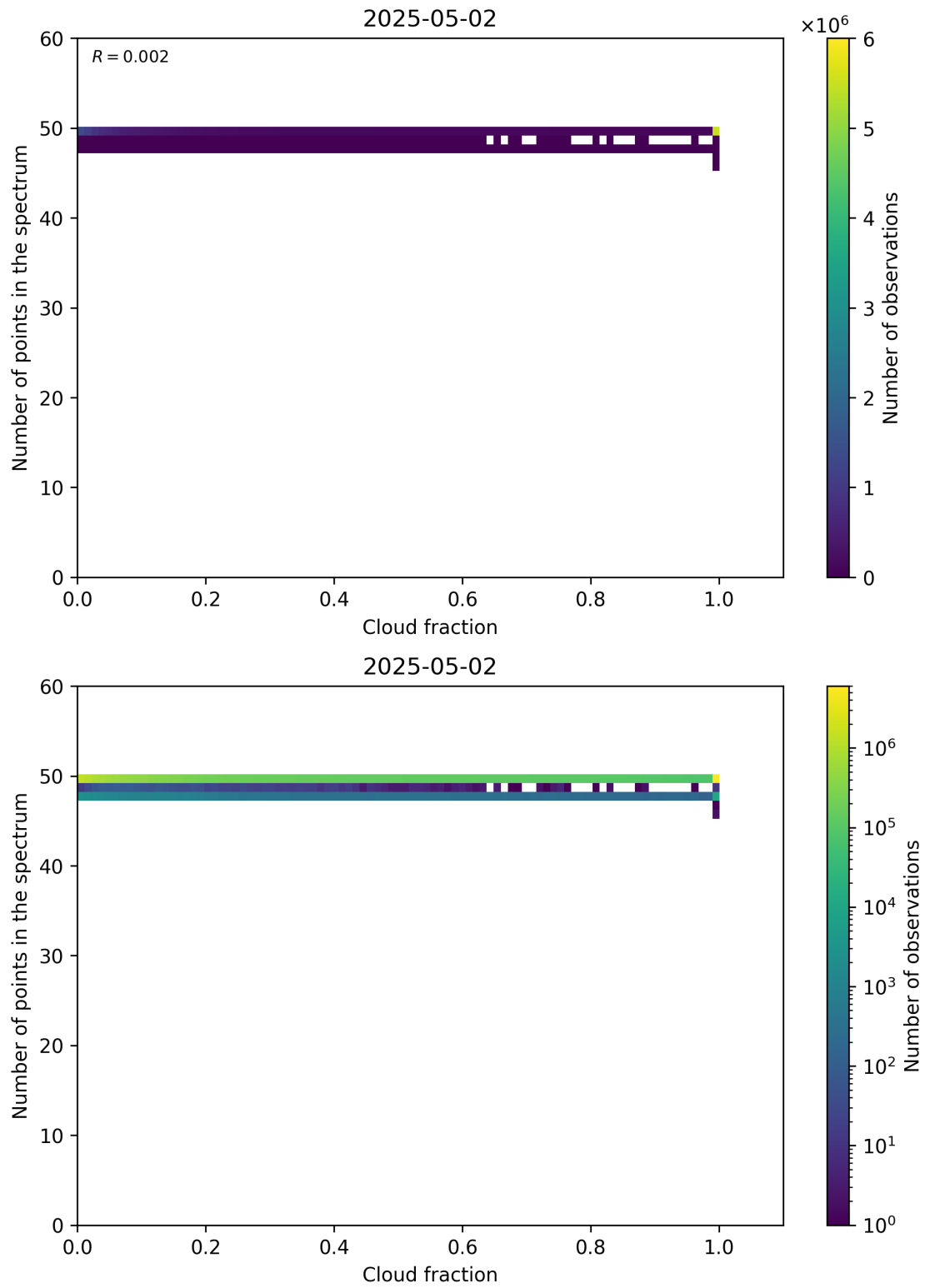
Figure 74: Scatter density plot of “Cloud fraction” against “Number of points in the spectrum” for 2025-05-01 to 2025-05-03.
