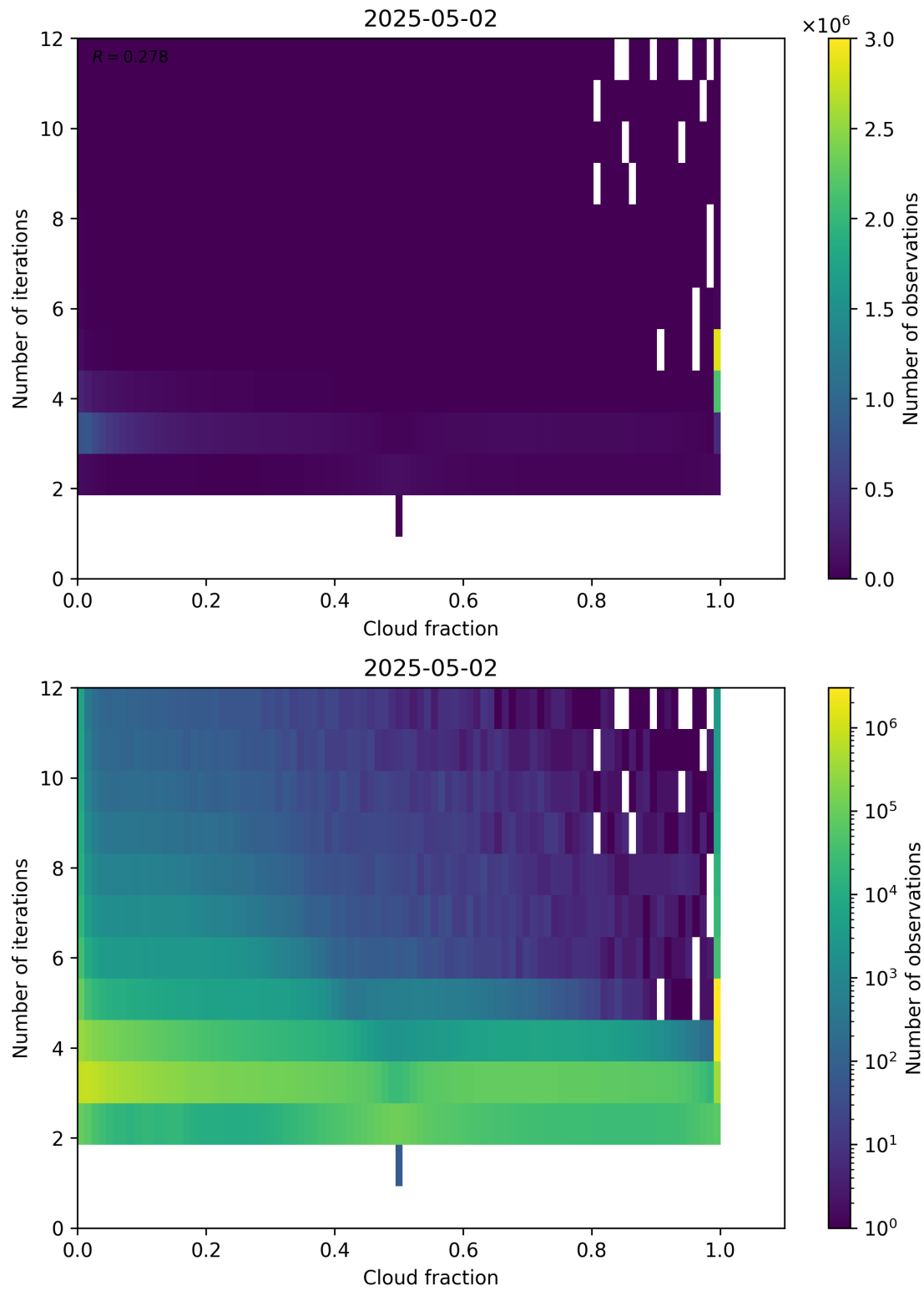
Figure 73: Scatter density plot of “Cloud fraction” against “Number of iterations” for 2025-05-01 to 2025-05-03.
