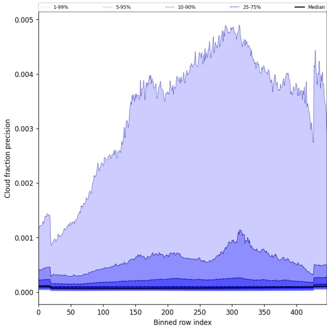
Figure 50: Along track statistics of “Cloud fraction precision” for 2025-05-01 to 2025-05-03
