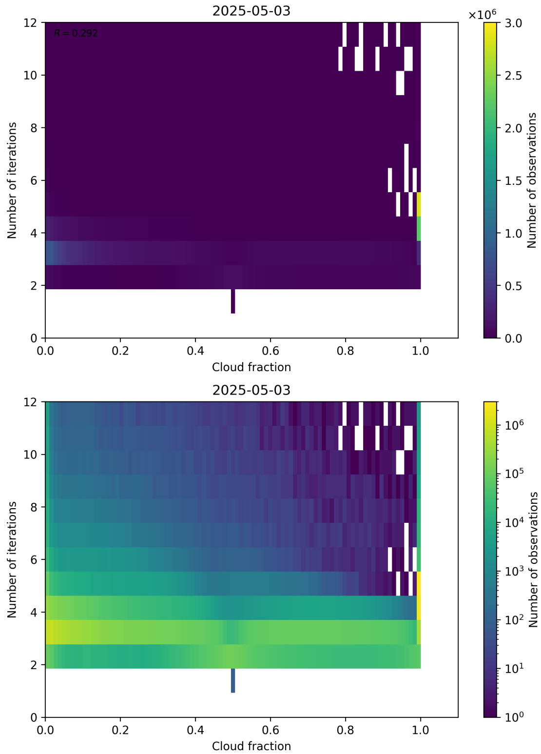
Figure 73: Scatter density plot of “Cloud fraction” against “Number of iterations” for 2025-05-02 to 2025-05-04.
