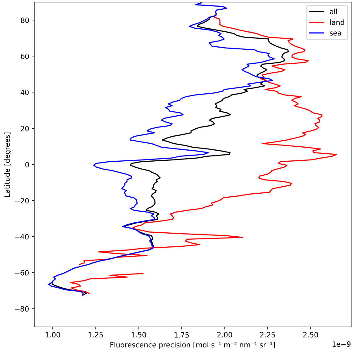
Figure 24: Zonal average of “Fluorescence precision” for 2025-05-02 to 2025-05-04.
