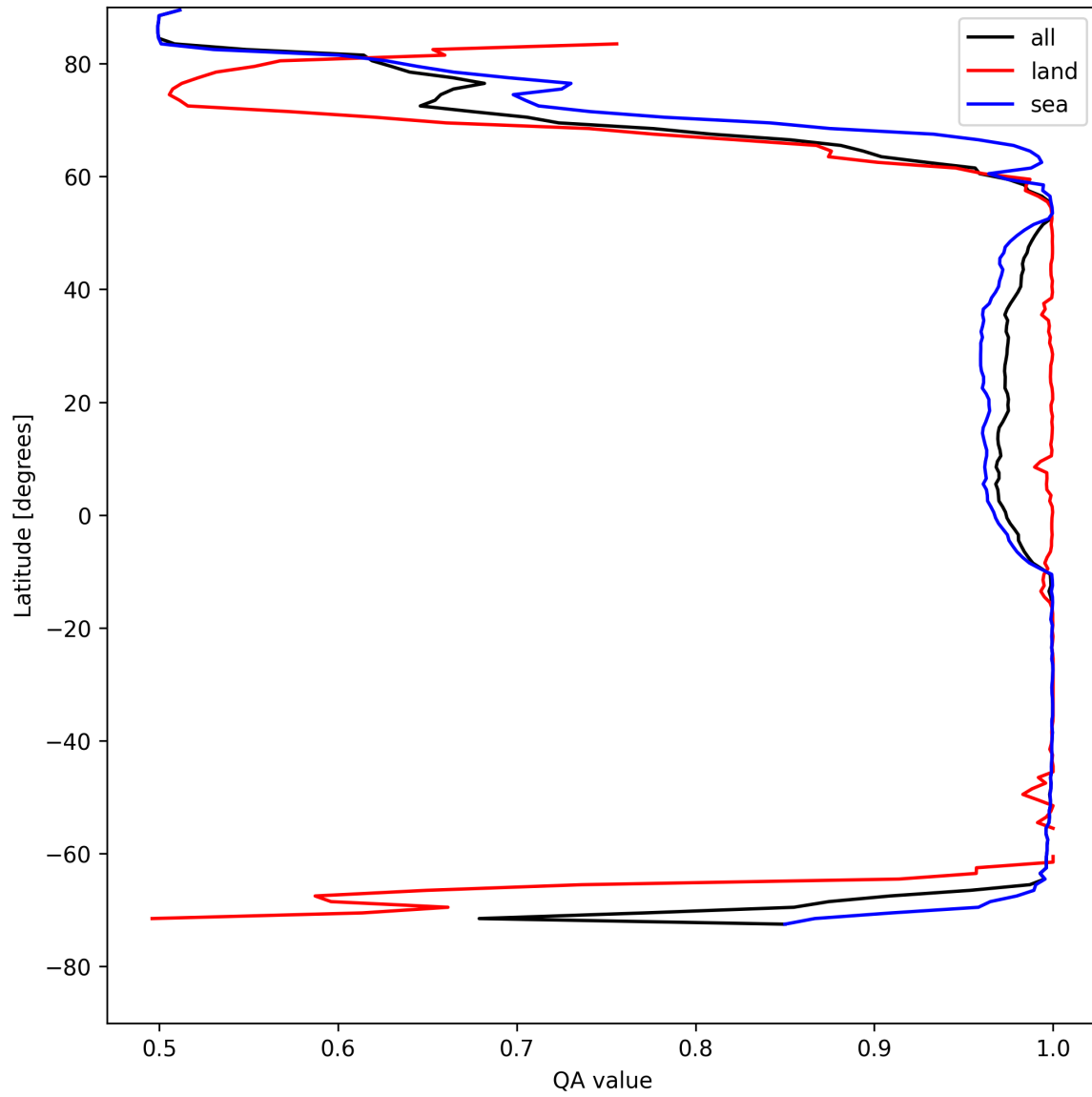
Figure 12: Zonal average of “QA value” for 2025-05-02 to 2025-05-04.
