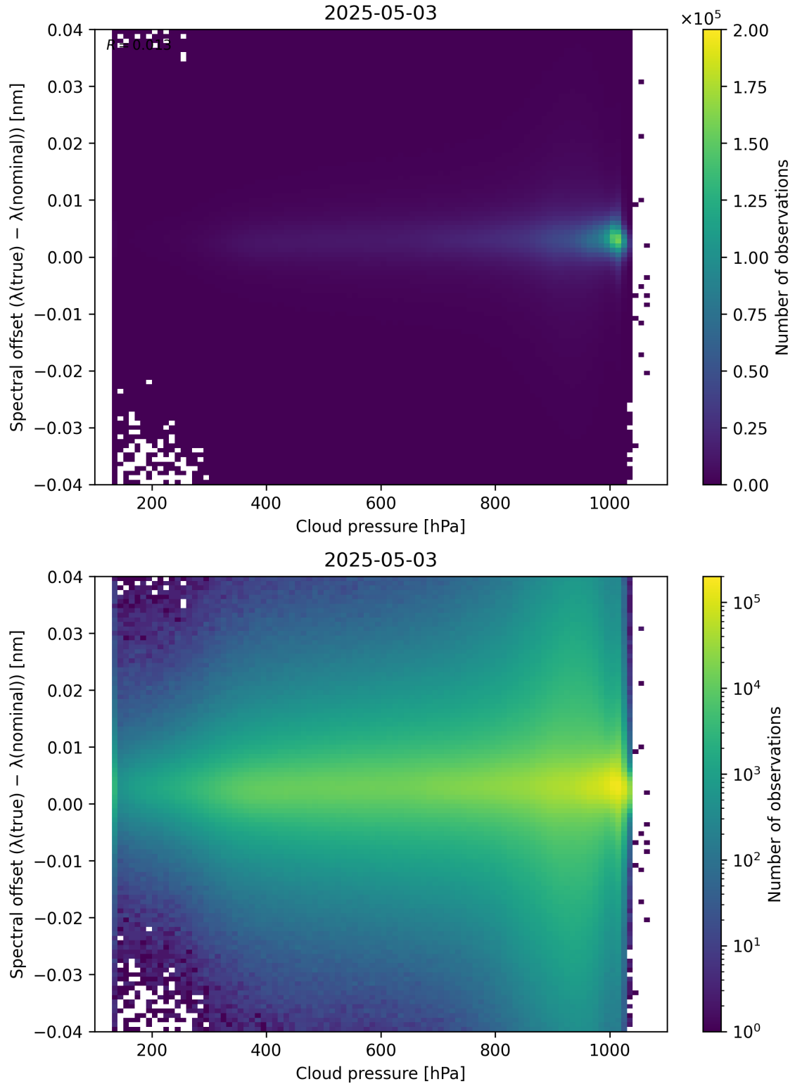
Figure 84: Scatter density plot of “Cloud pressure” against “Spectral offset ( \lambda_{\text{true}} - \lambda_{\text{nominal}} )” for 2025-05-02 to 2025-05-04.
