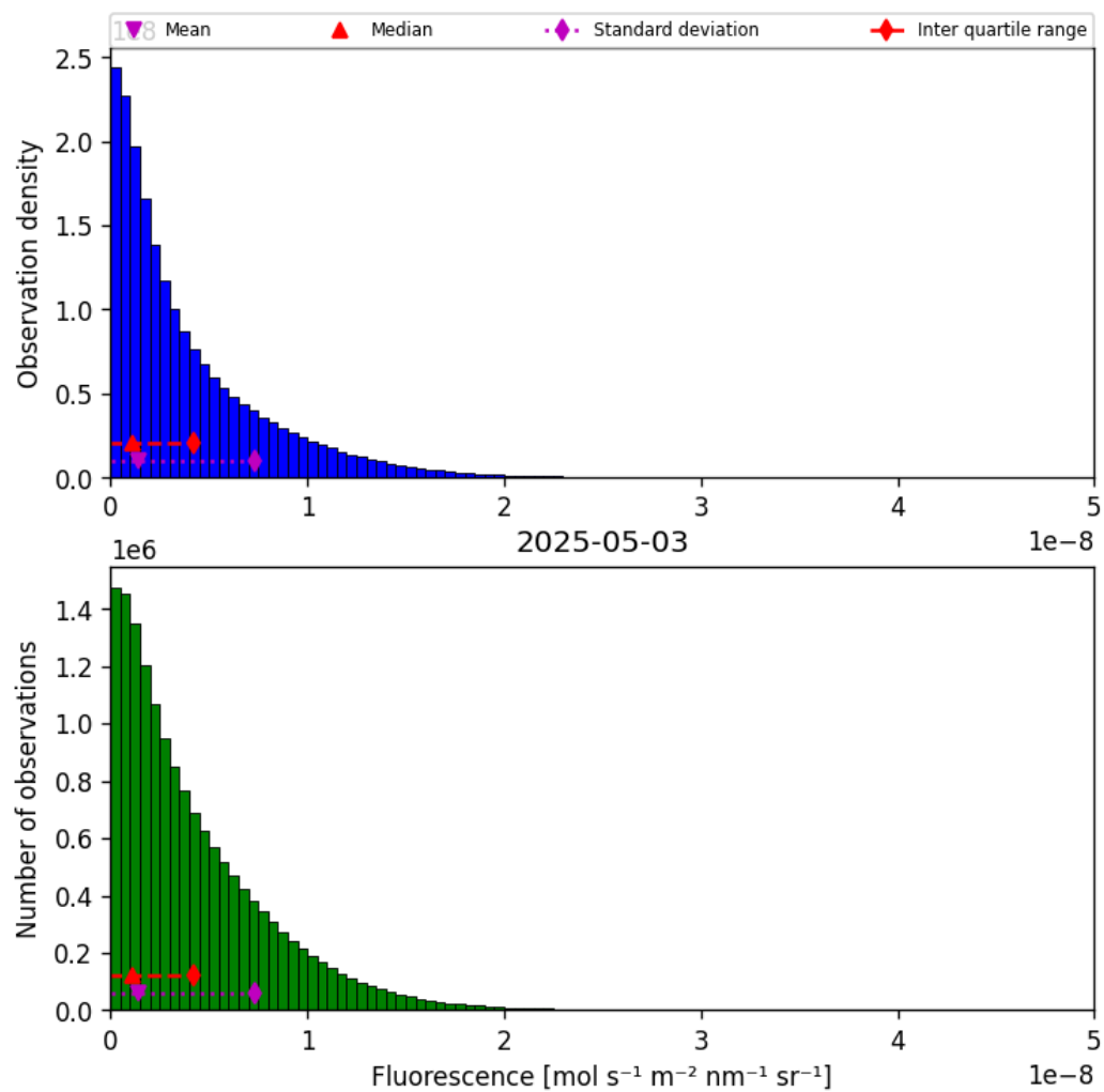
Figure 40: Histogram of “Fluorescence” for 2025-05-02 to 2025-05-04
