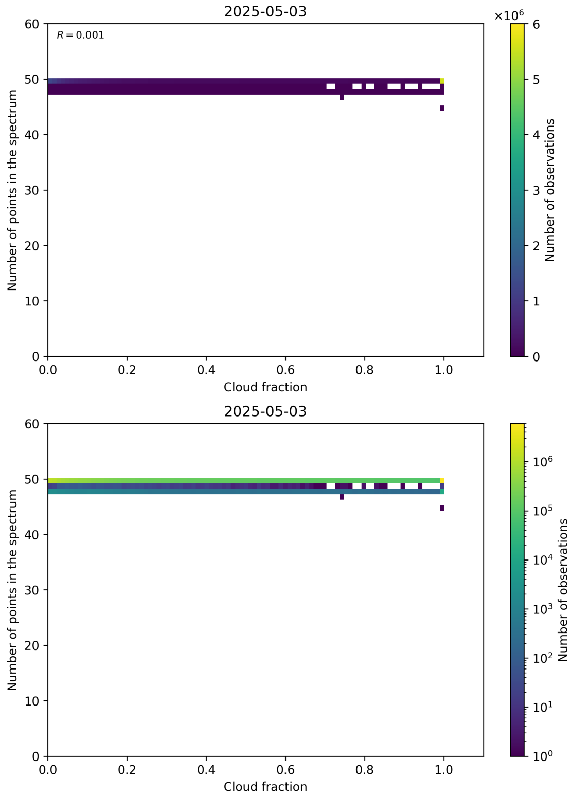
Figure 74: Scatter density plot of “Cloud fraction” against “Number of points in the spectrum” for 2025-05-02 to 2025-05-04.
