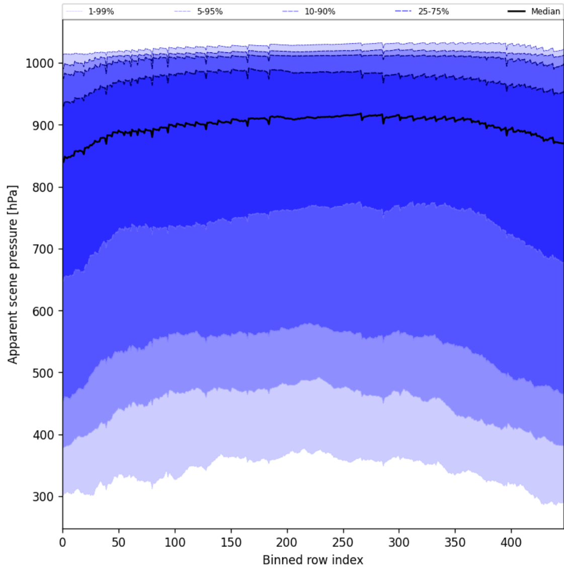
Figure 53: Along track statistics of “Apparent scene pressure” for 2025-05-02 to 2025-05-04
