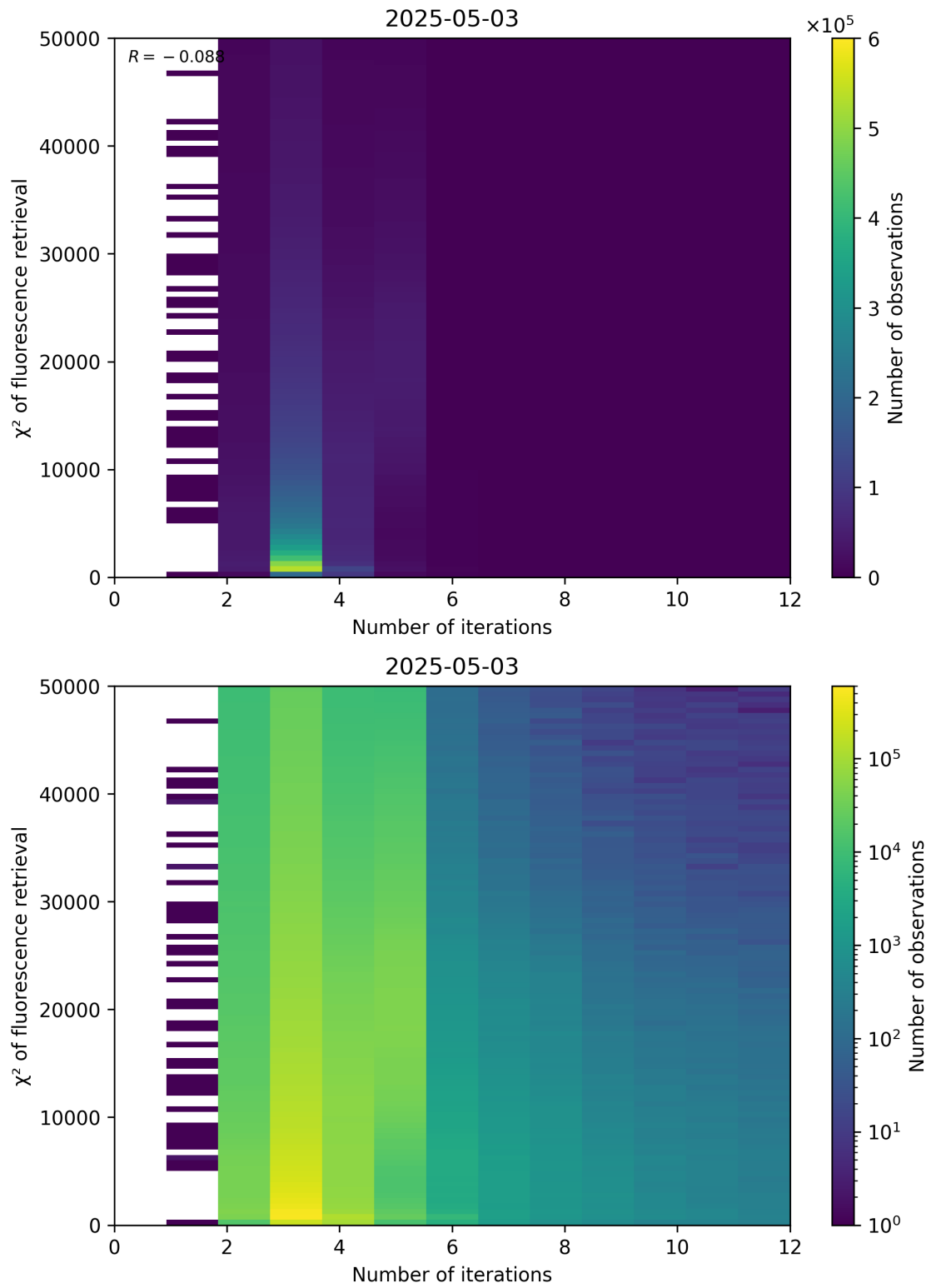
Figure 97: Scatter density plot of “Number of iterations” against “ \chi^2 of fluorescence retrieval” for 2025-05-02 to 2025-05-04.
