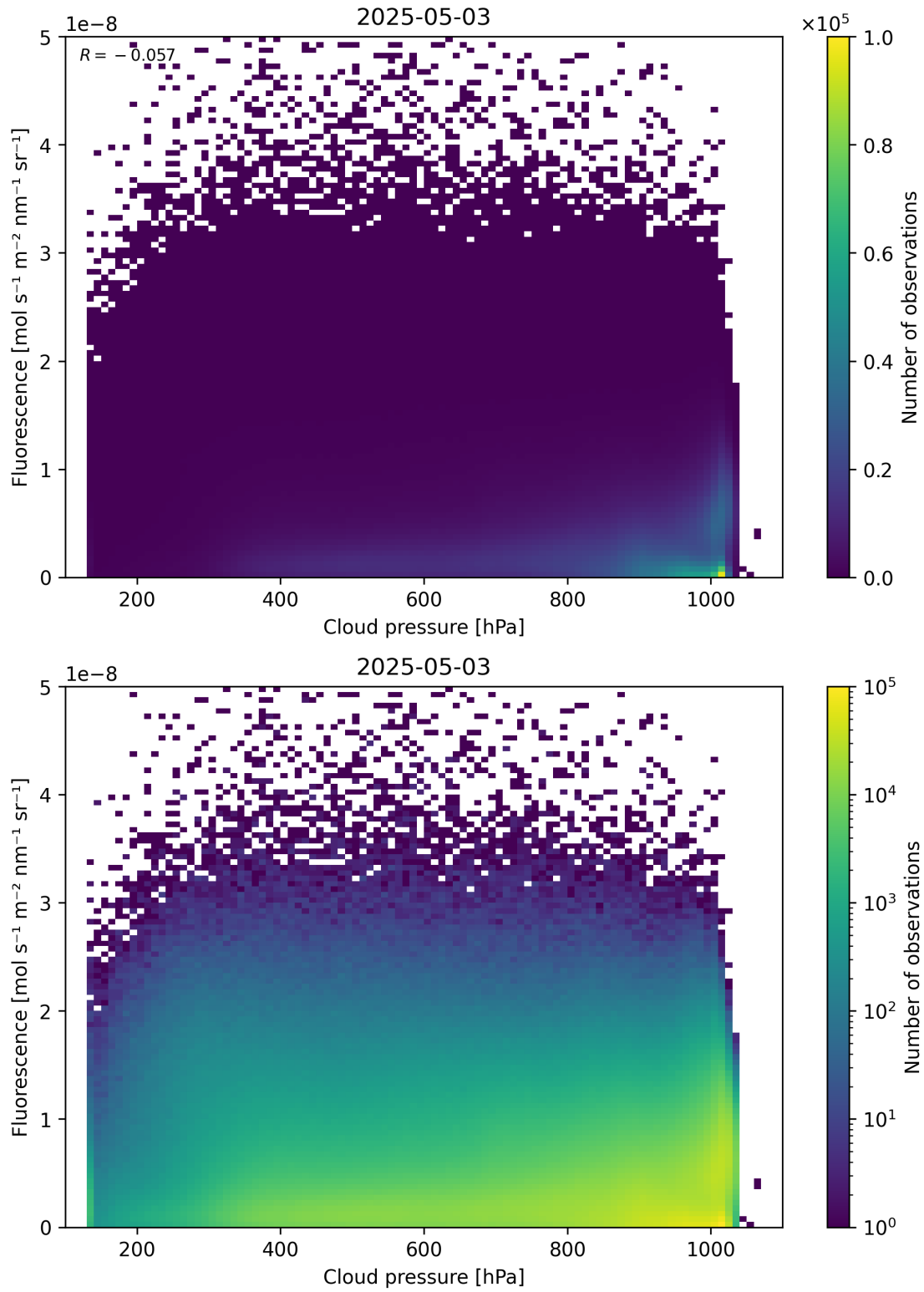
Figure 80: Scatter density plot of “Cloud pressure” against “Fluorescence” for 2025-05-02 to 2025-05-04.
