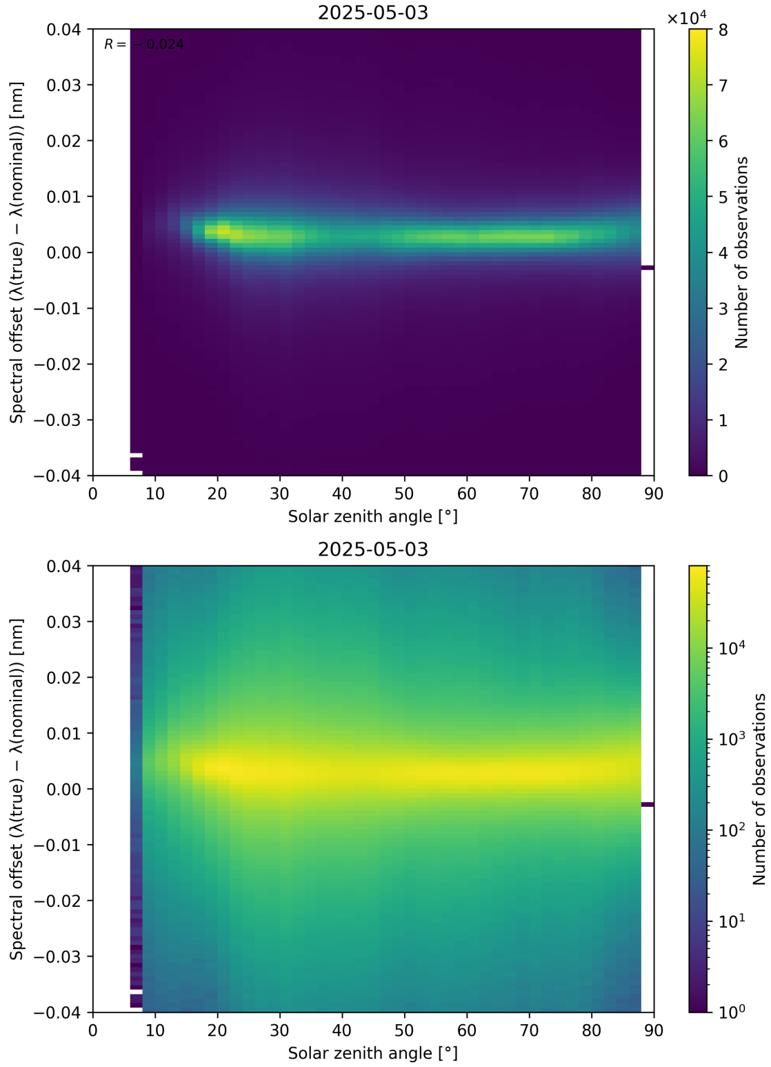
Figure 117: Scatter density plot of “Solar zenith angle” against “Spectral offset ( \lambda_{\text{true}} - \lambda_{\text{nominal}} )” for 2025-05-02 to 2025-05-04.
