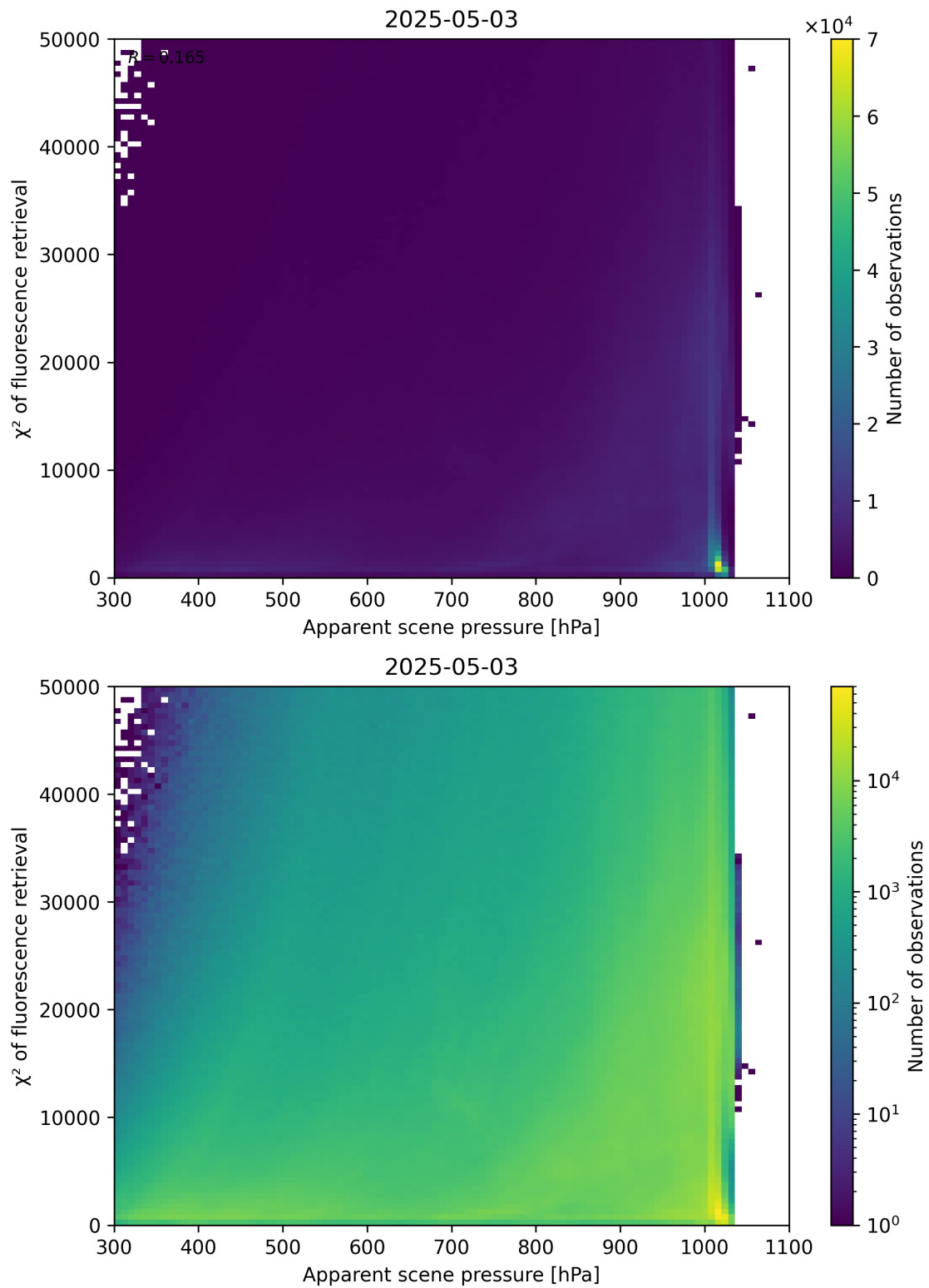
Figure 63: Scatter density plot of “Apparent scene pressure” against “ \chi^2 of fluorescence retrieval” for 2025-05-02 to 2025-05-04.
