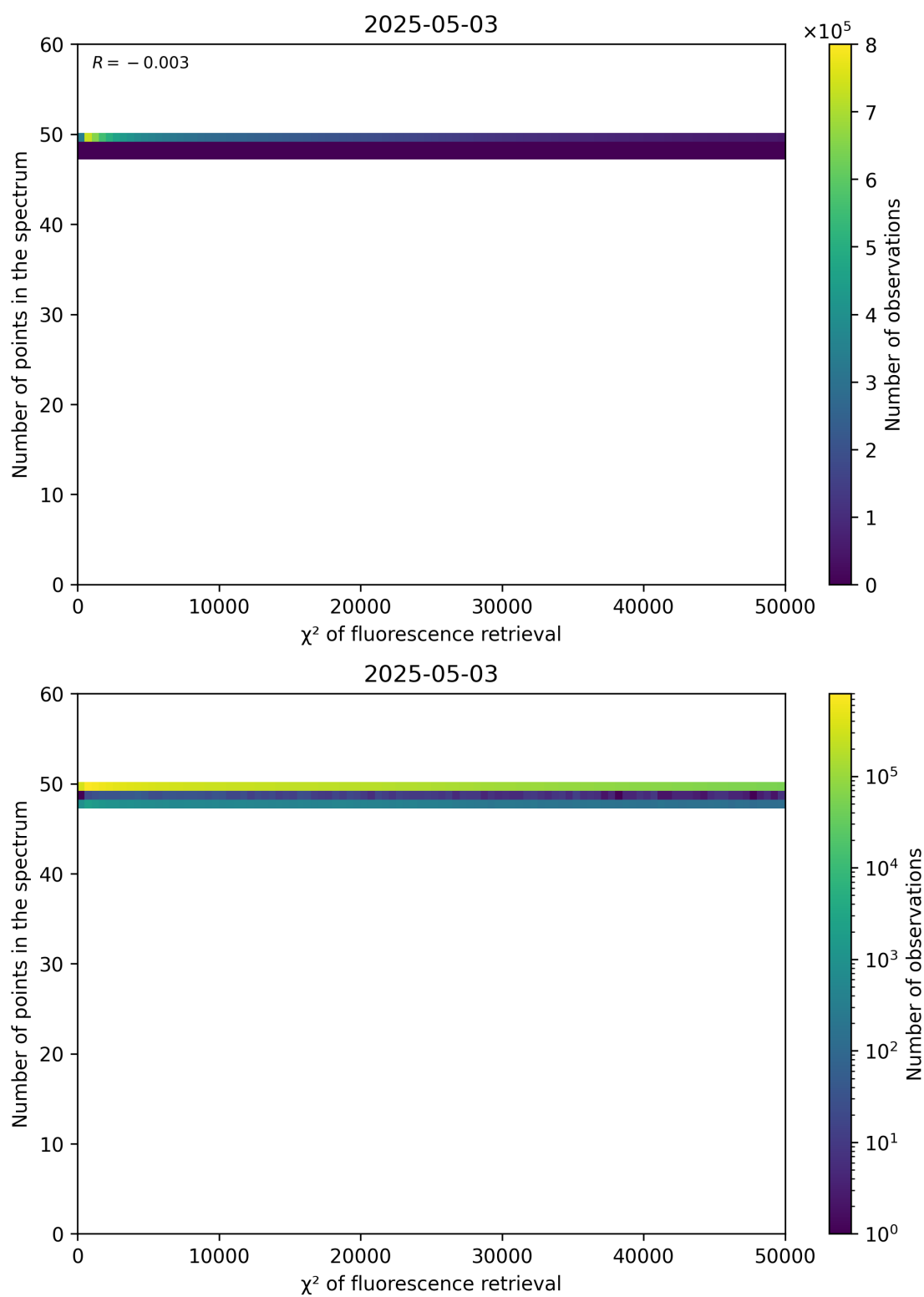
Figure 68: Scatter density plot of " \chi^2 of fluorescence retrieval" against "Number of points in the spectrum" for 2025-05-02 to 2025-05-04.
