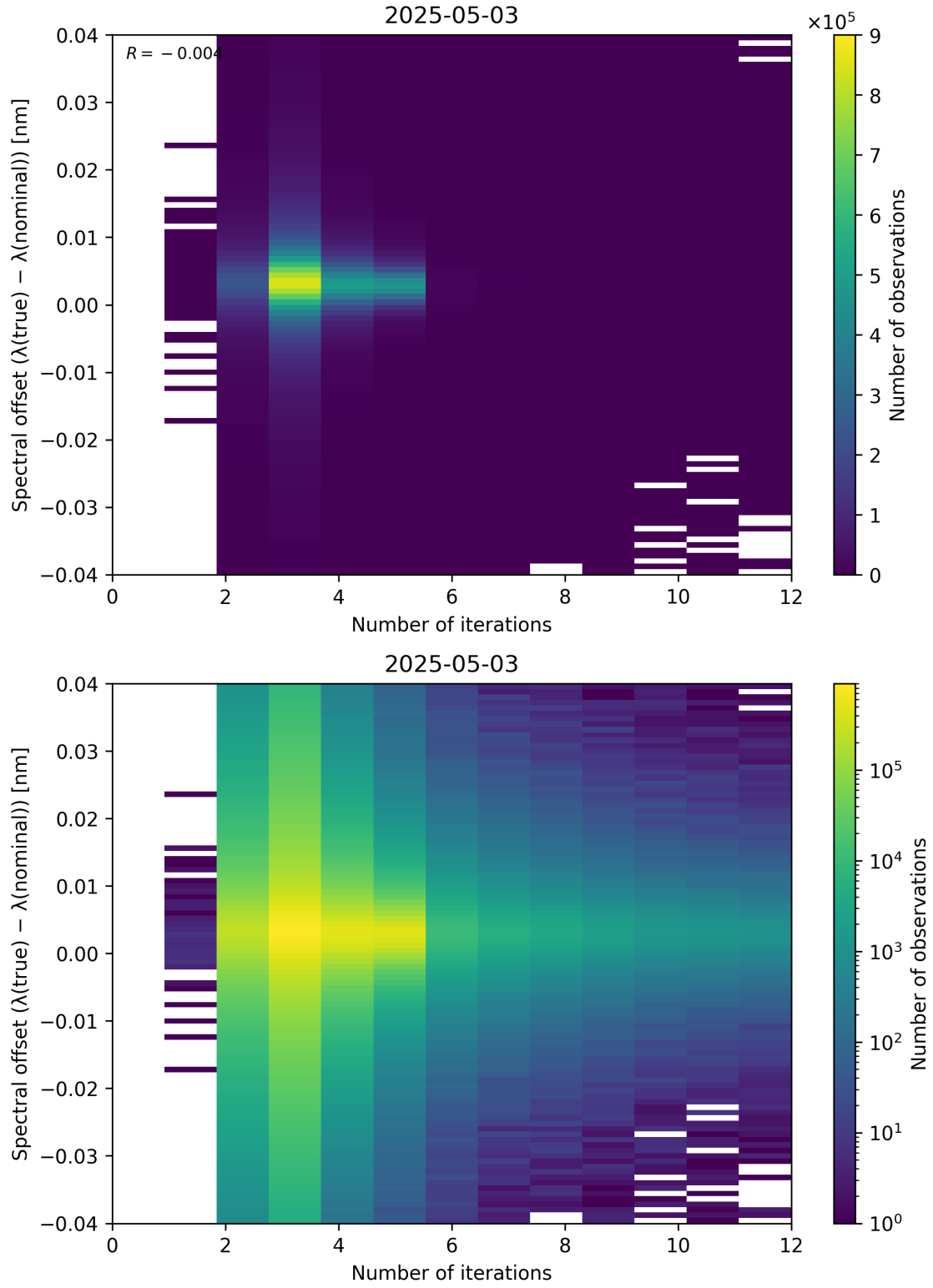
Figure 100: Scatter density plot of “Number of iterations” against “Spectral offset ( \lambda_{\text{true}} - \lambda_{\text{nominal}} )” for 2025-05-02 to 2025-05-04.
