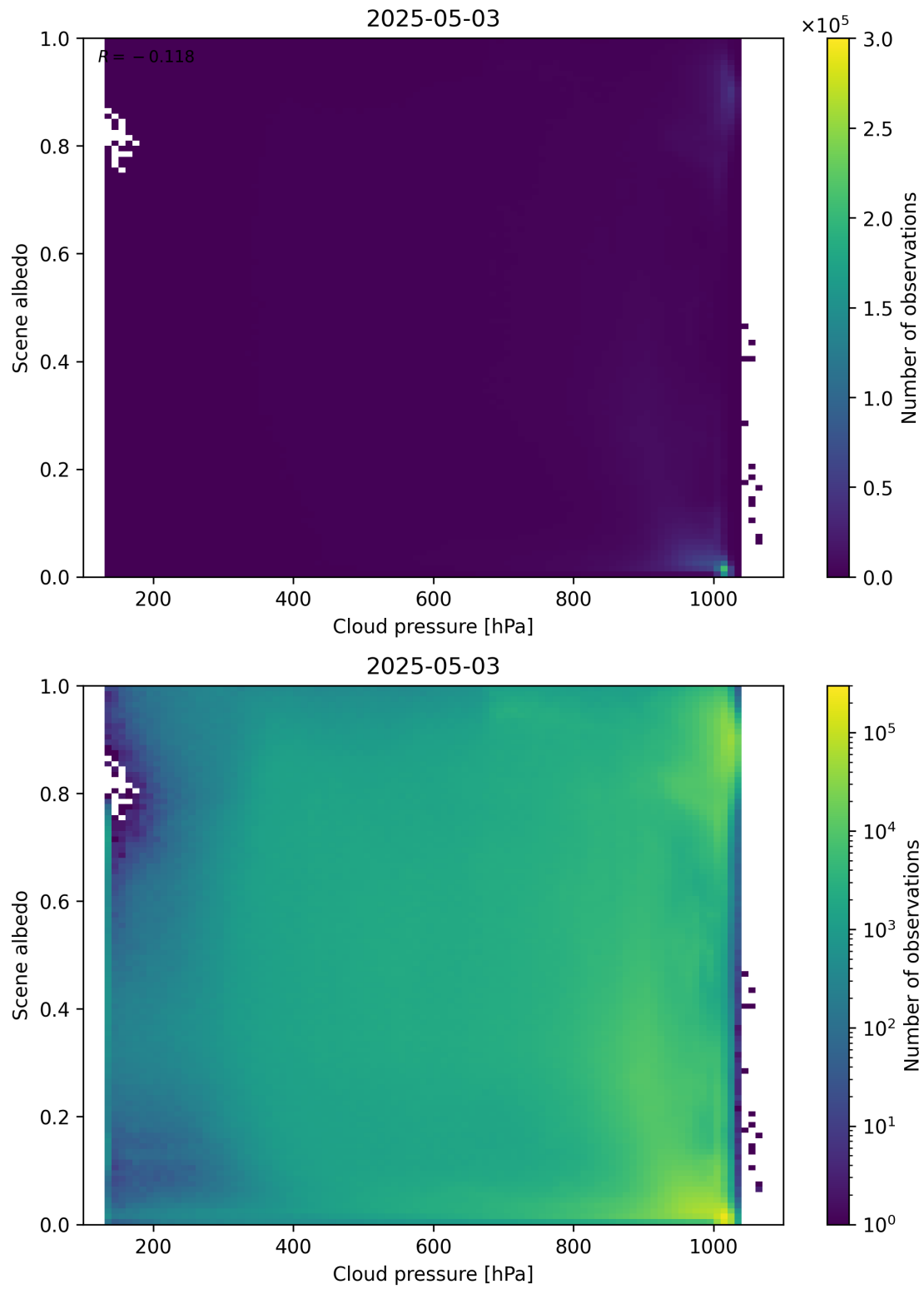
Figure 83: Scatter density plot of “Cloud pressure” against “Scene albedo” for 2025-05-02 to 2025-05-04.
