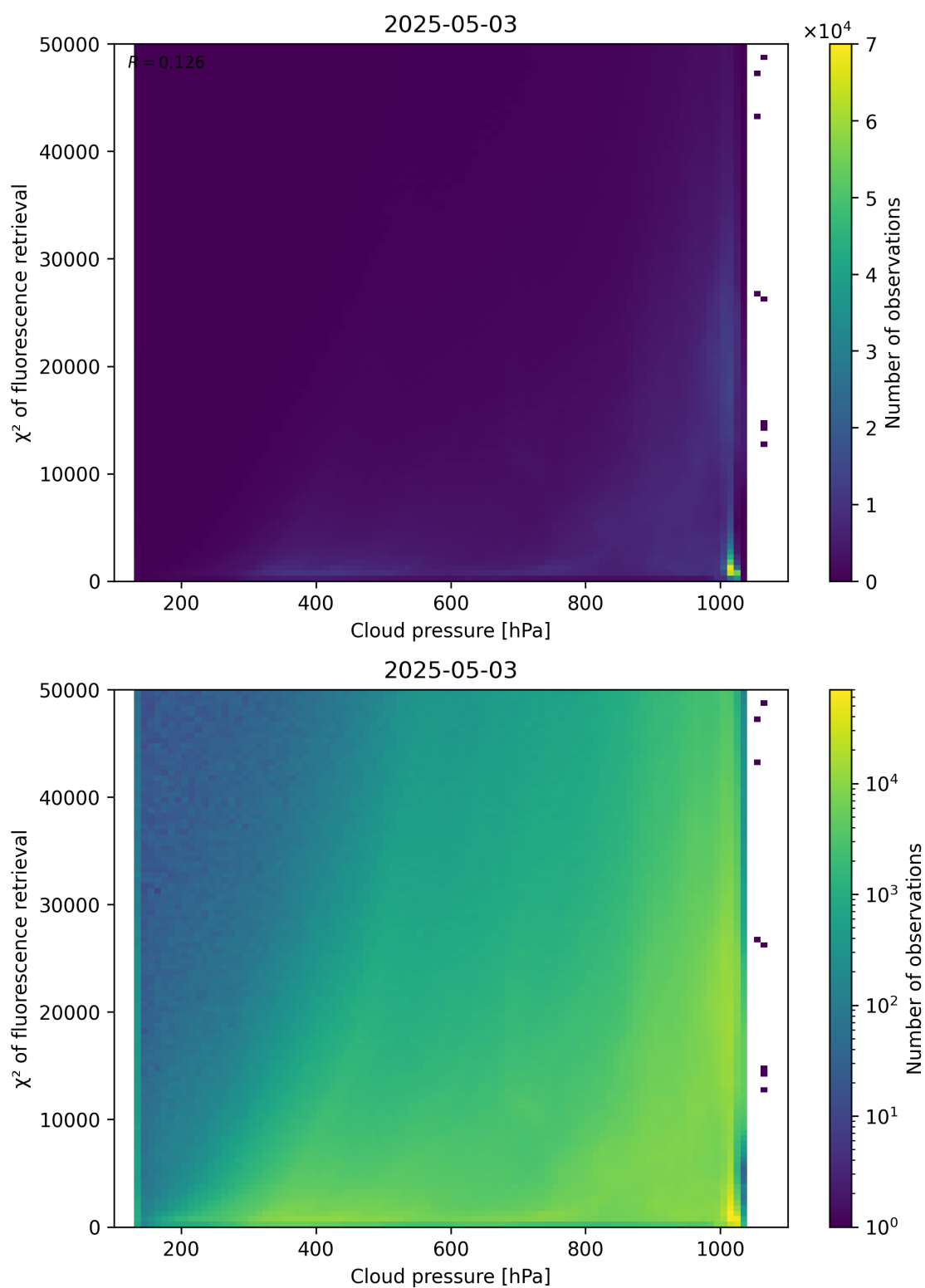
Figure 78: Scatter density plot of “Cloud pressure” against “ \chi^2 of fluorescence retrieval” for 2025-05-02 to 2025-05-04.
