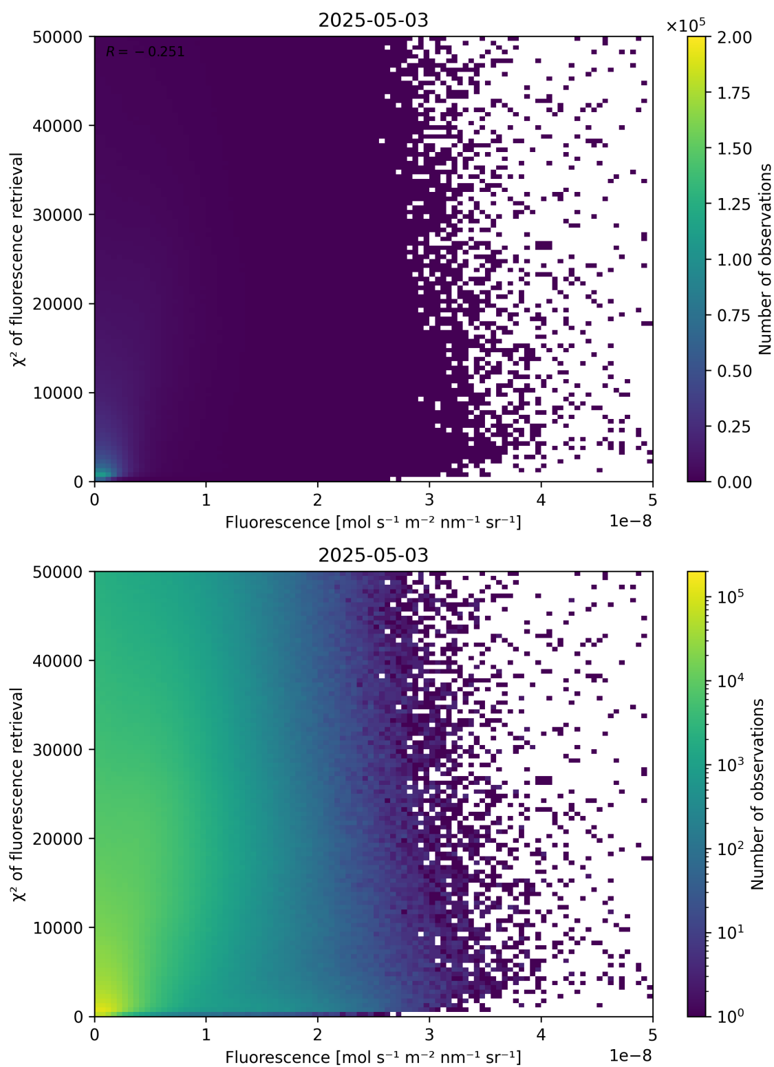
Figure 85: Scatter density plot of “Fluorescence” against “ \chi^2 of fluorescence retrieval” for 2025-05-02 to 2025-05-04.
