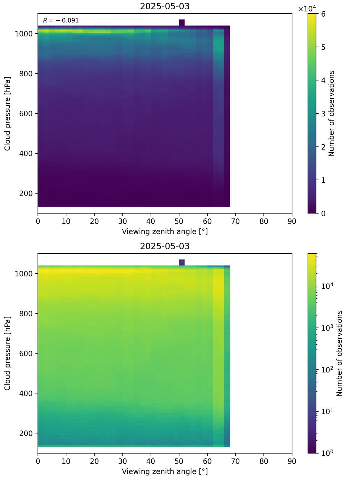
Figure 121: Scatter density plot of “Viewing zenith angle” against “Cloud pressure” for 2025-05-02 to 2025-05-04.
