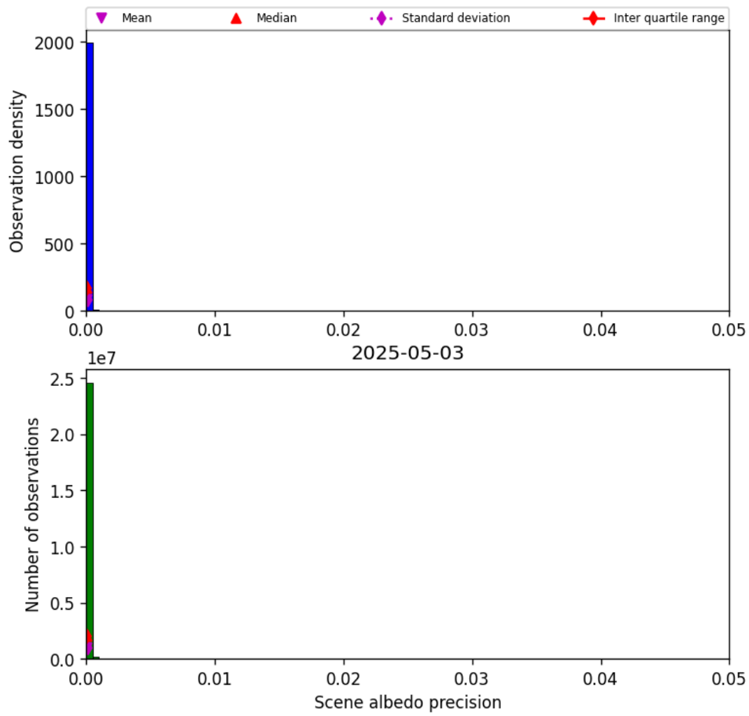
Figure 35: Histogram of “Scene albedo precision” for 2025-05-02 to 2025-05-04
