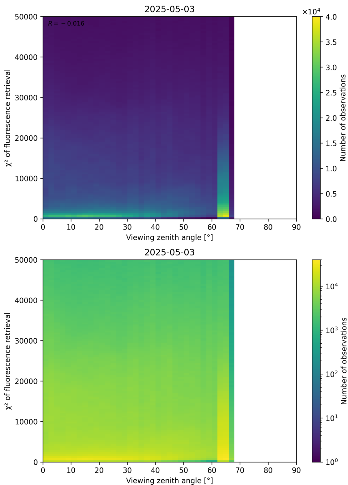
Figure 119: Scatter density plot of “Viewing zenith angle” against “ \chi^2 of fluorescence retrieval” for 2025-05-02 to 2025-05-04.
