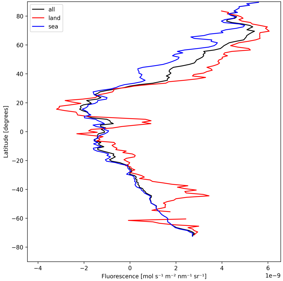
Figure 23: Zonal average of “Fluorescence” for 2025-05-02 to 2025-05-04.
