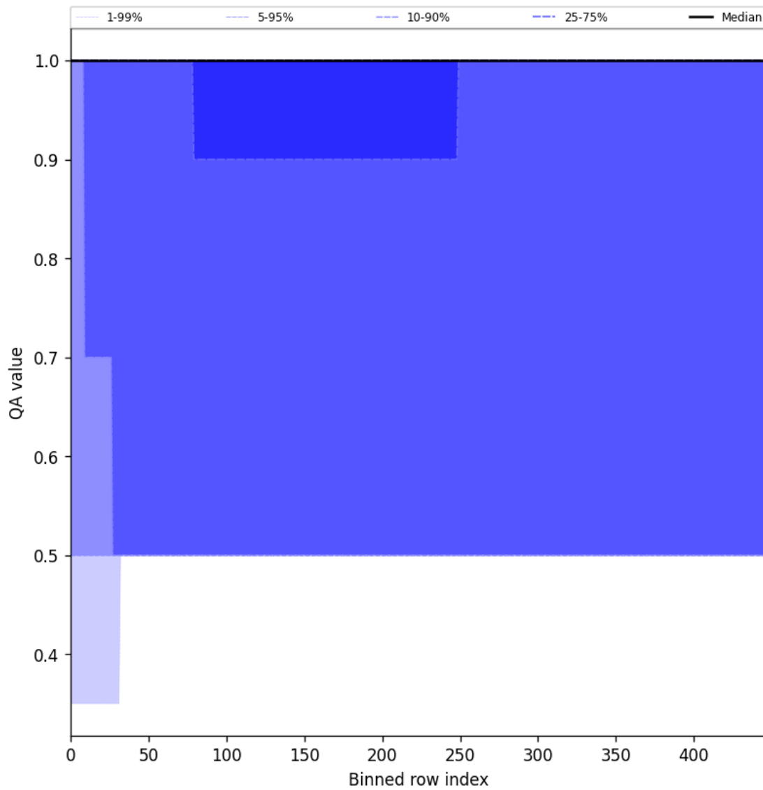
Figure 46: Along track statistics of “QA value” for 2025-05-02 to 2025-05-04
