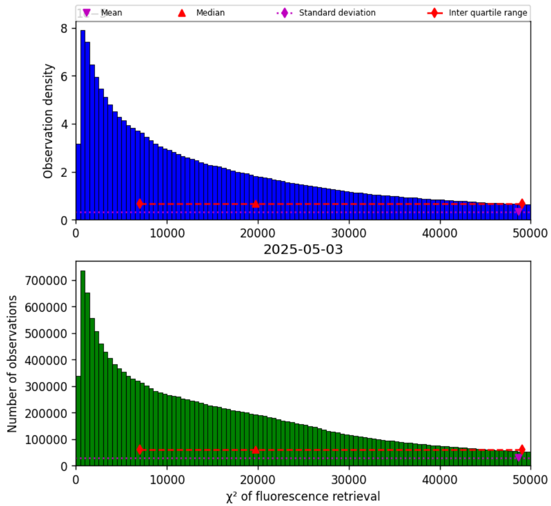
Figure 42: Histogram of “ \chi^2 of fluorescence retrieval” for 2025-05-02 to 2025-05-04
