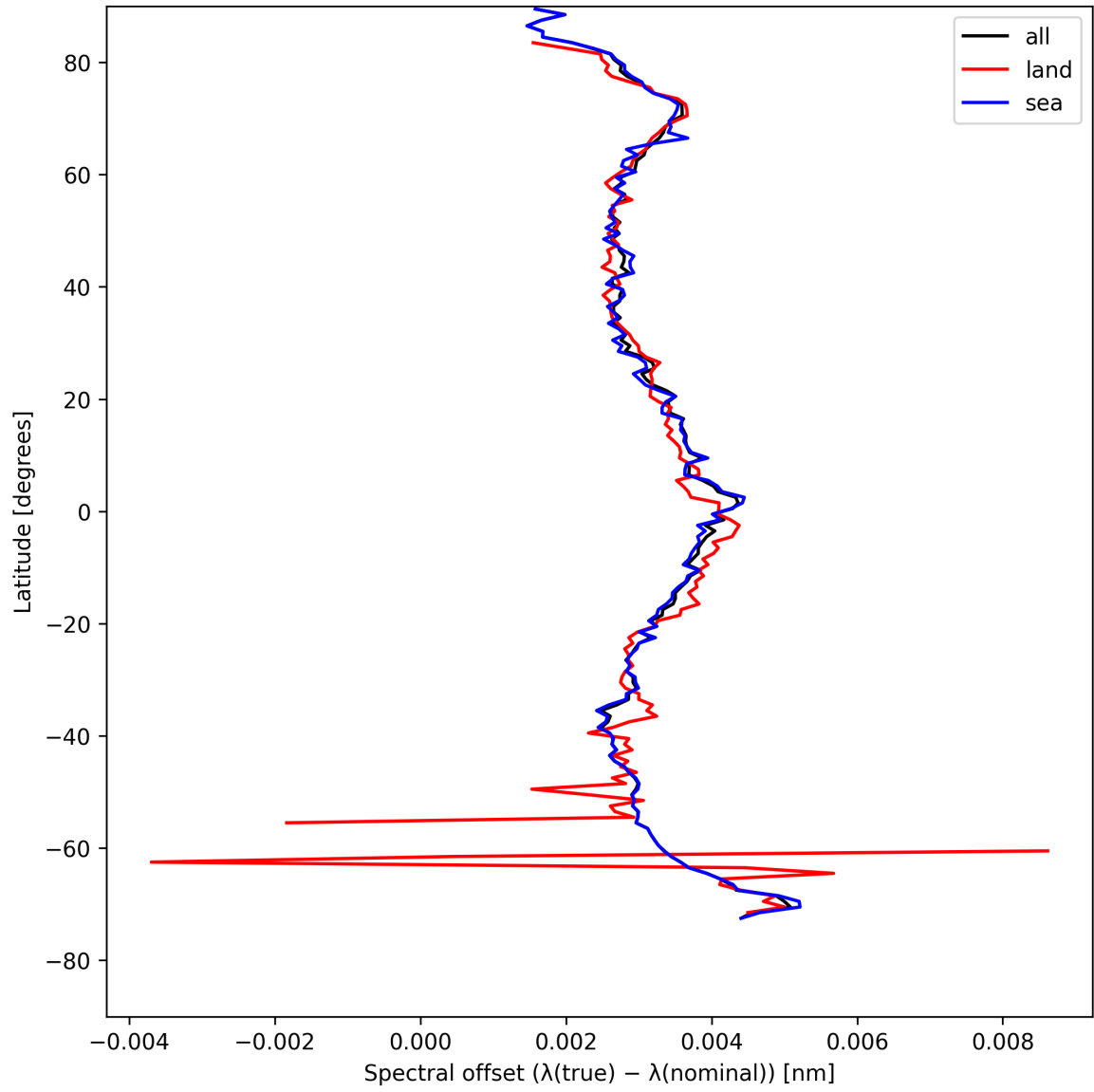
Figure 28: Zonal average of “Spectral offset ( \lambda_{\text{true}} - \lambda_{\text{nominal}} )” for 2025-05-02 to 2025-05-04.
