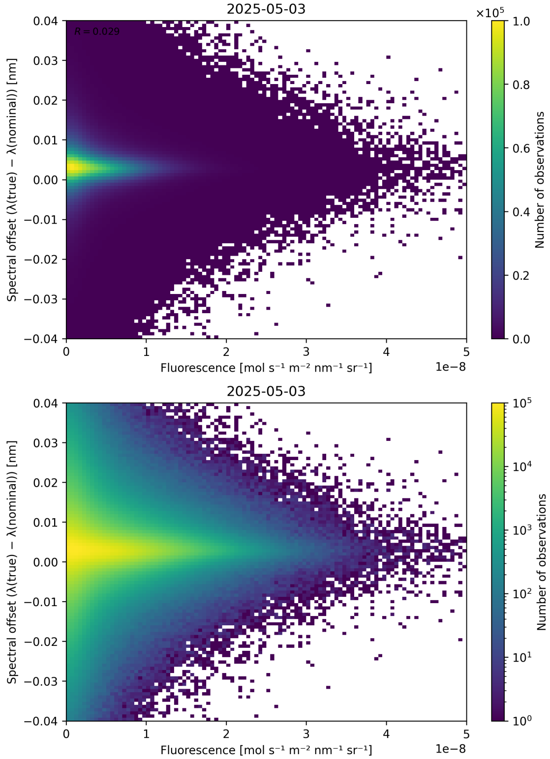
Figure 87: Scatter density plot of “Fluorescence” against “Spectral offset ( \lambda_{\text{true}} - \lambda_{\text{nominal}} )” for 2025-05-02 to 2025-05-04.
