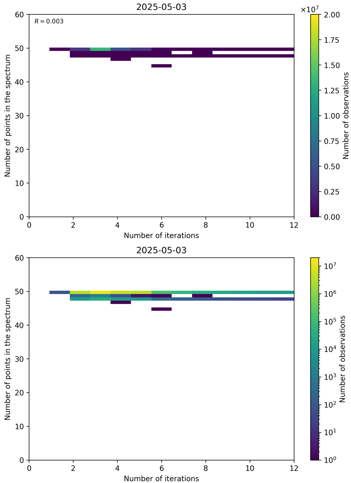
Figure 99: Scatter density plot of “Number of iterations” against “Number of points in the spectrum” for 2025-05-02 to 2025-05-04.
