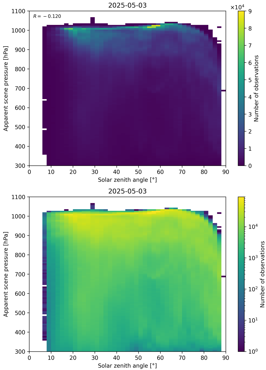
Figure 108: Scatter density plot of “Solar zenith angle” against “Apparent scene pressure” for 2025-05-02 to 2025-05-04.
