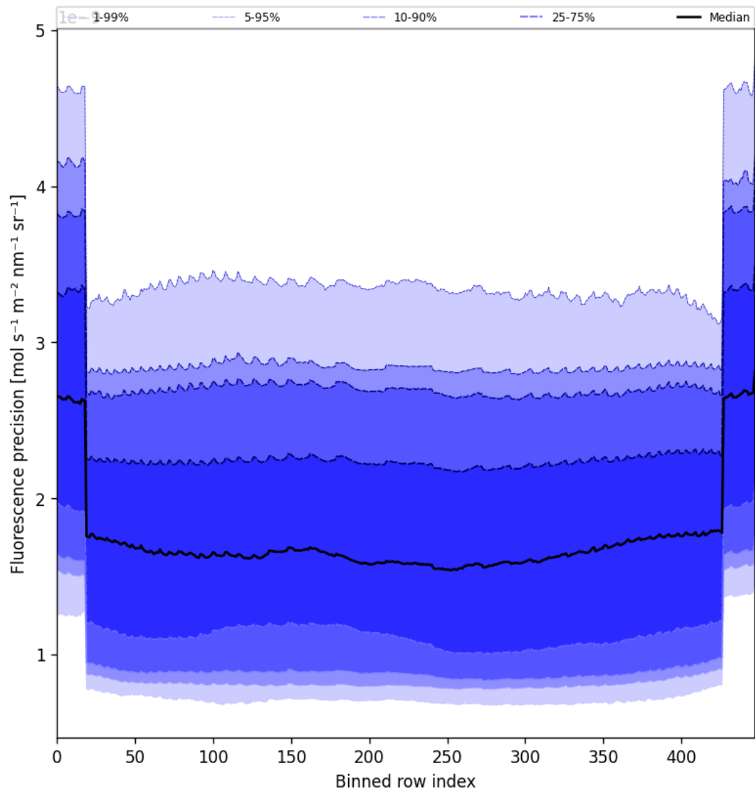
Figure 58: Along track statistics of “Fluorescence precision” for 2025-05-02 to 2025-05-04
