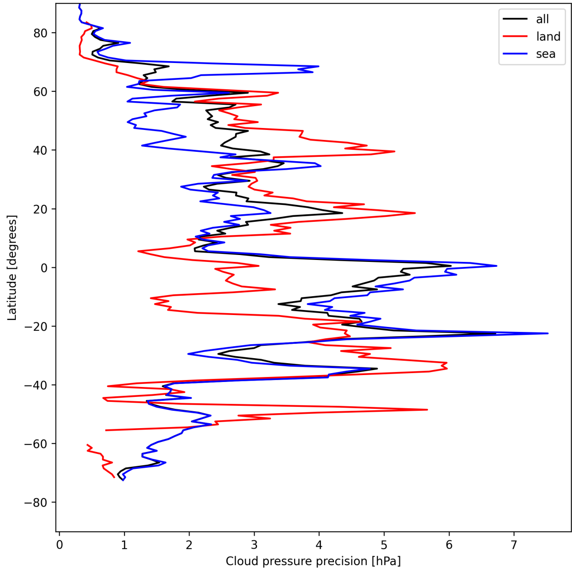
Figure 14: Zonal average of “Cloud pressure precision” for 2025-05-02 to 2025-05-04.
