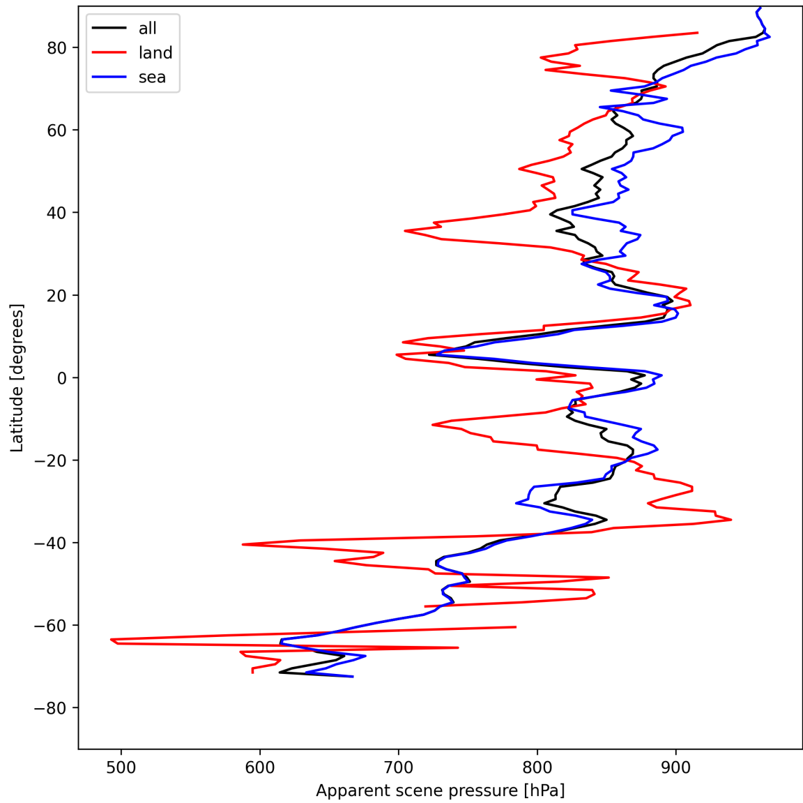
Figure 19: Zonal average of “Apparent scene pressure” for 2025-05-02 to 2025-05-04.
