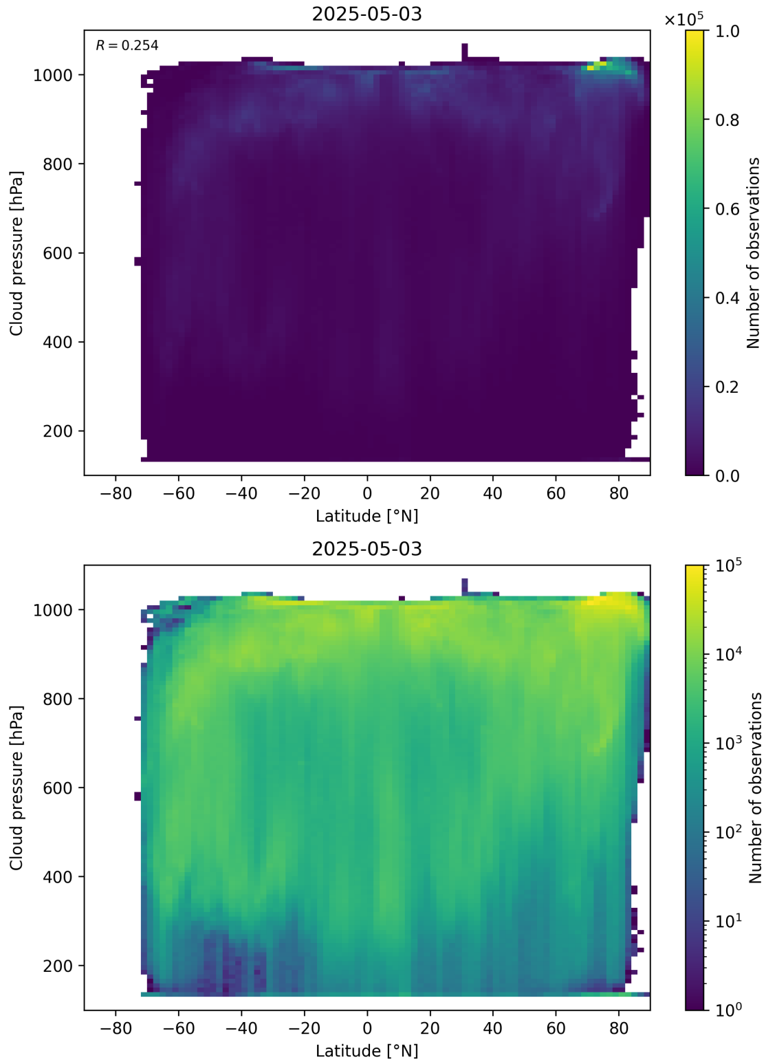
Figure 91: Scatter density plot of “Latitude” against “Cloud pressure” for 2025-05-02 to 2025-05-04.
