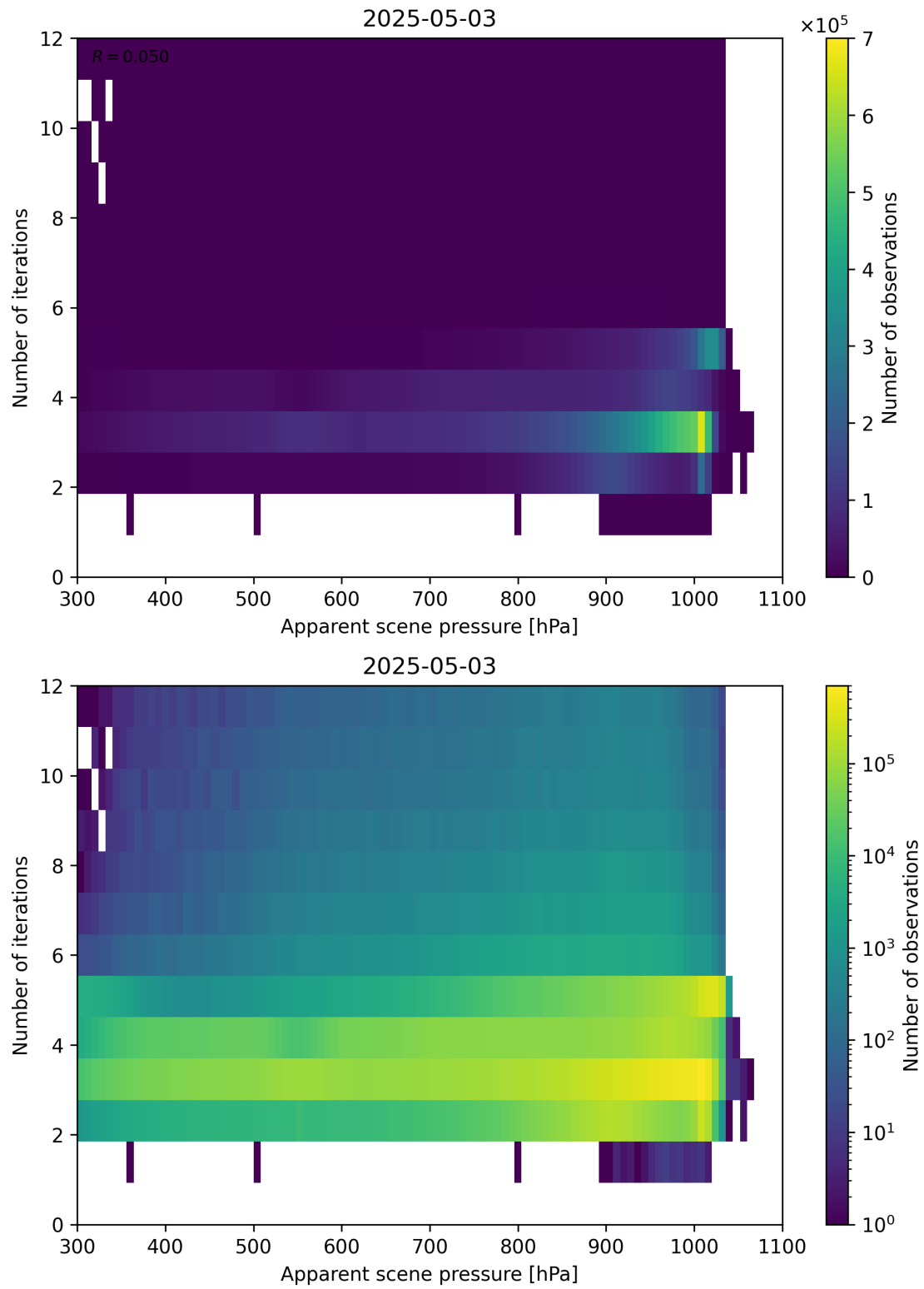
Figure 65: Scatter density plot of “Apparent scene pressure” against “Number of iterations” for 2025-05-02 to 2025-05-04.
