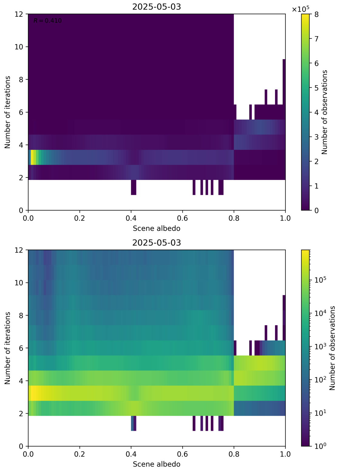
Figure 105: Scatter density plot of “Scene albedo” against “Number of iterations” for 2025-05-02 to 2025-05-04.
