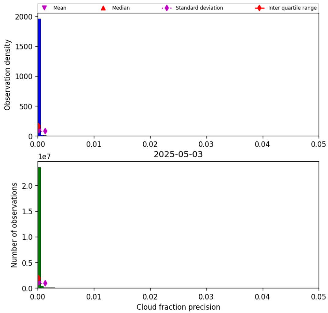
Figure 33: Histogram of “Cloud fraction precision” for 2025-05-02 to 2025-05-04
