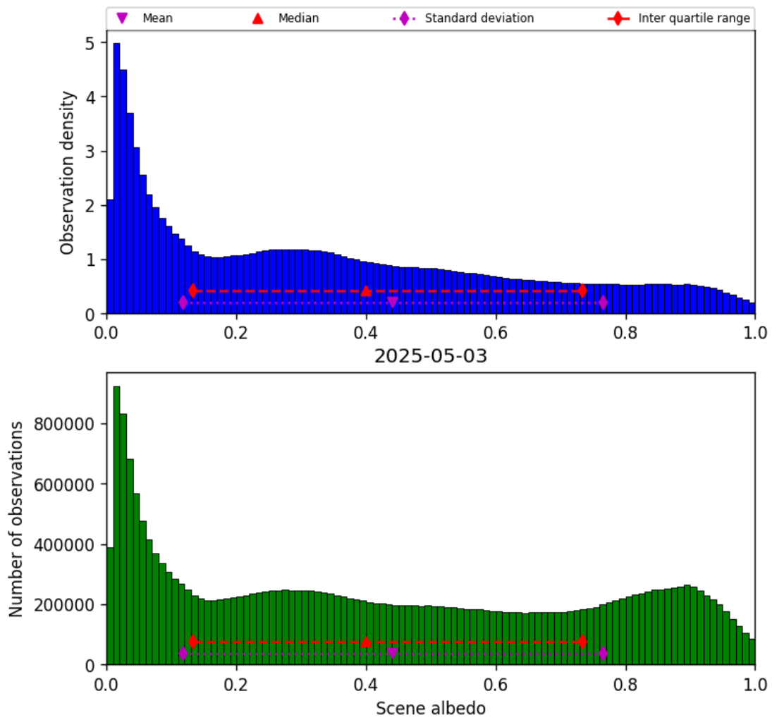
Figure 34: Histogram of “Scene albedo” for 2025-05-02 to 2025-05-04
