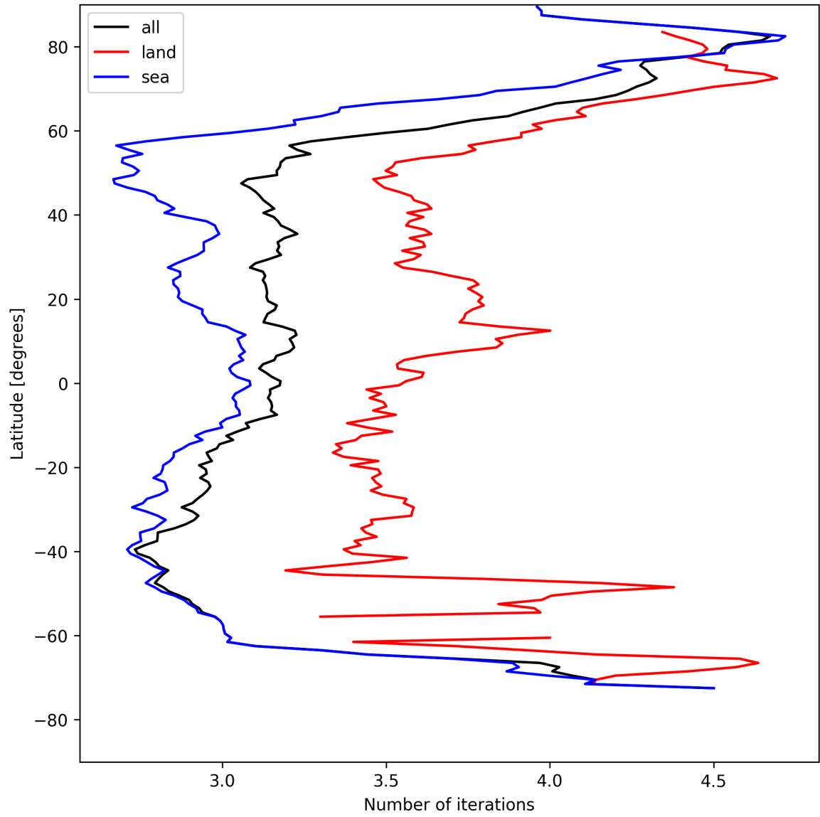
Figure 22: Zonal average of “Number of iterations” for 2025-05-02 to 2025-05-04.
