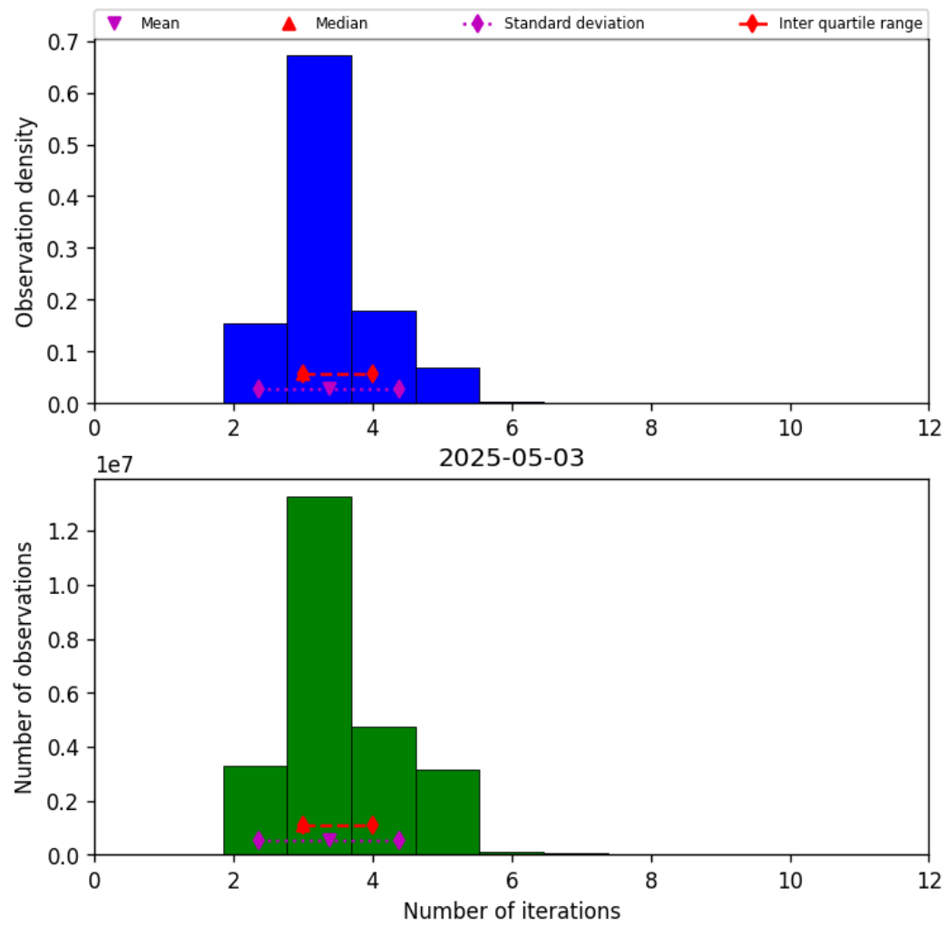
Figure 39: Histogram of “Number of iterations” for 2025-05-02 to 2025-05-04
