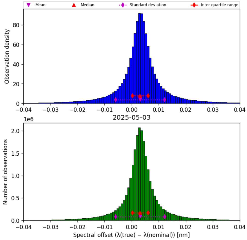
Figure 45: Histogram of “Spectral offset ( \lambda_{\text{true}} - \lambda_{\text{nominal}} )” for 2025-05-02 to 2025-05-04
