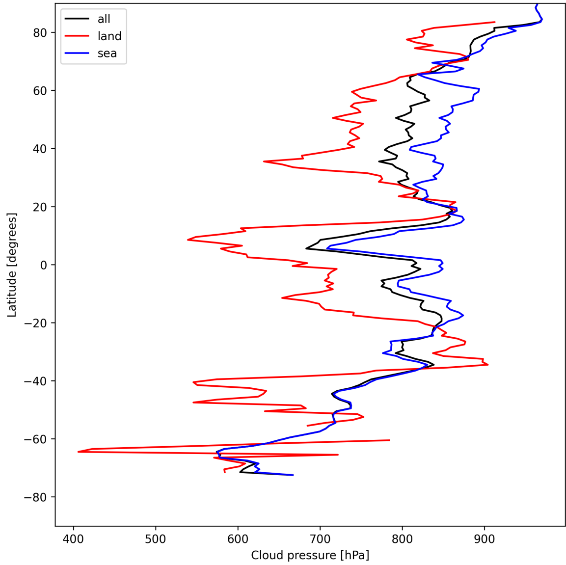
Figure 13: Zonal average of “Cloud pressure” for 2025-05-02 to 2025-05-04.
