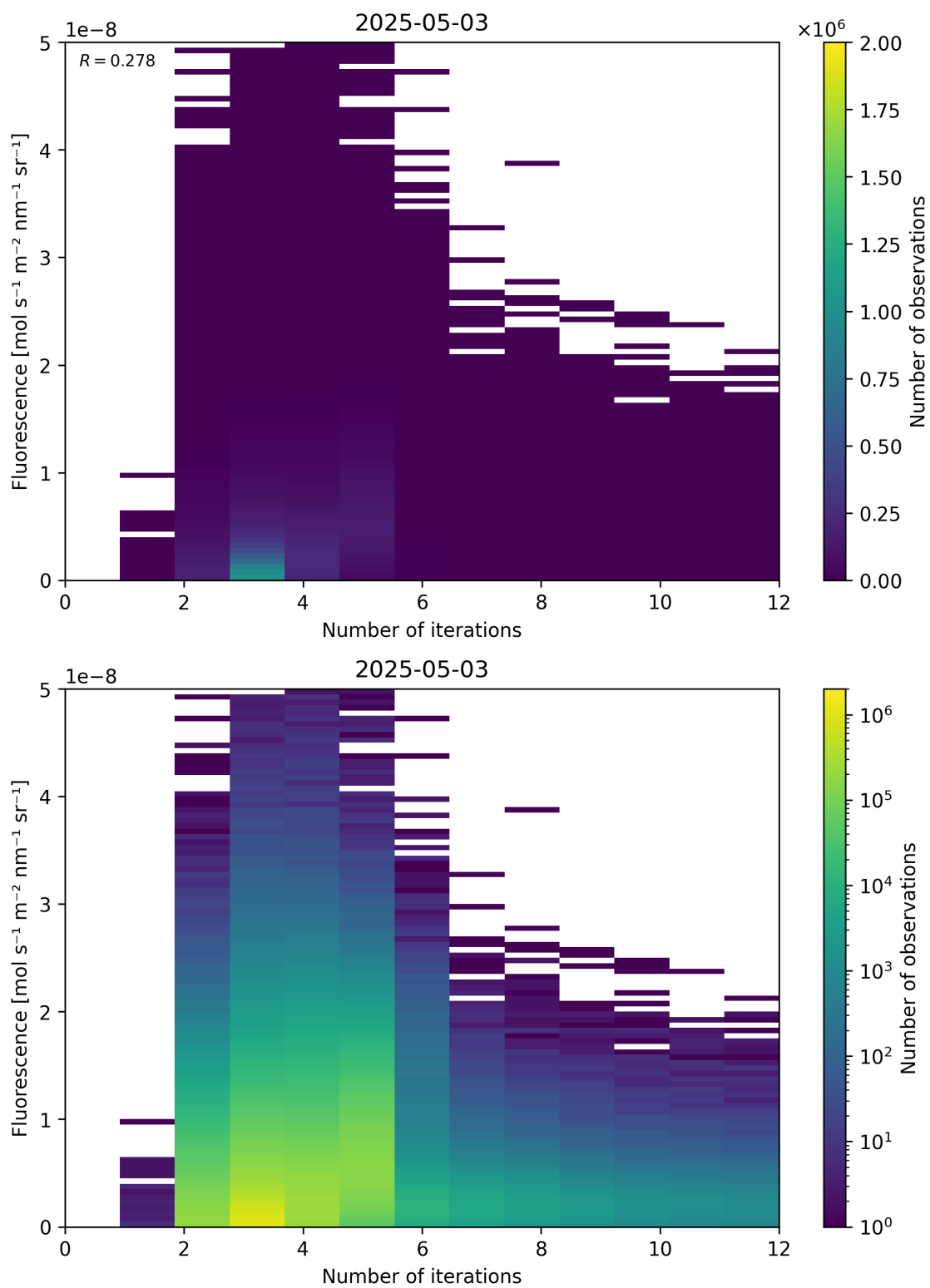
Figure 98: Scatter density plot of “Number of iterations” against “Fluorescence” for 2025-05-02 to 2025-05-04.
