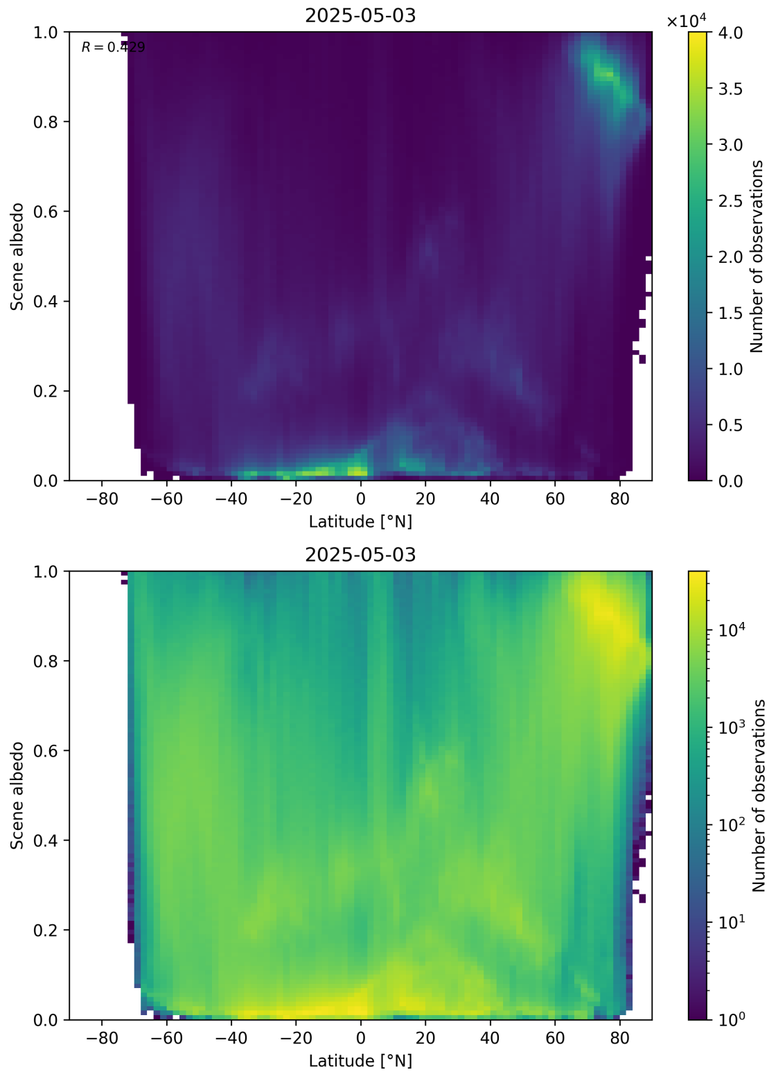
Figure 95: Scatter density plot of “Latitude” against “Scene albedo” for 2025-05-02 to 2025-05-04.
