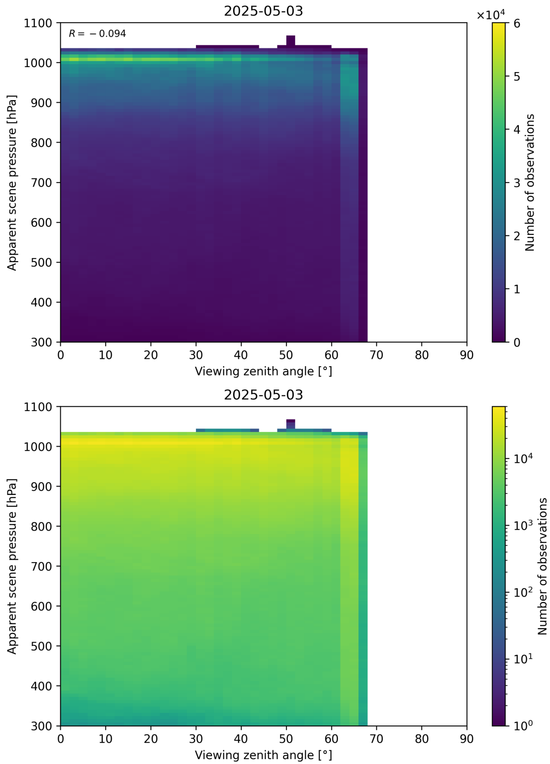
Figure 118: Scatter density plot of “Viewing zenith angle” against “Apparent scene pressure” for 2025-05-02 to 2025-05-04.
