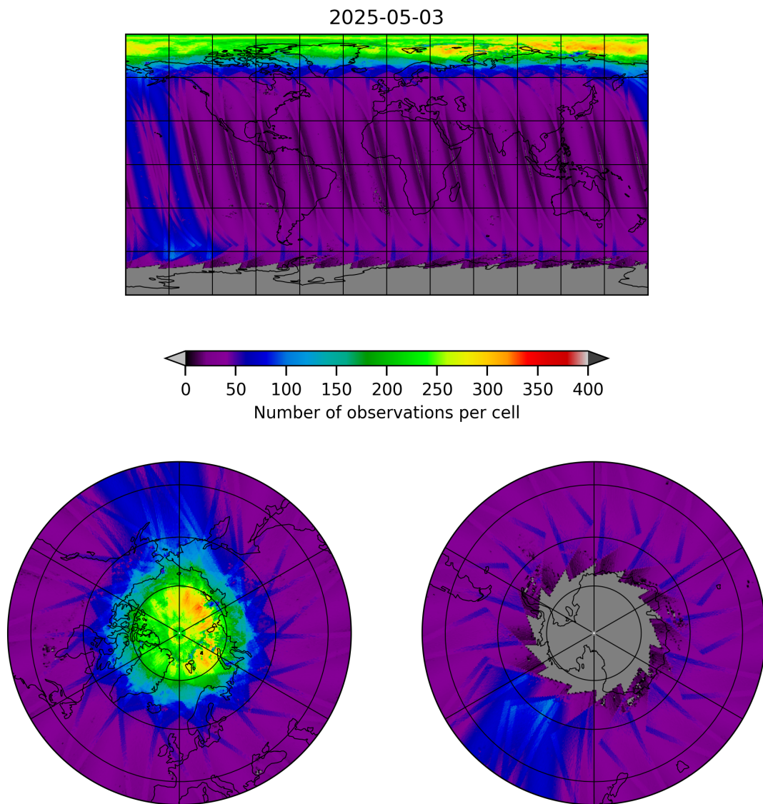
Figure 11: Map of the number of observations for 2025-05-02 to 2025-05-04
