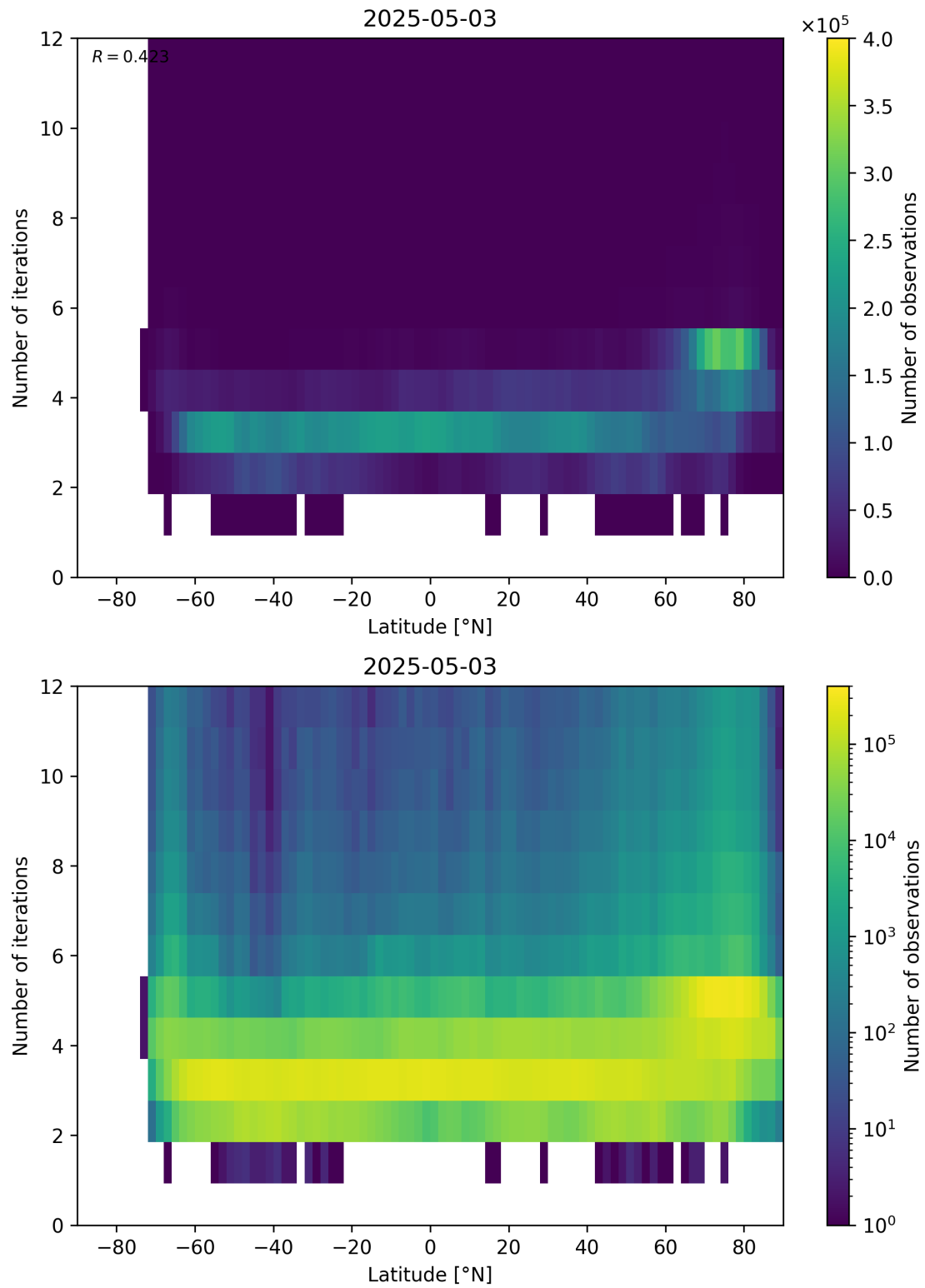
Figure 93: Scatter density plot of “Latitude” against “Number of iterations” for 2025-05-02 to 2025-05-04.
