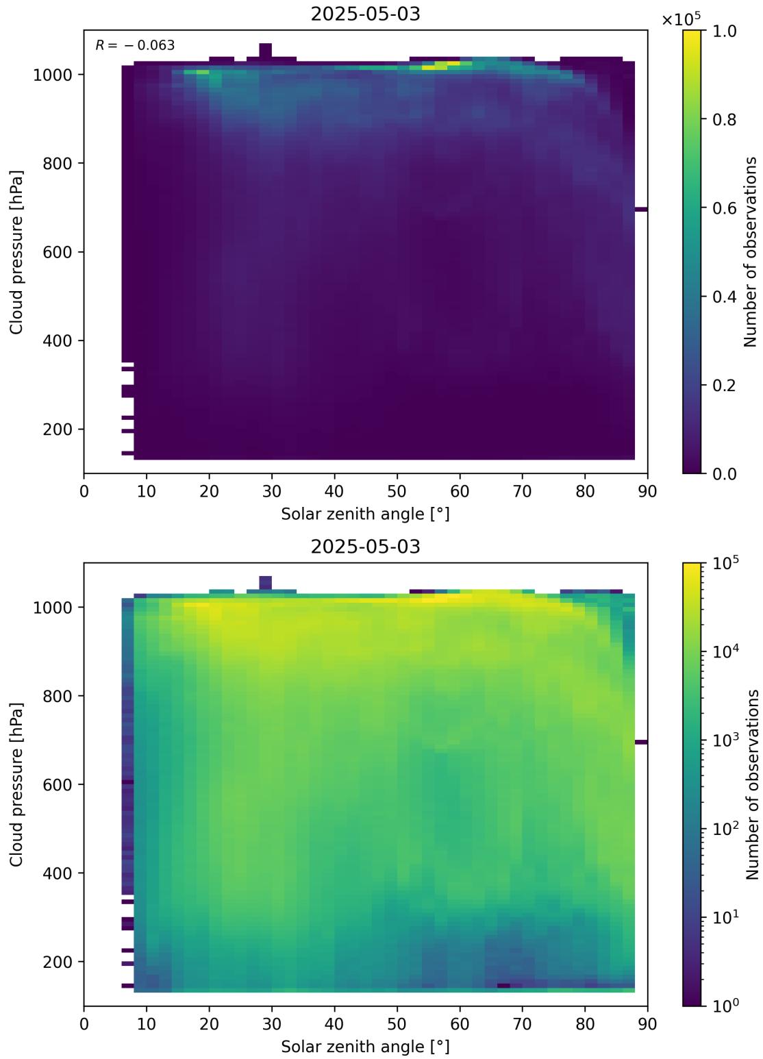
Figure 111: Scatter density plot of “Solar zenith angle” against “Cloud pressure” for 2025-05-02 to 2025-05-04.
