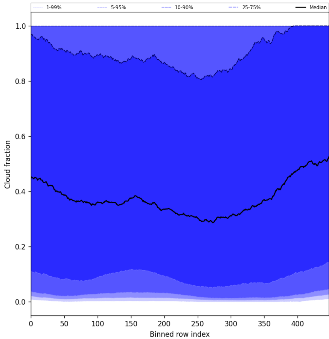
Figure 49: Along track statistics of “Cloud fraction” for 2025-05-02 to 2025-05-04
