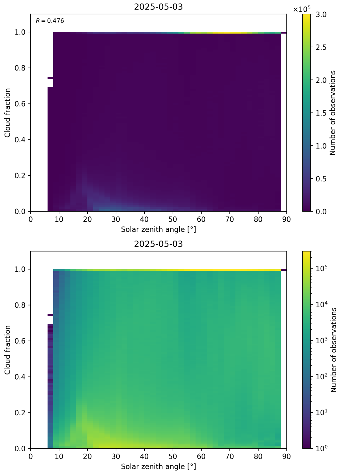
Figure 110: Scatter density plot of “Solar zenith angle” against “Cloud fraction” for 2025-05-02 to 2025-05-04.
