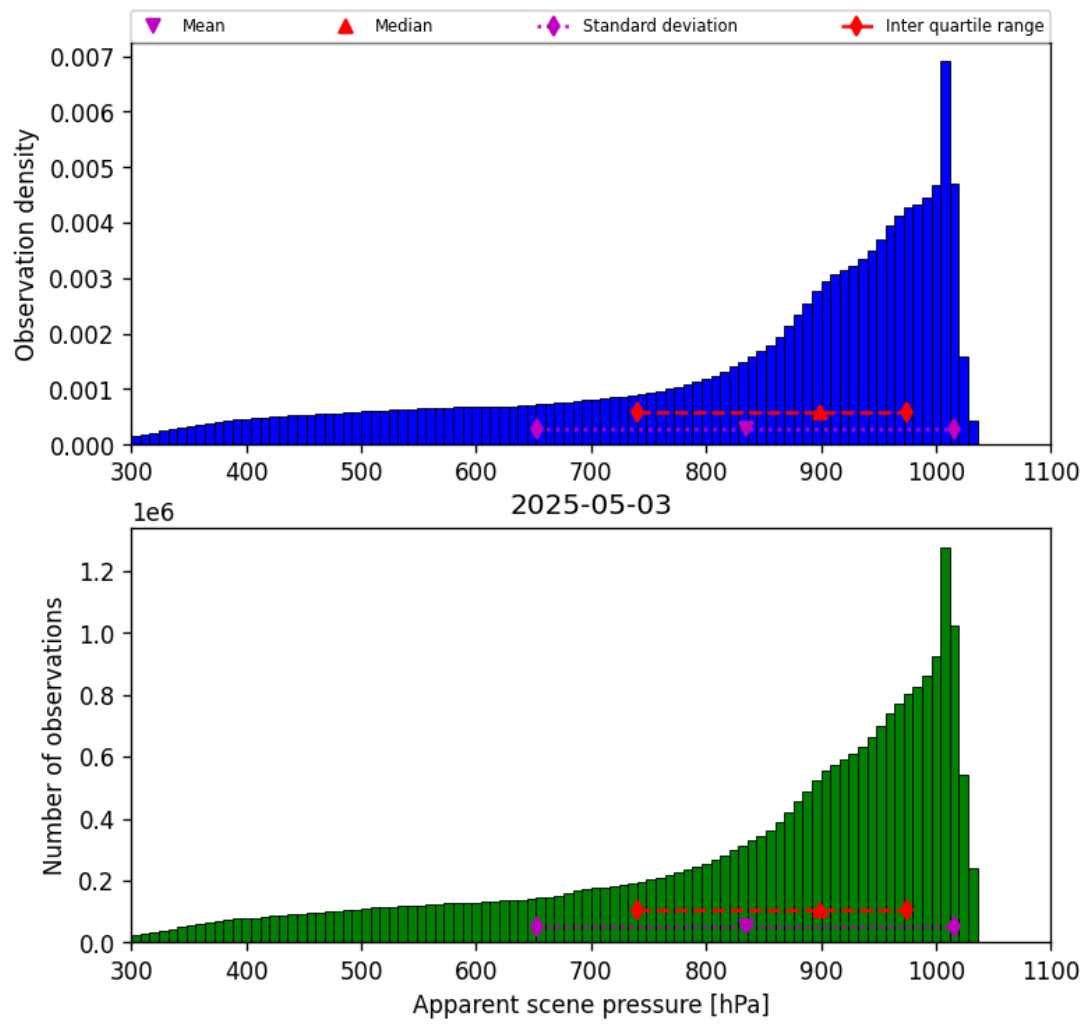
Figure 36: Histogram of “Apparent scene pressure” for 2025-05-02 to 2025-05-04
