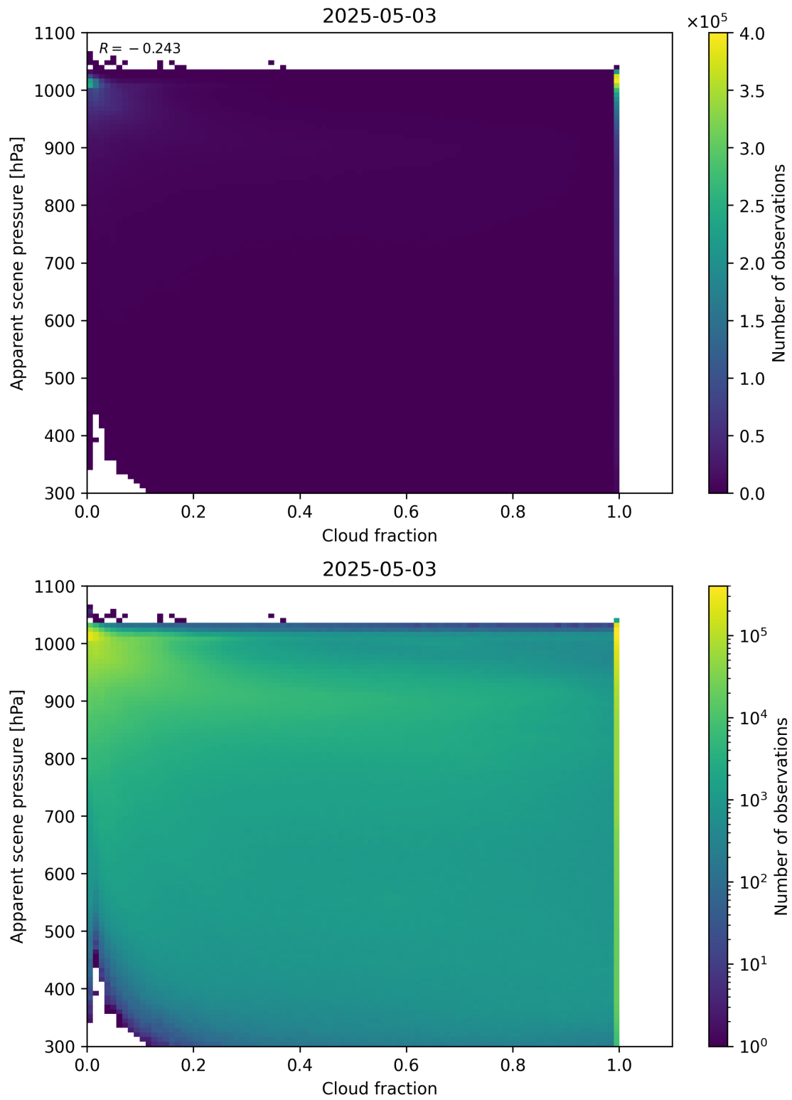
Figure 70: Scatter density plot of “Cloud fraction” against “Apparent scene pressure” for 2025-05-02 to 2025-05-04.
