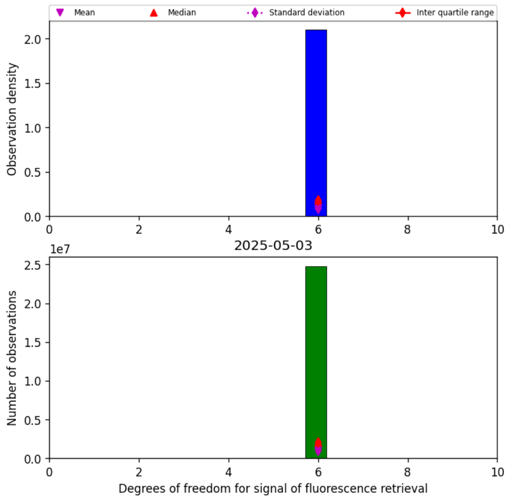
Figure 43: Histogram of “Degrees of freedom for signal of fluorescence retrieval” for 2025-05-02 to 2025-05-04
