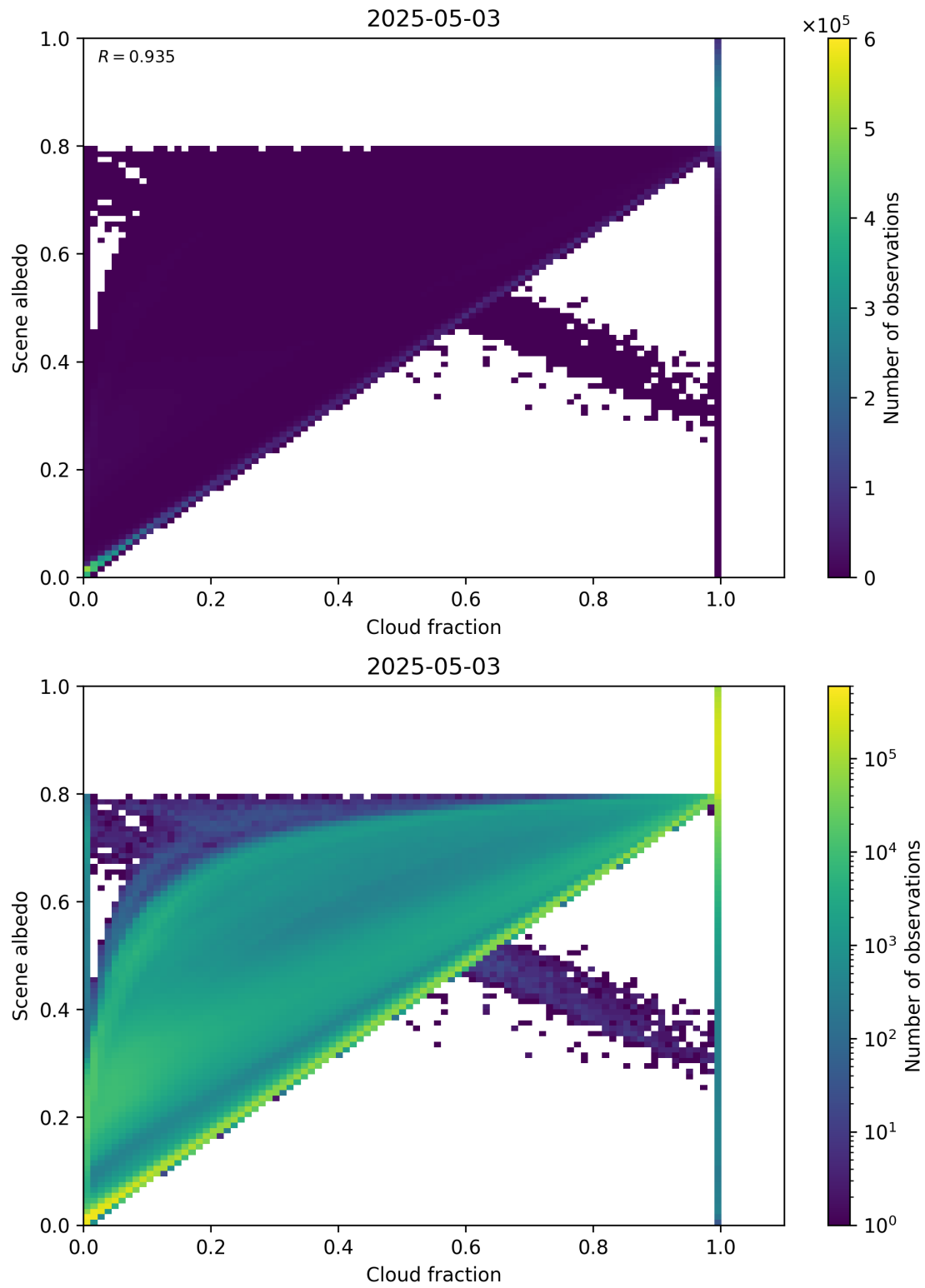
Figure 75: Scatter density plot of “Cloud fraction” against “Scene albedo” for 2025-05-02 to 2025-05-04.
