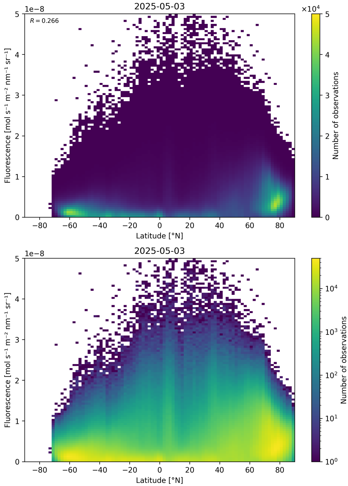
Figure 92: Scatter density plot of “Latitude” against “Fluorescence” for 2025-05-02 to 2025-05-04.
