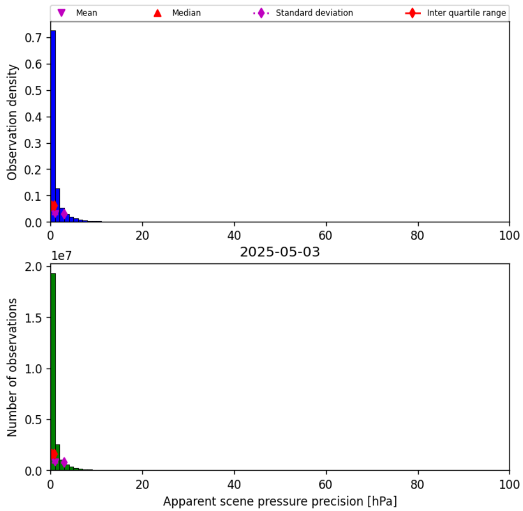
Figure 37: Histogram of “Apparent scene pressure precision” for 2025-05-02 to 2025-05-04
