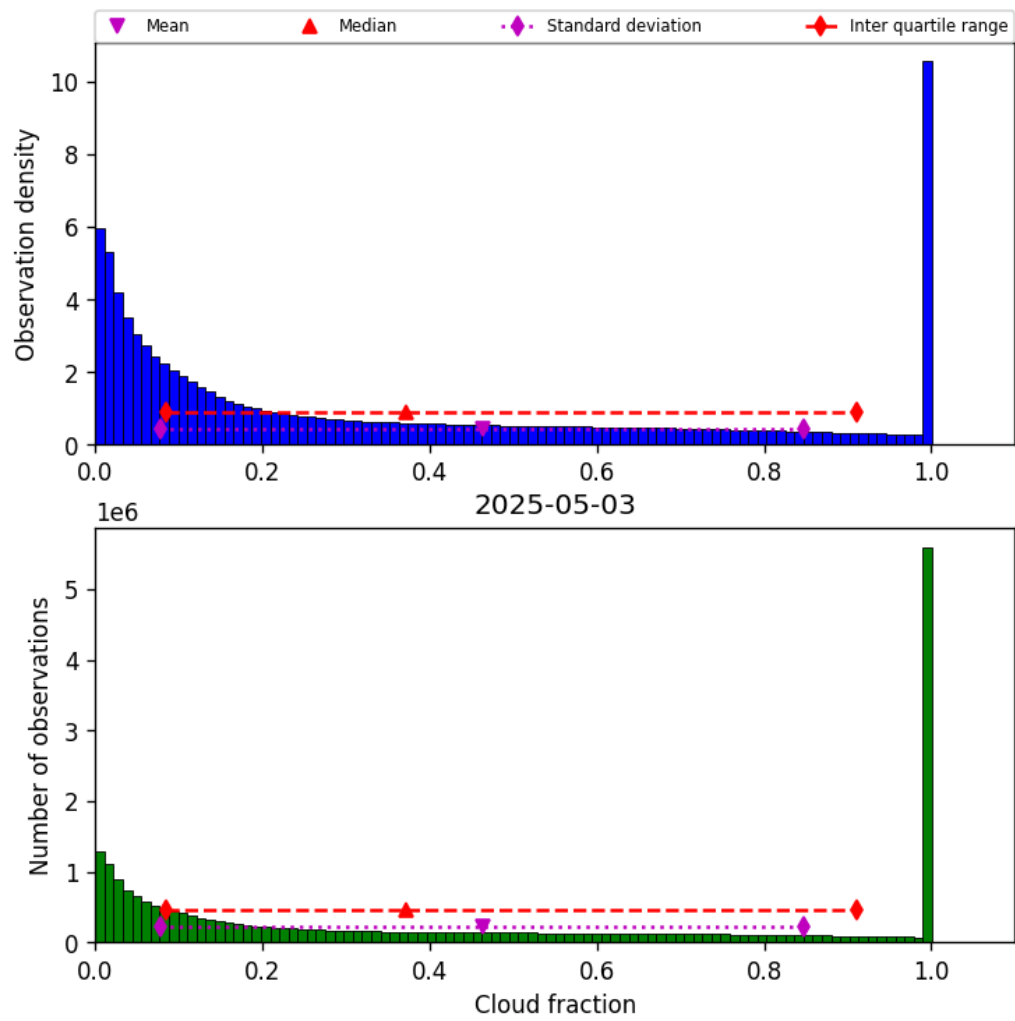
Figure 32: Histogram of “Cloud fraction” for 2025-05-02 to 2025-05-04
