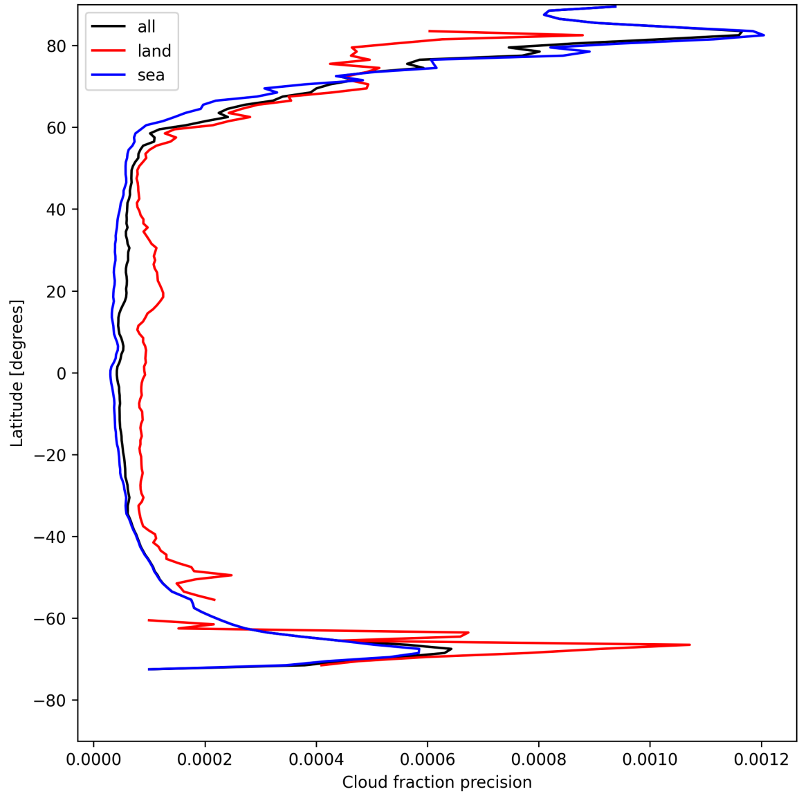
Figure 16: Zonal average of “Cloud fraction precision” for 2025-05-02 to 2025-05-04.
