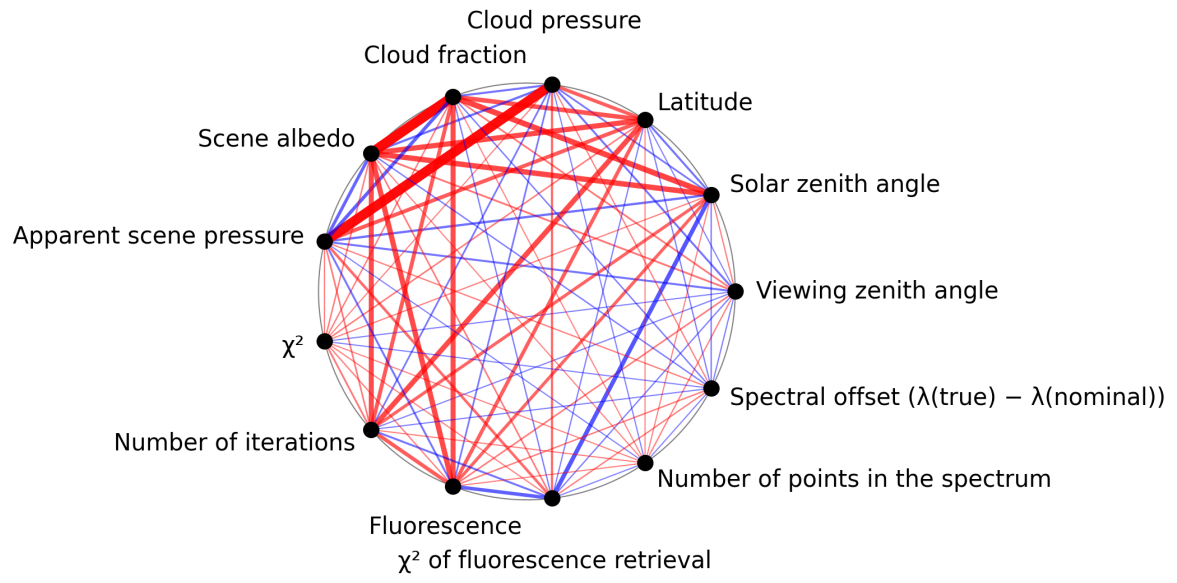
Figure 1: Map of correlation graph for 2025-05-02 to 2025-05-04.
