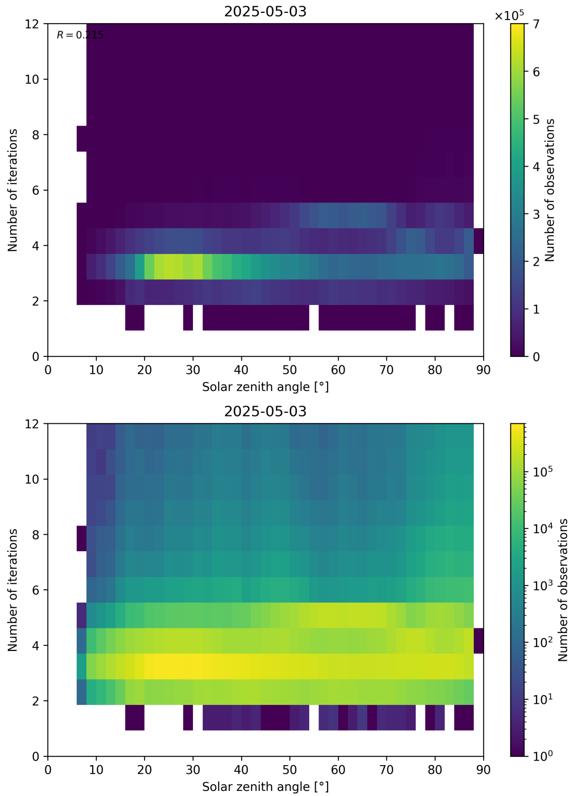
Figure 114: Scatter density plot of “Solar zenith angle” against “Number of iterations” for 2025-05-02 to 2025-05-04.
