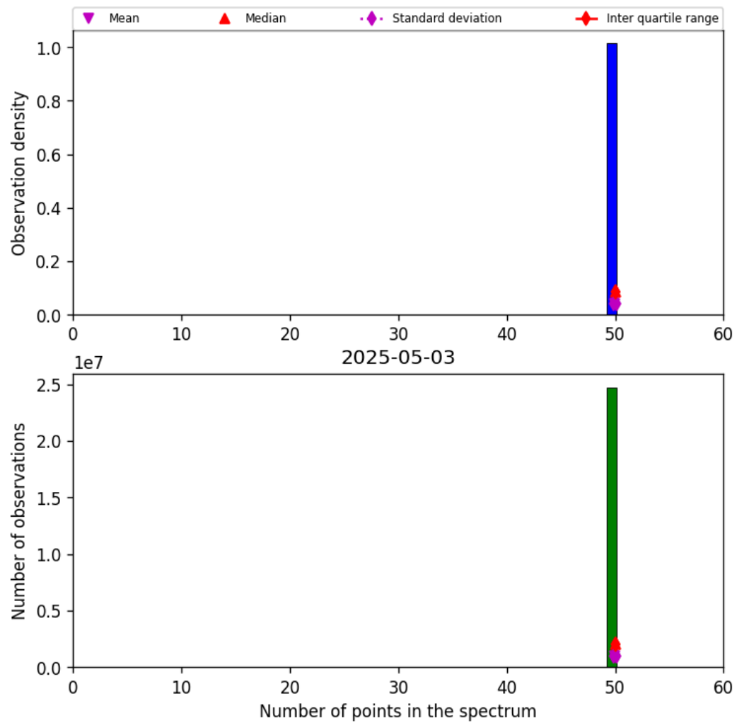
Figure 44: Histogram of “Number of points in the spectrum” for 2025-05-02 to 2025-05-04
