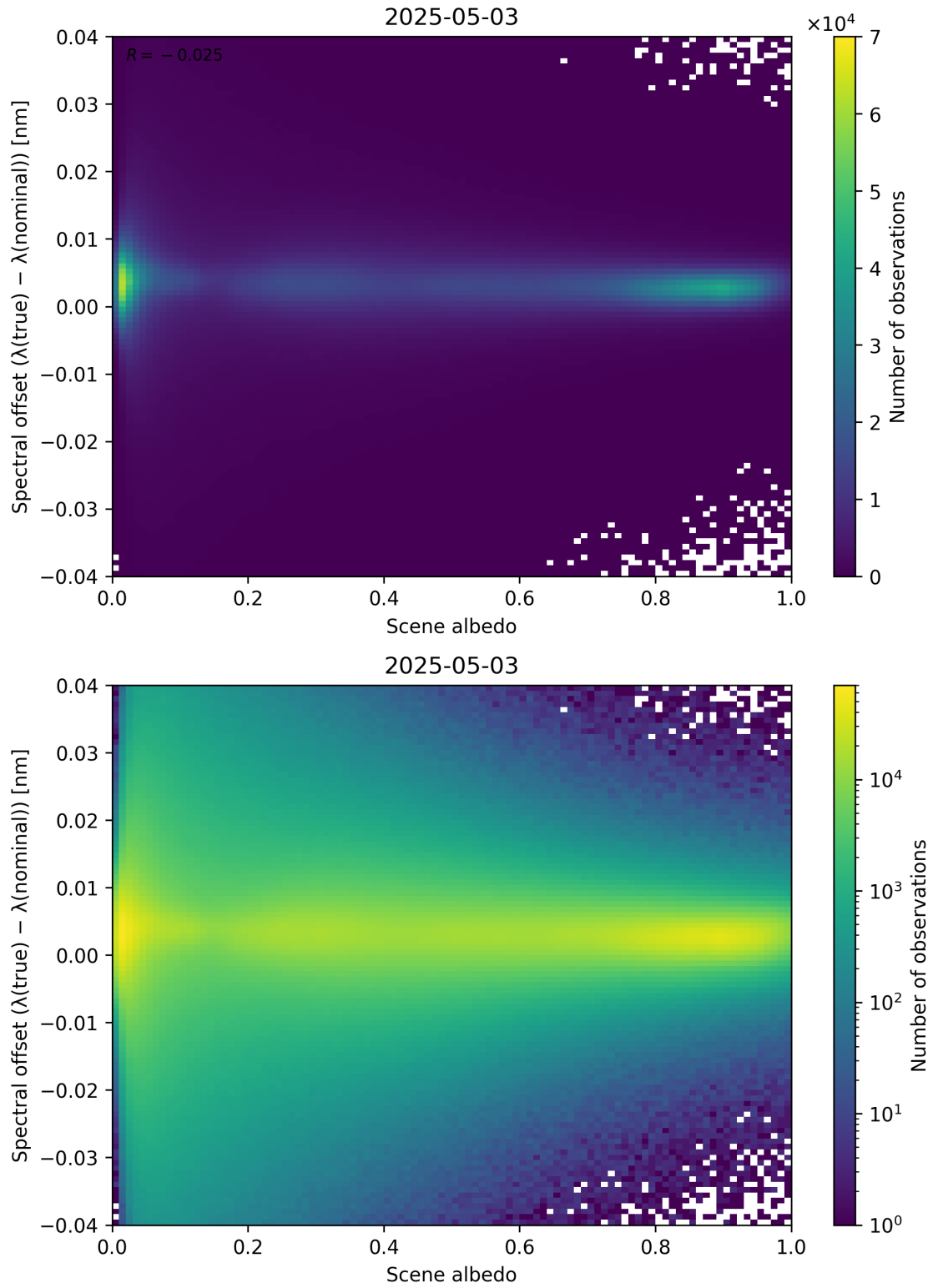
Figure 107: Scatter density plot of “Scene albedo” against “Spectral offset ( \lambda_{\text{true}} - \lambda_{\text{nominal}} )” for 2025-05-02 to 2025-05-04.
