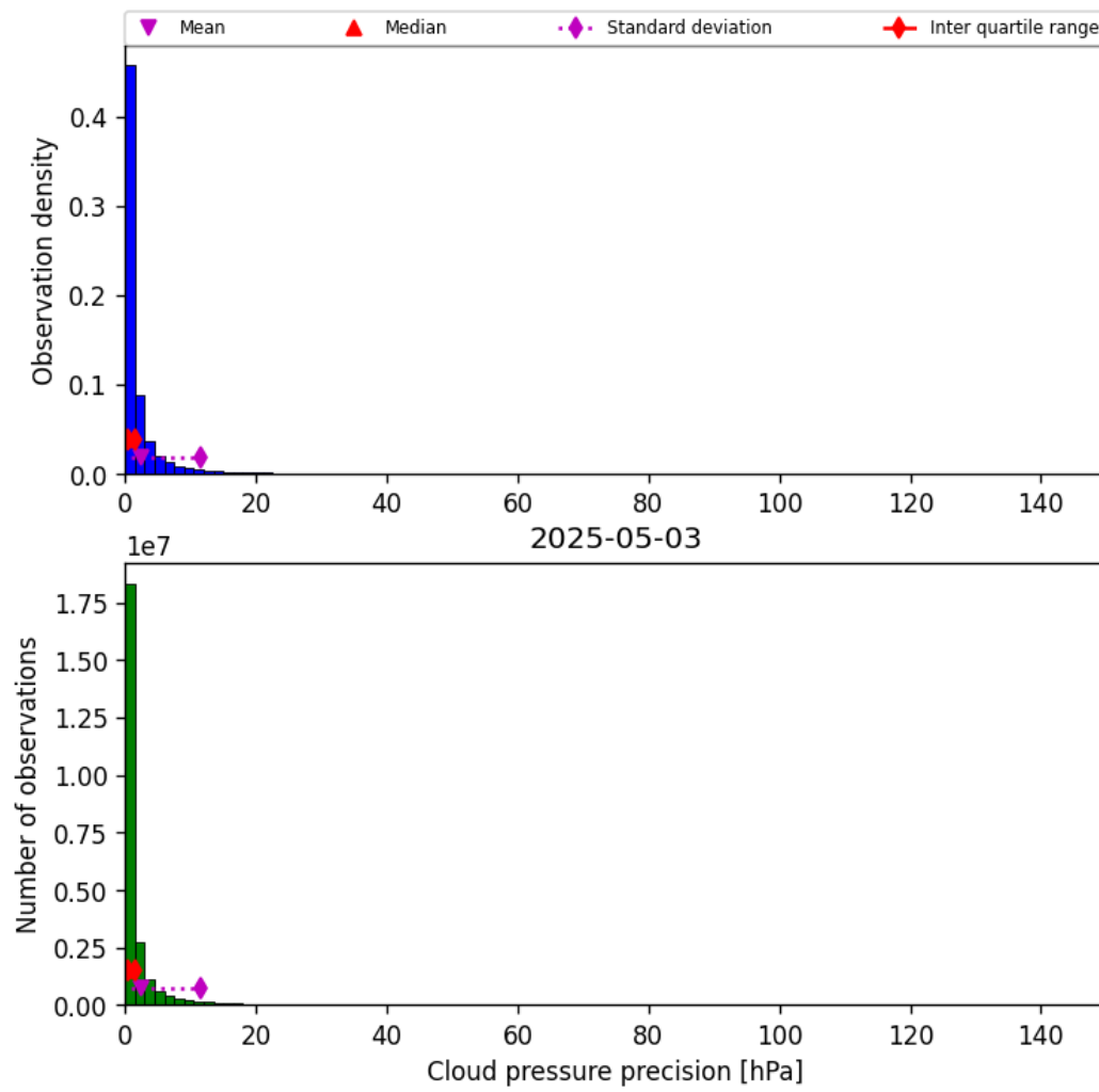
Figure 31: Histogram of “Cloud pressure precision” for 2025-05-02 to 2025-05-04
