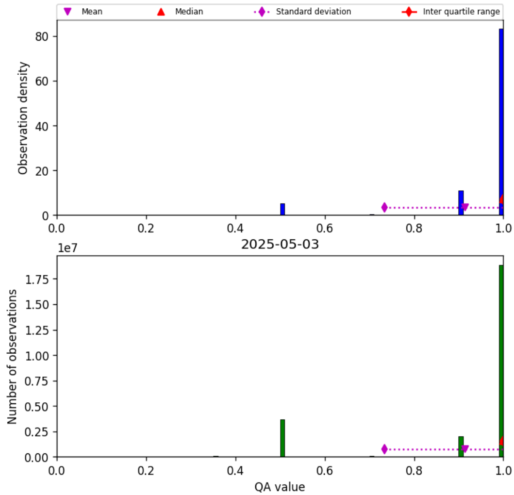
Figure 29: Histogram of “QA value” for 2025-05-02 to 2025-05-04
