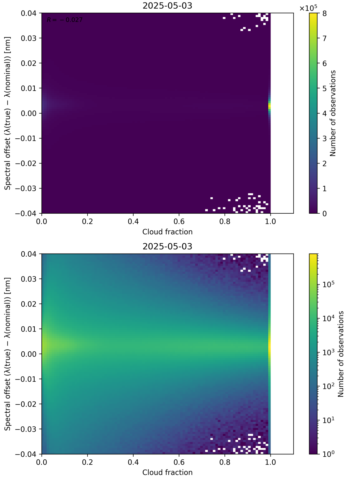
Figure 76: Scatter density plot of “Cloud fraction” against “Spectral offset ( \lambda_{\text{true}} - \lambda_{\text{nominal}} )” for 2025-05-02 to 2025-05-04.
