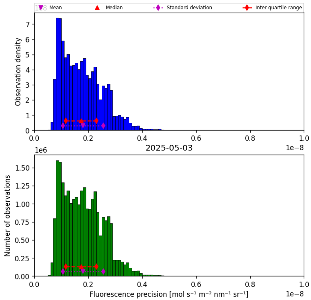
Figure 41: Histogram of “Fluorescence precision” for 2025-05-02 to 2025-05-04
