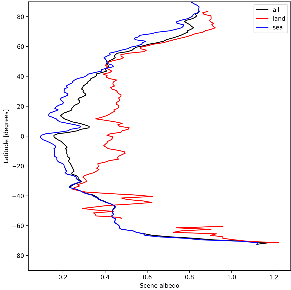
Figure 17: Zonal average of “Scene albedo” for 2025-05-02 to 2025-05-04.
