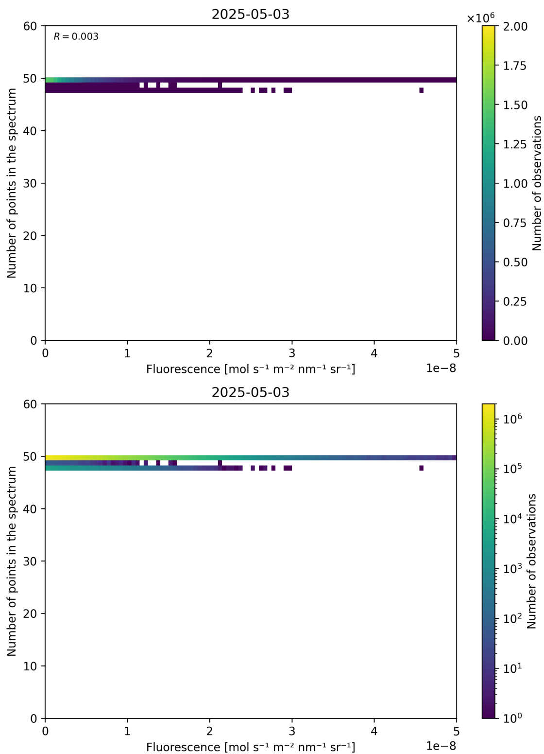
Figure 86: Scatter density plot of “Fluorescence” against “Number of points in the spectrum” for 2025-05-02 to 2025-05-04.
