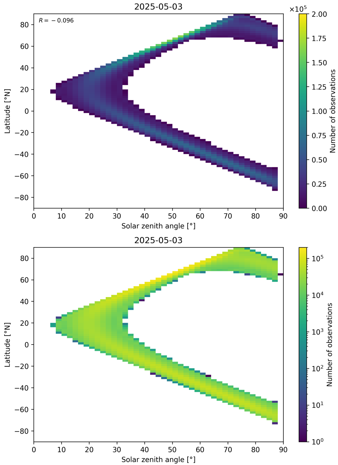
Figure 113: Scatter density plot of “Solar zenith angle” against “Latitude” for 2025-05-02 to 2025-05-04.
