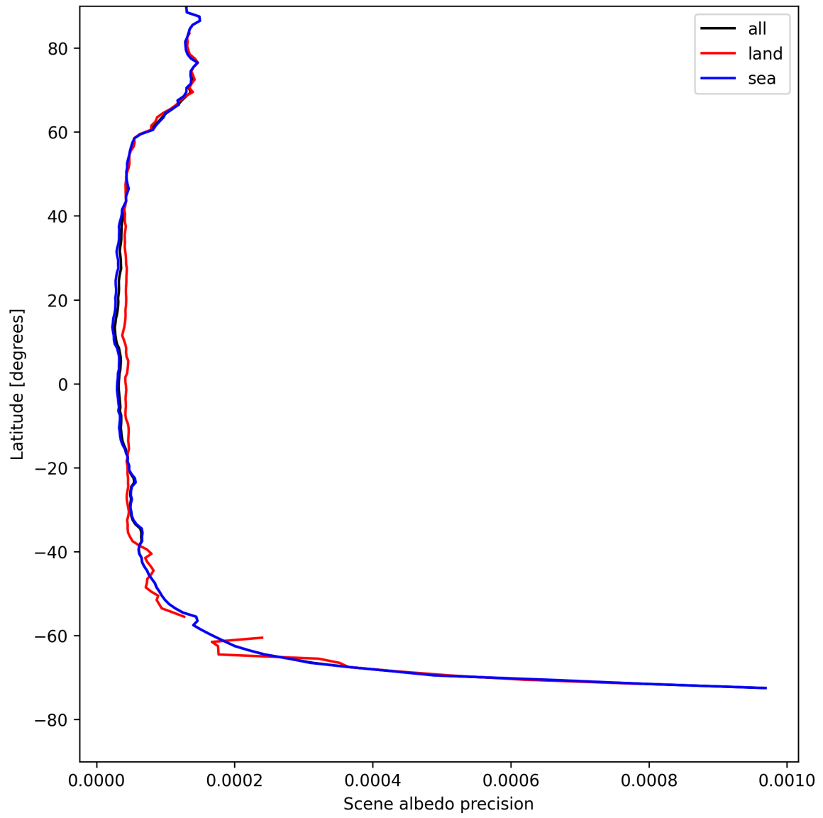
Figure 18: Zonal average of “Scene albedo precision” for 2025-05-02 to 2025-05-04.
