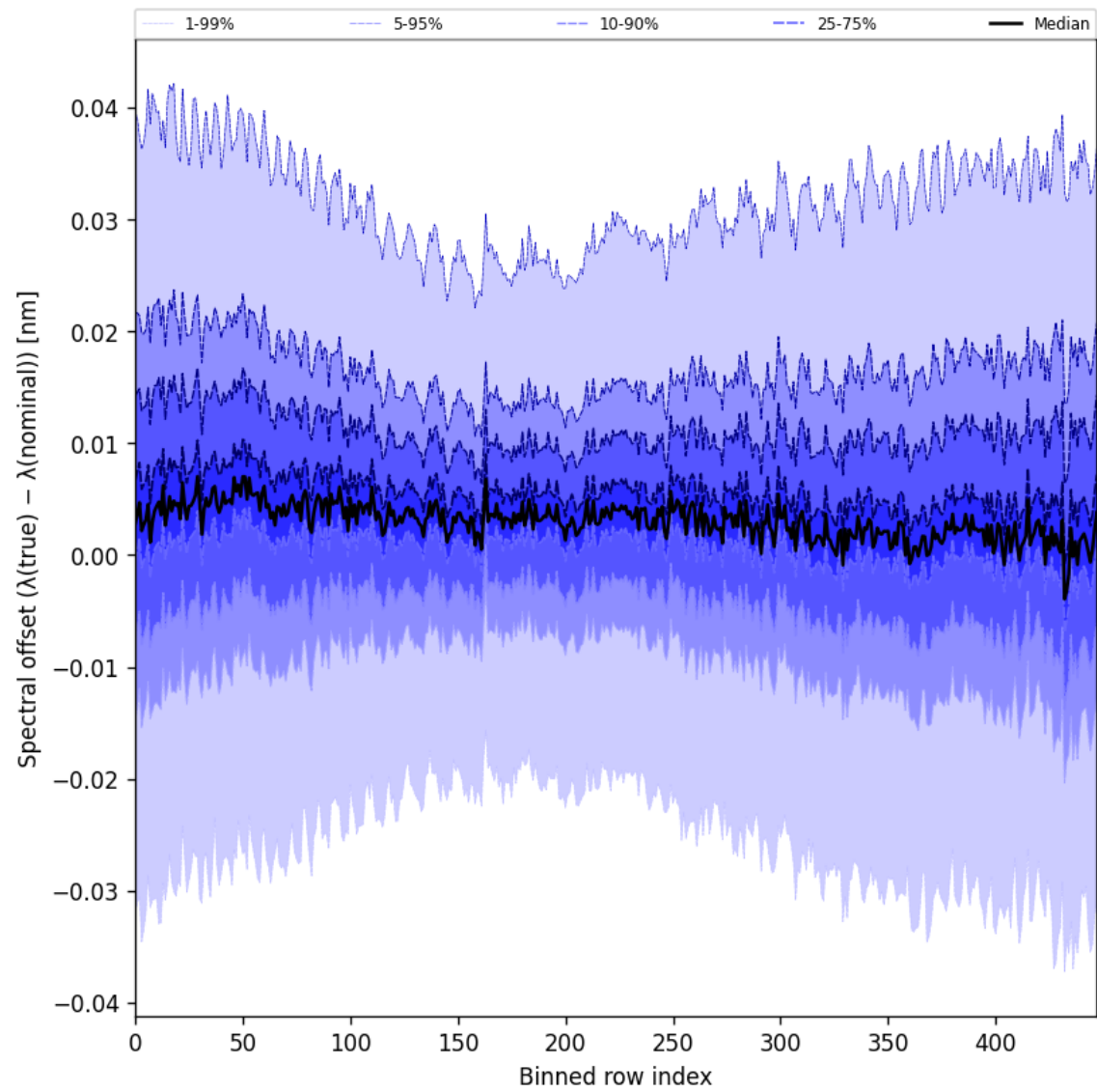
Figure 62: Along track statistics of “Spectral offset ( \lambda_{\text{true}} - \lambda_{\text{nominal}} )” for 2025-05-02 to 2025-05-04
