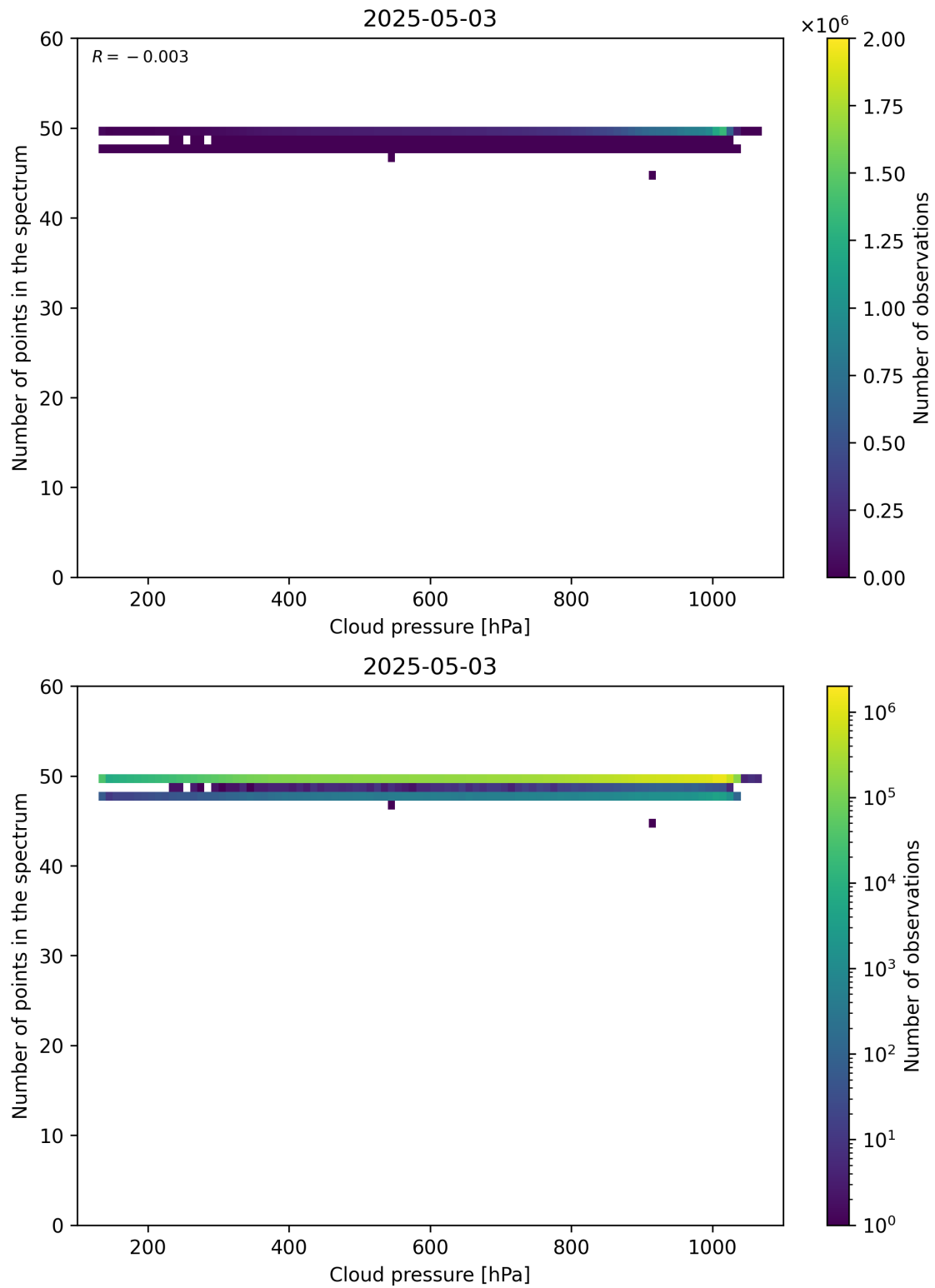
Figure 82: Scatter density plot of “Cloud pressure” against “Number of points in the spectrum” for 2025-05-02 to 2025-05-04.
