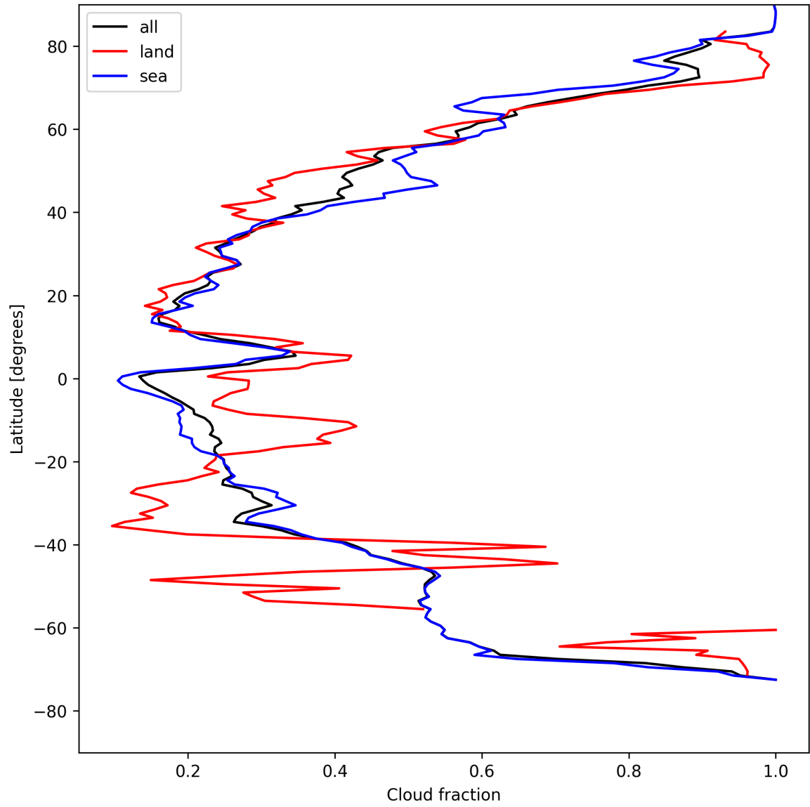
Figure 15: Zonal average of “Cloud fraction” for 2025-05-02 to 2025-05-04.
