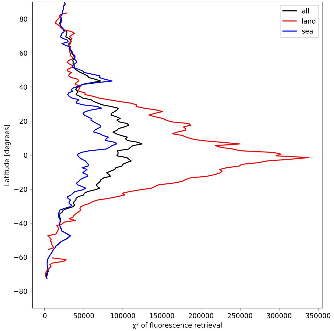
Figure 25: Zonal average of “ \chi^2 of fluorescence retrieval” for 2025-05-02 to 2025-05-04.
