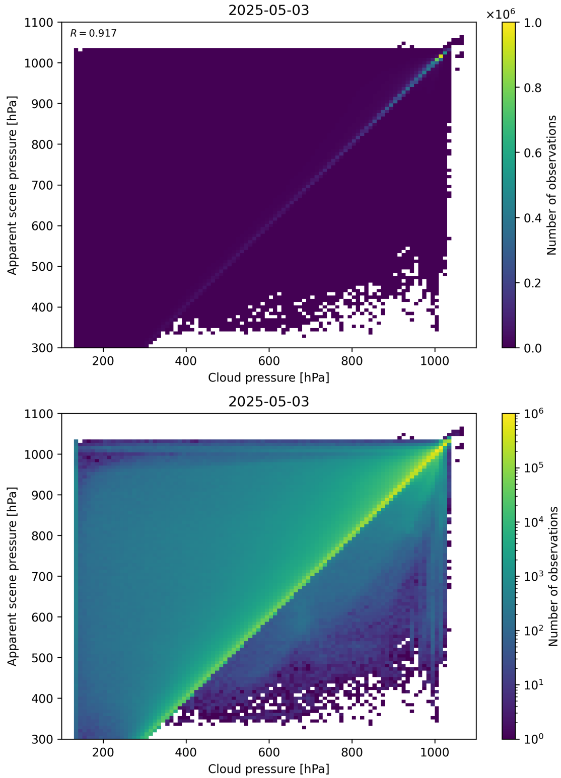
Figure 77: Scatter density plot of “Cloud pressure” against “Apparent scene pressure” for 2025-05-02 to 2025-05-04.
