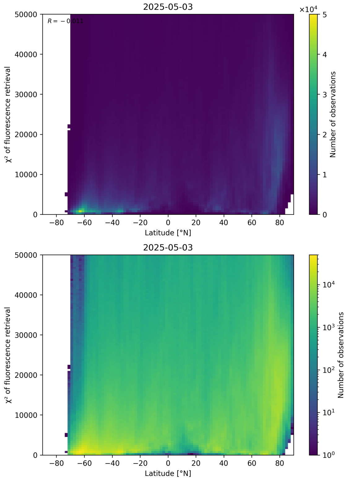
Figure 89: Scatter density plot of “Latitude” against “ \chi^2 of fluorescence retrieval” for 2025-05-02 to 2025-05-04.
