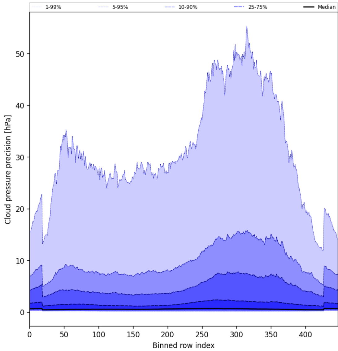
Figure 48: Along track statistics of “Cloud pressure precision” for 2025-05-02 to 2025-05-04
