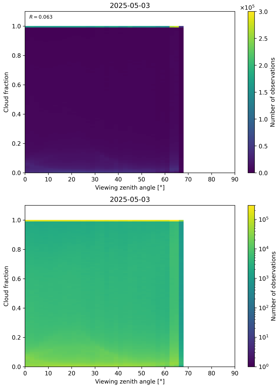
Figure 120: Scatter density plot of “Viewing zenith angle” against “Cloud fraction” for 2025-05-02 to 2025-05-04.
