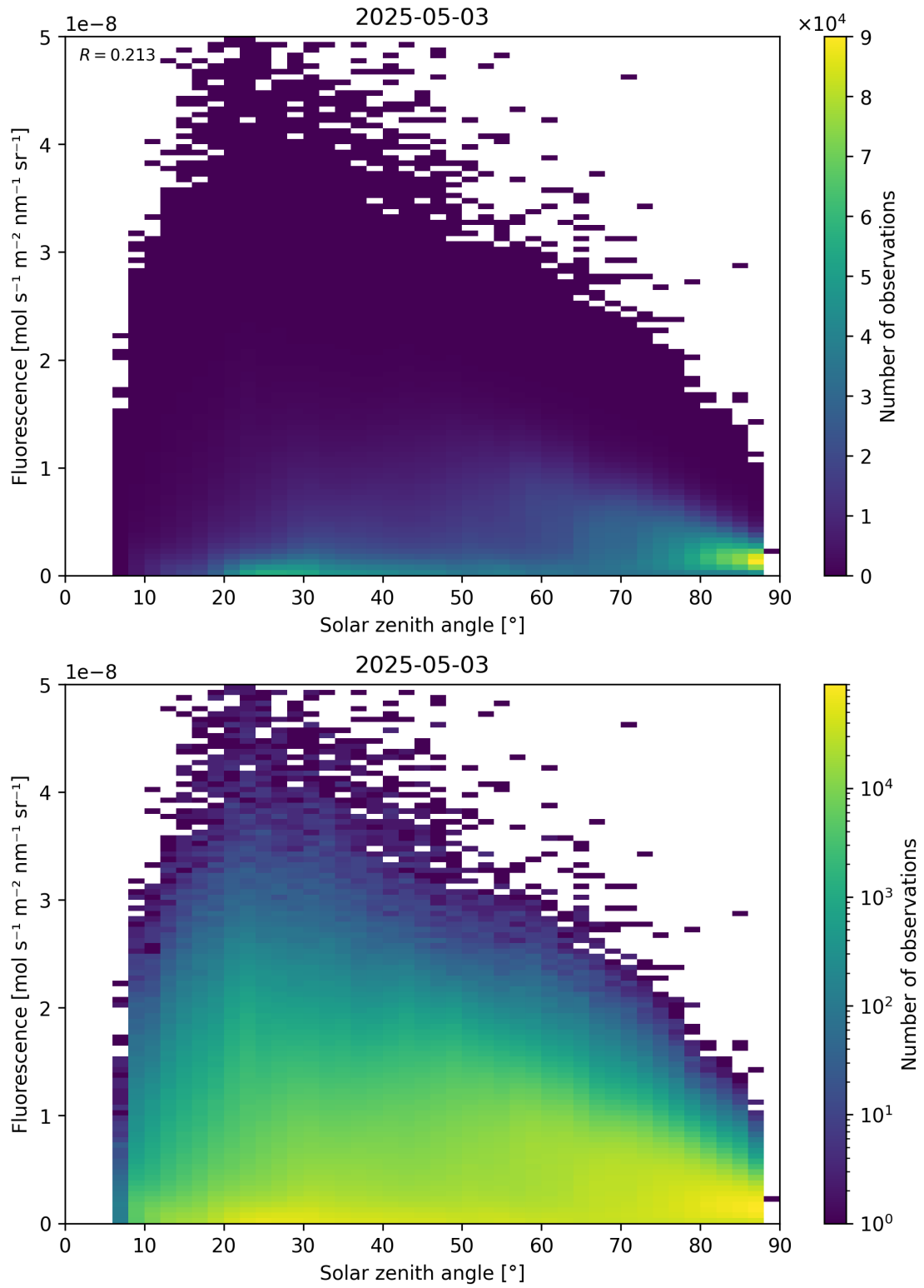
Figure 112: Scatter density plot of “Solar zenith angle” against “Fluorescence” for 2025-05-02 to 2025-05-04.
