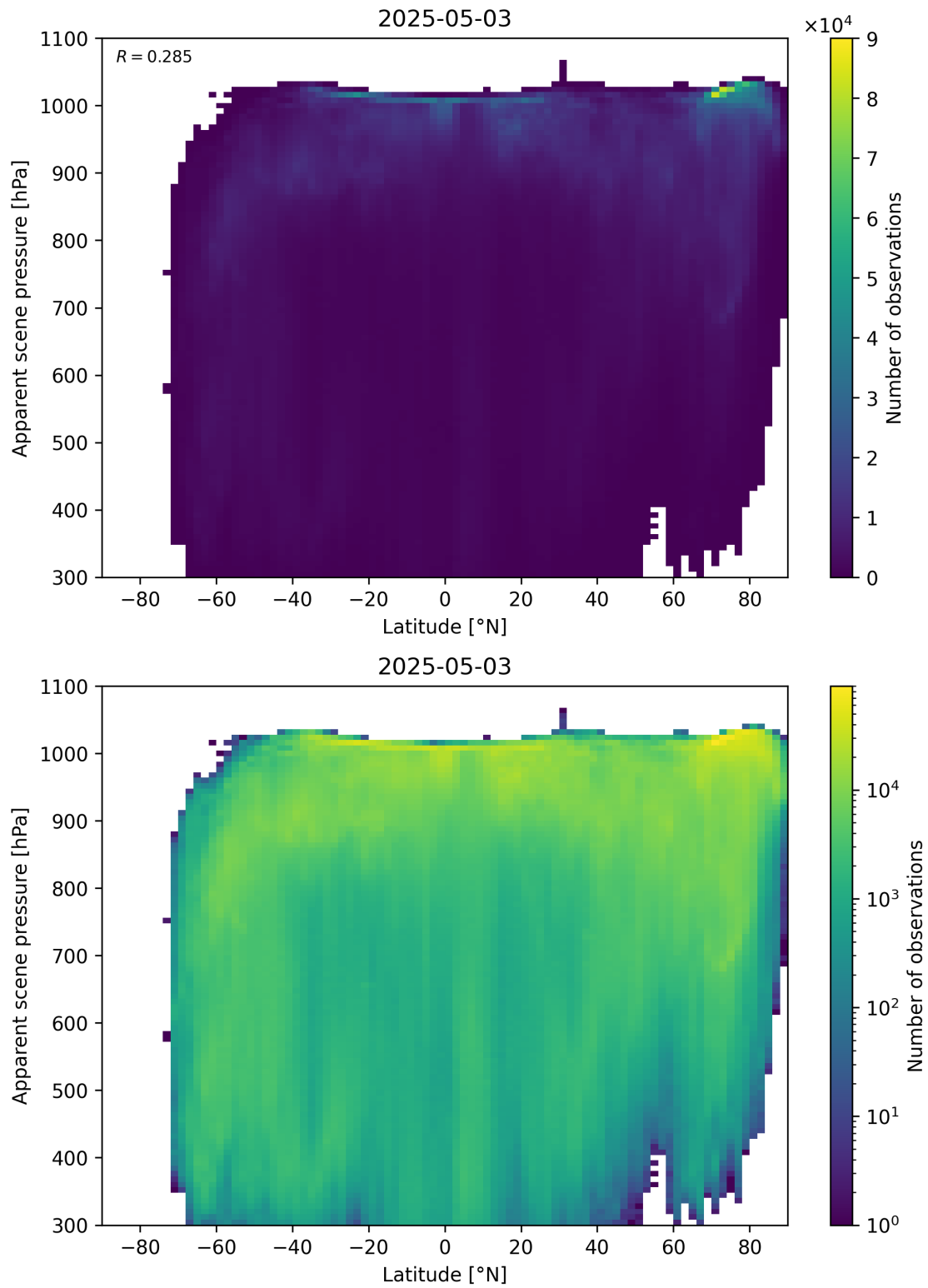
Figure 88: Scatter density plot of “Latitude” against “Apparent scene pressure” for 2025-05-02 to 2025-05-04.
