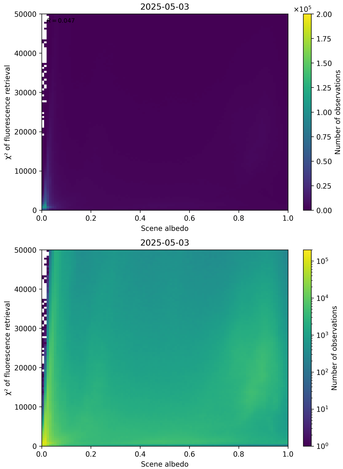
Figure 103: Scatter density plot of “Scene albedo” against “ \chi^2 of fluorescence retrieval” for 2025-05-02 to 2025-05-04.
