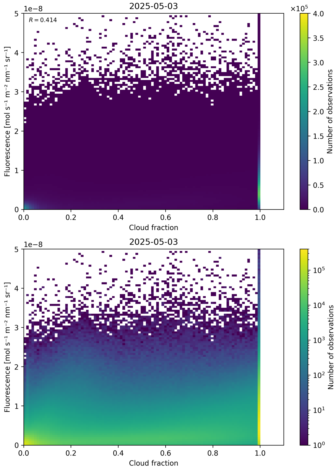
Figure 72: Scatter density plot of “Cloud fraction” against “Fluorescence” for 2025-05-02 to 2025-05-04.
