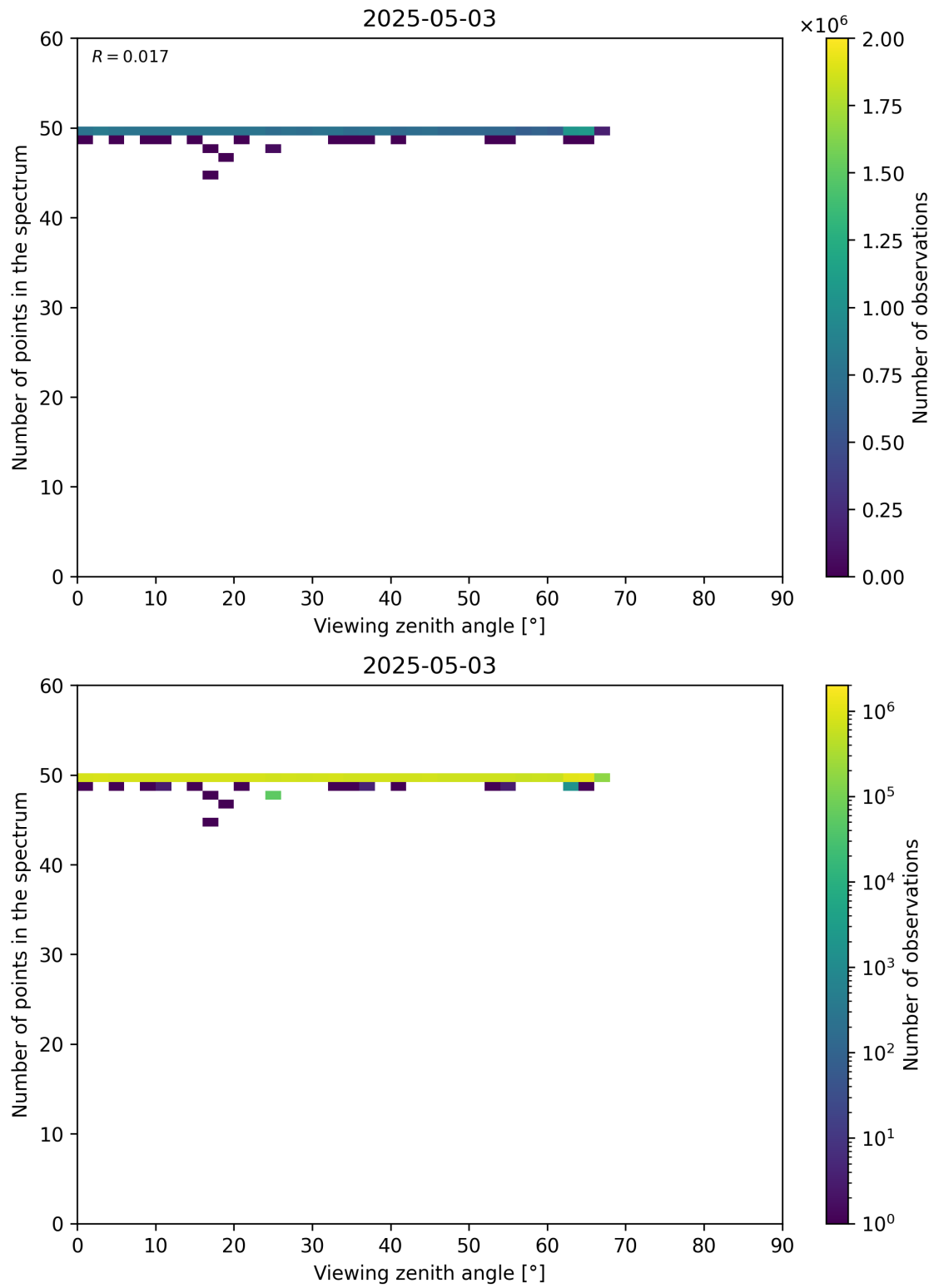
Figure 125: Scatter density plot of “Viewing zenith angle” against “Number of points in the spectrum” for 2025-05-02 to 2025-05-04.
