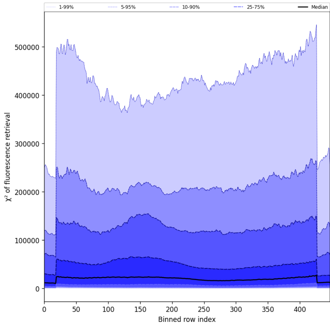
Figure 59: Along track statistics of “ \chi^2 of fluorescence retrieval” for 2025-05-02 to 2025-05-04
