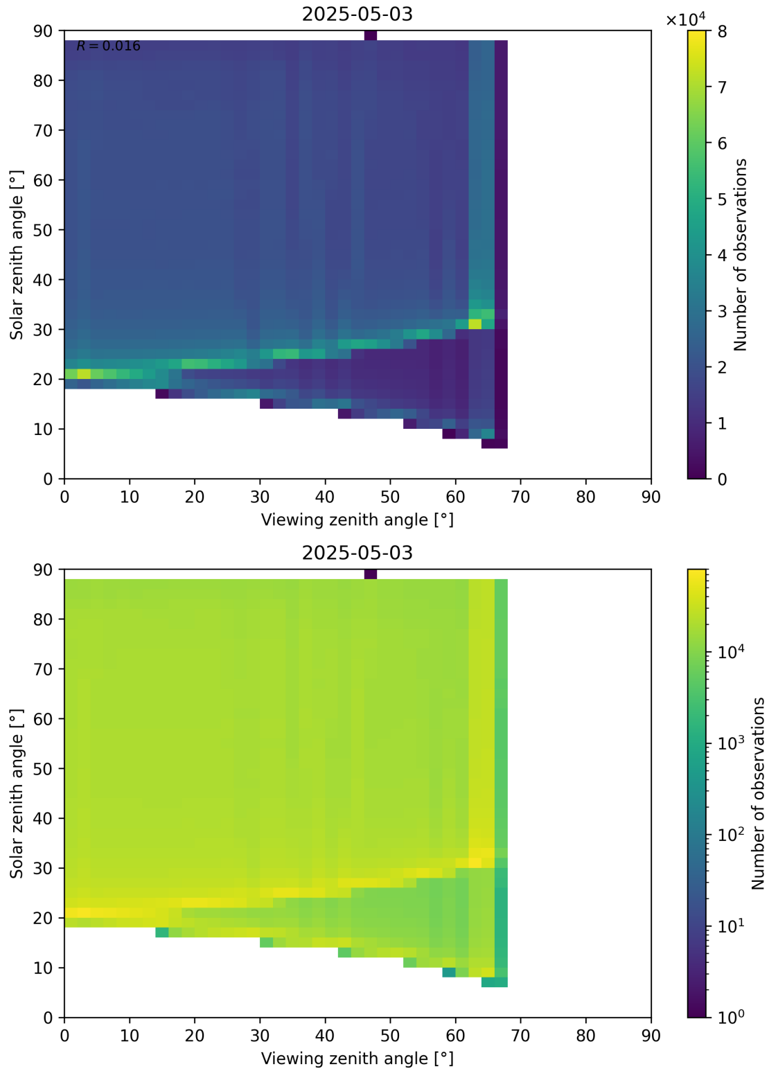
Figure 127: Scatter density plot of “Viewing zenith angle” against “Solar zenith angle” for 2025-05-02 to 2025-05-04.
