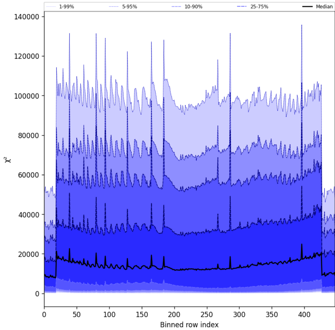
Figure 55: Along track statistics of “ \chi^2 ” for 2025-05-02 to 2025-05-04
