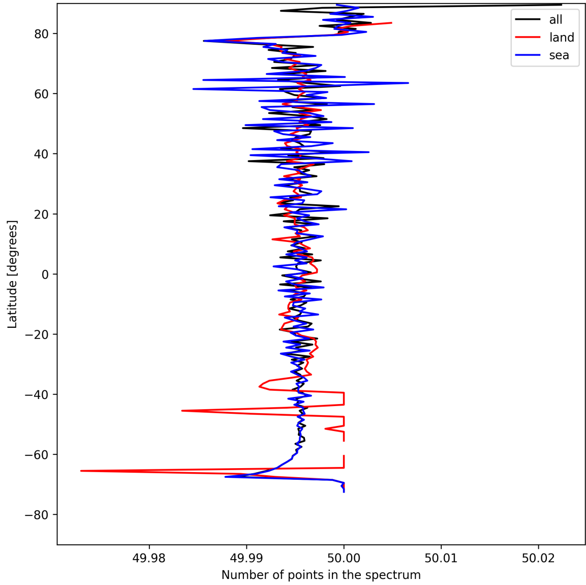
Figure 27: Zonal average of “Number of points in the spectrum” for 2025-05-02 to 2025-05-04.
