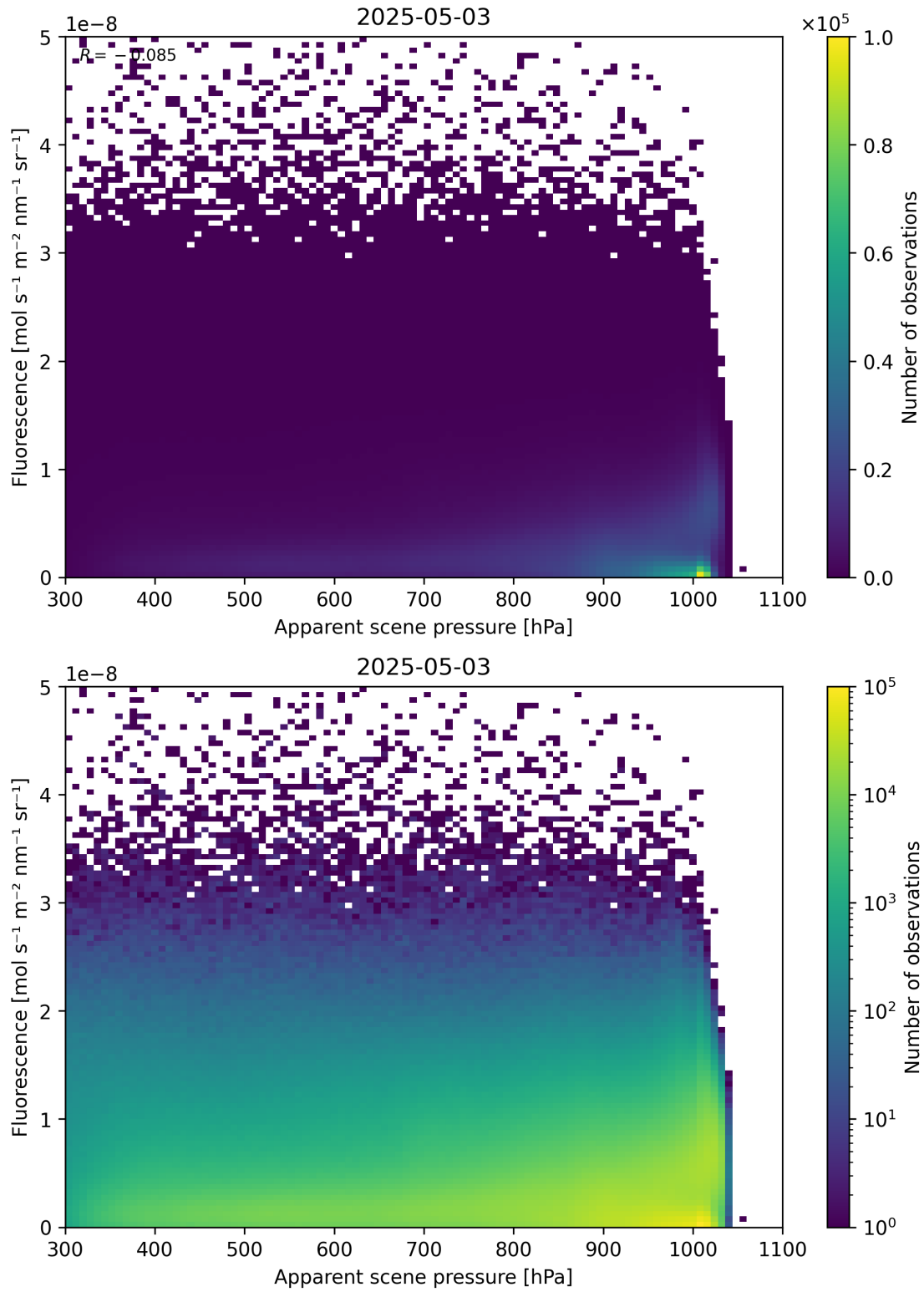
Figure 64: Scatter density plot of “Apparent scene pressure” against “Fluorescence” for 2025-05-02 to 2025-05-04.
