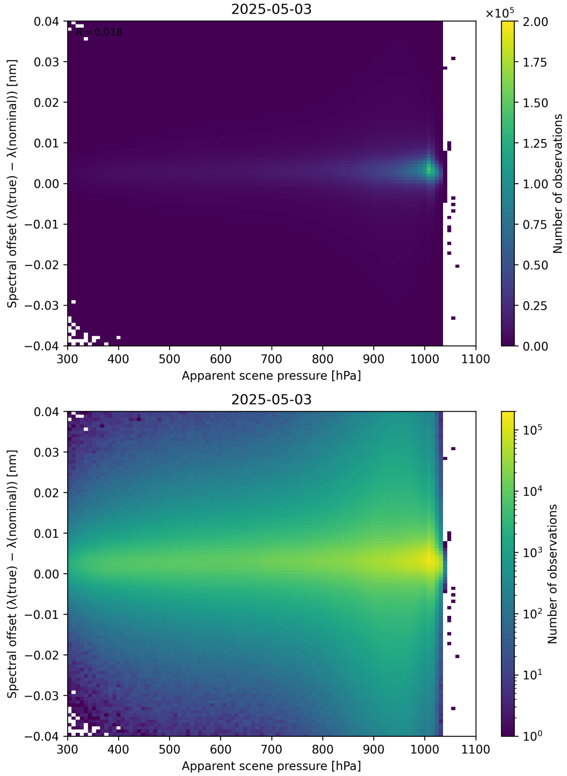
Figure 67: Scatter density plot of “Apparent scene pressure” against “Spectral offset ( \lambda_{\text{true}} - \lambda_{\text{nominal}} )” for 2025-05-02 to 2025-05-04.
