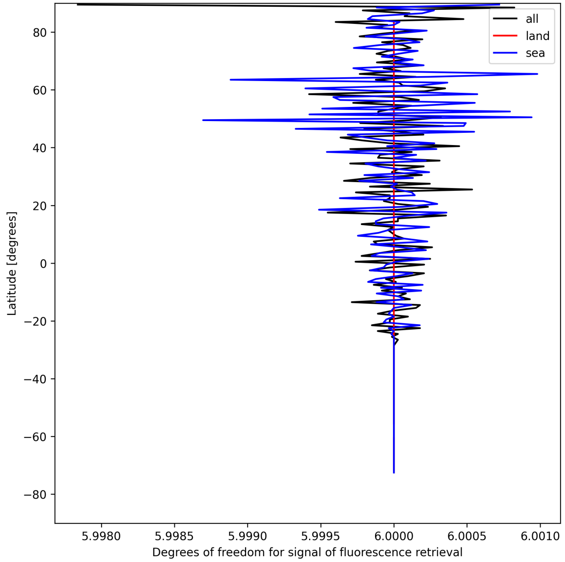
Figure 26: Zonal average of “Degrees of freedom for signal of fluorescence retrieval” for 2025-05-02 to 2025-05-04.
