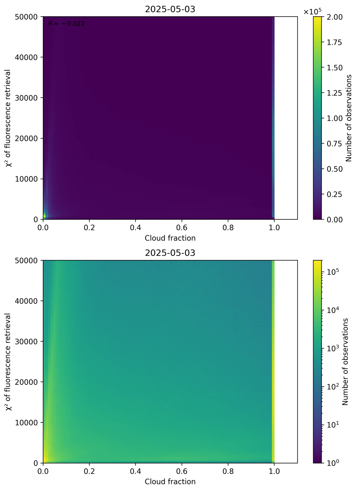
Figure 71: Scatter density plot of “Cloud fraction” against “ \chi^2 of fluorescence retrieval” for 2025-05-02 to 2025-05-04.
