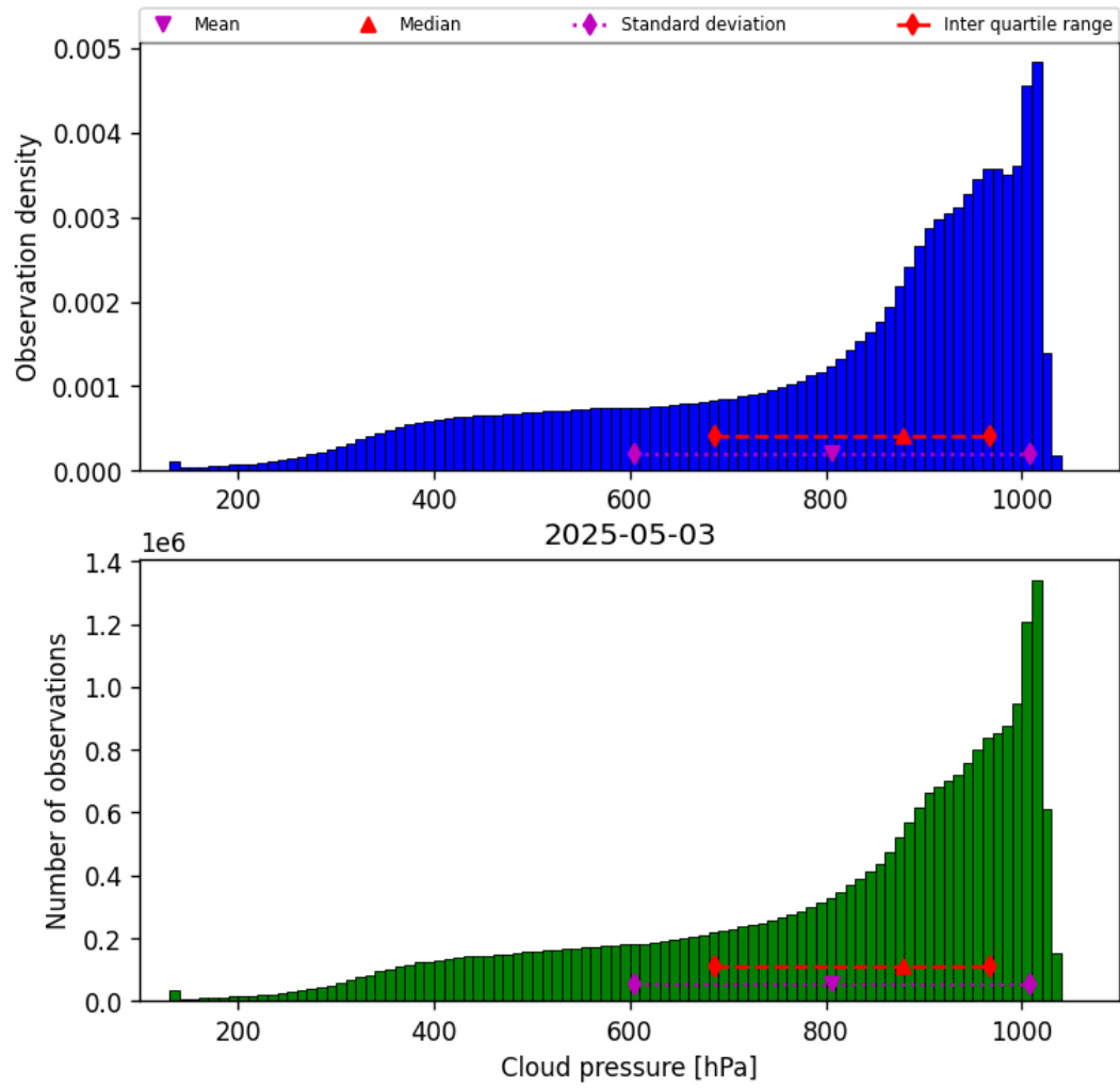
Figure 30: Histogram of “Cloud pressure” for 2025-05-02 to 2025-05-04
