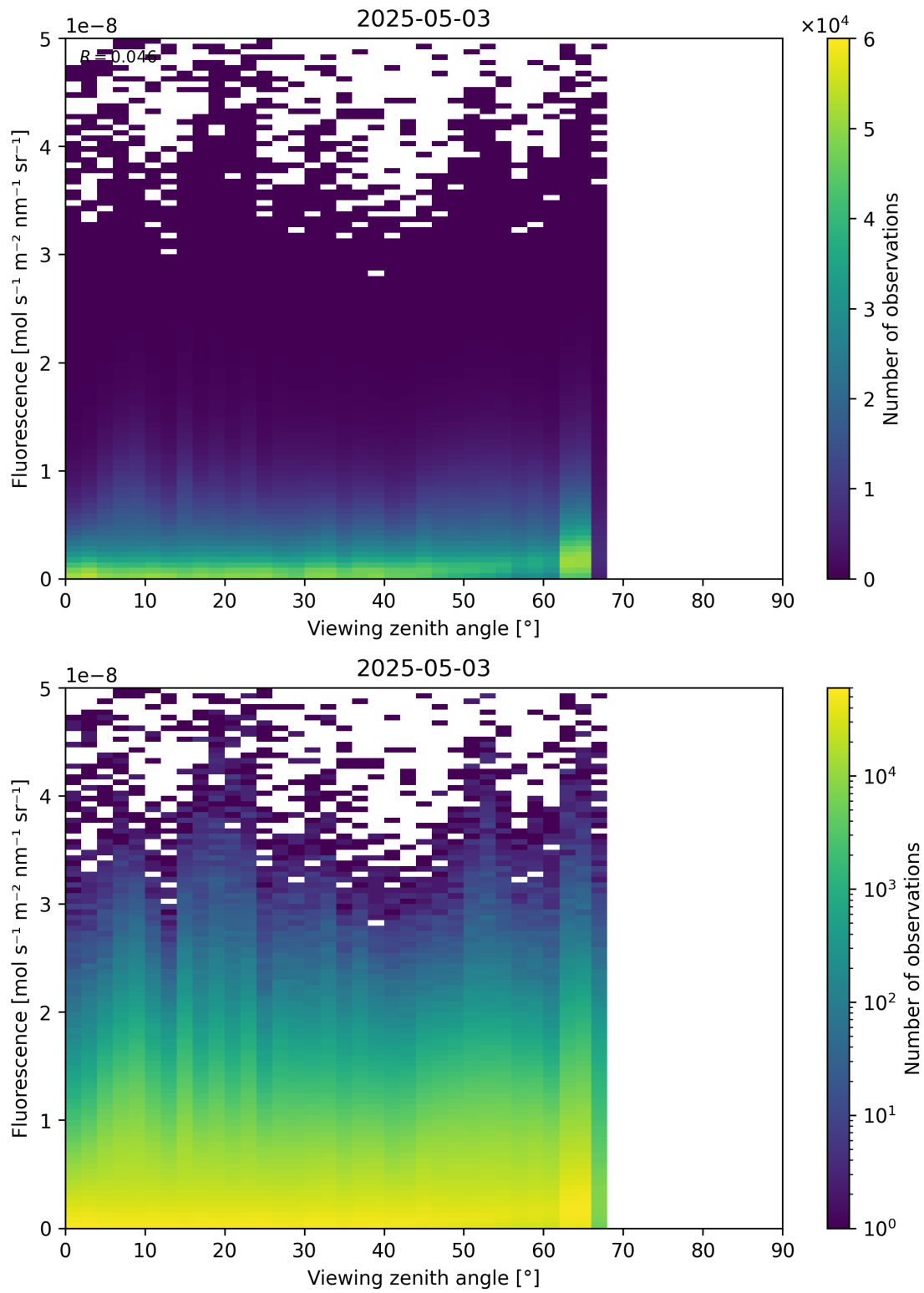
Figure 122: Scatter density plot of “Viewing zenith angle” against “Fluorescence” for 2025-05-02 to 2025-05-04.
