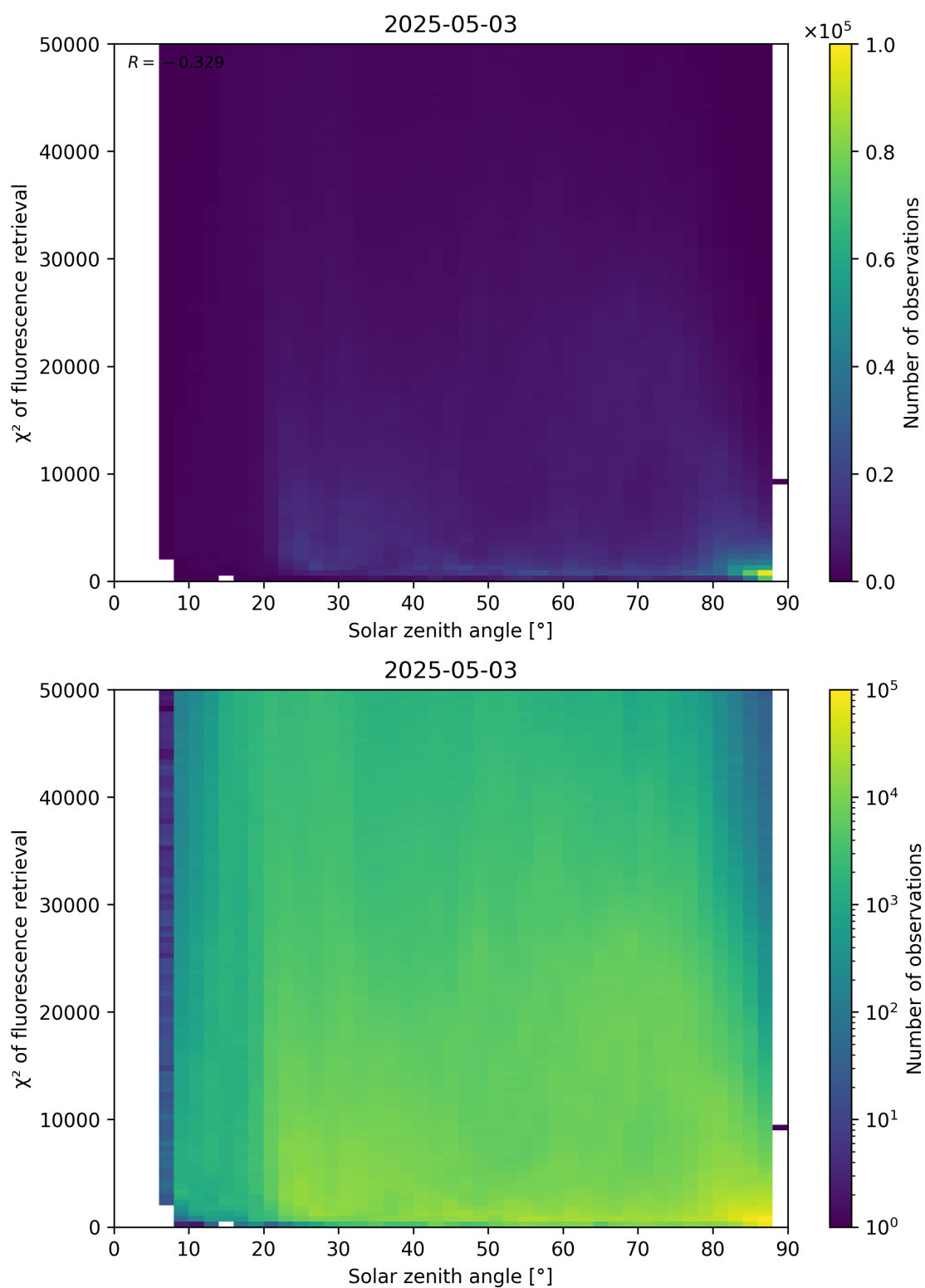
Figure 109: Scatter density plot of “Solar zenith angle” against “ \chi^2 of fluorescence retrieval” for 2025-05-02 to 2025-05-04.
