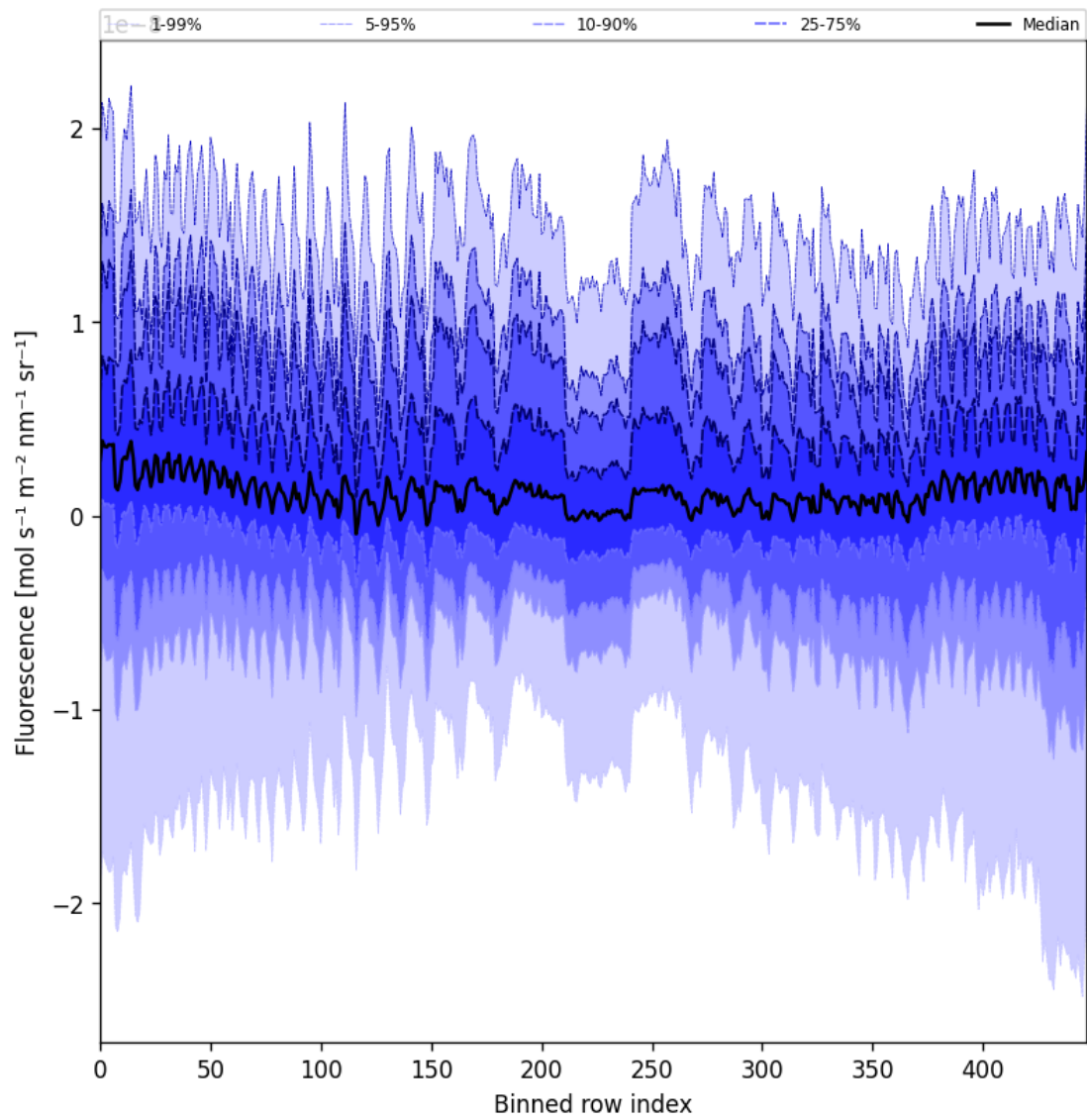
Figure 57: Along track statistics of “Fluorescence” for 2025-05-02 to 2025-05-04
