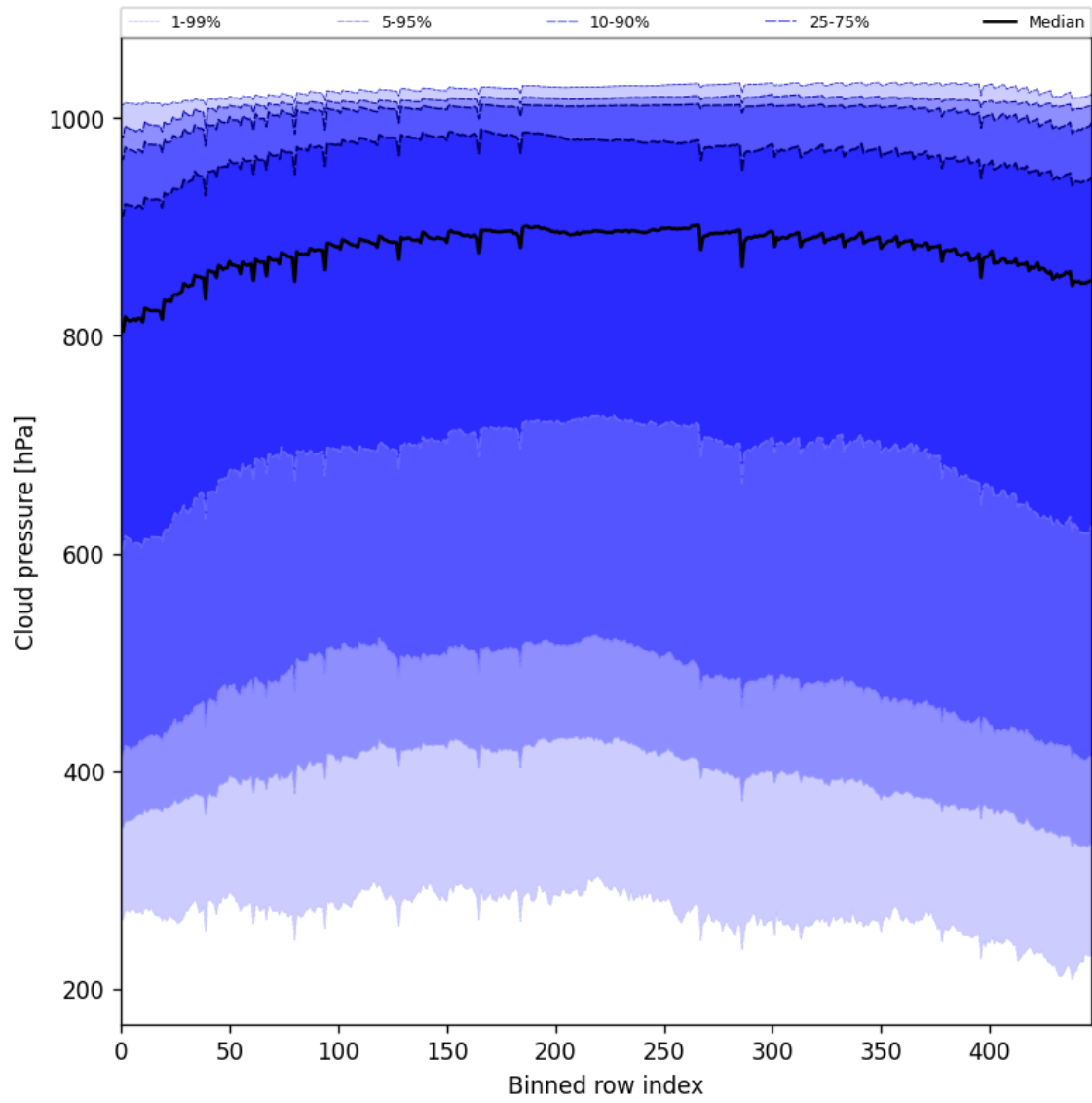
Figure 47: Along track statistics of “Cloud pressure” for 2025-05-02 to 2025-05-04
