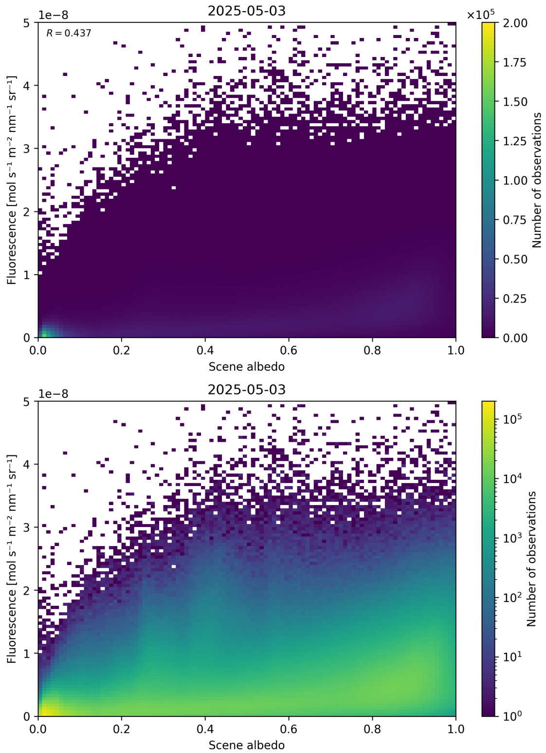
Figure 104: Scatter density plot of “Scene albedo” against “Fluorescence” for 2025-05-02 to 2025-05-04.
