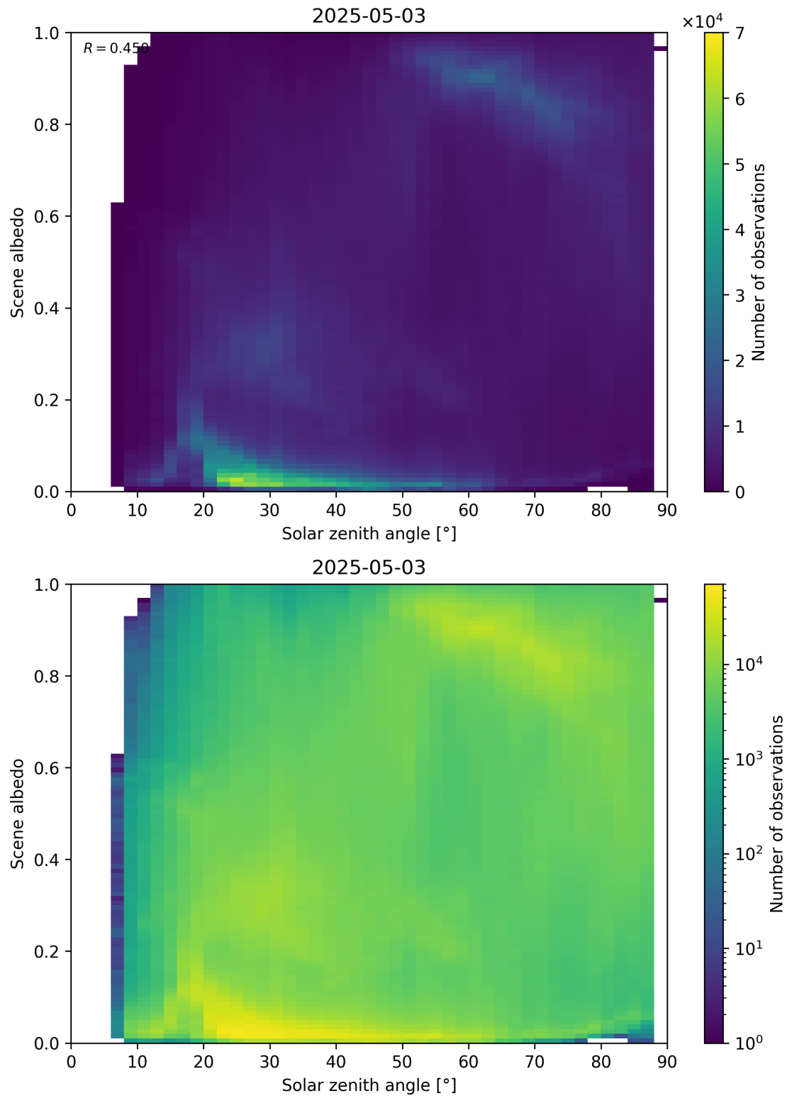
Figure 116: Scatter density plot of “Solar zenith angle” against “Scene albedo” for 2025-05-02 to 2025-05-04.
