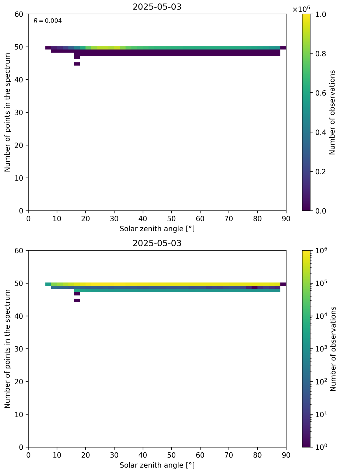
Figure 115: Scatter density plot of “Solar zenith angle” against “Number of points in the spectrum” for 2025-05-02 to 2025-05-04.
