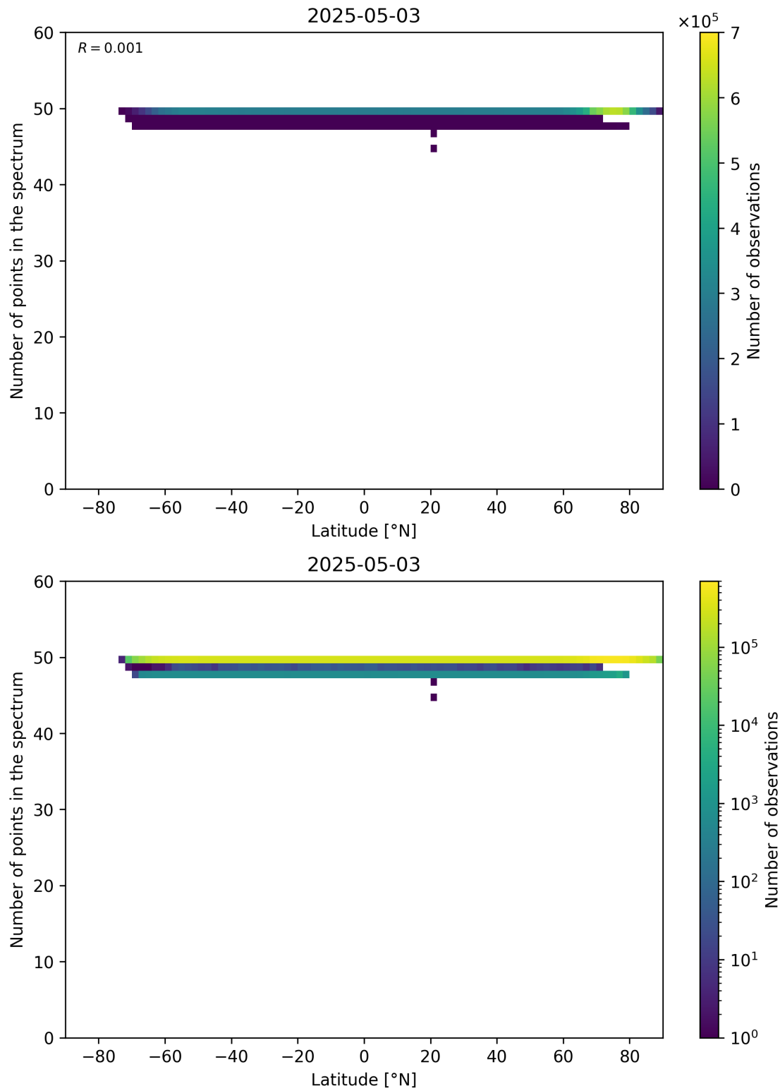
Figure 94: Scatter density plot of “Latitude” against “Number of points in the spectrum” for 2025-05-02 to 2025-05-04.
