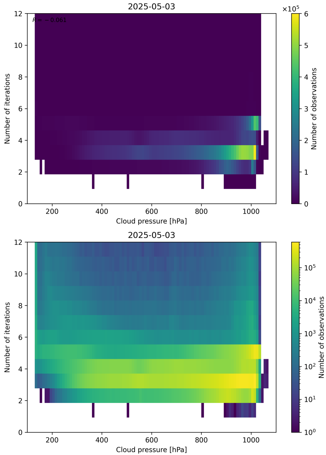
Figure 81: Scatter density plot of “Cloud pressure” against “Number of iterations” for 2025-05-02 to 2025-05-04.
