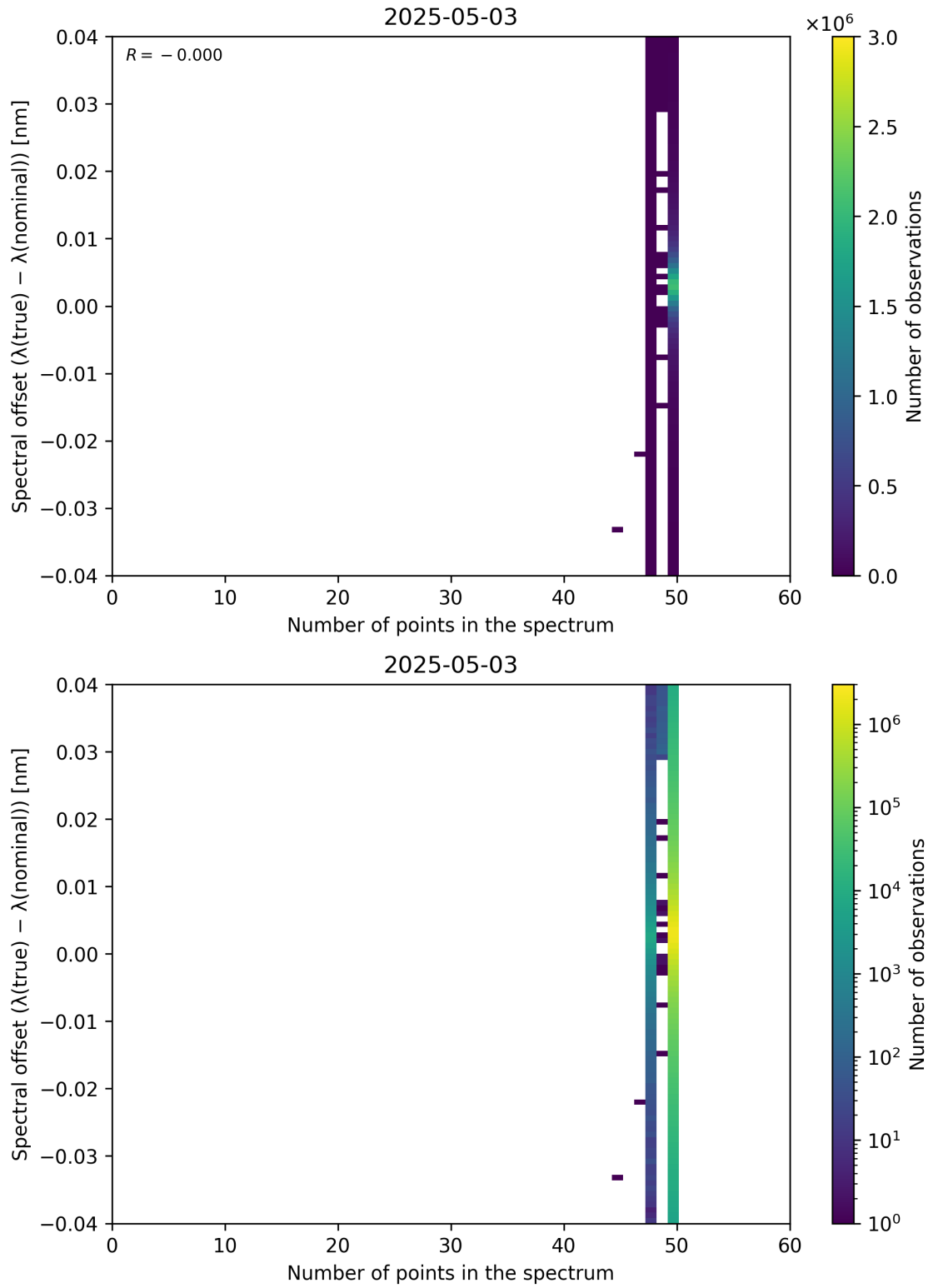
Figure 101: Scatter density plot of “Number of points in the spectrum” against “Spectral offset ( \lambda_{\text{true}} - \lambda_{\text{nominal}} )” for 2025-05-02 to 2025-05-04.
