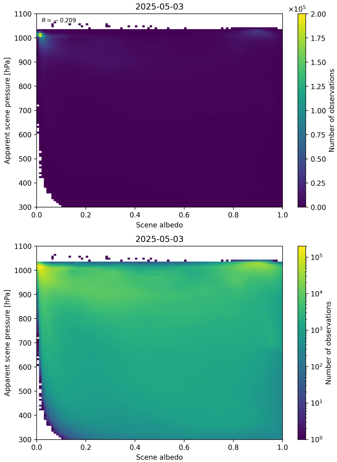
Figure 102: Scatter density plot of “Scene albedo” against “Apparent scene pressure” for 2025-05-02 to 2025-05-04.
