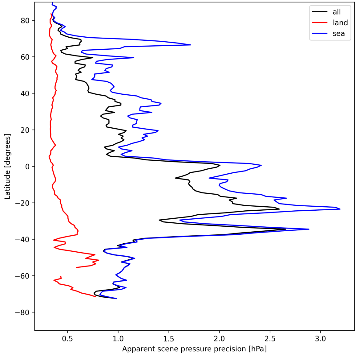
Figure 20: Zonal average of “Apparent scene pressure precision” for 2025-05-02 to 2025-05-04.
