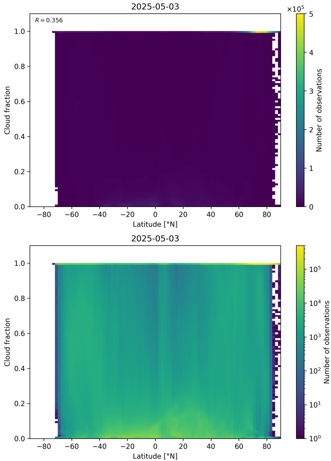
Figure 90: Scatter density plot of “Latitude” against “Cloud fraction” for 2025-05-02 to 2025-05-04.
