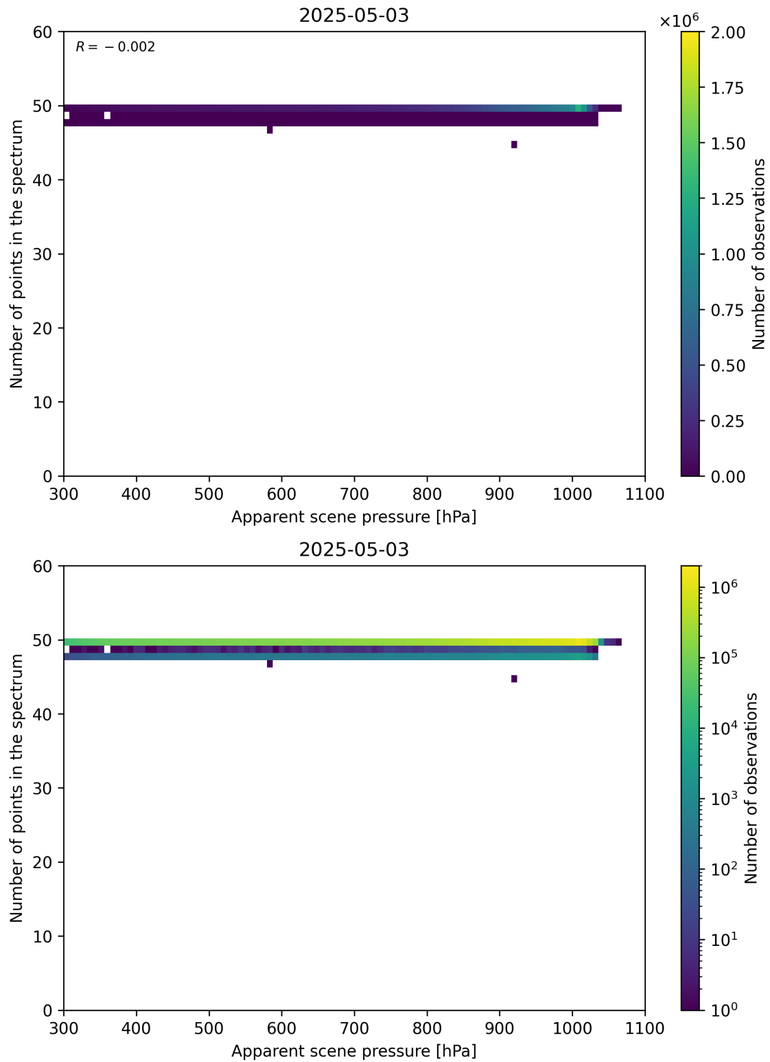
Figure 66: Scatter density plot of “Apparent scene pressure” against “Number of points in the spectrum” for 2025-05-02 to 2025-05-04.
