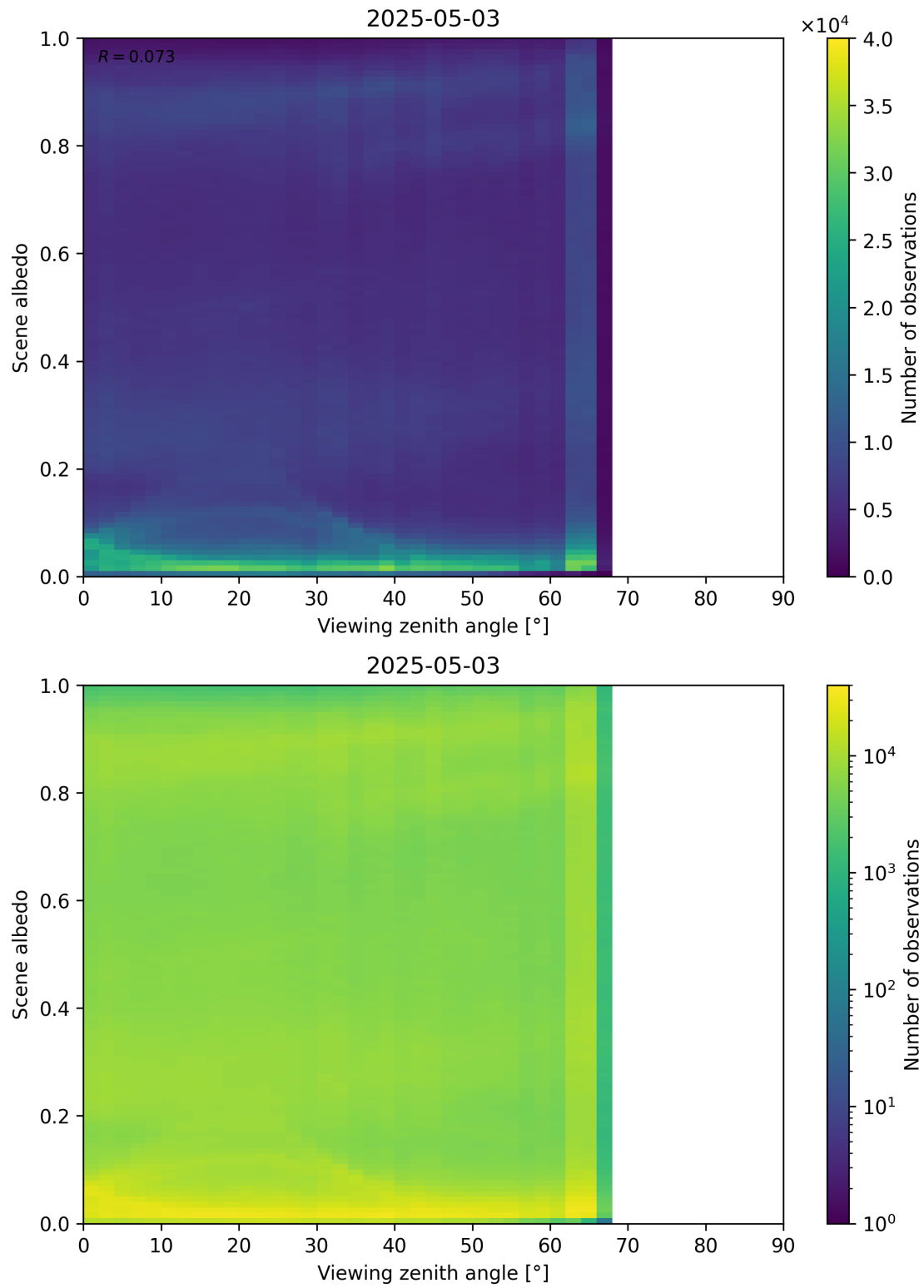
Figure 126: Scatter density plot of “Viewing zenith angle” against “Scene albedo” for 2025-05-02 to 2025-05-04.
