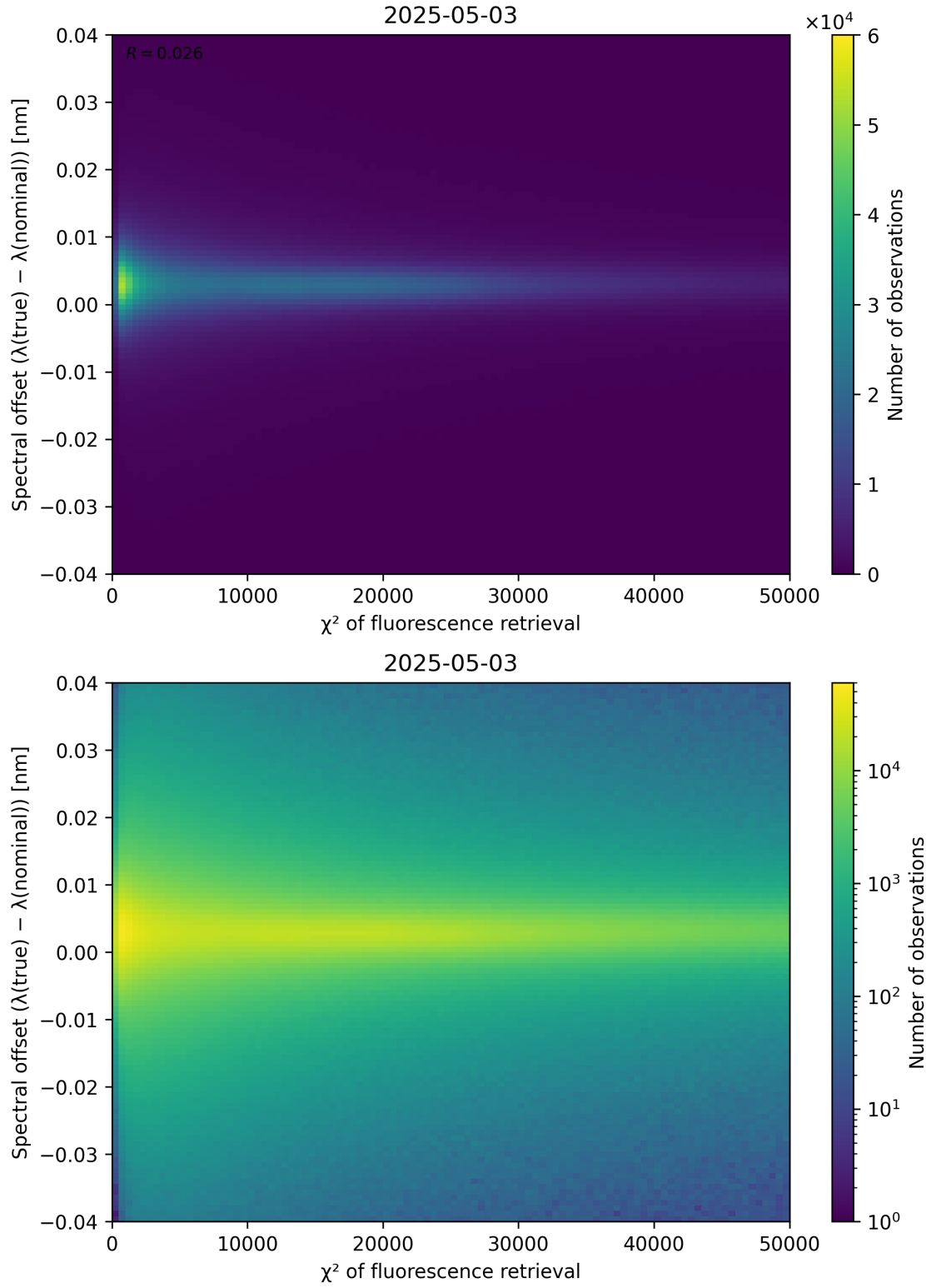
Figure 69: Scatter density plot of “ \chi^2 of fluorescence retrieval” against “Spectral offset ( \lambda_{\text{true}} - \lambda_{\text{nominal}} )” for 2025-05-02 to 2025-05-04.
