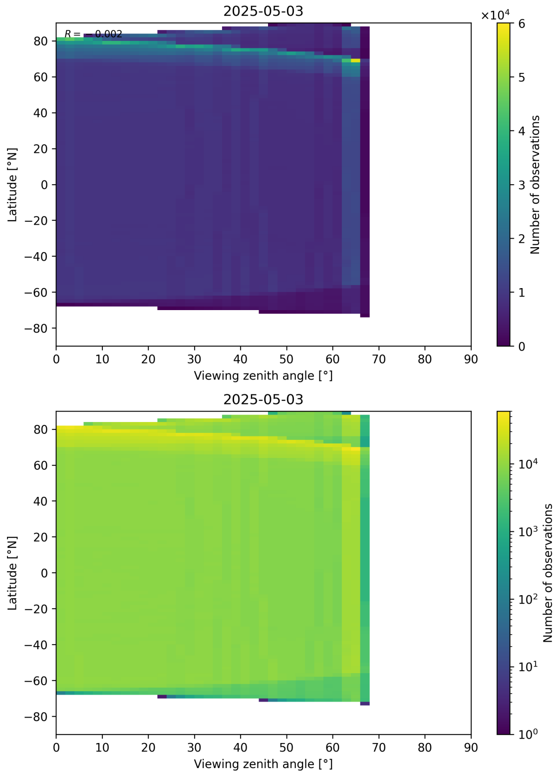
Figure 123: Scatter density plot of “Viewing zenith angle” against “Latitude” for 2025-05-02 to 2025-05-04.
