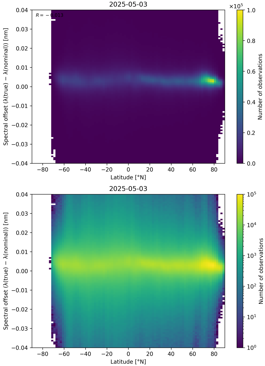
Figure 96: Scatter density plot of “Latitude” against “Spectral offset ( \lambda_{\text{true}} - \lambda_{\text{nominal}} )” for 2025-05-02 to 2025-05-04.
