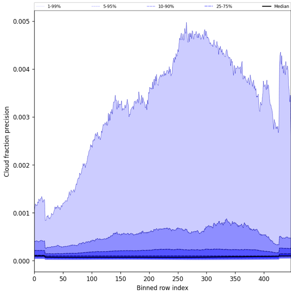
Figure 50: Along track statistics of “Cloud fraction precision” for 2025-05-02 to 2025-05-04
