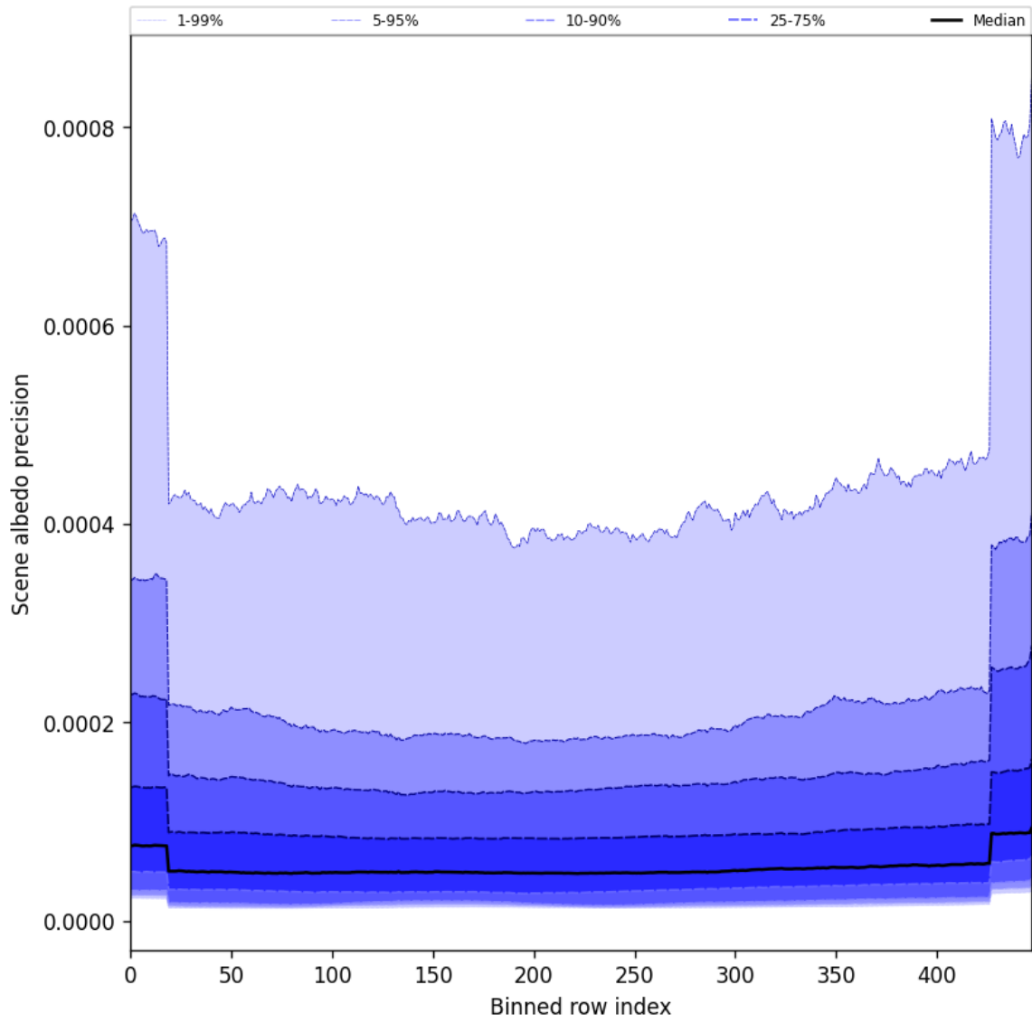
Figure 52: Along track statistics of “Scene albedo precision” for 2025-05-02 to 2025-05-04
