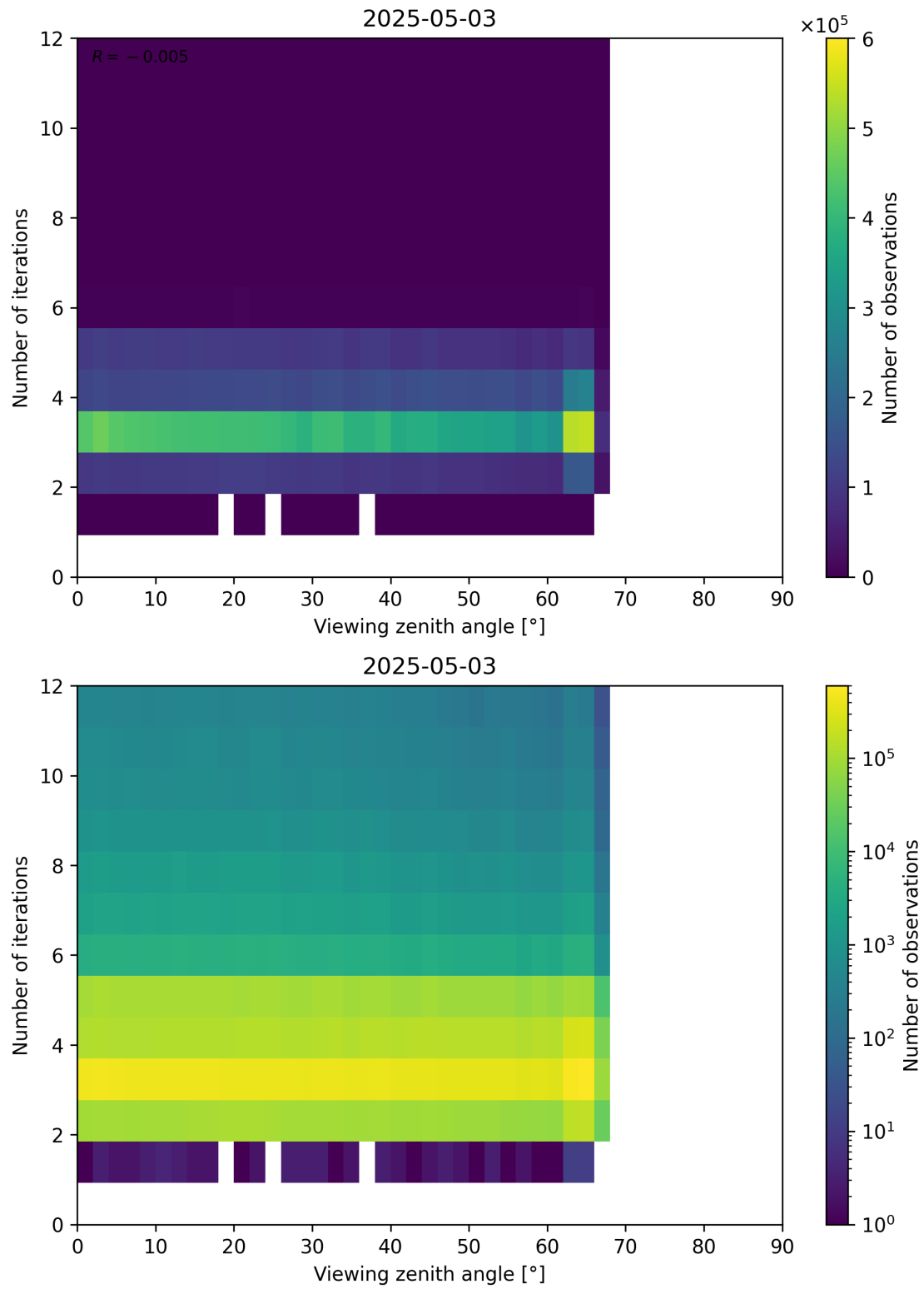
Figure 124: Scatter density plot of “Viewing zenith angle” against “Number of iterations” for 2025-05-02 to 2025-05-04.
