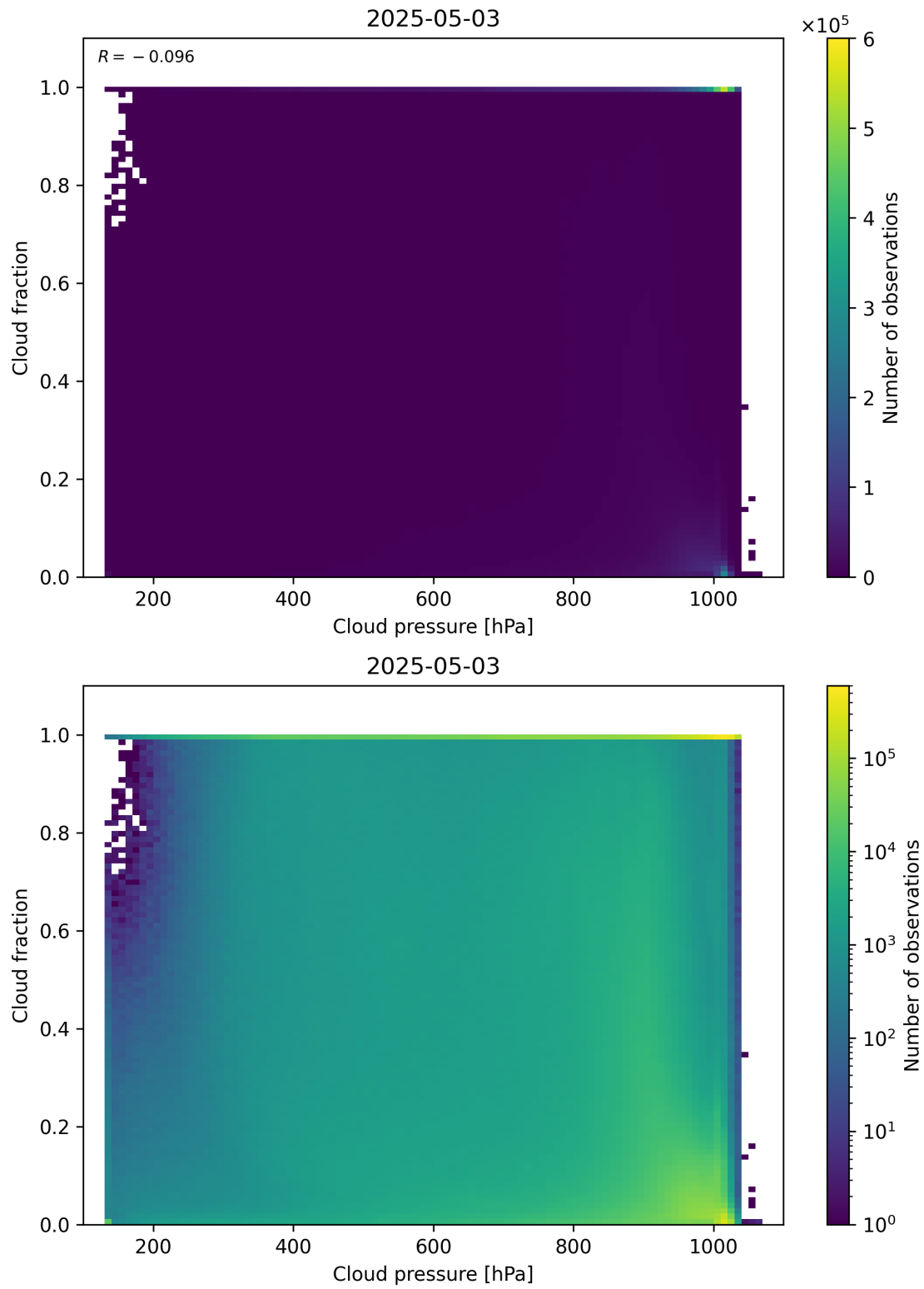
Figure 79: Scatter density plot of “Cloud pressure” against “Cloud fraction” for 2025-05-02 to 2025-05-04.
