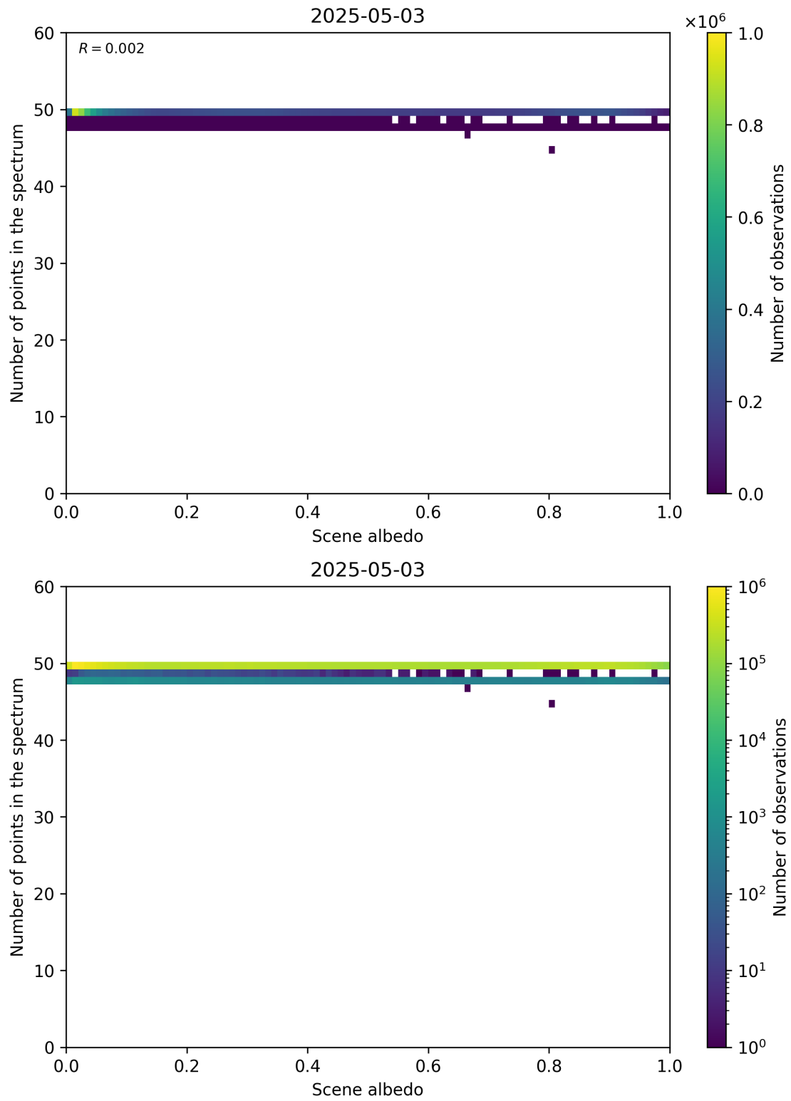
Figure 106: Scatter density plot of “Scene albedo” against “Number of points in the spectrum” for 2025-05-02 to 2025-05-04.
