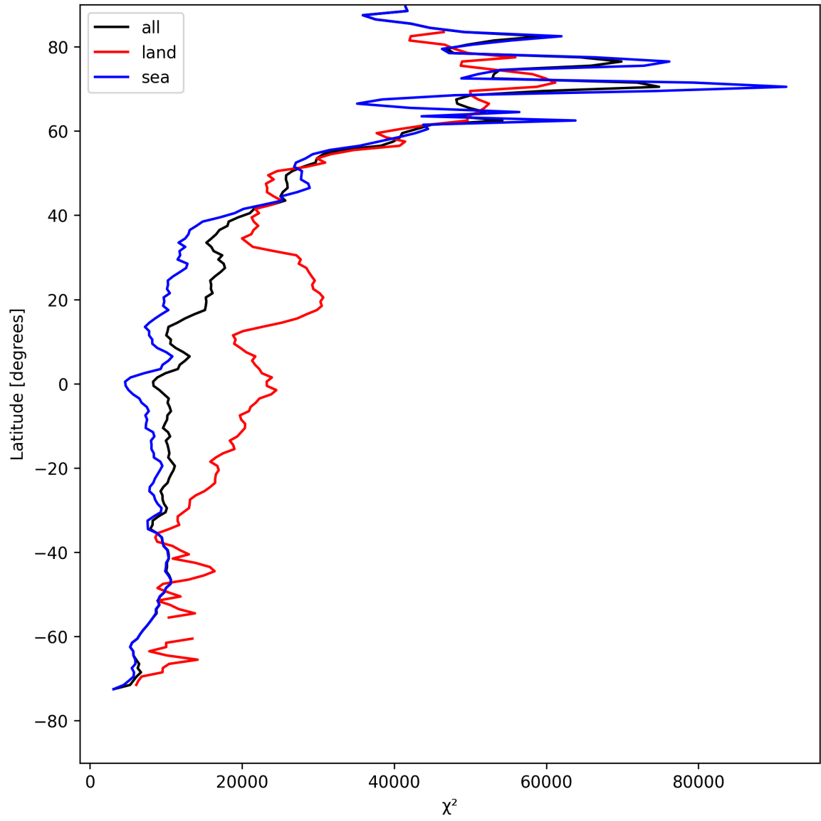
Figure 21: Zonal average of “ \chi^2 ” for 2025-05-02 to 2025-05-04.
