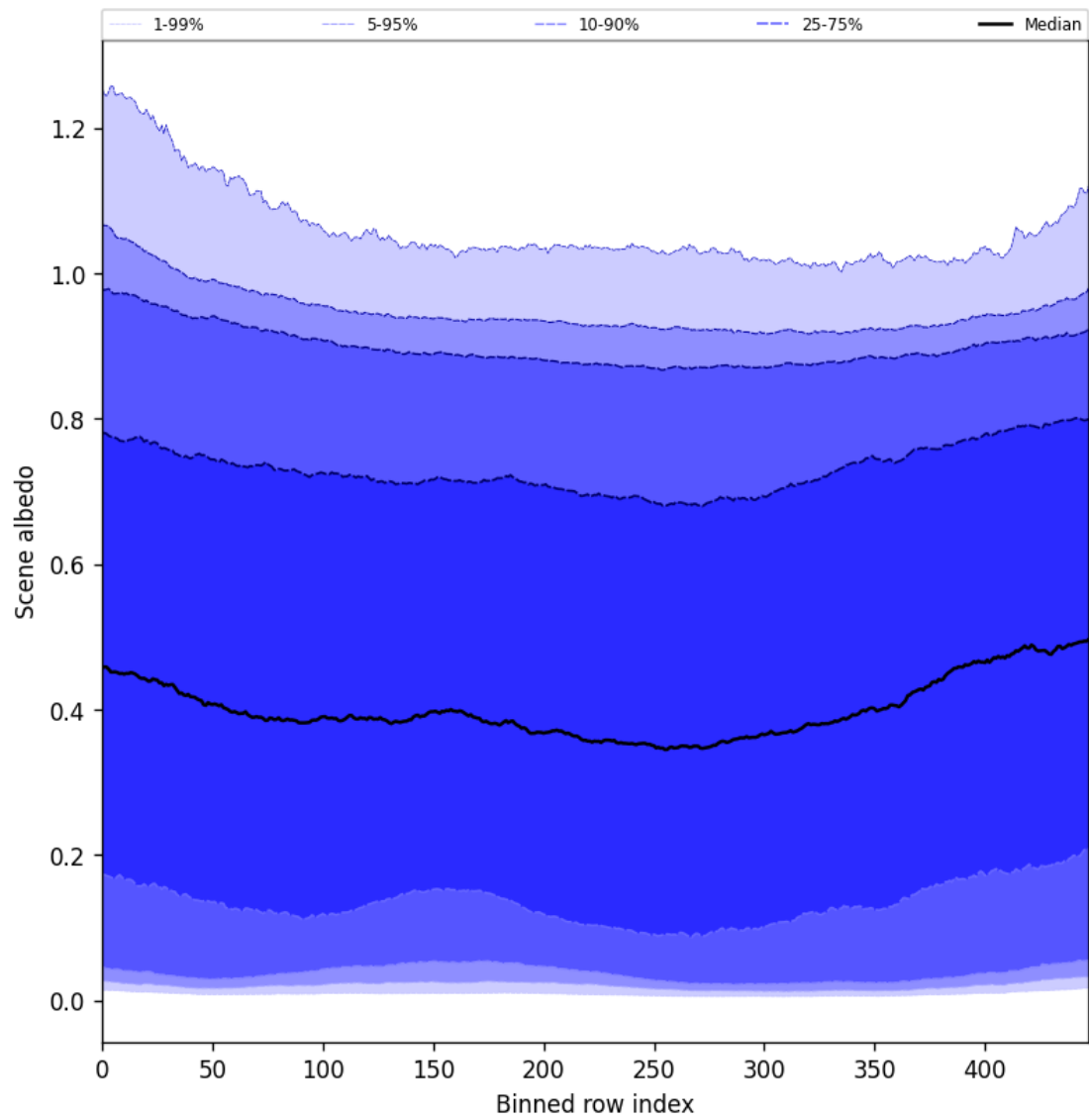
Figure 51: Along track statistics of “Scene albedo” for 2025-05-02 to 2025-05-04
