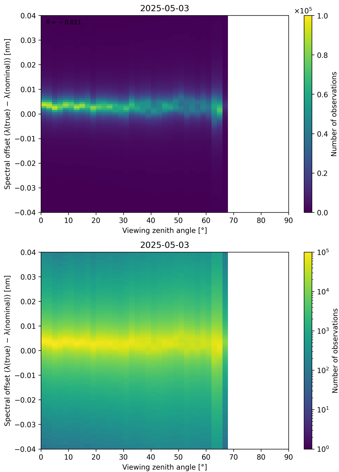
Figure 128: Scatter density plot of “Viewing zenith angle” against “Spectral offset ( \lambda_{\text{true}} - \lambda_{\text{nominal}} )” for 2025-05-02 to 2025-05-04.
