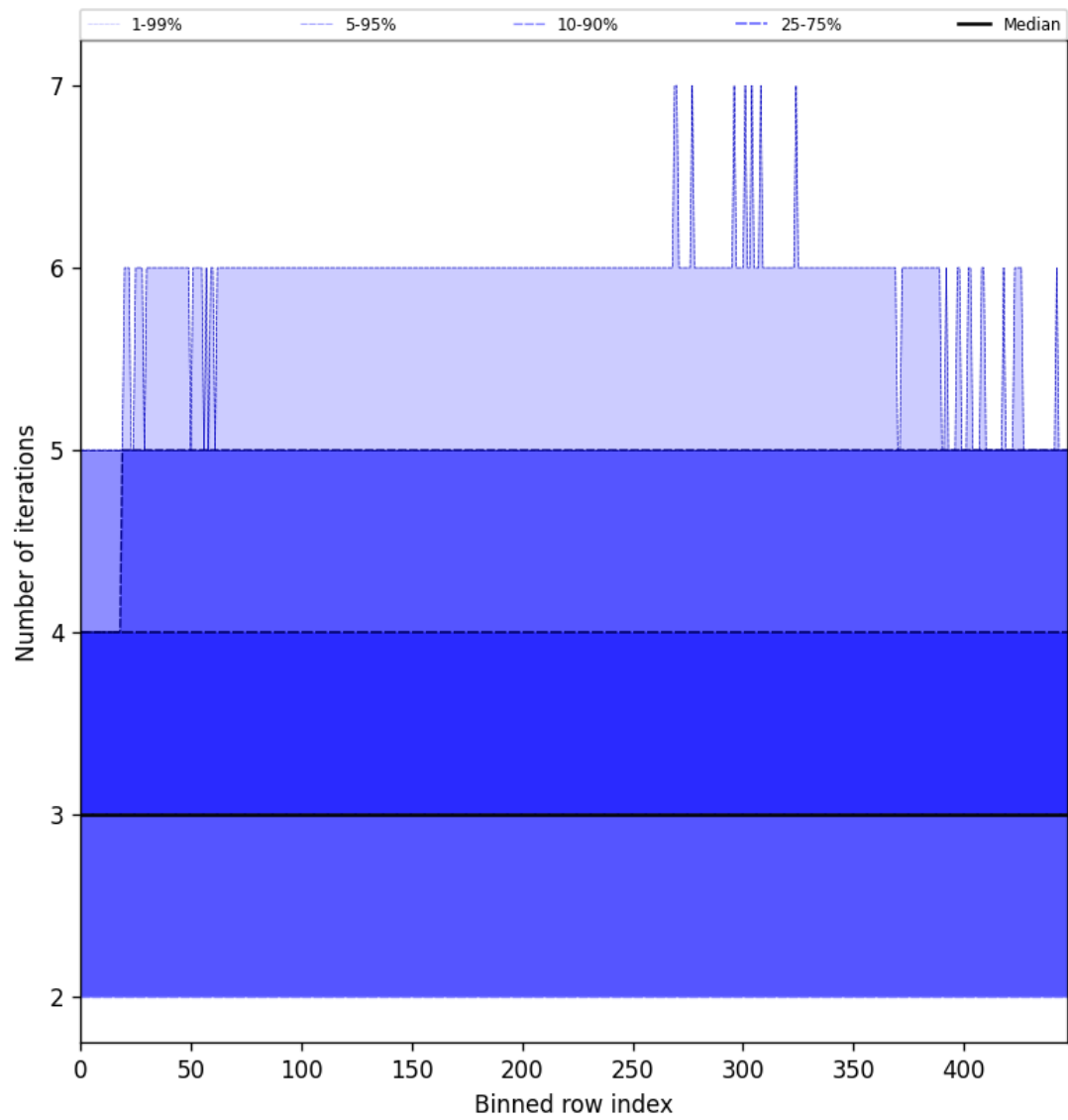
Figure 56: Along track statistics of “Number of iterations” for 2025-05-02 to 2025-05-04
