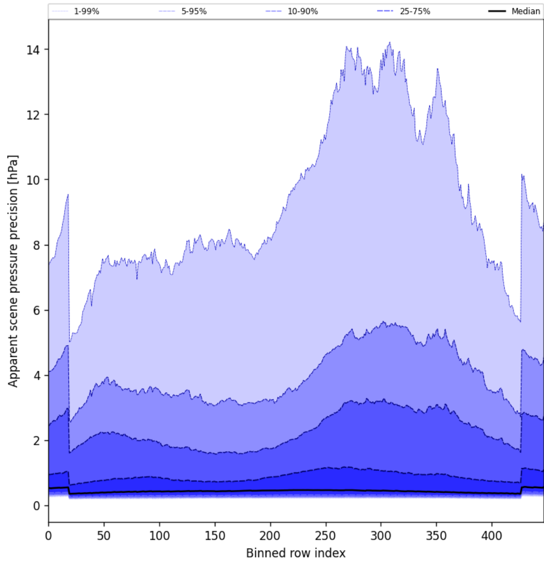
Figure 54: Along track statistics of “Apparent scene pressure precision” for 2025-05-02 to 2025-05-04
