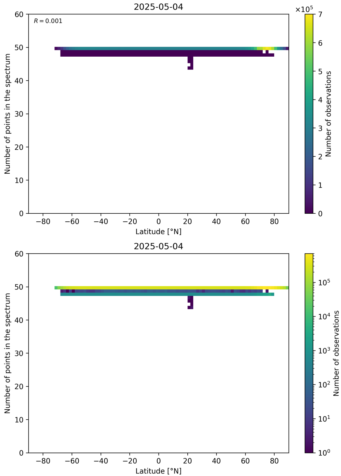
Figure 94: Scatter density plot of “Latitude” against “Number of points in the spectrum” for 2025-05-03 to 2025-05-05.
