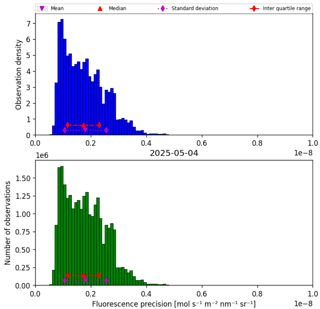
Figure 41: Histogram of “Fluorescence precision” for 2025-05-03 to 2025-05-05
