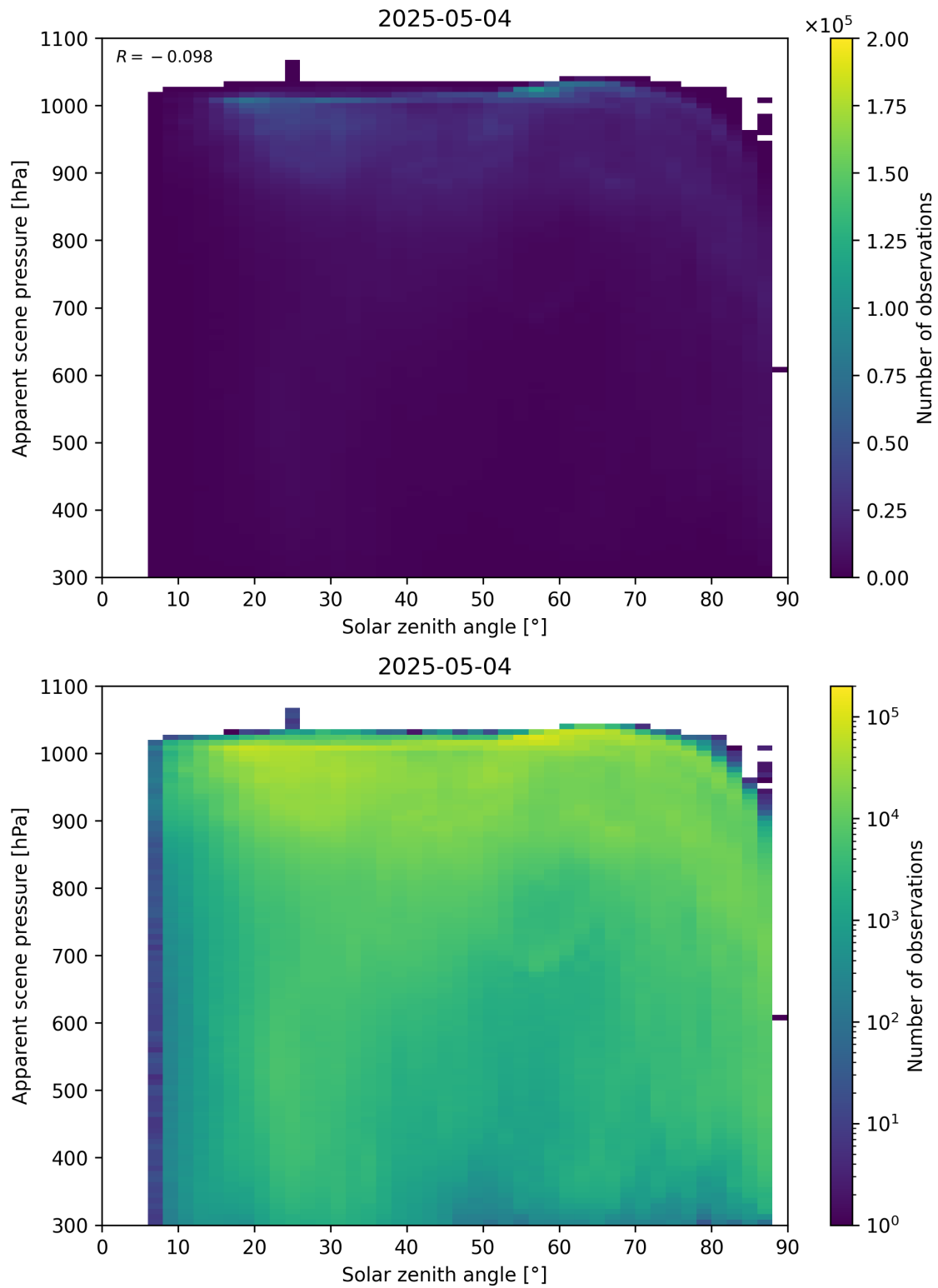
Figure 108: Scatter density plot of “Solar zenith angle” against “Apparent scene pressure” for 2025-05-03 to 2025-05-05.
