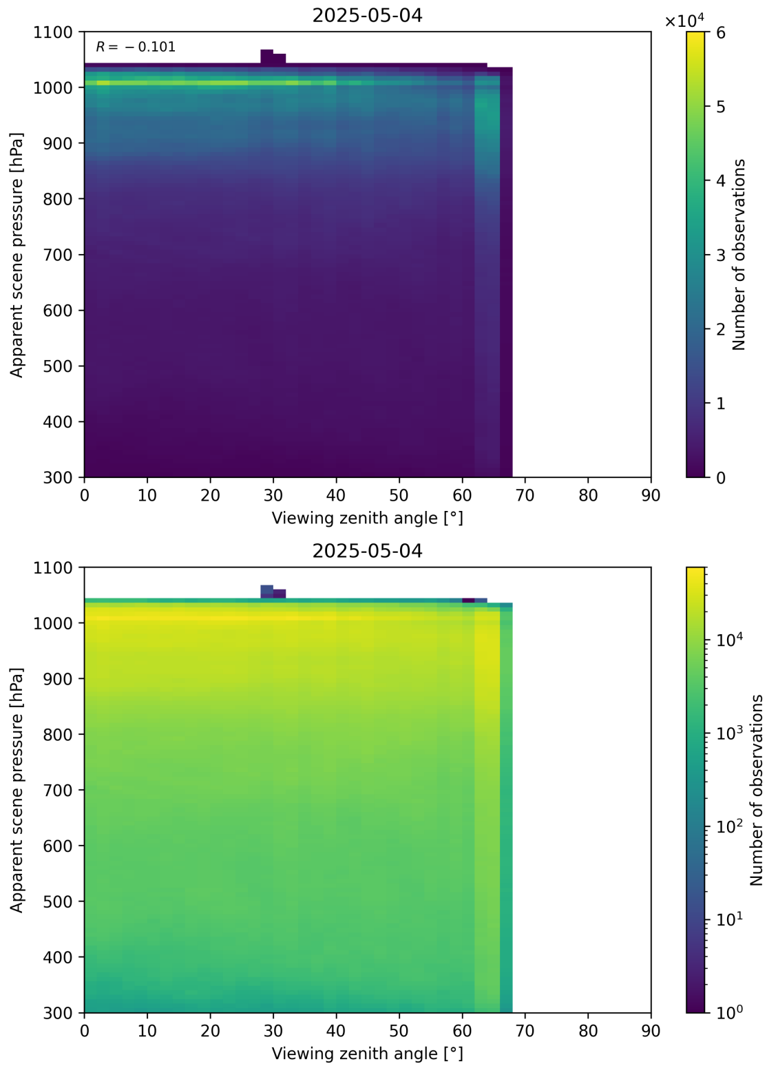
Figure 118: Scatter density plot of “Viewing zenith angle” against “Apparent scene pressure” for 2025-05-03 to 2025-05-05.
