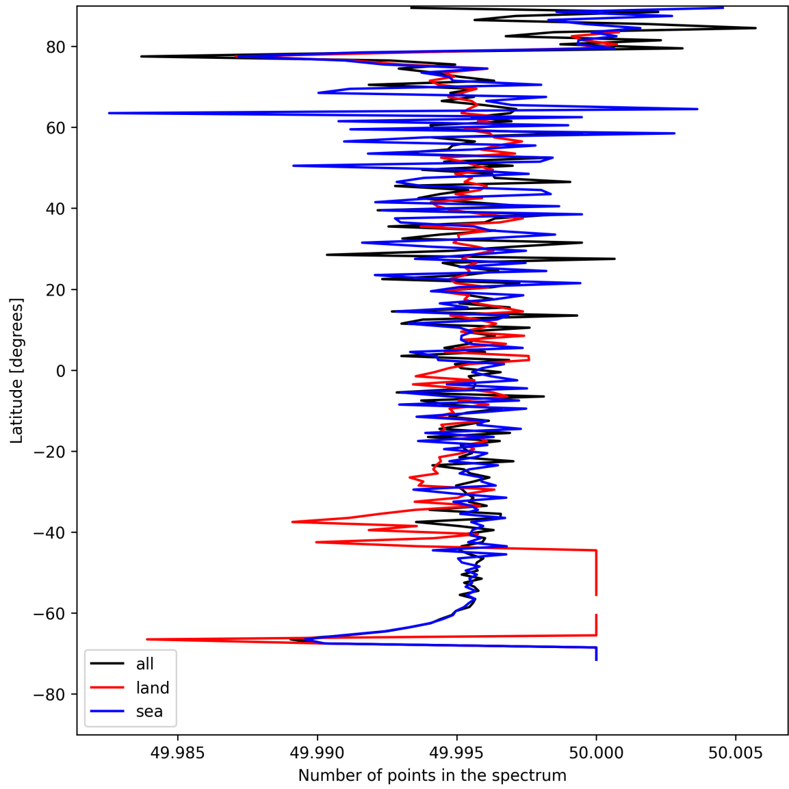
Figure 27: Zonal average of “Number of points in the spectrum” for 2025-05-03 to 2025-05-05.
