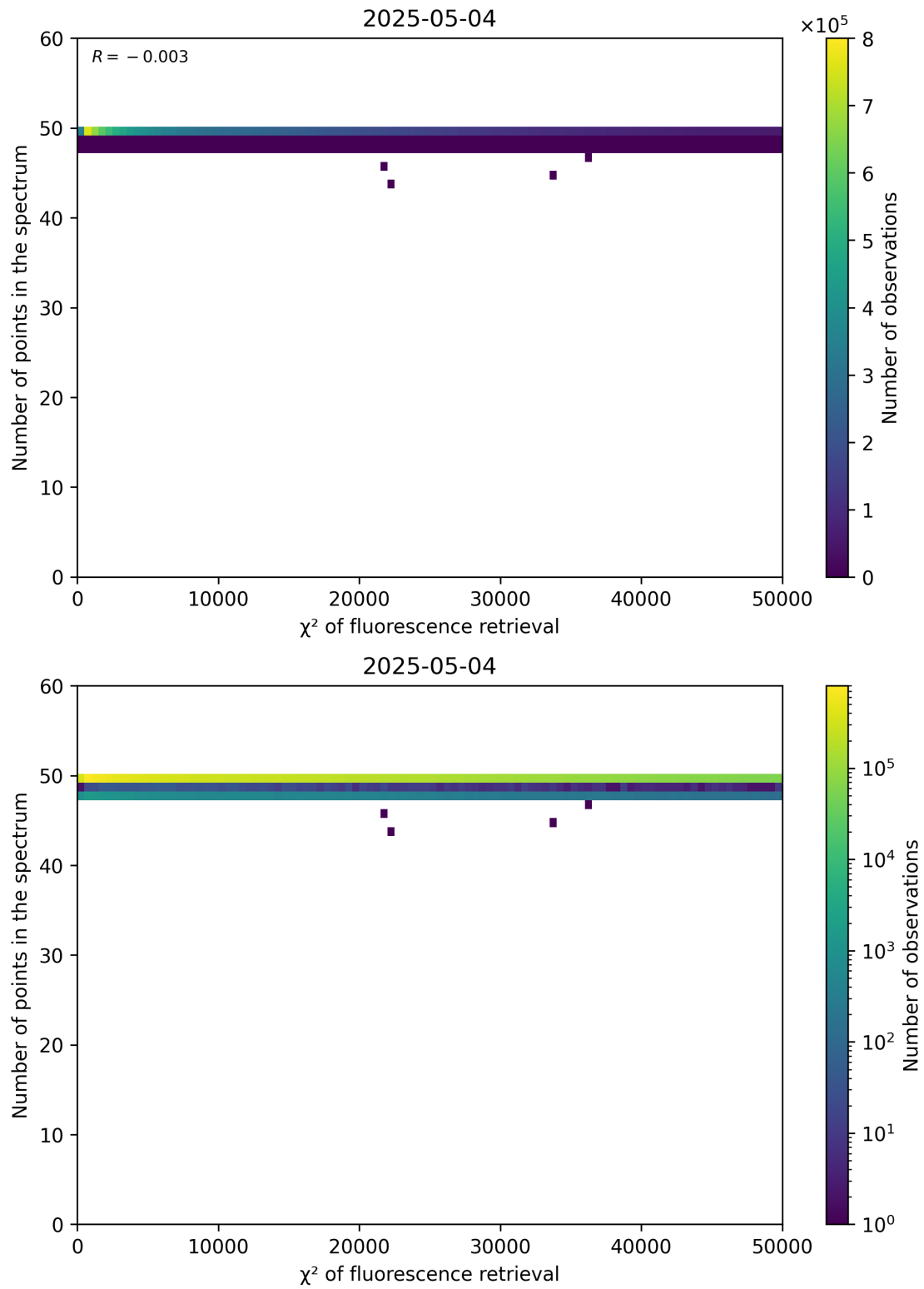
Figure 68: Scatter density plot of “ \chi^2 of fluorescence retrieval” against “Number of points in the spectrum” for 2025-05-03 to 2025-05-05.
