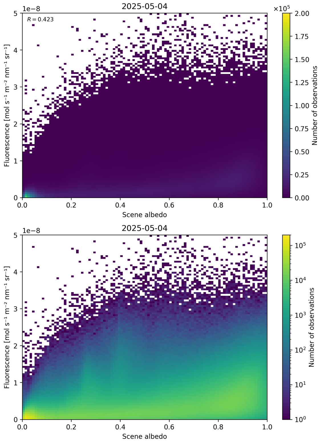
Figure 104: Scatter density plot of “Scene albedo” against “Fluorescence” for 2025-05-03 to 2025-05-05.
