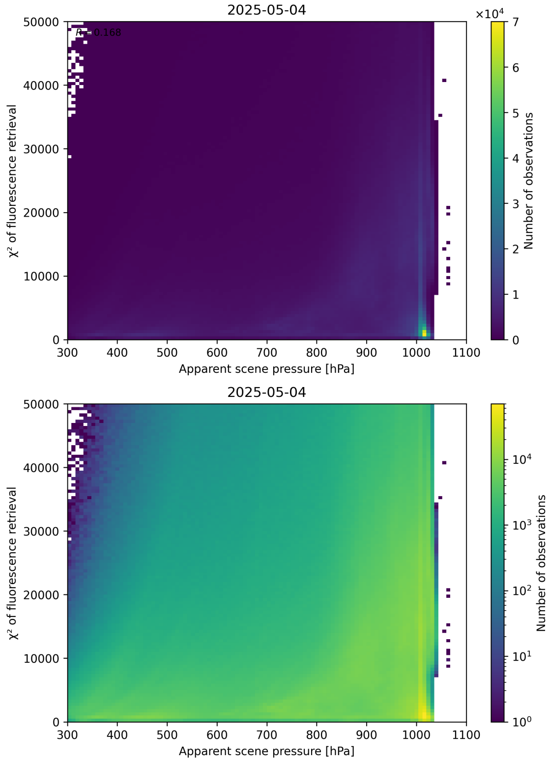
Figure 63: Scatter density plot of “Apparent scene pressure” against “ \chi^2 of fluorescence retrieval” for 2025-05-03 to 2025-05-05.
