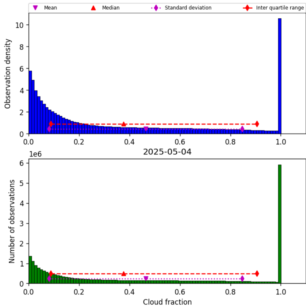
Figure 32: Histogram of “Cloud fraction” for 2025-05-03 to 2025-05-05
