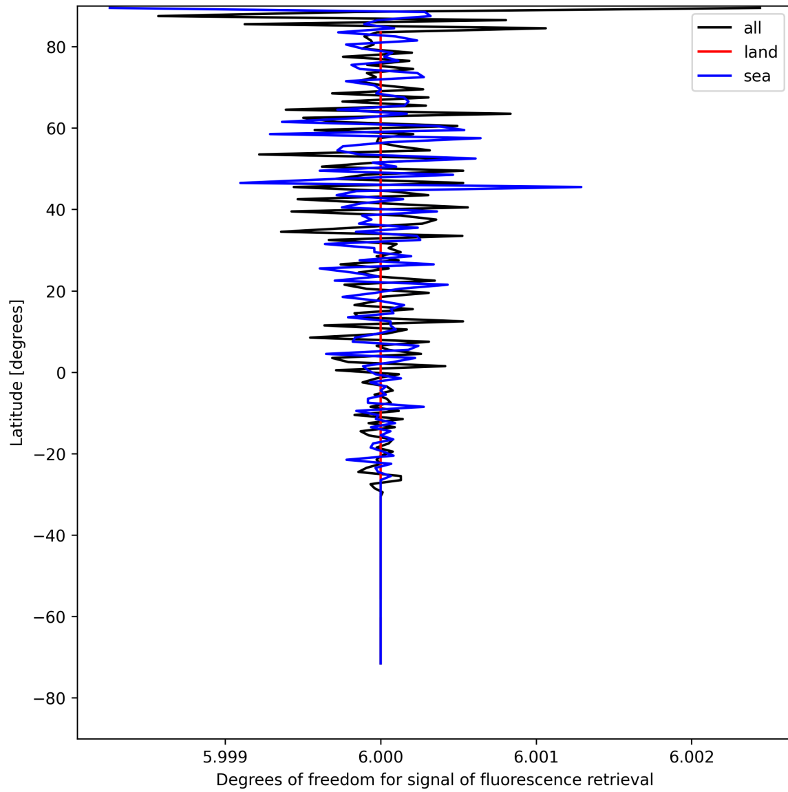
Figure 26: Zonal average of “Degrees of freedom for signal of fluorescence retrieval” for 2025-05-03 to 2025-05-05.
