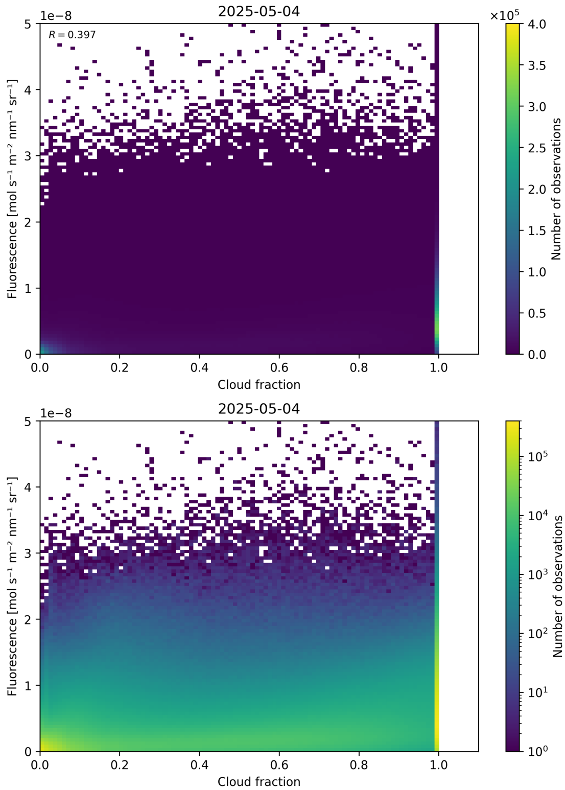
Figure 72: Scatter density plot of “Cloud fraction” against “Fluorescence” for 2025-05-03 to 2025-05-05.
