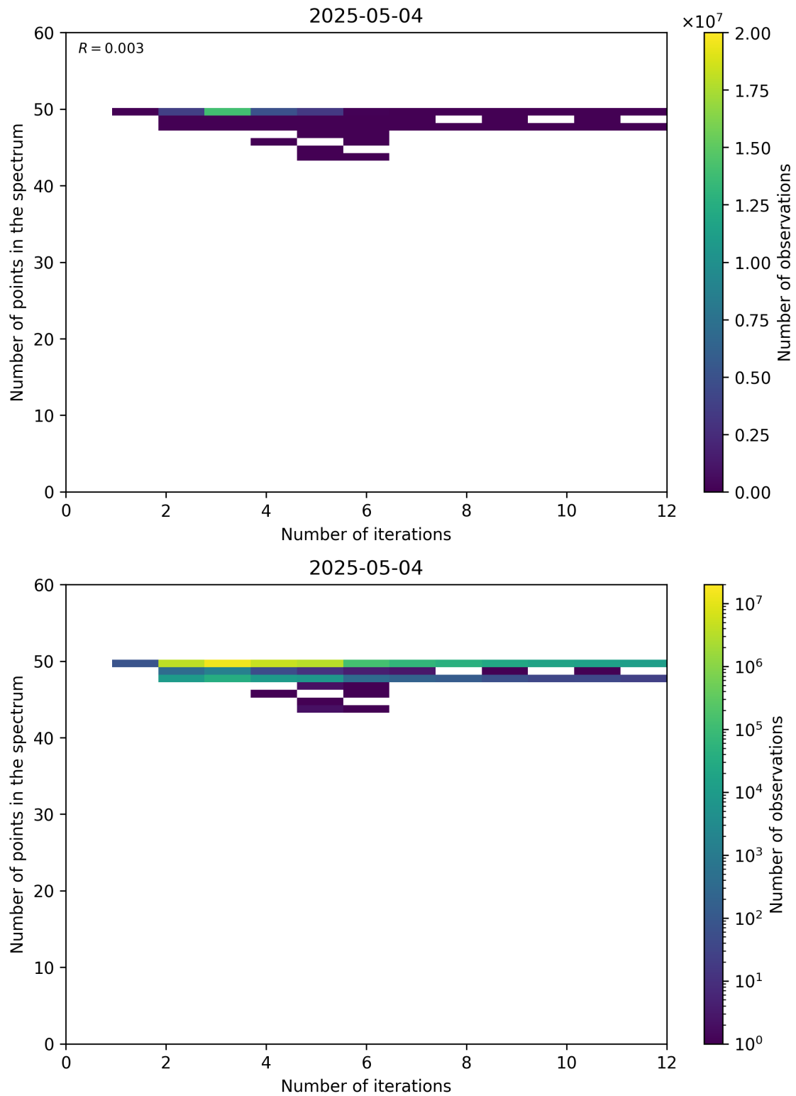
Figure 99: Scatter density plot of “Number of iterations” against “Number of points in the spectrum” for 2025-05-03 to 2025-05-05.
