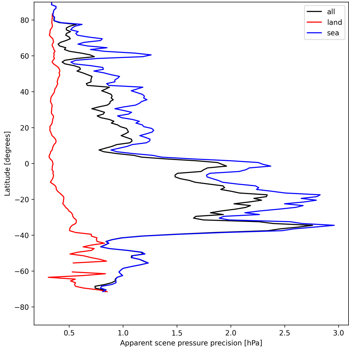
Figure 20: Zonal average of “Apparent scene pressure precision” for 2025-05-03 to 2025-05-05.
