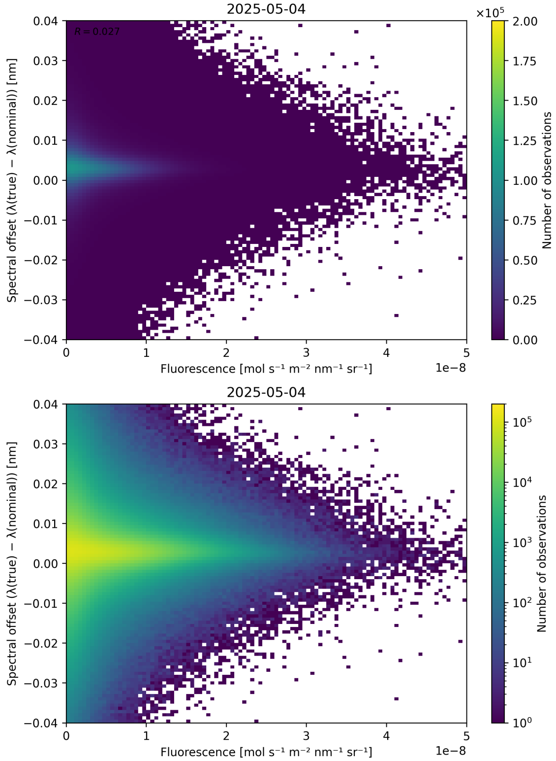
Figure 87: Scatter density plot of “Fluorescence” against “Spectral offset ( \lambda_{\text{true}} - \lambda_{\text{nominal}} )” for 2025-05-03 to 2025-05-05.
