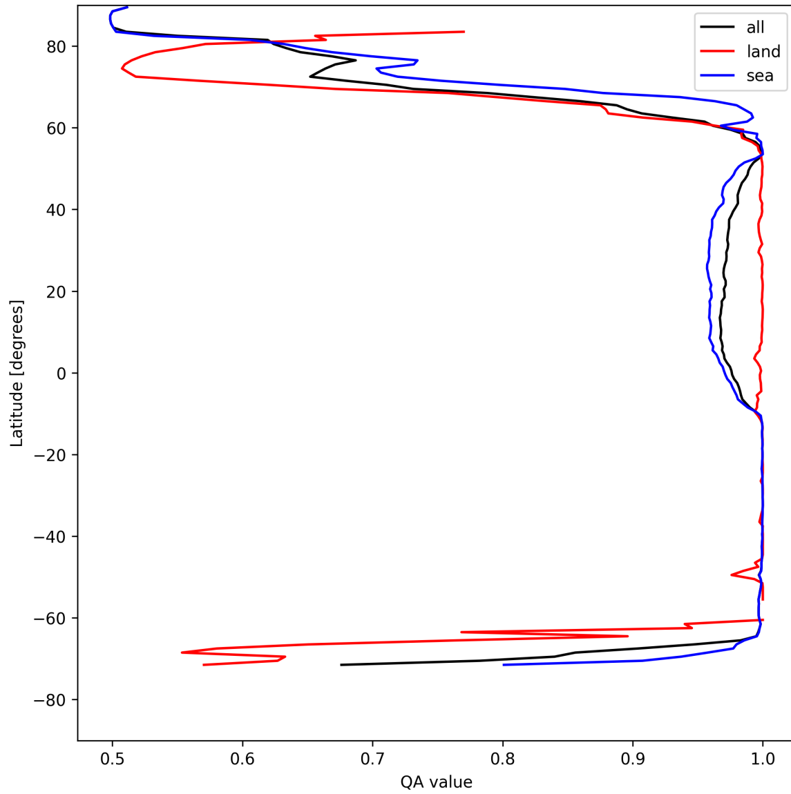
Figure 12: Zonal average of “QA value” for 2025-05-03 to 2025-05-05.
