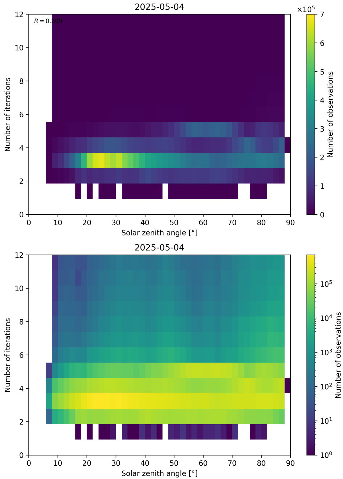
Figure 114: Scatter density plot of “Solar zenith angle” against “Number of iterations” for 2025-05-03 to 2025-05-05.
