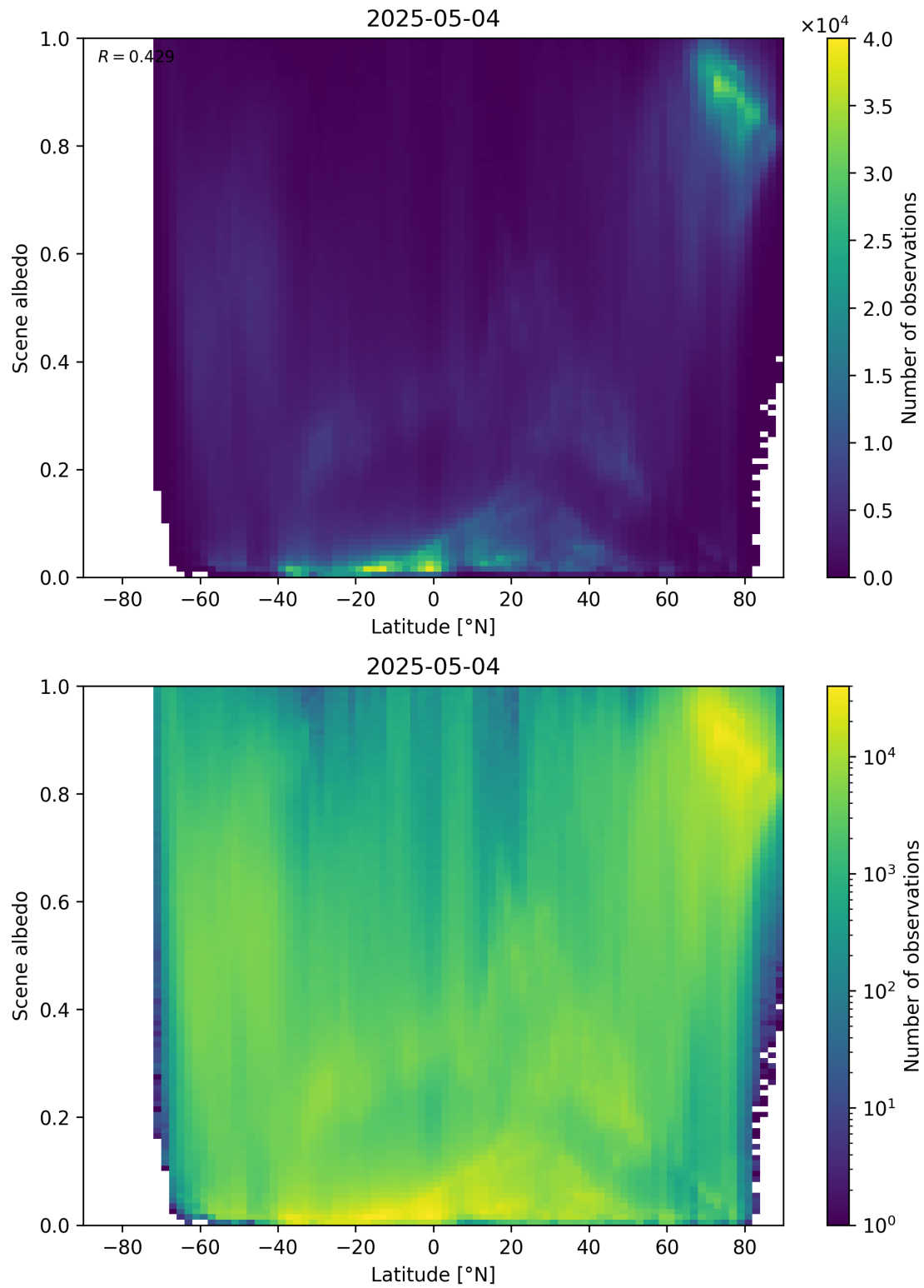
Figure 95: Scatter density plot of “Latitude” against “Scene albedo” for 2025-05-03 to 2025-05-05.
