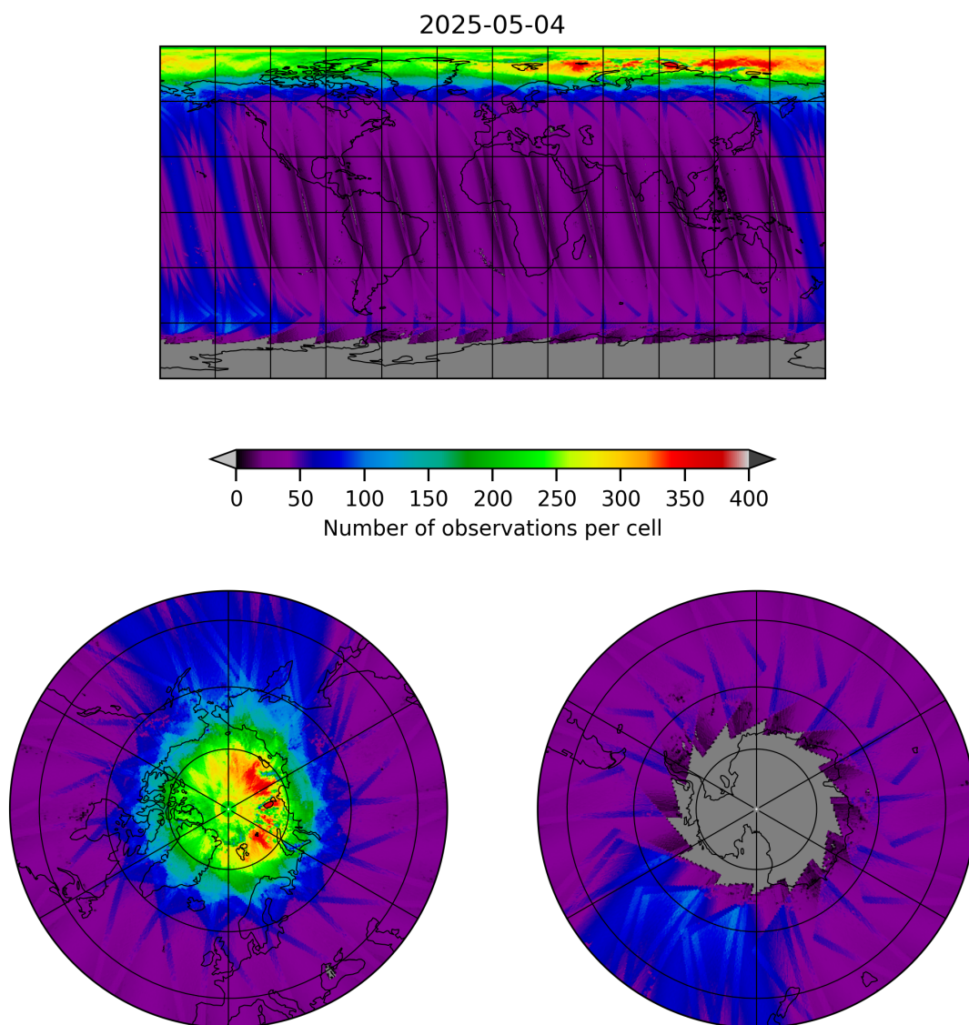
Figure 11: Map of the number of observations for 2025-05-03 to 2025-05-05
