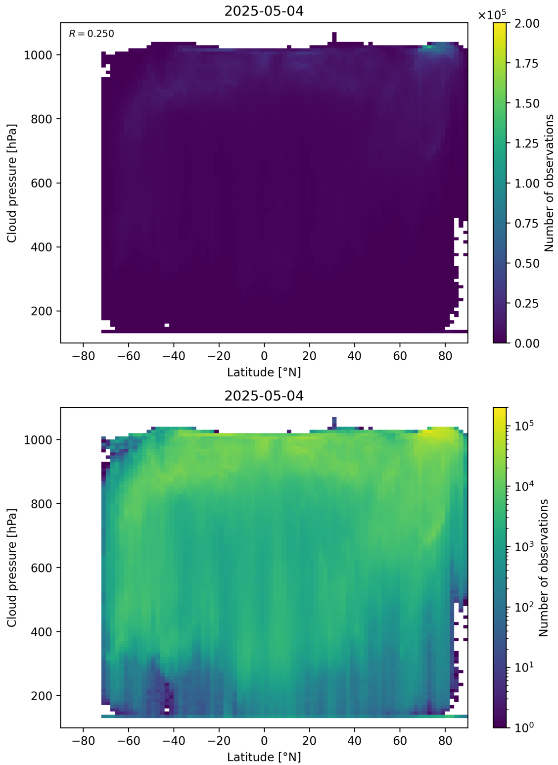
Figure 91: Scatter density plot of “Latitude” against “Cloud pressure” for 2025-05-03 to 2025-05-05.
