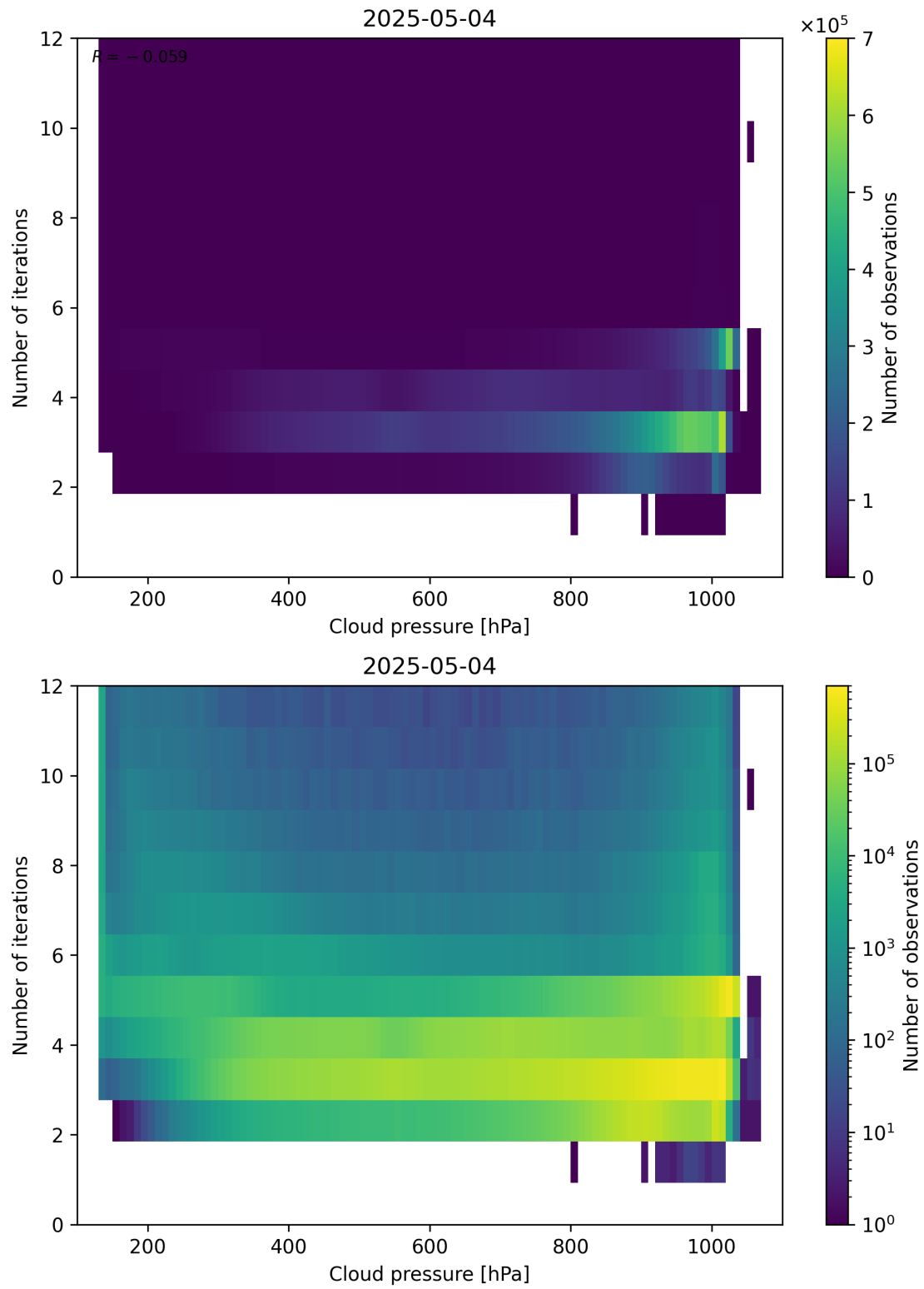
Figure 81: Scatter density plot of “Cloud pressure” against “Number of iterations” for 2025-05-03 to 2025-05-05.
