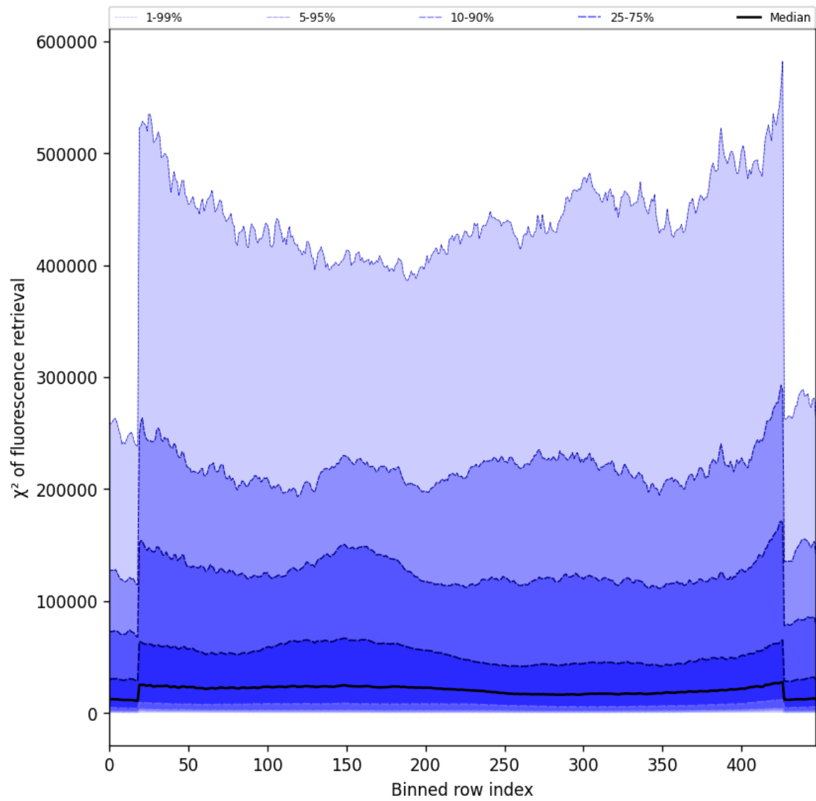
Figure 59: Along track statistics of “ \chi^2 of fluorescence retrieval” for 2025-05-03 to 2025-05-05
