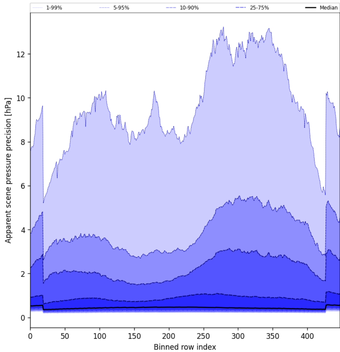
Figure 54: Along track statistics of “Apparent scene pressure precision” for 2025-05-03 to 2025-05-05
