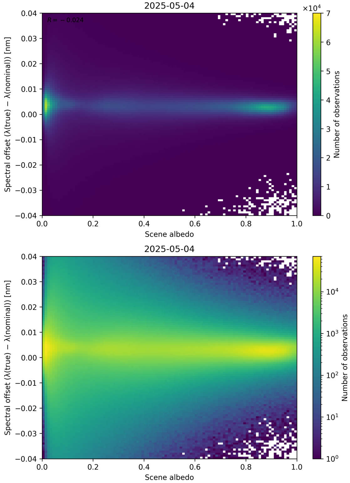
Figure 107: Scatter density plot of “Scene albedo” against “Spectral offset ( \lambda_{\text{true}} - \lambda_{\text{nominal}} )” for 2025-05-03 to 2025-05-05.
