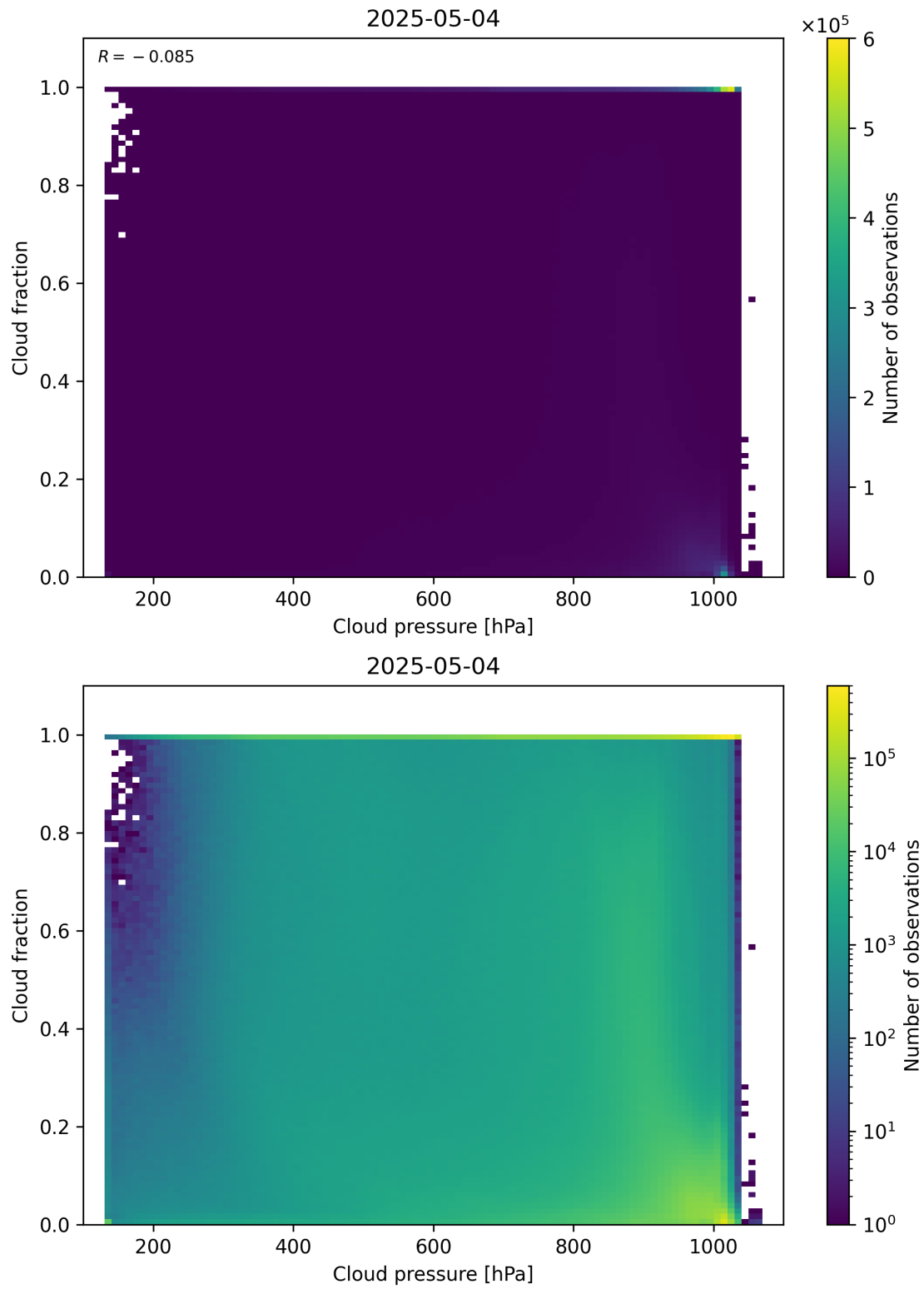
Figure 79: Scatter density plot of “Cloud pressure” against “Cloud fraction” for 2025-05-03 to 2025-05-05.
