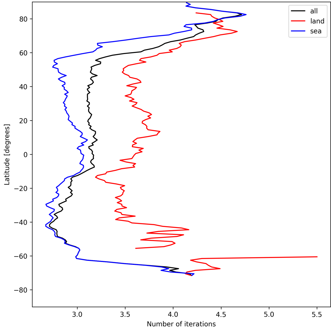
Figure 22: Zonal average of “Number of iterations” for 2025-05-03 to 2025-05-05.
