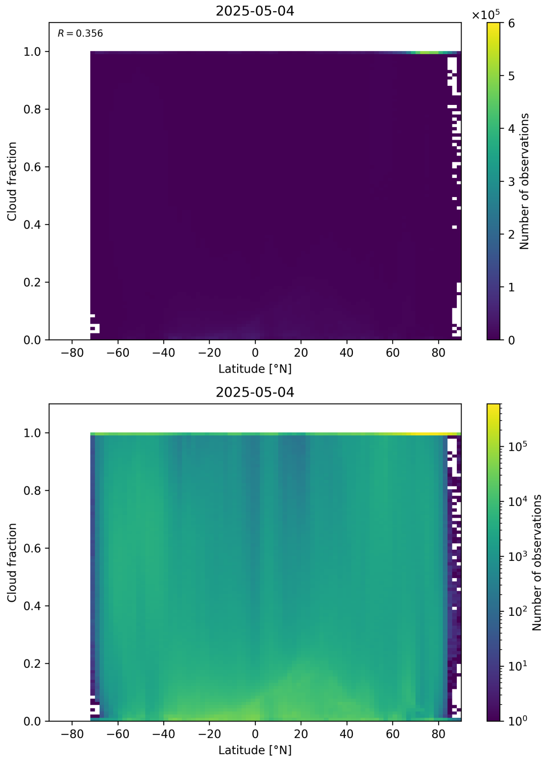
Figure 90: Scatter density plot of “Latitude” against “Cloud fraction” for 2025-05-03 to 2025-05-05.
