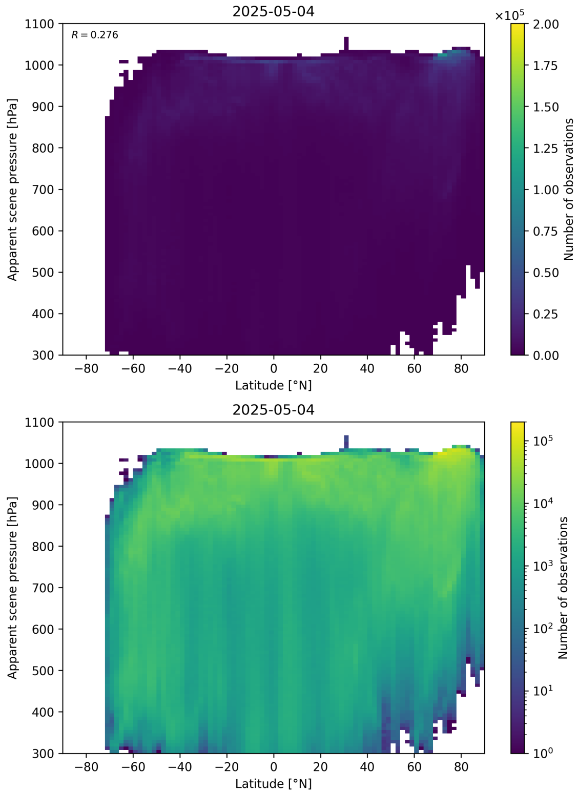
Figure 88: Scatter density plot of “Latitude” against “Apparent scene pressure” for 2025-05-03 to 2025-05-05.
