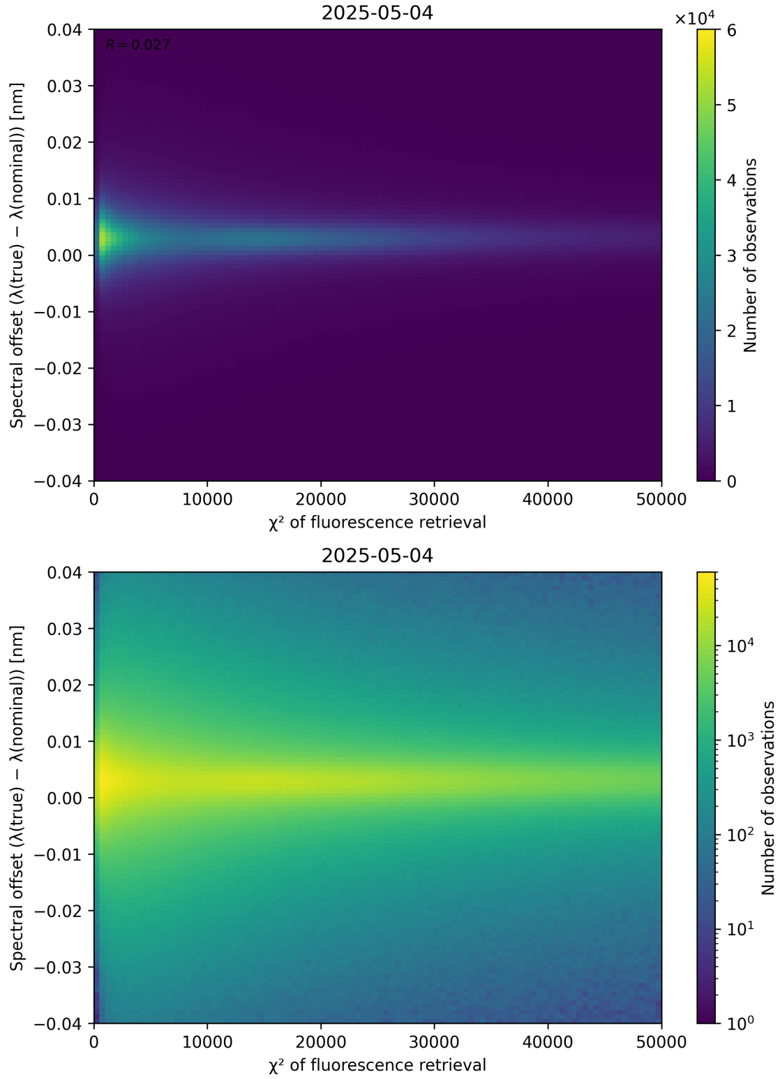
Figure 69: Scatter density plot of “ \chi^2 of fluorescence retrieval” against “Spectral offset ( \lambda_{\text{true}} - \lambda_{\text{nominal}} )” for 2025-05-03 to 2025-05-05.
