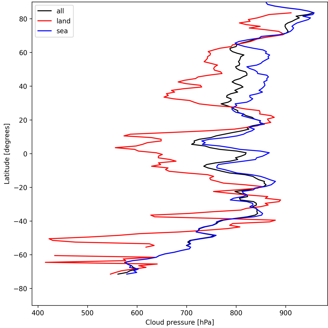
Figure 13: Zonal average of “Cloud pressure” for 2025-05-03 to 2025-05-05.
