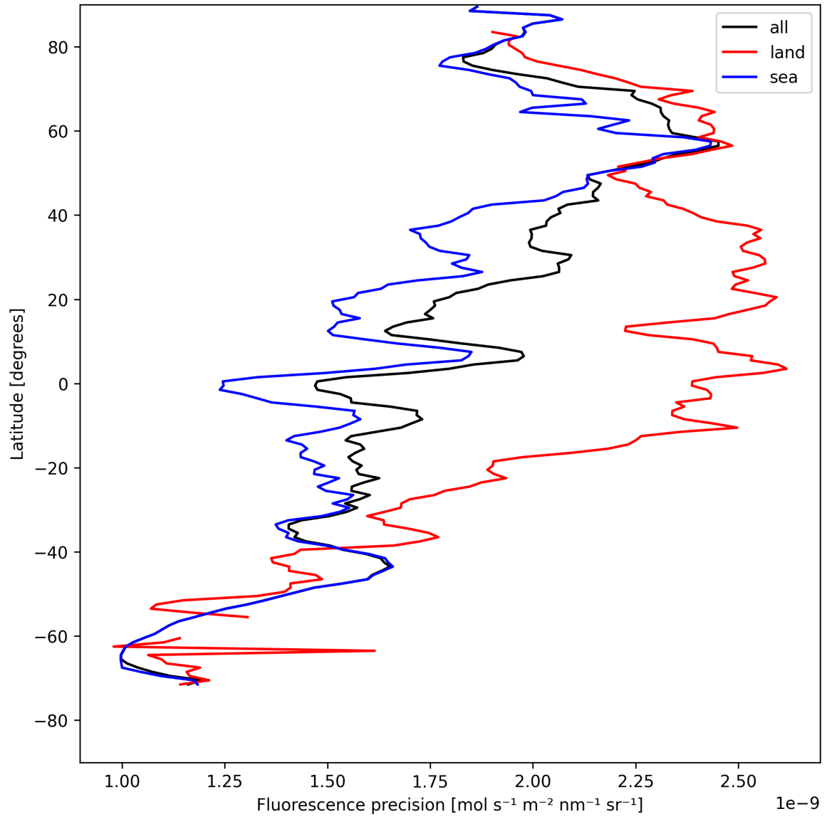
Figure 24: Zonal average of “Fluorescence precision” for 2025-05-03 to 2025-05-05.
