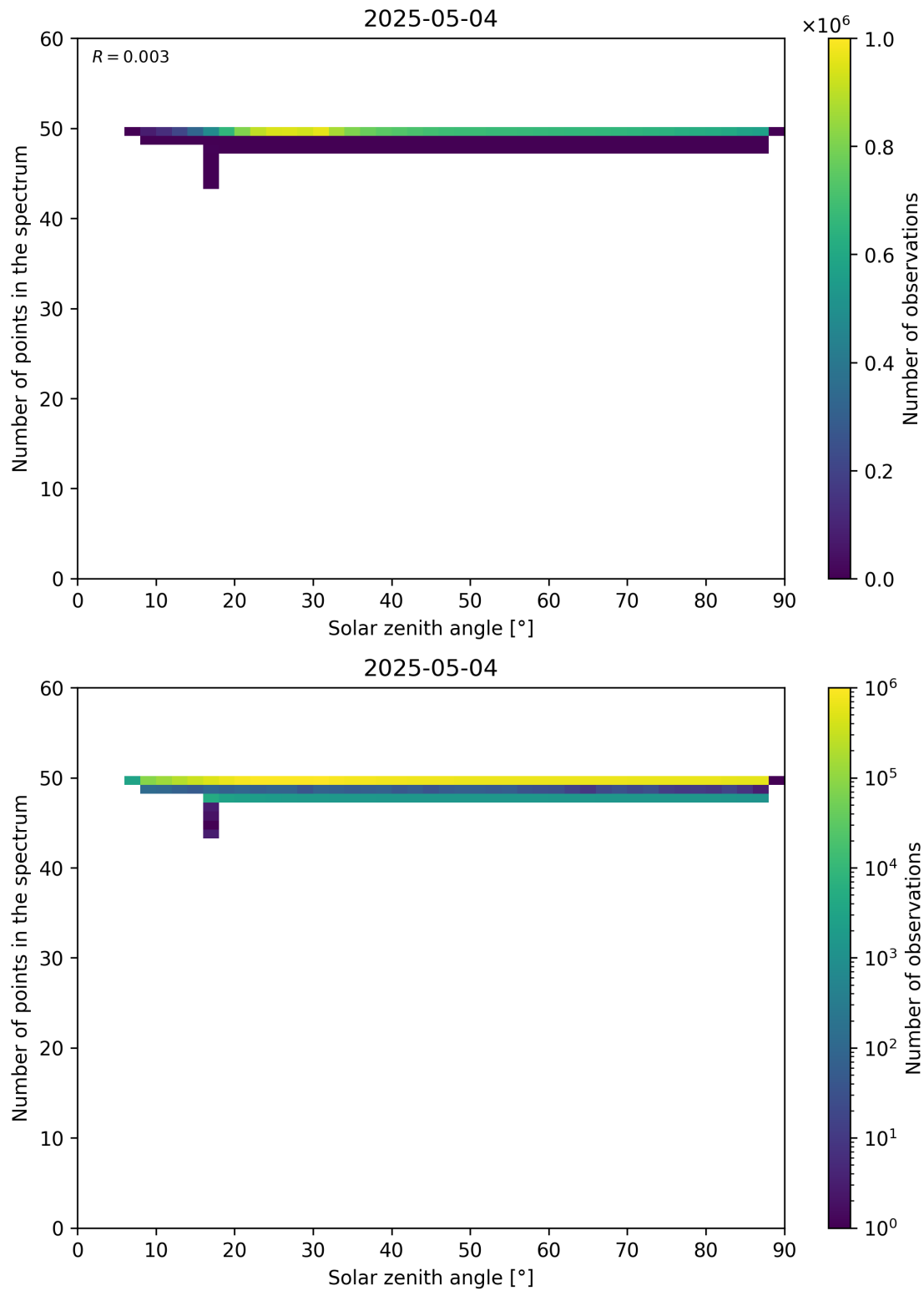
Figure 115: Scatter density plot of “Solar zenith angle” against “Number of points in the spectrum” for 2025-05-03 to 2025-05-05.
