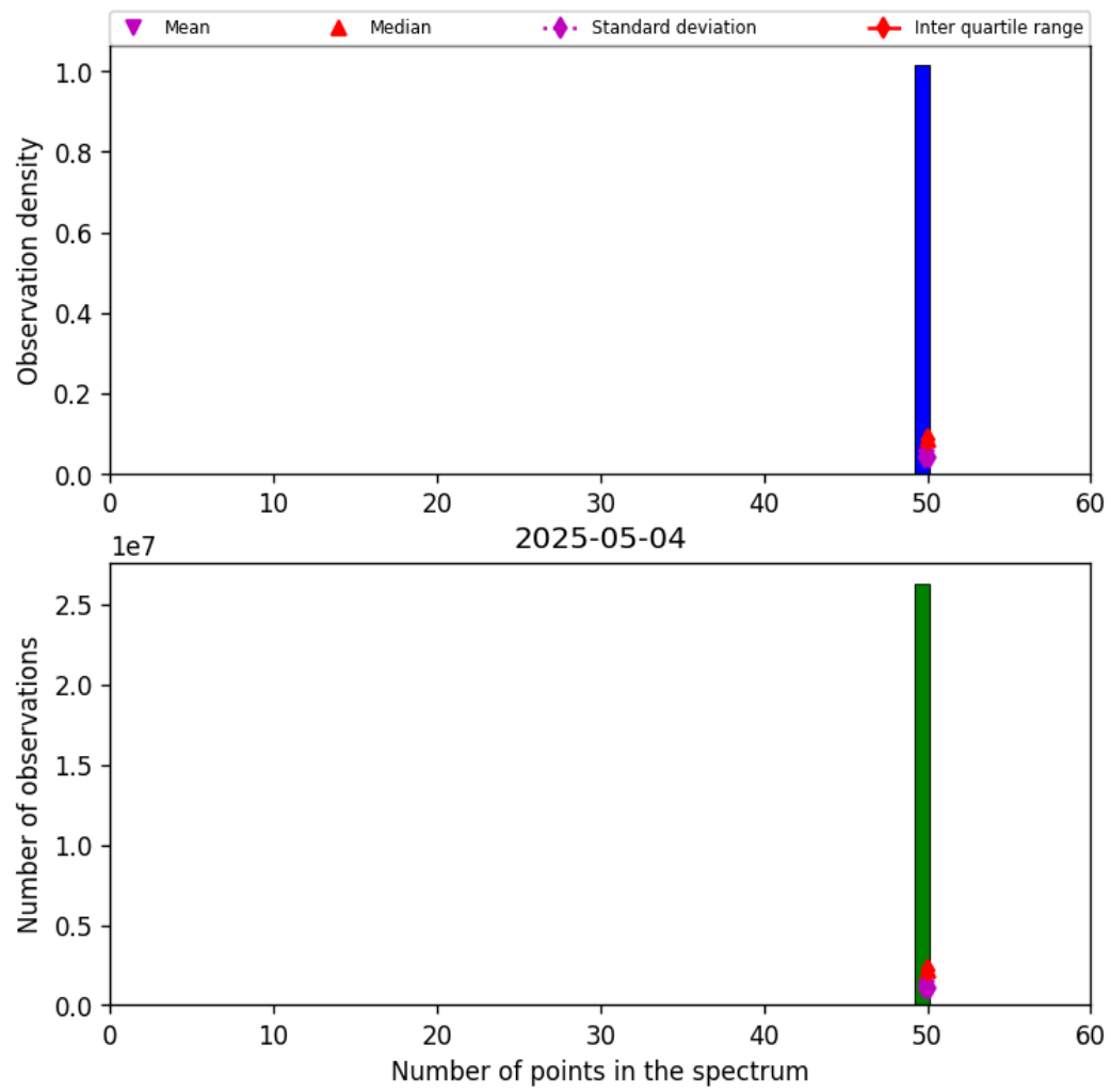
Figure 44: Histogram of “Number of points in the spectrum” for 2025-05-03 to 2025-05-05
