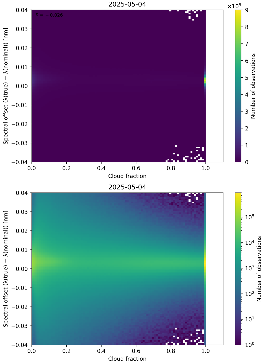
Figure 76: Scatter density plot of “Cloud fraction” against “Spectral offset ( \lambda_{\text{true}} - \lambda_{\text{nominal}} )” for 2025-05-03 to 2025-05-05.
