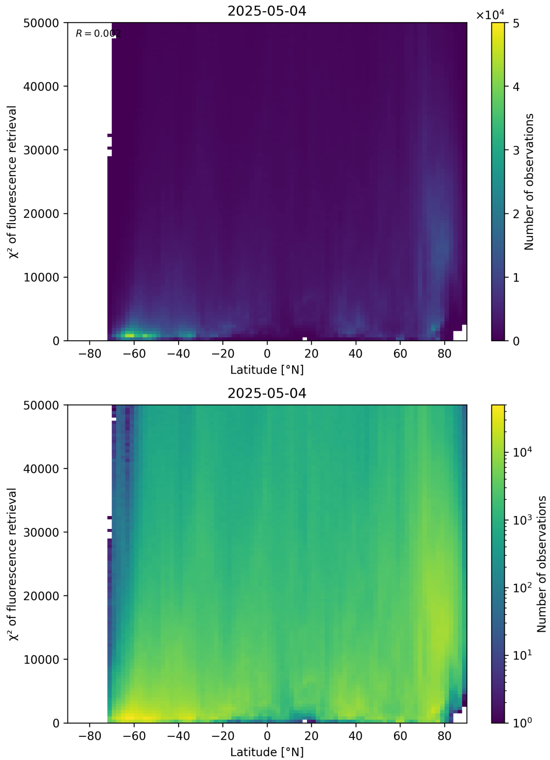
Figure 89: Scatter density plot of “Latitude” against “ \chi^2 of fluorescence retrieval” for 2025-05-03 to 2025-05-05.
