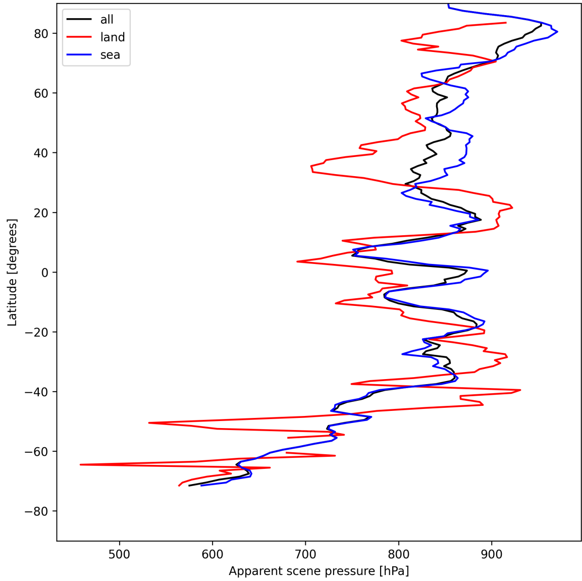
Figure 19: Zonal average of “Apparent scene pressure” for 2025-05-03 to 2025-05-05.
