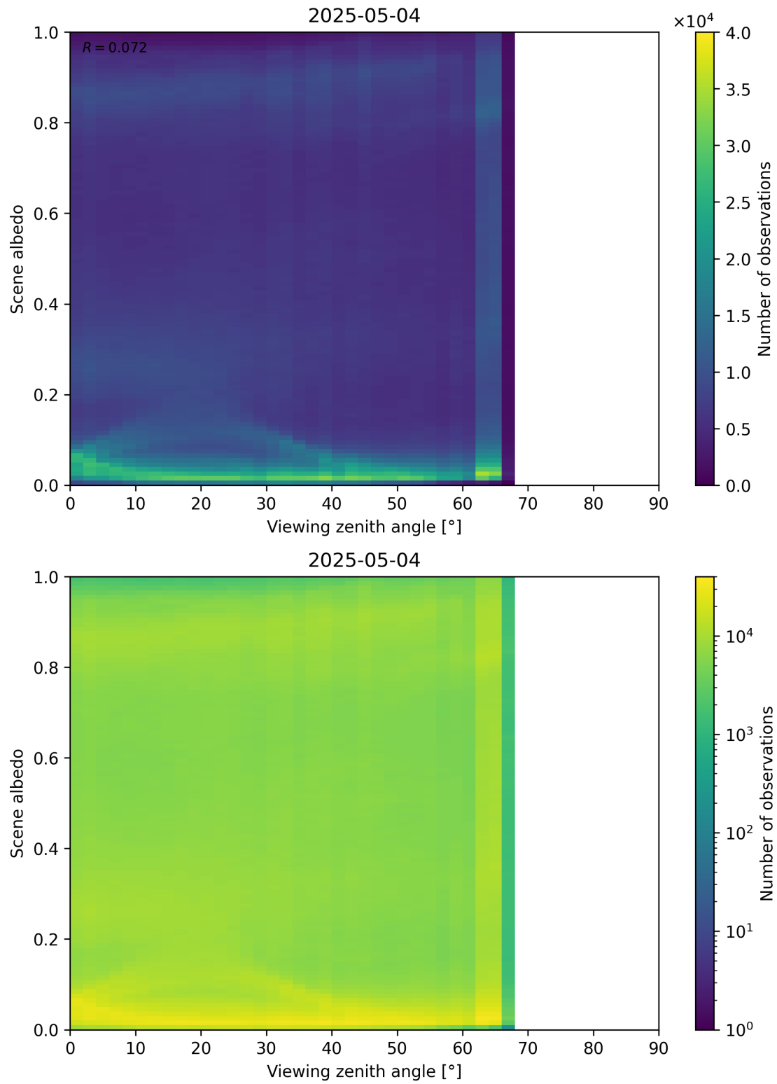
Figure 126: Scatter density plot of “Viewing zenith angle” against “Scene albedo” for 2025-05-03 to 2025-05-05.
