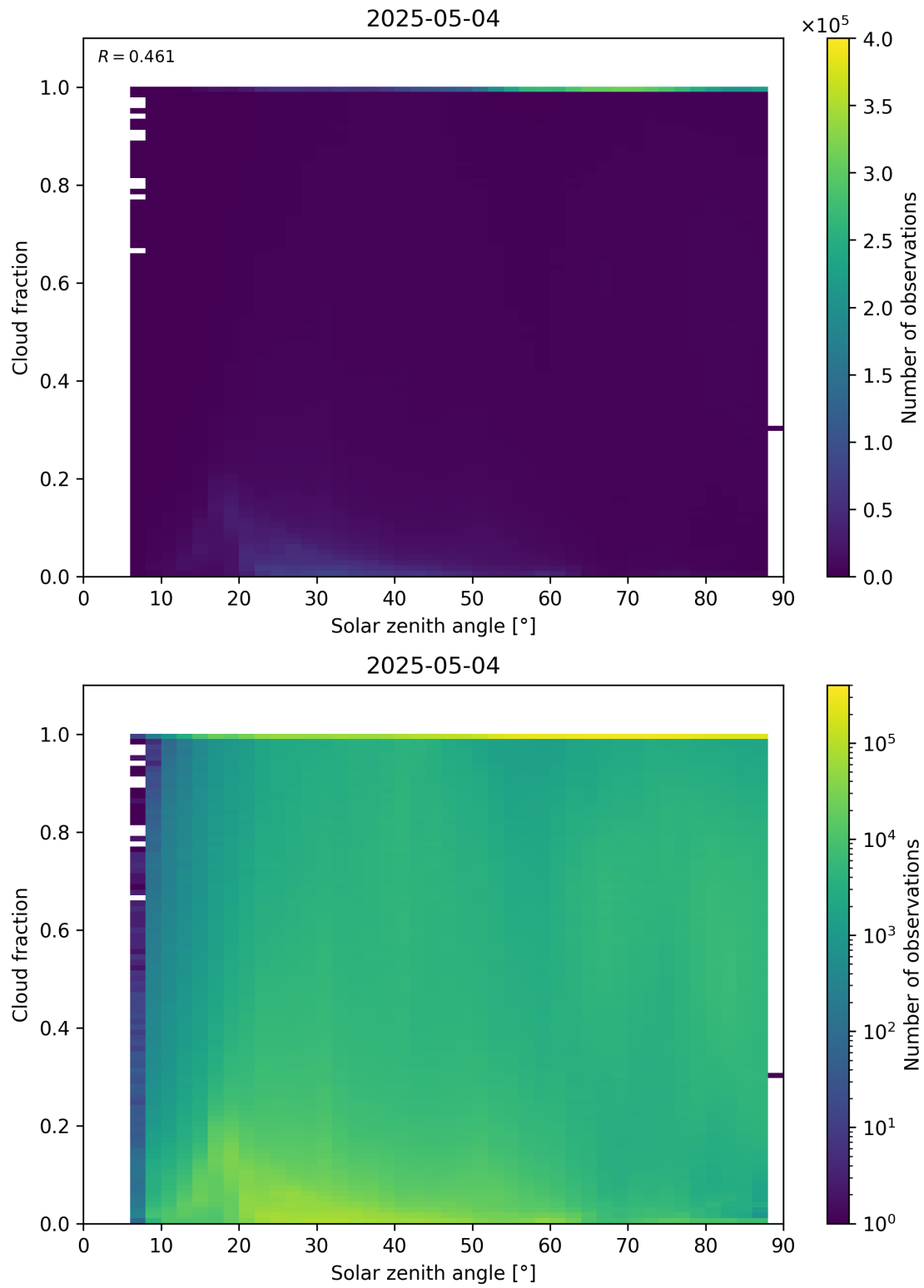
Figure 110: Scatter density plot of “Solar zenith angle” against “Cloud fraction” for 2025-05-03 to 2025-05-05.
