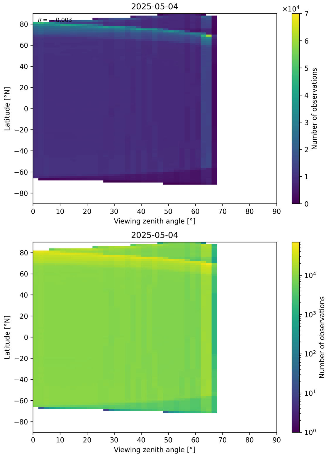
Figure 123: Scatter density plot of “Viewing zenith angle” against “Latitude” for 2025-05-03 to 2025-05-05.
