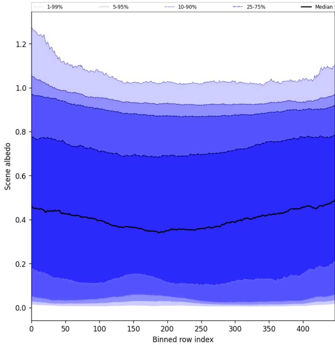
Figure 51: Along track statistics of “Scene albedo” for 2025-05-03 to 2025-05-05
