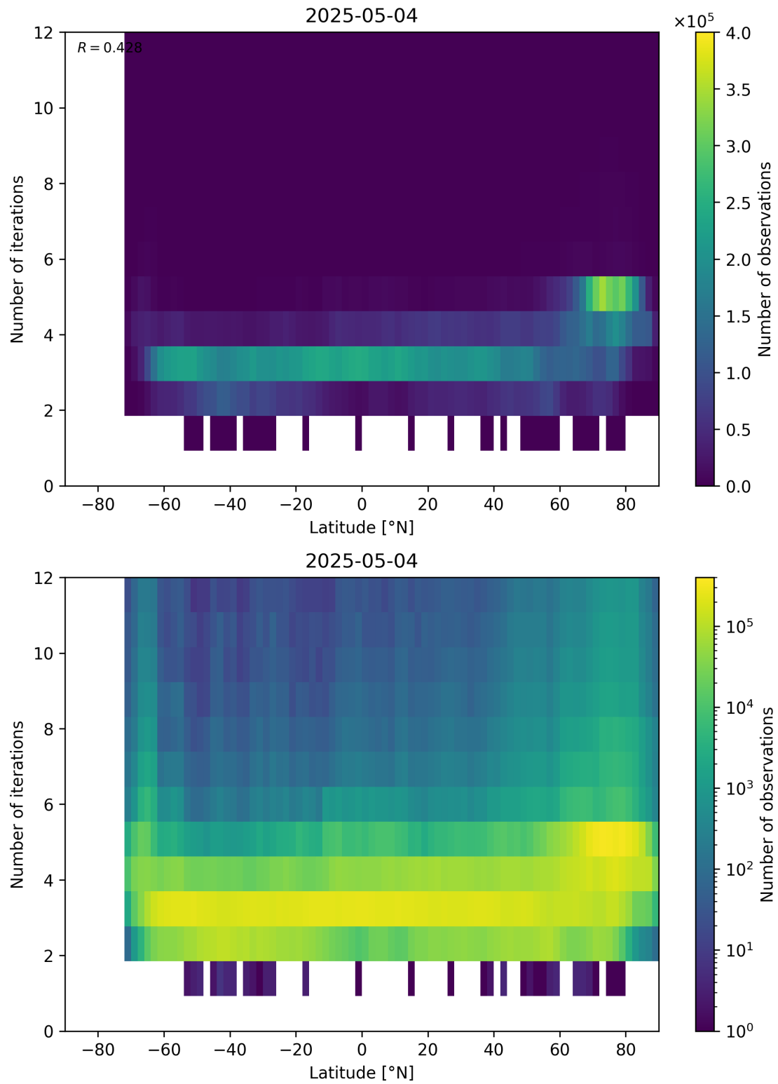
Figure 93: Scatter density plot of “Latitude” against “Number of iterations” for 2025-05-03 to 2025-05-05.
