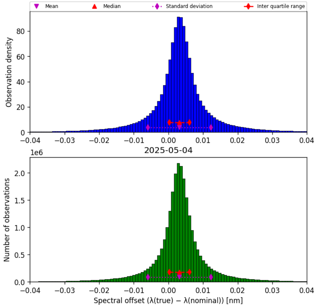
Figure 45: Histogram of “Spectral offset ( \lambda_{\text{true}} - \lambda_{\text{nominal}} )” for 2025-05-03 to 2025-05-05
