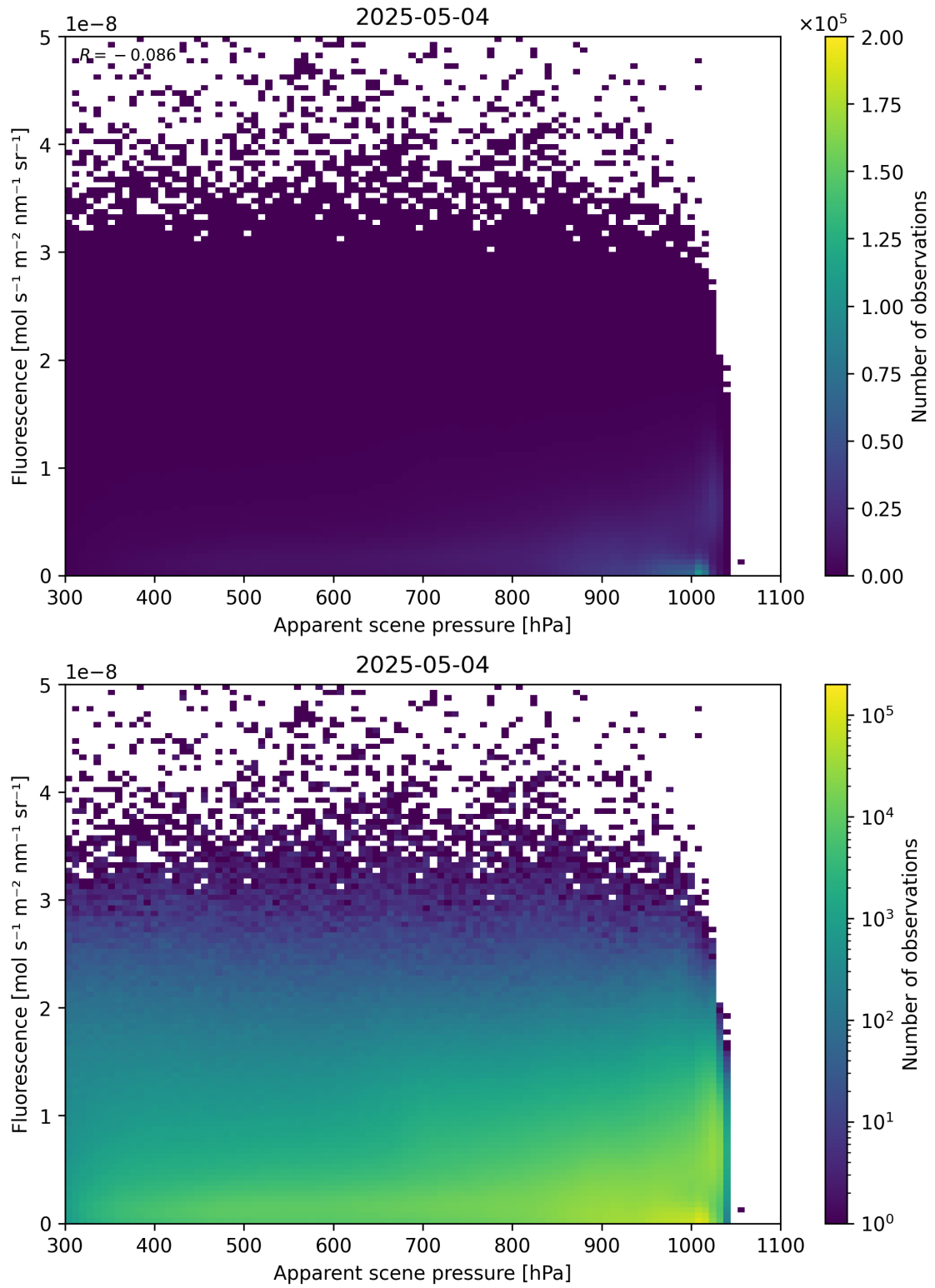
Figure 64: Scatter density plot of “Apparent scene pressure” against “Fluorescence” for 2025-05-03 to 2025-05-05.
