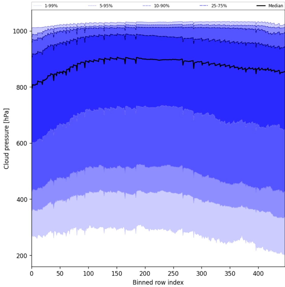
Figure 47: Along track statistics of “Cloud pressure” for 2025-05-03 to 2025-05-05
