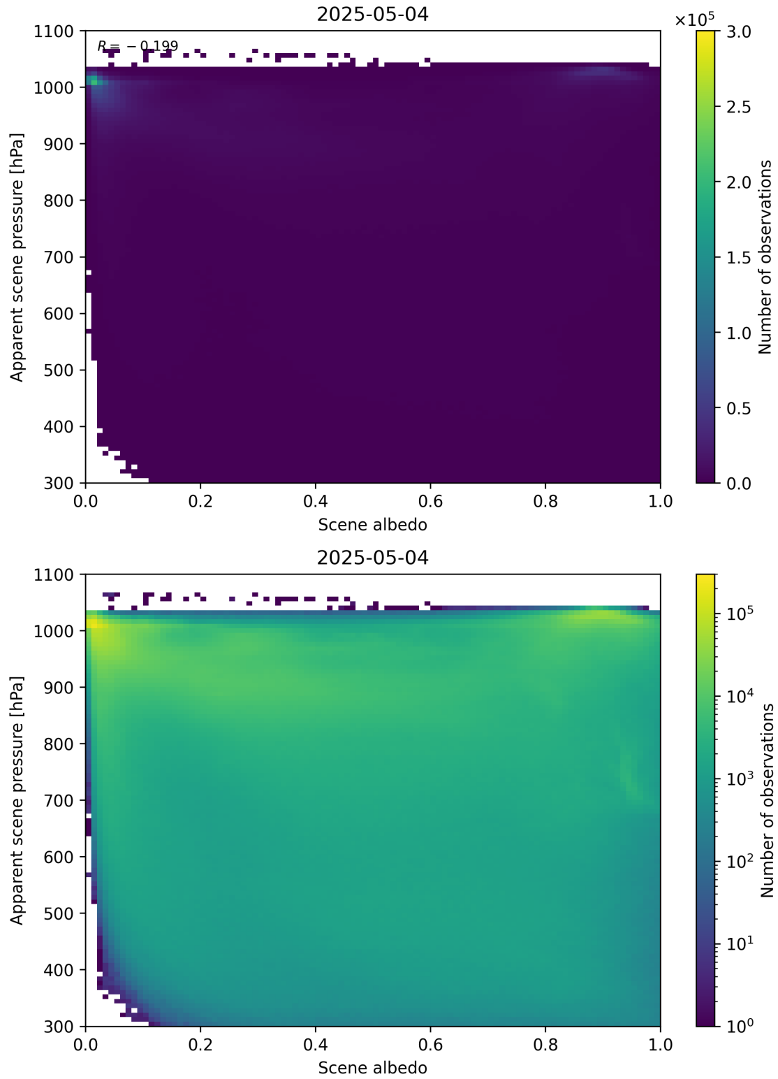
Figure 102: Scatter density plot of “Scene albedo” against “Apparent scene pressure” for 2025-05-03 to 2025-05-05.
