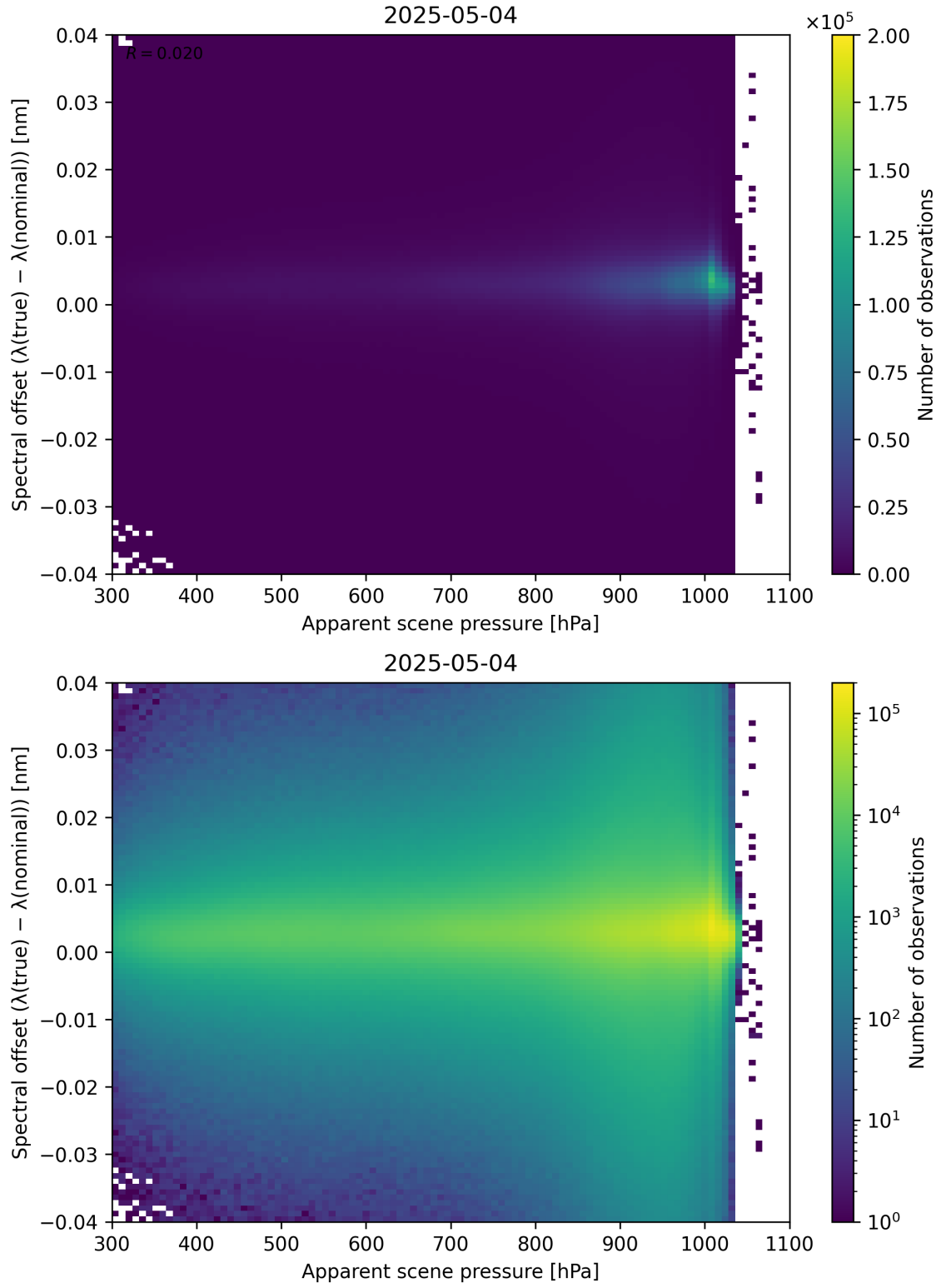
Figure 67: Scatter density plot of “Apparent scene pressure” against “Spectral offset ( \lambda_{\text{true}} - \lambda_{\text{nominal}} )” for 2025-05-03 to 2025-05-05.
