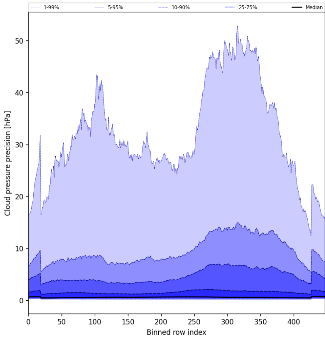
Figure 48: Along track statistics of “Cloud pressure precision” for 2025-05-03 to 2025-05-05
