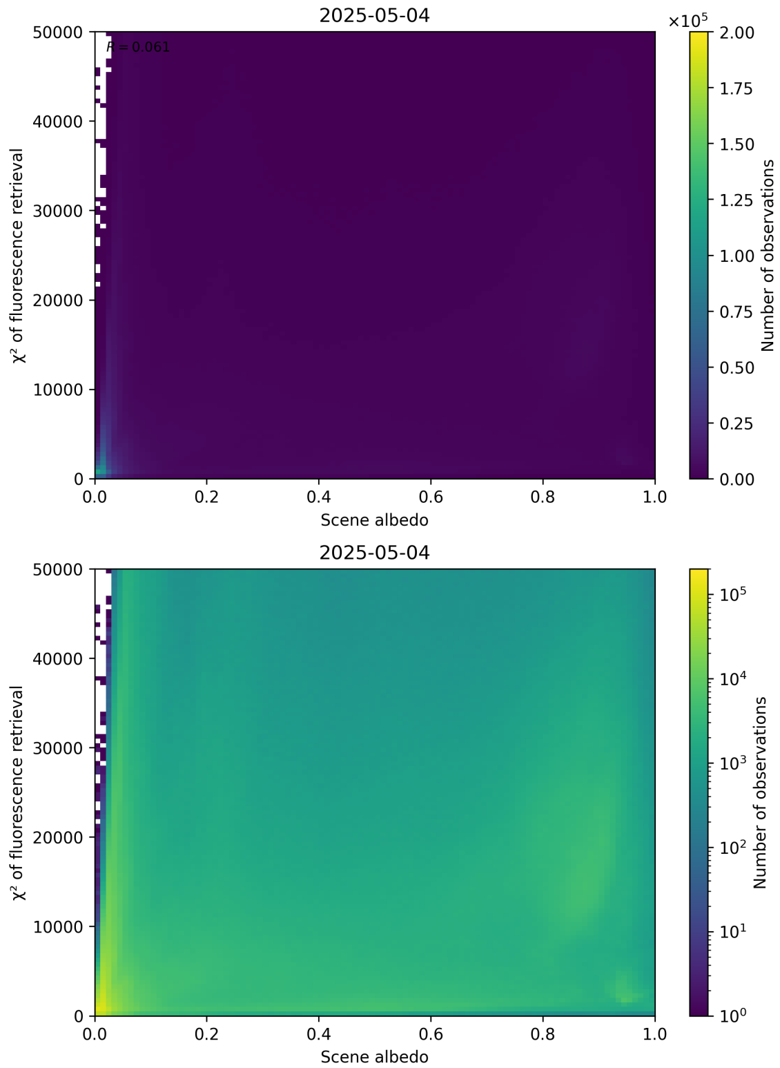
Figure 103: Scatter density plot of “Scene albedo” against “ \chi^2 of fluorescence retrieval” for 2025-05-03 to 2025-05-05.
