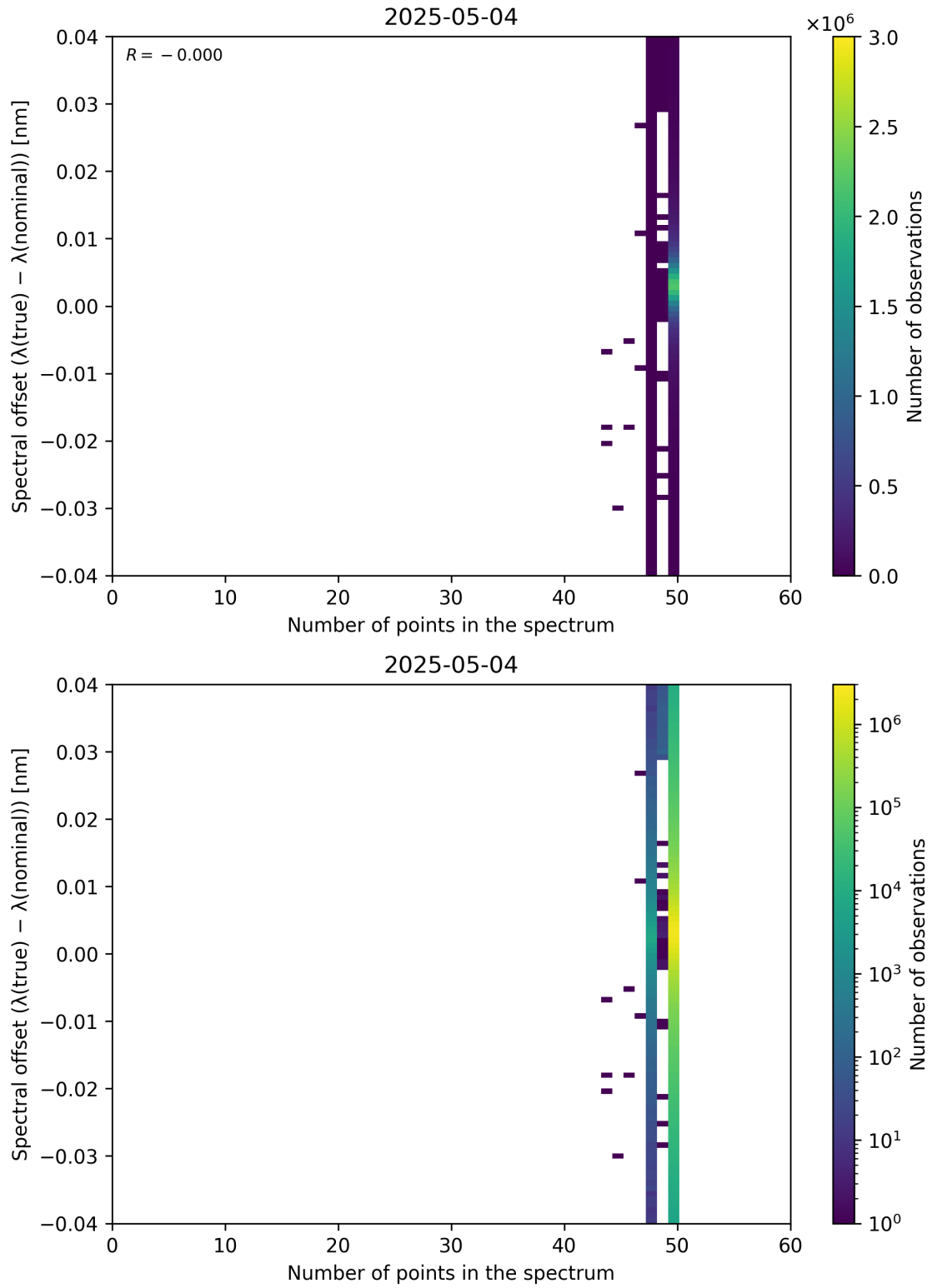
Figure 101: Scatter density plot of “Number of points in the spectrum” against “Spectral offset ( \lambda_{\text{true}} - \lambda_{\text{nominal}} )” for 2025-05-03 to 2025-05-05.
