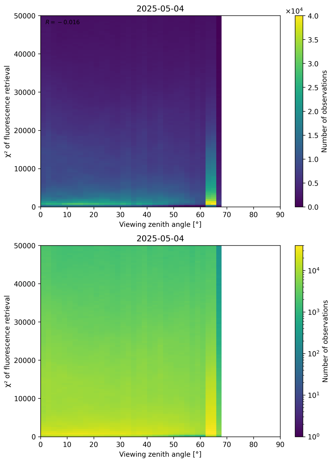
Figure 119: Scatter density plot of “Viewing zenith angle” against “ \chi^2 of fluorescence retrieval” for 2025-05-03 to 2025-05-05.
