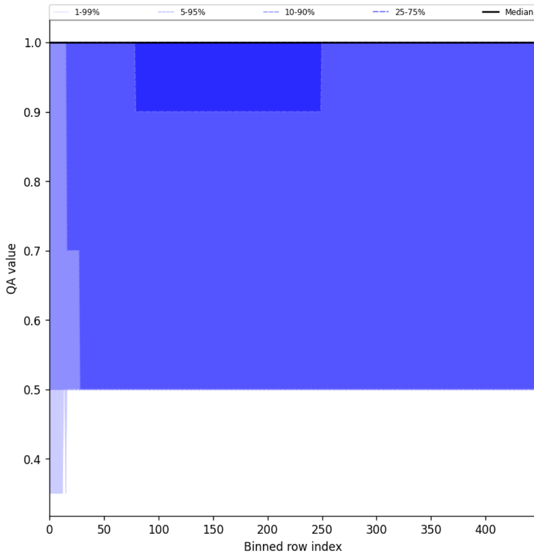
Figure 46: Along track statistics of “QA value” for 2025-05-03 to 2025-05-05
