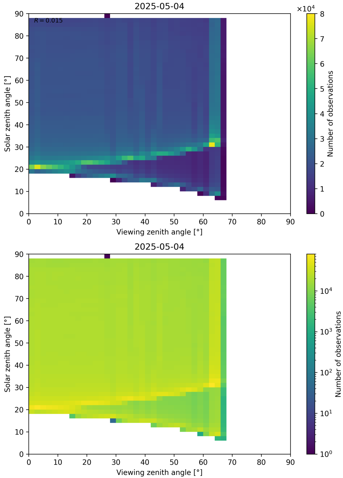
Figure 127: Scatter density plot of “Viewing zenith angle” against “Solar zenith angle” for 2025-05-03 to 2025-05-05.
