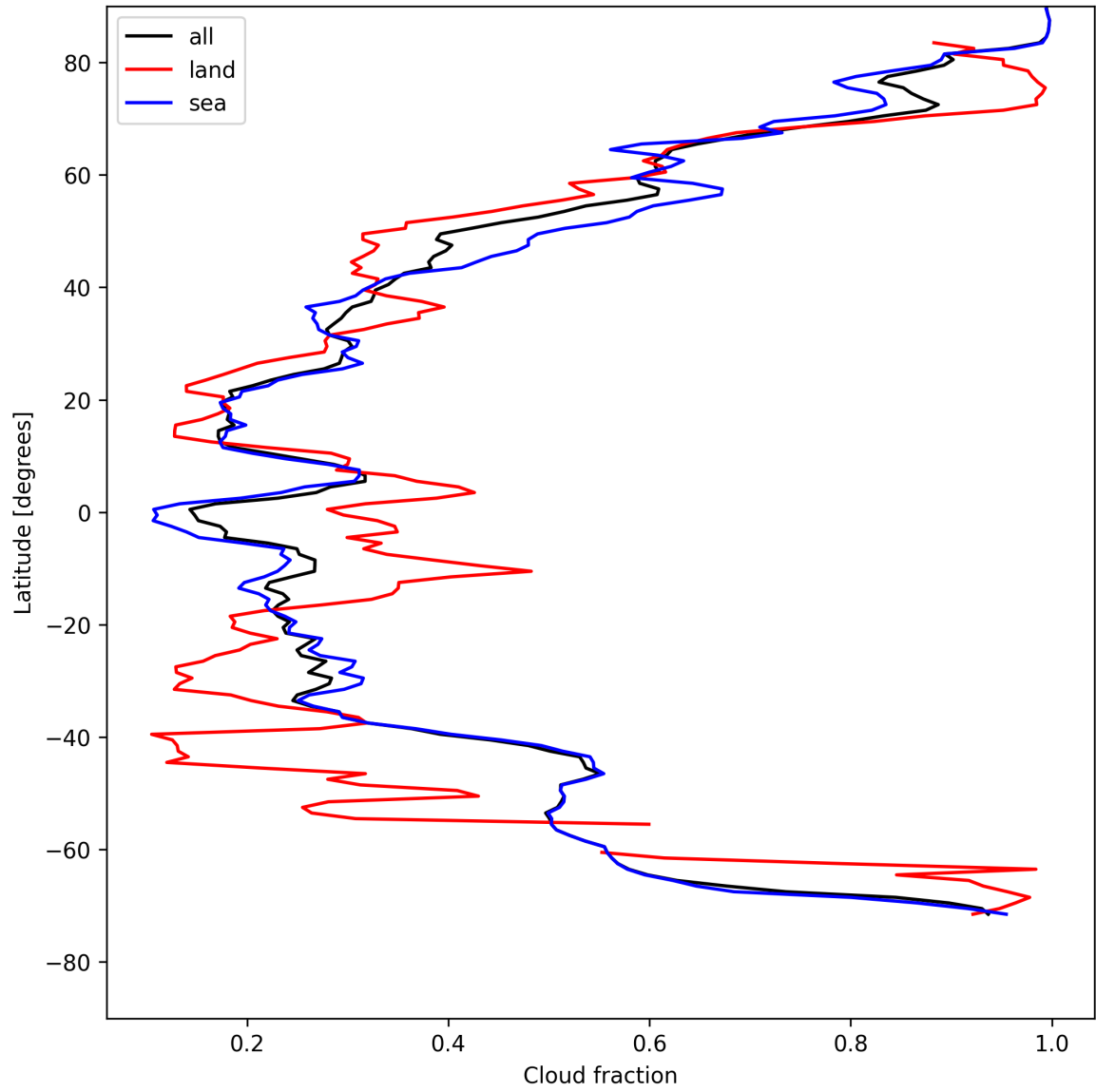
Figure 15: Zonal average of “Cloud fraction” for 2025-05-03 to 2025-05-05.
