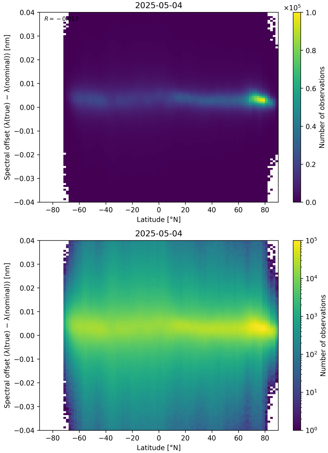
Figure 96: Scatter density plot of “Latitude” against “Spectral offset ( \lambda_{\text{true}} - \lambda_{\text{nominal}} )” for 2025-05-03 to 2025-05-05.
