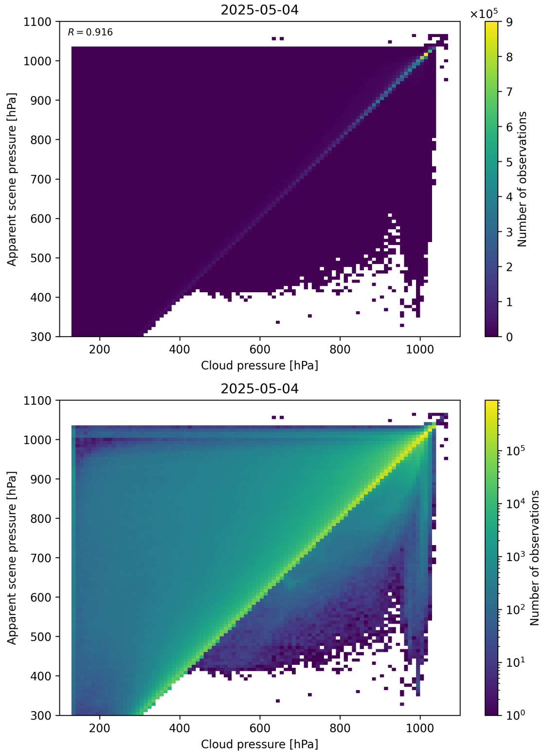
Figure 77: Scatter density plot of “Cloud pressure” against “Apparent scene pressure” for 2025-05-03 to 2025-05-05.
