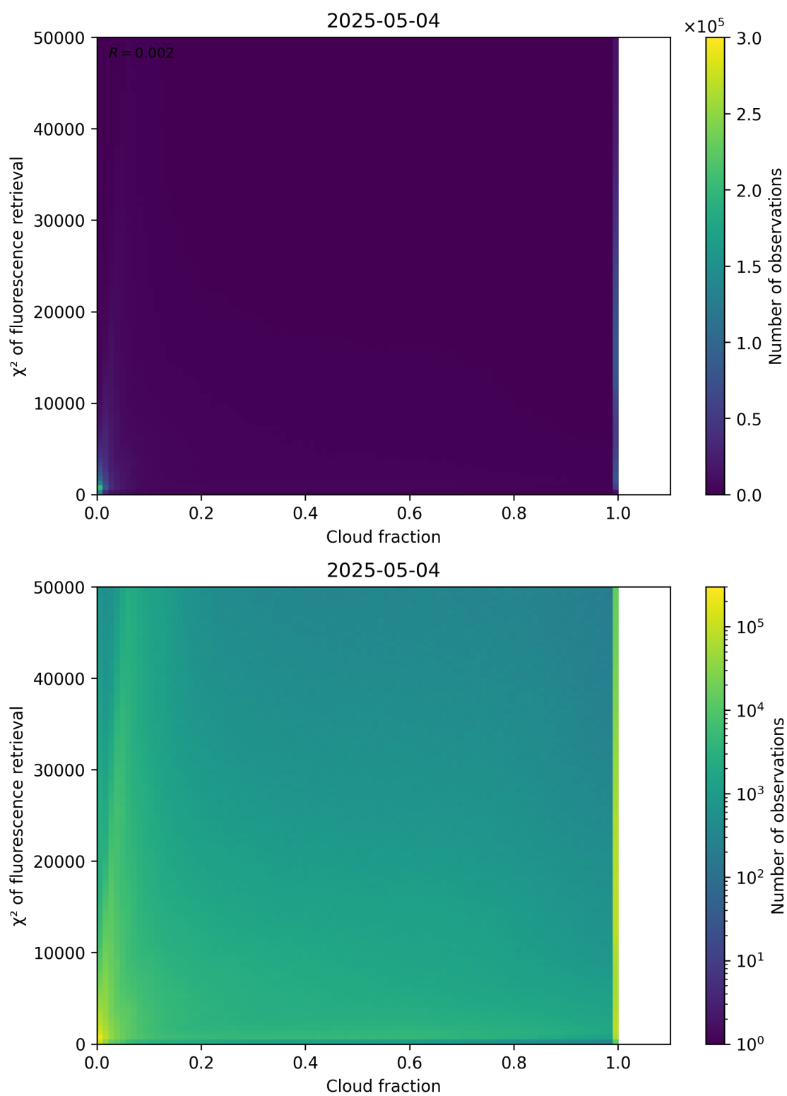
Figure 71: Scatter density plot of “Cloud fraction” against “ \chi^2 of fluorescence retrieval” for 2025-05-03 to 2025-05-05.
