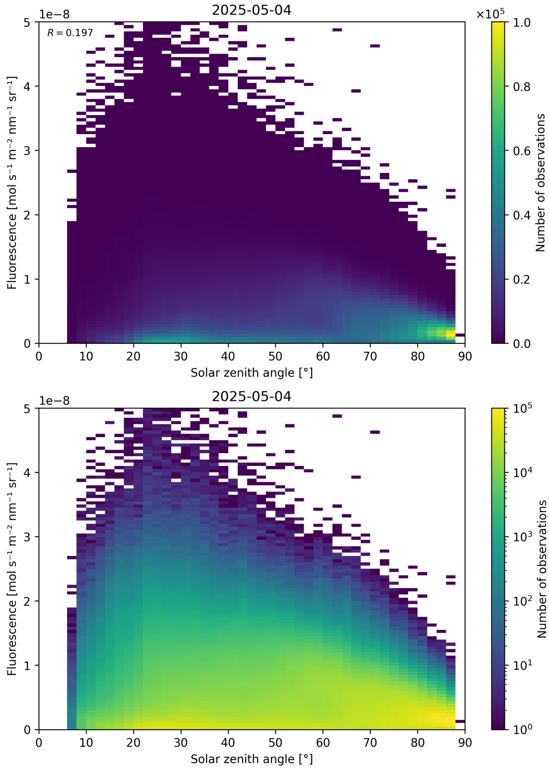
Figure 112: Scatter density plot of “Solar zenith angle” against “Fluorescence” for 2025-05-03 to 2025-05-05.
