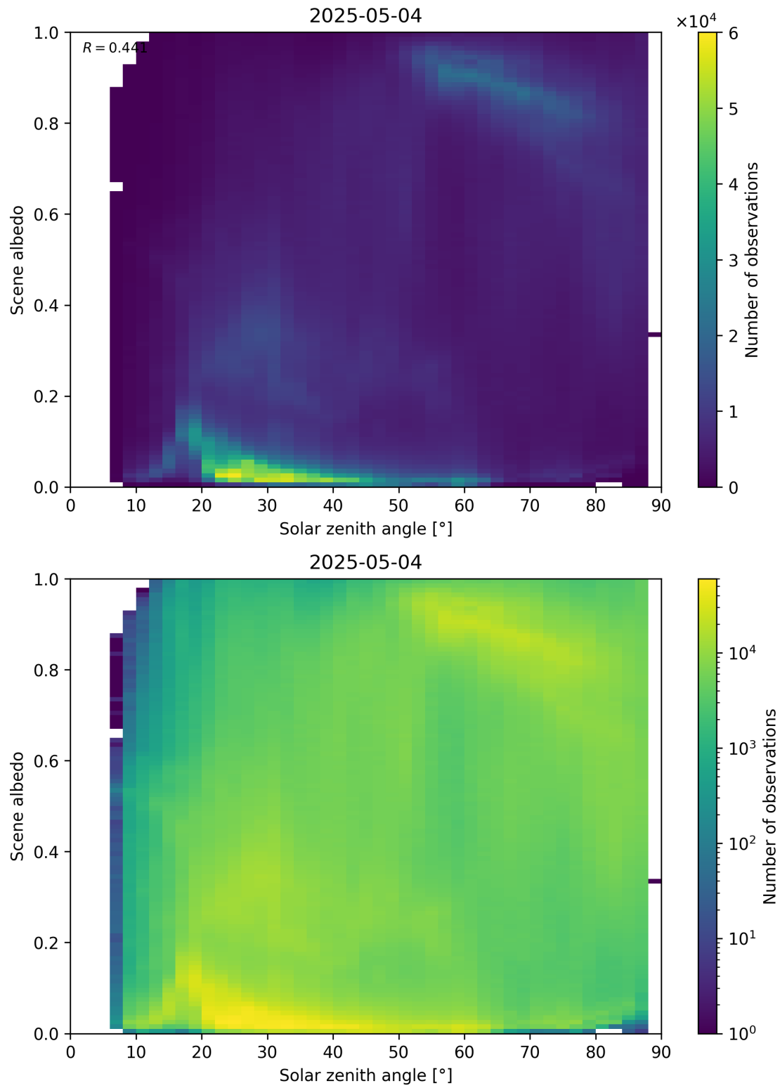
Figure 116: Scatter density plot of “Solar zenith angle” against “Scene albedo” for 2025-05-03 to 2025-05-05.
