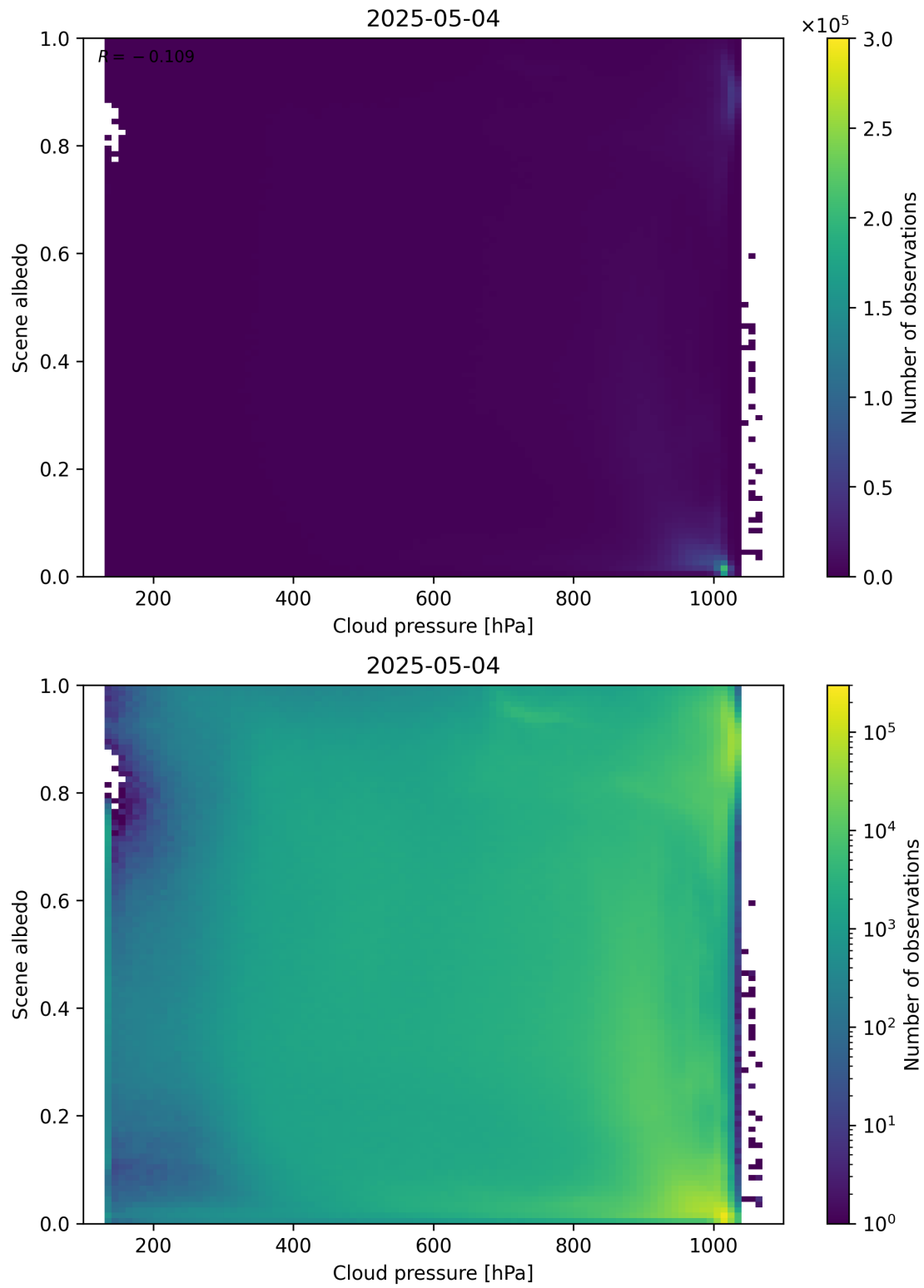
Figure 83: Scatter density plot of “Cloud pressure” against “Scene albedo” for 2025-05-03 to 2025-05-05.
