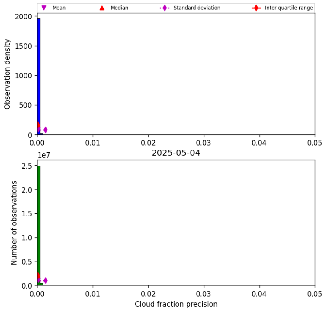
Figure 33: Histogram of “Cloud fraction precision” for 2025-05-03 to 2025-05-05
