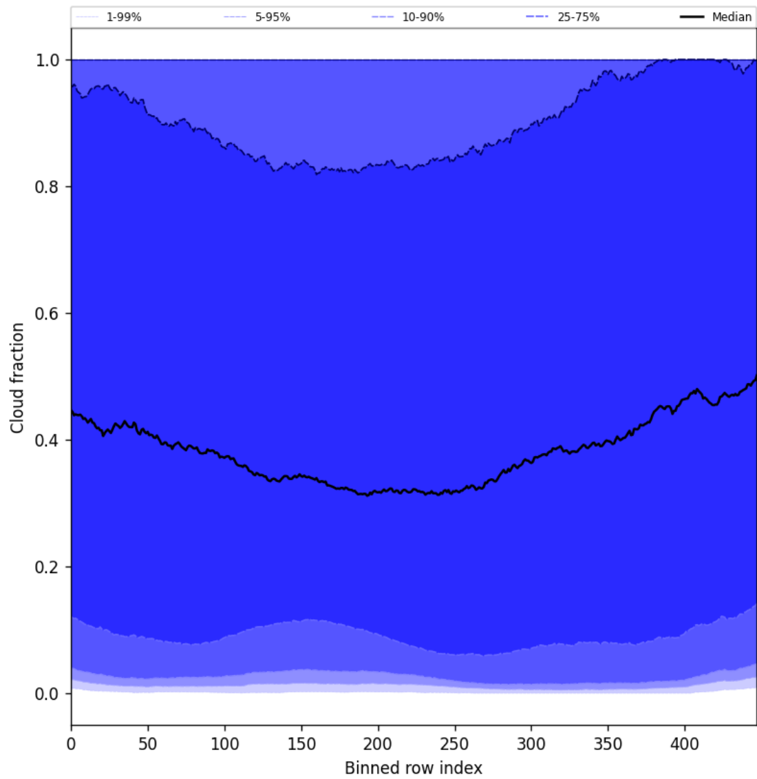
Figure 49: Along track statistics of “Cloud fraction” for 2025-05-03 to 2025-05-05
