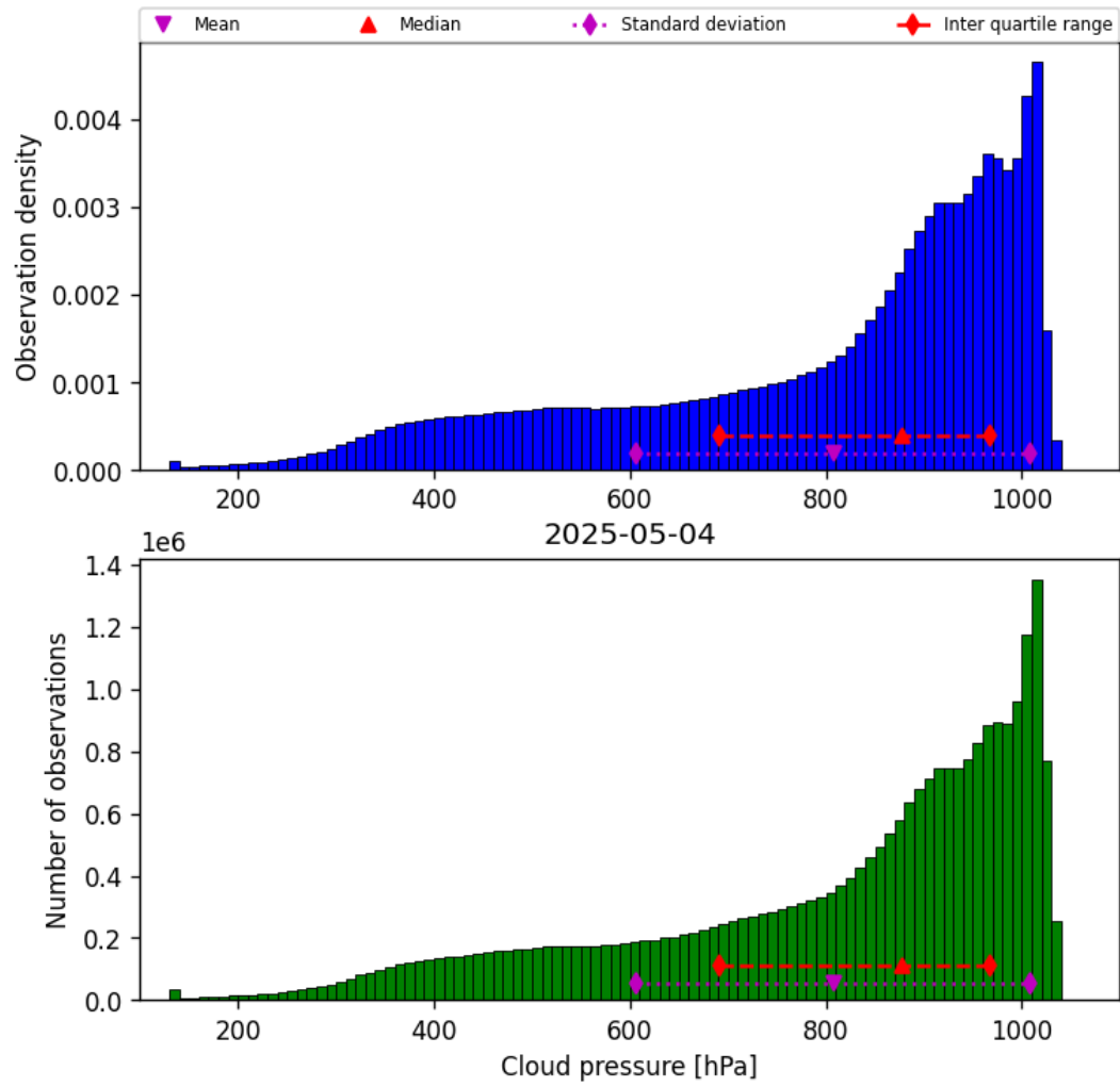
Figure 30: Histogram of “Cloud pressure” for 2025-05-03 to 2025-05-05
