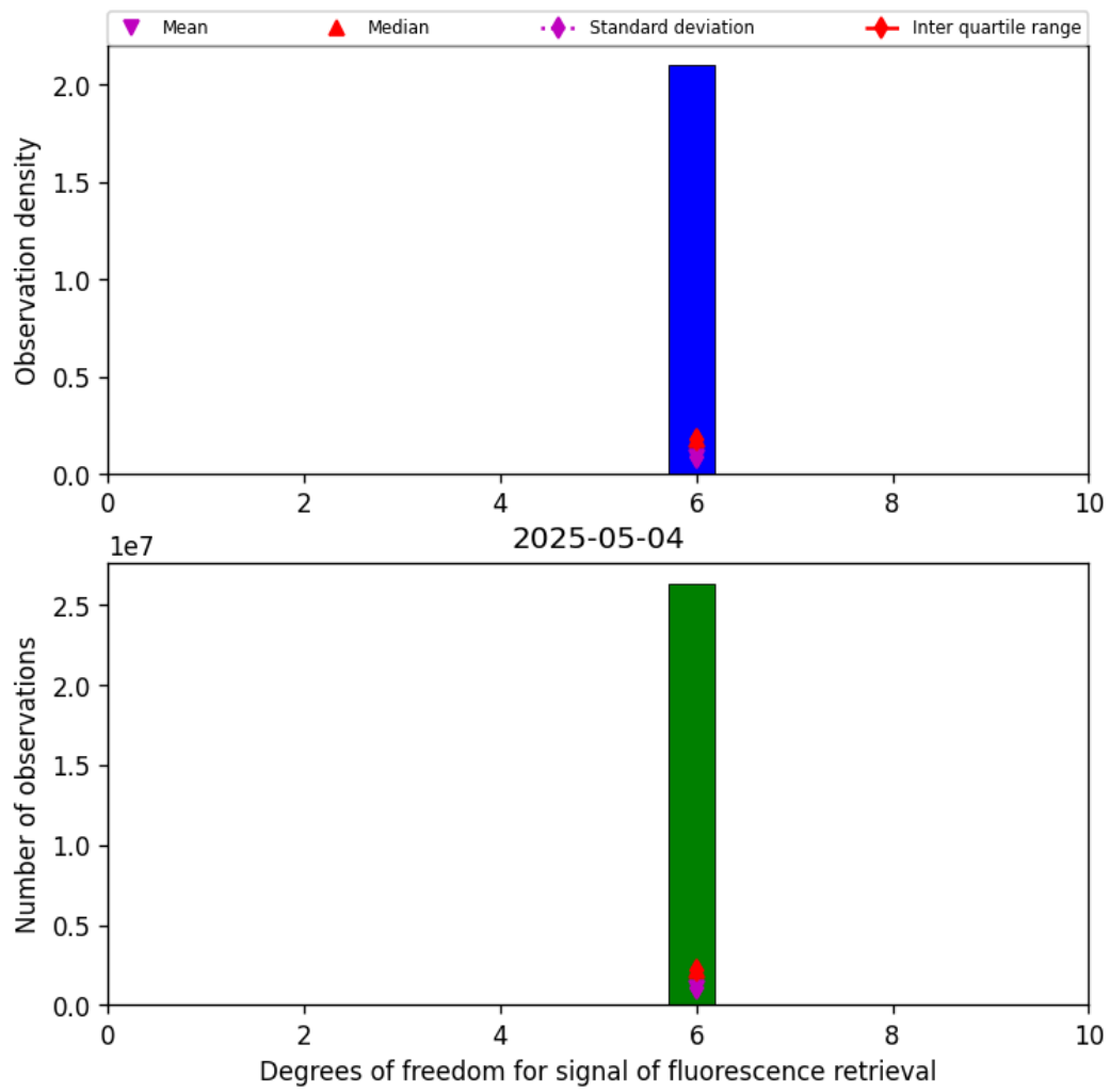
Figure 43: Histogram of “Degrees of freedom for signal of fluorescence retrieval” for 2025-05-03 to 2025-05-05
