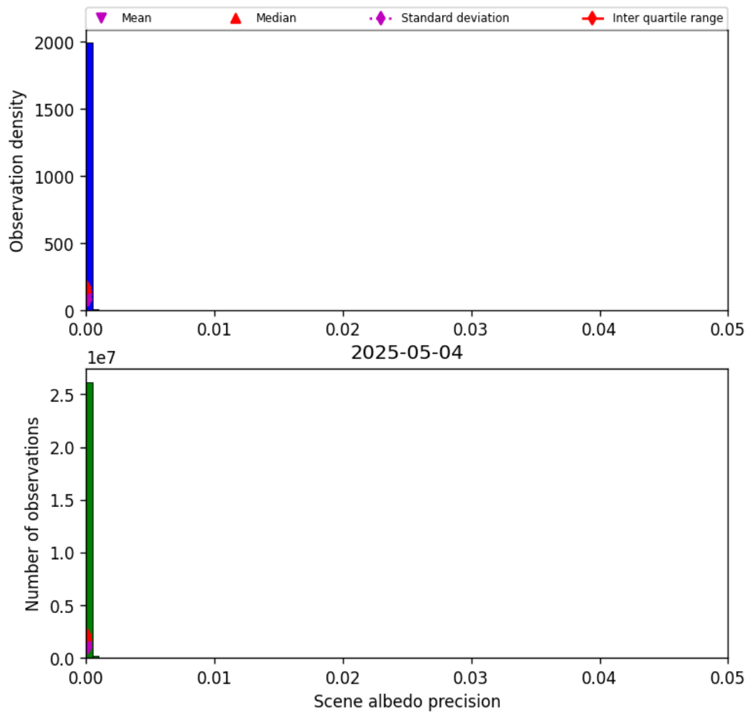
Figure 35: Histogram of “Scene albedo precision” for 2025-05-03 to 2025-05-05
