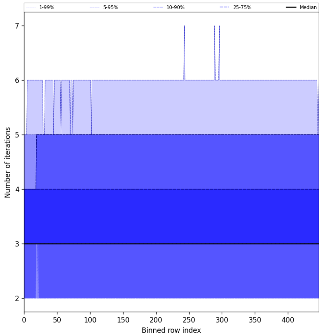
Figure 56: Along track statistics of “Number of iterations” for 2025-05-03 to 2025-05-05
