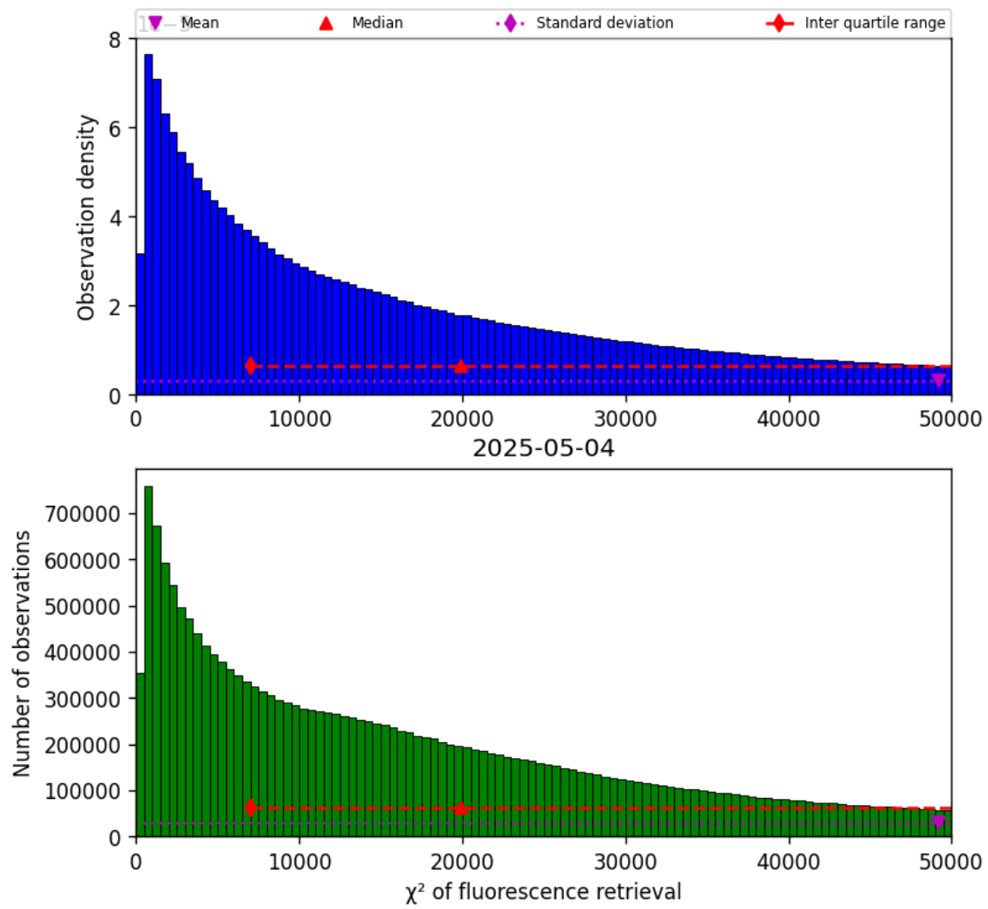
Figure 42: Histogram of “ \chi^2 of fluorescence retrieval” for 2025-05-03 to 2025-05-05
