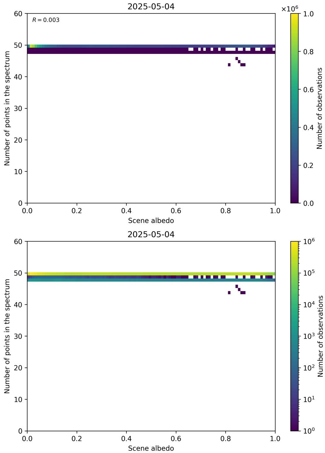
Figure 106: Scatter density plot of “Scene albedo” against “Number of points in the spectrum” for 2025-05-03 to 2025-05-05.
