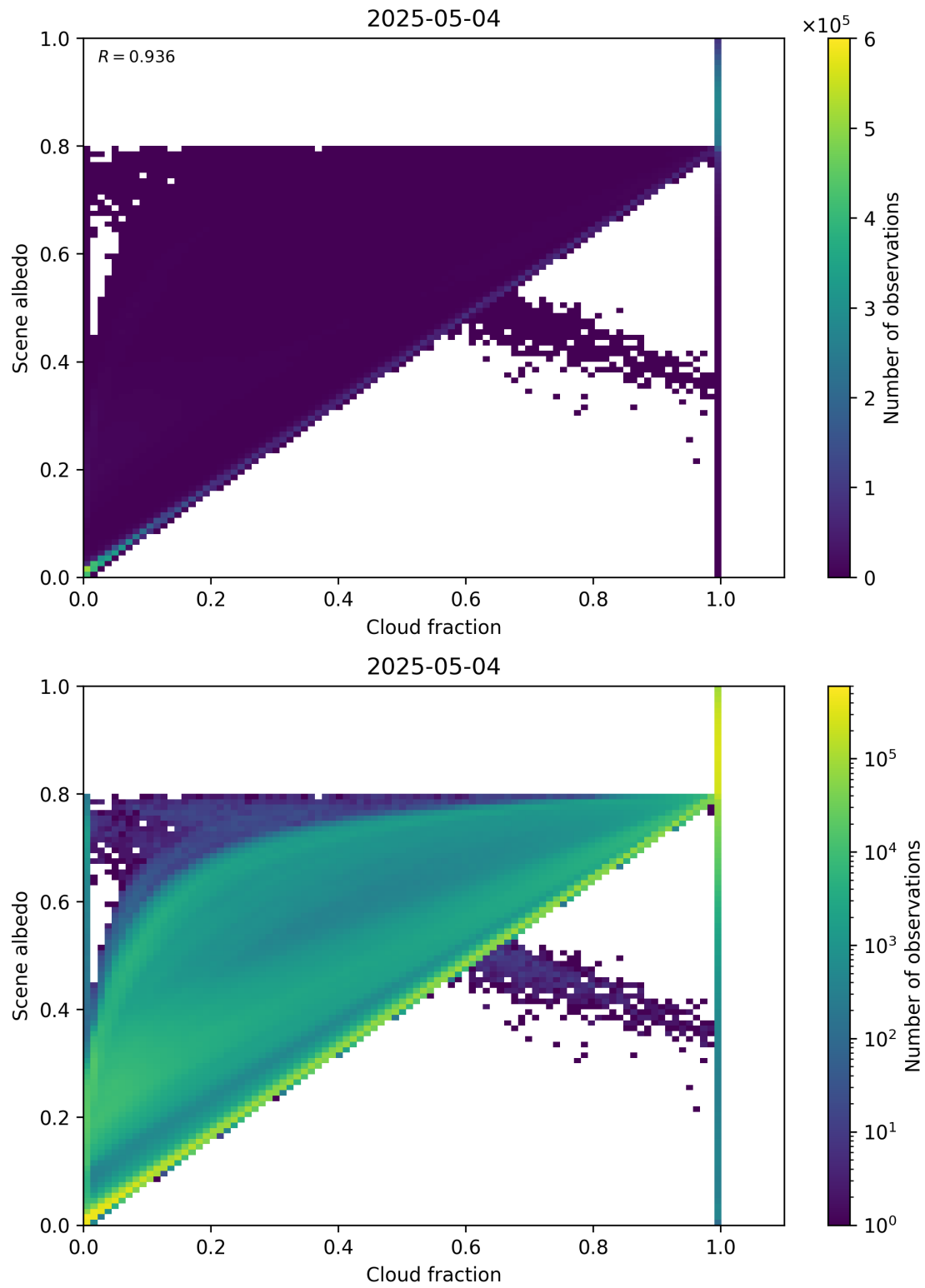
Figure 75: Scatter density plot of “Cloud fraction” against “Scene albedo” for 2025-05-03 to 2025-05-05.
