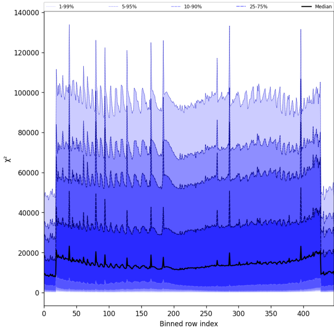
Figure 55: Along track statistics of “ \chi^2 ” for 2025-05-03 to 2025-05-05
