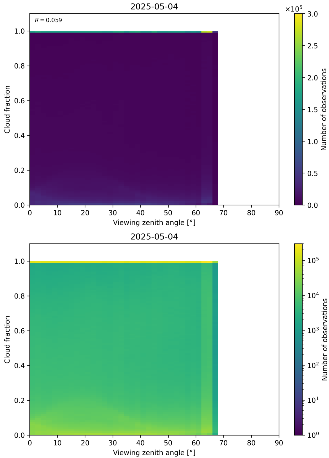
Figure 120: Scatter density plot of “Viewing zenith angle” against “Cloud fraction” for 2025-05-03 to 2025-05-05.
