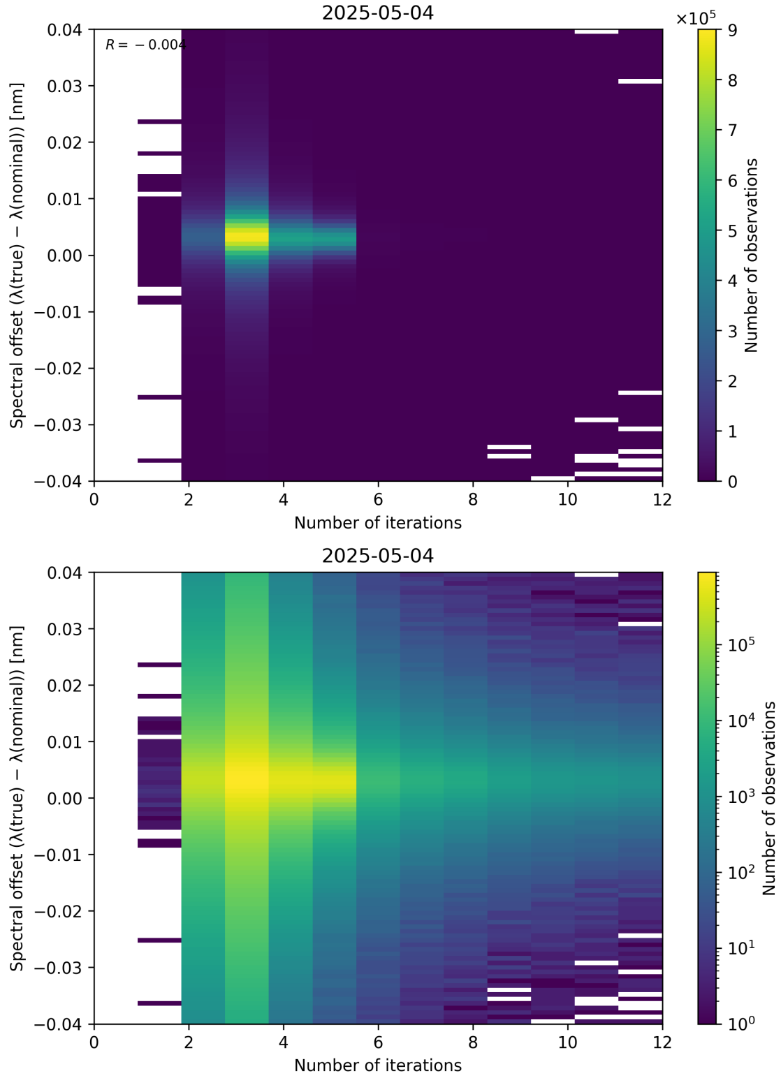
Figure 100: Scatter density plot of “Number of iterations” against “Spectral offset ( \lambda_{\text{true}} - \lambda_{\text{nominal}} )” for 2025-05-03 to 2025-05-05.
