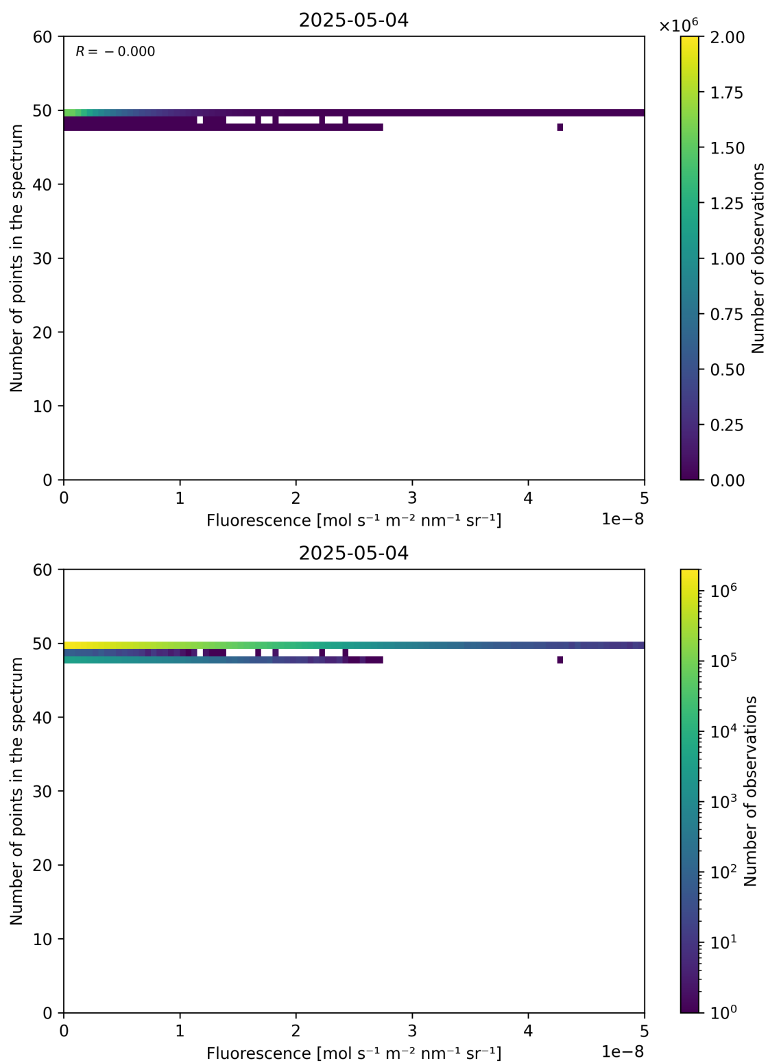
Figure 86: Scatter density plot of “Fluorescence” against “Number of points in the spectrum” for 2025-05-03 to 2025-05-05.
