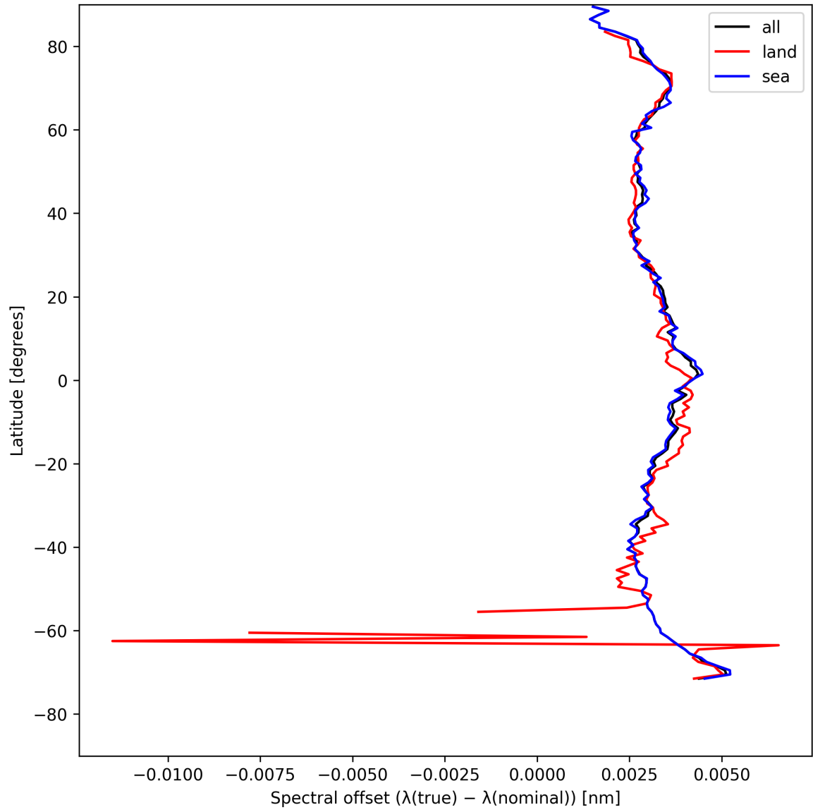
Figure 28: Zonal average of “Spectral offset ( \lambda_{\text{true}} - \lambda_{\text{nominal}} )” for 2025-05-03 to 2025-05-05.
