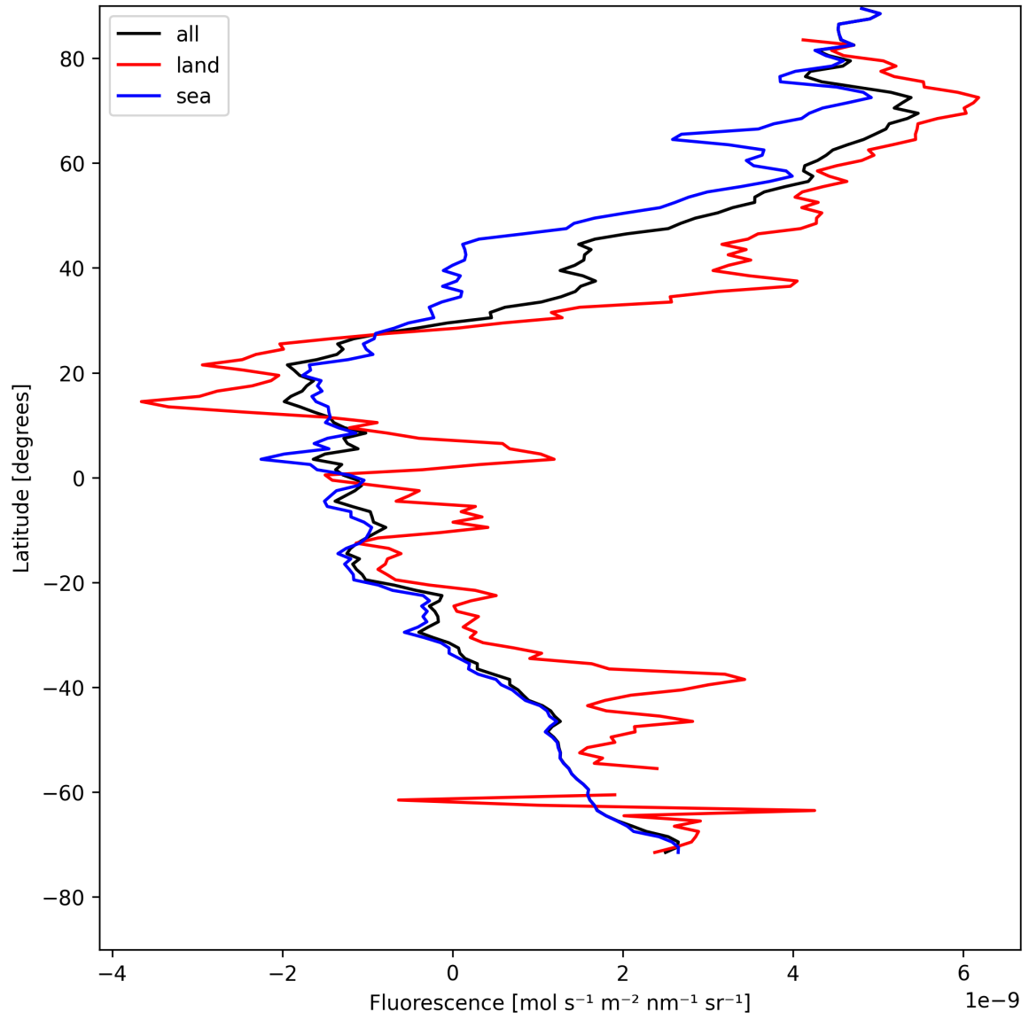
Figure 23: Zonal average of “Fluorescence” for 2025-05-03 to 2025-05-05.
