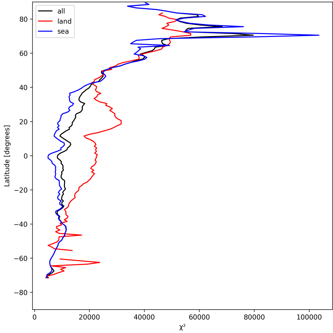
Figure 21: Zonal average of “ \chi^2 ” for 2025-05-03 to 2025-05-05.
