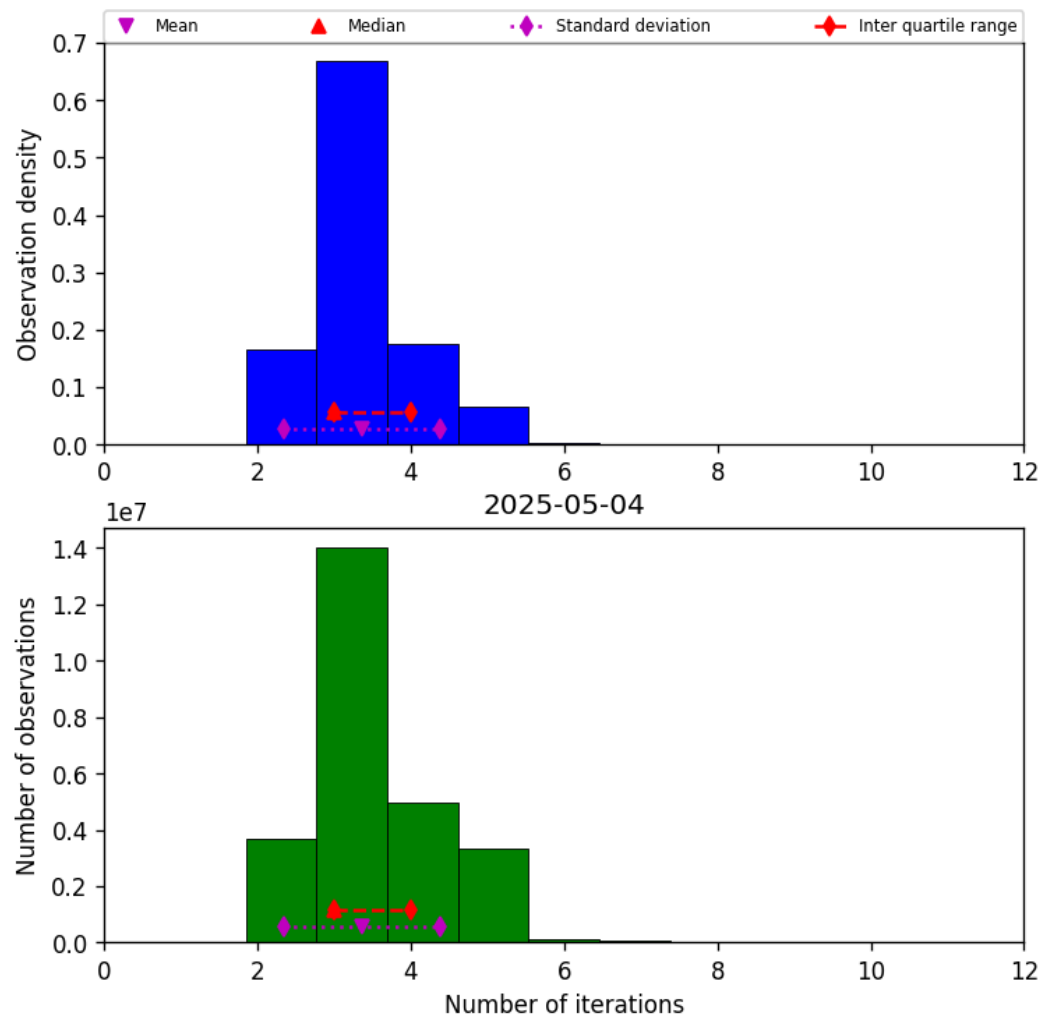
Figure 39: Histogram of “Number of iterations” for 2025-05-03 to 2025-05-05
