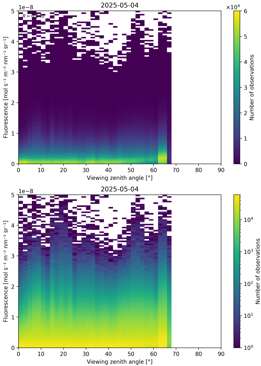
Figure 122: Scatter density plot of “Viewing zenith angle” against “Fluorescence” for 2025-05-03 to 2025-05-05.
