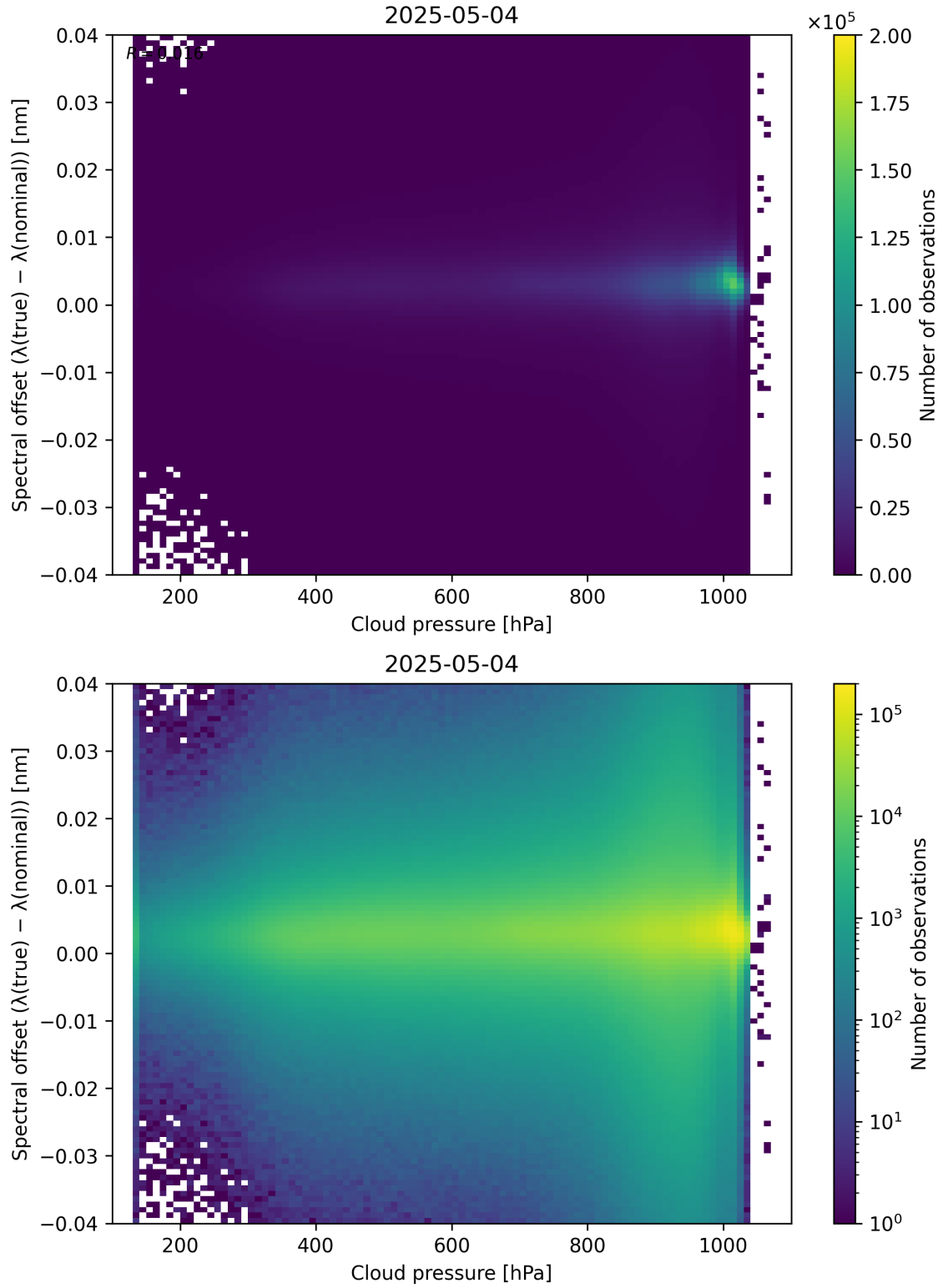
Figure 84: Scatter density plot of “Cloud pressure” against “Spectral offset ( \lambda_{\text{true}} - \lambda_{\text{nominal}} )” for 2025-05-03 to 2025-05-05.
