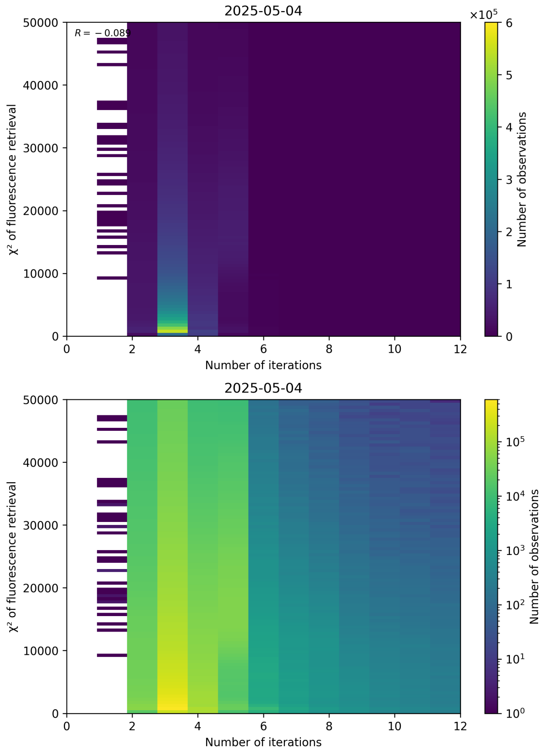
Figure 97: Scatter density plot of “Number of iterations” against “ \chi^2 of fluorescence retrieval” for 2025-05-03 to 2025-05-05.
