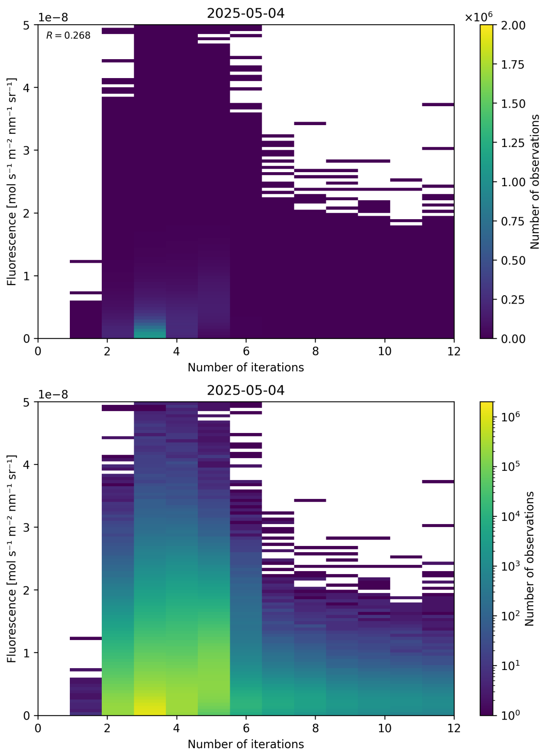
Figure 98: Scatter density plot of “Number of iterations” against “Fluorescence” for 2025-05-03 to 2025-05-05.
