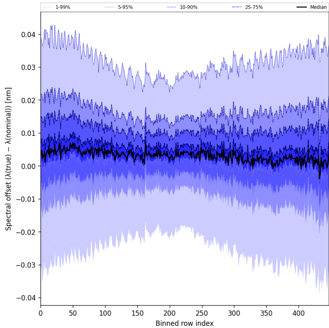
Figure 62: Along track statistics of “Spectral offset ( \lambda_{\text{true}} - \lambda_{\text{nominal}} )” for 2025-05-03 to 2025-05-05
