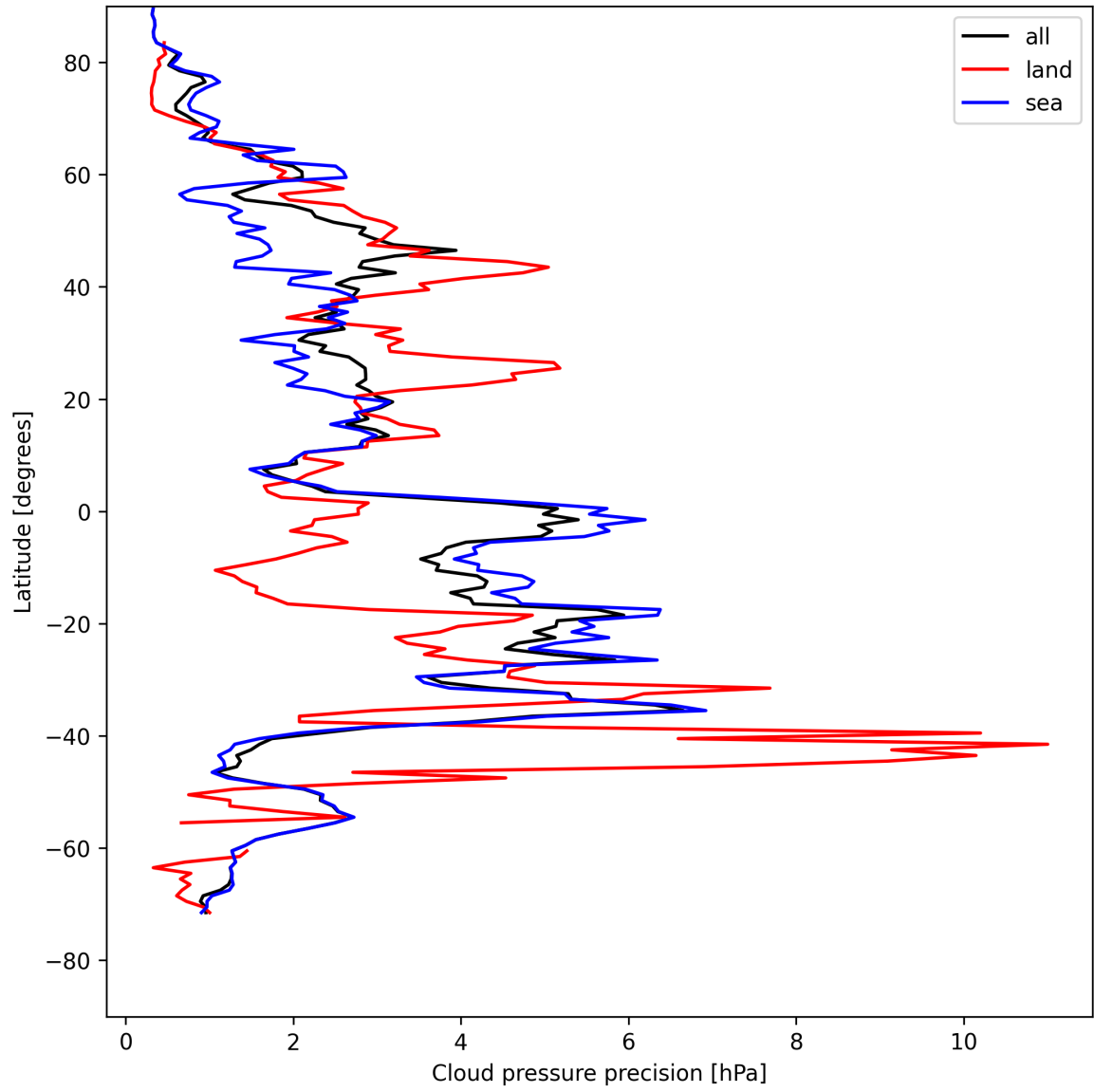
Figure 14: Zonal average of “Cloud pressure precision” for 2025-05-03 to 2025-05-05.
