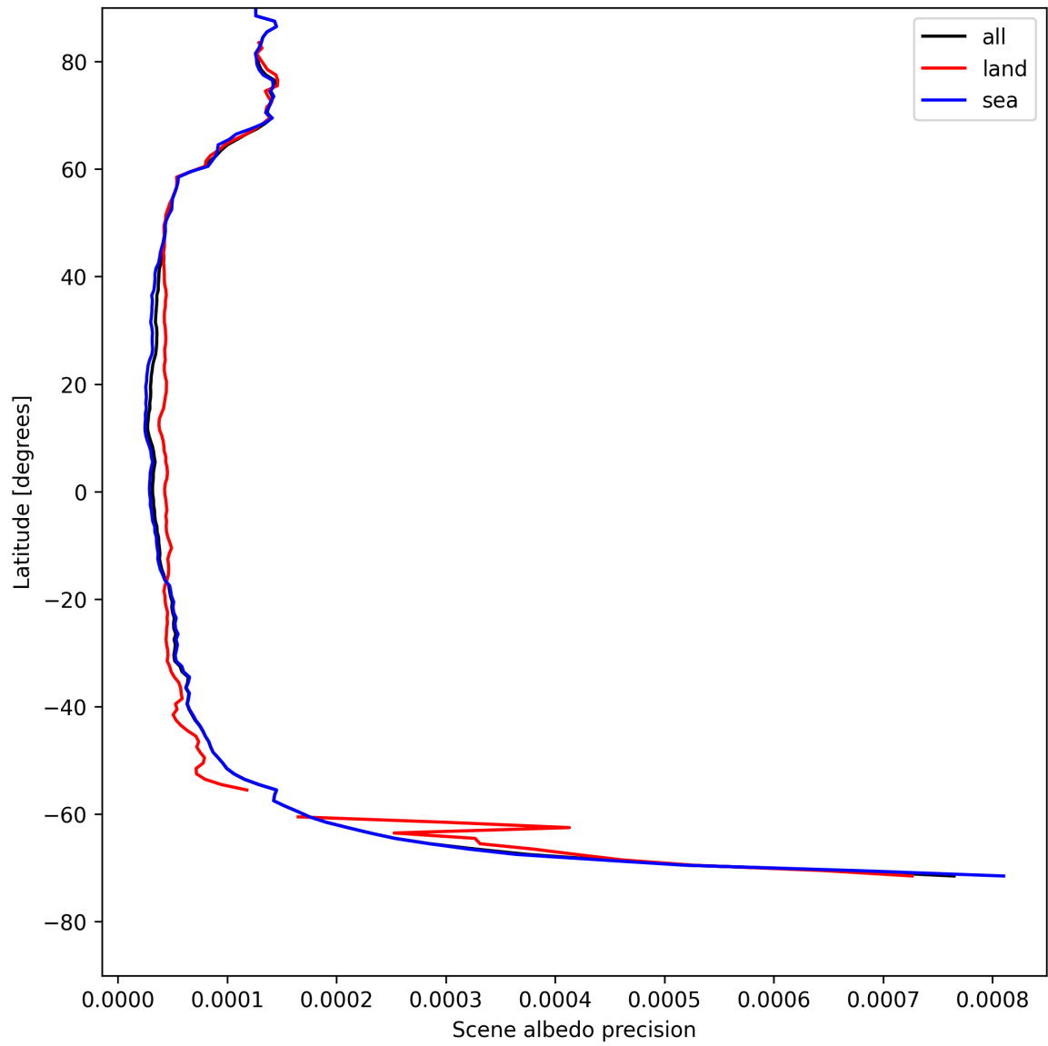
Figure 18: Zonal average of “Scene albedo precision” for 2025-05-03 to 2025-05-05.
