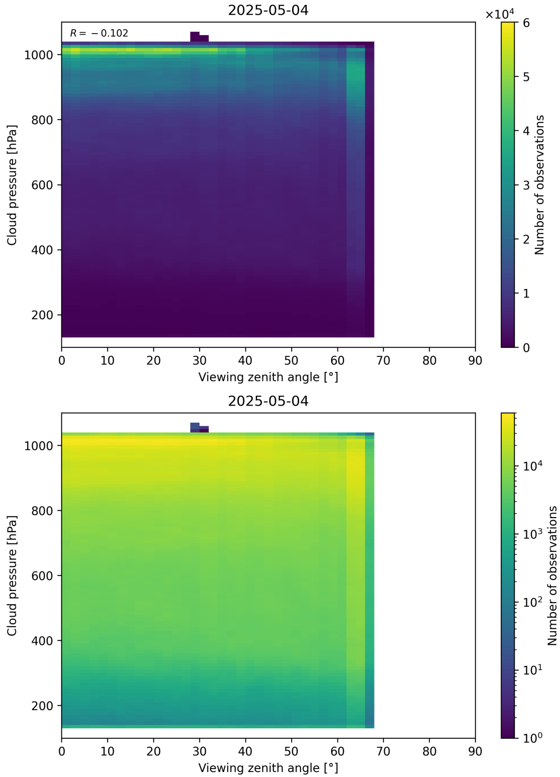
Figure 121: Scatter density plot of “Viewing zenith angle” against “Cloud pressure” for 2025-05-03 to 2025-05-05.
