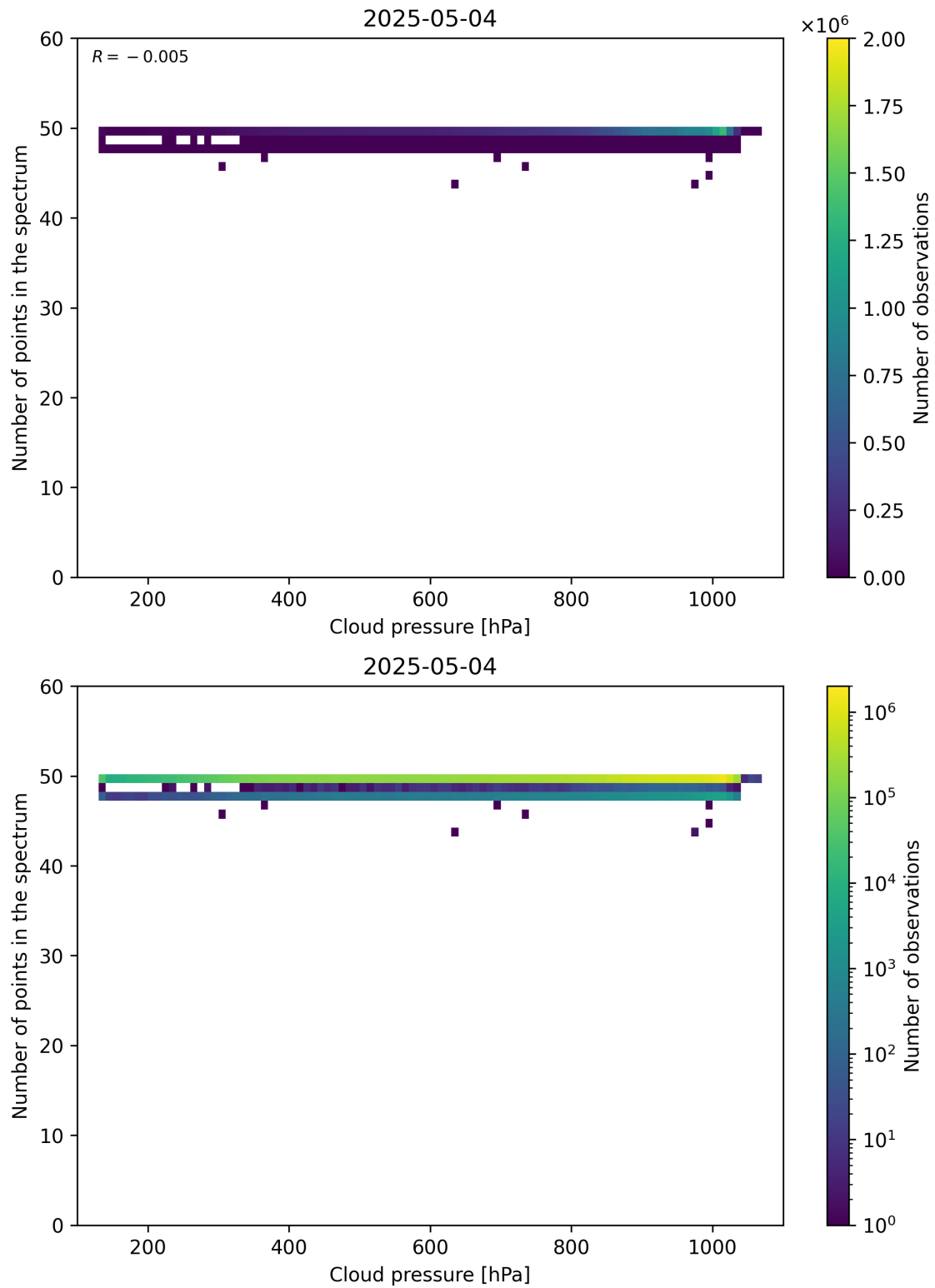
Figure 82: Scatter density plot of “Cloud pressure” against “Number of points in the spectrum” for 2025-05-03 to 2025-05-05.
