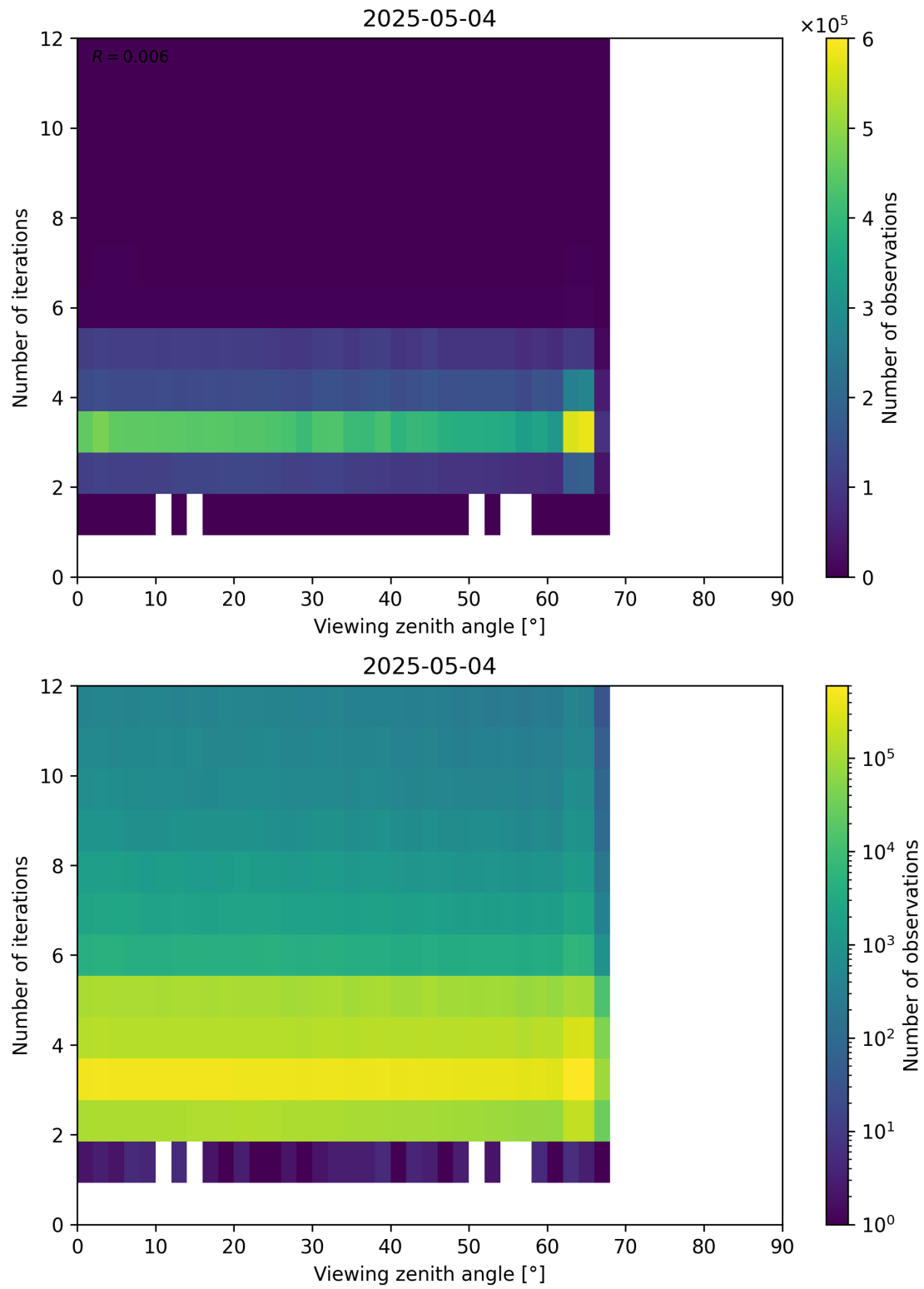
Figure 124: Scatter density plot of “Viewing zenith angle” against “Number of iterations” for 2025-05-03 to 2025-05-05.
