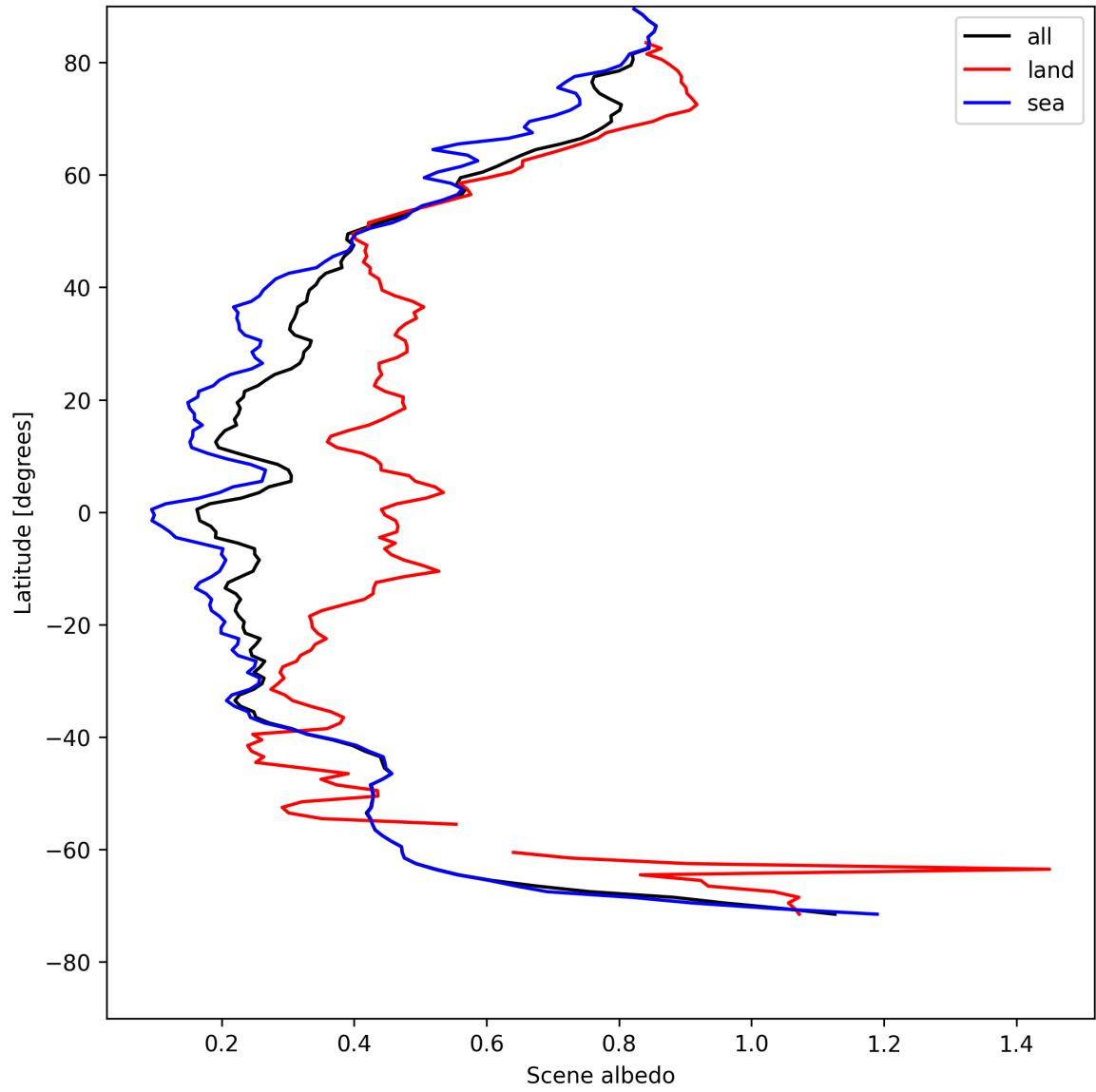
Figure 17: Zonal average of “Scene albedo” for 2025-05-03 to 2025-05-05.
