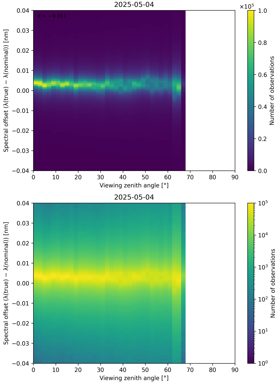
Figure 128: Scatter density plot of “Viewing zenith angle” against “Spectral offset ( \lambda_{\text{true}} - \lambda_{\text{nominal}} )” for 2025-05-03 to 2025-05-05.
