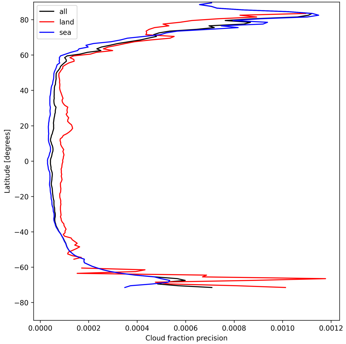
Figure 16: Zonal average of “Cloud fraction precision” for 2025-05-03 to 2025-05-05.
