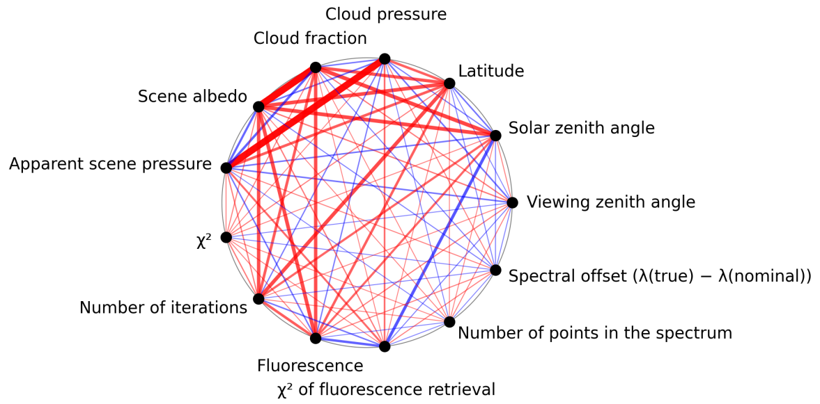
Figure 1: Map of correlation graph for 2025-05-03 to 2025-05-05.
