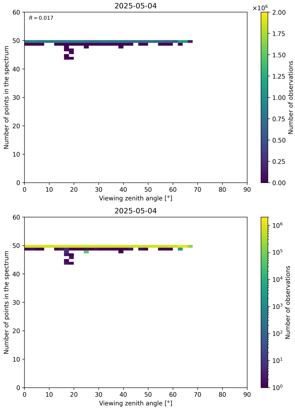
Figure 125: Scatter density plot of “Viewing zenith angle” against “Number of points in the spectrum” for 2025-05-03 to 2025-05-05.
