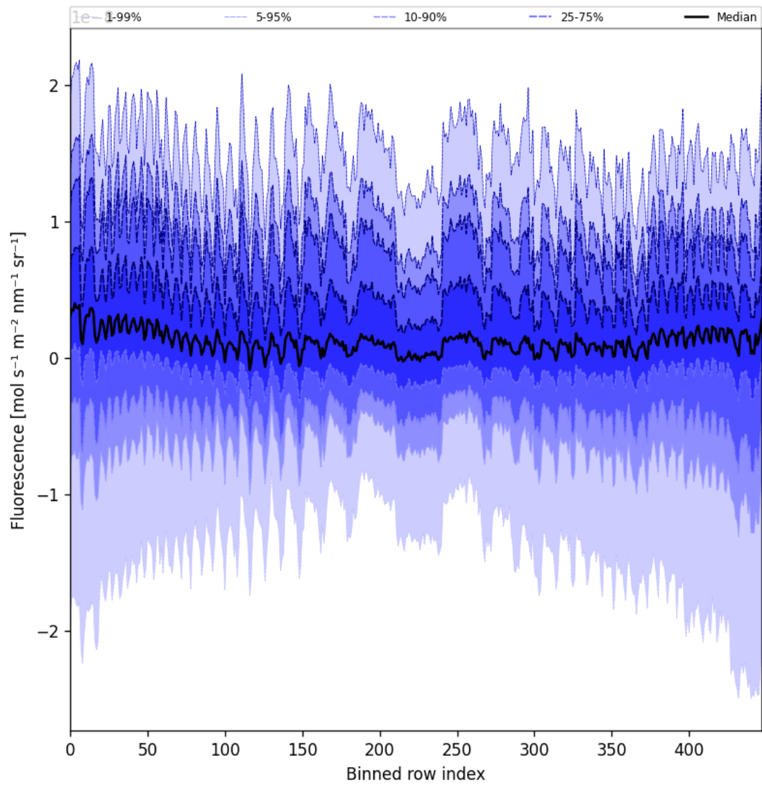
Figure 57: Along track statistics of “Fluorescence” for 2025-05-03 to 2025-05-05
