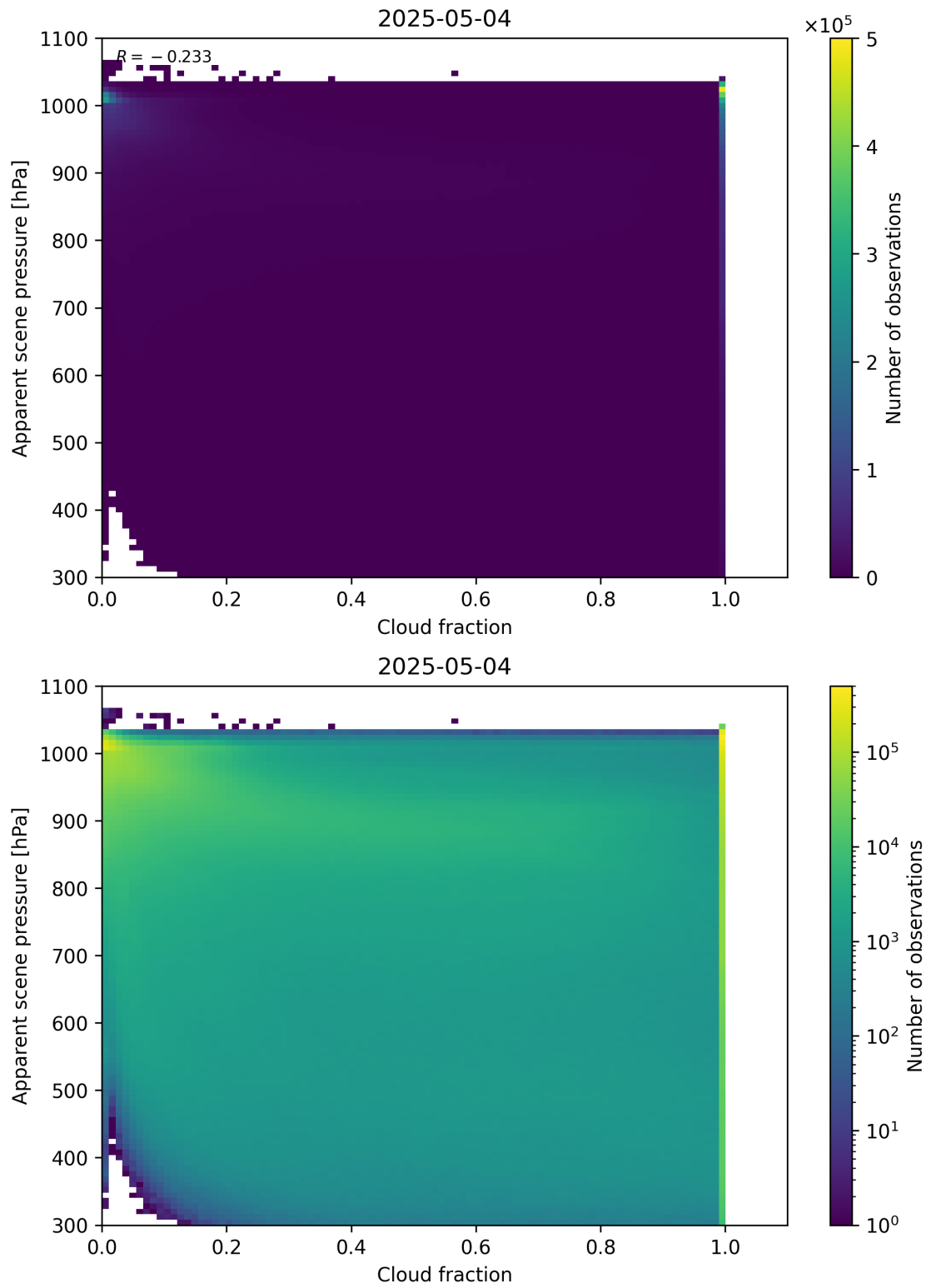
Figure 70: Scatter density plot of “Cloud fraction” against “Apparent scene pressure” for 2025-05-03 to 2025-05-05.
