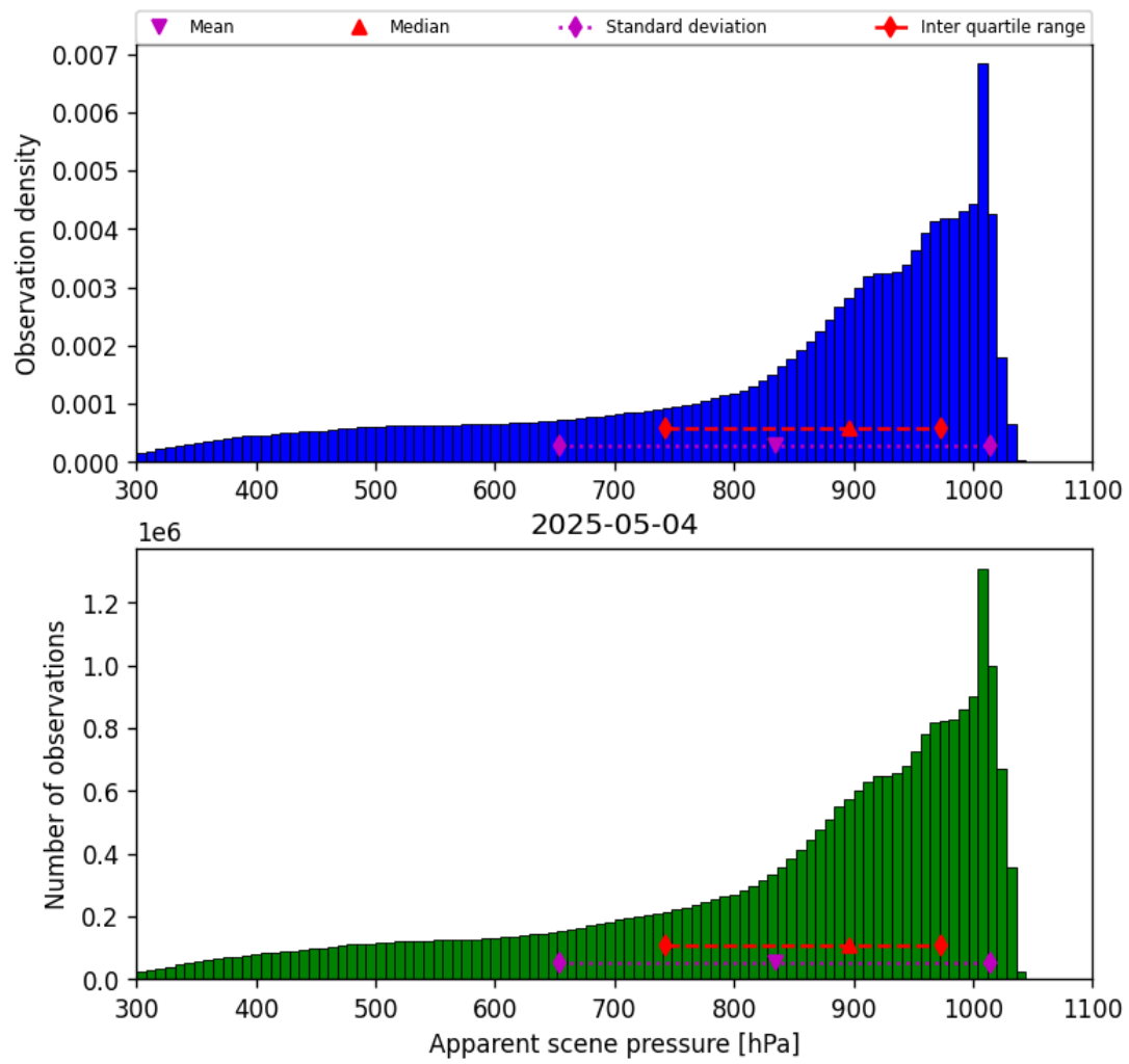
Figure 36: Histogram of “Apparent scene pressure” for 2025-05-03 to 2025-05-05
