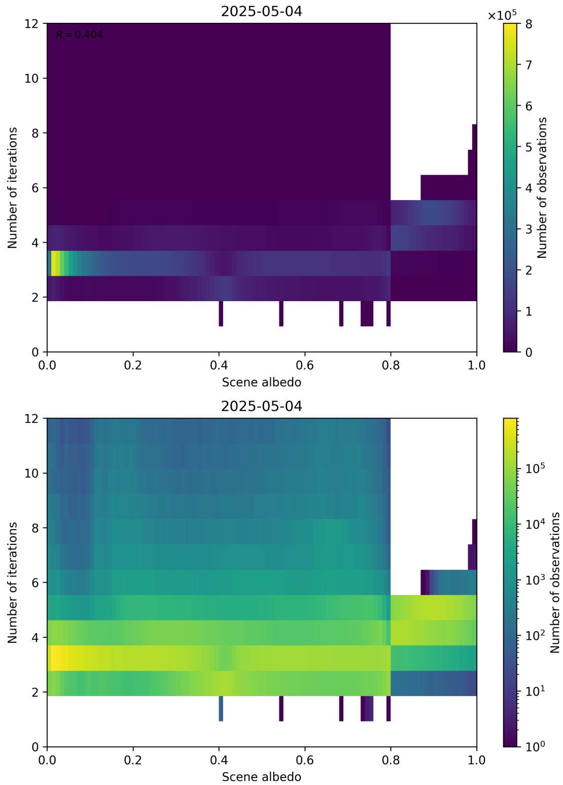
Figure 105: Scatter density plot of “Scene albedo” against “Number of iterations” for 2025-05-03 to 2025-05-05.
