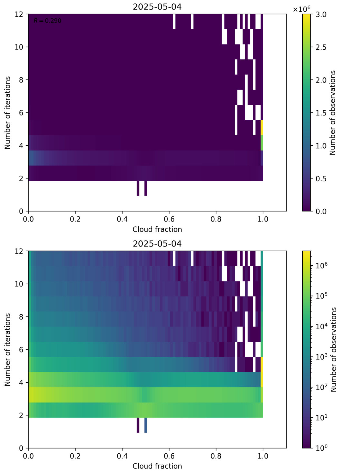
Figure 73: Scatter density plot of “Cloud fraction” against “Number of iterations” for 2025-05-03 to 2025-05-05.
