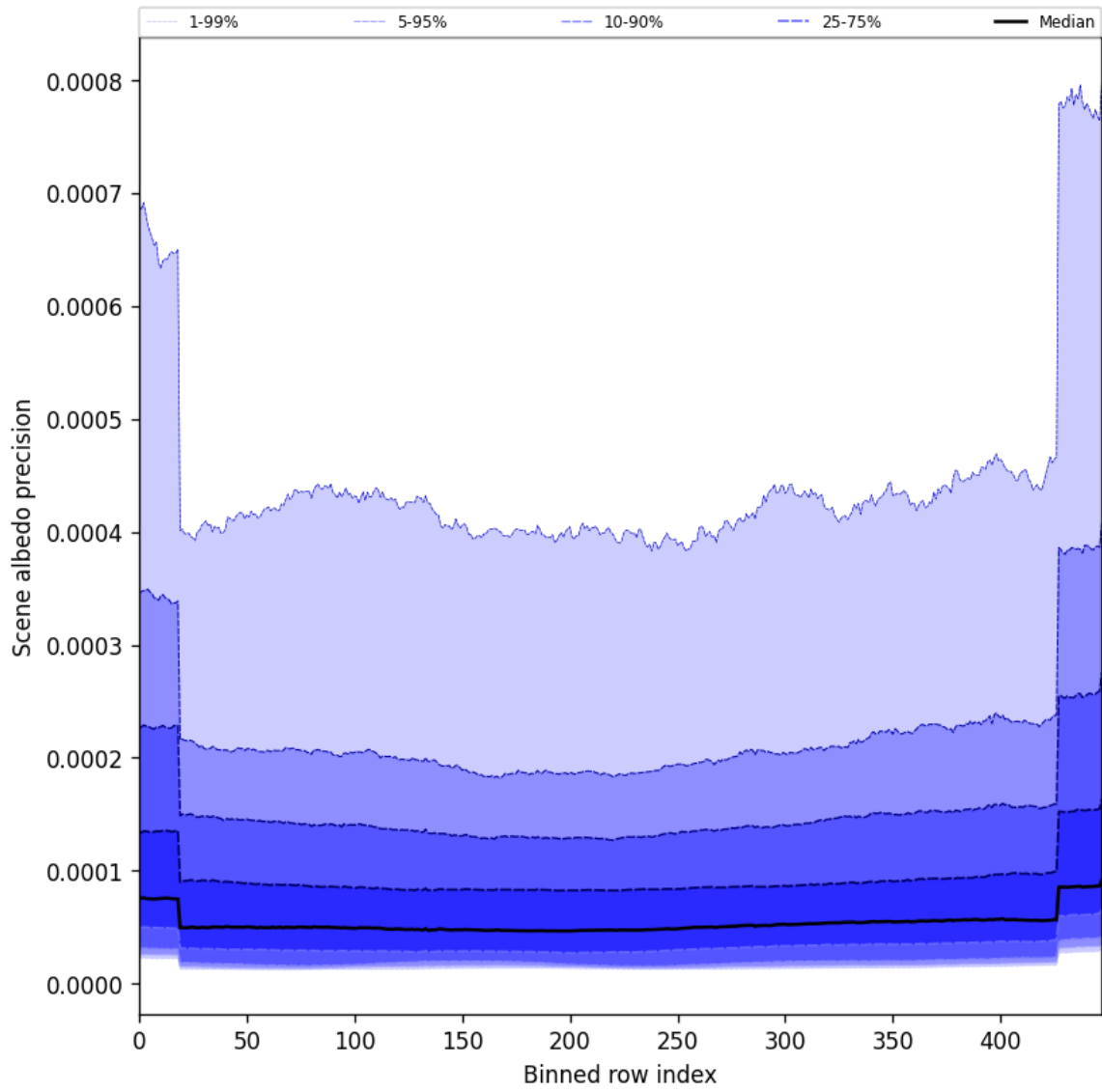
Figure 52: Along track statistics of “Scene albedo precision” for 2025-05-03 to 2025-05-05
