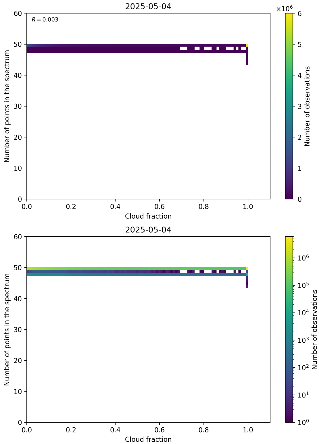
Figure 74: Scatter density plot of “Cloud fraction” against “Number of points in the spectrum” for 2025-05-03 to 2025-05-05.
