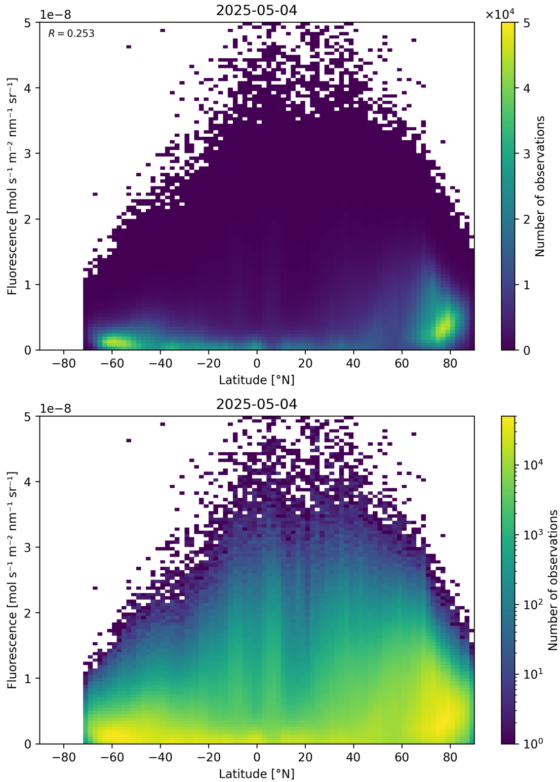
Figure 92: Scatter density plot of “Latitude” against “Fluorescence” for 2025-05-03 to 2025-05-05.
