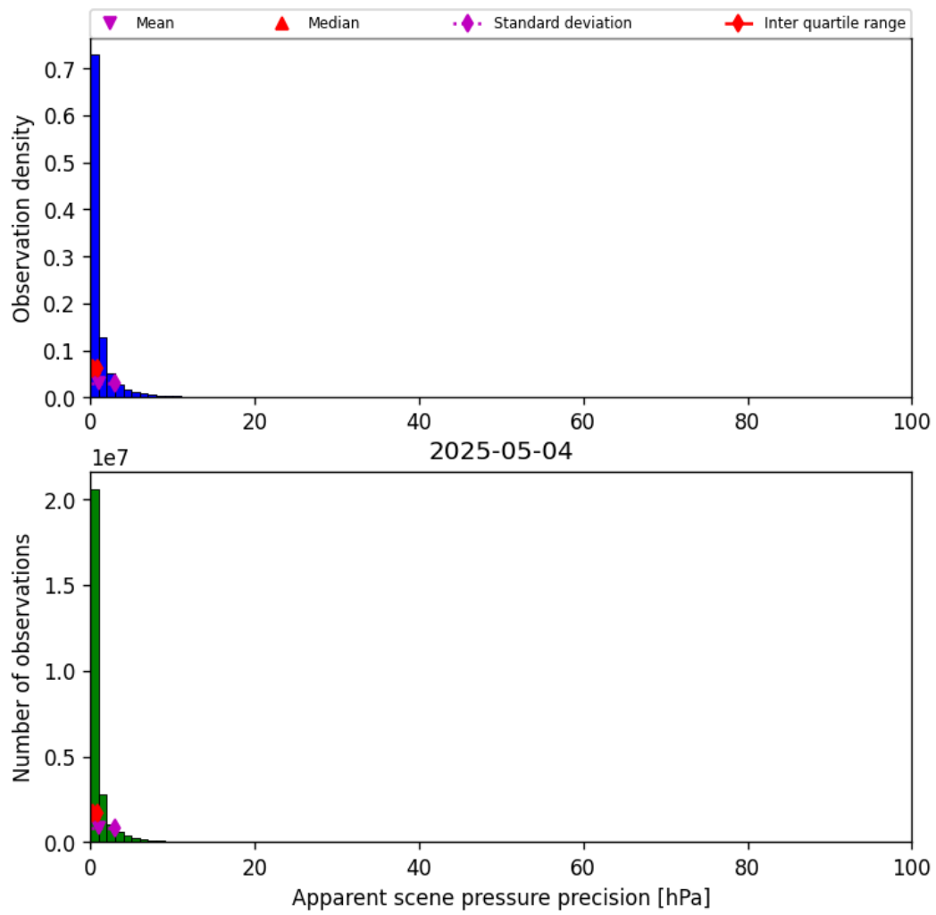
Figure 37: Histogram of “Apparent scene pressure precision” for 2025-05-03 to 2025-05-05
