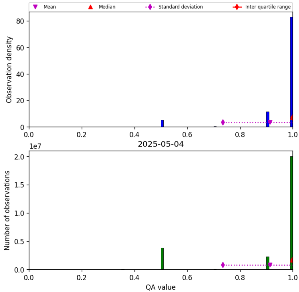
Figure 29: Histogram of “QA value” for 2025-05-03 to 2025-05-05
