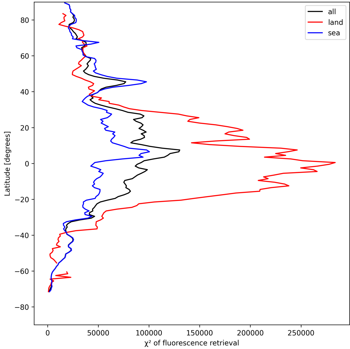
Figure 25: Zonal average of “ \chi^2 of fluorescence retrieval” for 2025-05-03 to 2025-05-05.
