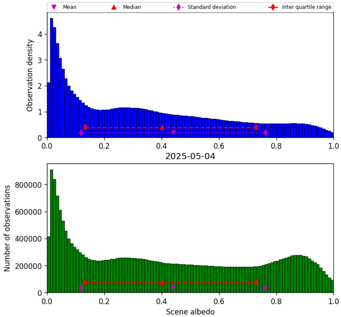
Figure 34: Histogram of “Scene albedo” for 2025-05-03 to 2025-05-05
