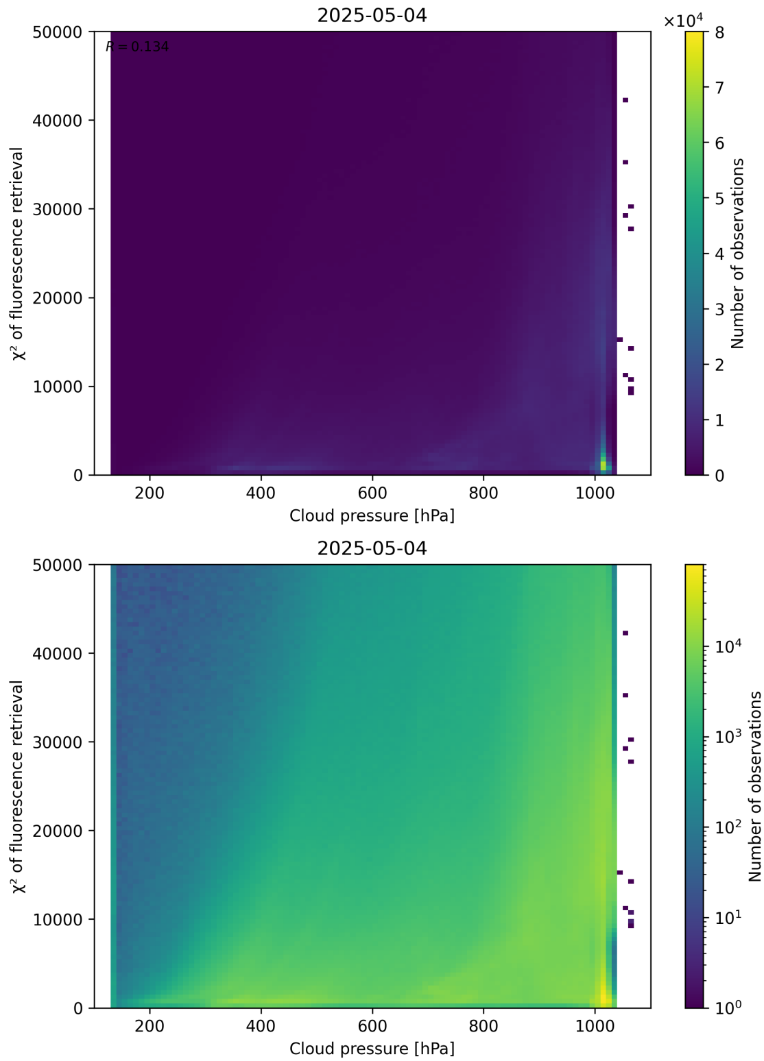
Figure 78: Scatter density plot of “Cloud pressure” against “ \chi^2 of fluorescence retrieval” for 2025-05-03 to 2025-05-05.
