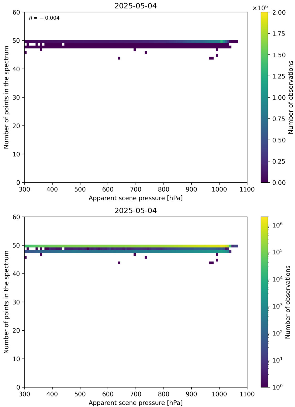
Figure 66: Scatter density plot of “Apparent scene pressure” against “Number of points in the spectrum” for 2025-05-03 to 2025-05-05.
