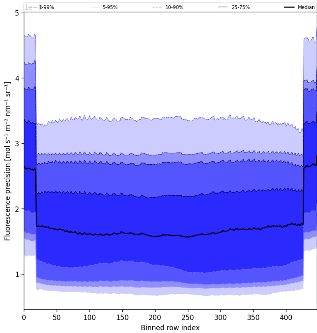
Figure 58: Along track statistics of “Fluorescence precision” for 2025-05-03 to 2025-05-05
