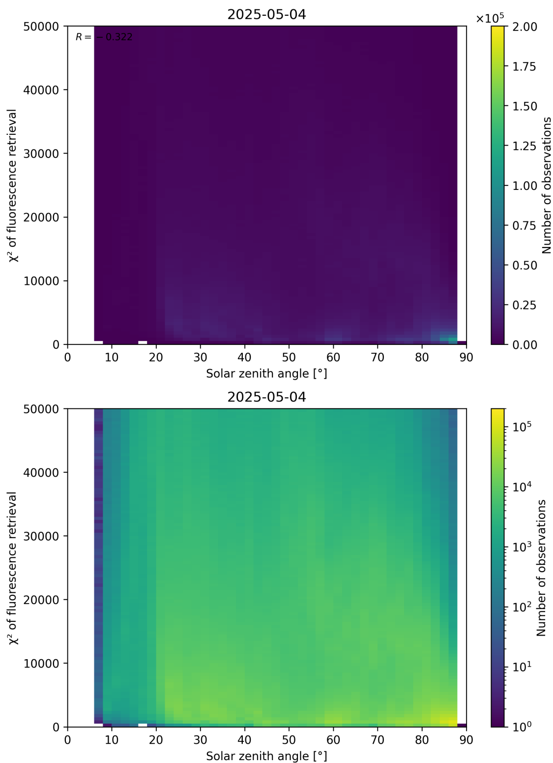
Figure 109: Scatter density plot of “Solar zenith angle” against “ \chi^2 of fluorescence retrieval” for 2025-05-03 to 2025-05-05.
