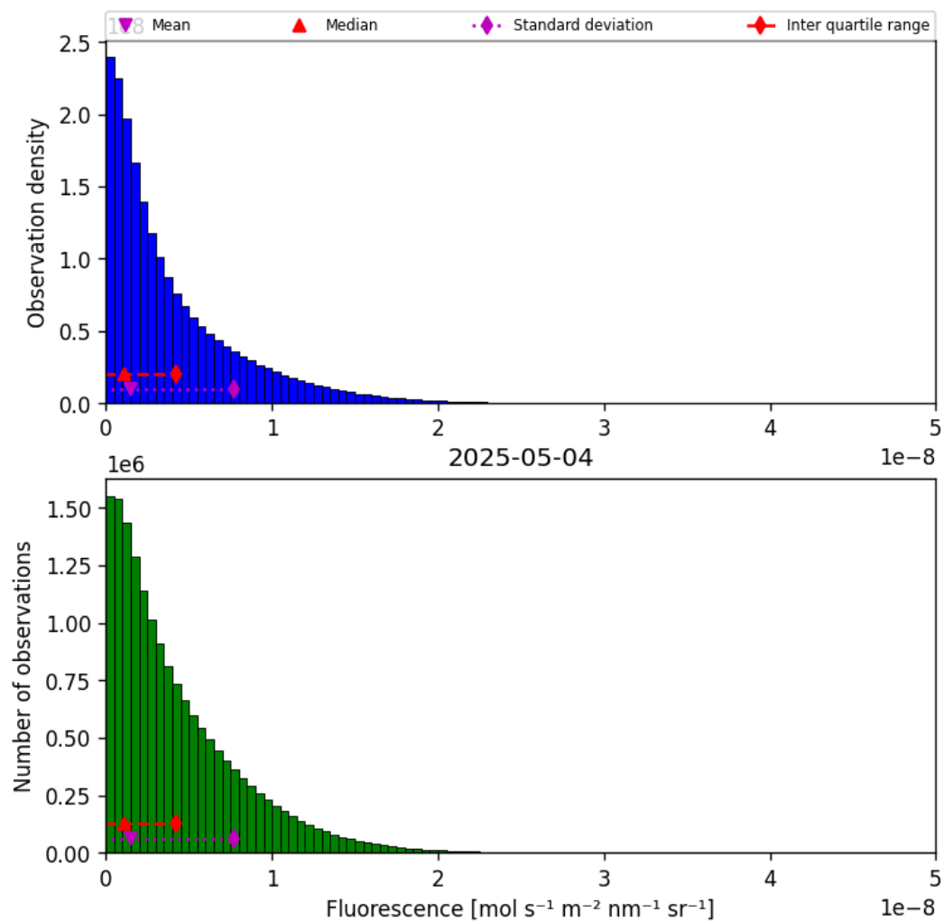
Figure 40: Histogram of “Fluorescence” for 2025-05-03 to 2025-05-05
