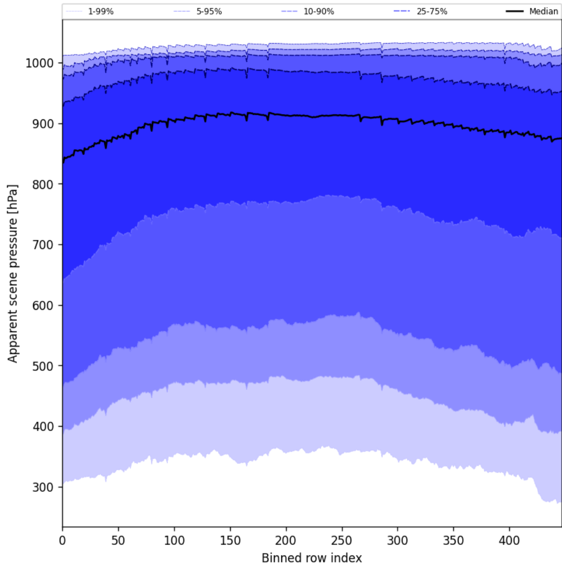
Figure 53: Along track statistics of “Apparent scene pressure” for 2025-05-03 to 2025-05-05
