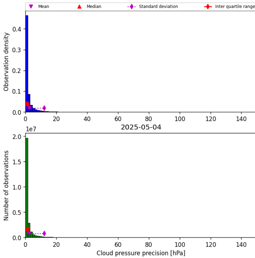
Figure 31: Histogram of “Cloud pressure precision” for 2025-05-03 to 2025-05-05
