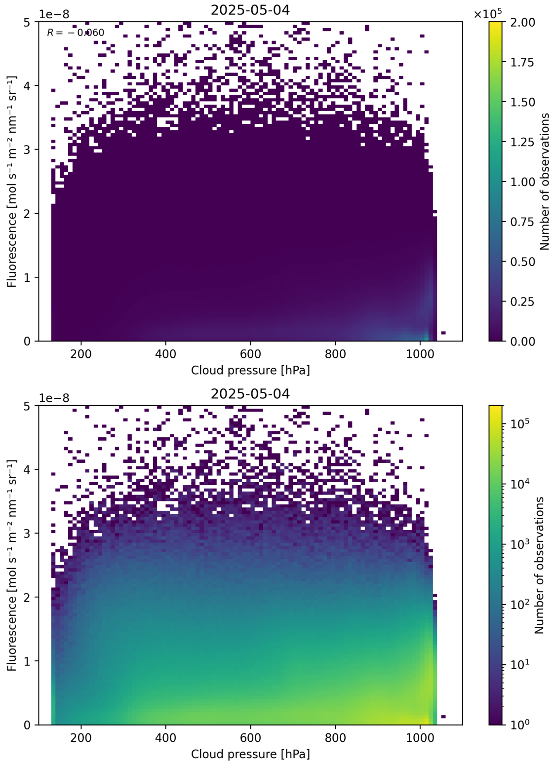
Figure 80: Scatter density plot of “Cloud pressure” against “Fluorescence” for 2025-05-03 to 2025-05-05.
