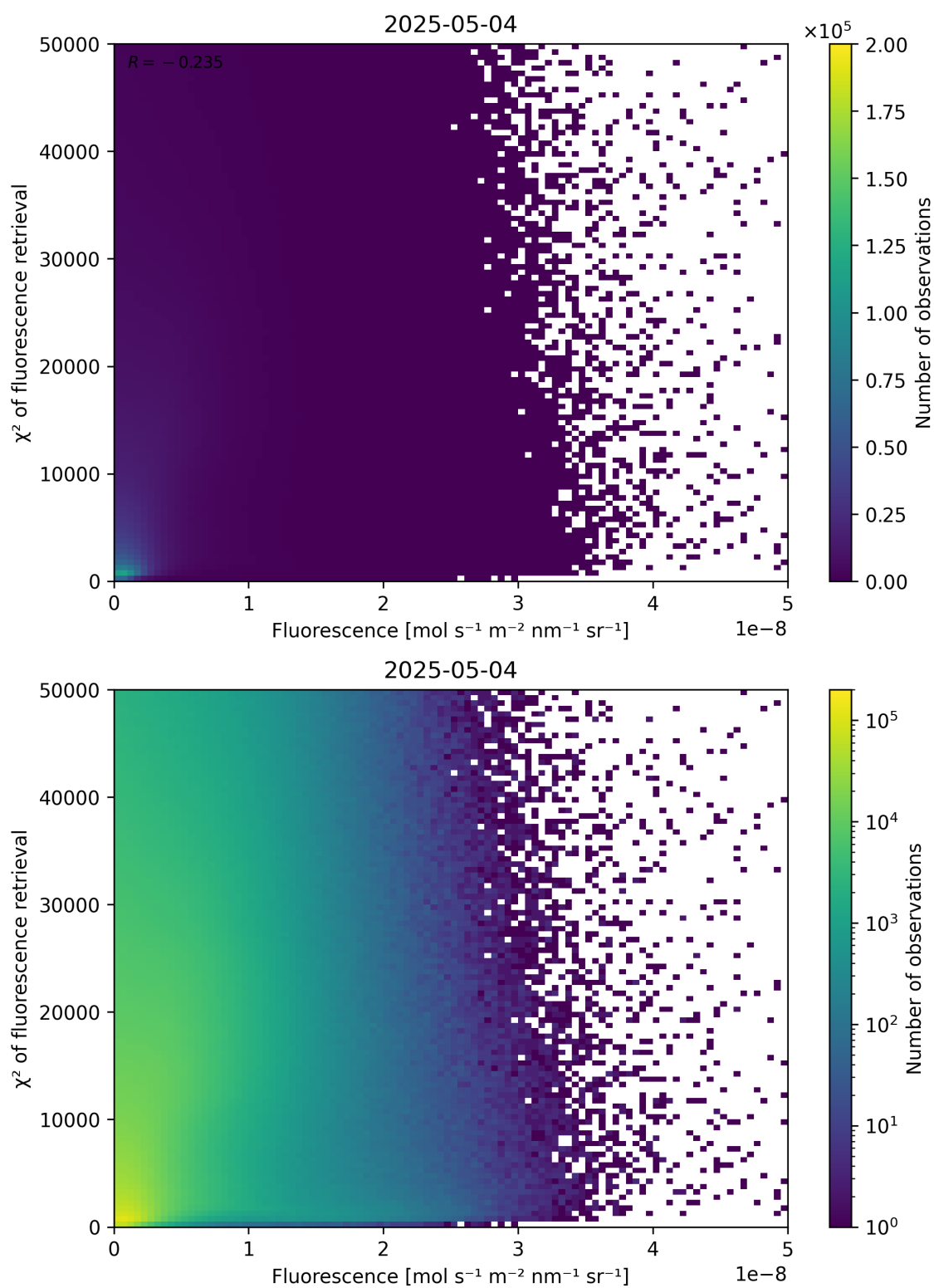
Figure 85: Scatter density plot of “Fluorescence” against “ \chi^2 of fluorescence retrieval” for 2025-05-03 to 2025-05-05.
