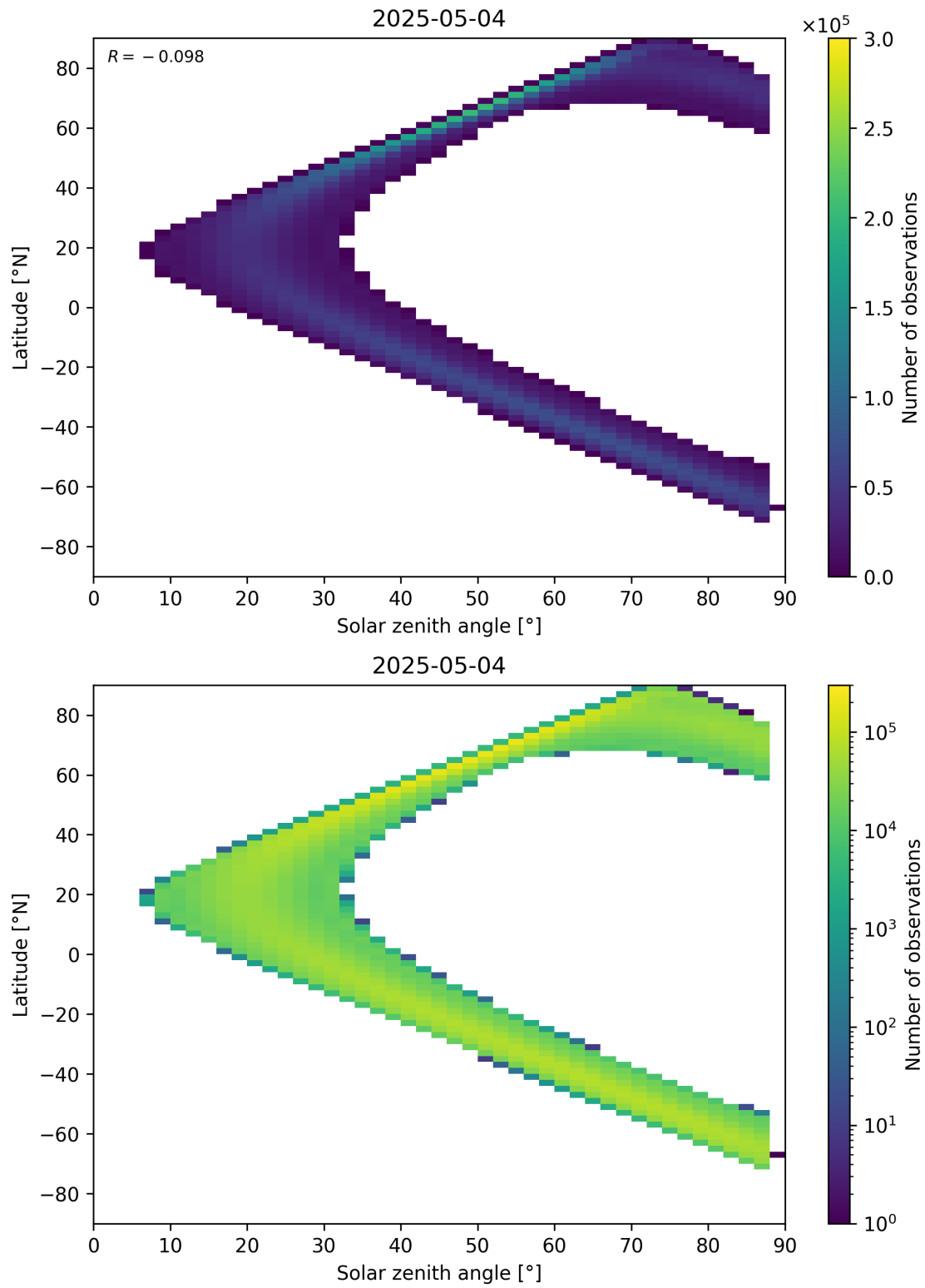
Figure 113: Scatter density plot of “Solar zenith angle” against “Latitude” for 2025-05-03 to 2025-05-05.
