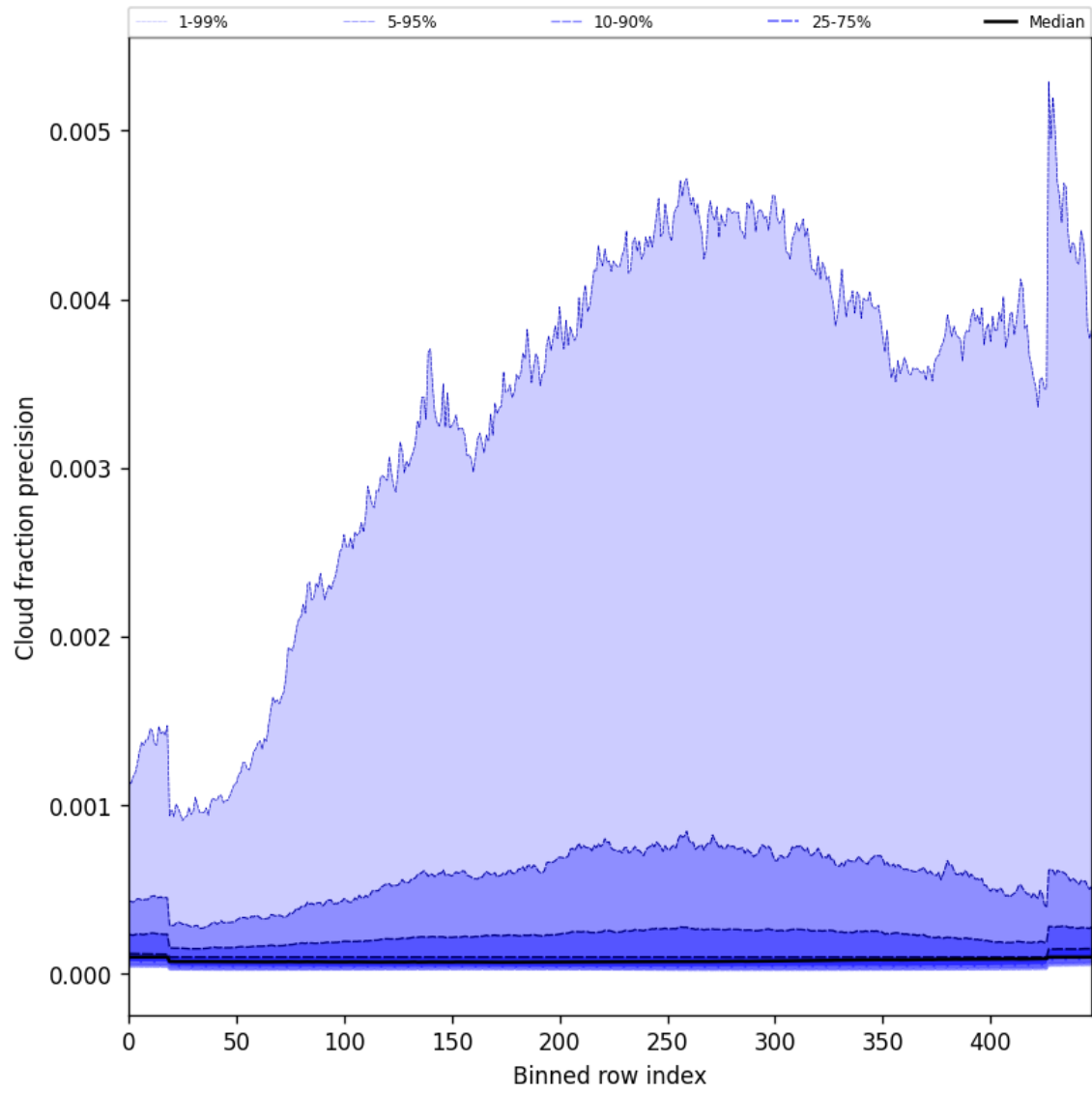
Figure 50: Along track statistics of “Cloud fraction precision” for 2025-05-03 to 2025-05-05
