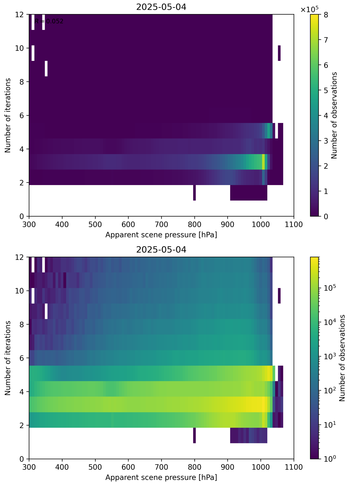
Figure 65: Scatter density plot of “Apparent scene pressure” against “Number of iterations” for 2025-05-03 to 2025-05-05.
