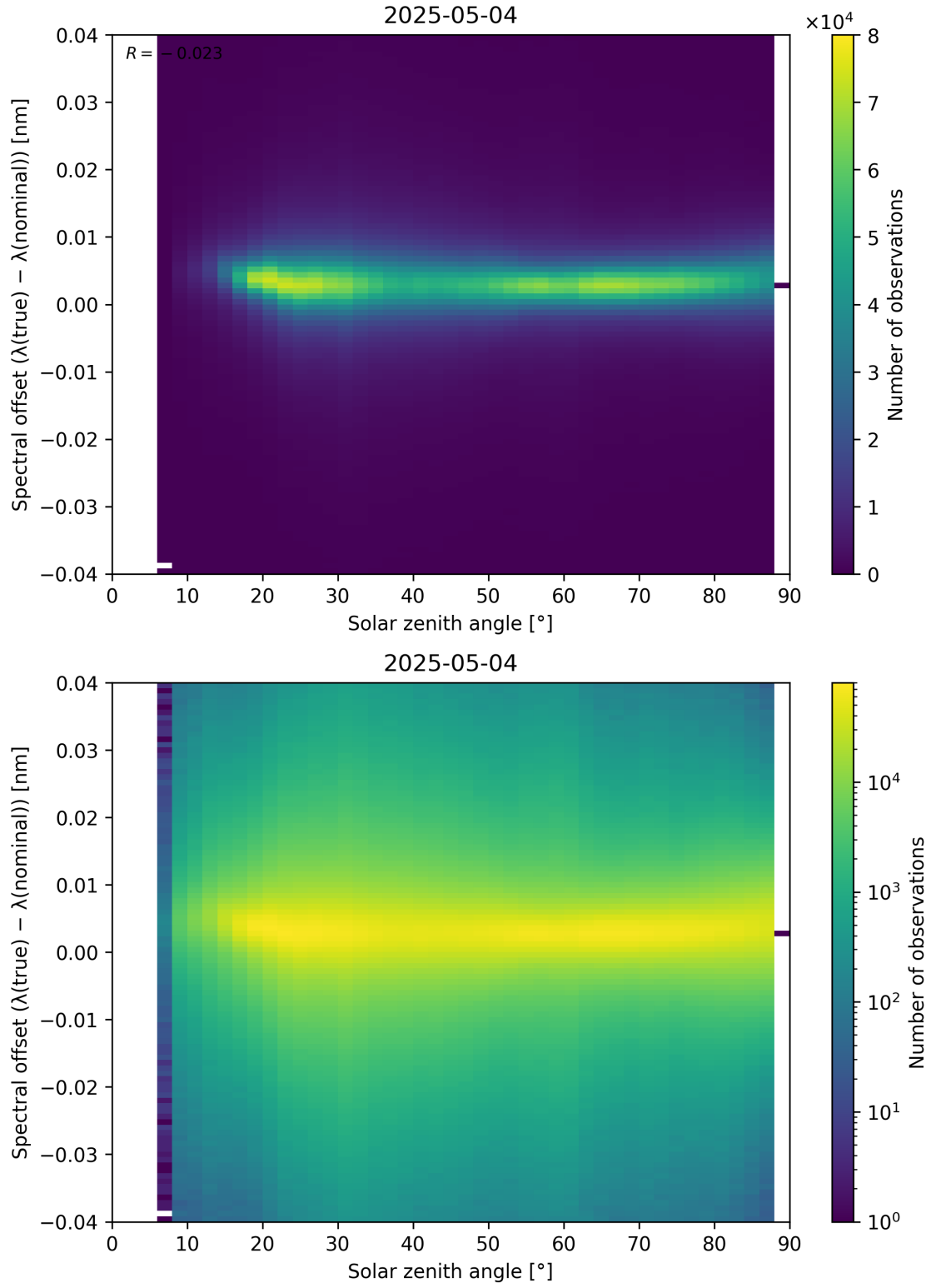
Figure 117: Scatter density plot of “Solar zenith angle” against “Spectral offset ( \lambda_{\text{true}} - \lambda_{\text{nominal}} )” for 2025-05-03 to 2025-05-05.
