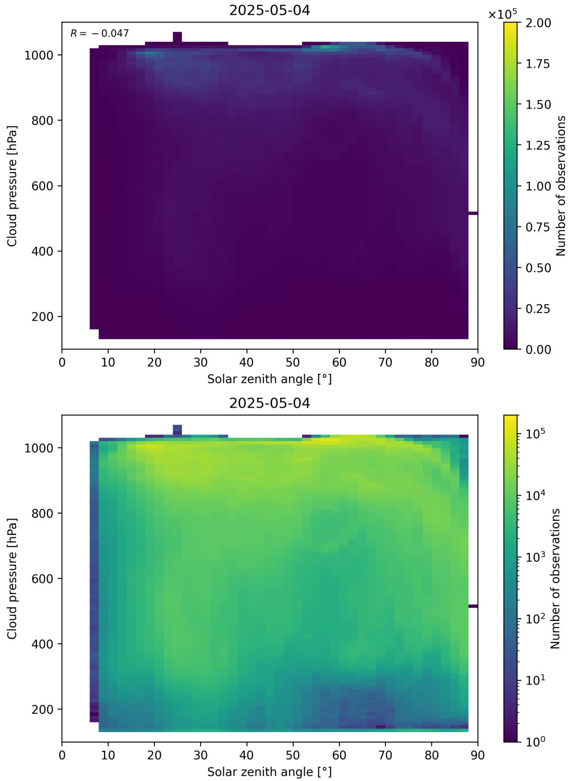
Figure 111: Scatter density plot of “Solar zenith angle” against “Cloud pressure” for 2025-05-03 to 2025-05-05.
