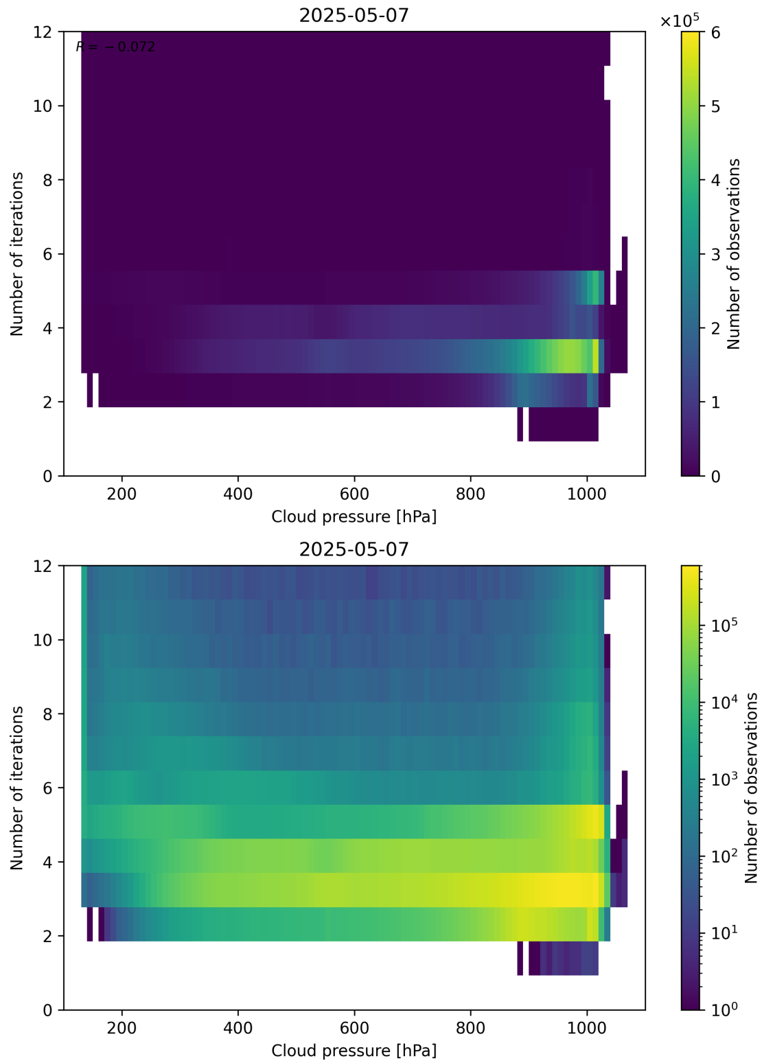
Figure 81: Scatter density plot of “Cloud pressure” against “Number of iterations” for 2025-05-06 to 2025-05-08.
