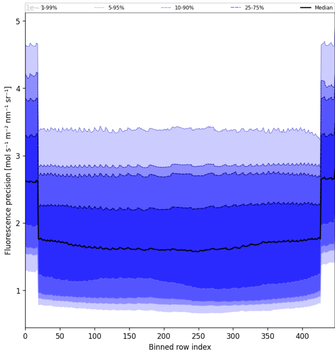
Figure 58: Along track statistics of “Fluorescence precision” for 2025-05-06 to 2025-05-08
