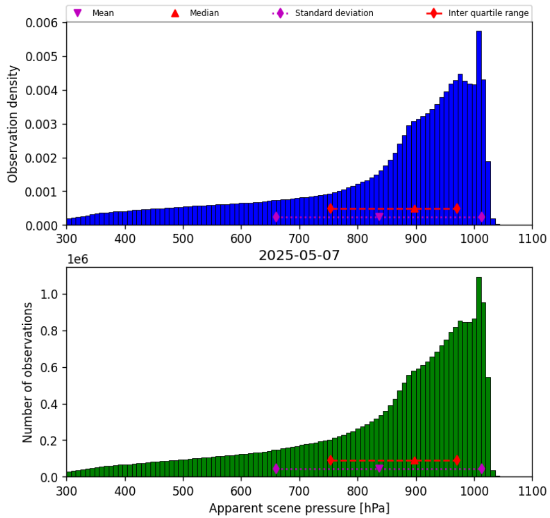
Figure 36: Histogram of “Apparent scene pressure” for 2025-05-06 to 2025-05-08
