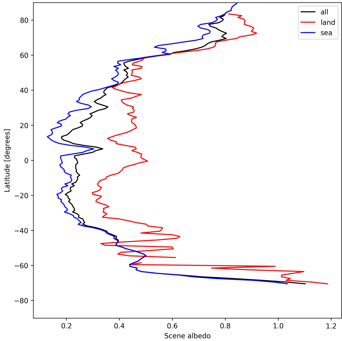
Figure 17: Zonal average of “Scene albedo” for 2025-05-06 to 2025-05-08.
