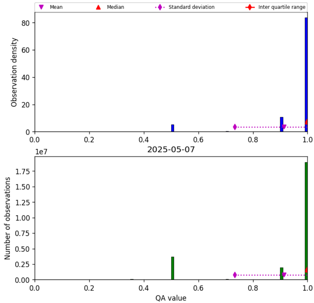
Figure 29: Histogram of “QA value” for 2025-05-06 to 2025-05-08
