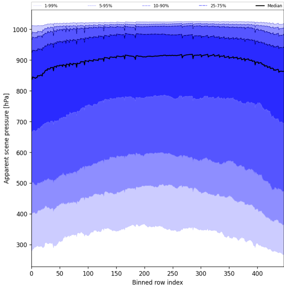
Figure 53: Along track statistics of “Apparent scene pressure” for 2025-05-06 to 2025-05-08
