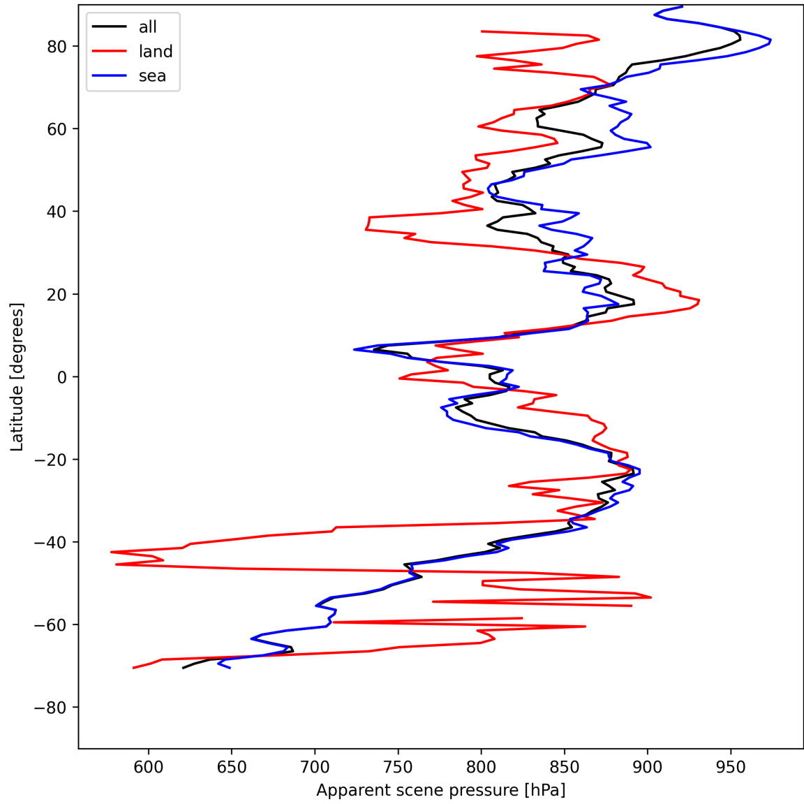
Figure 19: Zonal average of “Apparent scene pressure” for 2025-05-06 to 2025-05-08.
