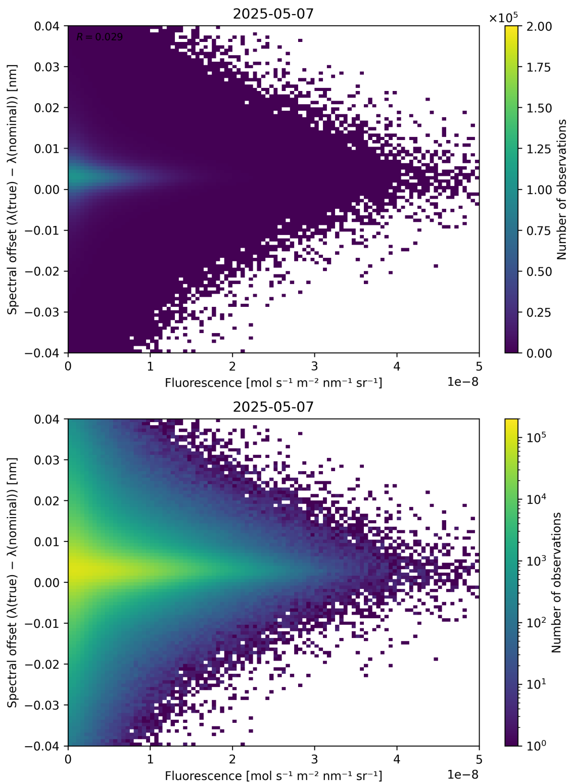
Figure 87: Scatter density plot of “Fluorescence” against “Spectral offset ( \lambda_{\text{true}} - \lambda_{\text{nominal}} )” for 2025-05-06 to 2025-05-08.
