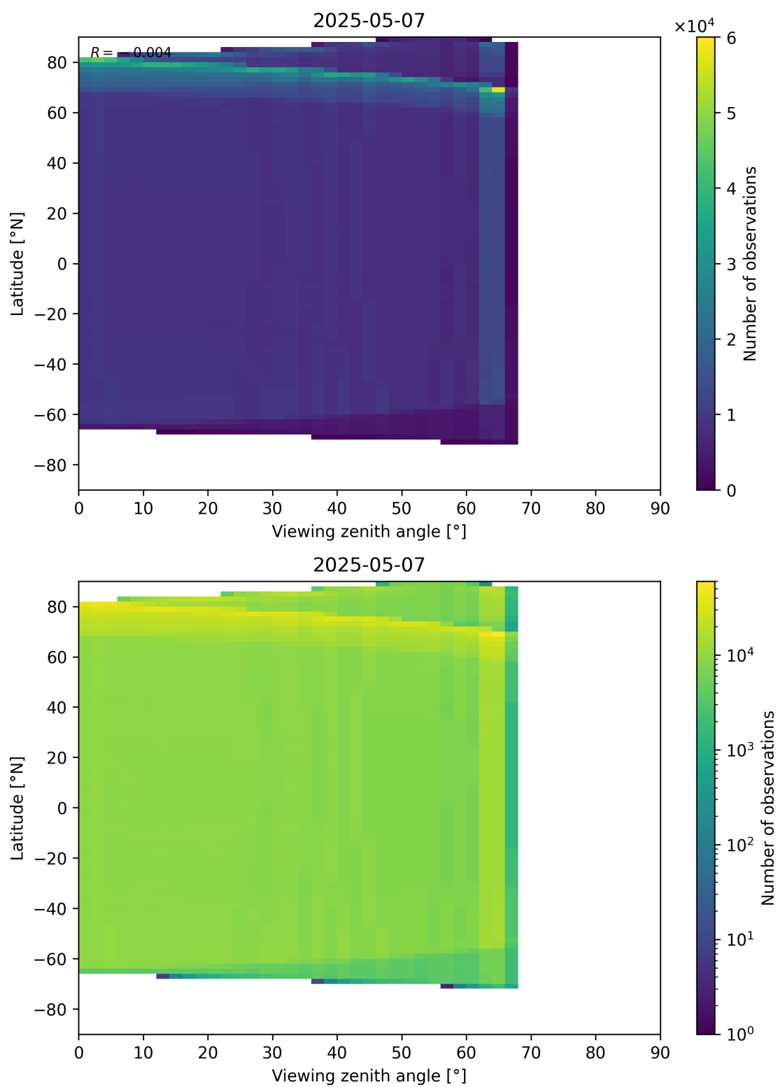
Figure 123: Scatter density plot of “Viewing zenith angle” against “Latitude” for 2025-05-06 to 2025-05-08.
