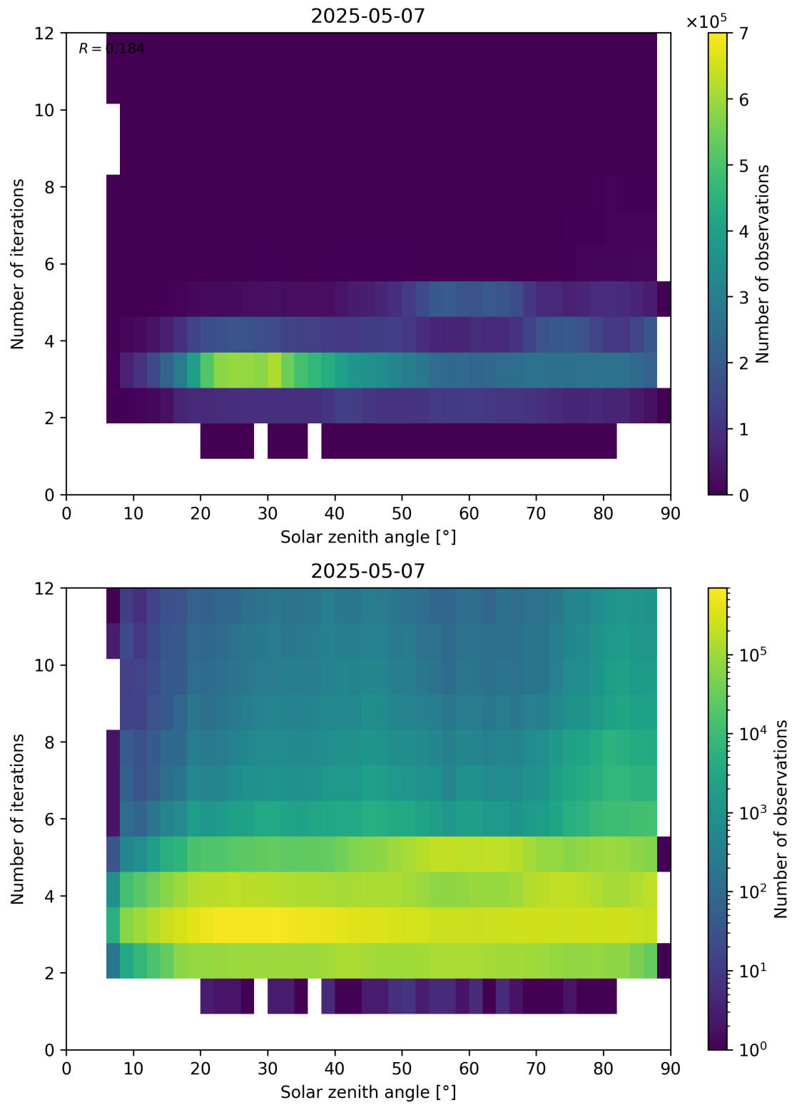
Figure 114: Scatter density plot of “Solar zenith angle” against “Number of iterations” for 2025-05-06 to 2025-05-08.
