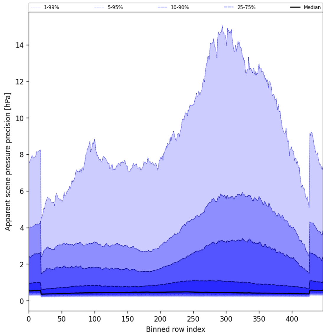
Figure 54: Along track statistics of “Apparent scene pressure precision” for 2025-05-06 to 2025-05-08
