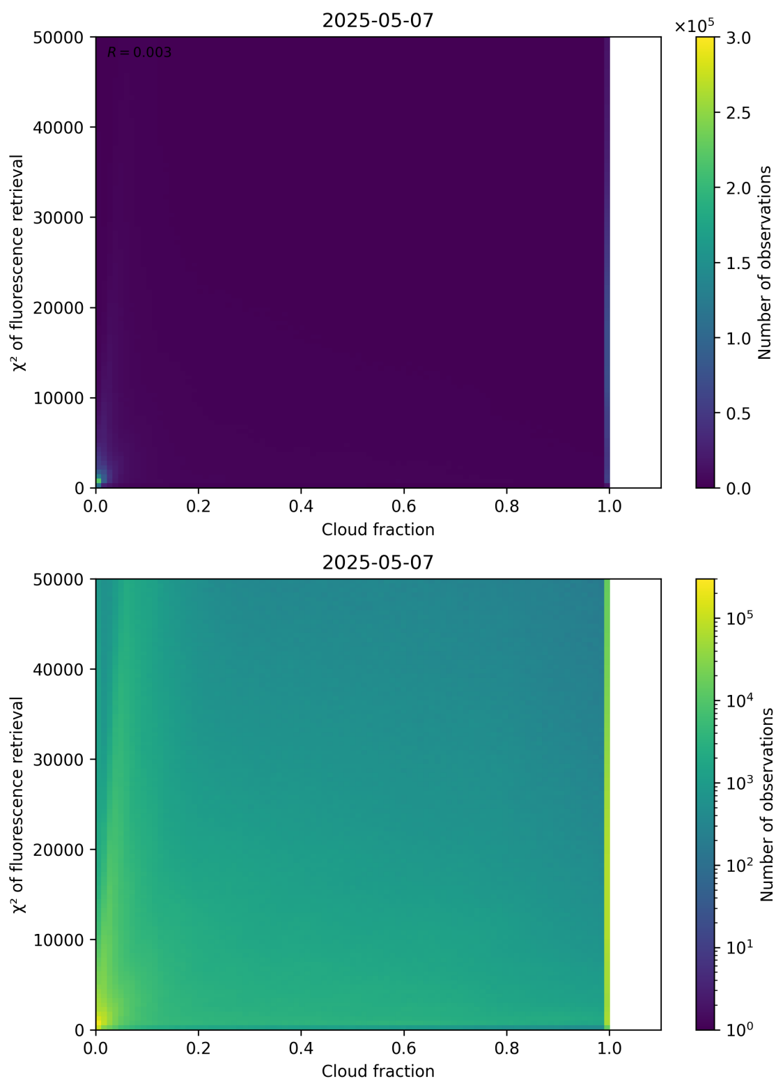
Figure 71: Scatter density plot of “Cloud fraction” against “ \chi^2 of fluorescence retrieval” for 2025-05-06 to 2025-05-08.
