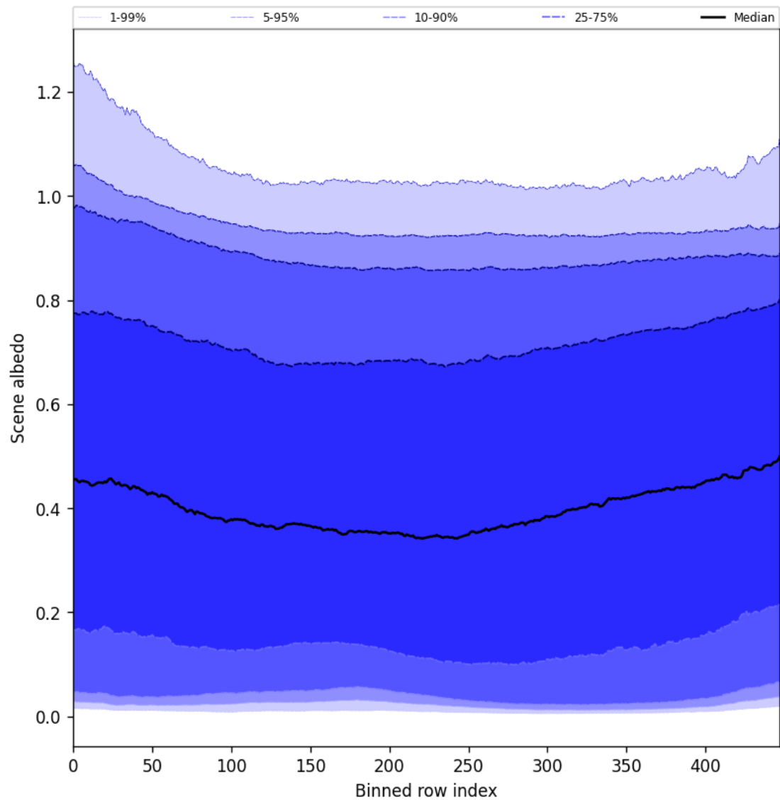
Figure 51: Along track statistics of “Scene albedo” for 2025-05-06 to 2025-05-08
