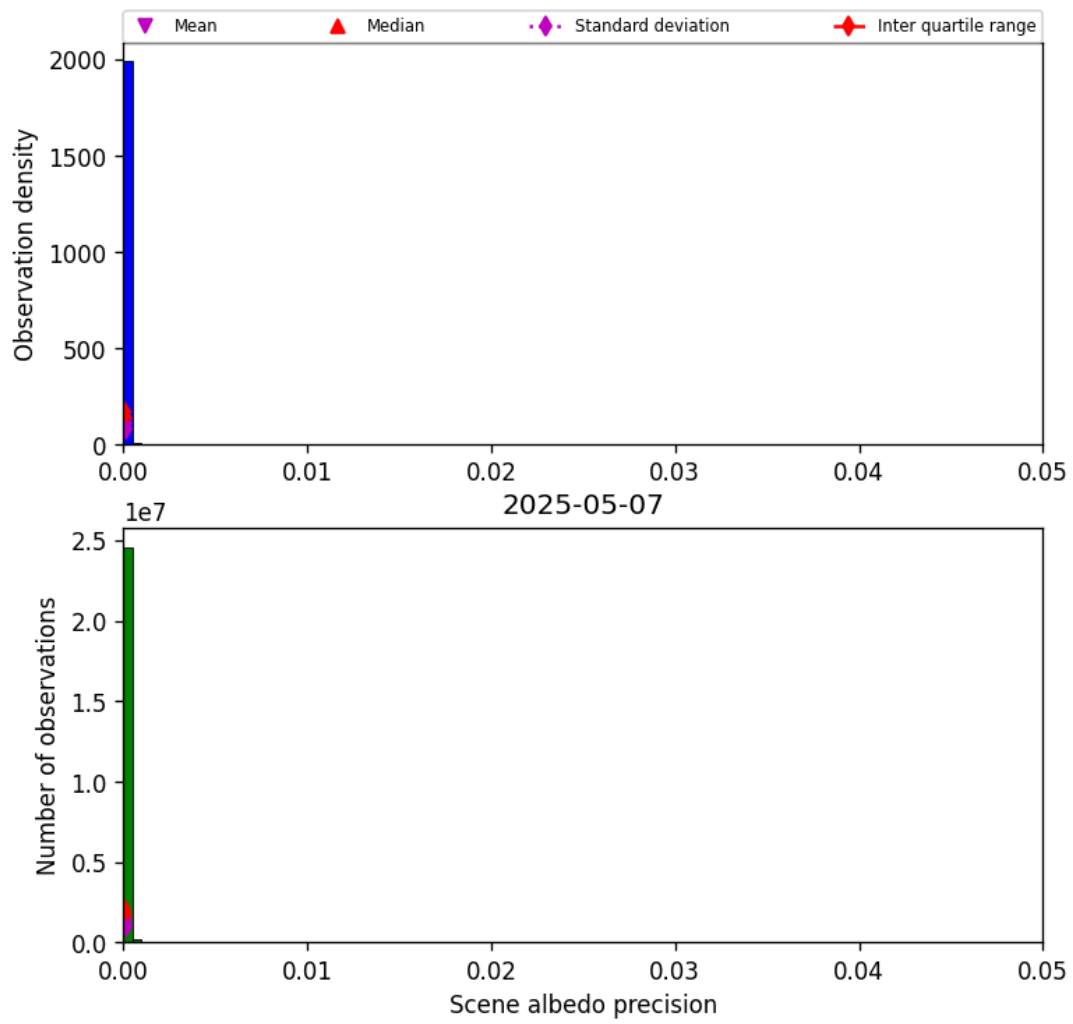
Figure 35: Histogram of “Scene albedo precision” for 2025-05-06 to 2025-05-08
