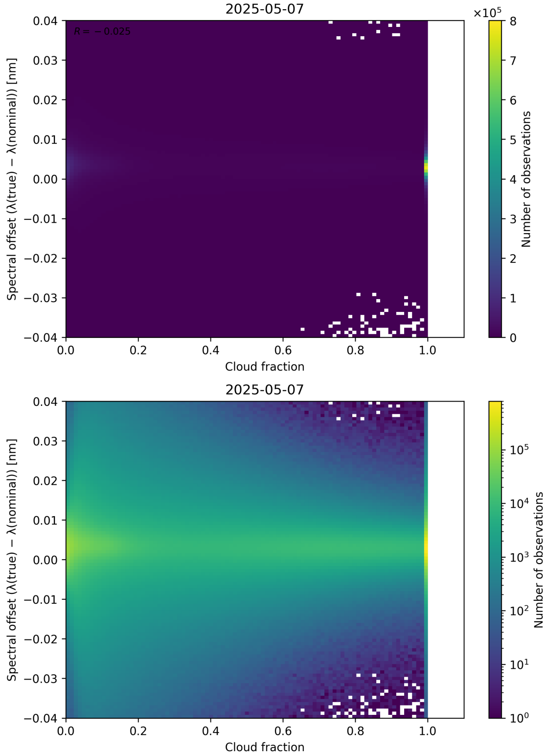
Figure 76: Scatter density plot of “Cloud fraction” against “Spectral offset ( \lambda_{\text{true}} - \lambda_{\text{nominal}} )” for 2025-05-06 to 2025-05-08.
