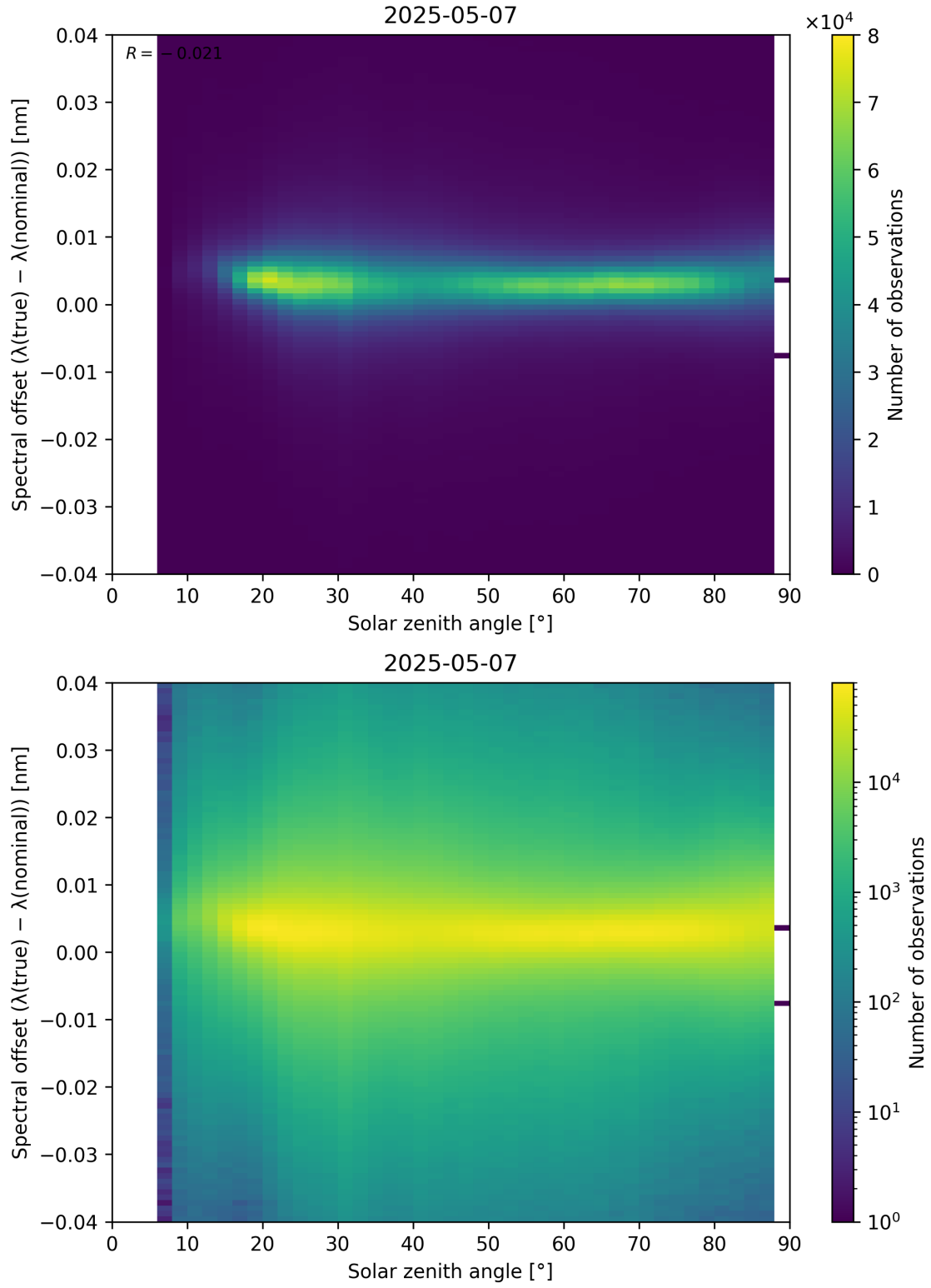
Figure 117: Scatter density plot of “Solar zenith angle” against “Spectral offset ( \lambda_{\text{true}} - \lambda_{\text{nominal}} )” for 2025-05-06 to 2025-05-08.
