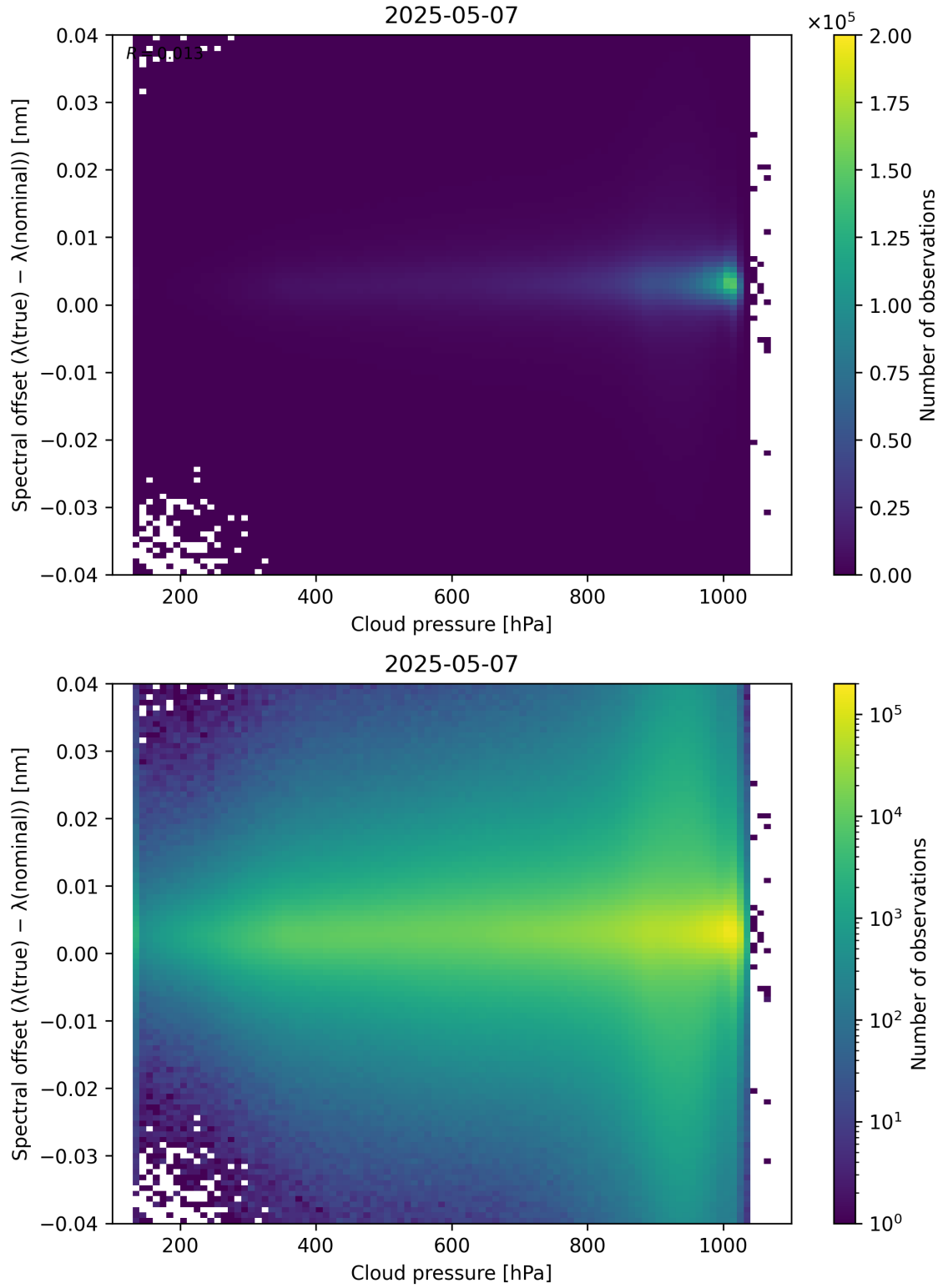
Figure 84: Scatter density plot of “Cloud pressure” against “Spectral offset ( \lambda_{\text{true}} - \lambda_{\text{nominal}} )” for 2025-05-06 to 2025-05-08.
