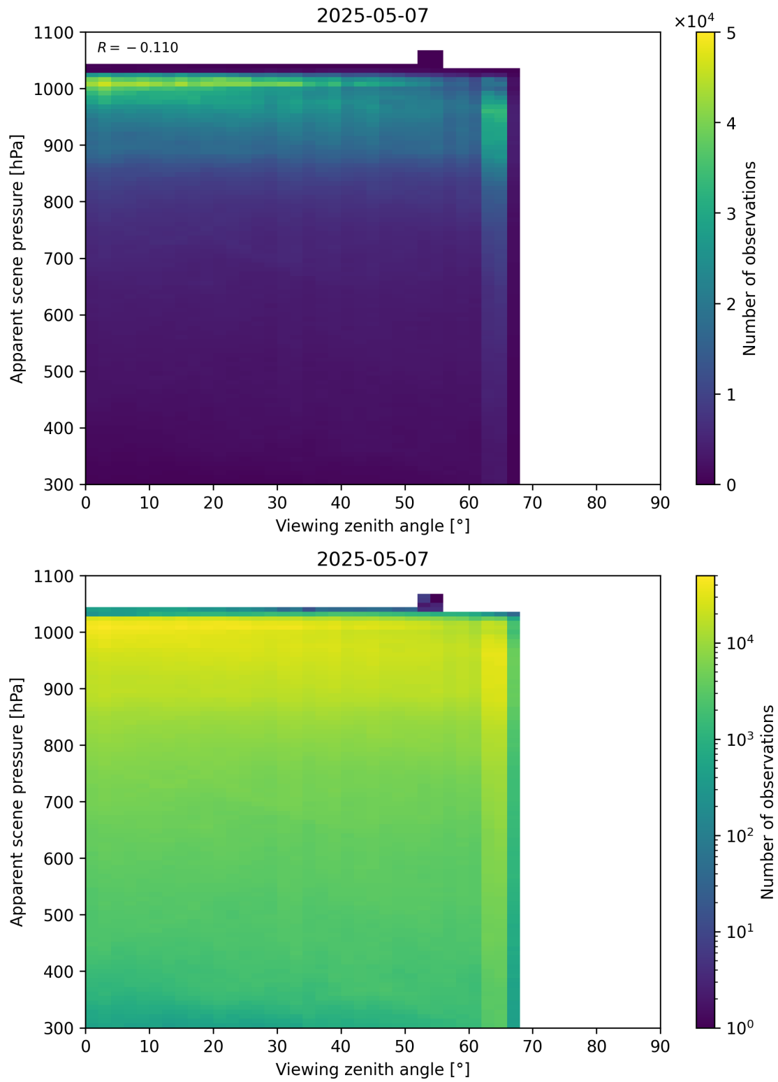
Figure 118: Scatter density plot of “Viewing zenith angle” against “Apparent scene pressure” for 2025-05-06 to 2025-05-08.
