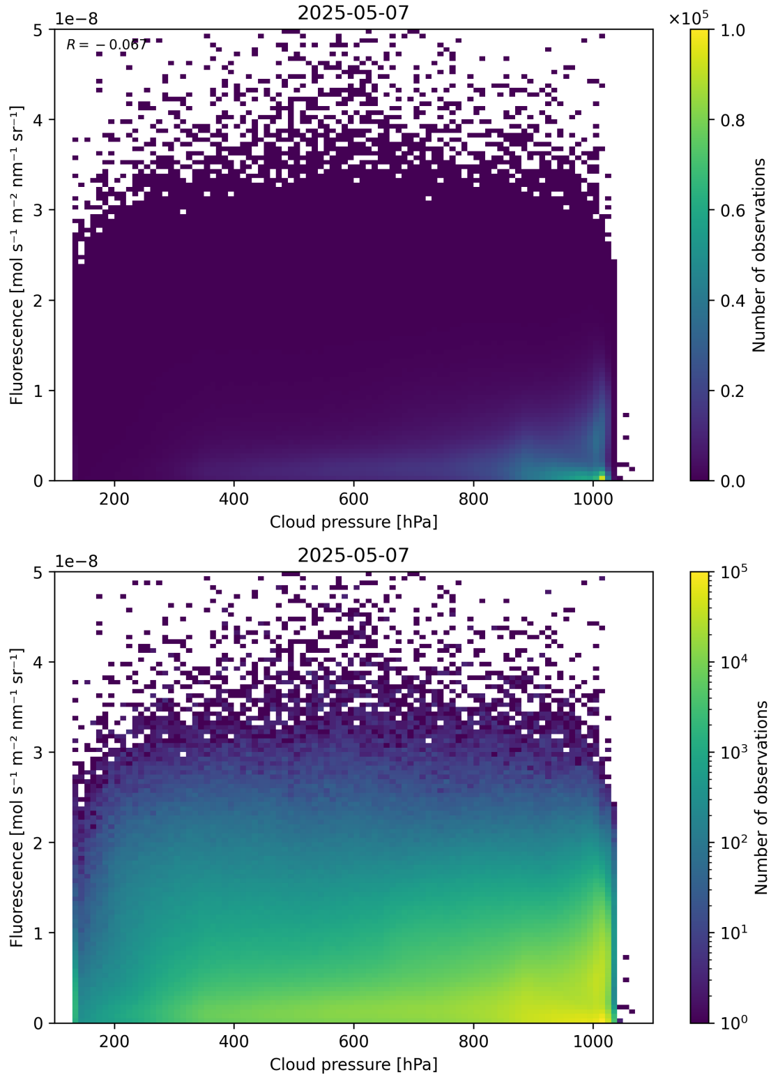
Figure 80: Scatter density plot of “Cloud pressure” against “Fluorescence” for 2025-05-06 to 2025-05-08.
