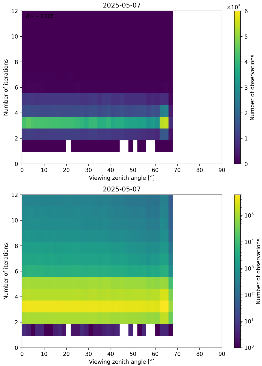
Figure 124: Scatter density plot of “Viewing zenith angle” against “Number of iterations” for 2025-05-06 to 2025-05-08.
