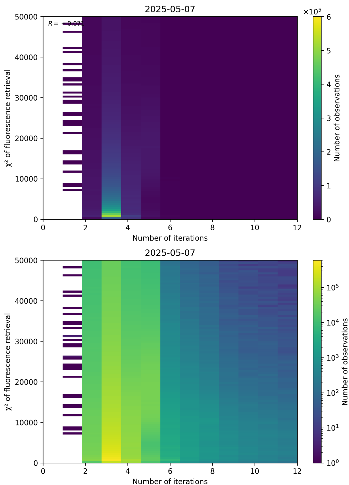
Figure 97: Scatter density plot of “Number of iterations” against “ \chi^2 of fluorescence retrieval” for 2025-05-06 to 2025-05-08.
