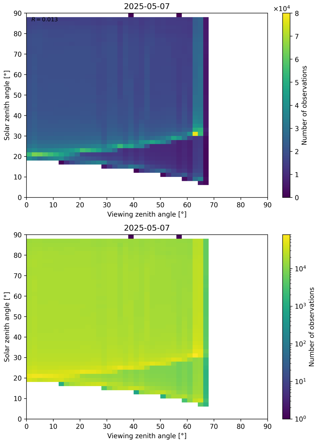
Figure 127: Scatter density plot of “Viewing zenith angle” against “Solar zenith angle” for 2025-05-06 to 2025-05-08.
