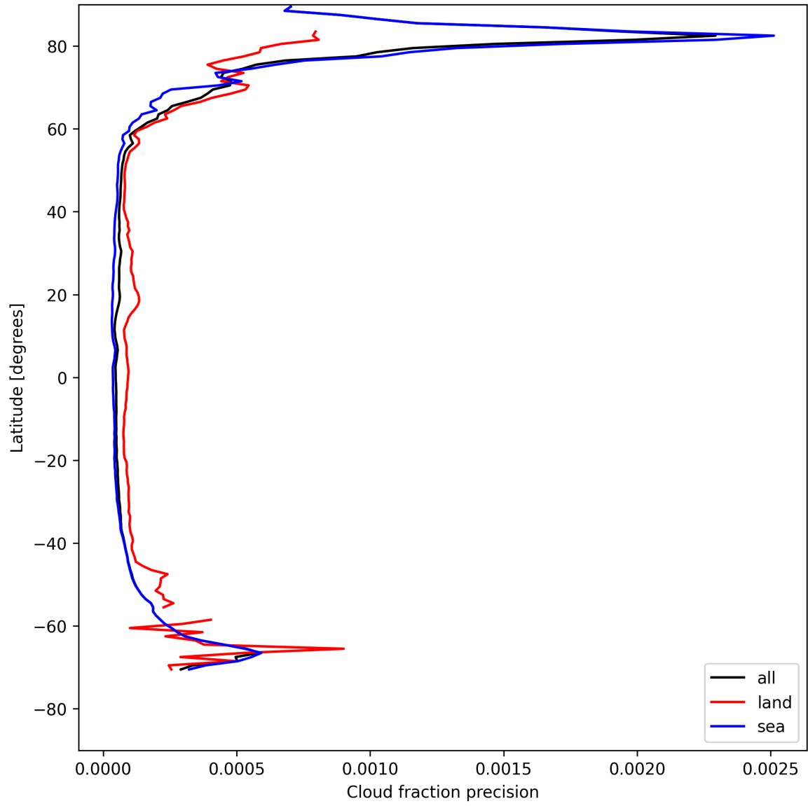
Figure 16: Zonal average of “Cloud fraction precision” for 2025-05-06 to 2025-05-08.
