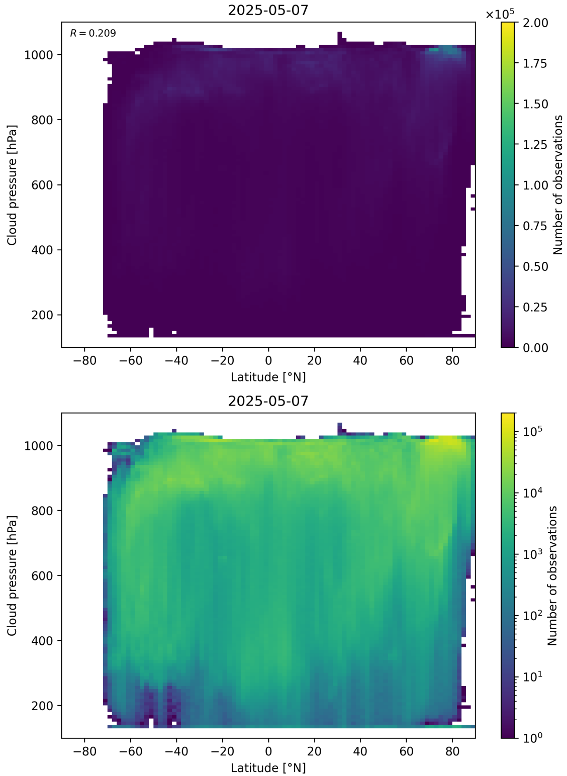
Figure 91: Scatter density plot of “Latitude” against “Cloud pressure” for 2025-05-06 to 2025-05-08.
