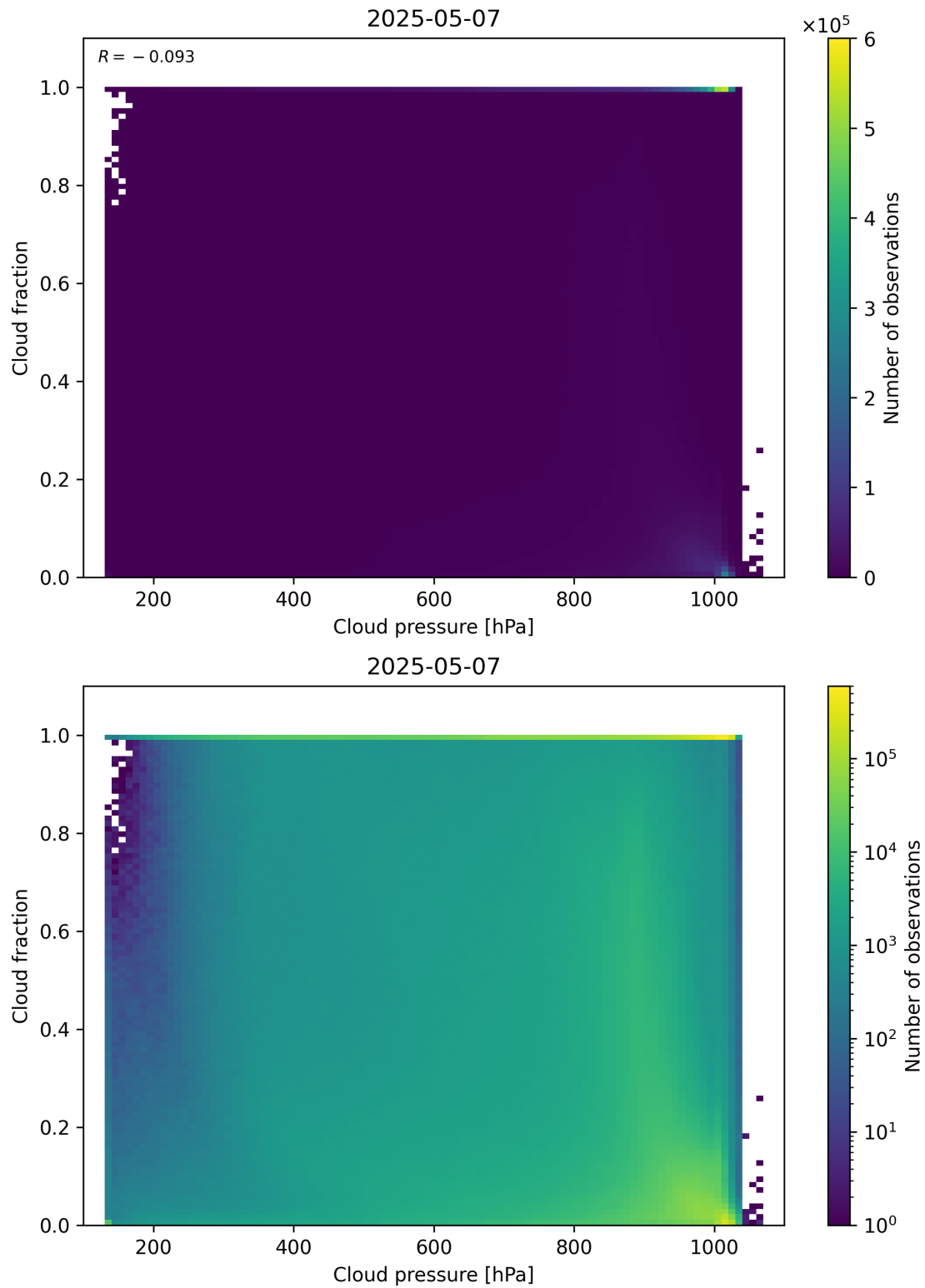
Figure 79: Scatter density plot of “Cloud pressure” against “Cloud fraction” for 2025-05-06 to 2025-05-08.
