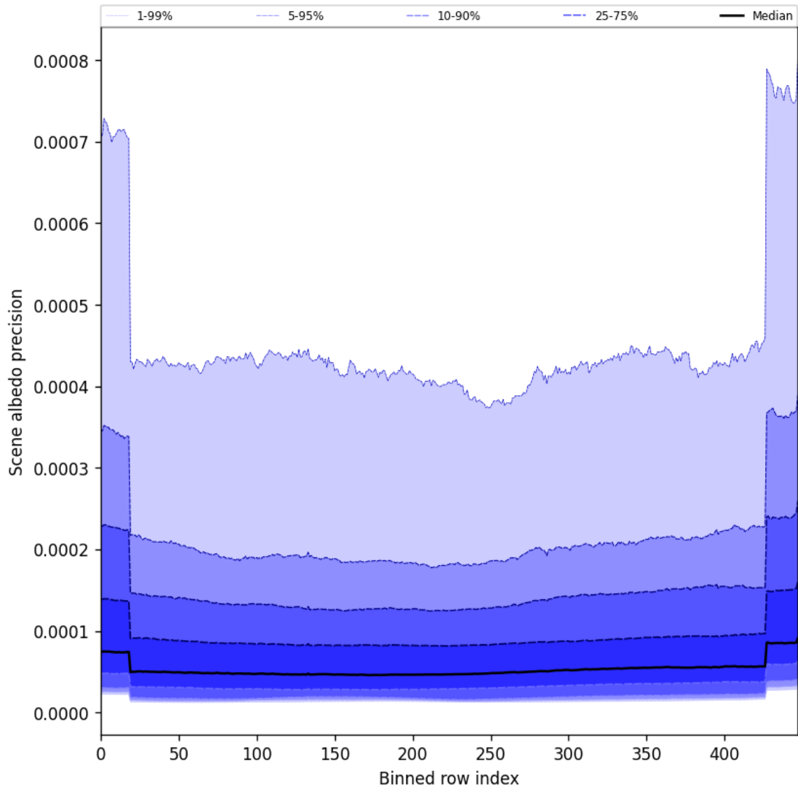
Figure 52: Along track statistics of “Scene albedo precision” for 2025-05-06 to 2025-05-08
