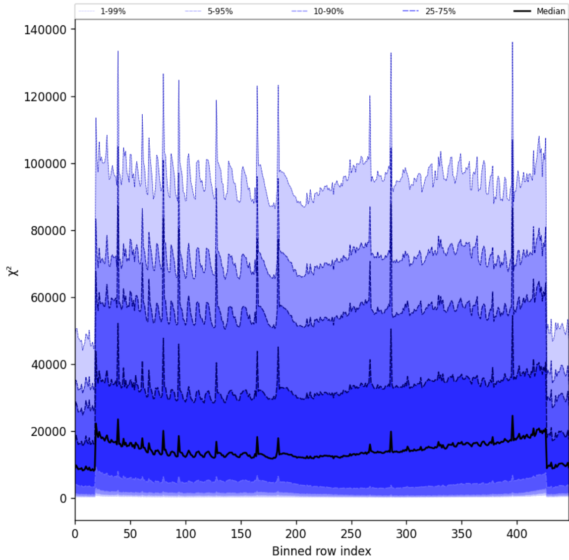
Figure 55: Along track statistics of “ \chi^2 ” for 2025-05-06 to 2025-05-08
