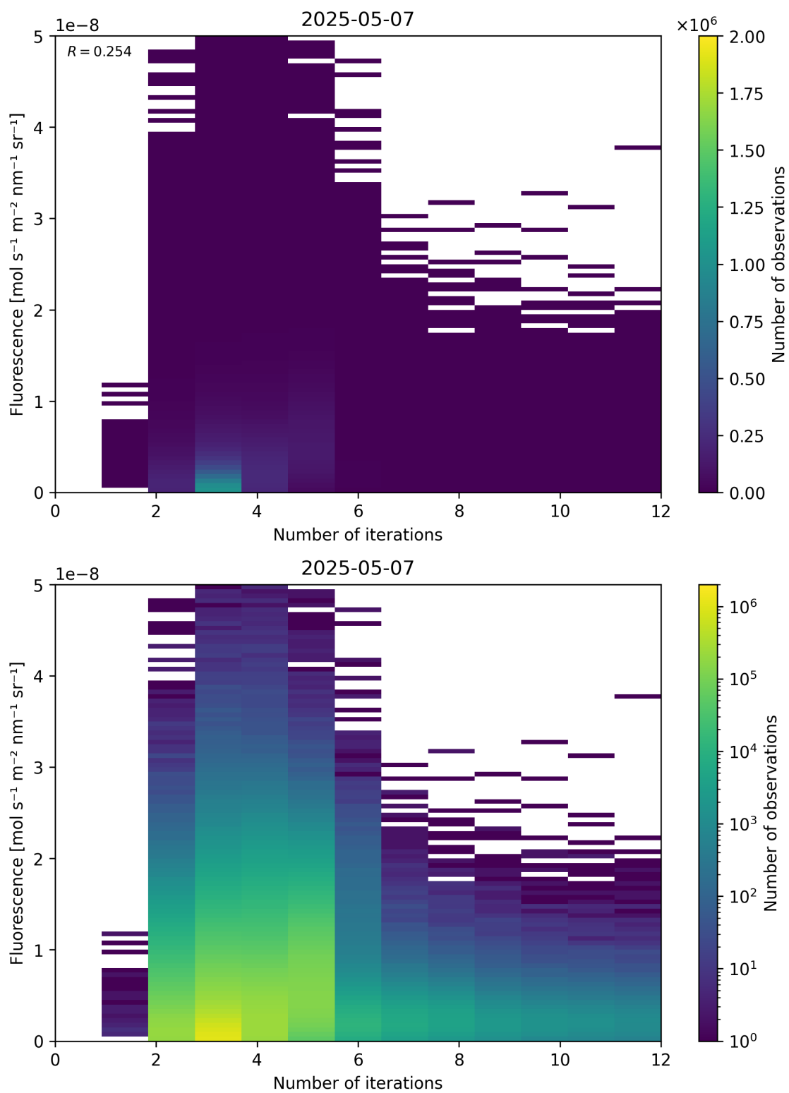
Figure 98: Scatter density plot of “Number of iterations” against “Fluorescence” for 2025-05-06 to 2025-05-08.
