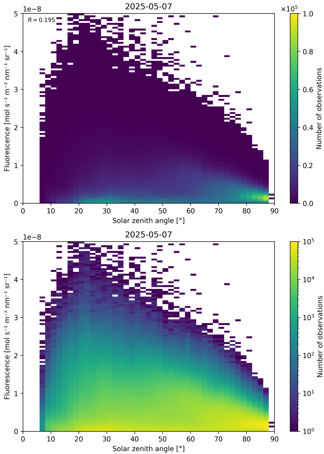
Figure 112: Scatter density plot of “Solar zenith angle” against “Fluorescence” for 2025-05-06 to 2025-05-08.
