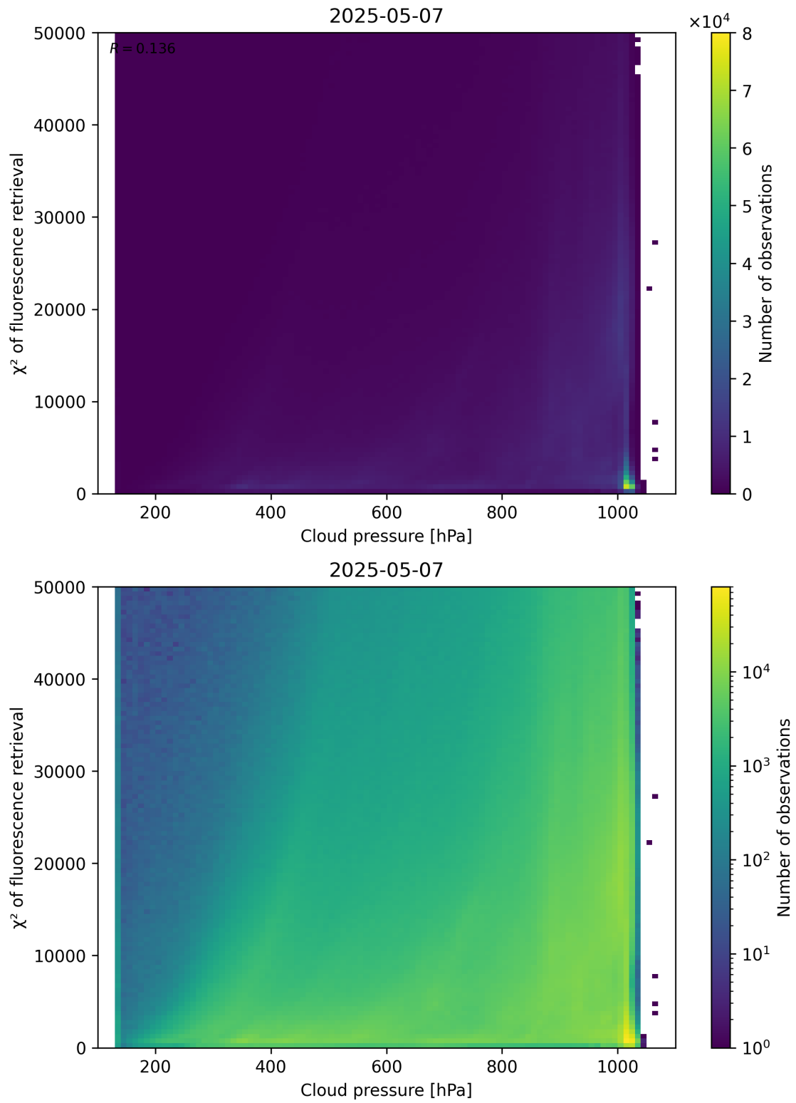
Figure 78: Scatter density plot of “Cloud pressure” against “ \chi^2 of fluorescence retrieval” for 2025-05-06 to 2025-05-08.
