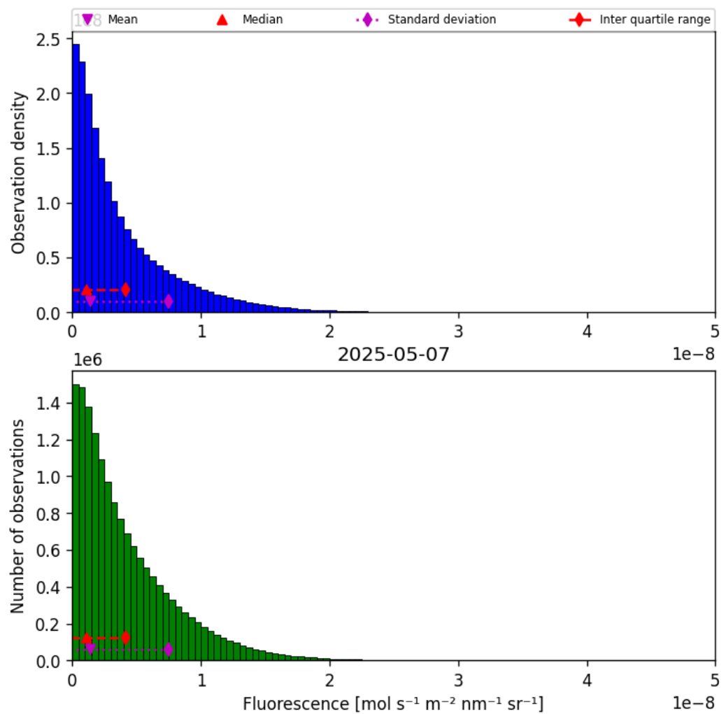
Figure 40: Histogram of “Fluorescence” for 2025-05-06 to 2025-05-08
