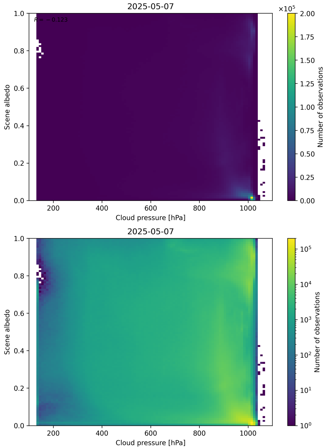
Figure 83: Scatter density plot of “Cloud pressure” against “Scene albedo” for 2025-05-06 to 2025-05-08.
