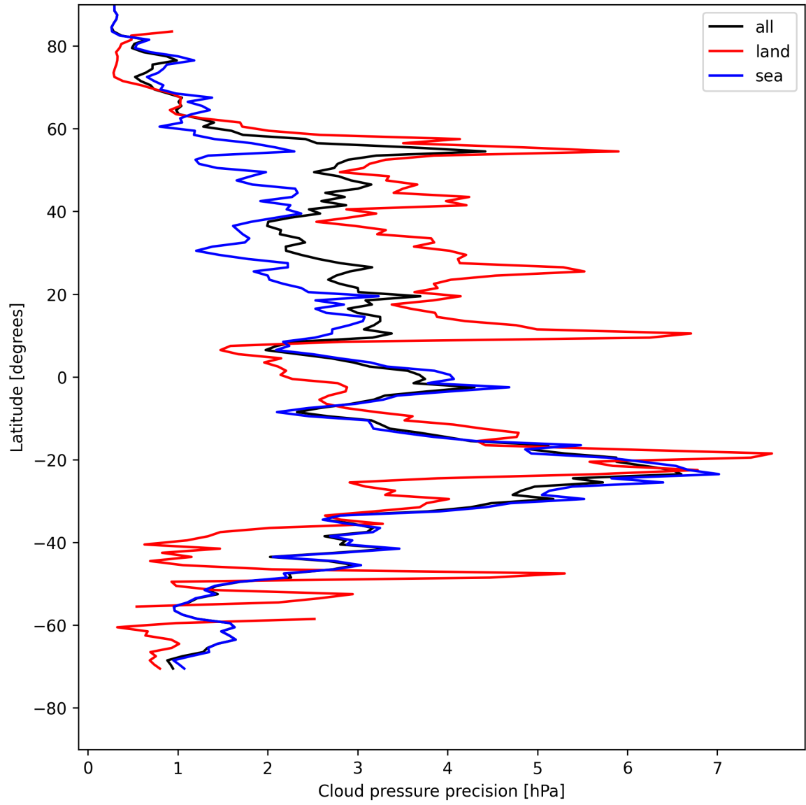
Figure 14: Zonal average of “Cloud pressure precision” for 2025-05-06 to 2025-05-08.
