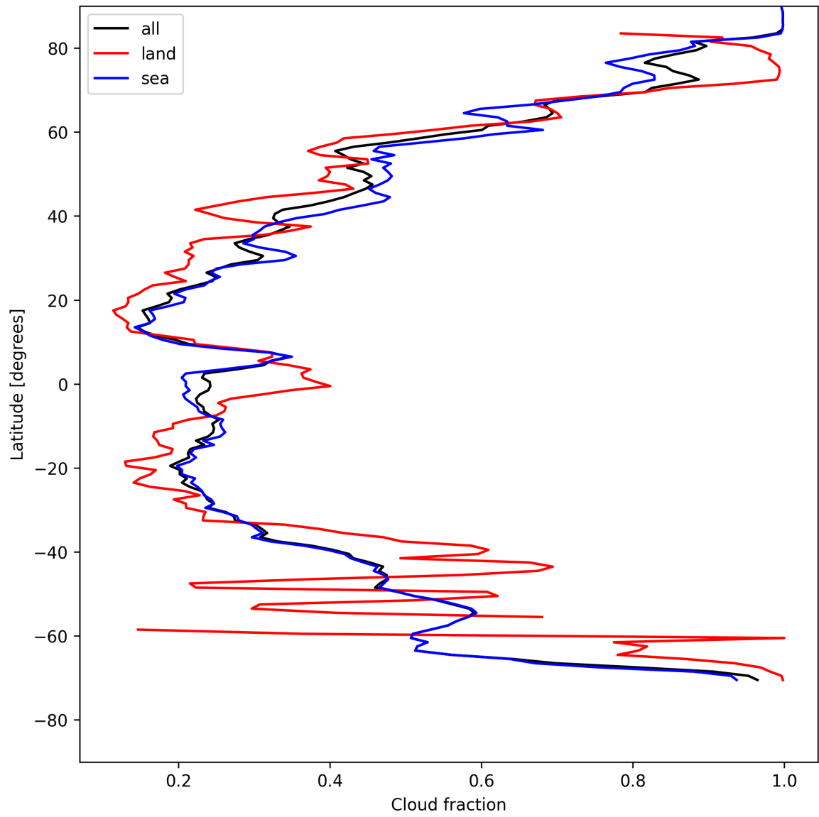
Figure 15: Zonal average of “Cloud fraction” for 2025-05-06 to 2025-05-08.
