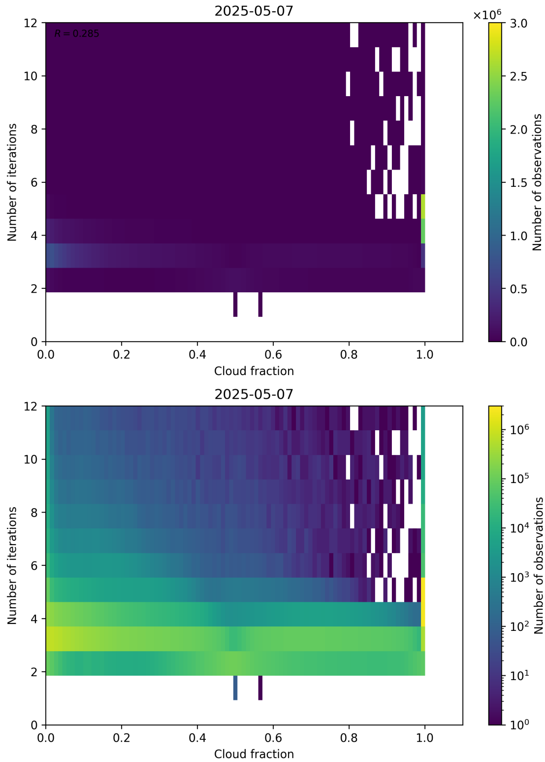
Figure 73: Scatter density plot of “Cloud fraction” against “Number of iterations” for 2025-05-06 to 2025-05-08.
