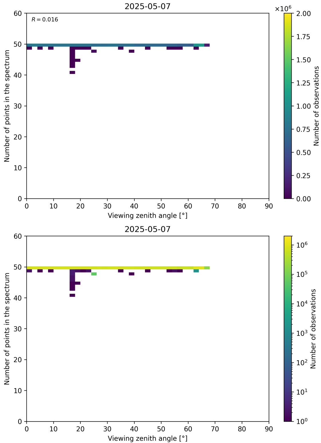
Figure 125: Scatter density plot of “Viewing zenith angle” against “Number of points in the spectrum” for 2025-05-06 to 2025-05-08.
