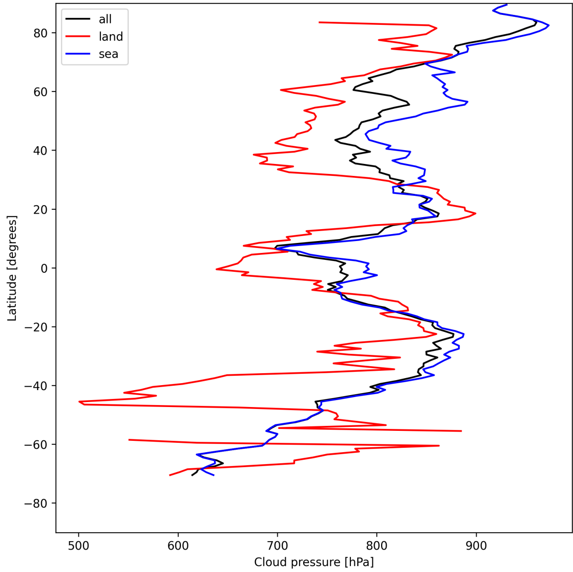
Figure 13: Zonal average of “Cloud pressure” for 2025-05-06 to 2025-05-08.
