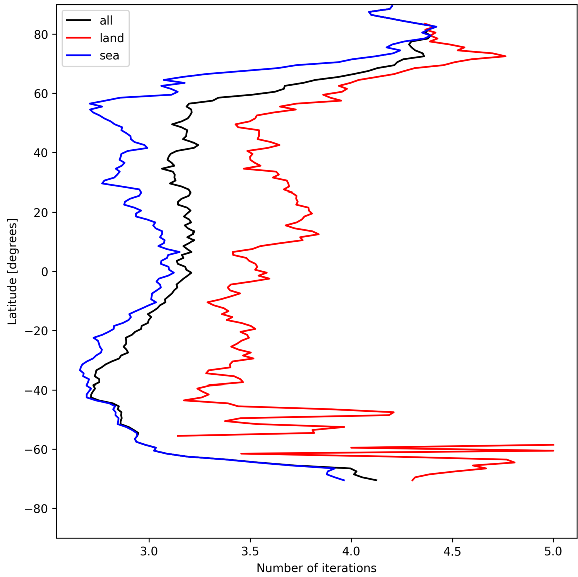
Figure 22: Zonal average of “Number of iterations” for 2025-05-06 to 2025-05-08.
