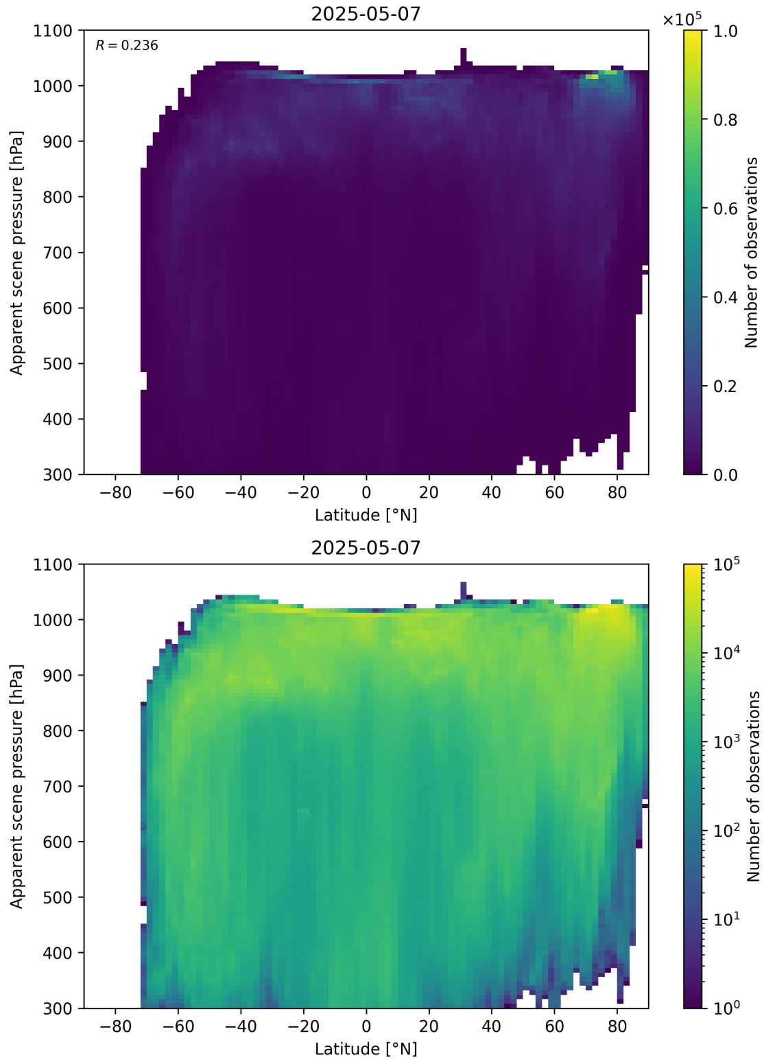
Figure 88: Scatter density plot of “Latitude” against “Apparent scene pressure” for 2025-05-06 to 2025-05-08.
