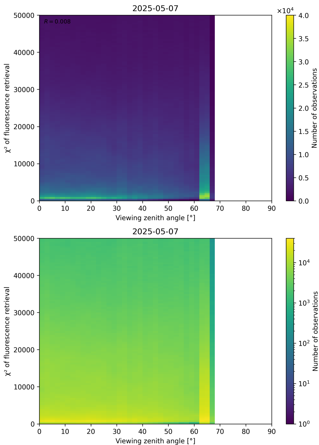
Figure 119: Scatter density plot of “Viewing zenith angle” against “ \chi^2 of fluorescence retrieval” for 2025-05-06 to 2025-05-08.
