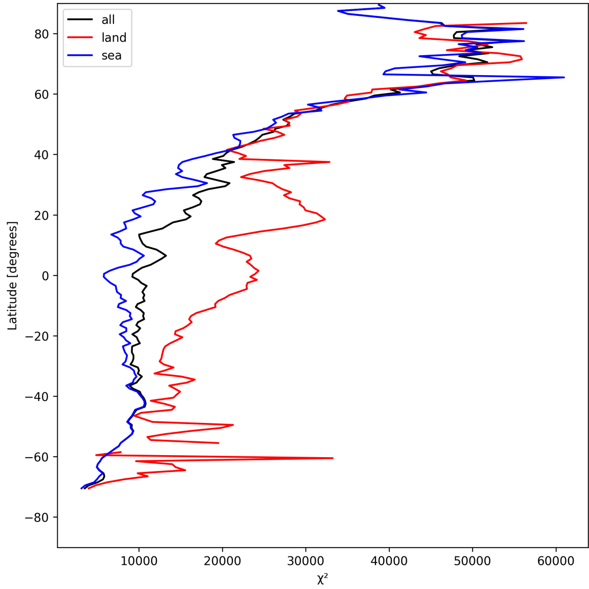
Figure 21: Zonal average of “ \chi^2 ” for 2025-05-06 to 2025-05-08.
