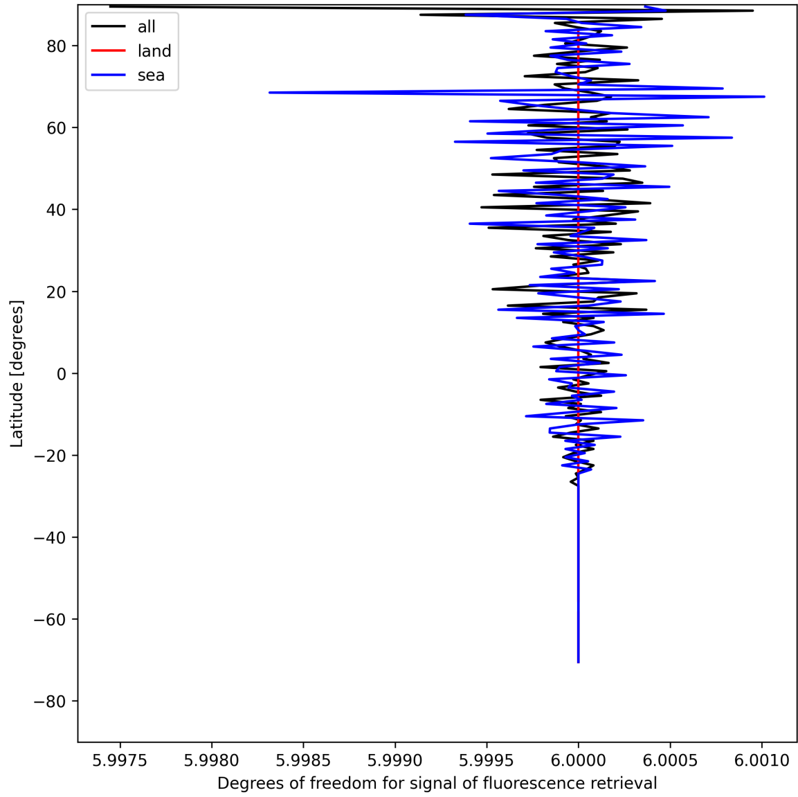
Figure 26: Zonal average of “Degrees of freedom for signal of fluorescence retrieval” for 2025-05-06 to 2025-05-08.
