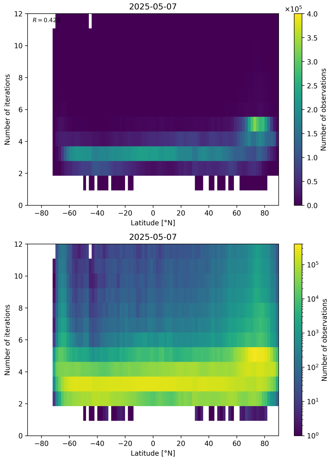
Figure 93: Scatter density plot of “Latitude” against “Number of iterations” for 2025-05-06 to 2025-05-08.
