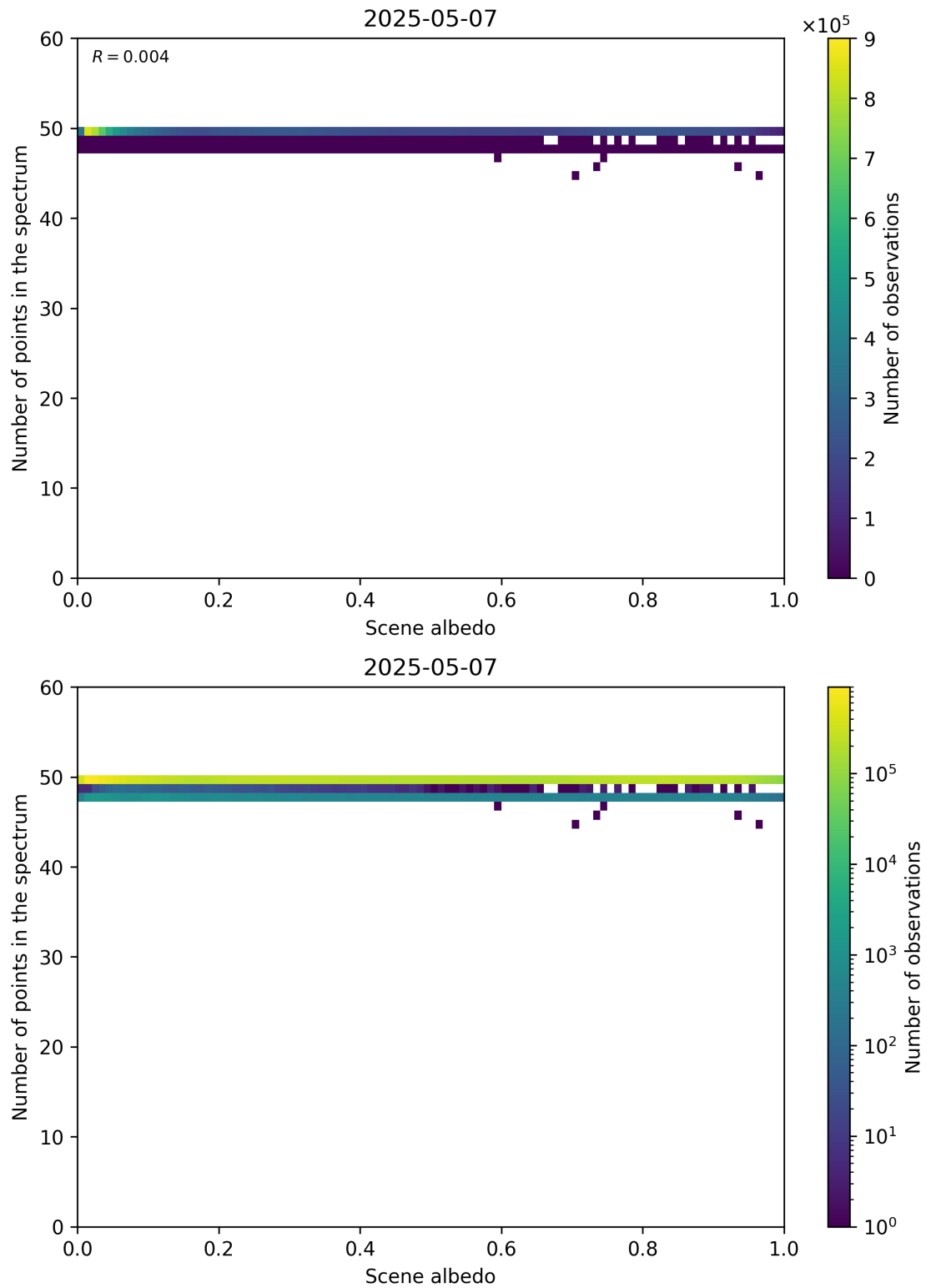
Figure 106: Scatter density plot of “Scene albedo” against “Number of points in the spectrum” for 2025-05-06 to 2025-05-08.
