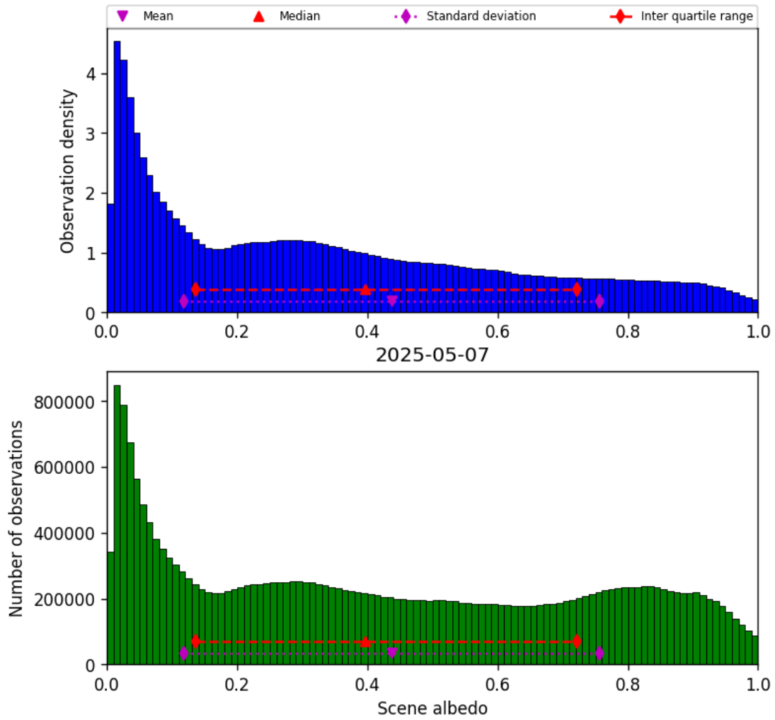
Figure 34: Histogram of “Scene albedo” for 2025-05-06 to 2025-05-08
