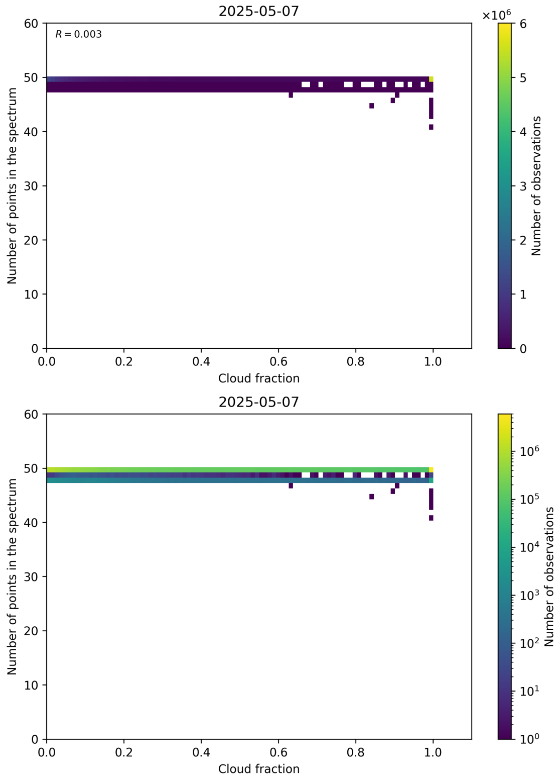
Figure 74: Scatter density plot of “Cloud fraction” against “Number of points in the spectrum” for 2025-05-06 to 2025-05-08.
