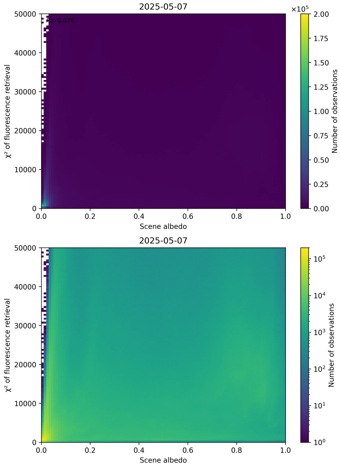
Figure 103: Scatter density plot of “Scene albedo” against “ \chi^2 of fluorescence retrieval” for 2025-05-06 to 2025-05-08.
