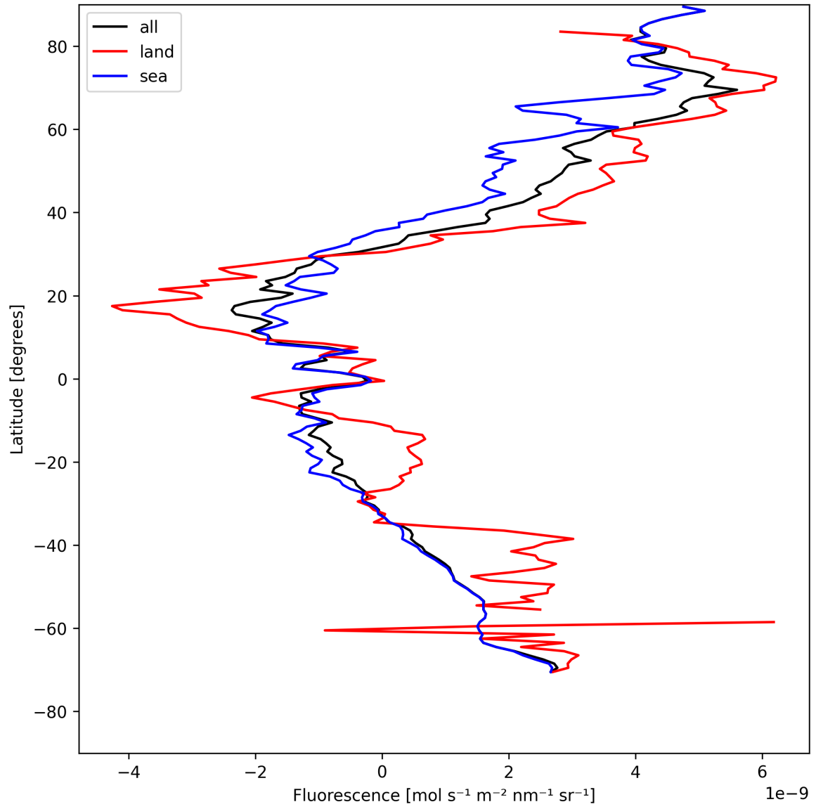
Figure 23: Zonal average of “Fluorescence” for 2025-05-06 to 2025-05-08.
