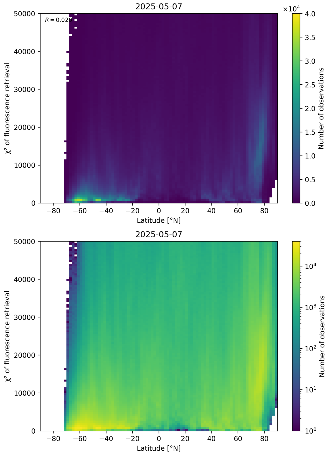
Figure 89: Scatter density plot of “Latitude” against “ \chi^2 of fluorescence retrieval” for 2025-05-06 to 2025-05-08.
