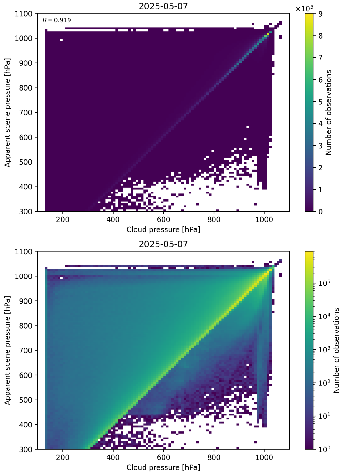
Figure 77: Scatter density plot of “Cloud pressure” against “Apparent scene pressure” for 2025-05-06 to 2025-05-08.
