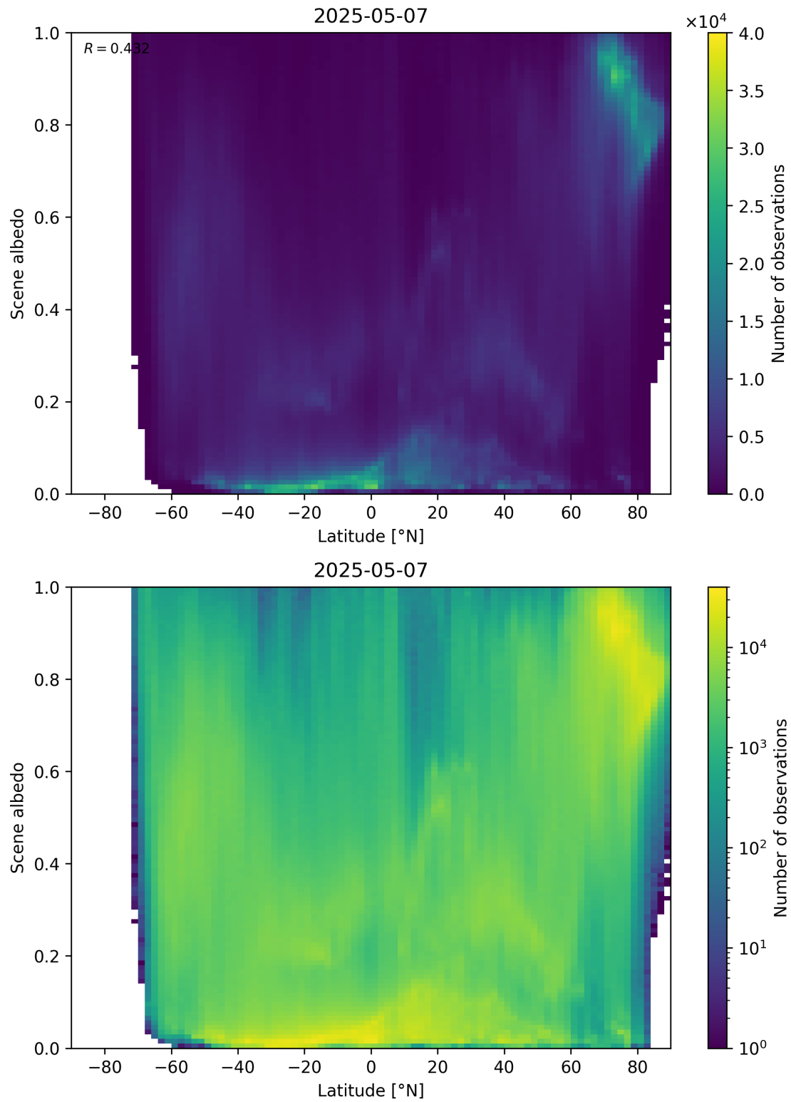
Figure 95: Scatter density plot of “Latitude” against “Scene albedo” for 2025-05-06 to 2025-05-08.
