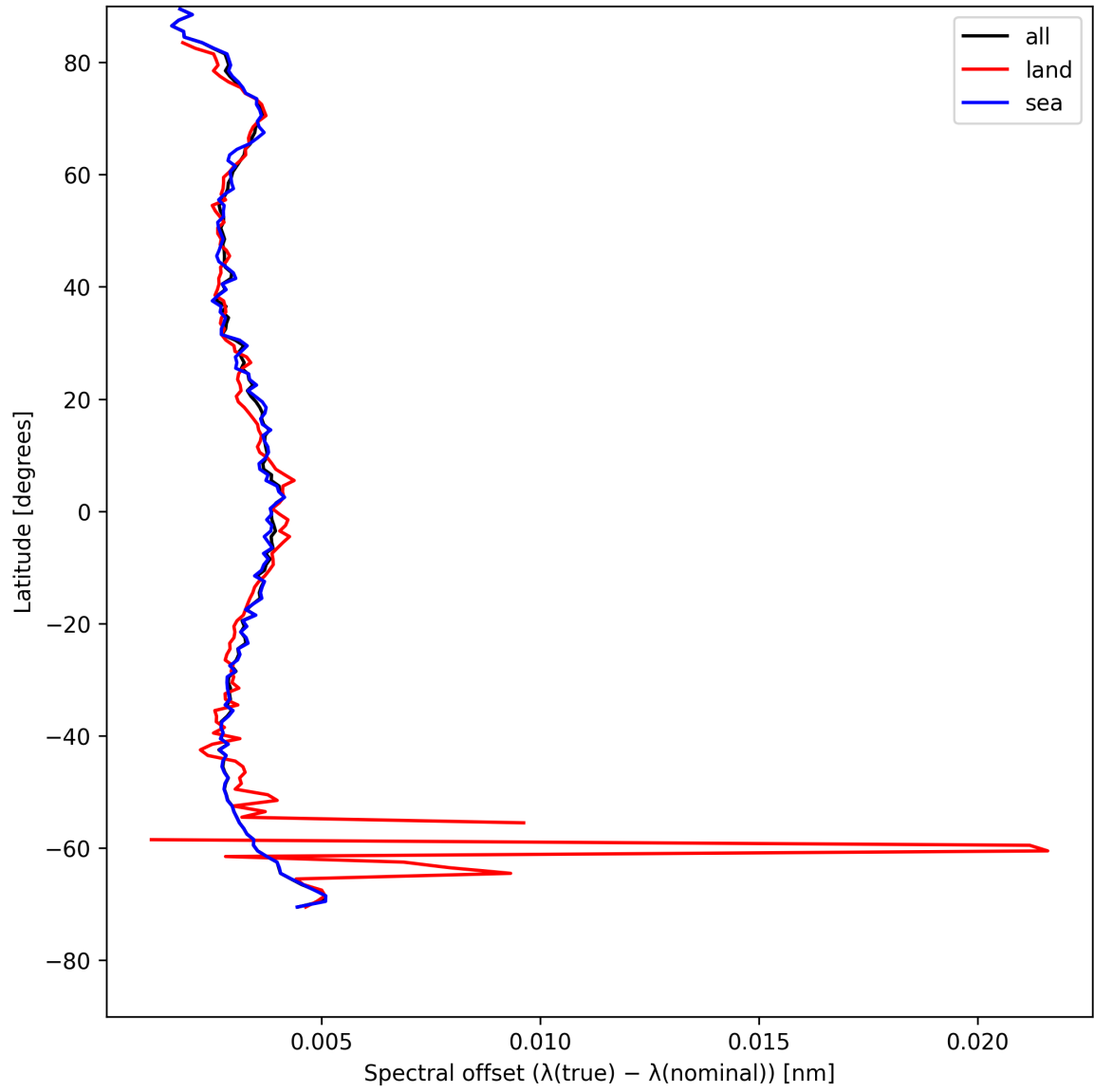
Figure 28: Zonal average of “Spectral offset ( \lambda_{\text{true}} - \lambda_{\text{nominal}} )” for 2025-05-06 to 2025-05-08.
