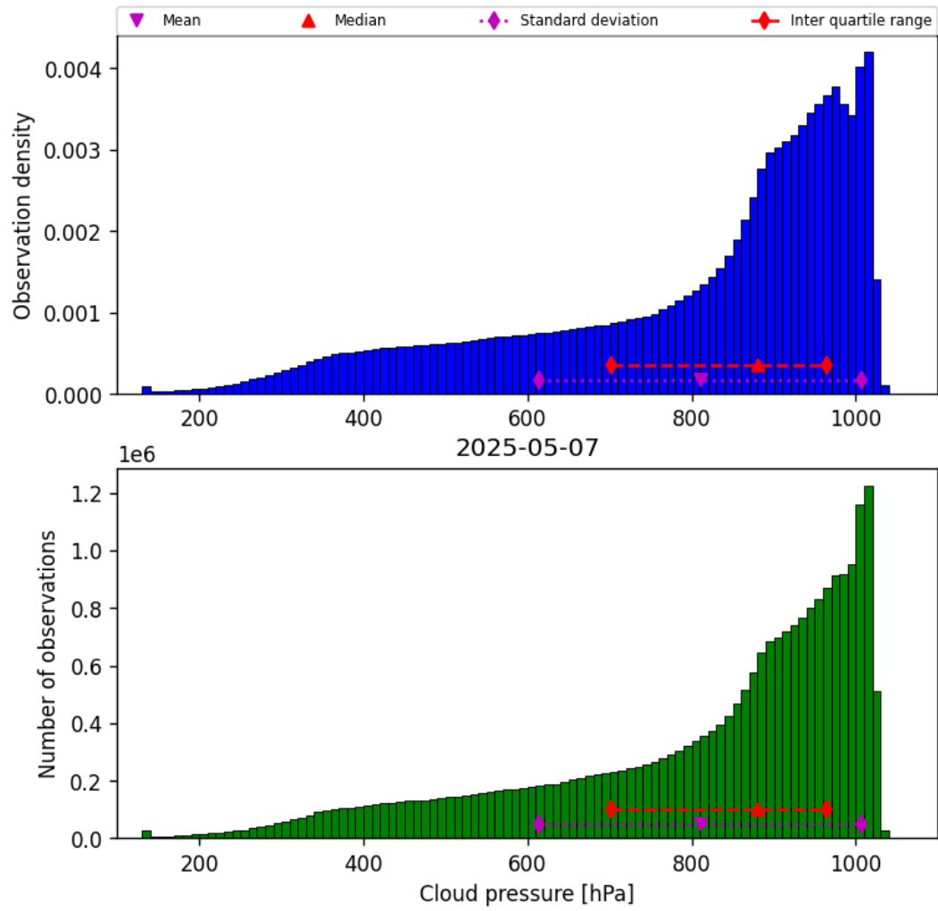
Figure 30: Histogram of “Cloud pressure” for 2025-05-06 to 2025-05-08
