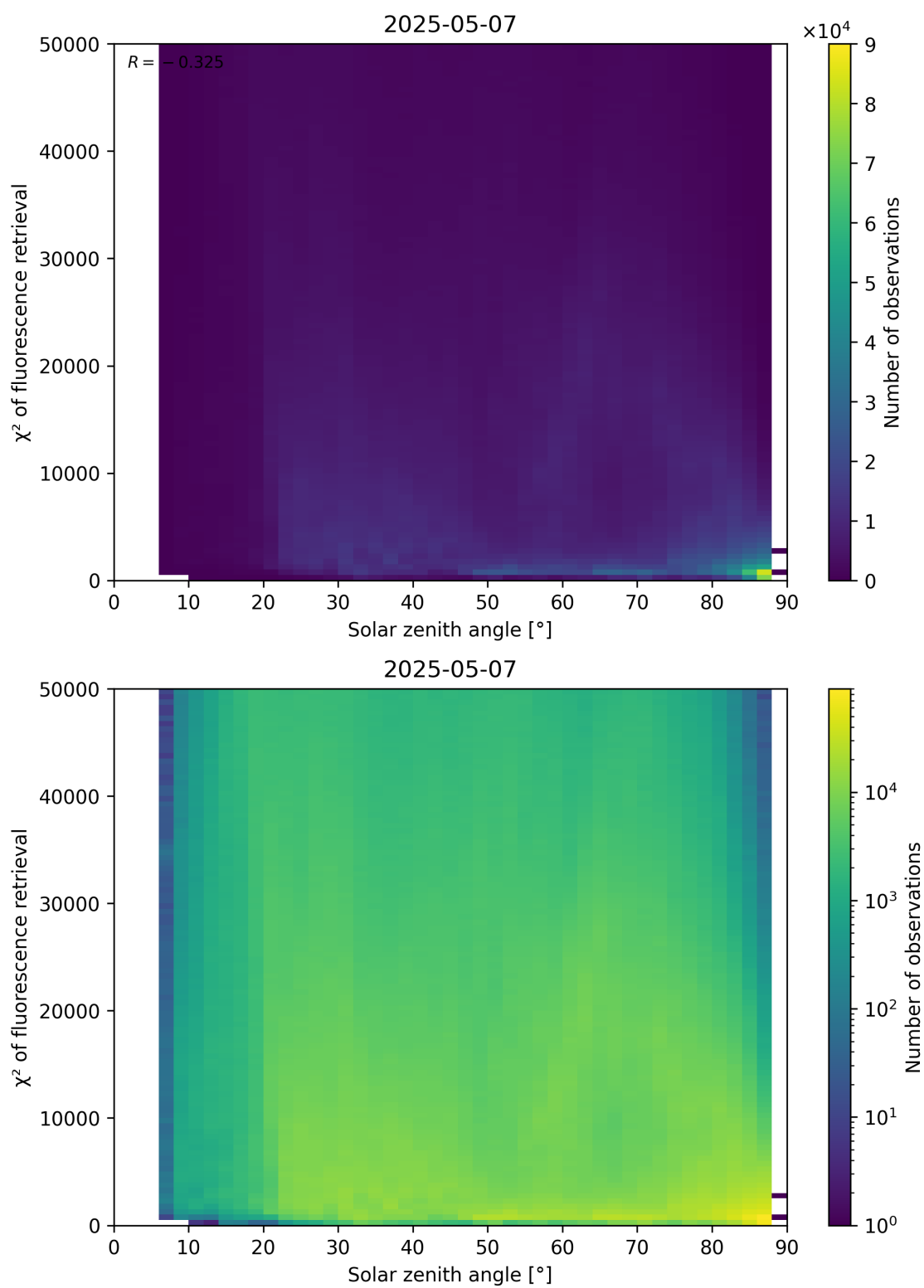
Figure 109: Scatter density plot of “Solar zenith angle” against “ \chi^2 of fluorescence retrieval” for 2025-05-06 to 2025-05-08.
