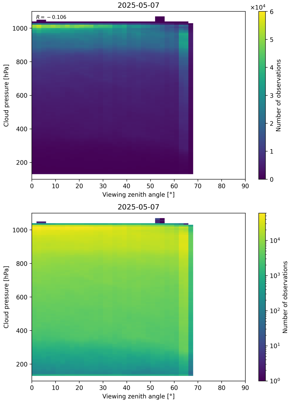
Figure 121: Scatter density plot of “Viewing zenith angle” against “Cloud pressure” for 2025-05-06 to 2025-05-08.
