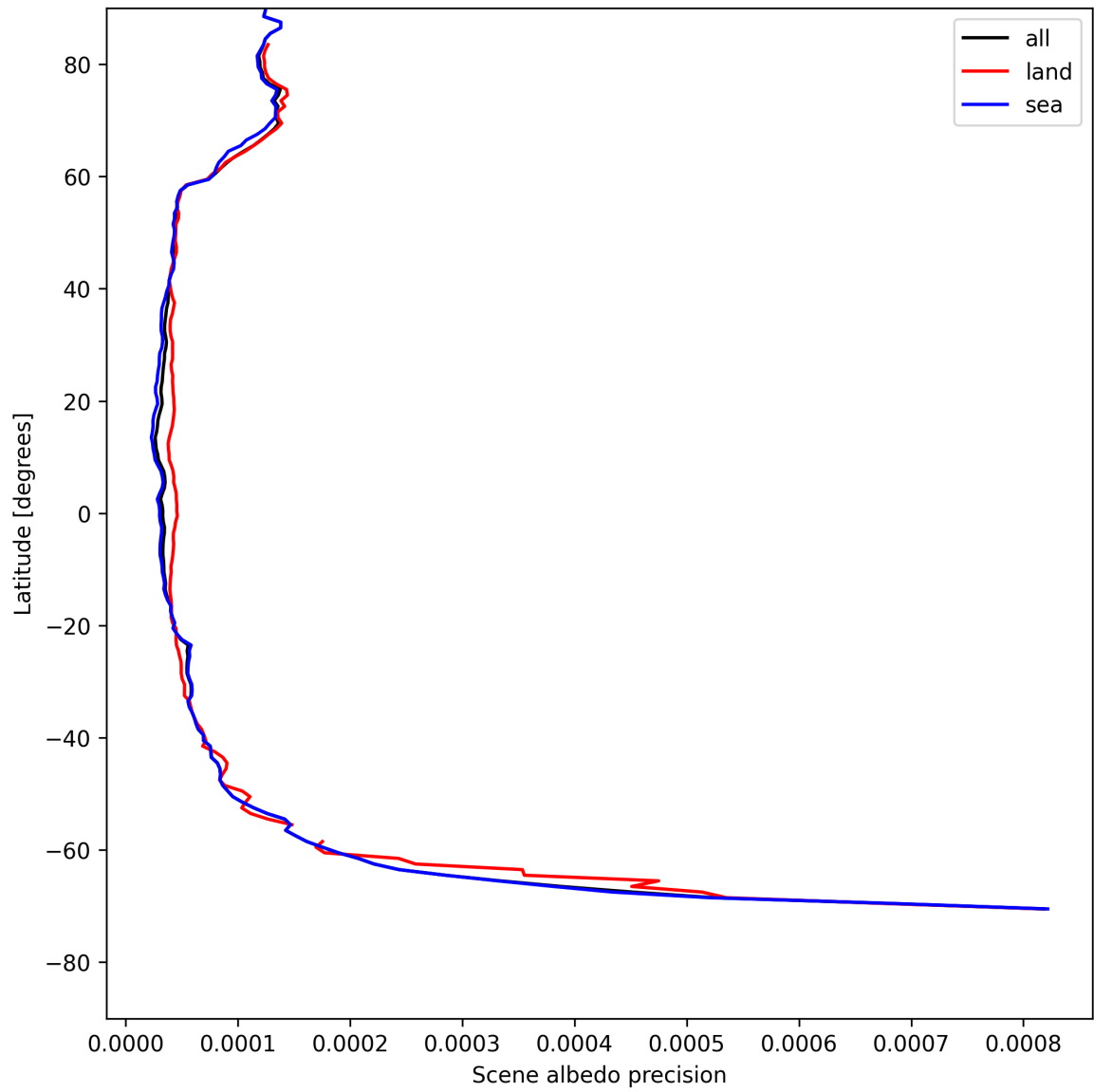
Figure 18: Zonal average of “Scene albedo precision” for 2025-05-06 to 2025-05-08.
