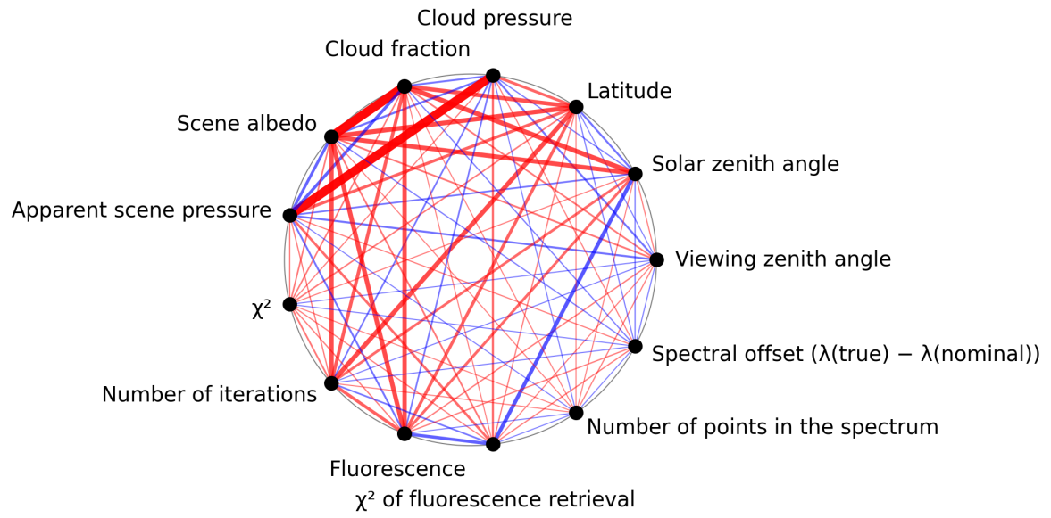
Figure 1: Map of correlation graph for 2025-05-06 to 2025-05-08.
