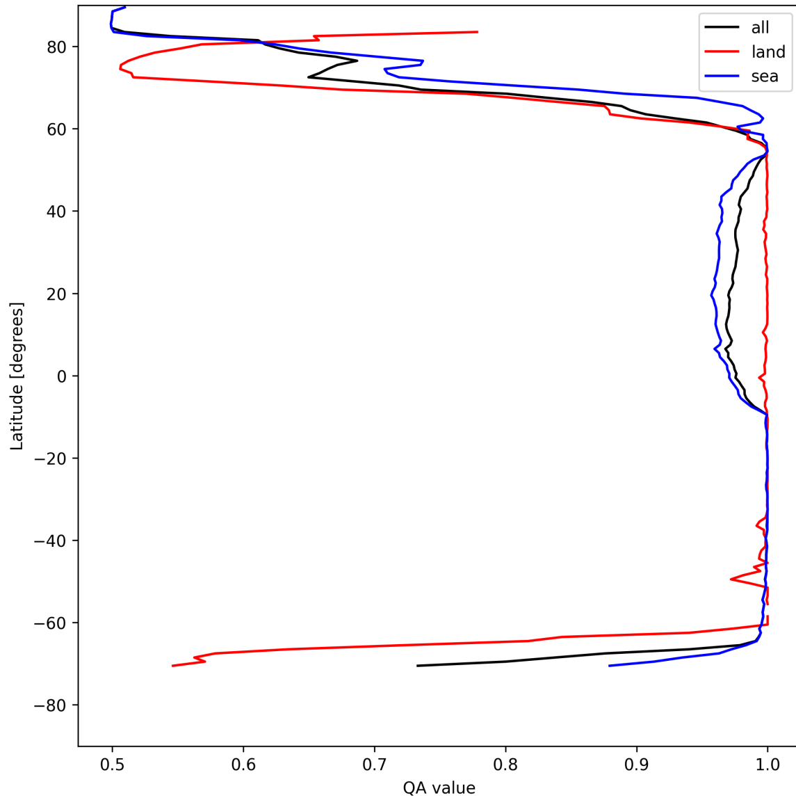
Figure 12: Zonal average of “QA value” for 2025-05-06 to 2025-05-08.
