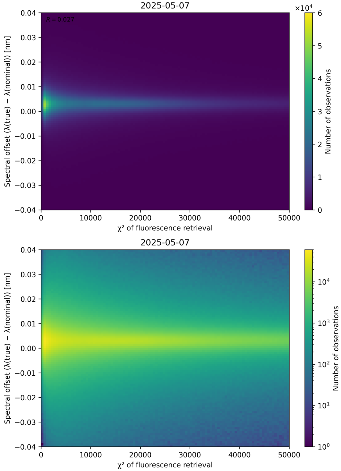
Figure 69: Scatter density plot of “ \chi^2 of fluorescence retrieval” against “Spectral offset ( \lambda_{\text{true}} - \lambda_{\text{nominal}} )” for 2025-05-06 to 2025-05-08.
