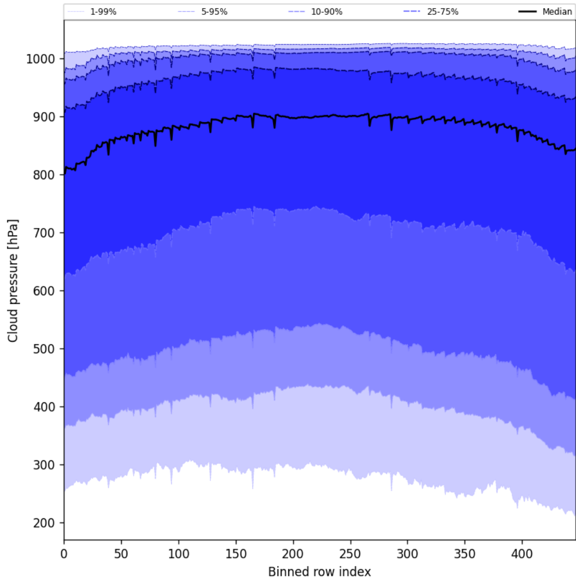
Figure 47: Along track statistics of “Cloud pressure” for 2025-05-06 to 2025-05-08
