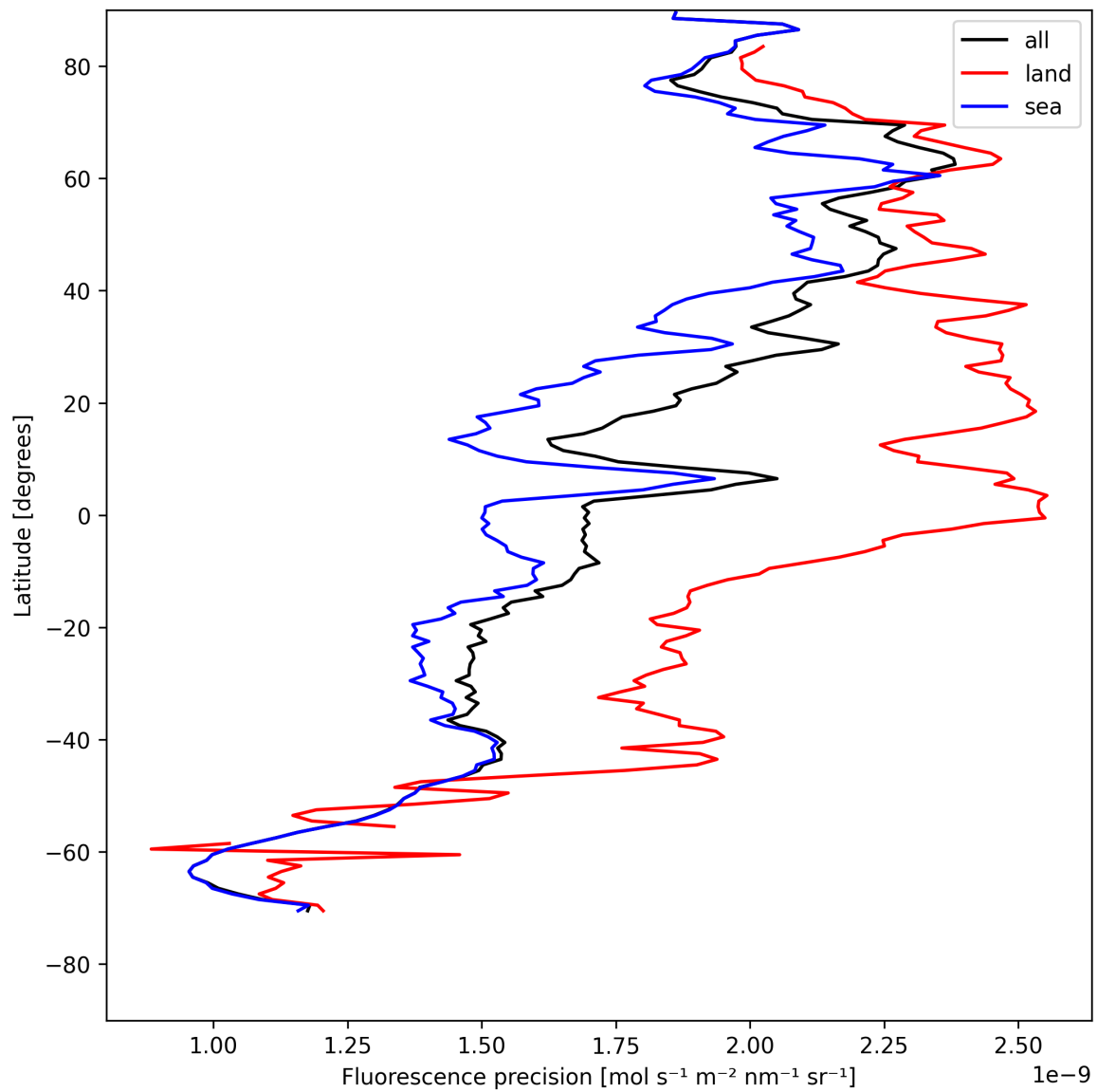
Figure 24: Zonal average of “Fluorescence precision” for 2025-05-06 to 2025-05-08.
