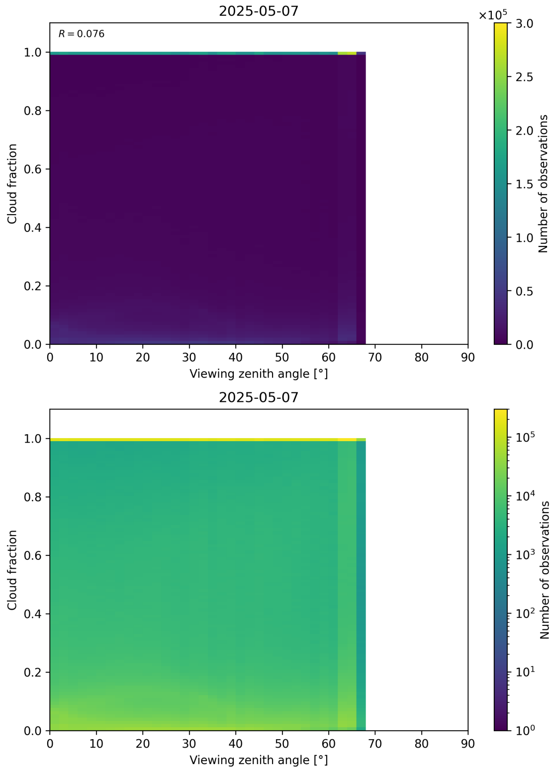
Figure 120: Scatter density plot of “Viewing zenith angle” against “Cloud fraction” for 2025-05-06 to 2025-05-08.
