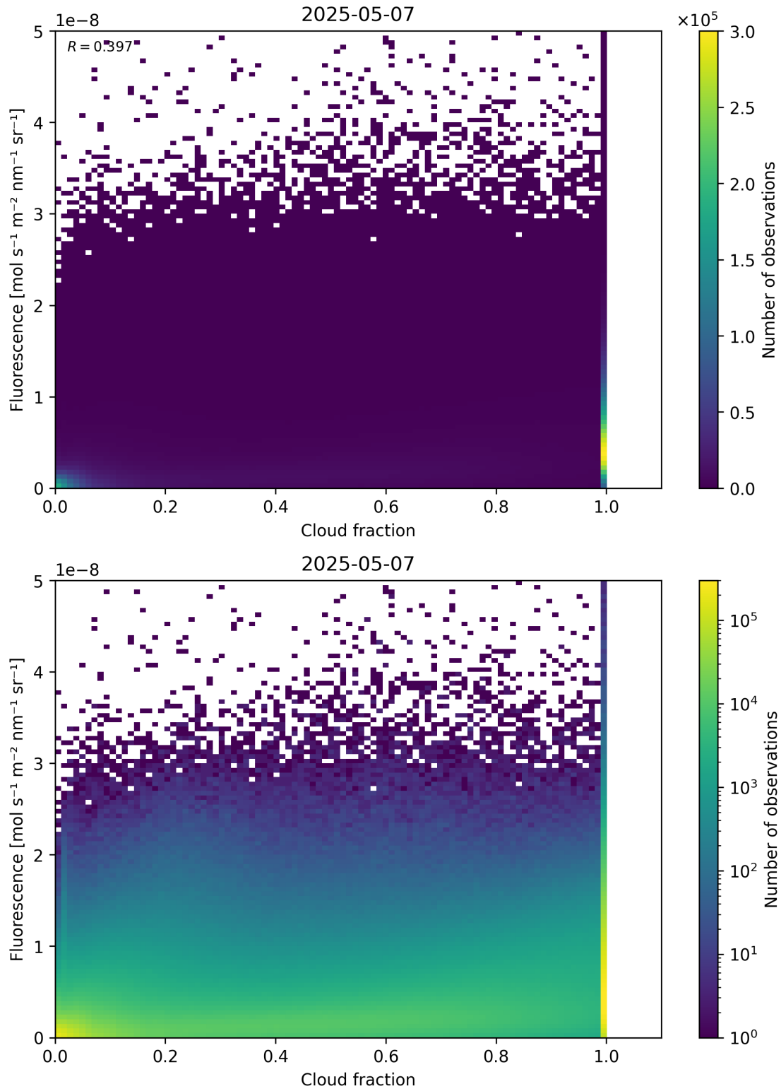
Figure 72: Scatter density plot of “Cloud fraction” against “Fluorescence” for 2025-05-06 to 2025-05-08.
