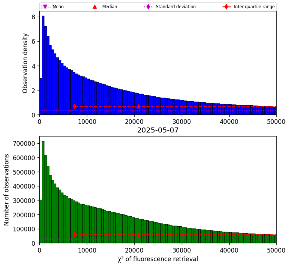
Figure 42: Histogram of “ \chi^2 of fluorescence retrieval” for 2025-05-06 to 2025-05-08
