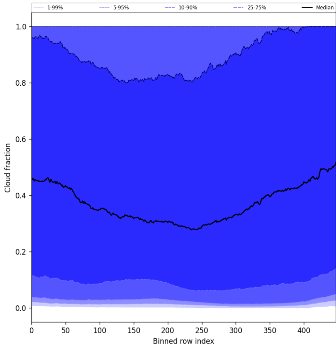
Figure 49: Along track statistics of “Cloud fraction” for 2025-05-06 to 2025-05-08
