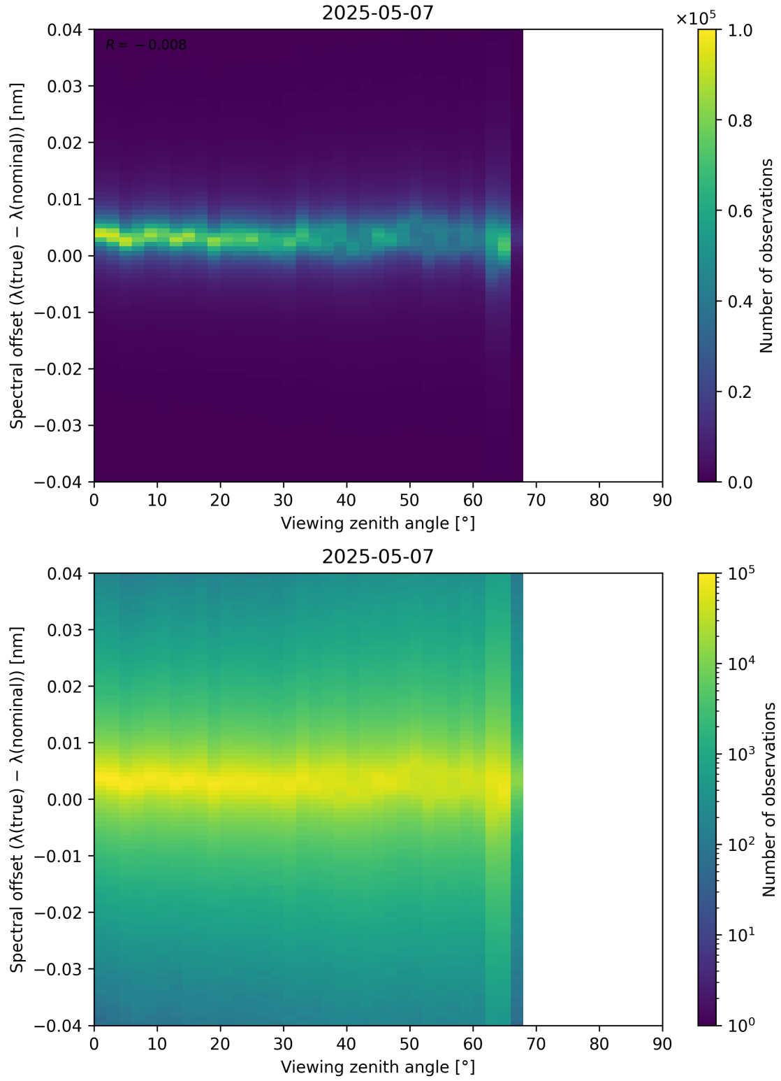
Figure 128: Scatter density plot of “Viewing zenith angle” against “Spectral offset ( \lambda_{\text{true}} - \lambda_{\text{nominal}} )” for 2025-05-06 to 2025-05-08.
