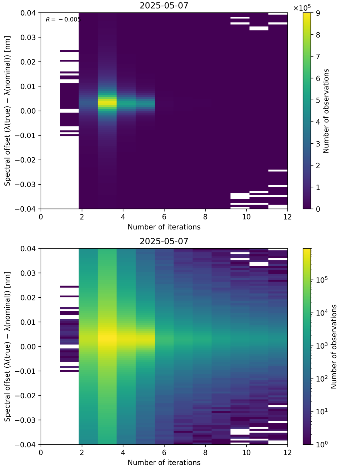
Figure 100: Scatter density plot of “Number of iterations” against “Spectral offset ( \lambda_{\text{true}} - \lambda_{\text{nominal}} )” for 2025-05-06 to 2025-05-08.
