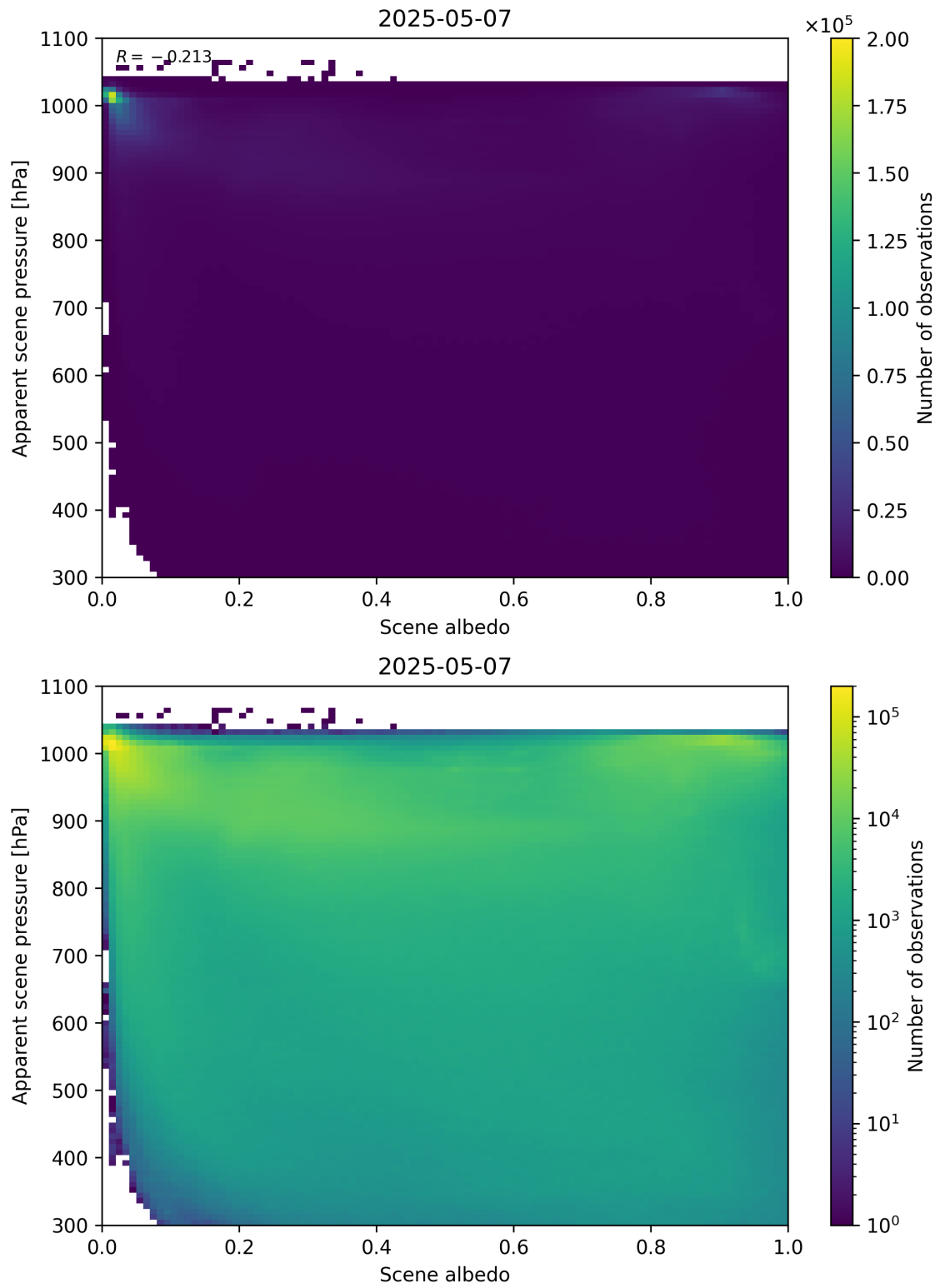
Figure 102: Scatter density plot of “Scene albedo” against “Apparent scene pressure” for 2025-05-06 to 2025-05-08.
