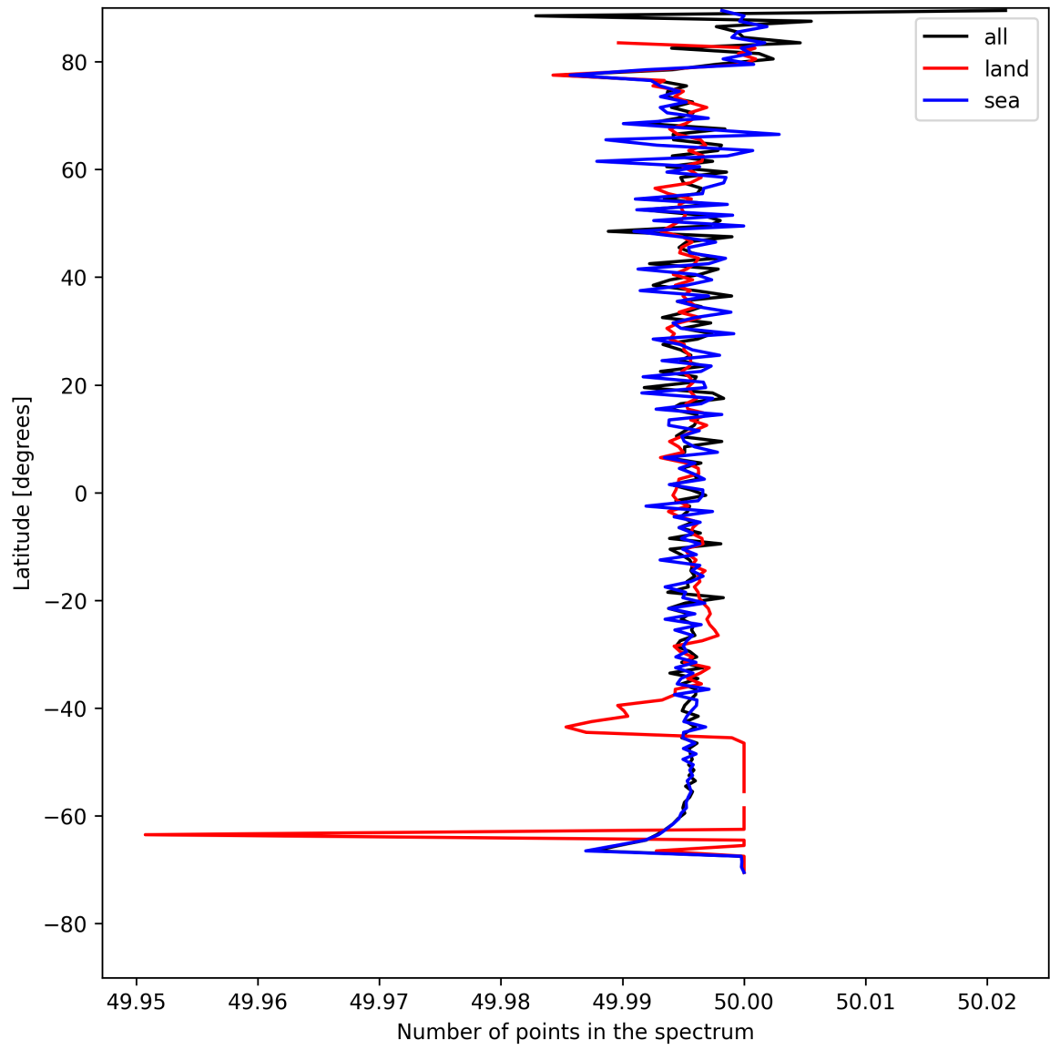
Figure 27: Zonal average of “Number of points in the spectrum” for 2025-05-06 to 2025-05-08.
