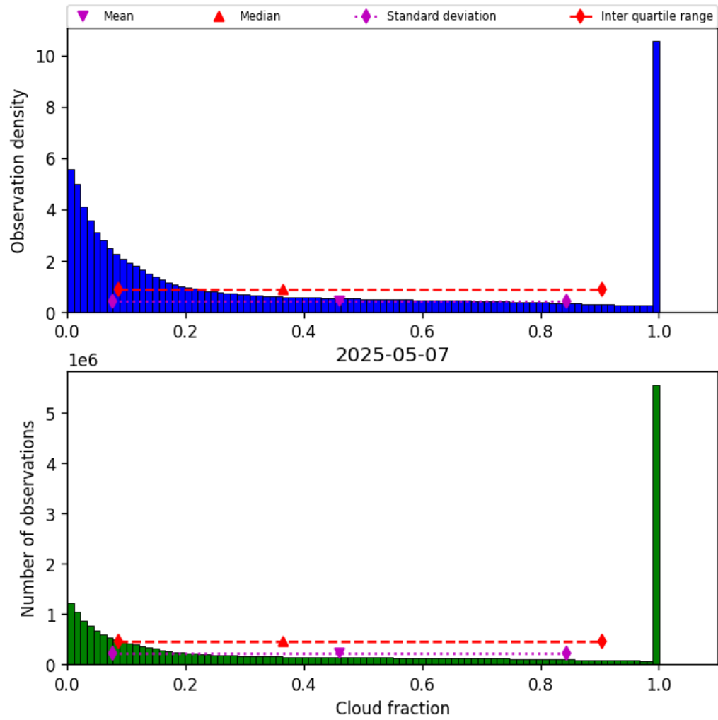
Figure 32: Histogram of “Cloud fraction” for 2025-05-06 to 2025-05-08
