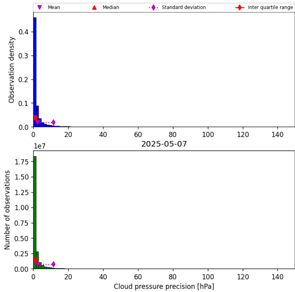
Figure 31: Histogram of “Cloud pressure precision” for 2025-05-06 to 2025-05-08
