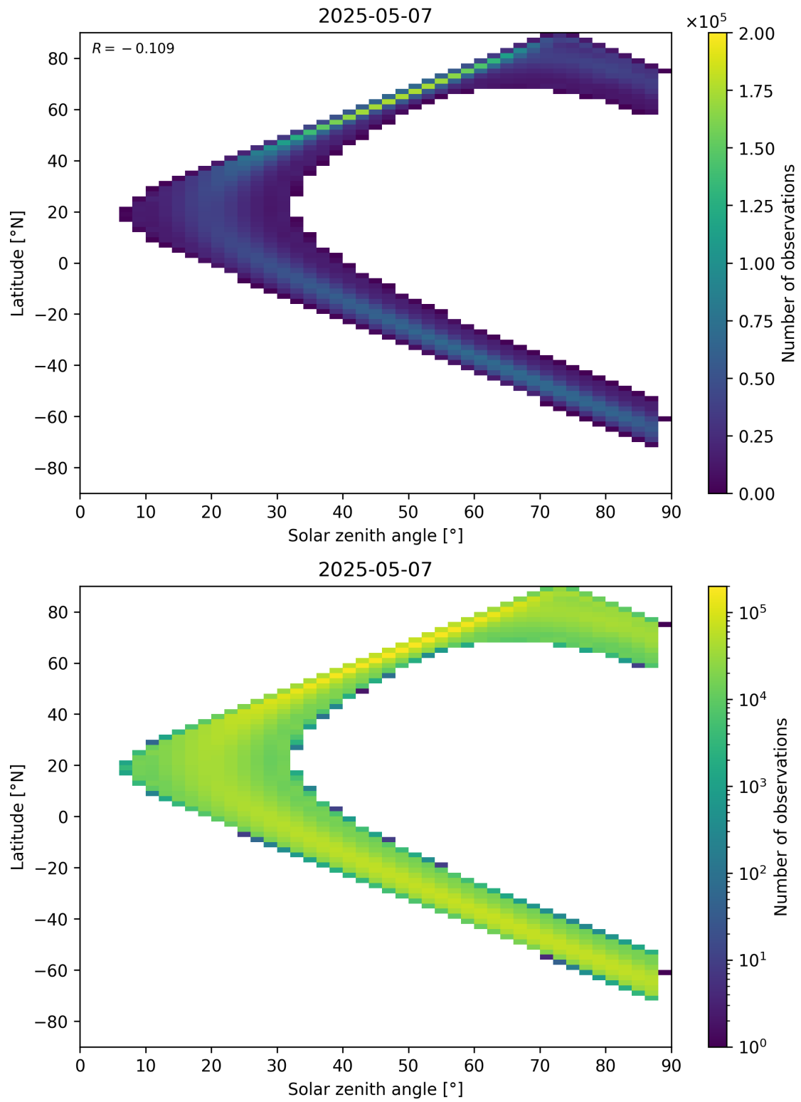
Figure 113: Scatter density plot of “Solar zenith angle” against “Latitude” for 2025-05-06 to 2025-05-08.
