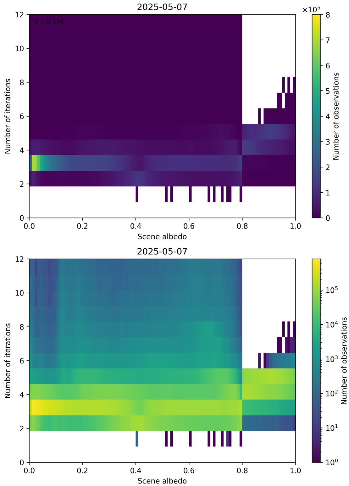
Figure 105: Scatter density plot of “Scene albedo” against “Number of iterations” for 2025-05-06 to 2025-05-08.
