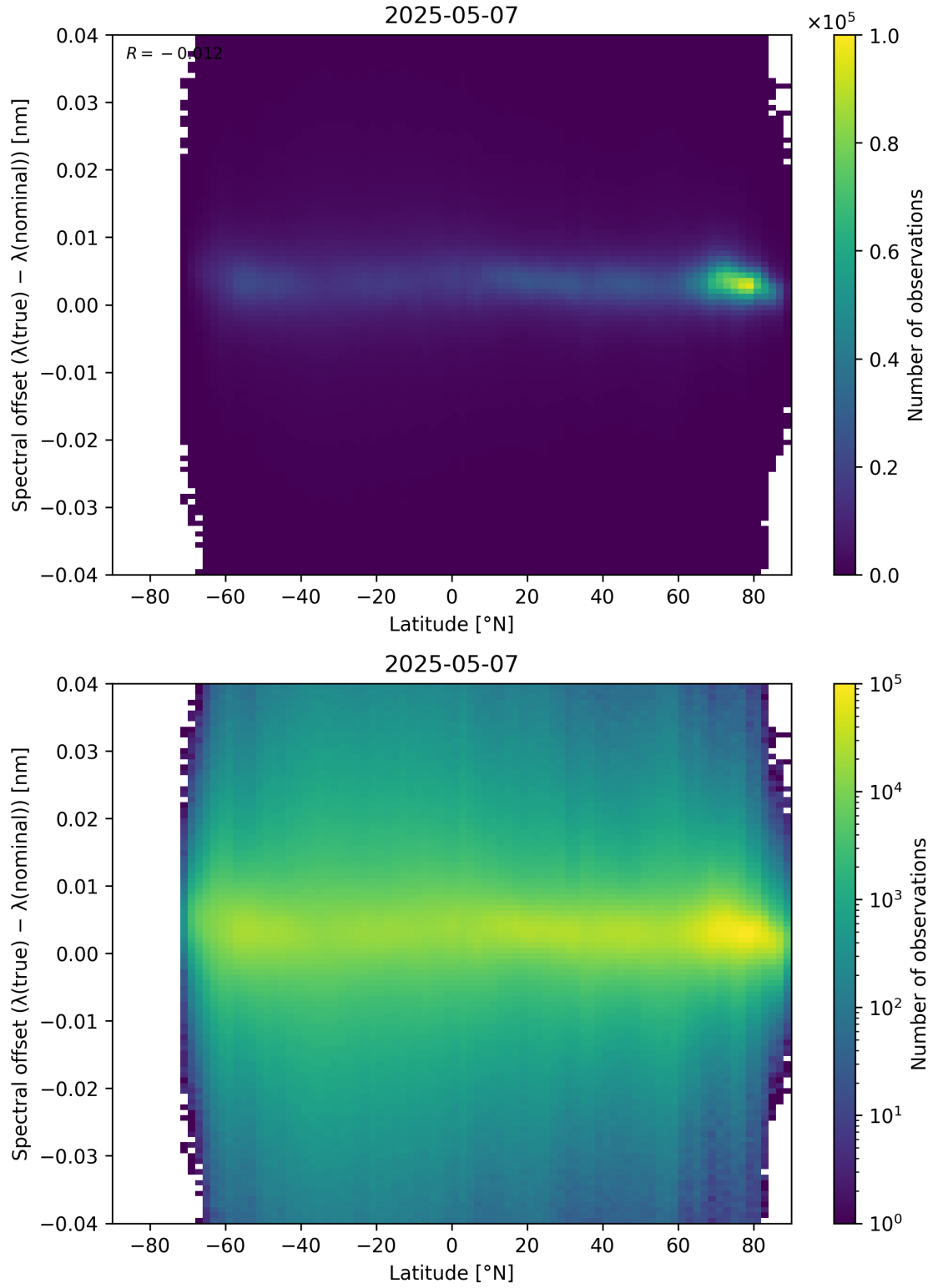
Figure 96: Scatter density plot of “Latitude” against “Spectral offset ( \lambda_{\text{true}} - \lambda_{\text{nominal}} )” for 2025-05-06 to 2025-05-08.
