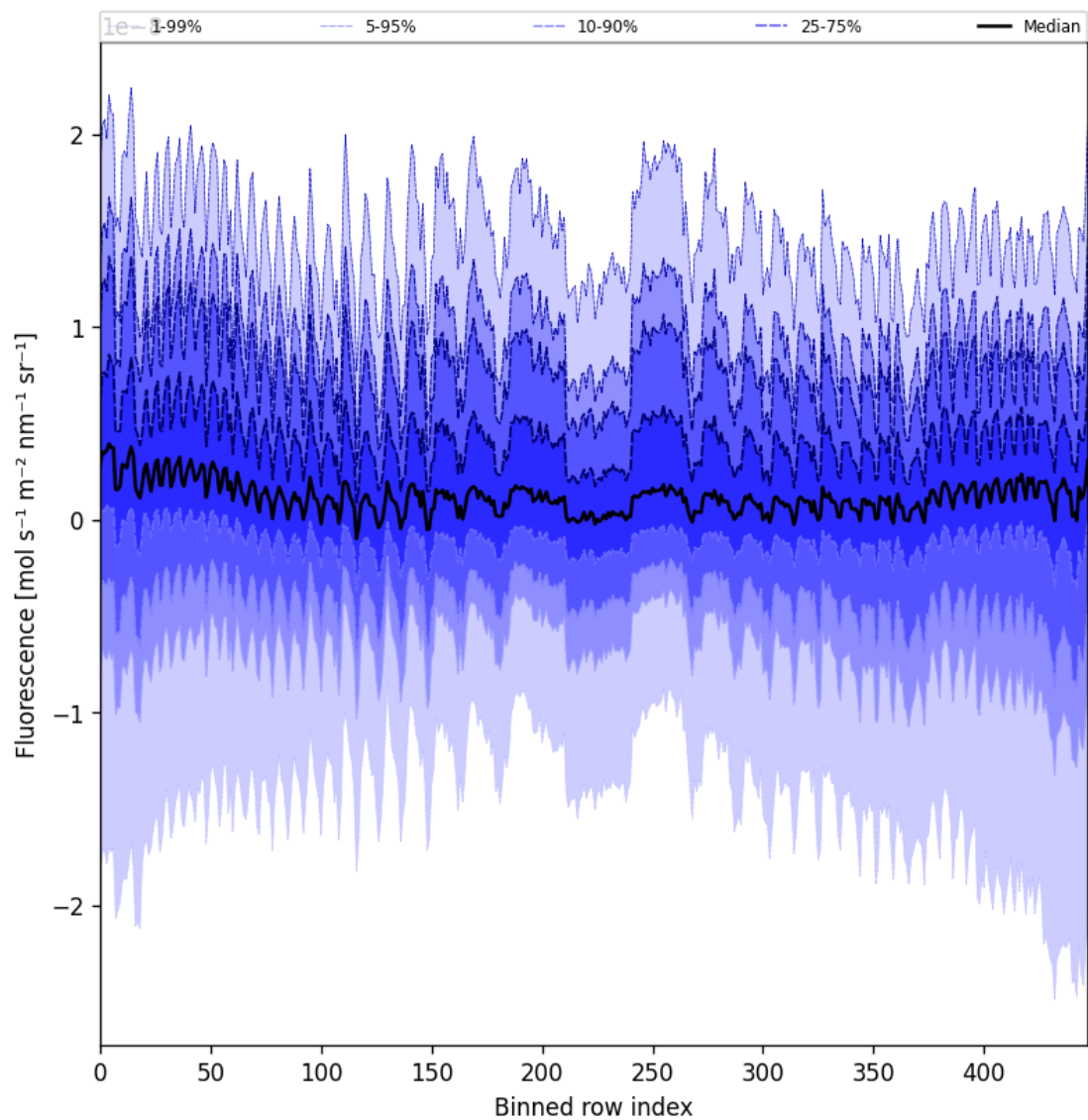
Figure 57: Along track statistics of “Fluorescence” for 2025-05-06 to 2025-05-08
