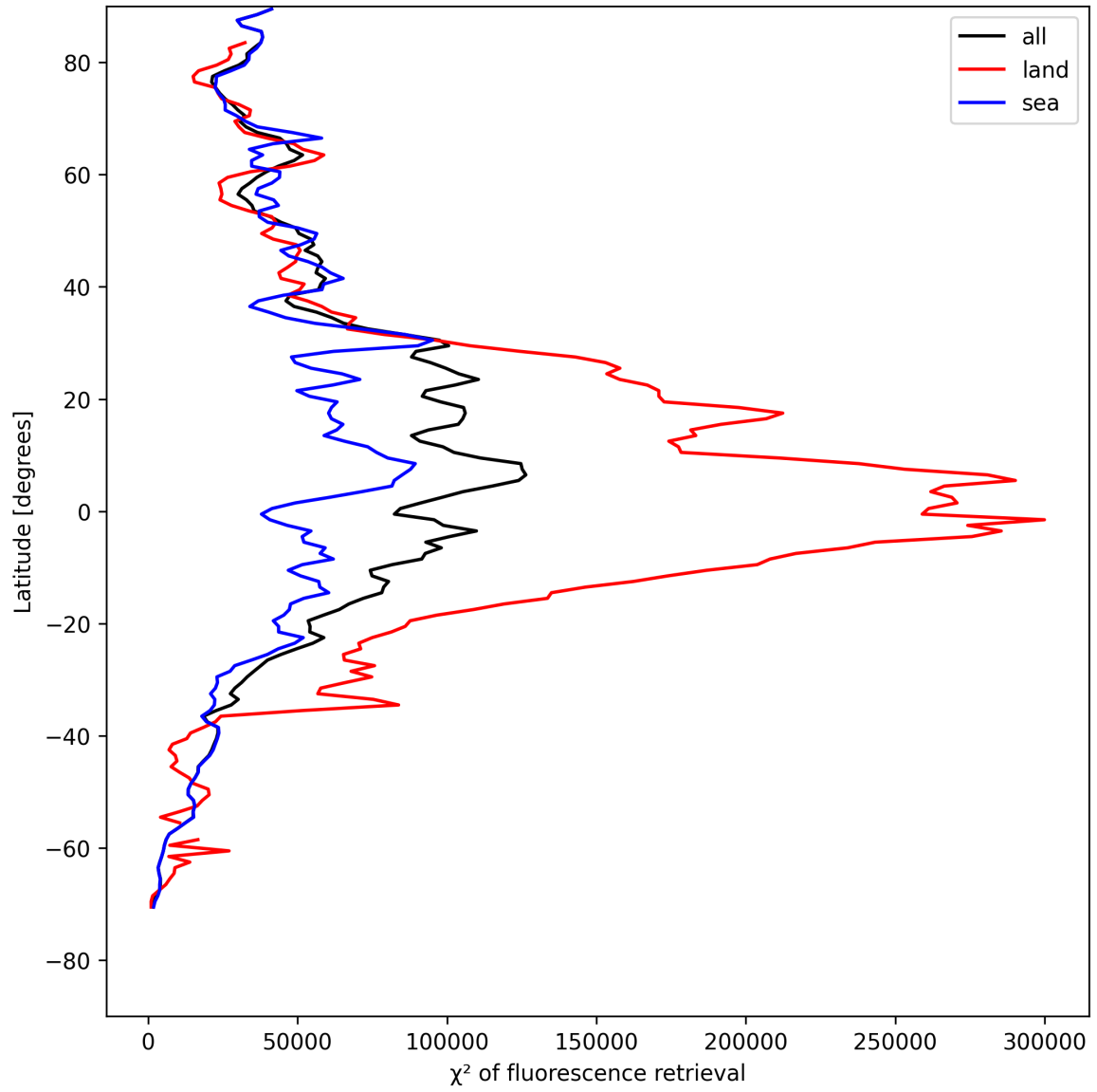
Figure 25: Zonal average of “ \chi^2 of fluorescence retrieval” for 2025-05-06 to 2025-05-08.
