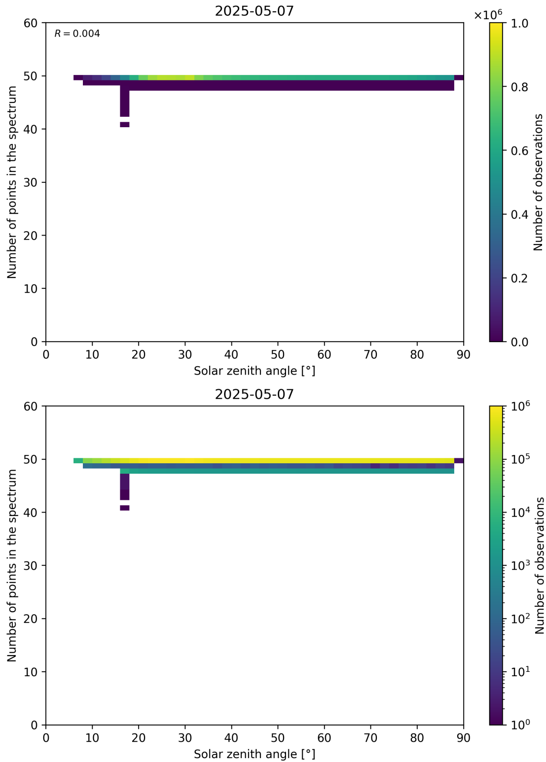
Figure 115: Scatter density plot of “Solar zenith angle” against “Number of points in the spectrum” for 2025-05-06 to 2025-05-08.
