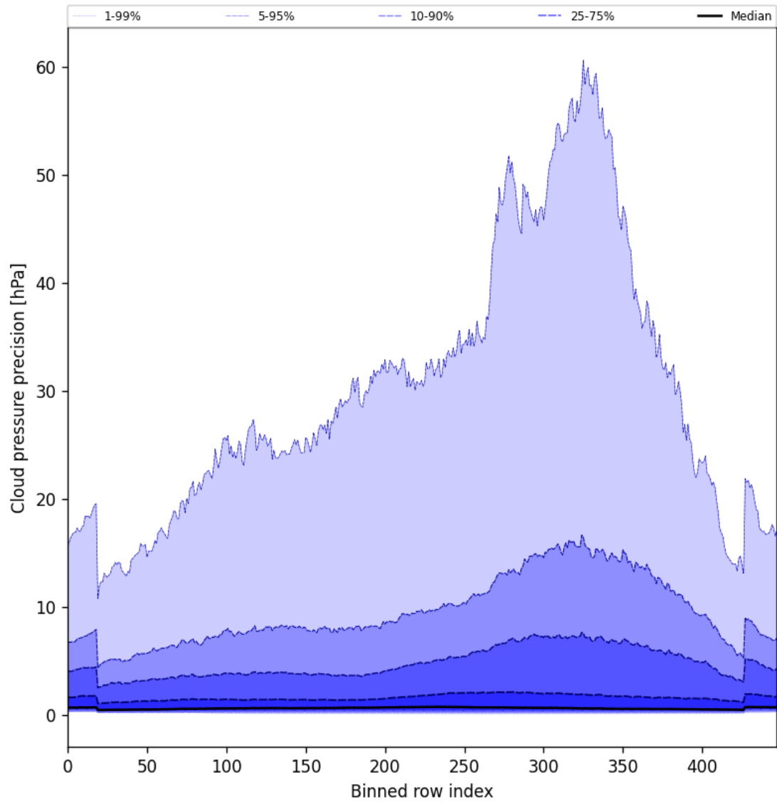
Figure 48: Along track statistics of “Cloud pressure precision” for 2025-05-06 to 2025-05-08
