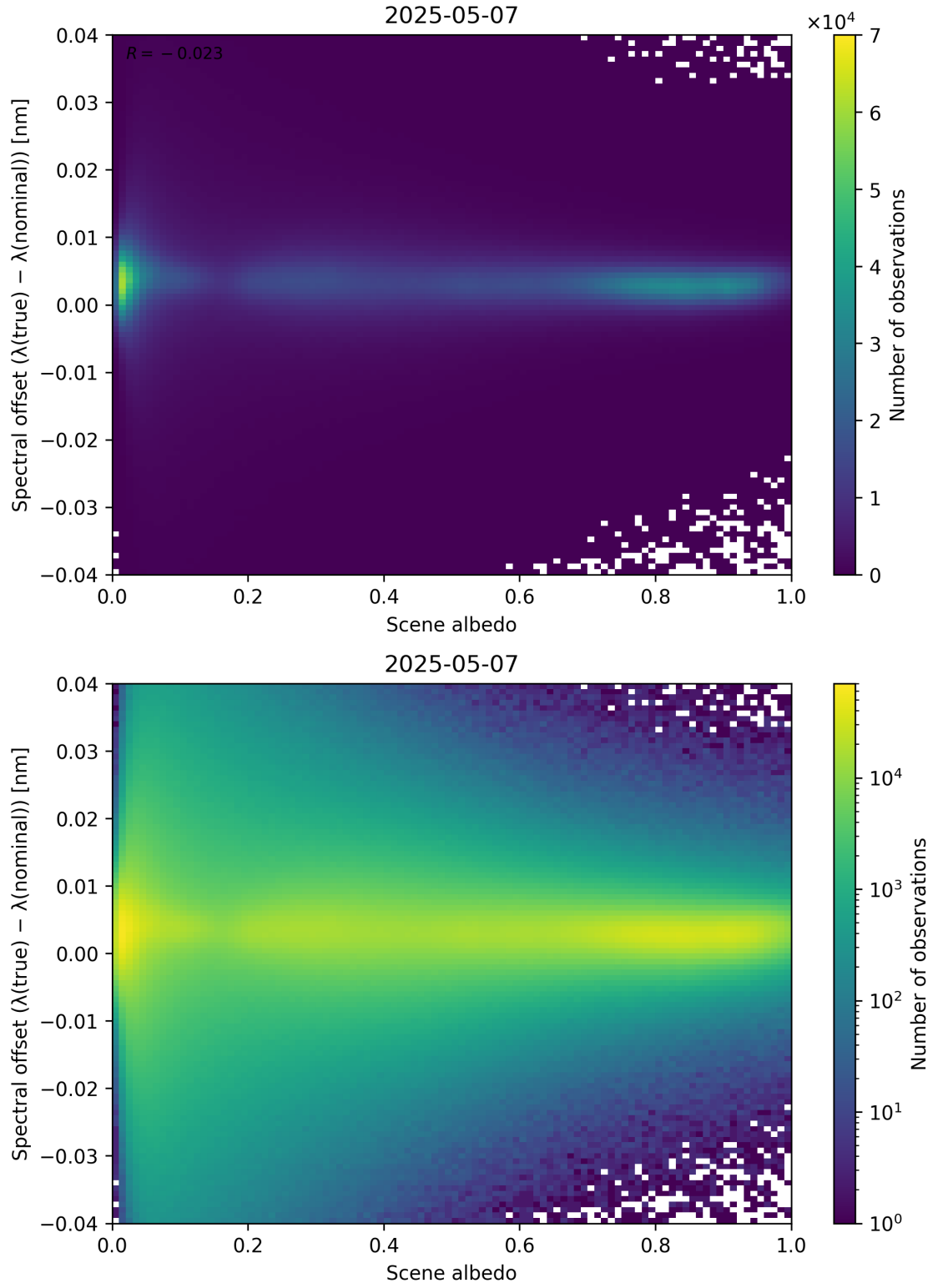
Figure 107: Scatter density plot of “Scene albedo” against “Spectral offset ( \lambda_{\text{true}} - \lambda_{\text{nominal}} )” for 2025-05-06 to 2025-05-08.
