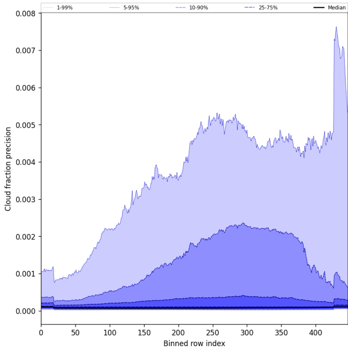
Figure 50: Along track statistics of “Cloud fraction precision” for 2025-05-06 to 2025-05-08
