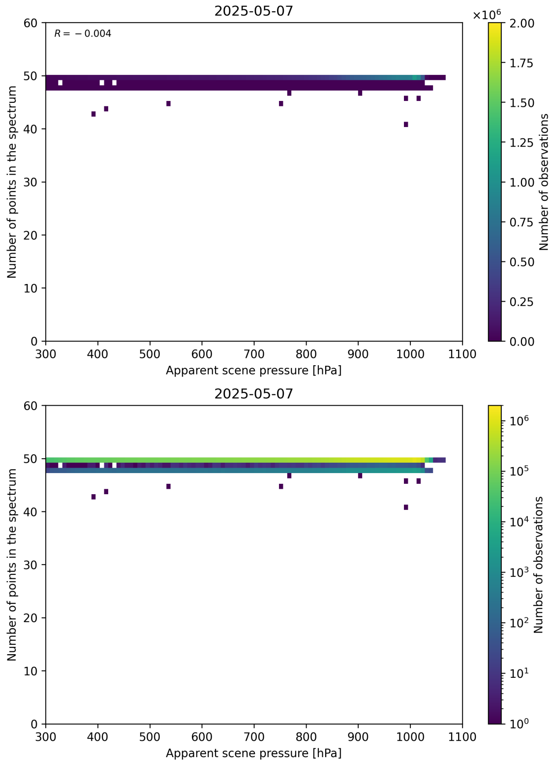
Figure 66: Scatter density plot of “Apparent scene pressure” against “Number of points in the spectrum” for 2025-05-06 to 2025-05-08.
