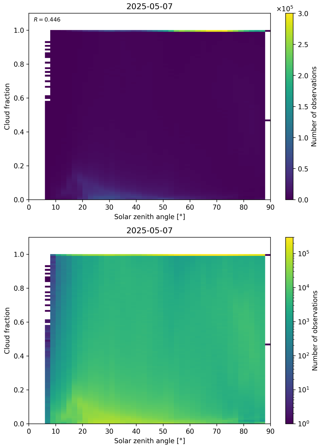
Figure 110: Scatter density plot of “Solar zenith angle” against “Cloud fraction” for 2025-05-06 to 2025-05-08.
