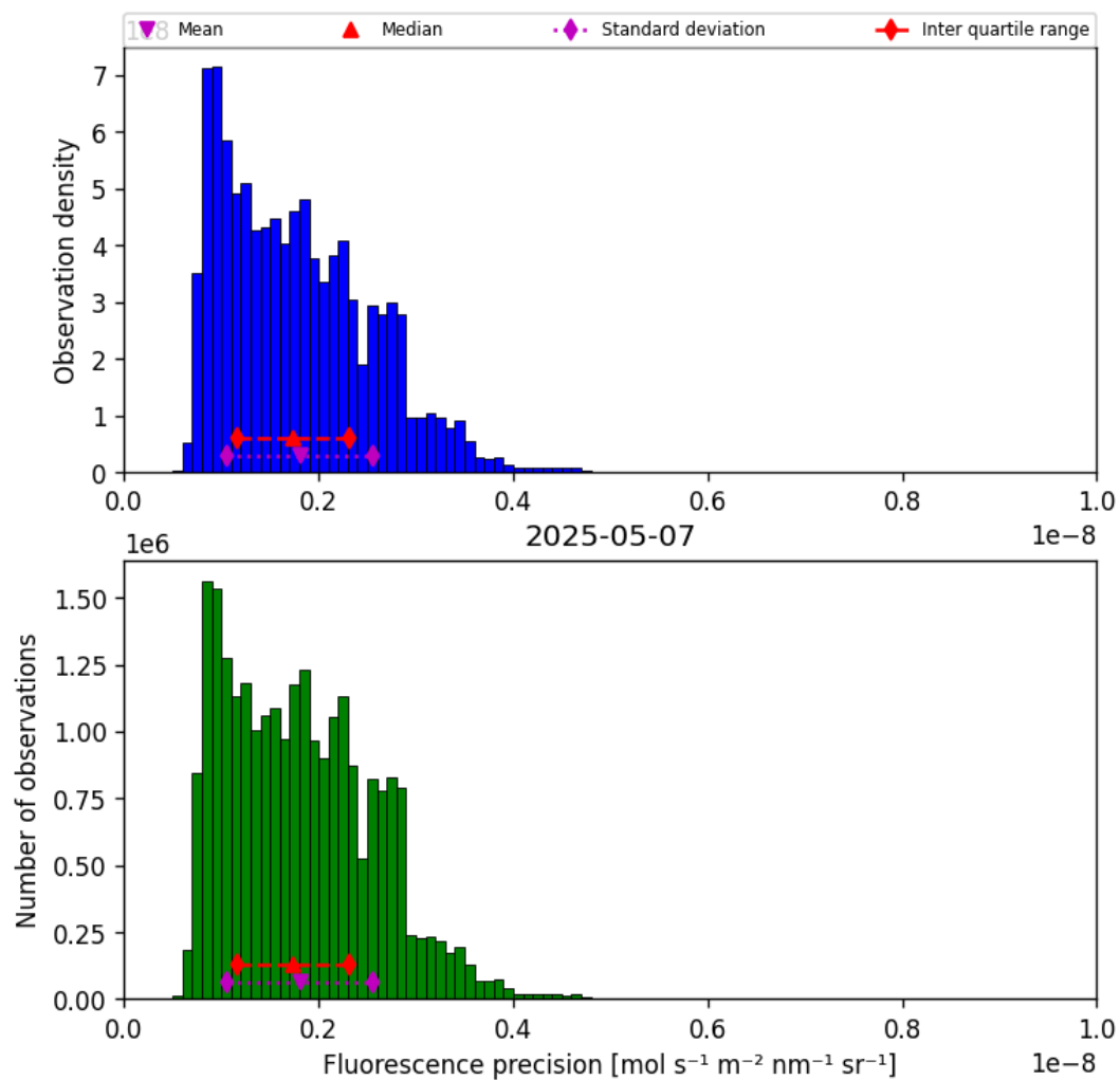
Figure 41: Histogram of “Fluorescence precision” for 2025-05-06 to 2025-05-08
