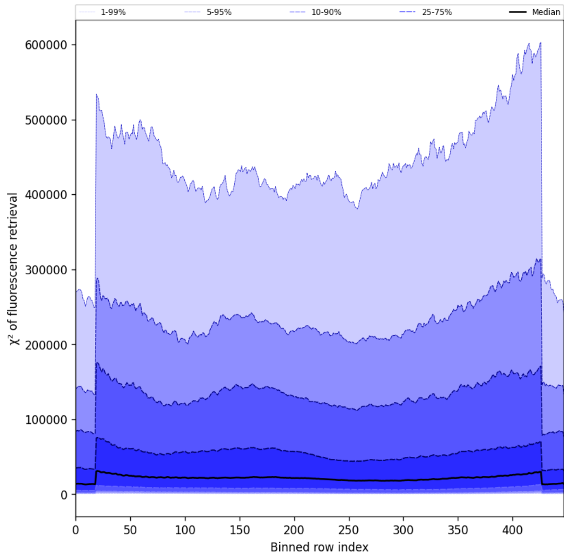
Figure 59: Along track statistics of “ \chi^2 of fluorescence retrieval” for 2025-05-06 to 2025-05-08
