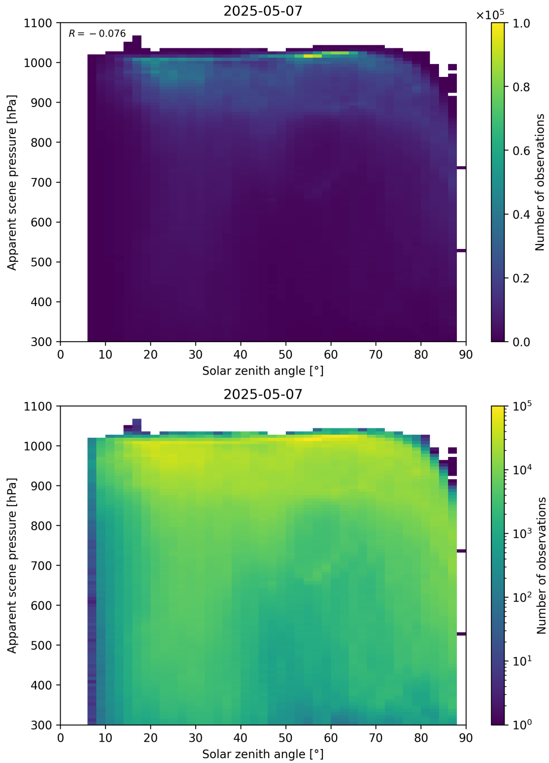
Figure 108: Scatter density plot of “Solar zenith angle” against “Apparent scene pressure” for 2025-05-06 to 2025-05-08.
