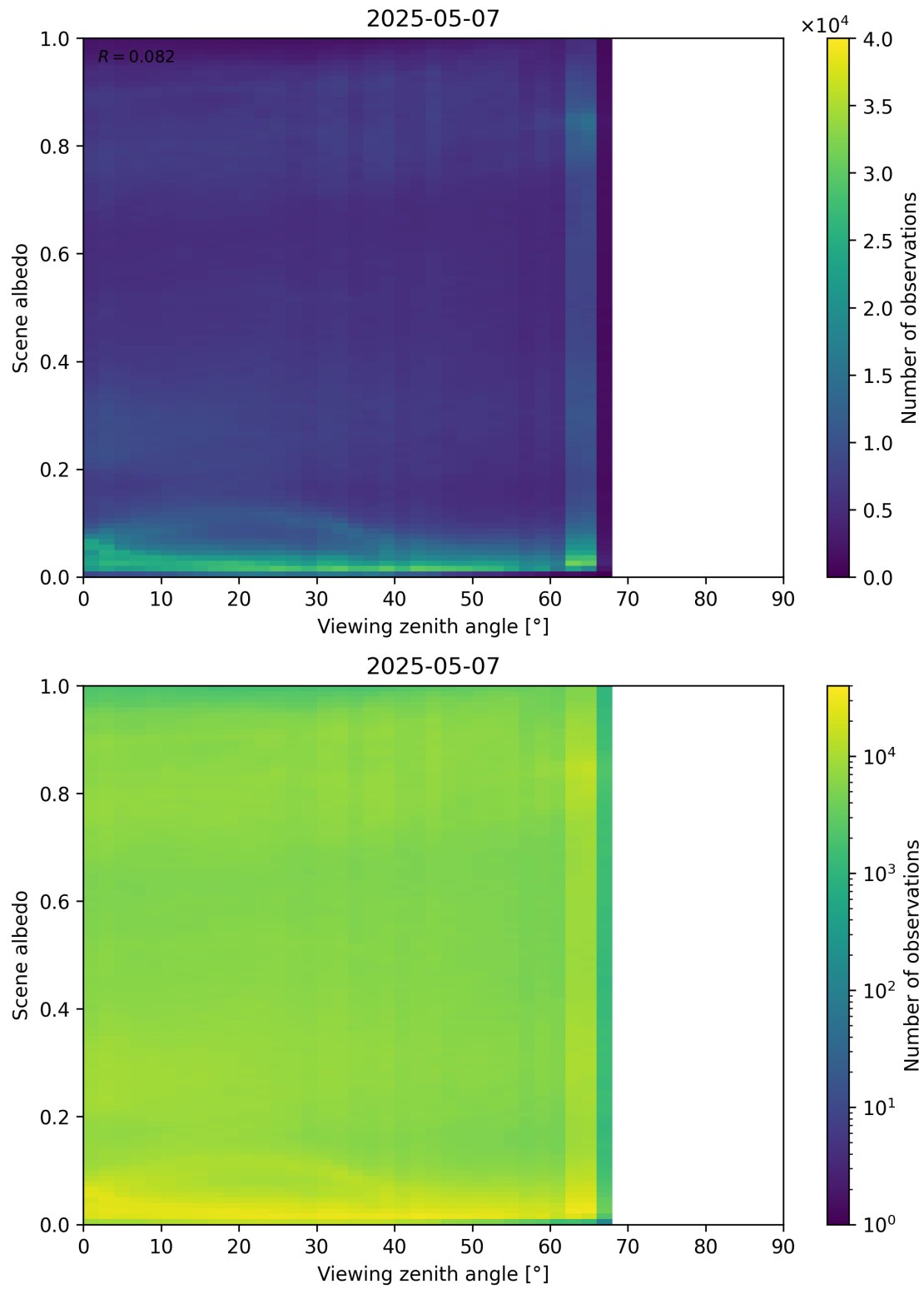
Figure 126: Scatter density plot of “Viewing zenith angle” against “Scene albedo” for 2025-05-06 to 2025-05-08.
