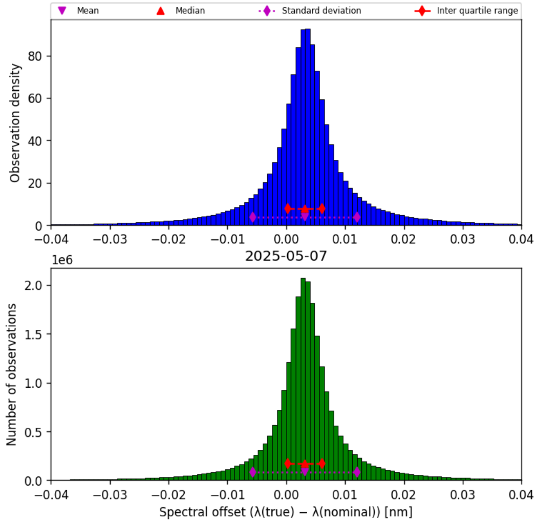
Figure 45: Histogram of “Spectral offset ( \lambda_{\text{true}} - \lambda_{\text{nominal}} )” for 2025-05-06 to 2025-05-08
