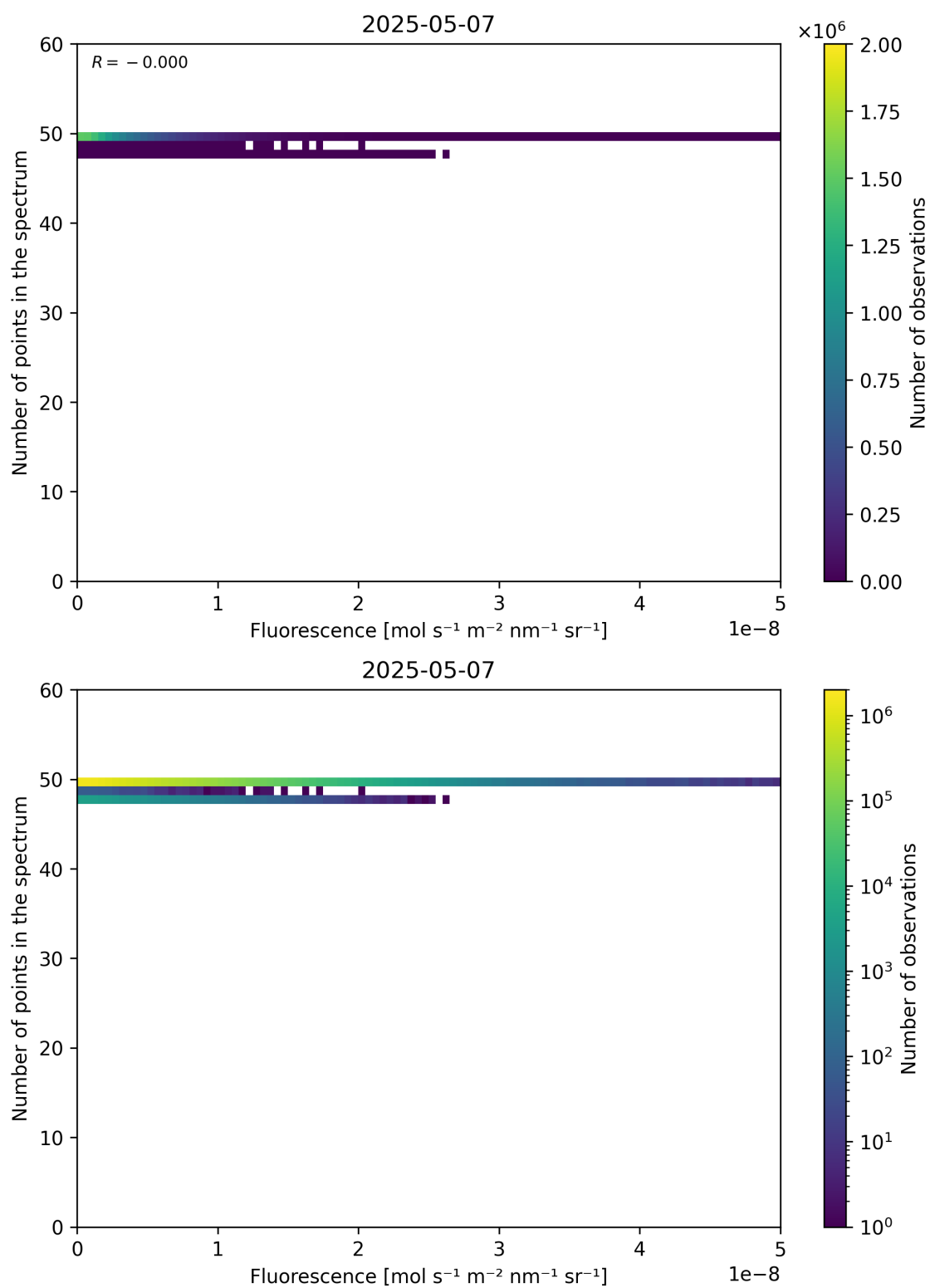
Figure 86: Scatter density plot of “Fluorescence” against “Number of points in the spectrum” for 2025-05-06 to 2025-05-08.
