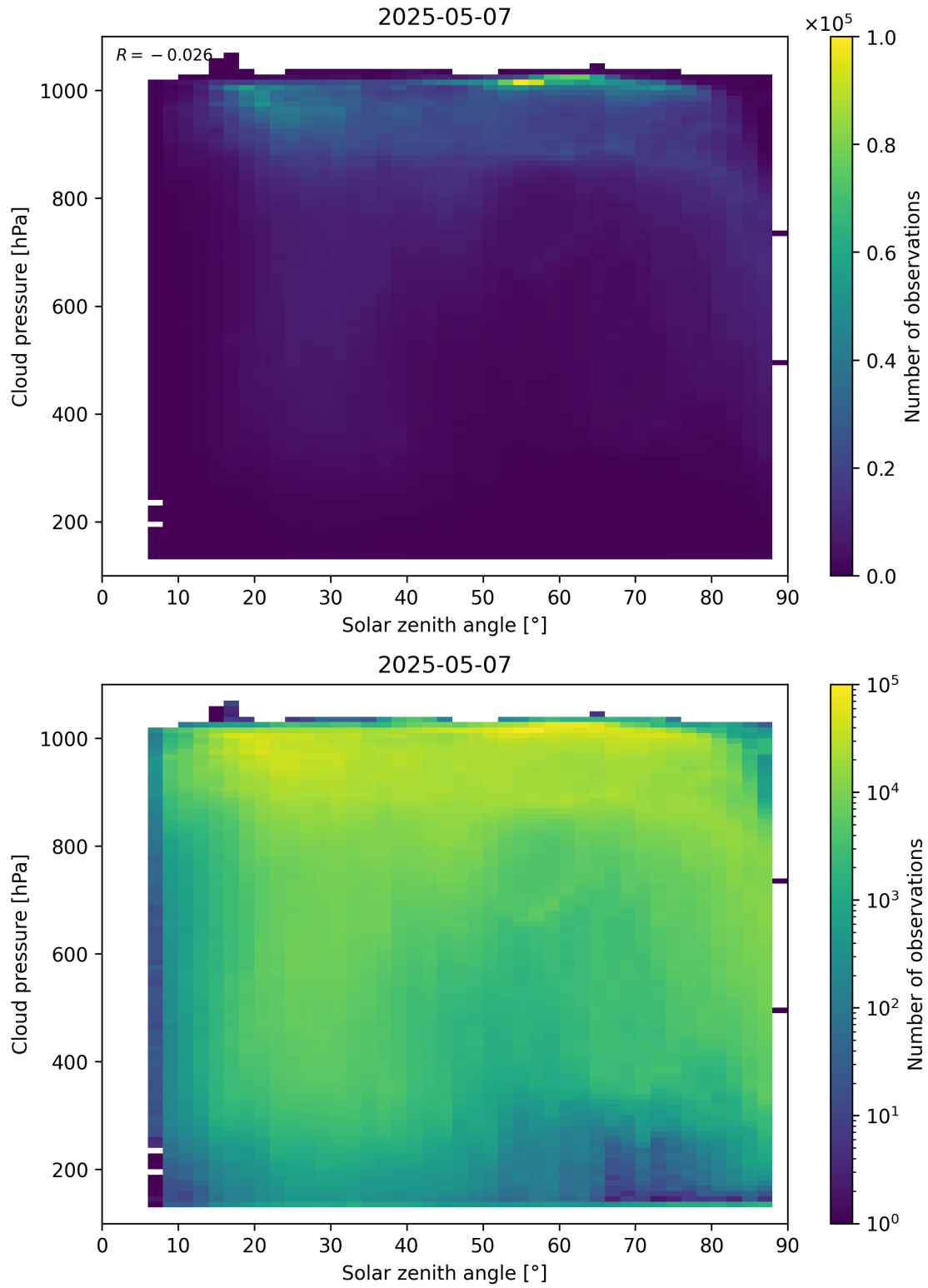
Figure 111: Scatter density plot of “Solar zenith angle” against “Cloud pressure” for 2025-05-06 to 2025-05-08.
