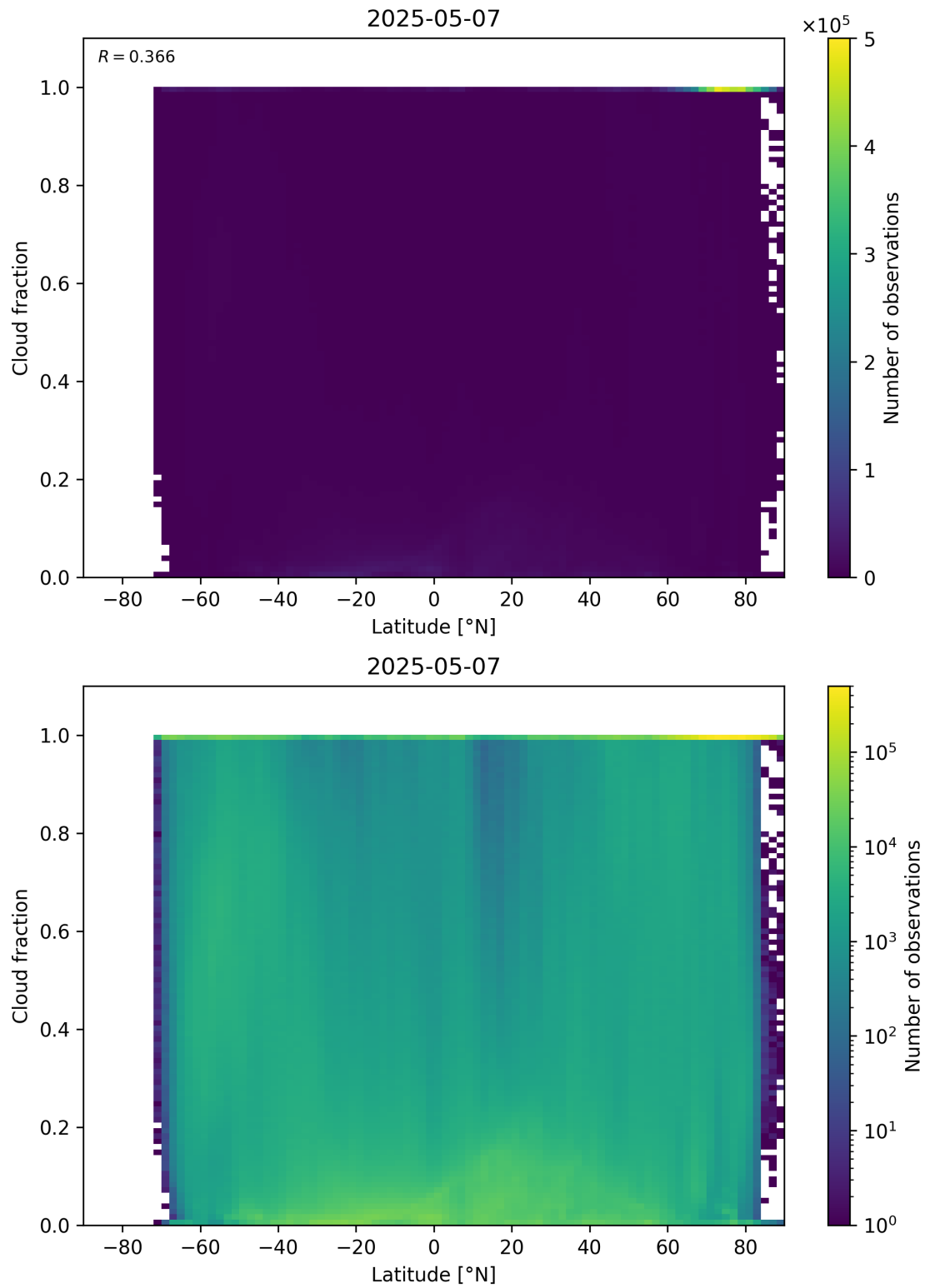
Figure 90: Scatter density plot of “Latitude” against “Cloud fraction” for 2025-05-06 to 2025-05-08.
