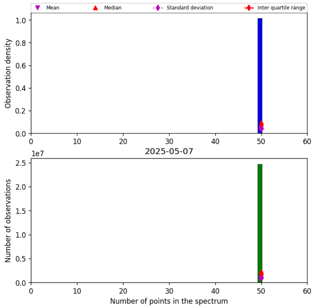
Figure 44: Histogram of “Number of points in the spectrum” for 2025-05-06 to 2025-05-08
