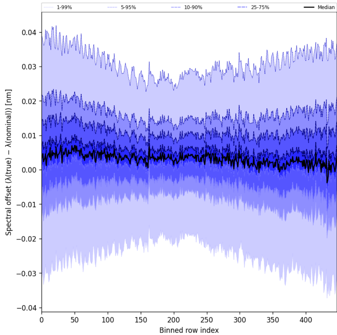
Figure 62: Along track statistics of “Spectral offset ( \lambda_{\text{true}} - \lambda_{\text{nominal}} )” for 2025-05-06 to 2025-05-08
