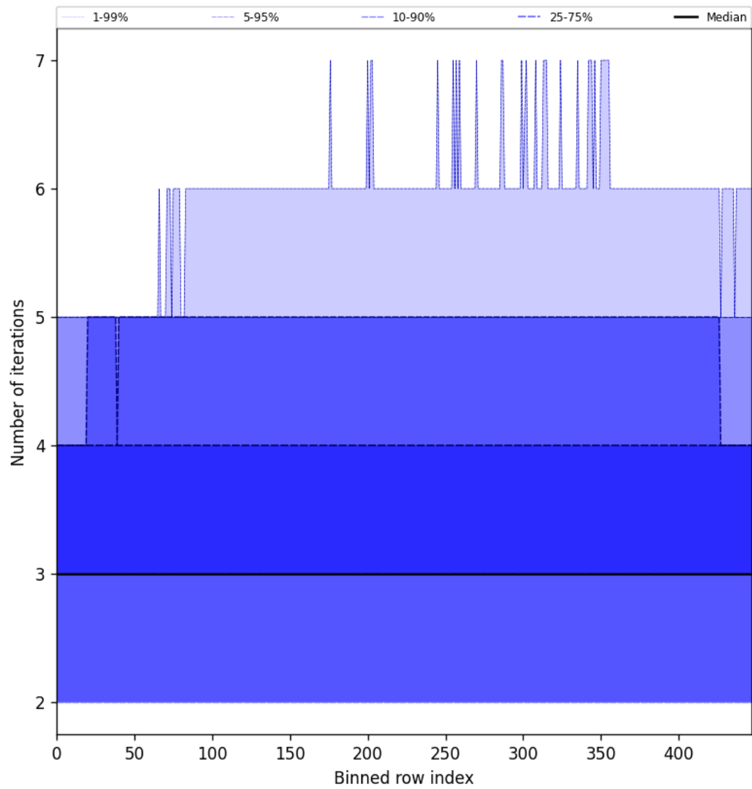
Figure 56: Along track statistics of “Number of iterations” for 2025-05-06 to 2025-05-08
