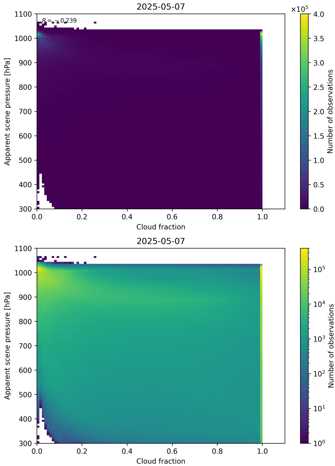
Figure 70: Scatter density plot of “Cloud fraction” against “Apparent scene pressure” for 2025-05-06 to 2025-05-08.
