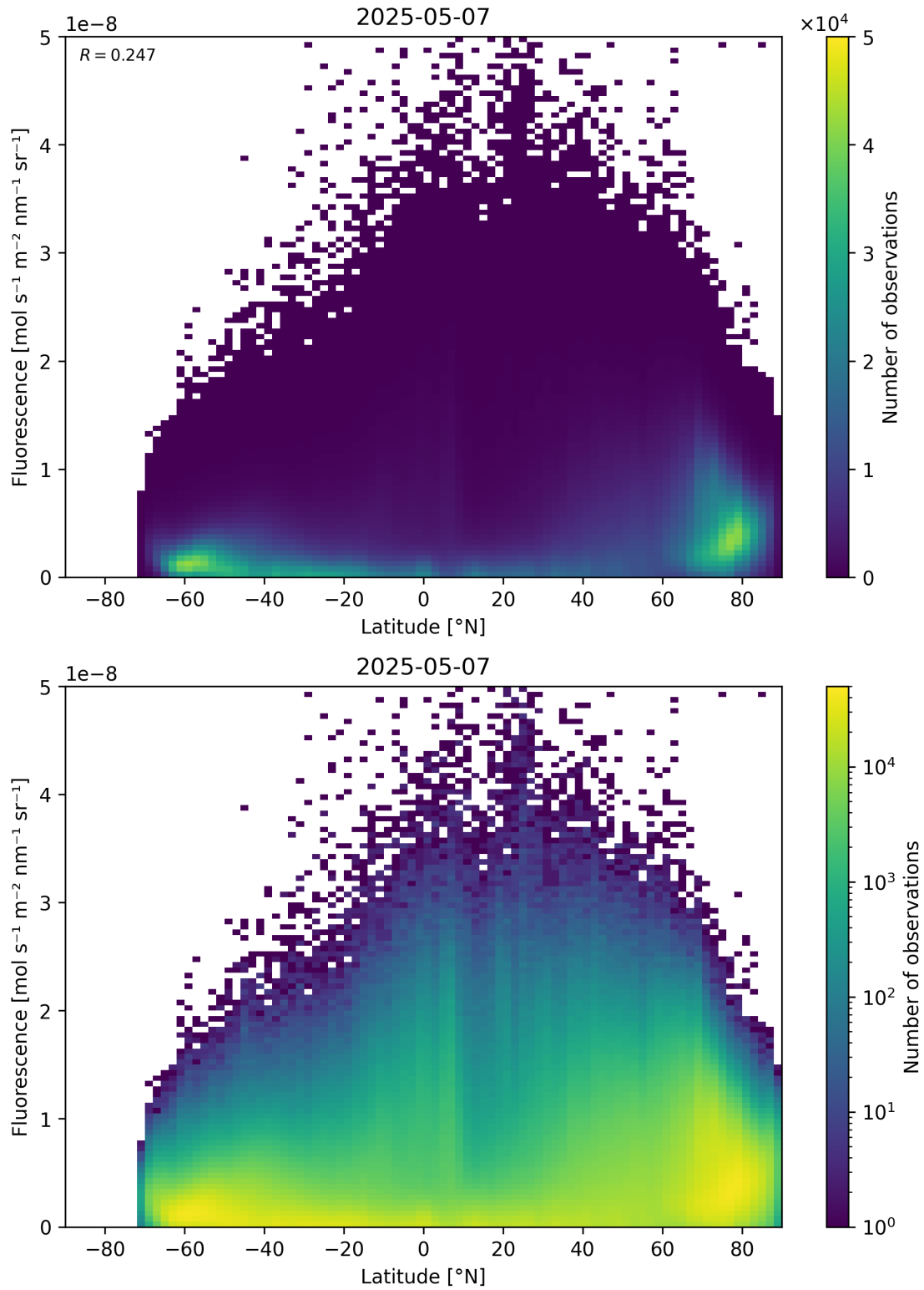
Figure 92: Scatter density plot of “Latitude” against “Fluorescence” for 2025-05-06 to 2025-05-08.
