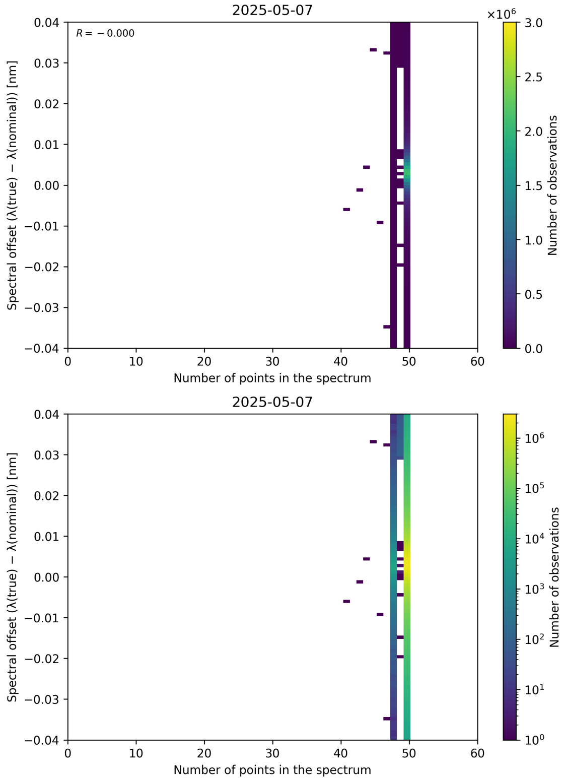
Figure 101: Scatter density plot of “Number of points in the spectrum” against “Spectral offset ( \lambda_{\text{true}} - \lambda_{\text{nominal}} )” for 2025-05-06 to 2025-05-08.
