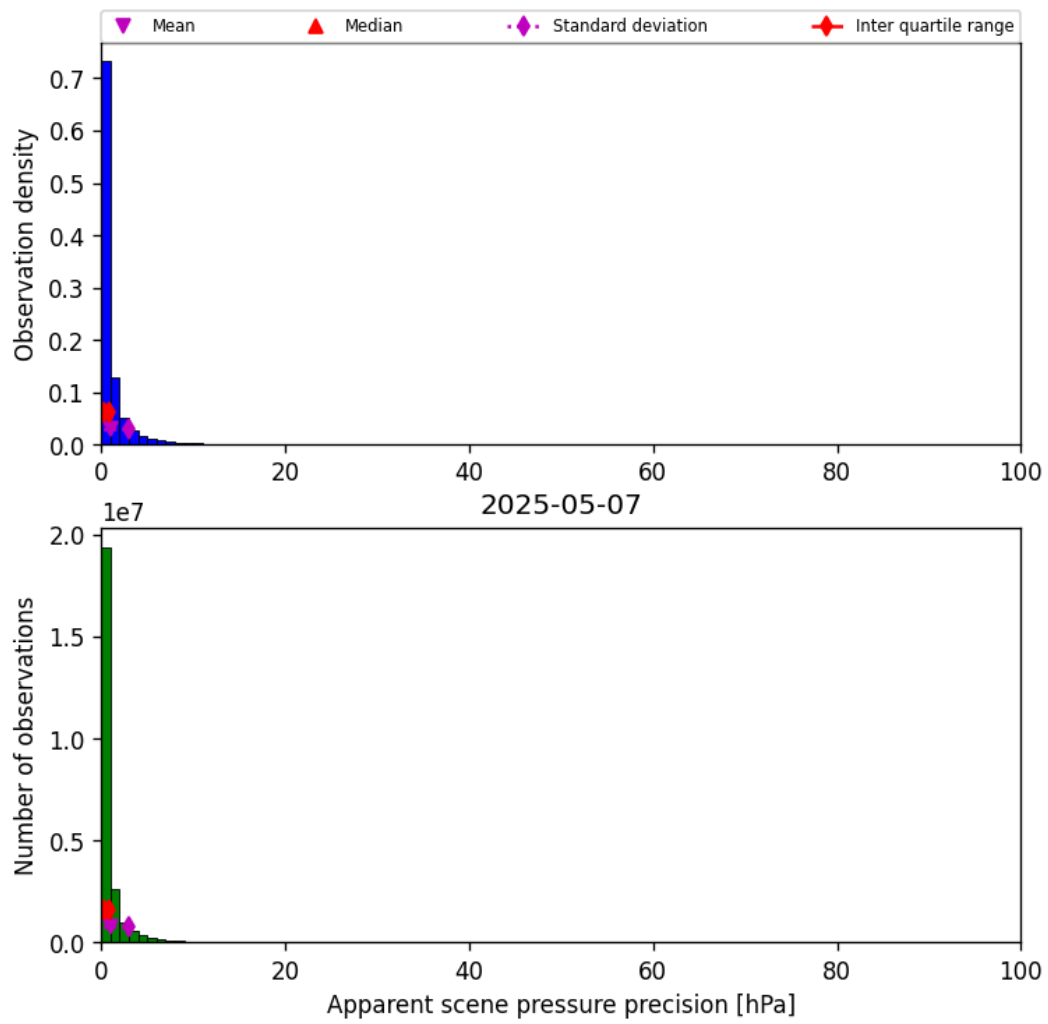
Figure 37: Histogram of “Apparent scene pressure precision” for 2025-05-06 to 2025-05-08
