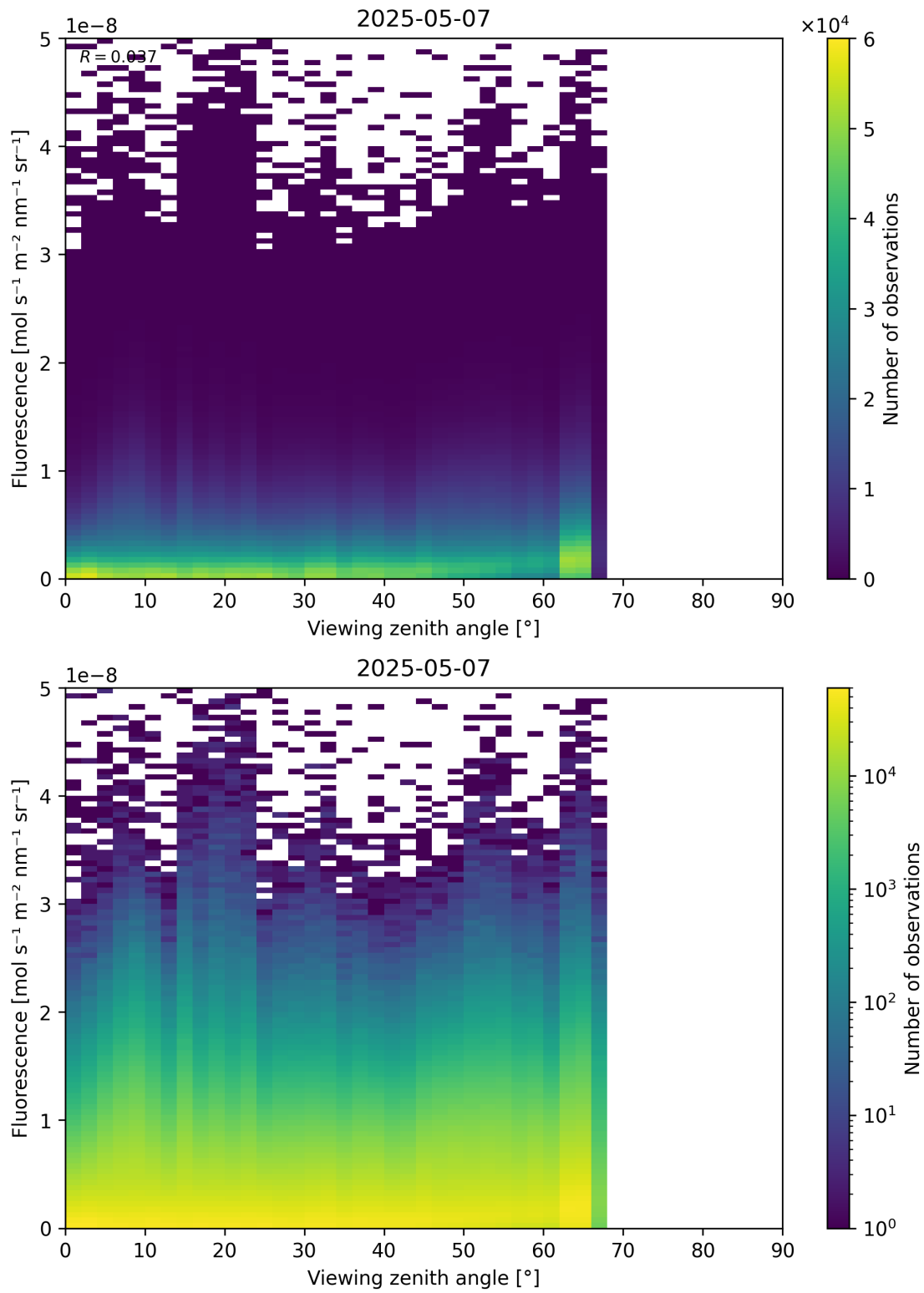
Figure 122: Scatter density plot of “Viewing zenith angle” against “Fluorescence” for 2025-05-06 to 2025-05-08.
