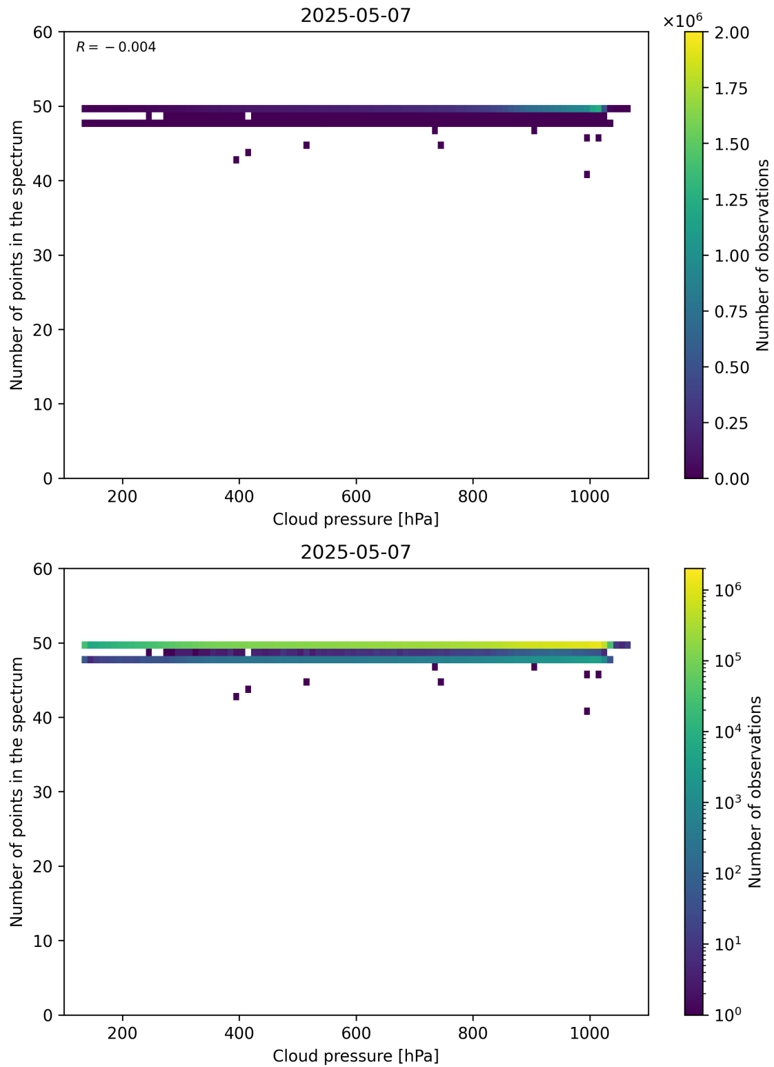
Figure 82: Scatter density plot of “Cloud pressure” against “Number of points in the spectrum” for 2025-05-06 to 2025-05-08.
