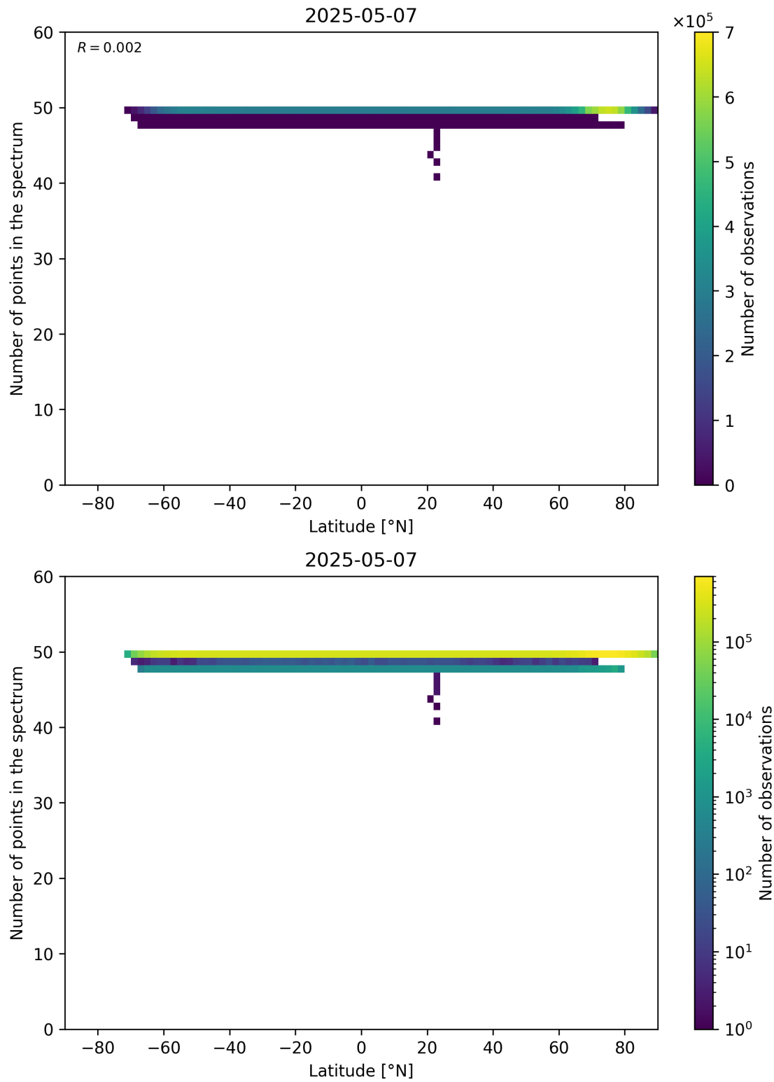
Figure 94: Scatter density plot of “Latitude” against “Number of points in the spectrum” for 2025-05-06 to 2025-05-08.
