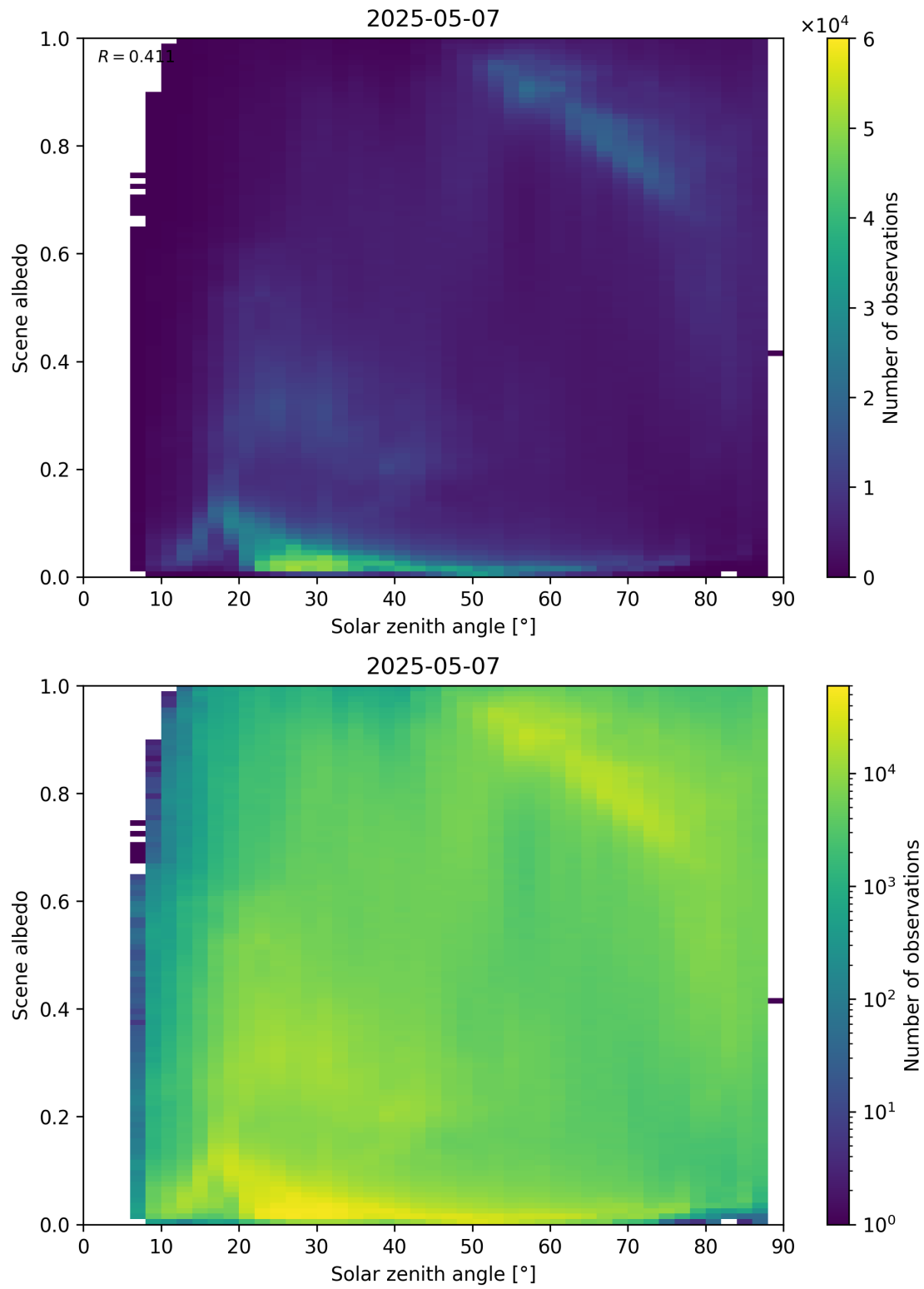
Figure 116: Scatter density plot of “Solar zenith angle” against “Scene albedo” for 2025-05-06 to 2025-05-08.
