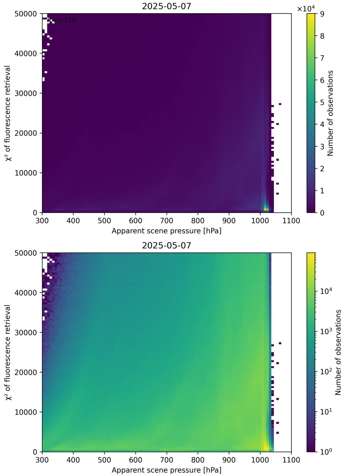
Figure 63: Scatter density plot of “Apparent scene pressure” against “ \chi^2 of fluorescence retrieval” for 2025-05-06 to 2025-05-08.
