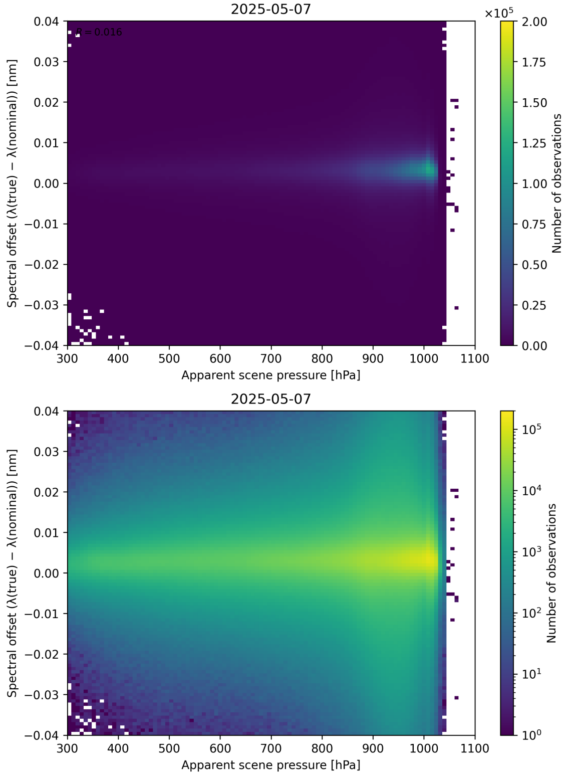
Figure 67: Scatter density plot of “Apparent scene pressure” against “Spectral offset ( \lambda_{\text{true}} - \lambda_{\text{nominal}} )” for 2025-05-06 to 2025-05-08.
