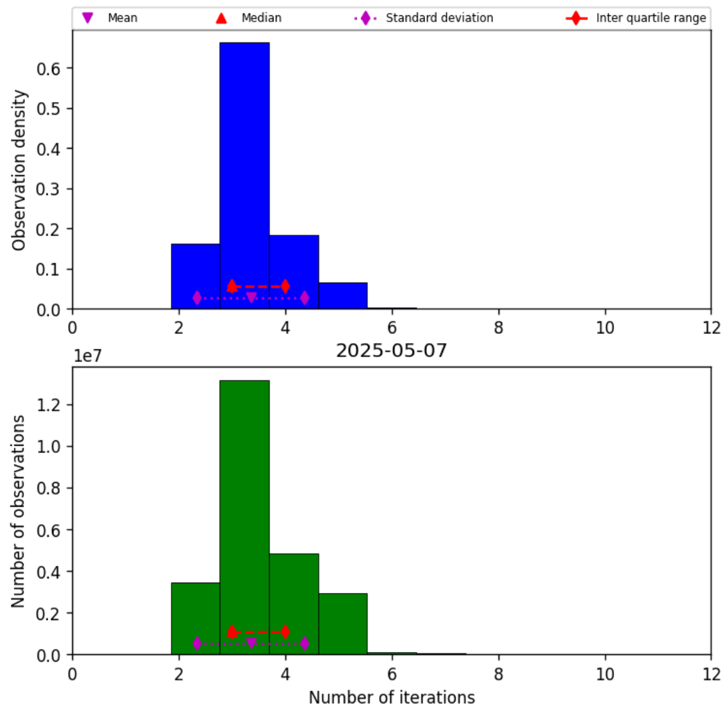
Figure 39: Histogram of “Number of iterations” for 2025-05-06 to 2025-05-08
