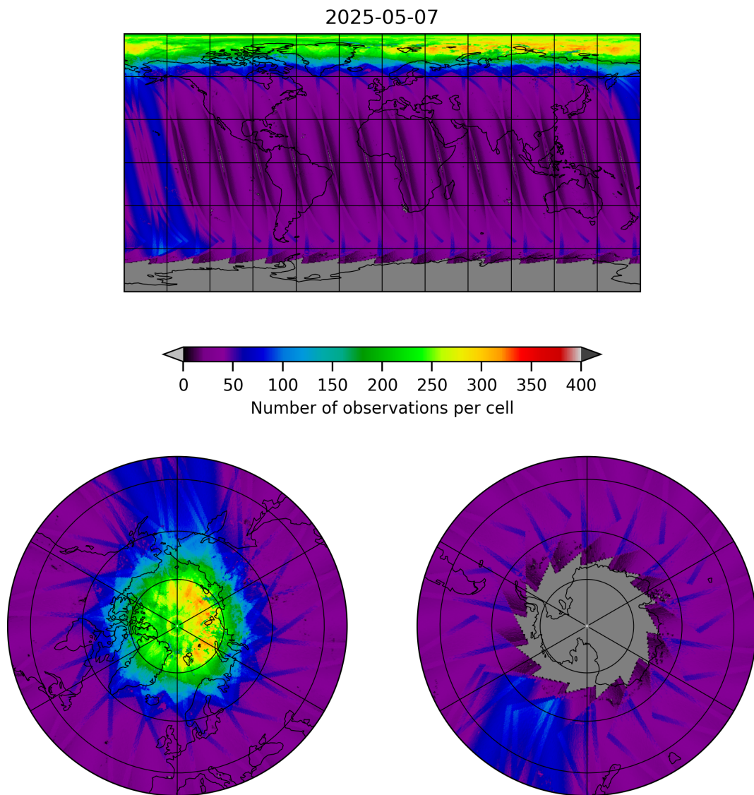
Figure 11: Map of the number of observations for 2025-05-06 to 2025-05-08
