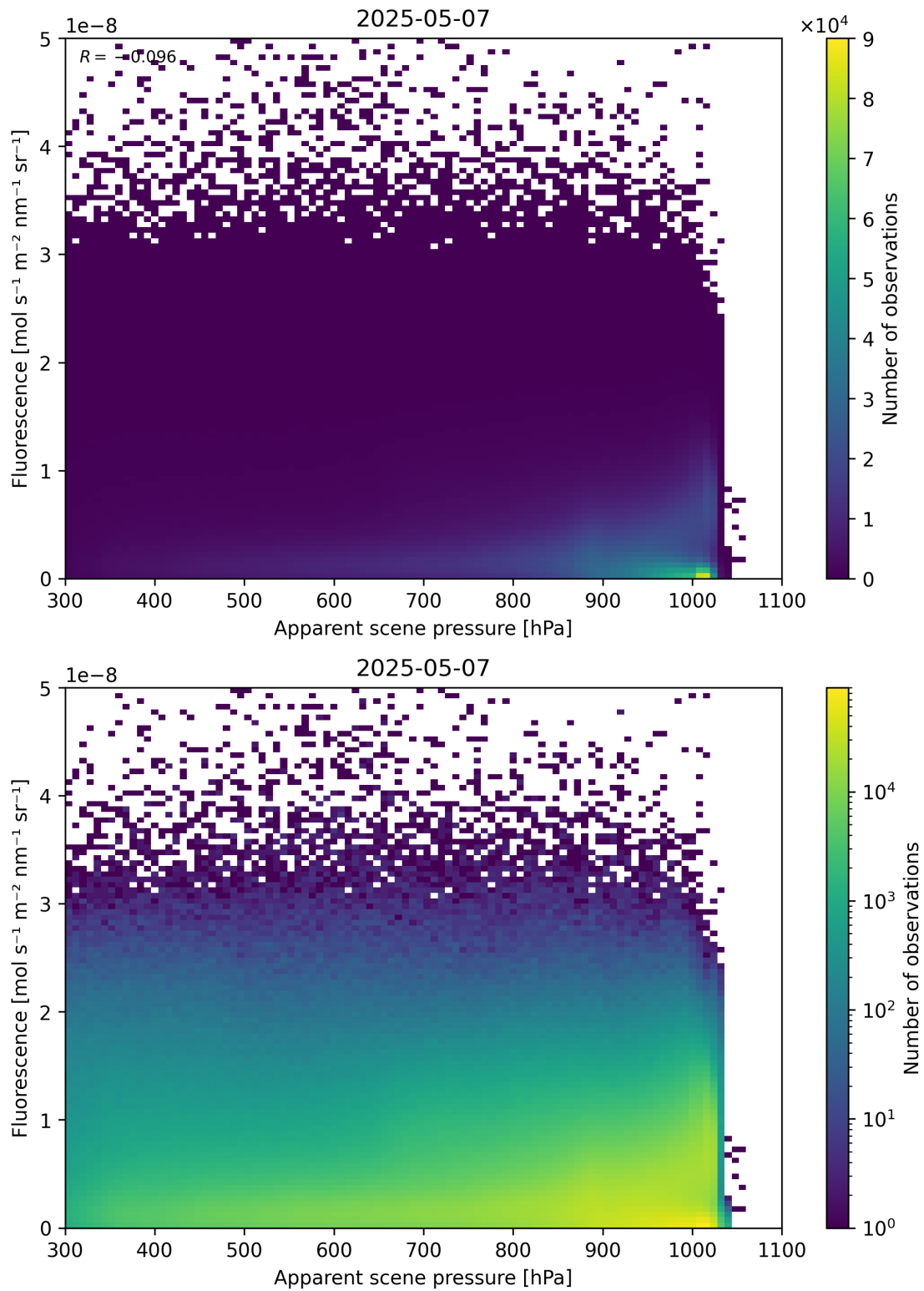
Figure 64: Scatter density plot of “Apparent scene pressure” against “Fluorescence” for 2025-05-06 to 2025-05-08.
