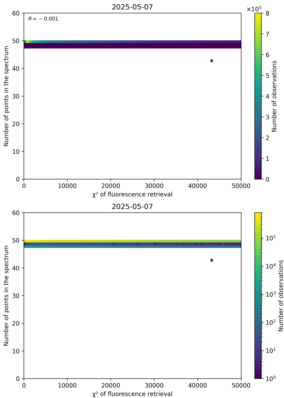
Figure 68: Scatter density plot of “ \chi^2 of fluorescence retrieval” against “Number of points in the spectrum” for 2025-05-06 to 2025-05-08.
