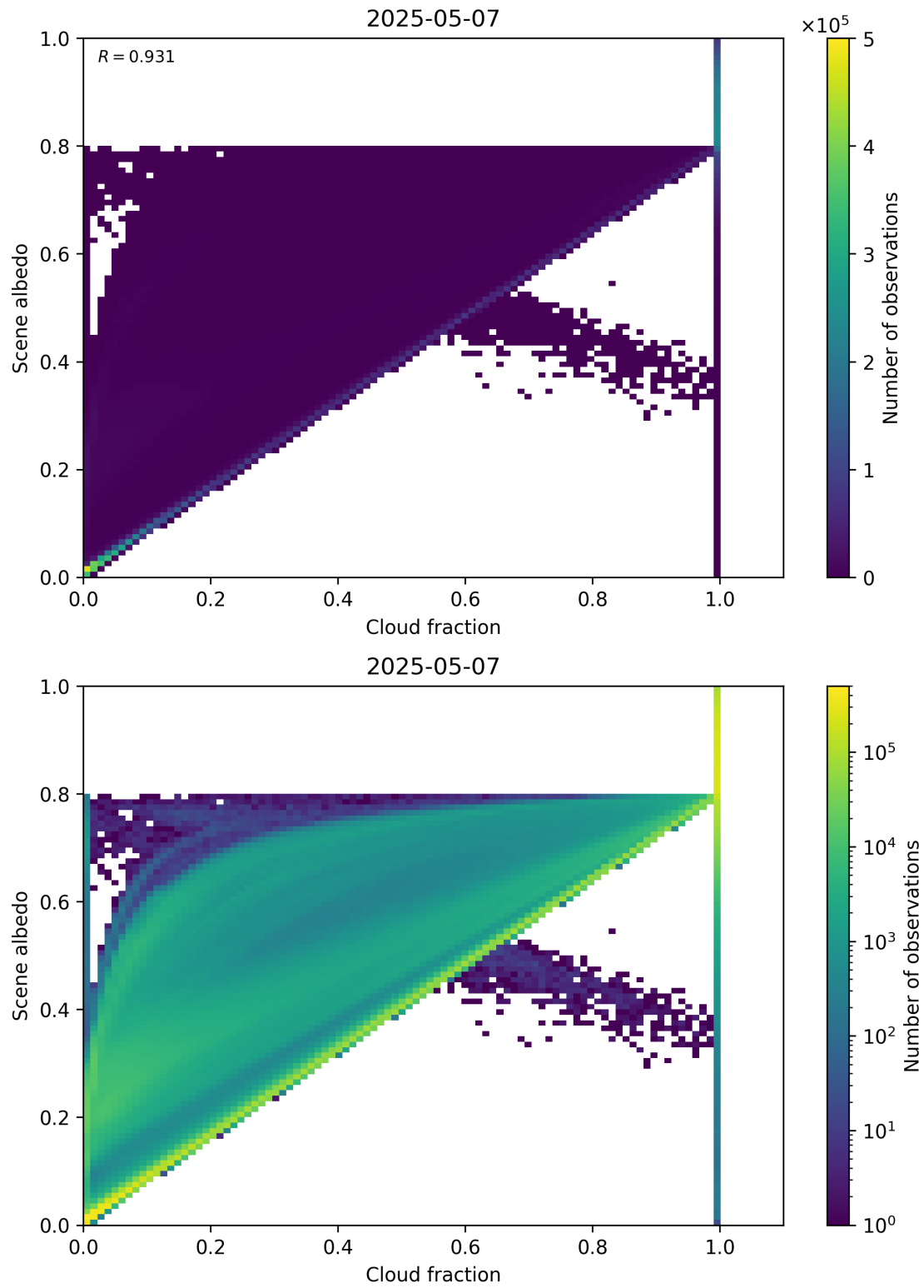
Figure 75: Scatter density plot of “Cloud fraction” against “Scene albedo” for 2025-05-06 to 2025-05-08.
