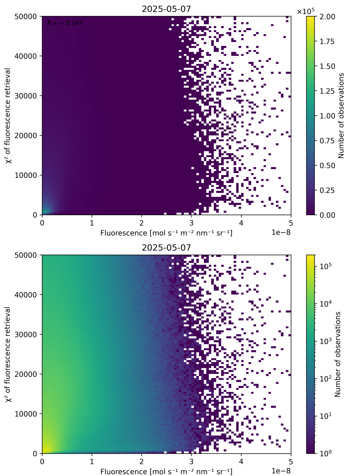
Figure 85: Scatter density plot of “Fluorescence” against “ \chi^2 of fluorescence retrieval” for 2025-05-06 to 2025-05-08.
