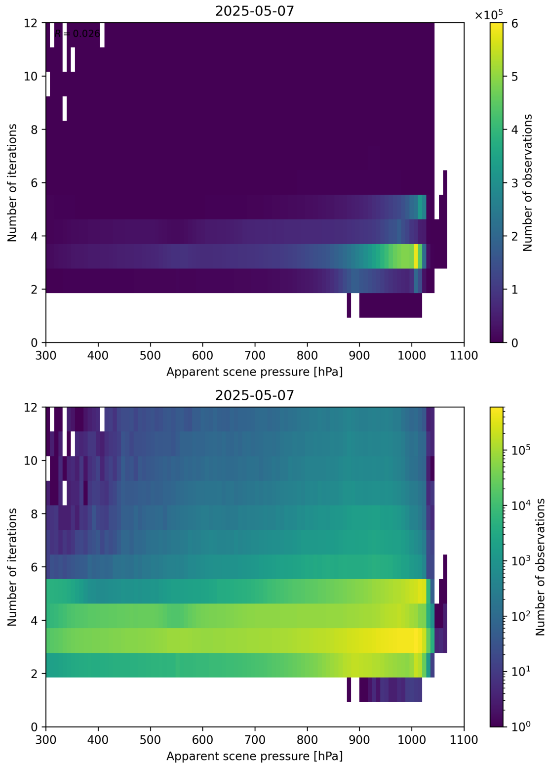
Figure 65: Scatter density plot of “Apparent scene pressure” against “Number of iterations” for 2025-05-06 to 2025-05-08.
