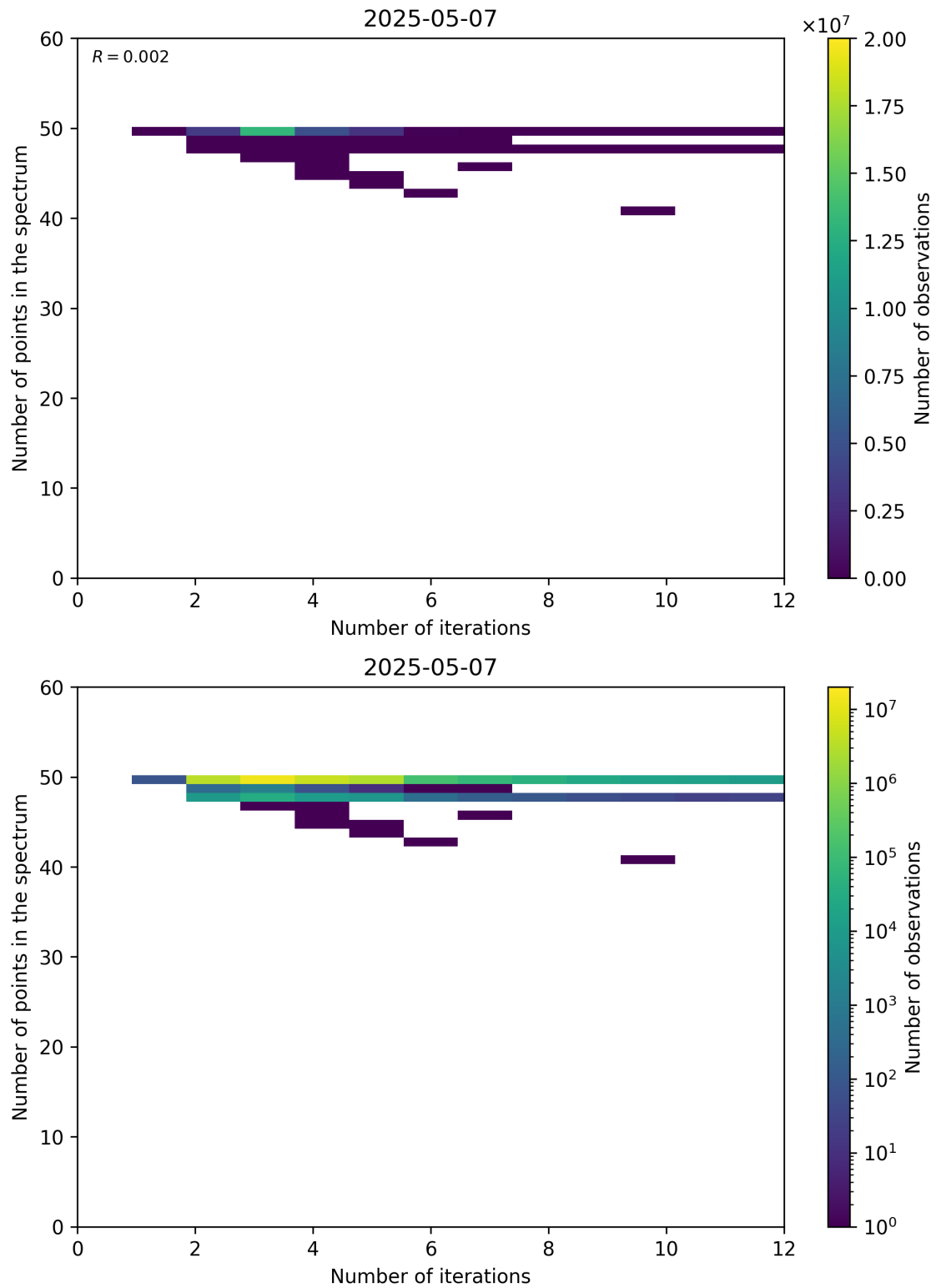
Figure 99: Scatter density plot of “Number of iterations” against “Number of points in the spectrum” for 2025-05-06 to 2025-05-08.
