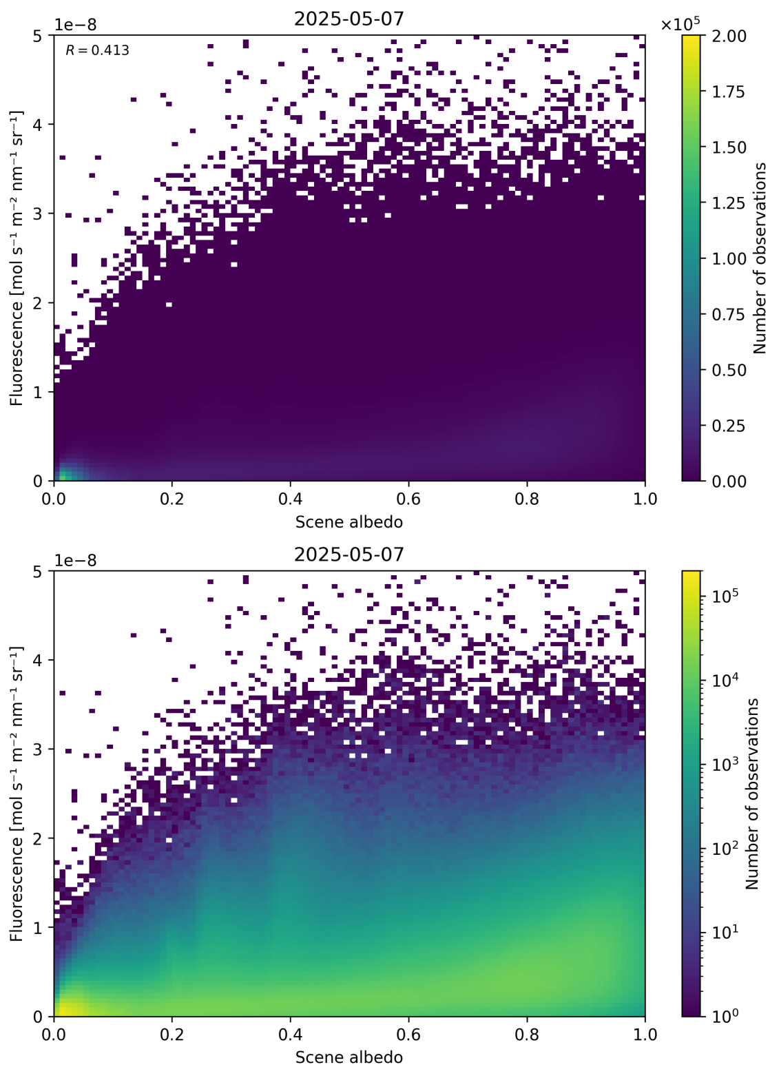
Figure 104: Scatter density plot of “Scene albedo” against “Fluorescence” for 2025-05-06 to 2025-05-08.
