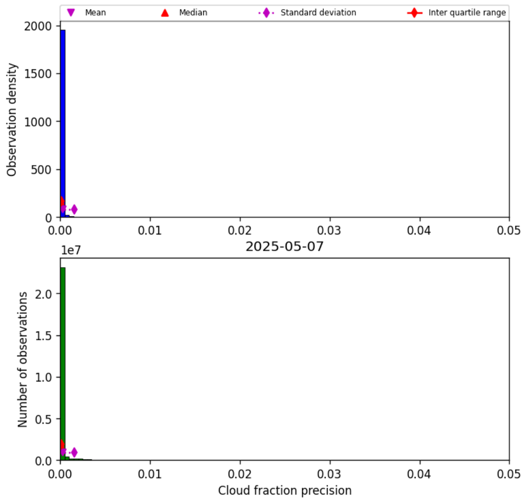
Figure 33: Histogram of “Cloud fraction precision” for 2025-05-06 to 2025-05-08
