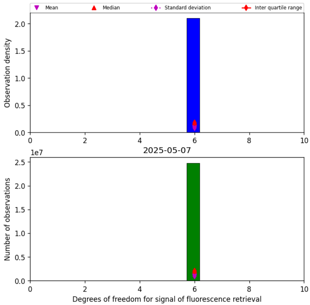
Figure 43: Histogram of “Degrees of freedom for signal of fluorescence retrieval” for 2025-05-06 to 2025-05-08
