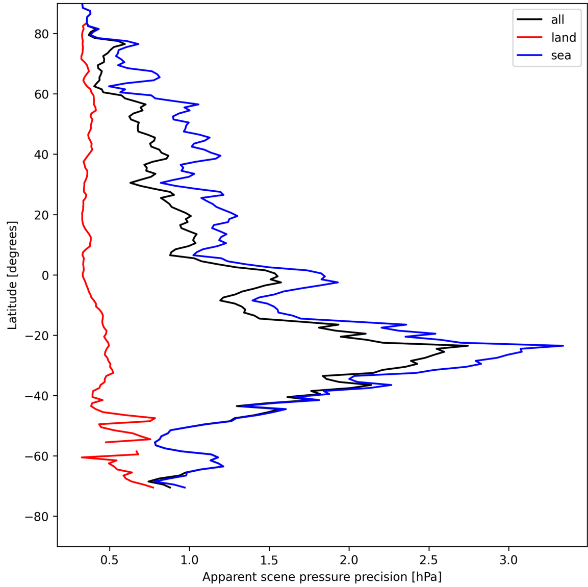
Figure 20: Zonal average of “Apparent scene pressure precision” for 2025-05-06 to 2025-05-08.
