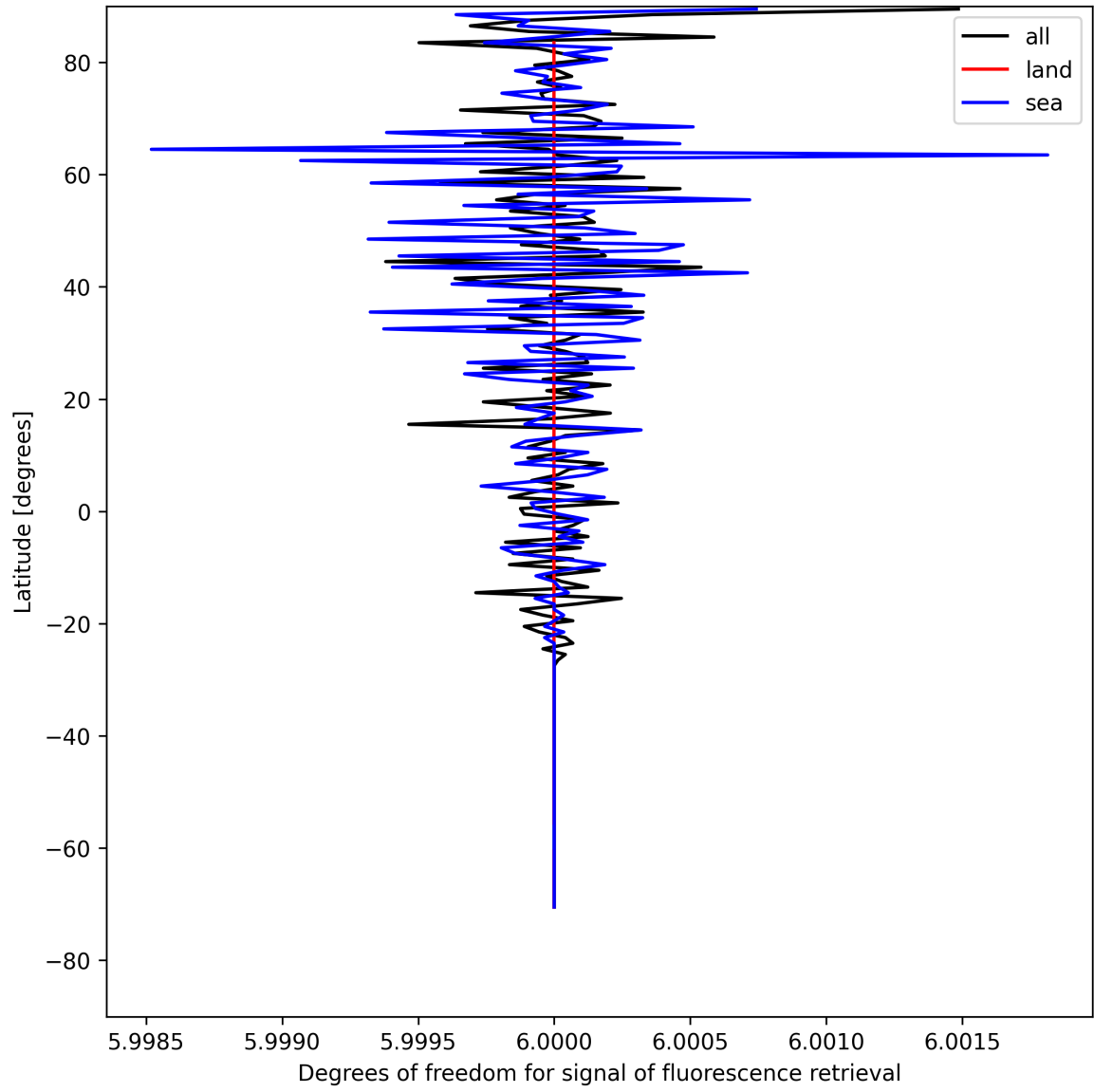
Figure 26: Zonal average of “Degrees of freedom for signal of fluorescence retrieval” for 2025-05-07 to 2025-05-09.
