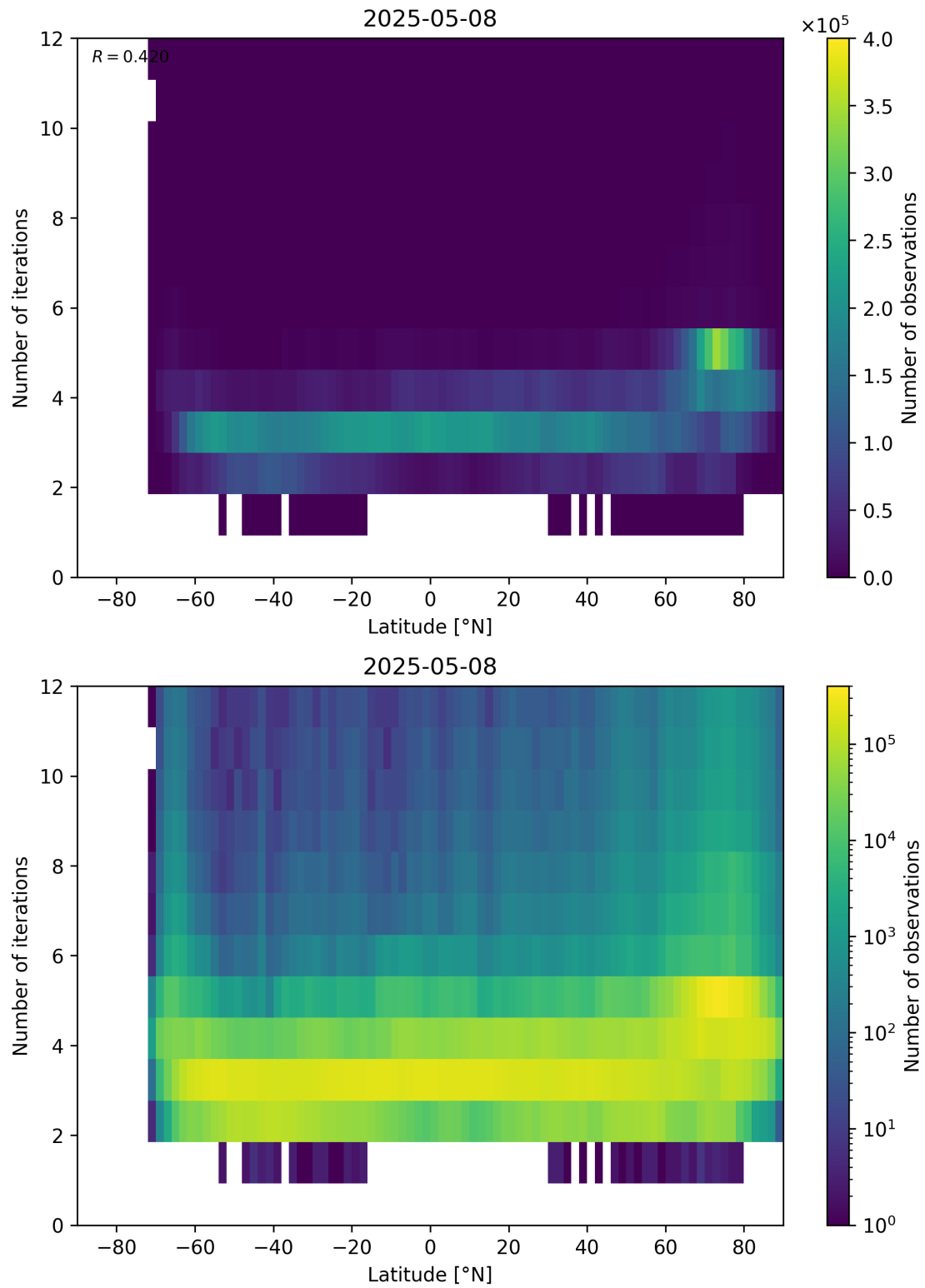
Figure 93: Scatter density plot of “Latitude” against “Number of iterations” for 2025-05-07 to 2025-05-09.
