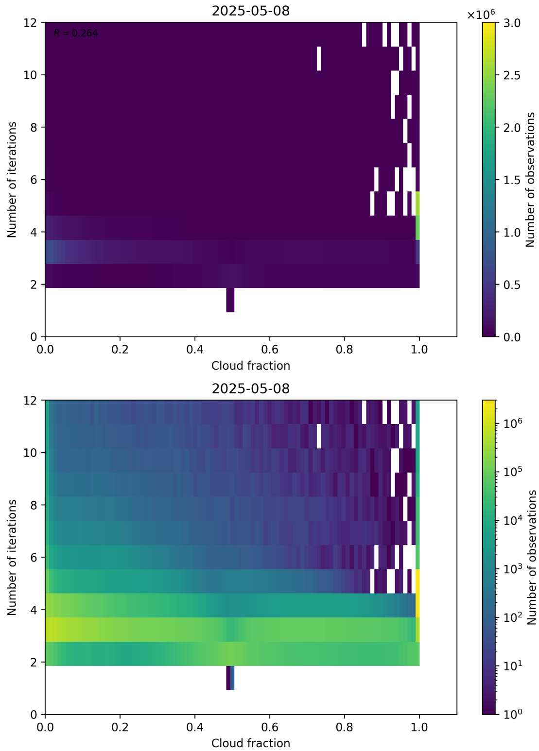
Figure 73: Scatter density plot of “Cloud fraction” against “Number of iterations” for 2025-05-07 to 2025-05-09.
