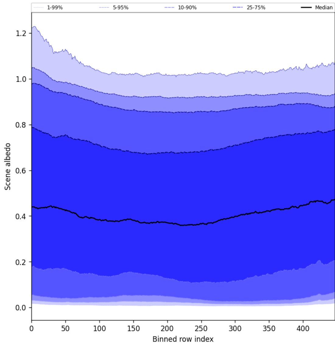
Figure 51: Along track statistics of “Scene albedo” for 2025-05-07 to 2025-05-09
