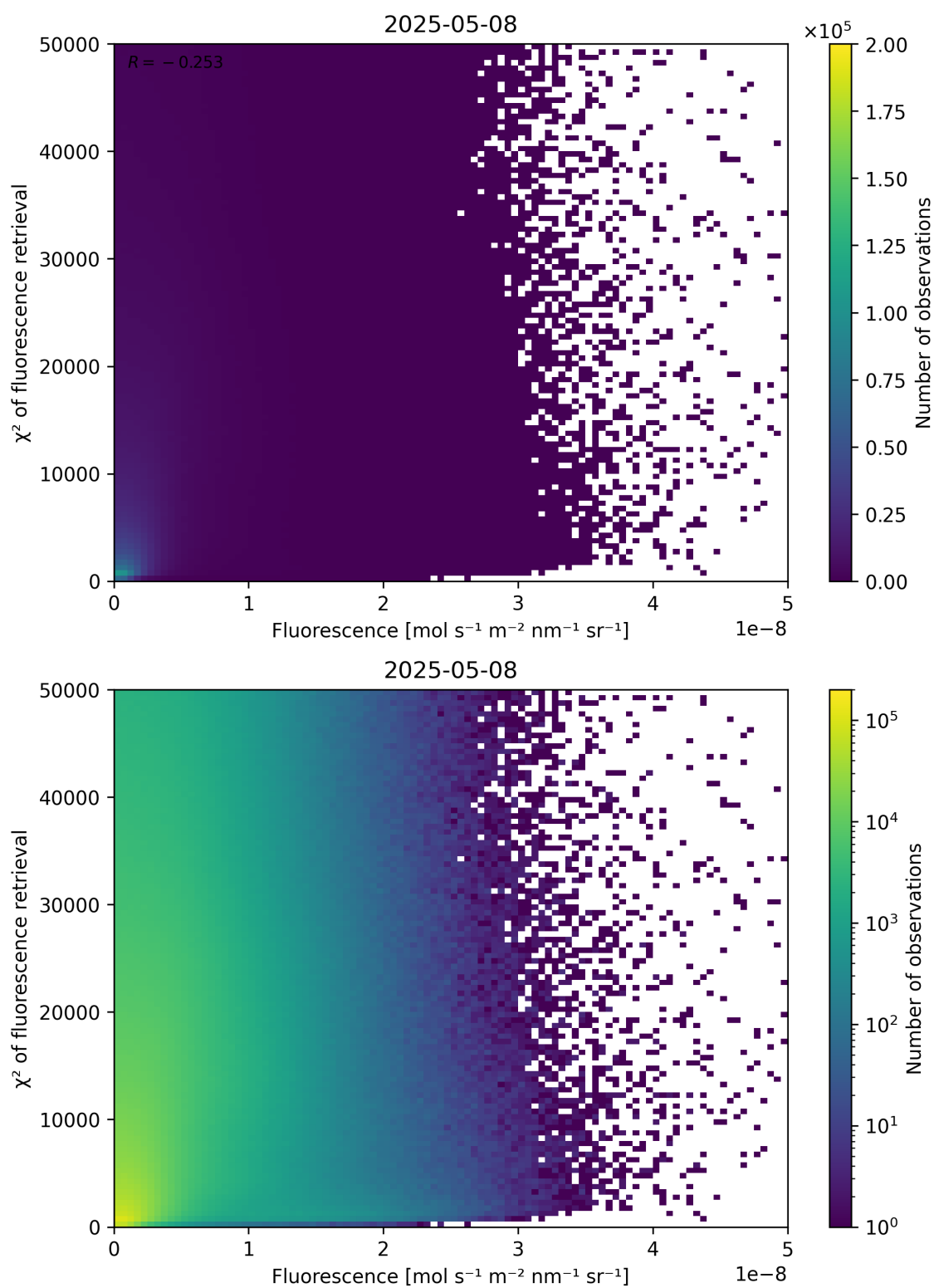
Figure 85: Scatter density plot of “Fluorescence” against “ \chi^2 of fluorescence retrieval” for 2025-05-07 to 2025-05-09.
