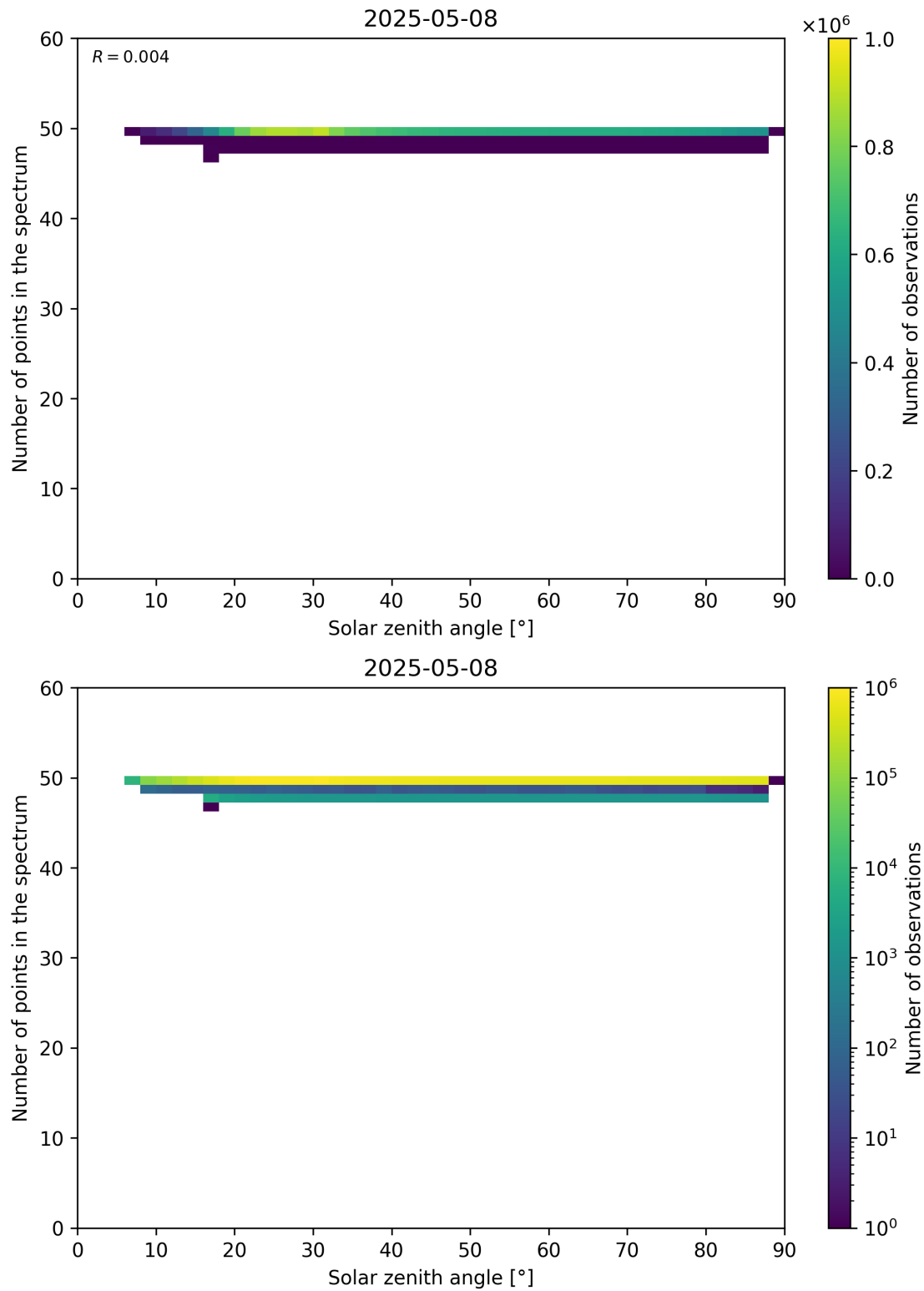
Figure 115: Scatter density plot of “Solar zenith angle” against “Number of points in the spectrum” for 2025-05-07 to 2025-05-09.
