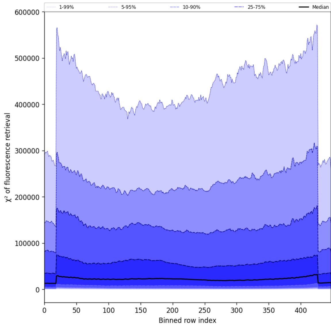
Figure 59: Along track statistics of " \chi^2 of fluorescence retrieval" for 2025-05-07 to 2025-05-09
