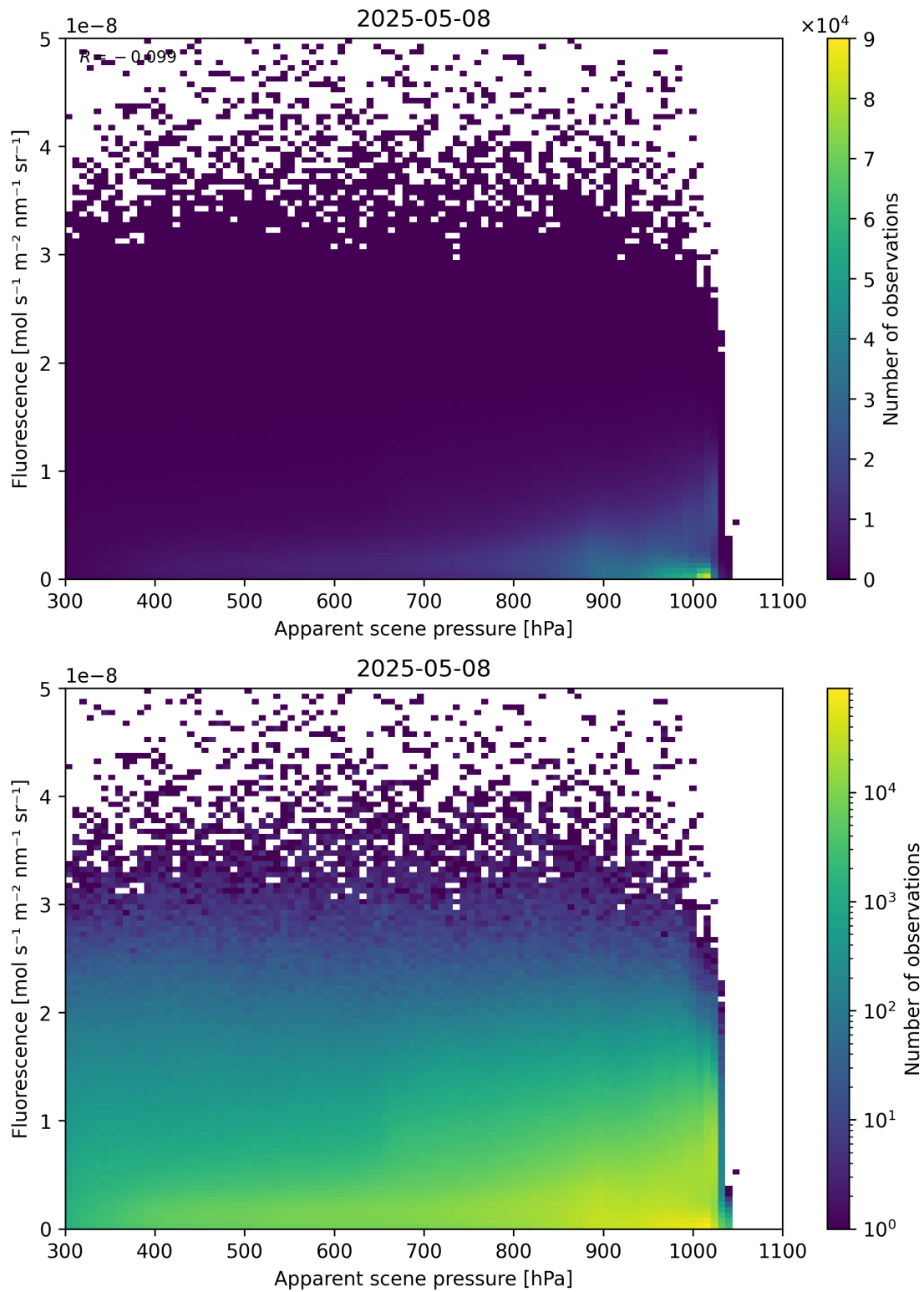
Figure 64: Scatter density plot of “Apparent scene pressure” against “Fluorescence” for 2025-05-07 to 2025-05-09.
