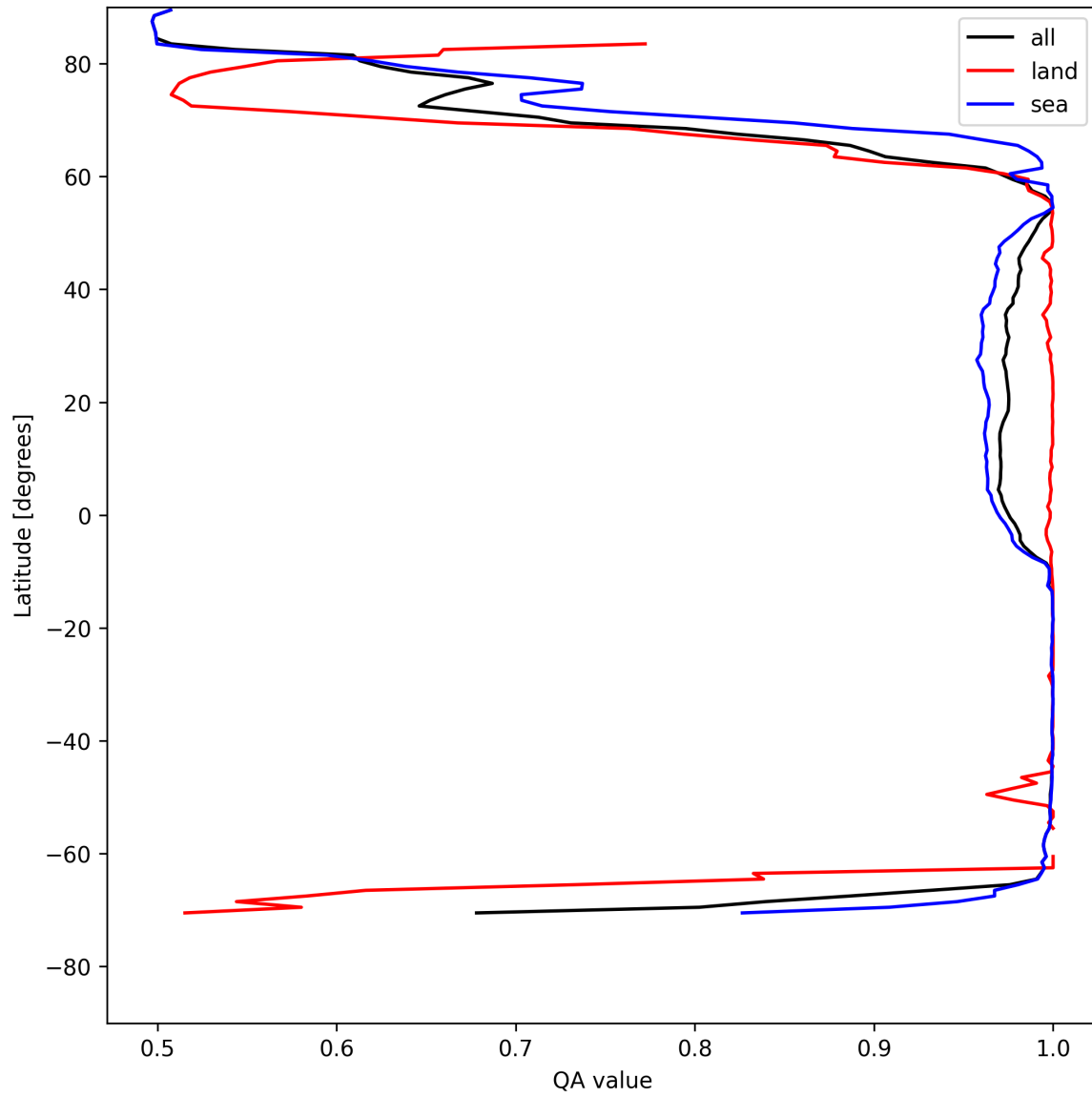
Figure 12: Zonal average of “QA value” for 2025-05-07 to 2025-05-09.
