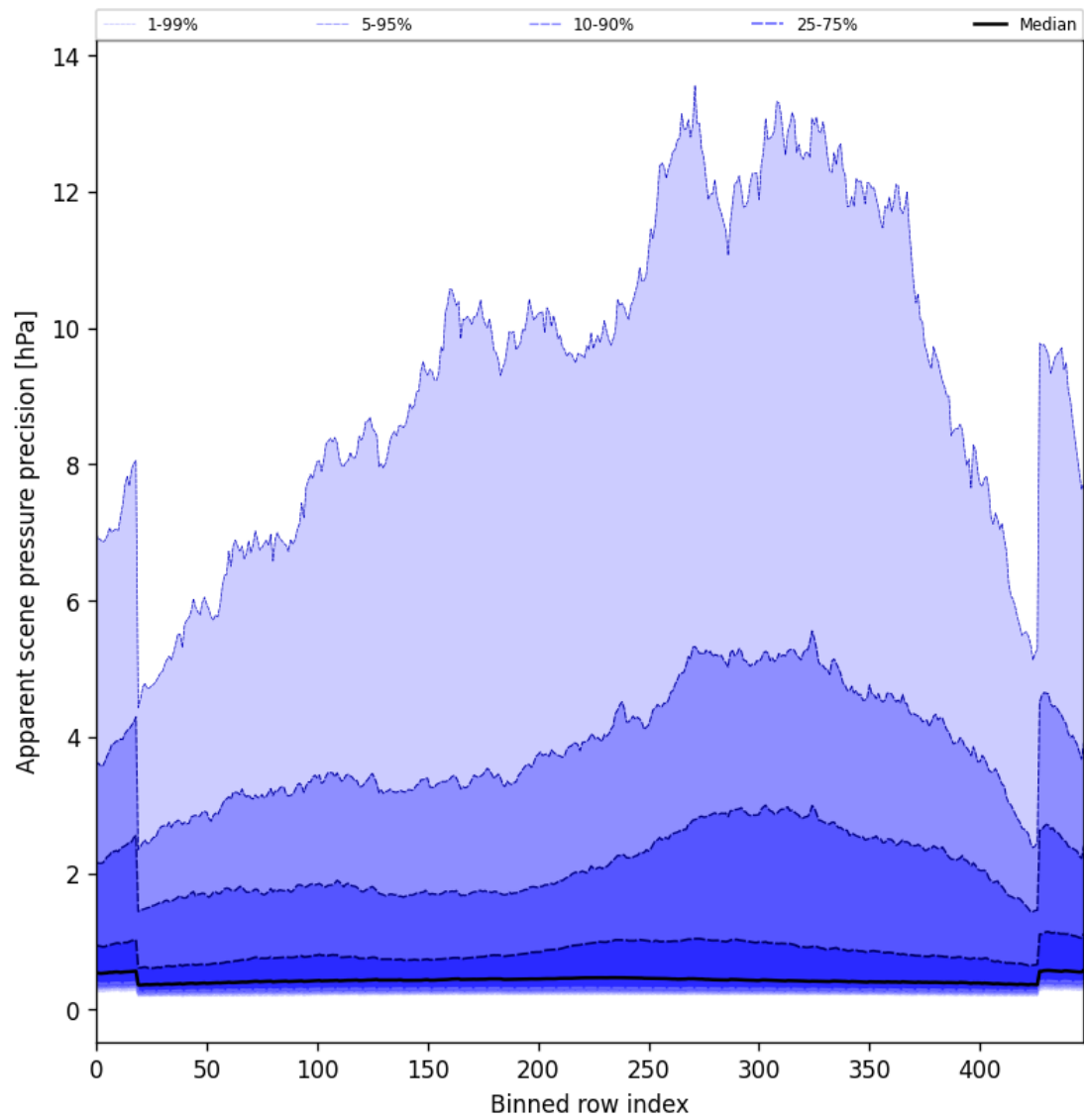
Figure 54: Along track statistics of “Apparent scene pressure precision” for 2025-05-07 to 2025-05-09
