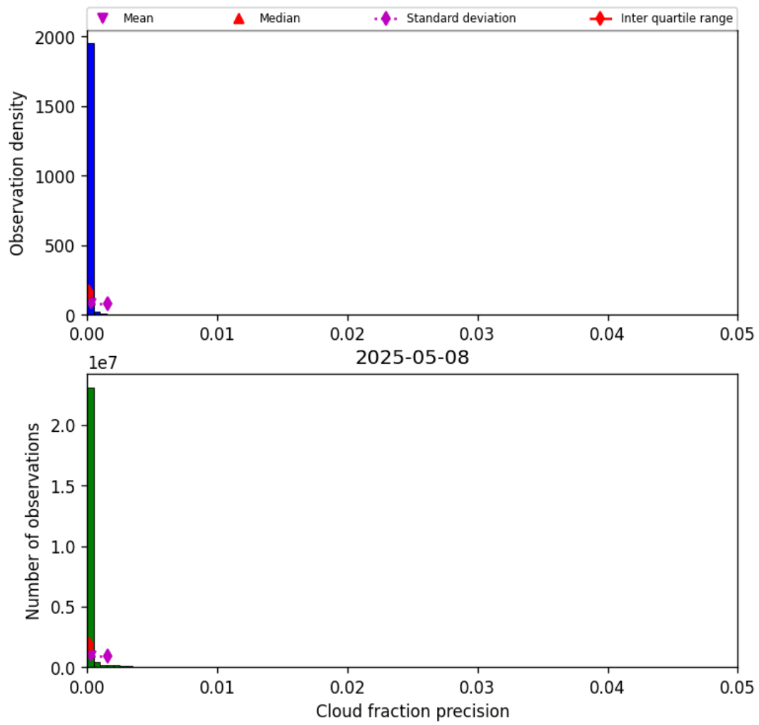
Figure 33: Histogram of “Cloud fraction precision” for 2025-05-07 to 2025-05-09
