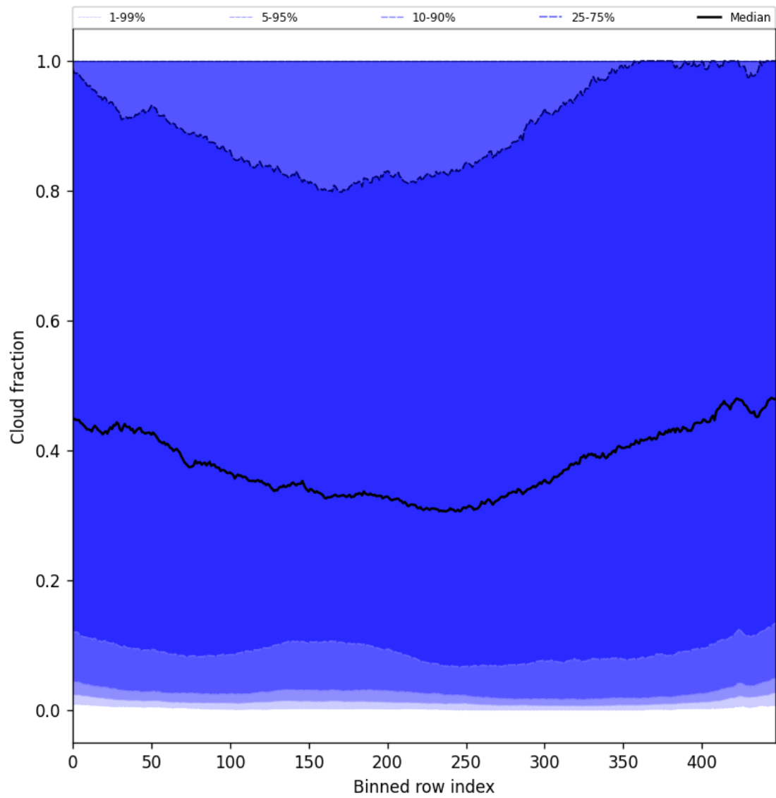
Figure 49: Along track statistics of “Cloud fraction” for 2025-05-07 to 2025-05-09
