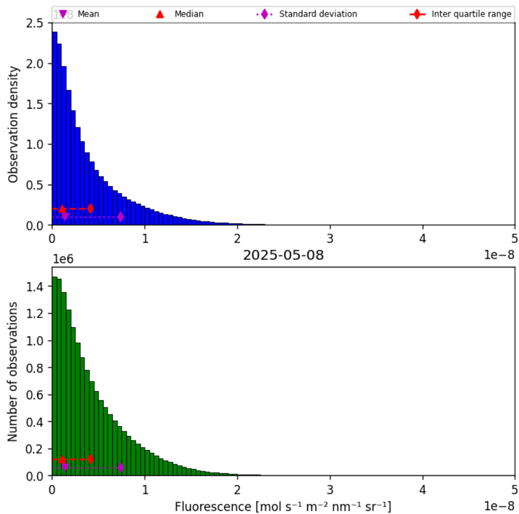
Figure 40: Histogram of “Fluorescence” for 2025-05-07 to 2025-05-09
