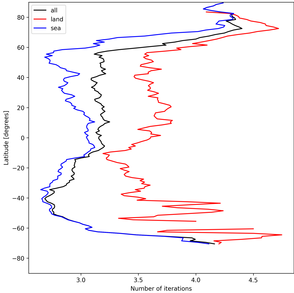
Figure 22: Zonal average of “Number of iterations” for 2025-05-07 to 2025-05-09.
