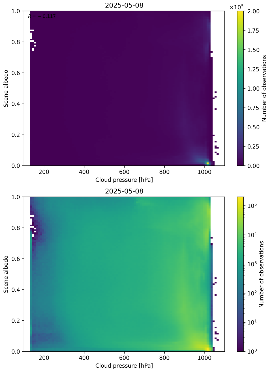
Figure 83: Scatter density plot of “Cloud pressure” against “Scene albedo” for 2025-05-07 to 2025-05-09.
