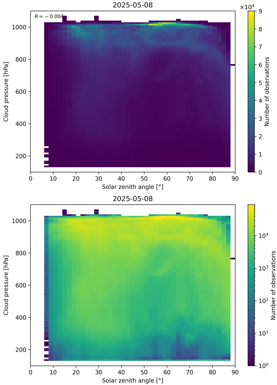
Figure 111: Scatter density plot of “Solar zenith angle” against “Cloud pressure” for 2025-05-07 to 2025-05-09.
