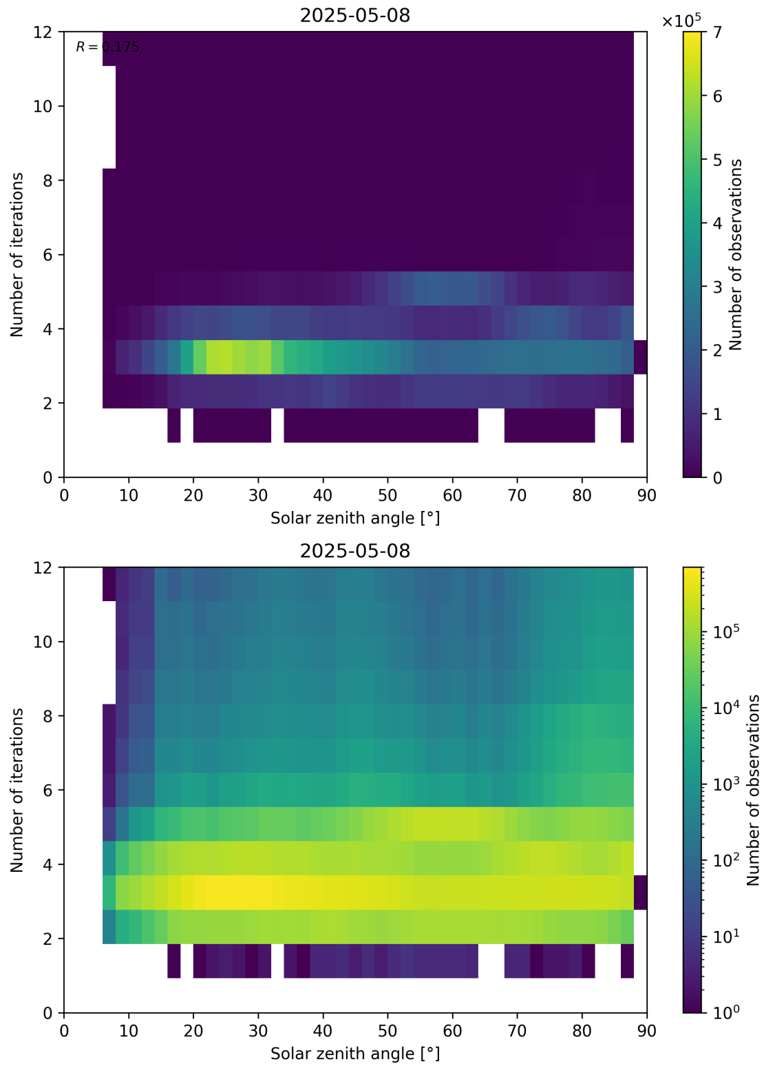
Figure 114: Scatter density plot of “Solar zenith angle” against “Number of iterations” for 2025-05-07 to 2025-05-09.
