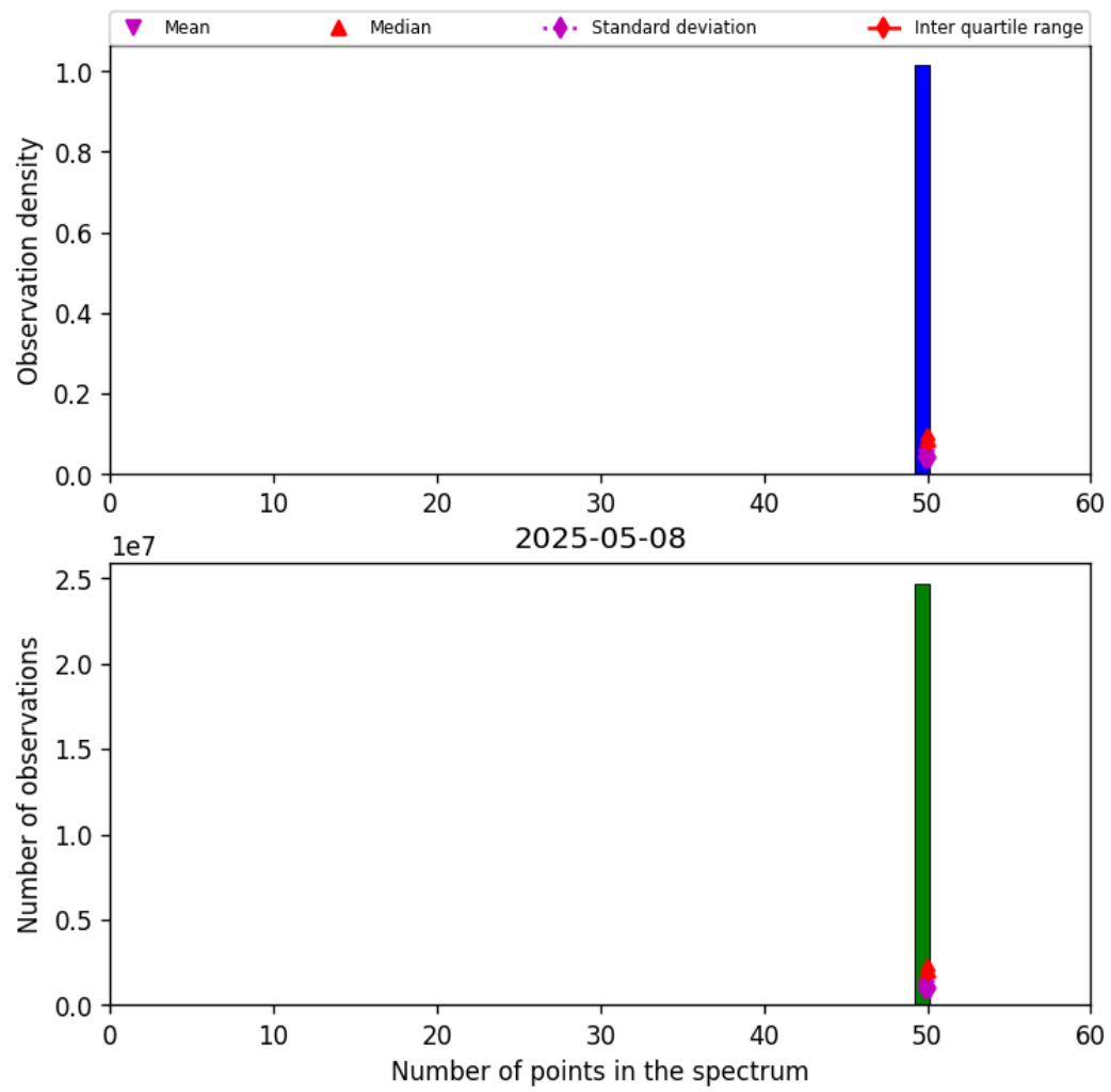
Figure 44: Histogram of “Number of points in the spectrum” for 2025-05-07 to 2025-05-09
