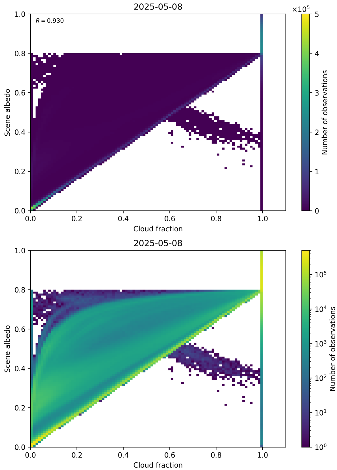
Figure 75: Scatter density plot of “Cloud fraction” against “Scene albedo” for 2025-05-07 to 2025-05-09.
