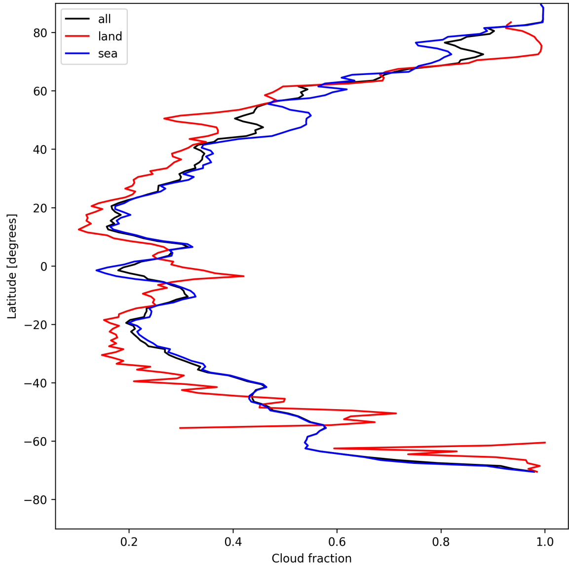
Figure 15: Zonal average of “Cloud fraction” for 2025-05-07 to 2025-05-09.
