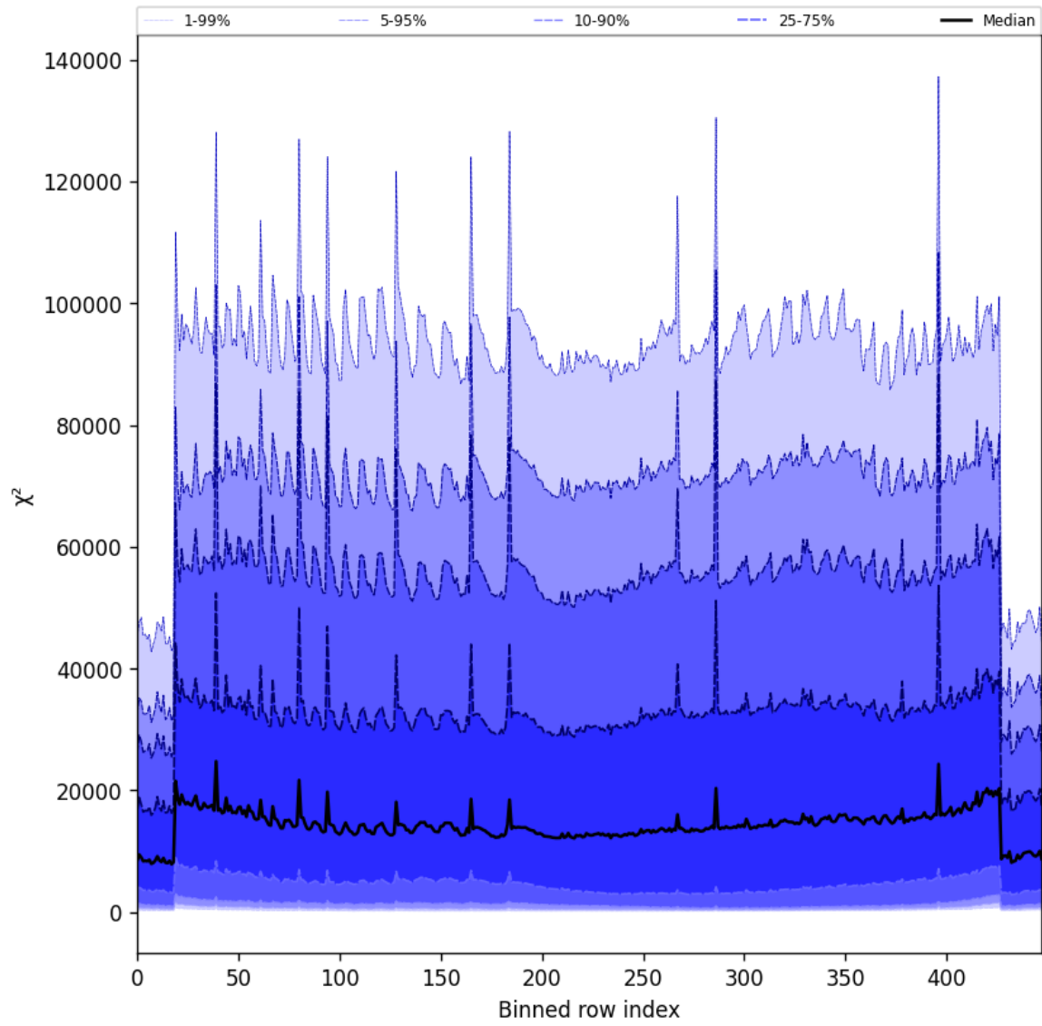
Figure 55: Along track statistics of “ \chi^2 ” for 2025-05-07 to 2025-05-09
