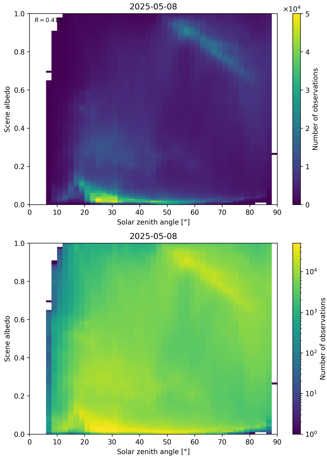
Figure 116: Scatter density plot of “Solar zenith angle” against “Scene albedo” for 2025-05-07 to 2025-05-09.
