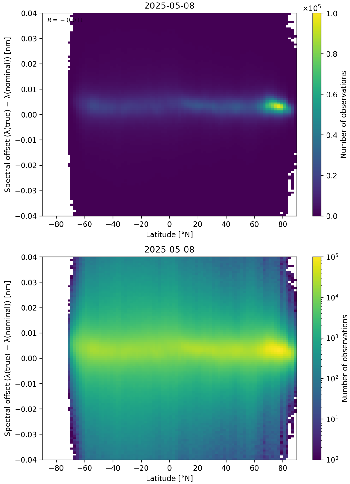
Figure 96: Scatter density plot of “Latitude” against “Spectral offset ( \lambda_{\text{true}} - \lambda_{\text{nominal}} )” for 2025-05-07 to 2025-05-09.
