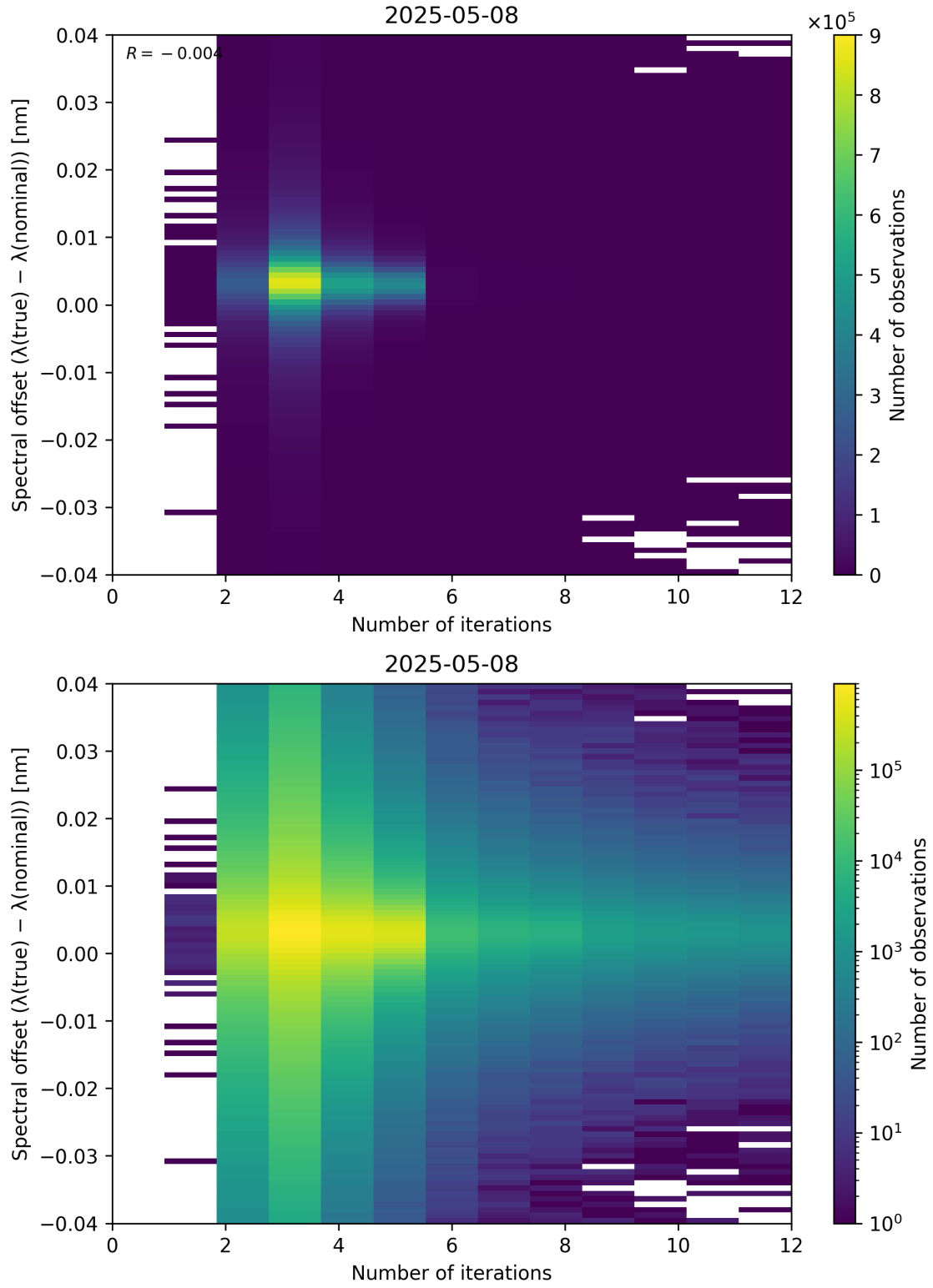
Figure 100: Scatter density plot of “Number of iterations” against “Spectral offset ( \lambda_{\text{true}} - \lambda_{\text{nominal}} )” for 2025-05-07 to 2025-05-09.
