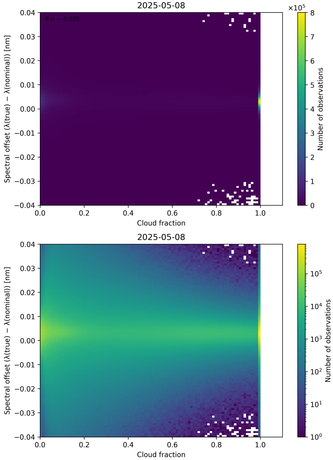
Figure 76: Scatter density plot of “Cloud fraction” against “Spectral offset ( \lambda_{\text{true}} - \lambda_{\text{nominal}} )” for 2025-05-07 to 2025-05-09.
