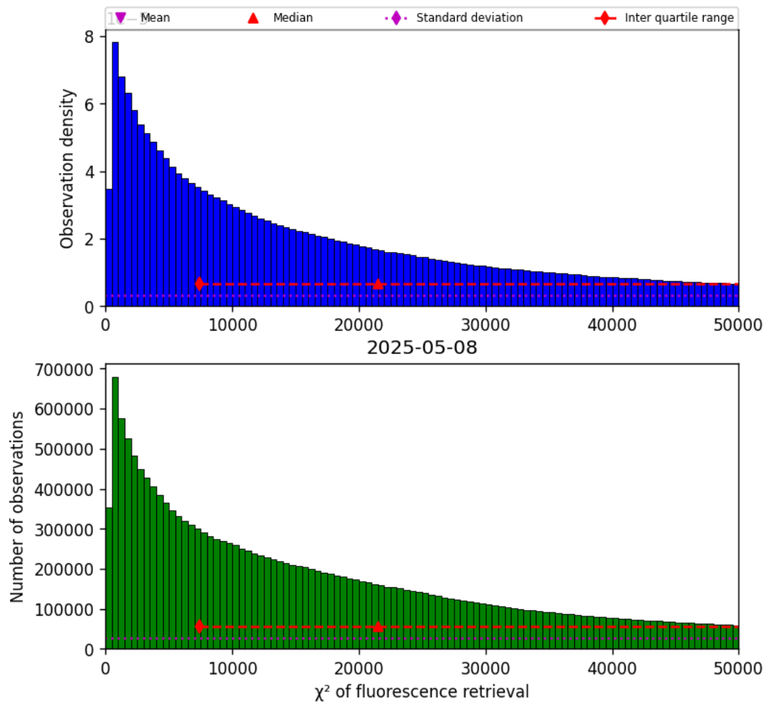
Figure 42: Histogram of “ \chi^2 of fluorescence retrieval” for 2025-05-07 to 2025-05-09
