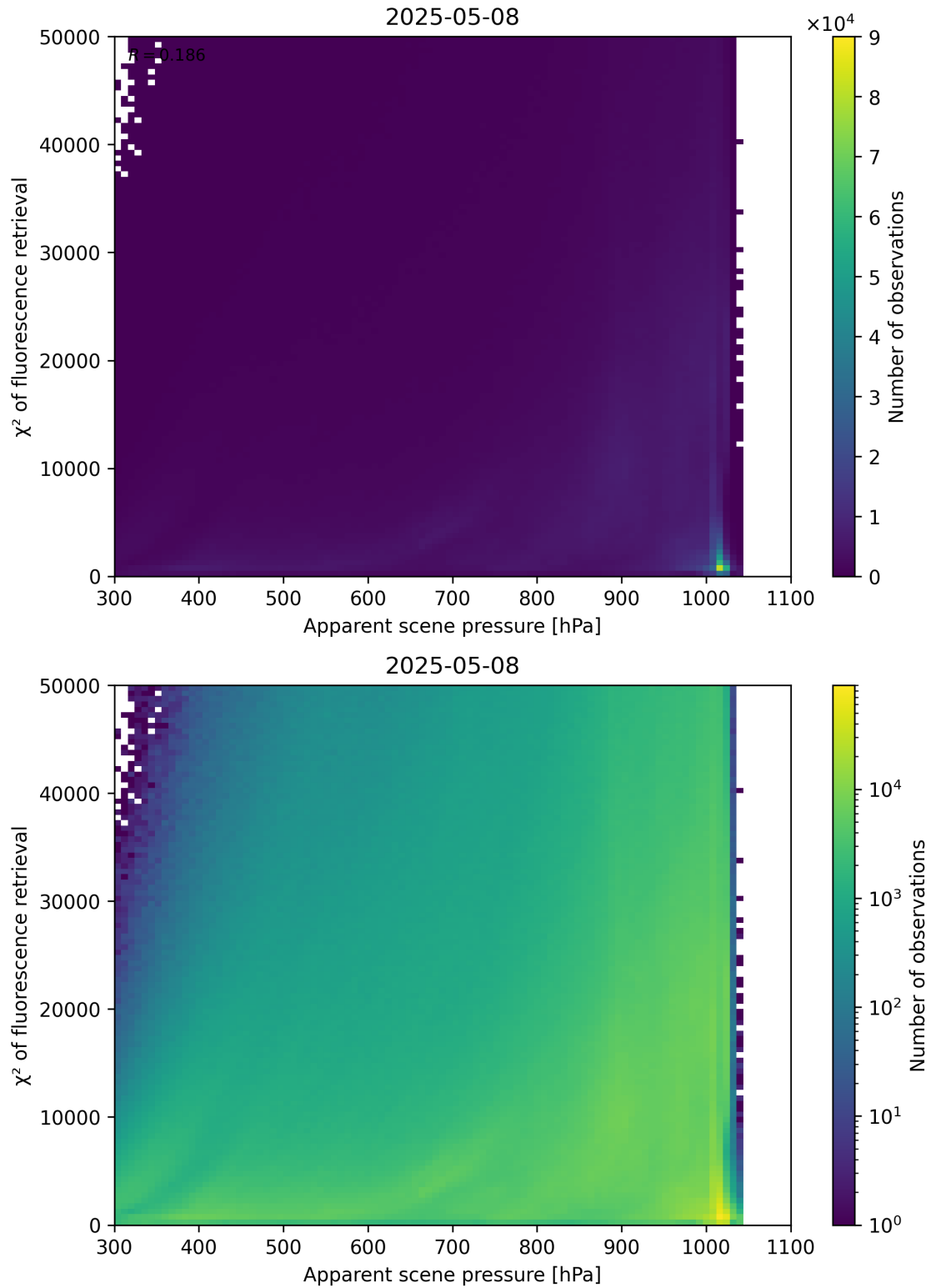
Figure 63: Scatter density plot of “Apparent scene pressure” against “ \chi^2 of fluorescence retrieval” for 2025-05-07 to 2025-05-09.
