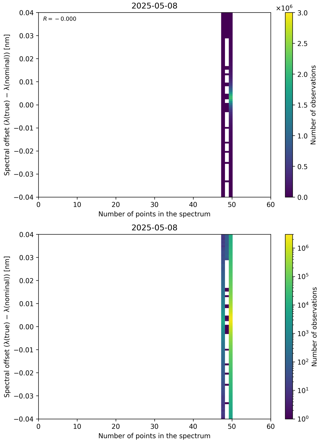
Figure 101: Scatter density plot of “Number of points in the spectrum” against “Spectral offset ( \lambda_{\text{true}} - \lambda_{\text{nominal}} )” for 2025-05-07 to 2025-05-09.
