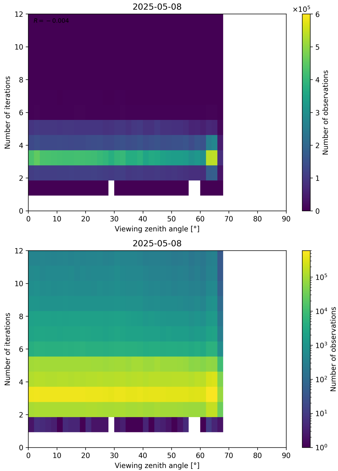
Figure 124: Scatter density plot of “Viewing zenith angle” against “Number of iterations” for 2025-05-07 to 2025-05-09.
