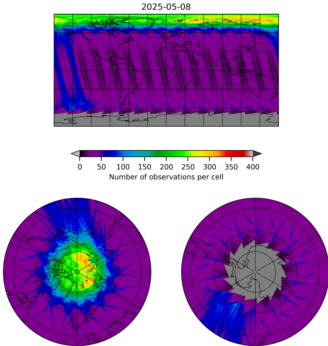
Figure 11: Map of the number of observations for 2025-05-07 to 2025-05-09
