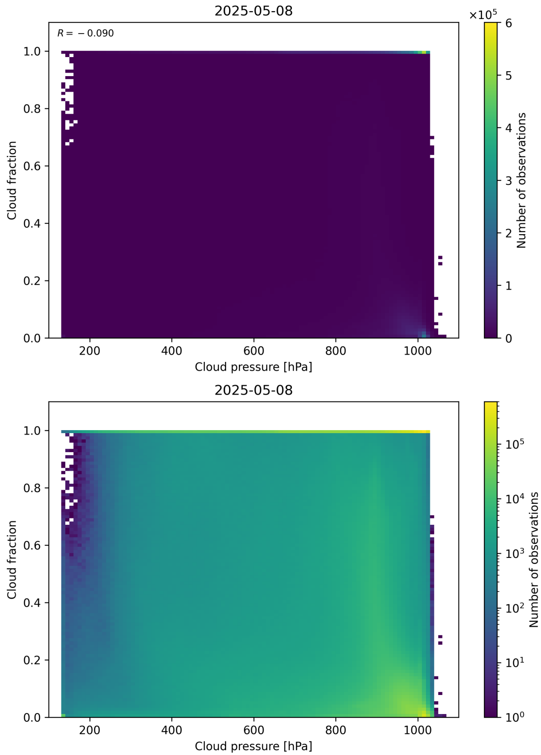
Figure 79: Scatter density plot of “Cloud pressure” against “Cloud fraction” for 2025-05-07 to 2025-05-09.
