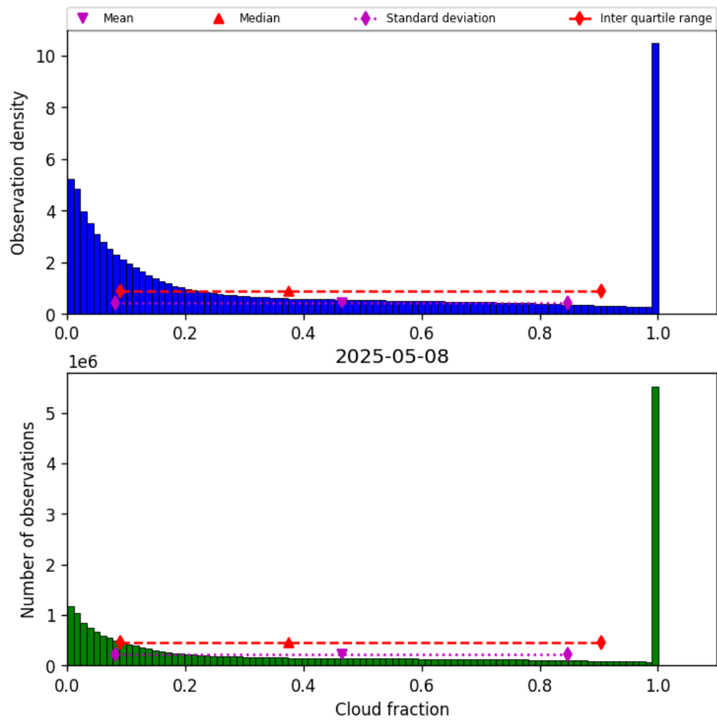
Figure 32: Histogram of “Cloud fraction” for 2025-05-07 to 2025-05-09
