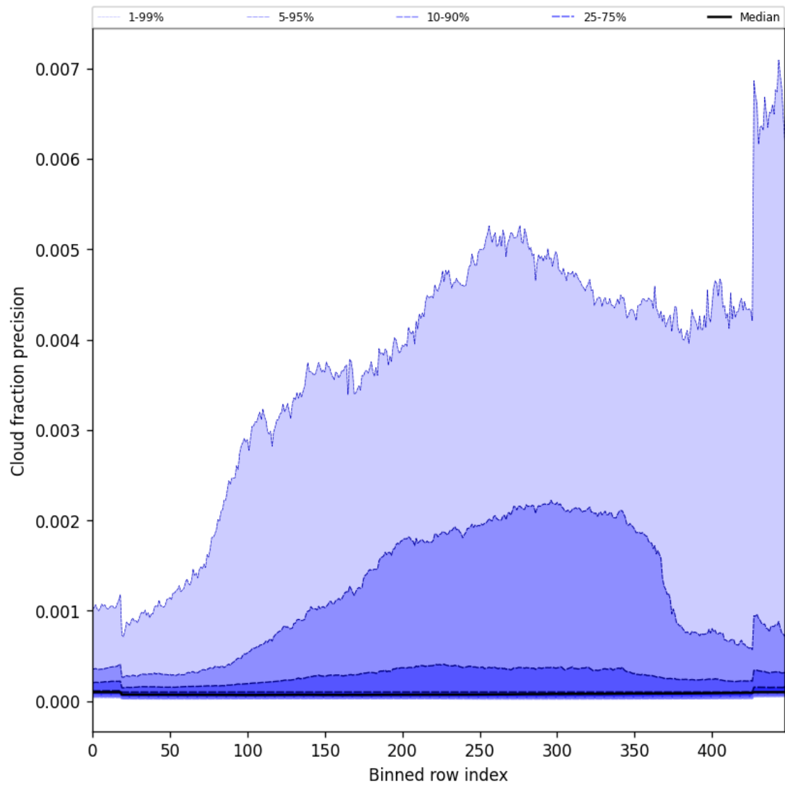
Figure 50: Along track statistics of “Cloud fraction precision” for 2025-05-07 to 2025-05-09
