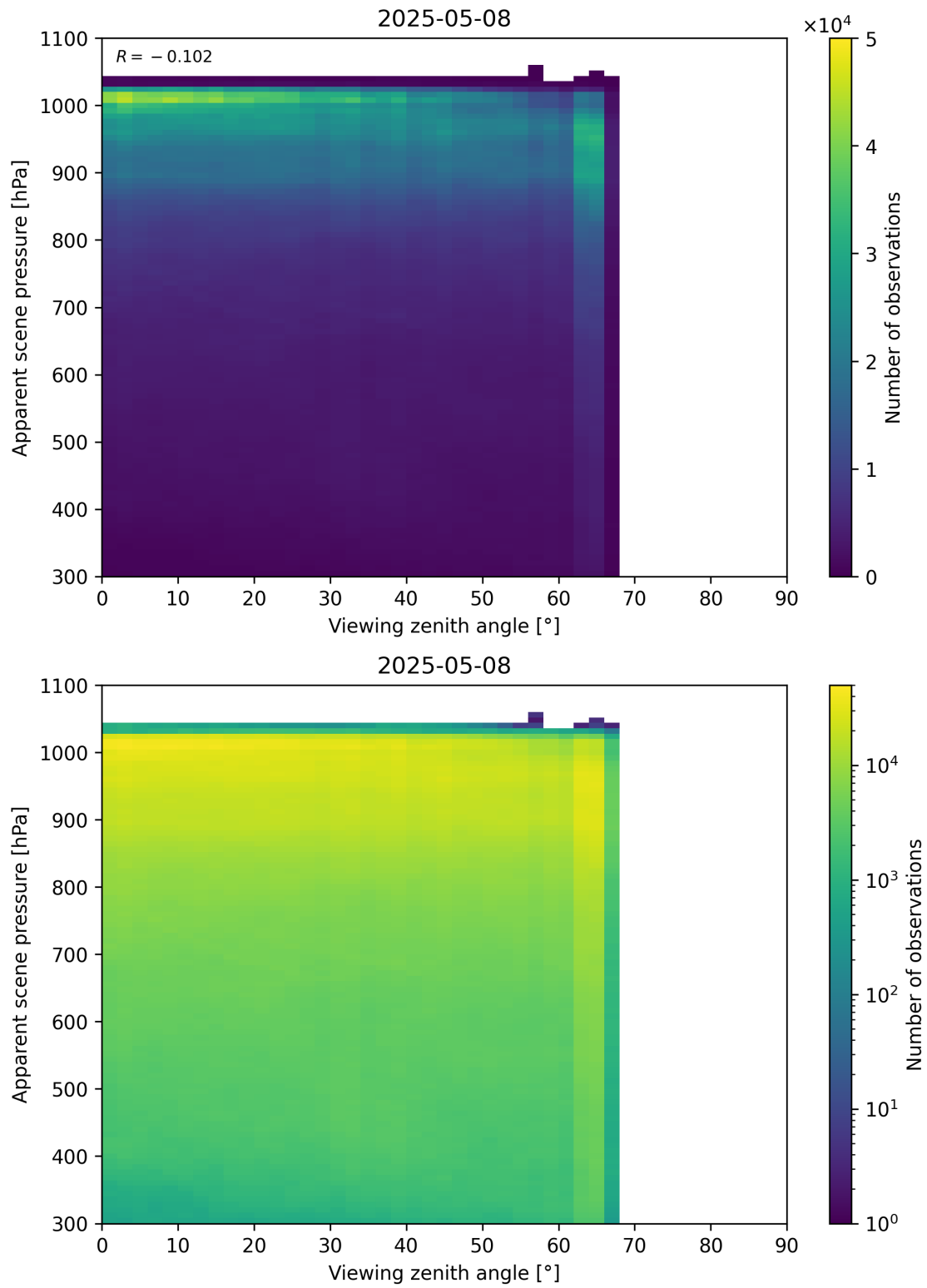
Figure 118: Scatter density plot of “Viewing zenith angle” against “Apparent scene pressure” for 2025-05-07 to 2025-05-09.
