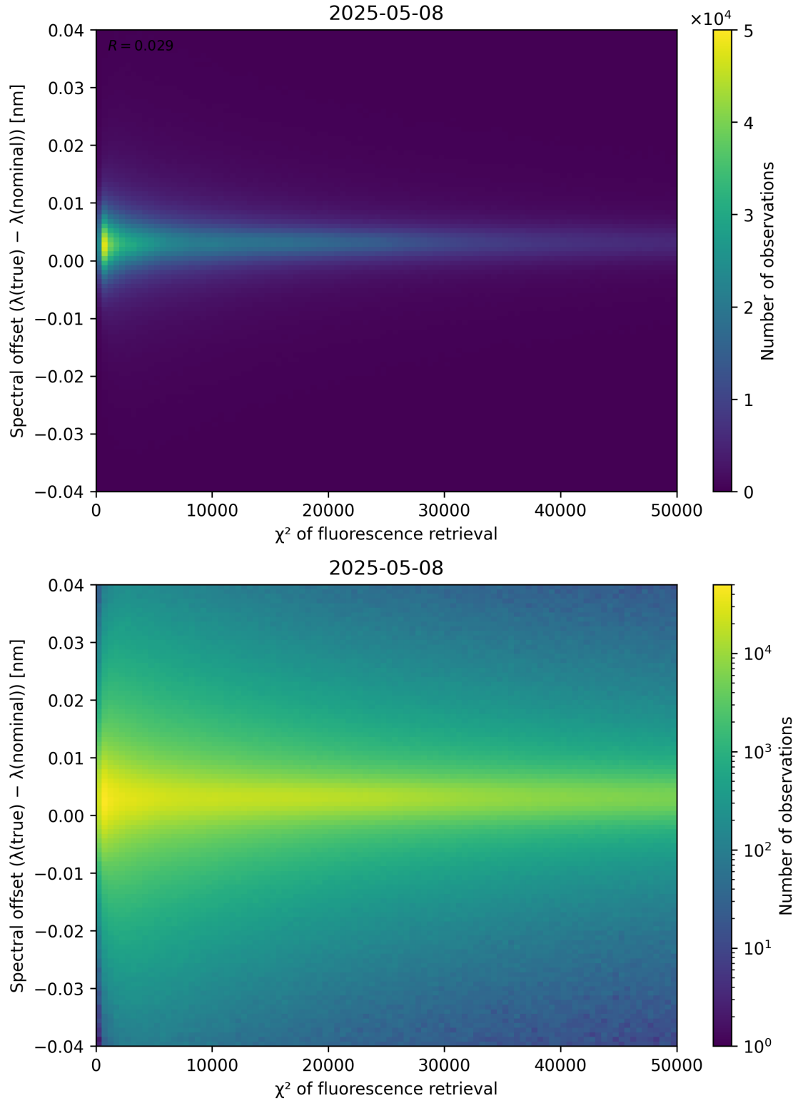
Figure 69: Scatter density plot of " \chi^2 of fluorescence retrieval" against "Spectral offset ( \lambda_{\text{true}} - \lambda_{\text{nominal}} )" for 2025-05-07 to 2025-05-09.
