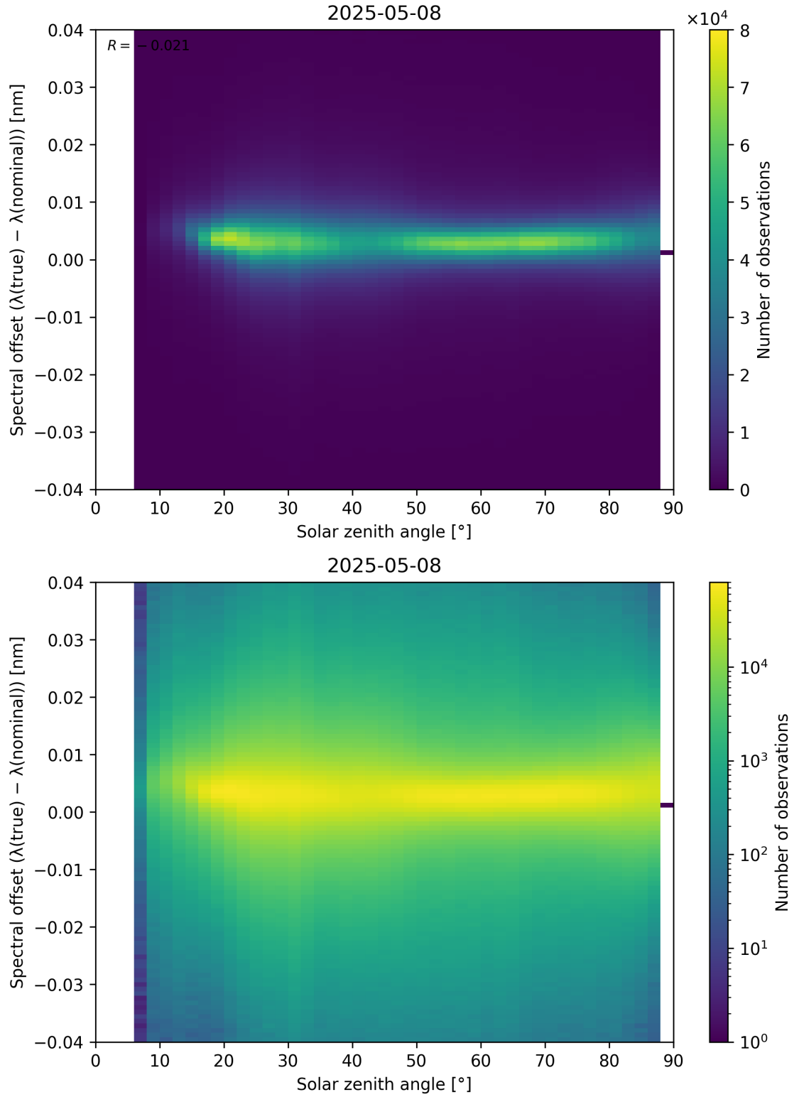
Figure 117: Scatter density plot of “Solar zenith angle” against “Spectral offset ( \lambda_{\text{true}} - \lambda_{\text{nominal}} )” for 2025-05-07 to 2025-05-09.
