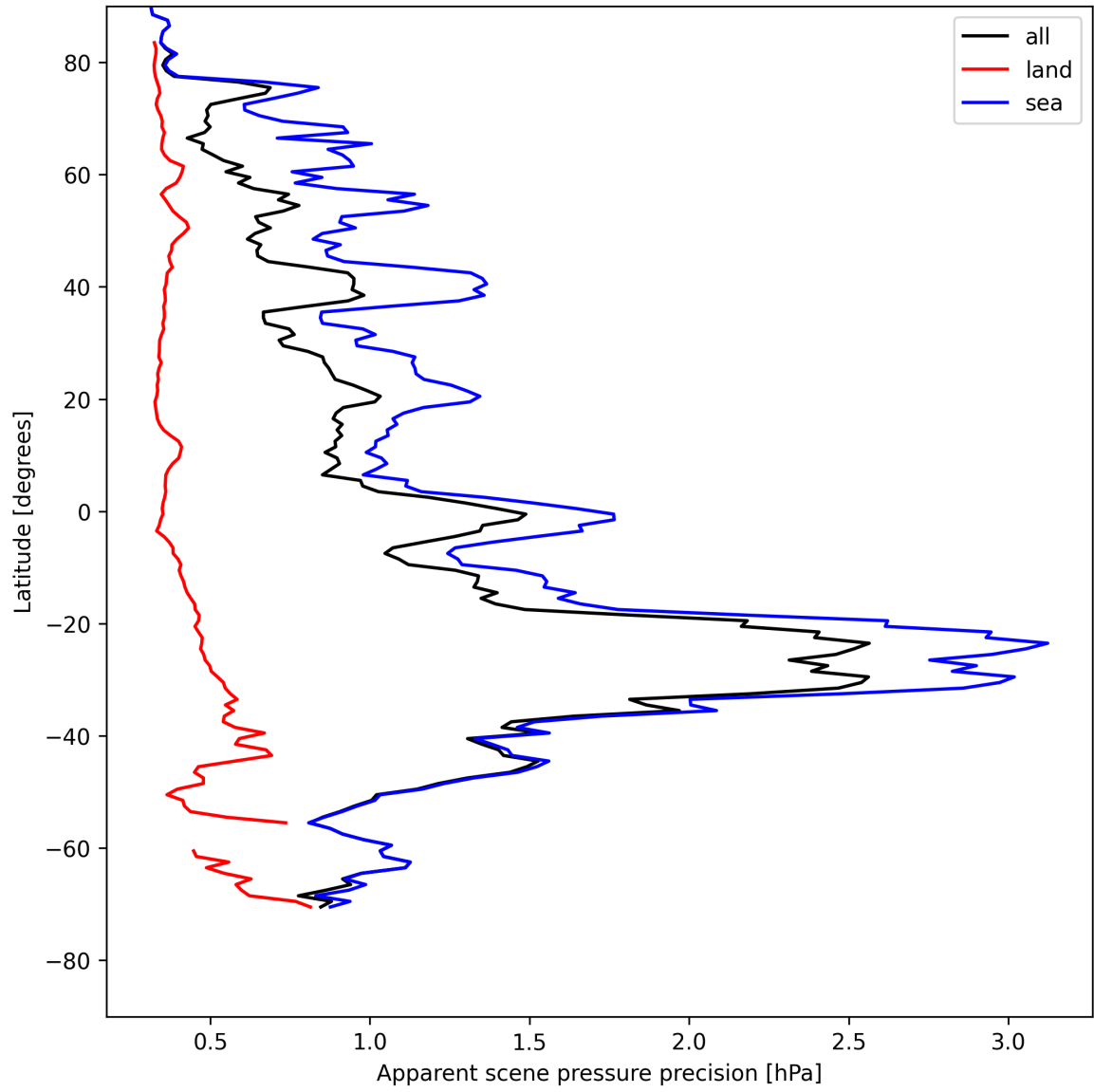
Figure 20: Zonal average of “Apparent scene pressure precision” for 2025-05-07 to 2025-05-09.
