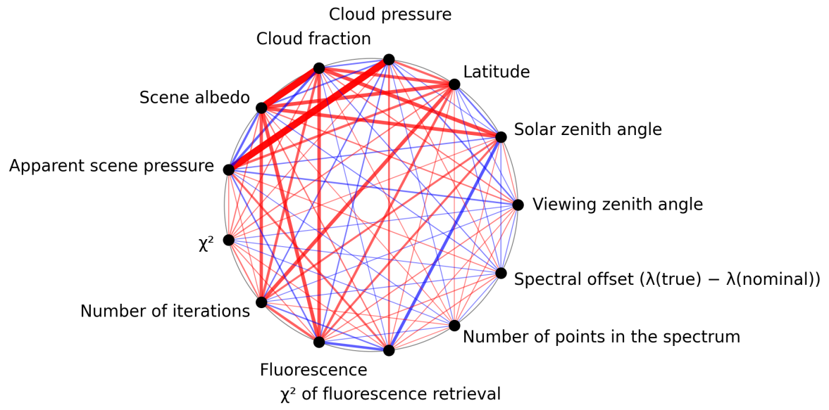
Figure 1: Map of correlation graph for 2025-05-07 to 2025-05-09.
