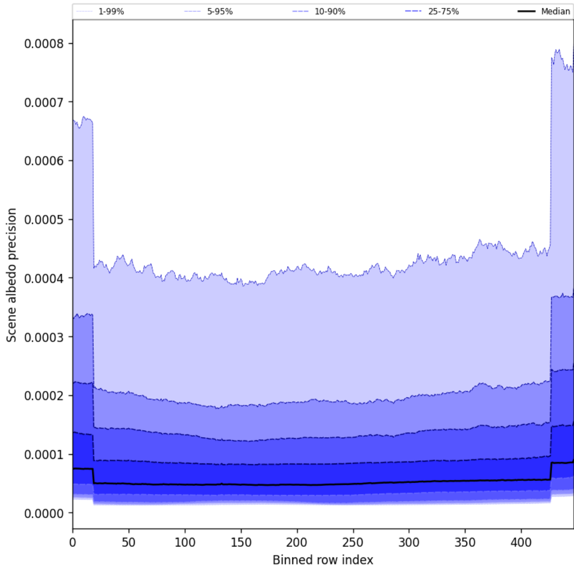
Figure 52: Along track statistics of “Scene albedo precision” for 2025-05-07 to 2025-05-09
