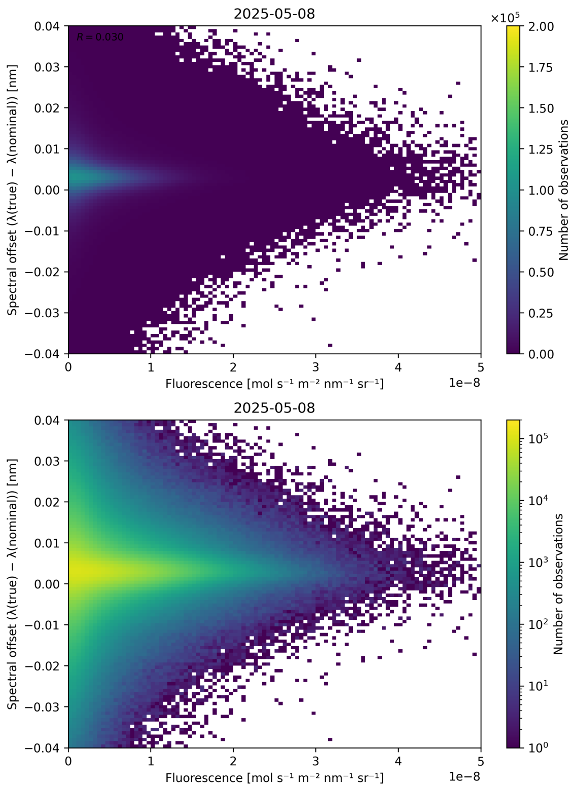
Figure 87: Scatter density plot of “Fluorescence” against “Spectral offset ( \lambda_{\text{true}} - \lambda_{\text{nominal}} )” for 2025-05-07 to 2025-05-09.
