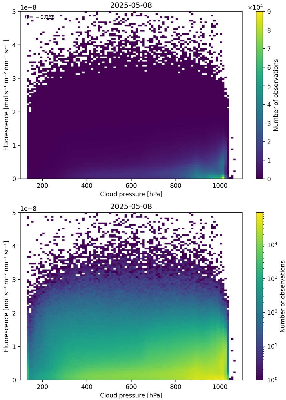
Figure 80: Scatter density plot of “Cloud pressure” against “Fluorescence” for 2025-05-07 to 2025-05-09.
