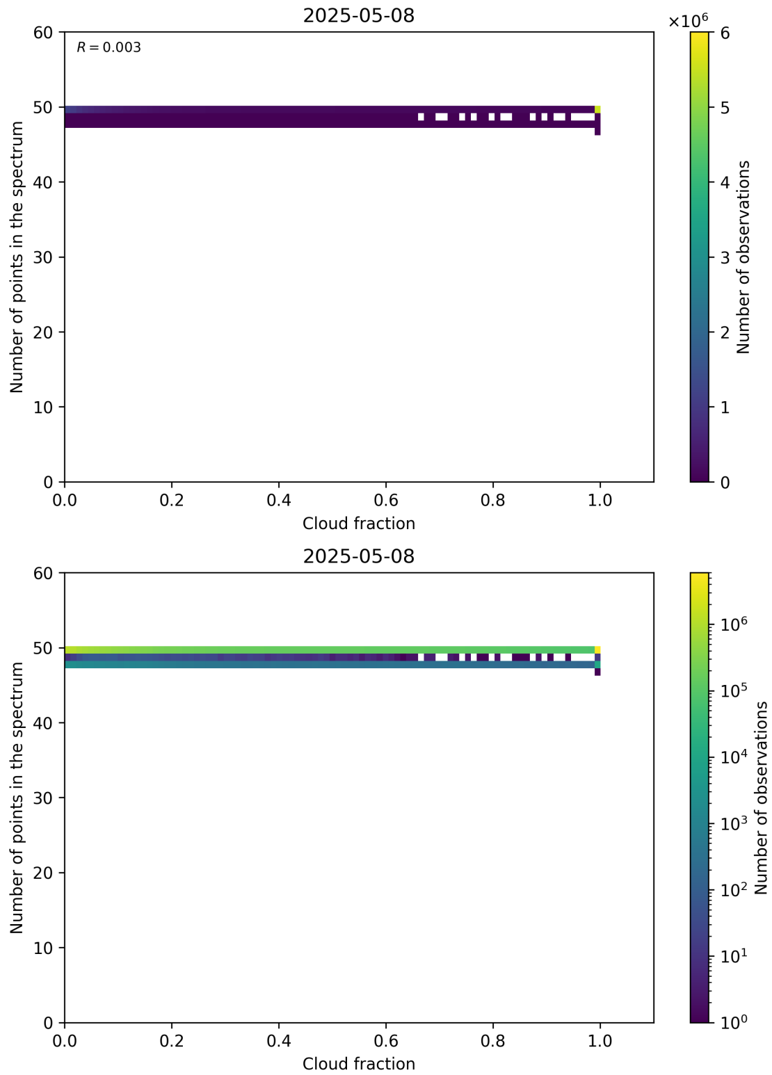
Figure 74: Scatter density plot of “Cloud fraction” against “Number of points in the spectrum” for 2025-05-07 to 2025-05-09.
