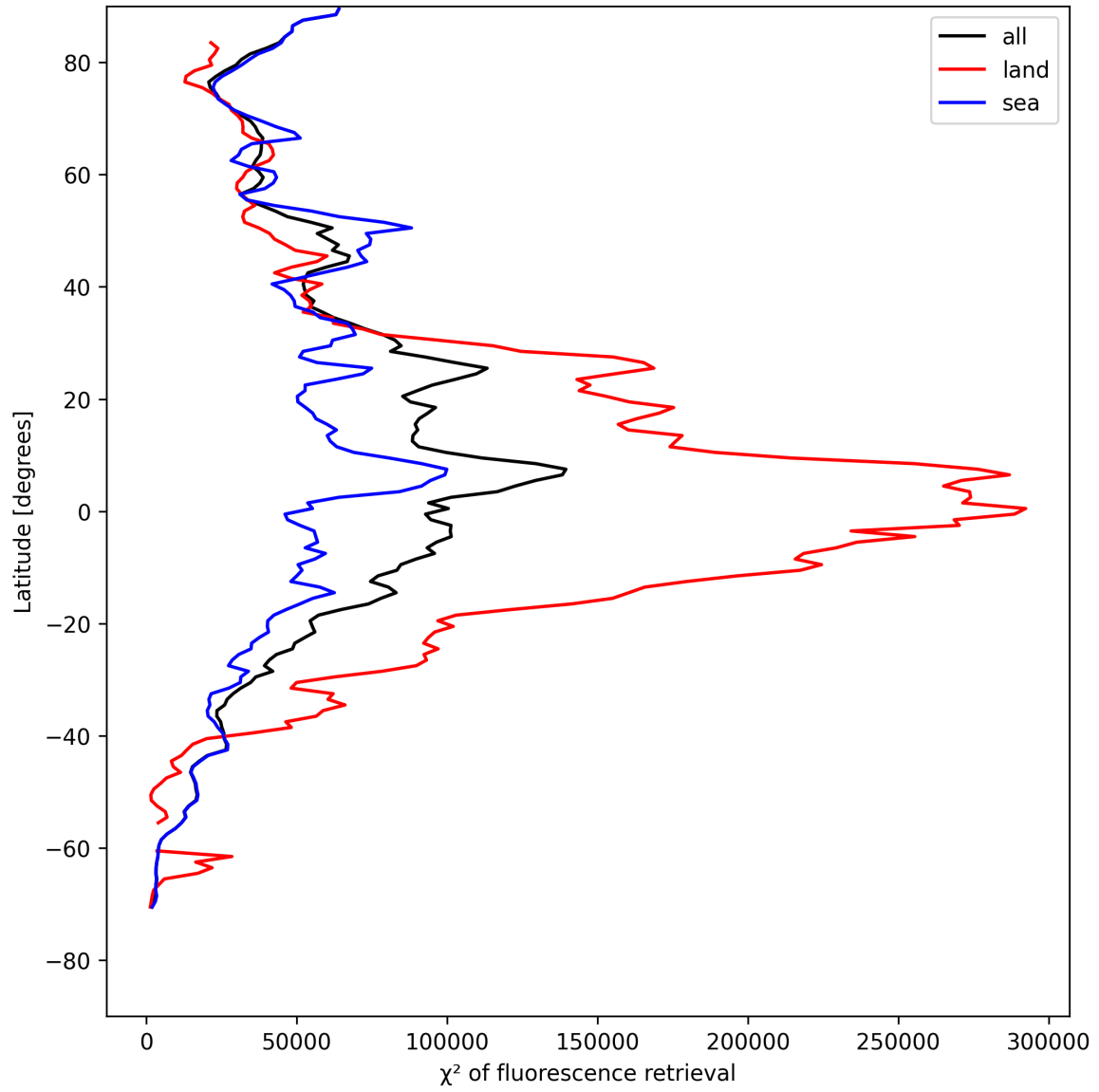
Figure 25: Zonal average of “ \chi^2 of fluorescence retrieval” for 2025-05-07 to 2025-05-09.
