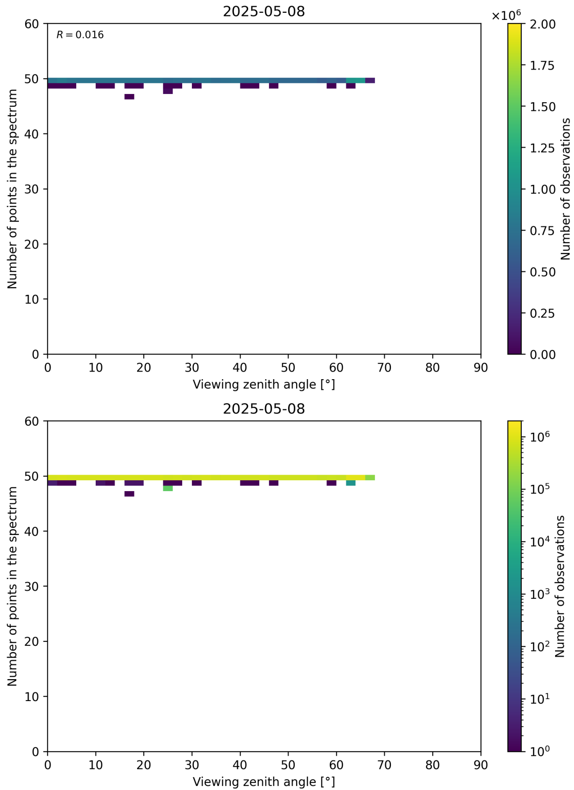
Figure 125: Scatter density plot of “Viewing zenith angle” against “Number of points in the spectrum” for 2025-05-07 to 2025-05-09.
