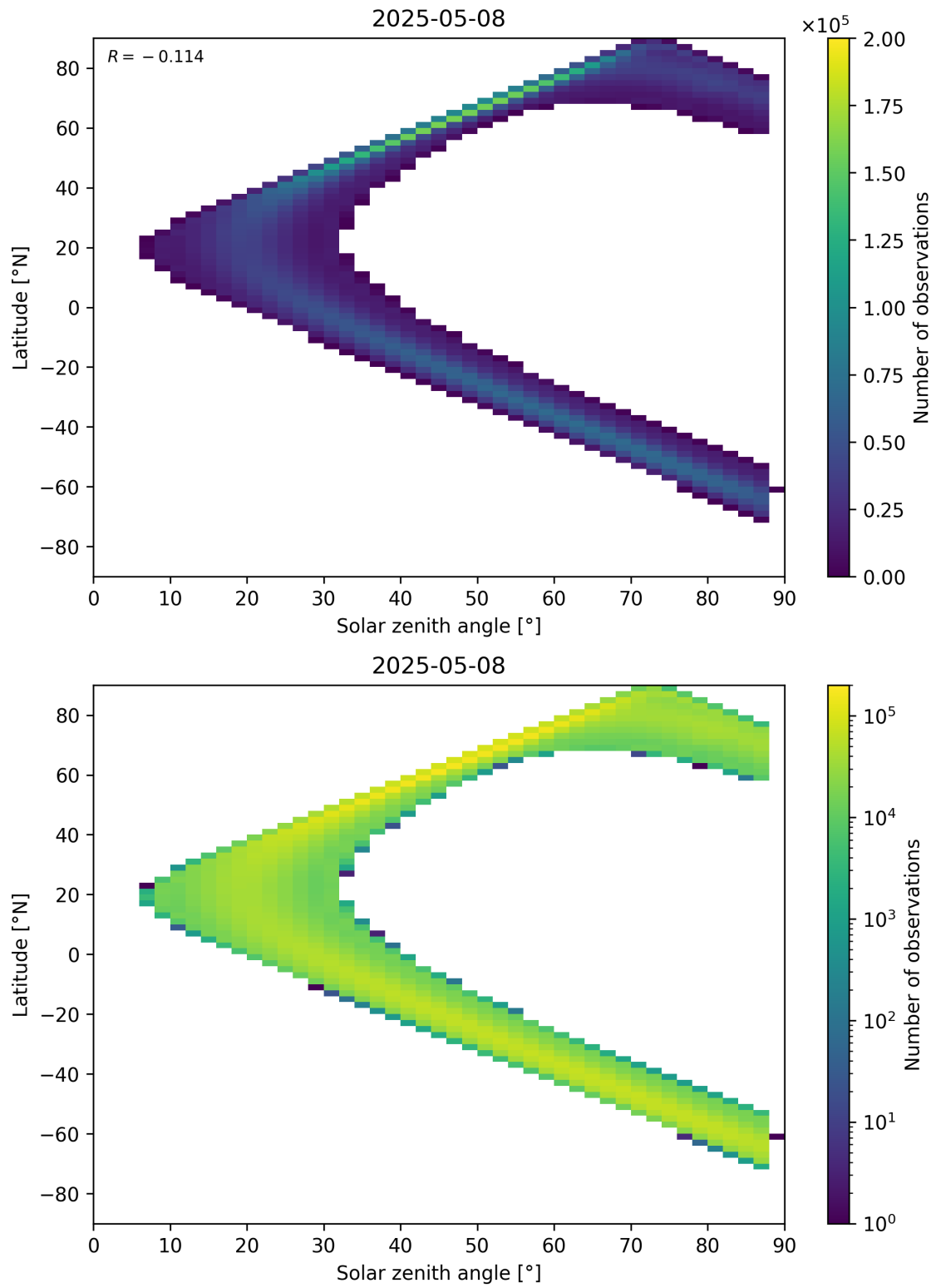
Figure 113: Scatter density plot of “Solar zenith angle” against “Latitude” for 2025-05-07 to 2025-05-09.
