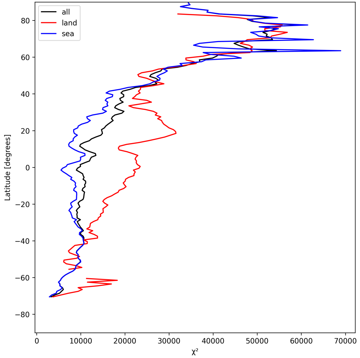
Figure 21: Zonal average of “ \chi^2 ” for 2025-05-07 to 2025-05-09.
