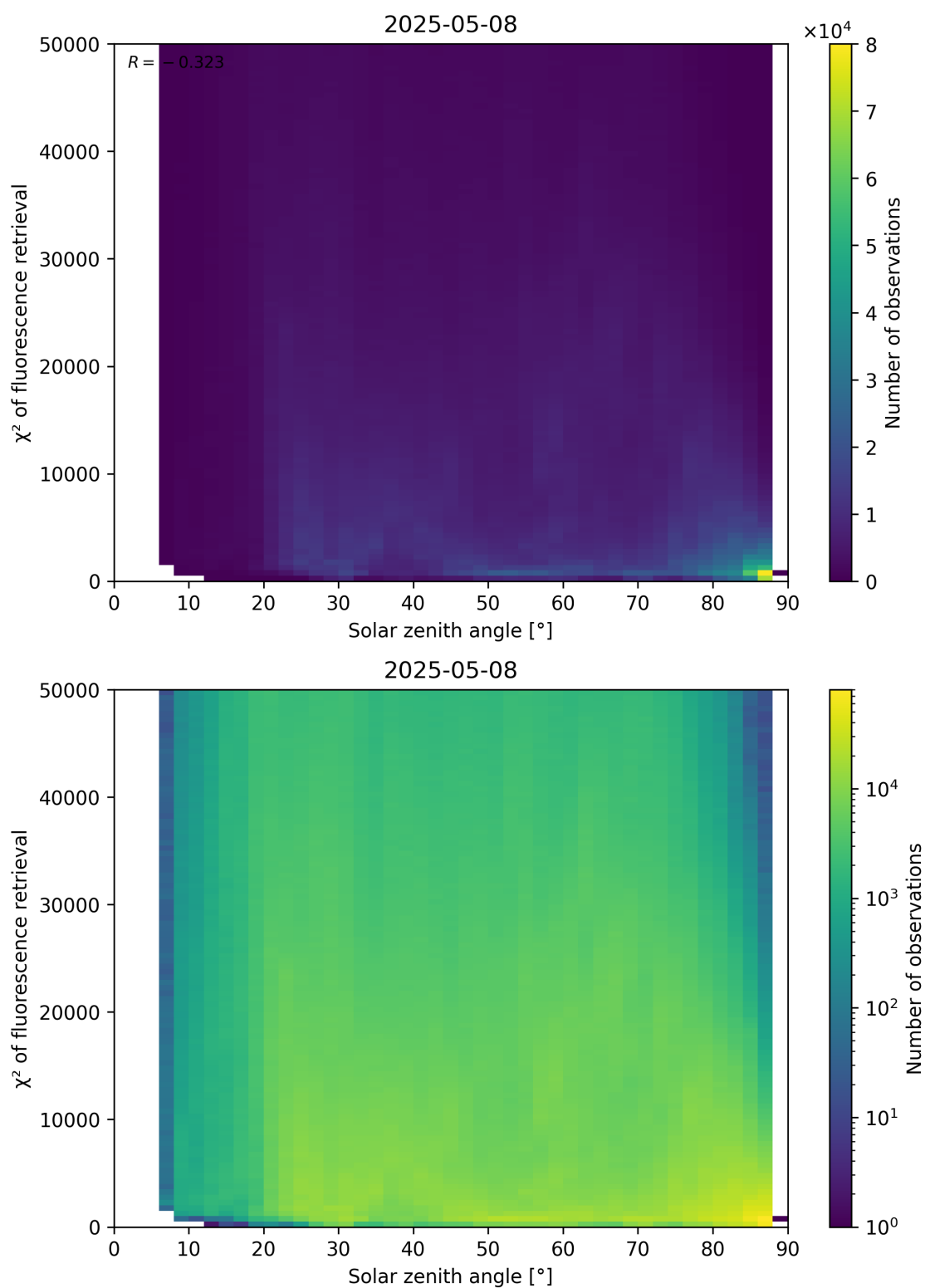
Figure 109: Scatter density plot of “Solar zenith angle” against “ \chi^2 of fluorescence retrieval” for 2025-05-07 to 2025-05-09.
