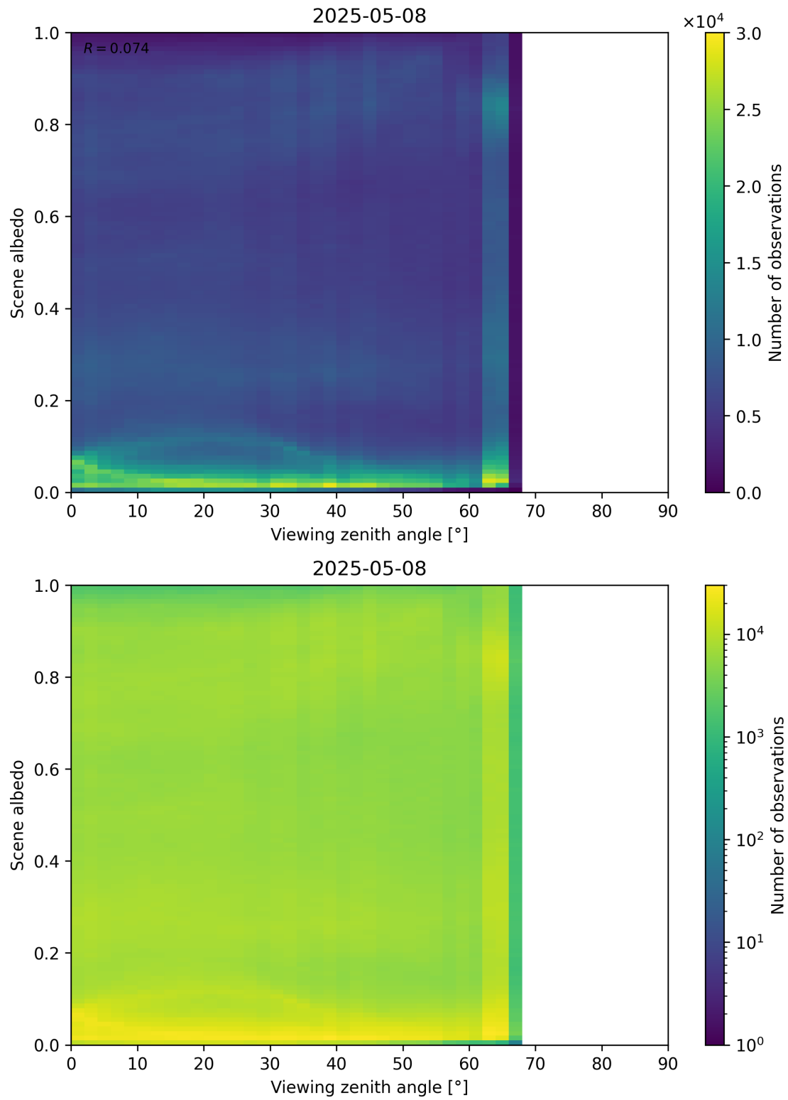
Figure 126: Scatter density plot of “Viewing zenith angle” against “Scene albedo” for 2025-05-07 to 2025-05-09.
