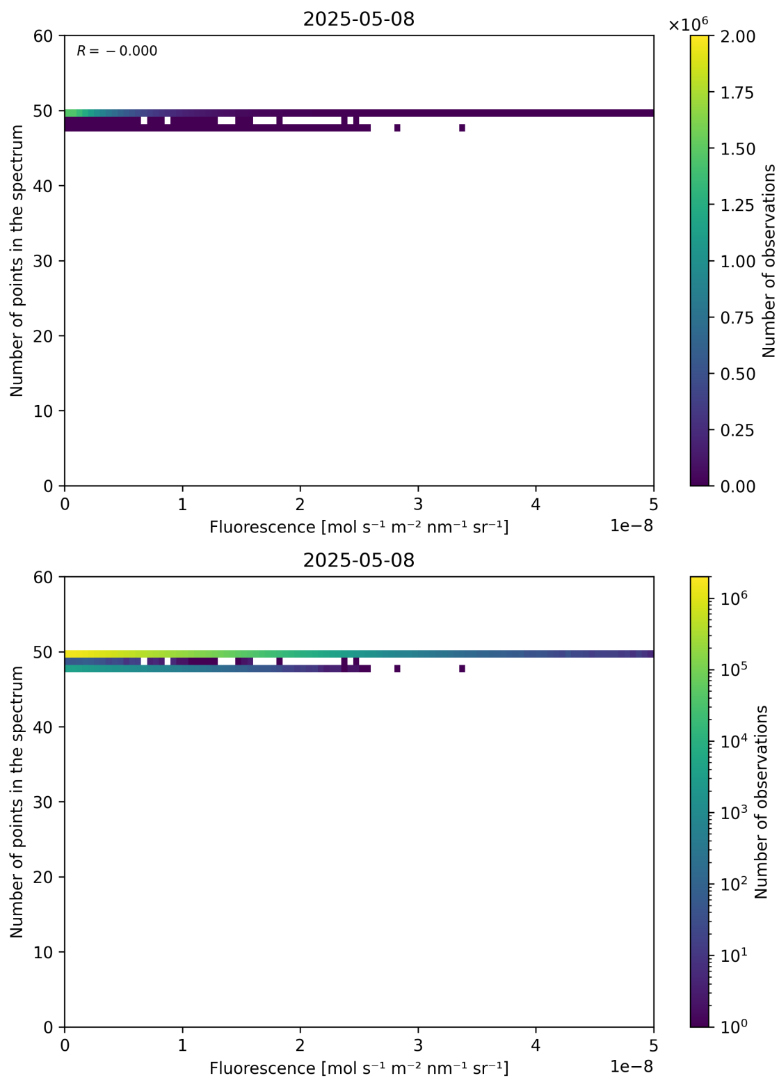
Figure 86: Scatter density plot of “Fluorescence” against “Number of points in the spectrum” for 2025-05-07 to 2025-05-09.
