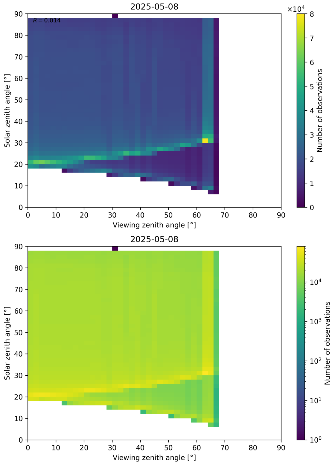
Figure 127: Scatter density plot of “Viewing zenith angle” against “Solar zenith angle” for 2025-05-07 to 2025-05-09.
