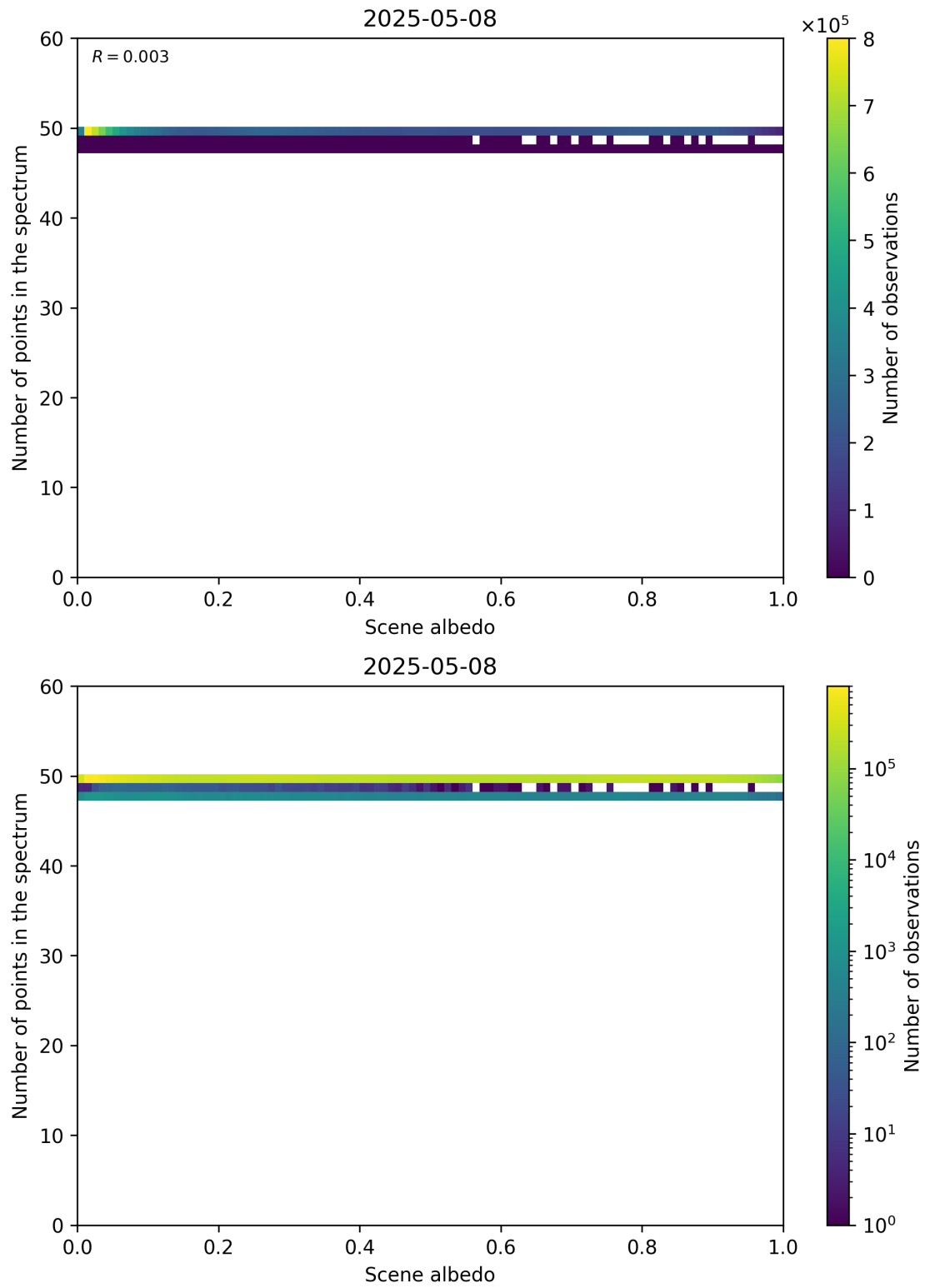
Figure 106: Scatter density plot of “Scene albedo” against “Number of points in the spectrum” for 2025-05-07 to 2025-05-09.
