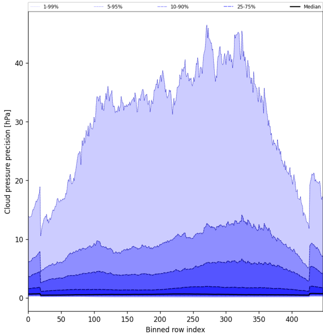
Figure 48: Along track statistics of “Cloud pressure precision” for 2025-05-07 to 2025-05-09
