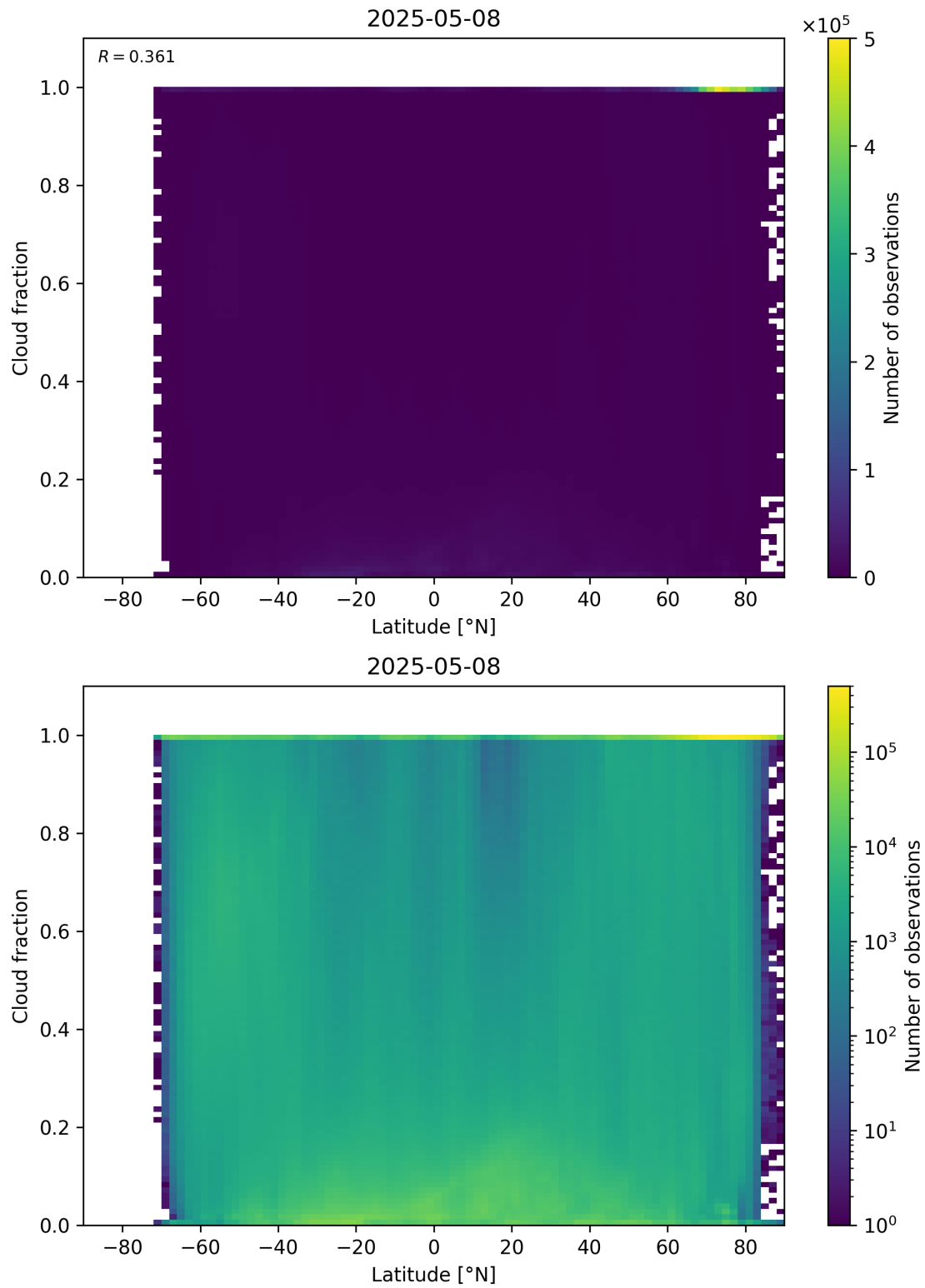
Figure 90: Scatter density plot of “Latitude” against “Cloud fraction” for 2025-05-07 to 2025-05-09.
