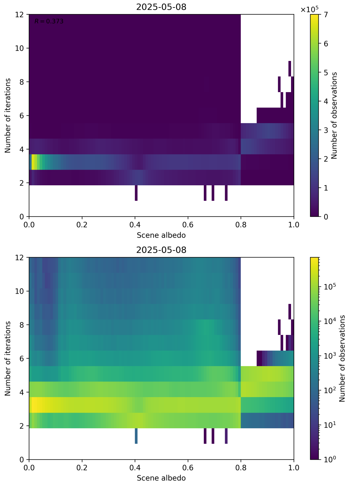
Figure 105: Scatter density plot of “Scene albedo” against “Number of iterations” for 2025-05-07 to 2025-05-09.
