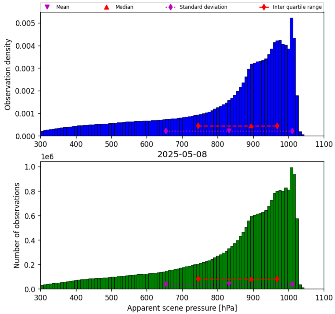
Figure 36: Histogram of “Apparent scene pressure” for 2025-05-07 to 2025-05-09
