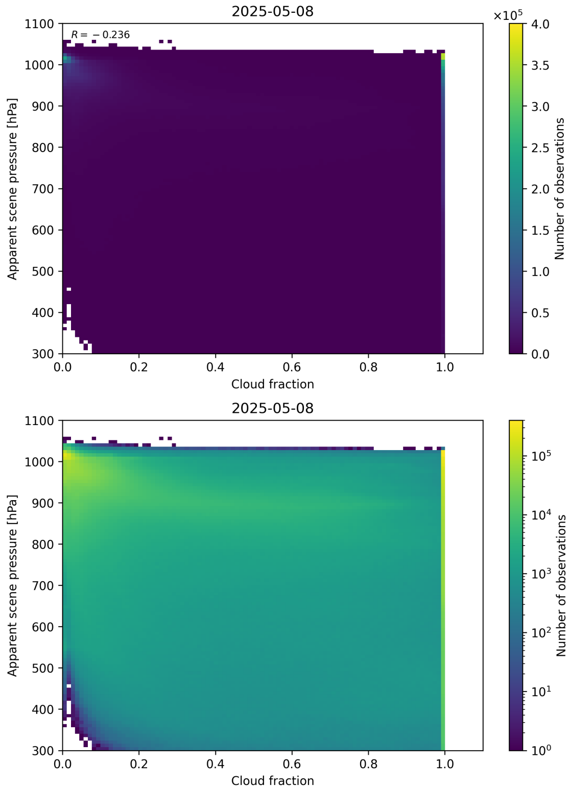
Figure 70: Scatter density plot of “Cloud fraction” against “Apparent scene pressure” for 2025-05-07 to 2025-05-09.
