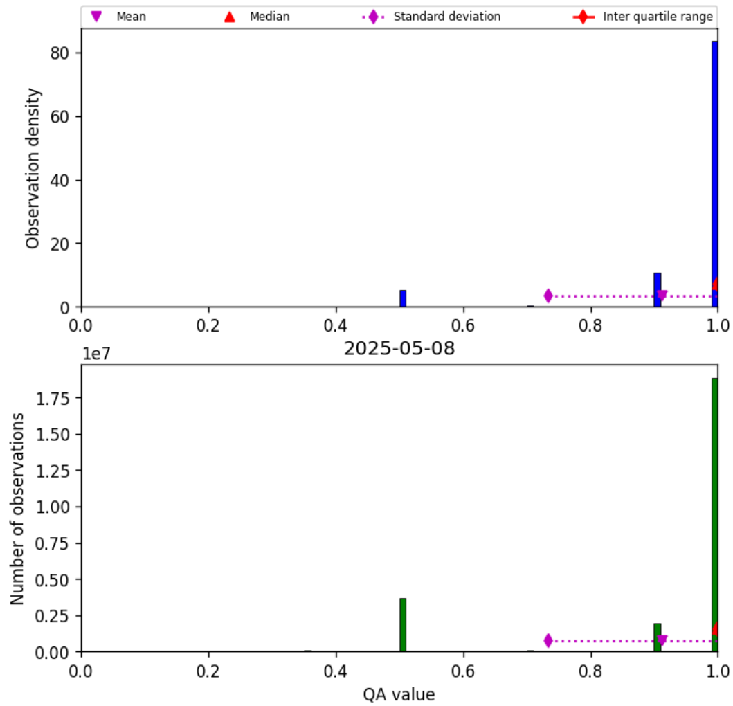
Figure 29: Histogram of “QA value” for 2025-05-07 to 2025-05-09
