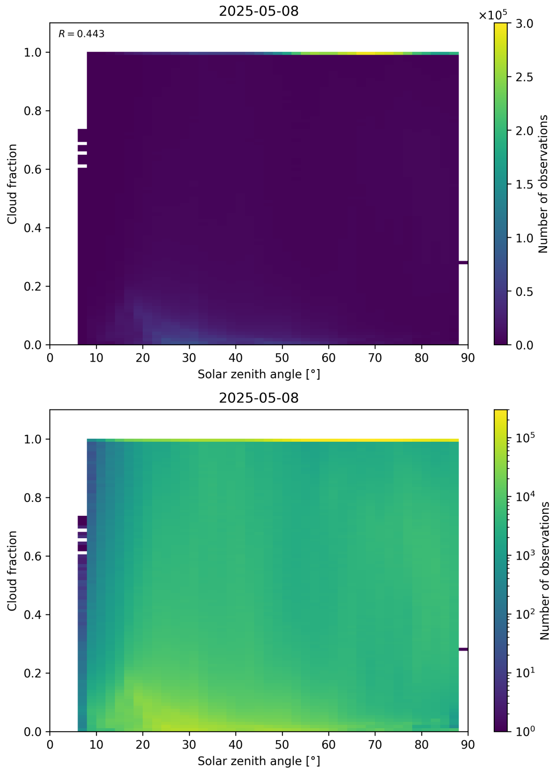
Figure 110: Scatter density plot of “Solar zenith angle” against “Cloud fraction” for 2025-05-07 to 2025-05-09.
