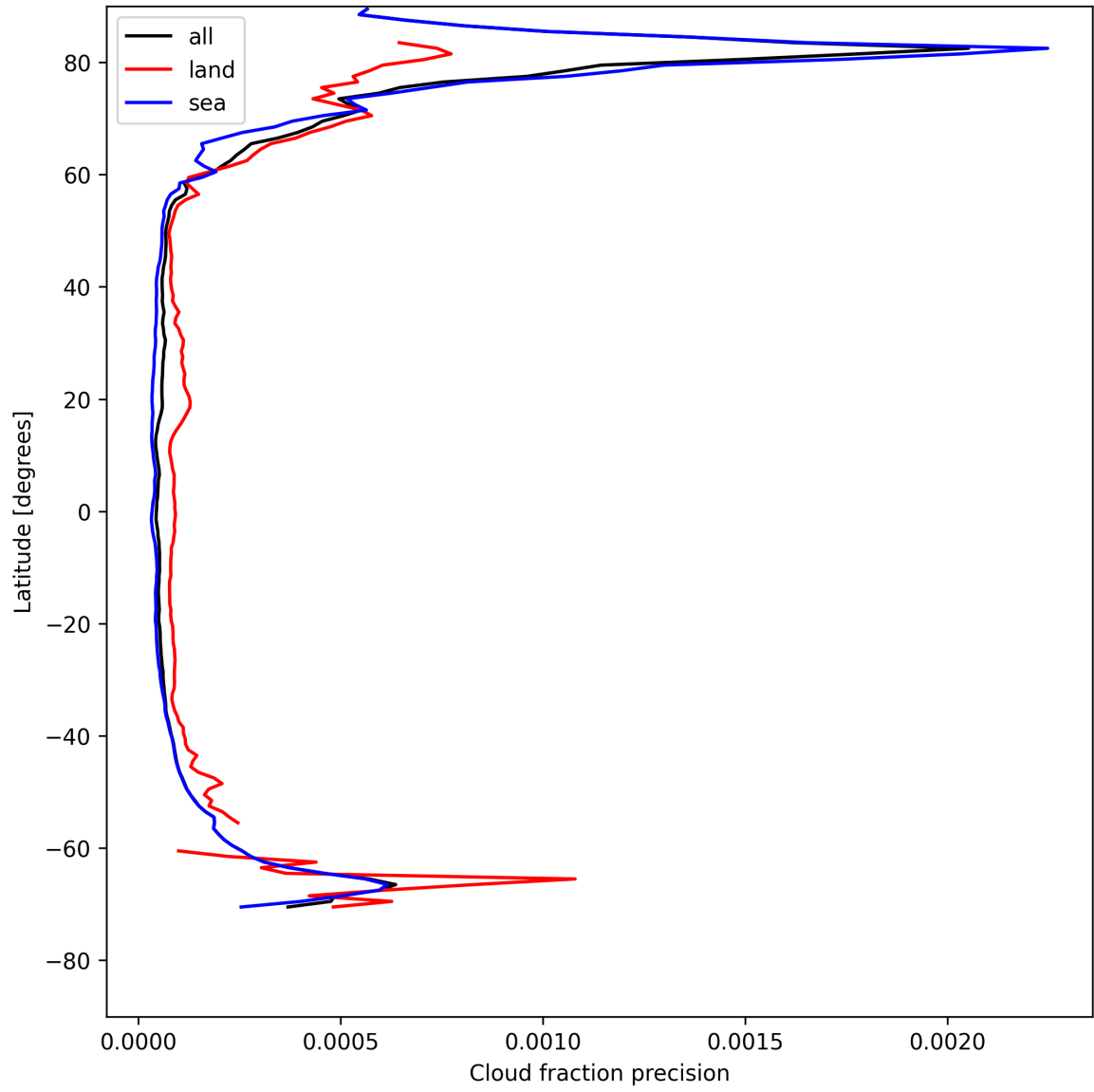
Figure 16: Zonal average of “Cloud fraction precision” for 2025-05-07 to 2025-05-09.
