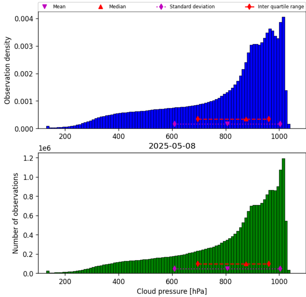
Figure 30: Histogram of “Cloud pressure” for 2025-05-07 to 2025-05-09
