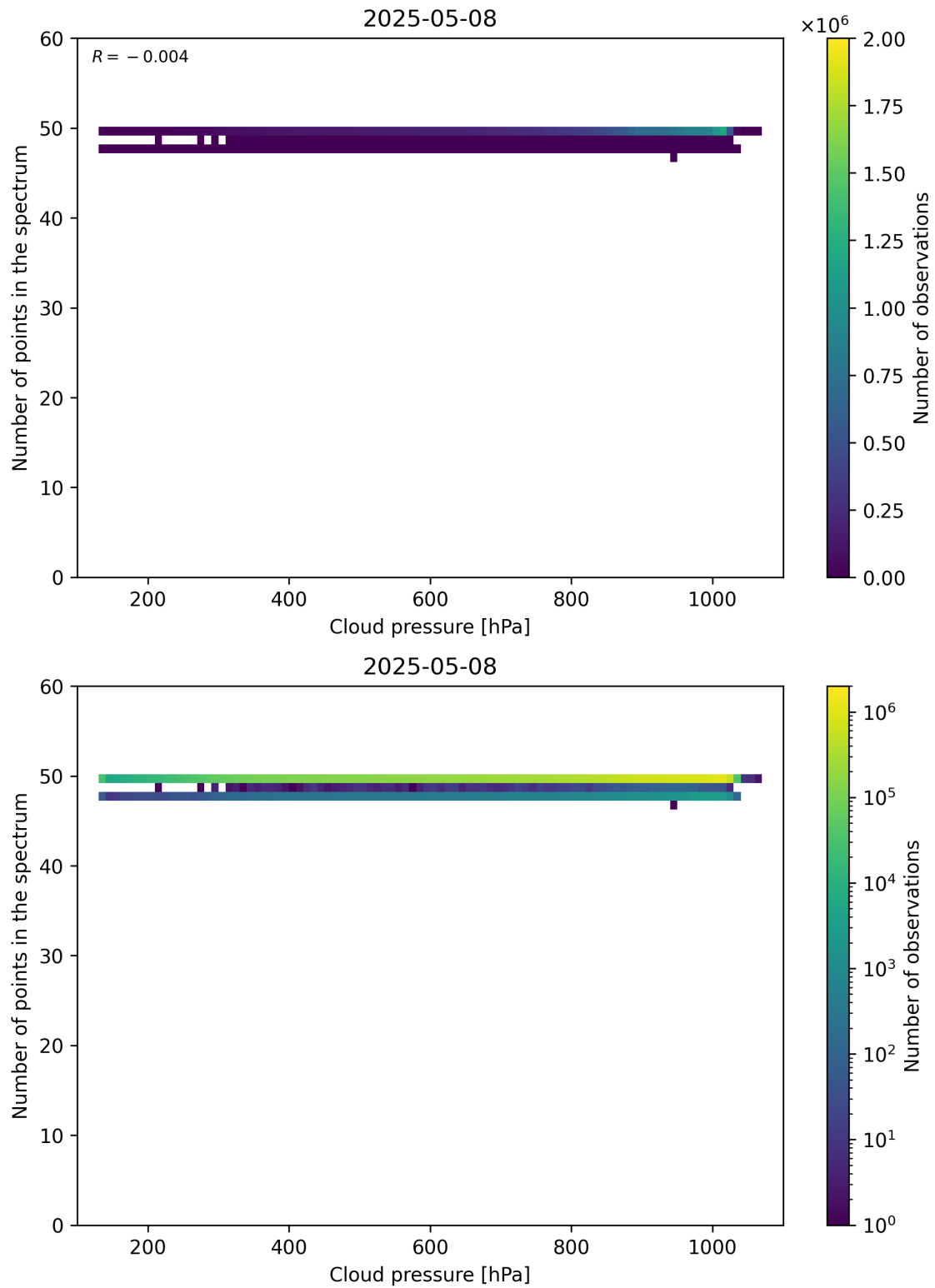
Figure 82: Scatter density plot of “Cloud pressure” against “Number of points in the spectrum” for 2025-05-07 to 2025-05-09.
