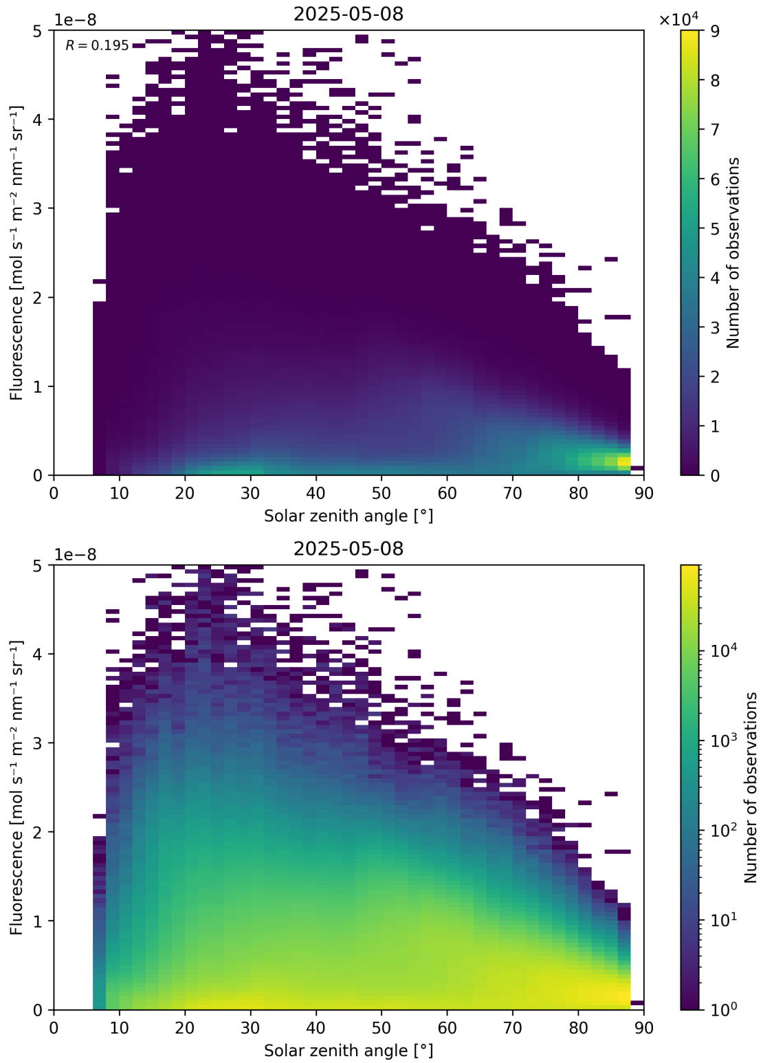
Figure 112: Scatter density plot of “Solar zenith angle” against “Fluorescence” for 2025-05-07 to 2025-05-09.
