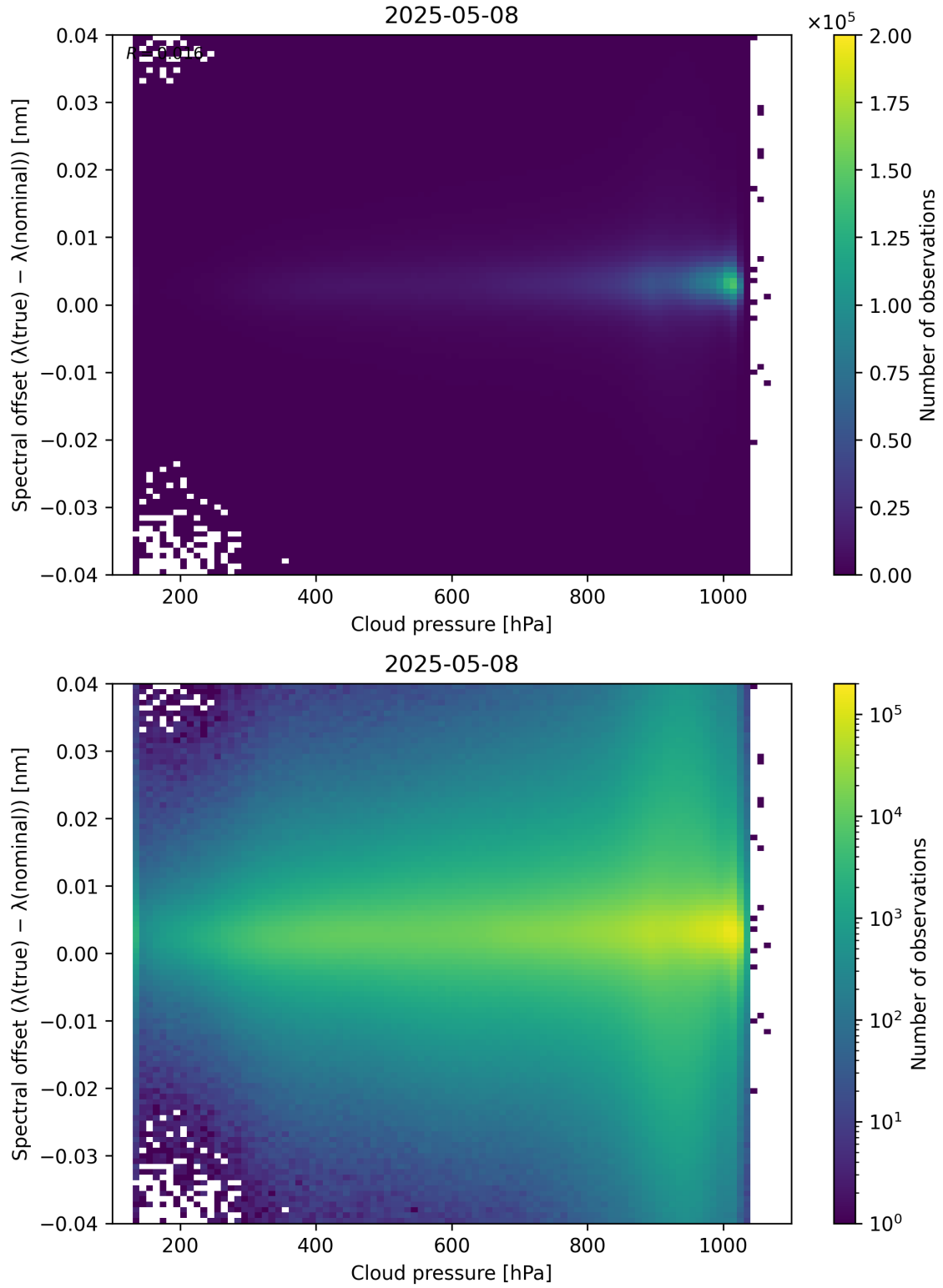
Figure 84: Scatter density plot of “Cloud pressure” against “Spectral offset ( \lambda_{\text{true}} - \lambda_{\text{nominal}} )” for 2025-05-07 to 2025-05-09.
