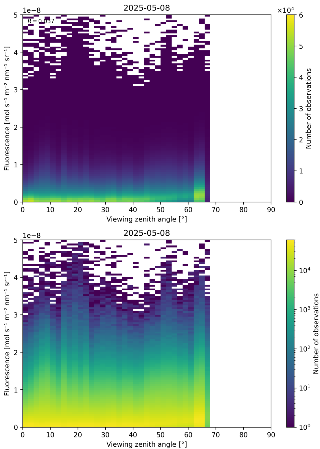
Figure 122: Scatter density plot of “Viewing zenith angle” against “Fluorescence” for 2025-05-07 to 2025-05-09.
