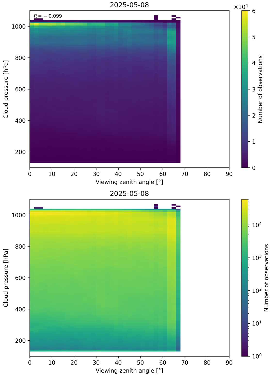
Figure 121: Scatter density plot of “Viewing zenith angle” against “Cloud pressure” for 2025-05-07 to 2025-05-09.
