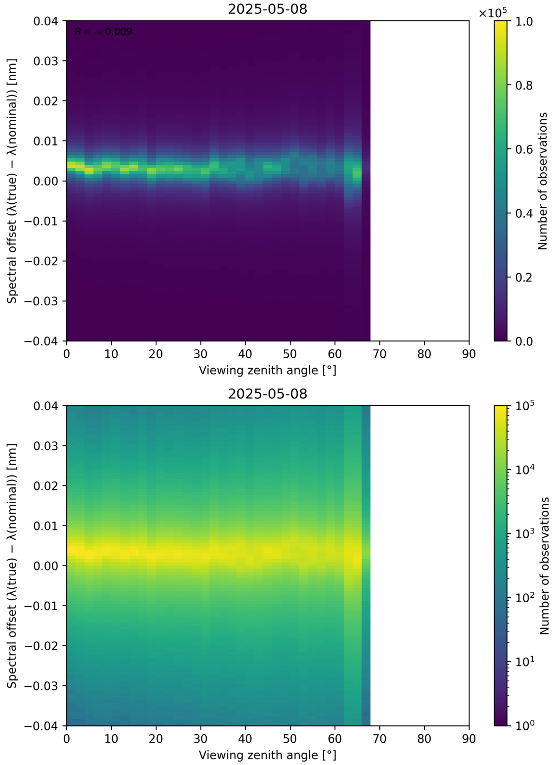
Figure 128: Scatter density plot of “Viewing zenith angle” against “Spectral offset ( \lambda_{\text{true}} - \lambda_{\text{nominal}} )” for 2025-05-07 to 2025-05-09.
