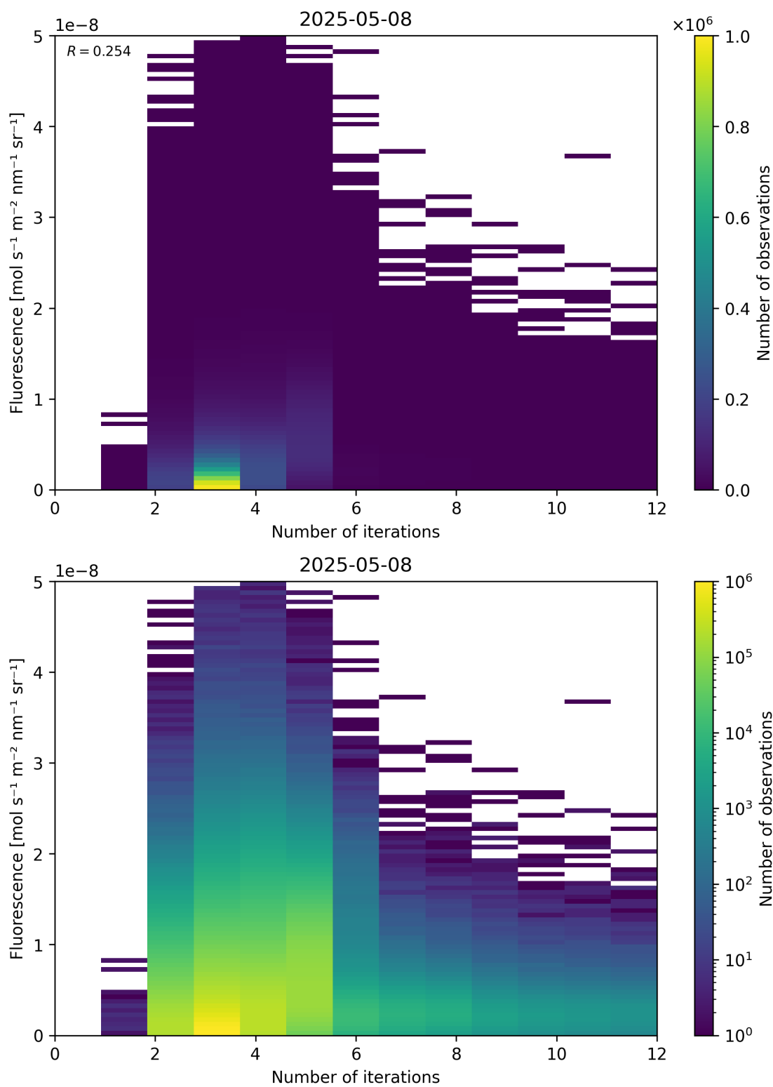
Figure 98: Scatter density plot of “Number of iterations” against “Fluorescence” for 2025-05-07 to 2025-05-09.
