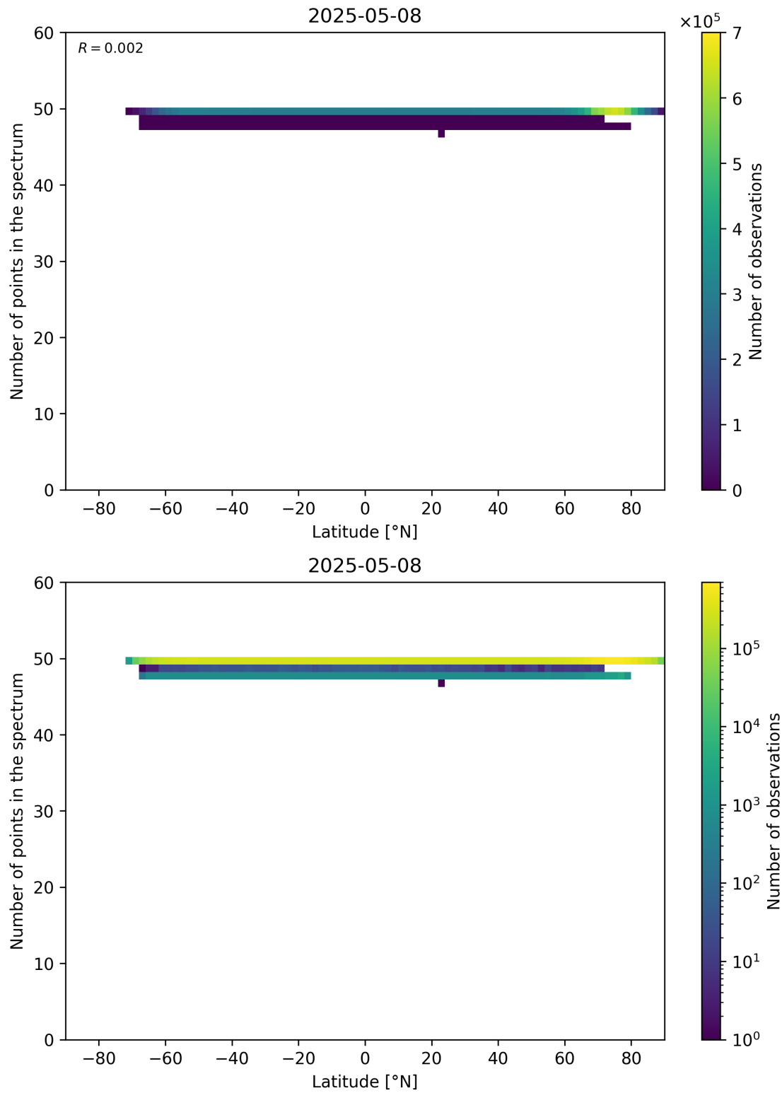
Figure 94: Scatter density plot of “Latitude” against “Number of points in the spectrum” for 2025-05-07 to 2025-05-09.
