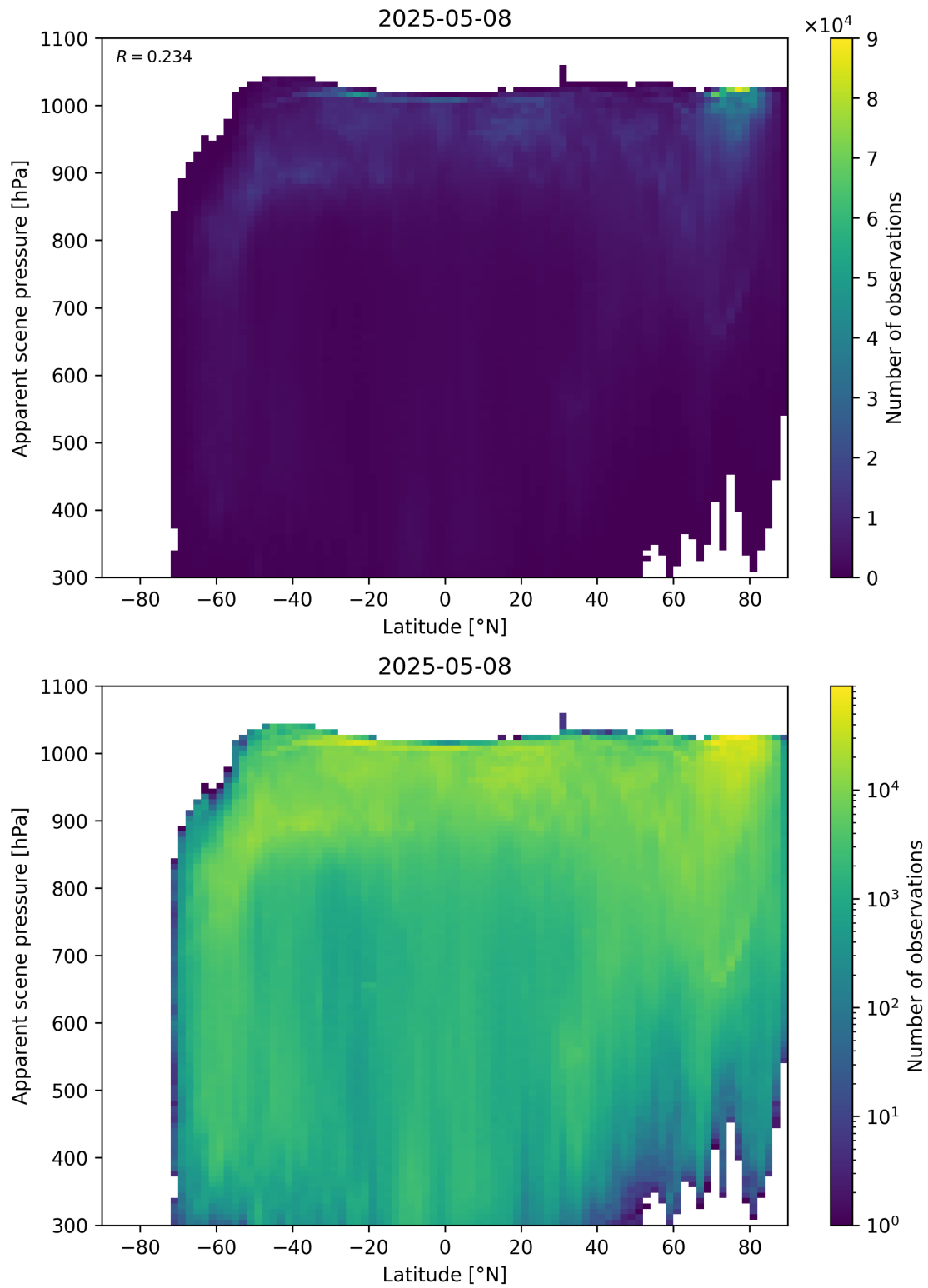
Figure 88: Scatter density plot of “Latitude” against “Apparent scene pressure” for 2025-05-07 to 2025-05-09.
