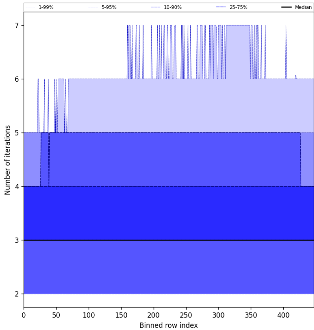
Figure 56: Along track statistics of “Number of iterations” for 2025-05-07 to 2025-05-09
