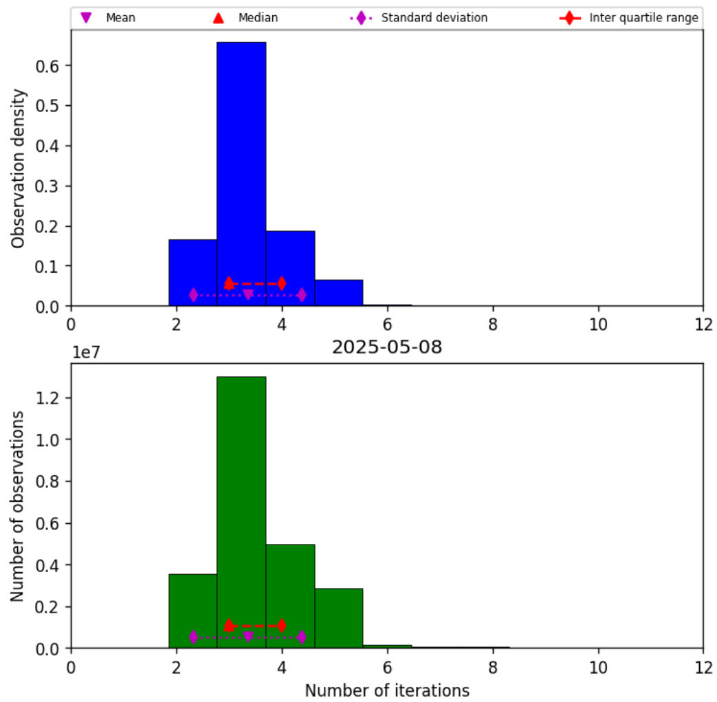
Figure 39: Histogram of “Number of iterations” for 2025-05-07 to 2025-05-09
