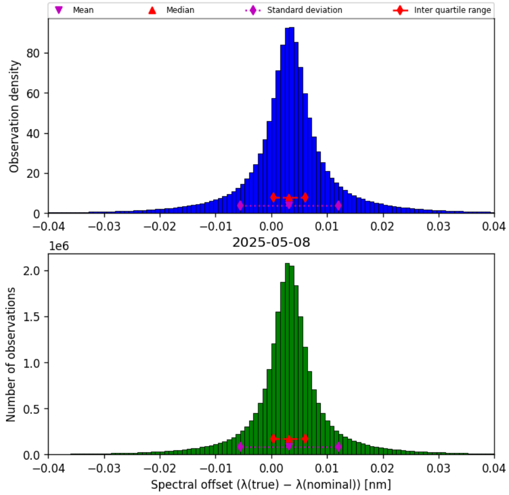
Figure 45: Histogram of “Spectral offset ( \lambda_{\text{true}} - \lambda_{\text{nominal}} )” for 2025-05-07 to 2025-05-09
