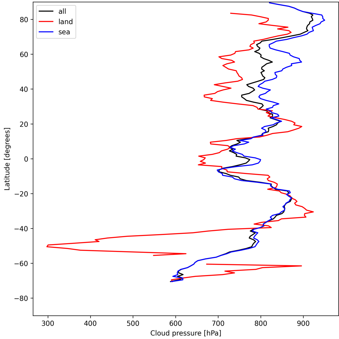
Figure 13: Zonal average of “Cloud pressure” for 2025-05-07 to 2025-05-09.
