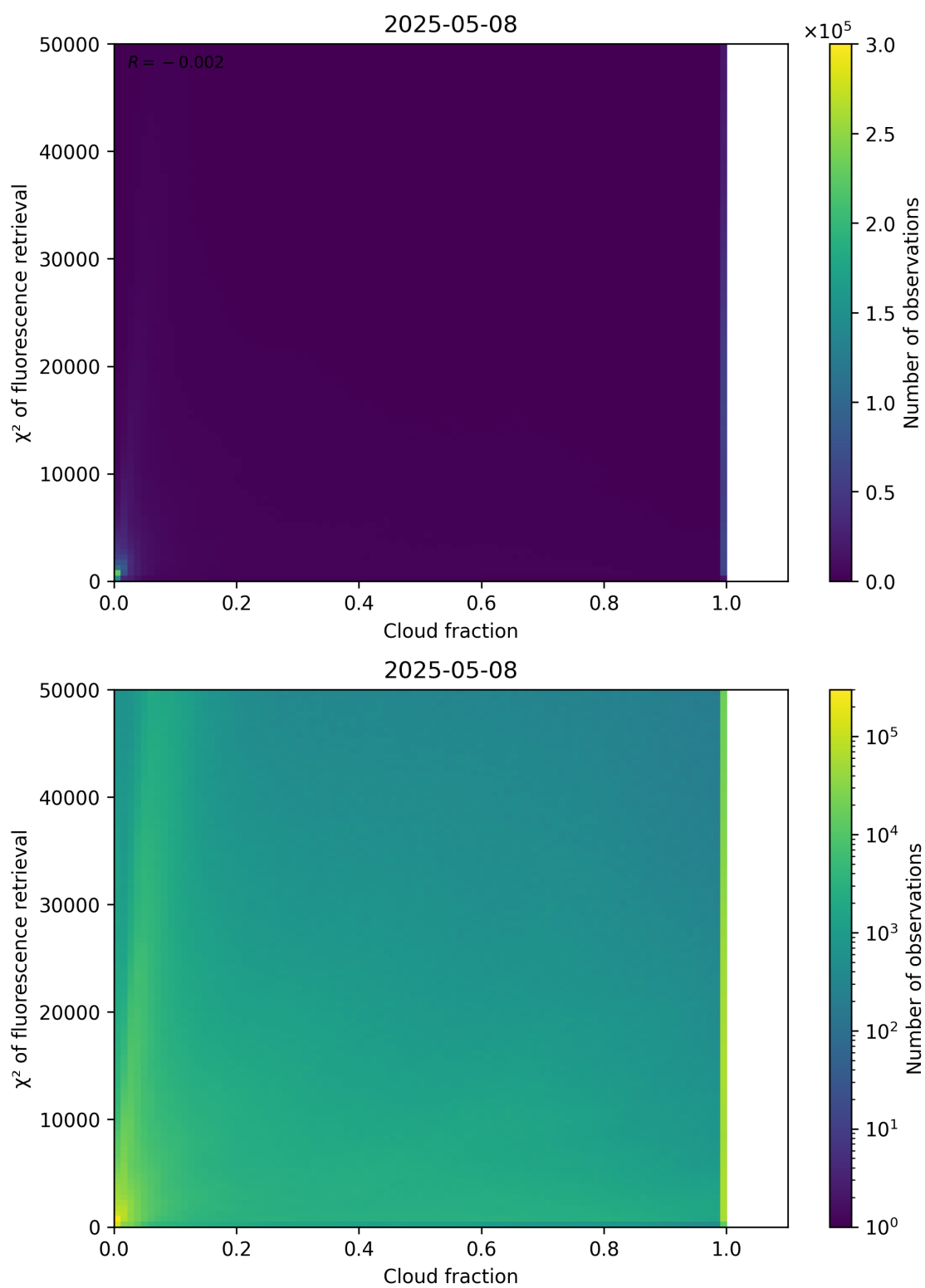
Figure 71: Scatter density plot of “Cloud fraction” against “ \chi^2 of fluorescence retrieval” for 2025-05-07 to 2025-05-09.
