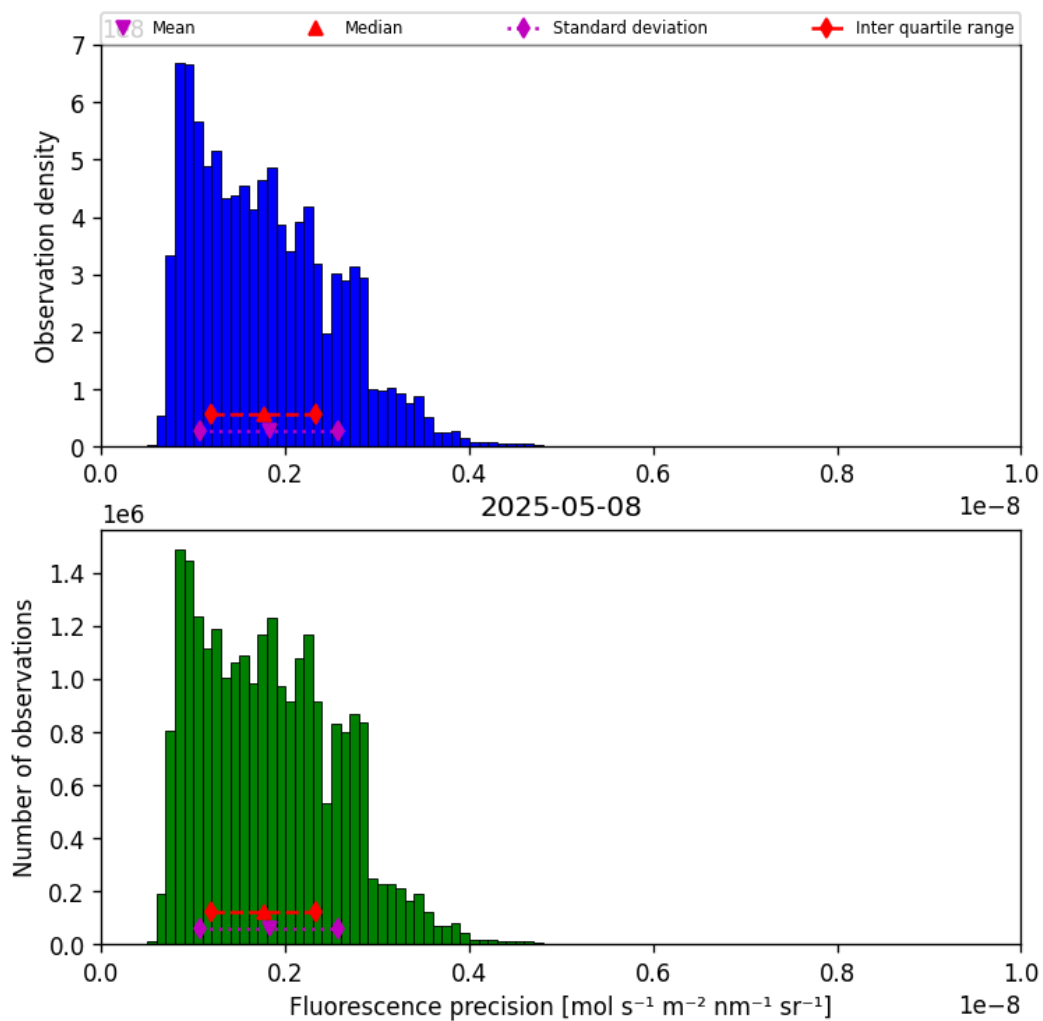
Figure 41: Histogram of “Fluorescence precision” for 2025-05-07 to 2025-05-09
