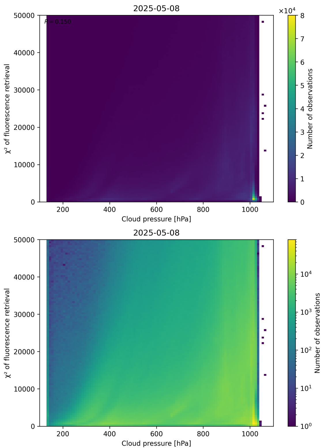
Figure 78: Scatter density plot of “Cloud pressure” against “ \chi^2 of fluorescence retrieval” for 2025-05-07 to 2025-05-09.
