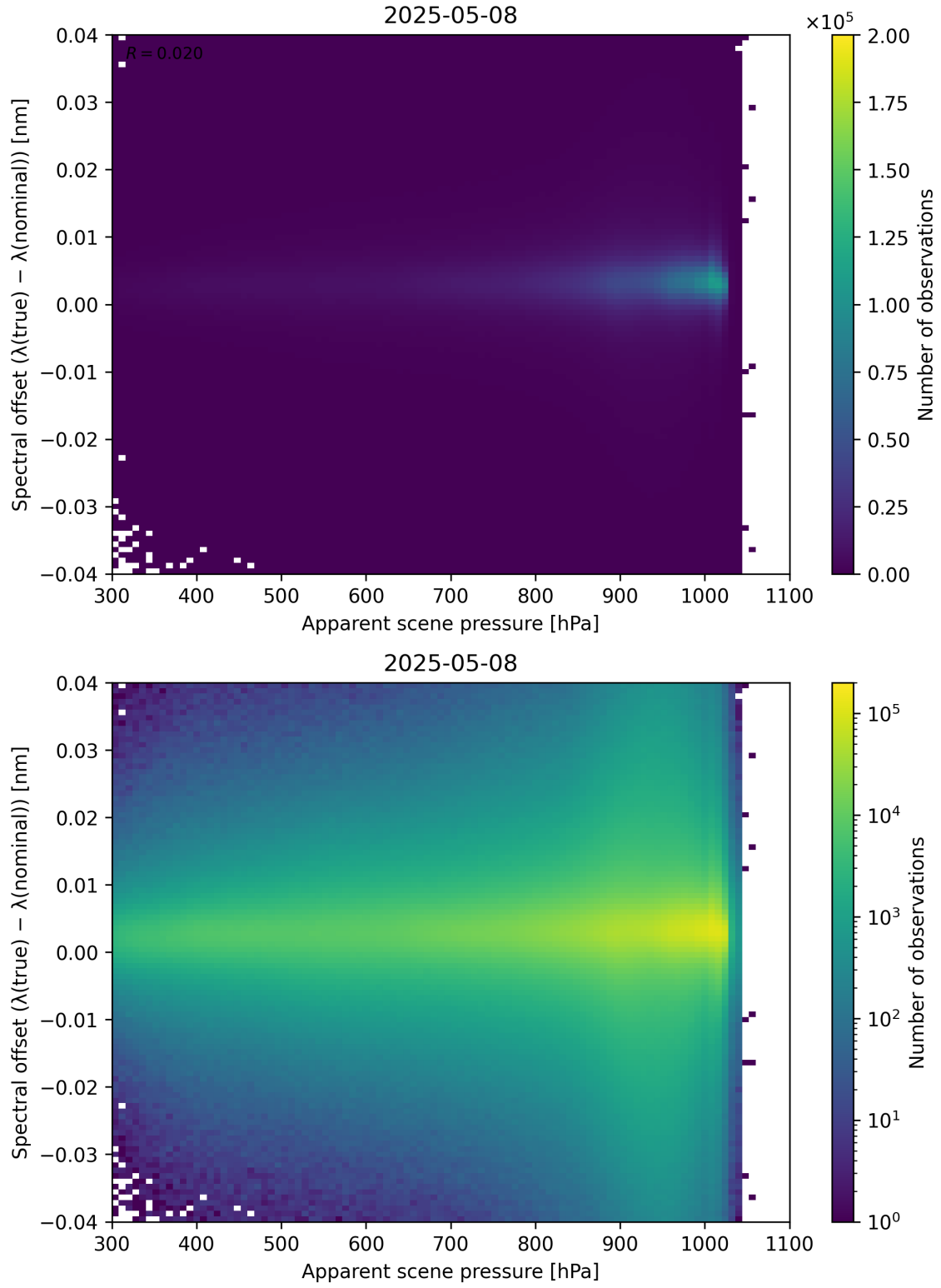
Figure 67: Scatter density plot of “Apparent scene pressure” against “Spectral offset ( \lambda_{\text{true}} - \lambda_{\text{nominal}} )” for 2025-05-07 to 2025-05-09.
