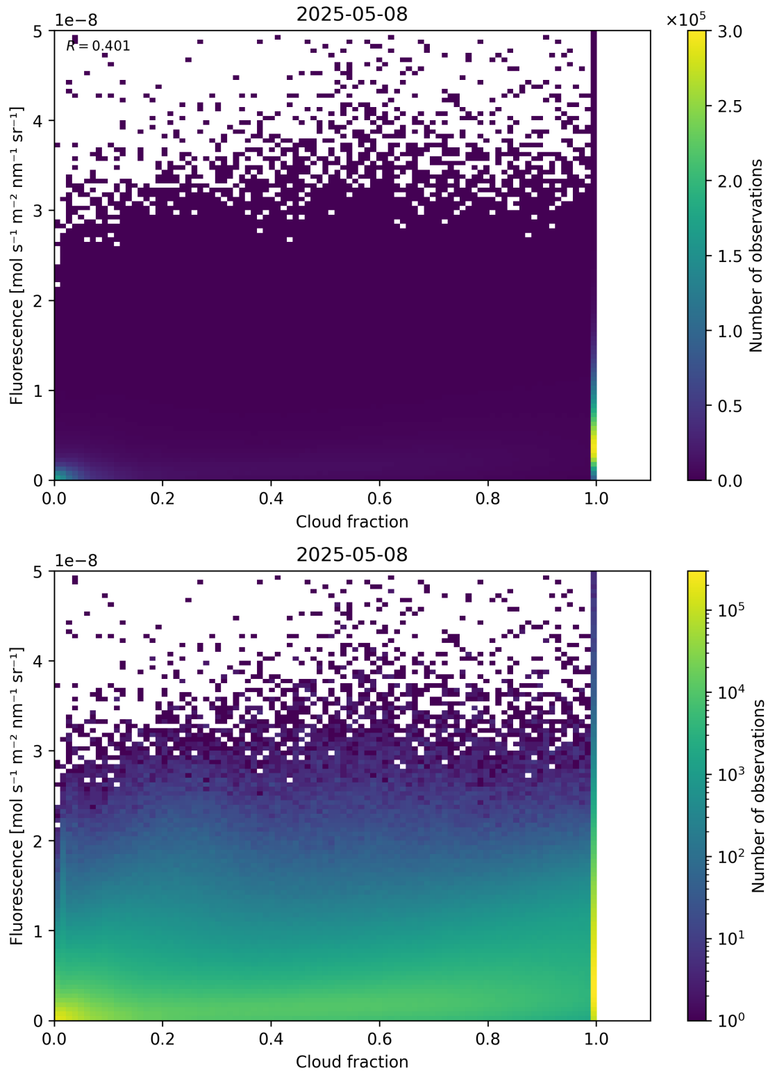
Figure 72: Scatter density plot of “Cloud fraction” against “Fluorescence” for 2025-05-07 to 2025-05-09.
