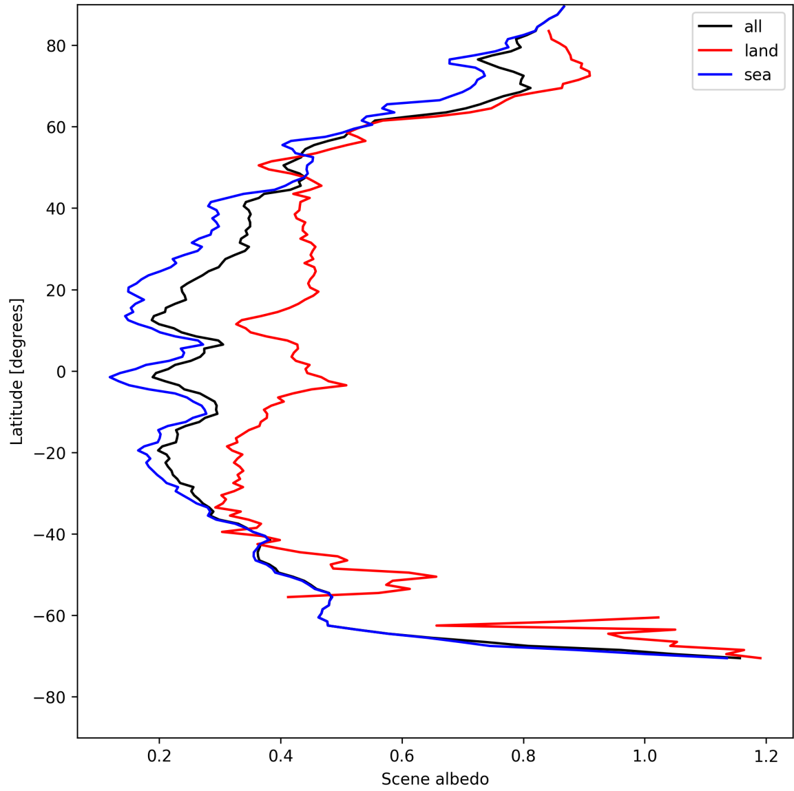
Figure 17: Zonal average of “Scene albedo” for 2025-05-07 to 2025-05-09.
