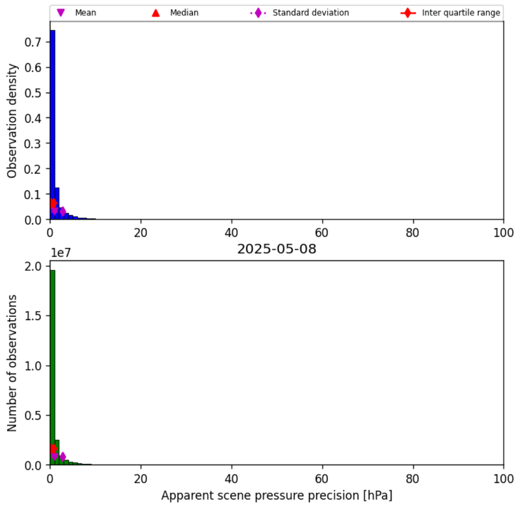
Figure 37: Histogram of “Apparent scene pressure precision” for 2025-05-07 to 2025-05-09
