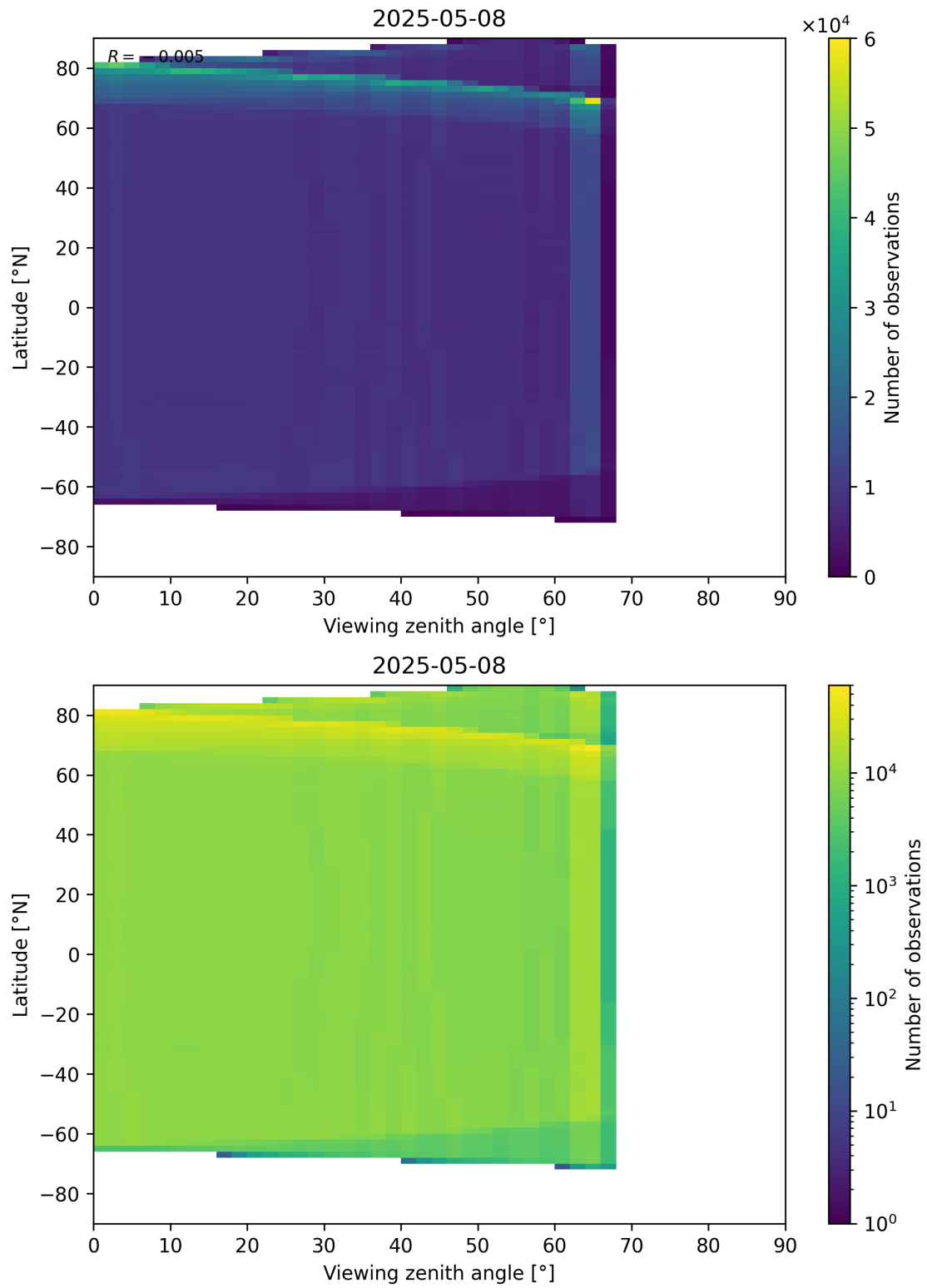
Figure 123: Scatter density plot of “Viewing zenith angle” against “Latitude” for 2025-05-07 to 2025-05-09.
