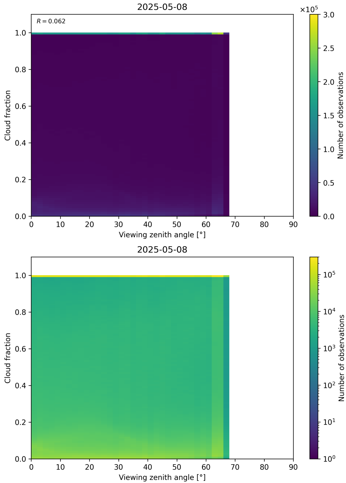
Figure 120: Scatter density plot of “Viewing zenith angle” against “Cloud fraction” for 2025-05-07 to 2025-05-09.
