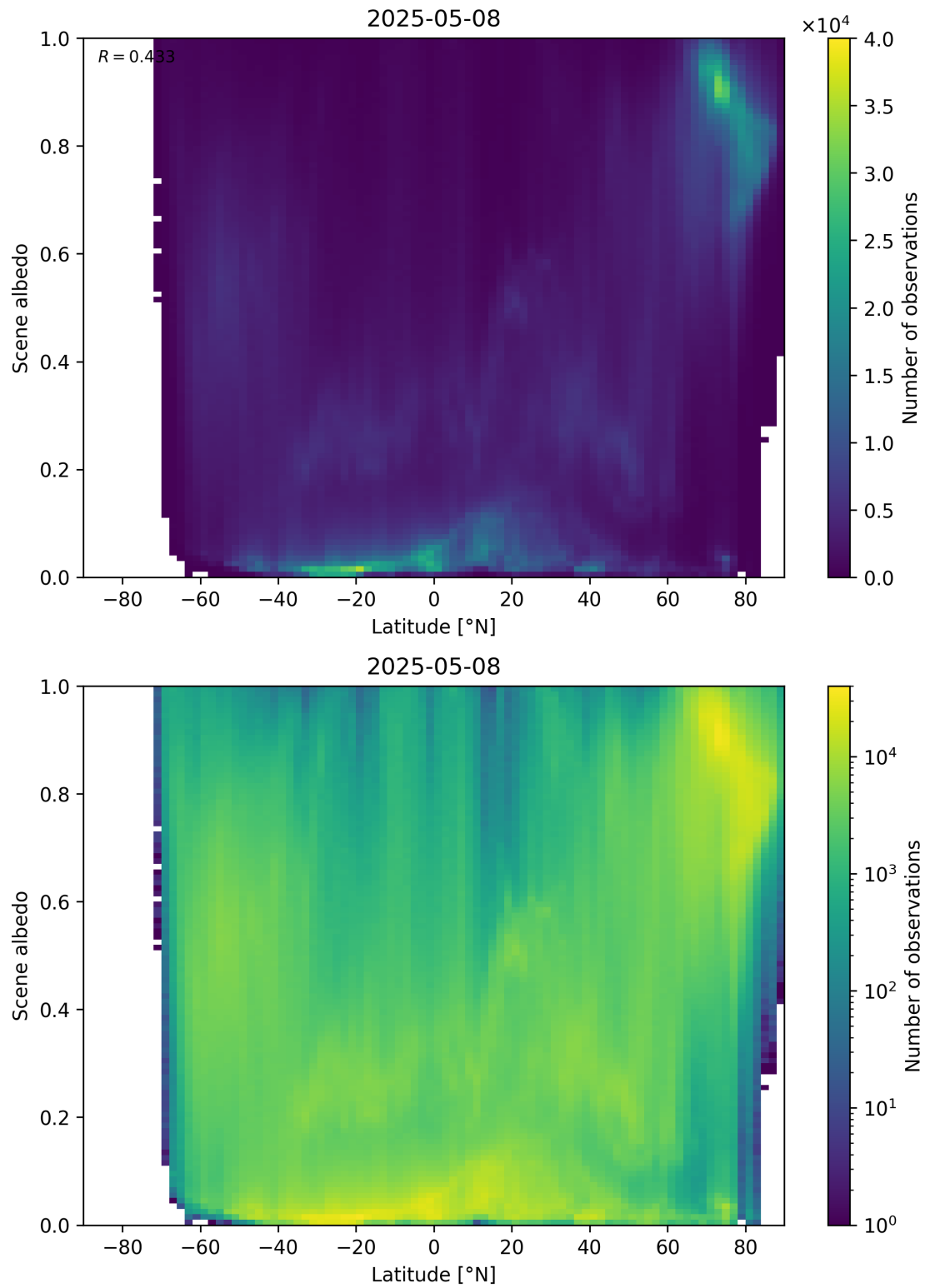
Figure 95: Scatter density plot of “Latitude” against “Scene albedo” for 2025-05-07 to 2025-05-09.
