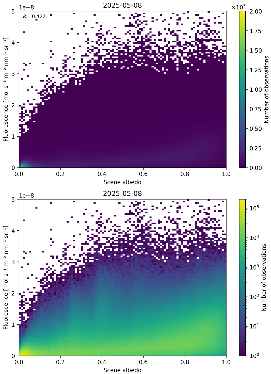
Figure 104: Scatter density plot of “Scene albedo” against “Fluorescence” for 2025-05-07 to 2025-05-09.
