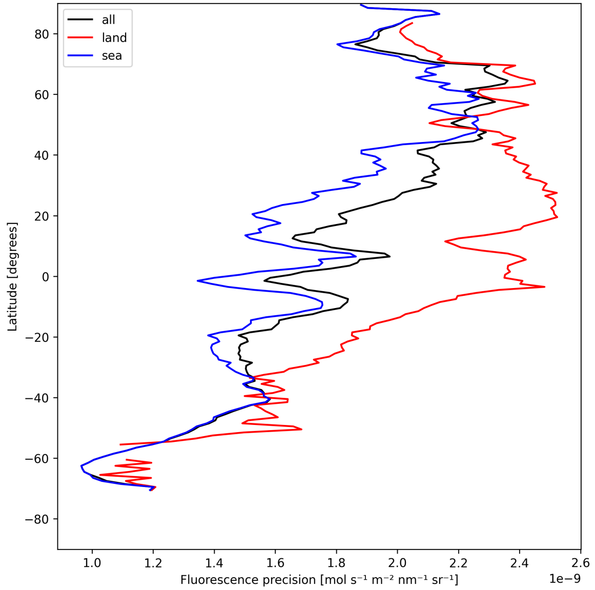
Figure 24: Zonal average of “Fluorescence precision” for 2025-05-07 to 2025-05-09.
