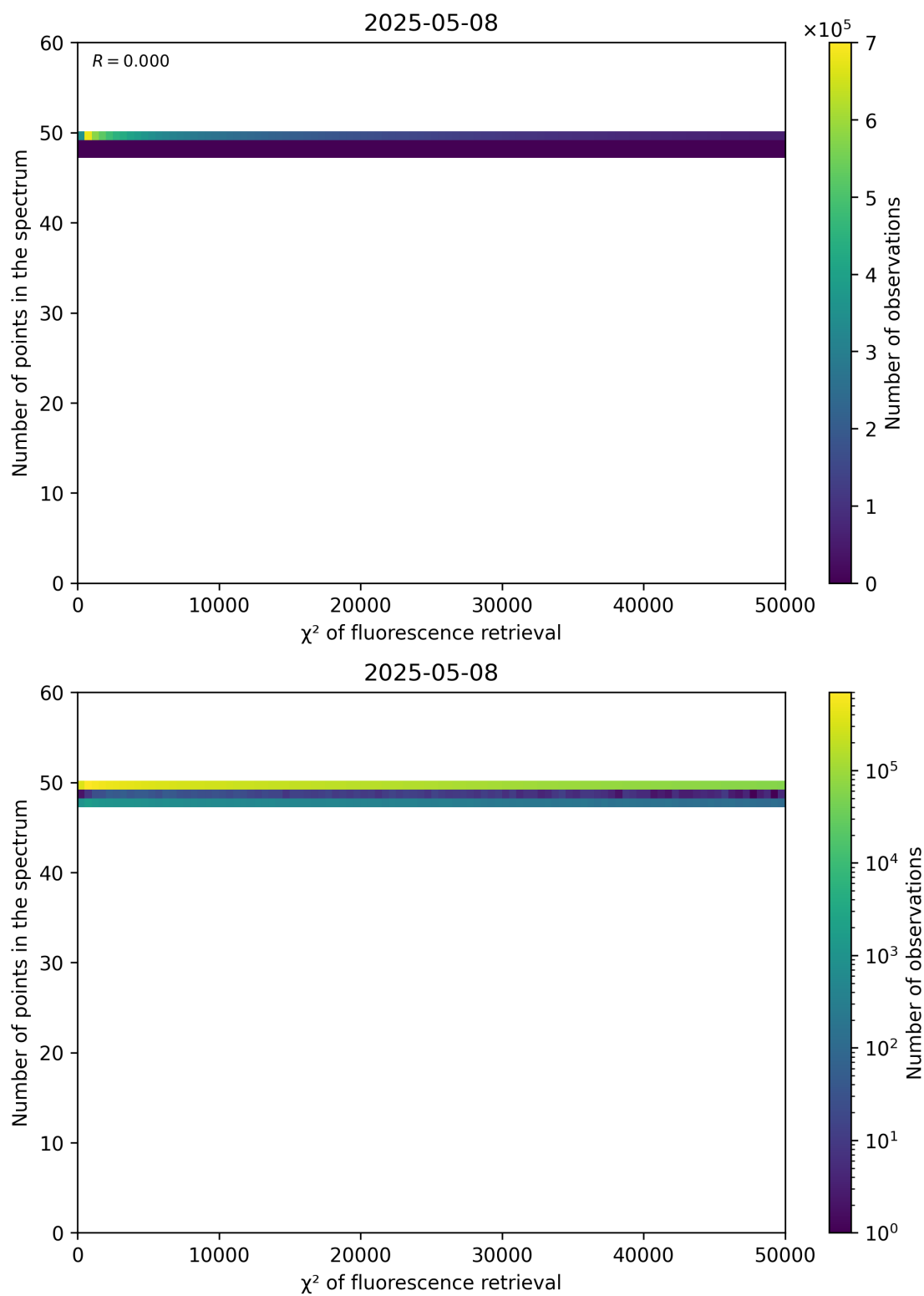
Figure 68: Scatter density plot of “ \chi^2 of fluorescence retrieval” against “Number of points in the spectrum” for 2025-05-07 to 2025-05-09.
