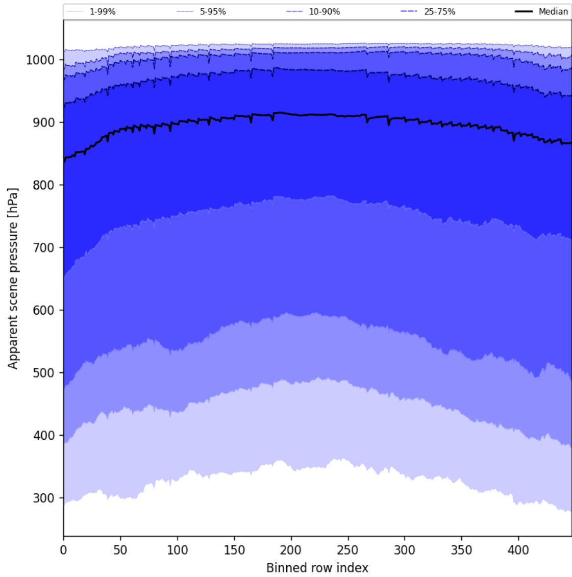
Figure 53: Along track statistics of “Apparent scene pressure” for 2025-05-07 to 2025-05-09
