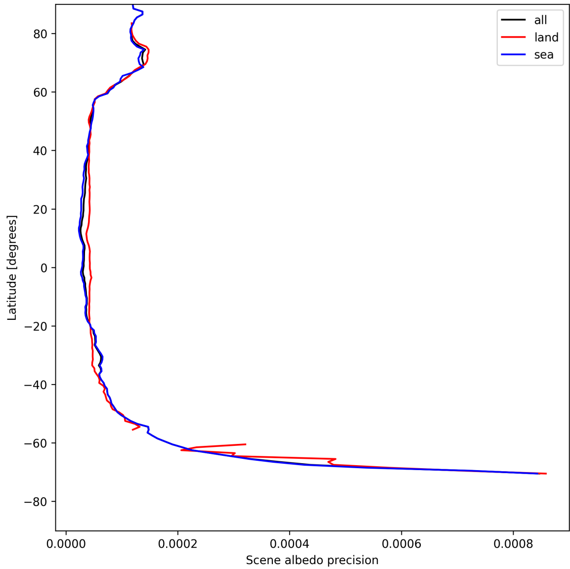
Figure 18: Zonal average of “Scene albedo precision” for 2025-05-07 to 2025-05-09.
