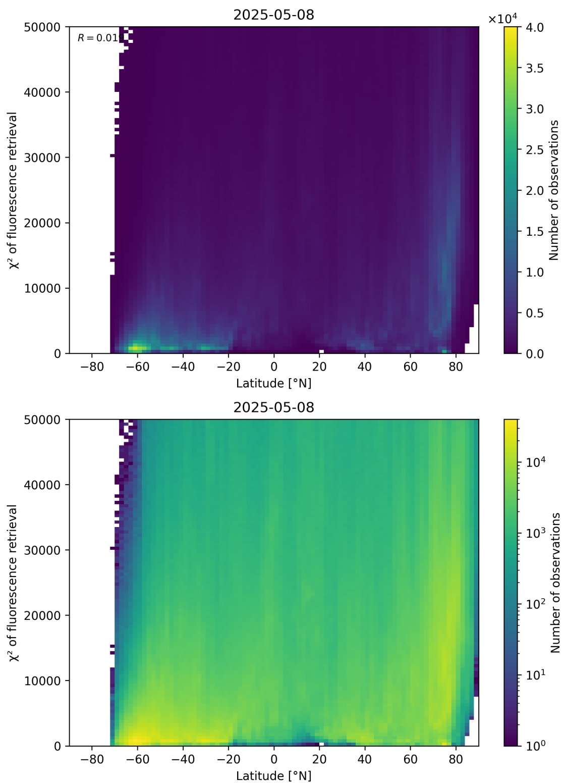
Figure 89: Scatter density plot of “Latitude” against “ \chi^2 of fluorescence retrieval” for 2025-05-07 to 2025-05-09.
