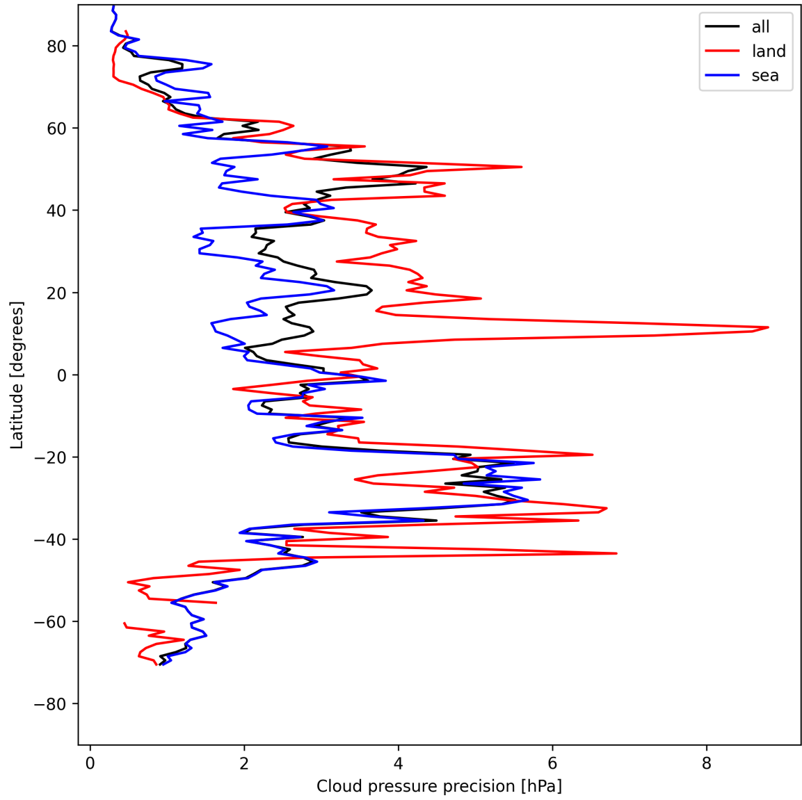
Figure 14: Zonal average of “Cloud pressure precision” for 2025-05-07 to 2025-05-09.
