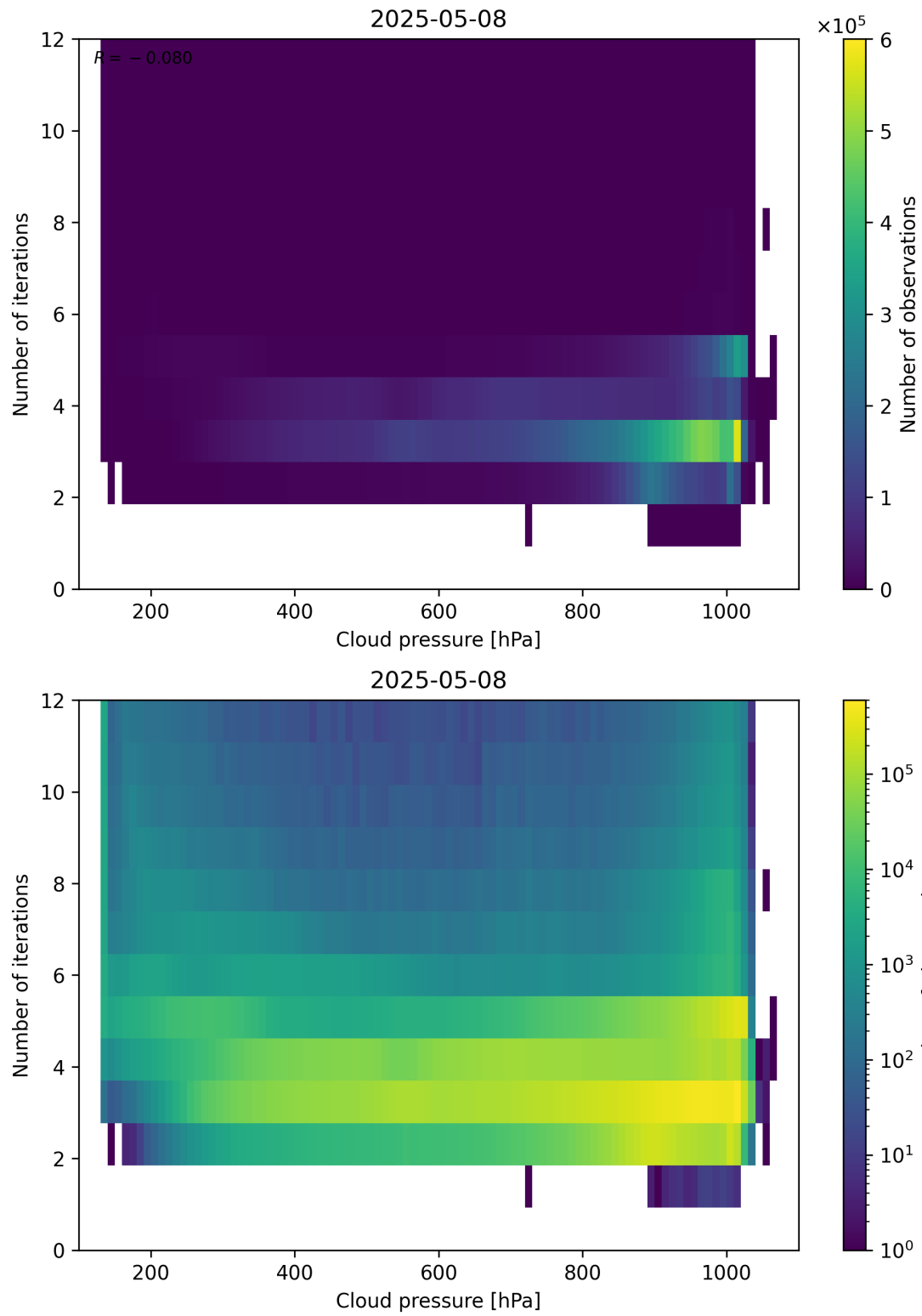
Figure 81: Scatter density plot of “Cloud pressure” against “Number of iterations” for 2025-05-07 to 2025-05-09.
