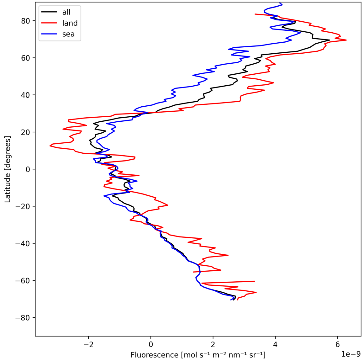
Figure 23: Zonal average of “Fluorescence” for 2025-05-07 to 2025-05-09.
