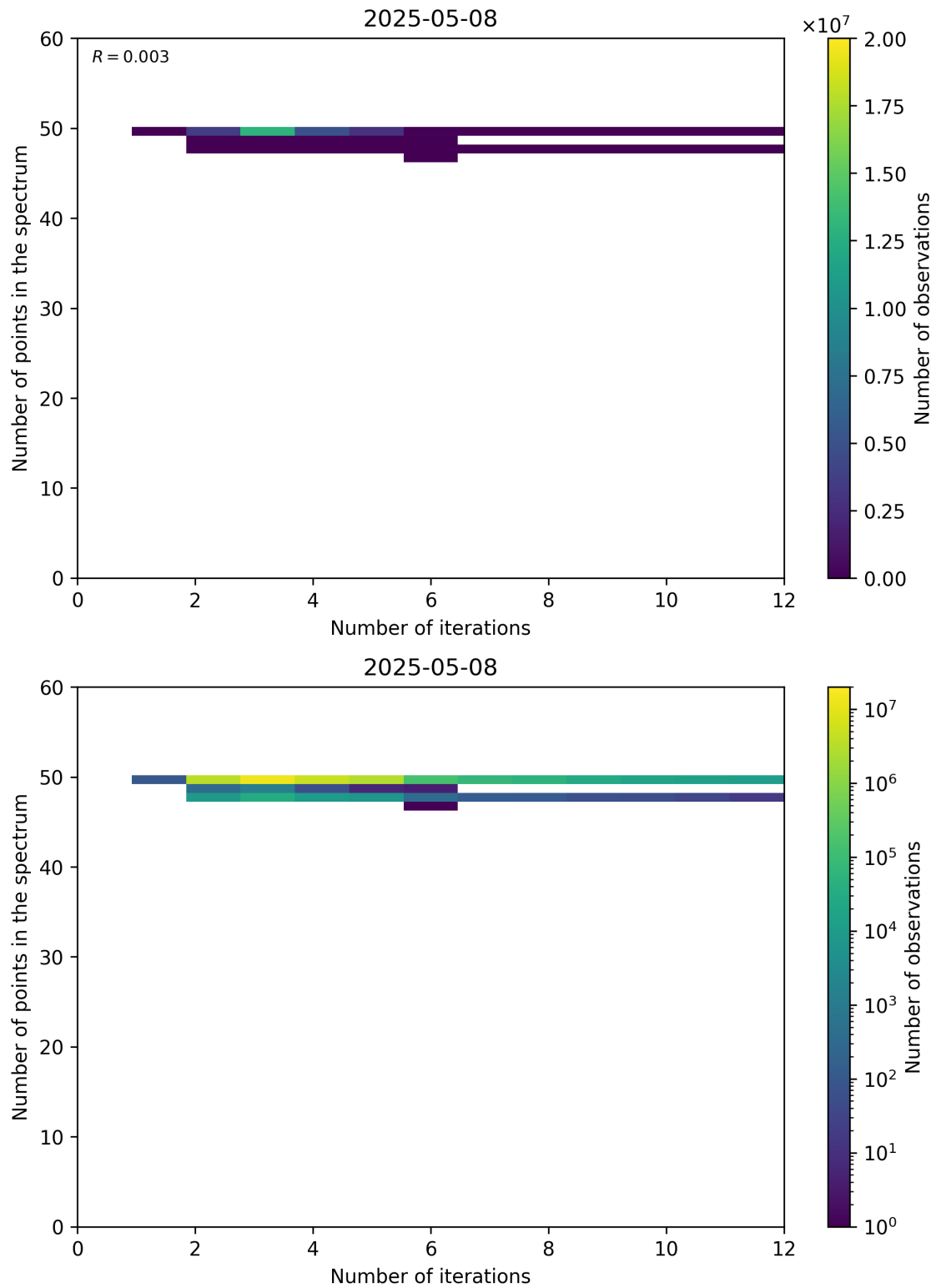
Figure 99: Scatter density plot of “Number of iterations” against “Number of points in the spectrum” for 2025-05-07 to 2025-05-09.
