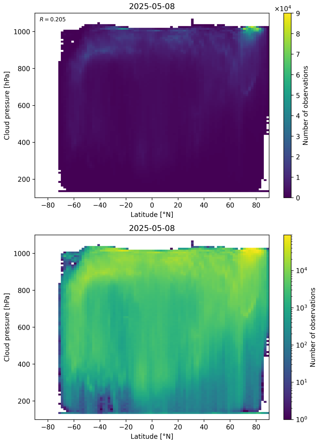
Figure 91: Scatter density plot of “Latitude” against “Cloud pressure” for 2025-05-07 to 2025-05-09.
