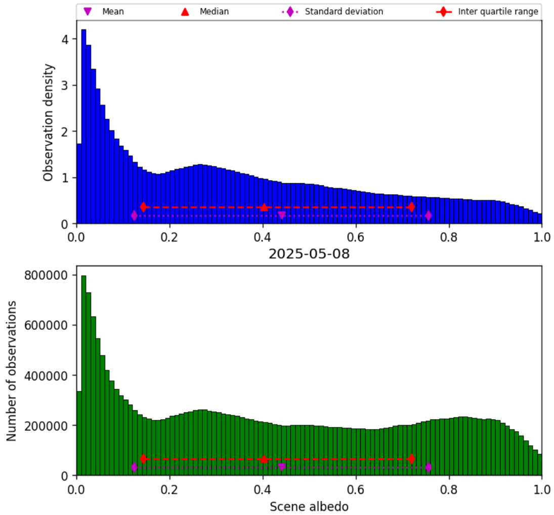
Figure 34: Histogram of “Scene albedo” for 2025-05-07 to 2025-05-09
