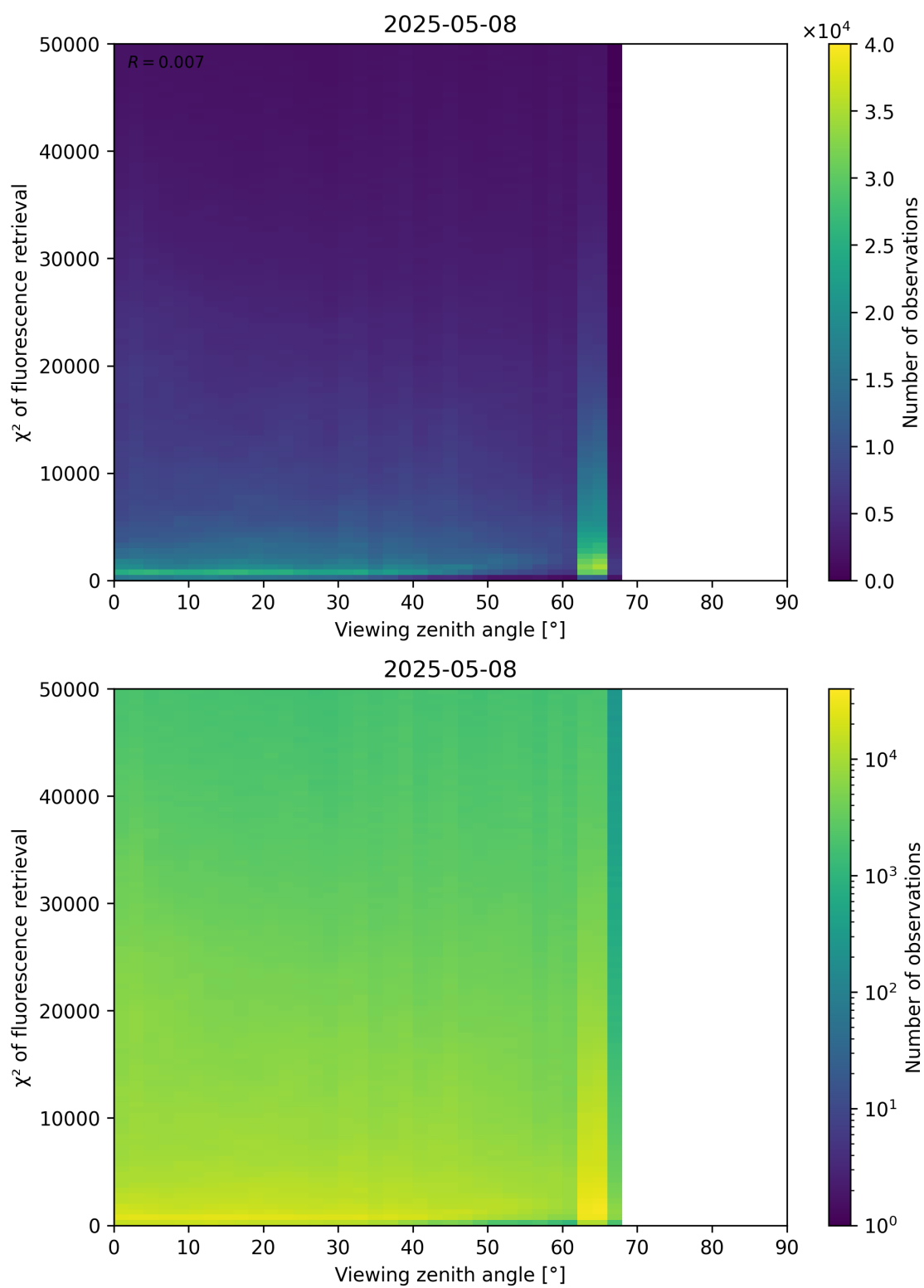
Figure 119: Scatter density plot of “Viewing zenith angle” against “ \chi^2 of fluorescence retrieval” for 2025-05-07 to 2025-05-09.
