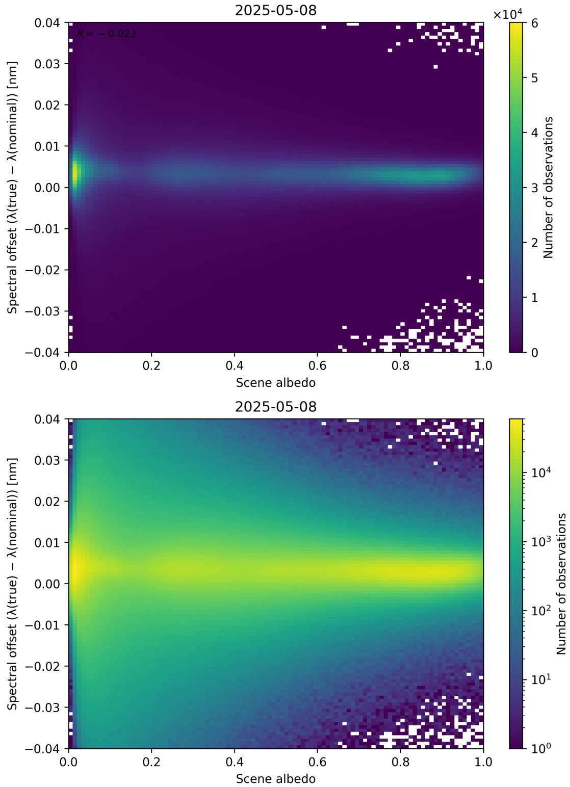
Figure 107: Scatter density plot of “Scene albedo” against “Spectral offset ( \lambda_{\text{true}} - \lambda_{\text{nominal}} )” for 2025-05-07 to 2025-05-09.
