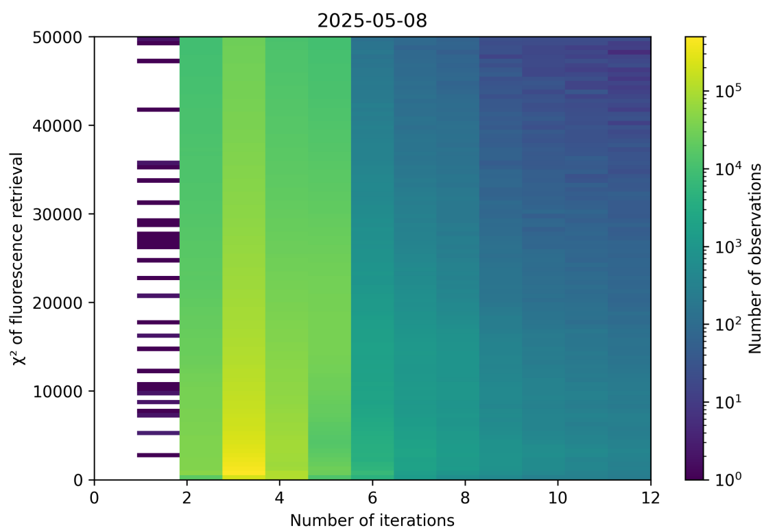
Figure 97: Scatter density plot of “Number of iterations” against “ \chi^2 of fluorescence retrieval” for 2025-05-07 to 2025-05-09.
