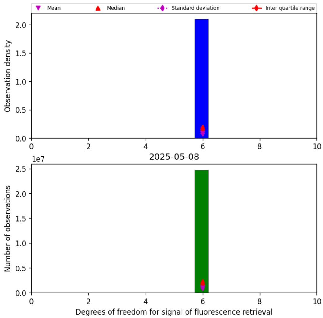
Figure 43: Histogram of “Degrees of freedom for signal of fluorescence retrieval” for 2025-05-07 to 2025-05-09
