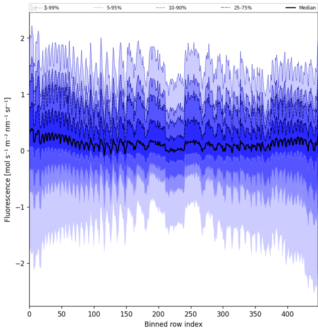
Figure 57: Along track statistics of “Fluorescence” for 2025-05-07 to 2025-05-09
