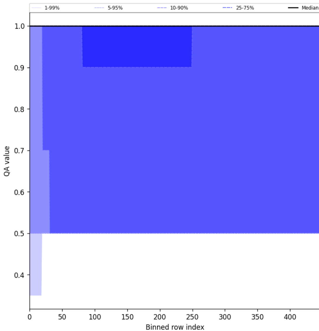
Figure 46: Along track statistics of “QA value” for 2025-05-07 to 2025-05-09
