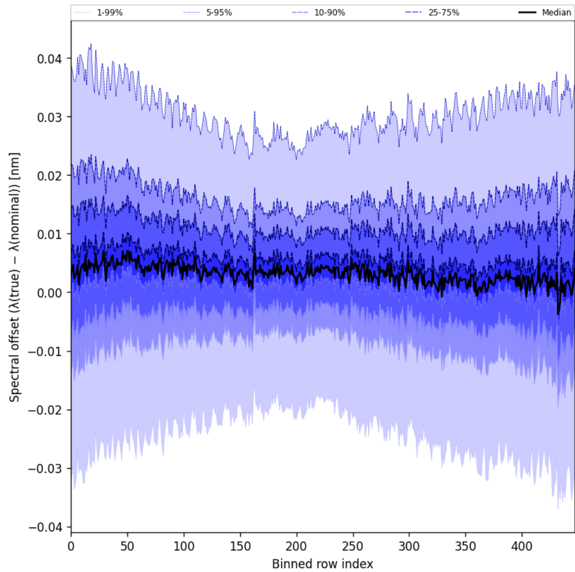
Figure 62: Along track statistics of “Spectral offset ( \lambda_{\text{true}} - \lambda_{\text{nominal}} )” for 2025-05-07 to 2025-05-09
