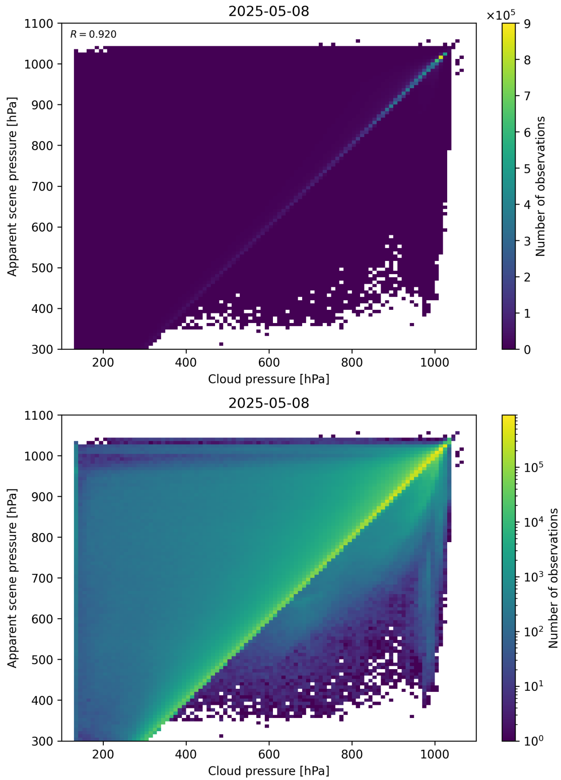
Figure 77: Scatter density plot of “Cloud pressure” against “Apparent scene pressure” for 2025-05-07 to 2025-05-09.
