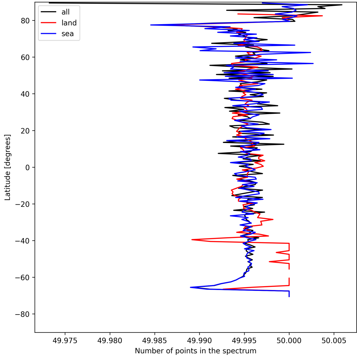
Figure 27: Zonal average of “Number of points in the spectrum” for 2025-05-07 to 2025-05-09.
