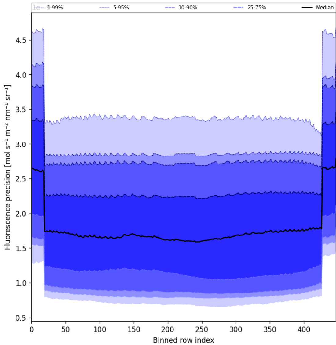
Figure 58: Along track statistics of “Fluorescence precision” for 2025-05-07 to 2025-05-09
