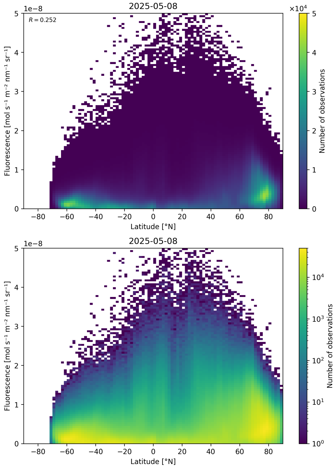
Figure 92: Scatter density plot of “Latitude” against “Fluorescence” for 2025-05-07 to 2025-05-09.
