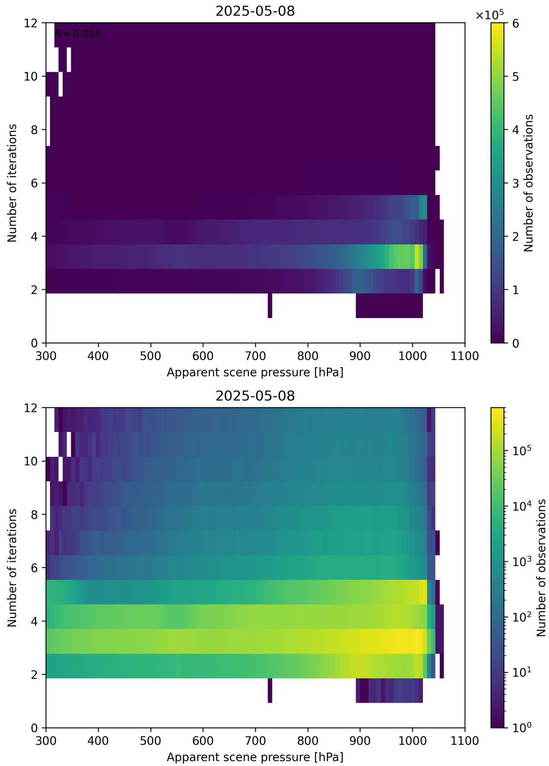
Figure 65: Scatter density plot of “Apparent scene pressure” against “Number of iterations” for 2025-05-07 to 2025-05-09.
