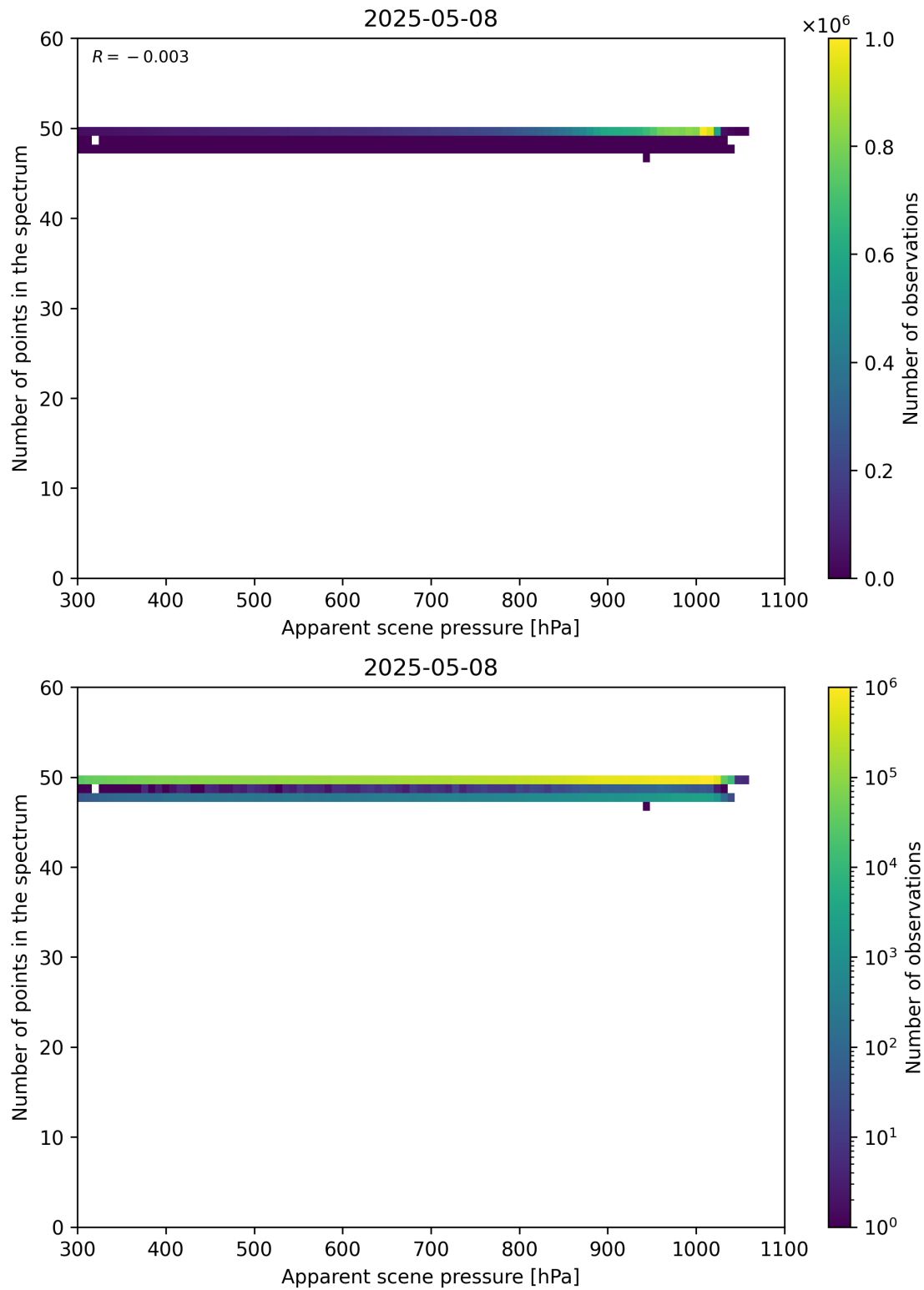
Figure 66: Scatter density plot of “Apparent scene pressure” against “Number of points in the spectrum” for 2025-05-07 to 2025-05-09.
