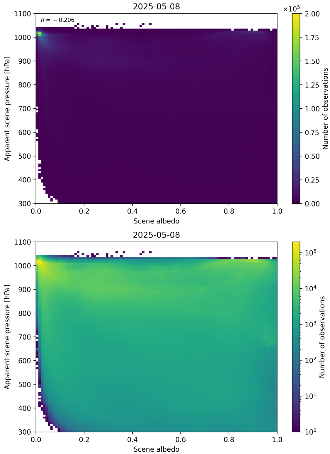
Figure 102: Scatter density plot of “Scene albedo” against “Apparent scene pressure” for 2025-05-07 to 2025-05-09.
