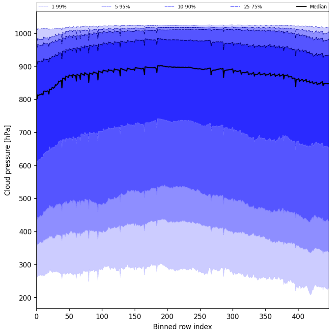
Figure 47: Along track statistics of “Cloud pressure” for 2025-05-07 to 2025-05-09
