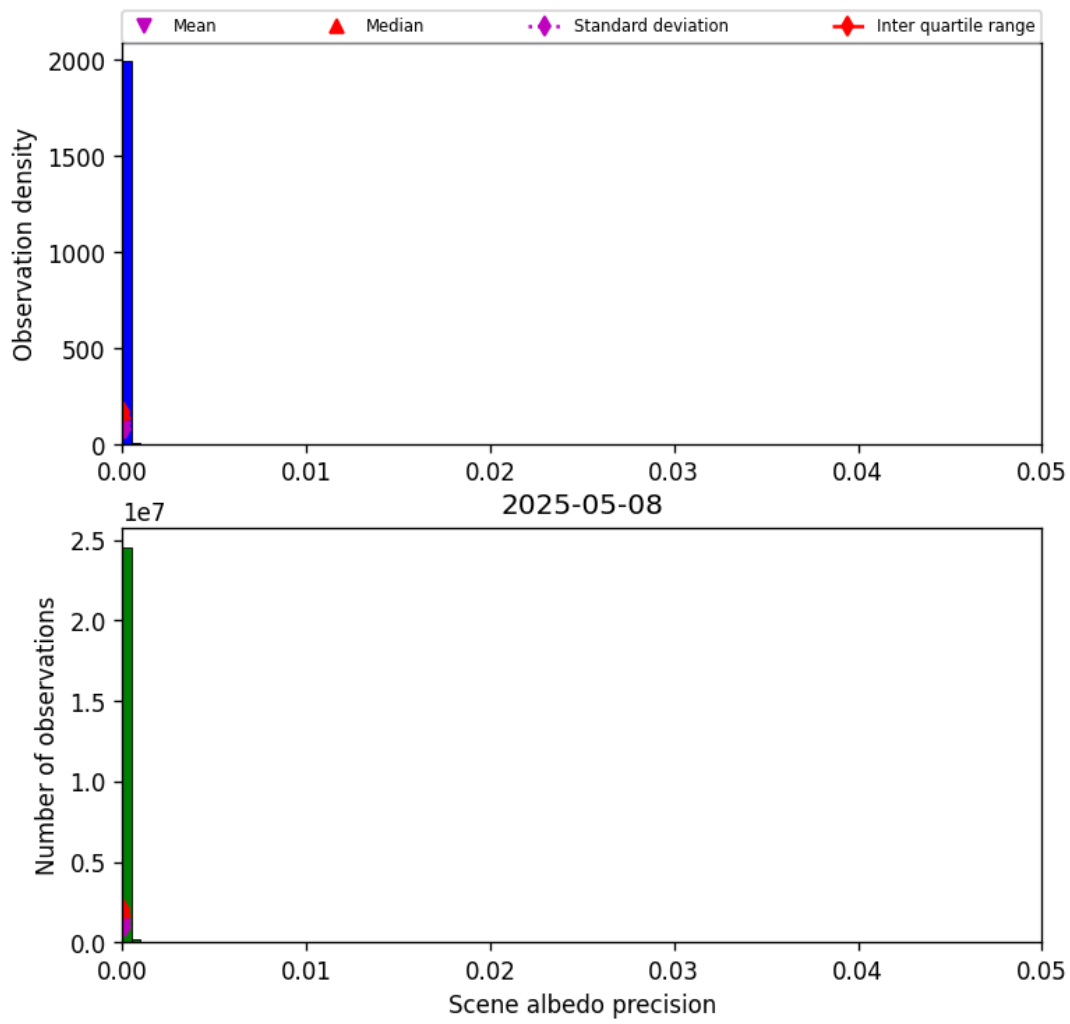
Figure 35: Histogram of “Scene albedo precision” for 2025-05-07 to 2025-05-09
