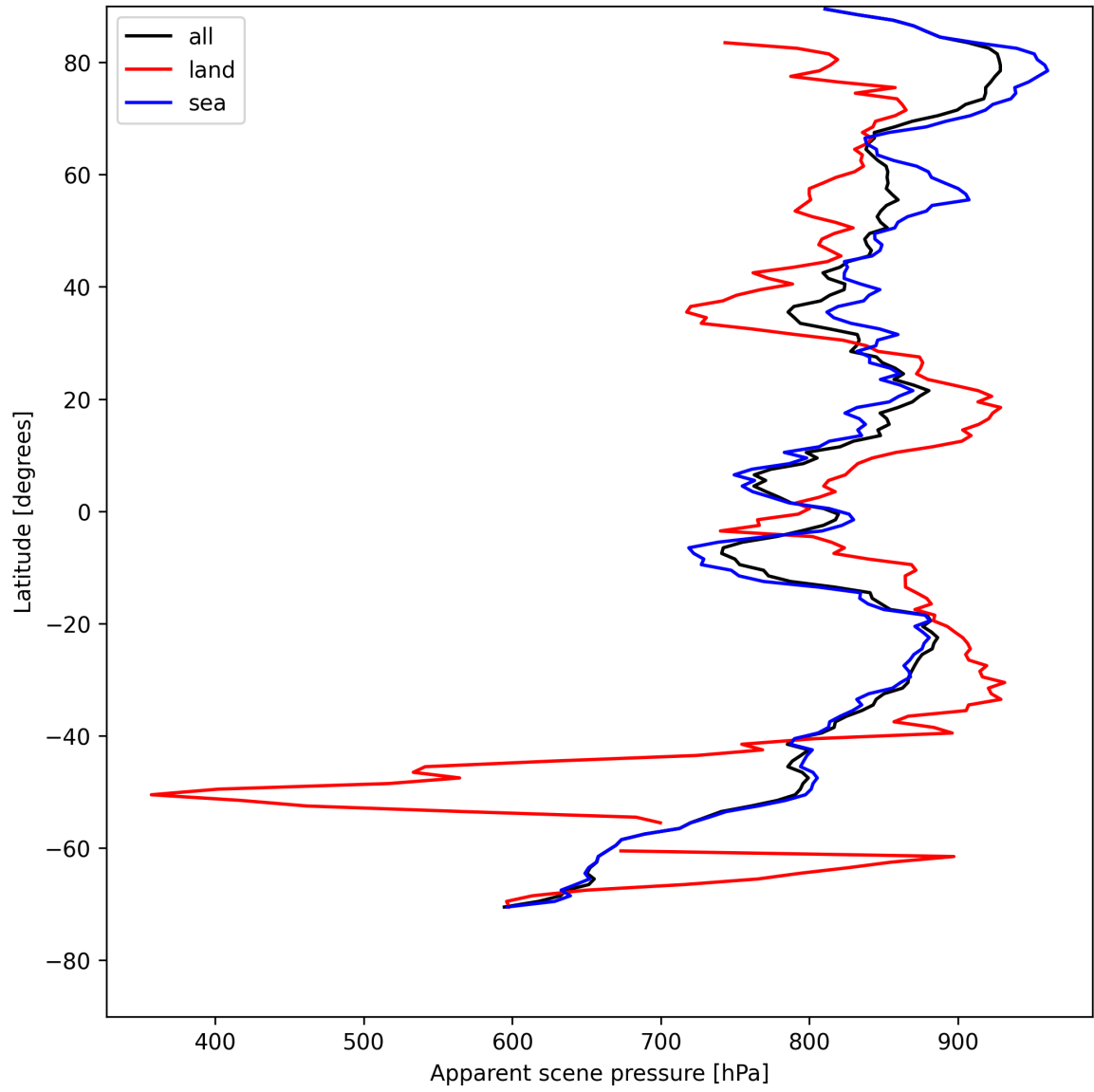
Figure 19: Zonal average of “Apparent scene pressure” for 2025-05-07 to 2025-05-09.
