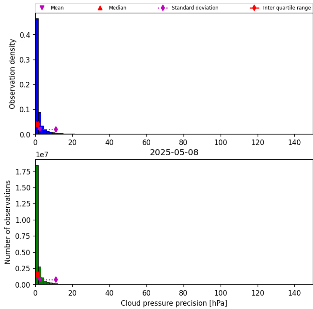
Figure 31: Histogram of “Cloud pressure precision” for 2025-05-07 to 2025-05-09
