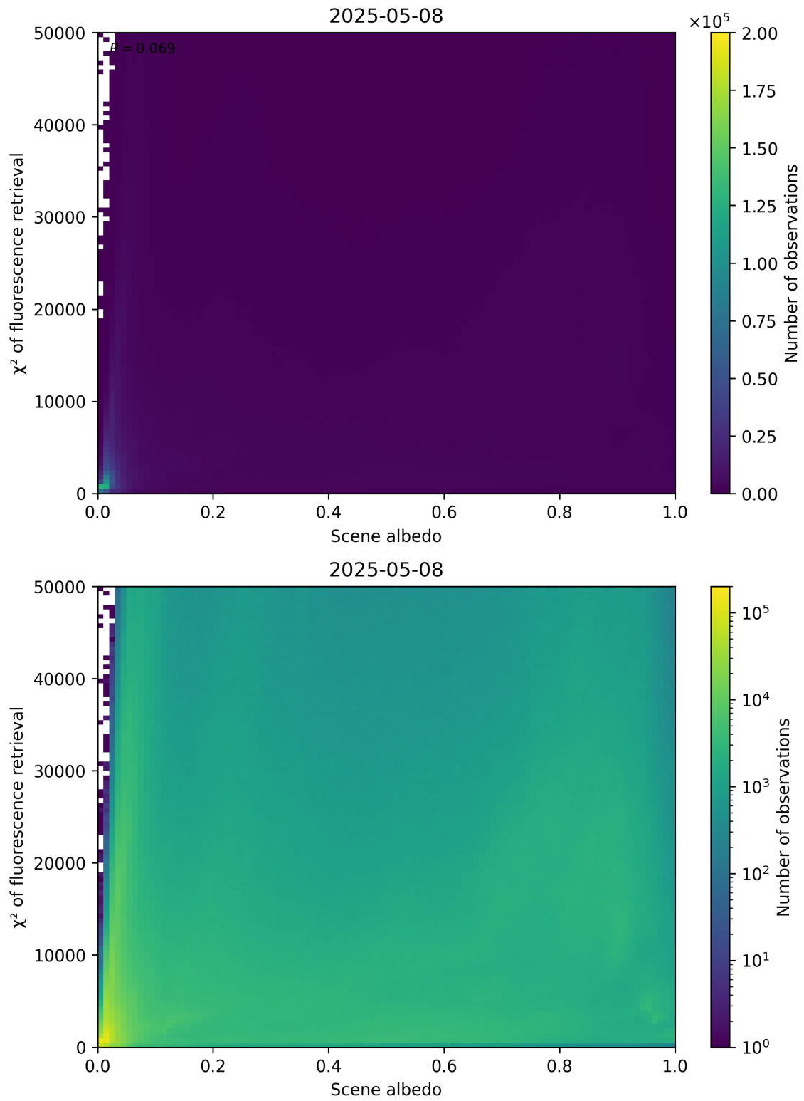
Figure 103: Scatter density plot of “Scene albedo” against “ \chi^2 of fluorescence retrieval” for 2025-05-07 to 2025-05-09.
