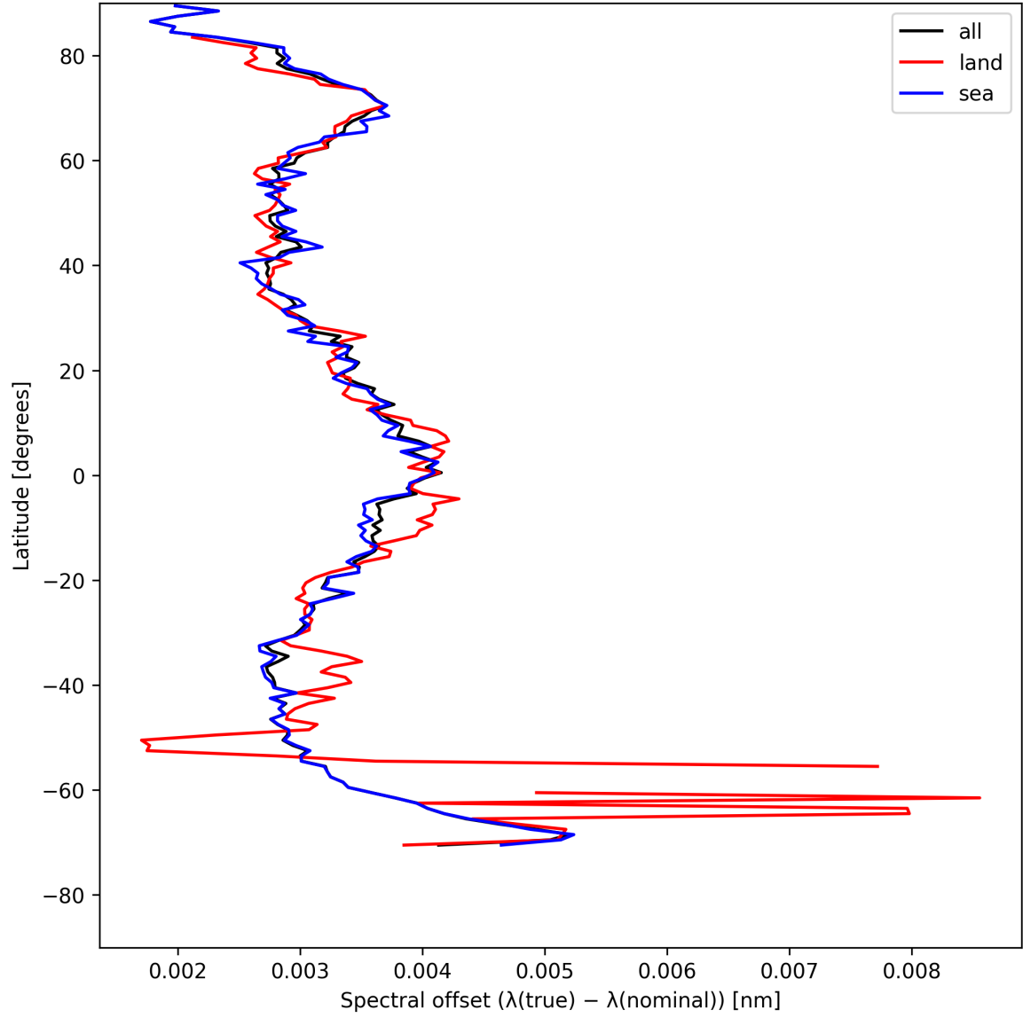
Figure 28: Zonal average of “Spectral offset ( \lambda_{\text{true}} - \lambda_{\text{nominal}} )” for 2025-05-07 to 2025-05-09.
