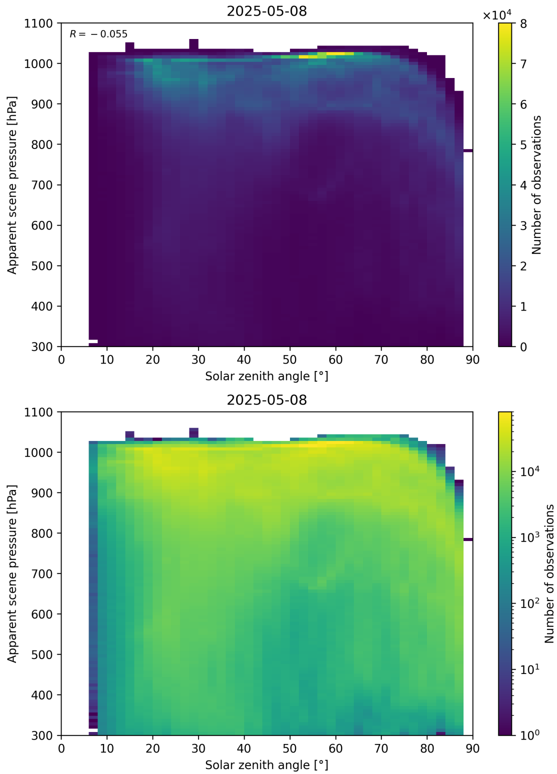
Figure 108: Scatter density plot of “Solar zenith angle” against “Apparent scene pressure” for 2025-05-07 to 2025-05-09.
