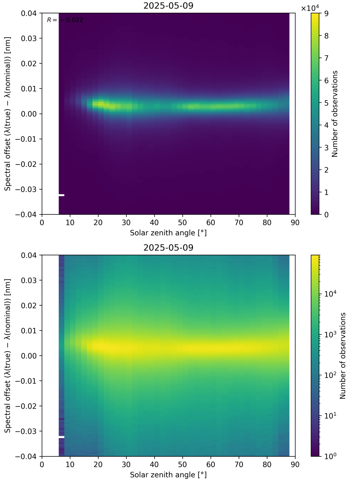
Figure 117: Scatter density plot of “Solar zenith angle” against “Spectral offset ( \lambda_{\text{true}} - \lambda_{\text{nominal}} )” for 2025-05-08 to 2025-05-10.
