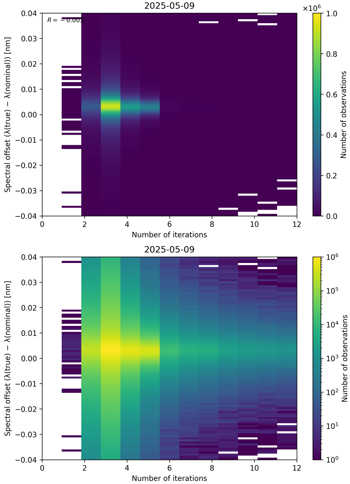
Figure 100: Scatter density plot of “Number of iterations” against “Spectral offset ( \lambda_{\text{true}} - \lambda_{\text{nominal}} )” for 2025-05-08 to 2025-05-10.
