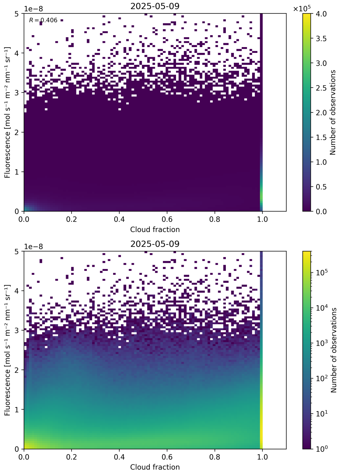
Figure 72: Scatter density plot of “Cloud fraction” against “Fluorescence” for 2025-05-08 to 2025-05-10.
