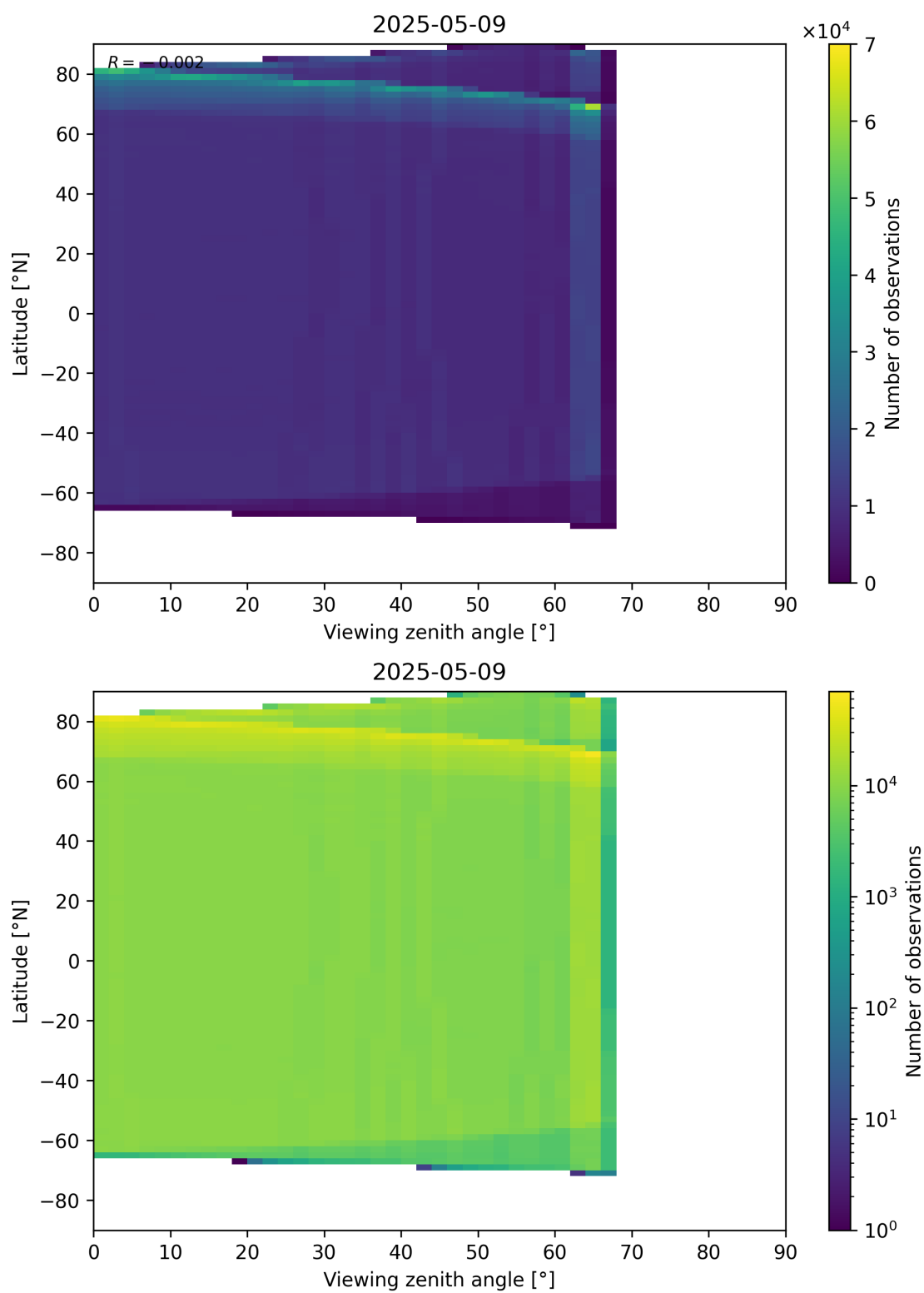
Figure 123: Scatter density plot of “Viewing zenith angle” against “Latitude” for 2025-05-08 to 2025-05-10.
