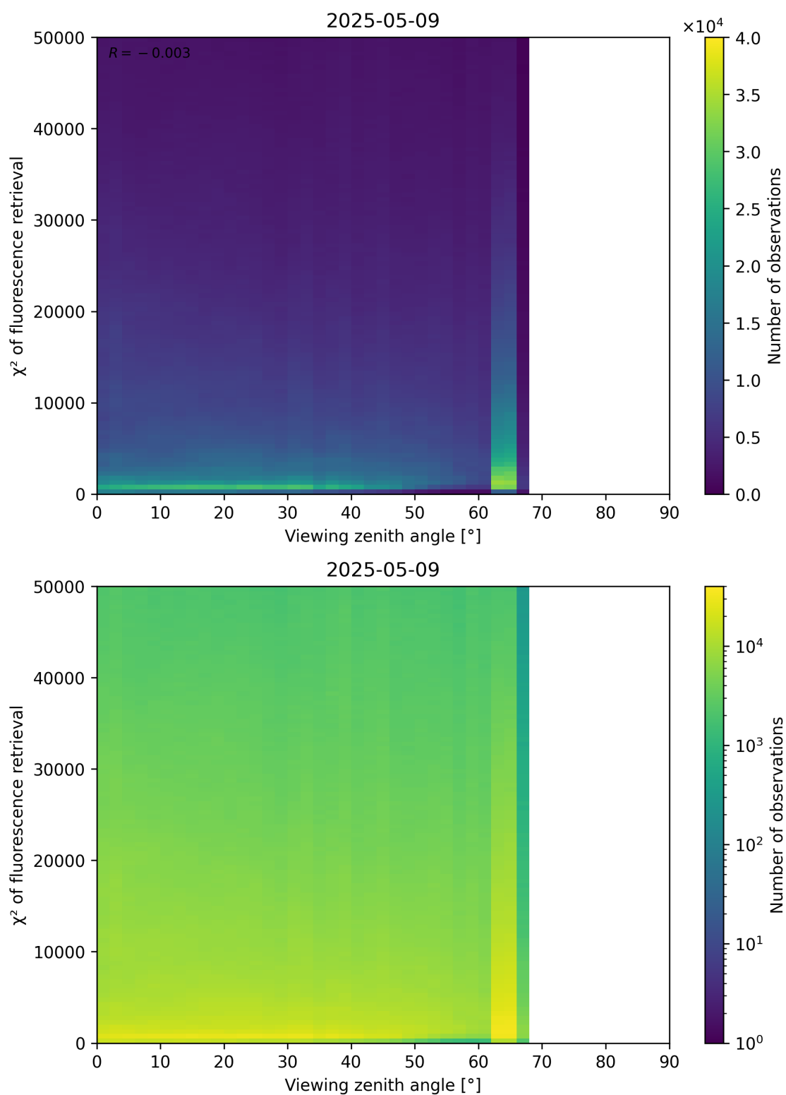
Figure 119: Scatter density plot of “Viewing zenith angle” against “ \chi^2 of fluorescence retrieval” for 2025-05-08 to 2025-05-10.
