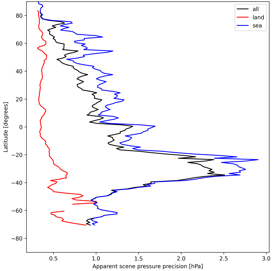
Figure 20: Zonal average of “Apparent scene pressure precision” for 2025-05-08 to 2025-05-10.
