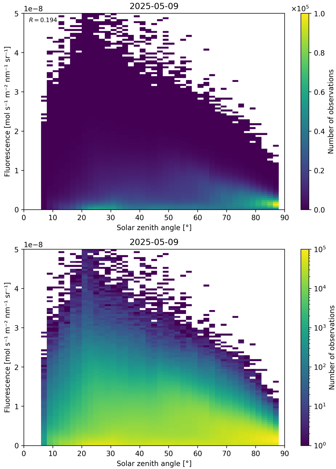
Figure 112: Scatter density plot of “Solar zenith angle” against “Fluorescence” for 2025-05-08 to 2025-05-10.
