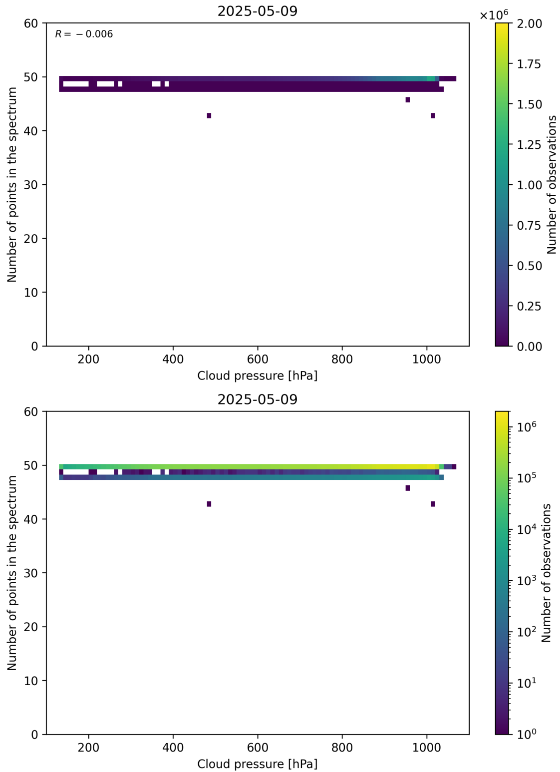
Figure 82: Scatter density plot of “Cloud pressure” against “Number of points in the spectrum” for 2025-05-08 to 2025-05-10.
