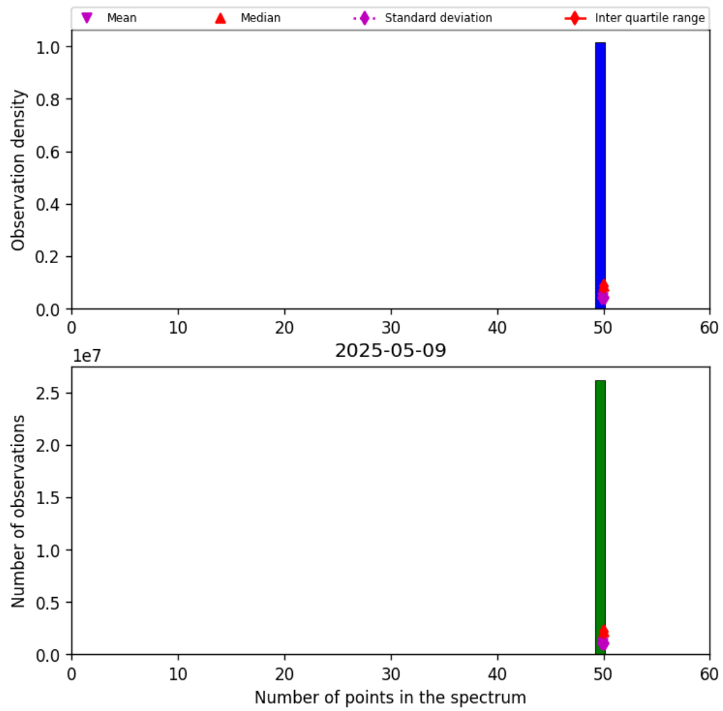
Figure 44: Histogram of “Number of points in the spectrum” for 2025-05-08 to 2025-05-10
