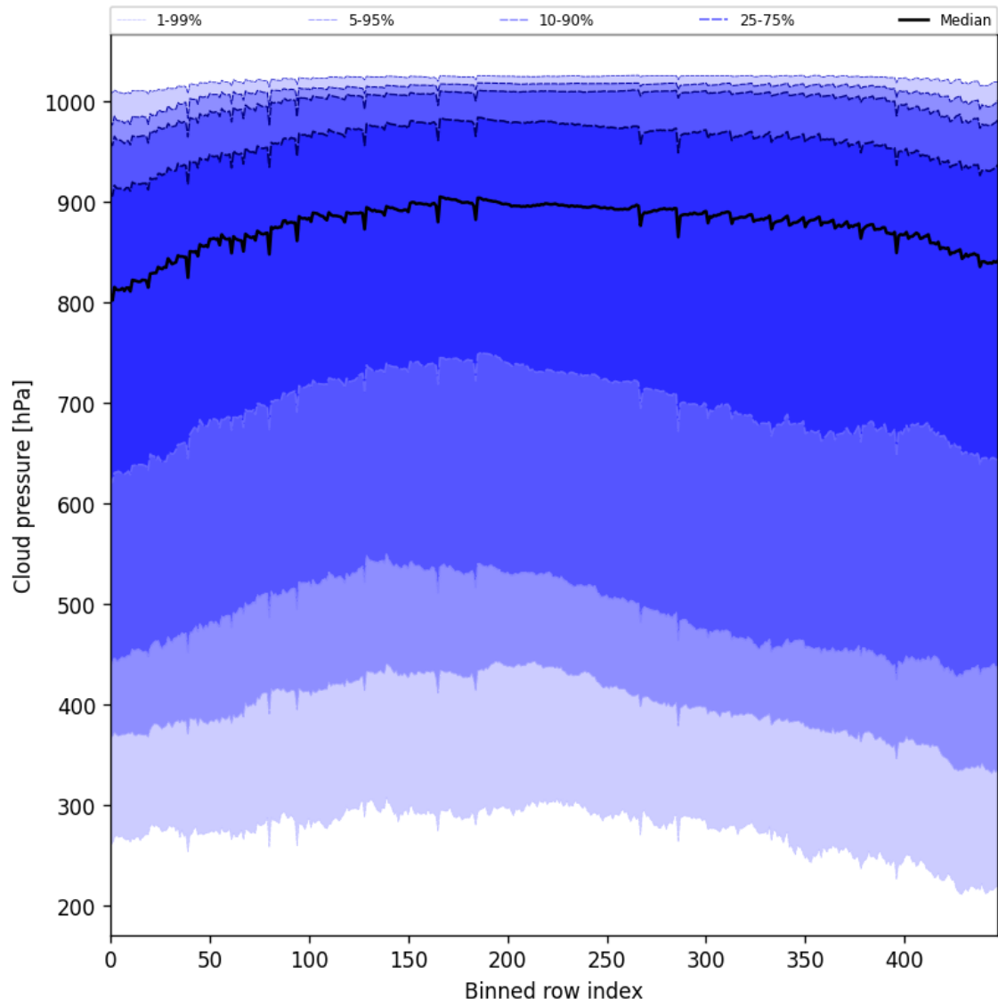
Figure 47: Along track statistics of “Cloud pressure” for 2025-05-08 to 2025-05-10
