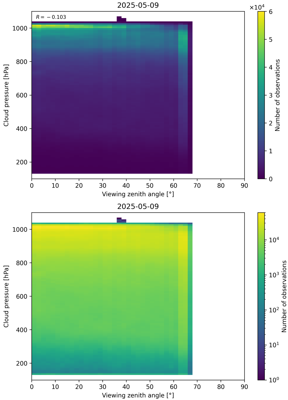
Figure 121: Scatter density plot of “Viewing zenith angle” against “Cloud pressure” for 2025-05-08 to 2025-05-10.
