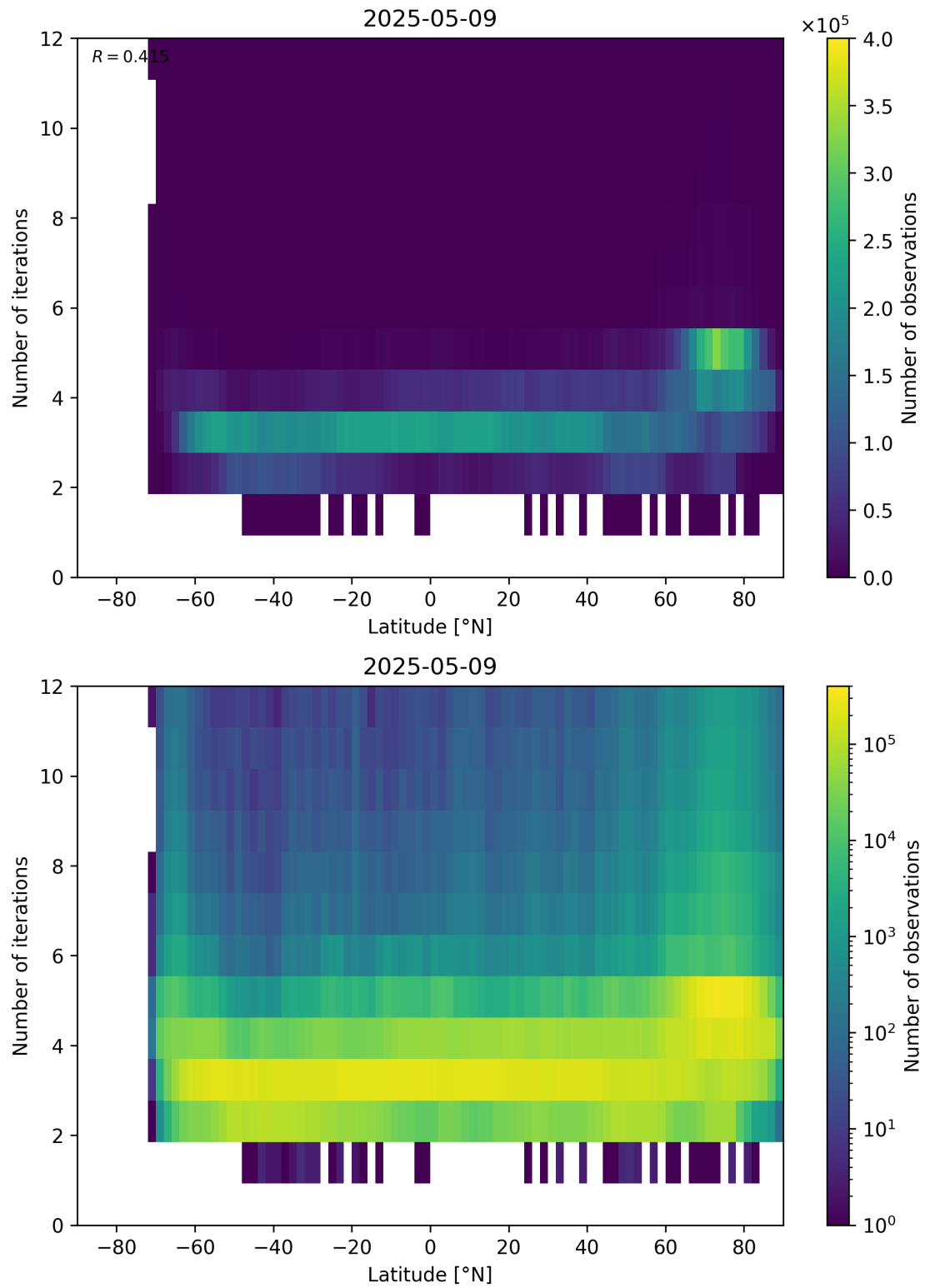
Figure 93: Scatter density plot of “Latitude” against “Number of iterations” for 2025-05-08 to 2025-05-10.
