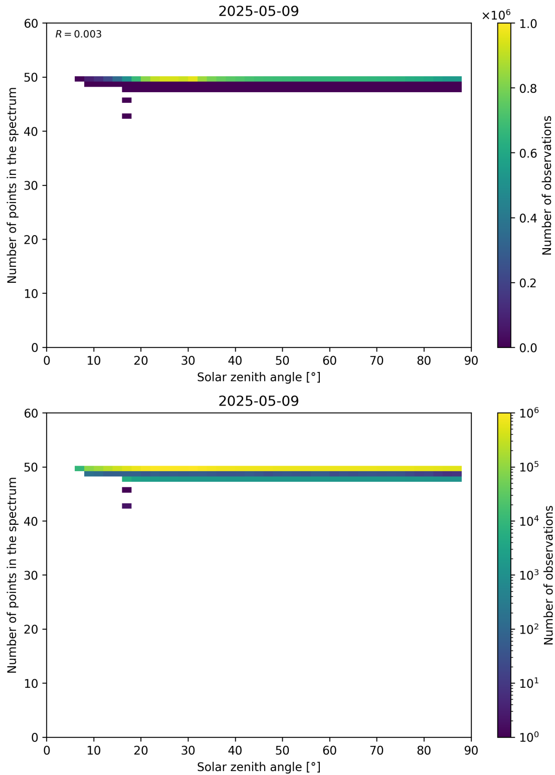
Figure 115: Scatter density plot of “Solar zenith angle” against “Number of points in the spectrum” for 2025-05-08 to 2025-05-10.
