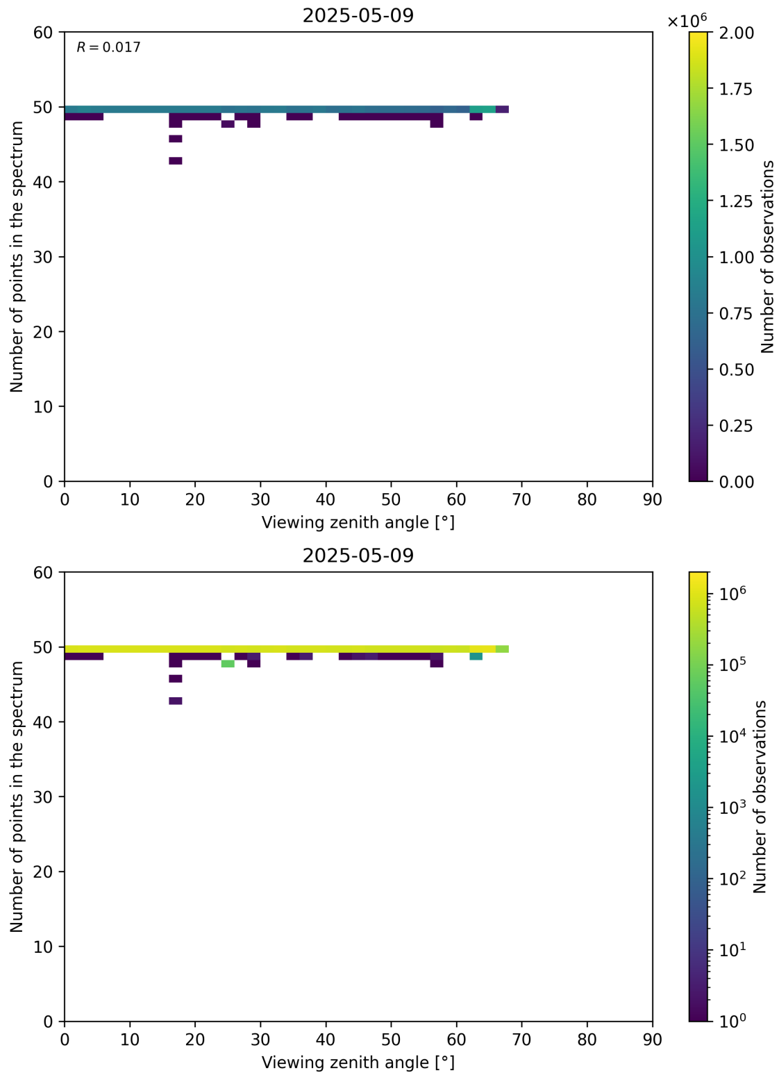
Figure 125: Scatter density plot of “Viewing zenith angle” against “Number of points in the spectrum” for 2025-05-08 to 2025-05-10.
