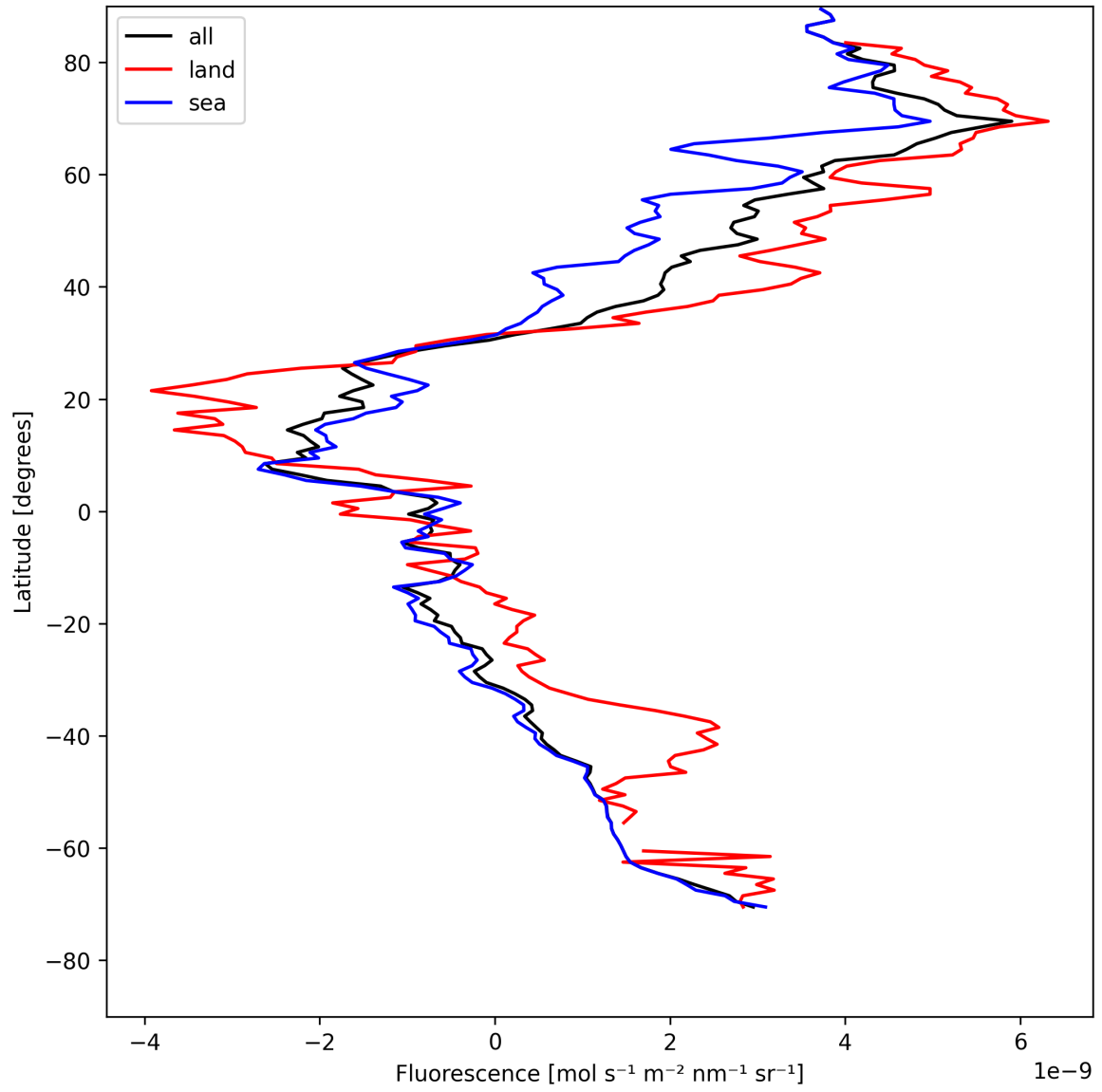
Figure 23: Zonal average of “Fluorescence” for 2025-05-08 to 2025-05-10.
