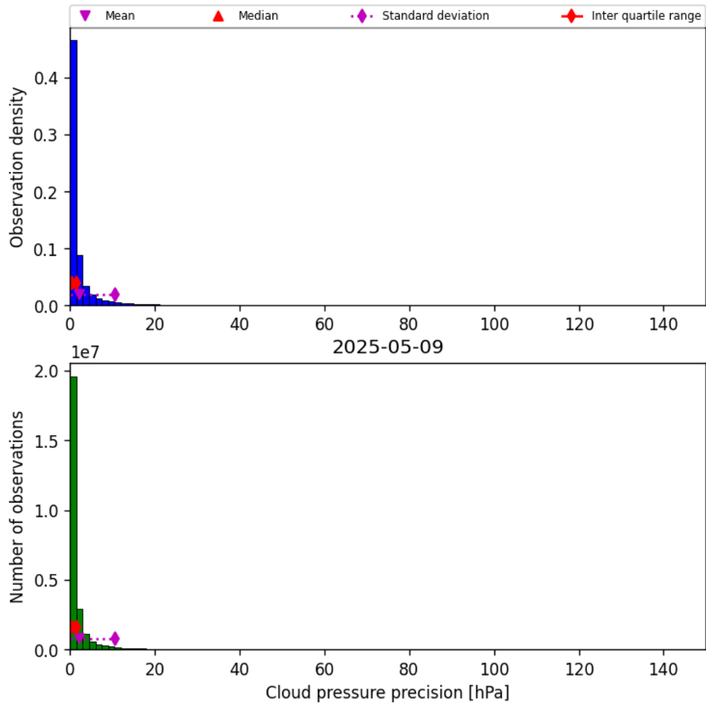
Figure 31: Histogram of “Cloud pressure precision” for 2025-05-08 to 2025-05-10
