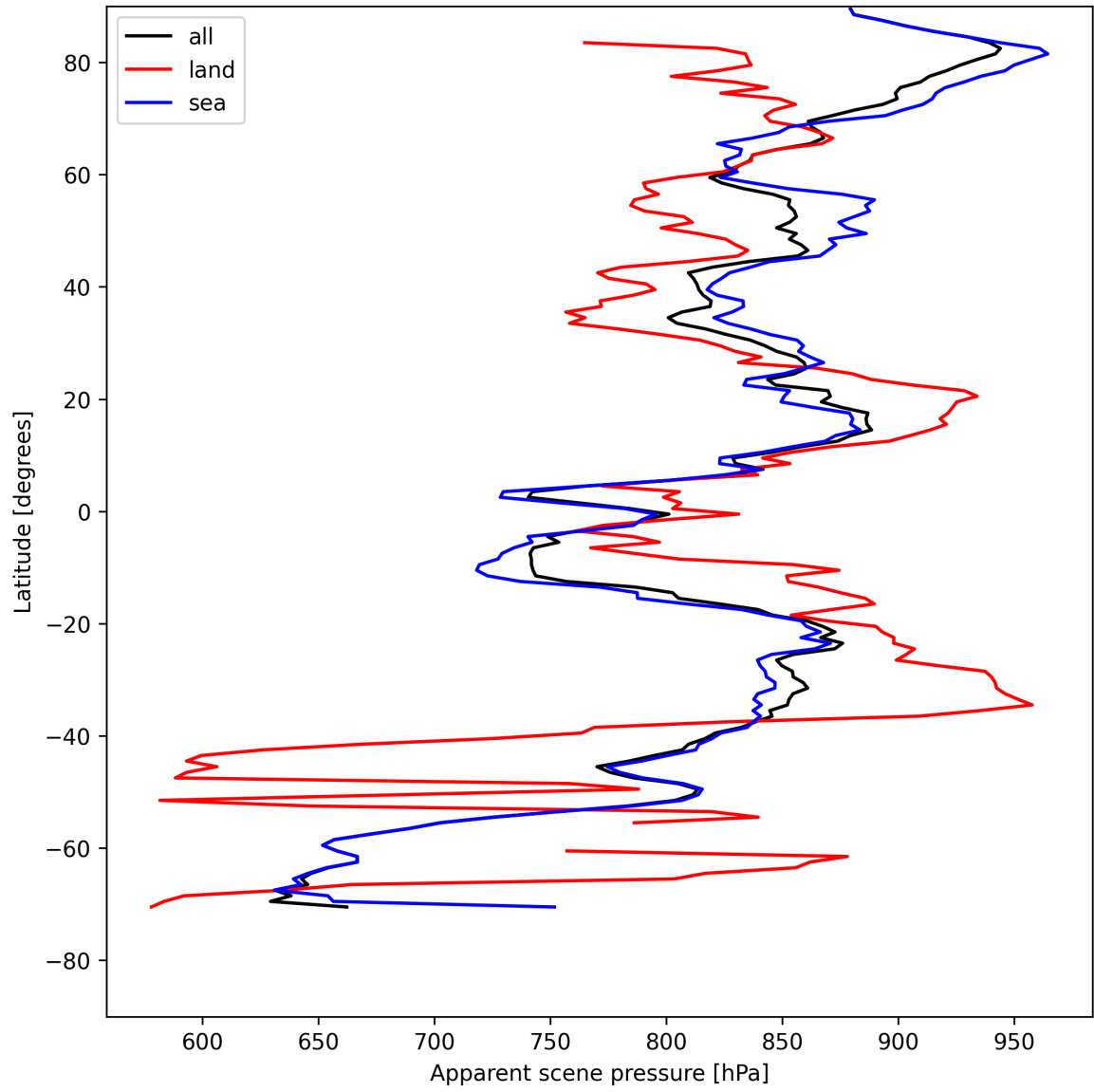
Figure 19: Zonal average of “Apparent scene pressure” for 2025-05-08 to 2025-05-10.
