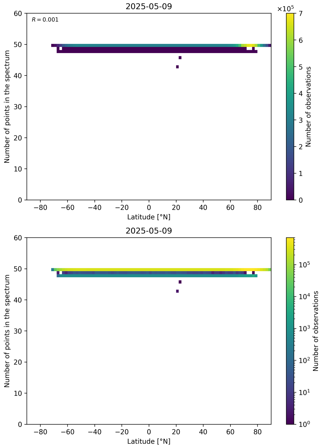
Figure 94: Scatter density plot of “Latitude” against “Number of points in the spectrum” for 2025-05-08 to 2025-05-10.
