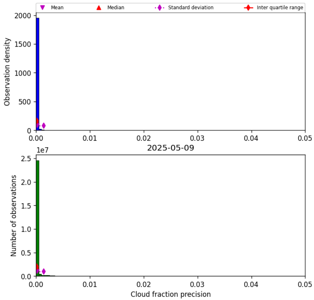
Figure 33: Histogram of “Cloud fraction precision” for 2025-05-08 to 2025-05-10
