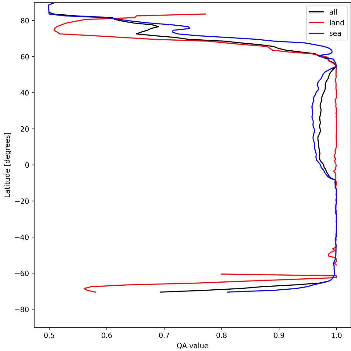
Figure 12: Zonal average of “QA value” for 2025-05-08 to 2025-05-10.
