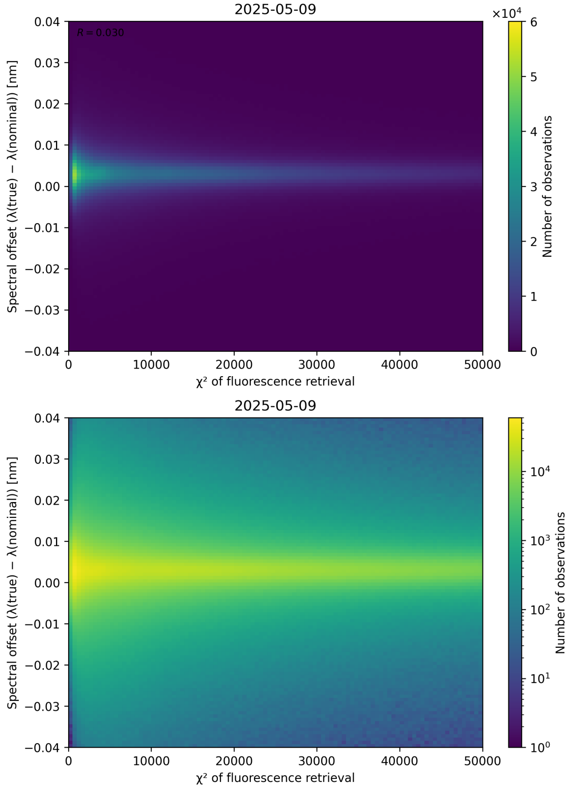
Figure 69: Scatter density plot of " \chi^2 of fluorescence retrieval" against "Spectral offset ( \lambda_{\text{true}} - \lambda_{\text{nominal}} )" for 2025-05-08 to 2025-05-10.
