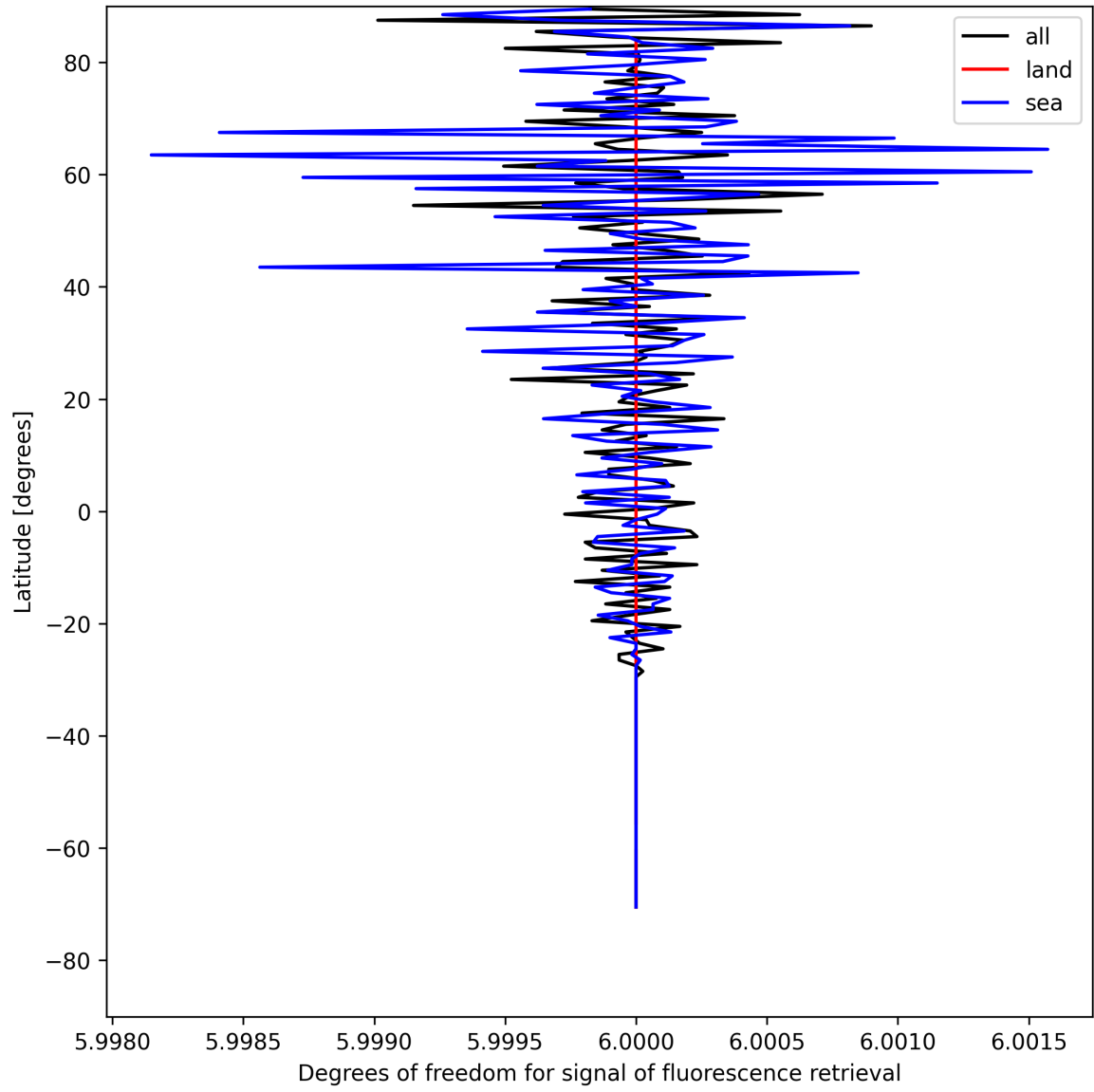
Figure 26: Zonal average of “Degrees of freedom for signal of fluorescence retrieval” for 2025-05-08 to 2025-05-10.
