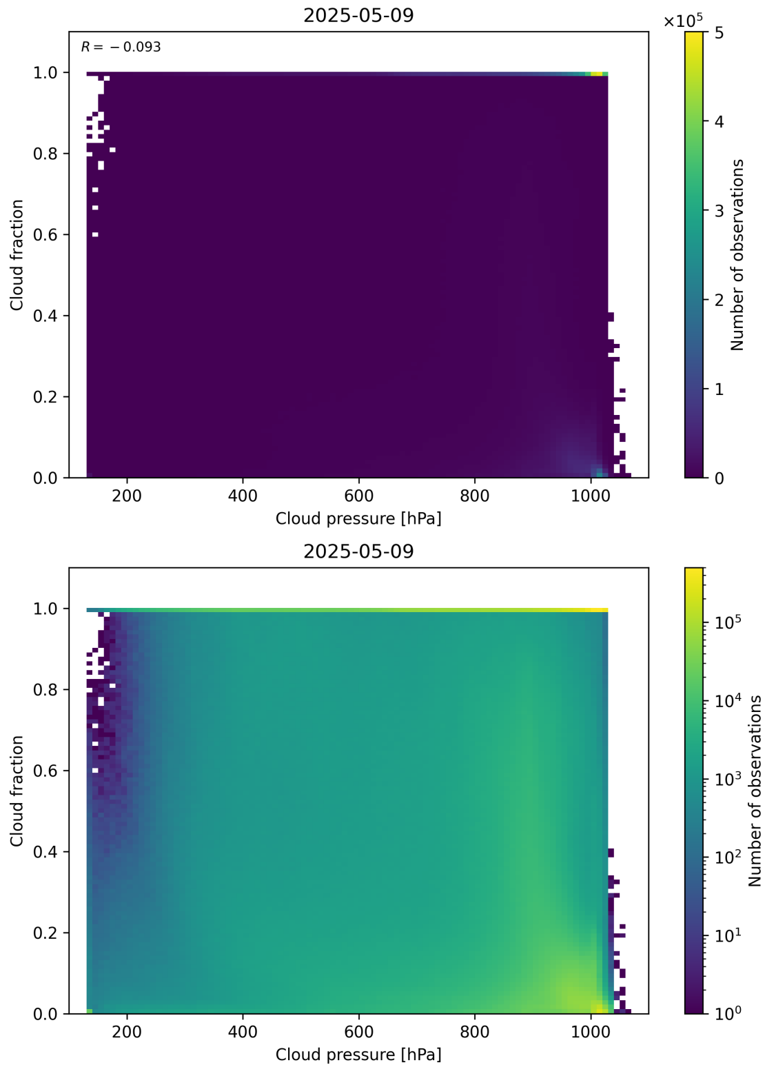
Figure 79: Scatter density plot of “Cloud pressure” against “Cloud fraction” for 2025-05-08 to 2025-05-10.
