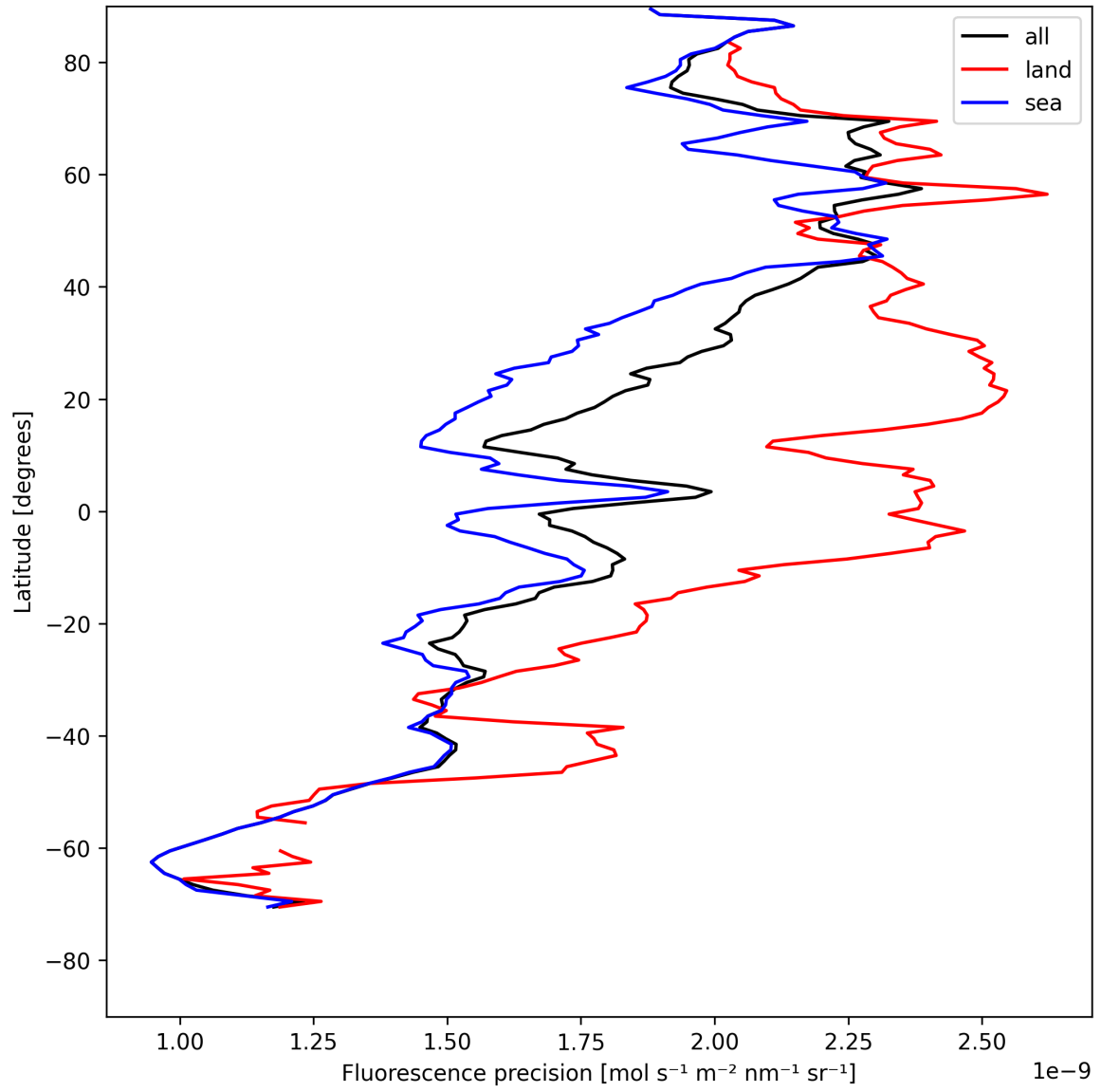
Figure 24: Zonal average of “Fluorescence precision” for 2025-05-08 to 2025-05-10.
