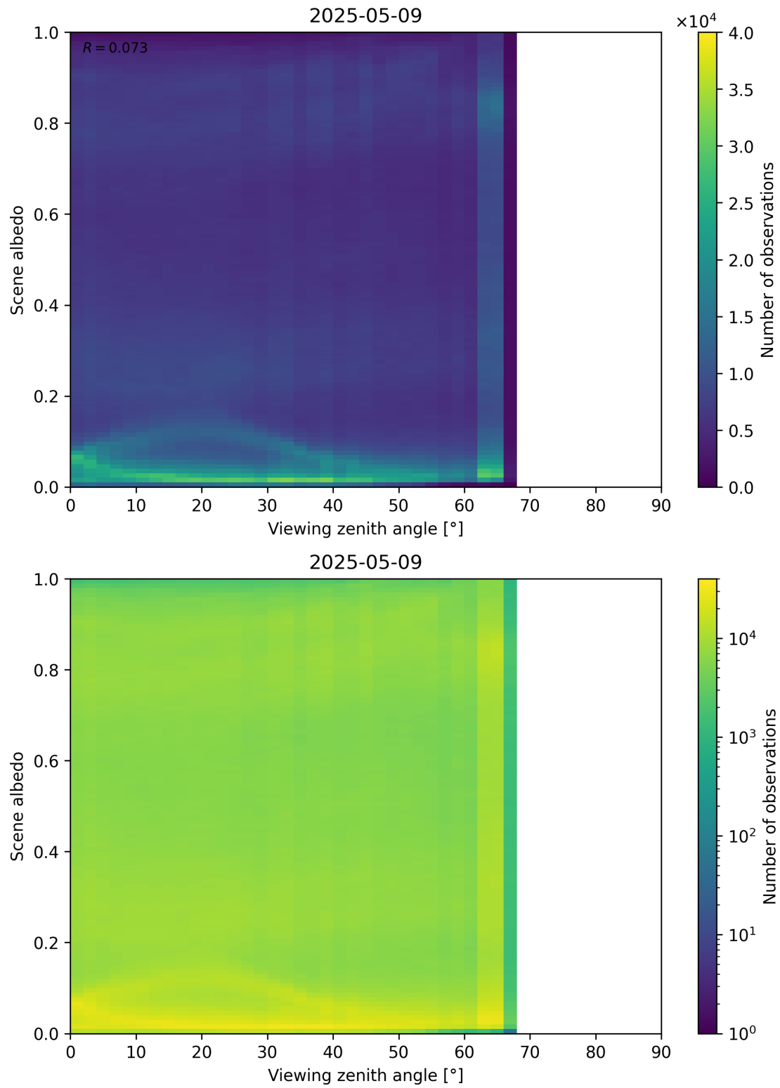
Figure 126: Scatter density plot of “Viewing zenith angle” against “Scene albedo” for 2025-05-08 to 2025-05-10.
