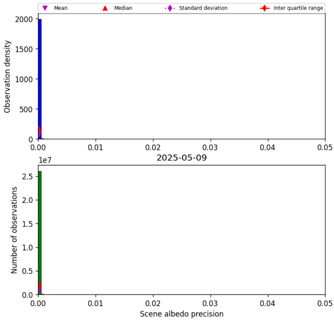
Figure 35: Histogram of “Scene albedo precision” for 2025-05-08 to 2025-05-10
