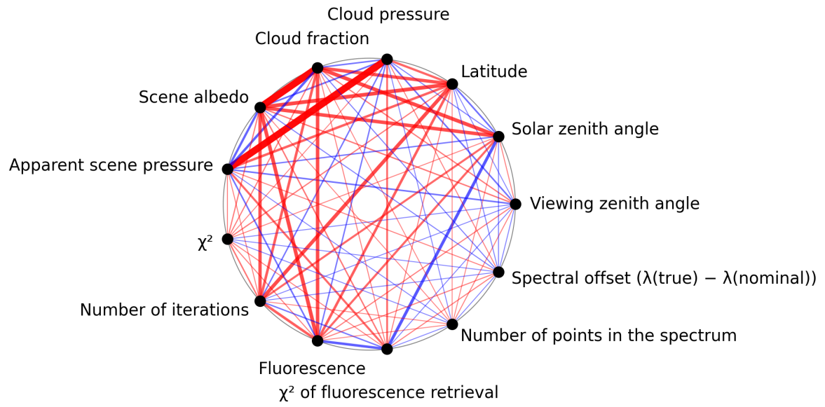
Figure 1: Map of correlation graph for 2025-05-08 to 2025-05-10.
