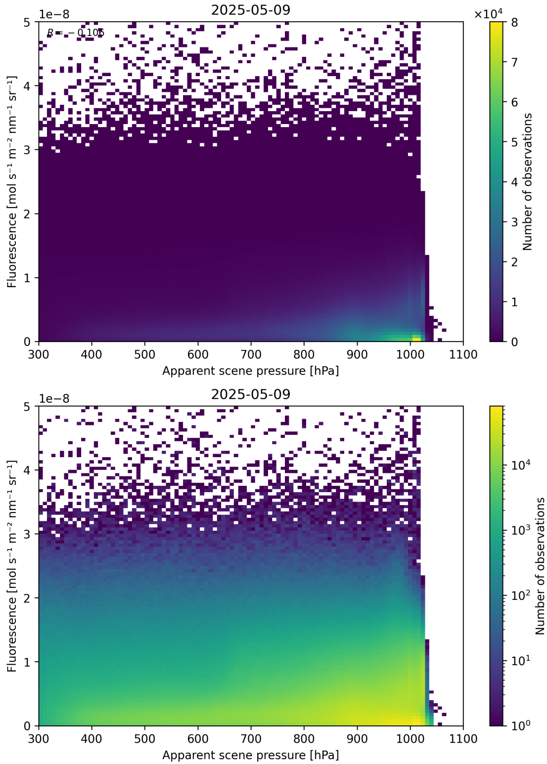
Figure 64: Scatter density plot of “Apparent scene pressure” against “Fluorescence” for 2025-05-08 to 2025-05-10.
