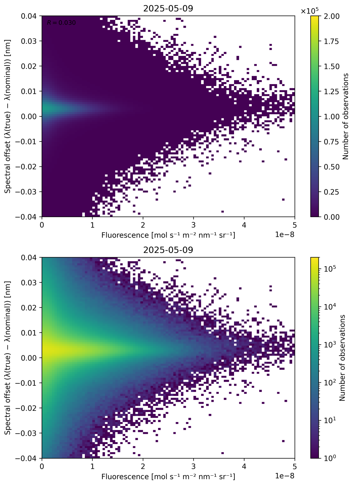
Figure 87: Scatter density plot of “Fluorescence” against “Spectral offset ( \lambda_{\text{true}} - \lambda_{\text{nominal}} )” for 2025-05-08 to 2025-05-10.
