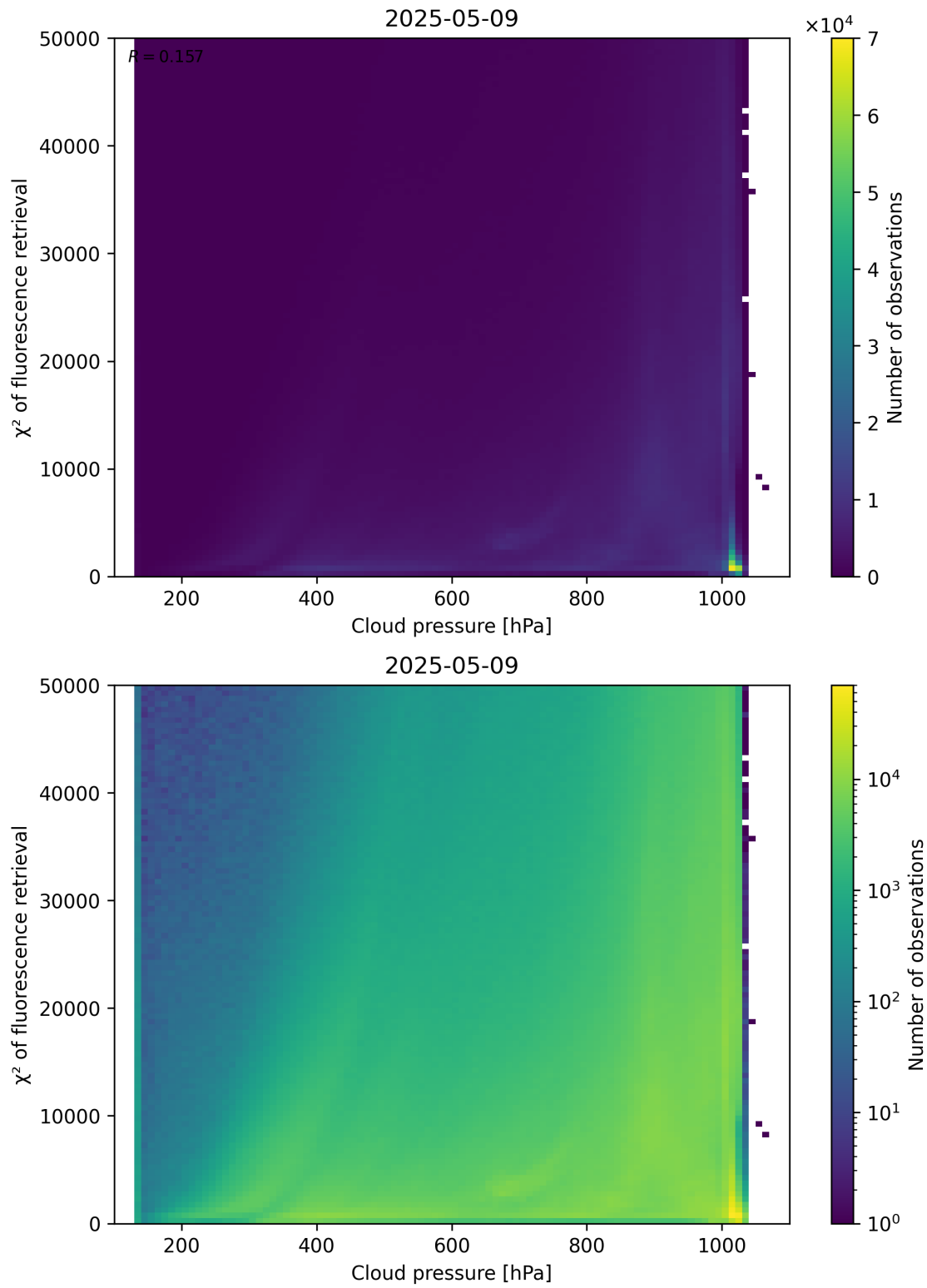
Figure 78: Scatter density plot of “Cloud pressure” against “ \chi^2 of fluorescence retrieval” for 2025-05-08 to 2025-05-10.
