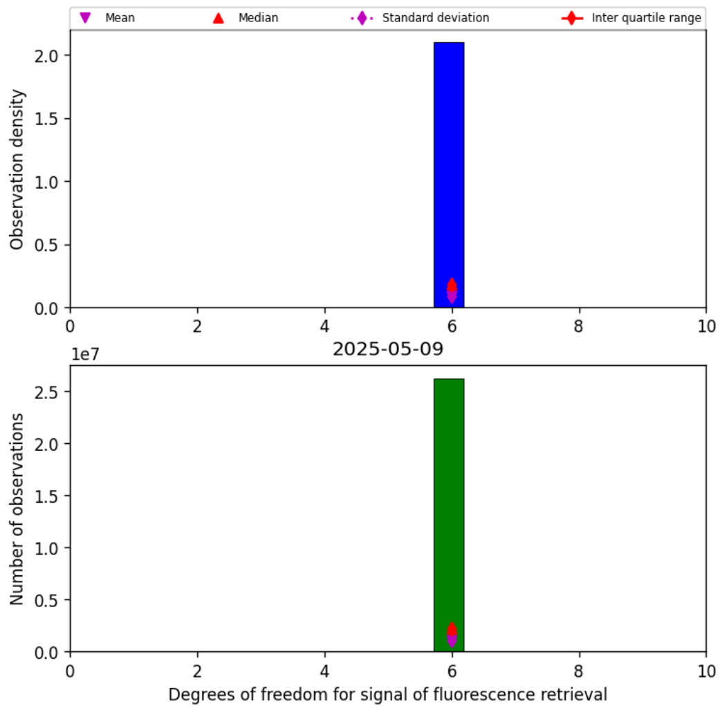
Figure 43: Histogram of "Degrees of freedom for signal of fluorescence retrieval" for 2025-05-08 to 2025-05-10
