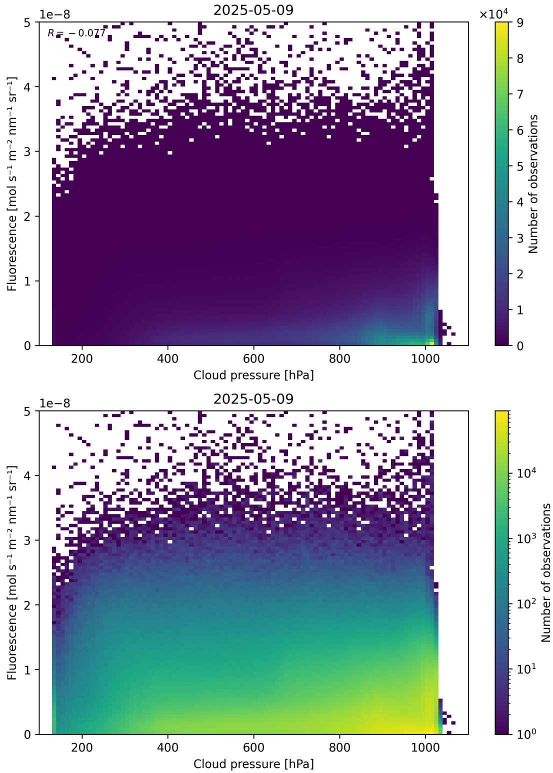
Figure 80: Scatter density plot of “Cloud pressure” against “Fluorescence” for 2025-05-08 to 2025-05-10.
