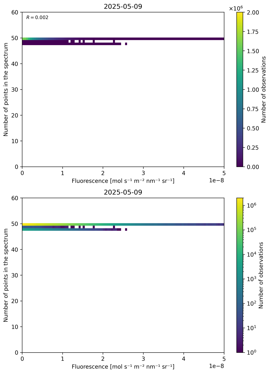
Figure 86: Scatter density plot of “Fluorescence” against “Number of points in the spectrum” for 2025-05-08 to 2025-05-10.
