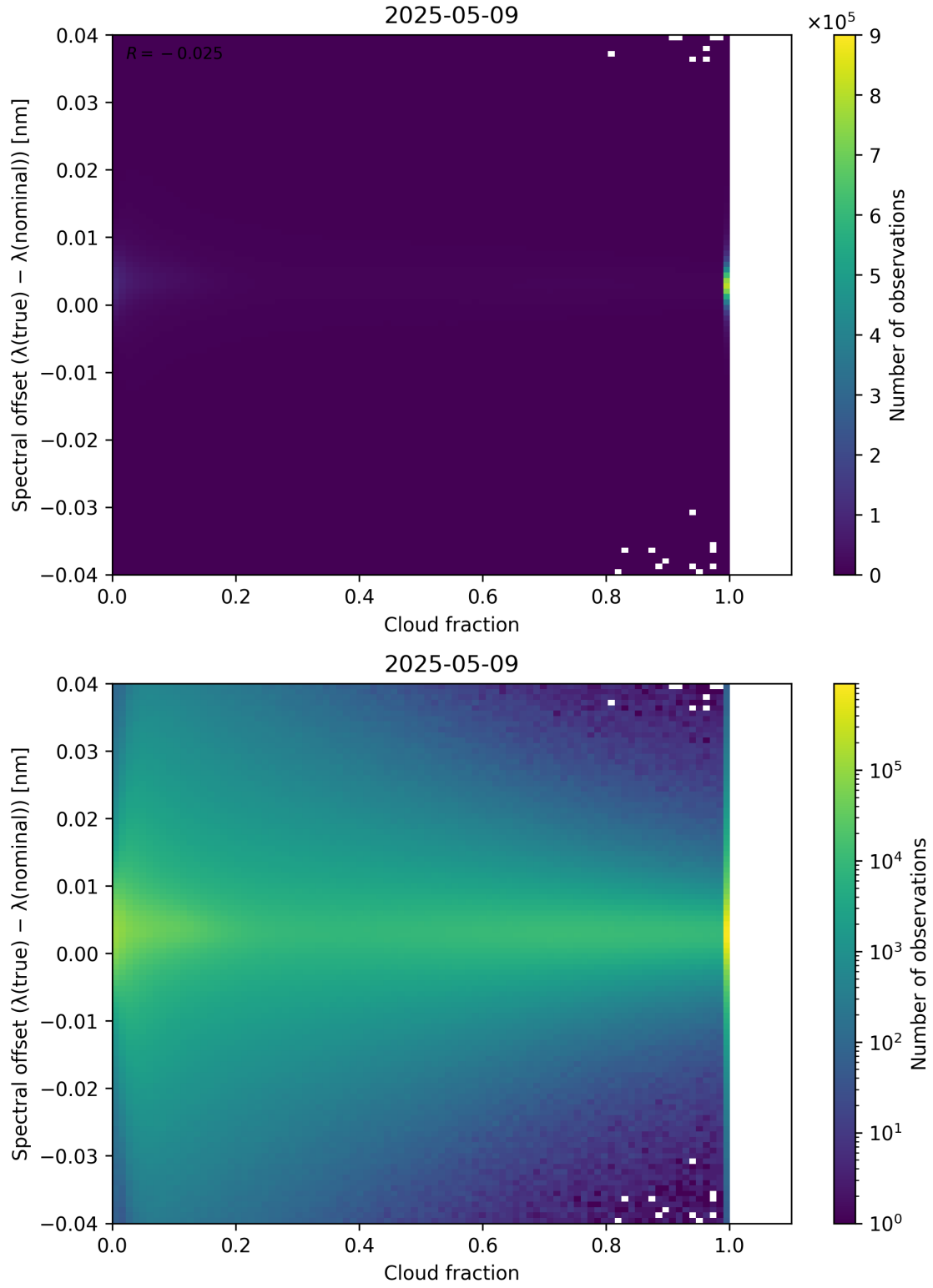
Figure 76: Scatter density plot of “Cloud fraction” against “Spectral offset ( \lambda_{\text{true}} - \lambda_{\text{nominal}} )” for 2025-05-08 to 2025-05-10.
