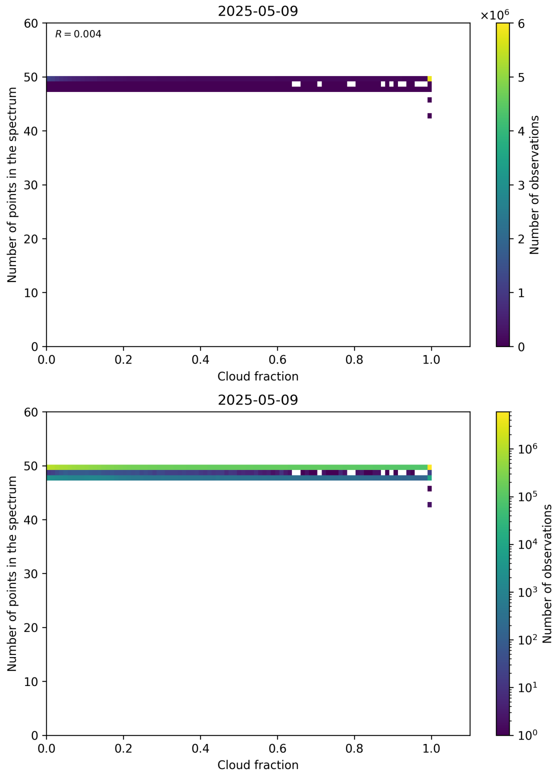
Figure 74: Scatter density plot of “Cloud fraction” against “Number of points in the spectrum” for 2025-05-08 to 2025-05-10.
