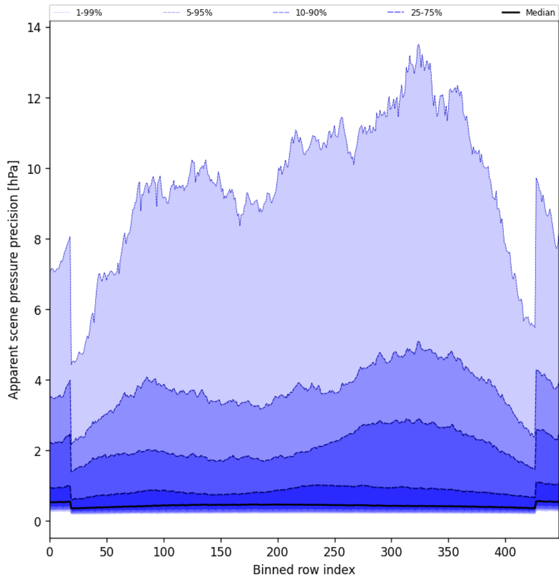
Figure 54: Along track statistics of “Apparent scene pressure precision” for 2025-05-08 to 2025-05-10
