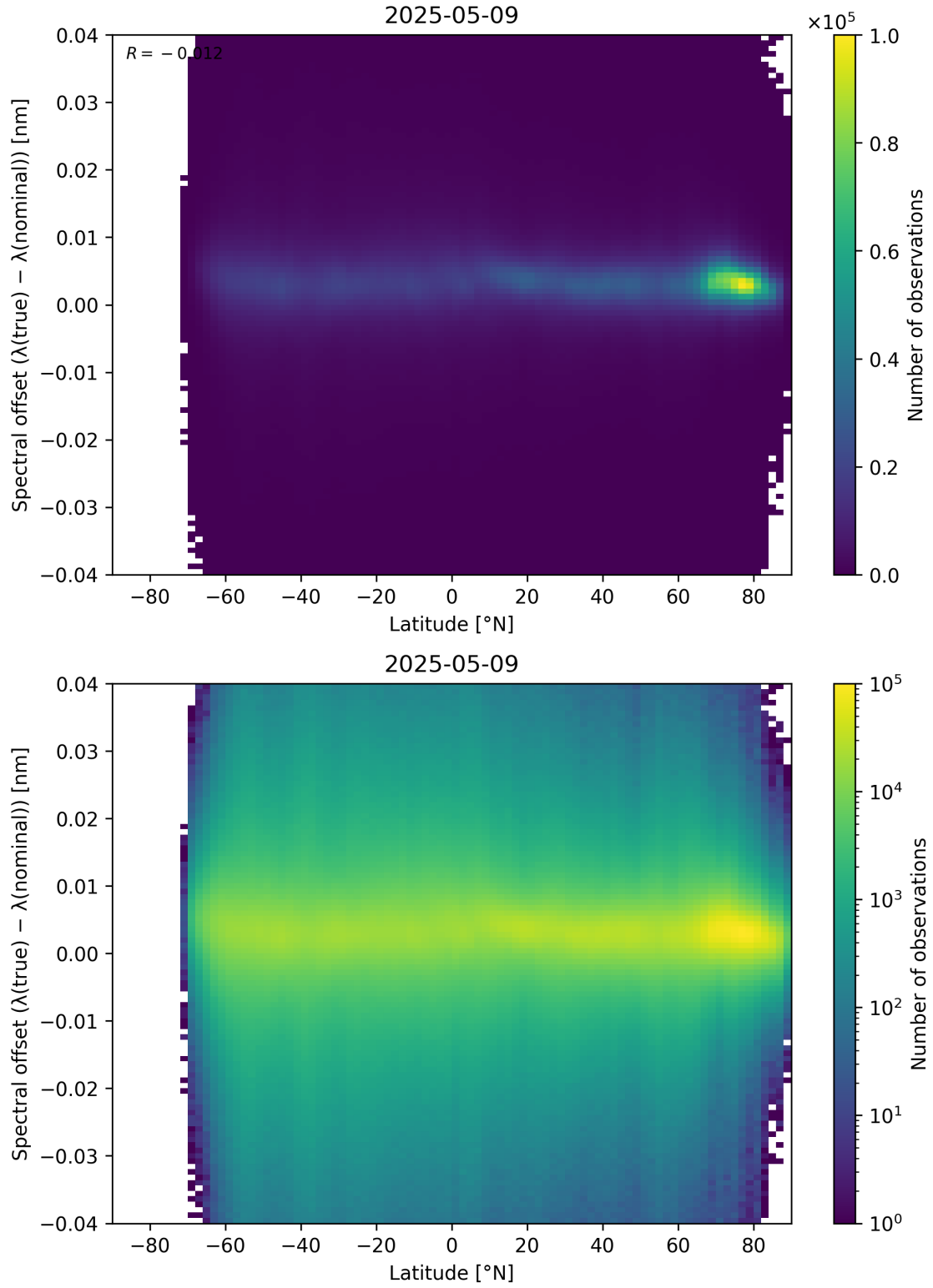
Figure 96: Scatter density plot of “Latitude” against “Spectral offset ( \lambda_{\text{true}} - \lambda_{\text{nominal}} )” for 2025-05-08 to 2025-05-10.
