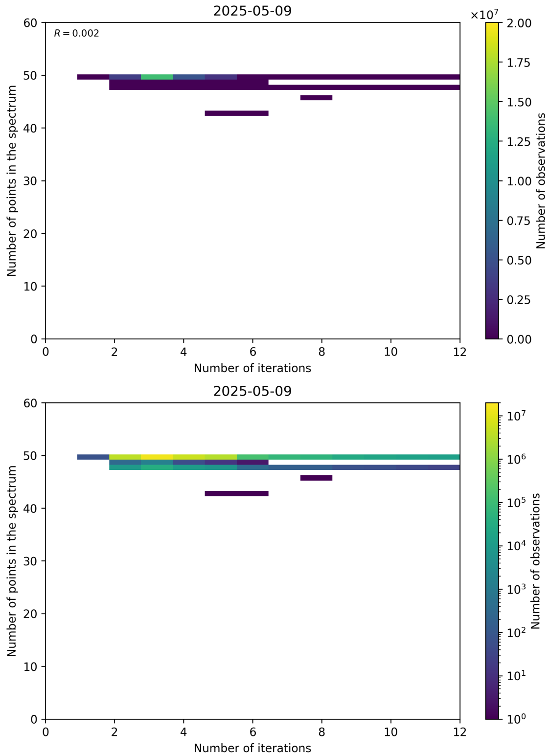
Figure 99: Scatter density plot of “Number of iterations” against “Number of points in the spectrum” for 2025-05-08 to 2025-05-10.
