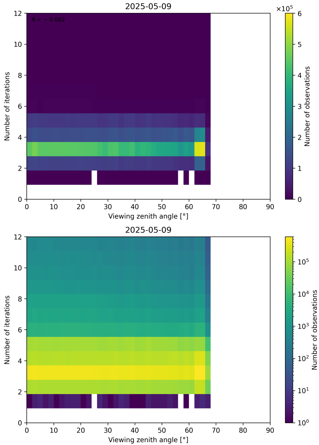
Figure 124: Scatter density plot of “Viewing zenith angle” against “Number of iterations” for 2025-05-08 to 2025-05-10.
