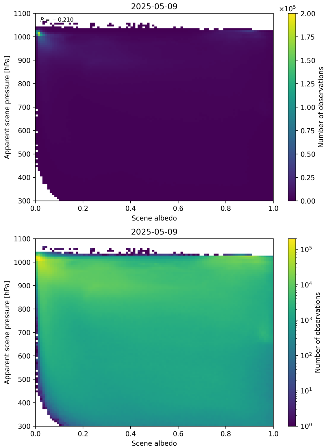
Figure 102: Scatter density plot of “Scene albedo” against “Apparent scene pressure” for 2025-05-08 to 2025-05-10.
