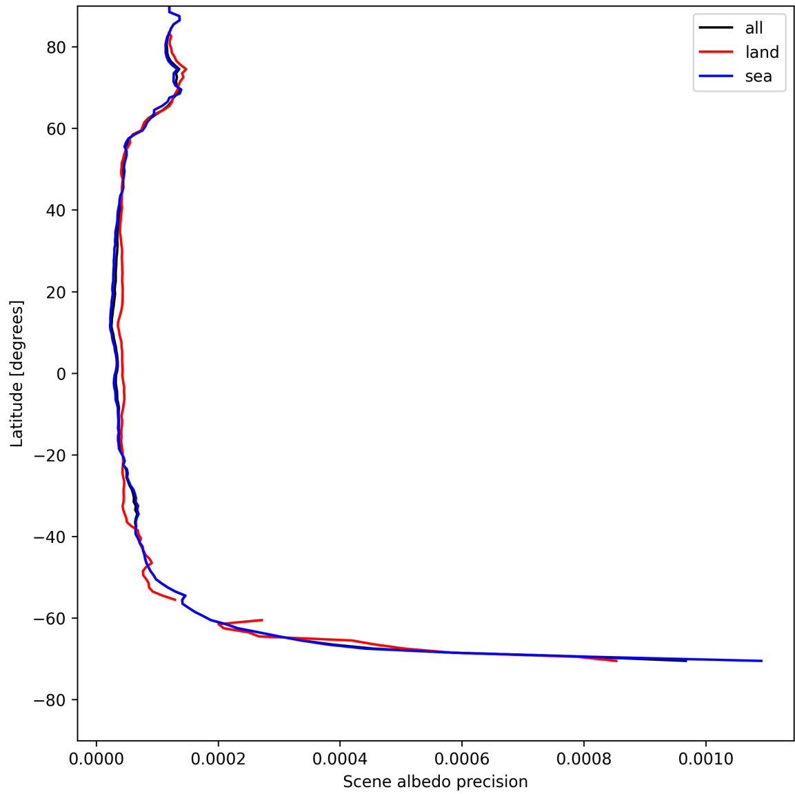
Figure 18: Zonal average of “Scene albedo precision” for 2025-05-08 to 2025-05-10.
