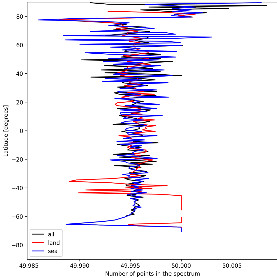
Figure 27: Zonal average of “Number of points in the spectrum” for 2025-05-08 to 2025-05-10.
