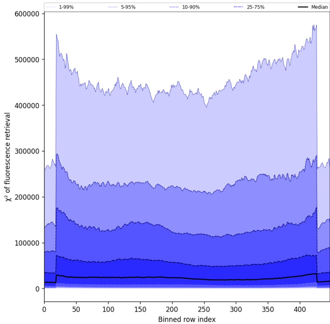
Figure 59: Along track statistics of “ \chi^2 of fluorescence retrieval” for 2025-05-08 to 2025-05-10
