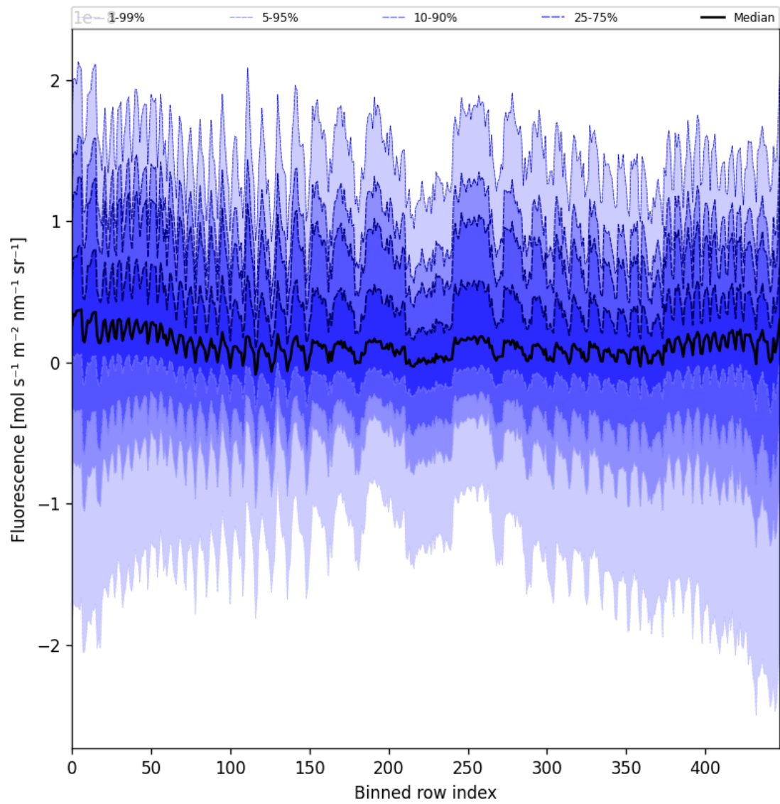
Figure 57: Along track statistics of “Fluorescence” for 2025-05-08 to 2025-05-10
