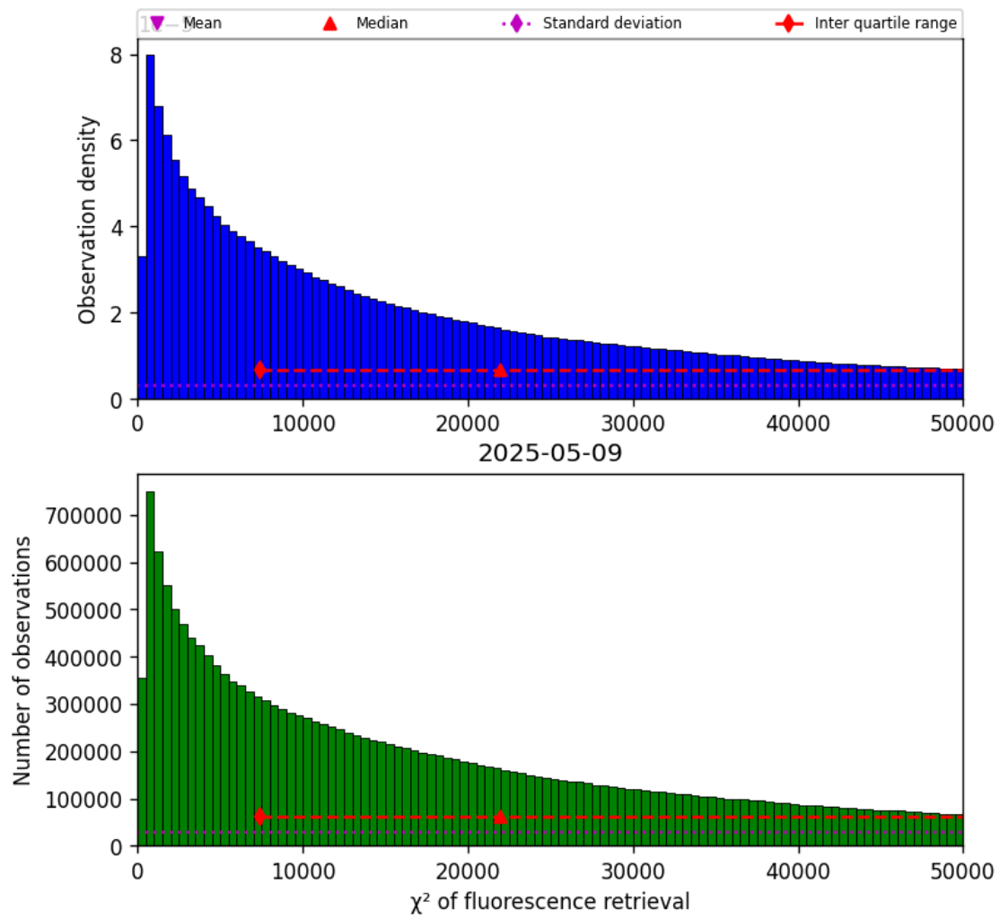
Figure 42: Histogram of “ \chi^2 of fluorescence retrieval” for 2025-05-08 to 2025-05-10
