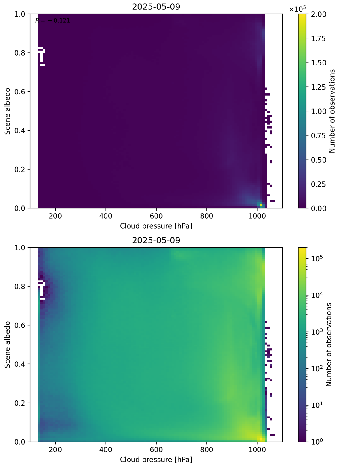
Figure 83: Scatter density plot of “Cloud pressure” against “Scene albedo” for 2025-05-08 to 2025-05-10.
