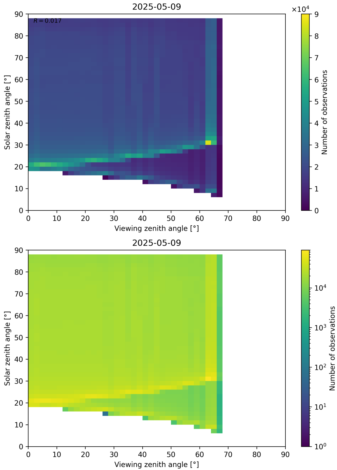
Figure 127: Scatter density plot of “Viewing zenith angle” against “Solar zenith angle” for 2025-05-08 to 2025-05-10.
