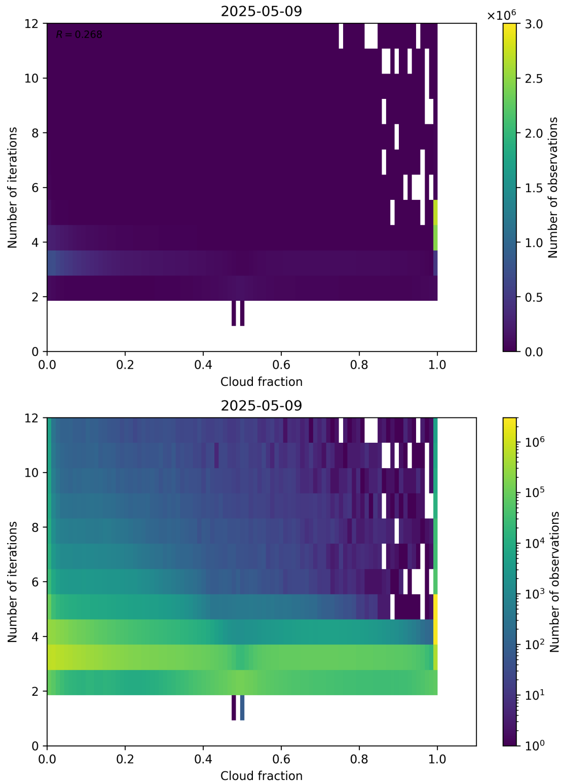
Figure 73: Scatter density plot of “Cloud fraction” against “Number of iterations” for 2025-05-08 to 2025-05-10.
