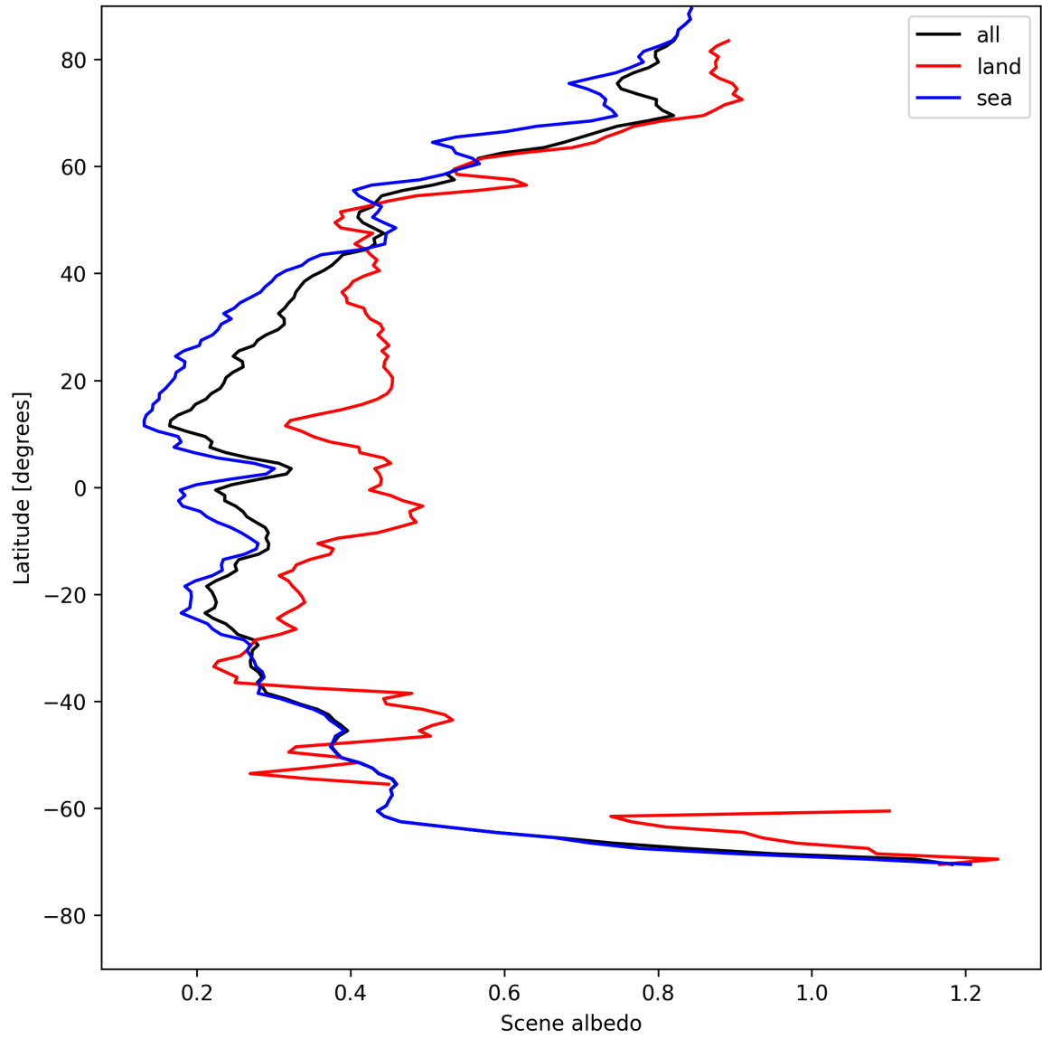
Figure 17: Zonal average of “Scene albedo” for 2025-05-08 to 2025-05-10.
