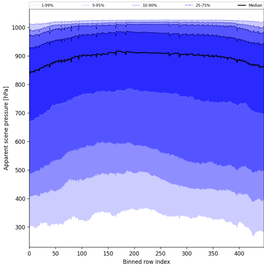
Figure 53: Along track statistics of “Apparent scene pressure” for 2025-05-08 to 2025-05-10
