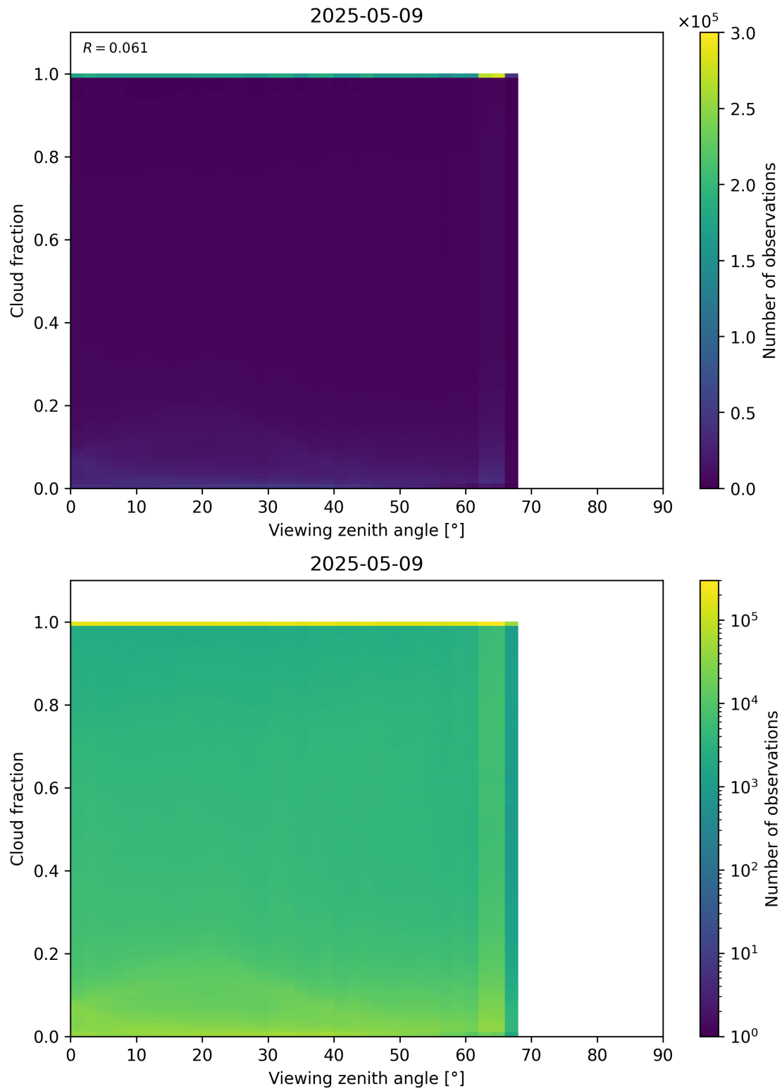
Figure 120: Scatter density plot of “Viewing zenith angle” against “Cloud fraction” for 2025-05-08 to 2025-05-10.
