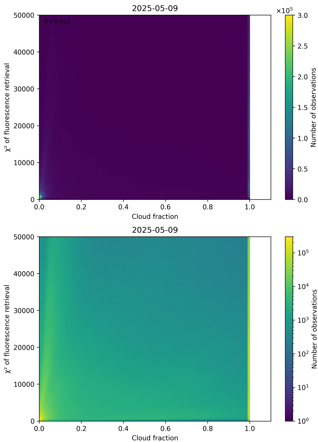
Figure 71: Scatter density plot of “Cloud fraction” against “ \chi^2 of fluorescence retrieval” for 2025-05-08 to 2025-05-10.
