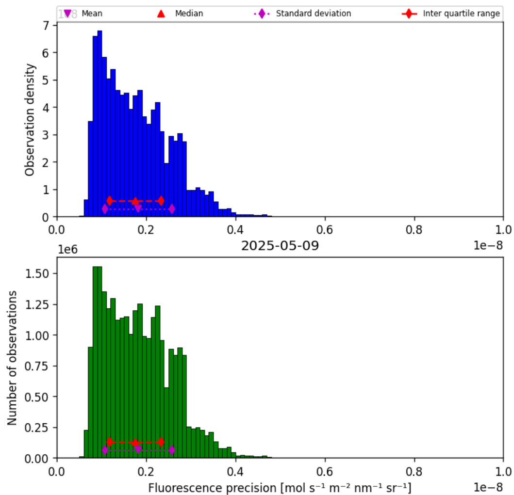
Figure 41: Histogram of “Fluorescence precision” for 2025-05-08 to 2025-05-10
