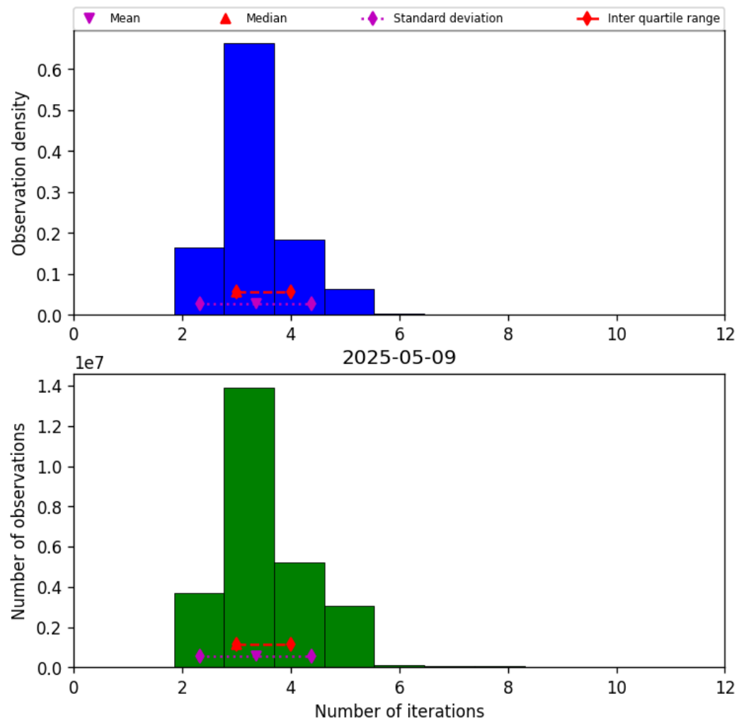
Figure 39: Histogram of “Number of iterations” for 2025-05-08 to 2025-05-10
