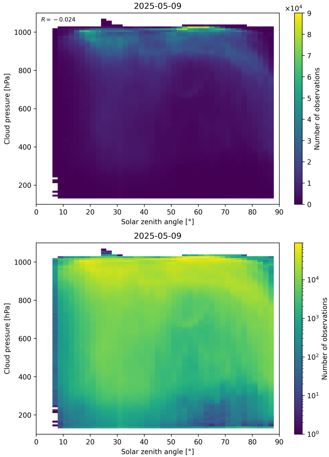
Figure 111: Scatter density plot of “Solar zenith angle” against “Cloud pressure” for 2025-05-08 to 2025-05-10.
