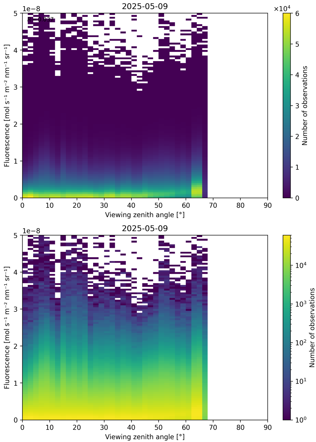
Figure 122: Scatter density plot of “Viewing zenith angle” against “Fluorescence” for 2025-05-08 to 2025-05-10.
