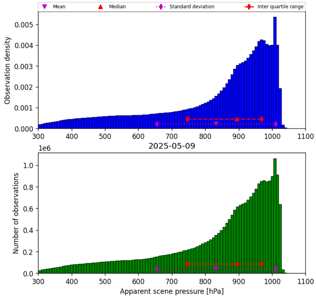
Figure 36: Histogram of “Apparent scene pressure” for 2025-05-08 to 2025-05-10
