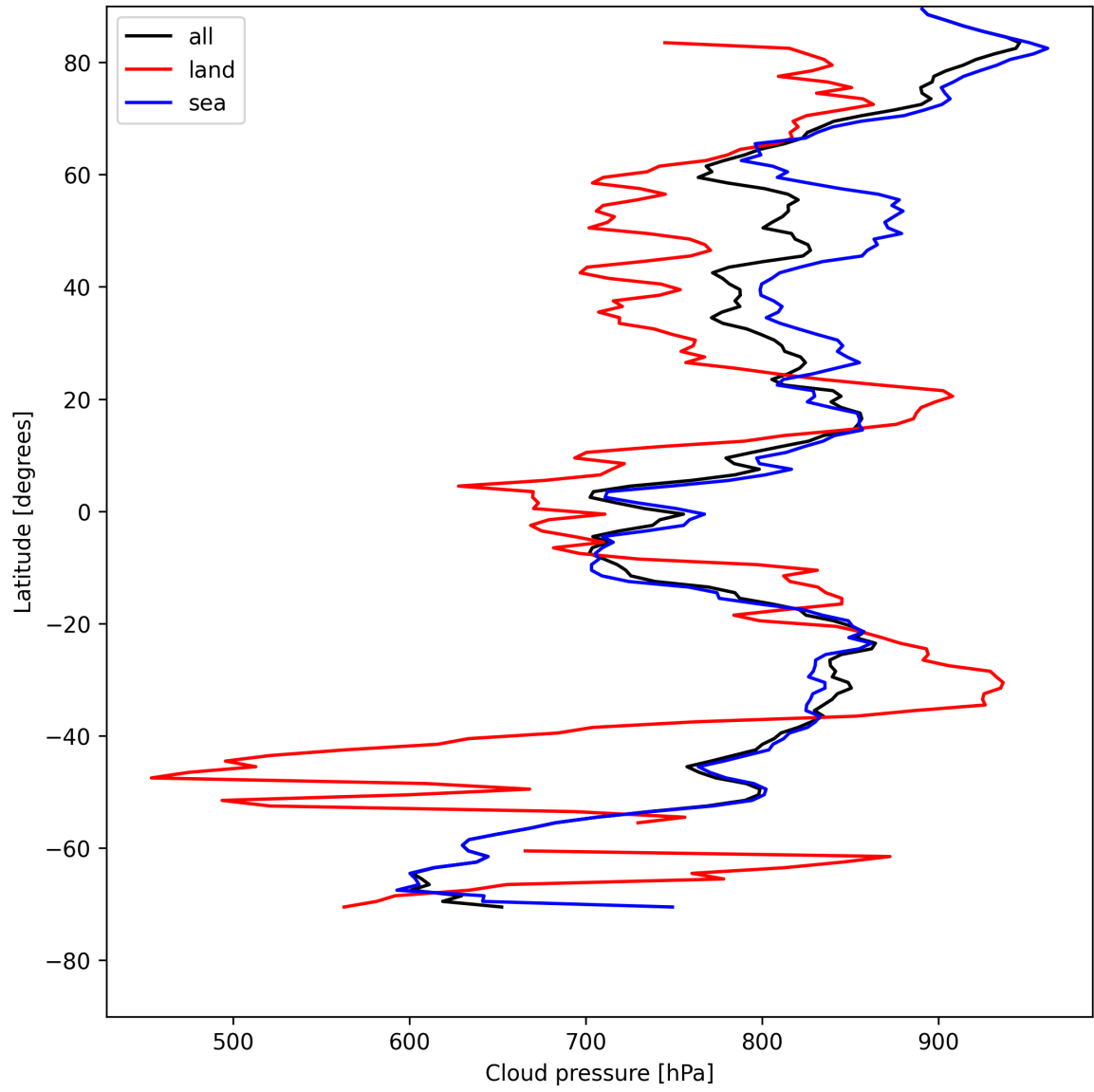
Figure 13: Zonal average of “Cloud pressure” for 2025-05-08 to 2025-05-10.
