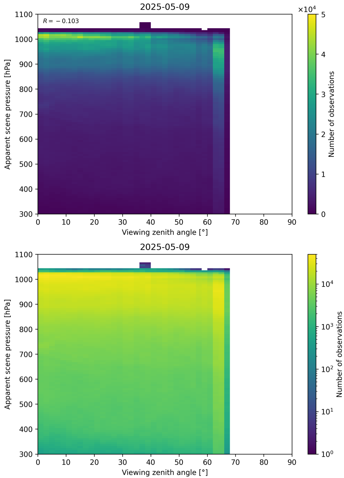
Figure 118: Scatter density plot of “Viewing zenith angle” against “Apparent scene pressure” for 2025-05-08 to 2025-05-10.
