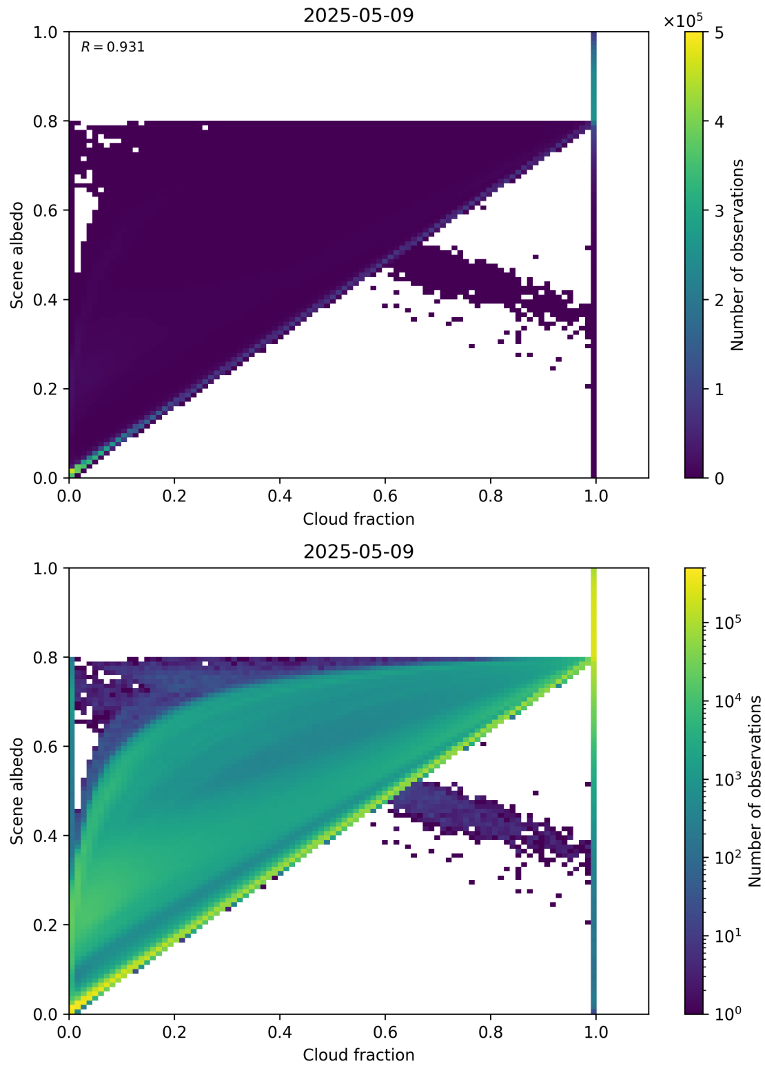
Figure 75: Scatter density plot of “Cloud fraction” against “Scene albedo” for 2025-05-08 to 2025-05-10.
