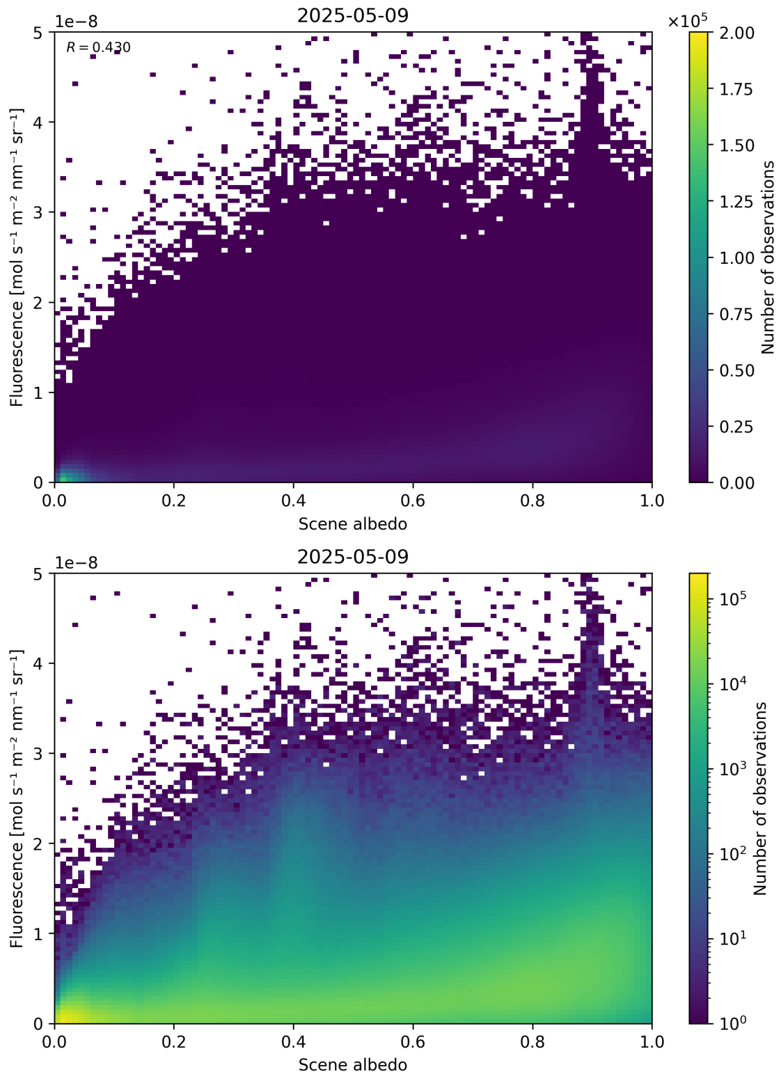
Figure 104: Scatter density plot of “Scene albedo” against “Fluorescence” for 2025-05-08 to 2025-05-10.
