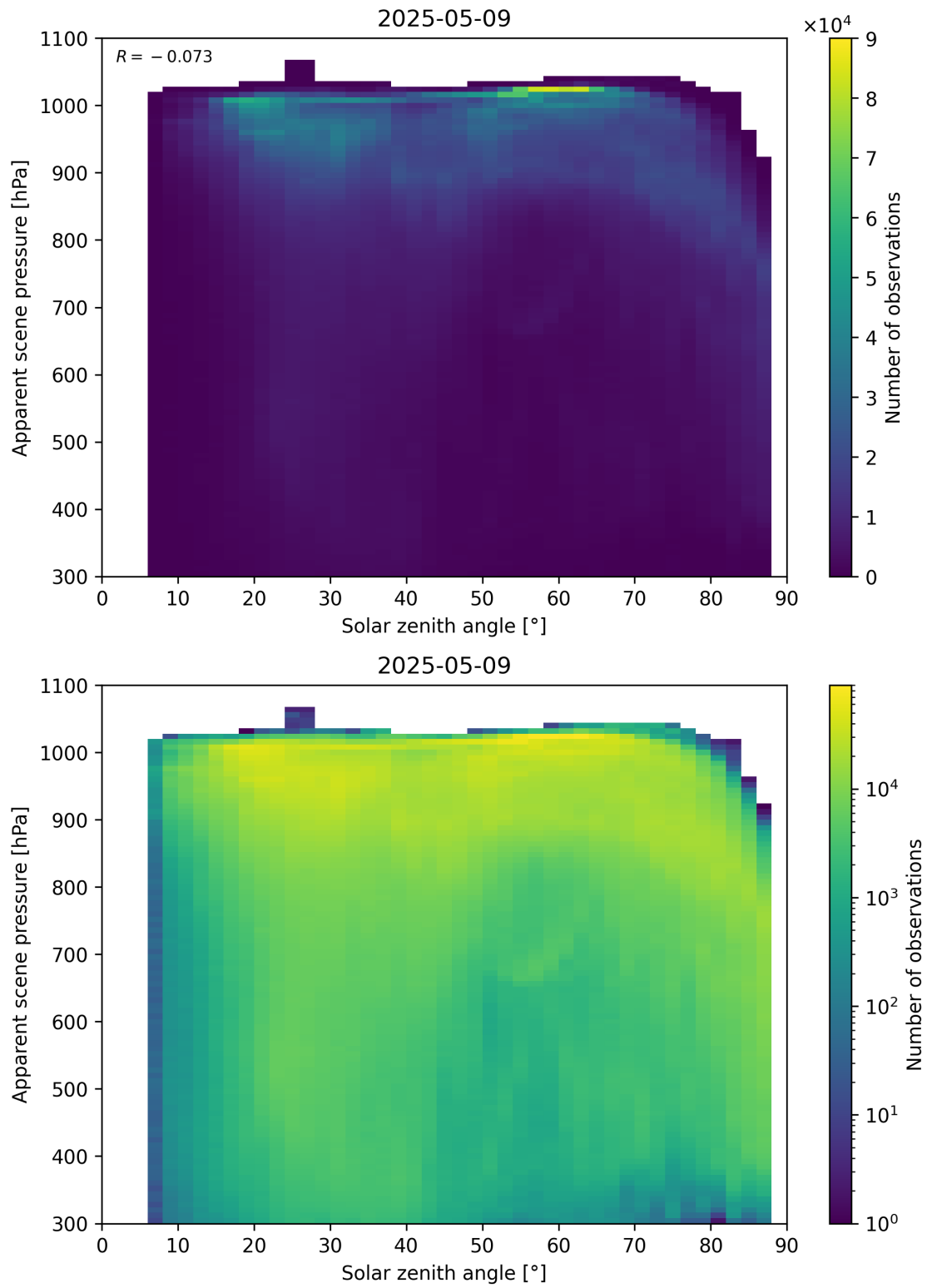
Figure 108: Scatter density plot of “Solar zenith angle” against “Apparent scene pressure” for 2025-05-08 to 2025-05-10.
