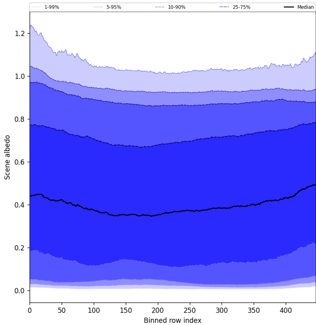
Figure 51: Along track statistics of “Scene albedo” for 2025-05-08 to 2025-05-10
