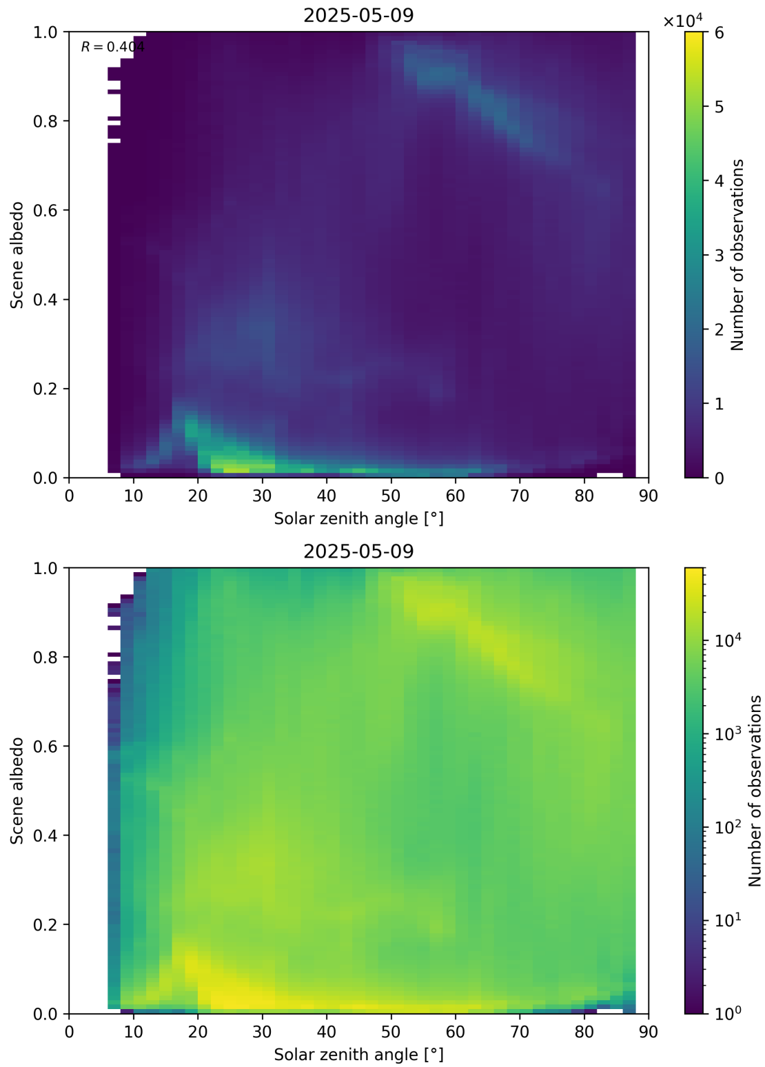
Figure 116: Scatter density plot of “Solar zenith angle” against “Scene albedo” for 2025-05-08 to 2025-05-10.
