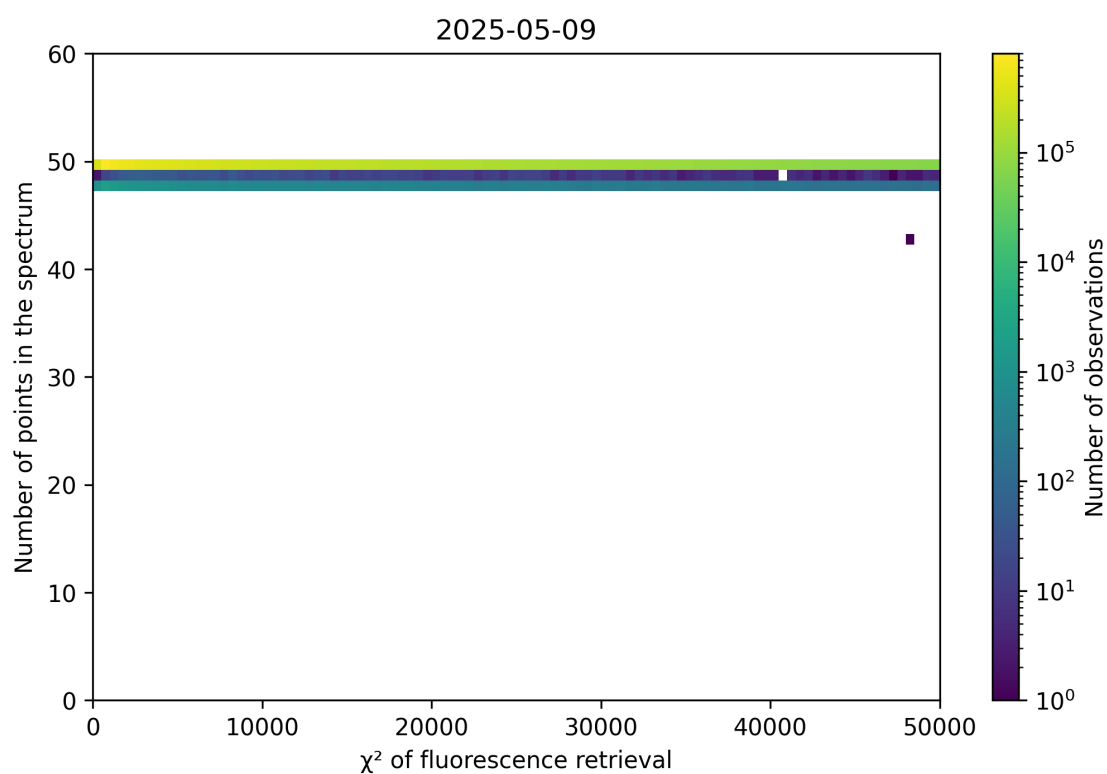
Figure 68: Scatter density plot of “ \chi^2 of fluorescence retrieval” against “Number of points in the spectrum” for 2025-05-08 to 2025-05-10.
