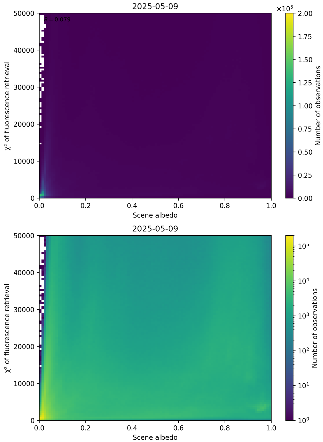
Figure 103: Scatter density plot of “Scene albedo” against “ \chi^2 of fluorescence retrieval” for 2025-05-08 to 2025-05-10.
