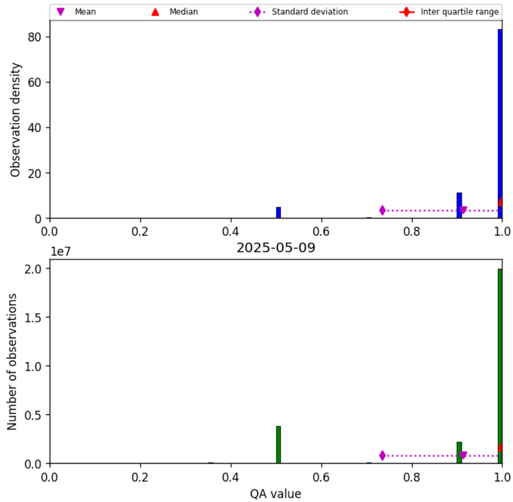
Figure 29: Histogram of “QA value” for 2025-05-08 to 2025-05-10
