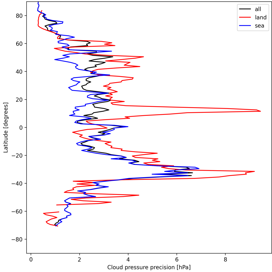
Figure 14: Zonal average of “Cloud pressure precision” for 2025-05-08 to 2025-05-10.
