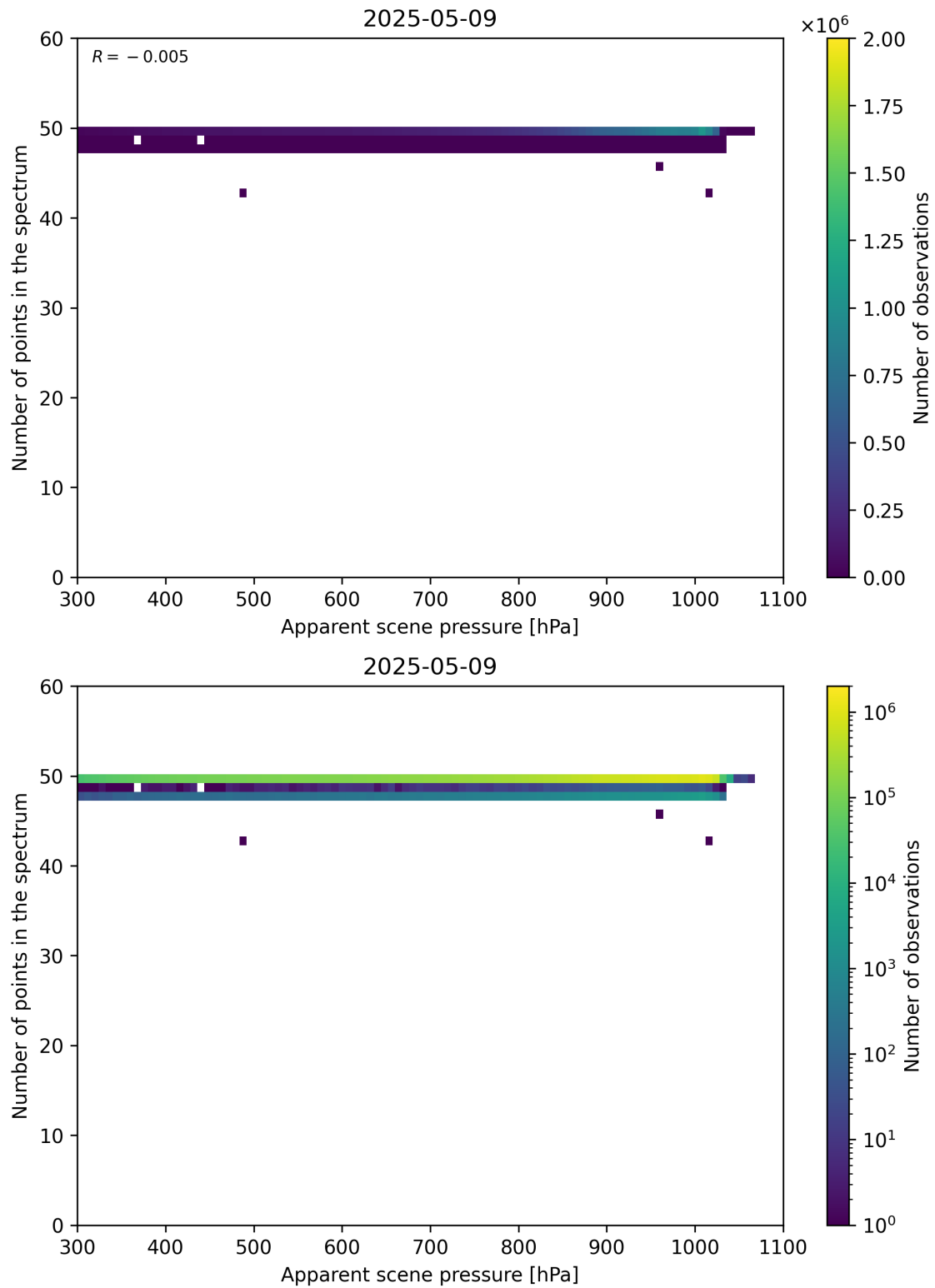
Figure 66: Scatter density plot of “Apparent scene pressure” against “Number of points in the spectrum” for 2025-05-08 to 2025-05-10.
