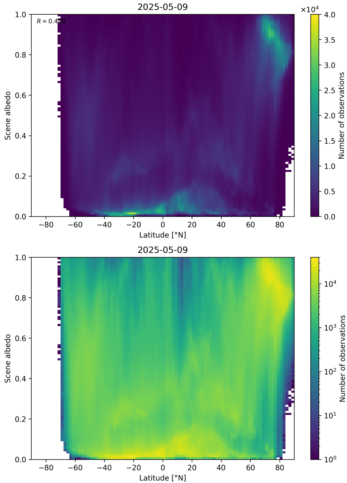
Figure 95: Scatter density plot of “Latitude” against “Scene albedo” for 2025-05-08 to 2025-05-10.
