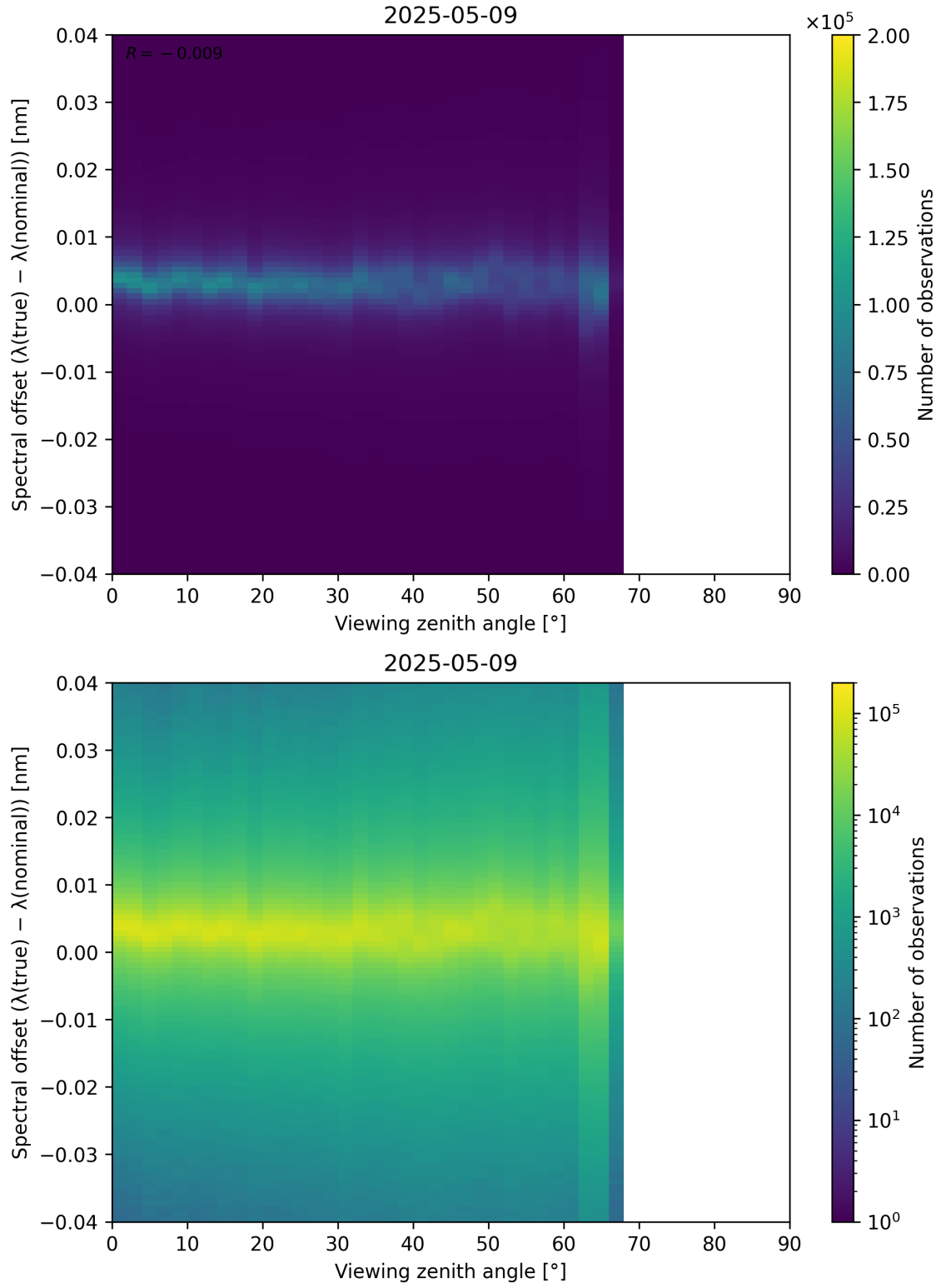
Figure 128: Scatter density plot of “Viewing zenith angle” against “Spectral offset ( \lambda_{\text{true}} - \lambda_{\text{nominal}} )” for 2025-05-08 to 2025-05-10.
