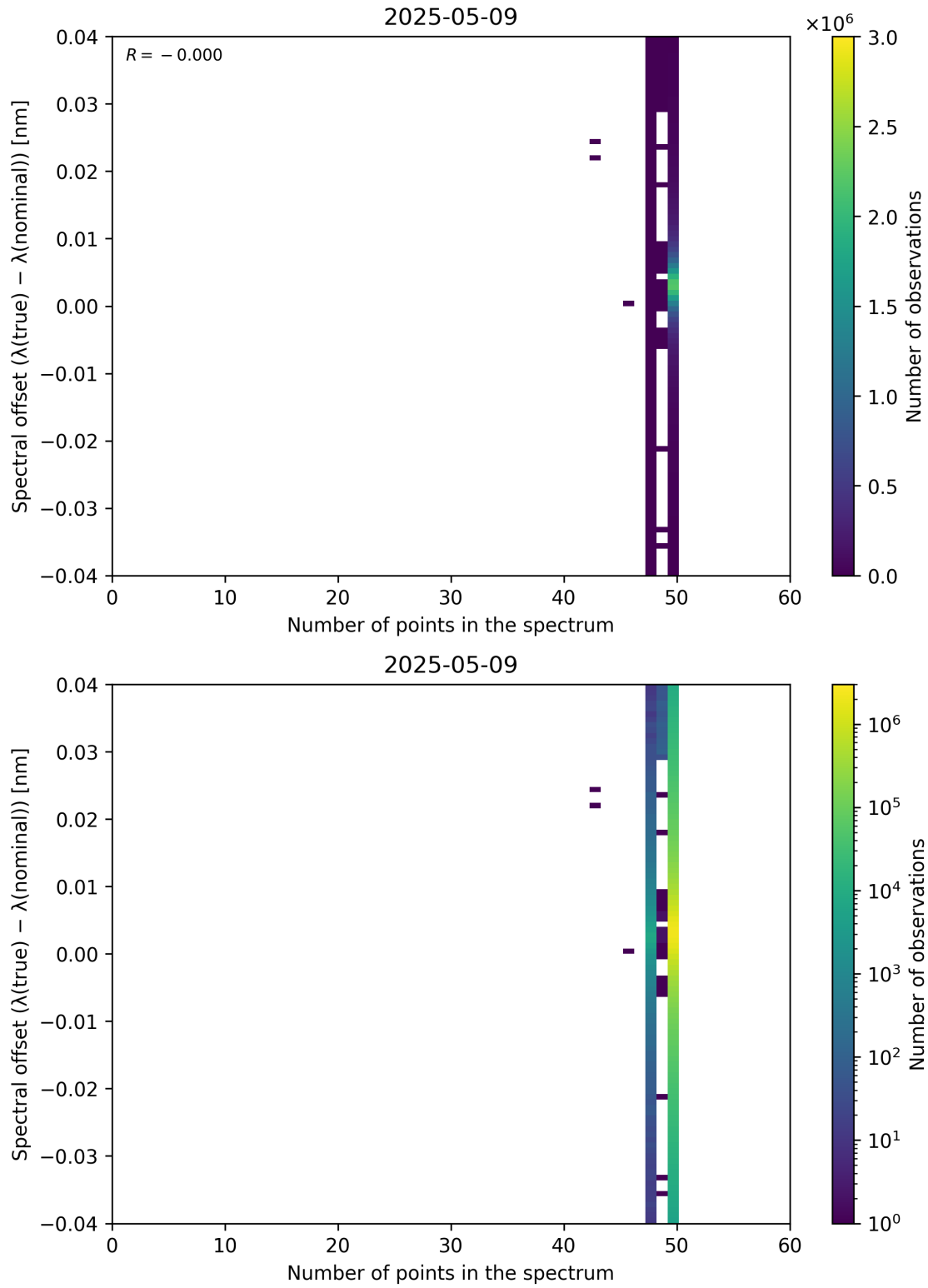
Figure 101: Scatter density plot of “Number of points in the spectrum” against “Spectral offset ( \lambda_{\text{true}} - \lambda_{\text{nominal}} )” for 2025-05-08 to 2025-05-10.
