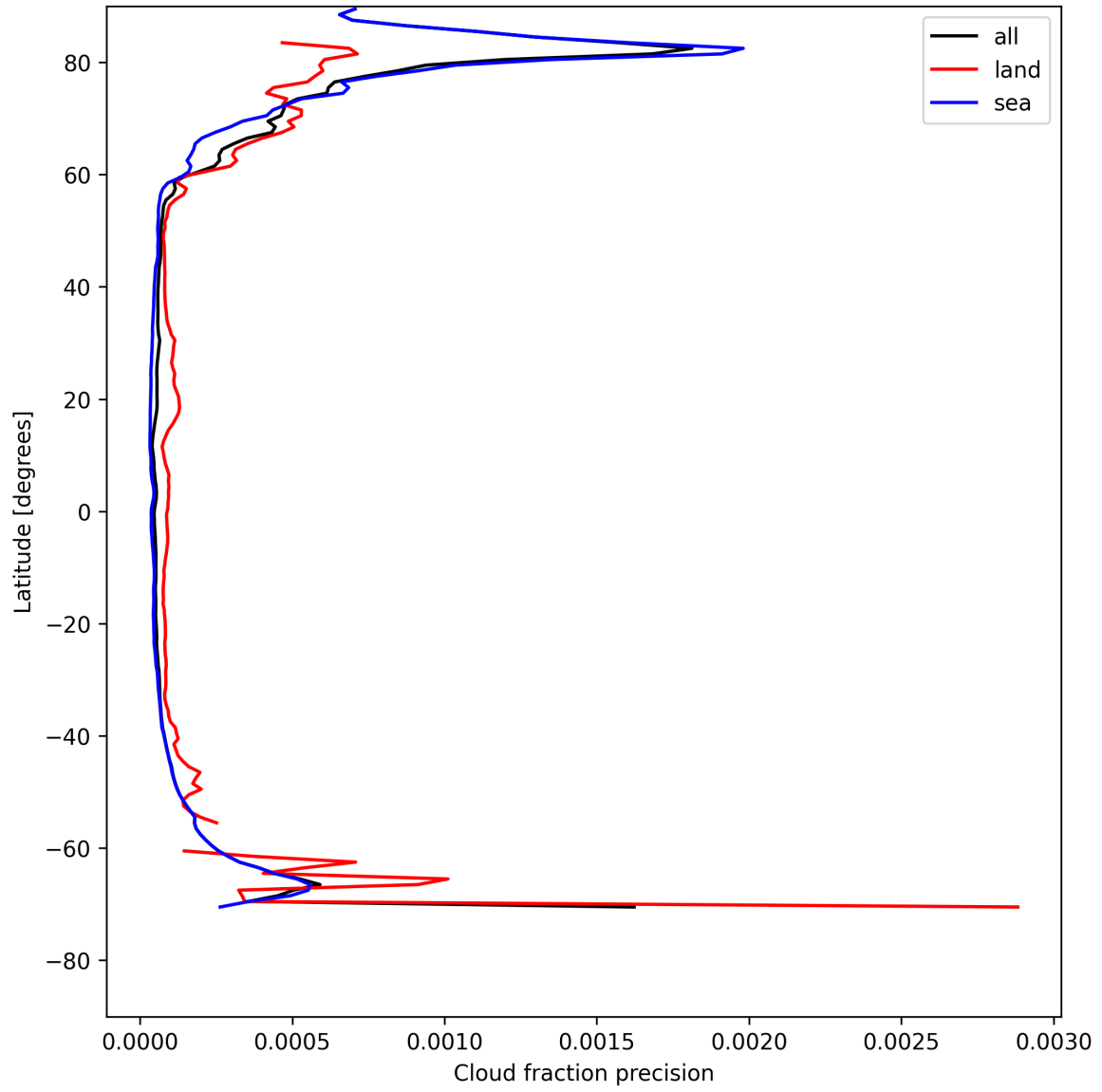
Figure 16: Zonal average of “Cloud fraction precision” for 2025-05-08 to 2025-05-10.
