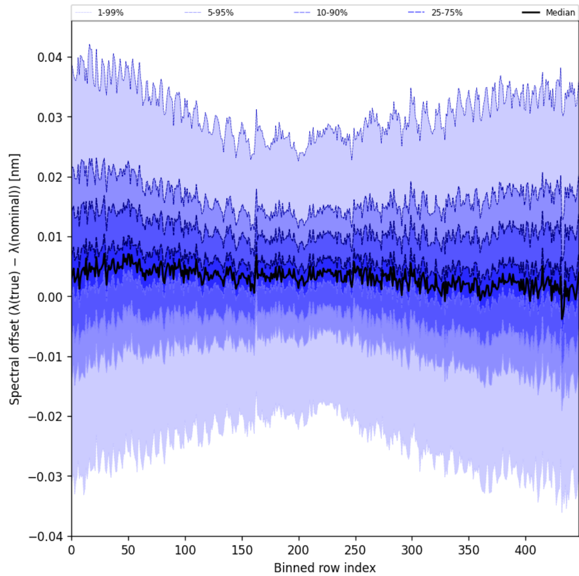
Figure 62: Along track statistics of “Spectral offset ( \lambda_{\text{true}} - \lambda_{\text{nominal}} )” for 2025-05-08 to 2025-05-10
