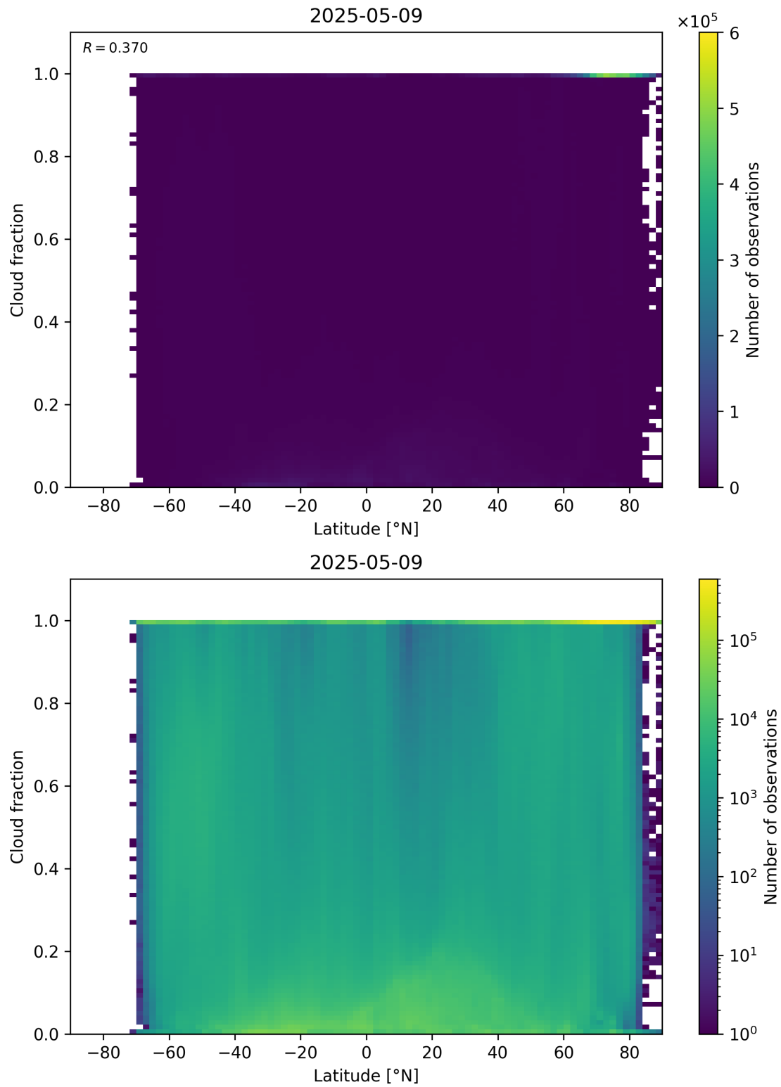
Figure 90: Scatter density plot of “Latitude” against “Cloud fraction” for 2025-05-08 to 2025-05-10.
