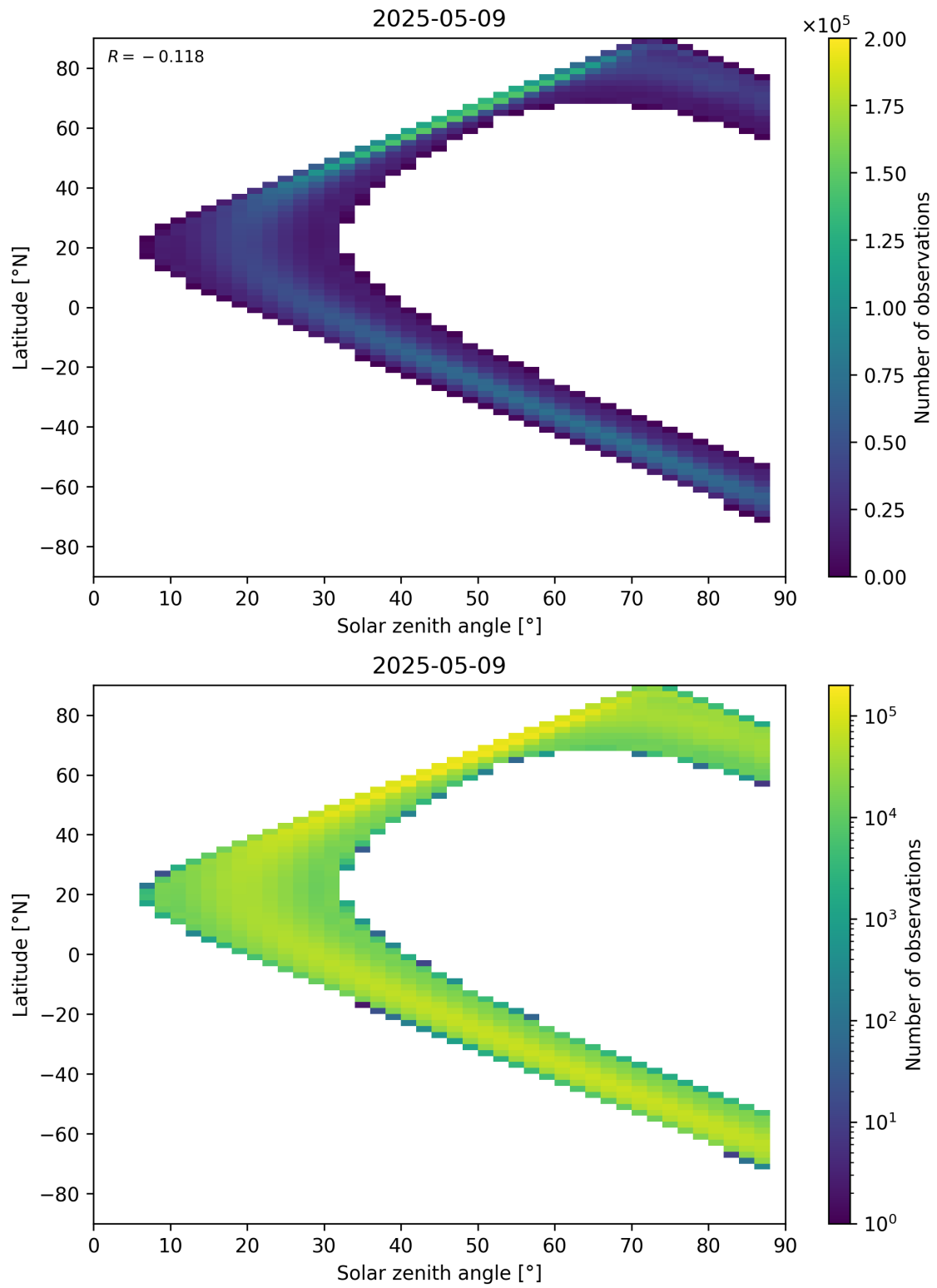
Figure 113: Scatter density plot of “Solar zenith angle” against “Latitude” for 2025-05-08 to 2025-05-10.
