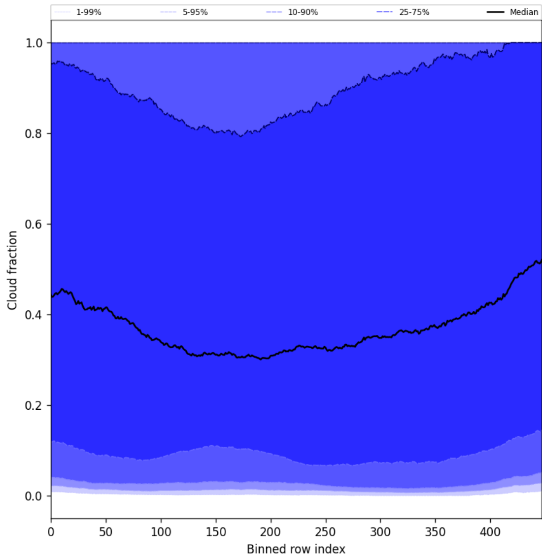
Figure 49: Along track statistics of “Cloud fraction” for 2025-05-08 to 2025-05-10
