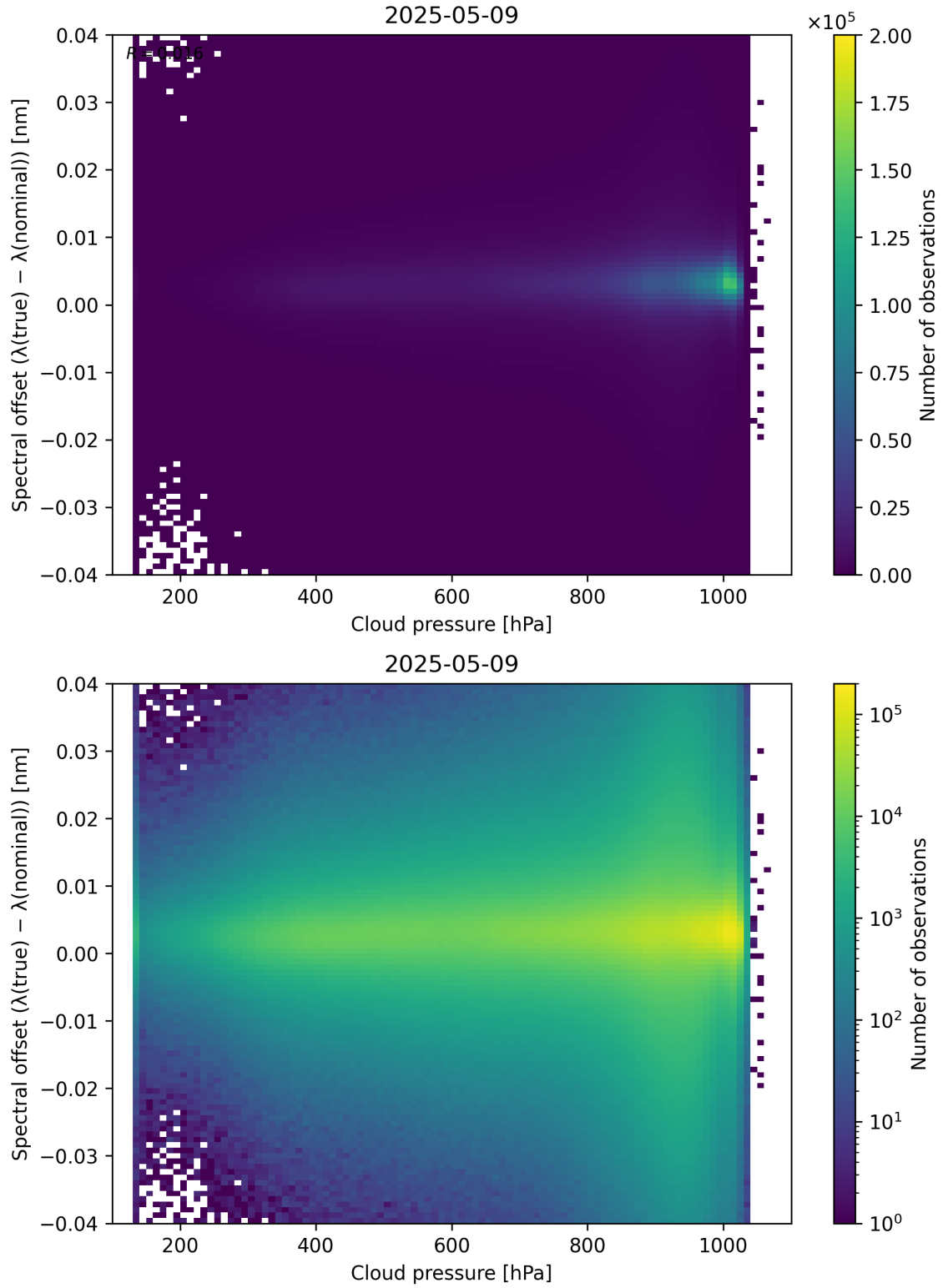
Figure 84: Scatter density plot of “Cloud pressure” against “Spectral offset ( \lambda_{\text{true}} - \lambda_{\text{nominal}} )” for 2025-05-08 to 2025-05-10.
