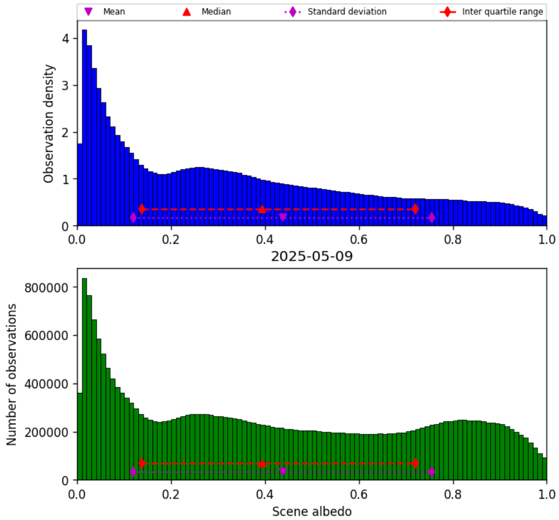
Figure 34: Histogram of “Scene albedo” for 2025-05-08 to 2025-05-10
