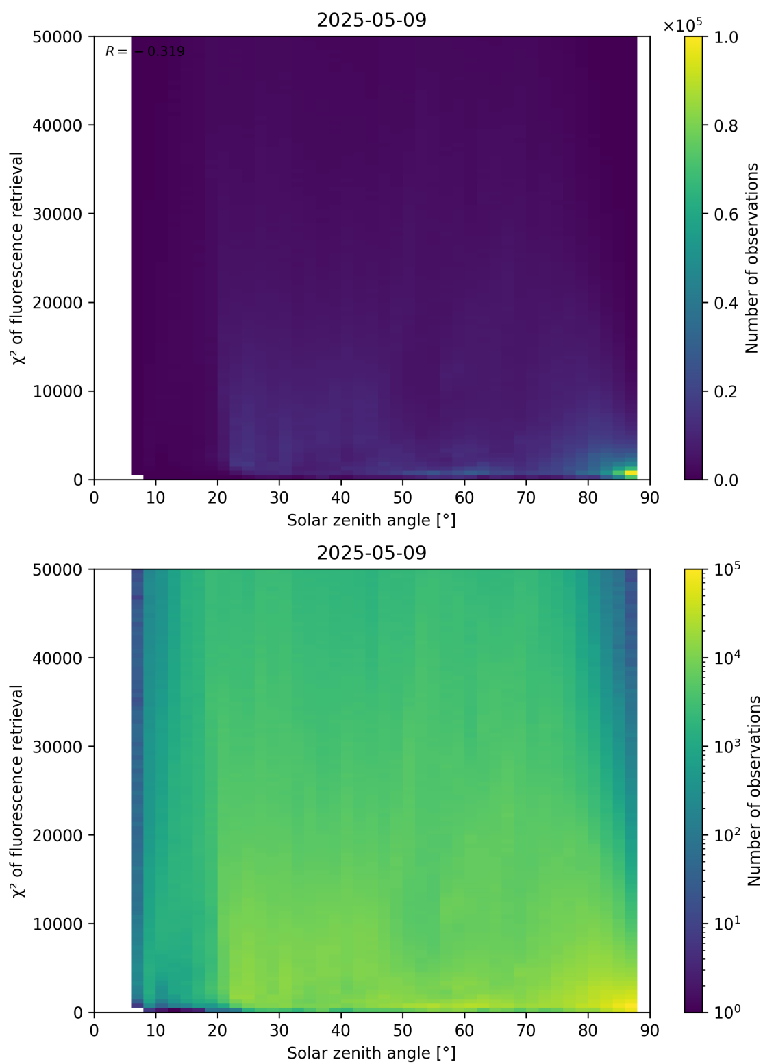
Figure 109: Scatter density plot of “Solar zenith angle” against “ \chi^2 of fluorescence retrieval” for 2025-05-08 to 2025-05-10.
