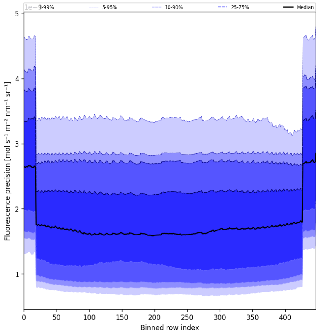
Figure 58: Along track statistics of “Fluorescence precision” for 2025-05-08 to 2025-05-10
