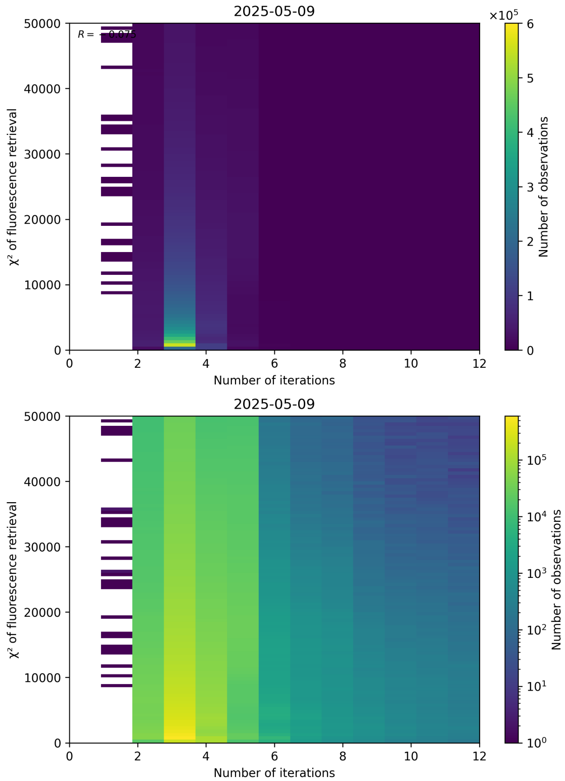
Figure 97: Scatter density plot of “Number of iterations” against “ \chi^2 of fluorescence retrieval” for 2025-05-08 to 2025-05-10.
