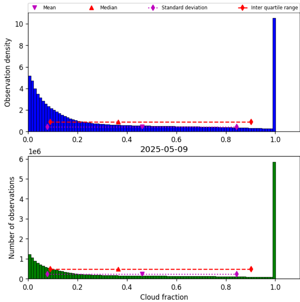
Figure 32: Histogram of “Cloud fraction” for 2025-05-08 to 2025-05-10
