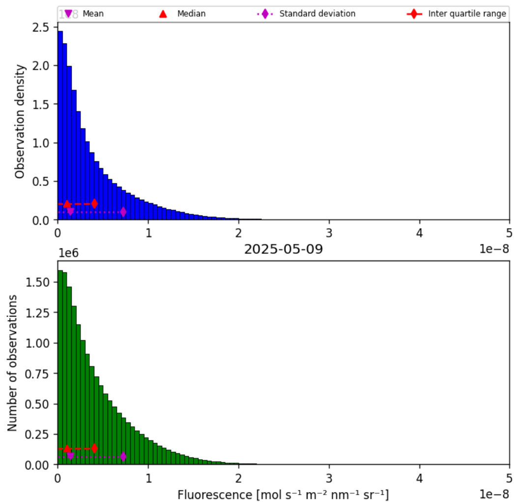
Figure 40: Histogram of “Fluorescence” for 2025-05-08 to 2025-05-10
