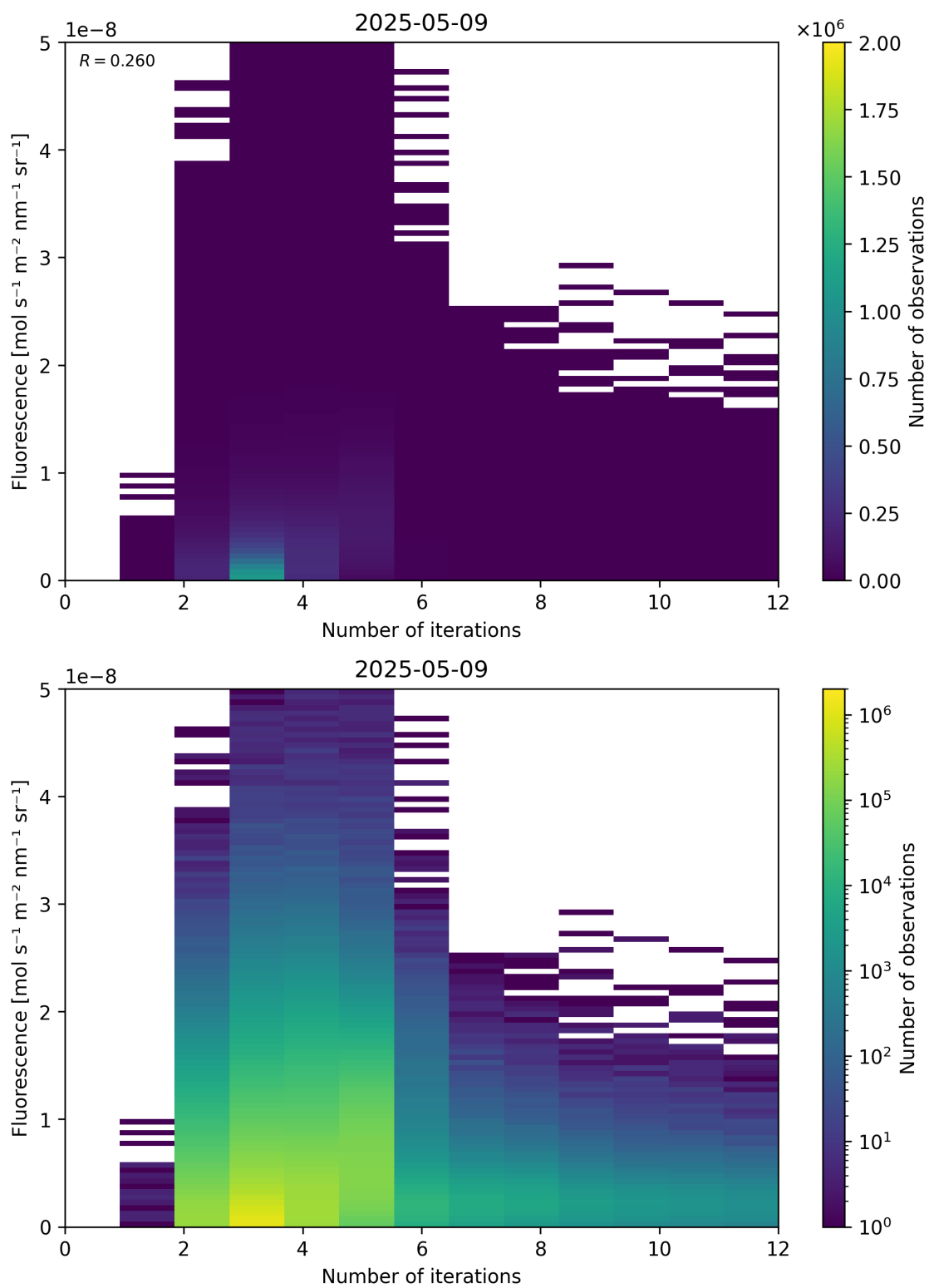
Figure 98: Scatter density plot of “Number of iterations” against “Fluorescence” for 2025-05-08 to 2025-05-10.
