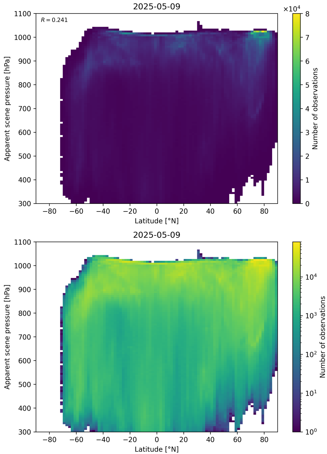
Figure 88: Scatter density plot of “Latitude” against “Apparent scene pressure” for 2025-05-08 to 2025-05-10.
