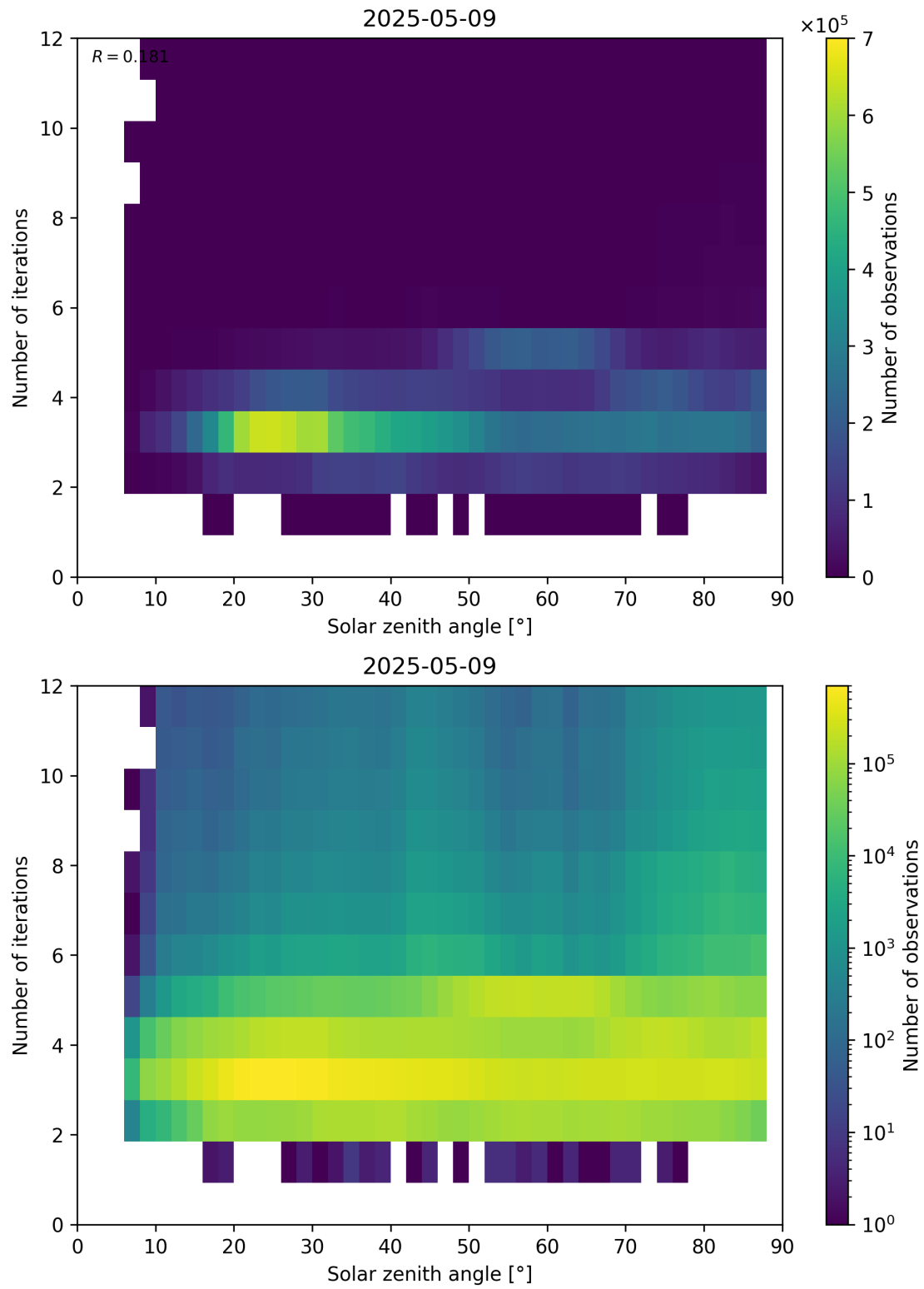
Figure 114: Scatter density plot of “Solar zenith angle” against “Number of iterations” for 2025-05-08 to 2025-05-10.
