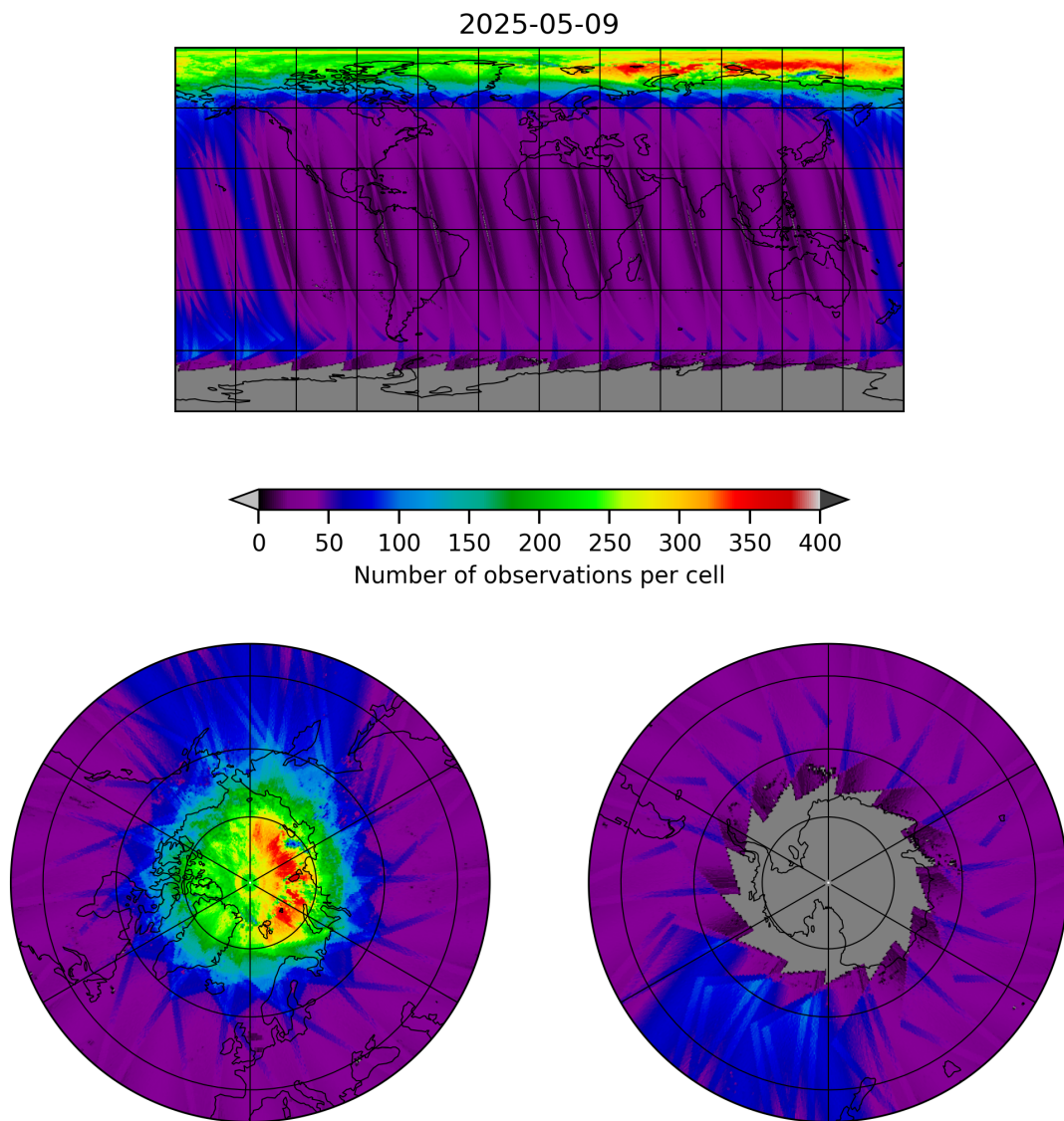
Figure 11: Map of the number of observations for 2025-05-08 to 2025-05-10
