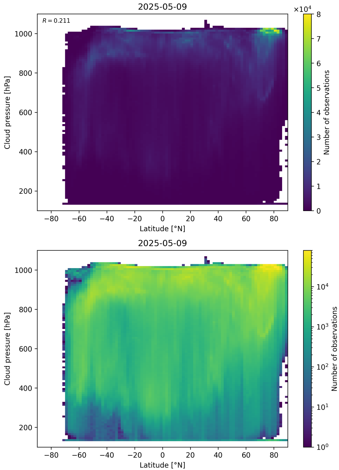
Figure 91: Scatter density plot of “Latitude” against “Cloud pressure” for 2025-05-08 to 2025-05-10.
