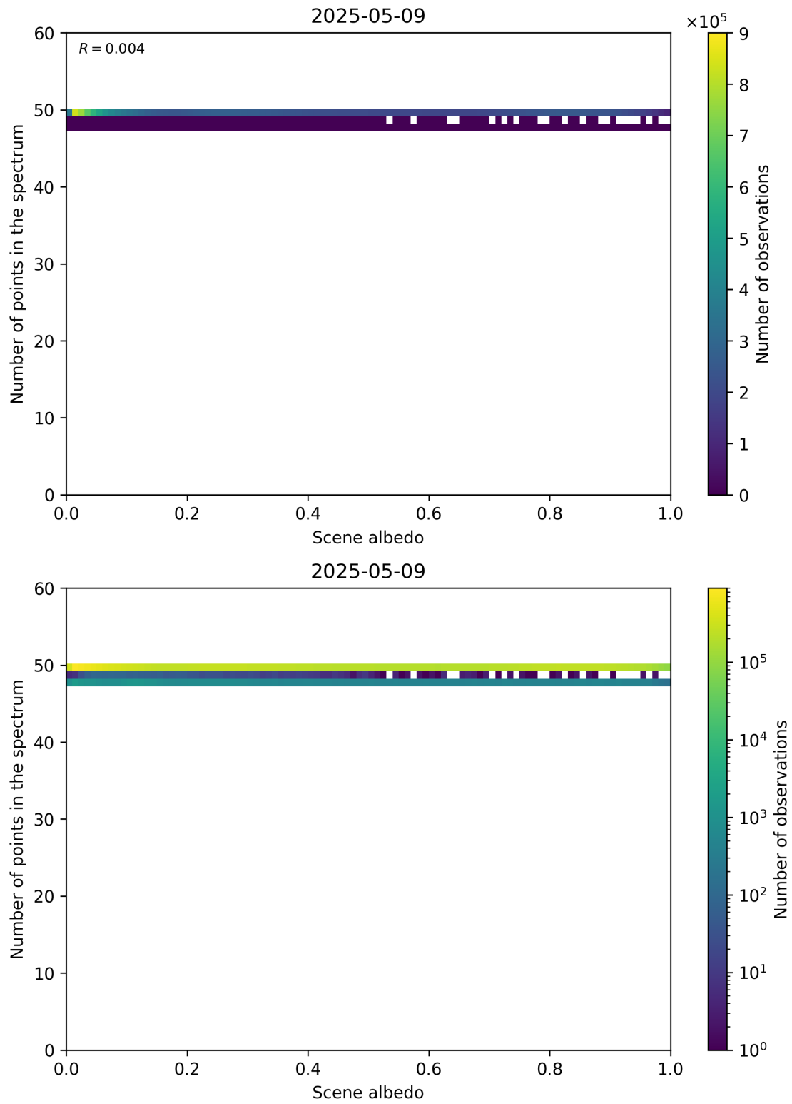
Figure 106: Scatter density plot of “Scene albedo” against “Number of points in the spectrum” for 2025-05-08 to 2025-05-10.
