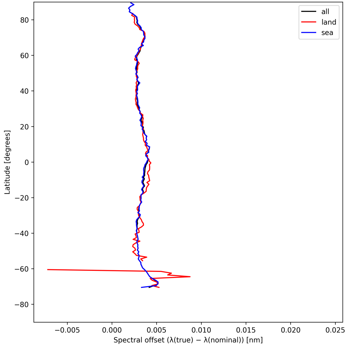
Figure 28: Zonal average of “Spectral offset ( \lambda_{\text{true}} - \lambda_{\text{nominal}} )” for 2025-05-08 to 2025-05-10.
