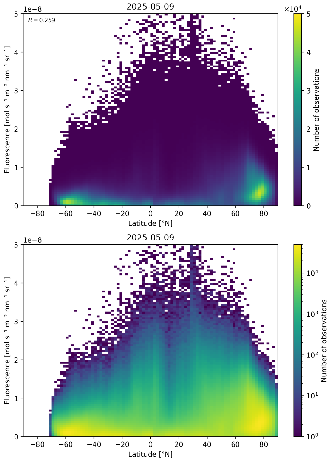
Figure 92: Scatter density plot of “Latitude” against “Fluorescence” for 2025-05-08 to 2025-05-10.
