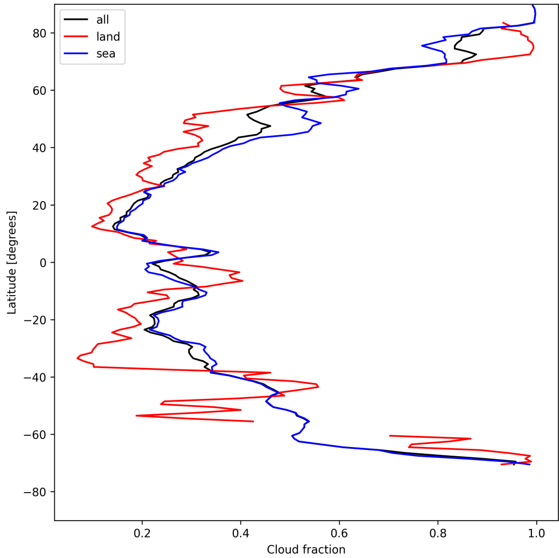
Figure 15: Zonal average of “Cloud fraction” for 2025-05-08 to 2025-05-10.
