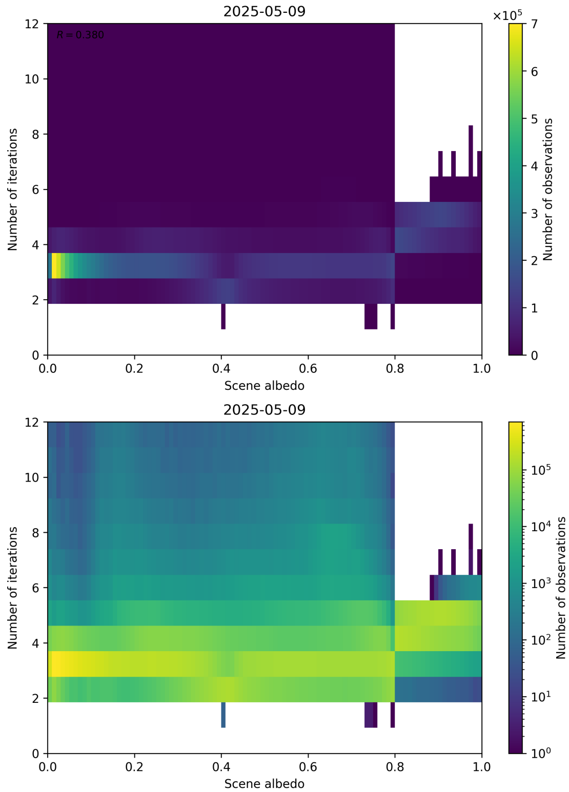
Figure 105: Scatter density plot of “Scene albedo” against “Number of iterations” for 2025-05-08 to 2025-05-10.
