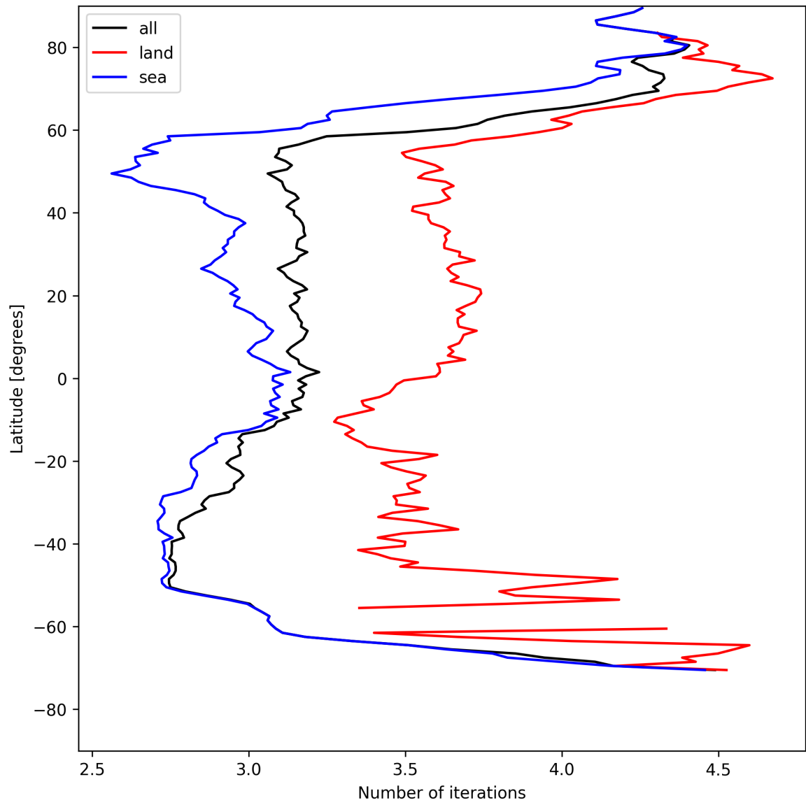
Figure 22: Zonal average of “Number of iterations” for 2025-05-08 to 2025-05-10.
