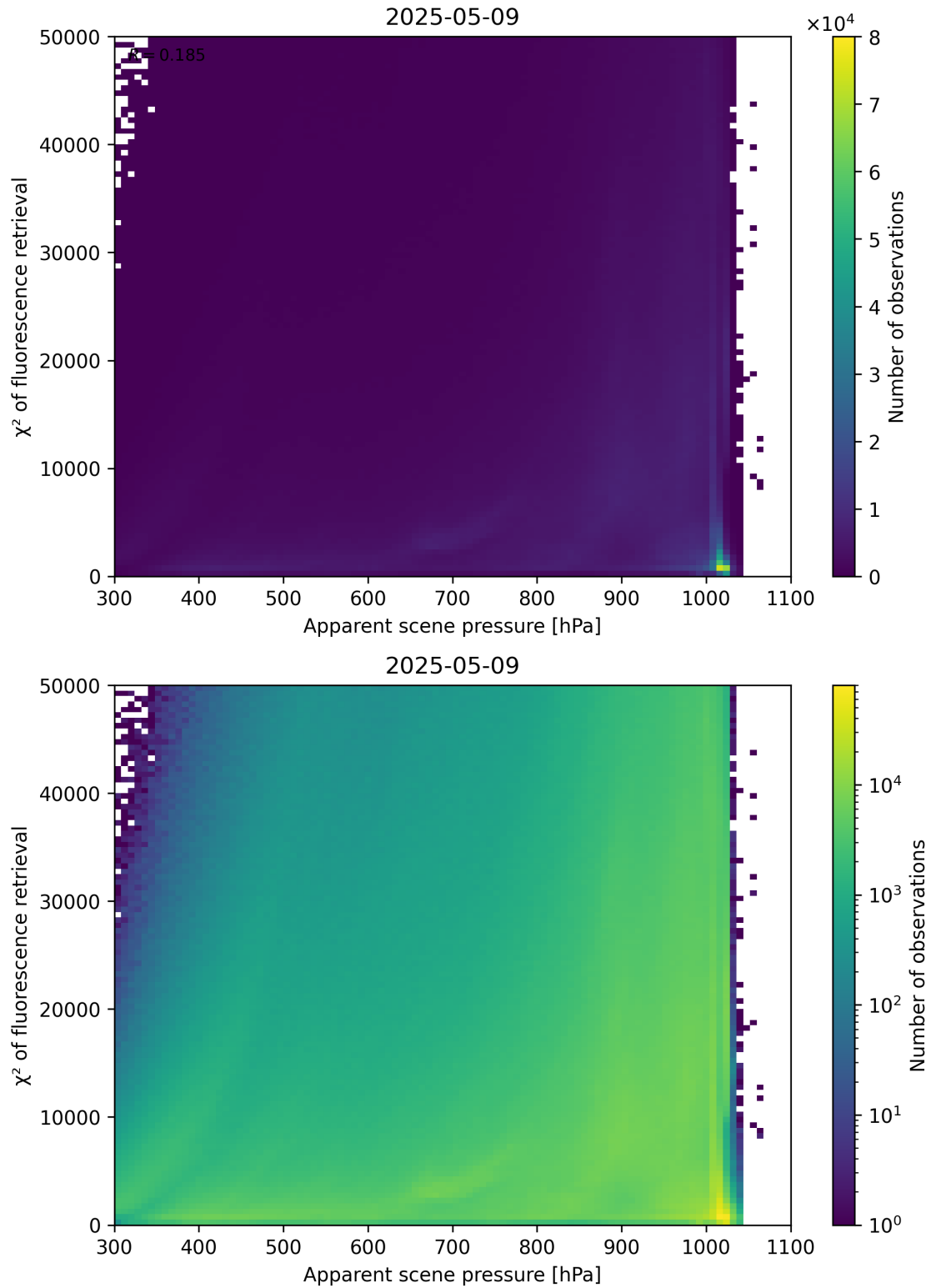
Figure 63: Scatter density plot of “Apparent scene pressure” against “ \chi^2 of fluorescence retrieval” for 2025-05-08 to 2025-05-10.
