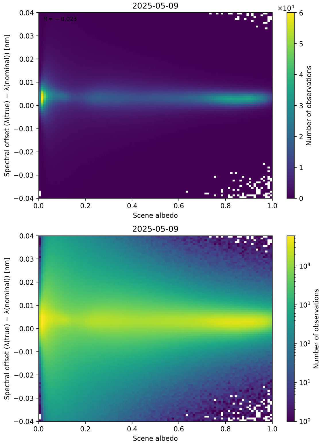
Figure 107: Scatter density plot of “Scene albedo” against “Spectral offset ( \lambda_{\text{true}} - \lambda_{\text{nominal}} )” for 2025-05-08 to 2025-05-10.
