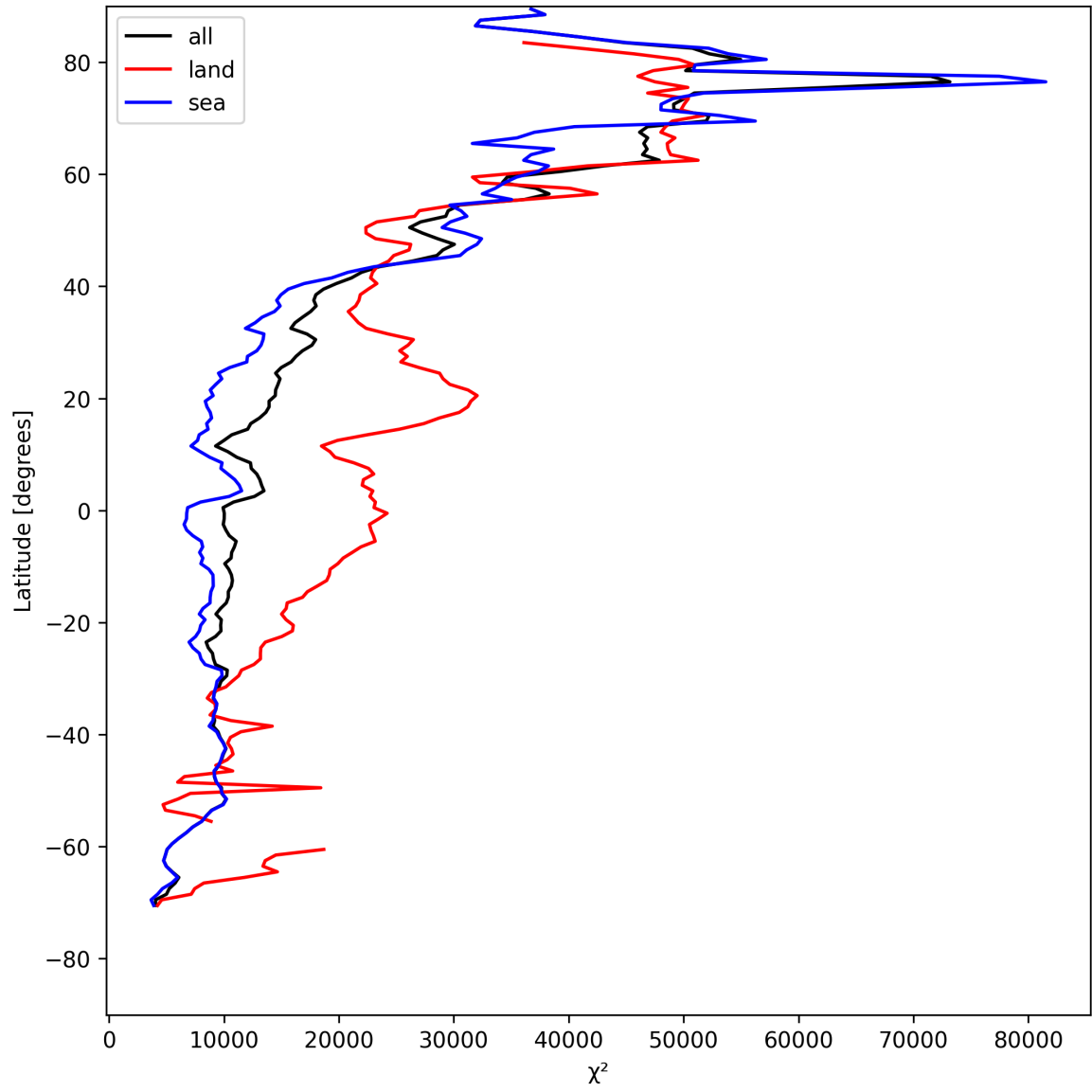
Figure 21: Zonal average of “ \chi^2 ” for 2025-05-08 to 2025-05-10.
