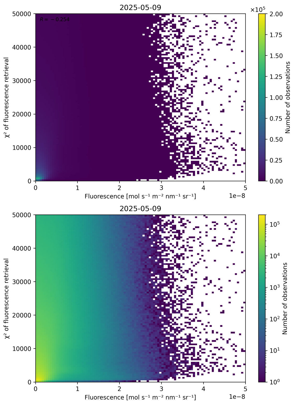
Figure 85: Scatter density plot of “Fluorescence” against “ \chi^2 of fluorescence retrieval” for 2025-05-08 to 2025-05-10.
