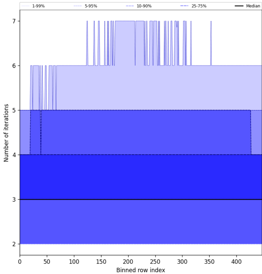
Figure 56: Along track statistics of “Number of iterations” for 2025-05-08 to 2025-05-10
