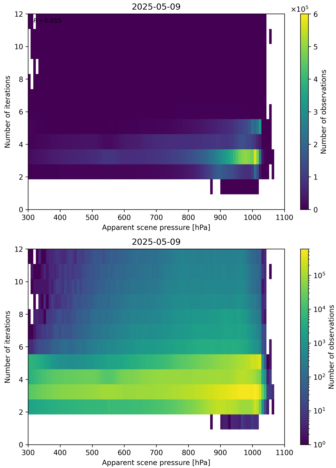
Figure 65: Scatter density plot of “Apparent scene pressure” against “Number of iterations” for 2025-05-08 to 2025-05-10.
