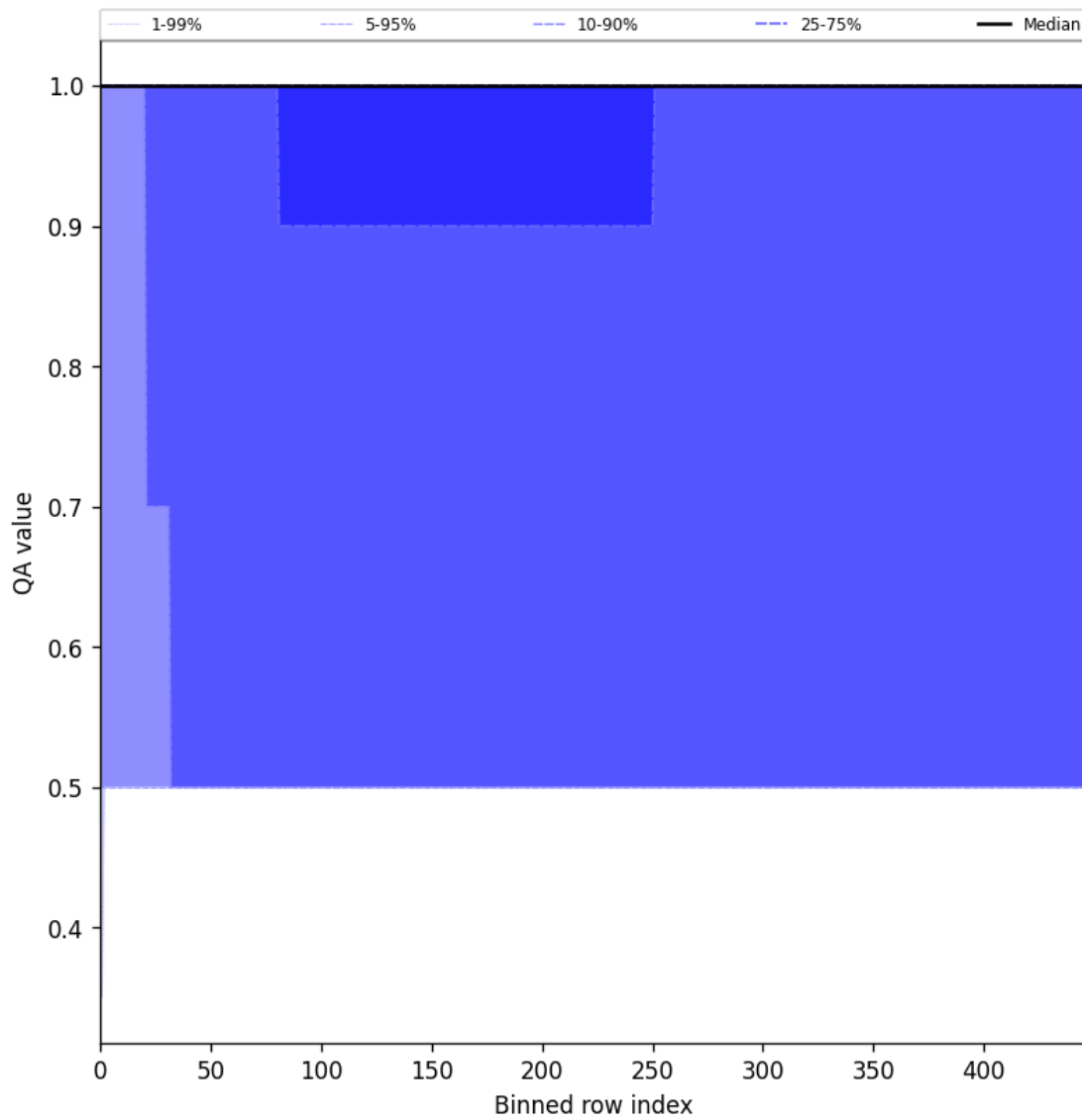
Figure 46: Along track statistics of “QA value” for 2025-05-08 to 2025-05-10
