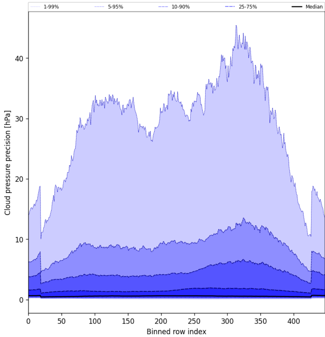
Figure 48: Along track statistics of “Cloud pressure precision” for 2025-05-08 to 2025-05-10
