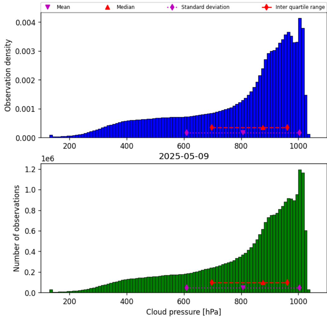
Figure 30: Histogram of “Cloud pressure” for 2025-05-08 to 2025-05-10
