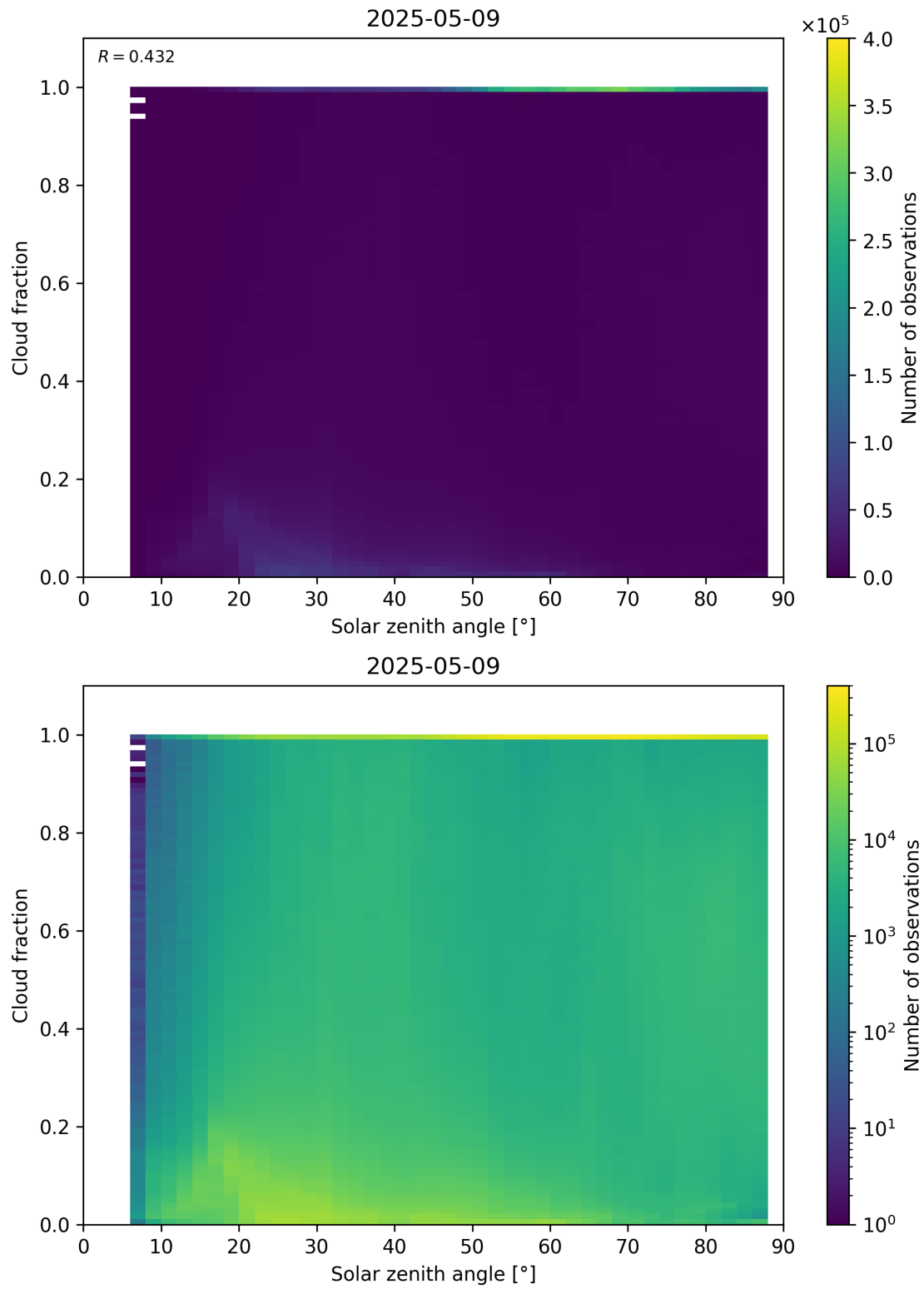
Figure 110: Scatter density plot of “Solar zenith angle” against “Cloud fraction” for 2025-05-08 to 2025-05-10.
