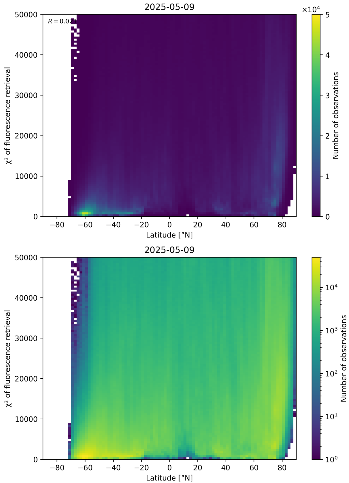
Figure 89: Scatter density plot of “Latitude” against “ \chi^2 of fluorescence retrieval” for 2025-05-08 to 2025-05-10.
