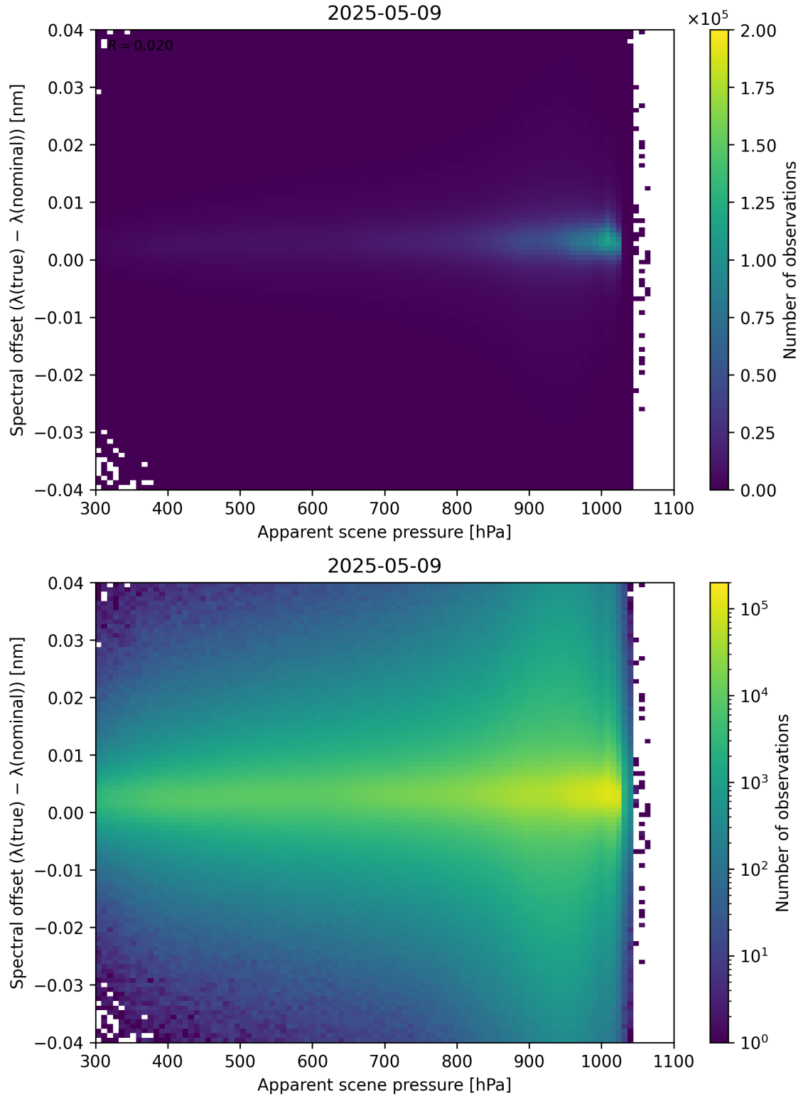
Figure 67: Scatter density plot of “Apparent scene pressure” against “Spectral offset ( \lambda_{\text{true}} - \lambda_{\text{nominal}} )” for 2025-05-08 to 2025-05-10.
