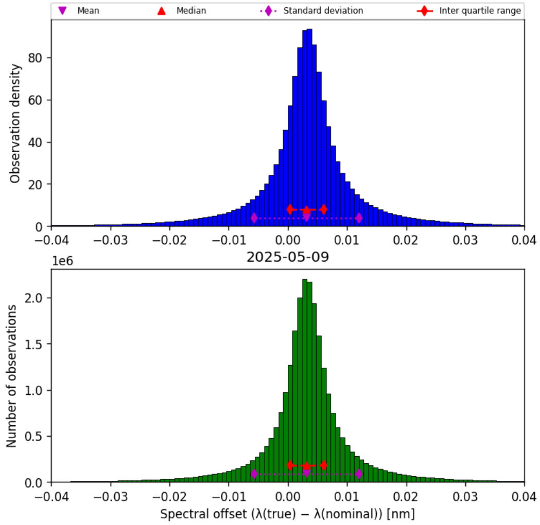
Figure 45: Histogram of “Spectral offset ( \lambda_{\text{true}} - \lambda_{\text{nominal}} )” for 2025-05-08 to 2025-05-10
