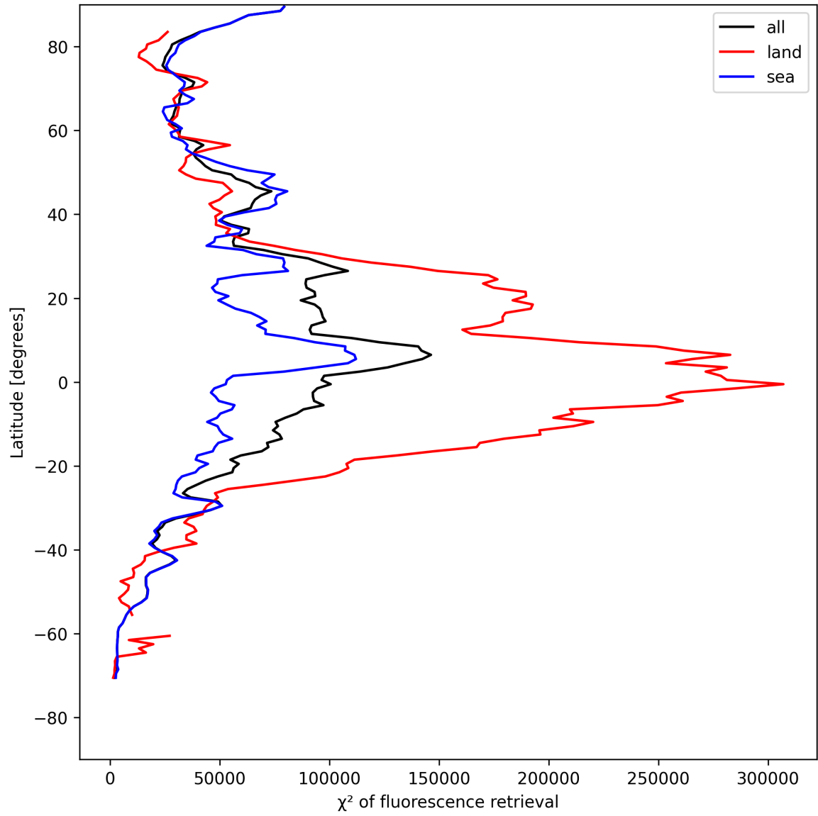
Figure 25: Zonal average of “ \chi^2 of fluorescence retrieval” for 2025-05-08 to 2025-05-10.
