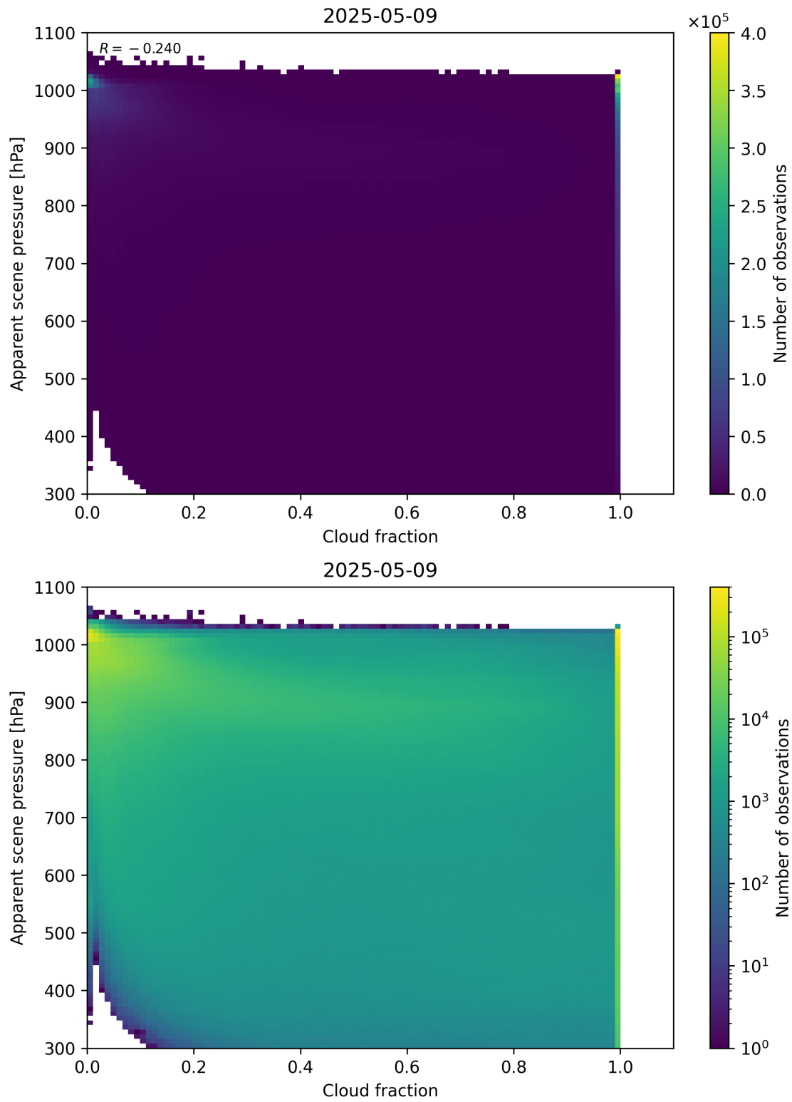
Figure 70: Scatter density plot of “Cloud fraction” against “Apparent scene pressure” for 2025-05-08 to 2025-05-10.
