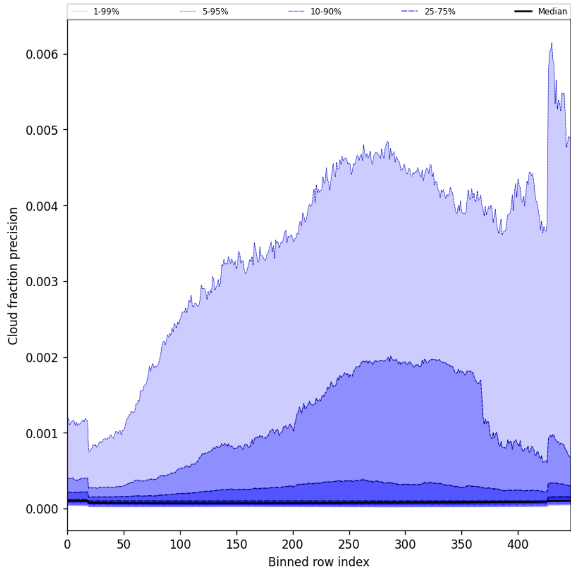
Figure 50: Along track statistics of “Cloud fraction precision” for 2025-05-08 to 2025-05-10
