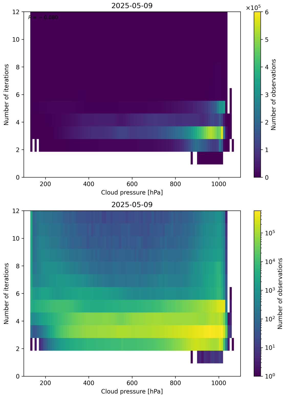
Figure 81: Scatter density plot of “Cloud pressure” against “Number of iterations” for 2025-05-08 to 2025-05-10.
