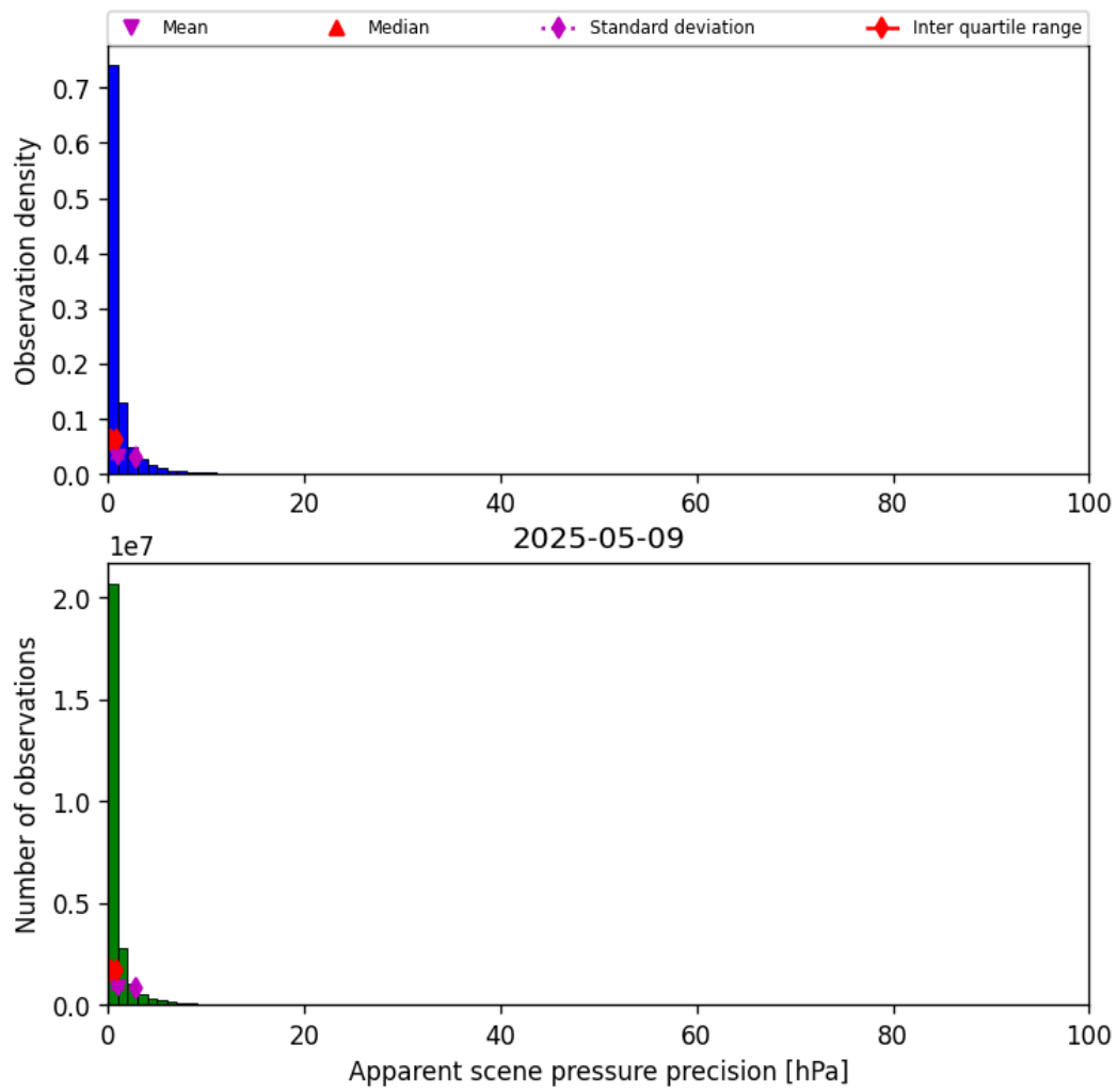
Figure 37: Histogram of “Apparent scene pressure precision” for 2025-05-08 to 2025-05-10
