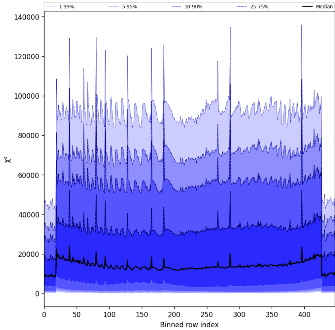
Figure 55: Along track statistics of “ \chi^2 ” for 2025-05-08 to 2025-05-10
