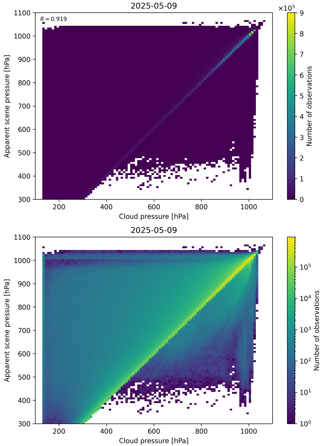
Figure 77: Scatter density plot of “Cloud pressure” against “Apparent scene pressure” for 2025-05-08 to 2025-05-10.
