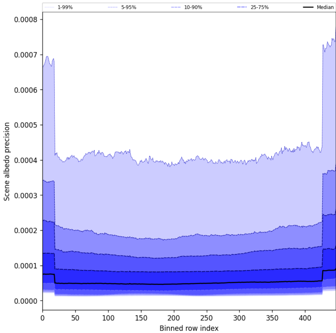
Figure 52: Along track statistics of “Scene albedo precision” for 2025-05-08 to 2025-05-10
