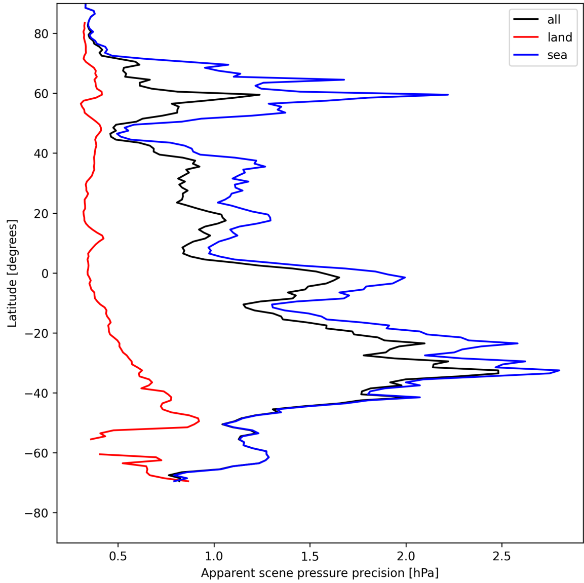
Figure 20: Zonal average of “Apparent scene pressure precision” for 2025-05-10 to 2025-05-11.
