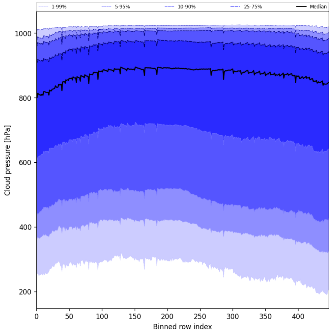
Figure 47: Along track statistics of “Cloud pressure” for 2025-05-10 to 2025-05-11
