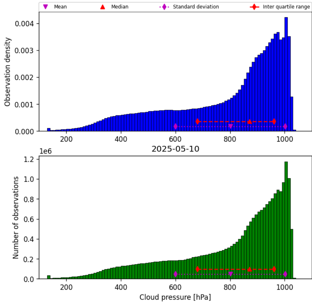
Figure 30: Histogram of “Cloud pressure” for 2025-05-10 to 2025-05-11
