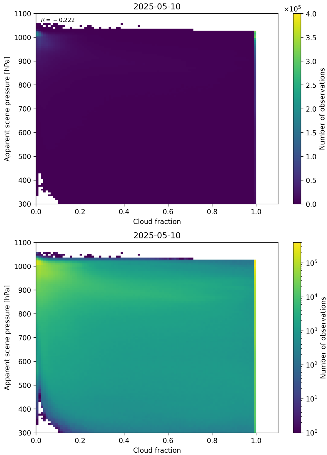
Figure 70: Scatter density plot of “Cloud fraction” against “Apparent scene pressure” for 2025-05-10 to 2025-05-11.
