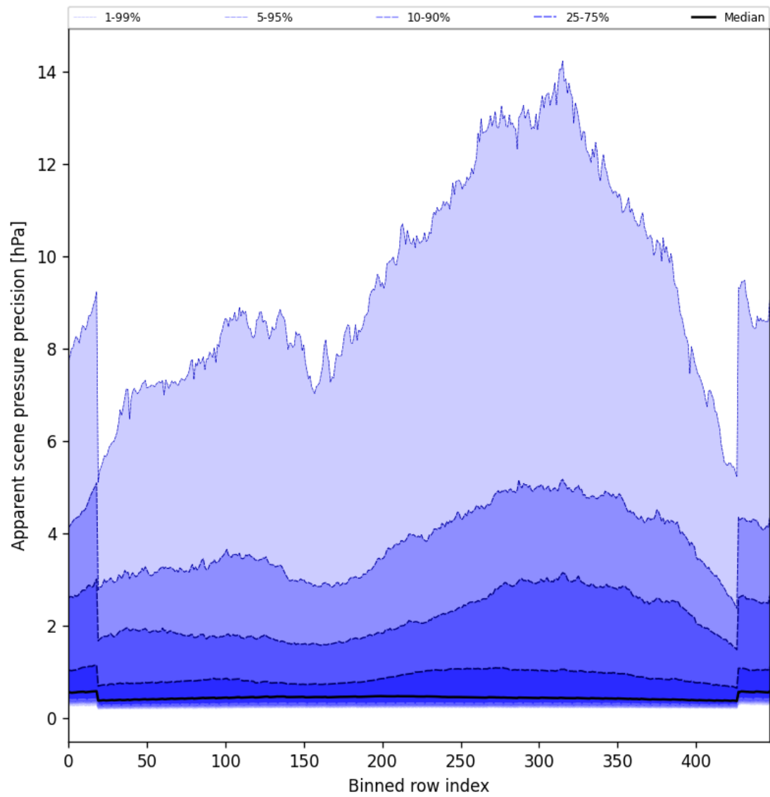
Figure 54: Along track statistics of “Apparent scene pressure precision” for 2025-05-10 to 2025-05-11
