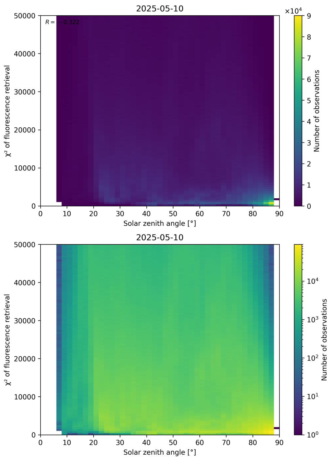
Figure 109: Scatter density plot of “Solar zenith angle” against “ \chi^2 of fluorescence retrieval” for 2025-05-10 to 2025-05-11.
