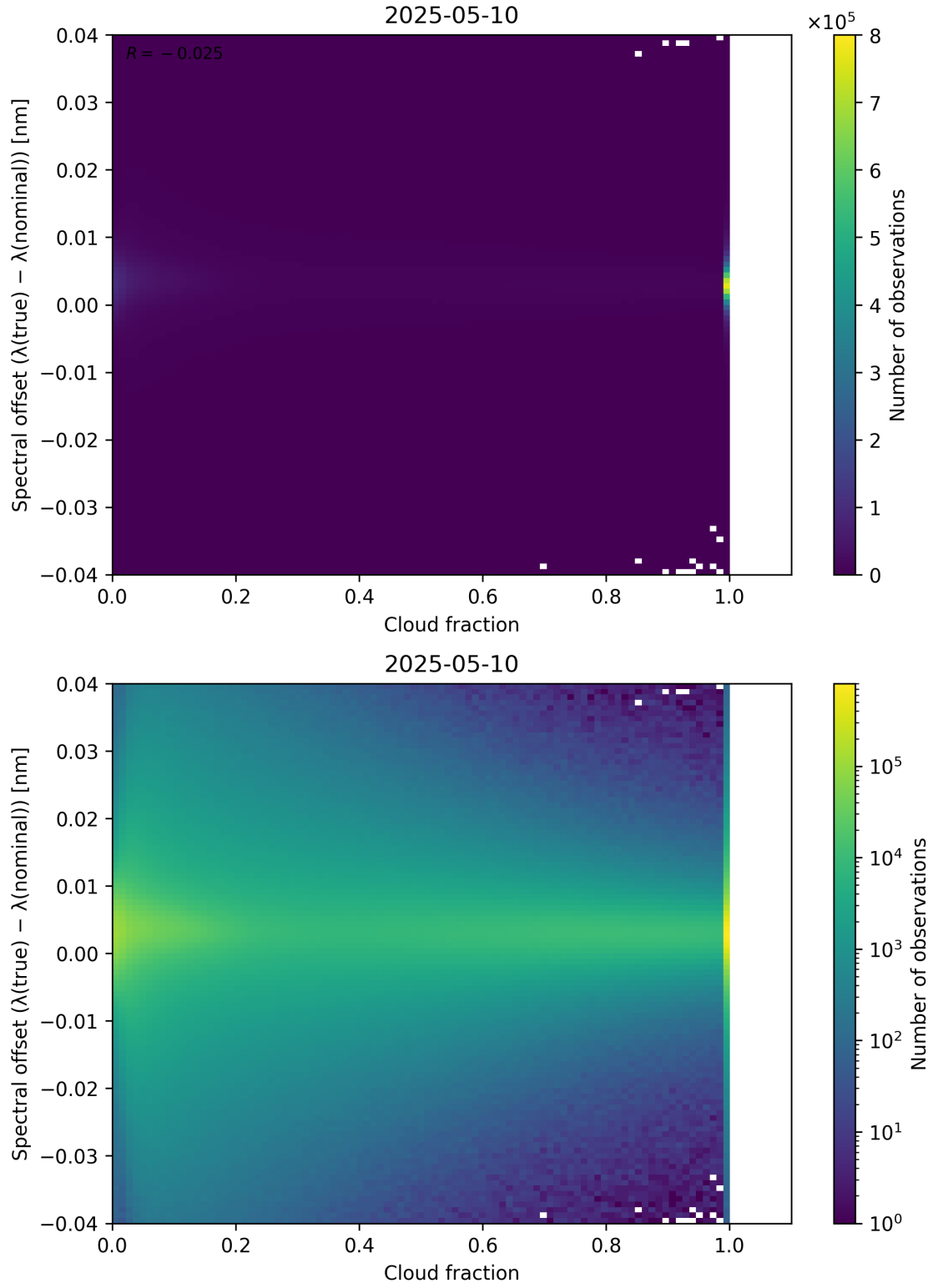
Figure 76: Scatter density plot of “Cloud fraction” against “Spectral offset ( \lambda_{\text{true}} - \lambda_{\text{nominal}} )” for 2025-05-10 to 2025-05-11.
