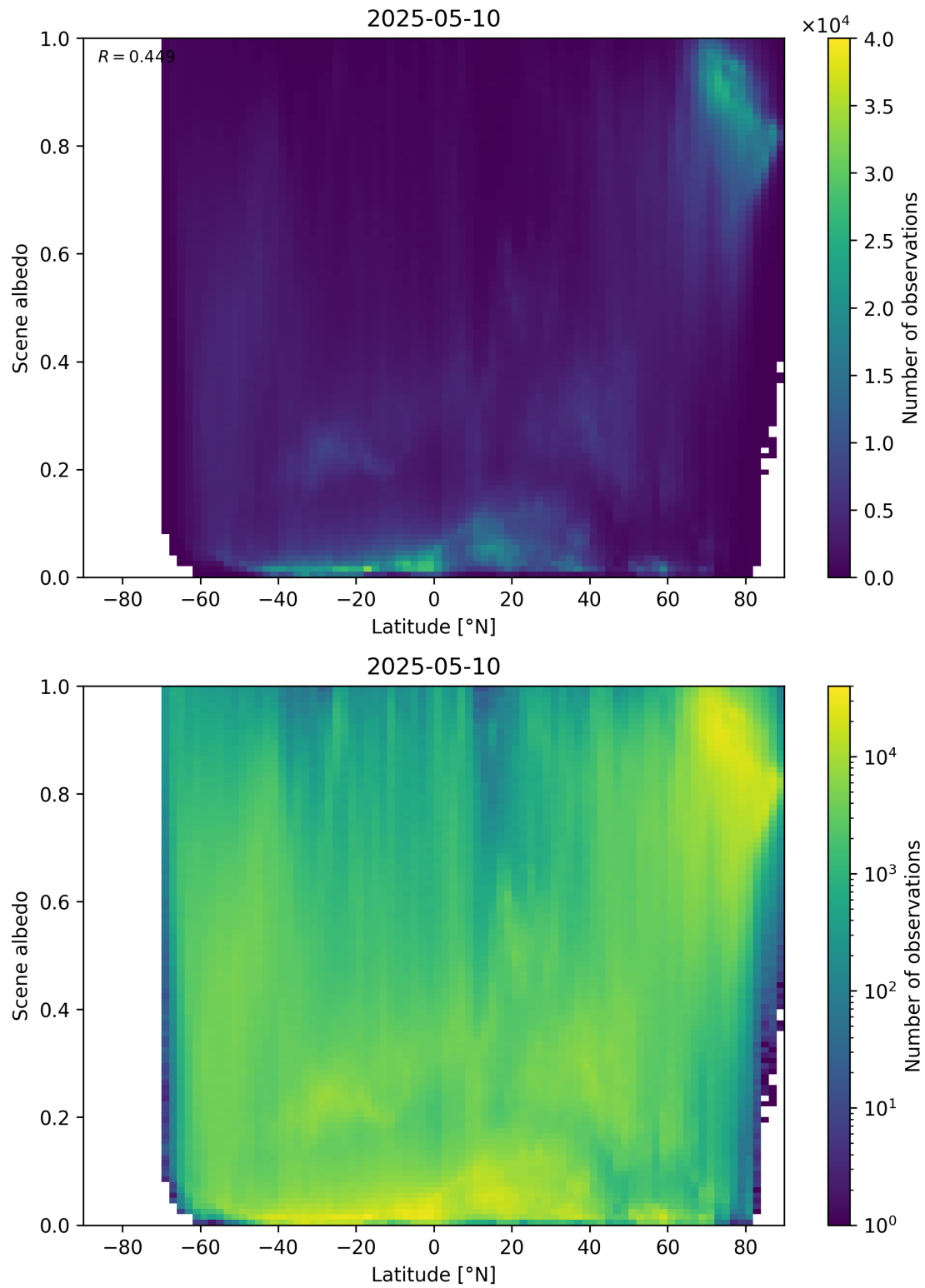
Figure 95: Scatter density plot of “Latitude” against “Scene albedo” for 2025-05-10 to 2025-05-11.
