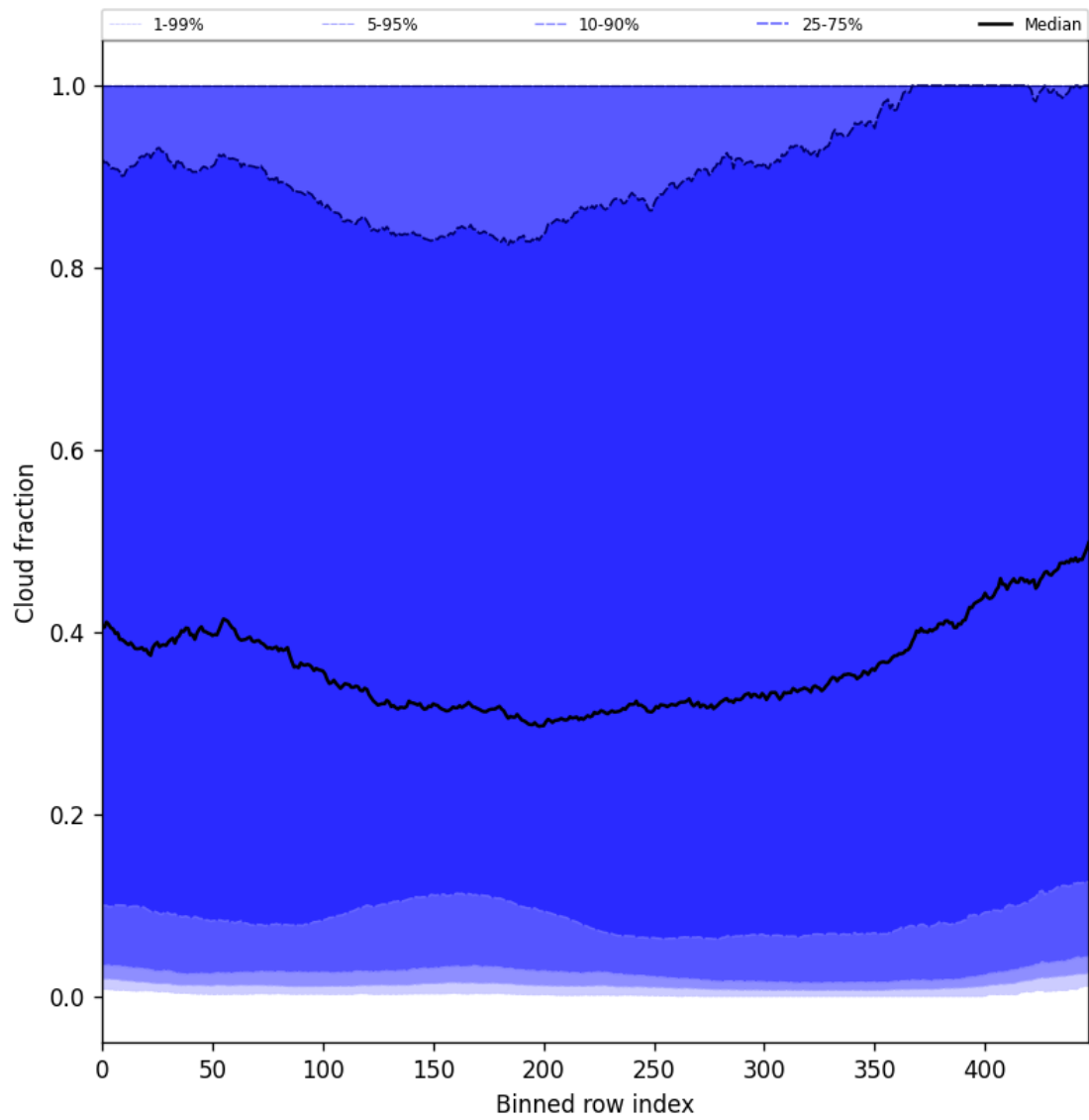
Figure 49: Along track statistics of “Cloud fraction” for 2025-05-10 to 2025-05-11
