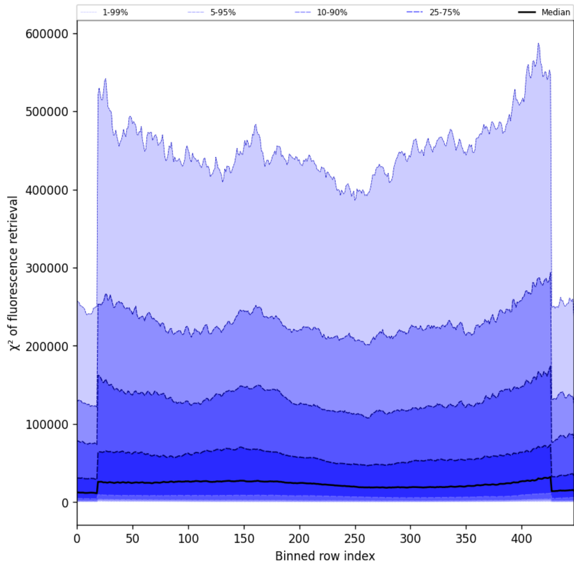
Figure 59: Along track statistics of “ \chi^2 of fluorescence retrieval” for 2025-05-10 to 2025-05-11
