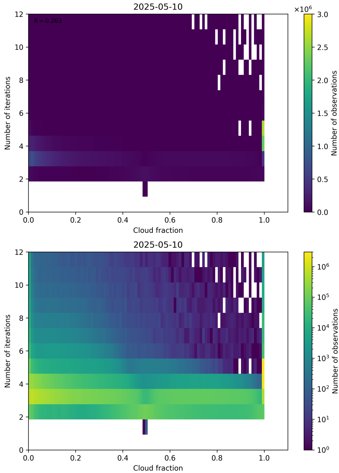
Figure 73: Scatter density plot of “Cloud fraction” against “Number of iterations” for 2025-05-10 to 2025-05-11.
