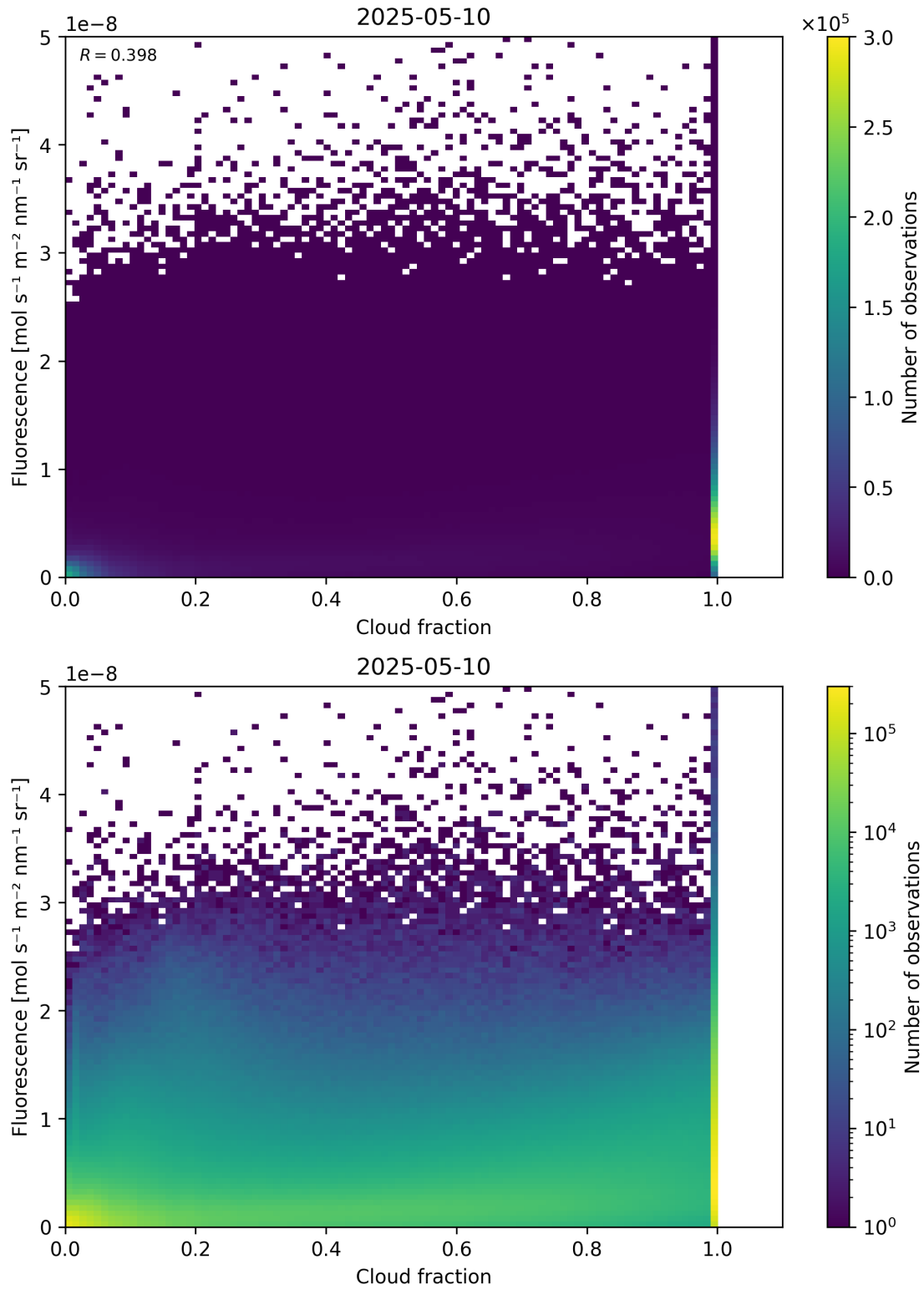
Figure 72: Scatter density plot of “Cloud fraction” against “Fluorescence” for 2025-05-10 to 2025-05-11.
