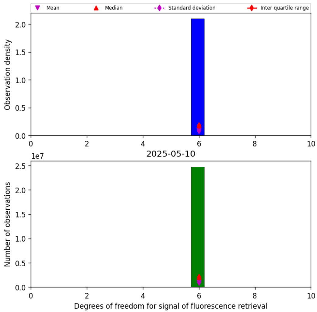
Figure 43: Histogram of “Degrees of freedom for signal of fluorescence retrieval” for 2025-05-10 to 2025-05-11
