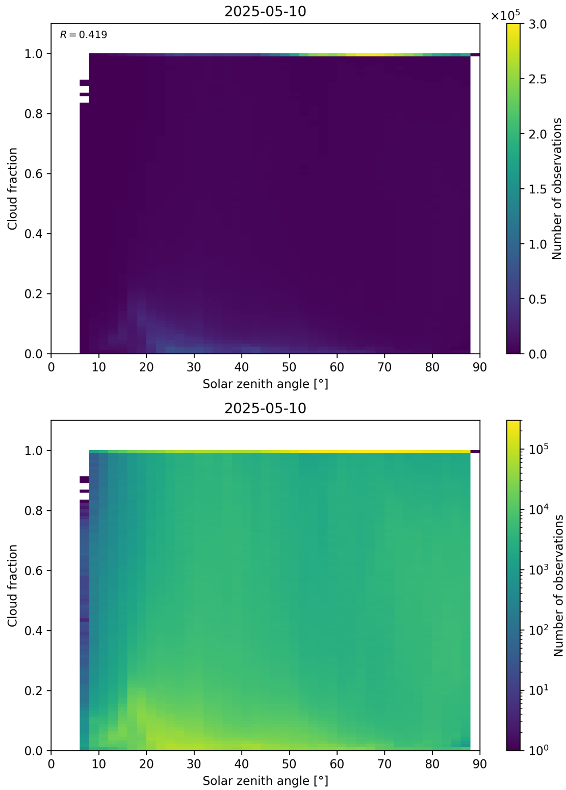
Figure 110: Scatter density plot of “Solar zenith angle” against “Cloud fraction” for 2025-05-10 to 2025-05-11.
