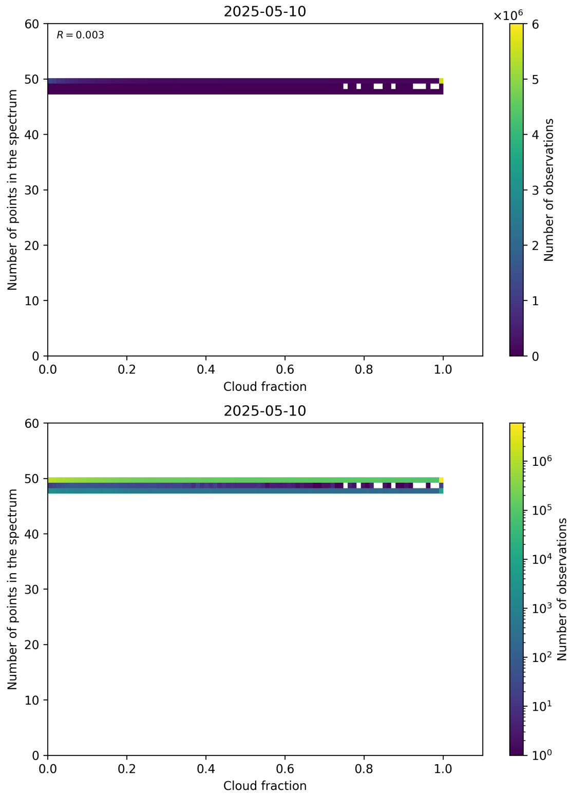
Figure 74: Scatter density plot of “Cloud fraction” against “Number of points in the spectrum” for 2025-05-10 to 2025-05-11.
