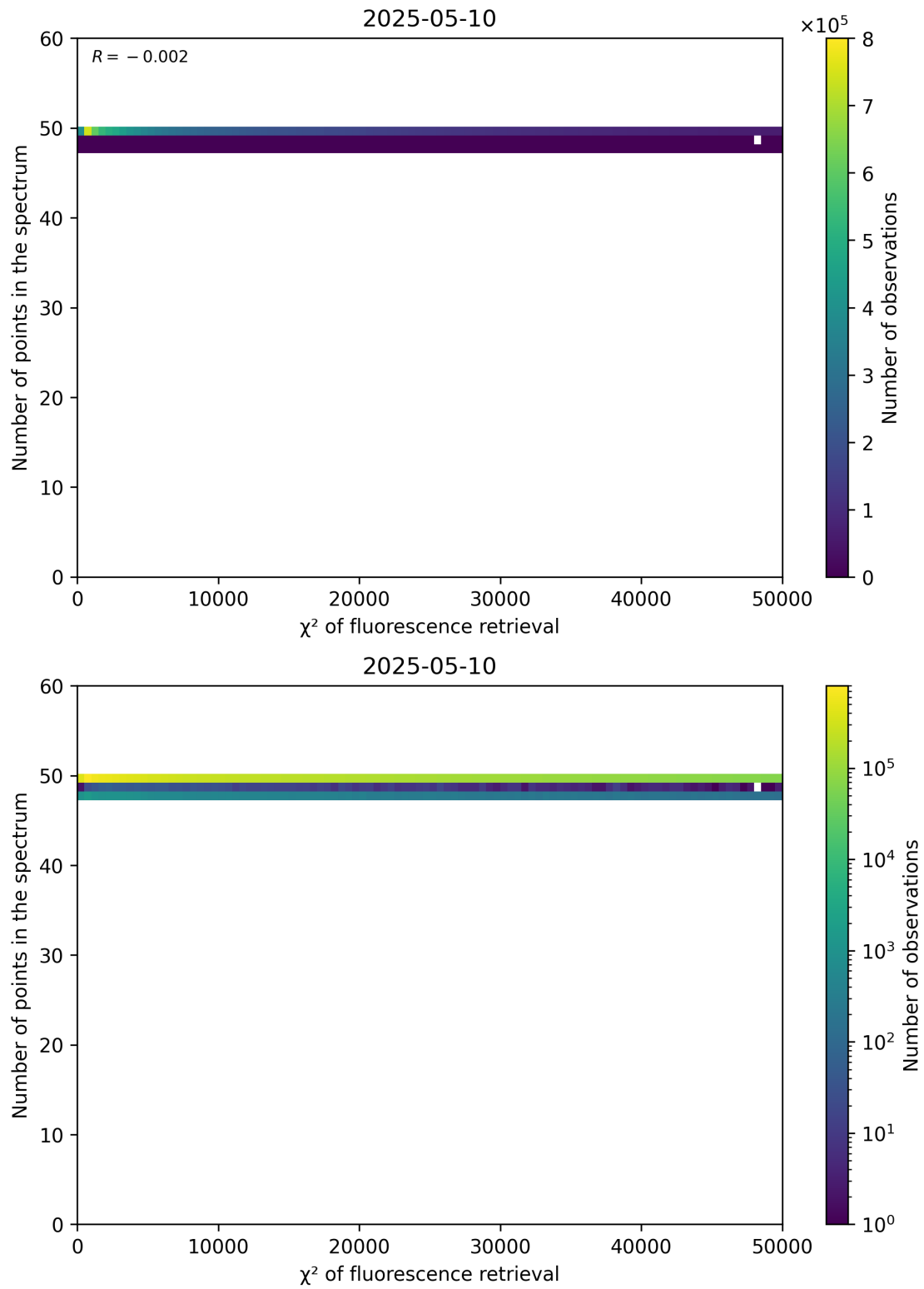
Figure 68: Scatter density plot of “ \chi^2 of fluorescence retrieval” against “Number of points in the spectrum” for 2025-05-10 to 2025-05-11.
