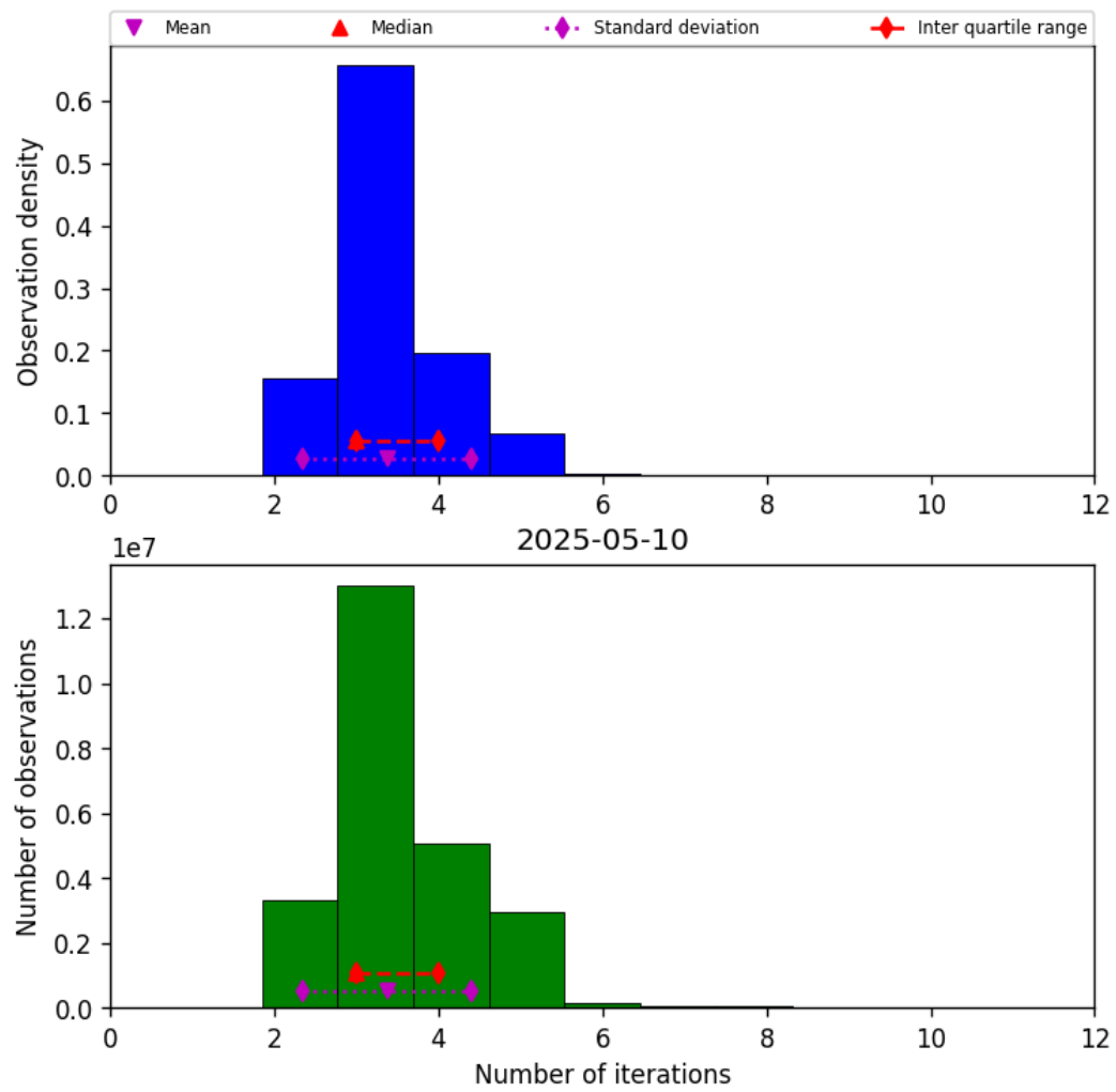
Figure 39: Histogram of “Number of iterations” for 2025-05-10 to 2025-05-11
