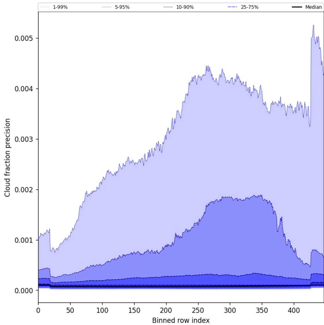
Figure 50: Along track statistics of “Cloud fraction precision” for 2025-05-10 to 2025-05-11
