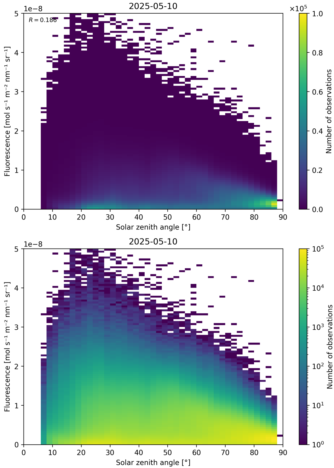
Figure 112: Scatter density plot of “Solar zenith angle” against “Fluorescence” for 2025-05-10 to 2025-05-11.
