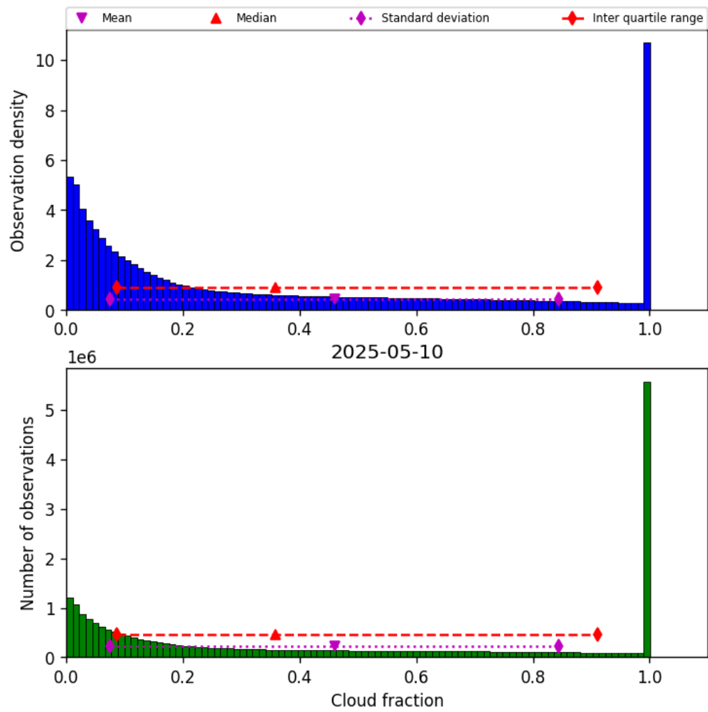
Figure 32: Histogram of “Cloud fraction” for 2025-05-10 to 2025-05-11
