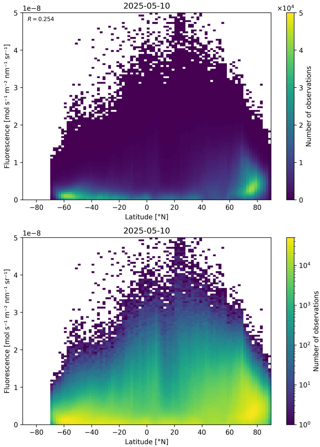
Figure 92: Scatter density plot of “Latitude” against “Fluorescence” for 2025-05-10 to 2025-05-11.
