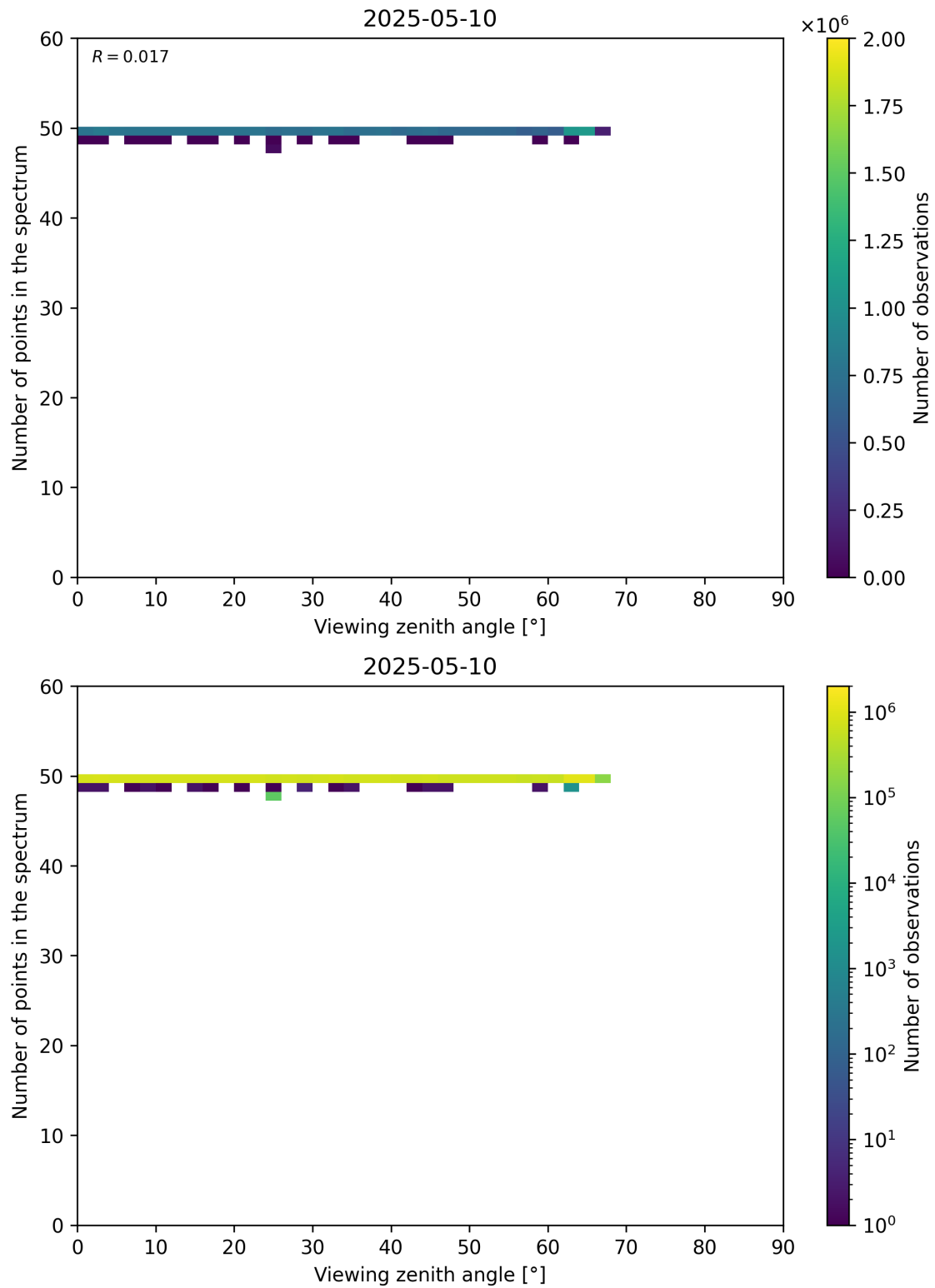
Figure 125: Scatter density plot of “Viewing zenith angle” against “Number of points in the spectrum” for 2025-05-10 to 2025-05-11.
