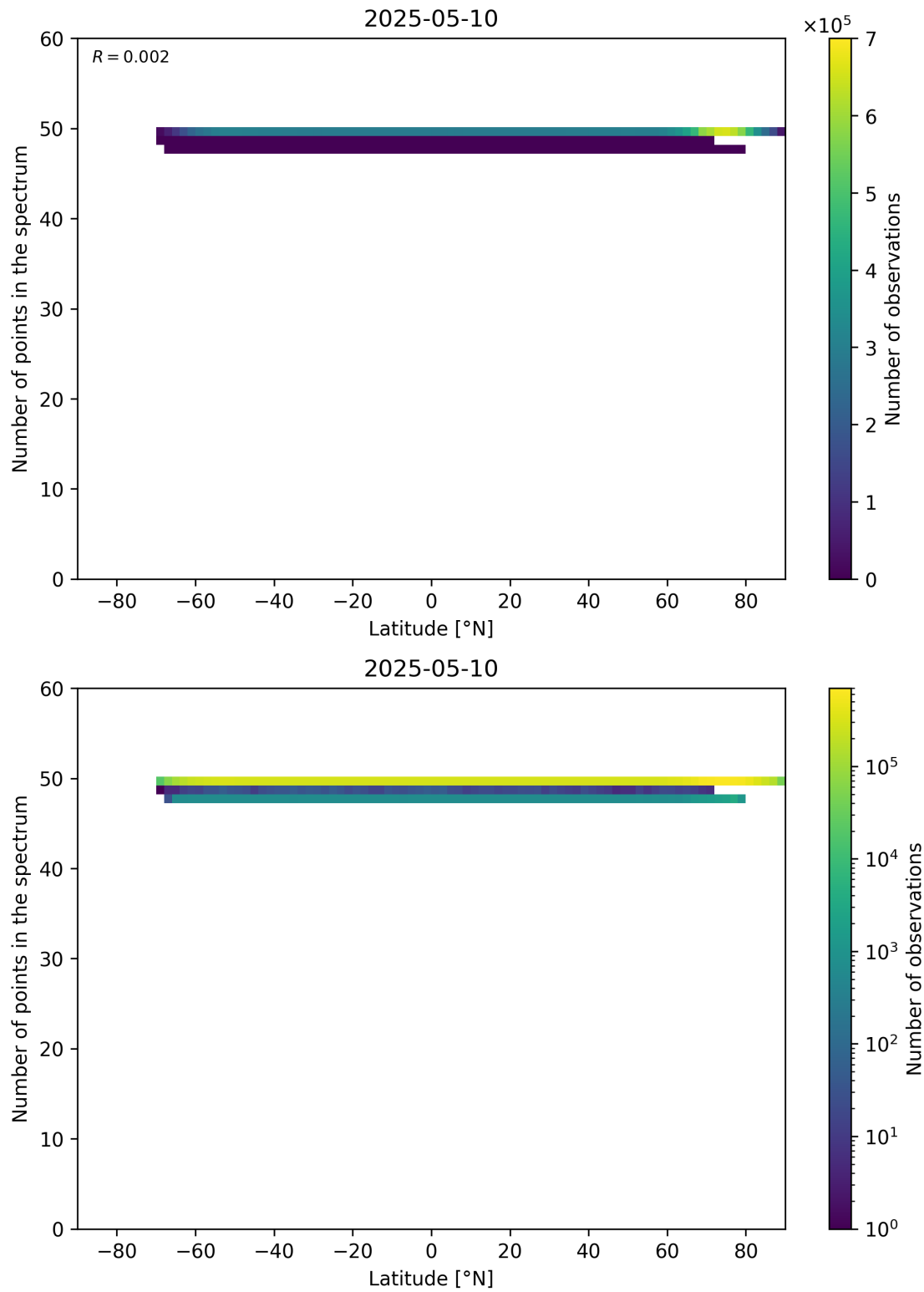
Figure 94: Scatter density plot of “Latitude” against “Number of points in the spectrum” for 2025-05-10 to 2025-05-11.
