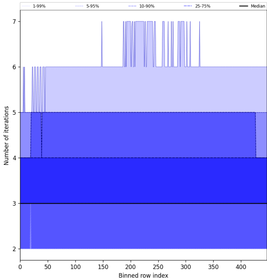
Figure 56: Along track statistics of “Number of iterations” for 2025-05-10 to 2025-05-11
