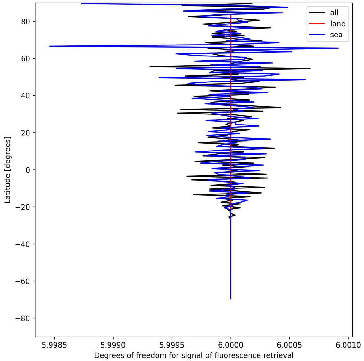
Figure 26: Zonal average of “Degrees of freedom for signal of fluorescence retrieval” for 2025-05-10 to 2025-05-11.
