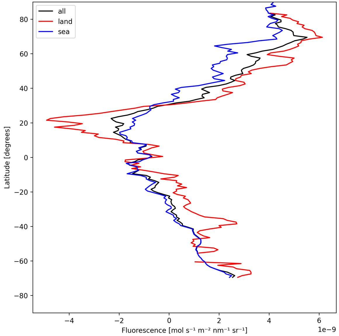
Figure 23: Zonal average of “Fluorescence” for 2025-05-10 to 2025-05-11.
