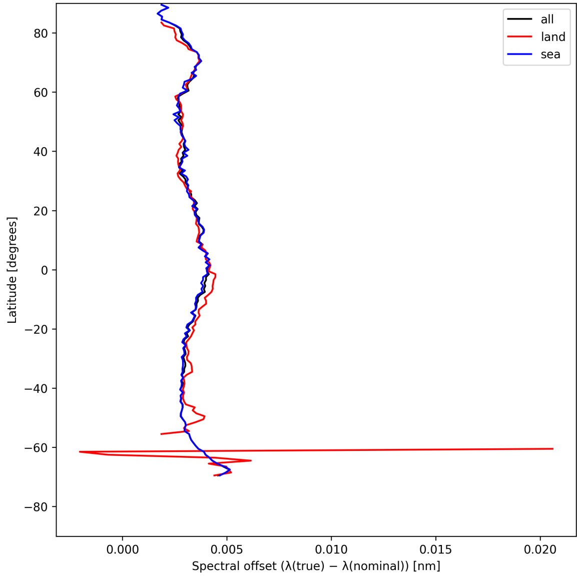
Figure 28: Zonal average of “Spectral offset ( \lambda_{\text{true}} - \lambda_{\text{nominal}} )” for 2025-05-10 to 2025-05-11.
