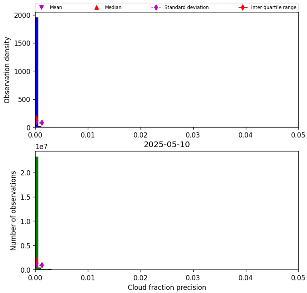
Figure 33: Histogram of “Cloud fraction precision” for 2025-05-10 to 2025-05-11
