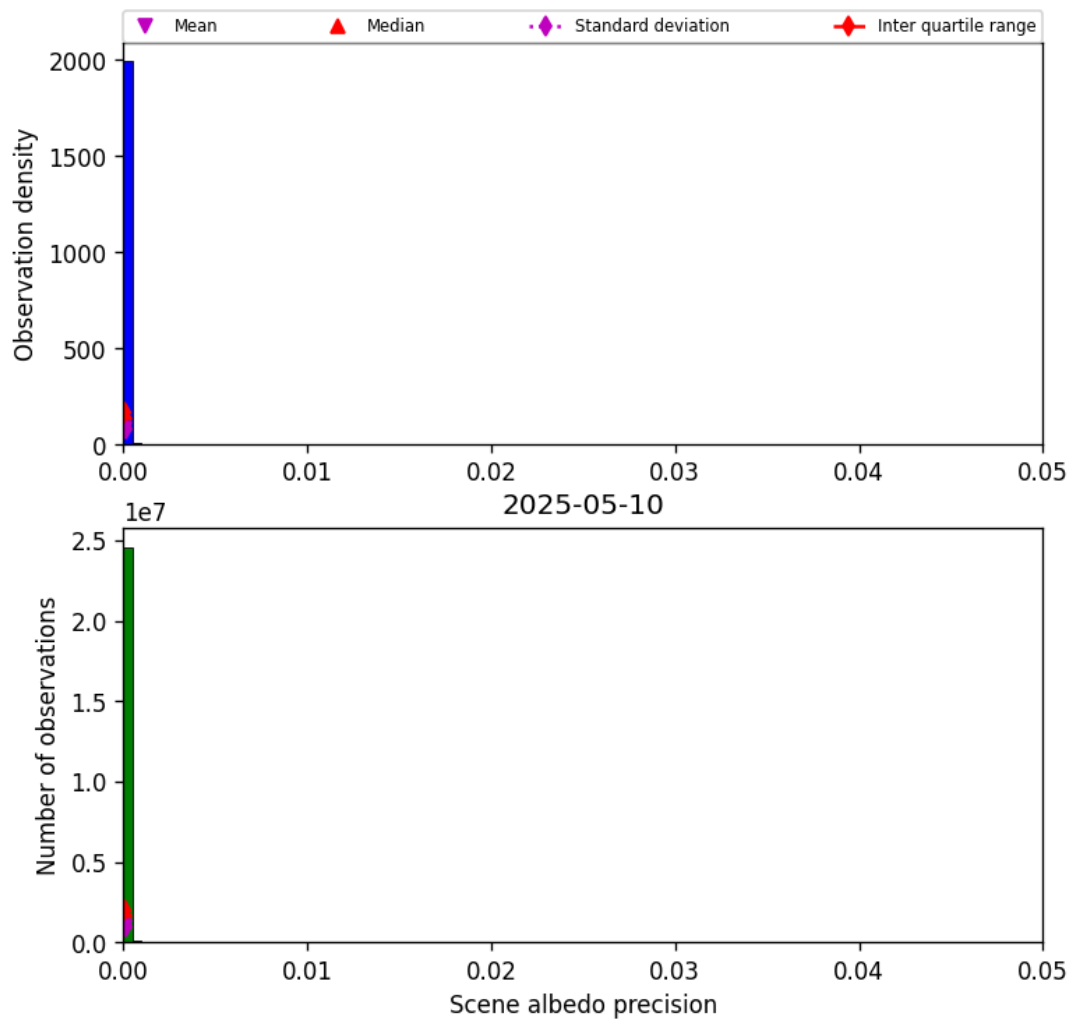
Figure 35: Histogram of “Scene albedo precision” for 2025-05-10 to 2025-05-11
