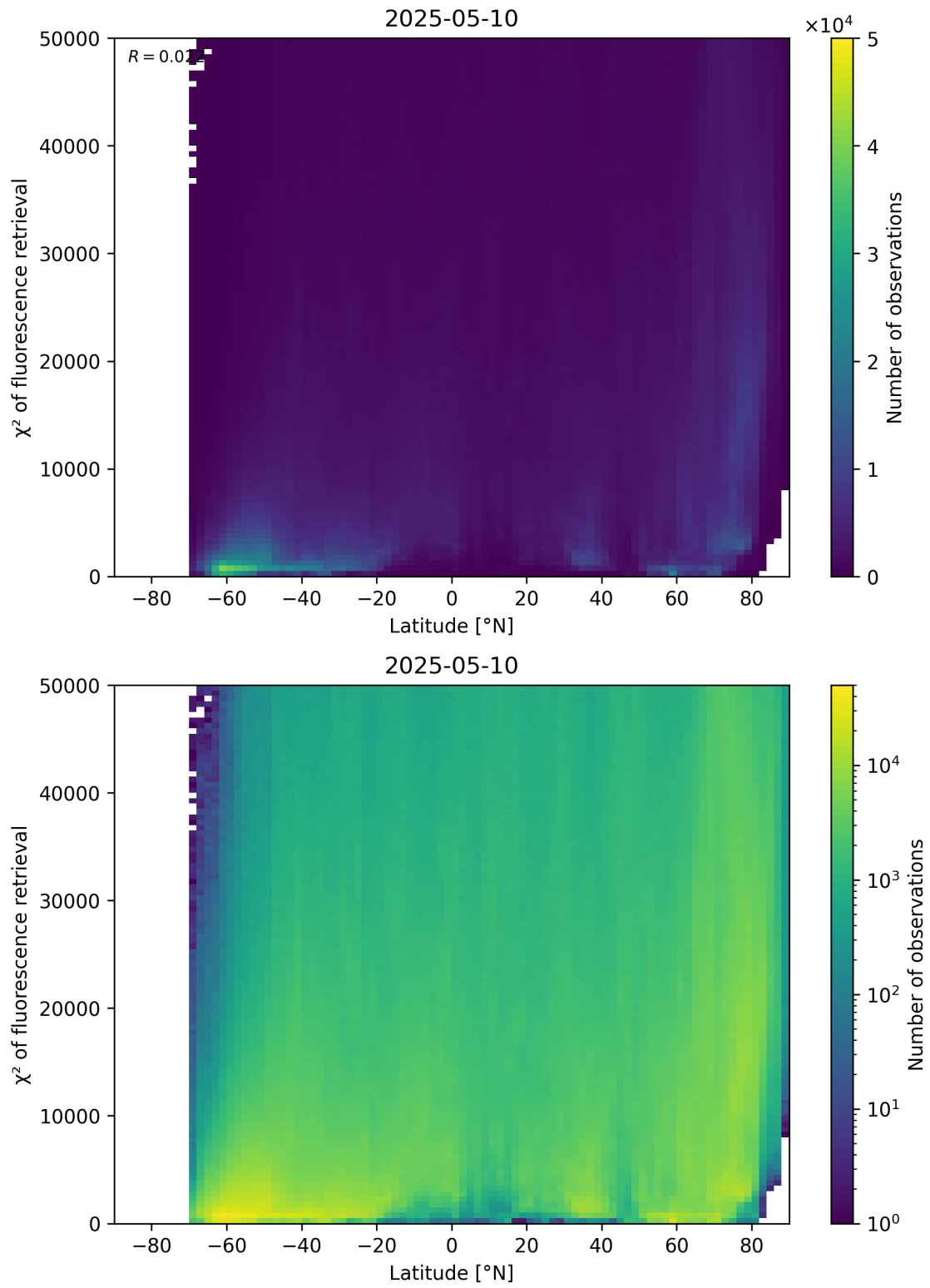
Figure 89: Scatter density plot of “Latitude” against “ \chi^2 of fluorescence retrieval” for 2025-05-10 to 2025-05-11.
