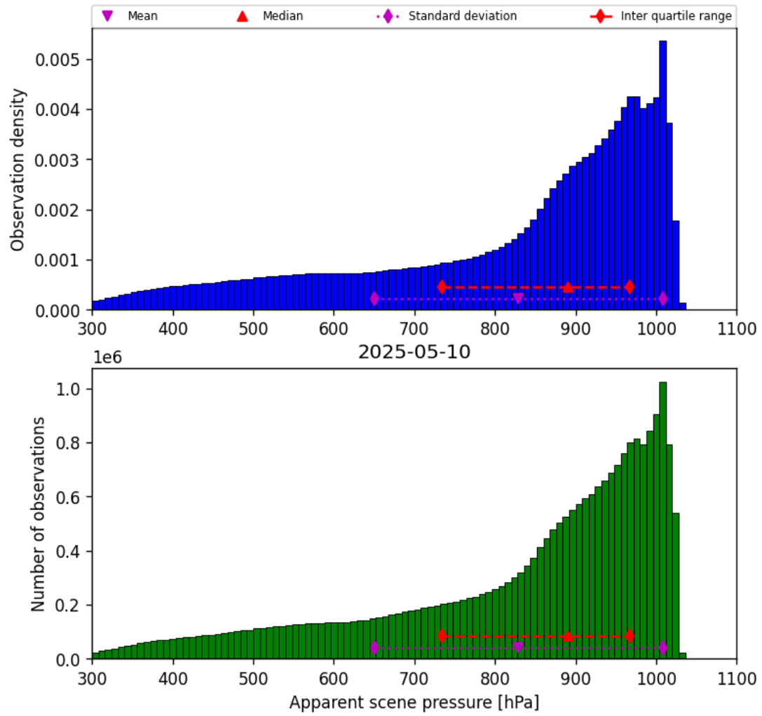
Figure 36: Histogram of “Apparent scene pressure” for 2025-05-10 to 2025-05-11
