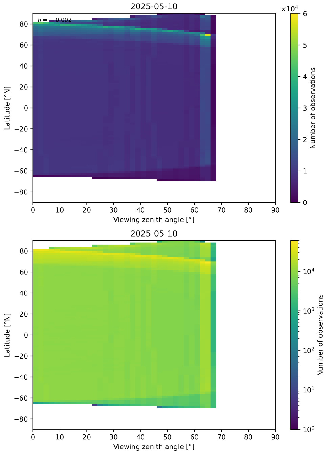
Figure 123: Scatter density plot of “Viewing zenith angle” against “Latitude” for 2025-05-10 to 2025-05-11.
