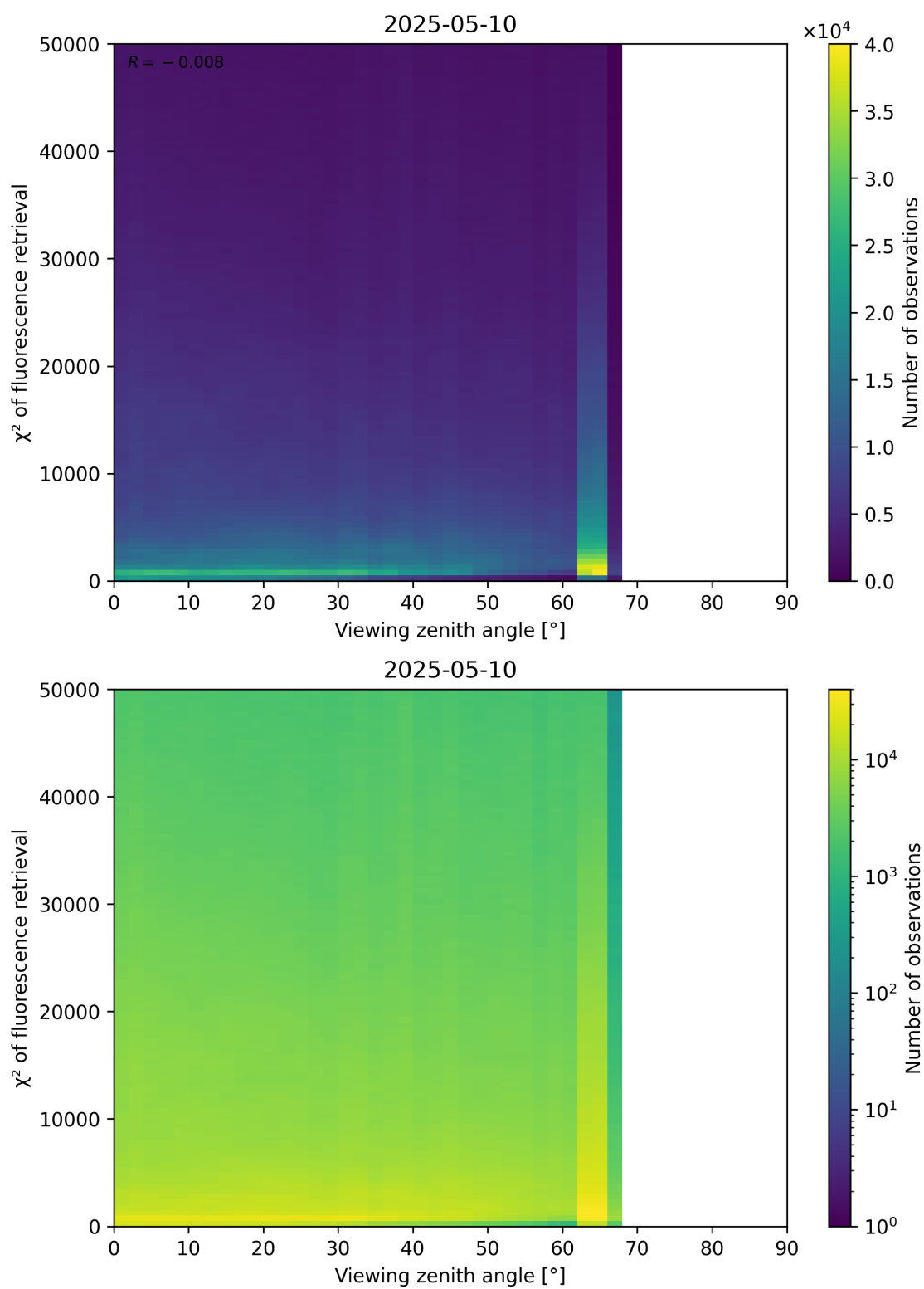
Figure 119: Scatter density plot of “Viewing zenith angle” against “ \chi^2 of fluorescence retrieval” for 2025-05-10 to 2025-05-11.
