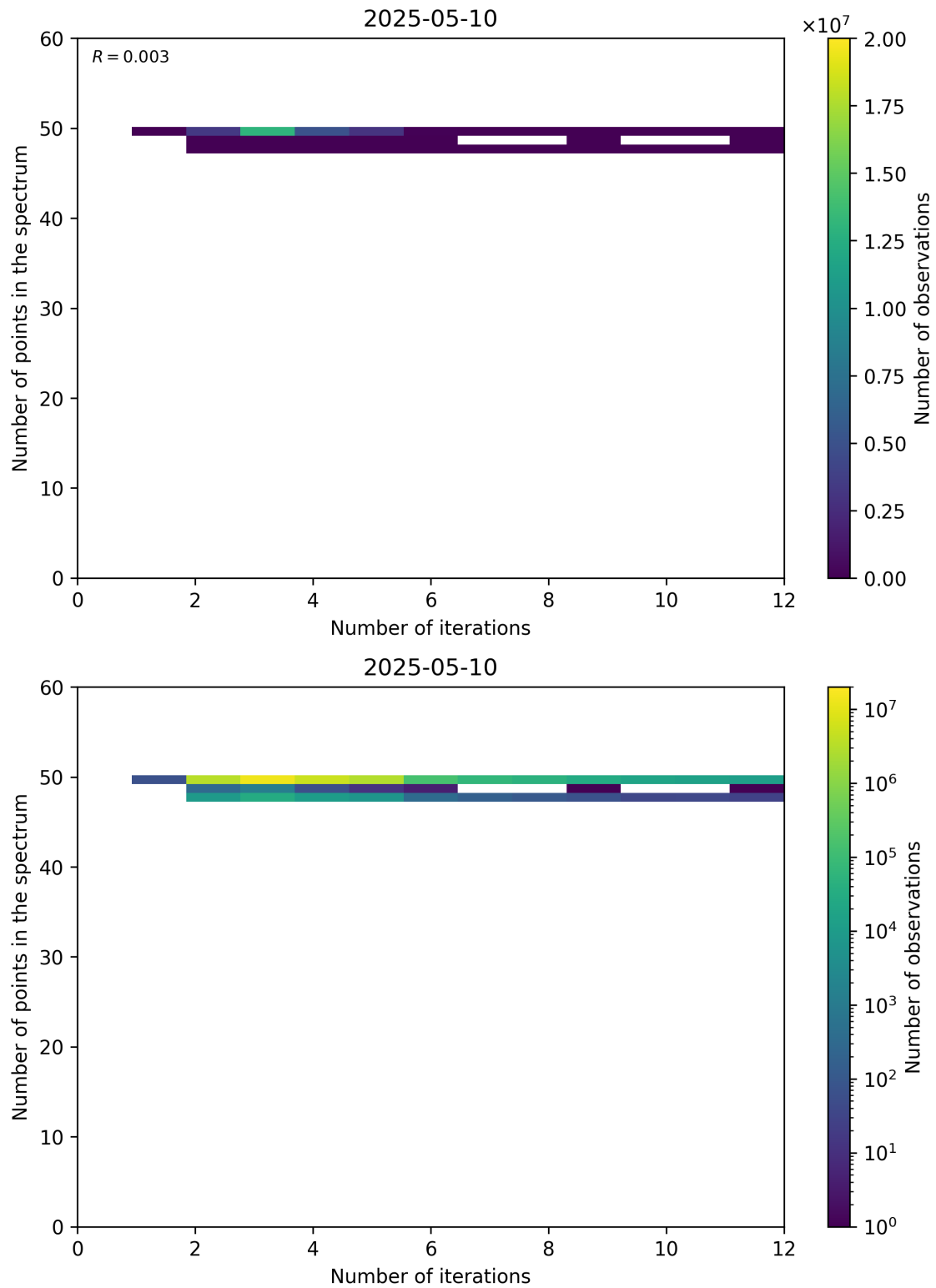
Figure 99: Scatter density plot of “Number of iterations” against “Number of points in the spectrum” for 2025-05-10 to 2025-05-11.
