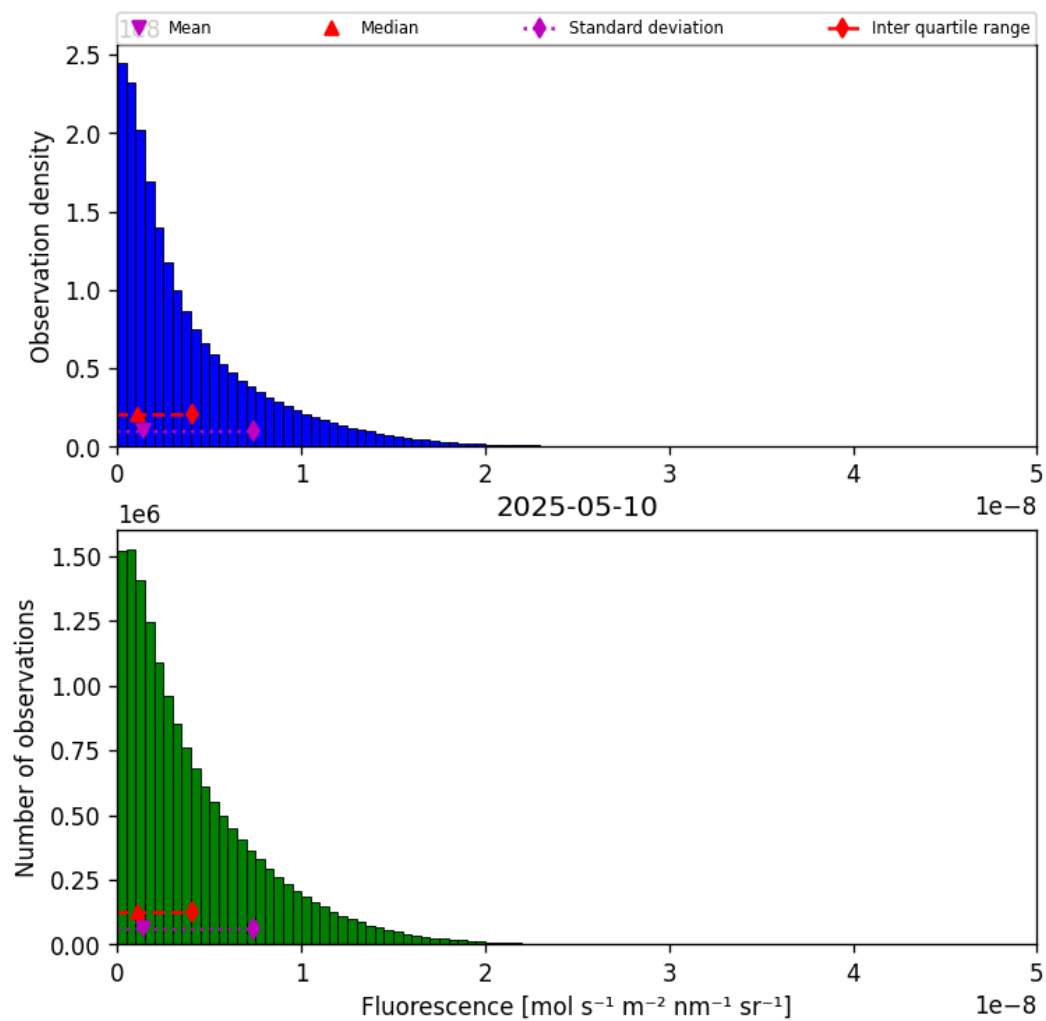
Figure 40: Histogram of “Fluorescence” for 2025-05-10 to 2025-05-11
