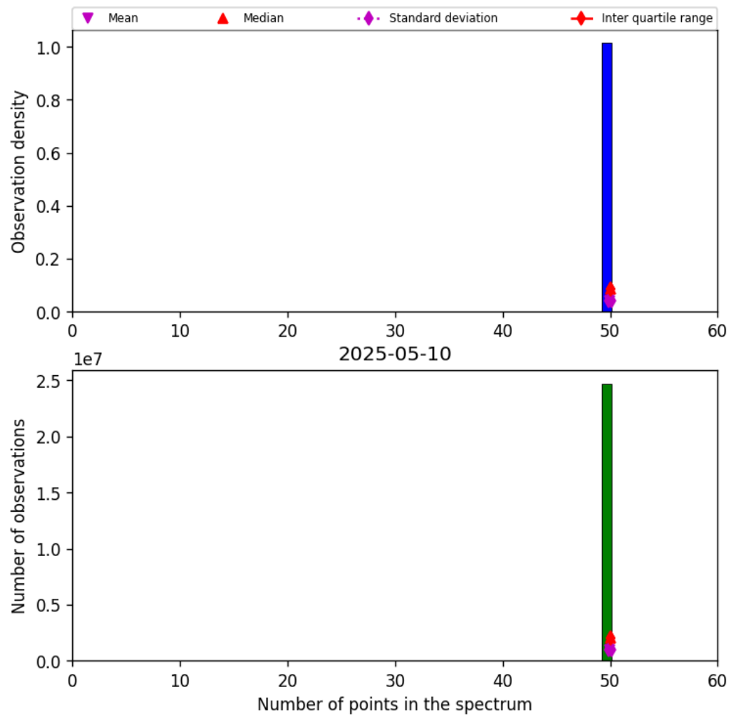
Figure 44: Histogram of “Number of points in the spectrum” for 2025-05-10 to 2025-05-11
