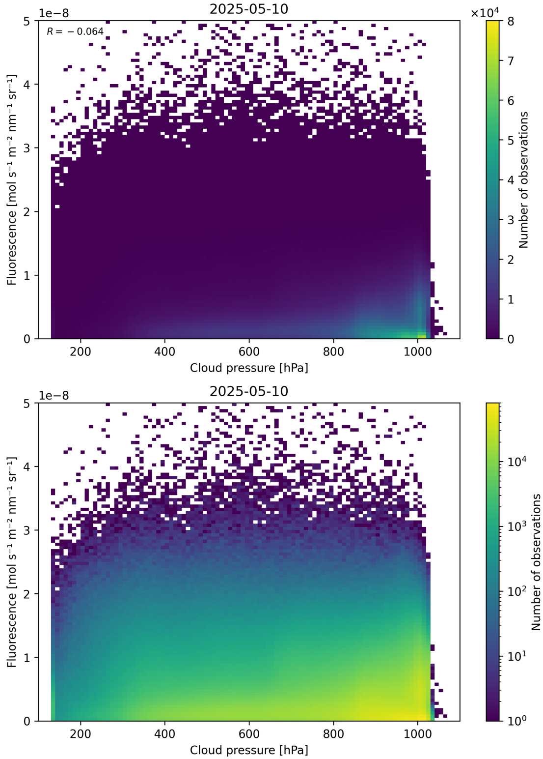
Figure 80: Scatter density plot of “Cloud pressure” against “Fluorescence” for 2025-05-10 to 2025-05-11.
