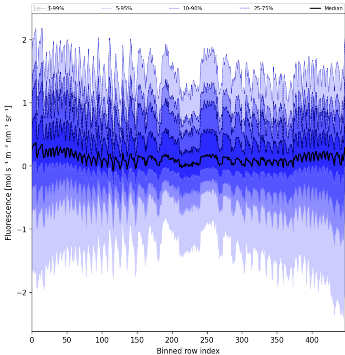
Figure 57: Along track statistics of “Fluorescence” for 2025-05-10 to 2025-05-11
