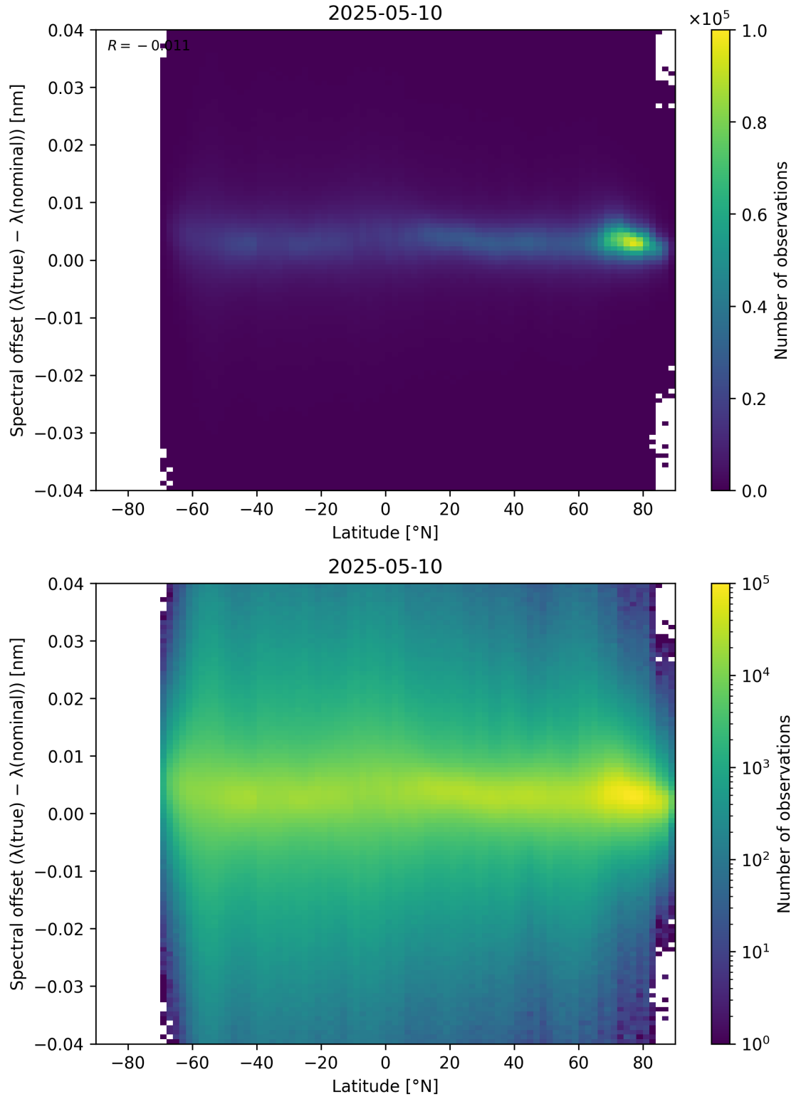
Figure 96: Scatter density plot of “Latitude” against “Spectral offset ( \lambda_{\text{true}} - \lambda_{\text{nominal}} )” for 2025-05-10 to 2025-05-11.
