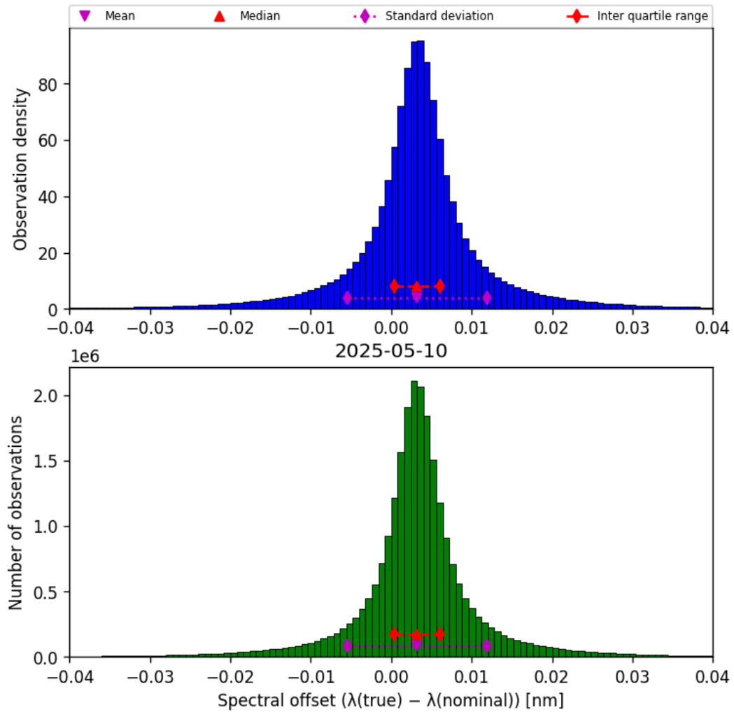
Figure 45: Histogram of “Spectral offset ( \lambda_{\text{true}} - \lambda_{\text{nominal}} )” for 2025-05-10 to 2025-05-11
