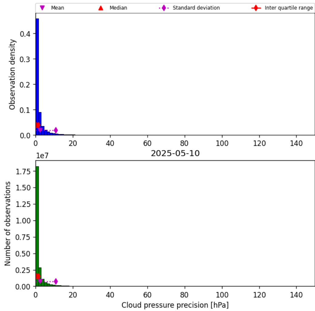
Figure 31: Histogram of “Cloud pressure precision” for 2025-05-10 to 2025-05-11
