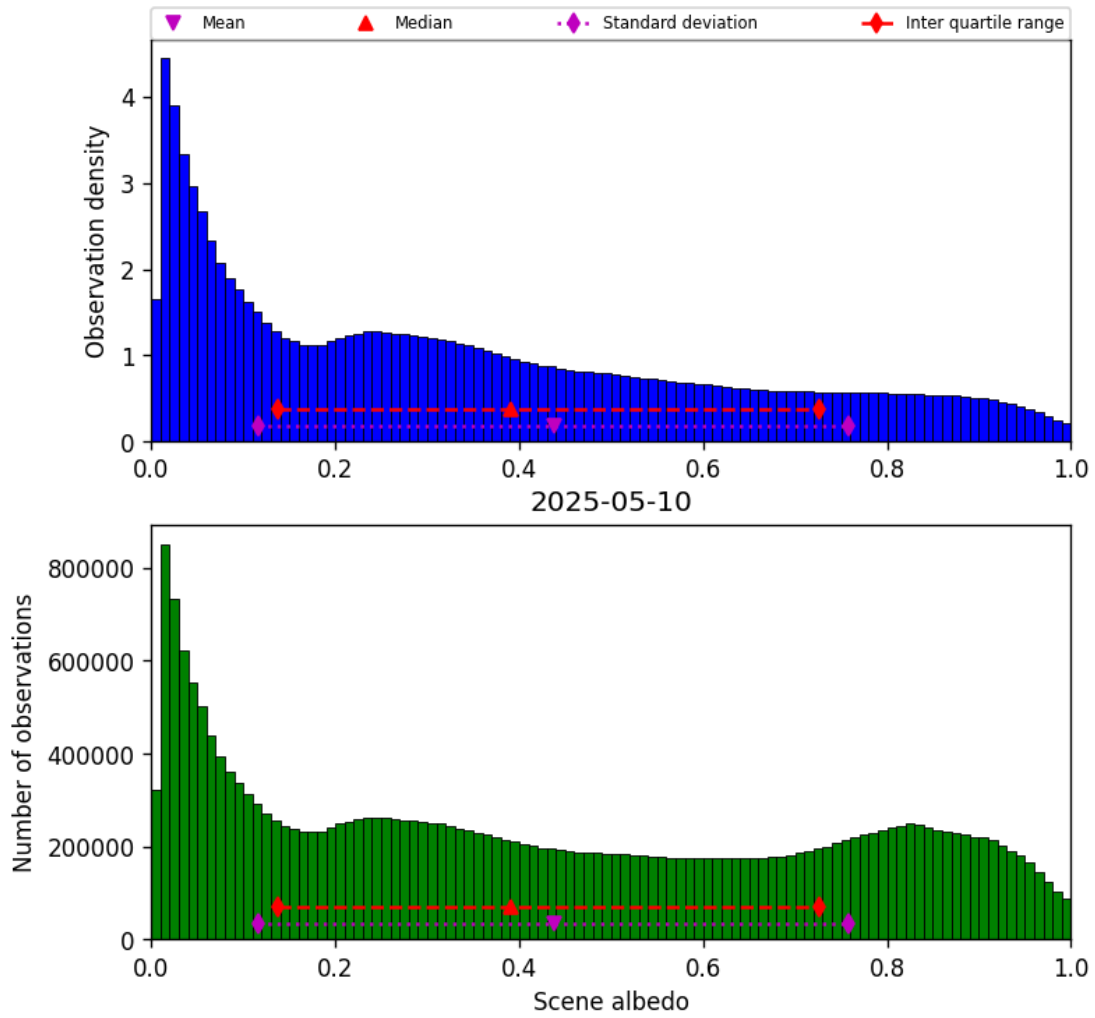
Figure 34: Histogram of “Scene albedo” for 2025-05-10 to 2025-05-11
