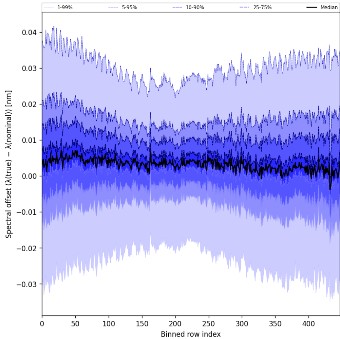
Figure 62: Along track statistics of “Spectral offset ( \lambda_{\text{true}} - \lambda_{\text{nominal}} )” for 2025-05-10 to 2025-05-11
