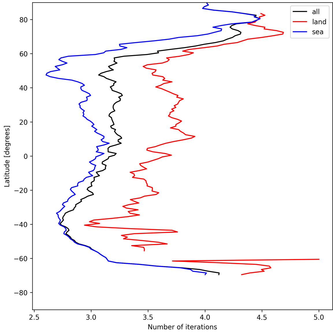
Figure 22: Zonal average of “Number of iterations” for 2025-05-10 to 2025-05-11.
