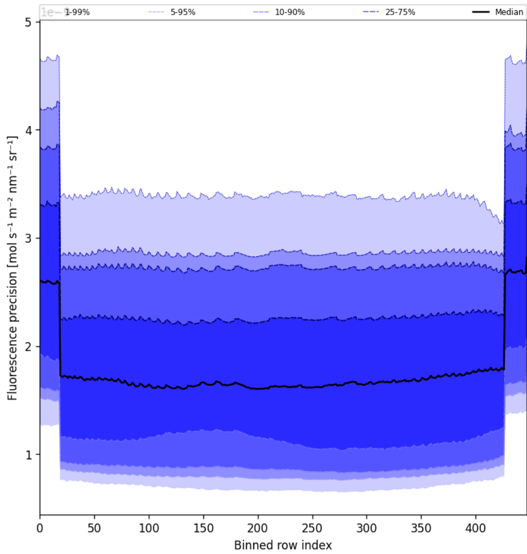
Figure 58: Along track statistics of “Fluorescence precision” for 2025-05-10 to 2025-05-11
