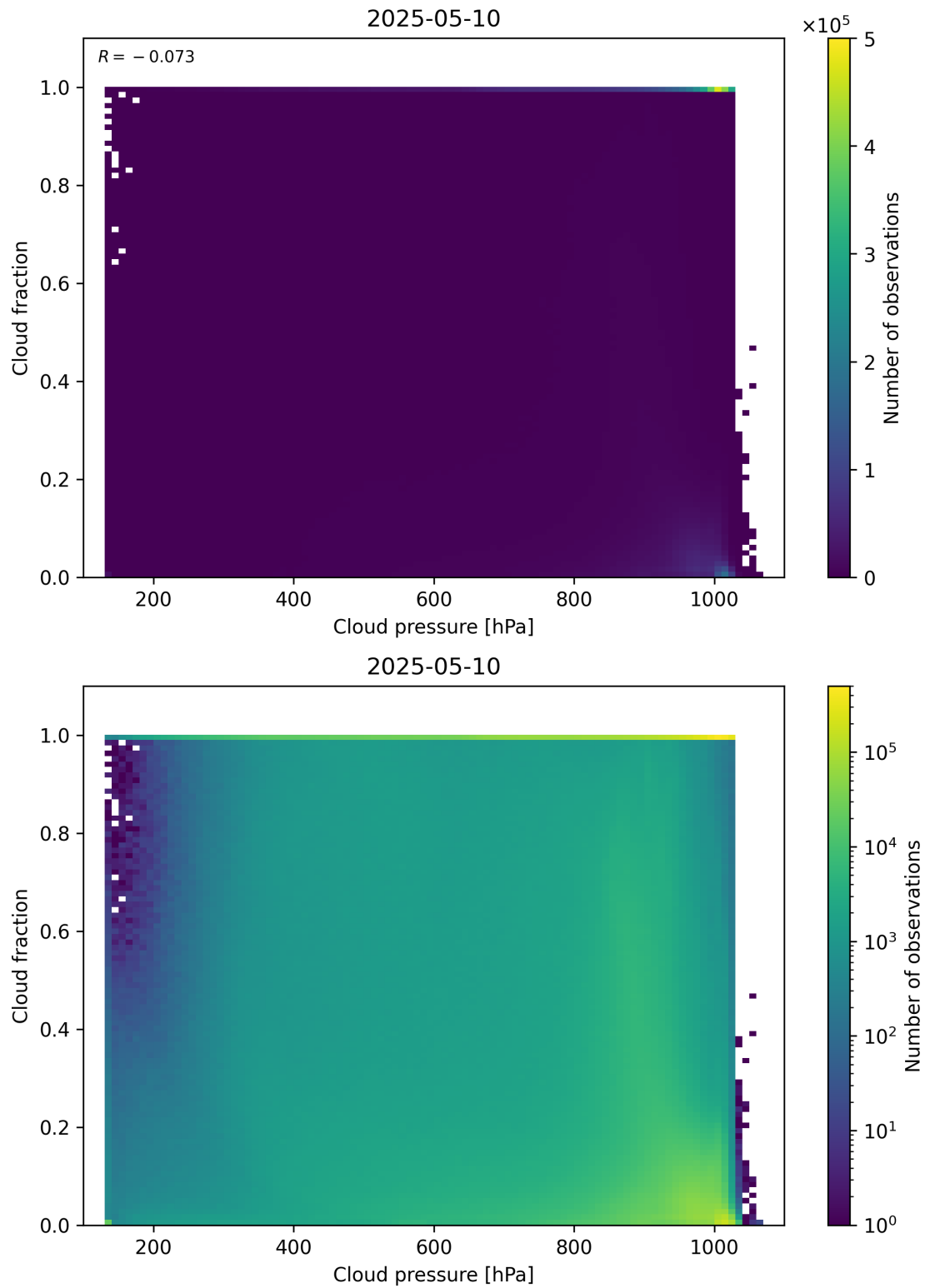
Figure 79: Scatter density plot of “Cloud pressure” against “Cloud fraction” for 2025-05-10 to 2025-05-11.
