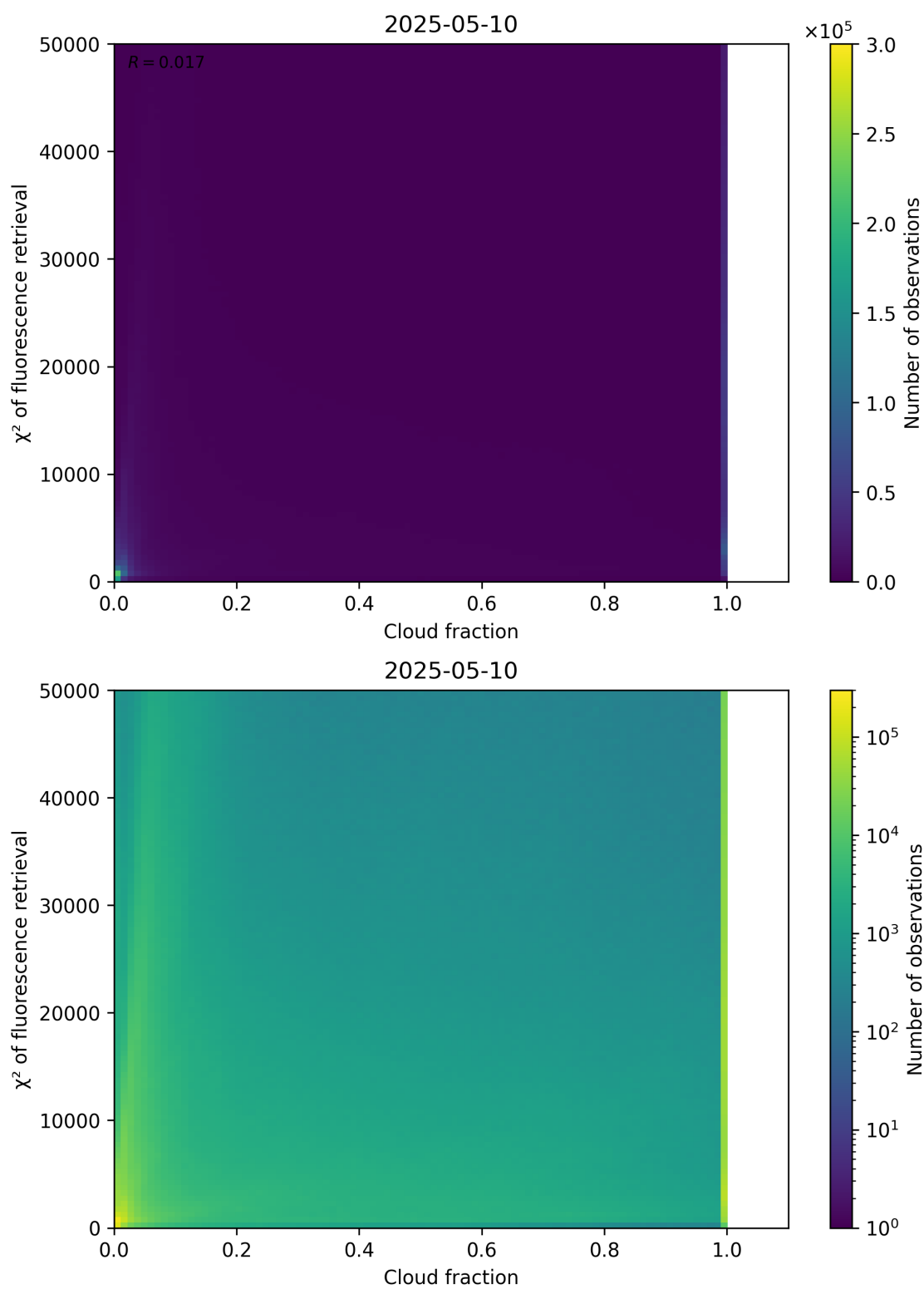
Figure 71: Scatter density plot of “Cloud fraction” against “ \chi^2 of fluorescence retrieval” for 2025-05-10 to 2025-05-11.
