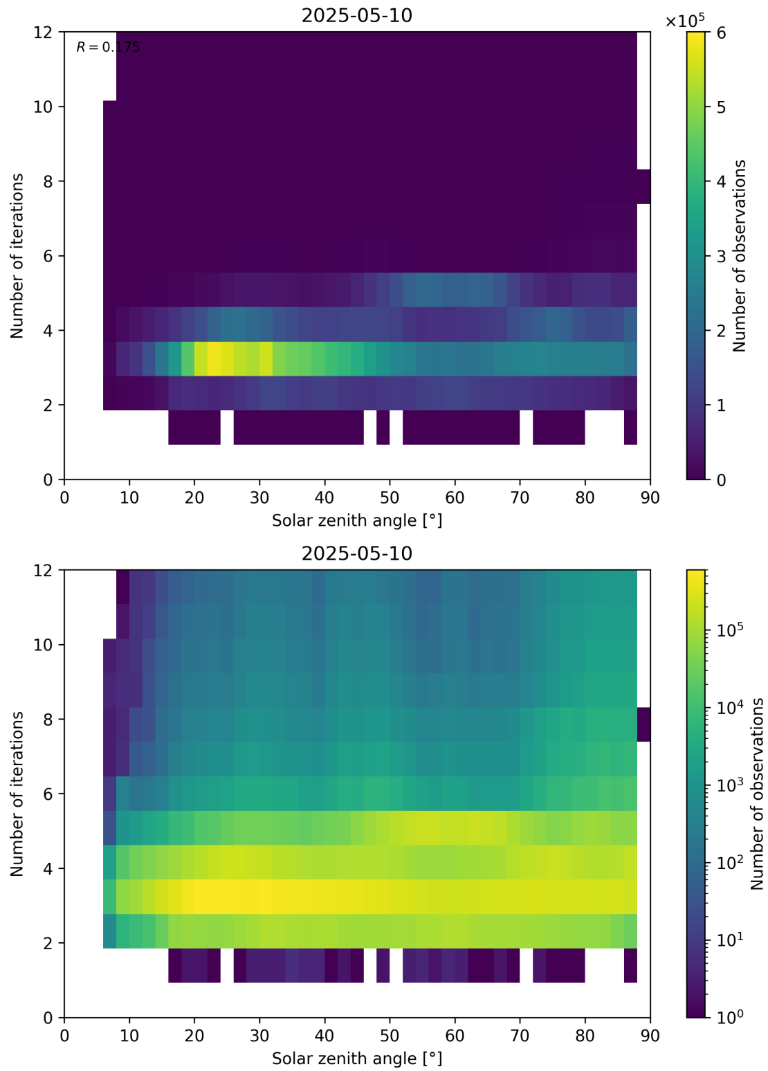
Figure 114: Scatter density plot of “Solar zenith angle” against “Number of iterations” for 2025-05-10 to 2025-05-11.
