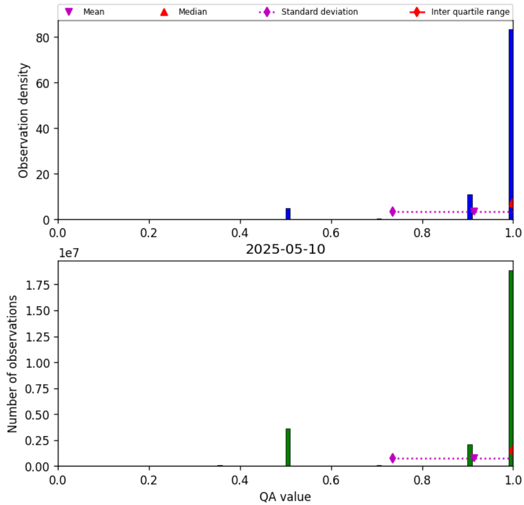
Figure 29: Histogram of “QA value” for 2025-05-10 to 2025-05-11
