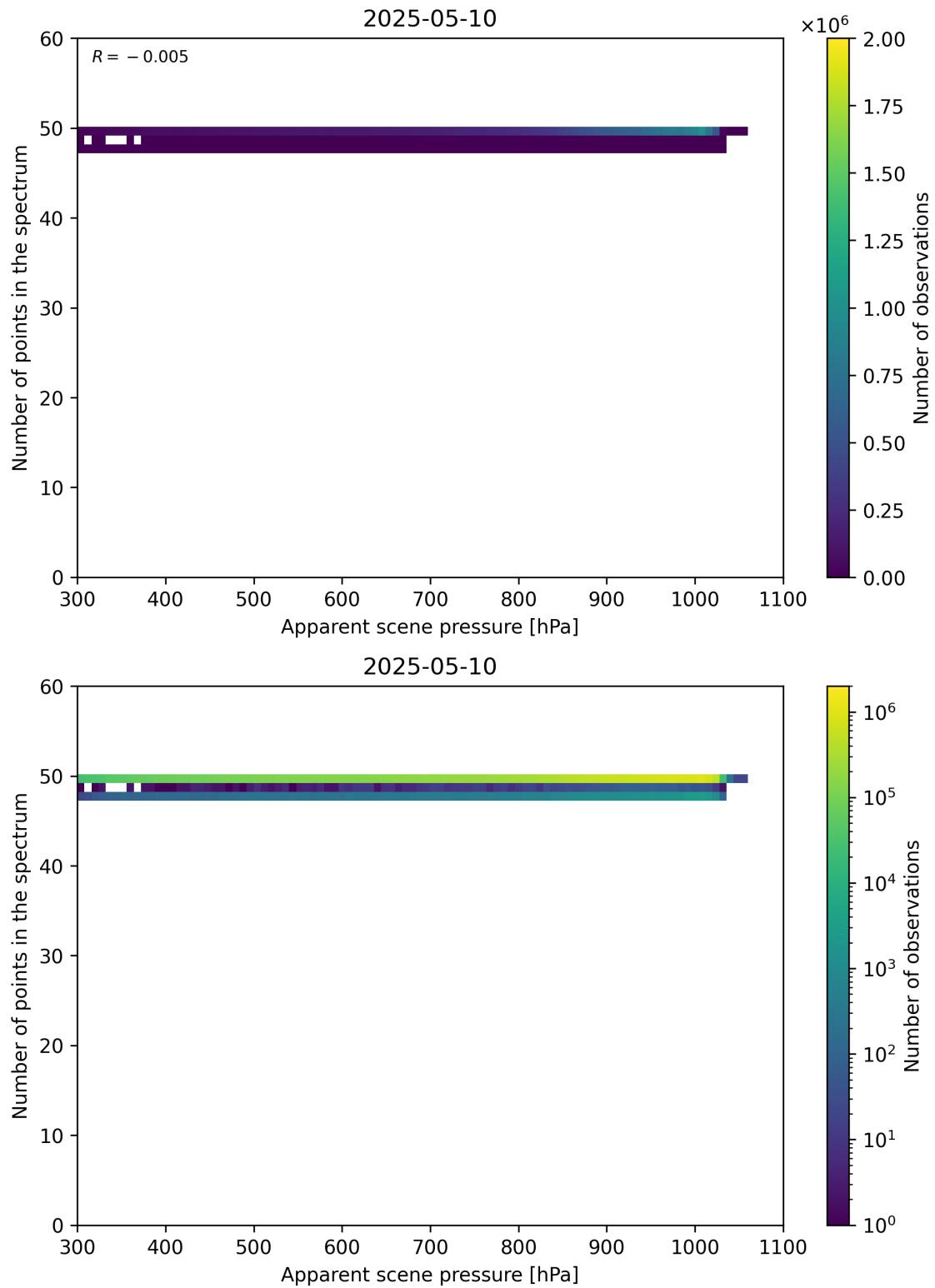
Figure 66: Scatter density plot of “Apparent scene pressure” against “Number of points in the spectrum” for 2025-05-10 to 2025-05-11.
