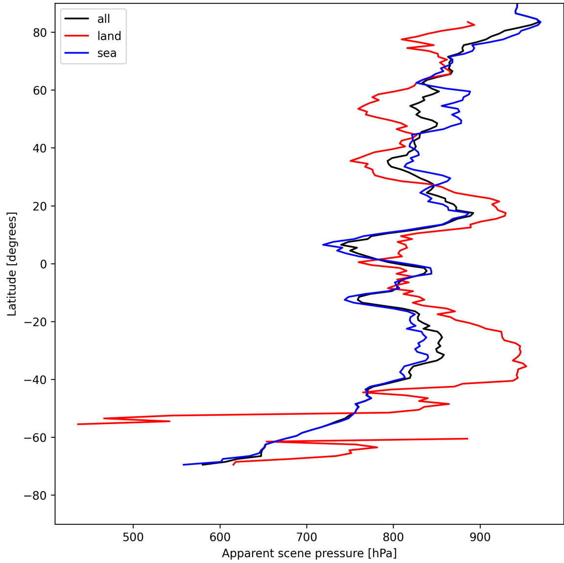
Figure 19: Zonal average of “Apparent scene pressure” for 2025-05-10 to 2025-05-11.
