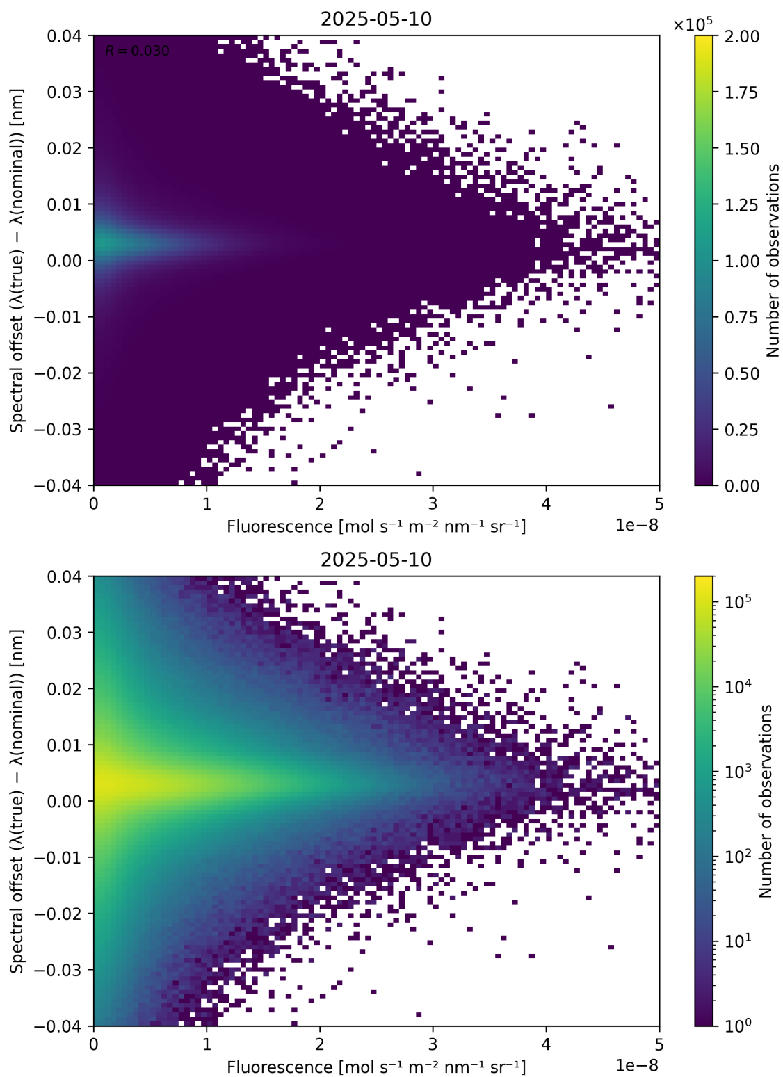
Figure 87: Scatter density plot of “Fluorescence” against “Spectral offset ( \lambda_{\text{true}} - \lambda_{\text{nominal}} )” for 2025-05-10 to 2025-05-11.
