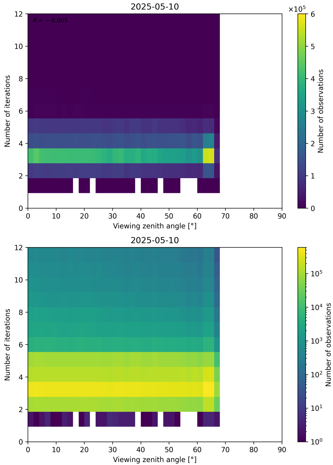
Figure 124: Scatter density plot of “Viewing zenith angle” against “Number of iterations” for 2025-05-10 to 2025-05-11.
