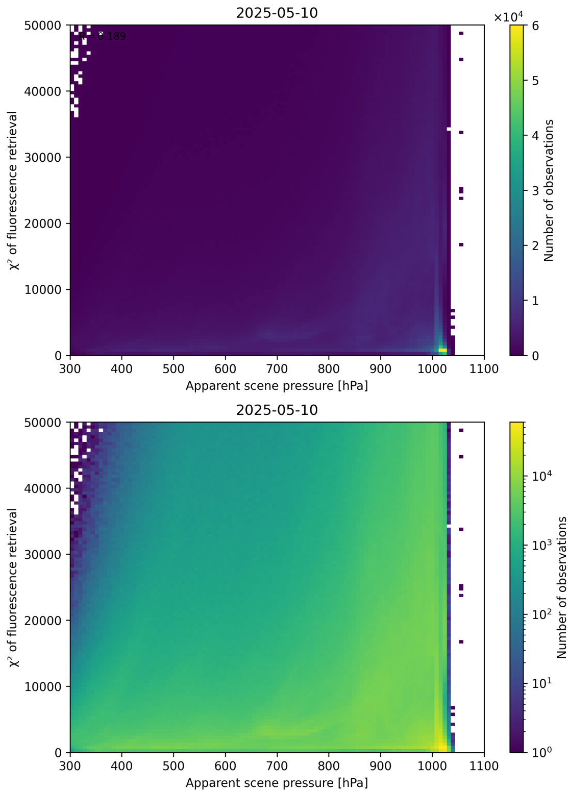
Figure 63: Scatter density plot of “Apparent scene pressure” against “ \chi^2 of fluorescence retrieval” for 2025-05-10 to 2025-05-11.
