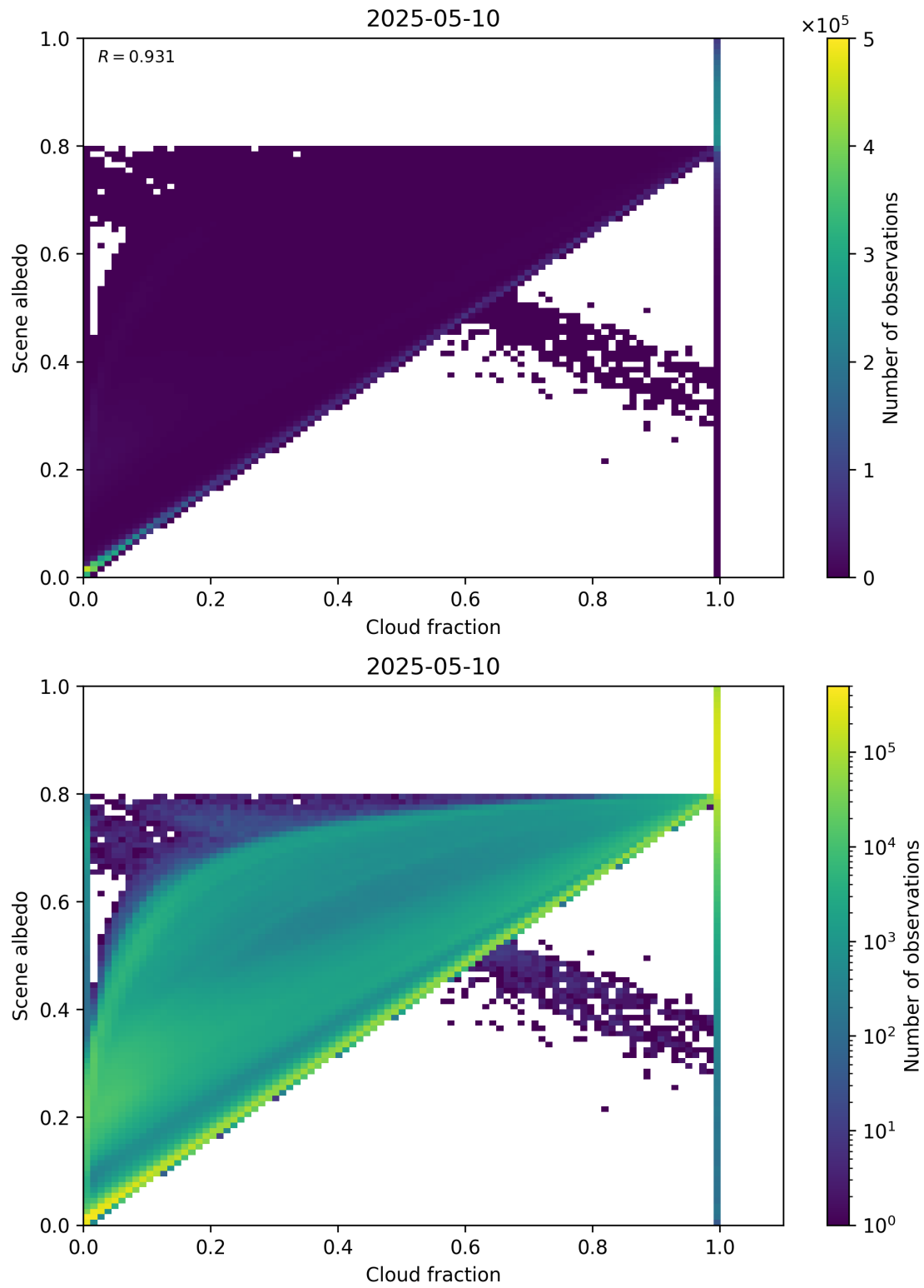
Figure 75: Scatter density plot of “Cloud fraction” against “Scene albedo” for 2025-05-10 to 2025-05-11.
