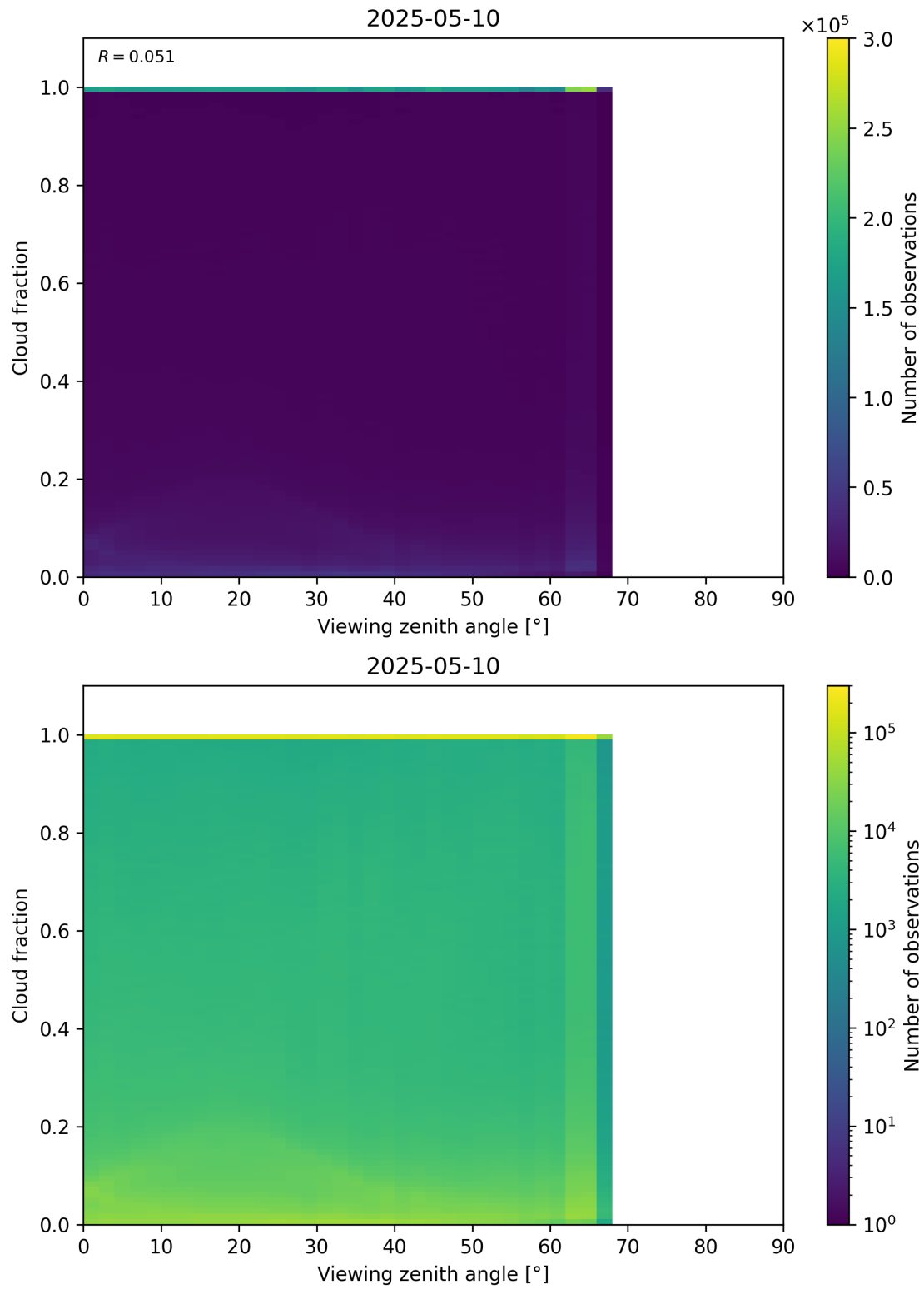
Figure 120: Scatter density plot of “Viewing zenith angle” against “Cloud fraction” for 2025-05-10 to 2025-05-11.
