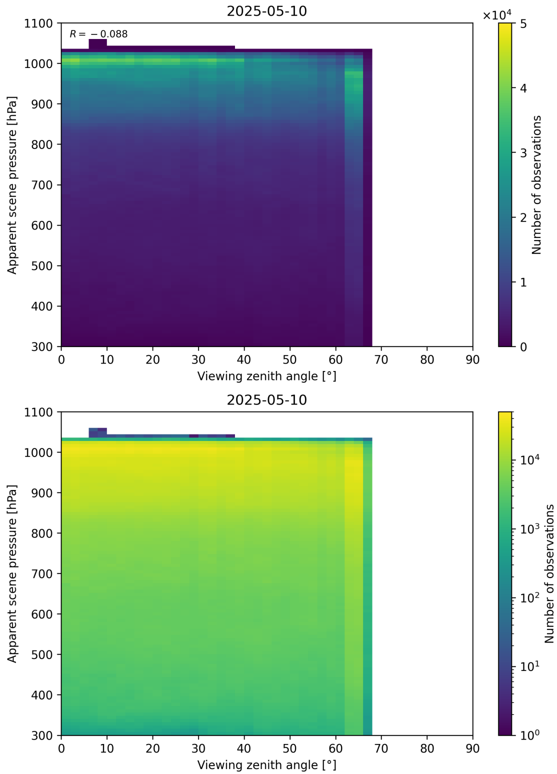
Figure 118: Scatter density plot of “Viewing zenith angle” against “Apparent scene pressure” for 2025-05-10 to 2025-05-11.
