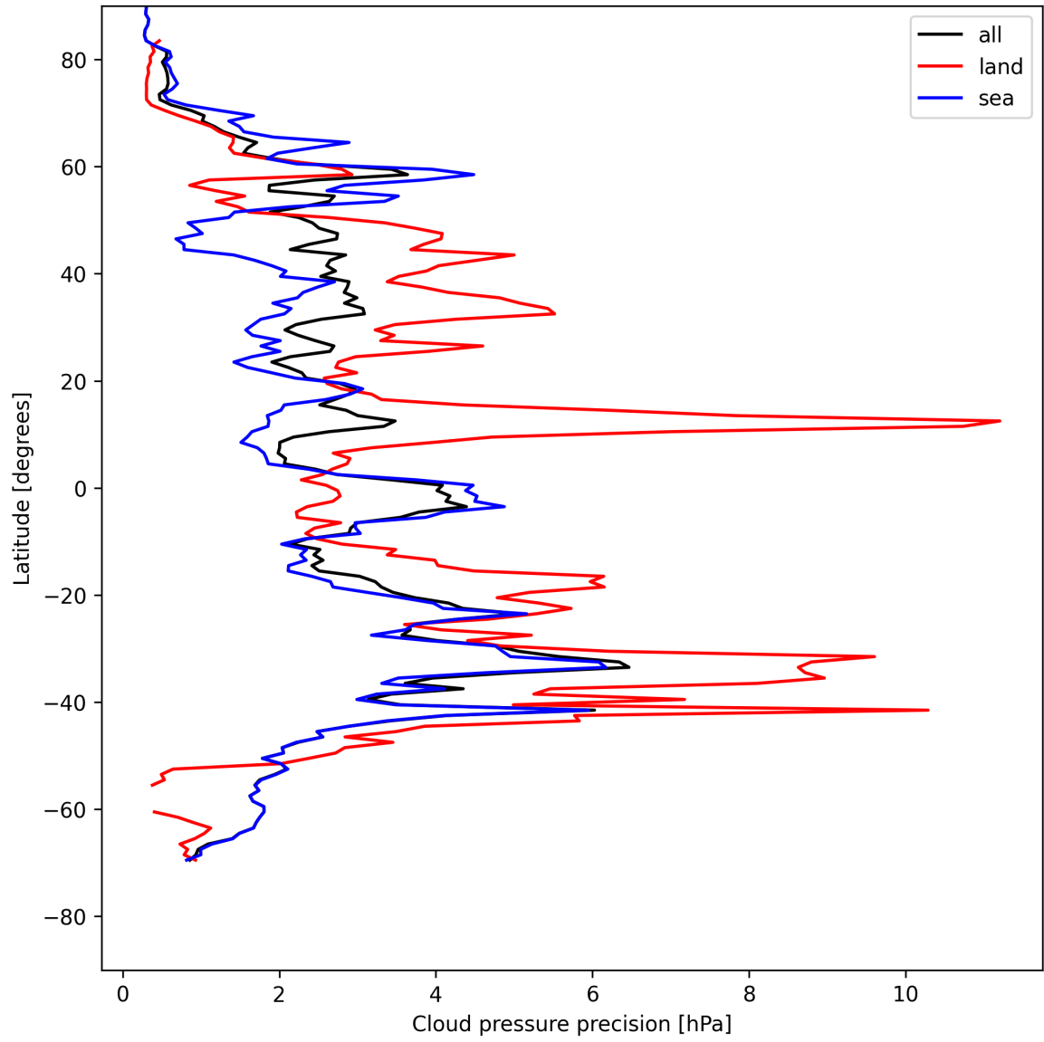
Figure 14: Zonal average of “Cloud pressure precision” for 2025-05-10 to 2025-05-11.
