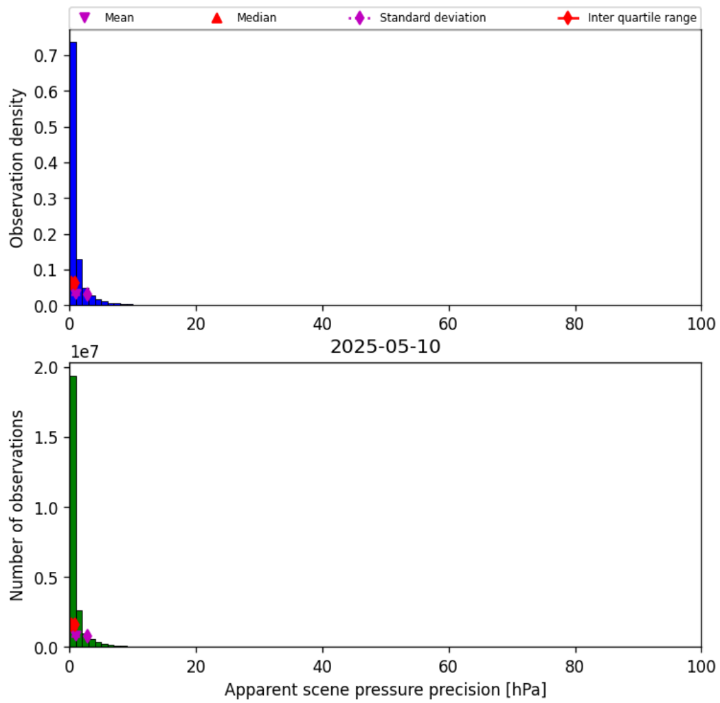
Figure 37: Histogram of “Apparent scene pressure precision” for 2025-05-10 to 2025-05-11
