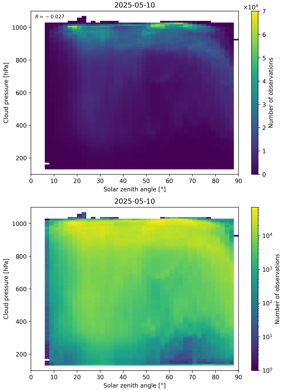
Figure 111: Scatter density plot of “Solar zenith angle” against “Cloud pressure” for 2025-05-10 to 2025-05-11.
