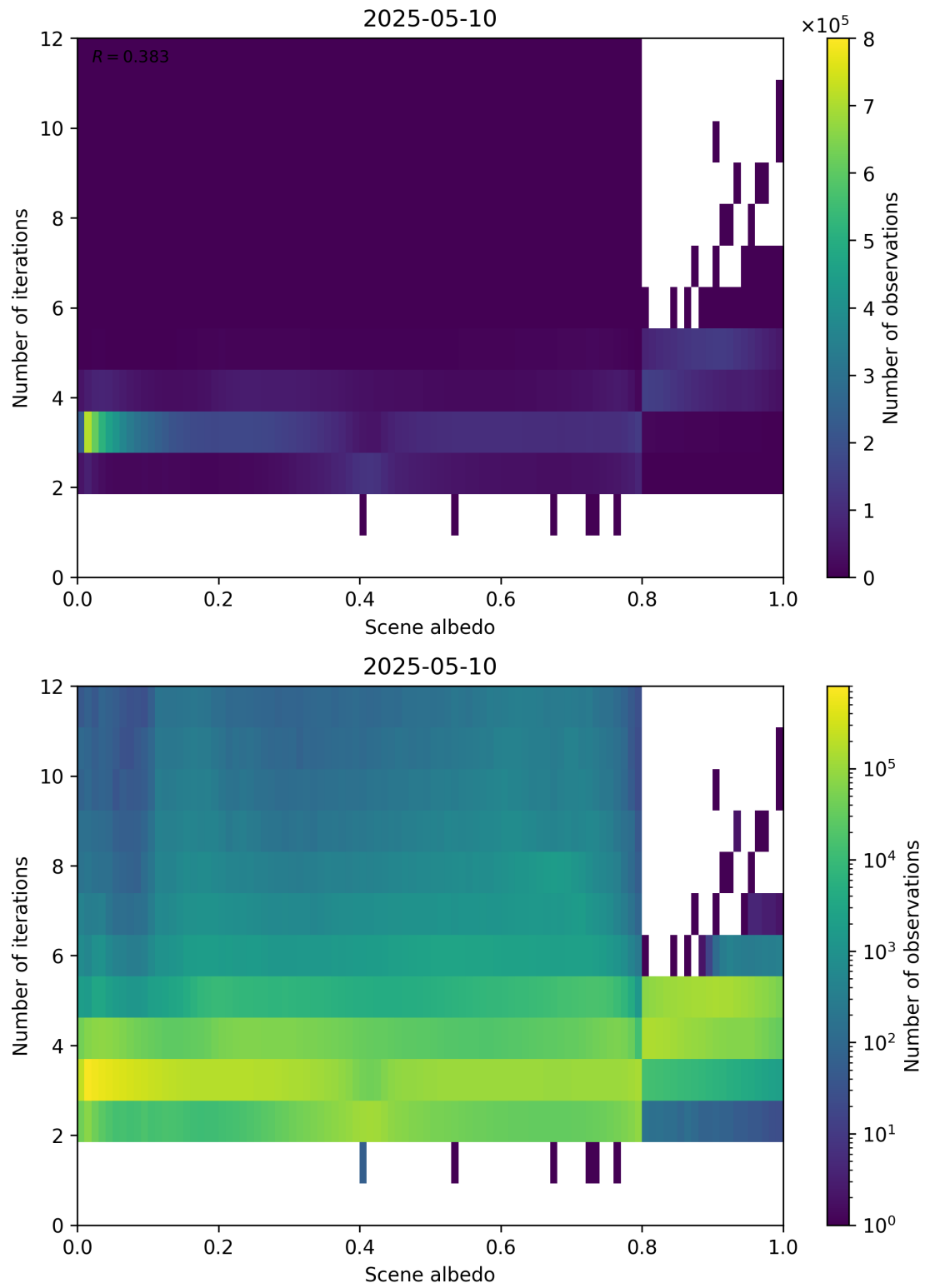
Figure 105: Scatter density plot of “Scene albedo” against “Number of iterations” for 2025-05-10 to 2025-05-11.
