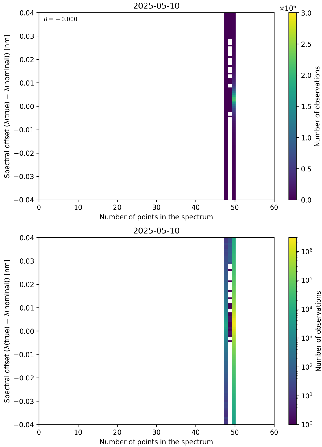
Figure 101: Scatter density plot of “Number of points in the spectrum” against “Spectral offset ( \lambda_{\text{true}} - \lambda_{\text{nominal}} )” for 2025-05-10 to 2025-05-11.
