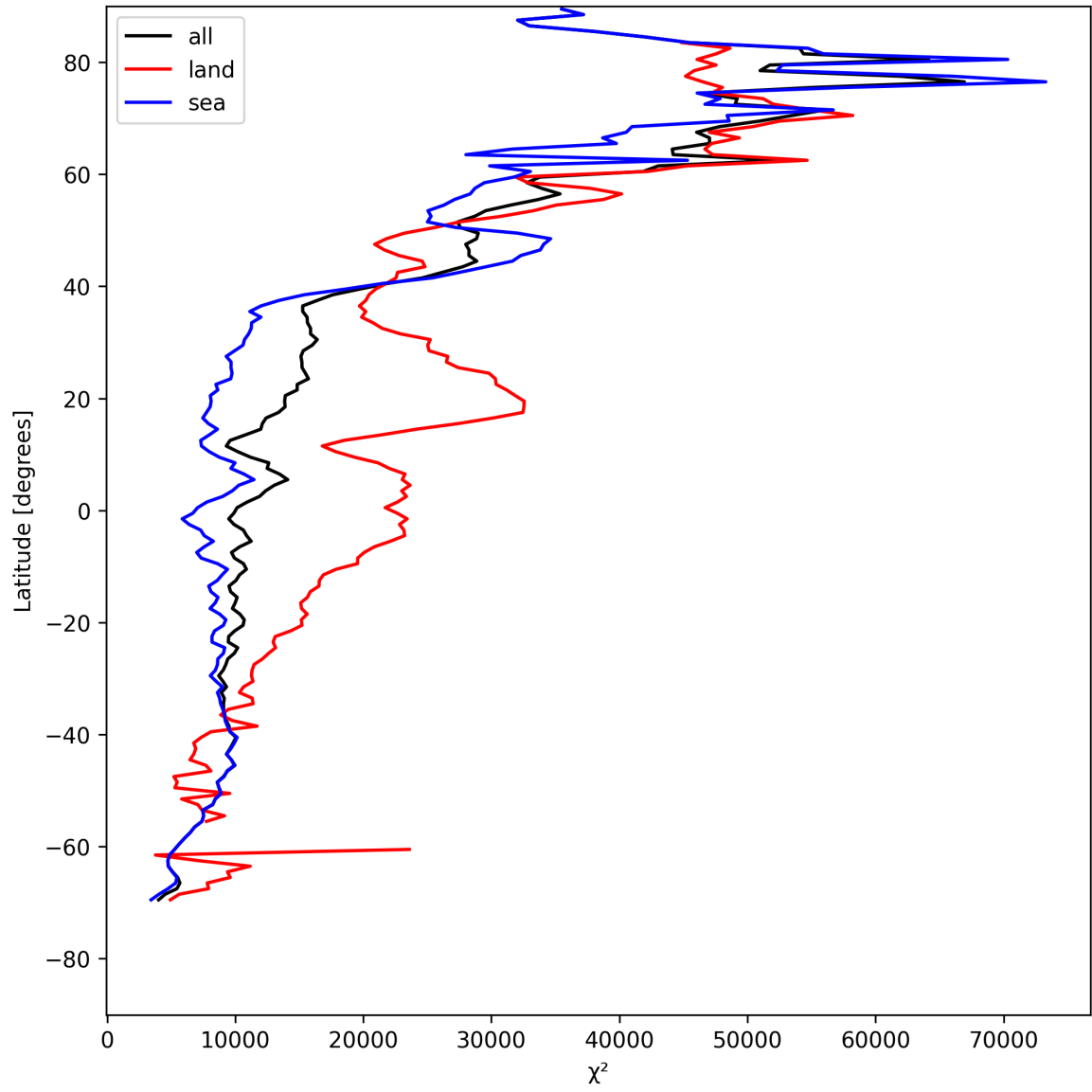
Figure 21: Zonal average of “ \chi^2 ” for 2025-05-10 to 2025-05-11.
