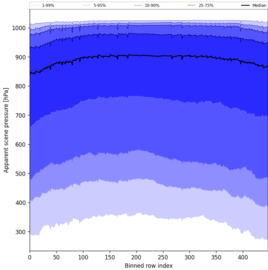
Figure 53: Along track statistics of “Apparent scene pressure” for 2025-05-10 to 2025-05-11
