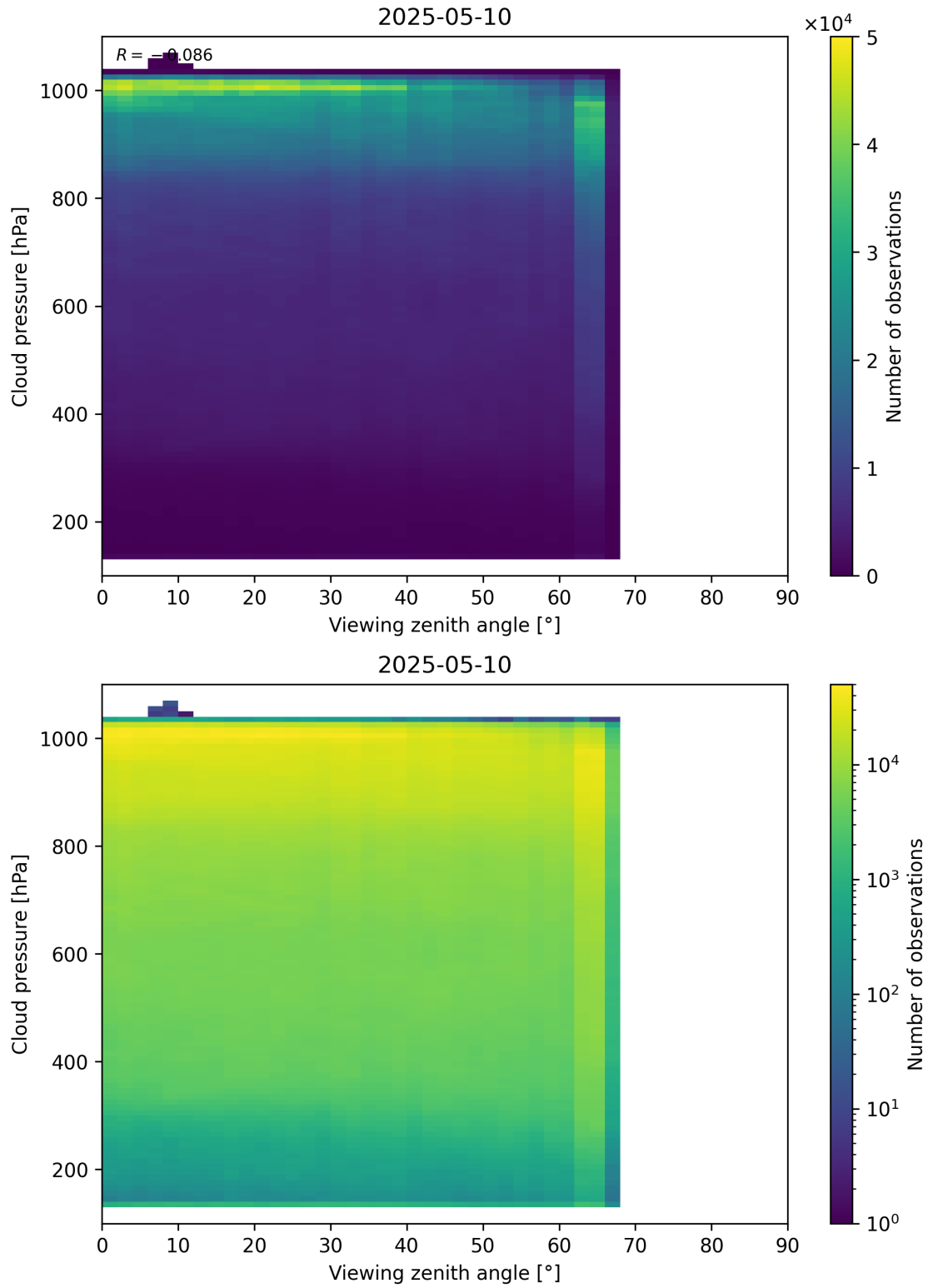
Figure 121: Scatter density plot of “Viewing zenith angle” against “Cloud pressure” for 2025-05-10 to 2025-05-11.
