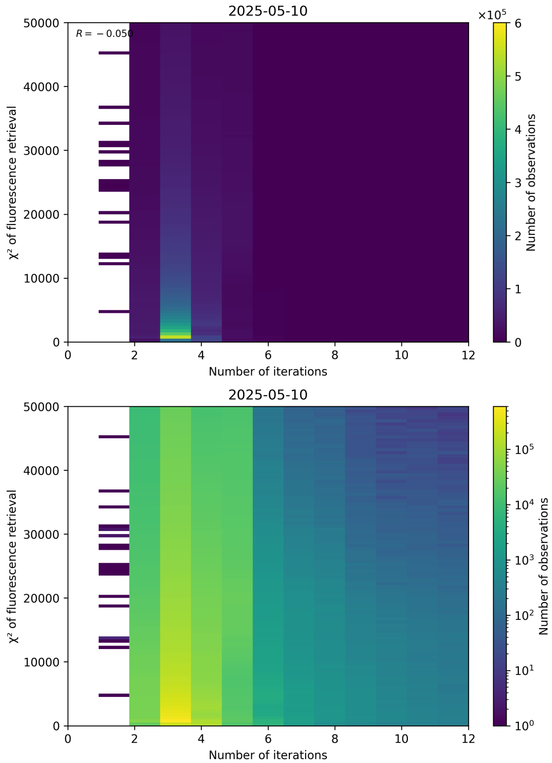
Figure 97: Scatter density plot of “Number of iterations” against “ \chi^2 of fluorescence retrieval” for 2025-05-10 to 2025-05-11.
