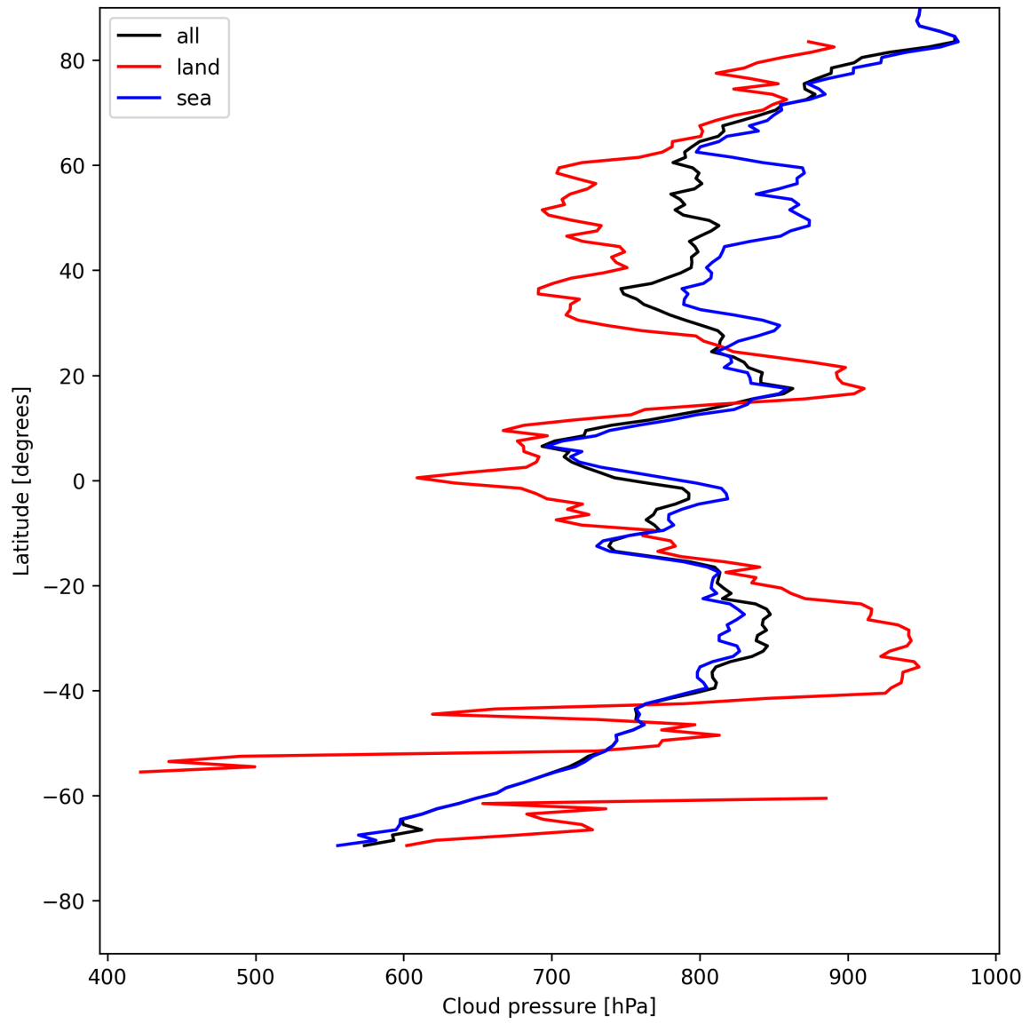
Figure 13: Zonal average of “Cloud pressure” for 2025-05-10 to 2025-05-11.
