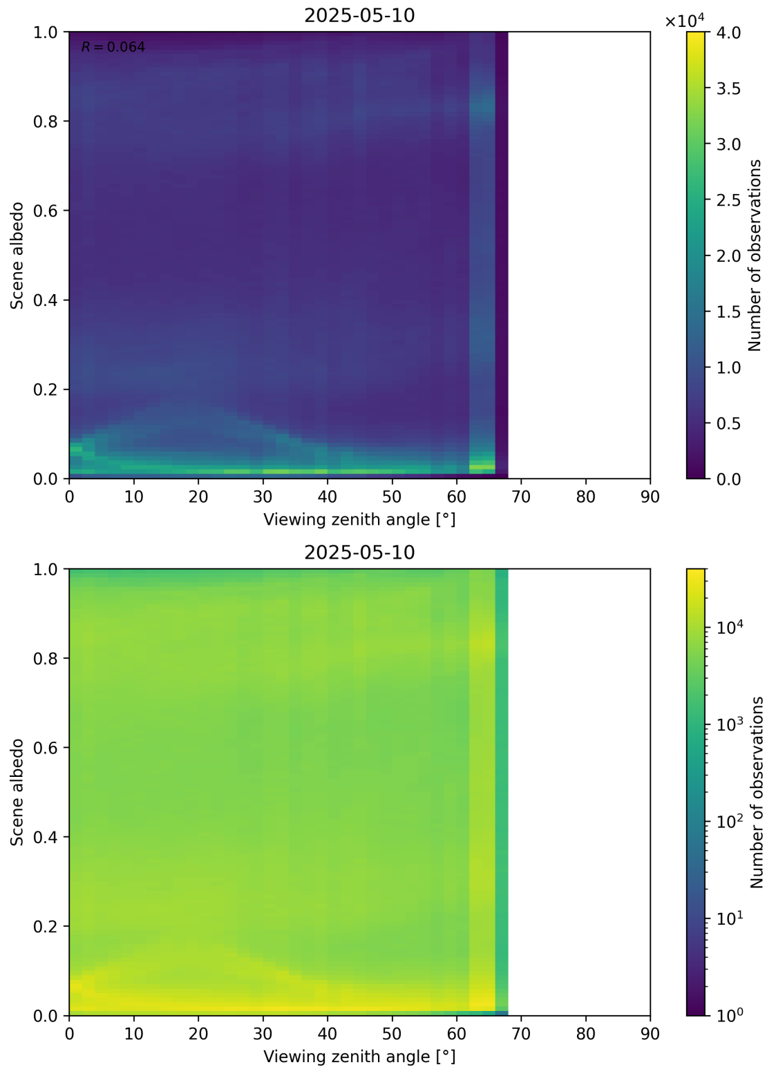
Figure 126: Scatter density plot of “Viewing zenith angle” against “Scene albedo” for 2025-05-10 to 2025-05-11.
