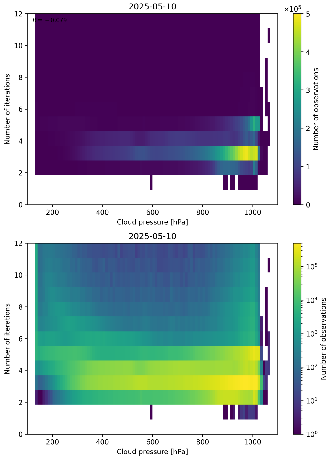
Figure 81: Scatter density plot of “Cloud pressure” against “Number of iterations” for 2025-05-10 to 2025-05-11.
