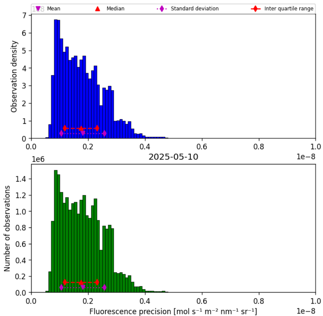
Figure 41: Histogram of “Fluorescence precision” for 2025-05-10 to 2025-05-11
