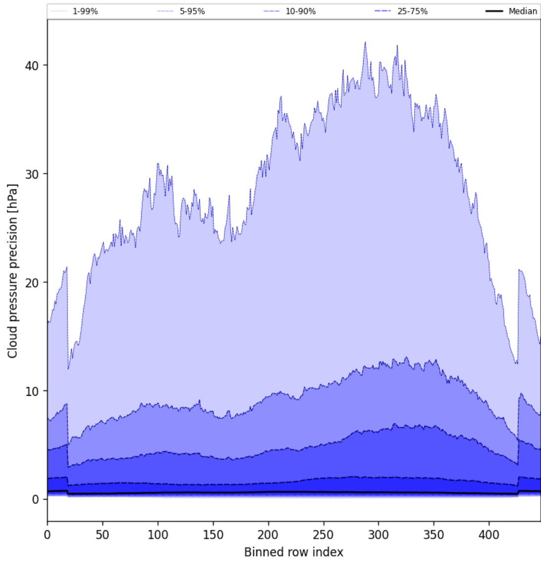
Figure 48: Along track statistics of “Cloud pressure precision” for 2025-05-10 to 2025-05-11
