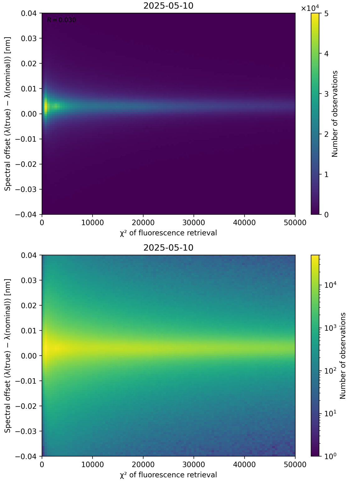
Figure 69: Scatter density plot of “ \chi^2 of fluorescence retrieval” against “Spectral offset ( \lambda_{\text{true}} - \lambda_{\text{nominal}} )” for 2025-05-10 to 2025-05-11.
