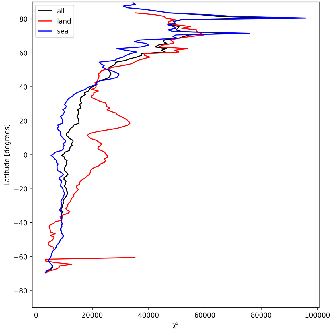
Figure 21: Zonal average of “ \chi^2 ” for 2025-05-10 to 2025-05-12.
