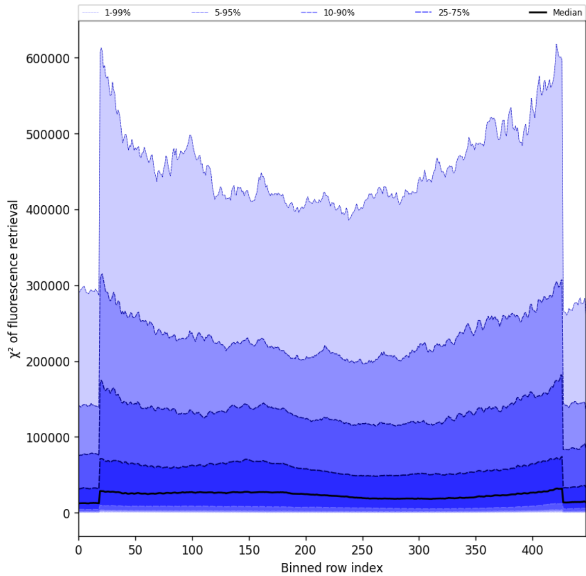
Figure 59: Along track statistics of “ \chi^2 of fluorescence retrieval” for 2025-05-10 to 2025-05-12
