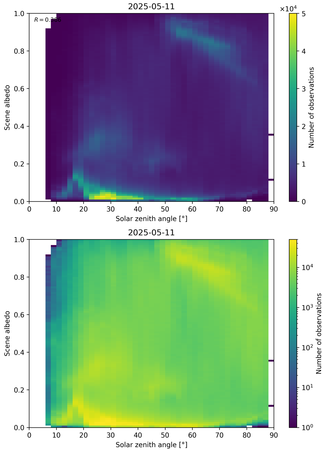
Figure 116: Scatter density plot of “Solar zenith angle” against “Scene albedo” for 2025-05-10 to 2025-05-12.
