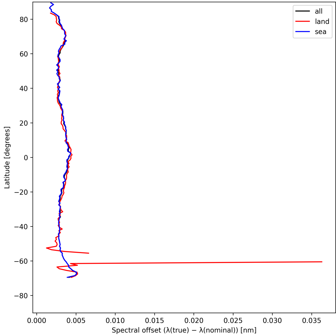
Figure 28: Zonal average of “Spectral offset ( \lambda_{\text{true}} - \lambda_{\text{nominal}} )” for 2025-05-10 to 2025-05-12.
