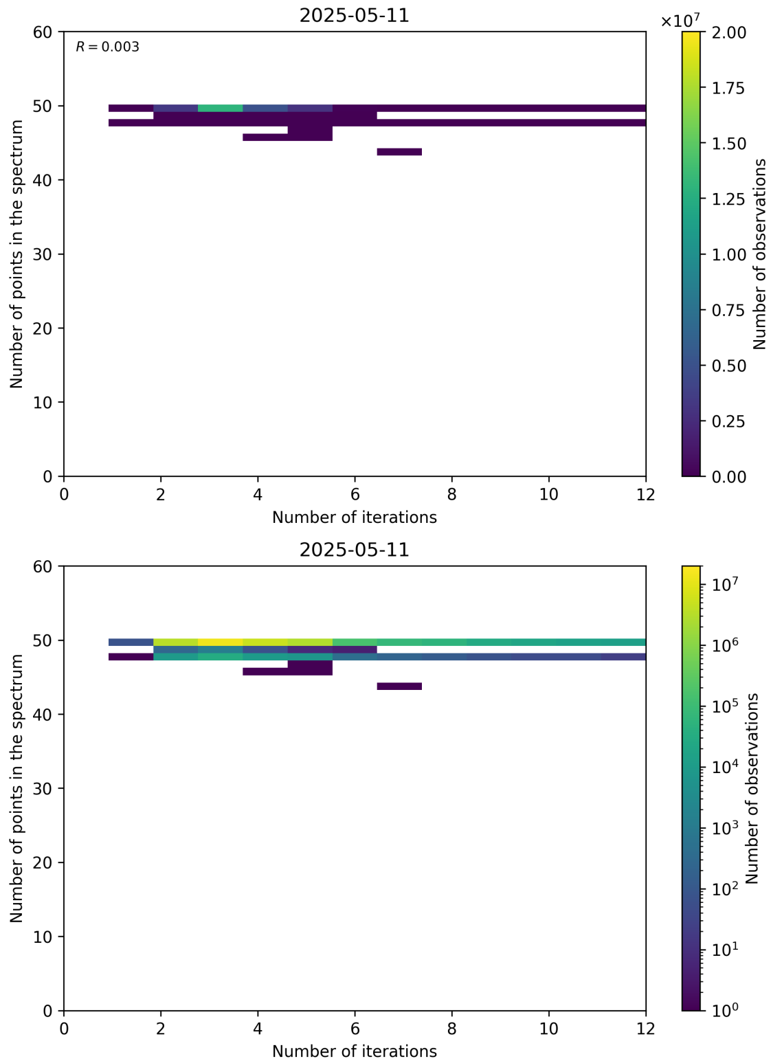
Figure 99: Scatter density plot of “Number of iterations” against “Number of points in the spectrum” for 2025-05-10 to 2025-05-12.
