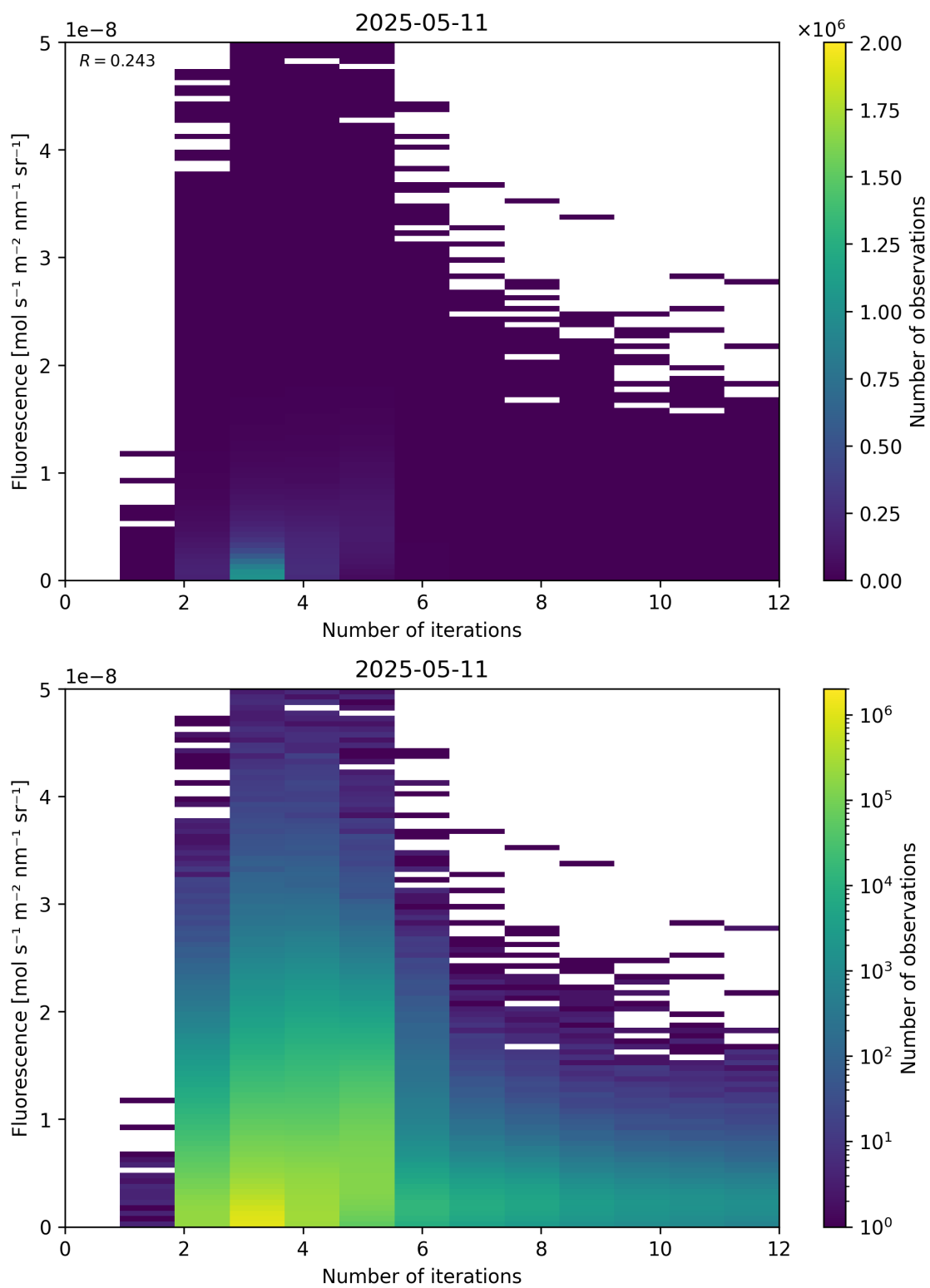
Figure 98: Scatter density plot of “Number of iterations” against “Fluorescence” for 2025-05-10 to 2025-05-12.
