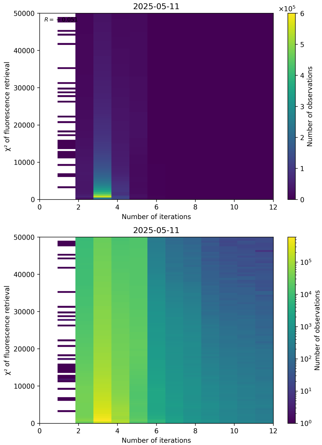
Figure 97: Scatter density plot of “Number of iterations” against “ \chi^2 of fluorescence retrieval” for 2025-05-10 to 2025-05-12.
