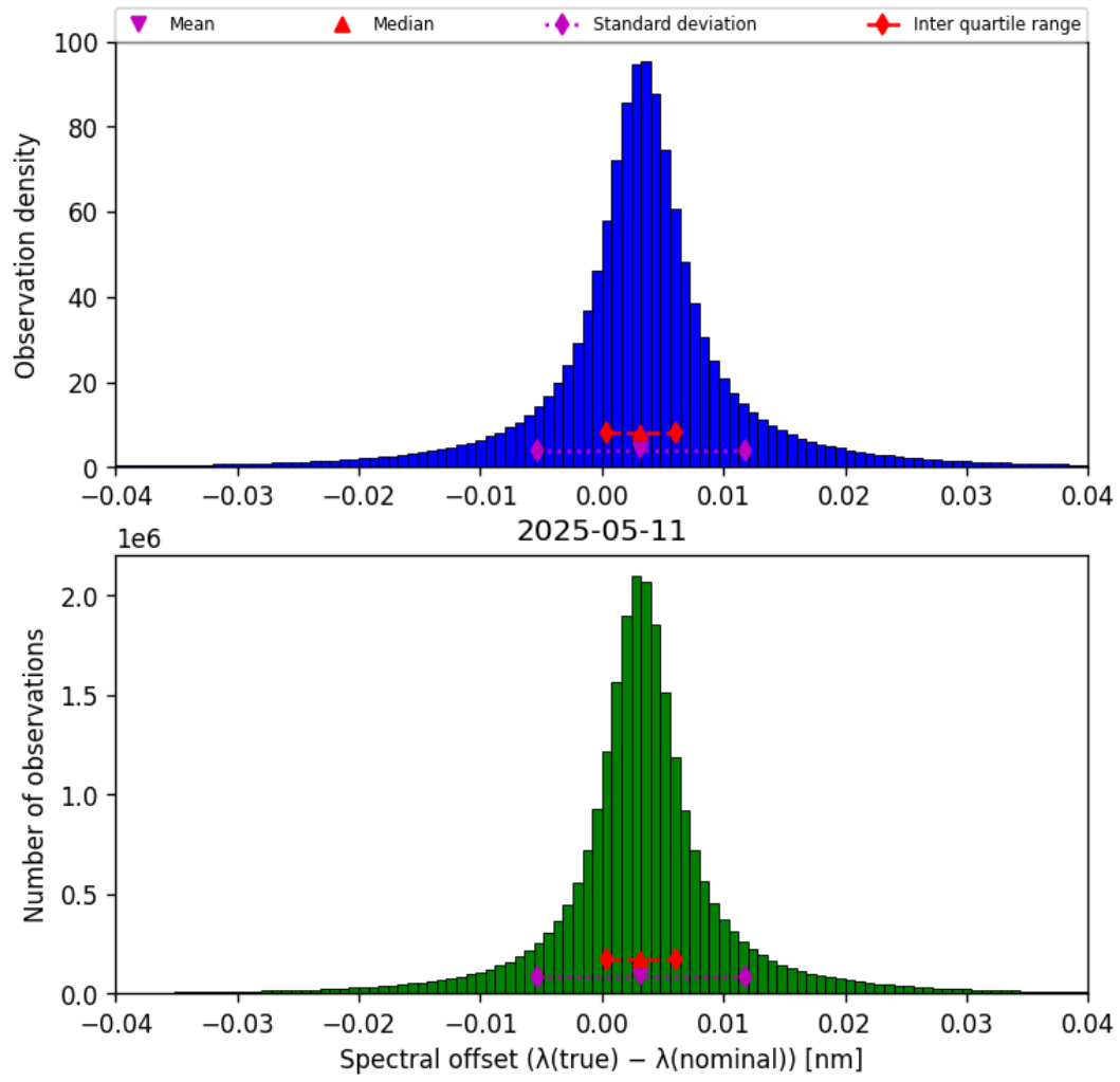
Figure 45: Histogram of “Spectral offset ( \lambda_{\text{true}} - \lambda_{\text{nominal}} )” for 2025-05-10 to 2025-05-12
