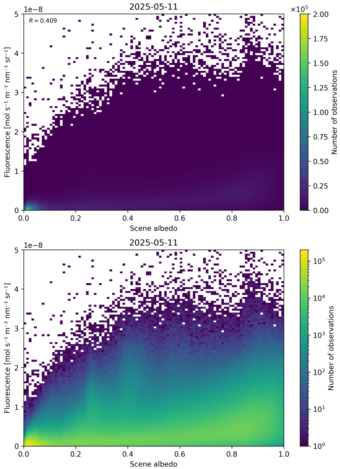
Figure 104: Scatter density plot of “Scene albedo” against “Fluorescence” for 2025-05-10 to 2025-05-12.
