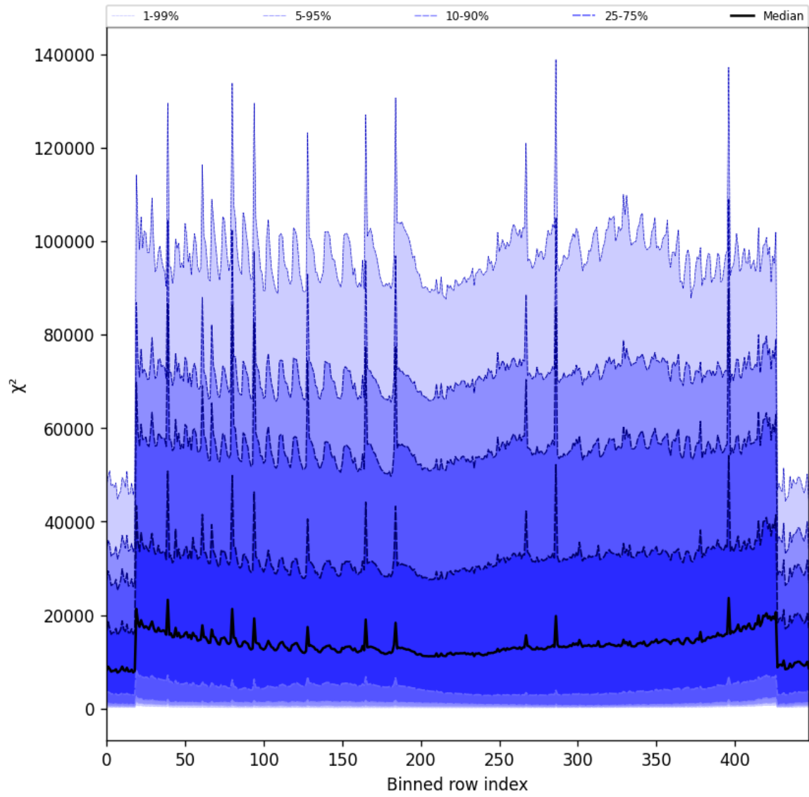
Figure 55: Along track statistics of “ \chi^2 ” for 2025-05-10 to 2025-05-12
