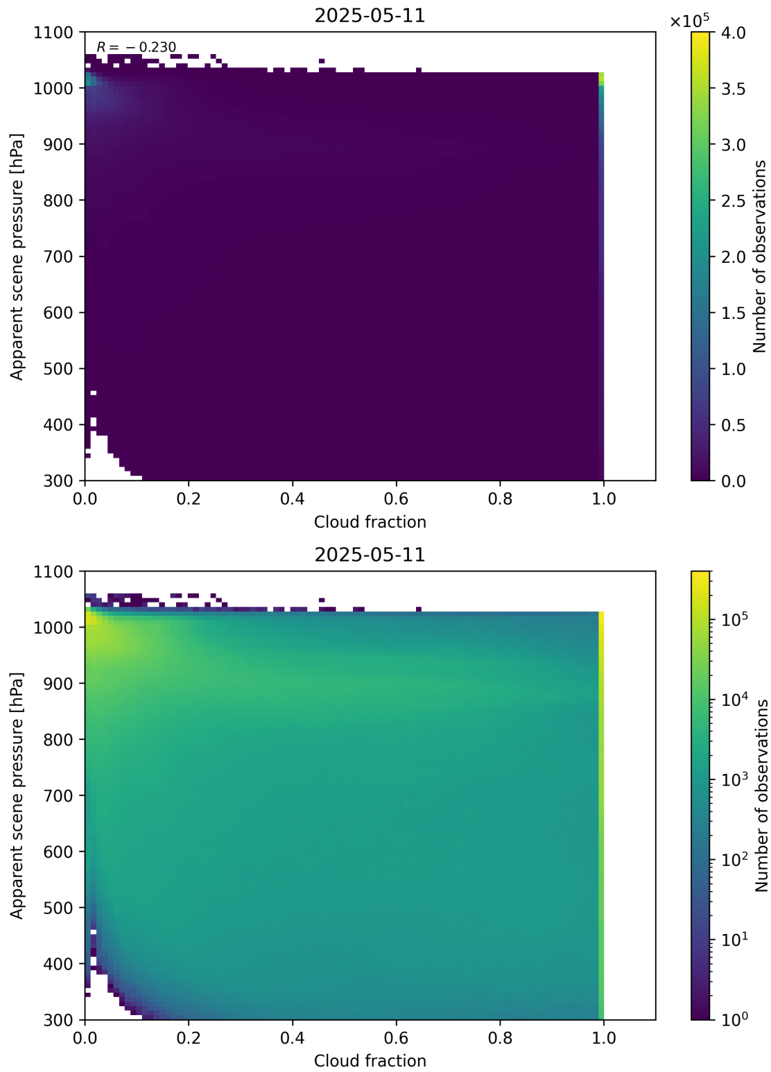
Figure 70: Scatter density plot of “Cloud fraction” against “Apparent scene pressure” for 2025-05-10 to 2025-05-12.
