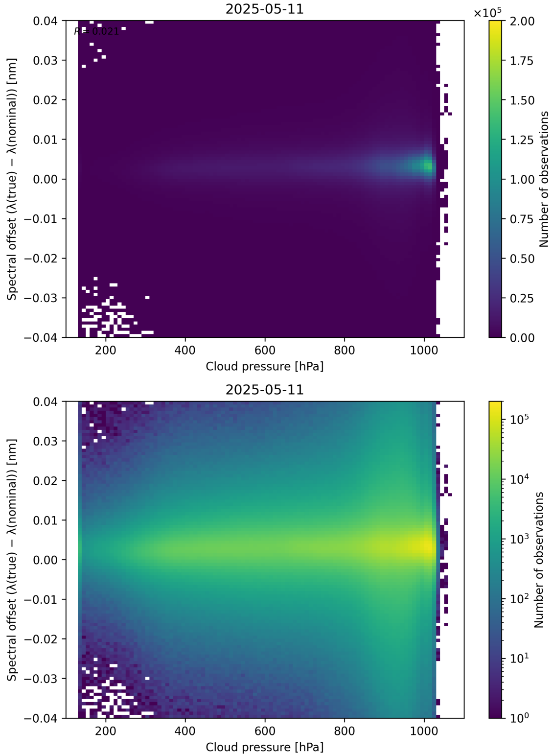
Figure 84: Scatter density plot of “Cloud pressure” against “Spectral offset ( \lambda_{\text{true}} - \lambda_{\text{nominal}} )” for 2025-05-10 to 2025-05-12.
