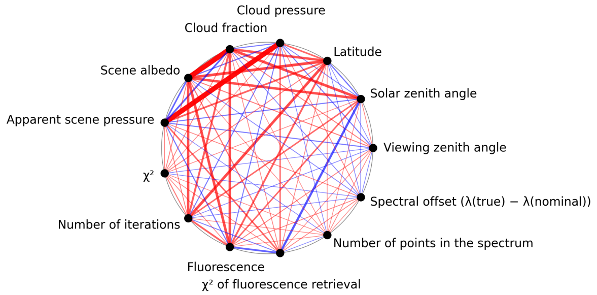
Figure 1: Map of correlation graph for 2025-05-10 to 2025-05-12.
