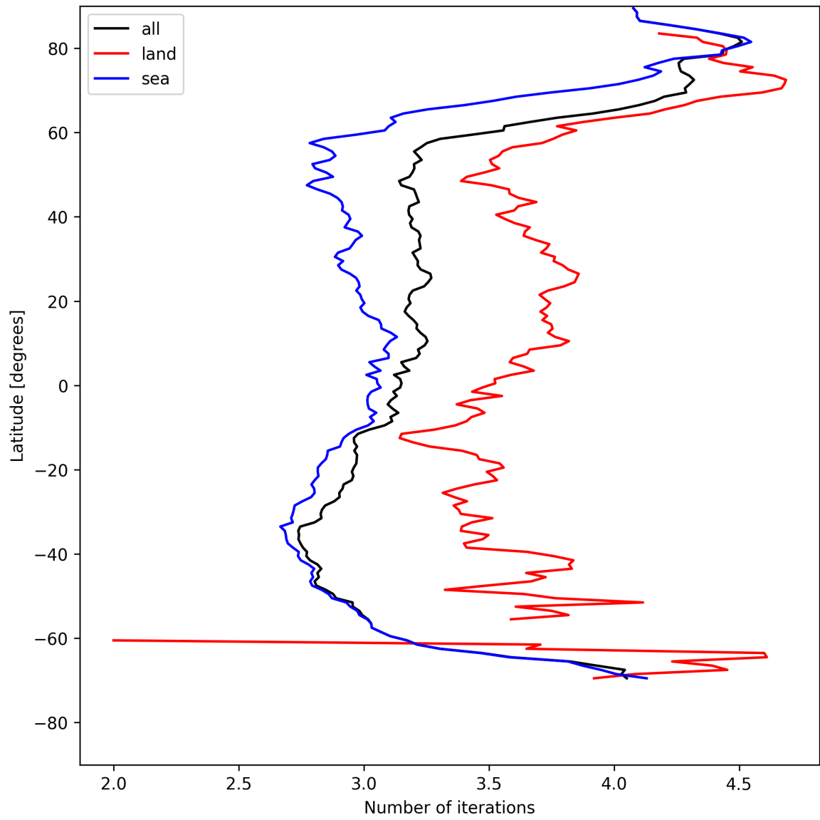
Figure 22: Zonal average of “Number of iterations” for 2025-05-10 to 2025-05-12.
