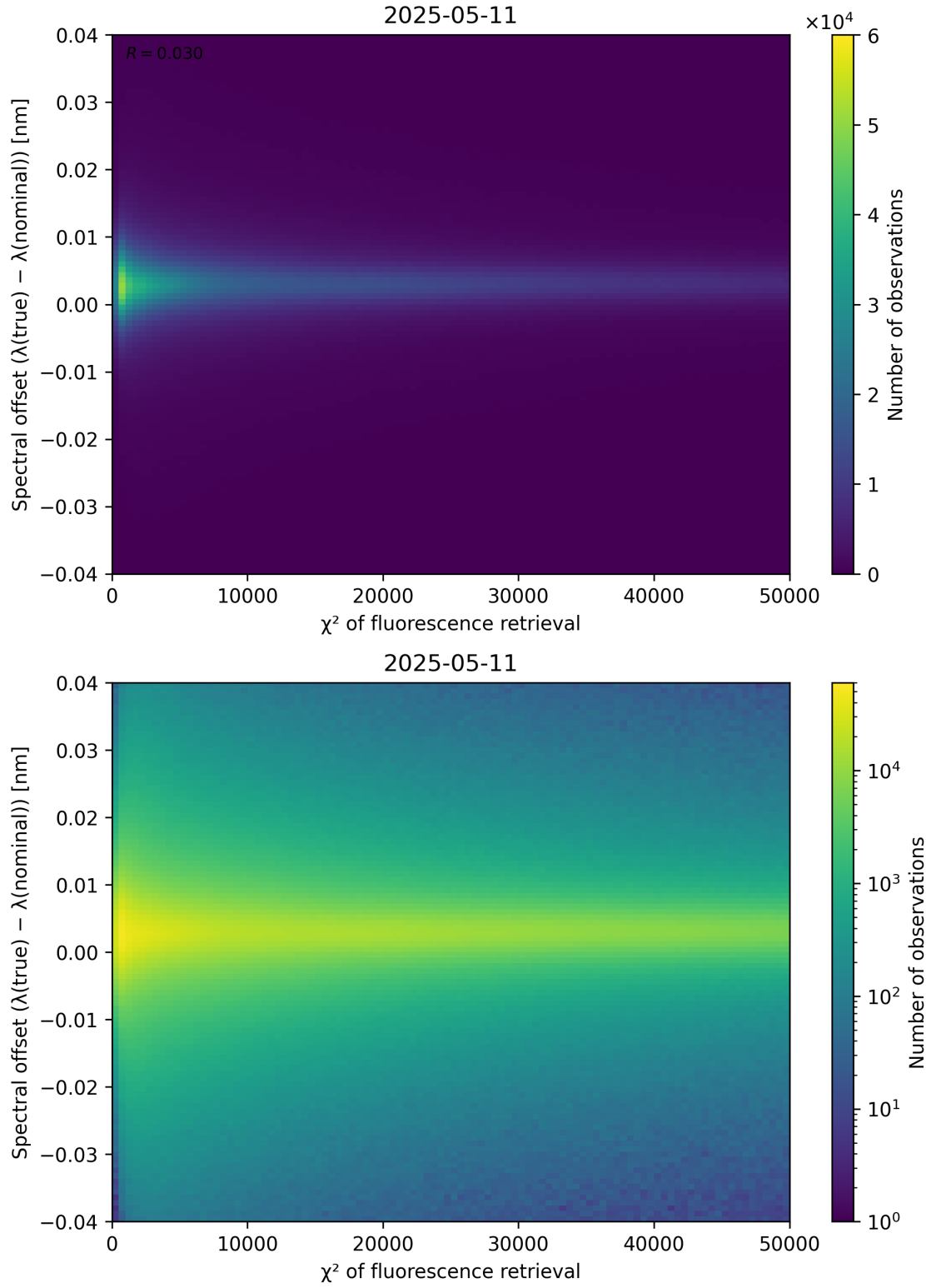
Figure 69: Scatter density plot of “ \chi^2 of fluorescence retrieval” against “Spectral offset ( \lambda_{\text{true}} - \lambda_{\text{nominal}} )” for 2025-05-10 to 2025-05-12.
