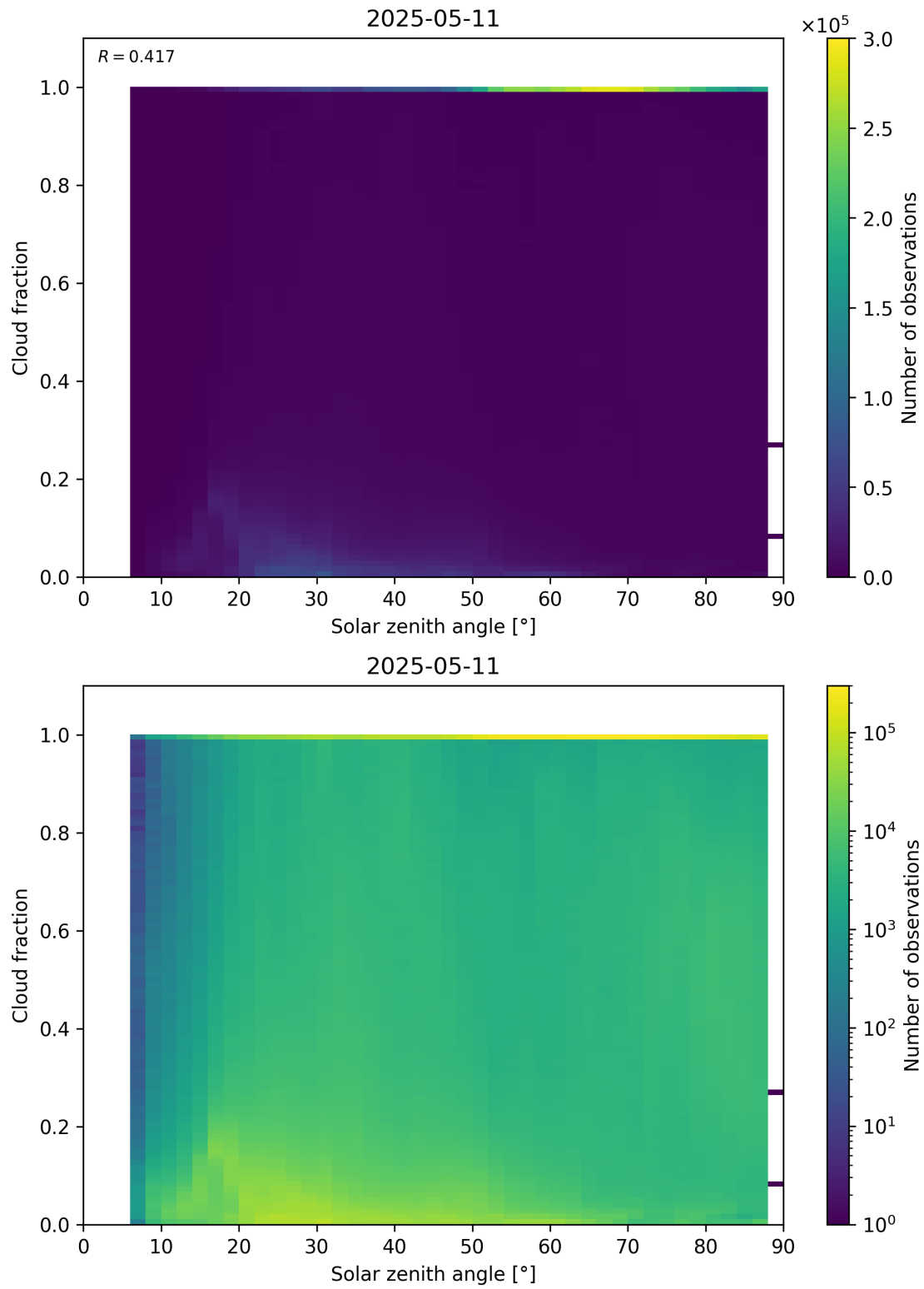
Figure 110: Scatter density plot of “Solar zenith angle” against “Cloud fraction” for 2025-05-10 to 2025-05-12.
