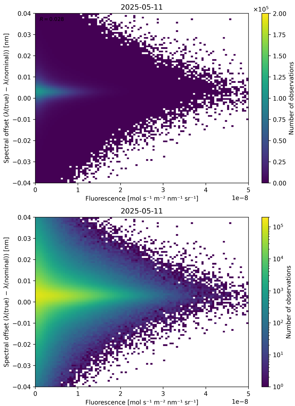
Figure 87: Scatter density plot of “Fluorescence” against “Spectral offset ( \lambda_{\text{true}} - \lambda_{\text{nominal}} )” for 2025-05-10 to 2025-05-12.
