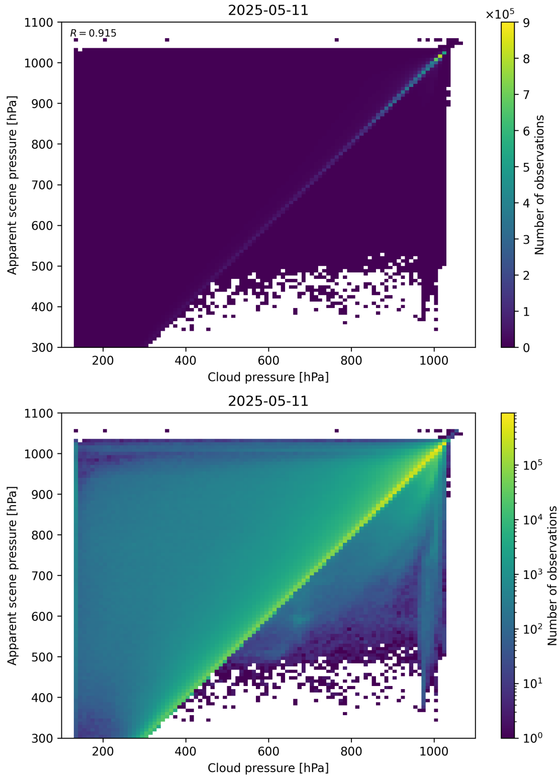
Figure 77: Scatter density plot of “Cloud pressure” against “Apparent scene pressure” for 2025-05-10 to 2025-05-12.
