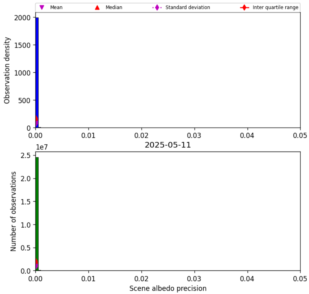
Figure 35: Histogram of “Scene albedo precision” for 2025-05-10 to 2025-05-12
