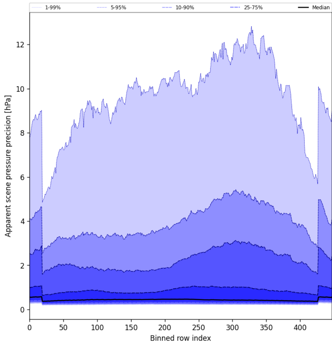
Figure 54: Along track statistics of “Apparent scene pressure precision” for 2025-05-10 to 2025-05-12
