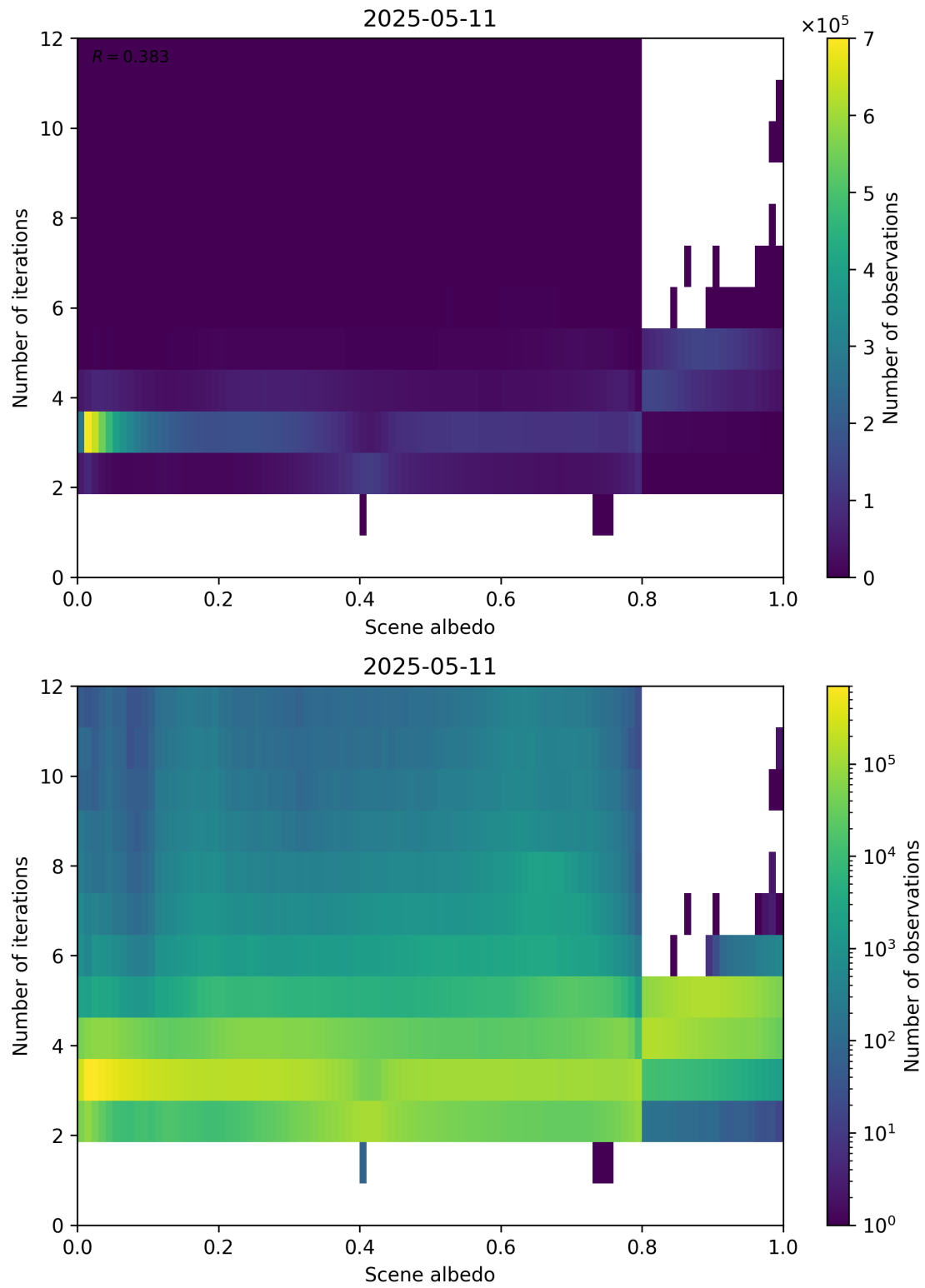
Figure 105: Scatter density plot of “Scene albedo” against “Number of iterations” for 2025-05-10 to 2025-05-12.
