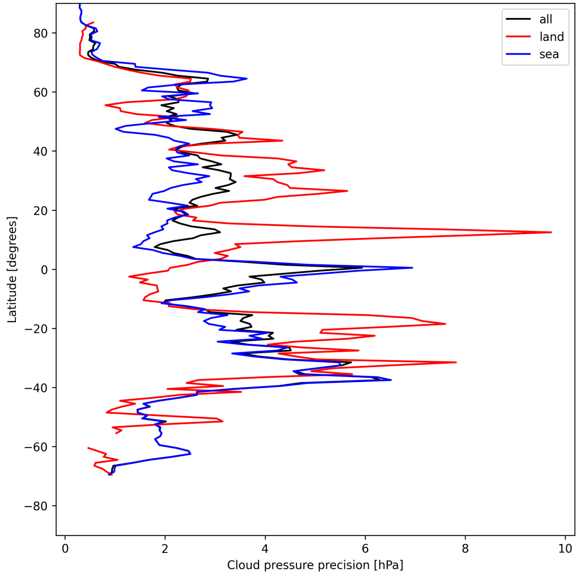
Figure 14: Zonal average of "Cloud pressure precision" for 2025-05-10 to 2025-05-12.
