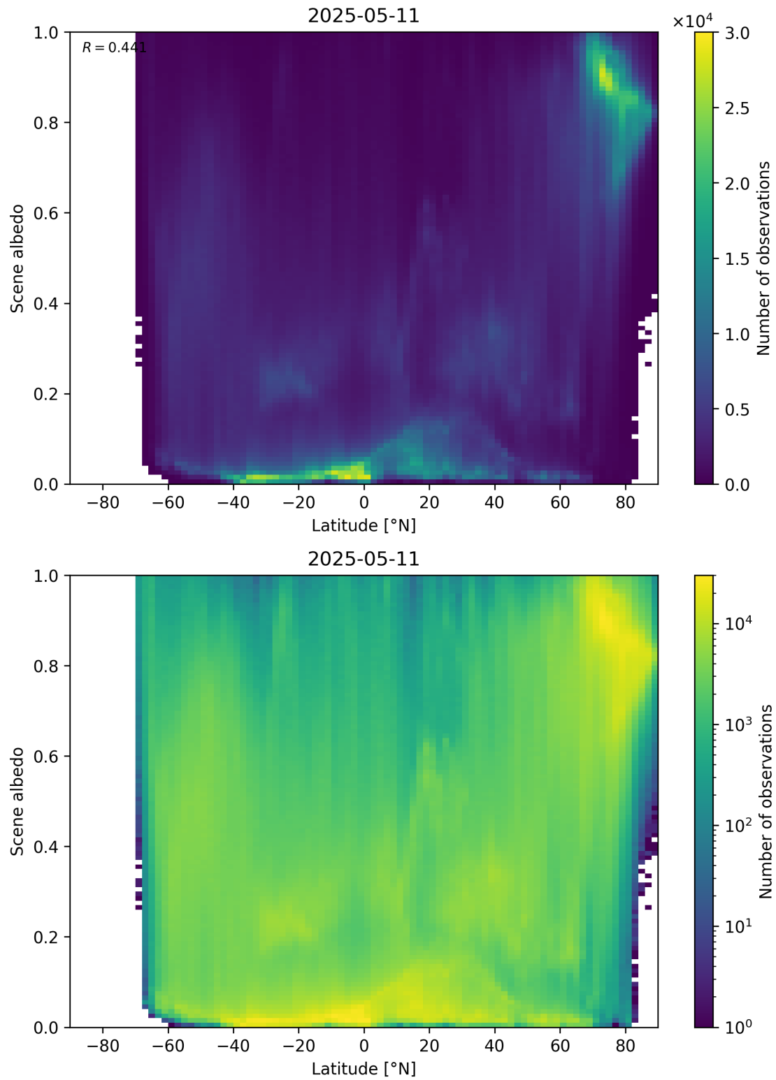
Figure 95: Scatter density plot of “Latitude” against “Scene albedo” for 2025-05-10 to 2025-05-12.
