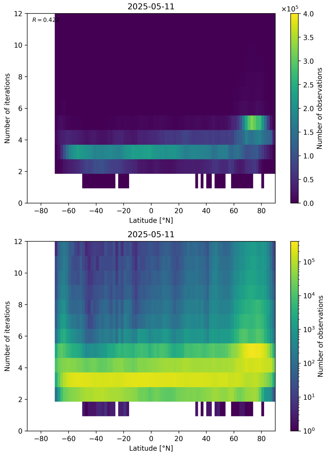
Figure 93: Scatter density plot of “Latitude” against “Number of iterations” for 2025-05-10 to 2025-05-12.
