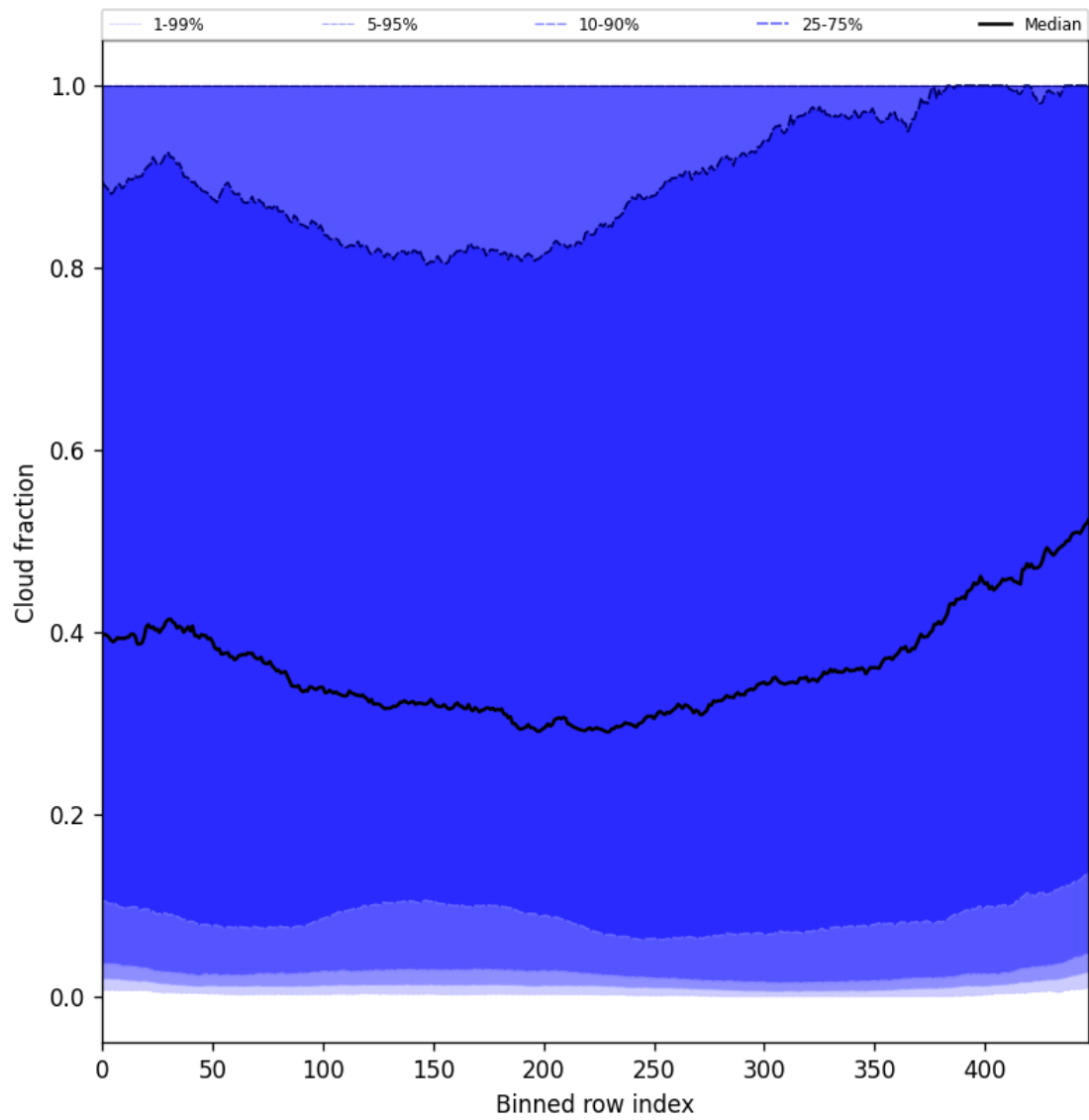
Figure 49: Along track statistics of “Cloud fraction” for 2025-05-10 to 2025-05-12
