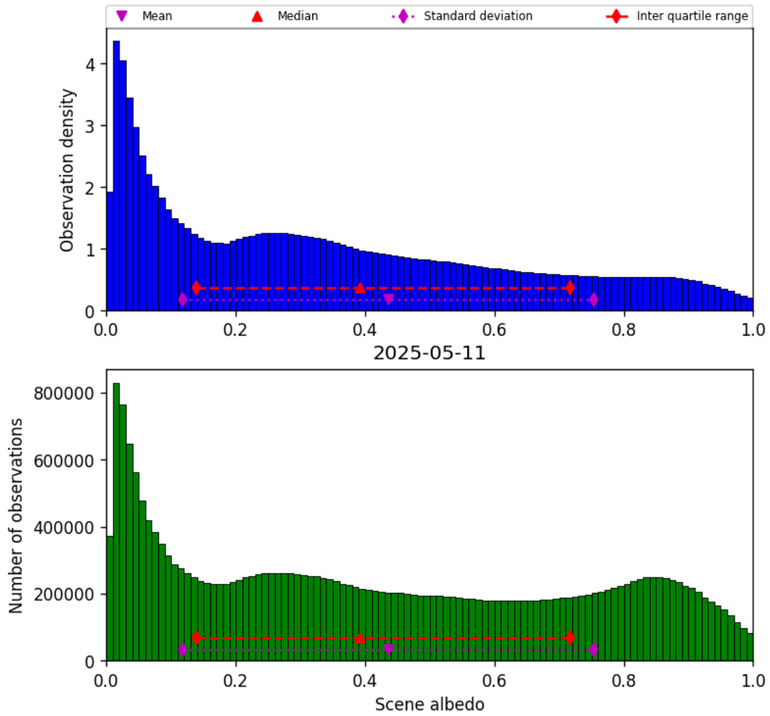
Figure 34: Histogram of “Scene albedo” for 2025-05-10 to 2025-05-12
