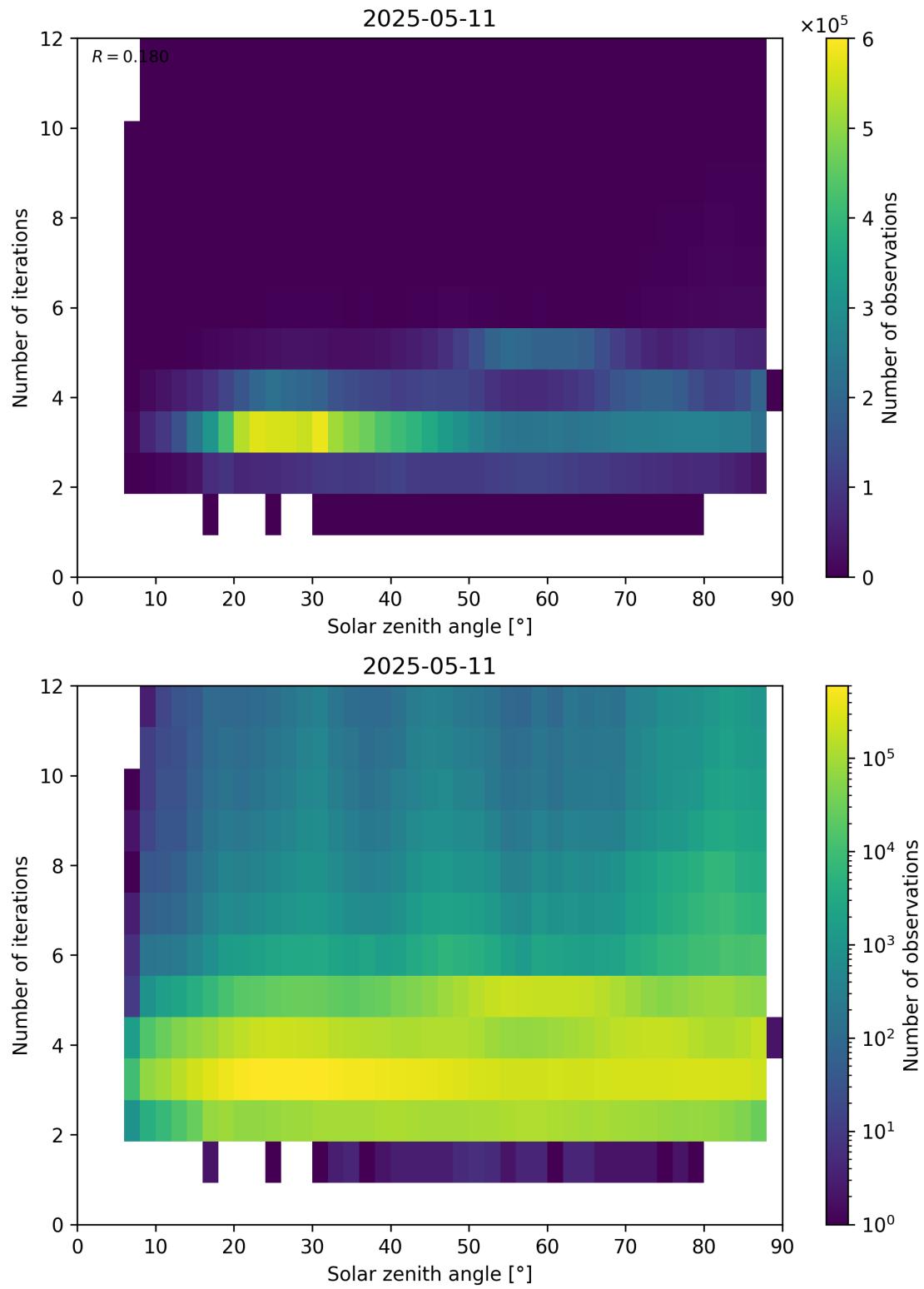
Figure 114: Scatter density plot of “Solar zenith angle” against “Number of iterations” for 2025-05-10 to 2025-05-12.
