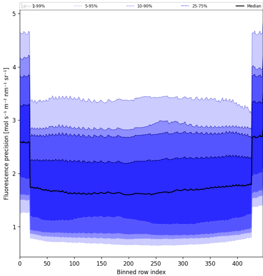
Figure 58: Along track statistics of “Fluorescence precision” for 2025-05-10 to 2025-05-12
