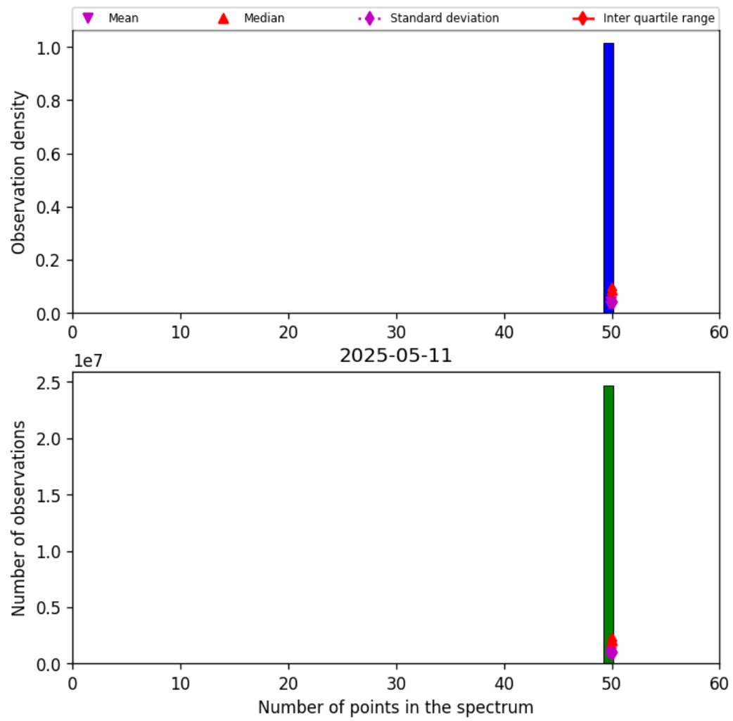
Figure 44: Histogram of “Number of points in the spectrum” for 2025-05-10 to 2025-05-12
