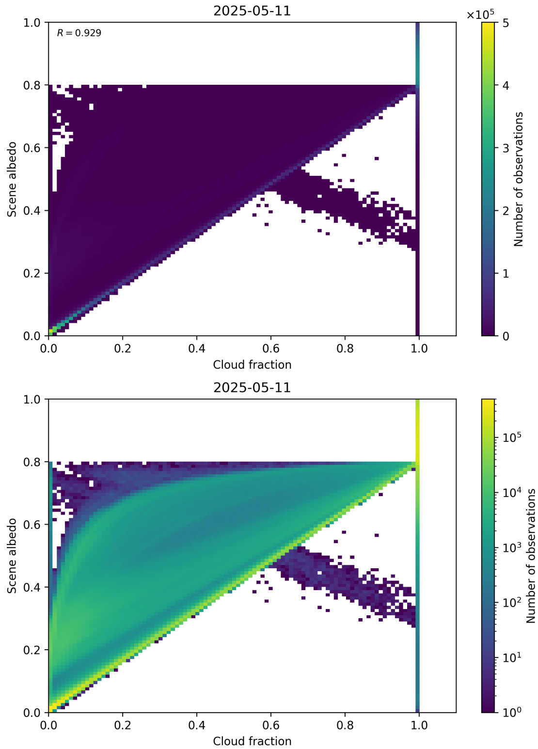
Figure 75: Scatter density plot of “Cloud fraction” against “Scene albedo” for 2025-05-10 to 2025-05-12.
