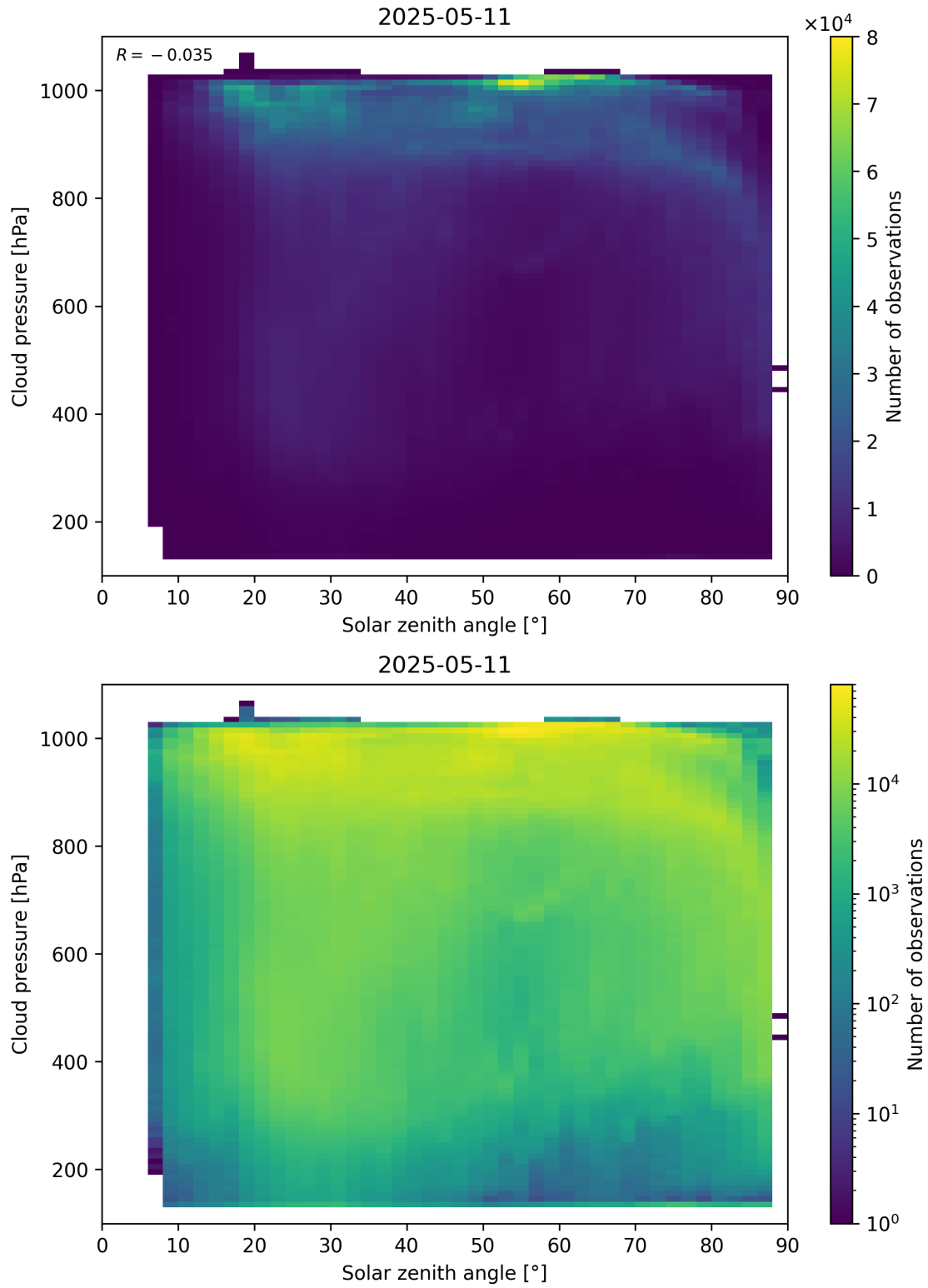
Figure 111: Scatter density plot of “Solar zenith angle” against “Cloud pressure” for 2025-05-10 to 2025-05-12.
