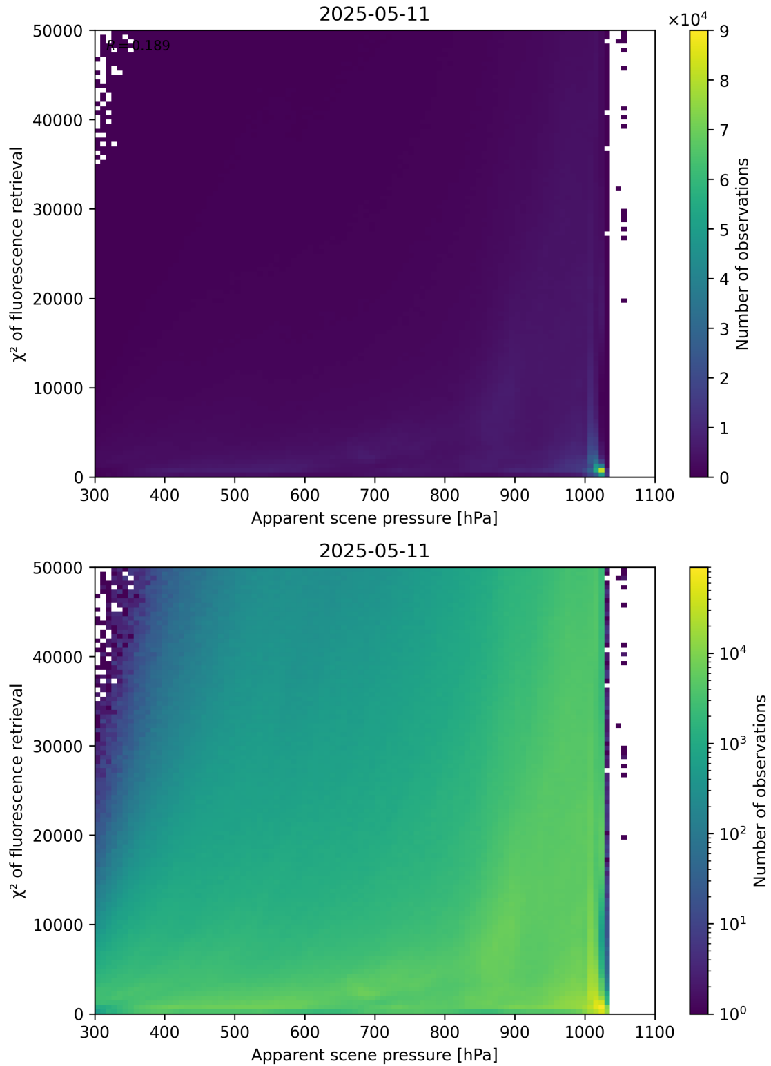
Figure 63: Scatter density plot of “Apparent scene pressure” against “ \chi^2 of fluorescence retrieval” for 2025-05-10 to 2025-05-12.
