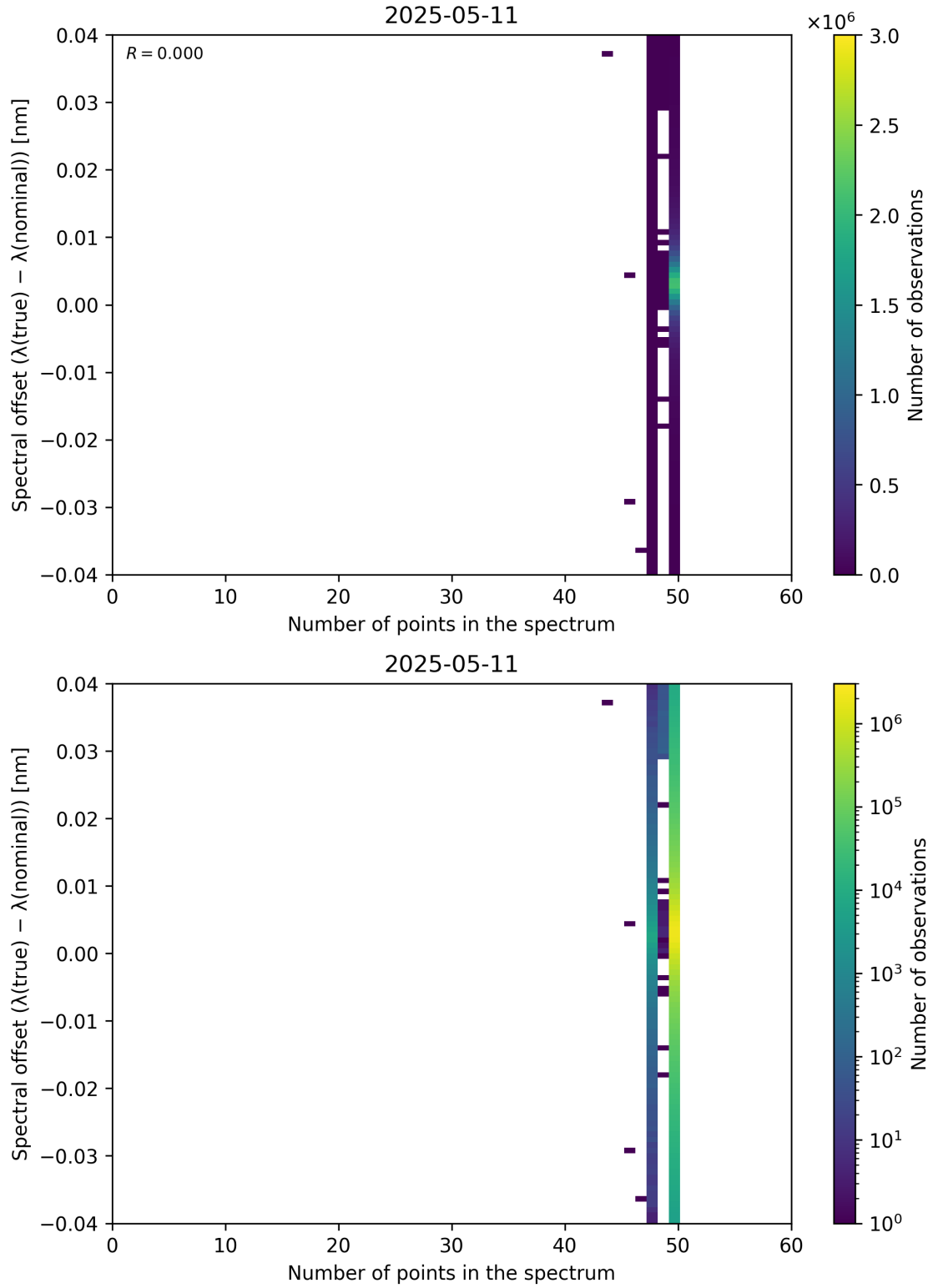
Figure 101: Scatter density plot of “Number of points in the spectrum” against “Spectral offset ( \lambda_{\text{true}} - \lambda_{\text{nominal}} )” for 2025-05-10 to 2025-05-12.
