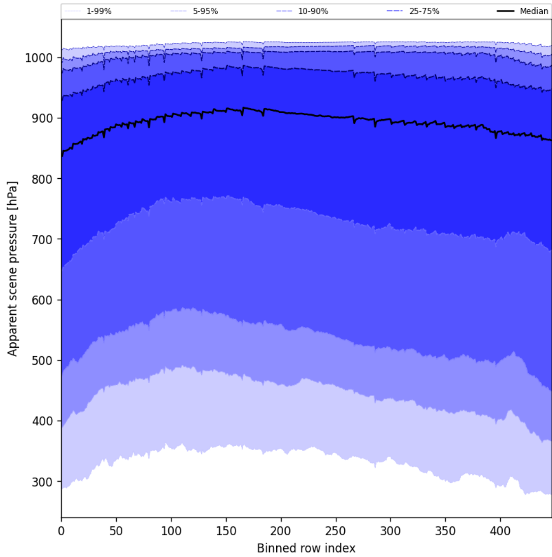
Figure 53: Along track statistics of “Apparent scene pressure” for 2025-05-10 to 2025-05-12
