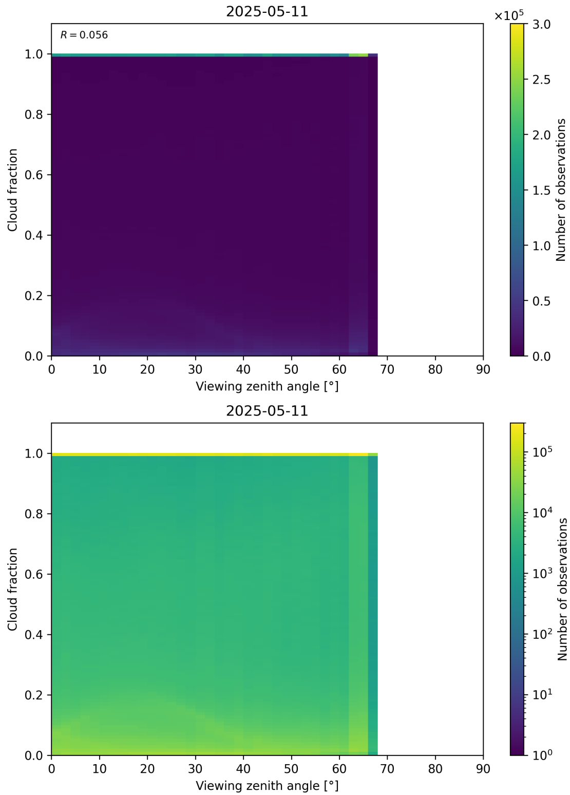
Figure 120: Scatter density plot of “Viewing zenith angle” against “Cloud fraction” for 2025-05-10 to 2025-05-12.
