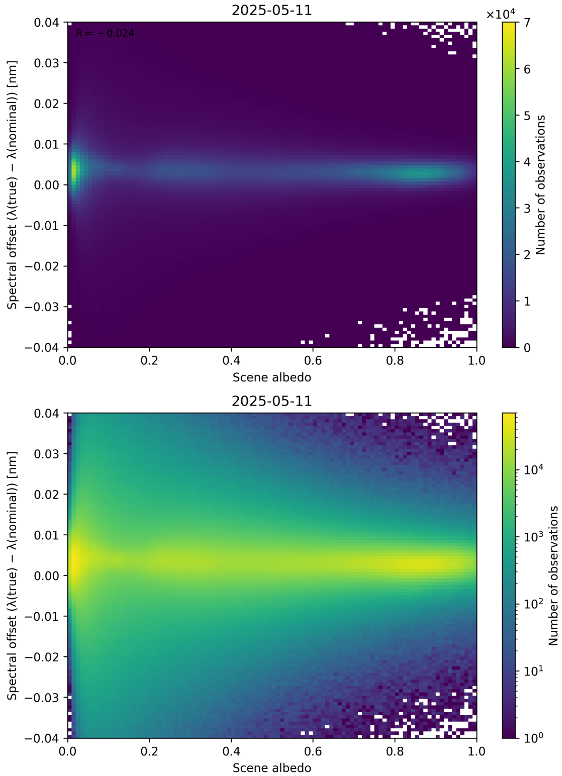
Figure 107: Scatter density plot of “Scene albedo” against “Spectral offset ( \lambda_{\text{true}} - \lambda_{\text{nominal}} )” for 2025-05-10 to 2025-05-12.
