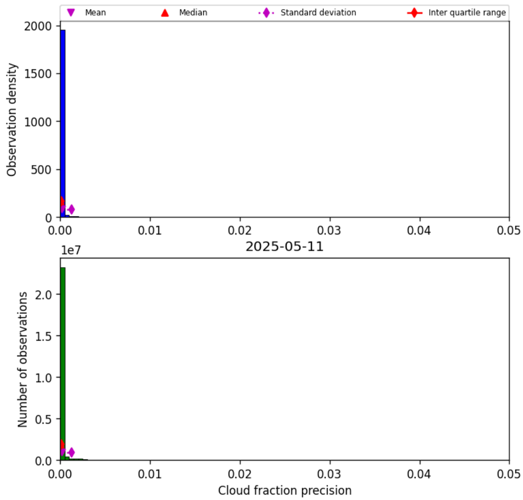
Figure 33: Histogram of “Cloud fraction precision” for 2025-05-10 to 2025-05-12
