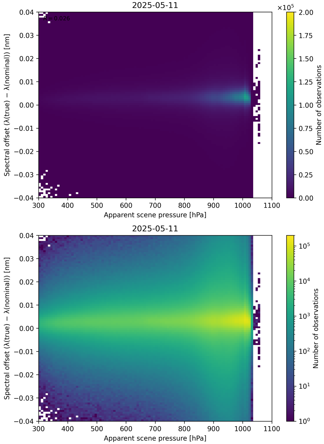
Figure 67: Scatter density plot of “Apparent scene pressure” against “Spectral offset ( \lambda_{\text{true}} - \lambda_{\text{nominal}} )” for 2025-05-10 to 2025-05-12.
