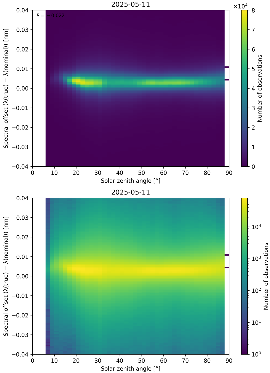
Figure 117: Scatter density plot of “Solar zenith angle” against “Spectral offset ( \lambda_{\text{true}} - \lambda_{\text{nominal}} )” for 2025-05-10 to 2025-05-12.
