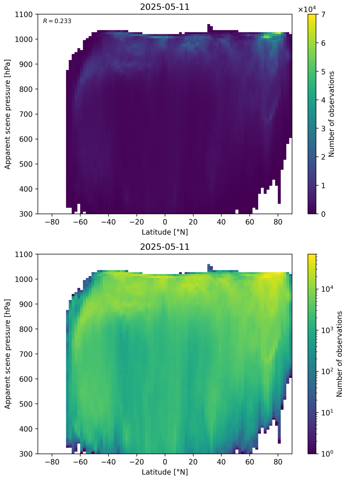
Figure 88: Scatter density plot of “Latitude” against “Apparent scene pressure” for 2025-05-10 to 2025-05-12.
