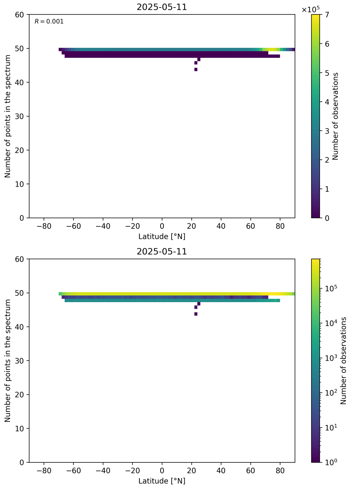
Figure 94: Scatter density plot of “Latitude” against “Number of points in the spectrum” for 2025-05-10 to 2025-05-12.
