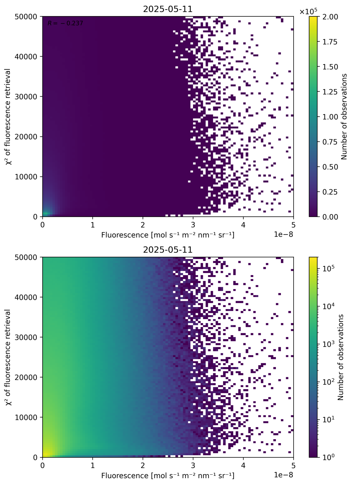
Figure 85: Scatter density plot of “Fluorescence” against “ \chi^2 of fluorescence retrieval” for 2025-05-10 to 2025-05-12.
