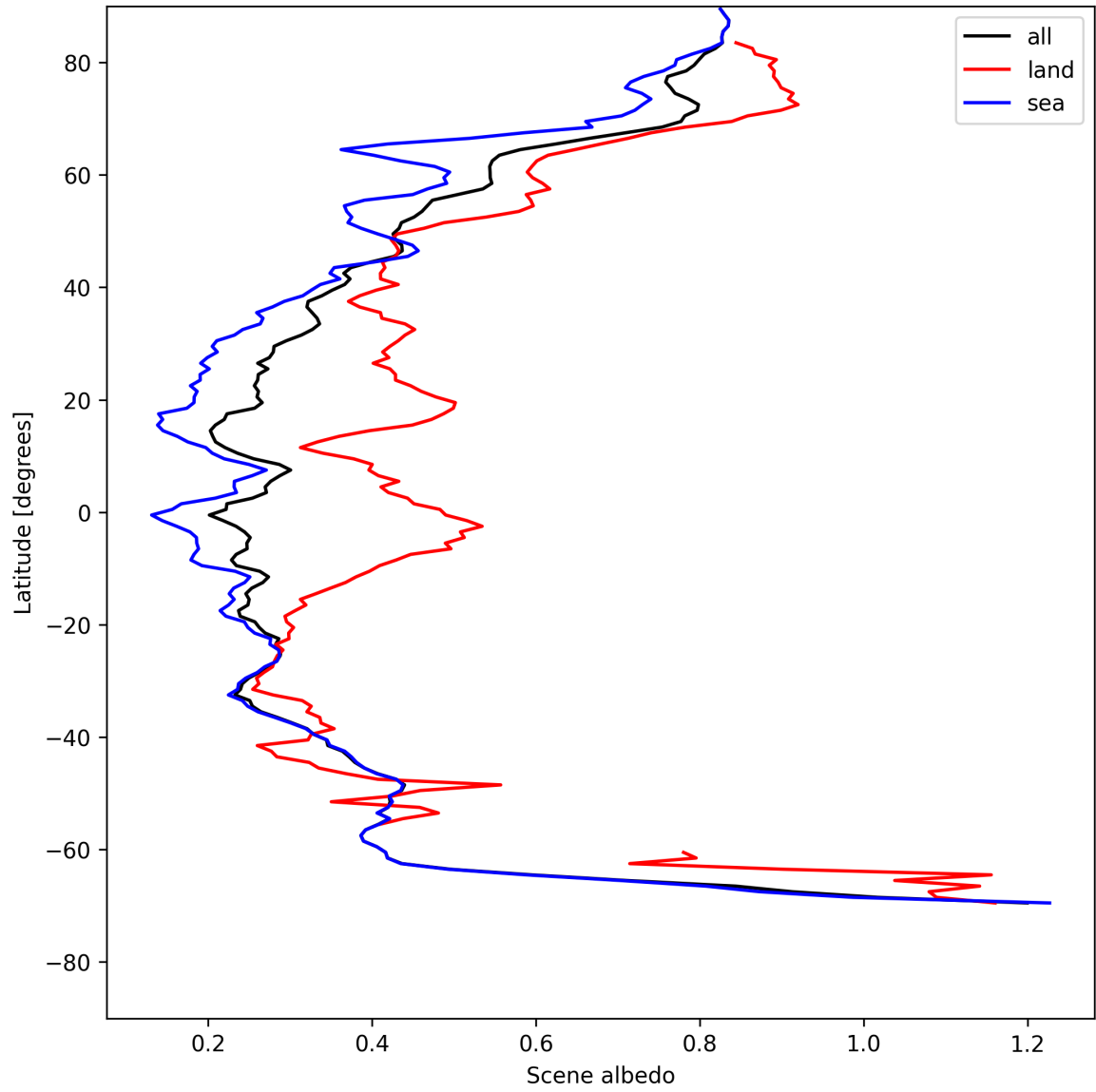
Figure 17: Zonal average of "Scene albedo" for 2025-05-10 to 2025-05-12.
