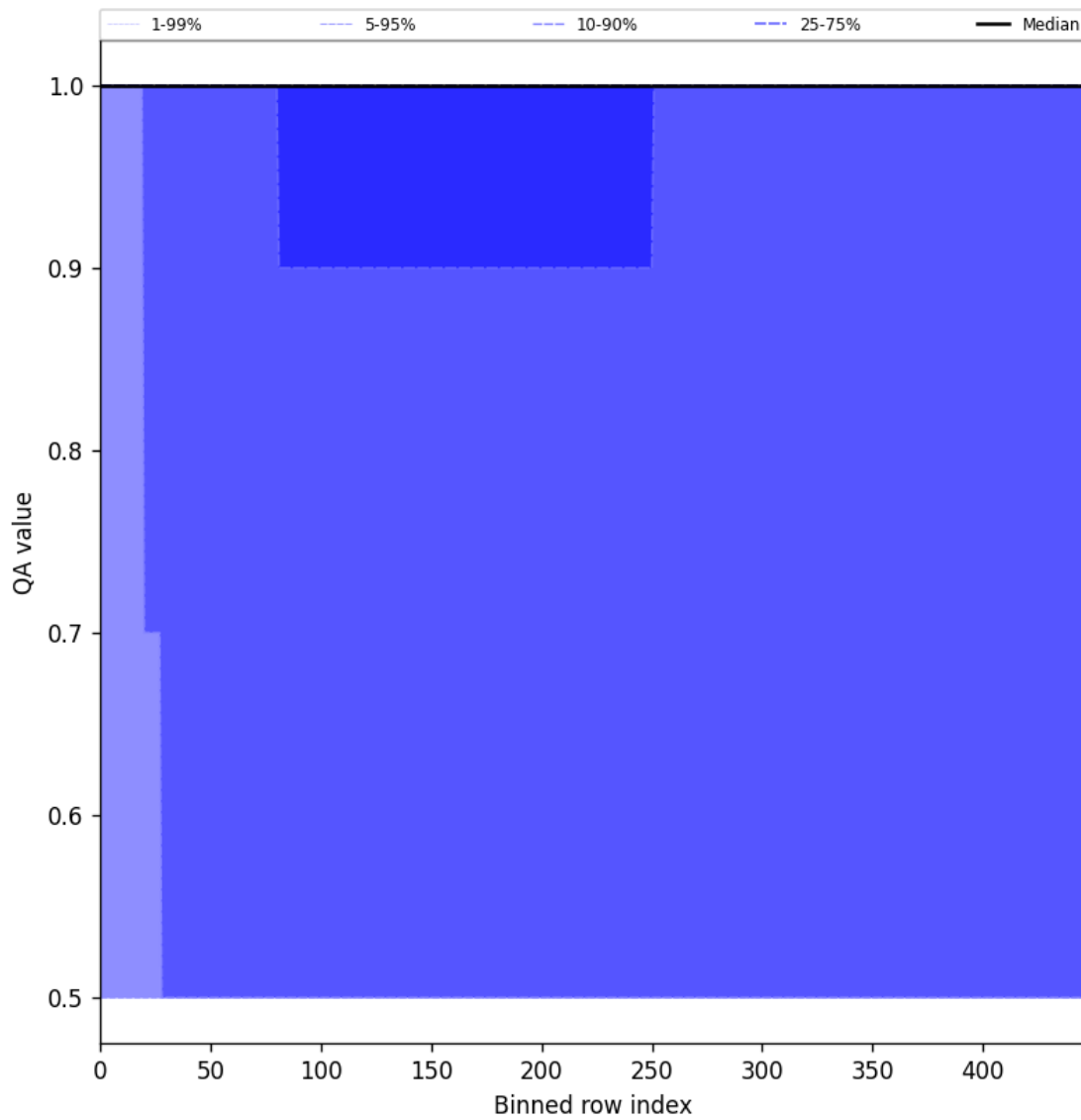
Figure 46: Along track statistics of “QA value” for 2025-05-10 to 2025-05-12
