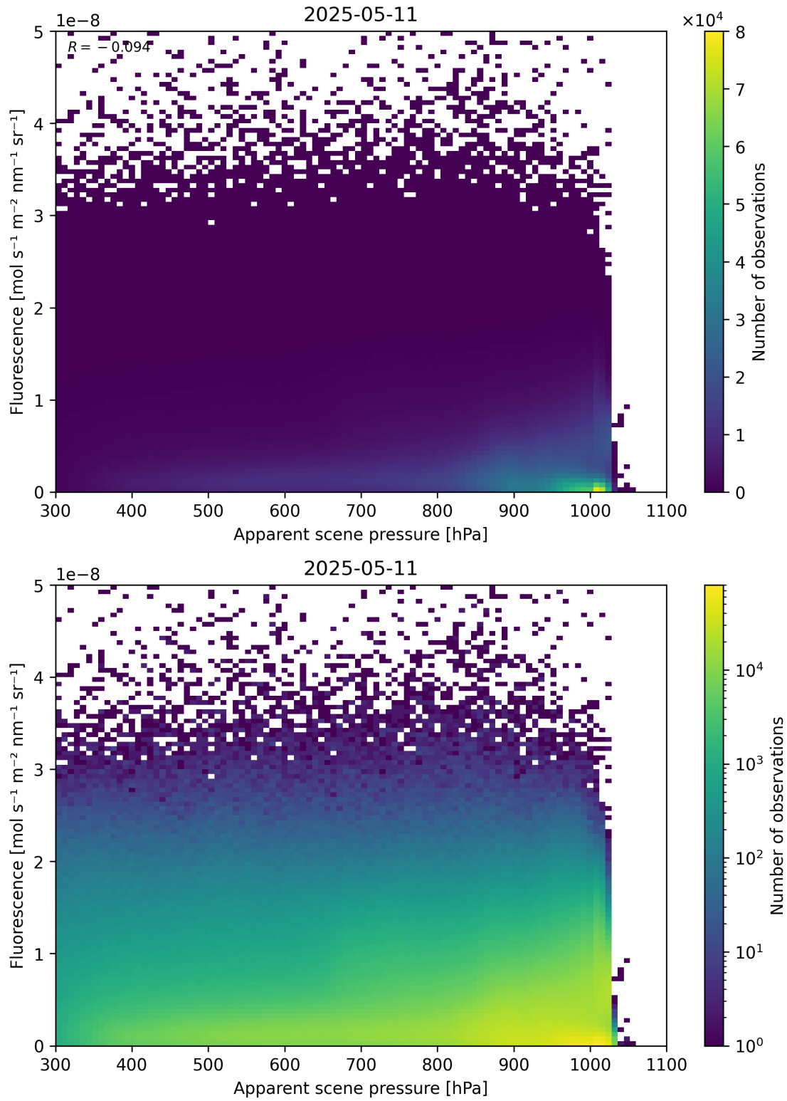
Figure 64: Scatter density plot of “Apparent scene pressure” against “Fluorescence” for 2025-05-10 to 2025-05-12.
