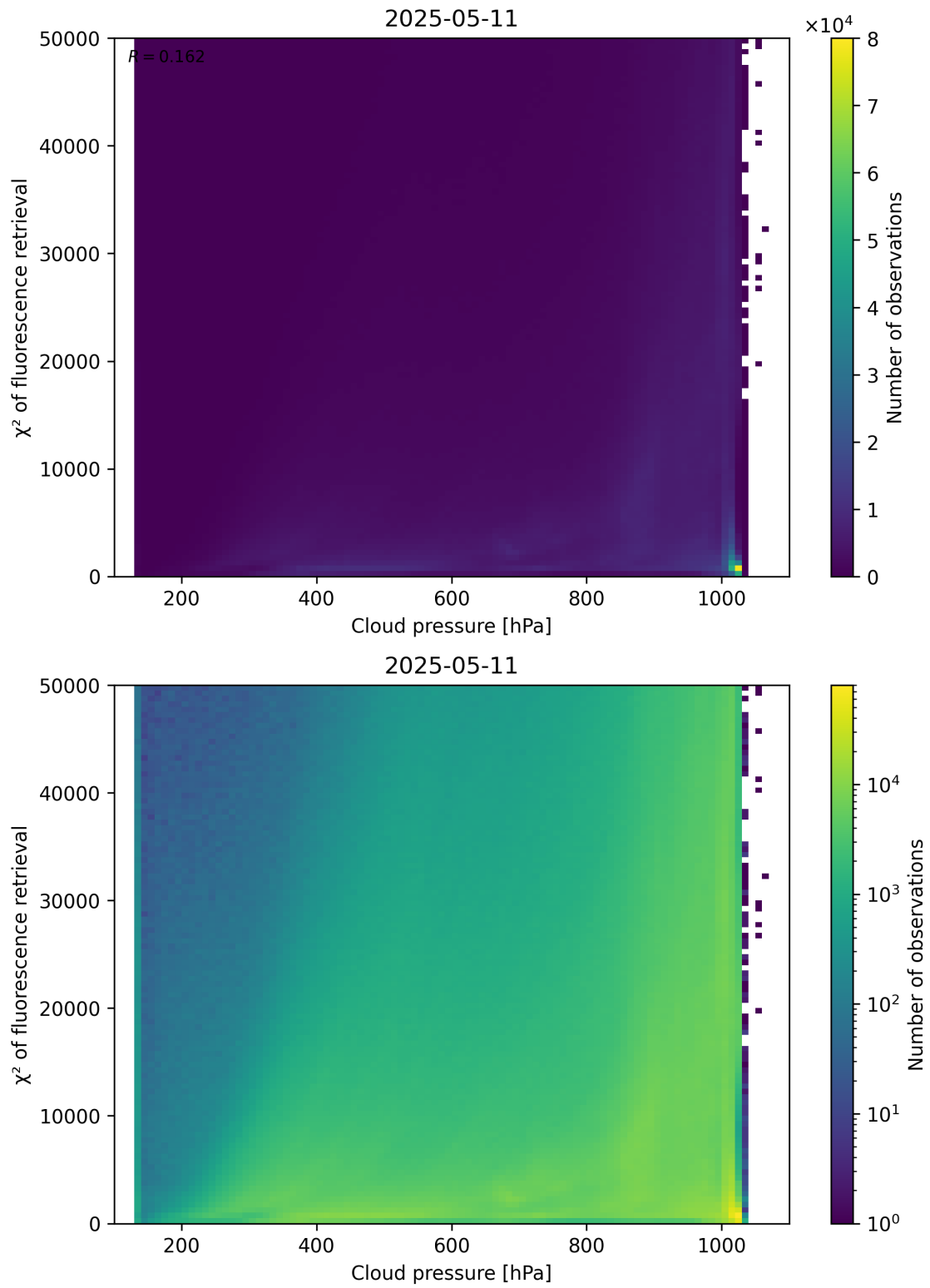
Figure 78: Scatter density plot of “Cloud pressure” against “ \chi^2 of fluorescence retrieval” for 2025-05-10 to 2025-05-12.
