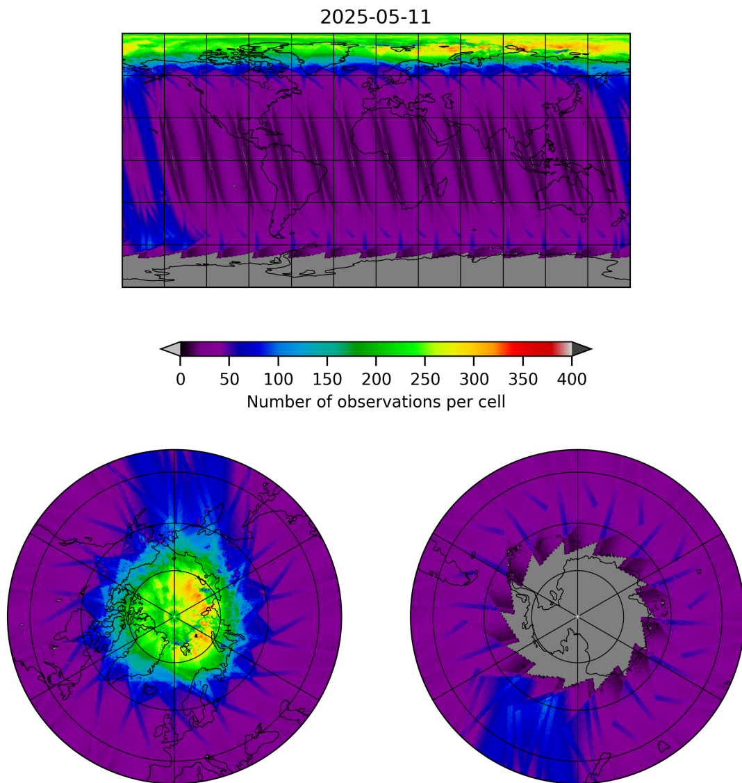
Figure 11: Map of the number of observations for 2025-05-10 to 2025-05-12
