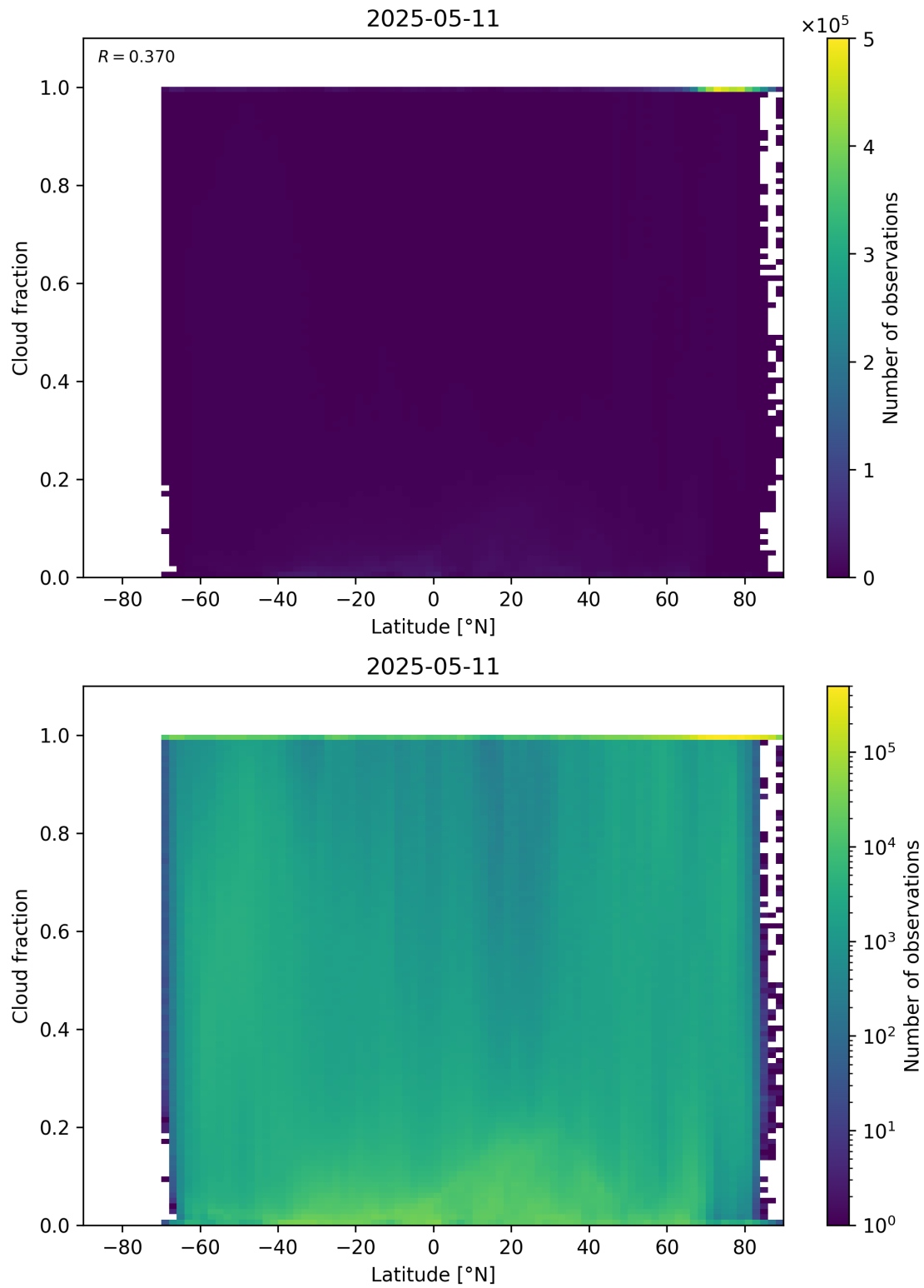
Figure 90: Scatter density plot of “Latitude” against “Cloud fraction” for 2025-05-10 to 2025-05-12.
