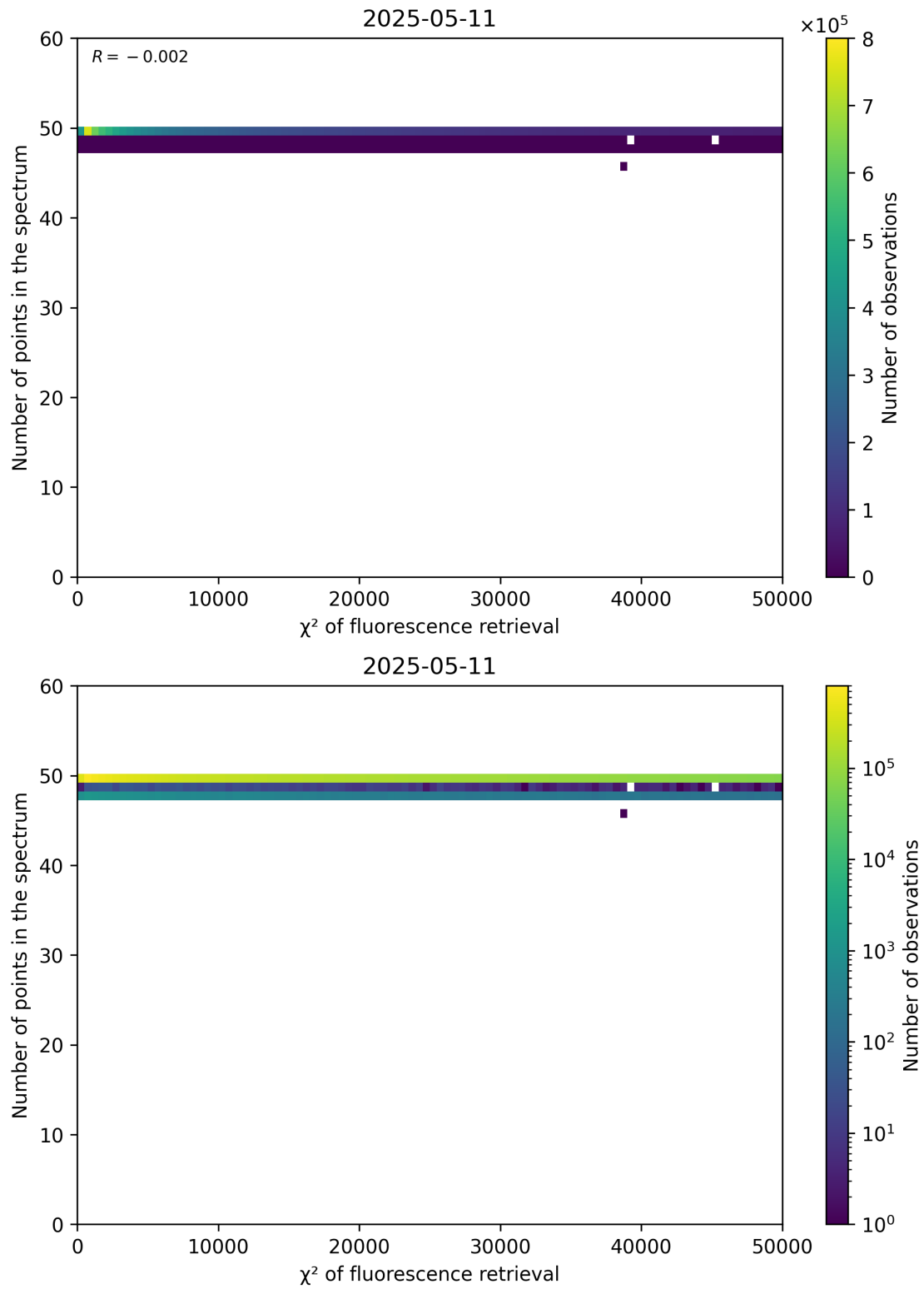
Figure 68: Scatter density plot of “ \chi^2 of fluorescence retrieval” against “Number of points in the spectrum” for 2025-05-10 to 2025-05-12.
