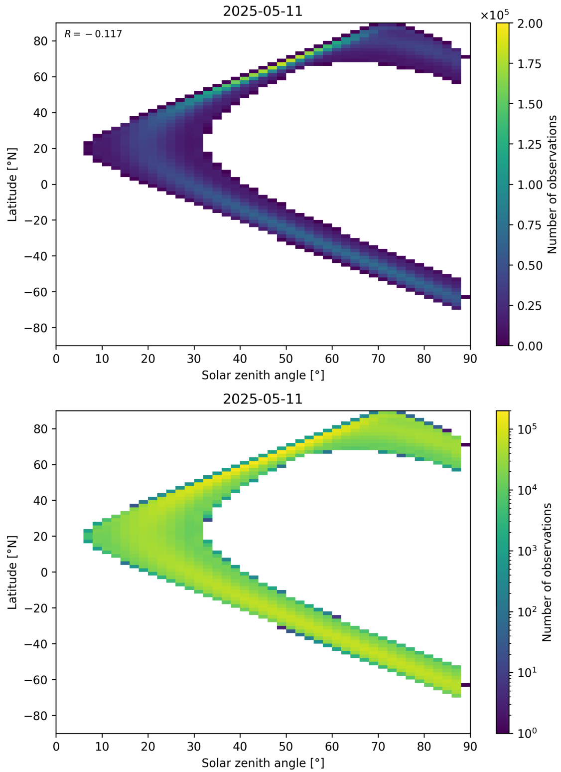
Figure 113: Scatter density plot of “Solar zenith angle” against “Latitude” for 2025-05-10 to 2025-05-12.
