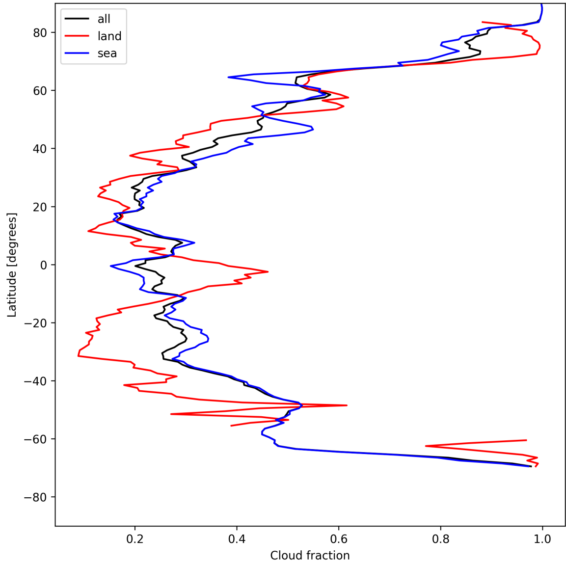
Figure 15: Zonal average of “Cloud fraction” for 2025-05-10 to 2025-05-12.
