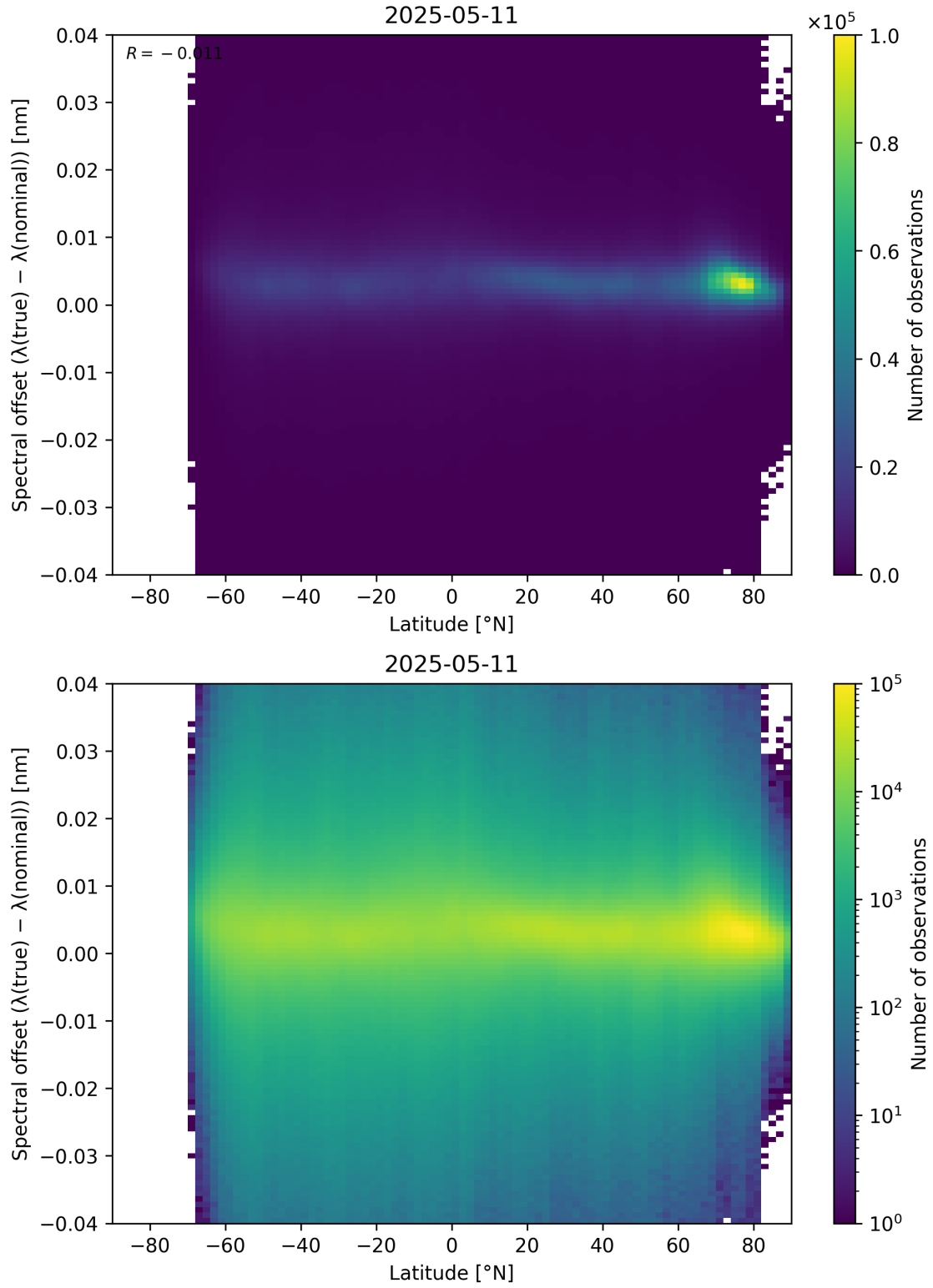
Figure 96: Scatter density plot of “Latitude” against “Spectral offset ( \lambda_{\text{true}} - \lambda_{\text{nominal}} )” for 2025-05-10 to 2025-05-12.
