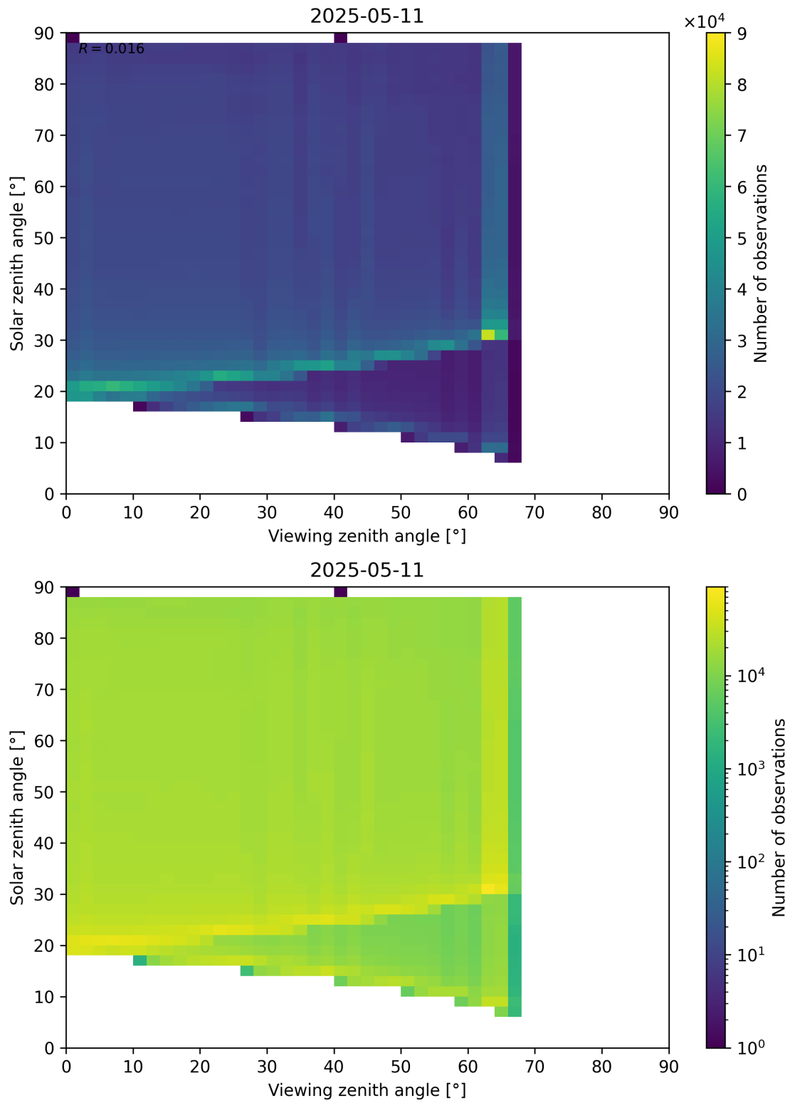
Figure 127: Scatter density plot of “Viewing zenith angle” against “Solar zenith angle” for 2025-05-10 to 2025-05-12.
