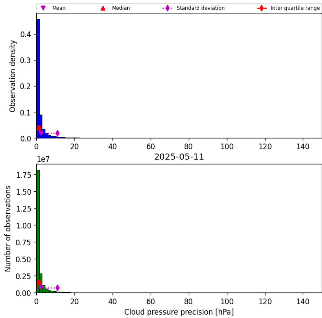
Figure 31: Histogram of “Cloud pressure precision” for 2025-05-10 to 2025-05-12
