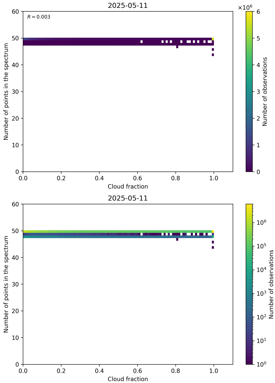
Figure 74: Scatter density plot of “Cloud fraction” against “Number of points in the spectrum” for 2025-05-10 to 2025-05-12.
