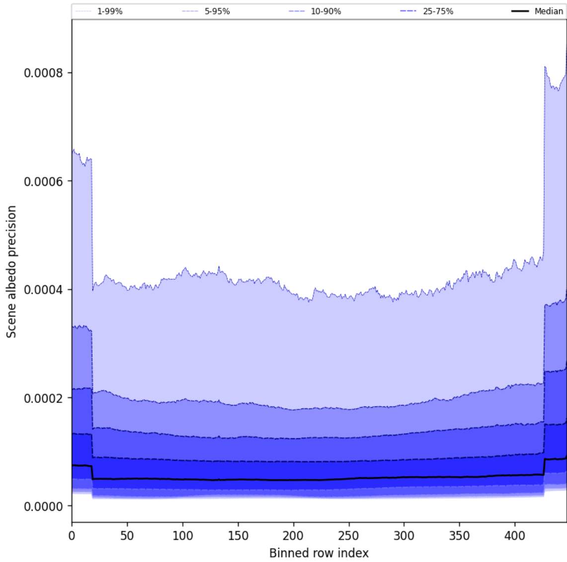
Figure 52: Along track statistics of “Scene albedo precision” for 2025-05-10 to 2025-05-12
