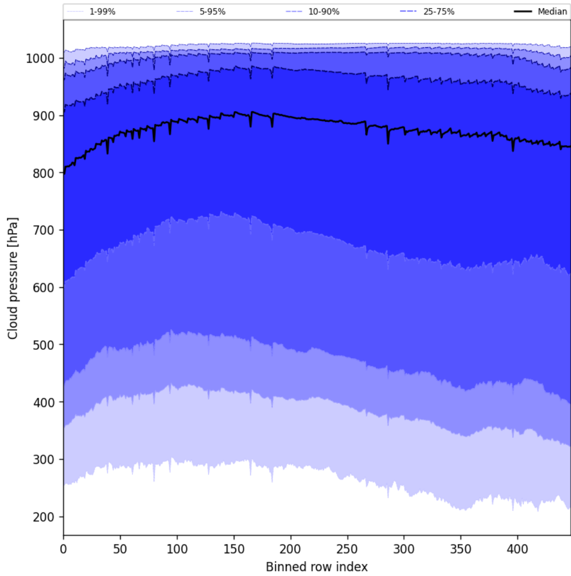
Figure 47: Along track statistics of “Cloud pressure” for 2025-05-10 to 2025-05-12
