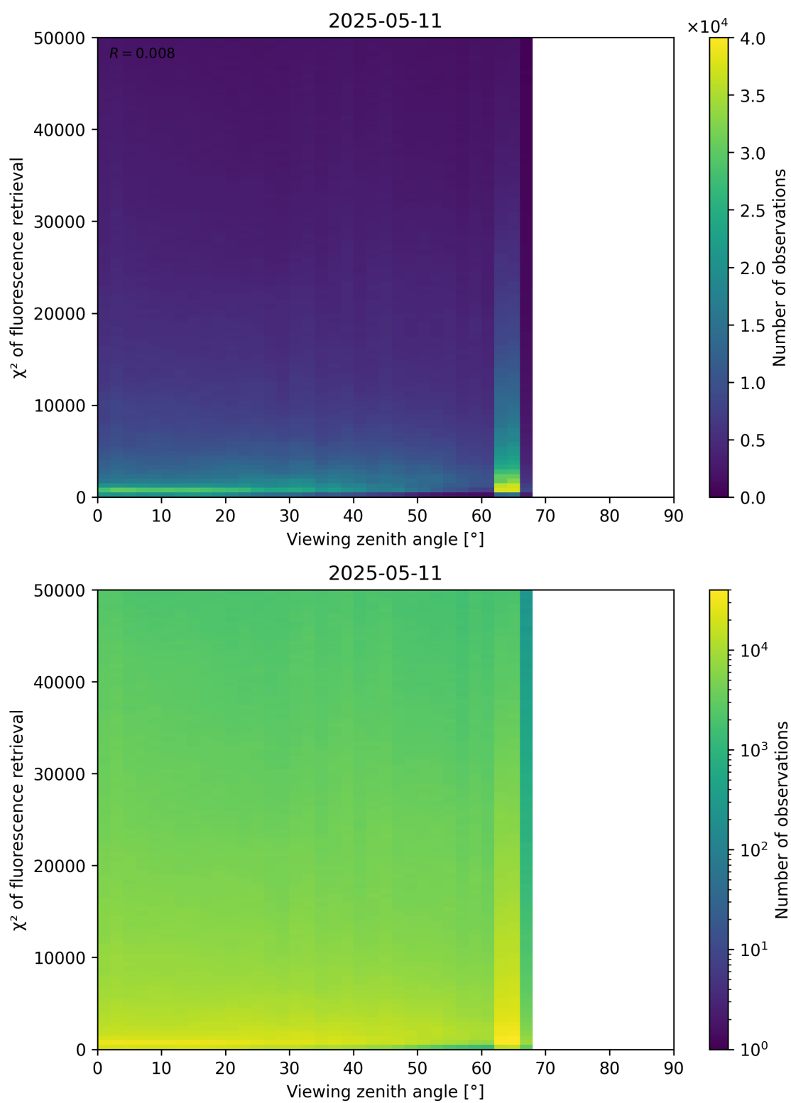
Figure 119: Scatter density plot of “Viewing zenith angle” against “ \chi^2 of fluorescence retrieval” for 2025-05-10 to 2025-05-12.
