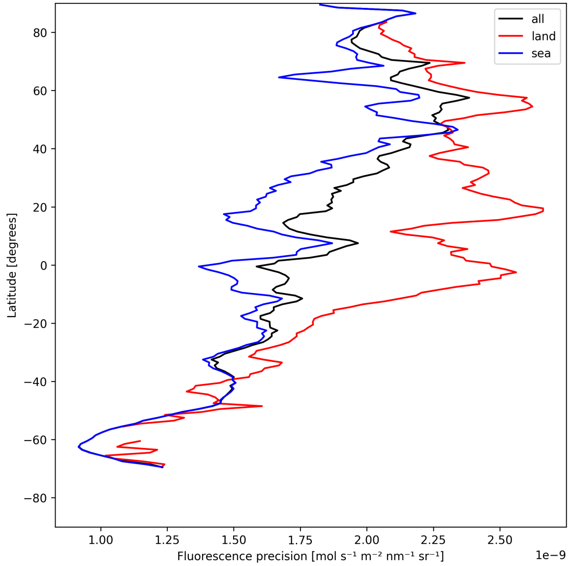
Figure 24: Zonal average of “Fluorescence precision” for 2025-05-10 to 2025-05-12.
