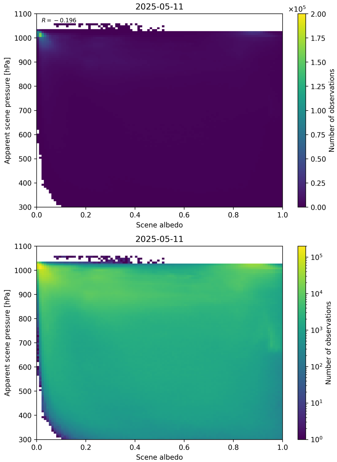
Figure 102: Scatter density plot of “Scene albedo” against “Apparent scene pressure” for 2025-05-10 to 2025-05-12.
