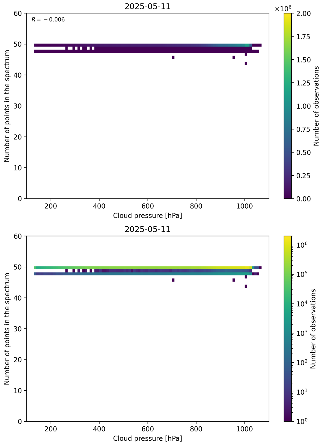
Figure 82: Scatter density plot of “Cloud pressure” against “Number of points in the spectrum” for 2025-05-10 to 2025-05-12.
