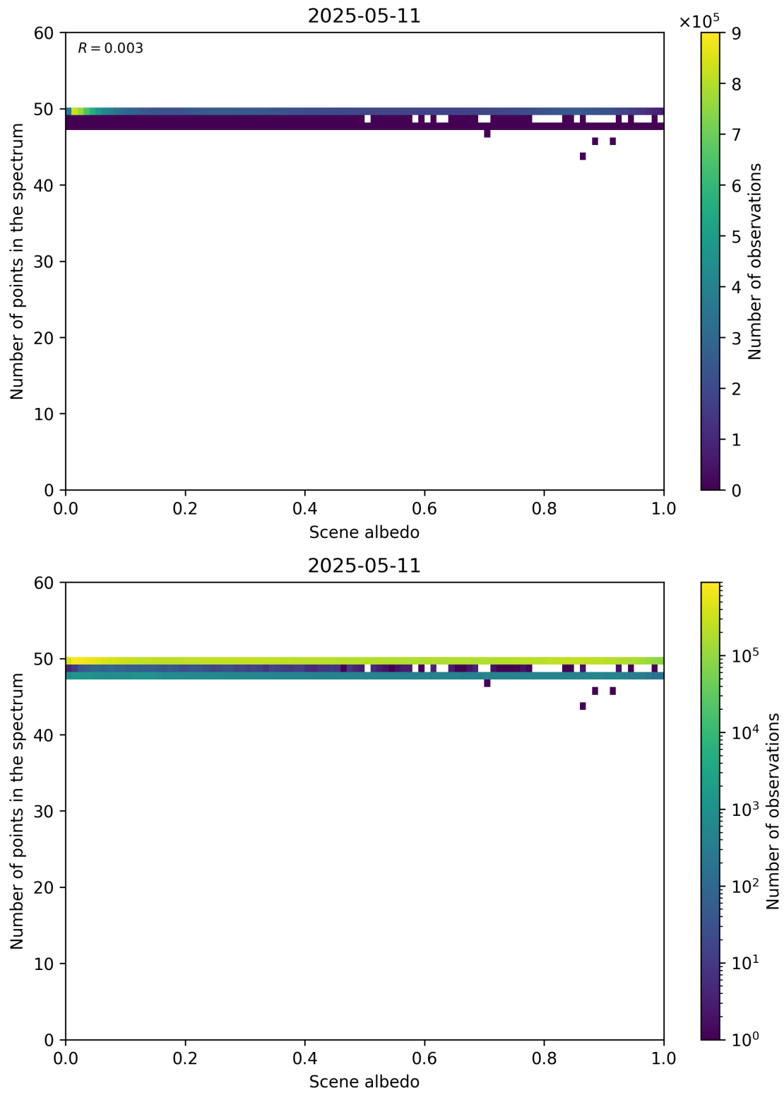
Figure 106: Scatter density plot of “Scene albedo” against “Number of points in the spectrum” for 2025-05-10 to 2025-05-12.
