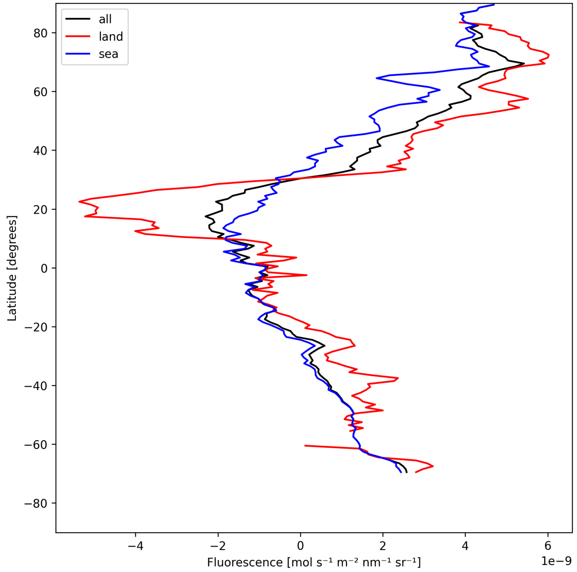
Figure 23: Zonal average of “Fluorescence” for 2025-05-10 to 2025-05-12.
