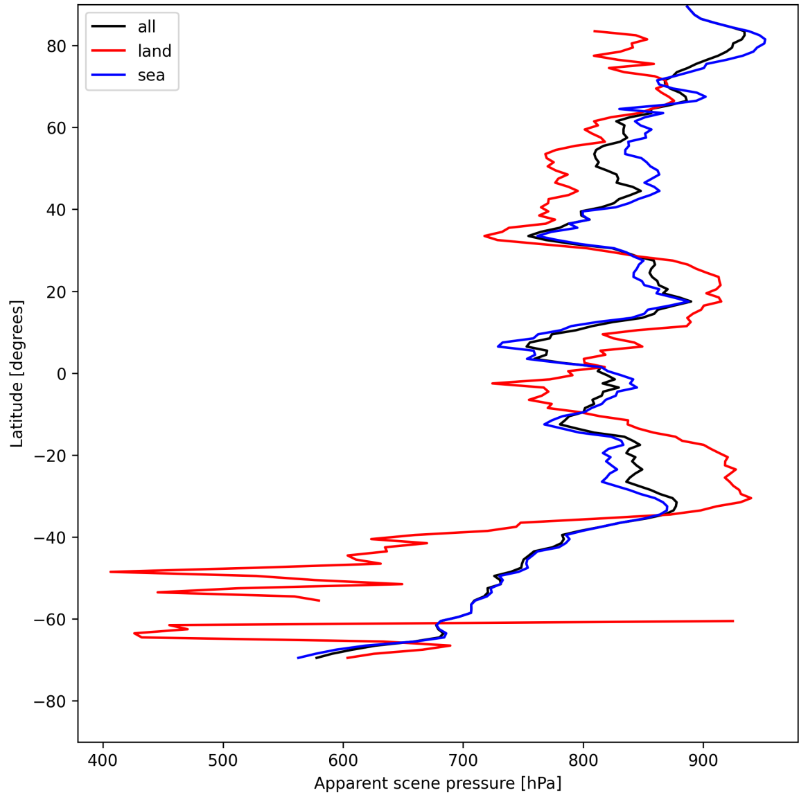
Figure 19: Zonal average of “Apparent scene pressure” for 2025-05-10 to 2025-05-12.
