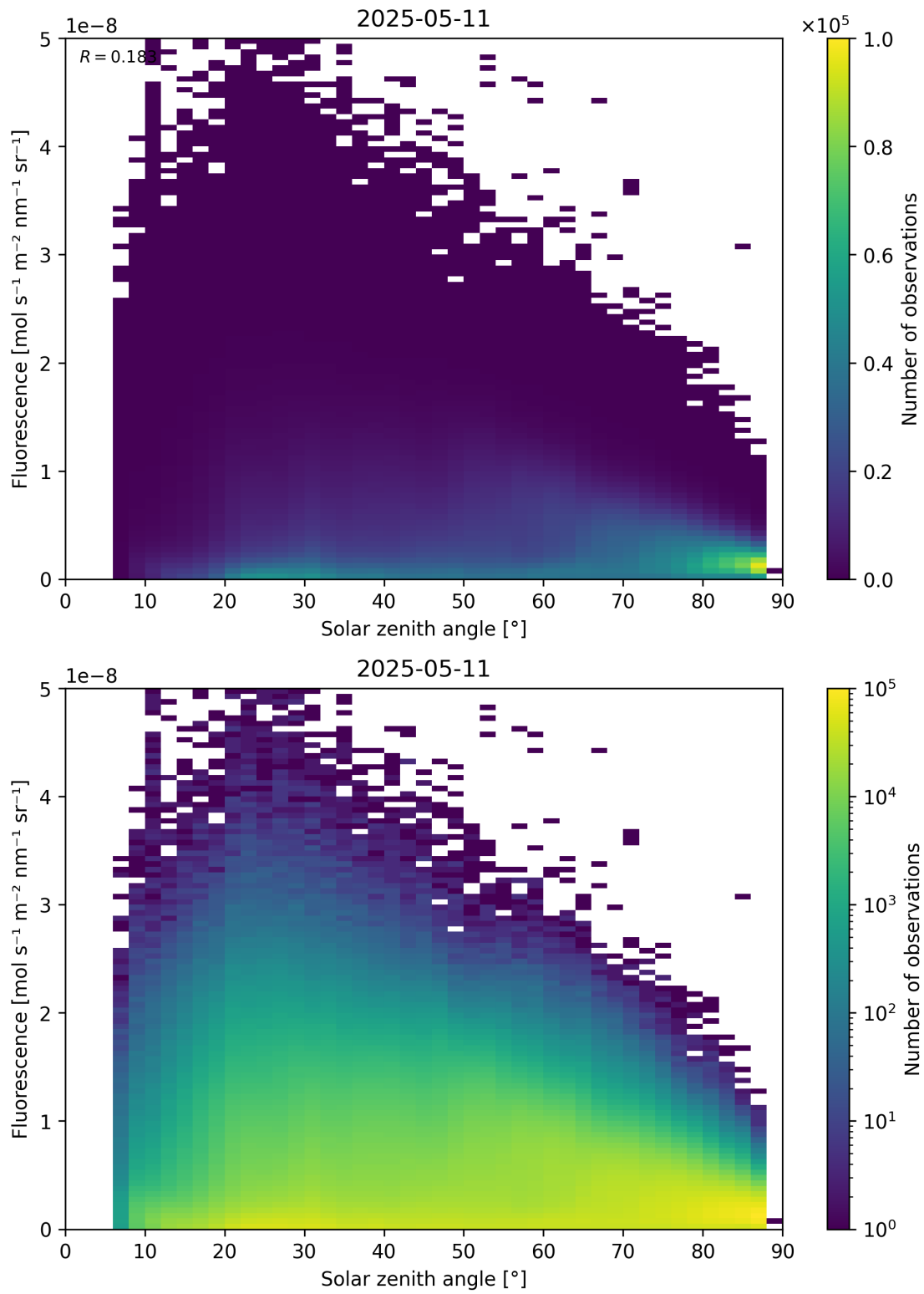
Figure 112: Scatter density plot of “Solar zenith angle” against “Fluorescence” for 2025-05-10 to 2025-05-12.
