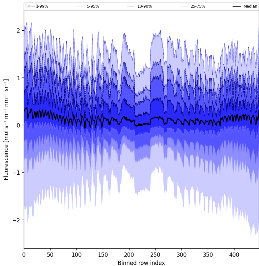
Figure 57: Along track statistics of “Fluorescence” for 2025-05-10 to 2025-05-12
