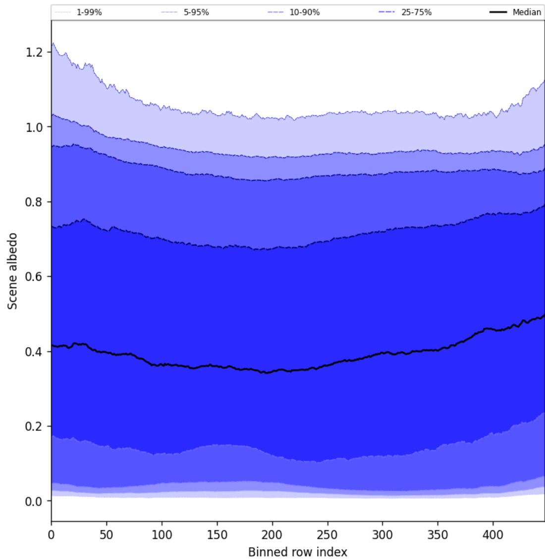
Figure 51: Along track statistics of “Scene albedo” for 2025-05-10 to 2025-05-12
