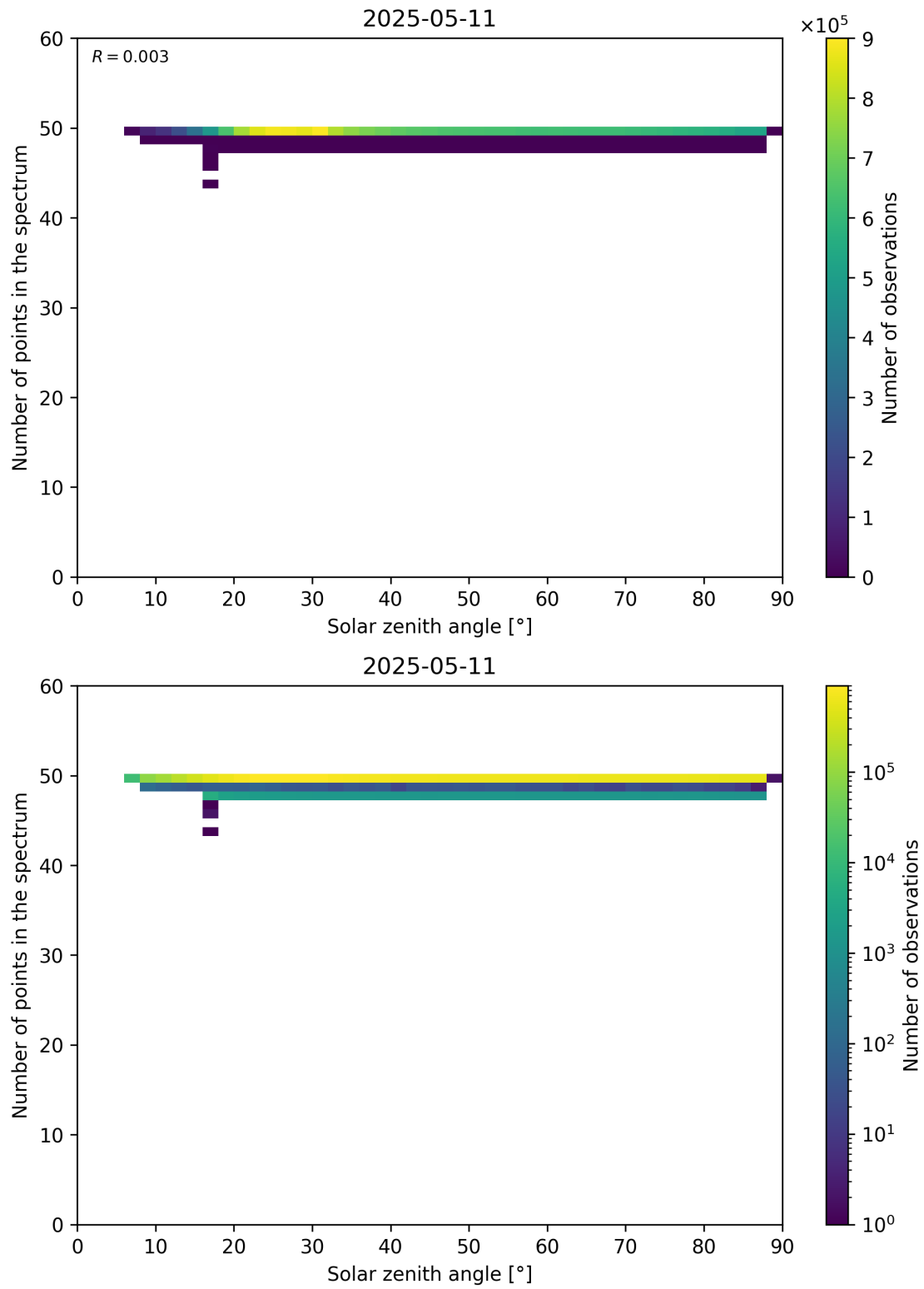
Figure 115: Scatter density plot of “Solar zenith angle” against “Number of points in the spectrum” for 2025-05-10 to 2025-05-12.
