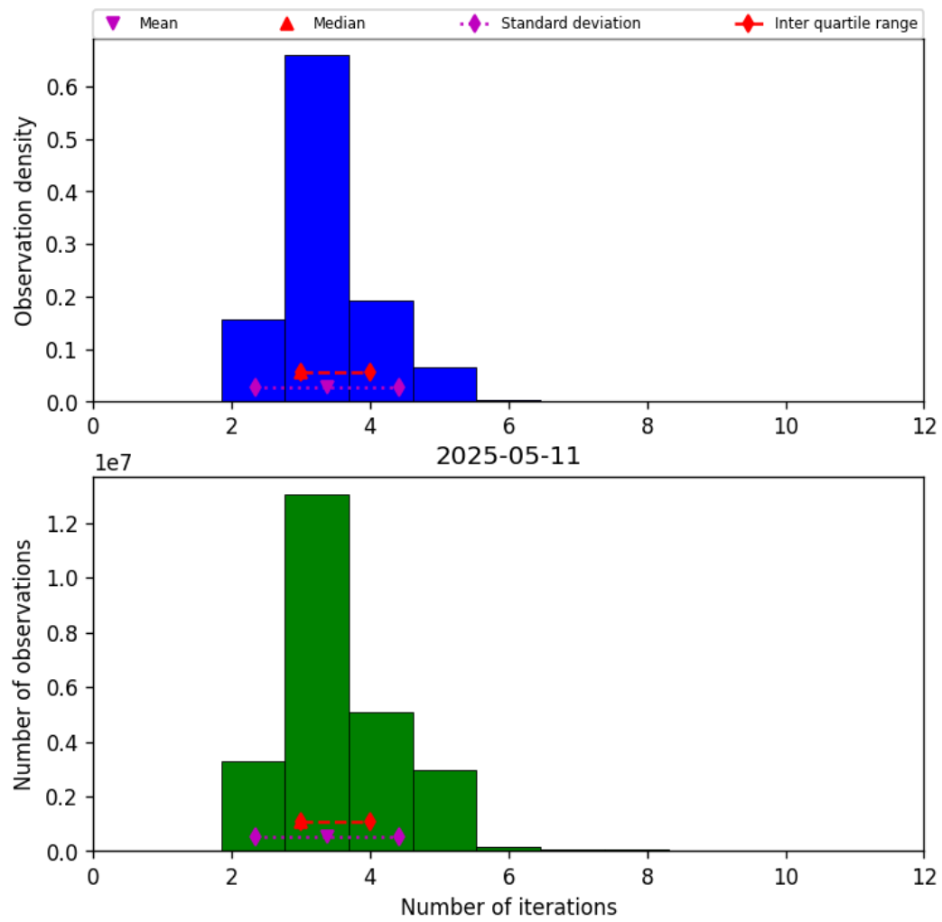
Figure 39: Histogram of “Number of iterations” for 2025-05-10 to 2025-05-12
