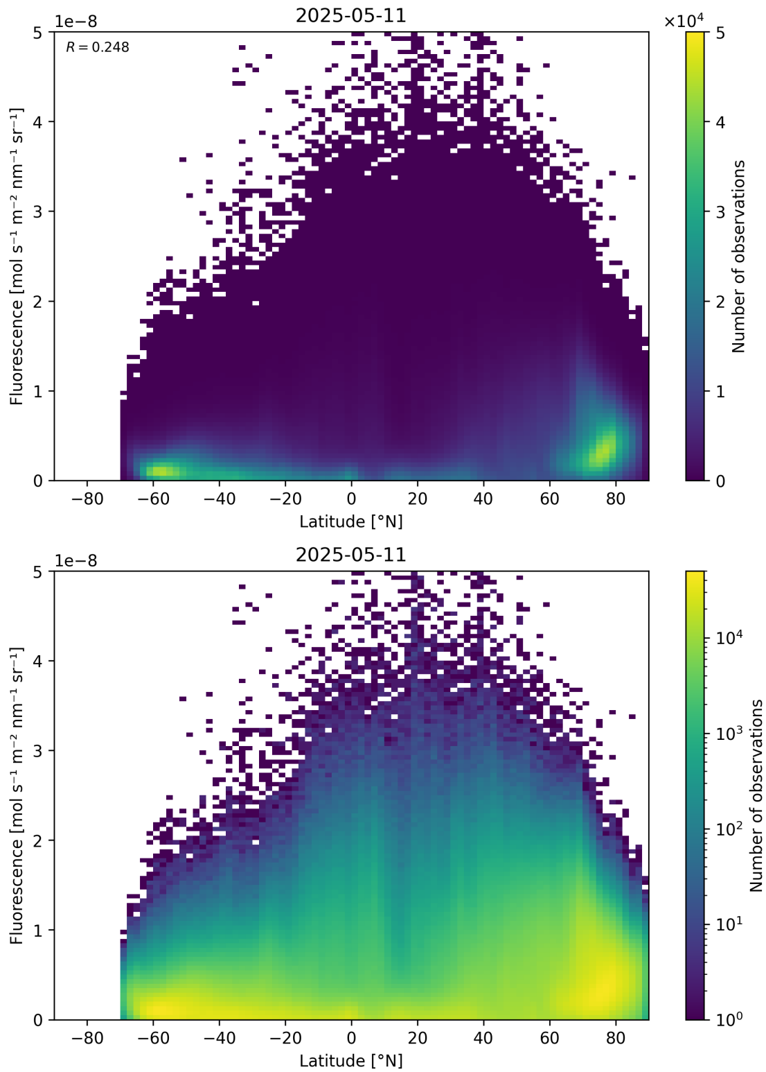
Figure 92: Scatter density plot of “Latitude” against “Fluorescence” for 2025-05-10 to 2025-05-12.
