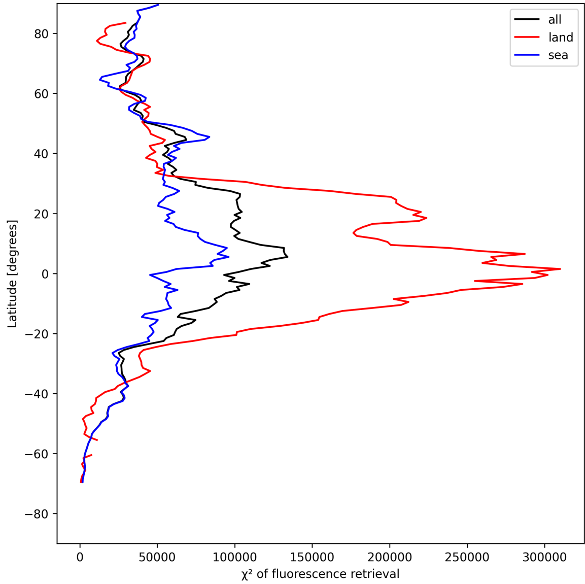
Figure 25: Zonal average of “ \chi^2 of fluorescence retrieval” for 2025-05-10 to 2025-05-12.
