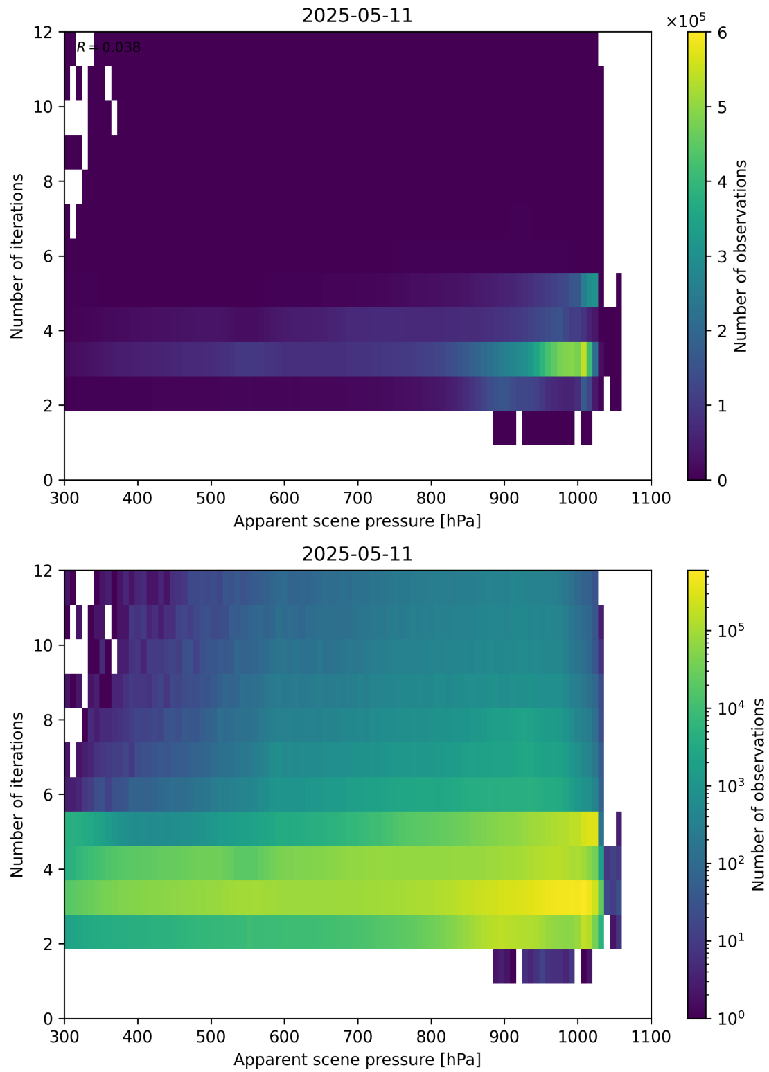
Figure 65: Scatter density plot of “Apparent scene pressure” against “Number of iterations” for 2025-05-10 to 2025-05-12.
