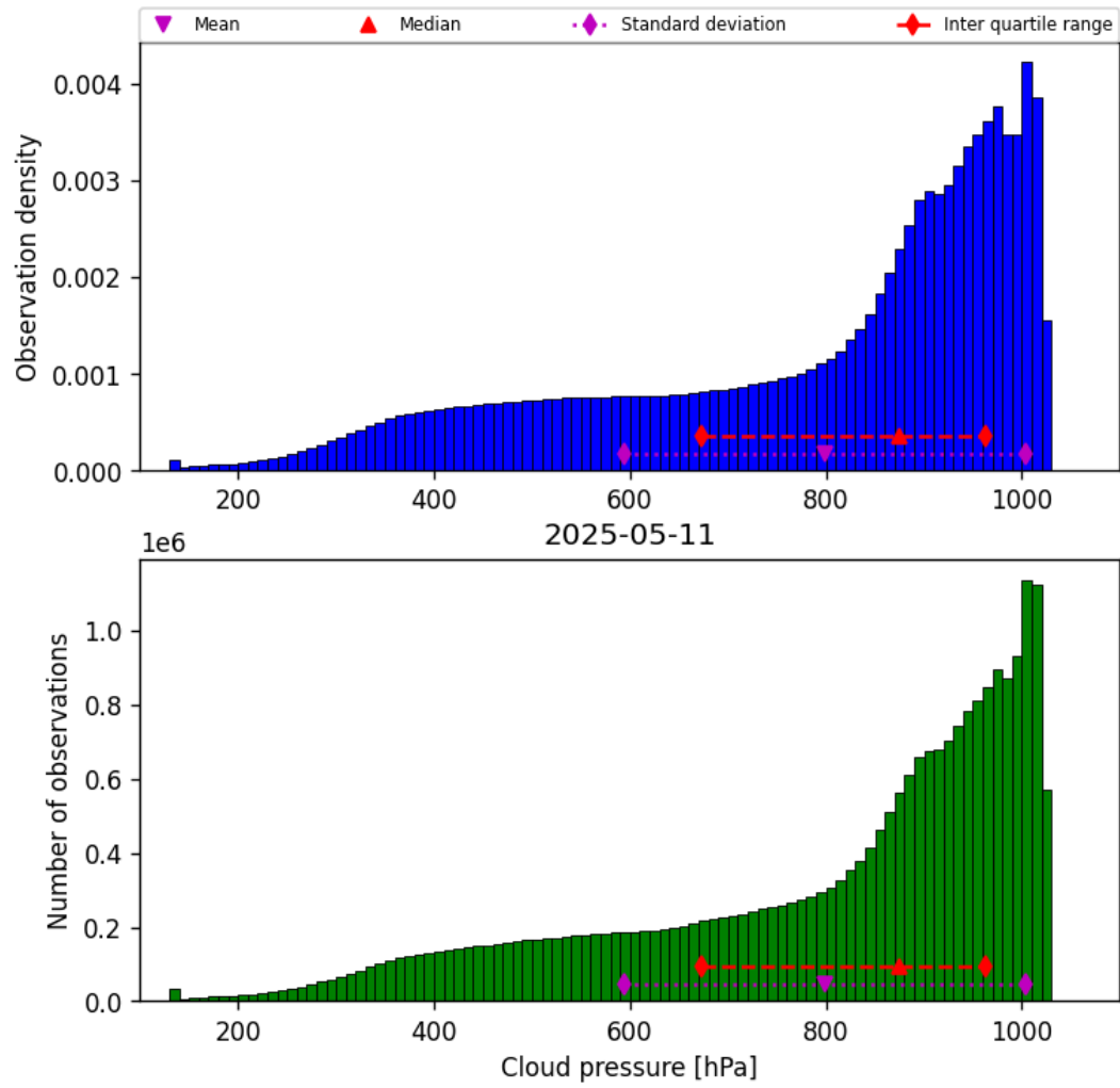
Figure 30: Histogram of “Cloud pressure” for 2025-05-10 to 2025-05-12
