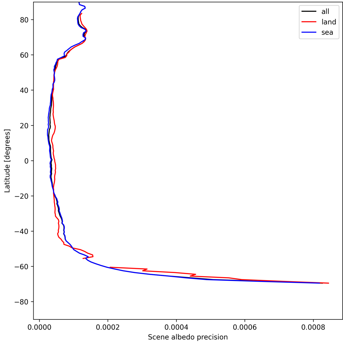
Figure 18: Zonal average of “Scene albedo precision” for 2025-05-10 to 2025-05-12.
