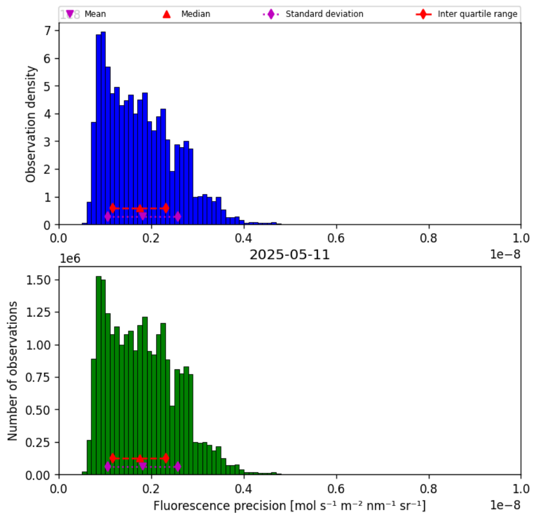
Figure 41: Histogram of “Fluorescence precision” for 2025-05-10 to 2025-05-12
