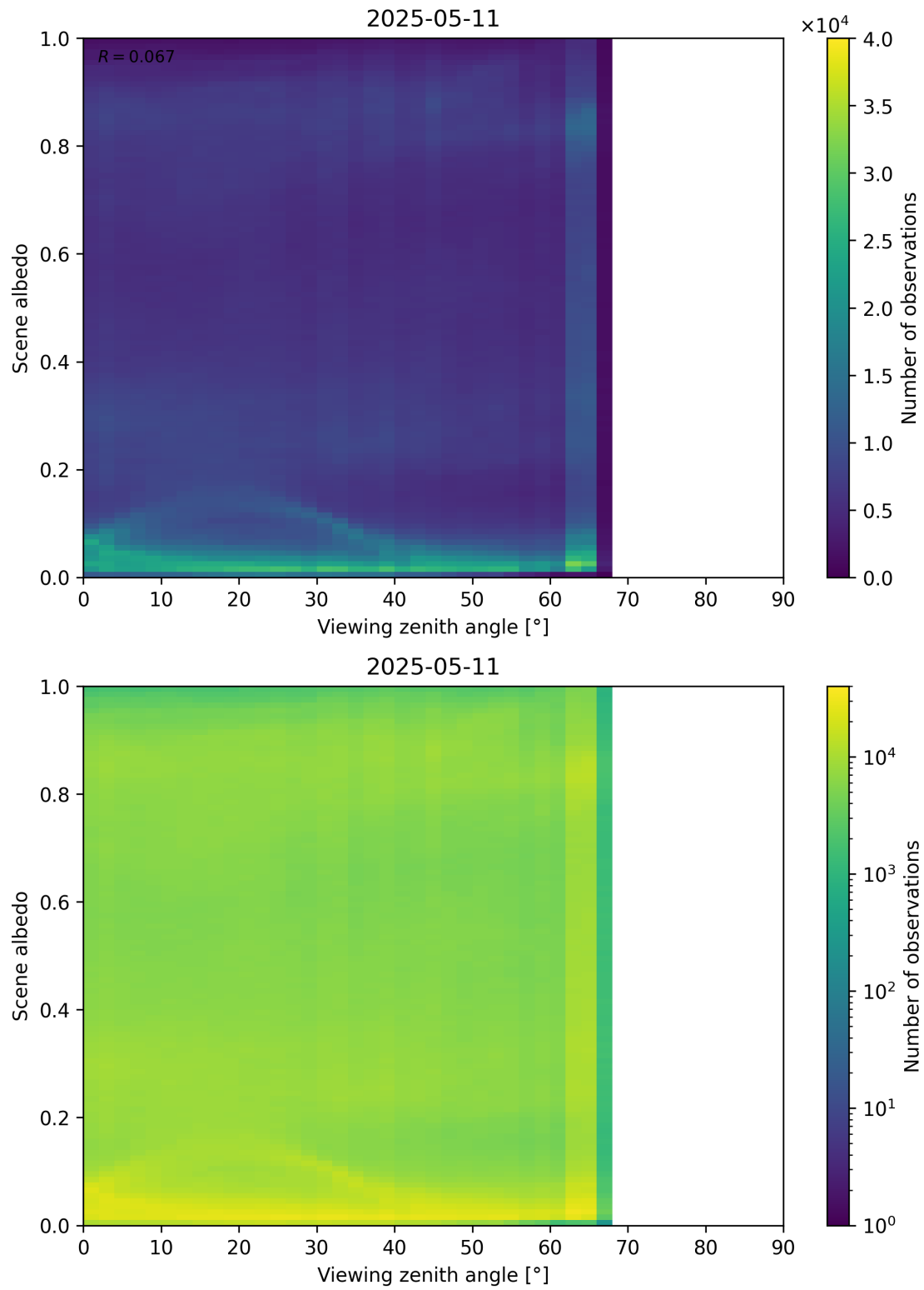
Figure 126: Scatter density plot of “Viewing zenith angle” against “Scene albedo” for 2025-05-10 to 2025-05-12.
