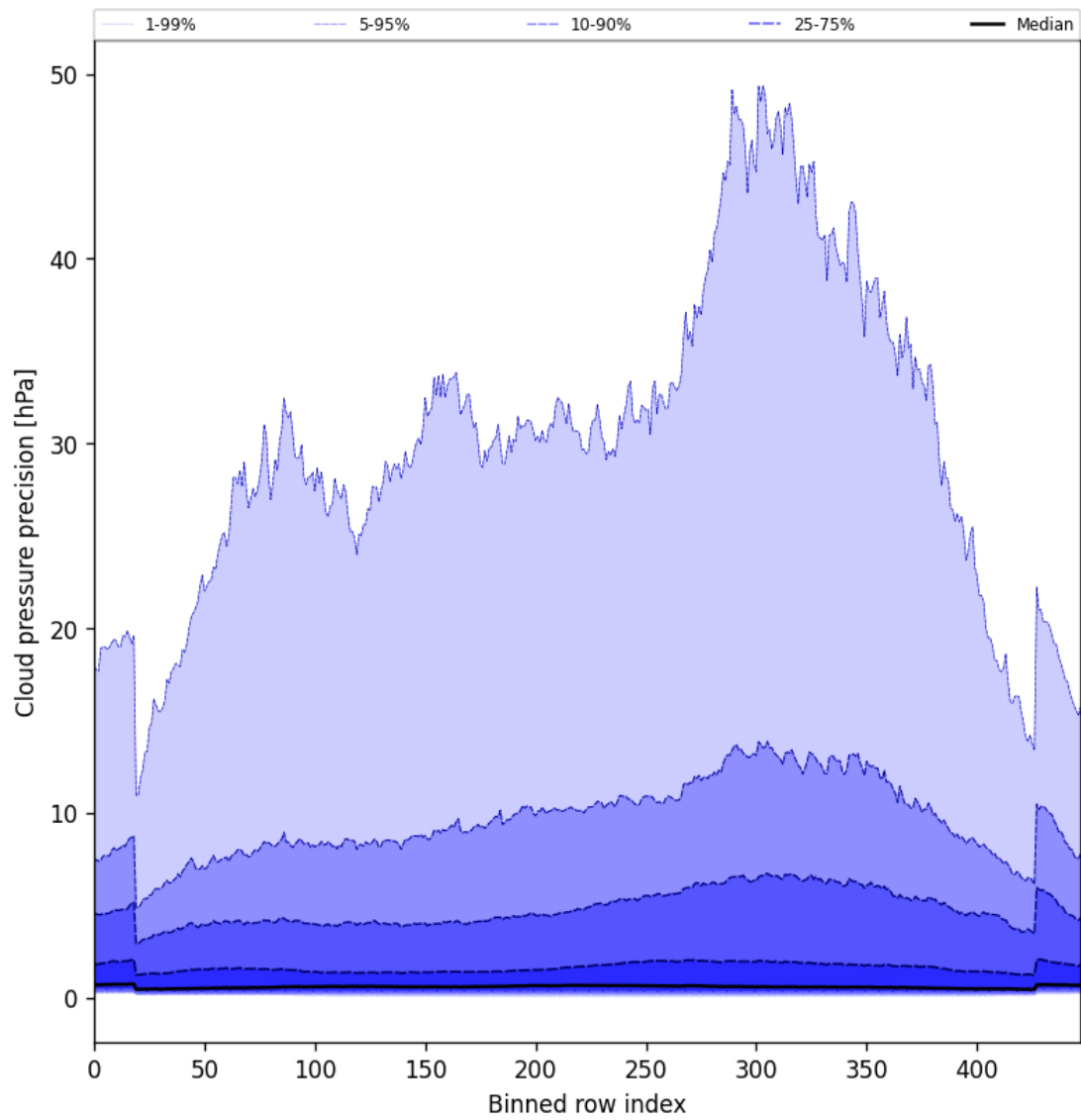
Figure 48: Along track statistics of “Cloud pressure precision” for 2025-05-10 to 2025-05-12
