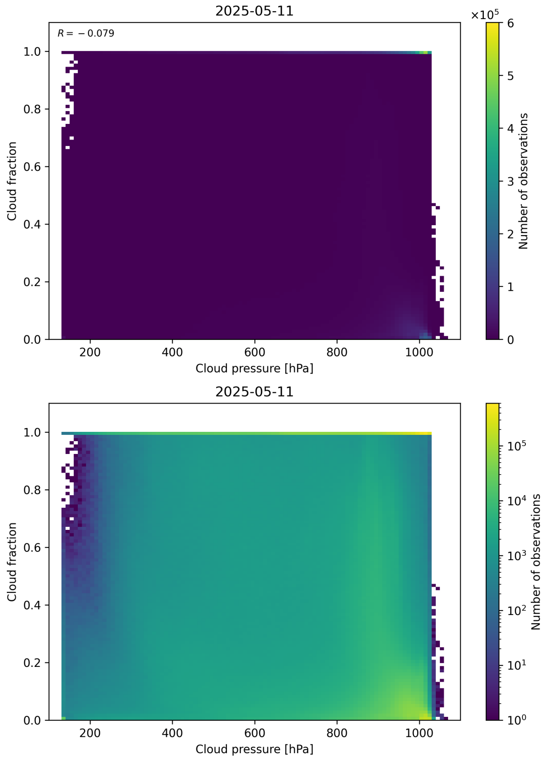
Figure 79: Scatter density plot of “Cloud pressure” against “Cloud fraction” for 2025-05-10 to 2025-05-12.
