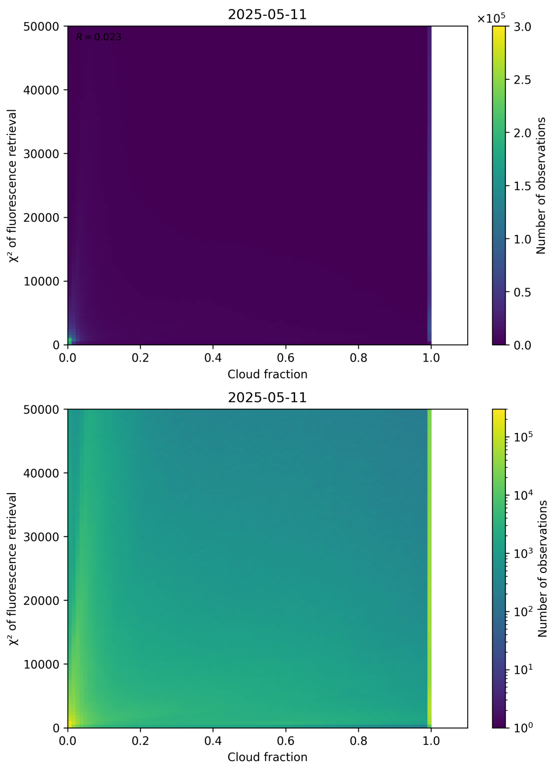
Figure 71: Scatter density plot of “Cloud fraction” against “ \chi^2 of fluorescence retrieval” for 2025-05-10 to 2025-05-12.
