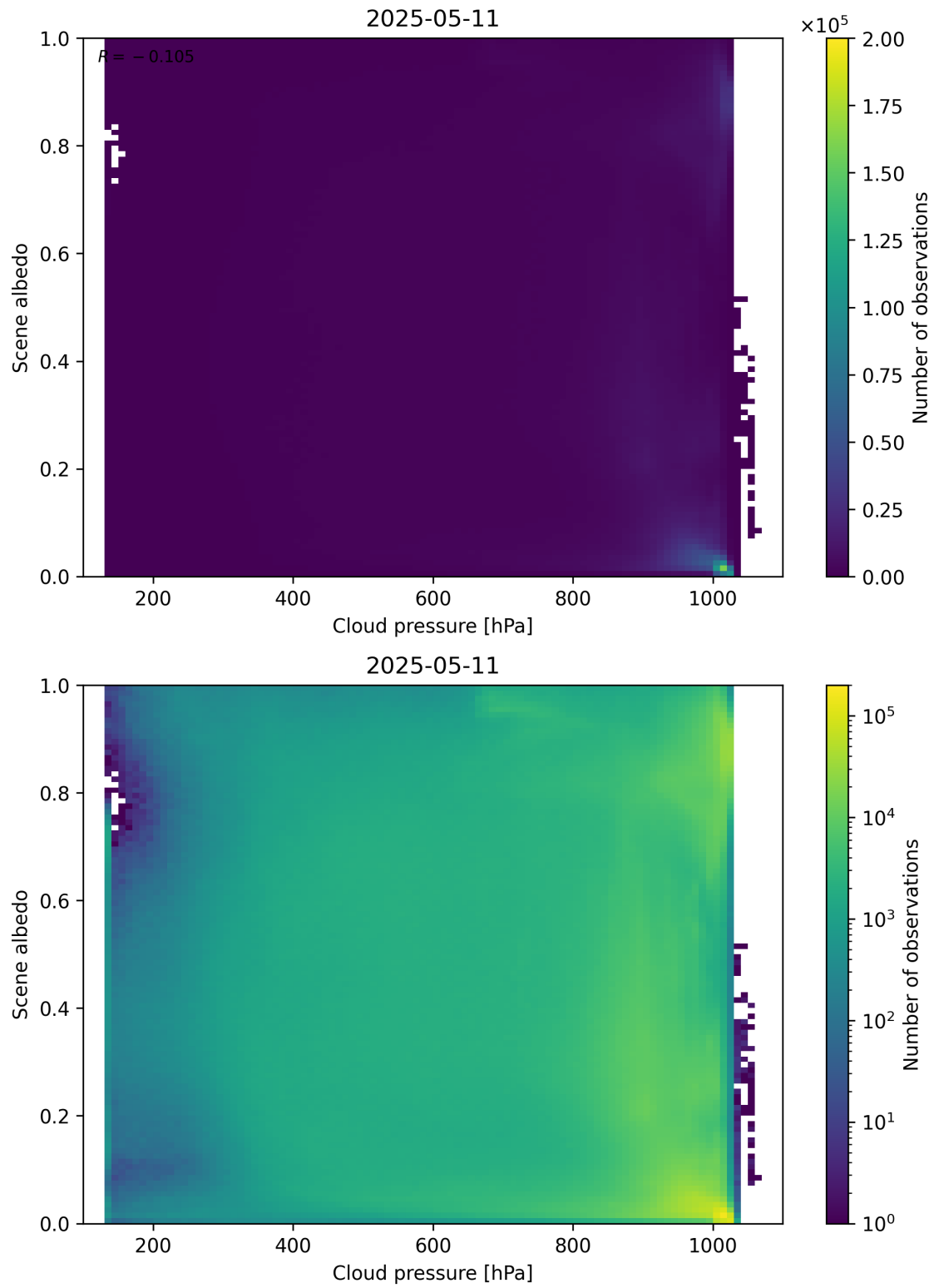
Figure 83: Scatter density plot of “Cloud pressure” against “Scene albedo” for 2025-05-10 to 2025-05-12.
