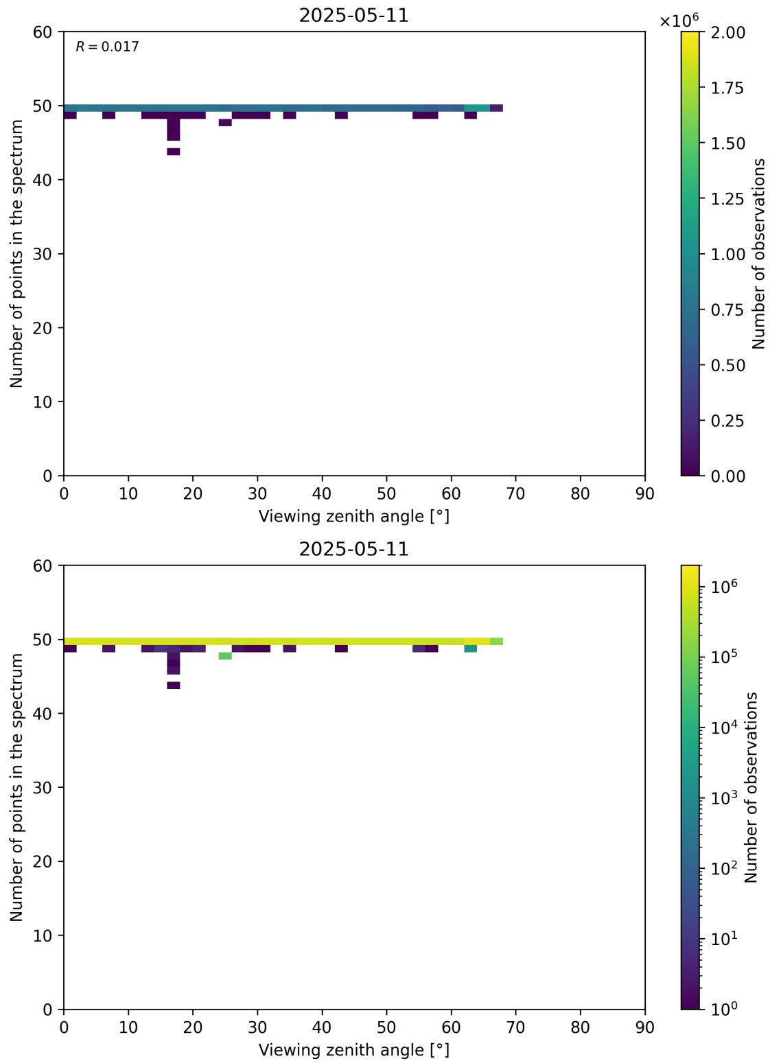
Figure 125: Scatter density plot of “Viewing zenith angle” against “Number of points in the spectrum” for 2025-05-10 to 2025-05-12.
