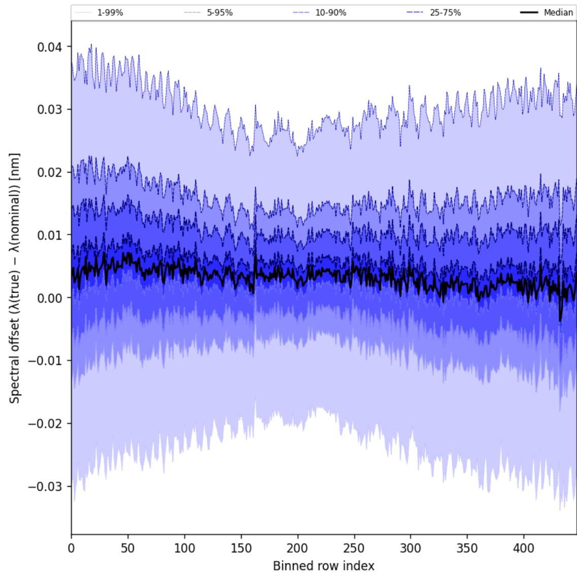
Figure 62: Along track statistics of “Spectral offset ( \lambda_{\text{true}} - \lambda_{\text{nominal}} )” for 2025-05-10 to 2025-05-12
