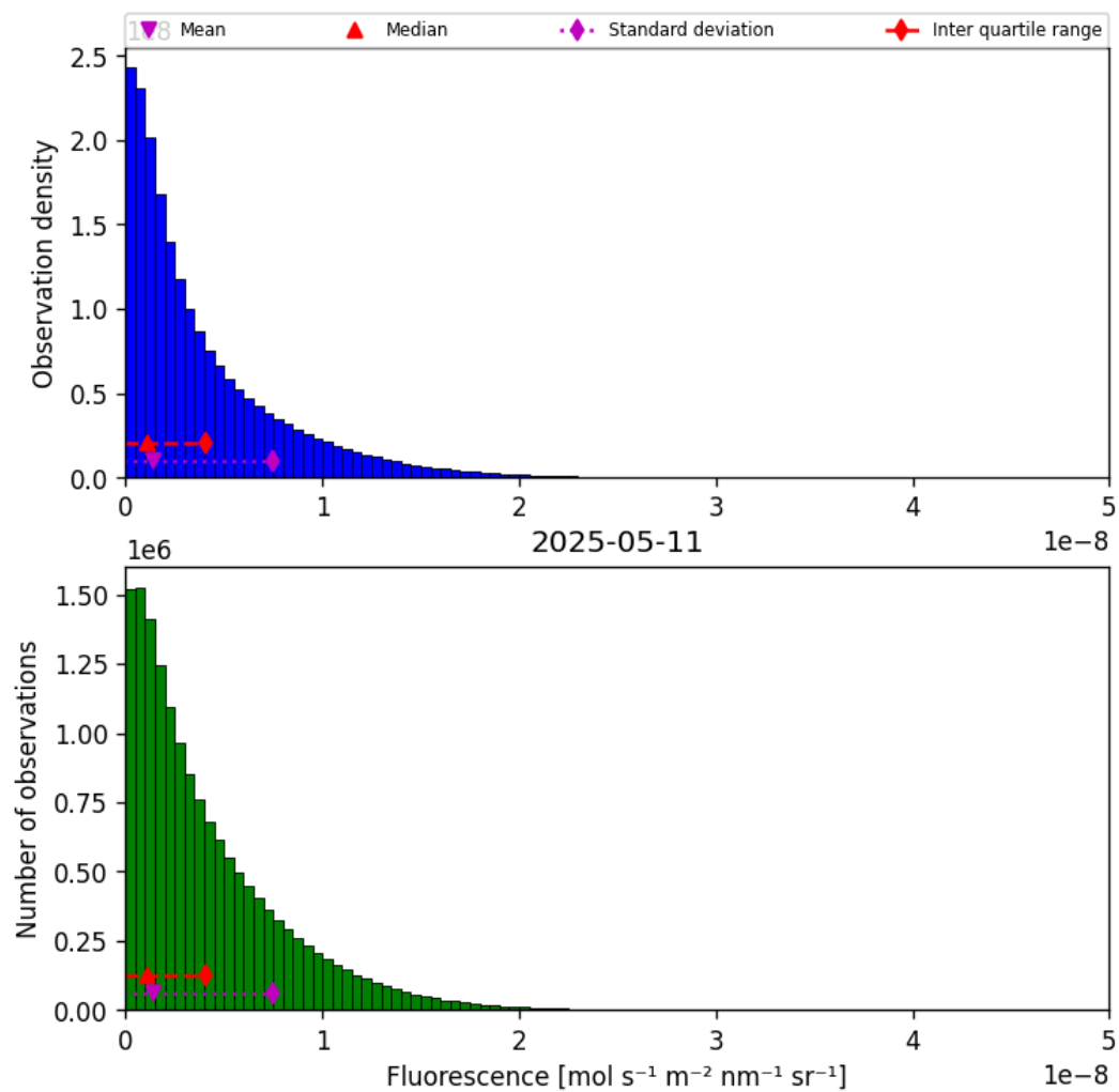
Figure 40: Histogram of “Fluorescence” for 2025-05-10 to 2025-05-12
