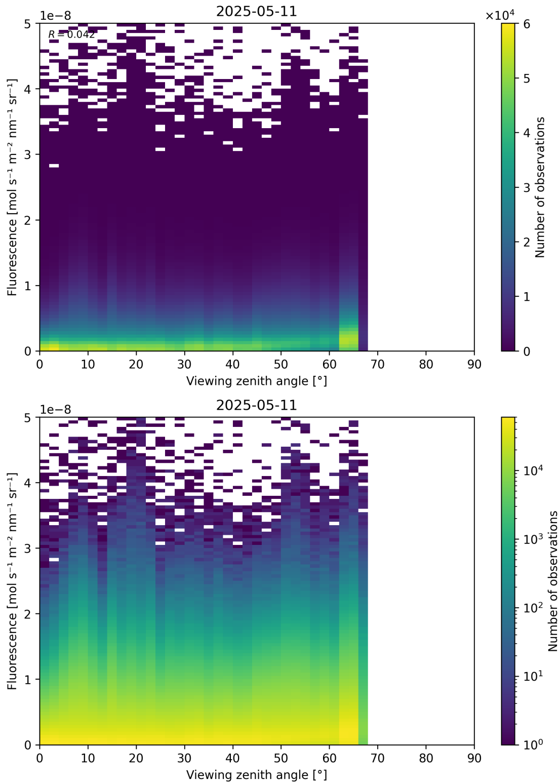
Figure 122: Scatter density plot of “Viewing zenith angle” against “Fluorescence” for 2025-05-10 to 2025-05-12.
