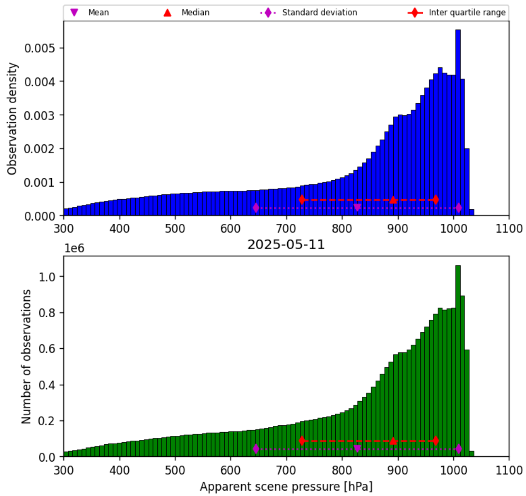
Figure 36: Histogram of “Apparent scene pressure” for 2025-05-10 to 2025-05-12
