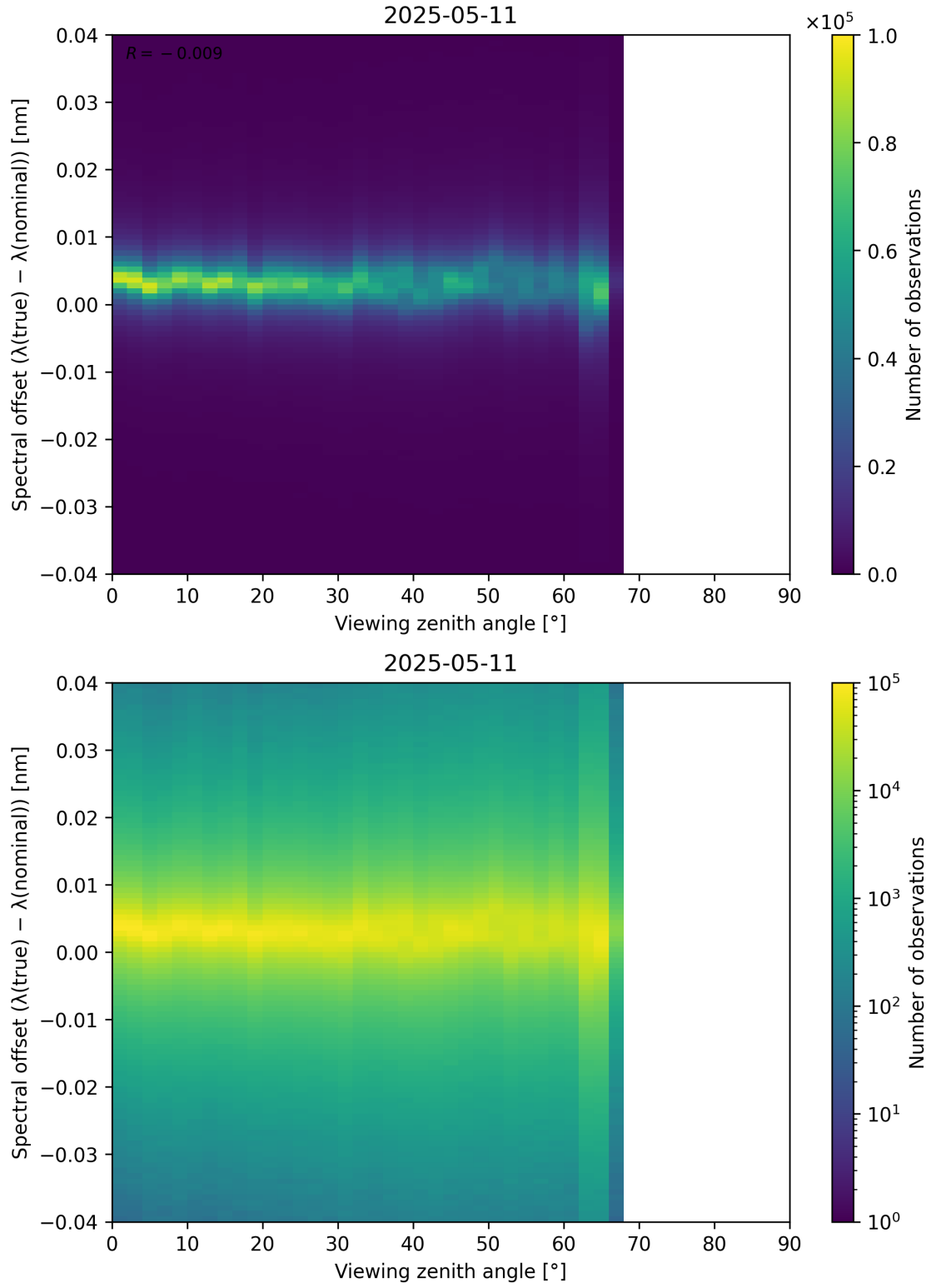
Figure 128: Scatter density plot of “Viewing zenith angle” against “Spectral offset ( \lambda_{\text{true}} - \lambda_{\text{nominal}} )” for 2025-05-10 to 2025-05-12.
