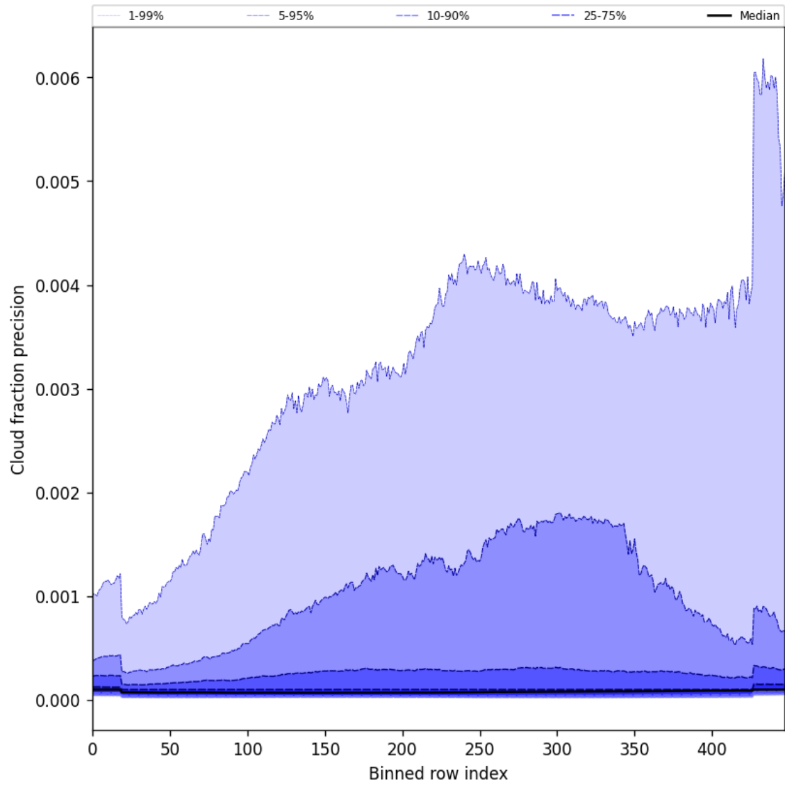
Figure 50: Along track statistics of “Cloud fraction precision” for 2025-05-10 to 2025-05-12
