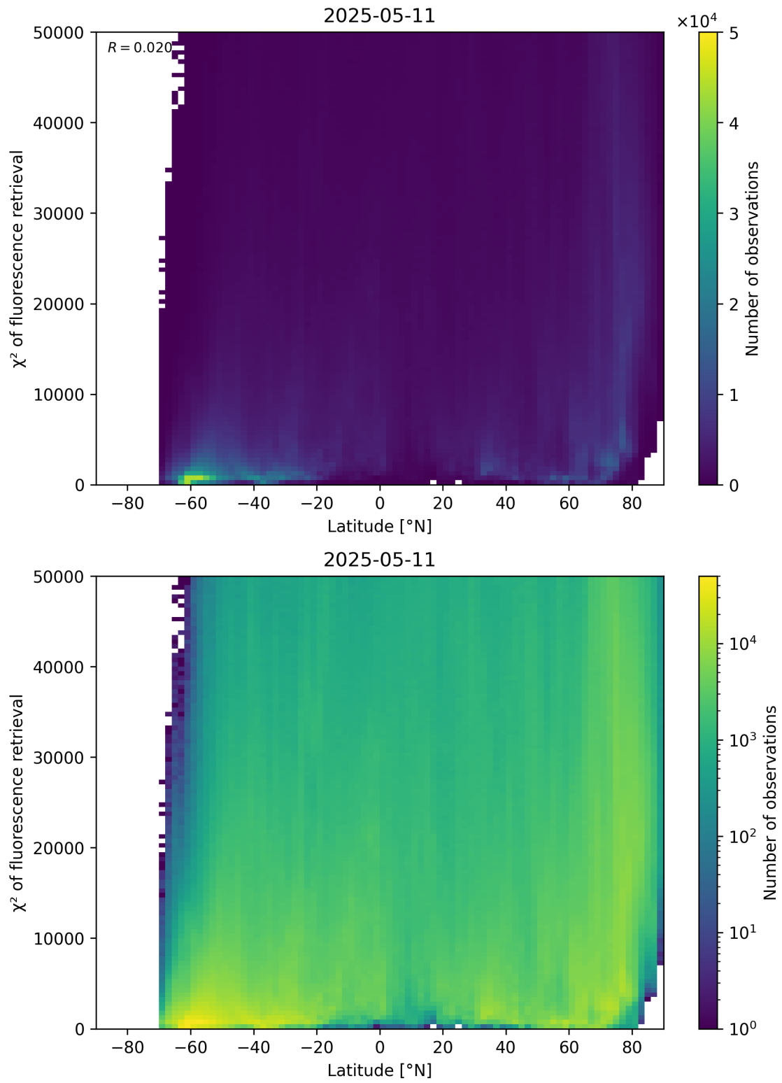
Figure 89: Scatter density plot of “Latitude” against “ \chi^2 of fluorescence retrieval” for 2025-05-10 to 2025-05-12.
