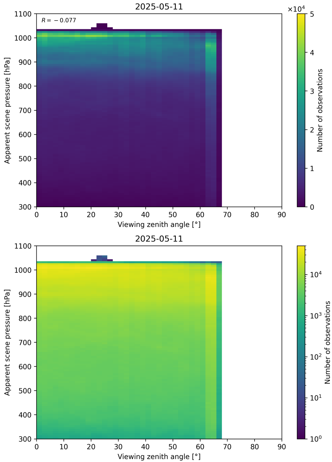
Figure 118: Scatter density plot of “Viewing zenith angle” against “Apparent scene pressure” for 2025-05-10 to 2025-05-12.
