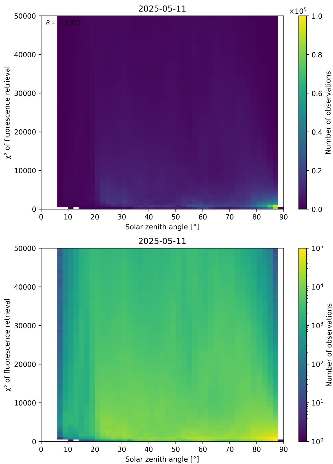
Figure 109: Scatter density plot of “Solar zenith angle” against “ \chi^2 of fluorescence retrieval” for 2025-05-10 to 2025-05-12.
