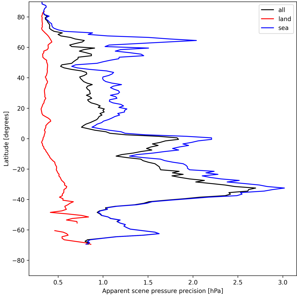
Figure 20: Zonal average of “Apparent scene pressure precision” for 2025-05-10 to 2025-05-12.
