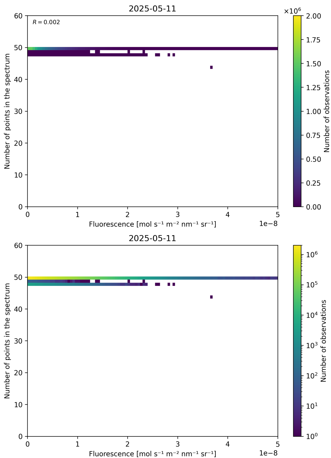
Figure 86: Scatter density plot of “Fluorescence” against “Number of points in the spectrum” for 2025-05-10 to 2025-05-12.
