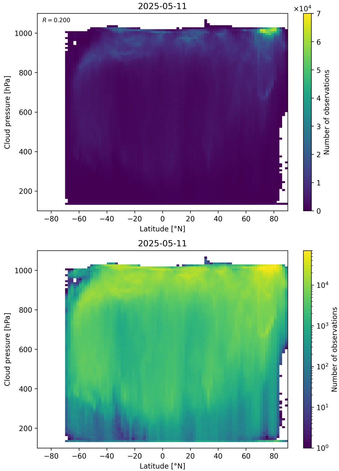
Figure 91: Scatter density plot of “Latitude” against “Cloud pressure” for 2025-05-10 to 2025-05-12.
