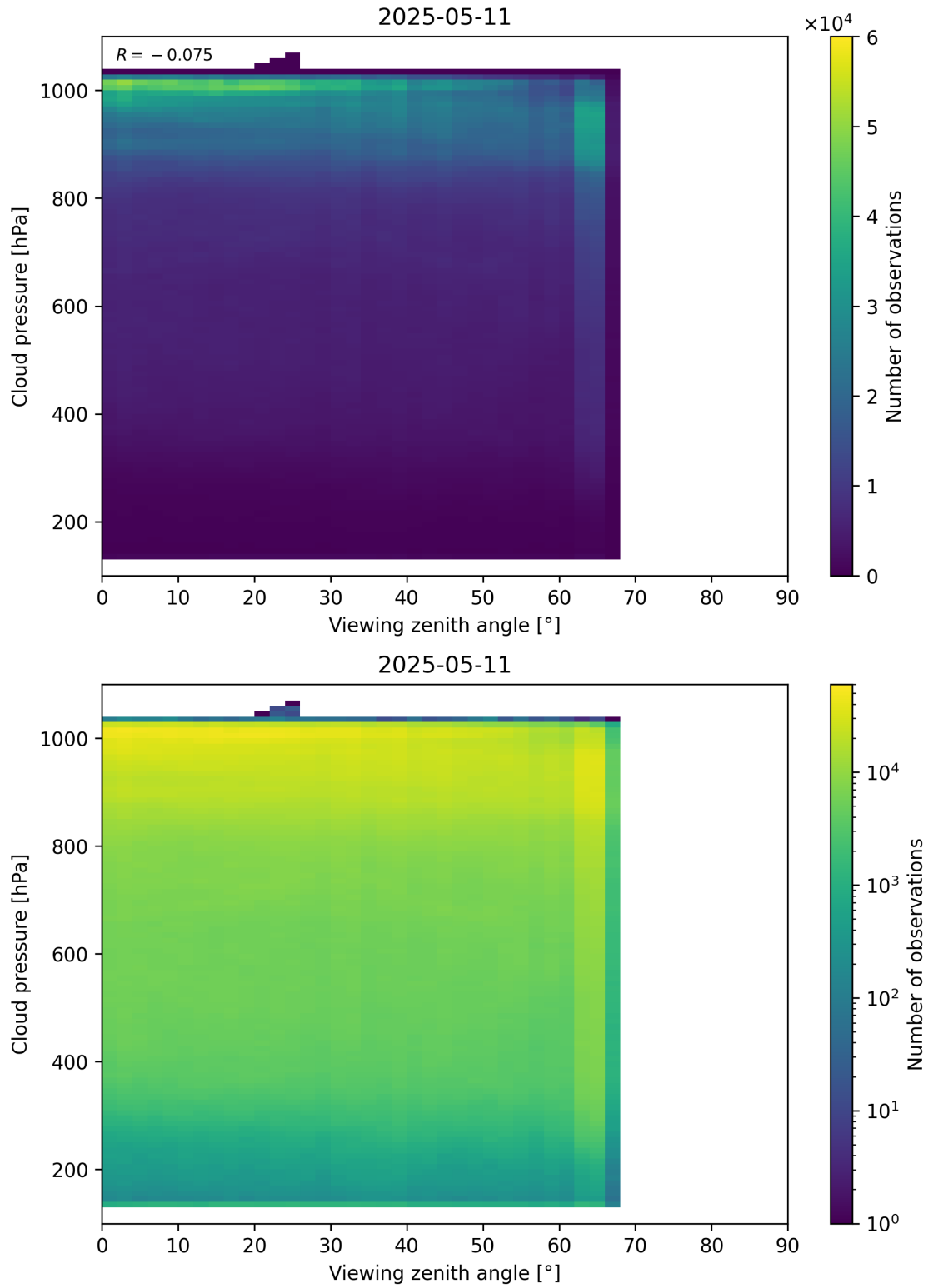
Figure 121: Scatter density plot of “Viewing zenith angle” against “Cloud pressure” for 2025-05-10 to 2025-05-12.
