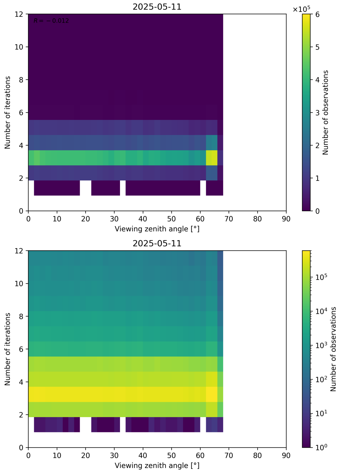
Figure 124: Scatter density plot of “Viewing zenith angle” against “Number of iterations” for 2025-05-10 to 2025-05-12.
