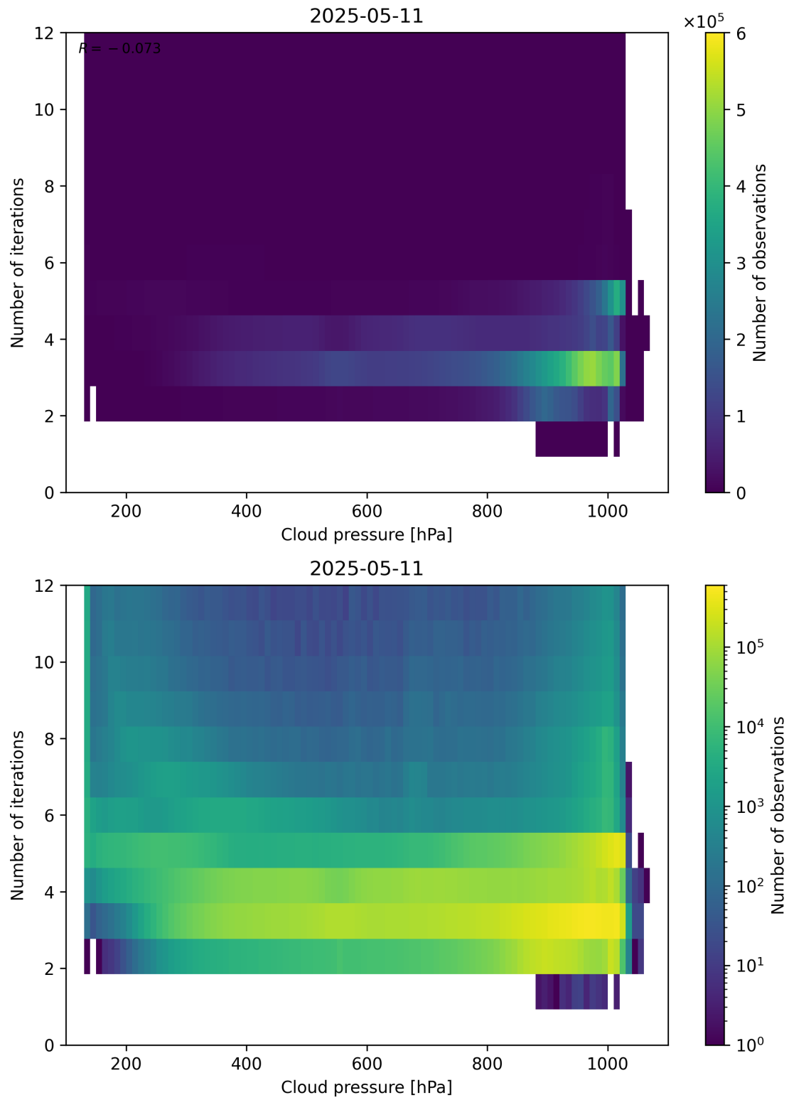
Figure 81: Scatter density plot of “Cloud pressure” against “Number of iterations” for 2025-05-10 to 2025-05-12.
