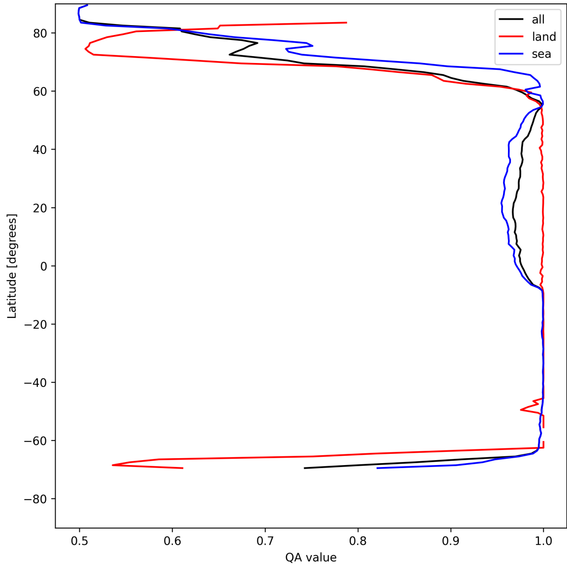
Figure 12: Zonal average of "QA value" for 2025-05-10 to 2025-05-12.
