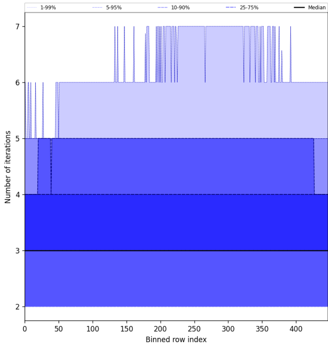
Figure 56: Along track statistics of “Number of iterations” for 2025-05-10 to 2025-05-12
