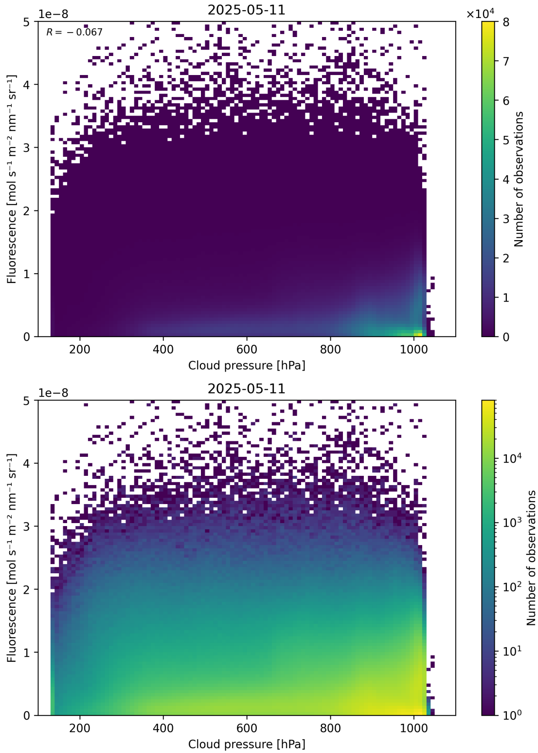
Figure 80: Scatter density plot of “Cloud pressure” against “Fluorescence” for 2025-05-10 to 2025-05-12.
