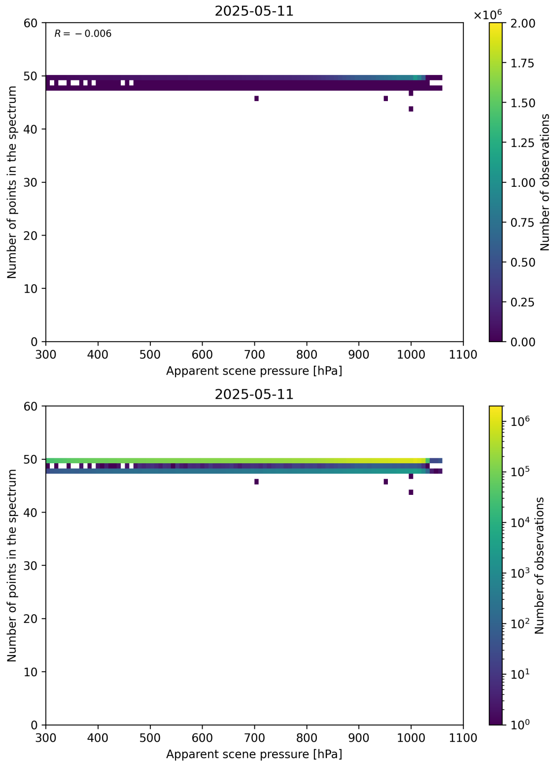
Figure 66: Scatter density plot of “Apparent scene pressure” against “Number of points in the spectrum” for 2025-05-10 to 2025-05-12.
