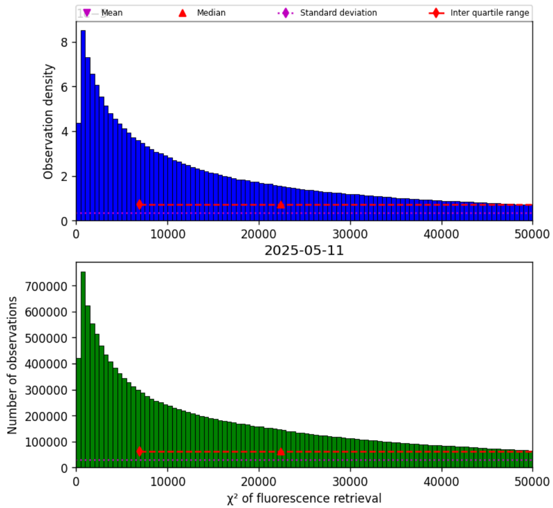
Figure 42: Histogram of “ \chi^2 of fluorescence retrieval” for 2025-05-10 to 2025-05-12
