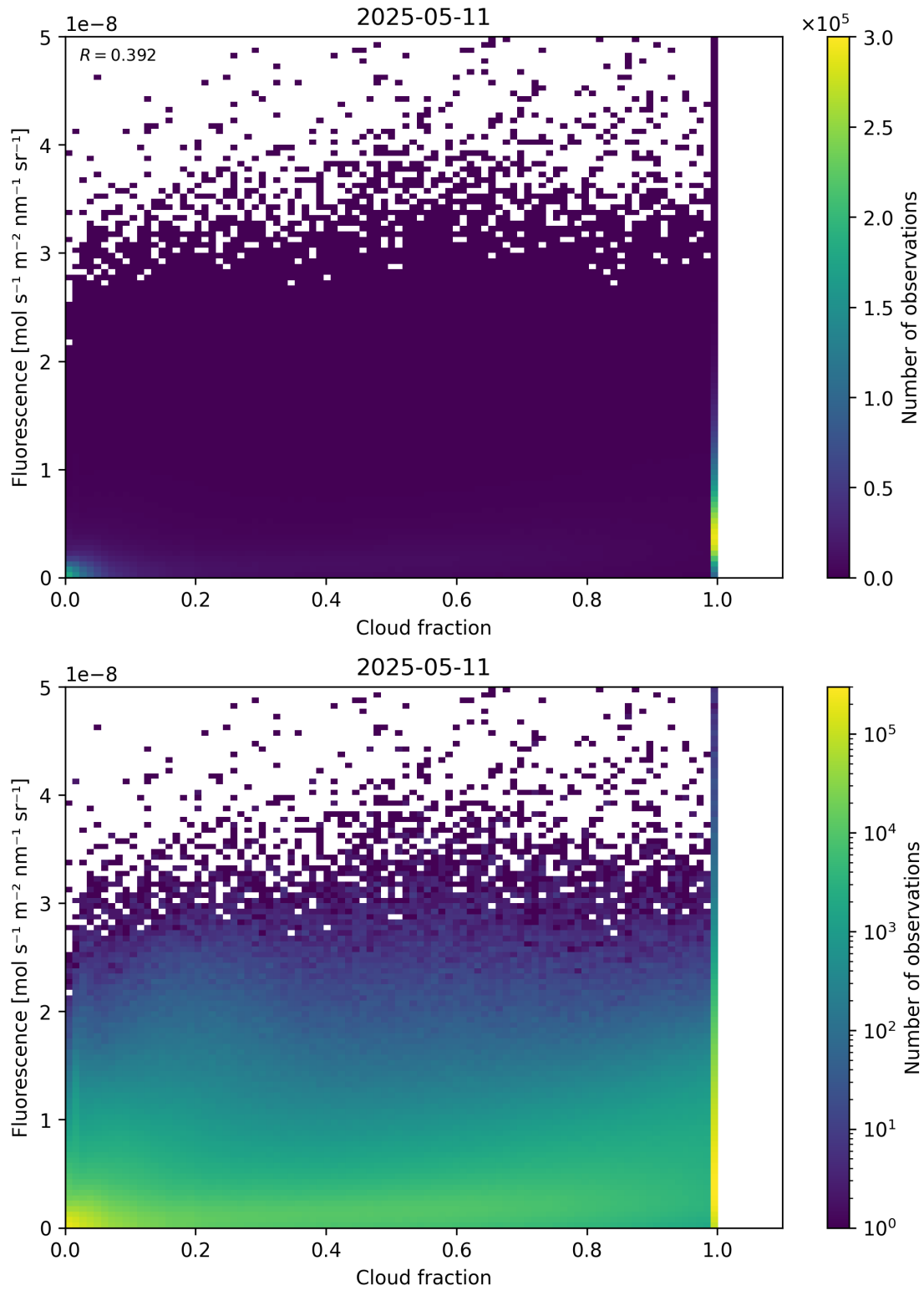
Figure 72: Scatter density plot of “Cloud fraction” against “Fluorescence” for 2025-05-10 to 2025-05-12.
