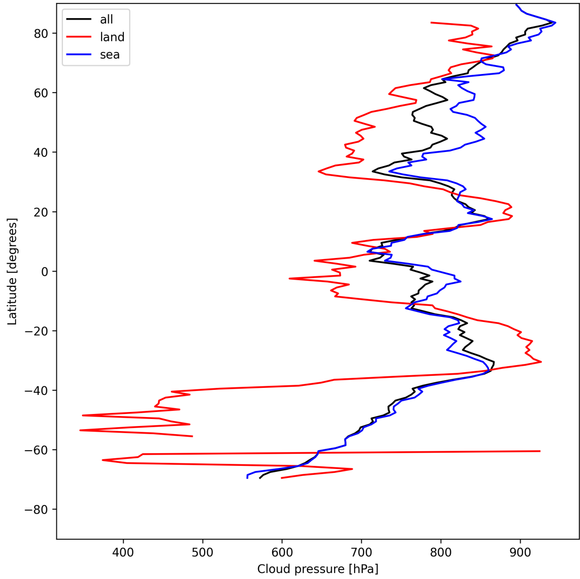
Figure 13: Zonal average of “Cloud pressure” for 2025-05-10 to 2025-05-12.
