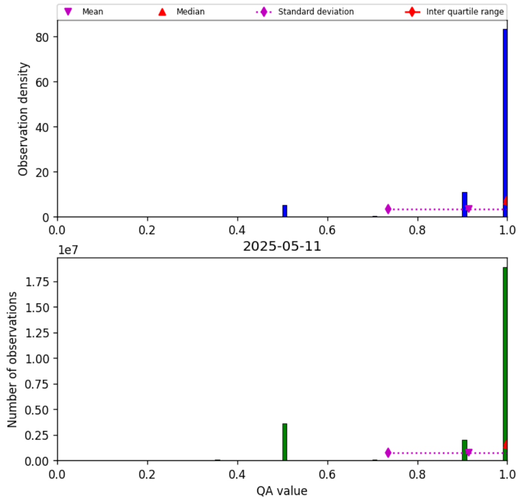
Figure 29: Histogram of “QA value” for 2025-05-10 to 2025-05-12
