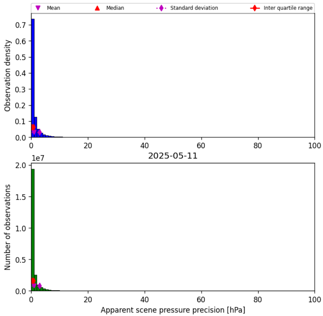
Figure 37: Histogram of “Apparent scene pressure precision” for 2025-05-10 to 2025-05-12
