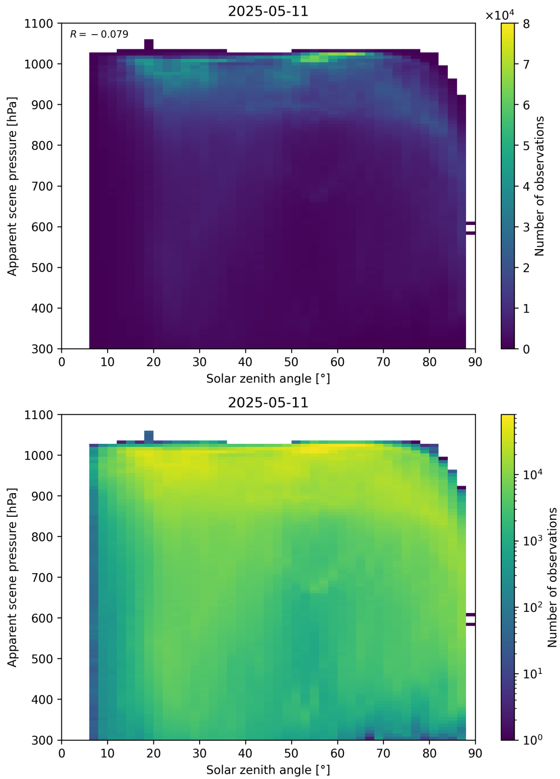
Figure 108: Scatter density plot of “Solar zenith angle” against “Apparent scene pressure” for 2025-05-10 to 2025-05-12.
