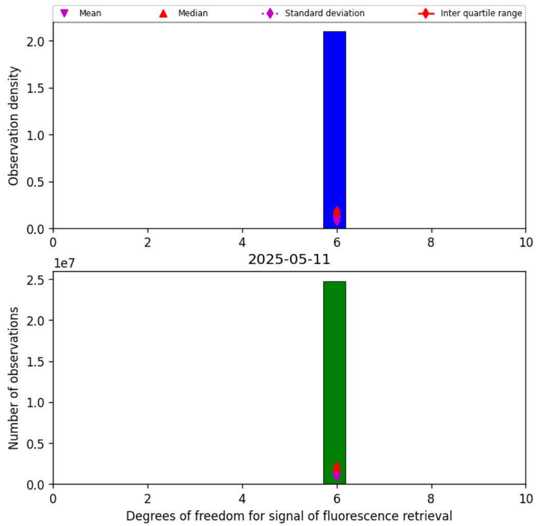
Figure 43: Histogram of “Degrees of freedom for signal of fluorescence retrieval” for 2025-05-10 to 2025-05-12
