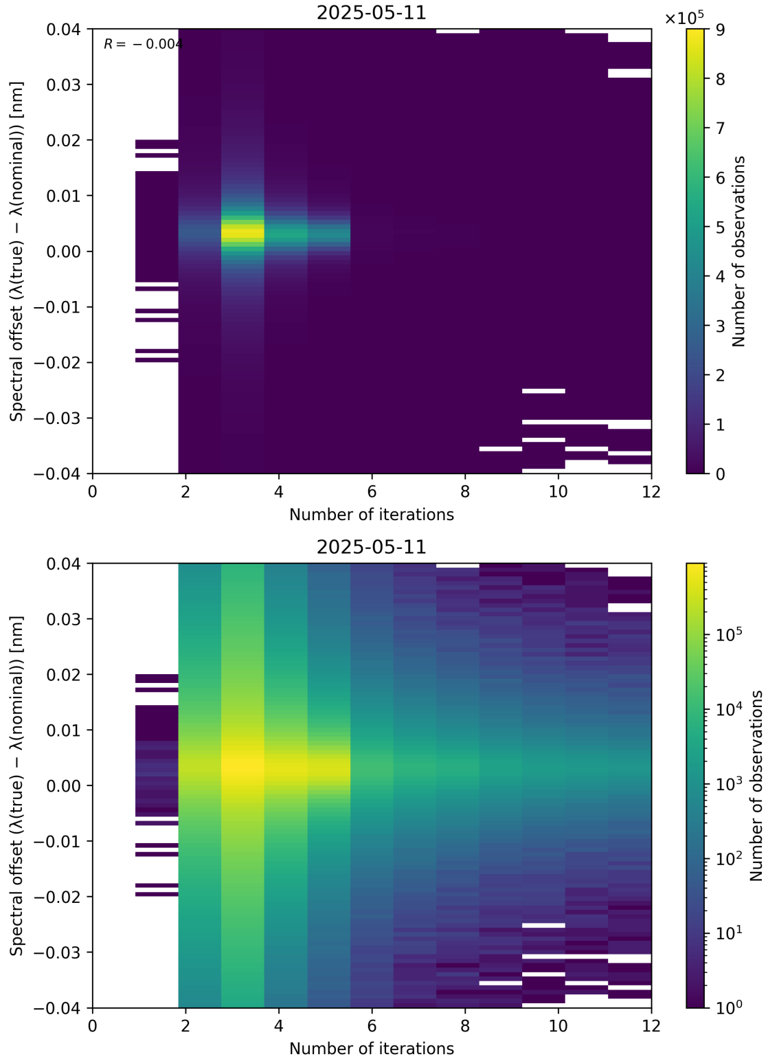
Figure 100: Scatter density plot of “Number of iterations” against “Spectral offset ( \lambda_{\text{true}} - \lambda_{\text{nominal}} )” for 2025-05-10 to 2025-05-12.
