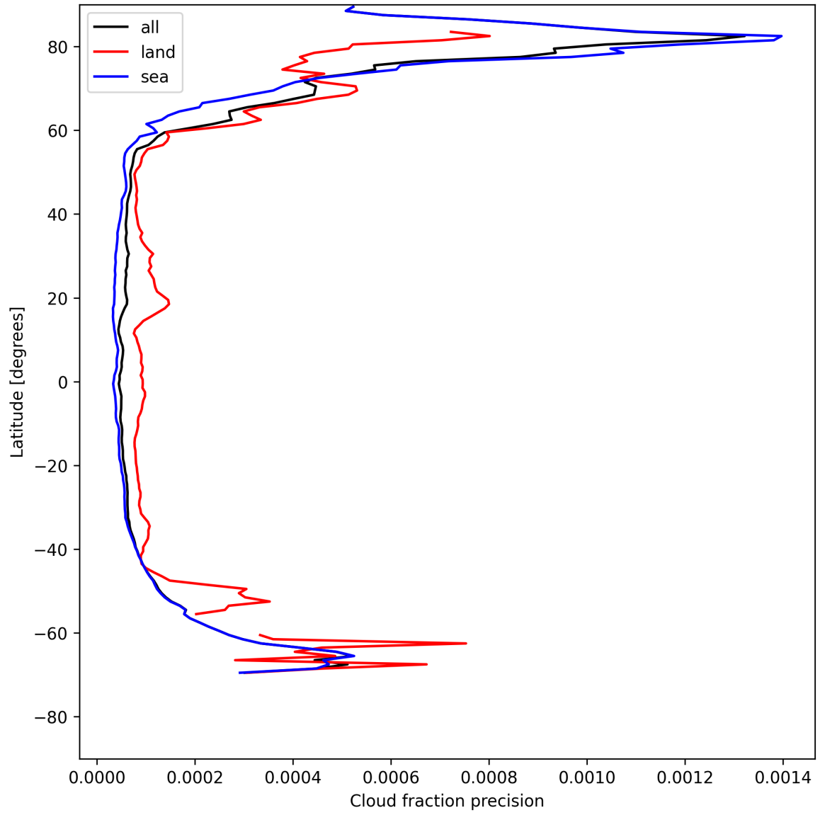
Figure 16: Zonal average of “Cloud fraction precision” for 2025-05-10 to 2025-05-12.
