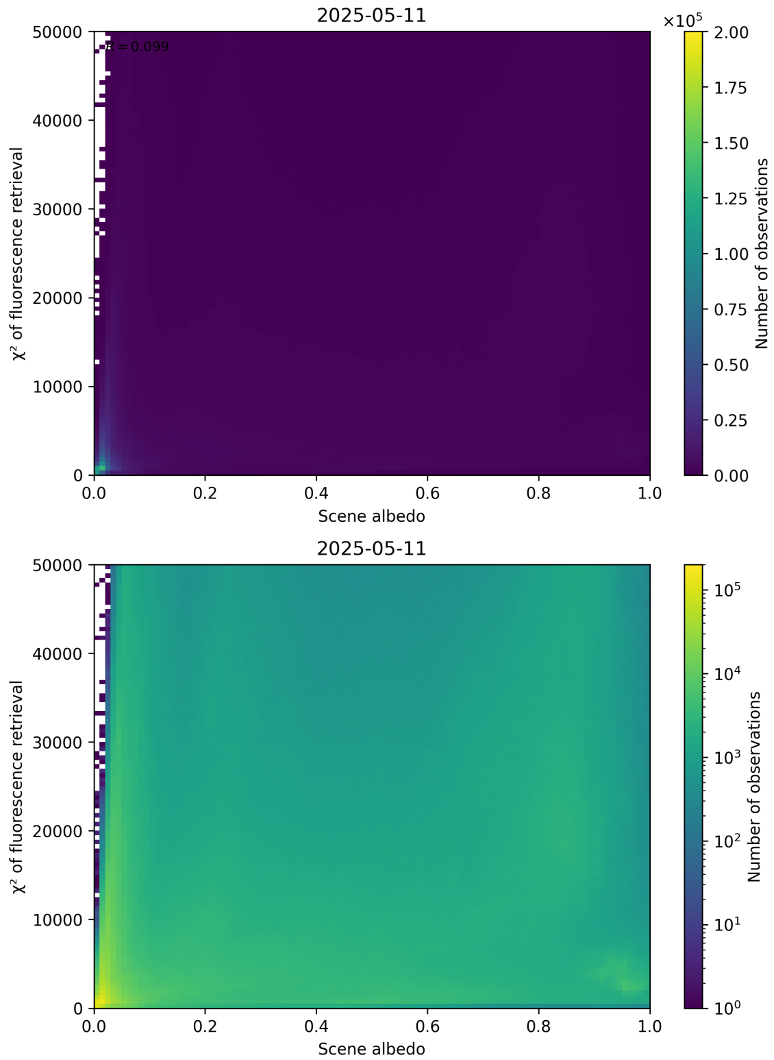
Figure 103: Scatter density plot of “Scene albedo” against “ \chi^2 of fluorescence retrieval” for 2025-05-10 to 2025-05-12.
