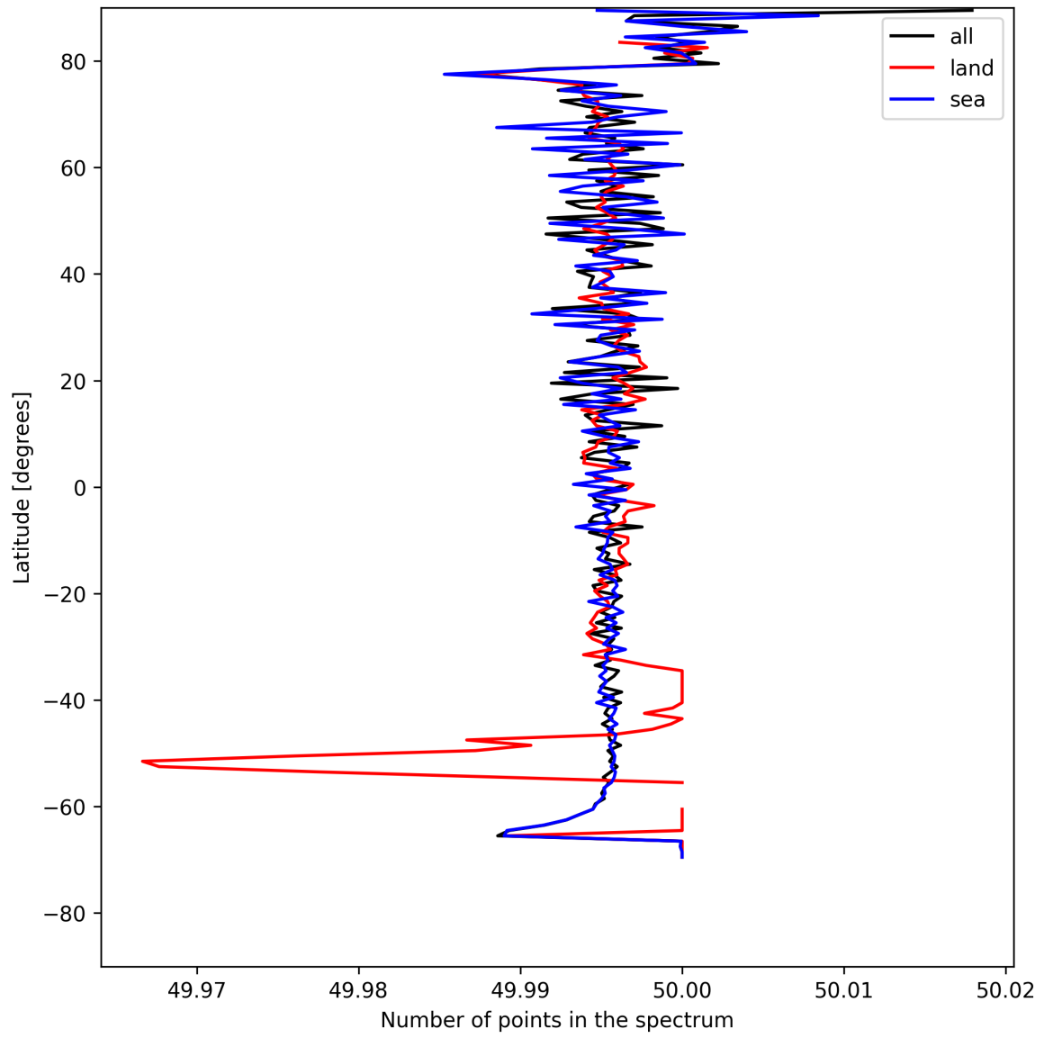
Figure 27: Zonal average of “Number of points in the spectrum” for 2025-05-10 to 2025-05-12.
