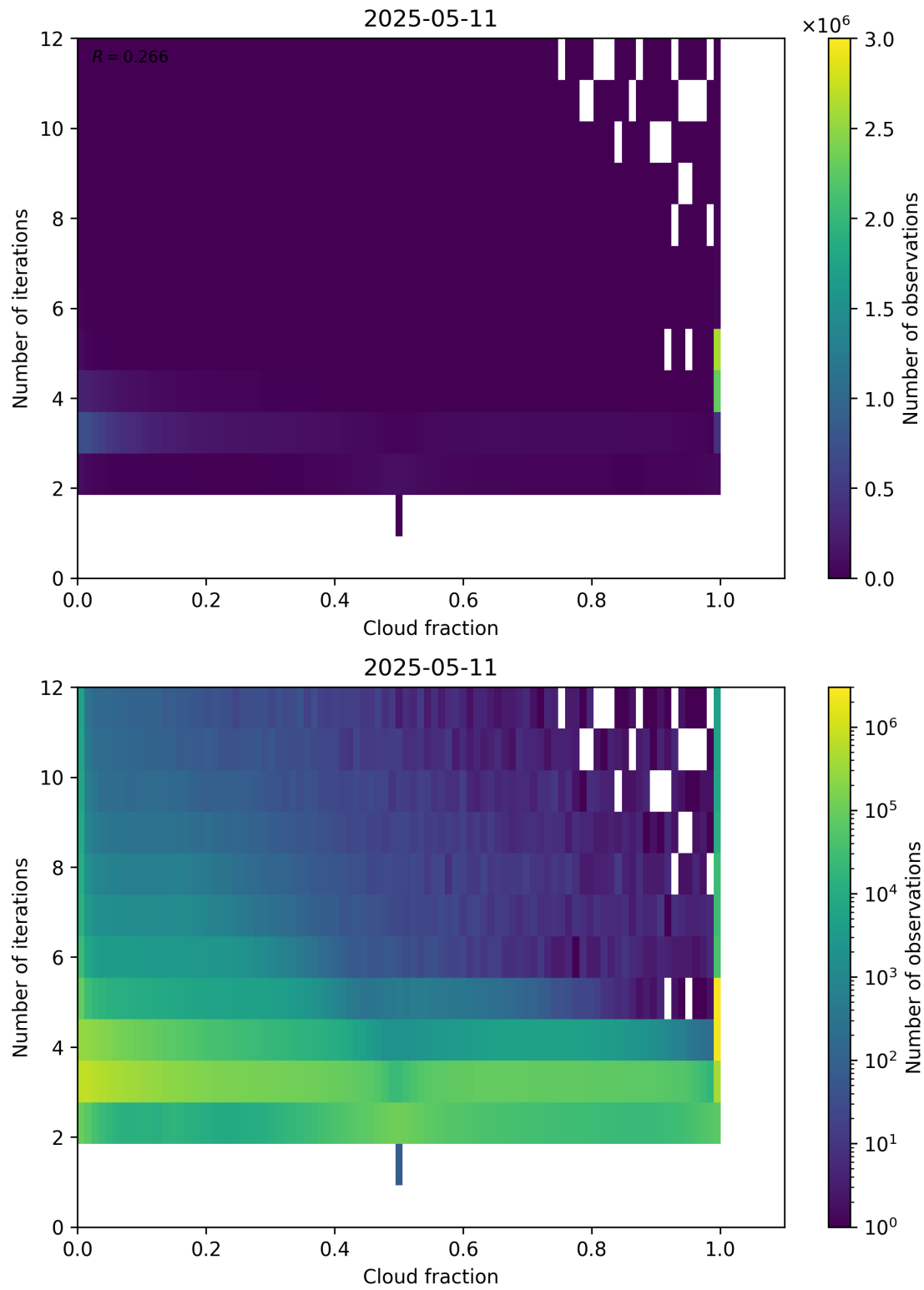
Figure 73: Scatter density plot of “Cloud fraction” against “Number of iterations” for 2025-05-10 to 2025-05-12.
