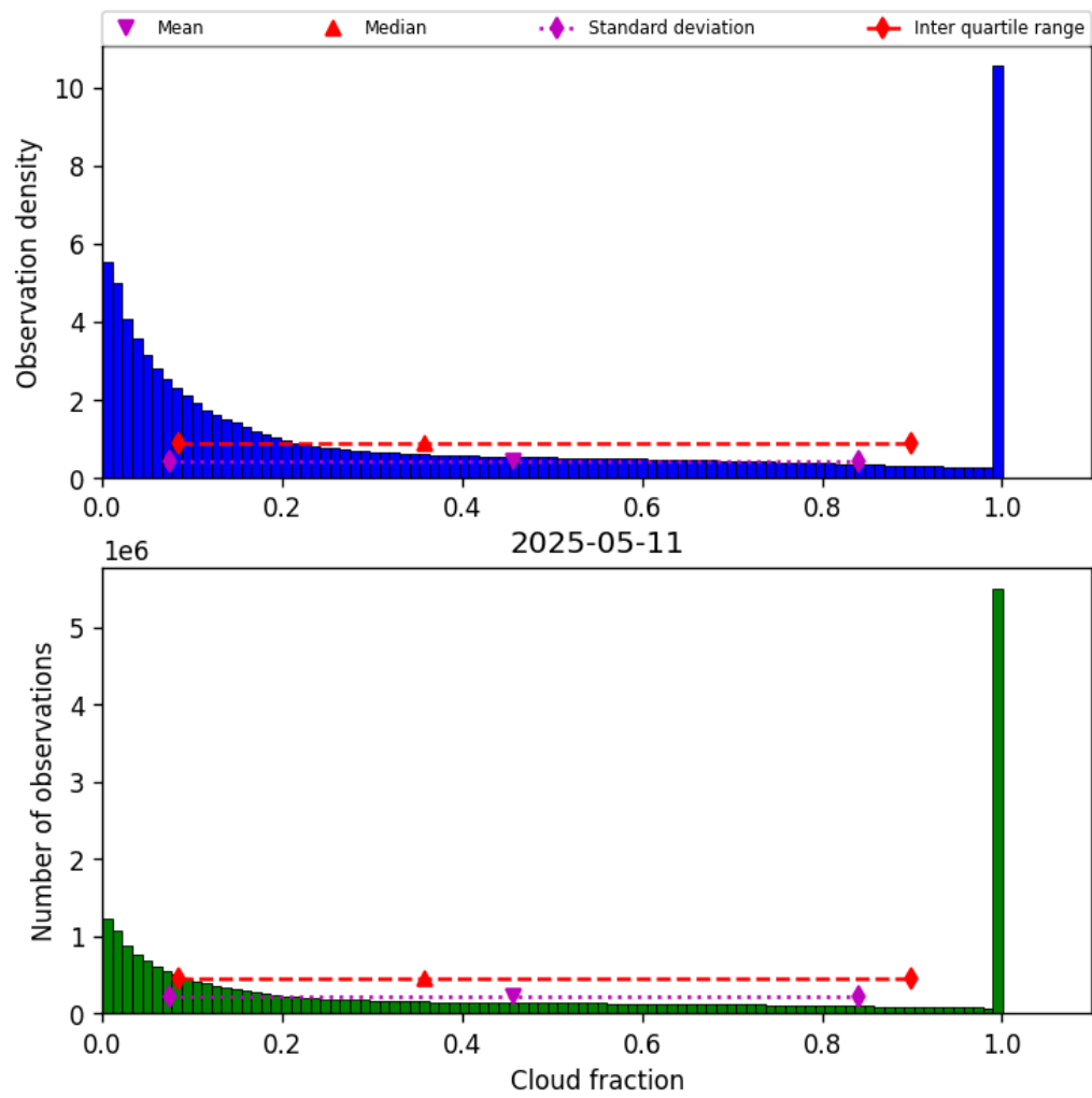
Figure 32: Histogram of “Cloud fraction” for 2025-05-10 to 2025-05-12
