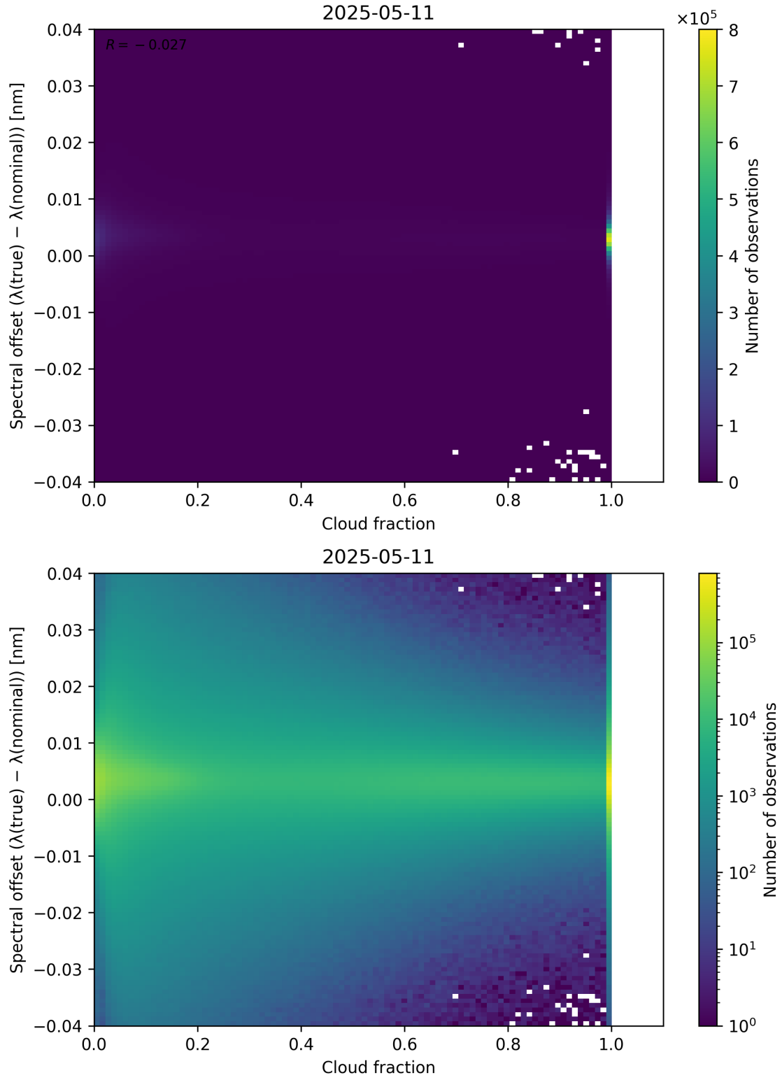
Figure 76: Scatter density plot of “Cloud fraction” against “Spectral offset ( \lambda_{\text{true}} - \lambda_{\text{nominal}} )” for 2025-05-10 to 2025-05-12.
