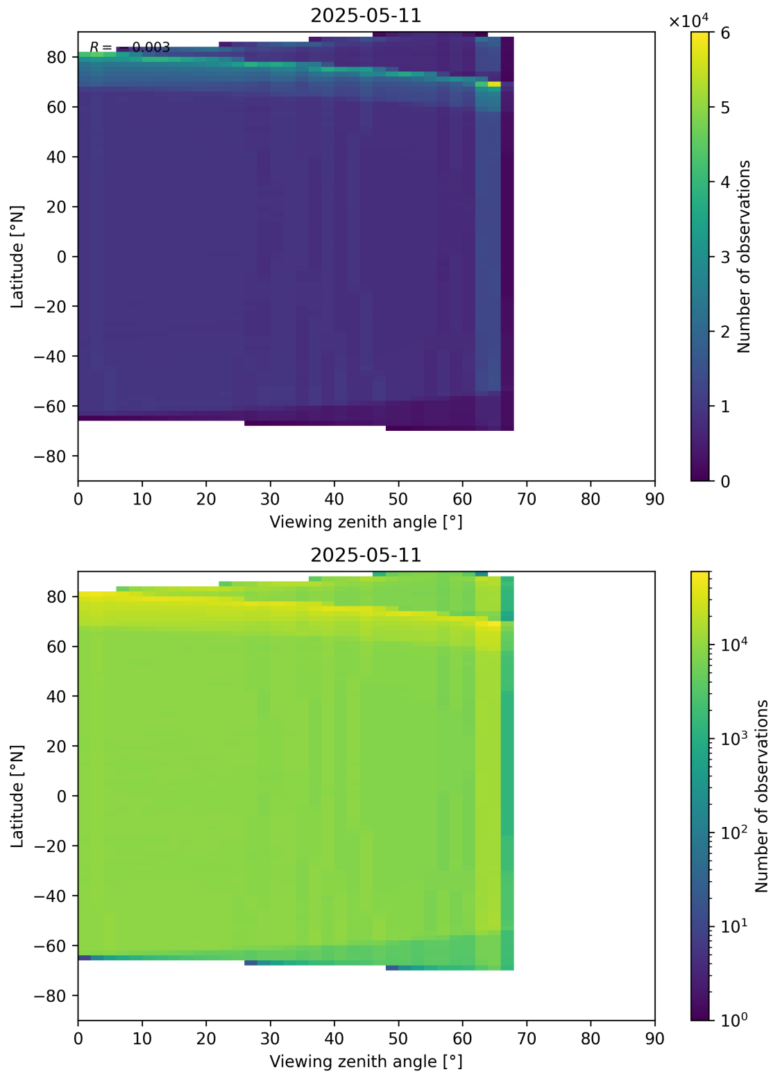
Figure 123: Scatter density plot of “Viewing zenith angle” against “Latitude” for 2025-05-10 to 2025-05-12.
