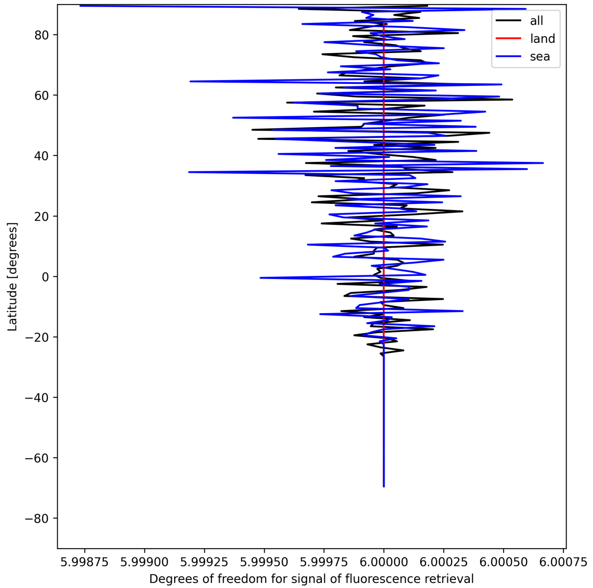
Figure 26: Zonal average of “Degrees of freedom for signal of fluorescence retrieval” for 2025-05-10 to 2025-05-12.
