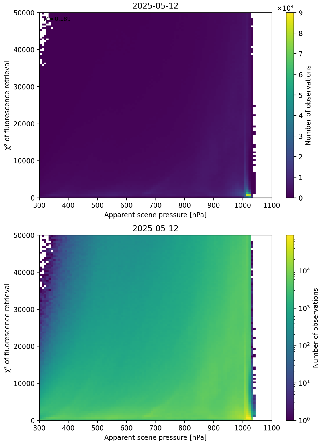
Figure 63: Scatter density plot of “Apparent scene pressure” against “ \chi^2 of fluorescence retrieval” for 2025-05-11 to 2025-05-13.
