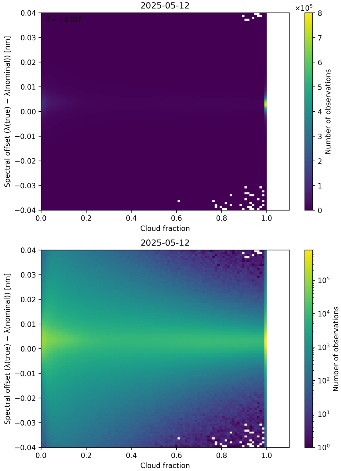
Figure 76: Scatter density plot of “Cloud fraction” against “Spectral offset ( \lambda_{\text{true}} - \lambda_{\text{nominal}} )” for 2025-05-11 to 2025-05-13.
