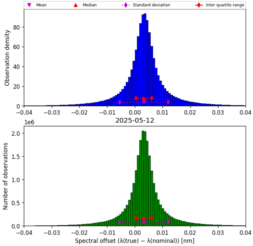
Figure 45: Histogram of “Spectral offset ( \lambda_{\text{true}} - \lambda_{\text{nominal}} )” for 2025-05-11 to 2025-05-13
