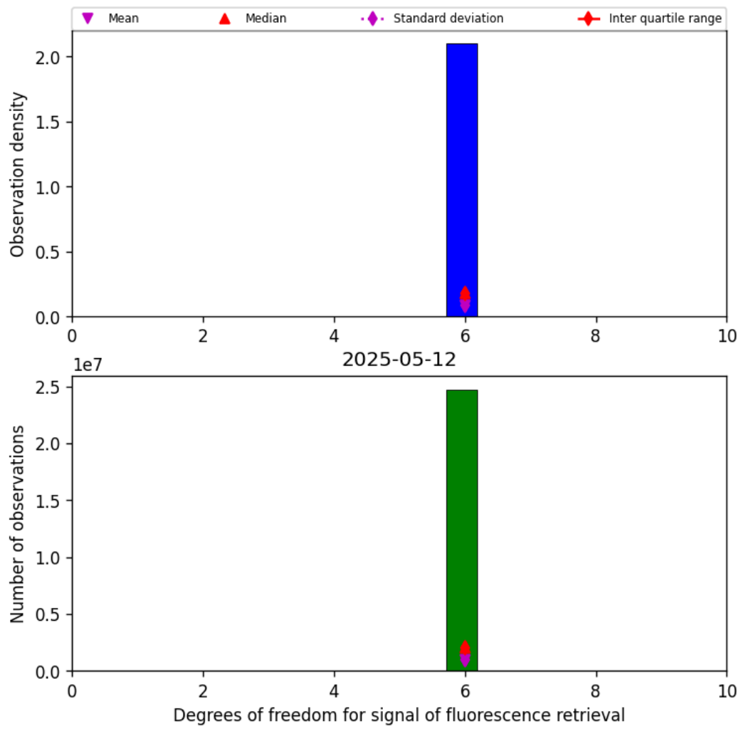
Figure 43: Histogram of “Degrees of freedom for signal of fluorescence retrieval” for 2025-05-11 to 2025-05-13
