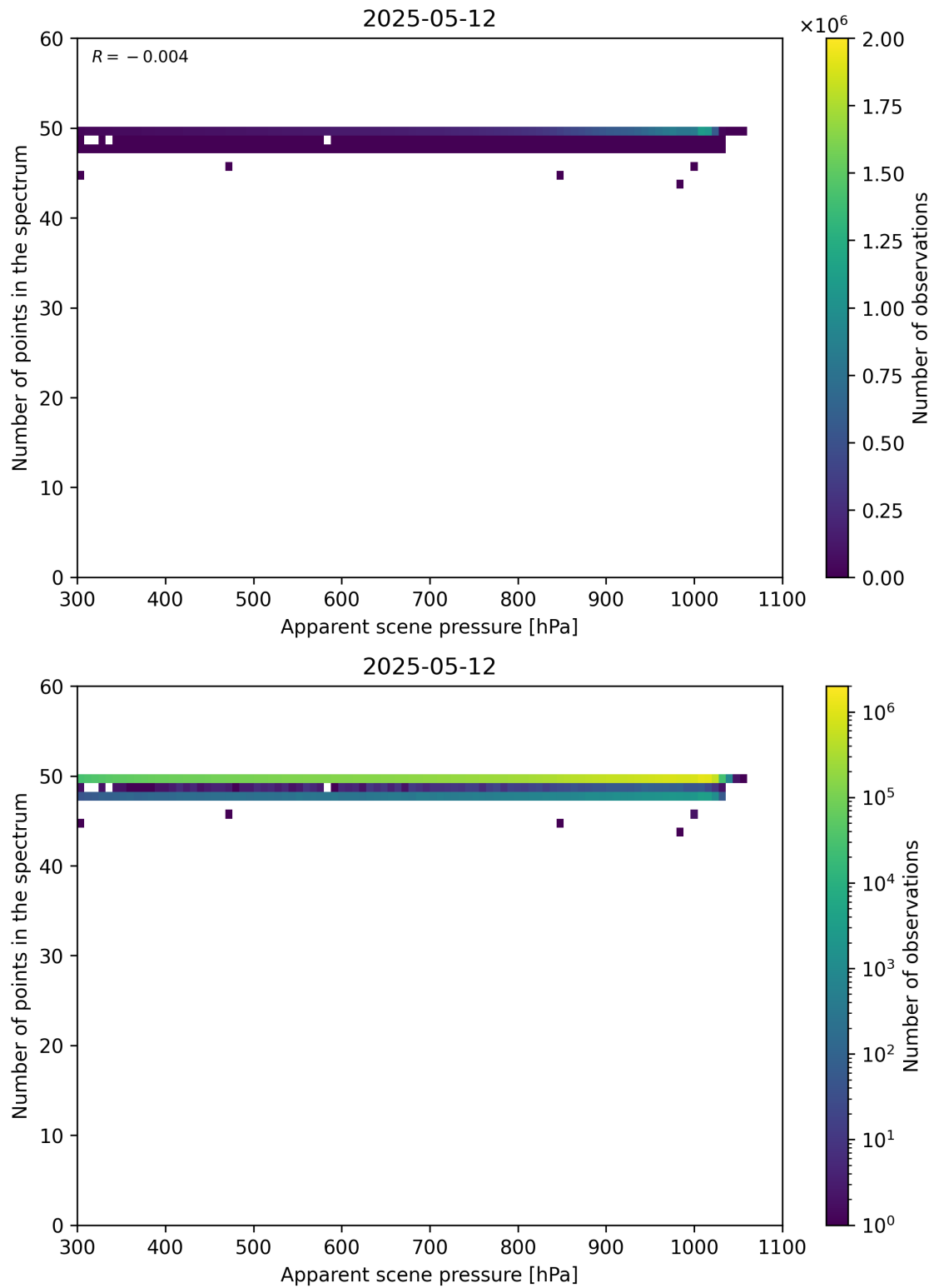
Figure 66: Scatter density plot of “Apparent scene pressure” against “Number of points in the spectrum” for 2025-05-11 to 2025-05-13.
