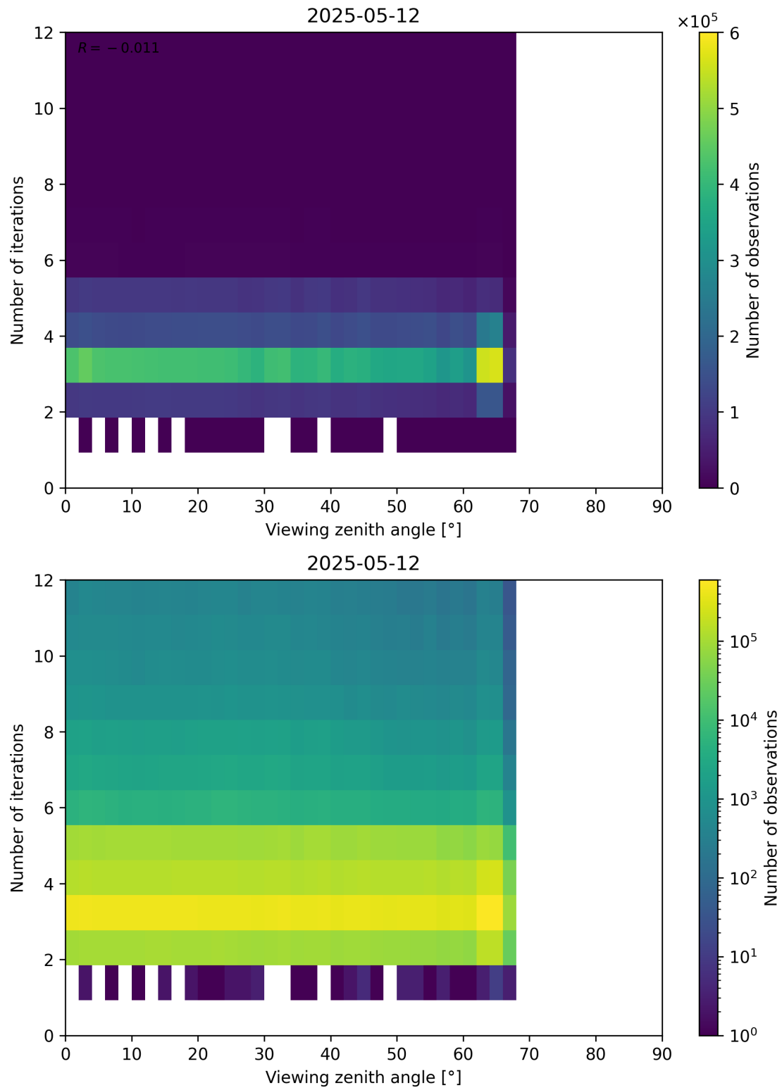
Figure 124: Scatter density plot of “Viewing zenith angle” against “Number of iterations” for 2025-05-11 to 2025-05-13.
