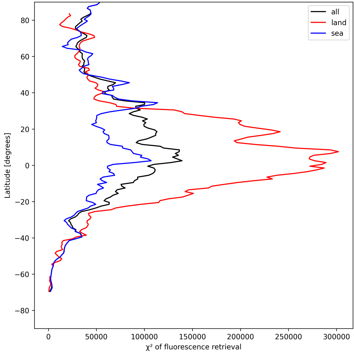
Figure 25: Zonal average of “ \chi^2 of fluorescence retrieval” for 2025-05-11 to 2025-05-13.
