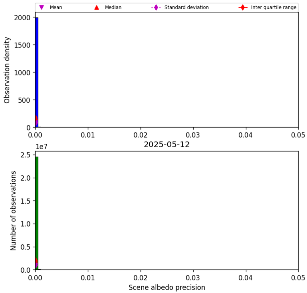
Figure 35: Histogram of “Scene albedo precision” for 2025-05-11 to 2025-05-13
