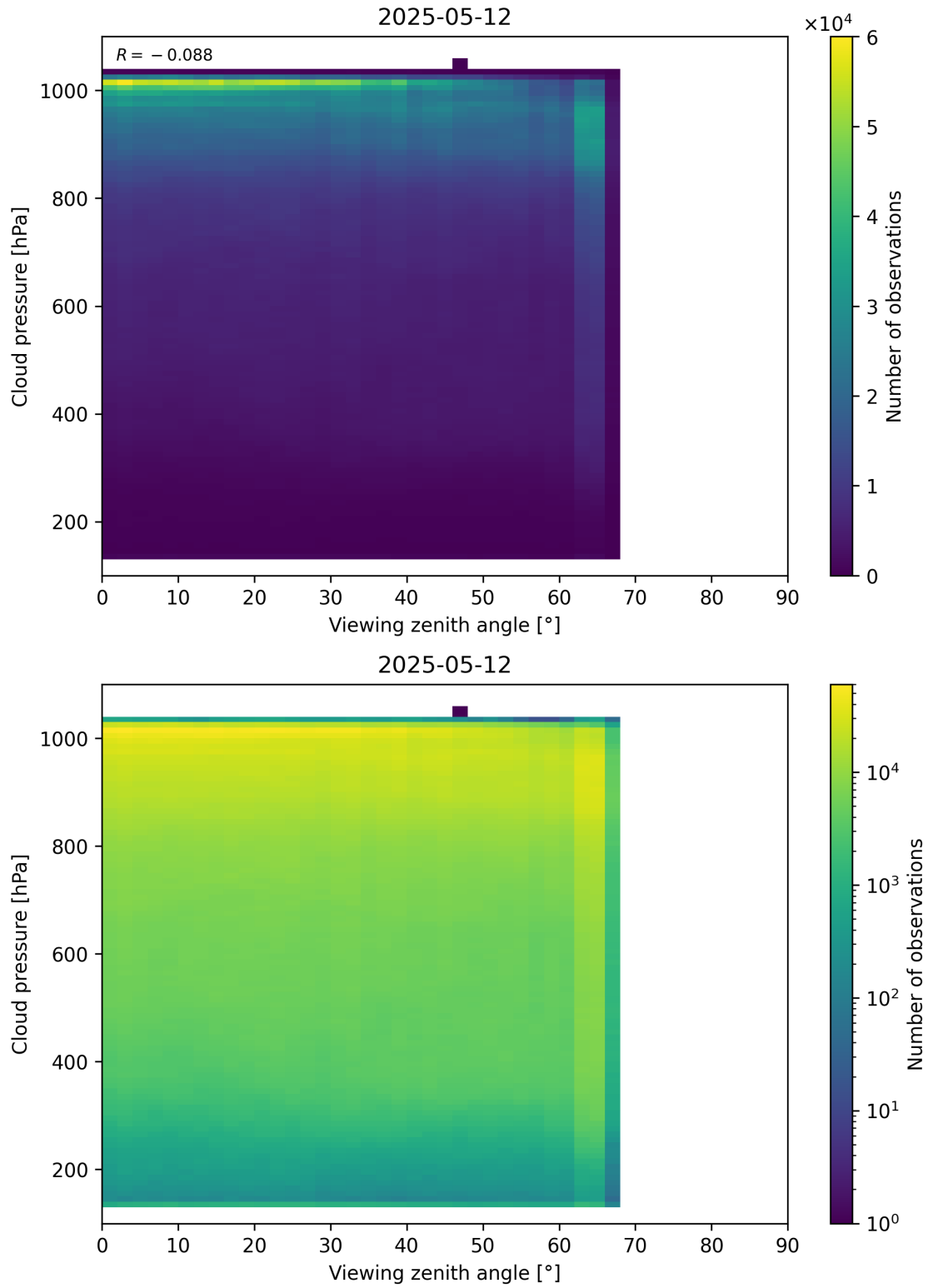
Figure 121: Scatter density plot of “Viewing zenith angle” against “Cloud pressure” for 2025-05-11 to 2025-05-13.
