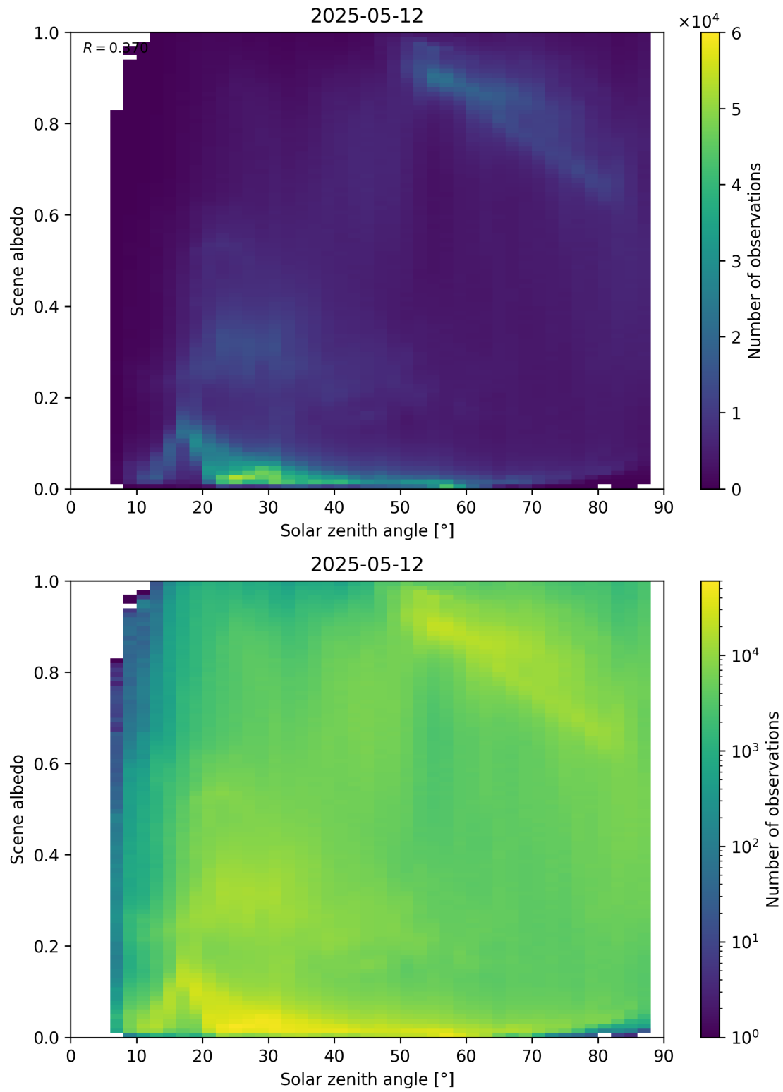
Figure 116: Scatter density plot of “Solar zenith angle” against “Scene albedo” for 2025-05-11 to 2025-05-13.
