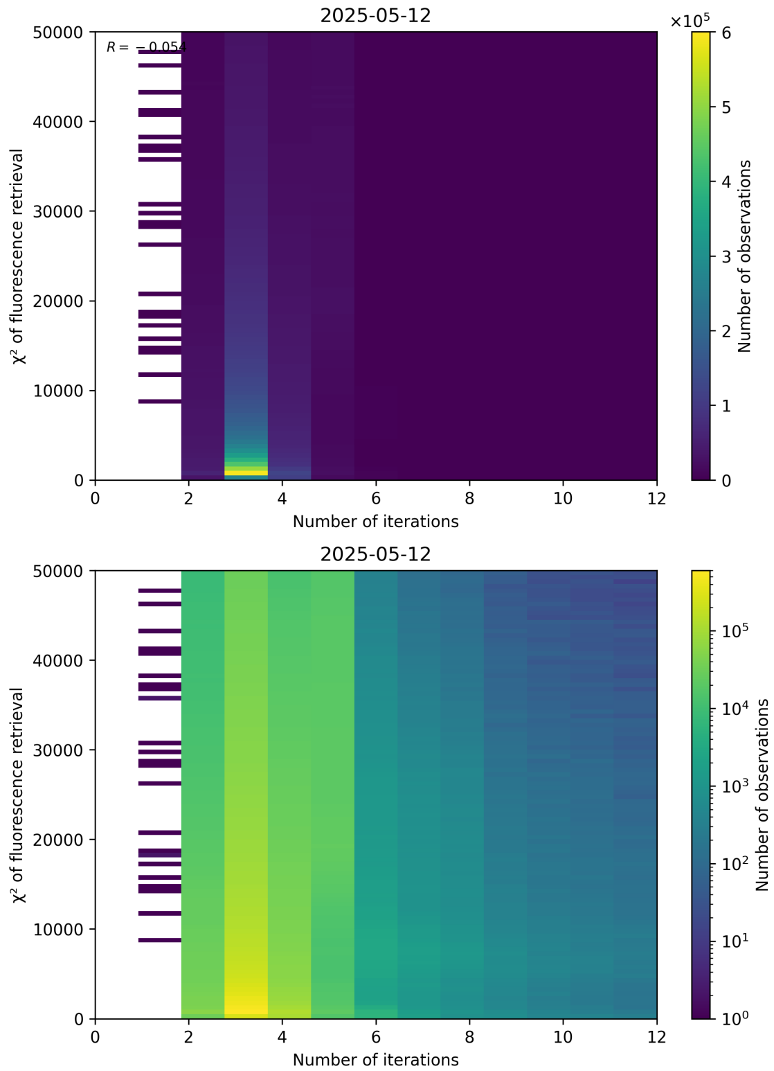
Figure 97: Scatter density plot of “Number of iterations” against “ \chi^2 of fluorescence retrieval” for 2025-05-11 to 2025-05-13.
