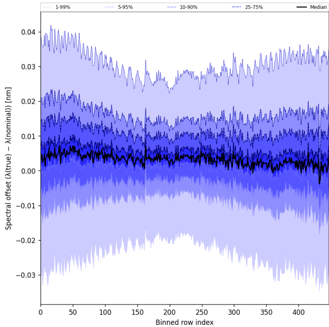
Figure 62: Along track statistics of “Spectral offset ( \lambda_{\text{true}} - \lambda_{\text{nominal}} )” for 2025-05-11 to 2025-05-13
