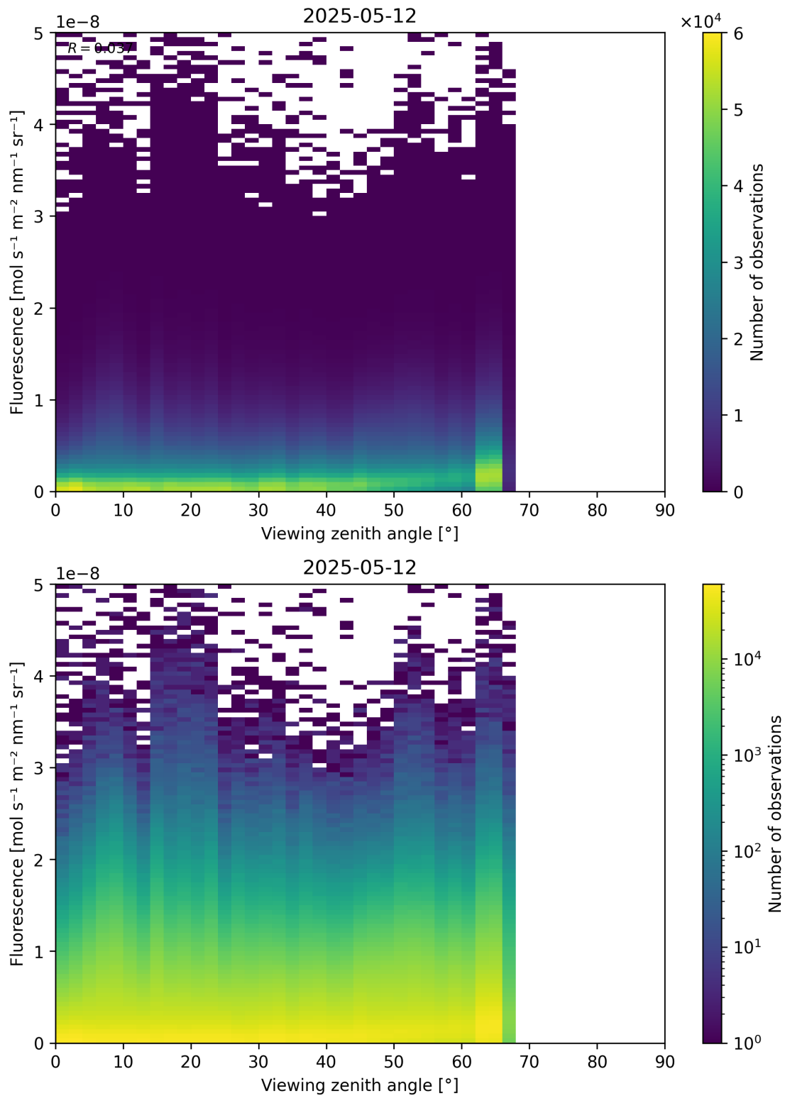
Figure 122: Scatter density plot of “Viewing zenith angle” against “Fluorescence” for 2025-05-11 to 2025-05-13.
