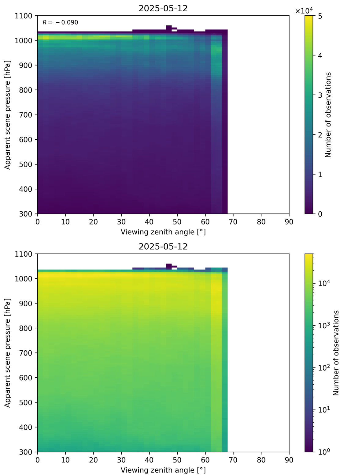
Figure 118: Scatter density plot of “Viewing zenith angle” against “Apparent scene pressure” for 2025-05-11 to 2025-05-13.
