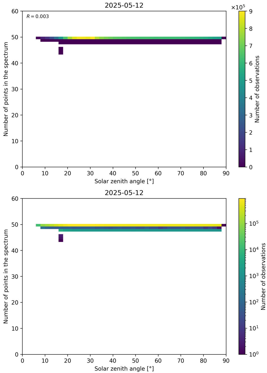
Figure 115: Scatter density plot of “Solar zenith angle” against “Number of points in the spectrum” for 2025-05-11 to 2025-05-13.
