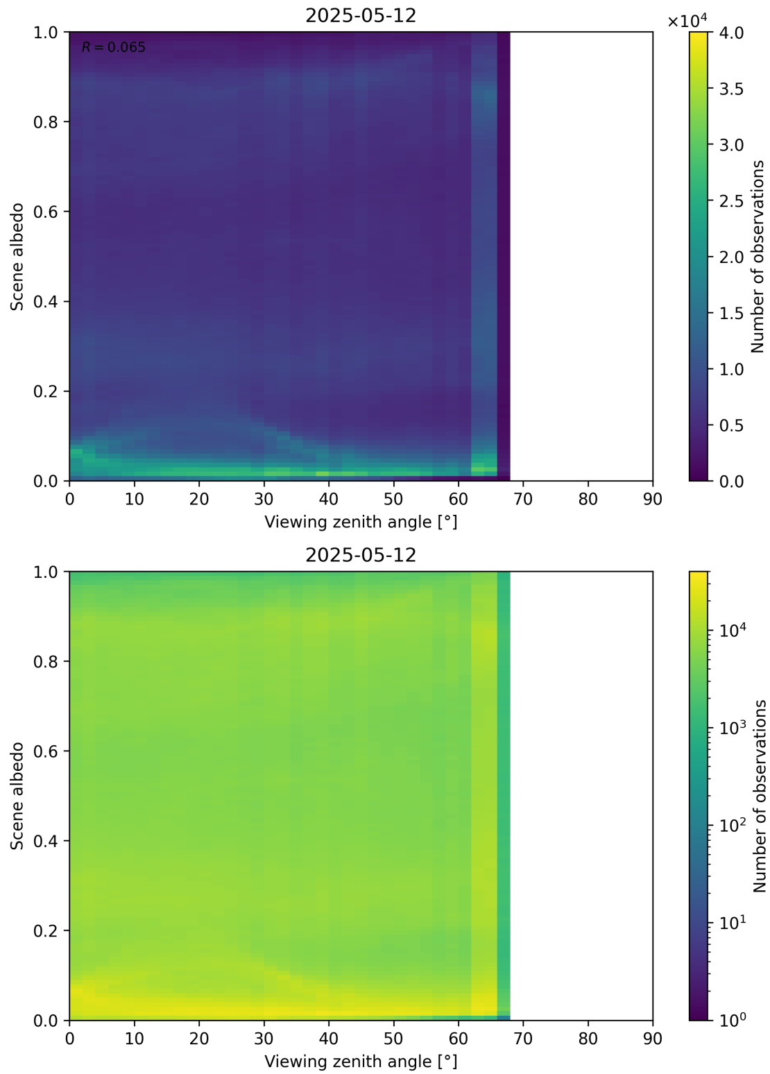
Figure 126: Scatter density plot of “Viewing zenith angle” against “Scene albedo” for 2025-05-11 to 2025-05-13.
