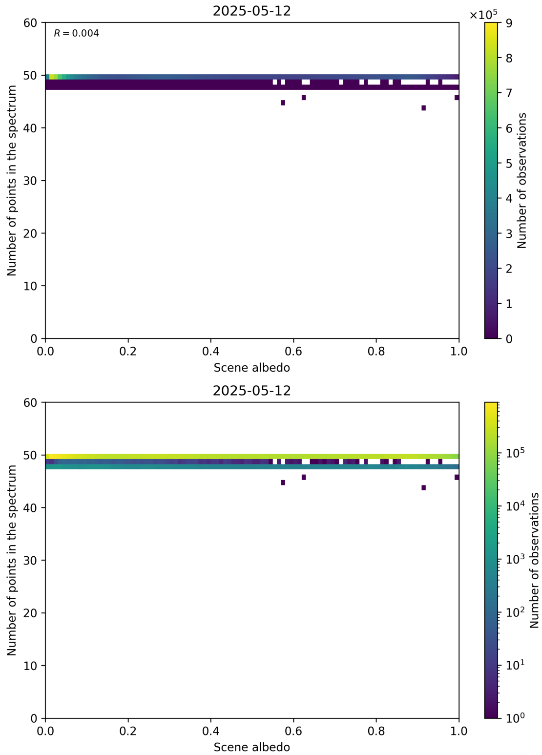
Figure 106: Scatter density plot of “Scene albedo” against “Number of points in the spectrum” for 2025-05-11 to 2025-05-13.
