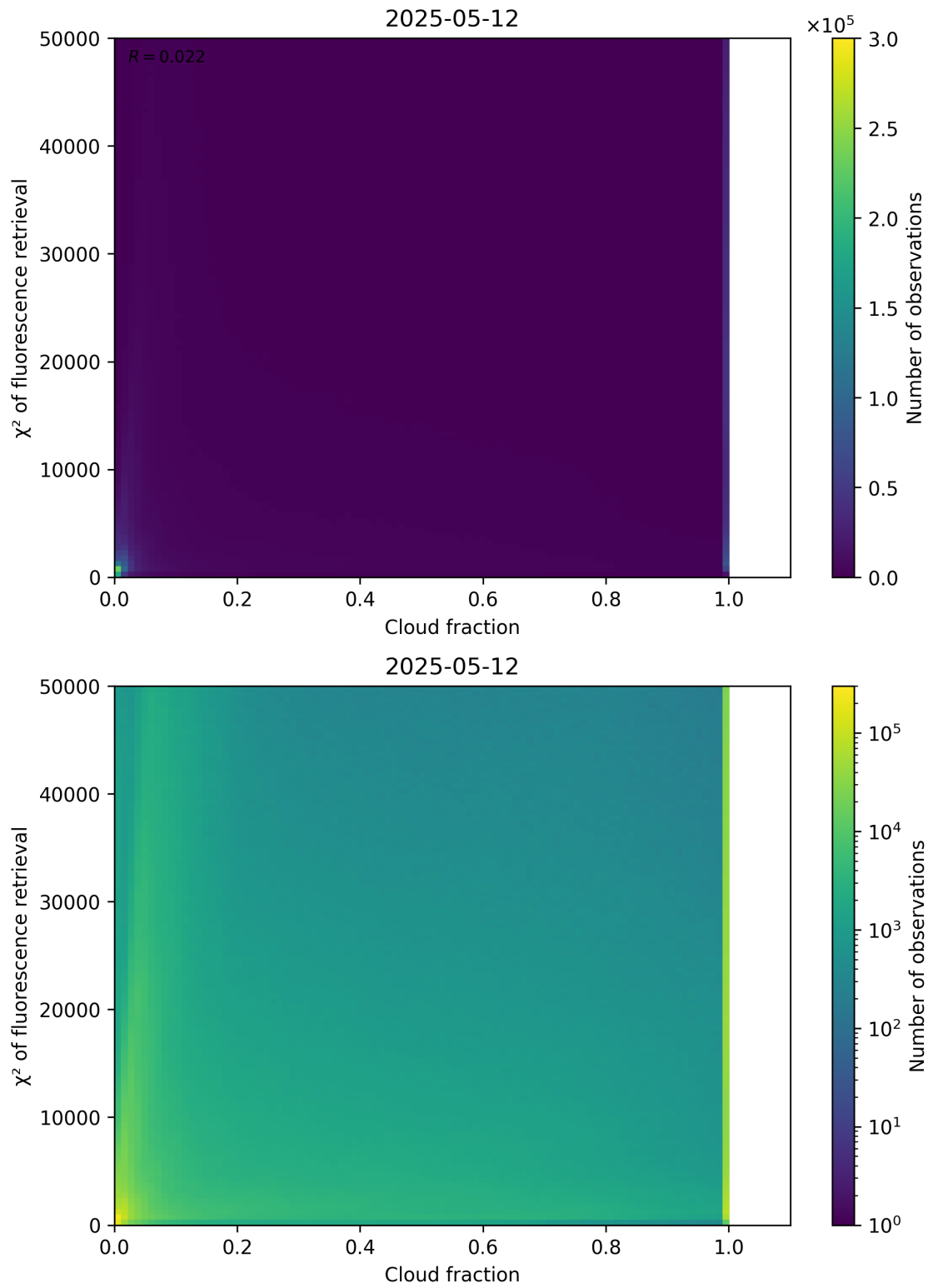
Figure 71: Scatter density plot of “Cloud fraction” against “ \chi^2 of fluorescence retrieval” for 2025-05-11 to 2025-05-13.
