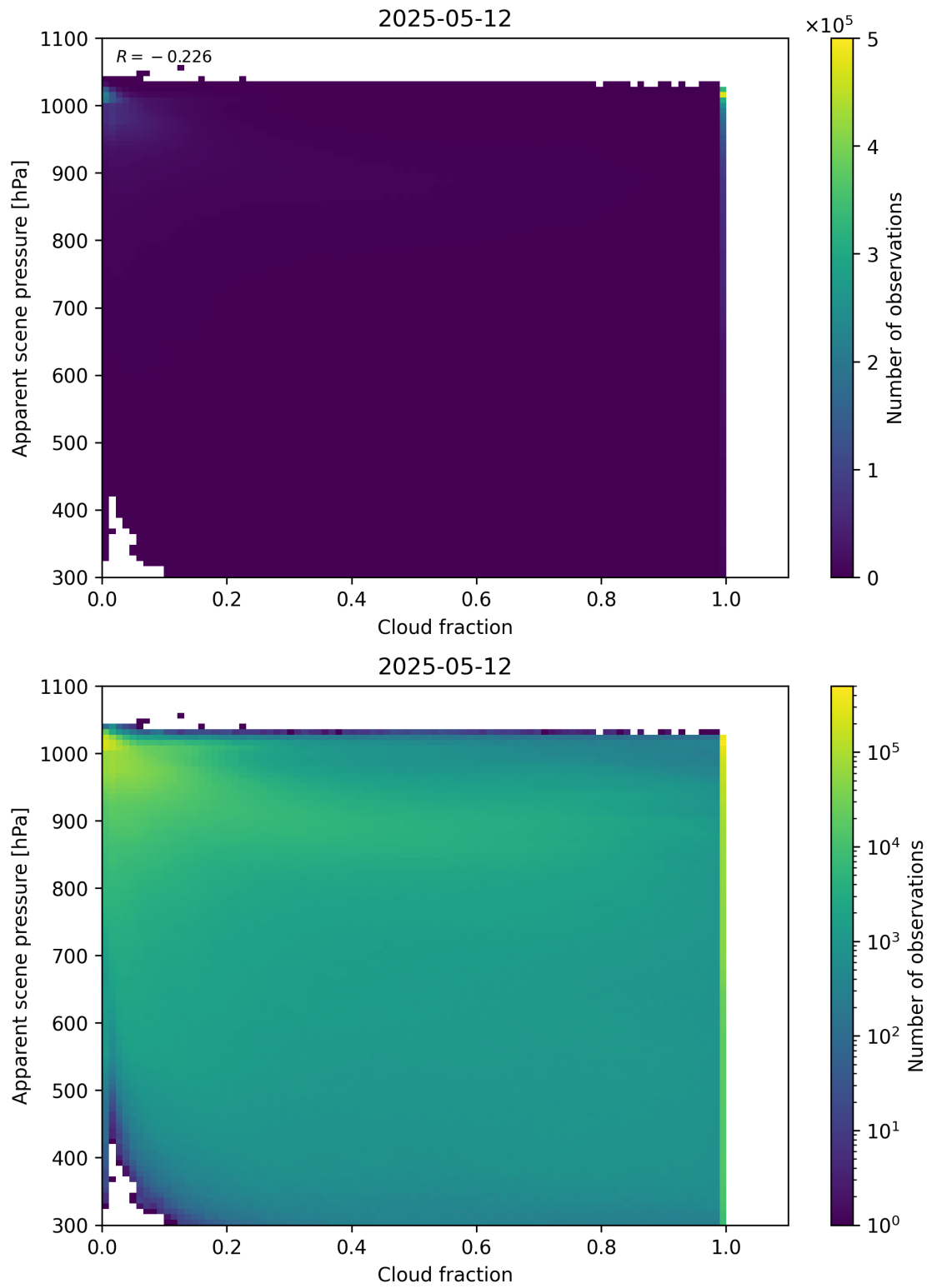
Figure 70: Scatter density plot of “Cloud fraction” against “Apparent scene pressure” for 2025-05-11 to 2025-05-13.
