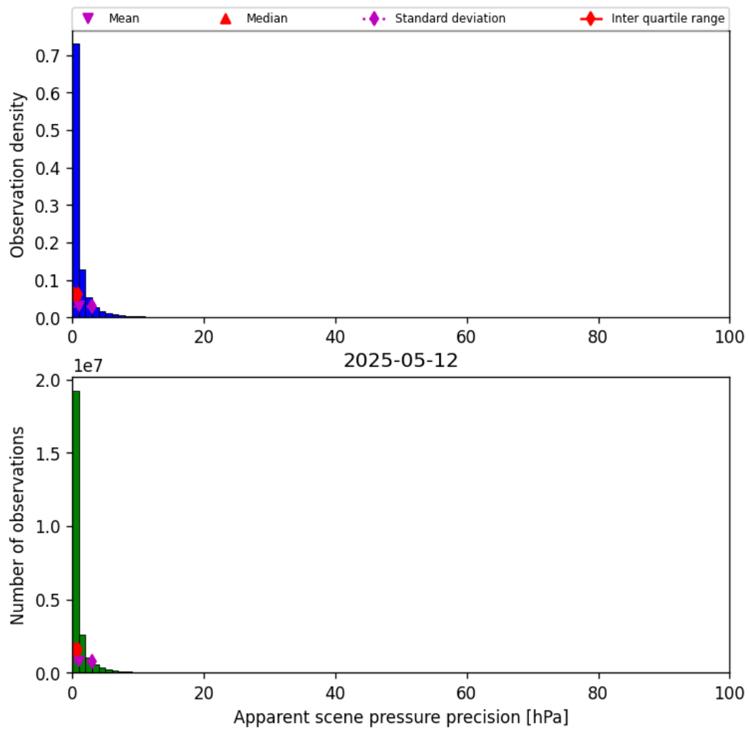
Figure 37: Histogram of “Apparent scene pressure precision” for 2025-05-11 to 2025-05-13
