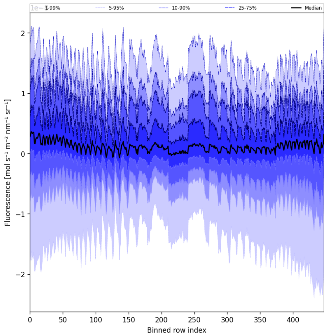
Figure 57: Along track statistics of “Fluorescence” for 2025-05-11 to 2025-05-13
