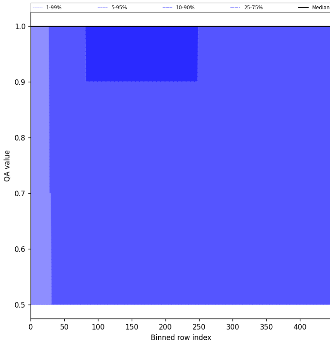
Figure 46: Along track statistics of “QA value” for 2025-05-11 to 2025-05-13
