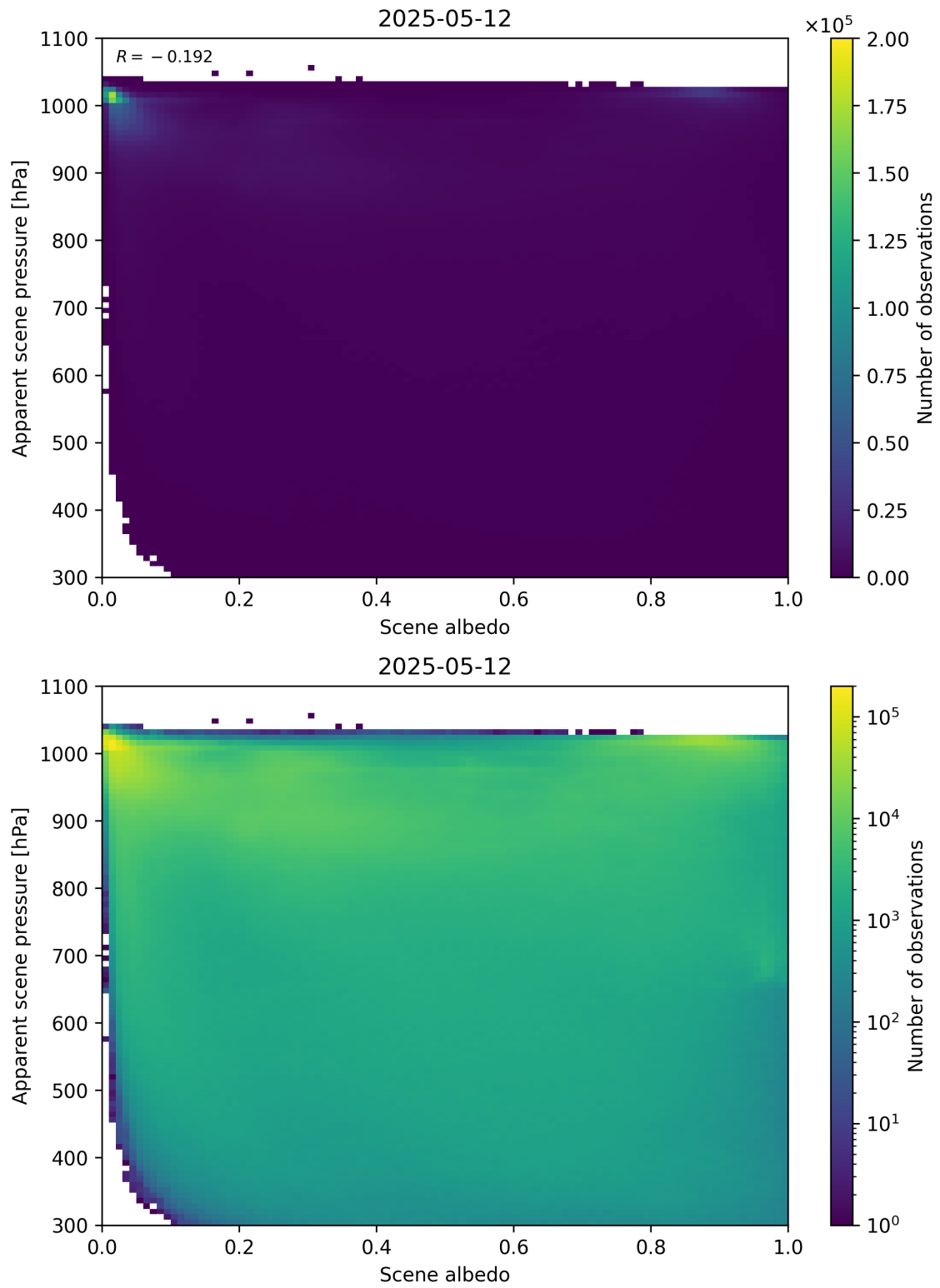
Figure 102: Scatter density plot of “Scene albedo” against “Apparent scene pressure” for 2025-05-11 to 2025-05-13.
