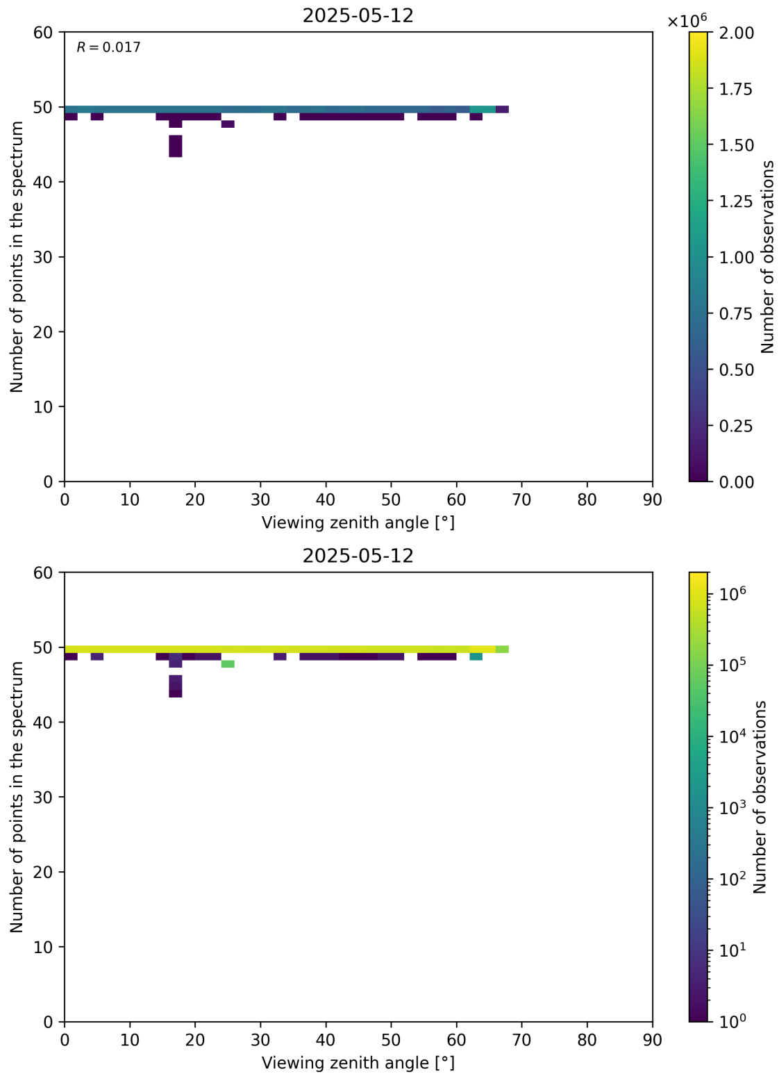
Figure 125: Scatter density plot of “Viewing zenith angle” against “Number of points in the spectrum” for 2025-05-11 to 2025-05-13.
