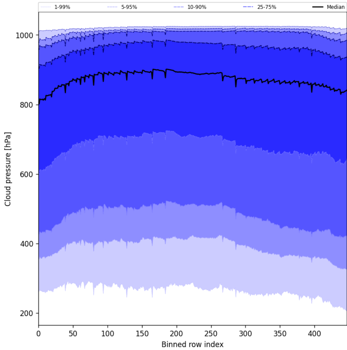
Figure 47: Along track statistics of “Cloud pressure” for 2025-05-11 to 2025-05-13
