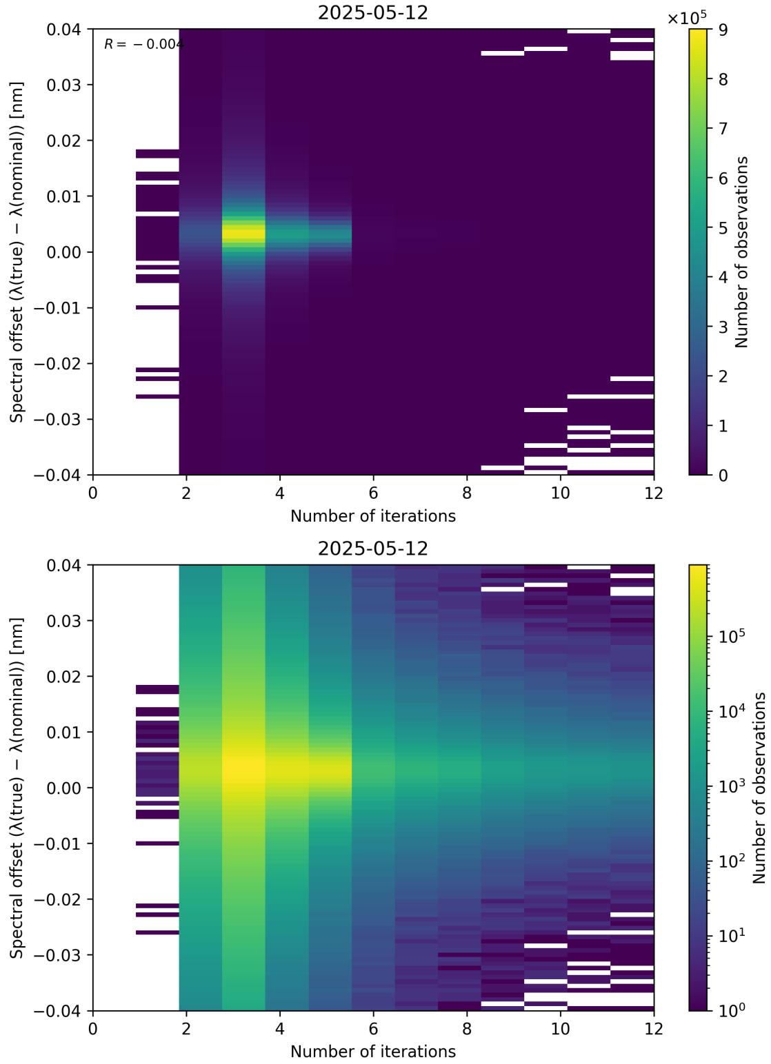
Figure 100: Scatter density plot of “Number of iterations” against “Spectral offset ( \lambda_{\text{true}} - \lambda_{\text{nominal}} )” for 2025-05-11 to 2025-05-13.
