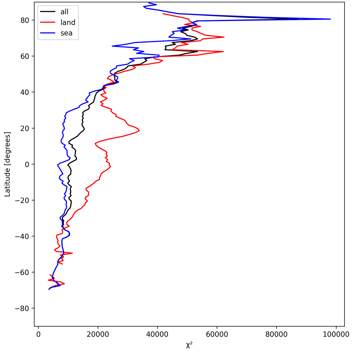
Figure 21: Zonal average of “ \chi^2 ” for 2025-05-11 to 2025-05-13.
