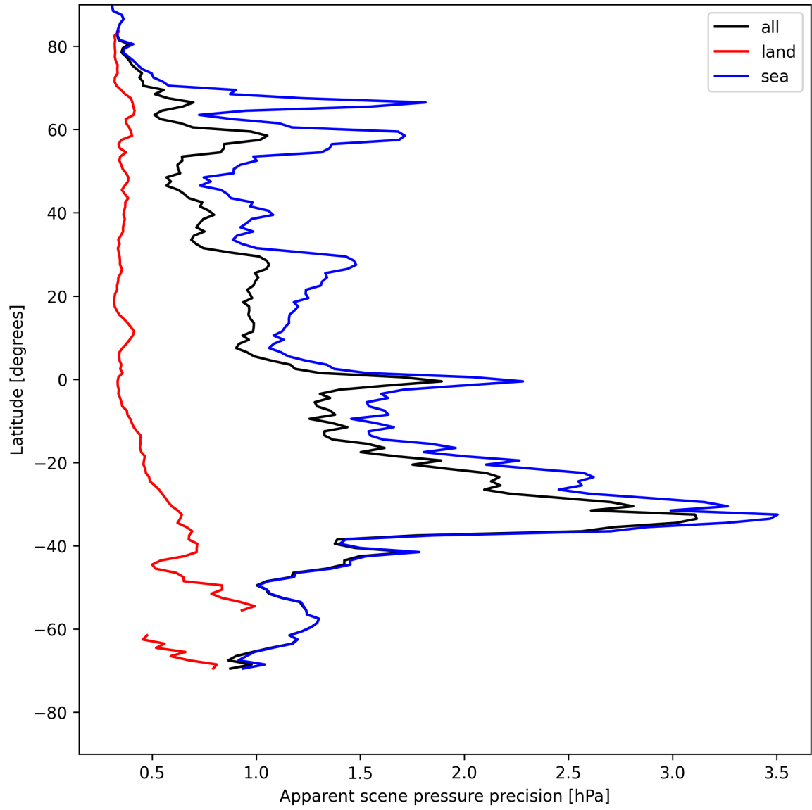
Figure 20: Zonal average of “Apparent scene pressure precision” for 2025-05-11 to 2025-05-13.
