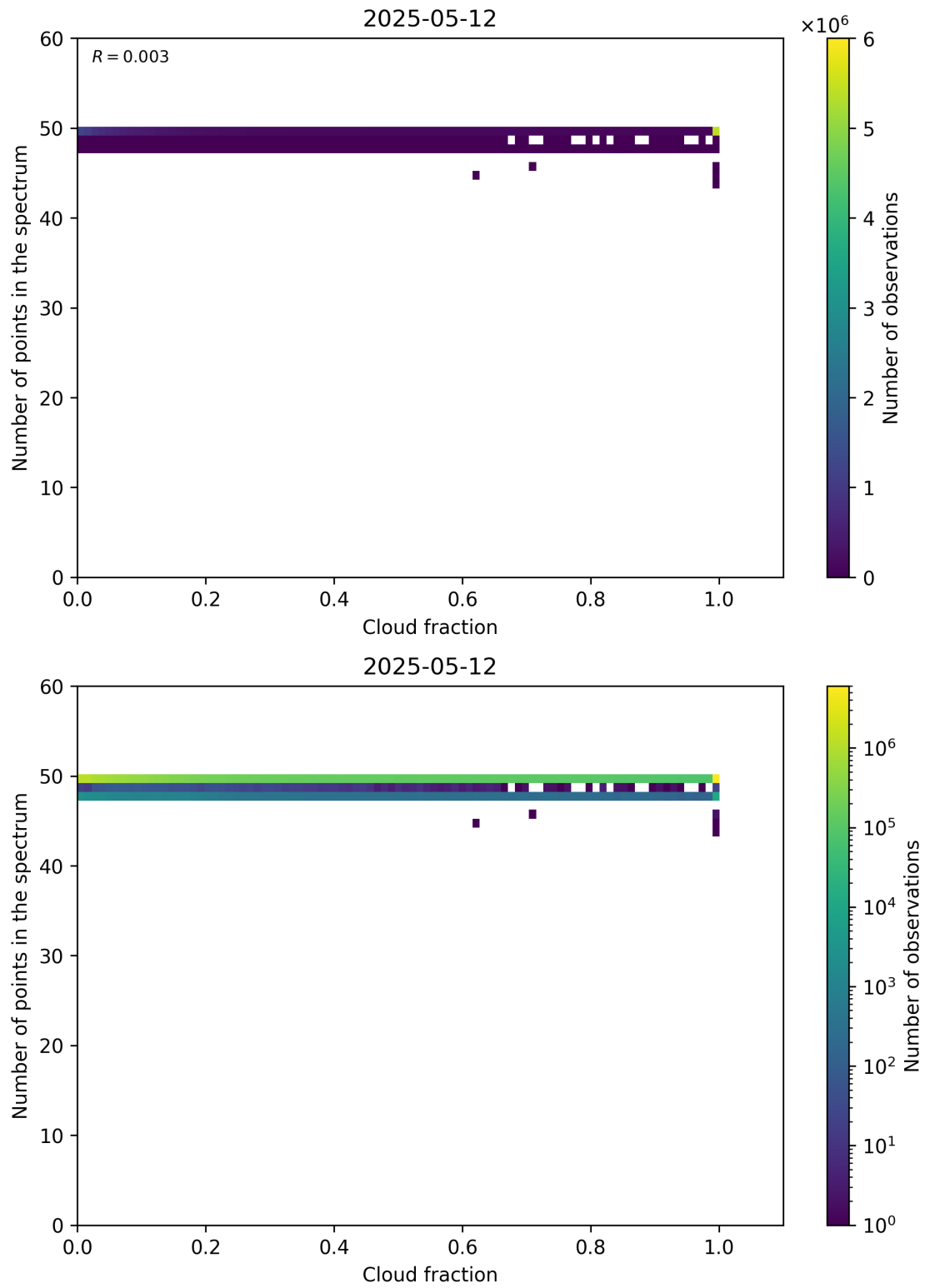
Figure 74: Scatter density plot of “Cloud fraction” against “Number of points in the spectrum” for 2025-05-11 to 2025-05-13.
