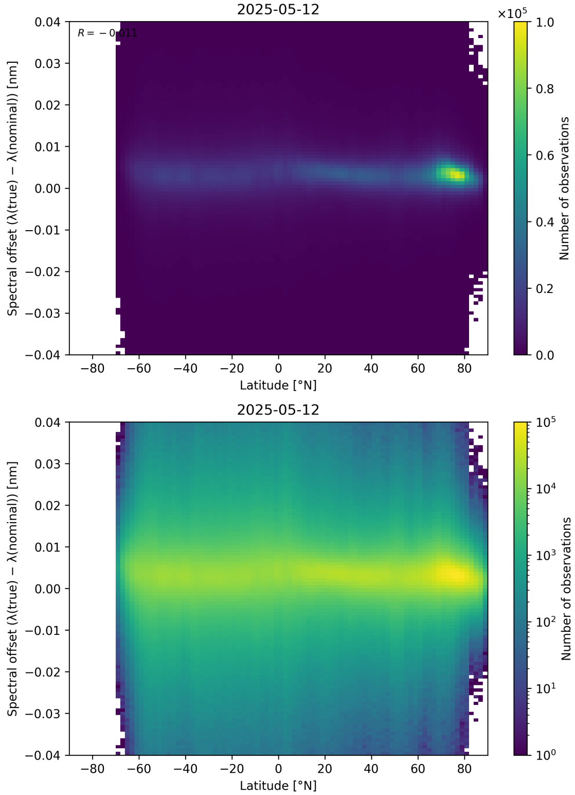
Figure 96: Scatter density plot of “Latitude” against “Spectral offset ( \lambda_{\text{true}} - \lambda_{\text{nominal}} )” for 2025-05-11 to 2025-05-13.
