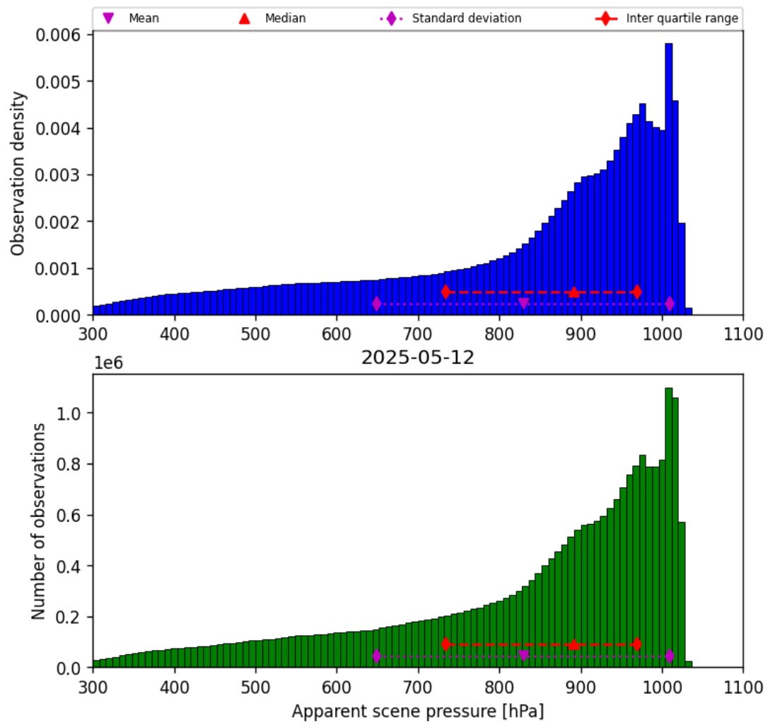
Figure 36: Histogram of “Apparent scene pressure” for 2025-05-11 to 2025-05-13
