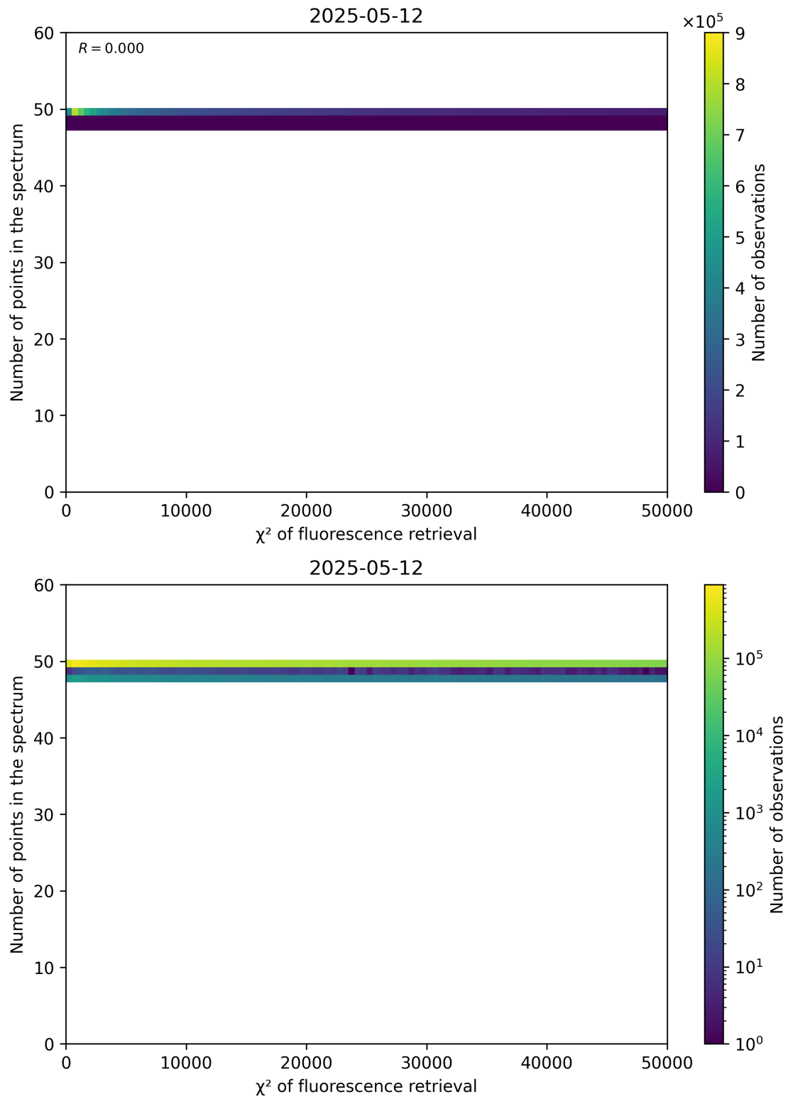
Figure 68: Scatter density plot of " \chi^2 of fluorescence retrieval" against "Number of points in the spectrum" for 2025-05-11 to 2025-05-13.
