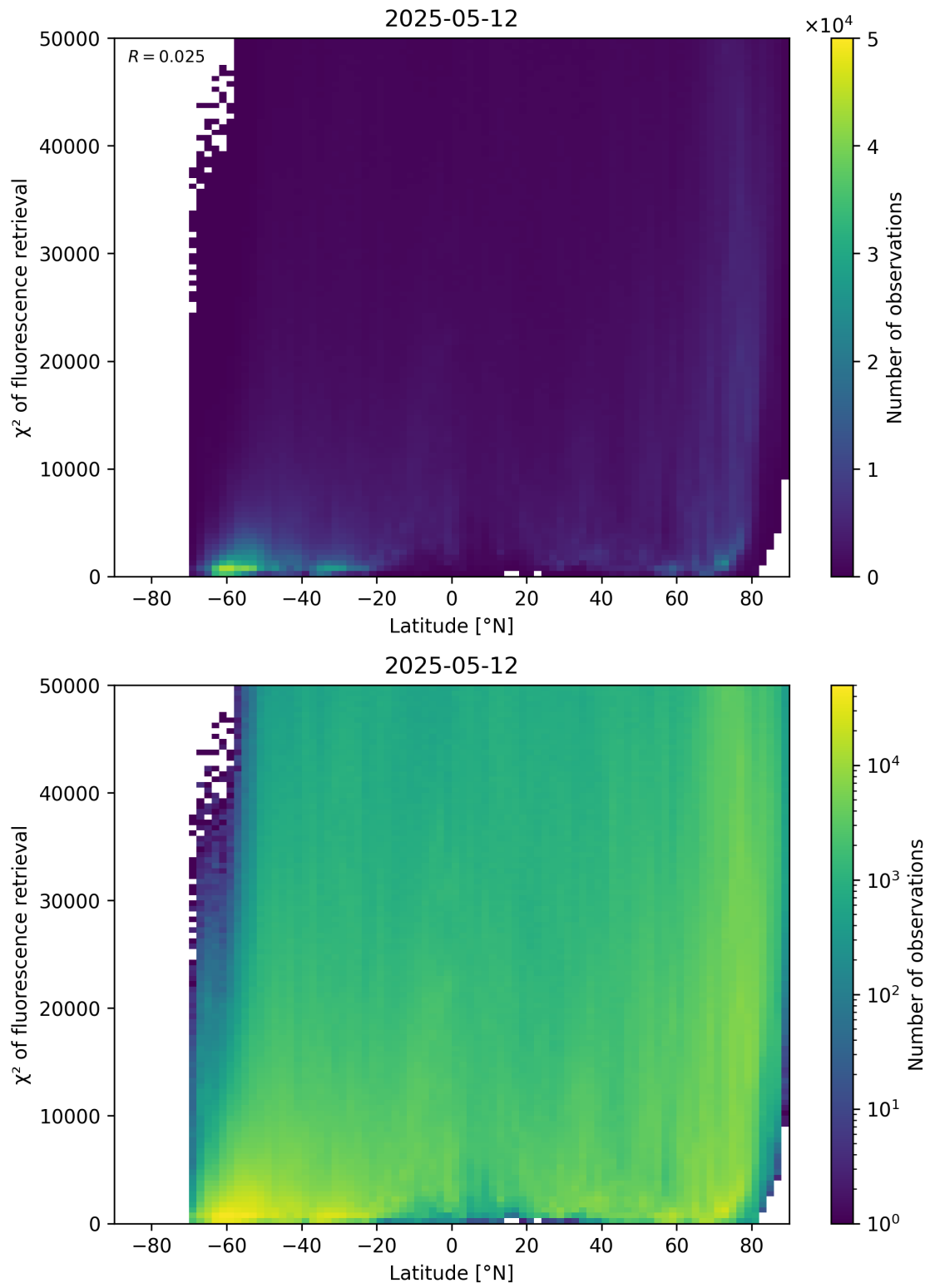
Figure 89: Scatter density plot of “Latitude” against “ \chi^2 of fluorescence retrieval” for 2025-05-11 to 2025-05-13.
