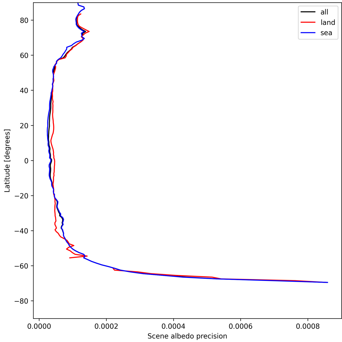
Figure 18: Zonal average of “Scene albedo precision” for 2025-05-11 to 2025-05-13.
