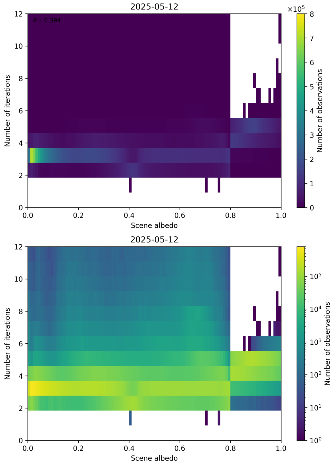
Figure 105: Scatter density plot of “Scene albedo” against “Number of iterations” for 2025-05-11 to 2025-05-13.
