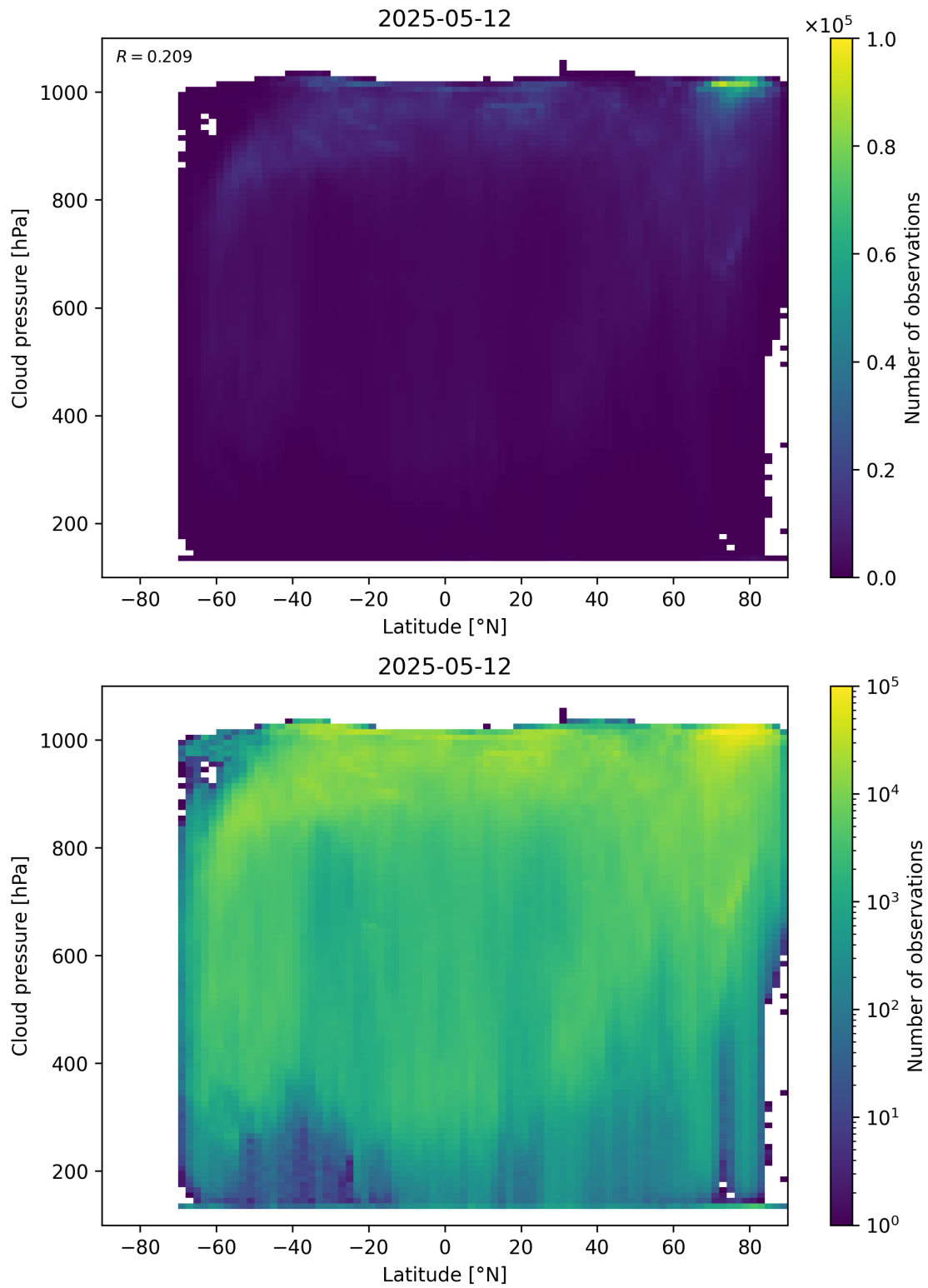
Figure 91: Scatter density plot of “Latitude” against “Cloud pressure” for 2025-05-11 to 2025-05-13.
