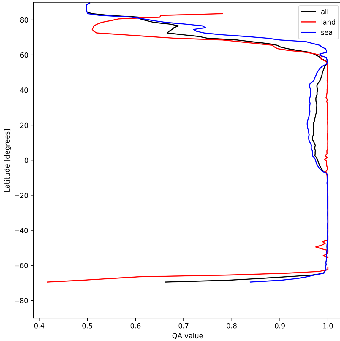
Figure 12: Zonal average of “QA value” for 2025-05-11 to 2025-05-13.
