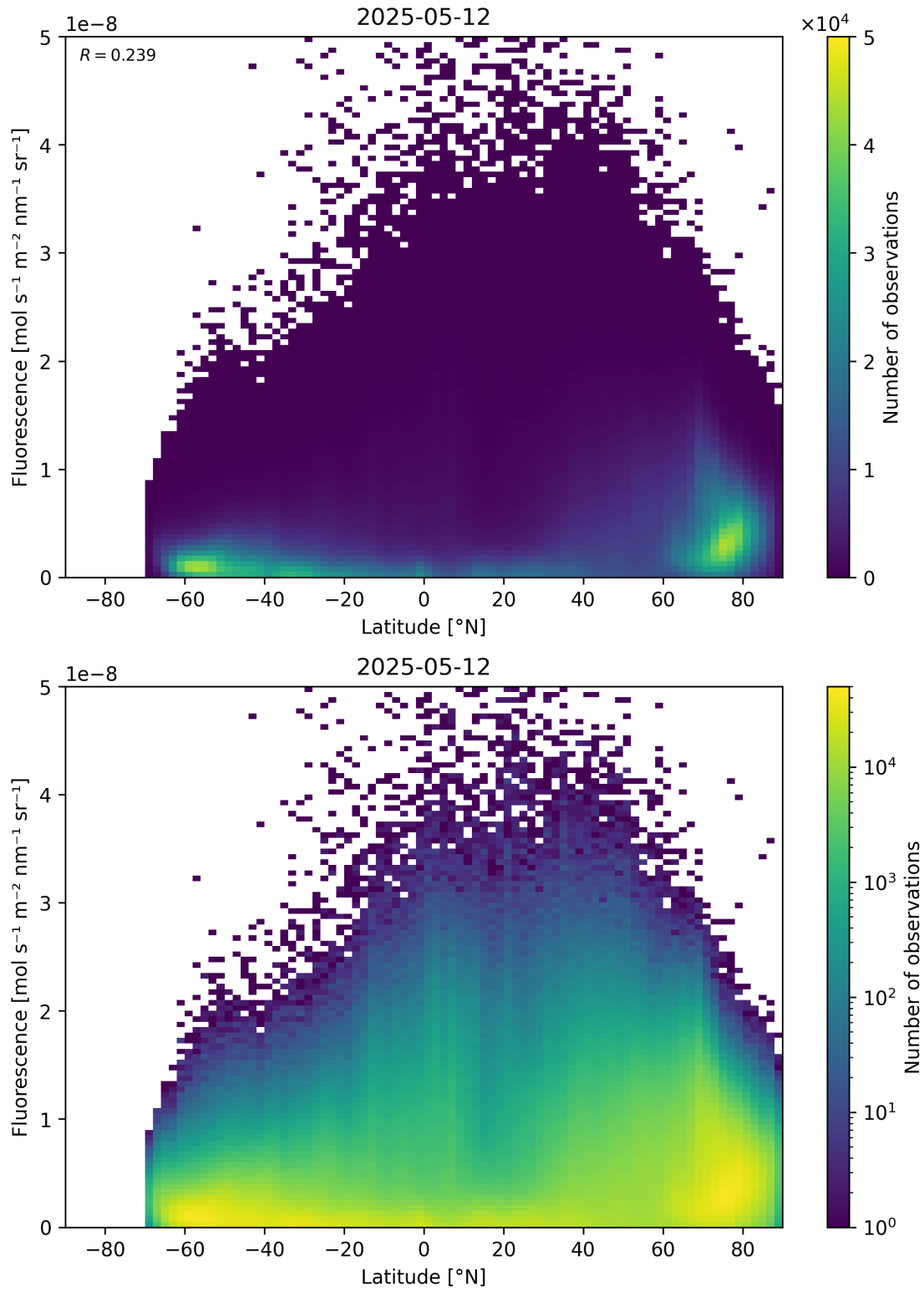
Figure 92: Scatter density plot of “Latitude” against “Fluorescence” for 2025-05-11 to 2025-05-13.
