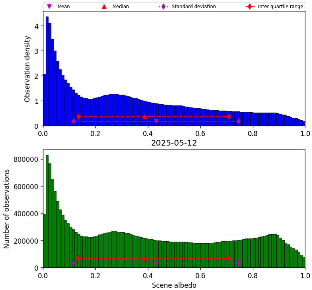
Figure 34: Histogram of “Scene albedo” for 2025-05-11 to 2025-05-13
