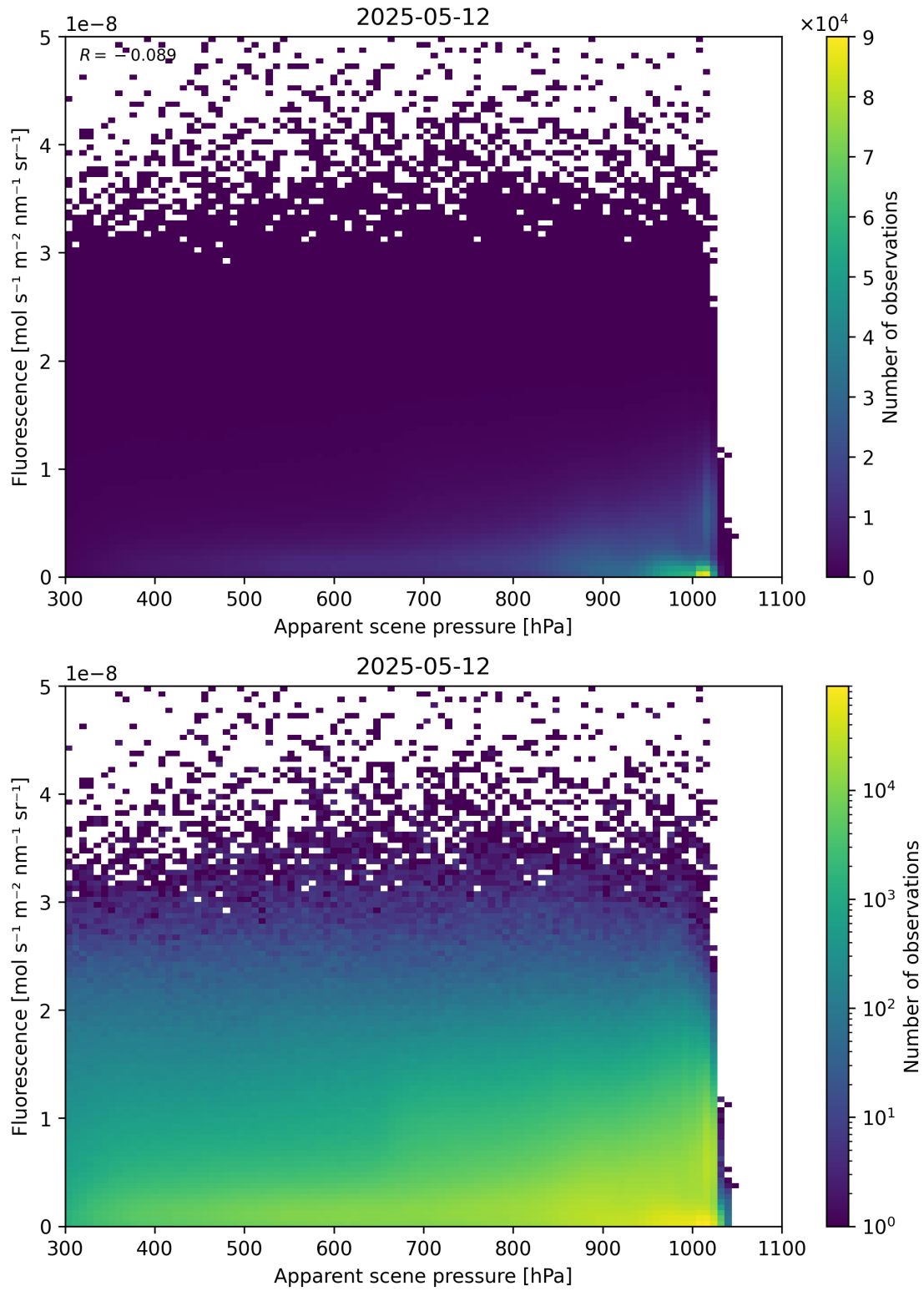
Figure 64: Scatter density plot of “Apparent scene pressure” against “Fluorescence” for 2025-05-11 to 2025-05-13.
