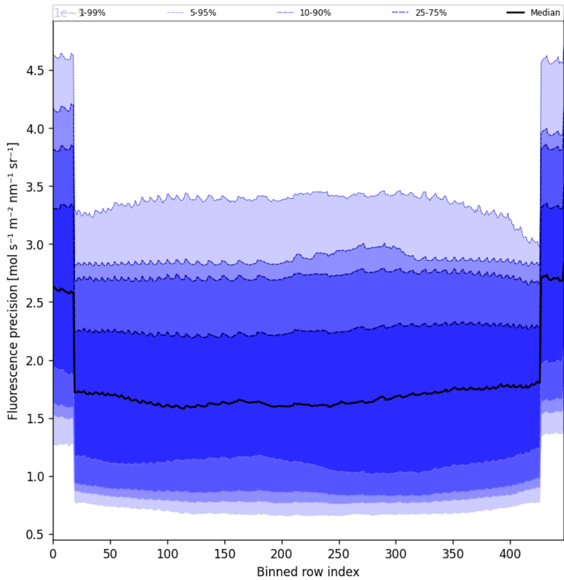
Figure 58: Along track statistics of “Fluorescence precision” for 2025-05-11 to 2025-05-13
