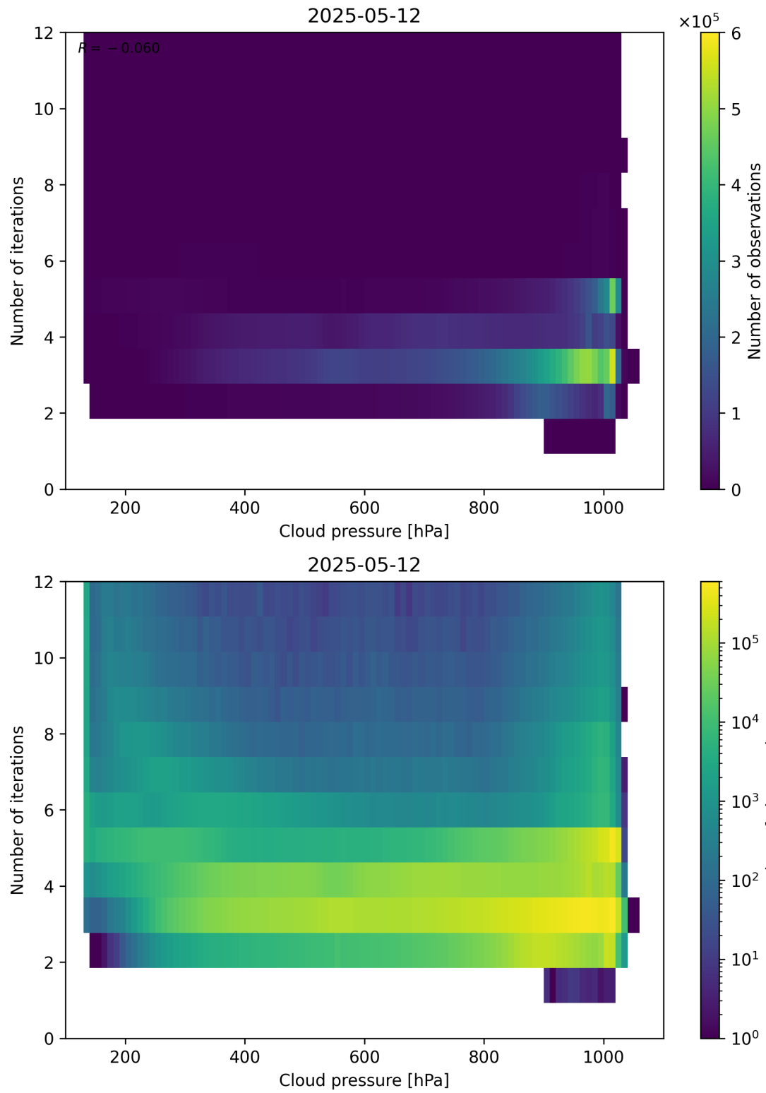
Figure 81: Scatter density plot of “Cloud pressure” against “Number of iterations” for 2025-05-11 to 2025-05-13.
