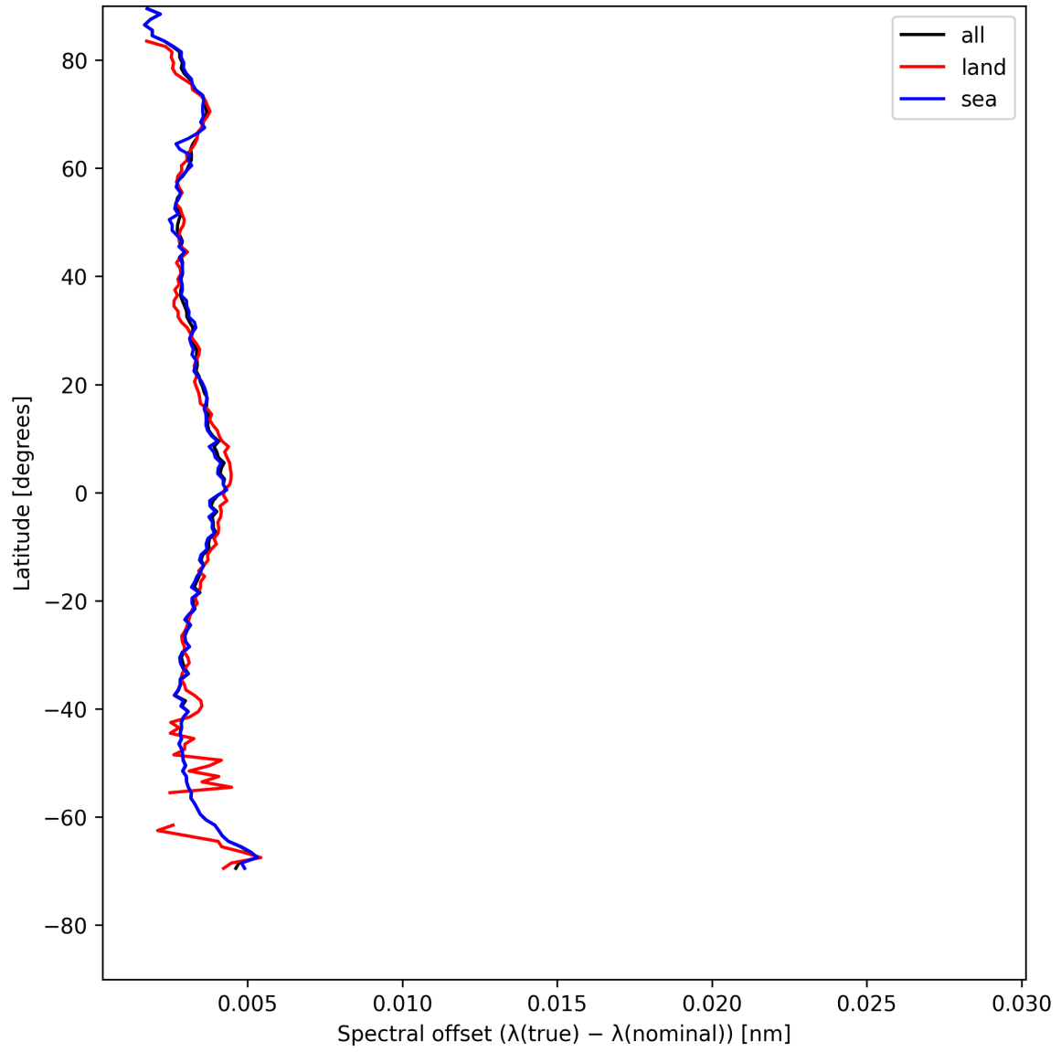
Figure 28: Zonal average of “Spectral offset ( \lambda_{\text{true}} - \lambda_{\text{nominal}} )” for 2025-05-11 to 2025-05-13.
