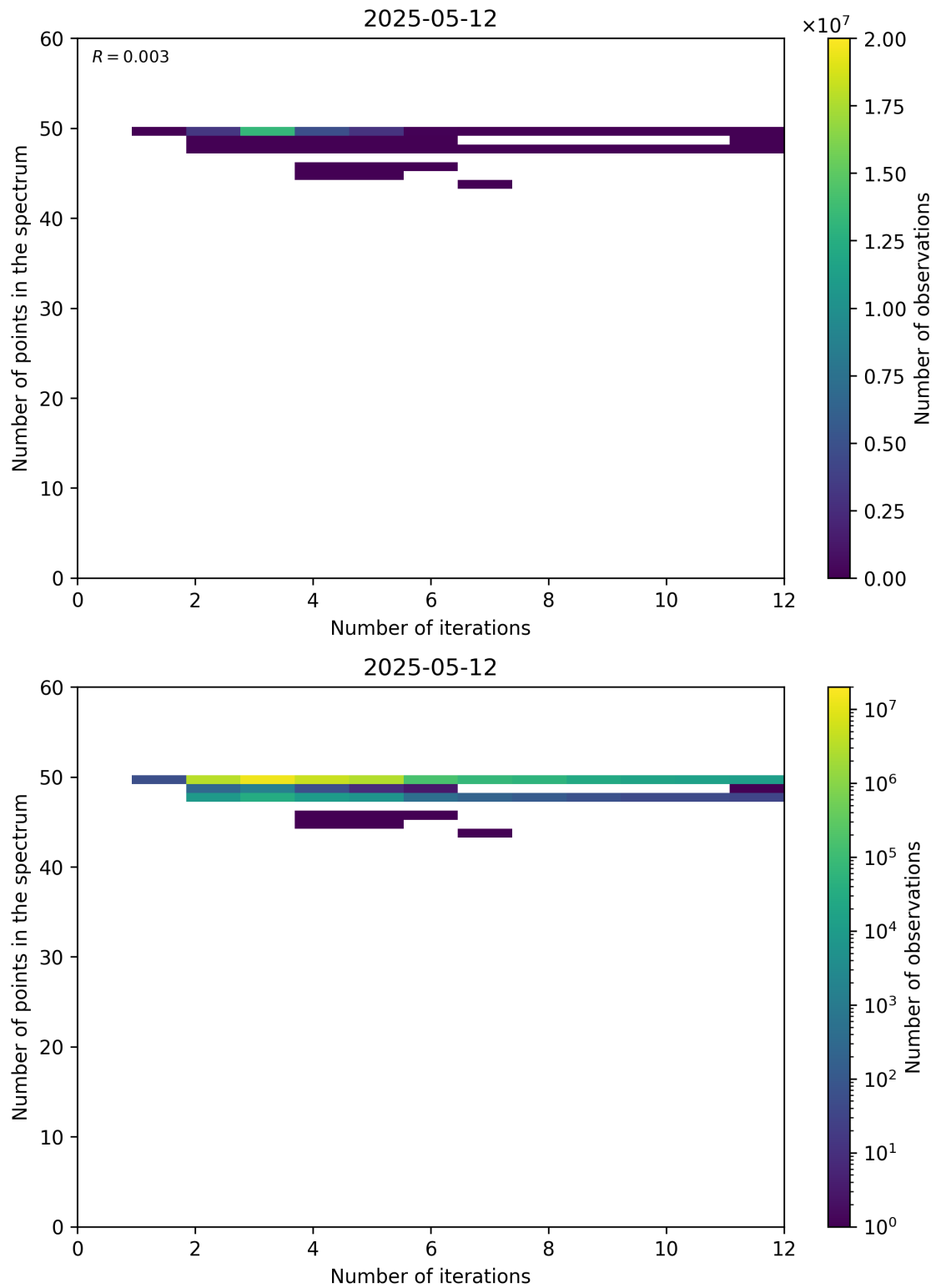
Figure 99: Scatter density plot of “Number of iterations” against “Number of points in the spectrum” for 2025-05-11 to 2025-05-13.
