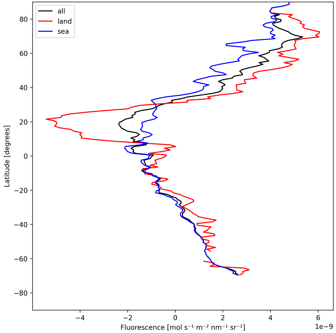
Figure 23: Zonal average of “Fluorescence” for 2025-05-11 to 2025-05-13.
