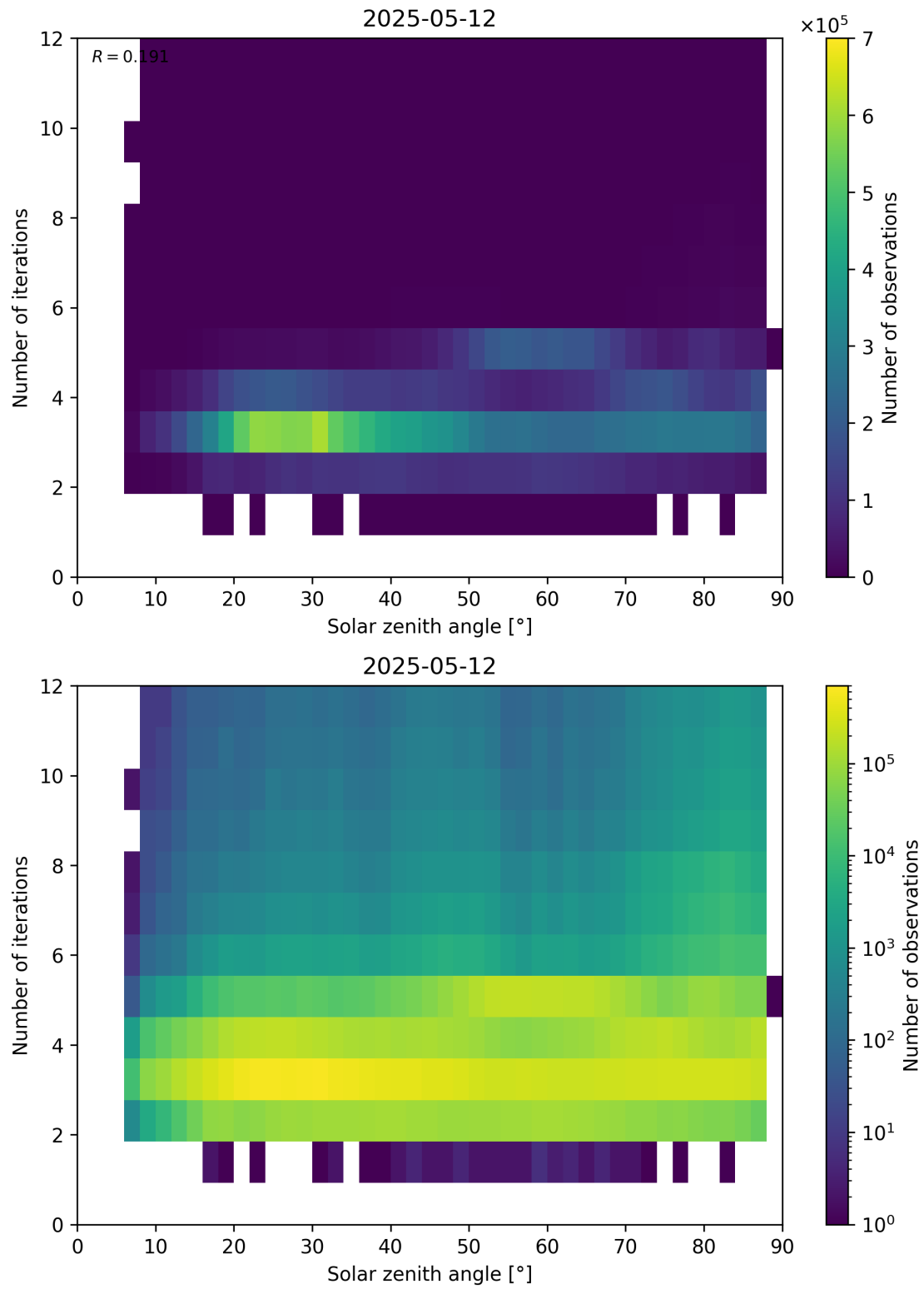
Figure 114: Scatter density plot of “Solar zenith angle” against “Number of iterations” for 2025-05-11 to 2025-05-13.
