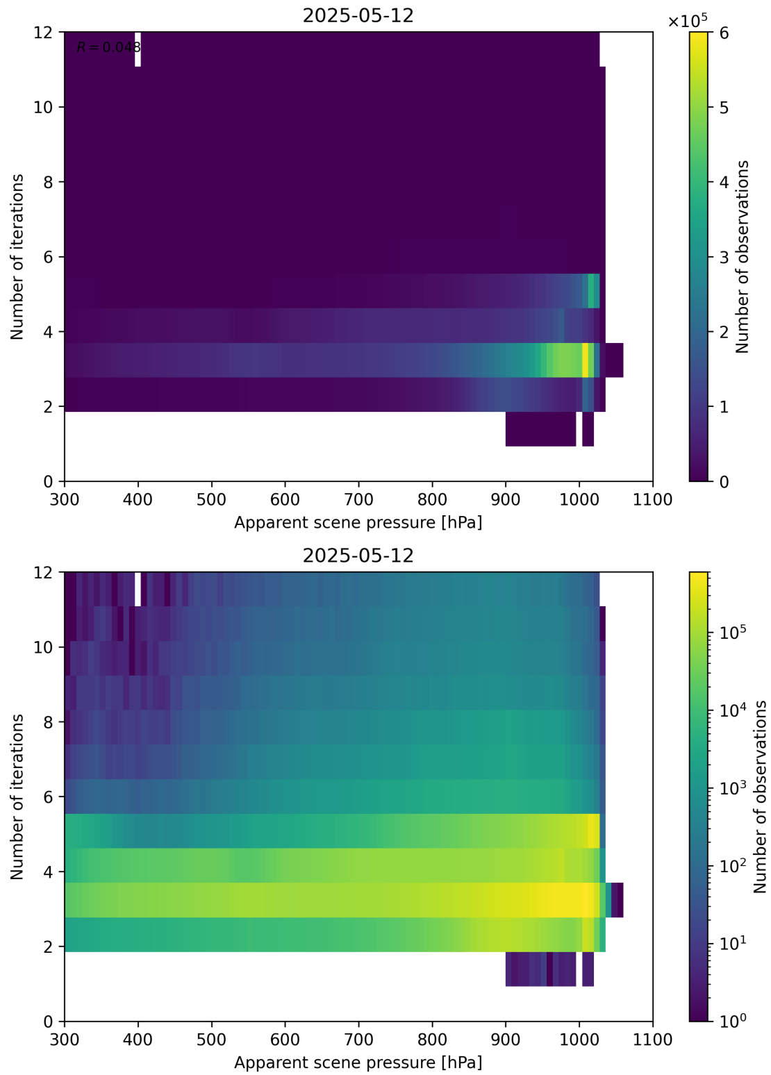
Figure 65: Scatter density plot of “Apparent scene pressure” against “Number of iterations” for 2025-05-11 to 2025-05-13.
