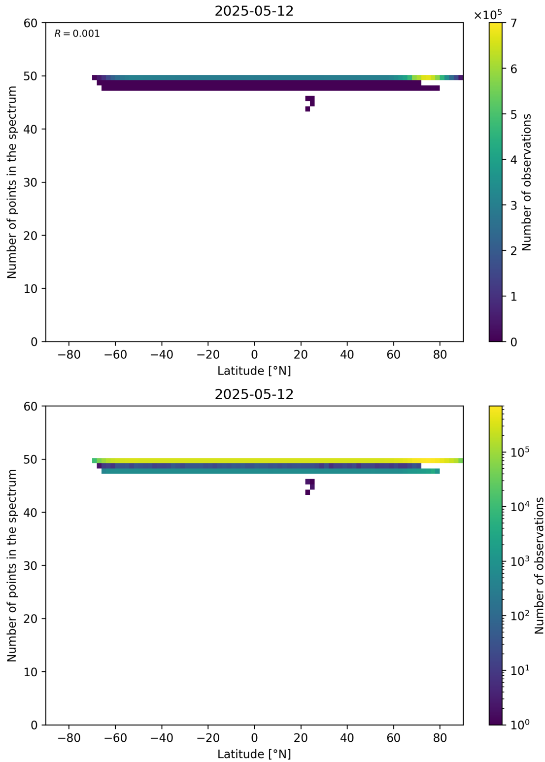
Figure 94: Scatter density plot of “Latitude” against “Number of points in the spectrum” for 2025-05-11 to 2025-05-13.
