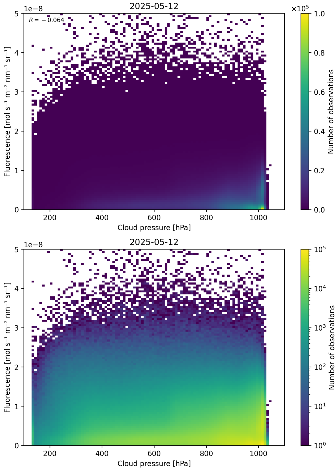
Figure 80: Scatter density plot of “Cloud pressure” against “Fluorescence” for 2025-05-11 to 2025-05-13.
