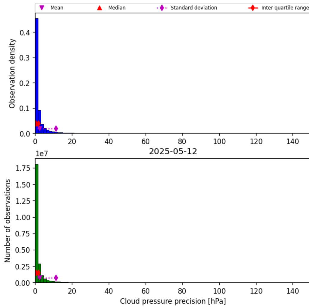
Figure 31: Histogram of “Cloud pressure precision” for 2025-05-11 to 2025-05-13
