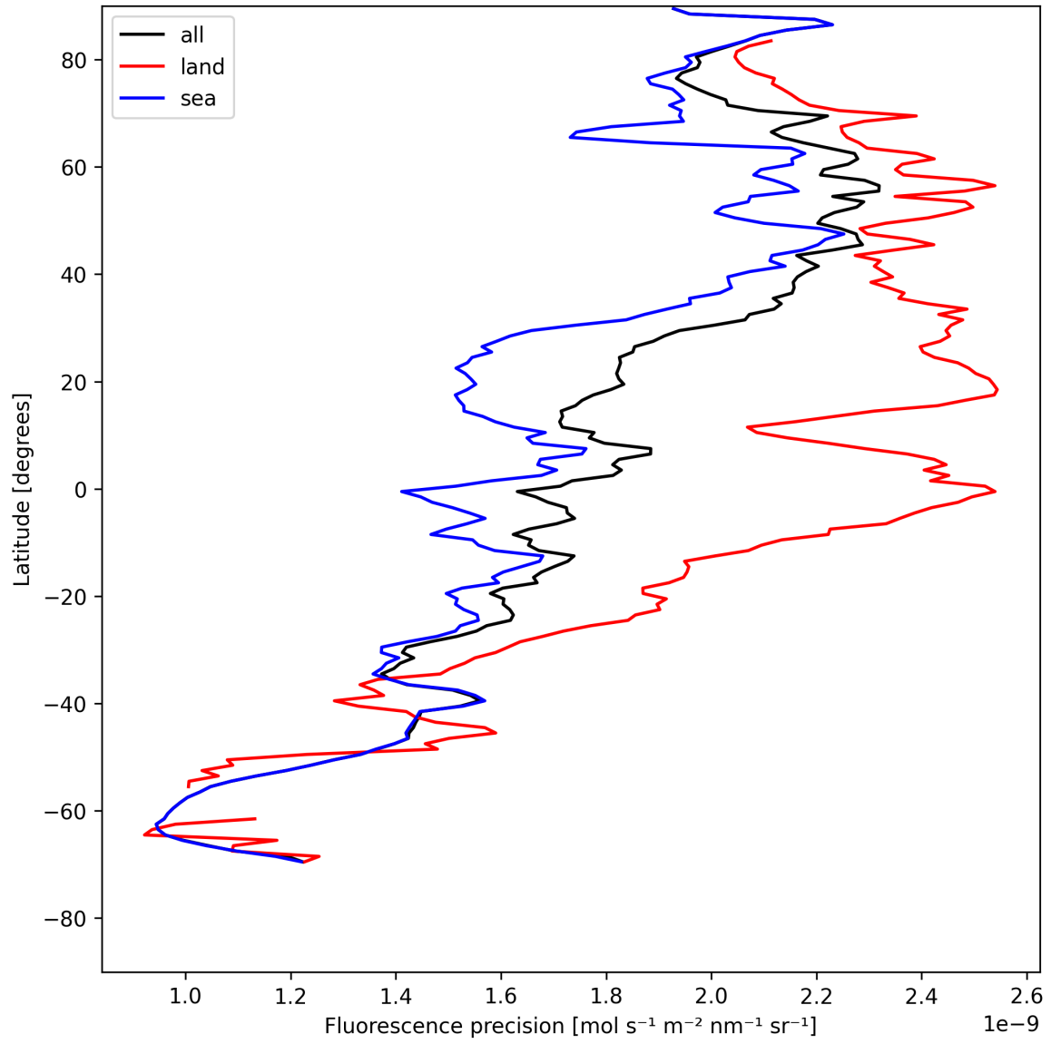
Figure 24: Zonal average of “Fluorescence precision” for 2025-05-11 to 2025-05-13.
