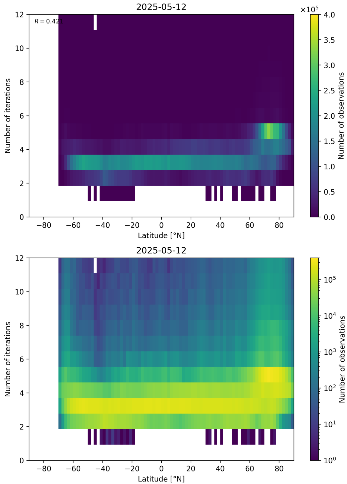
Figure 93: Scatter density plot of “Latitude” against “Number of iterations” for 2025-05-11 to 2025-05-13.
