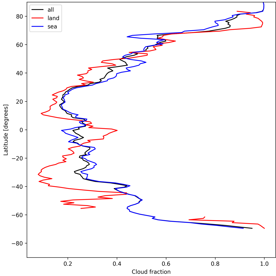
Figure 15: Zonal average of “Cloud fraction” for 2025-05-11 to 2025-05-13.
