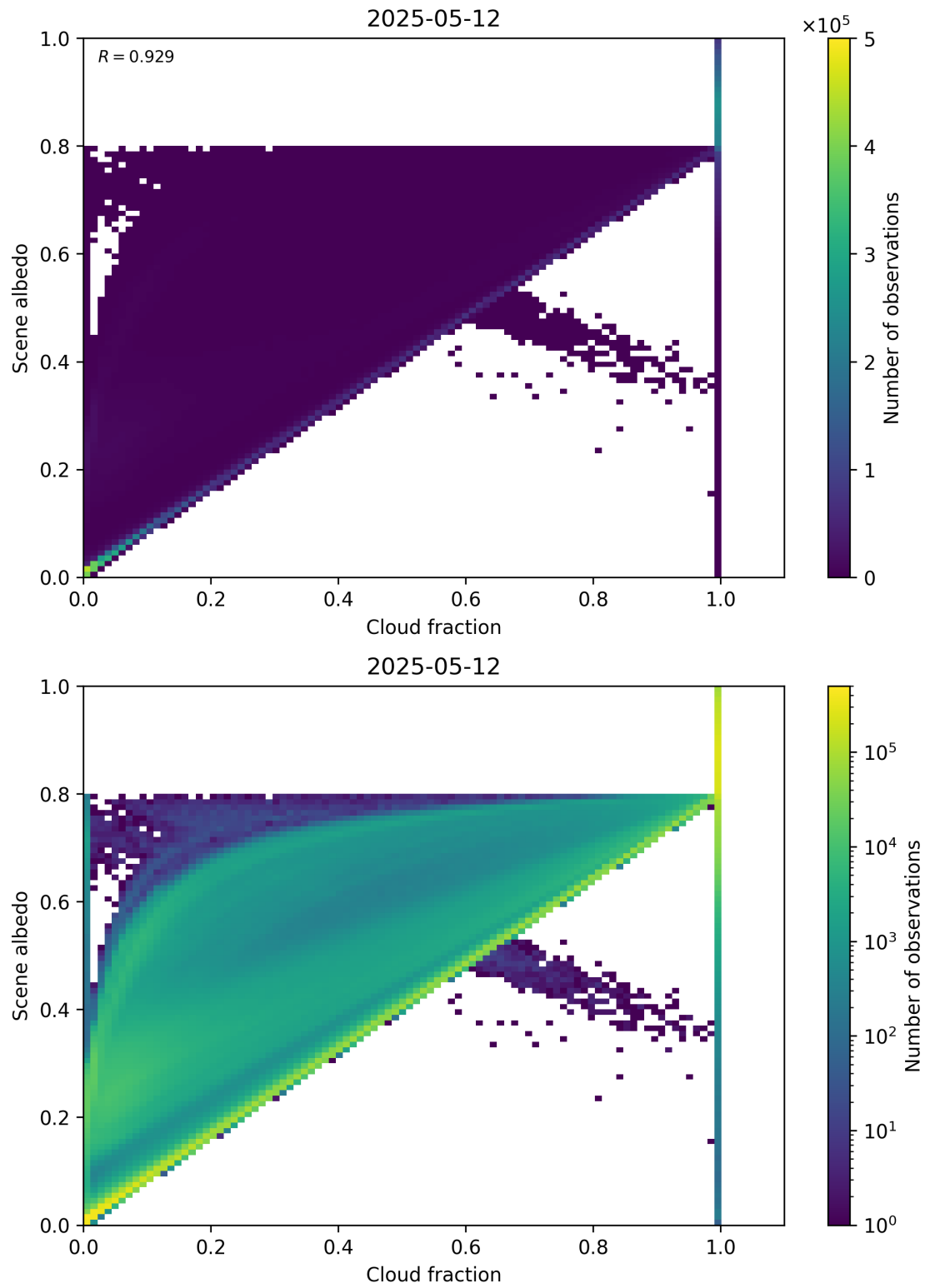
Figure 75: Scatter density plot of “Cloud fraction” against “Scene albedo” for 2025-05-11 to 2025-05-13.
