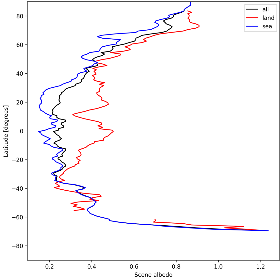
Figure 17: Zonal average of “Scene albedo” for 2025-05-11 to 2025-05-13.
