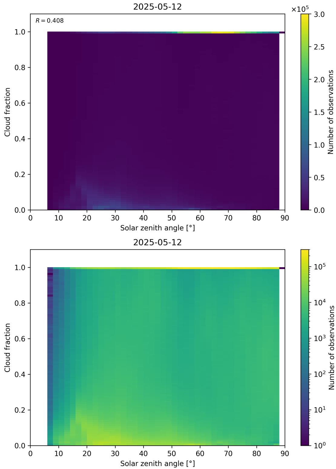
Figure 110: Scatter density plot of “Solar zenith angle” against “Cloud fraction” for 2025-05-11 to 2025-05-13.
