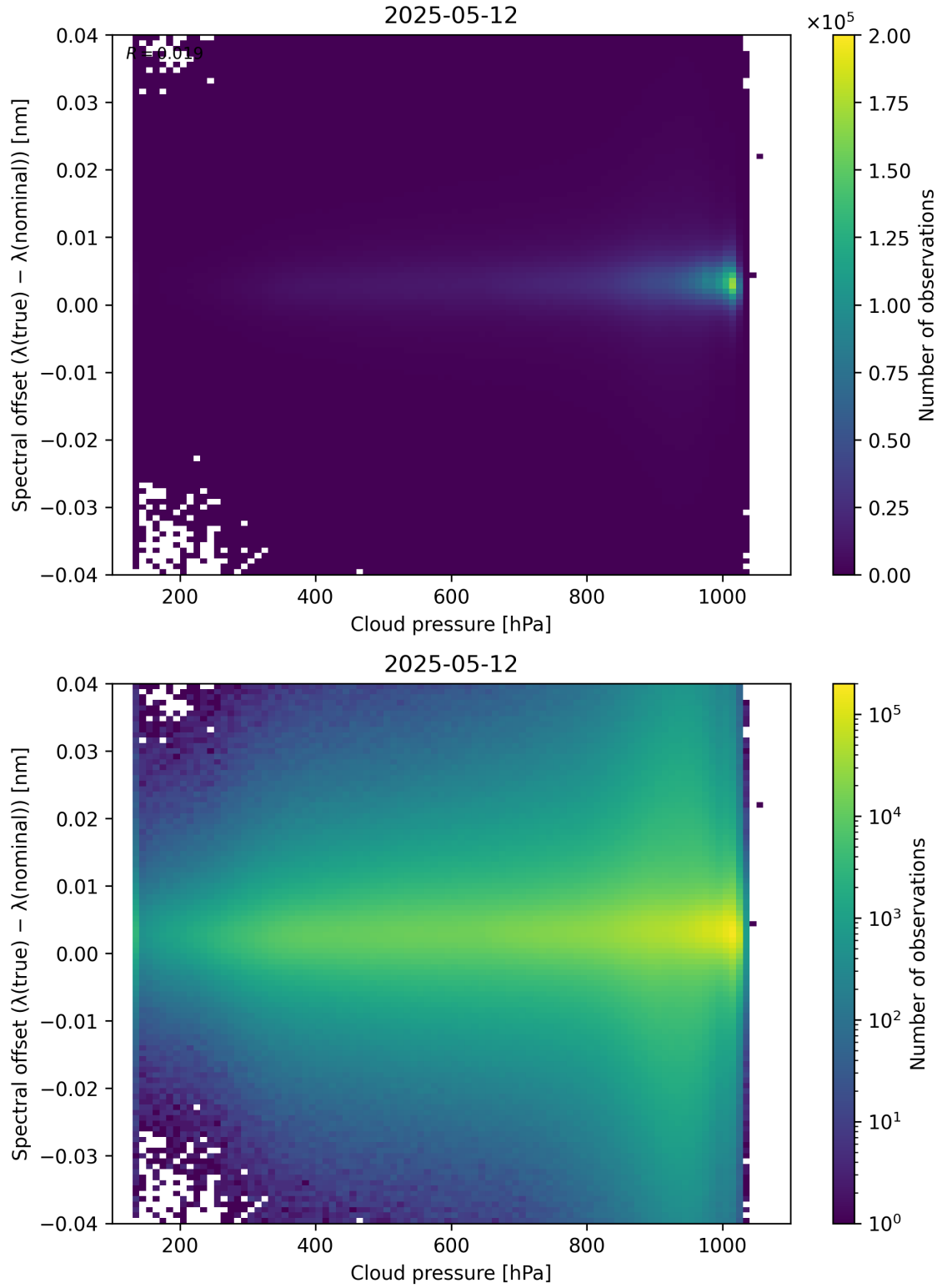
Figure 84: Scatter density plot of “Cloud pressure” against “Spectral offset ( \lambda_{\text{true}} - \lambda_{\text{nominal}} )” for 2025-05-11 to 2025-05-13.
