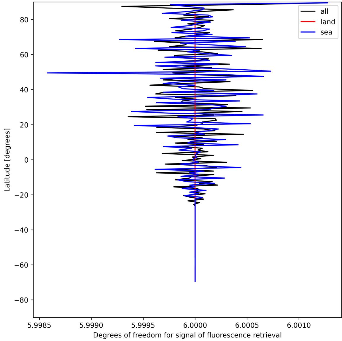
Figure 26: Zonal average of “Degrees of freedom for signal of fluorescence retrieval” for 2025-05-11 to 2025-05-13.
