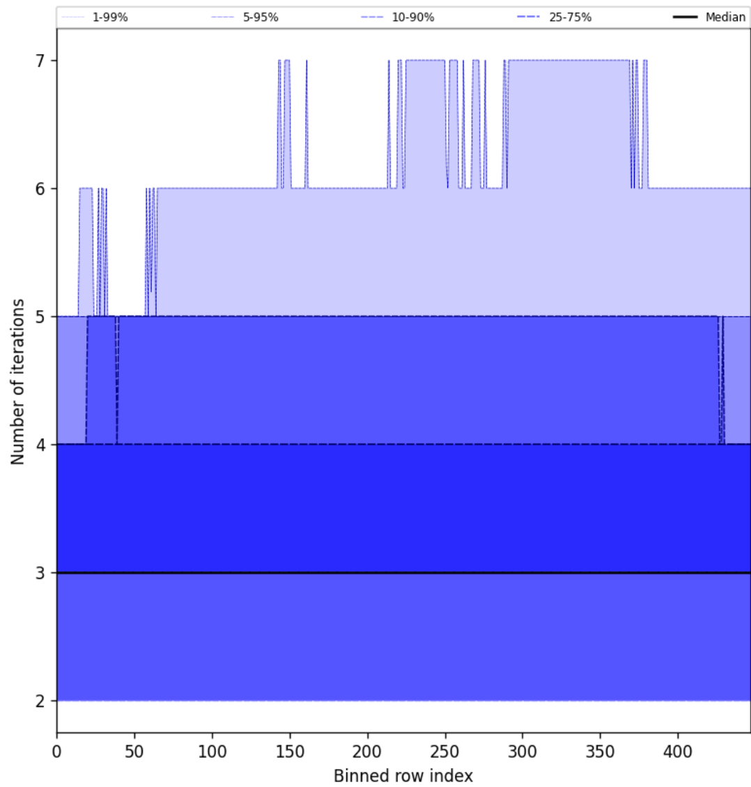
Figure 56: Along track statistics of “Number of iterations” for 2025-05-11 to 2025-05-13
