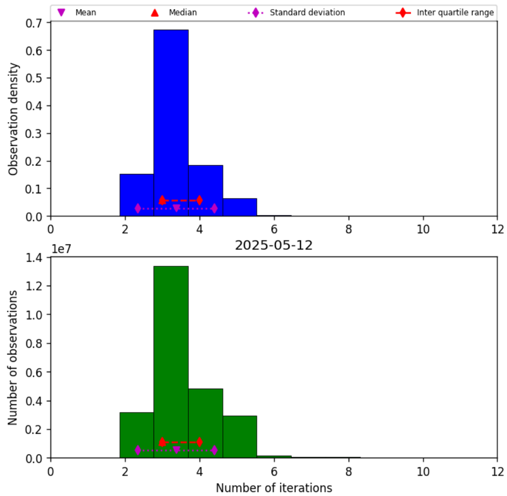
Figure 39: Histogram of “Number of iterations” for 2025-05-11 to 2025-05-13
