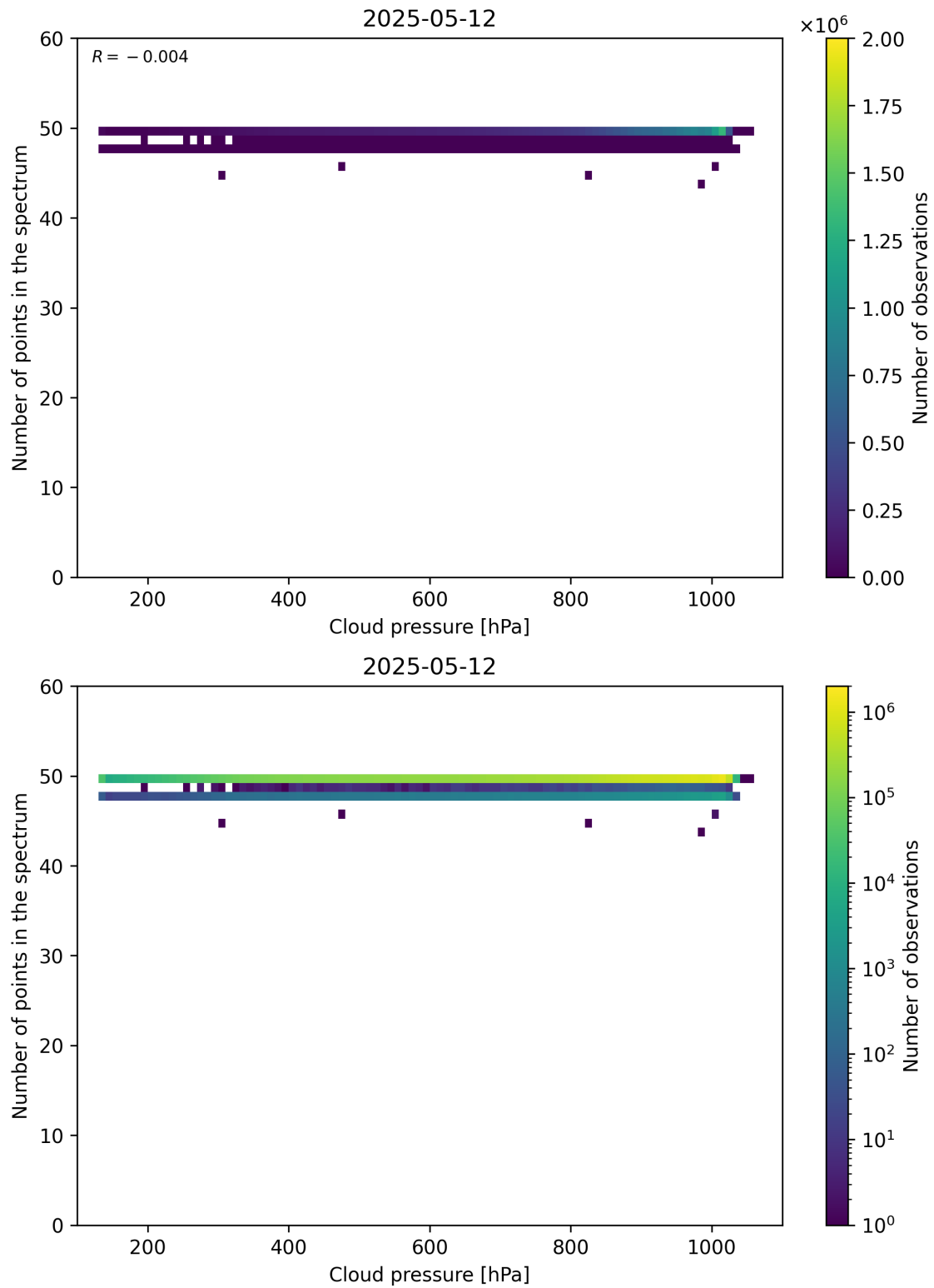
Figure 82: Scatter density plot of “Cloud pressure” against “Number of points in the spectrum” for 2025-05-11 to 2025-05-13.
