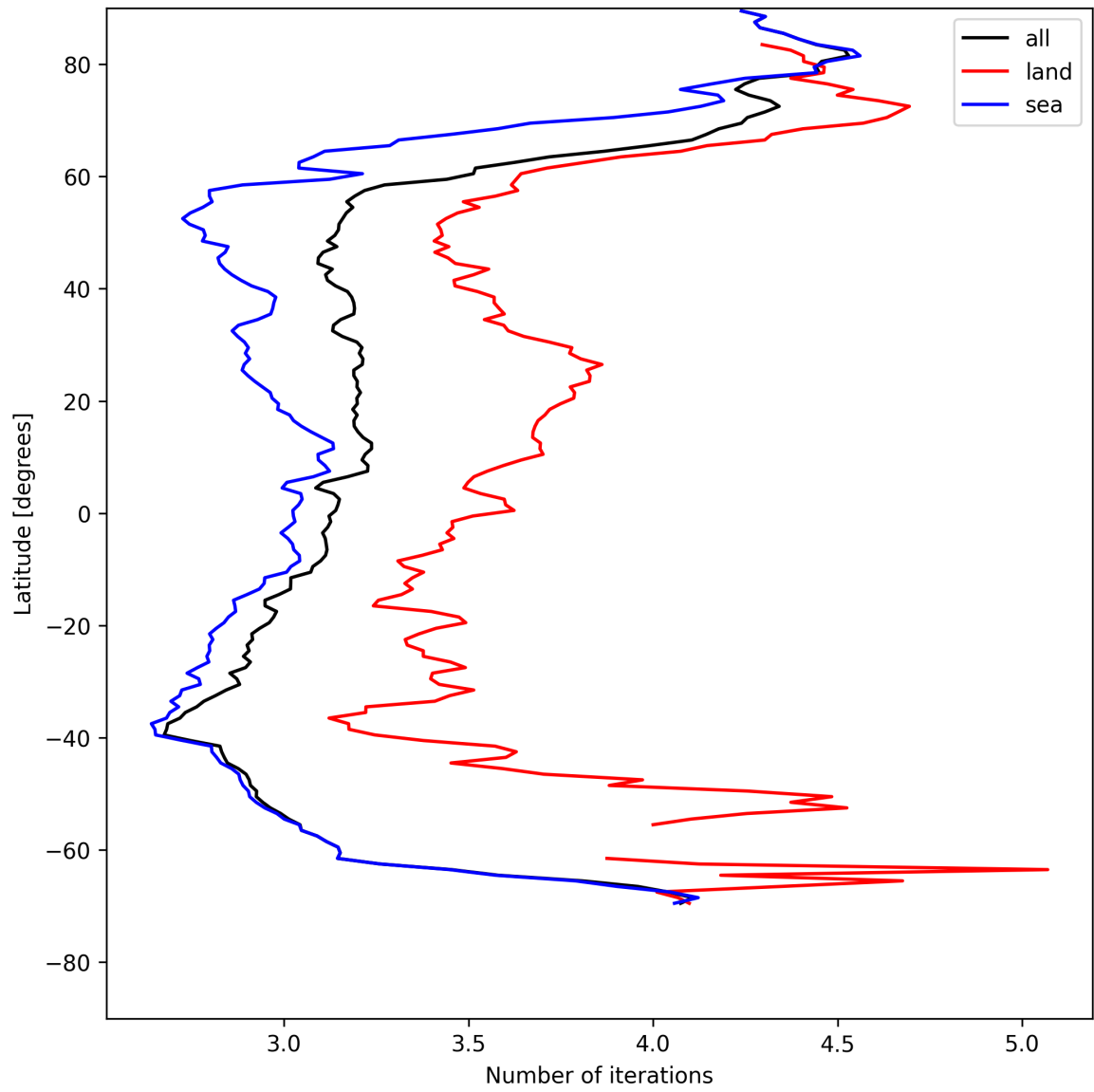
Figure 22: Zonal average of “Number of iterations” for 2025-05-11 to 2025-05-13.
