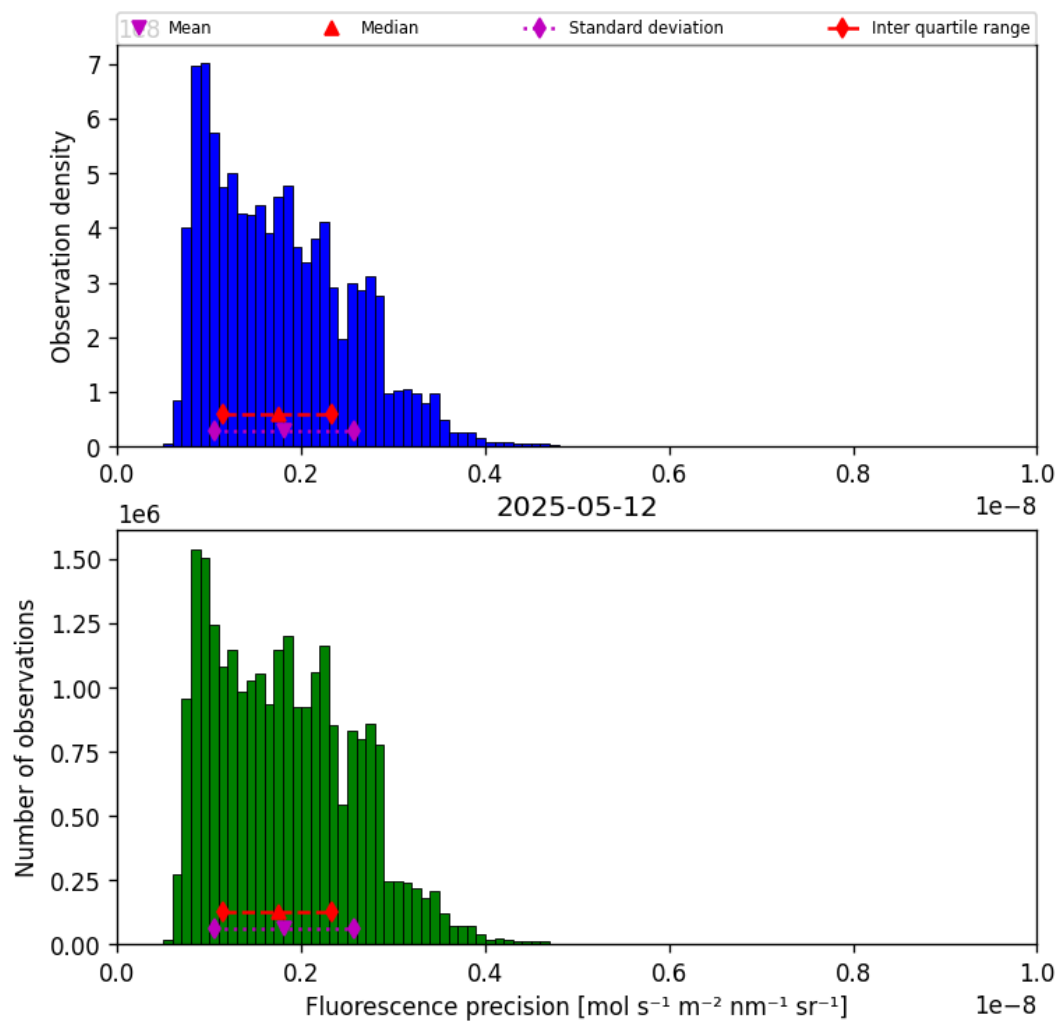
Figure 41: Histogram of “Fluorescence precision” for 2025-05-11 to 2025-05-13
