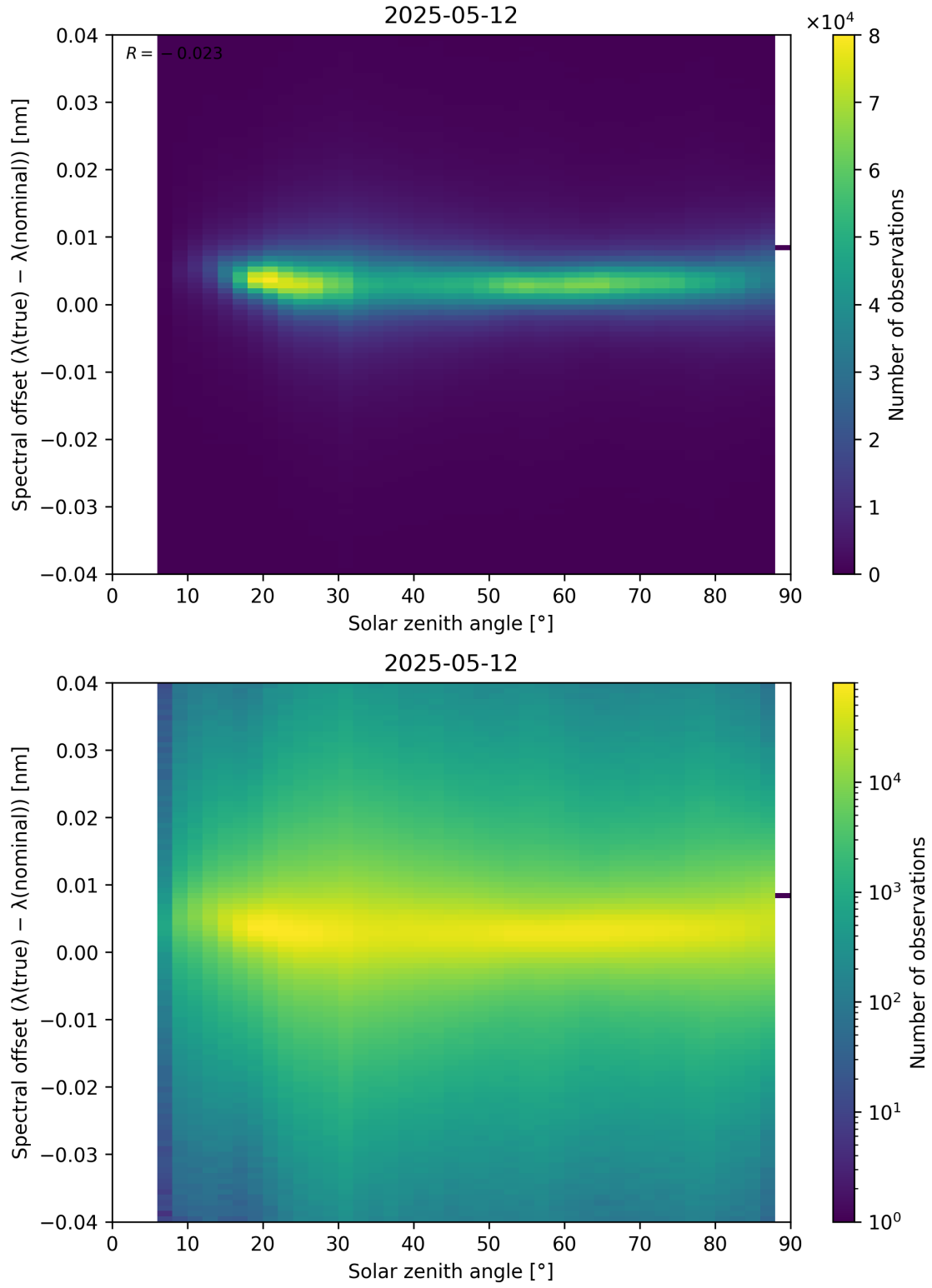
Figure 117: Scatter density plot of “Solar zenith angle” against “Spectral offset ( \lambda_{\text{true}} - \lambda_{\text{nominal}} )” for 2025-05-11 to 2025-05-13.
