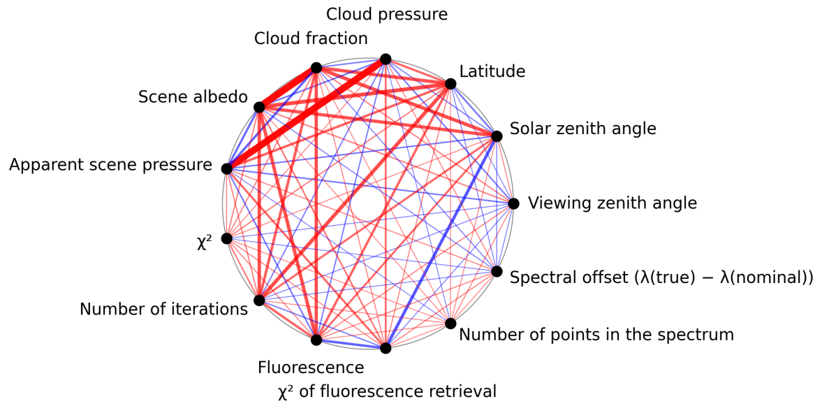
Figure 1: Map of correlation graph for 2025-05-11 to 2025-05-13.
