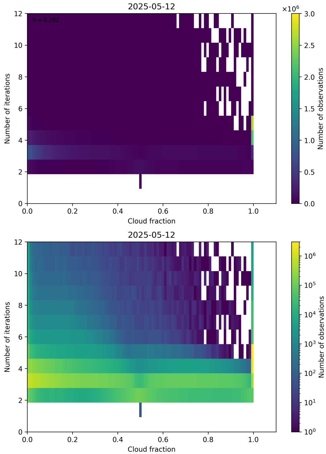
Figure 73: Scatter density plot of “Cloud fraction” against “Number of iterations” for 2025-05-11 to 2025-05-13.
