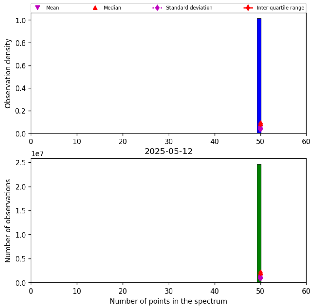
Figure 44: Histogram of “Number of points in the spectrum” for 2025-05-11 to 2025-05-13
