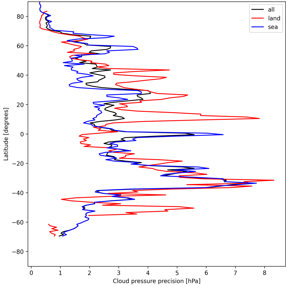
Figure 14: Zonal average of “Cloud pressure precision” for 2025-05-11 to 2025-05-13.
