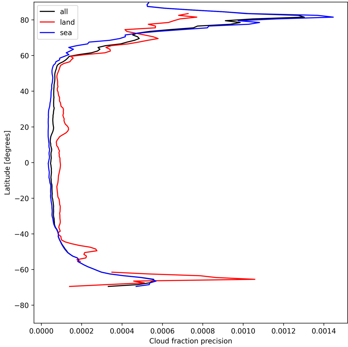
Figure 16: Zonal average of “Cloud fraction precision” for 2025-05-11 to 2025-05-13.
