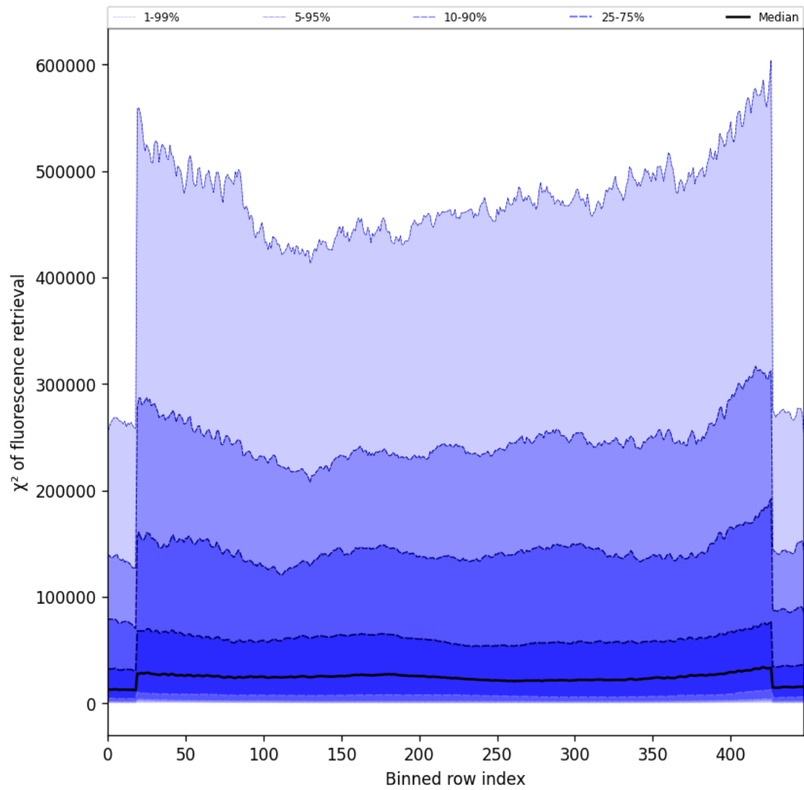
Figure 59: Along track statistics of “ \chi^2 of fluorescence retrieval” for 2025-05-11 to 2025-05-13
