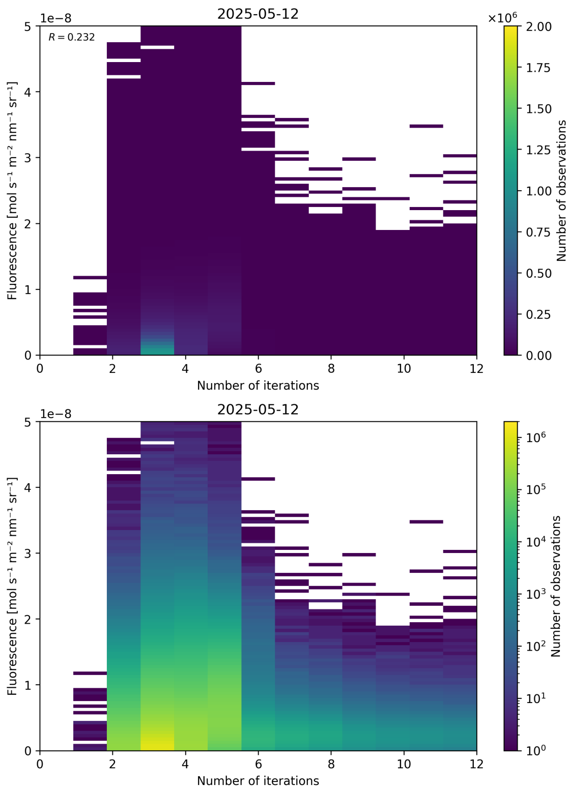
Figure 98: Scatter density plot of “Number of iterations” against “Fluorescence” for 2025-05-11 to 2025-05-13.
