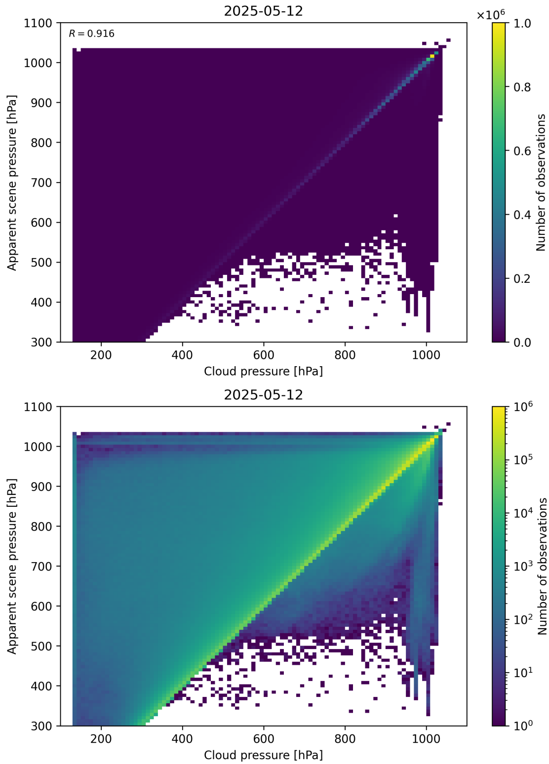
Figure 77: Scatter density plot of “Cloud pressure” against “Apparent scene pressure” for 2025-05-11 to 2025-05-13.
