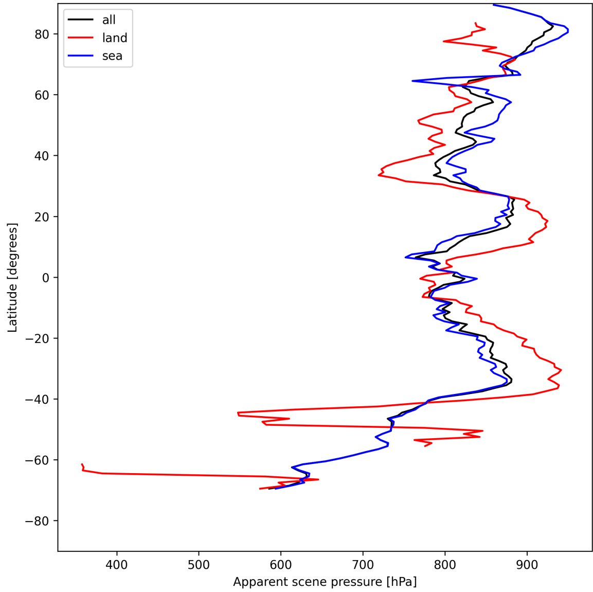
Figure 19: Zonal average of “Apparent scene pressure” for 2025-05-11 to 2025-05-13.
