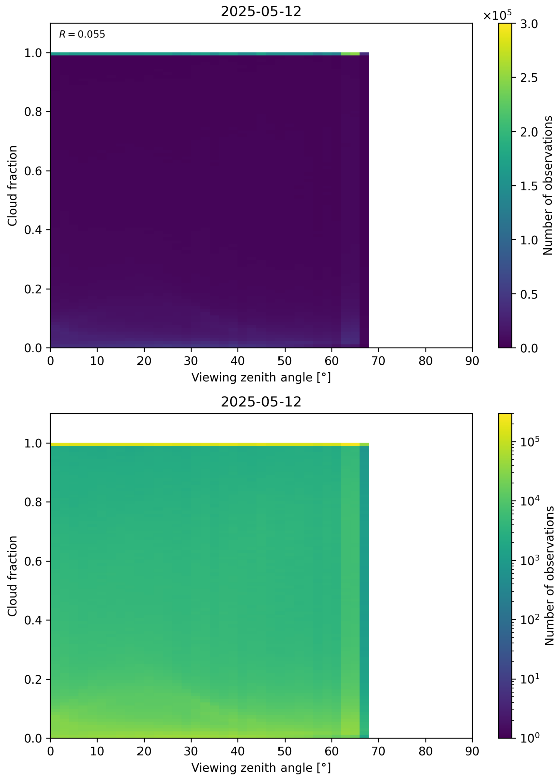
Figure 120: Scatter density plot of “Viewing zenith angle” against “Cloud fraction” for 2025-05-11 to 2025-05-13.
