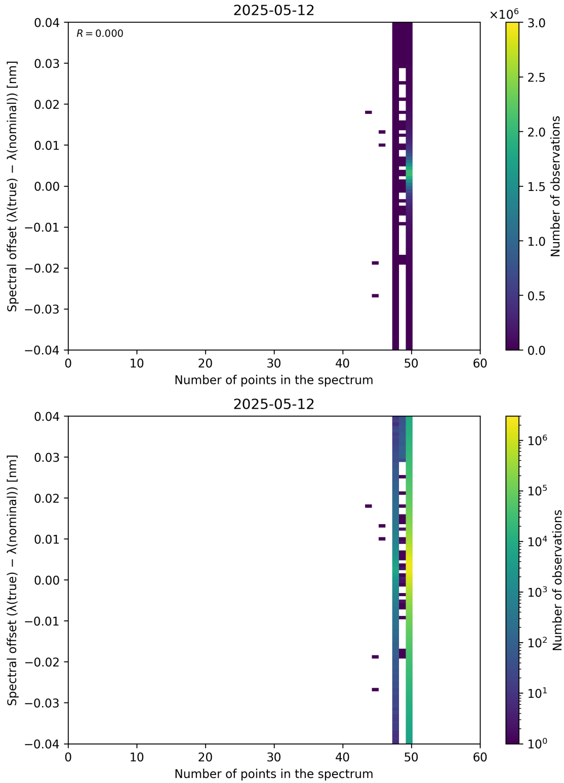
Figure 101: Scatter density plot of “Number of points in the spectrum” against “Spectral offset ( \lambda_{\text{true}} - \lambda_{\text{nominal}} )” for 2025-05-11 to 2025-05-13.
