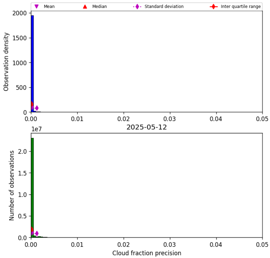
Figure 33: Histogram of “Cloud fraction precision” for 2025-05-11 to 2025-05-13
