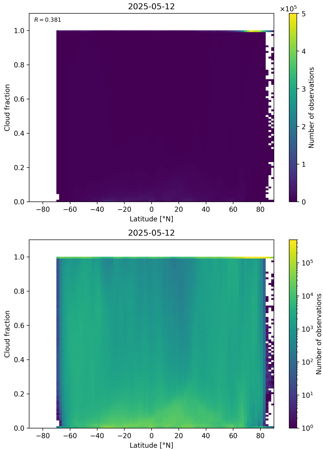
Figure 90: Scatter density plot of “Latitude” against “Cloud fraction” for 2025-05-11 to 2025-05-13.
