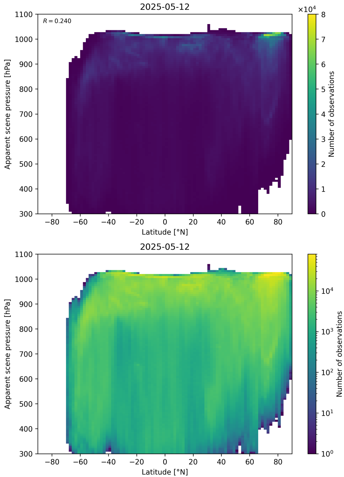
Figure 88: Scatter density plot of “Latitude” against “Apparent scene pressure” for 2025-05-11 to 2025-05-13.
