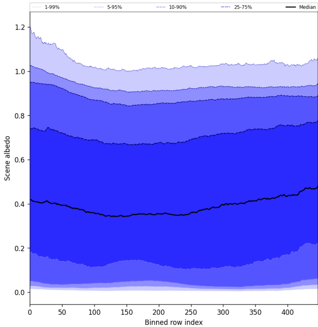
Figure 51: Along track statistics of “Scene albedo” for 2025-05-11 to 2025-05-13
