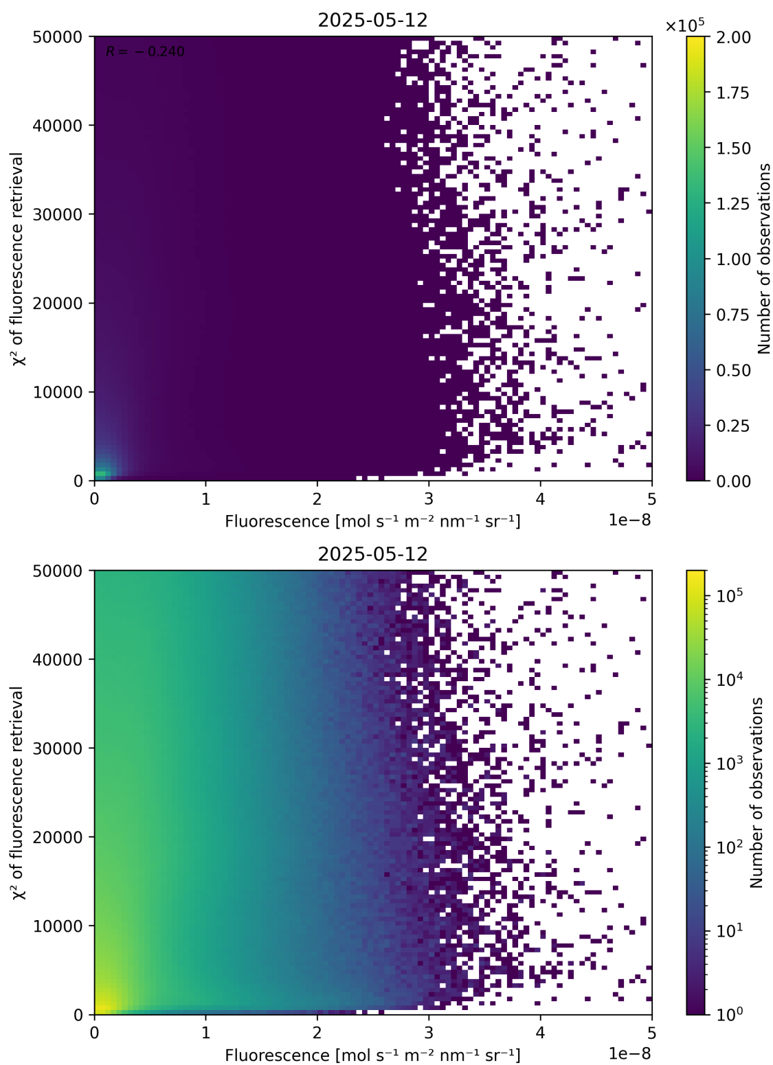
Figure 85: Scatter density plot of “Fluorescence” against “ \chi^2 of fluorescence retrieval” for 2025-05-11 to 2025-05-13.
