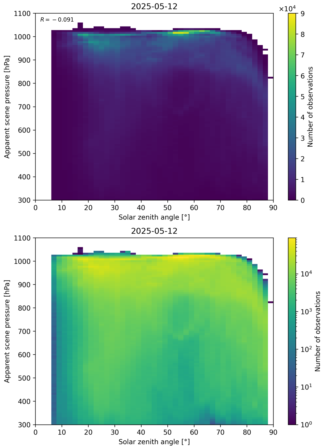
Figure 108: Scatter density plot of “Solar zenith angle” against “Apparent scene pressure” for 2025-05-11 to 2025-05-13.
