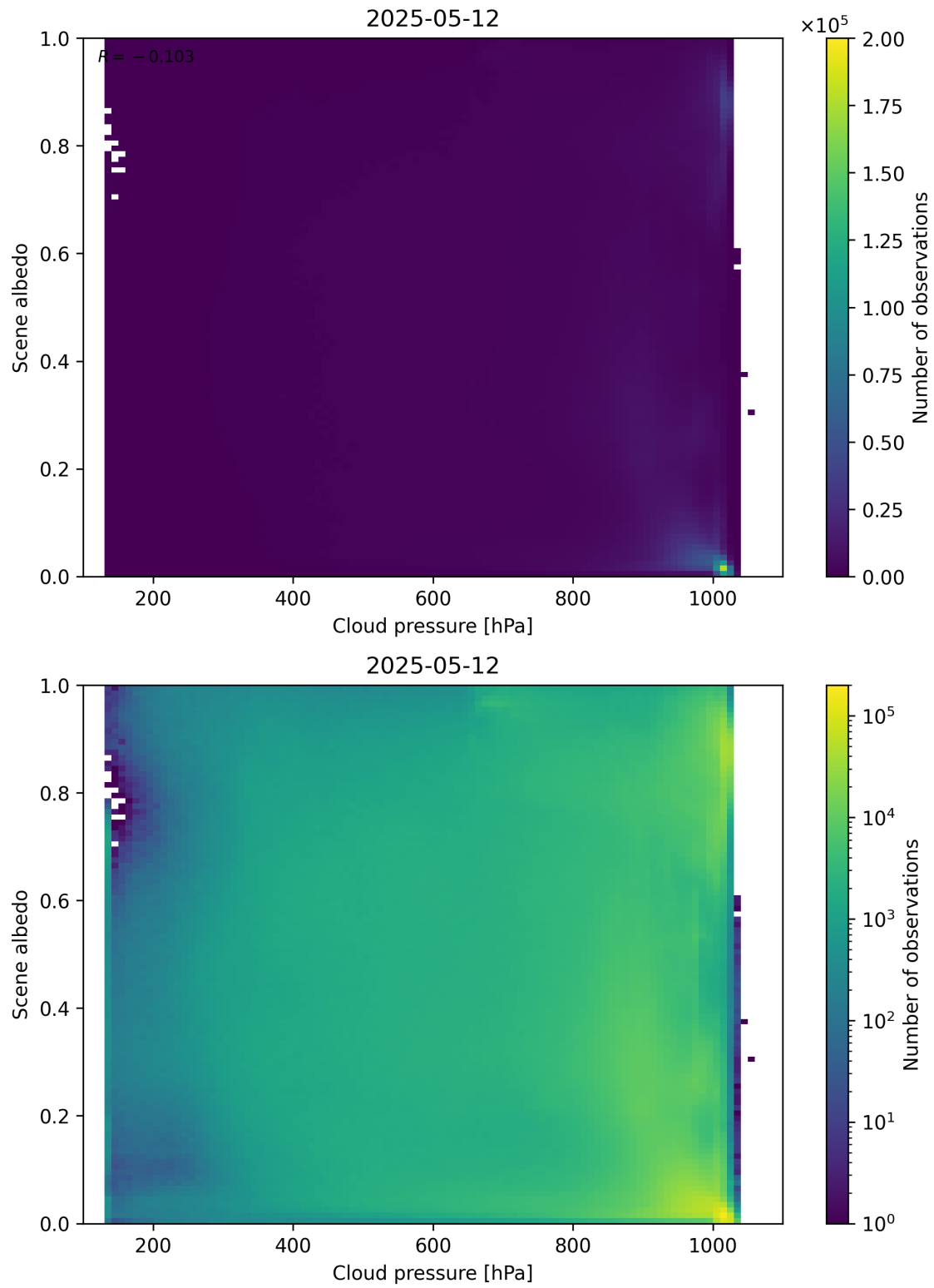
Figure 83: Scatter density plot of “Cloud pressure” against “Scene albedo” for 2025-05-11 to 2025-05-13.
