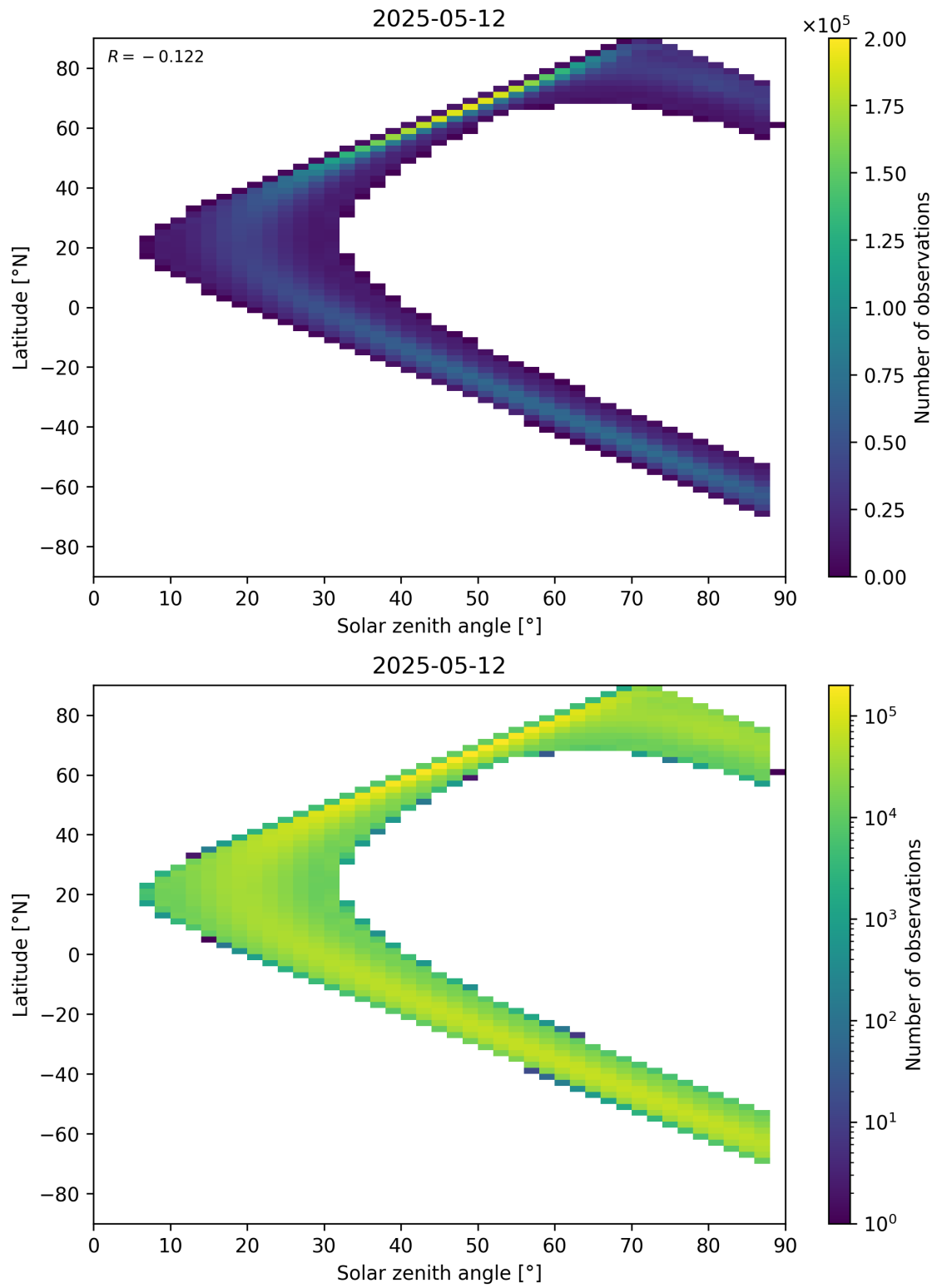
Figure 113: Scatter density plot of “Solar zenith angle” against “Latitude” for 2025-05-11 to 2025-05-13.
