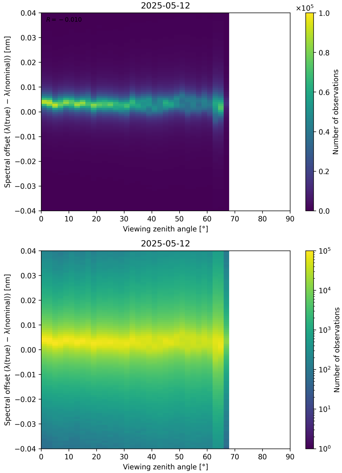
Figure 128: Scatter density plot of “Viewing zenith angle” against “Spectral offset ( \lambda_{\text{true}} - \lambda_{\text{nominal}} )” for 2025-05-11 to 2025-05-13.
