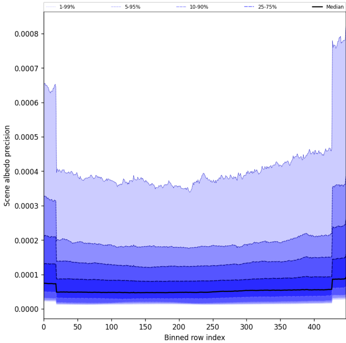
Figure 52: Along track statistics of “Scene albedo precision” for 2025-05-11 to 2025-05-13
