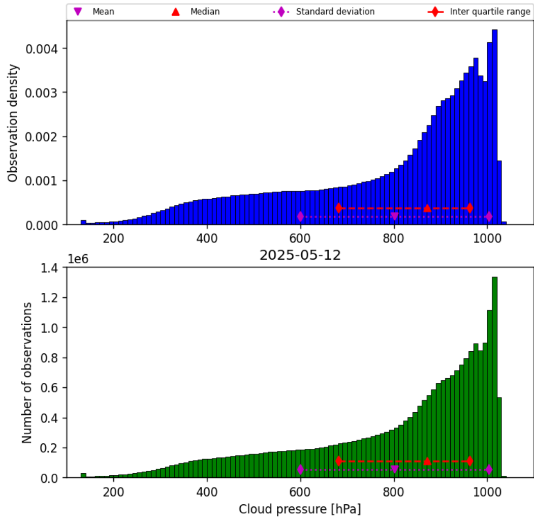
Figure 30: Histogram of “Cloud pressure” for 2025-05-11 to 2025-05-13
