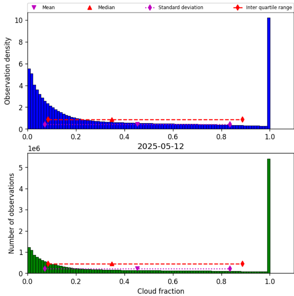
Figure 32: Histogram of “Cloud fraction” for 2025-05-11 to 2025-05-13
