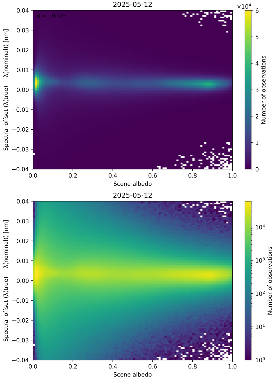
Figure 107: Scatter density plot of “Scene albedo” against “Spectral offset ( \lambda_{\text{true}} - \lambda_{\text{nominal}} )” for 2025-05-11 to 2025-05-13.
