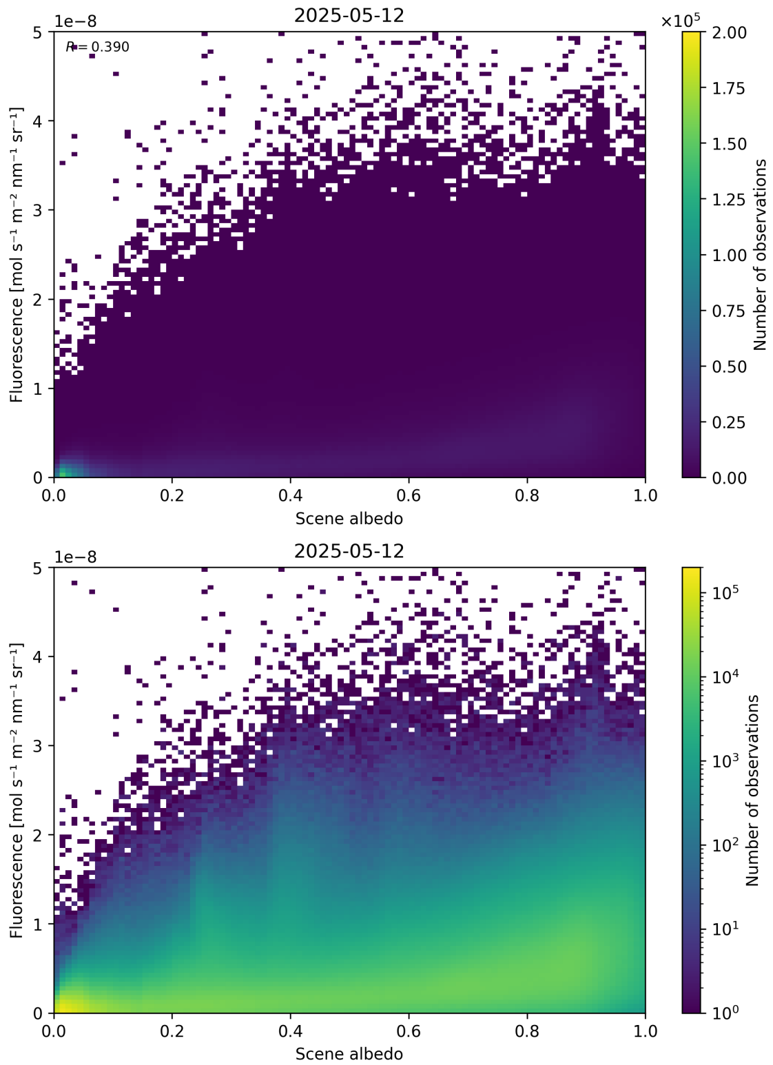
Figure 104: Scatter density plot of “Scene albedo” against “Fluorescence” for 2025-05-11 to 2025-05-13.
