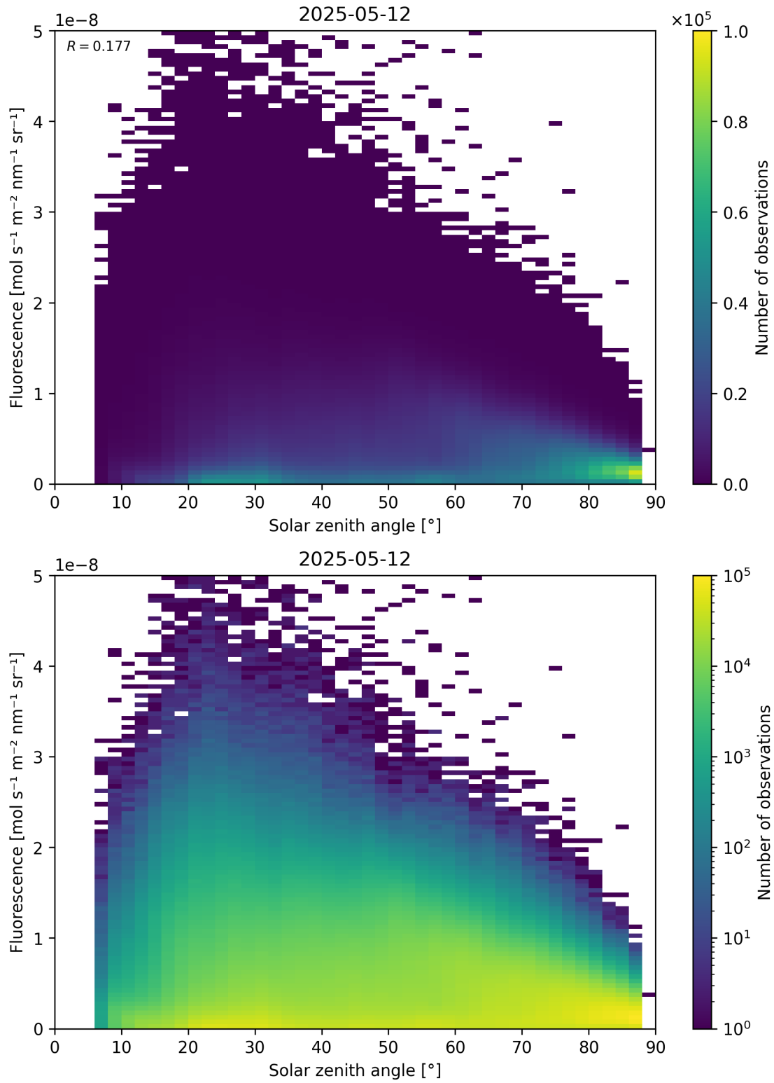
Figure 112: Scatter density plot of “Solar zenith angle” against “Fluorescence” for 2025-05-11 to 2025-05-13.
