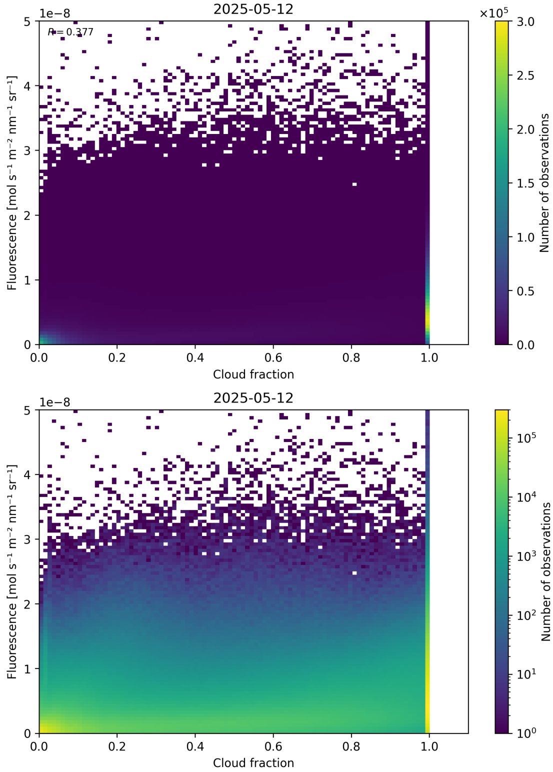
Figure 72: Scatter density plot of “Cloud fraction” against “Fluorescence” for 2025-05-11 to 2025-05-13.
