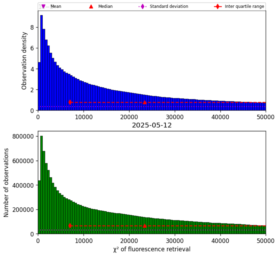
Figure 42: Histogram of “ \chi^2 of fluorescence retrieval” for 2025-05-11 to 2025-05-13
