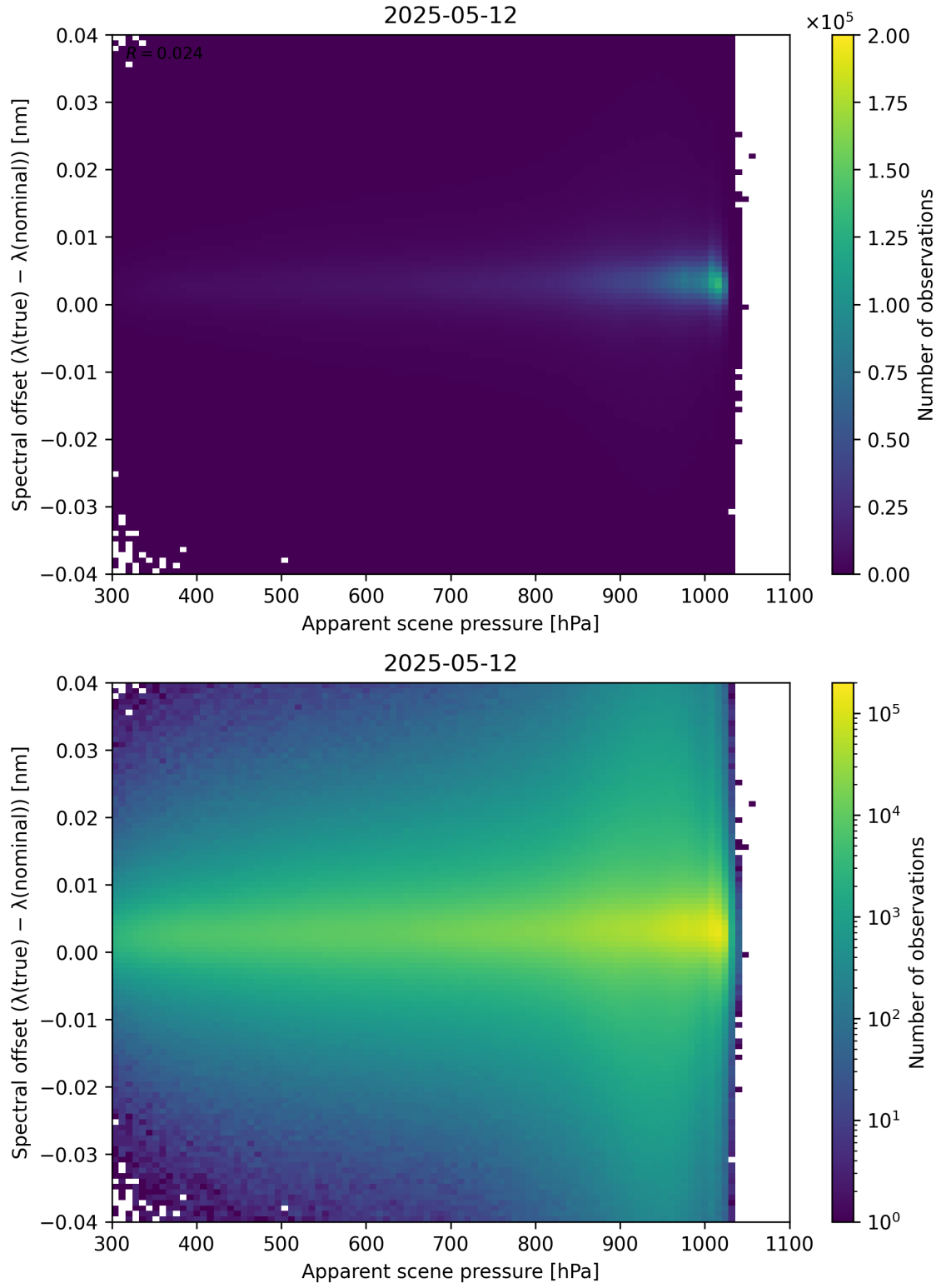
Figure 67: Scatter density plot of “Apparent scene pressure” against “Spectral offset ( \lambda_{\text{true}} - \lambda_{\text{nominal}} )” for 2025-05-11 to 2025-05-13.
