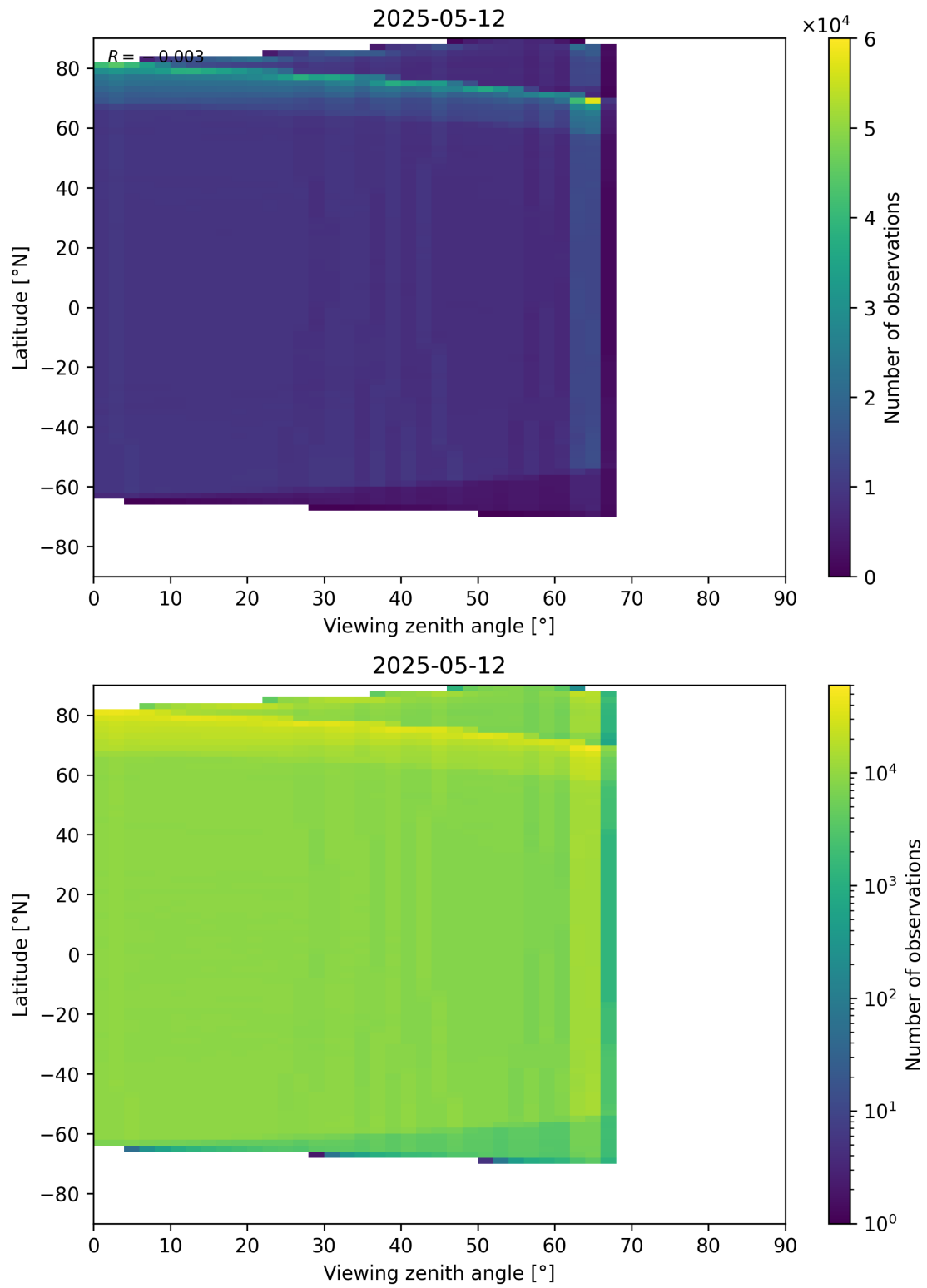
Figure 123: Scatter density plot of “Viewing zenith angle” against “Latitude” for 2025-05-11 to 2025-05-13.
