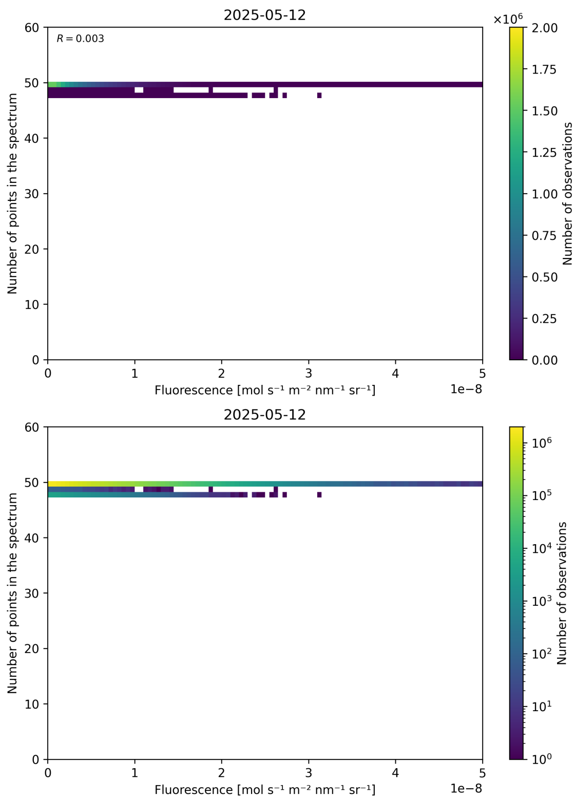
Figure 86: Scatter density plot of “Fluorescence” against “Number of points in the spectrum” for 2025-05-11 to 2025-05-13.
