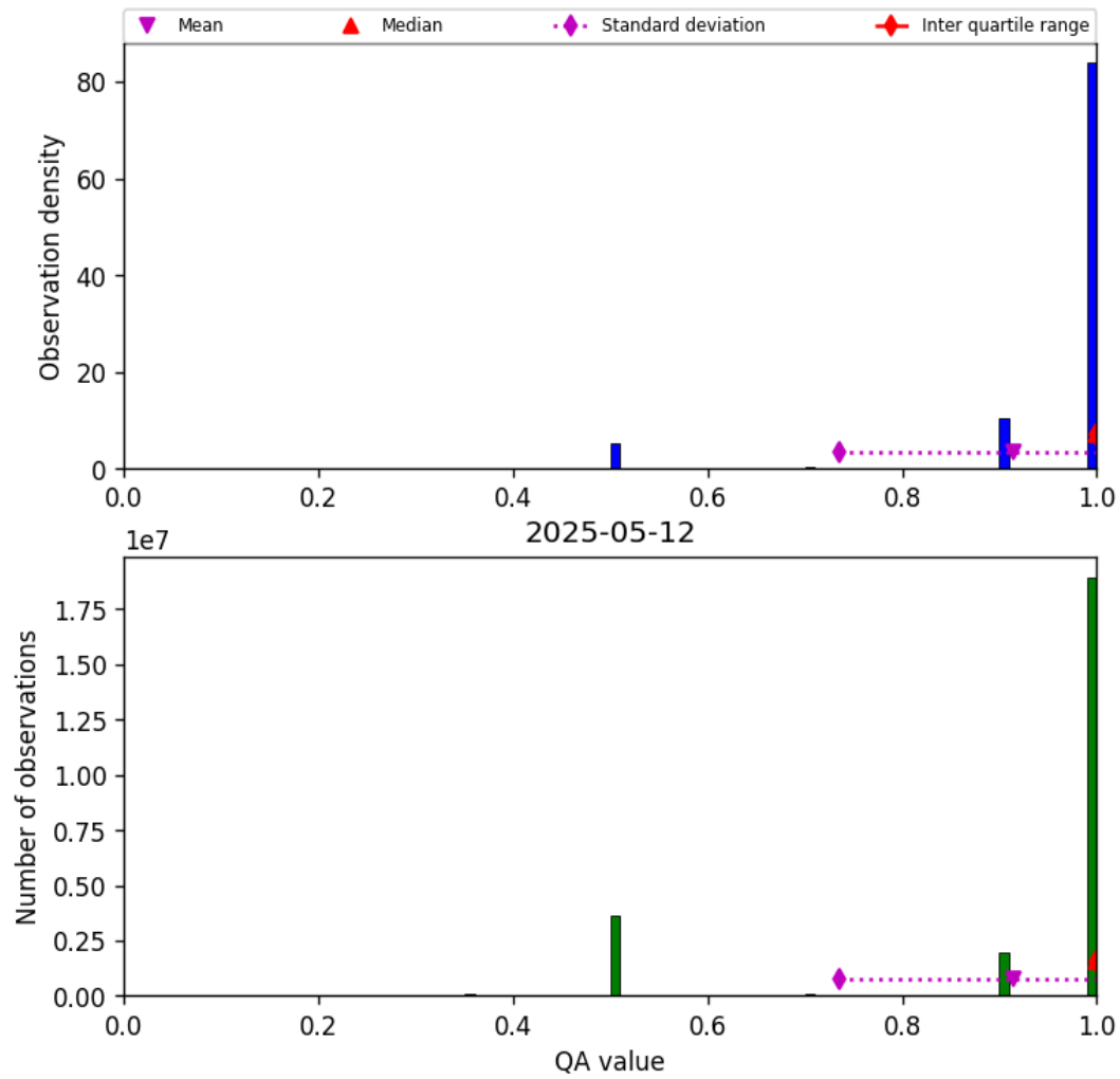
Figure 29: Histogram of “QA value” for 2025-05-11 to 2025-05-13
