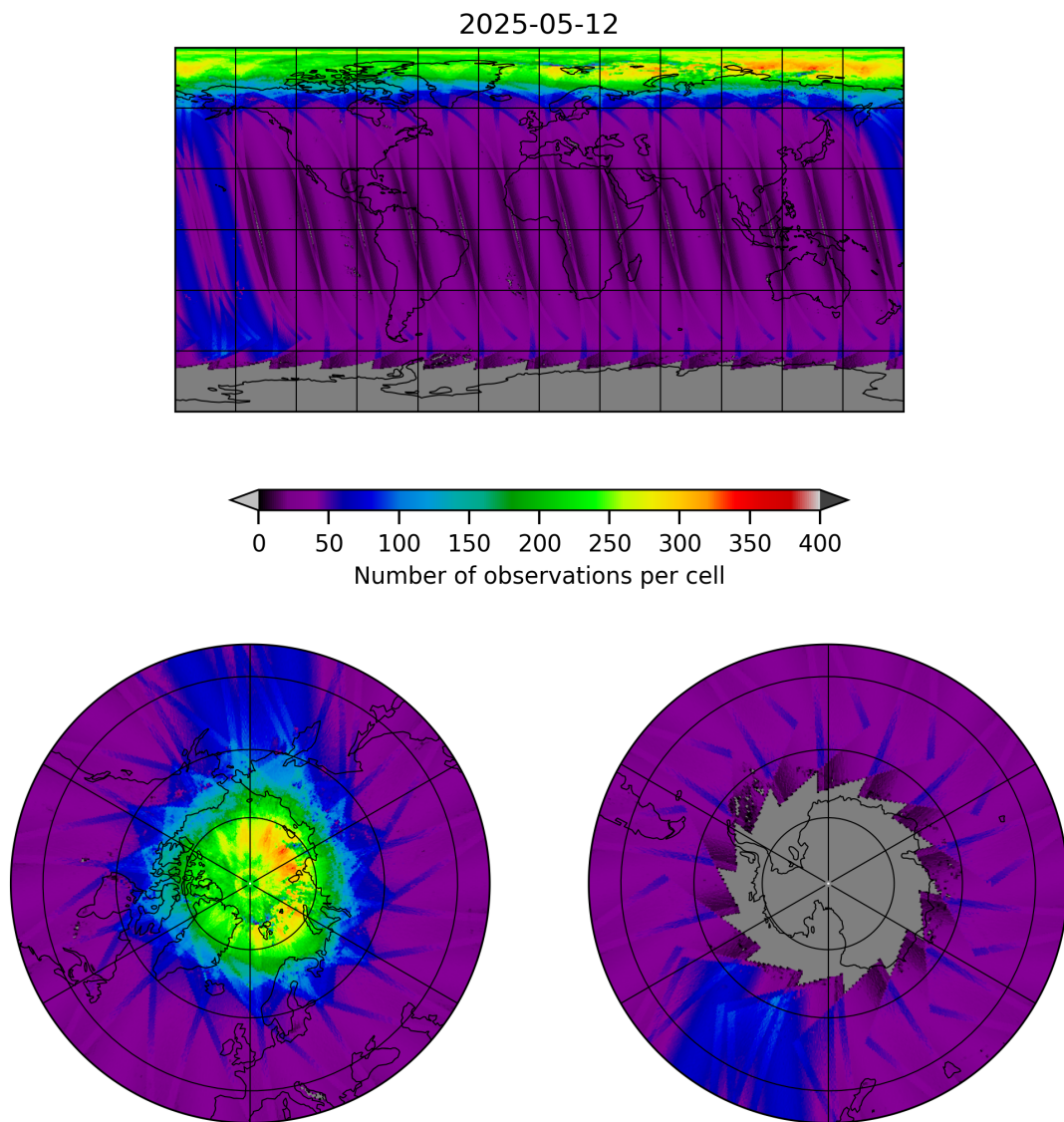
Figure 11: Map of the number of observations for 2025-05-11 to 2025-05-13
