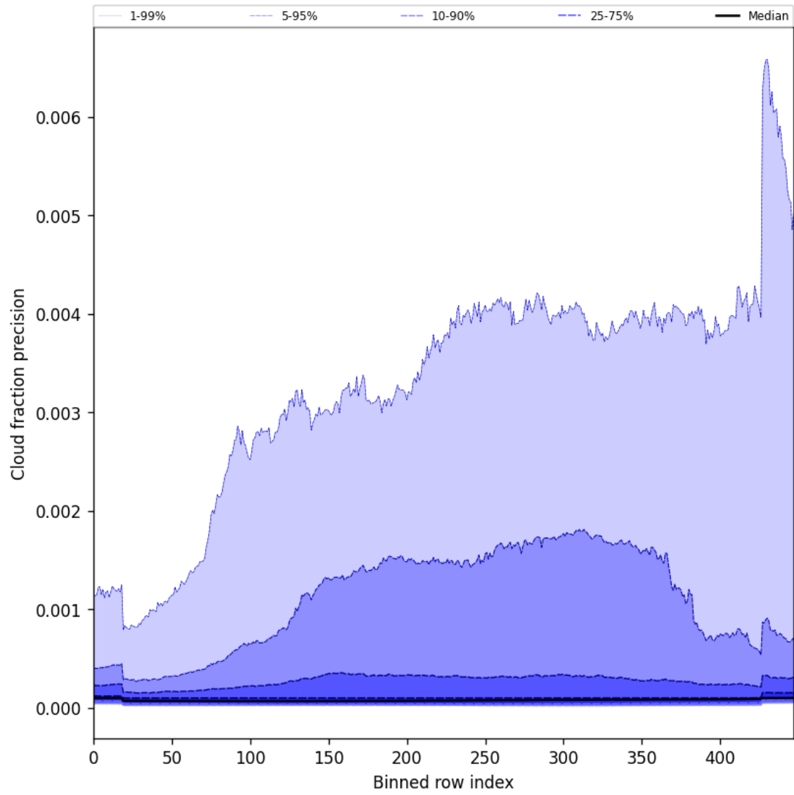
Figure 50: Along track statistics of “Cloud fraction precision” for 2025-05-11 to 2025-05-13
