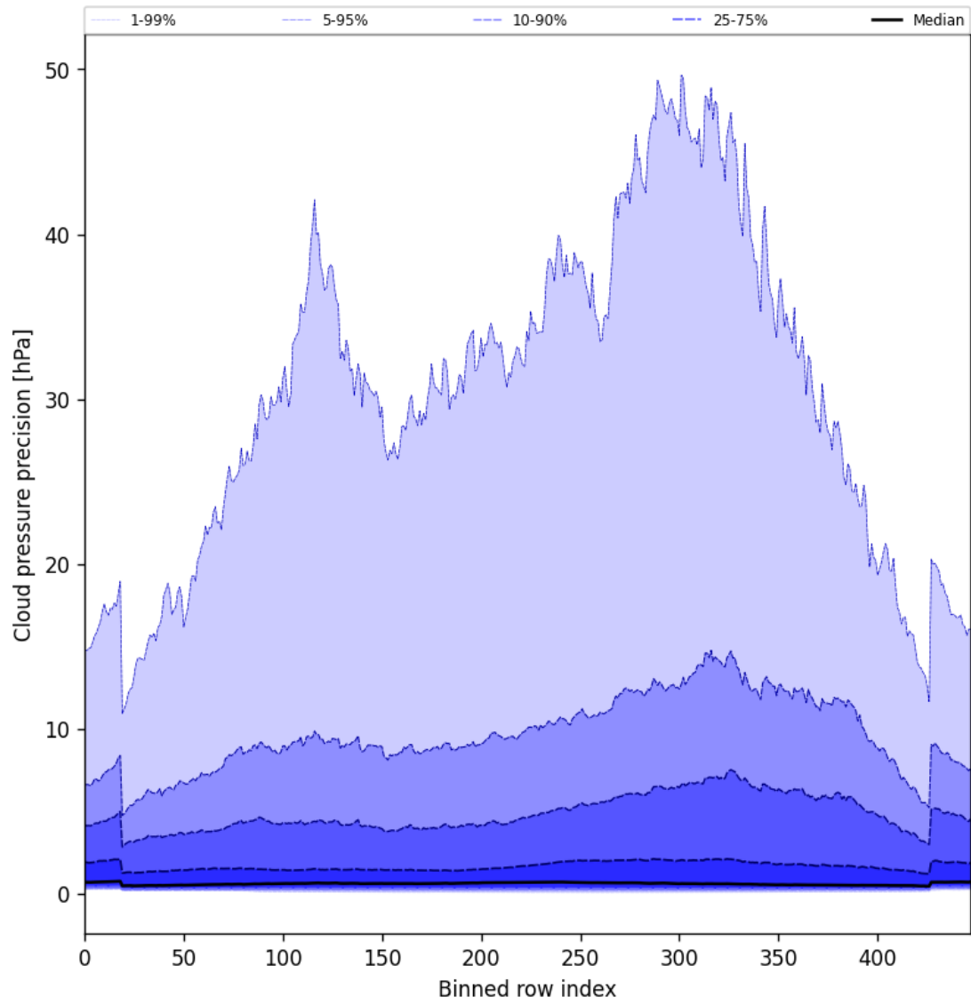
Figure 48: Along track statistics of “Cloud pressure precision” for 2025-05-11 to 2025-05-13
