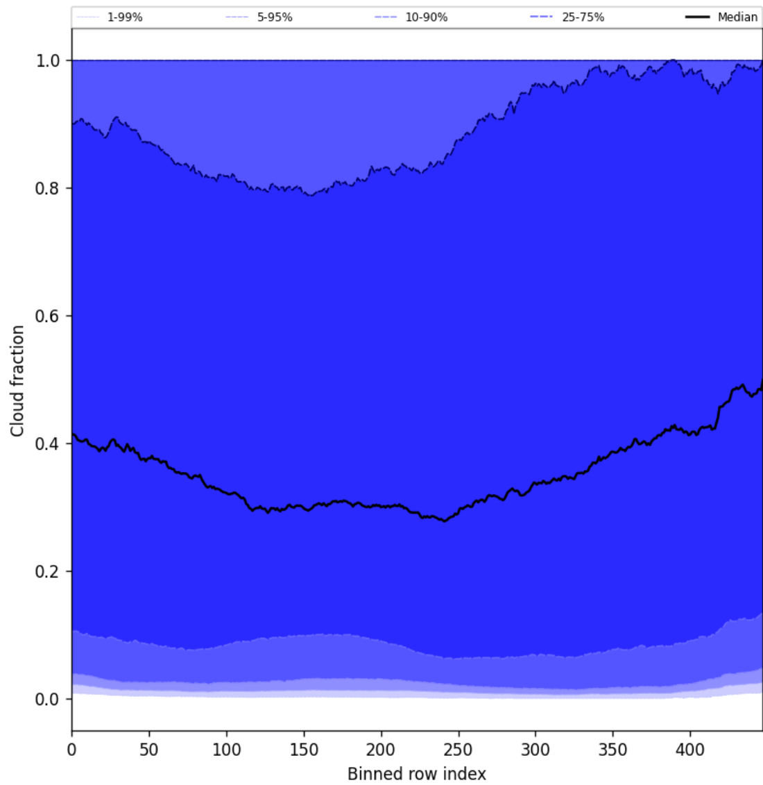
Figure 49: Along track statistics of “Cloud fraction” for 2025-05-11 to 2025-05-13
