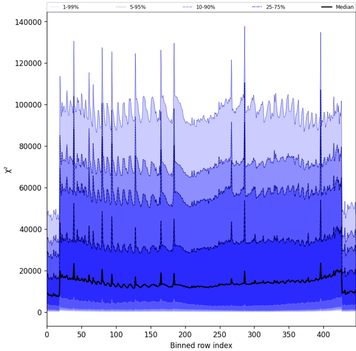
Figure 55: Along track statistics of “ \chi^2 ” for 2025-05-11 to 2025-05-13
