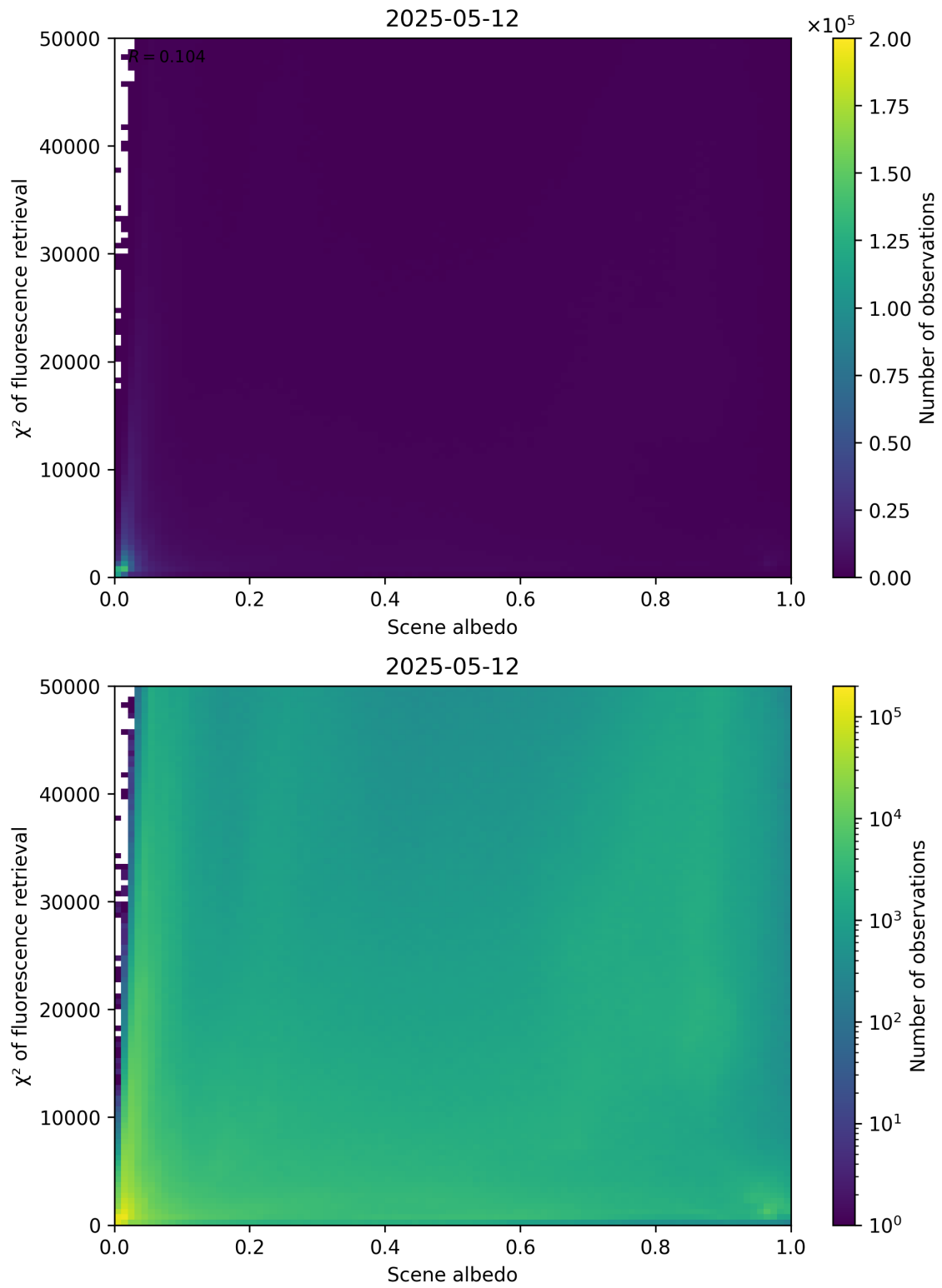
Figure 103: Scatter density plot of “Scene albedo” against “ \chi^2 of fluorescence retrieval” for 2025-05-11 to 2025-05-13.
