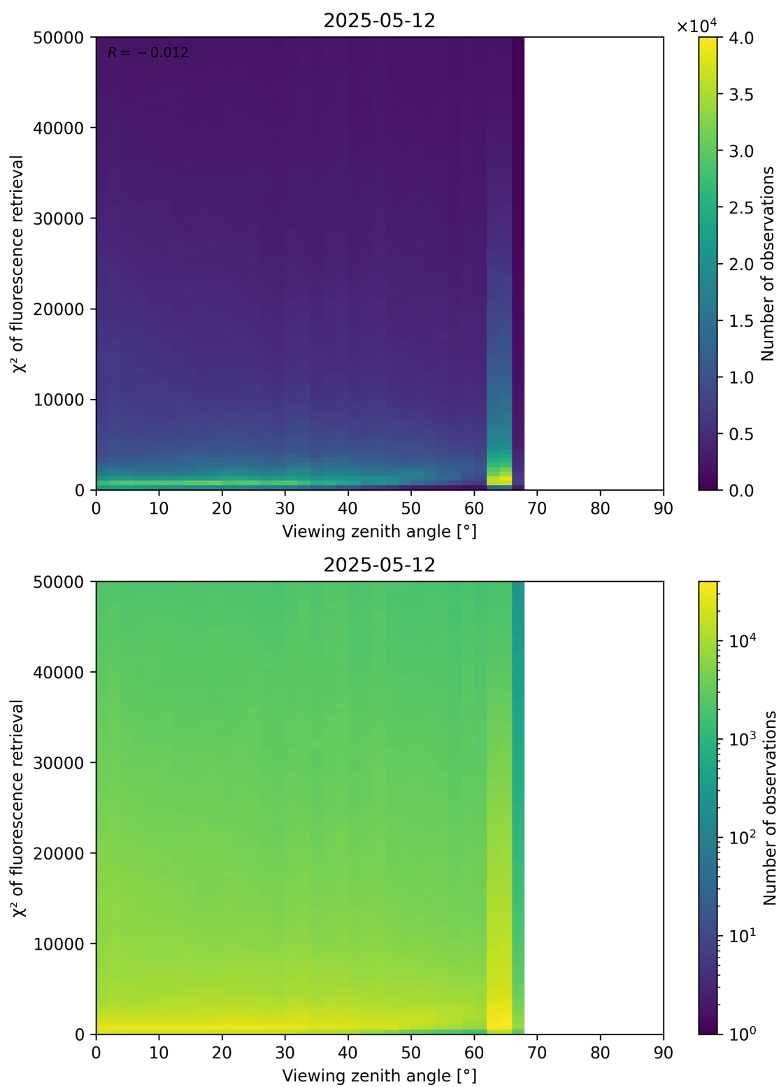
Figure 119: Scatter density plot of “Viewing zenith angle” against “ \chi^2 of fluorescence retrieval” for 2025-05-11 to 2025-05-13.
