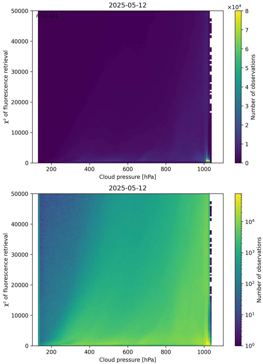
Figure 78: Scatter density plot of “Cloud pressure” against “ \chi^2 of fluorescence retrieval” for 2025-05-11 to 2025-05-13.
