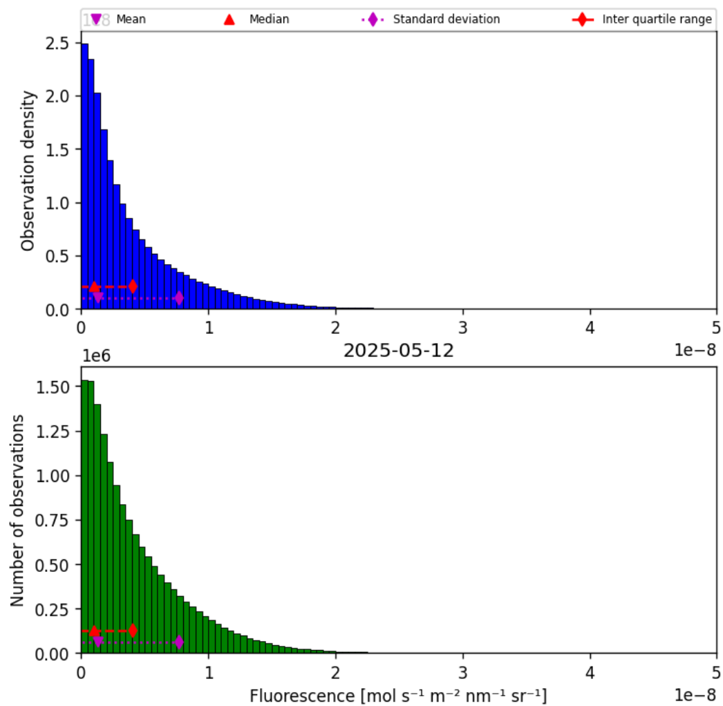
Figure 40: Histogram of “Fluorescence” for 2025-05-11 to 2025-05-13
