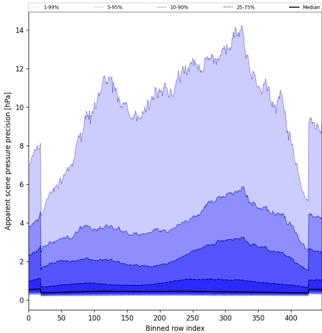
Figure 54: Along track statistics of “Apparent scene pressure precision” for 2025-05-11 to 2025-05-13
