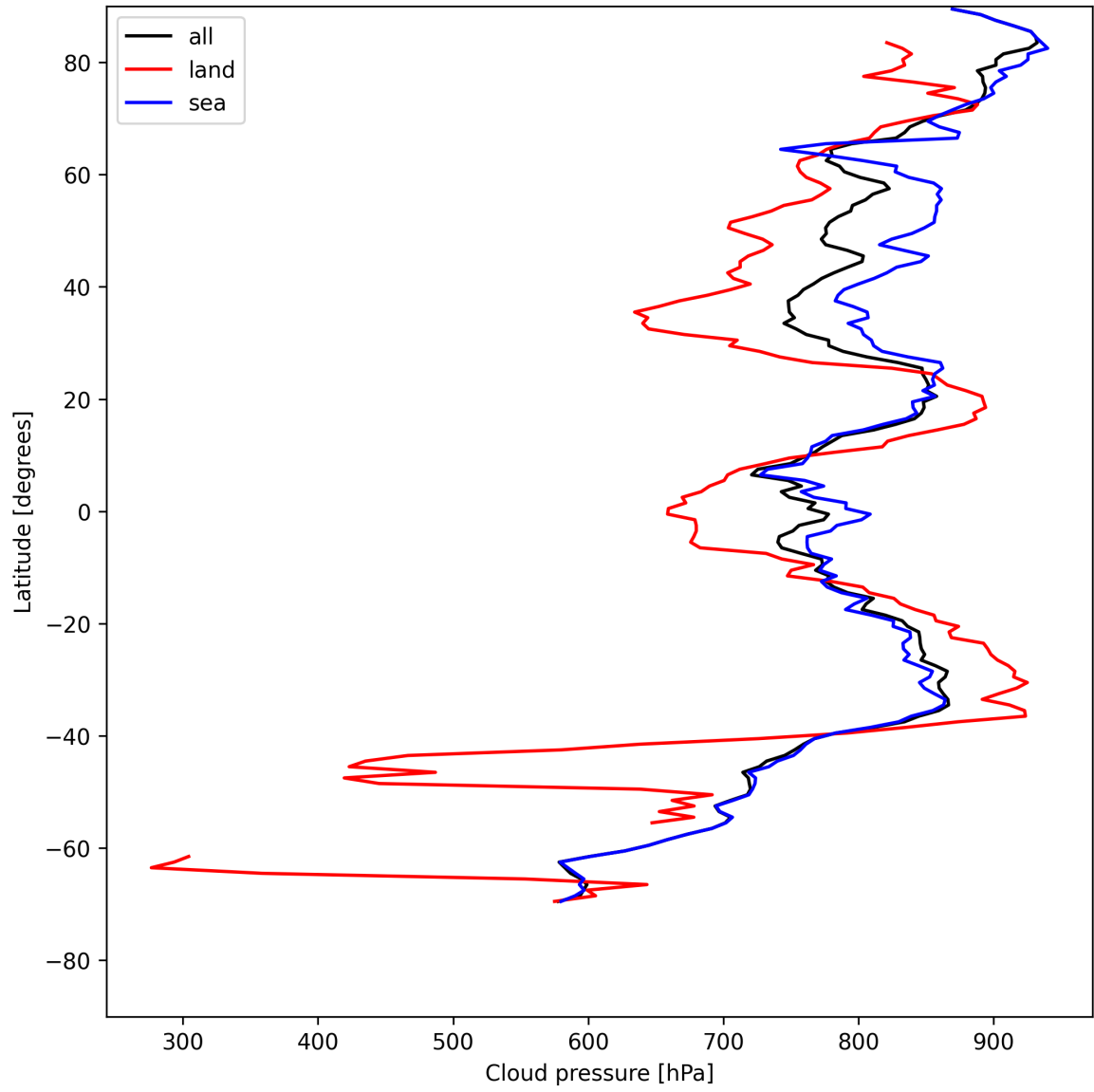
Figure 13: Zonal average of “Cloud pressure” for 2025-05-11 to 2025-05-13.
