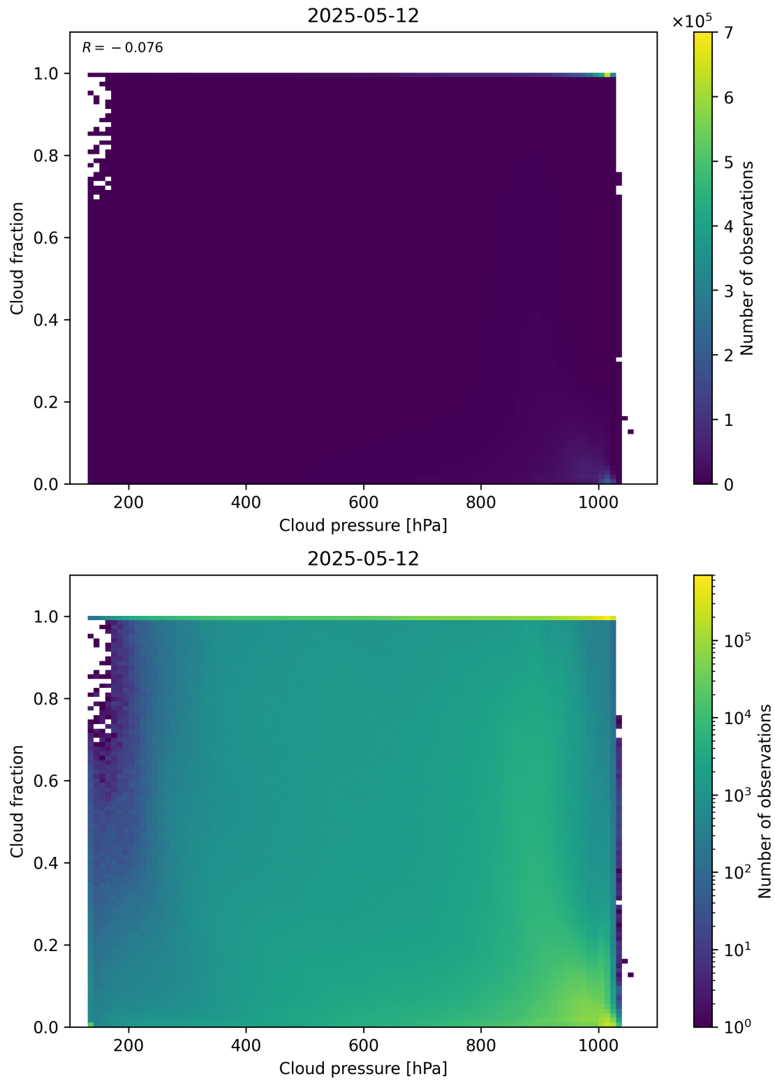
Figure 79: Scatter density plot of “Cloud pressure” against “Cloud fraction” for 2025-05-11 to 2025-05-13.
