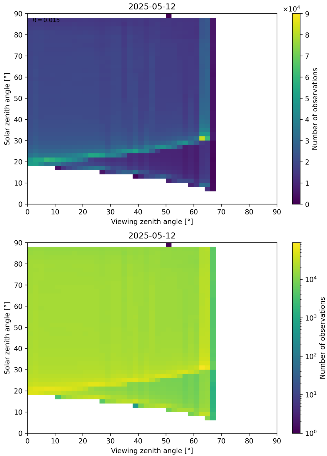
Figure 127: Scatter density plot of “Viewing zenith angle” against “Solar zenith angle” for 2025-05-11 to 2025-05-13.
