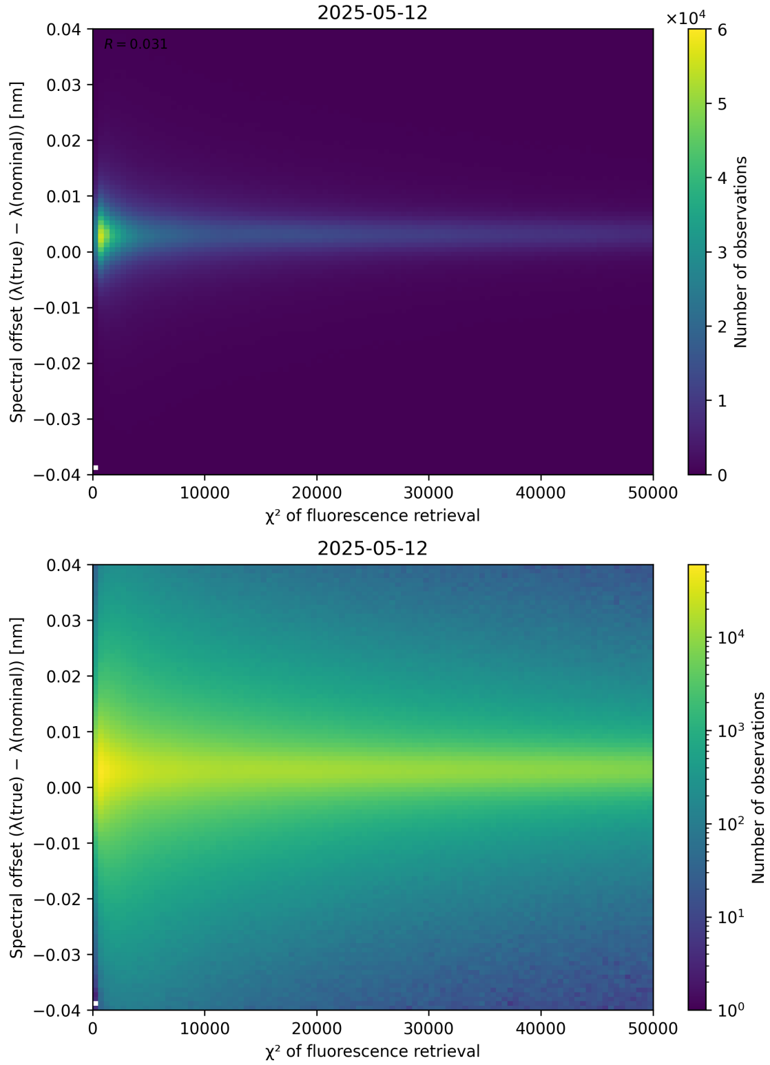
Figure 69: Scatter density plot of “ \chi^2 of fluorescence retrieval” against “Spectral offset ( \lambda_{\text{true}} - \lambda_{\text{nominal}} )” for 2025-05-11 to 2025-05-13.
