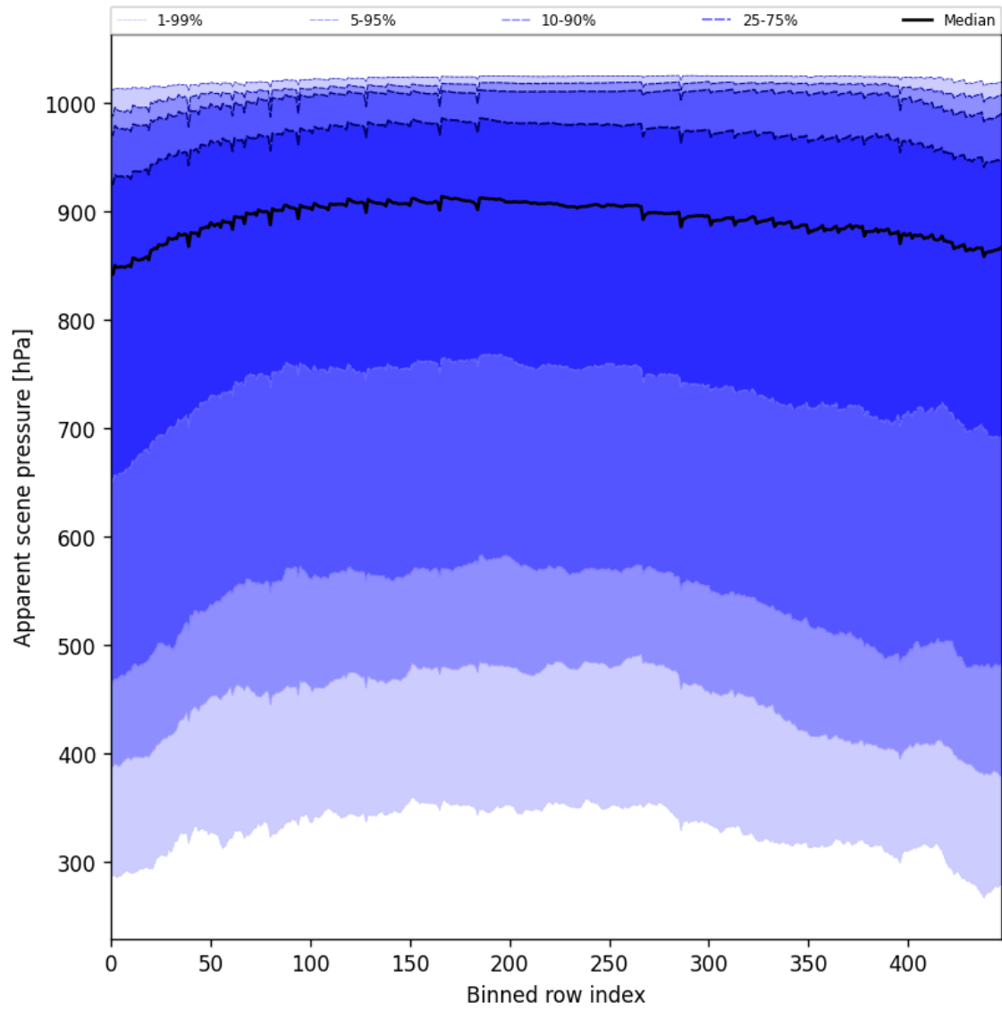
Figure 53: Along track statistics of “Apparent scene pressure” for 2025-05-11 to 2025-05-13
