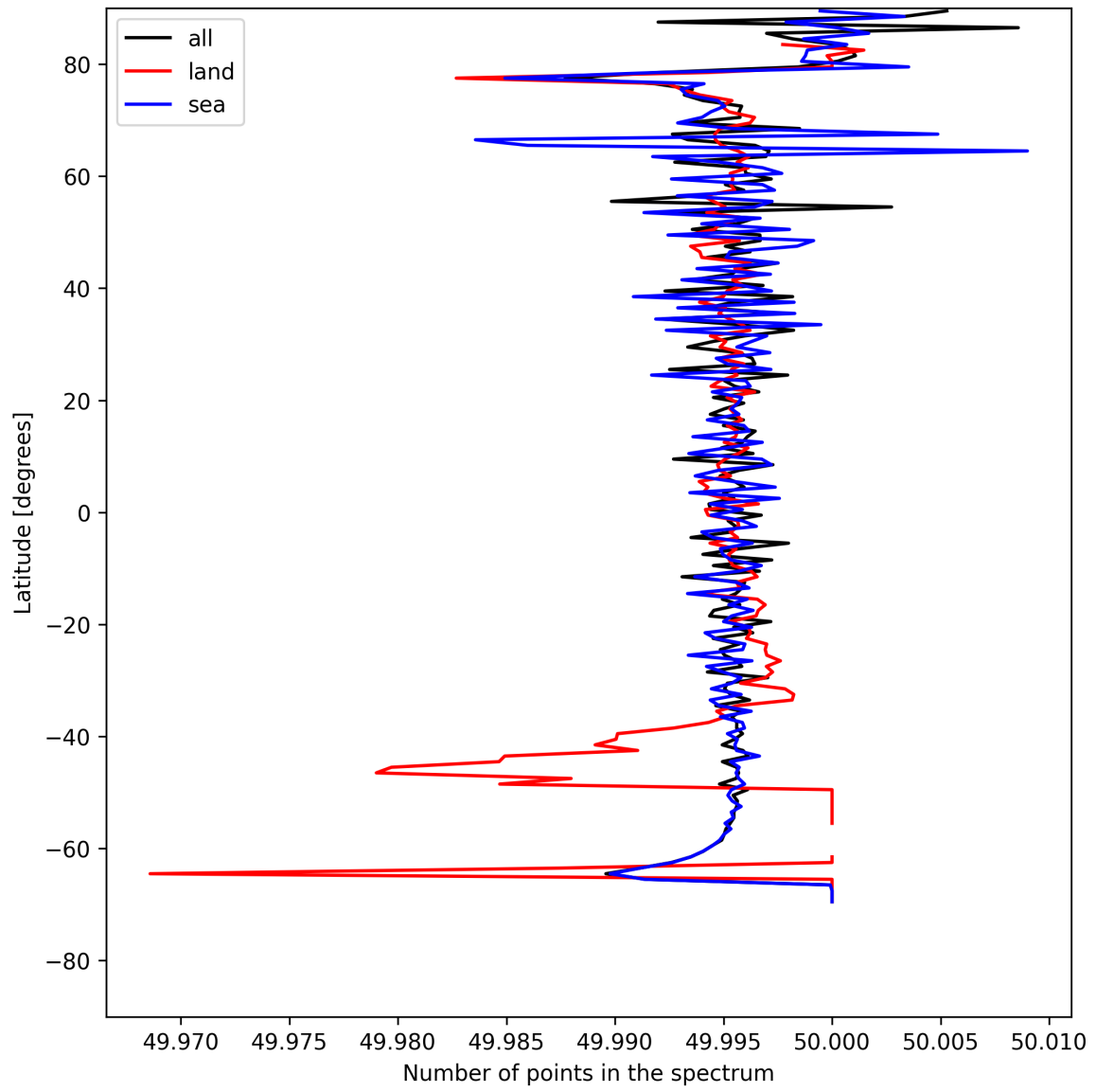
Figure 27: Zonal average of “Number of points in the spectrum” for 2025-05-11 to 2025-05-13.
