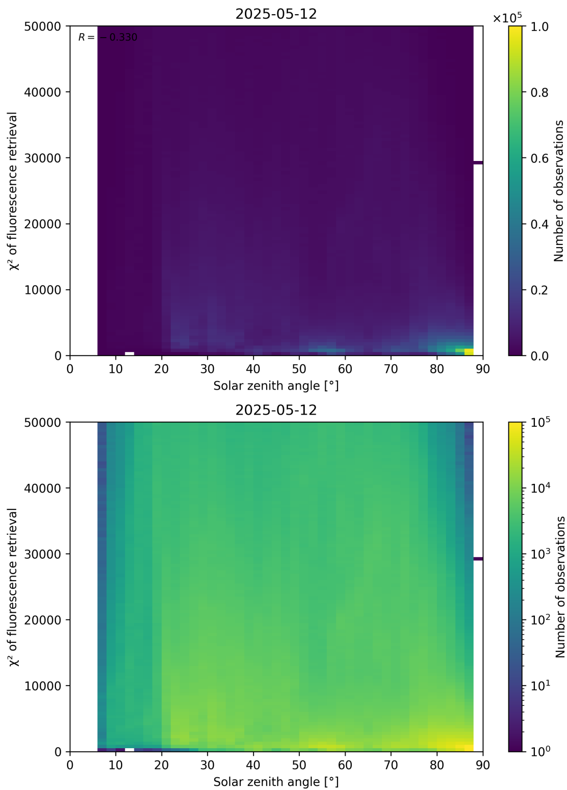
Figure 109: Scatter density plot of “Solar zenith angle” against “ \chi^2 of fluorescence retrieval” for 2025-05-11 to 2025-05-13.
