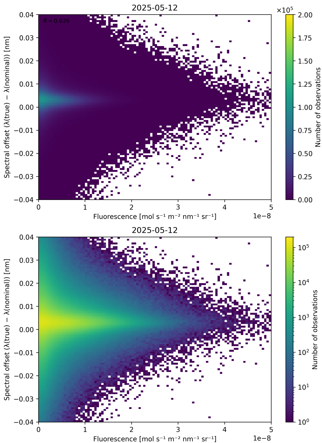
Figure 87: Scatter density plot of “Fluorescence” against “Spectral offset ( \lambda_{\text{true}} - \lambda_{\text{nominal}} )” for 2025-05-11 to 2025-05-13.
