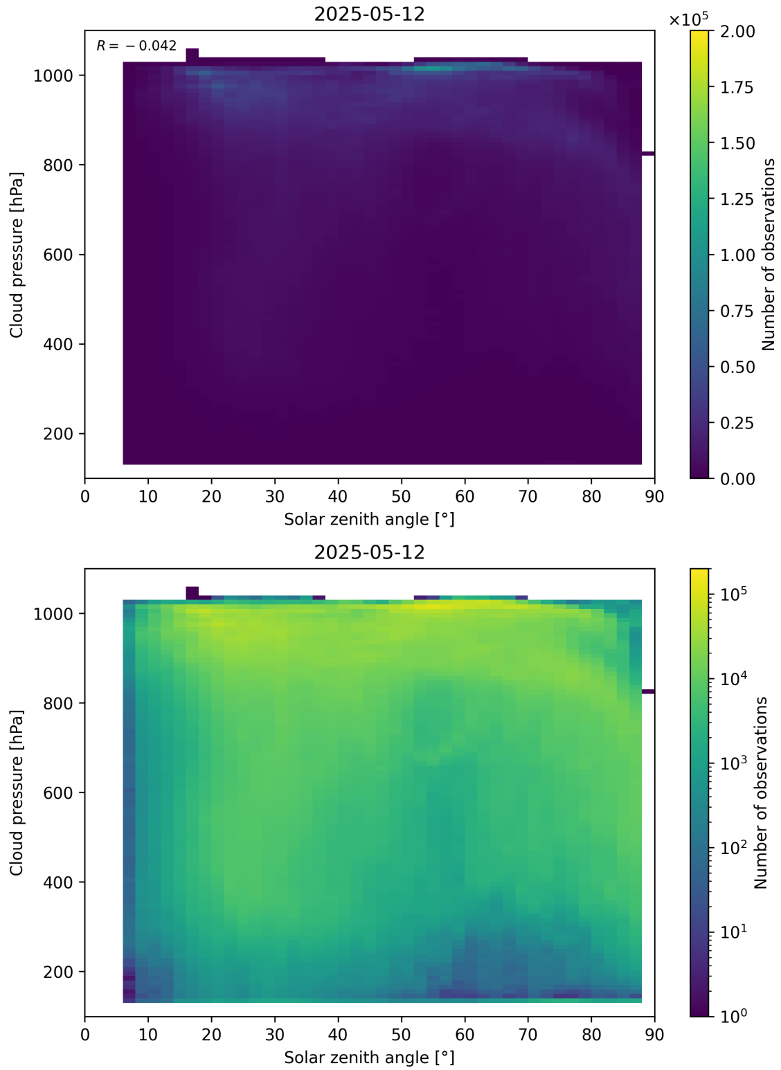
Figure 111: Scatter density plot of “Solar zenith angle” against “Cloud pressure” for 2025-05-11 to 2025-05-13.
