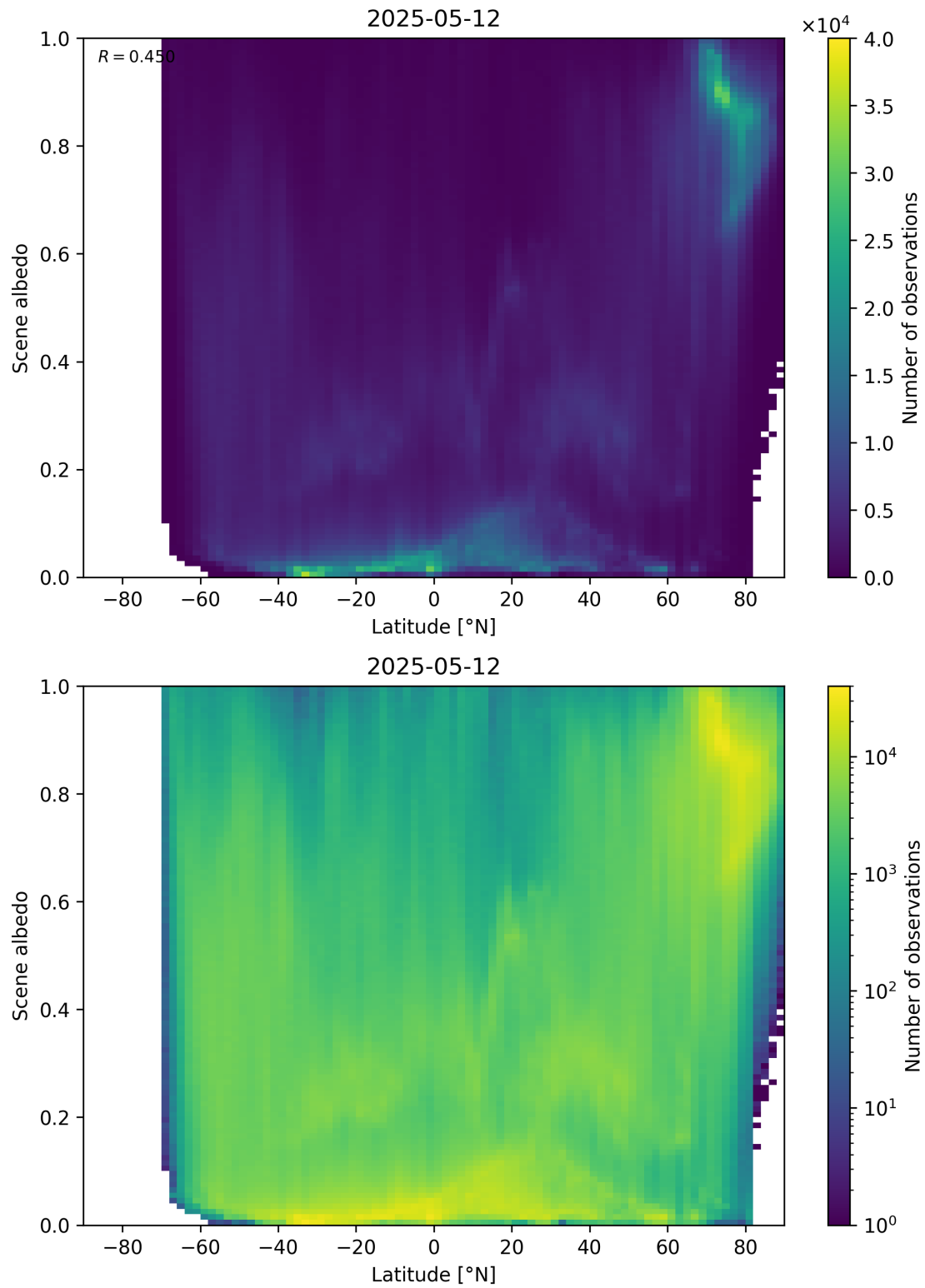
Figure 95: Scatter density plot of “Latitude” against “Scene albedo” for 2025-05-11 to 2025-05-13.
