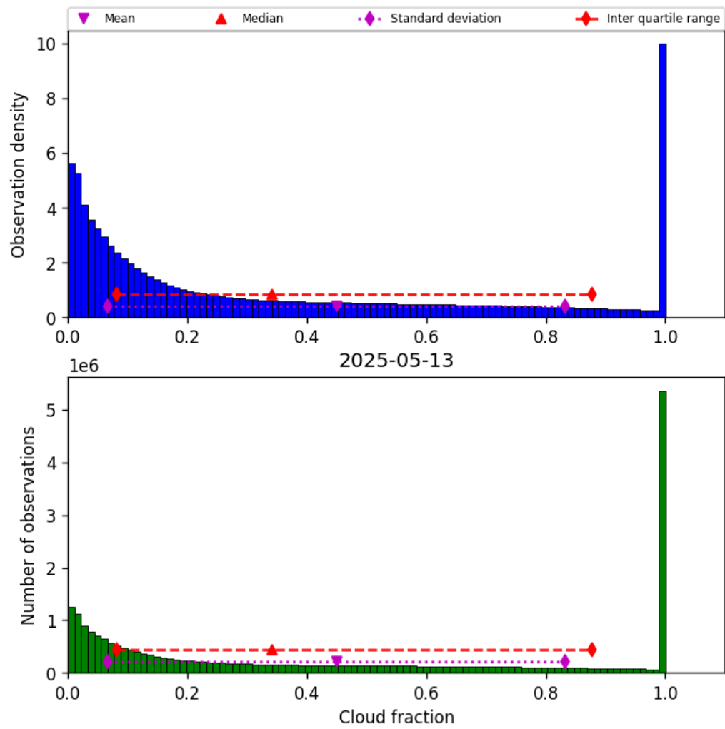
Figure 32: Histogram of “Cloud fraction” for 2025-05-12 to 2025-05-14
