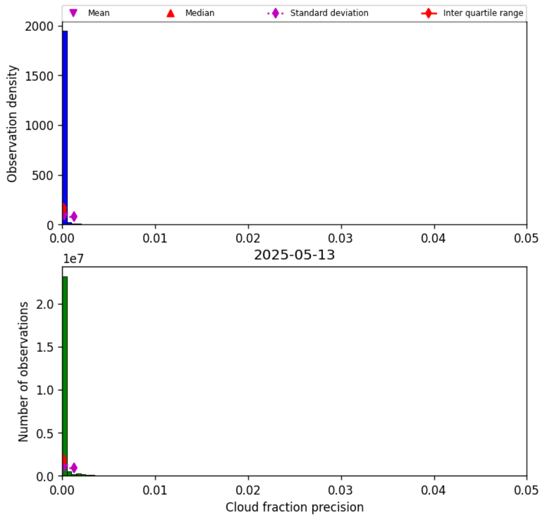
Figure 33: Histogram of “Cloud fraction precision” for 2025-05-12 to 2025-05-14
