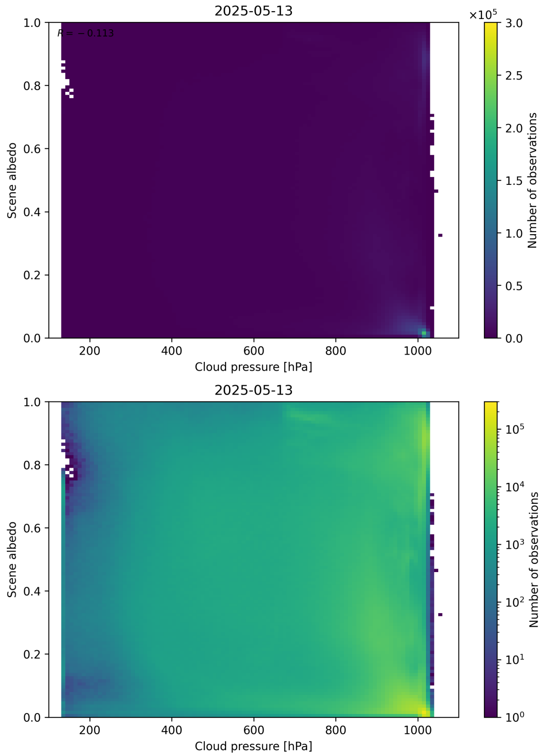
Figure 83: Scatter density plot of “Cloud pressure” against “Scene albedo” for 2025-05-12 to 2025-05-14.
