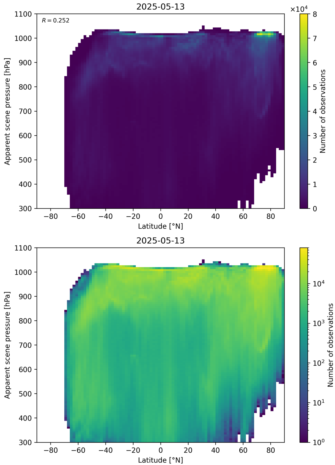
Figure 88: Scatter density plot of “Latitude” against “Apparent scene pressure” for 2025-05-12 to 2025-05-14.
