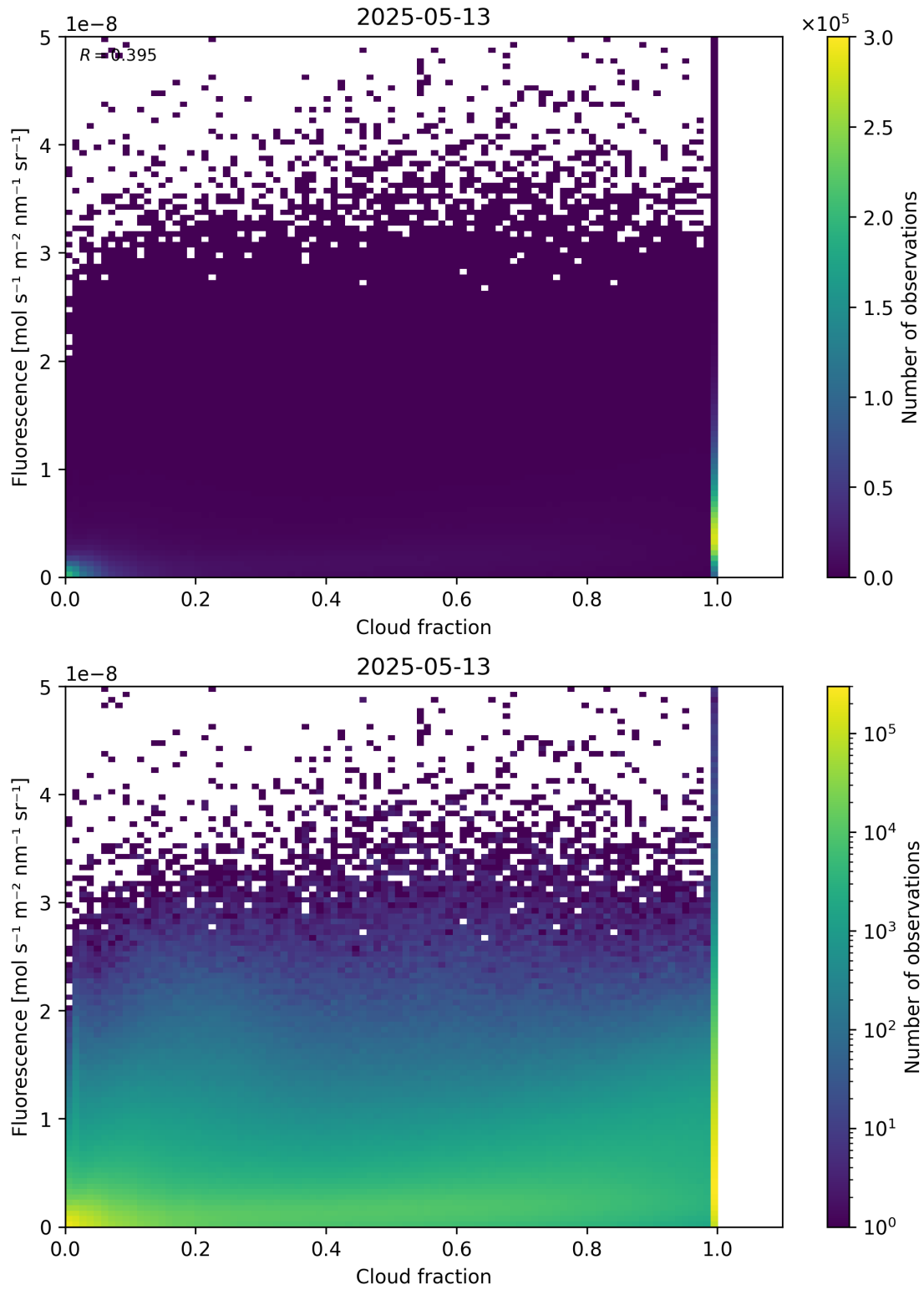
Figure 72: Scatter density plot of “Cloud fraction” against “Fluorescence” for 2025-05-12 to 2025-05-14.
