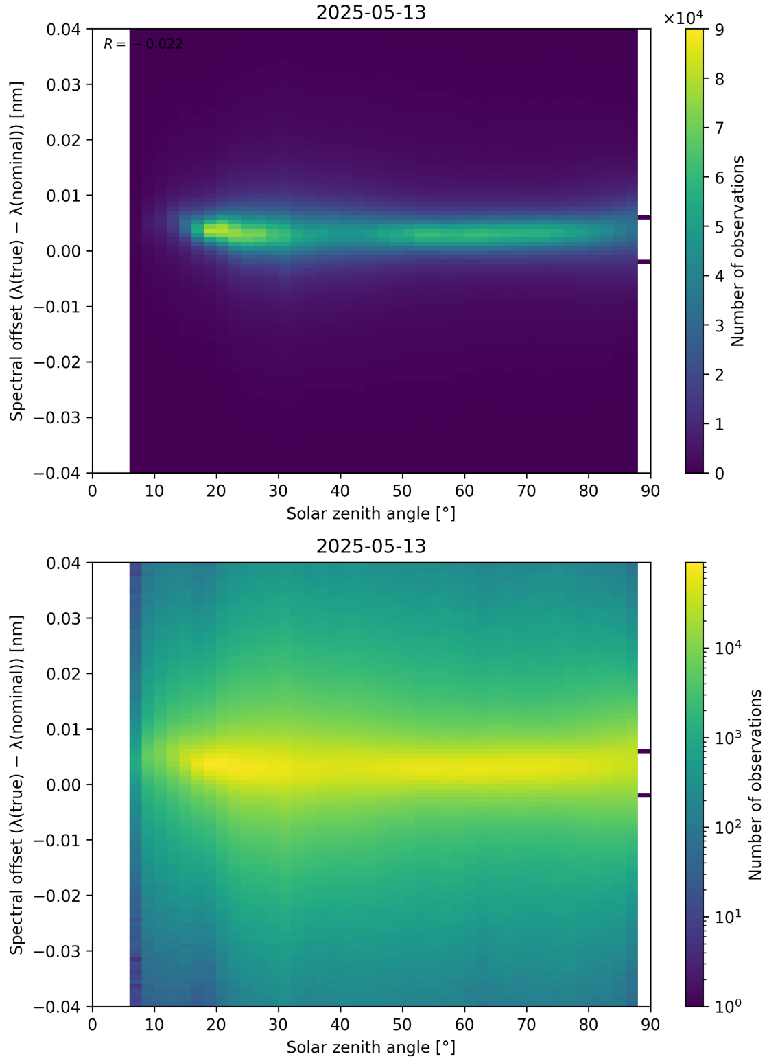
Figure 117: Scatter density plot of “Solar zenith angle” against “Spectral offset ( \lambda_{\text{true}} - \lambda_{\text{nominal}} )” for 2025-05-12 to 2025-05-14.
