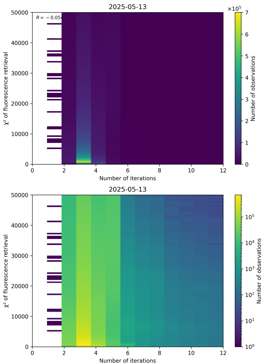
Figure 97: Scatter density plot of “Number of iterations” against “ \chi^2 of fluorescence retrieval” for 2025-05-12 to 2025-05-14.
