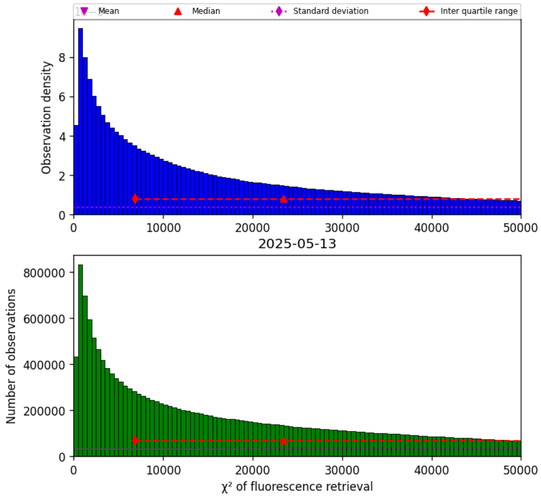
Figure 42: Histogram of “ \chi^2 of fluorescence retrieval” for 2025-05-12 to 2025-05-14
