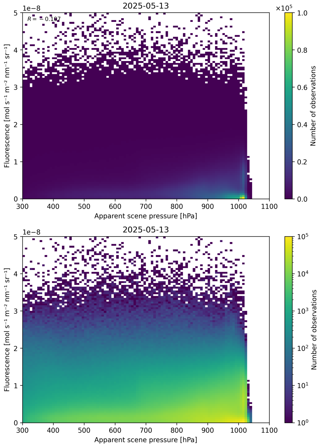
Figure 64: Scatter density plot of “Apparent scene pressure” against “Fluorescence” for 2025-05-12 to 2025-05-14.
