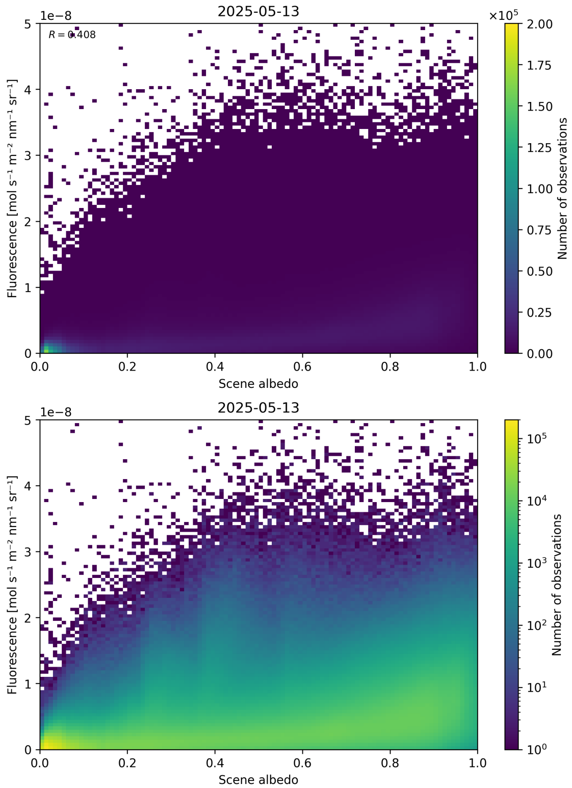
Figure 104: Scatter density plot of “Scene albedo” against “Fluorescence” for 2025-05-12 to 2025-05-14.
