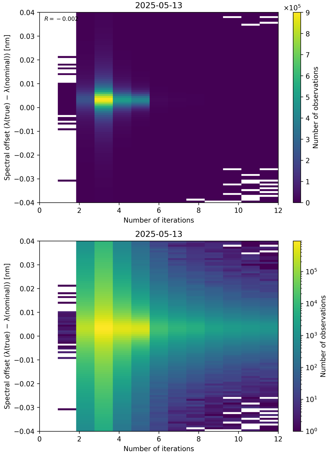
Figure 100: Scatter density plot of “Number of iterations” against “Spectral offset ( \lambda_{\text{true}} - \lambda_{\text{nominal}} )” for 2025-05-12 to 2025-05-14.
