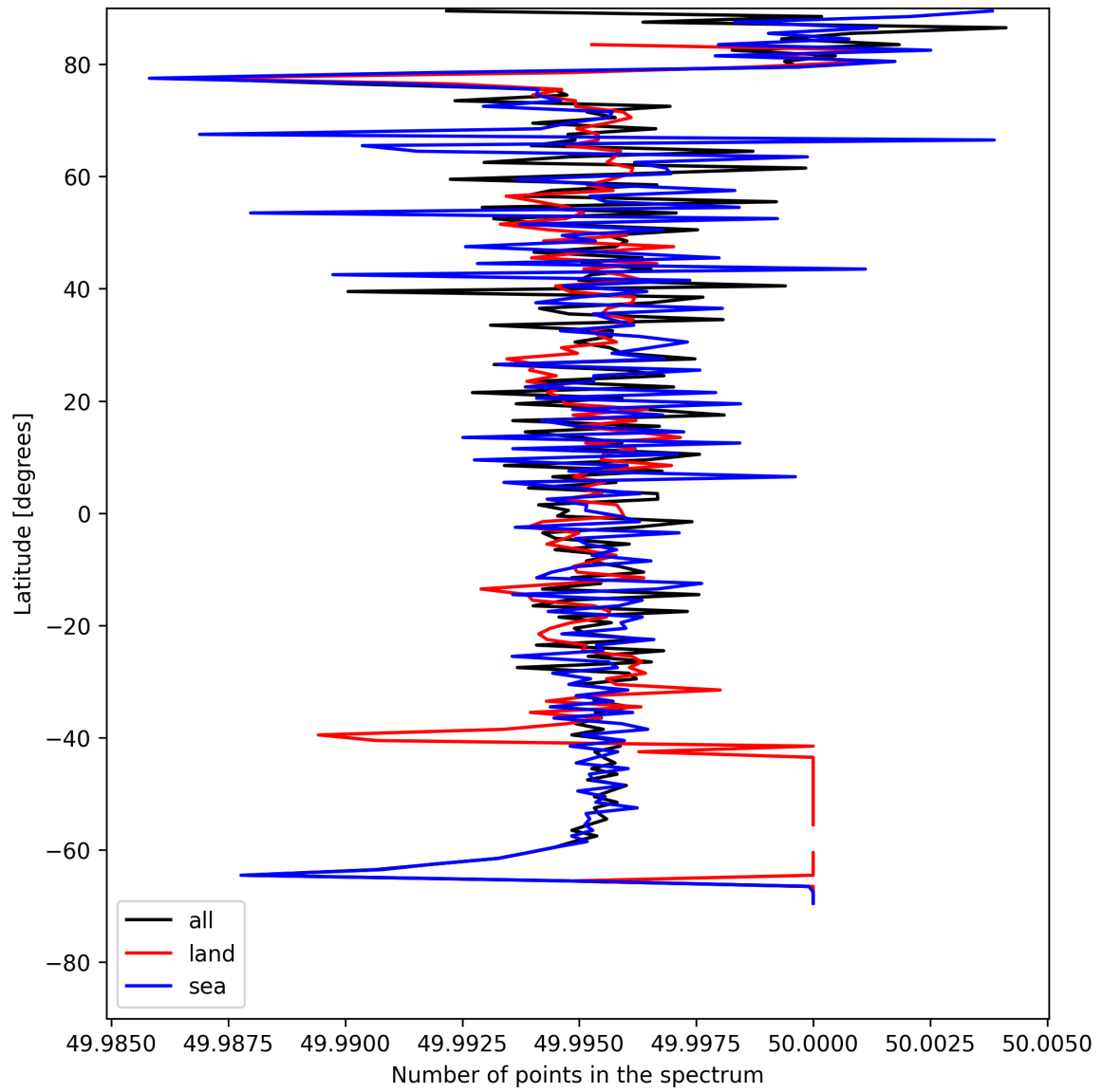
Figure 27: Zonal average of “Number of points in the spectrum” for 2025-05-12 to 2025-05-14.
