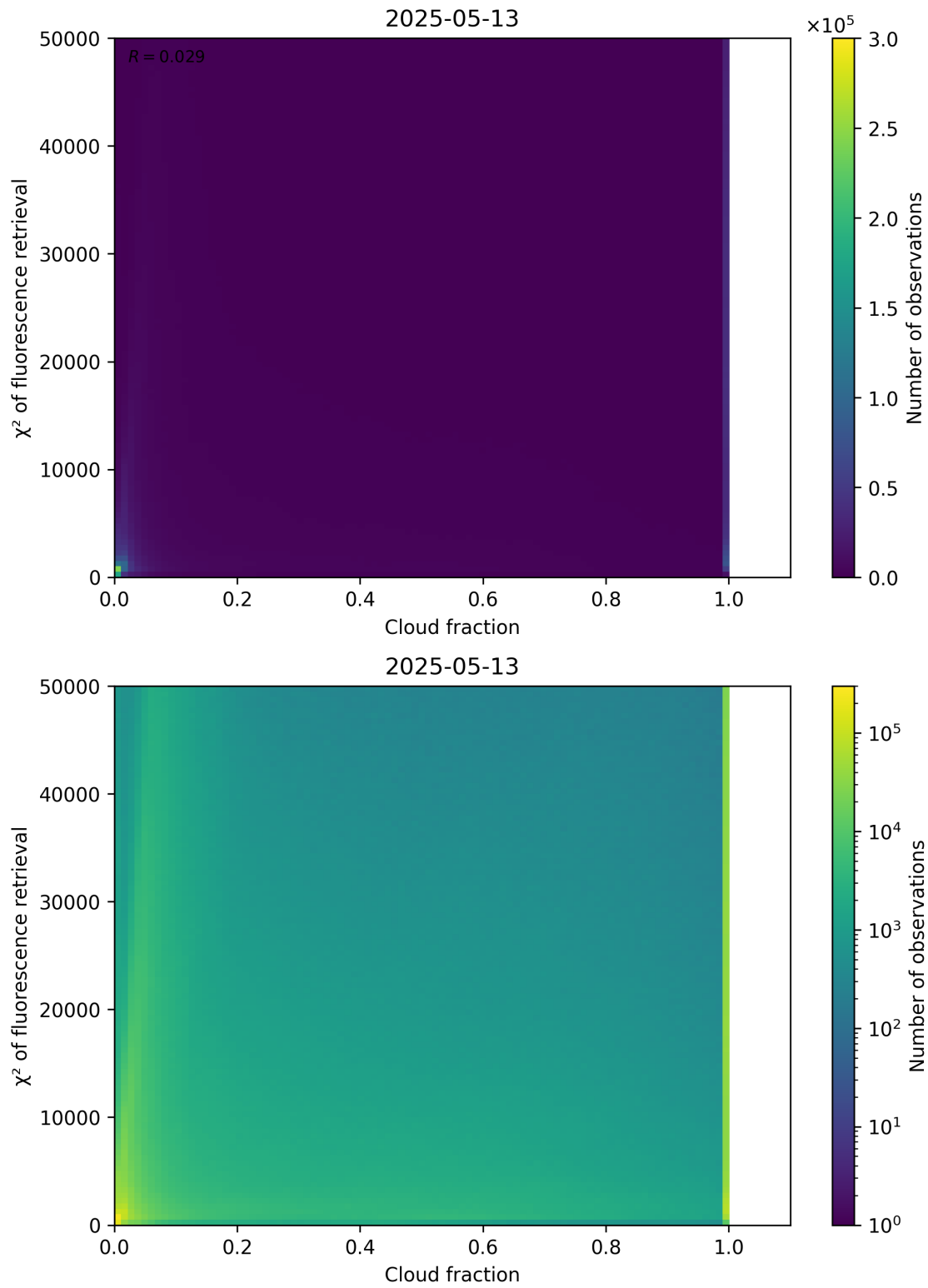
Figure 71: Scatter density plot of “Cloud fraction” against “ \chi^2 of fluorescence retrieval” for 2025-05-12 to 2025-05-14.
