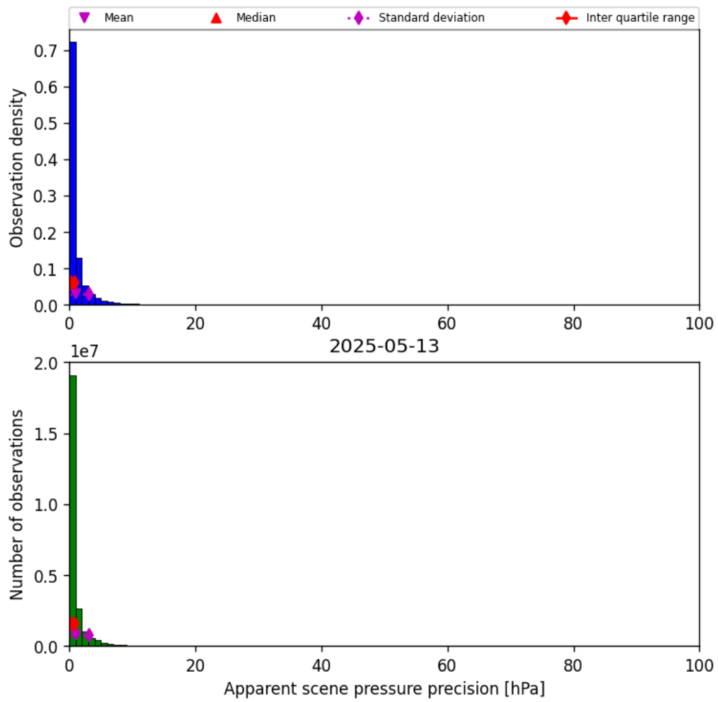
Figure 37: Histogram of "Apparent scene pressure precision" for 2025-05-12 to 2025-05-14
