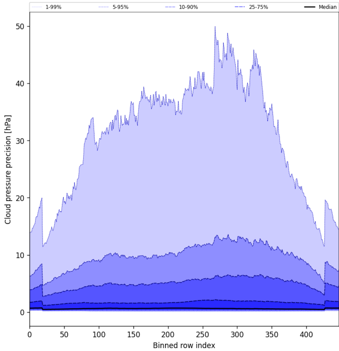
Figure 48: Along track statistics of “Cloud pressure precision” for 2025-05-12 to 2025-05-14
