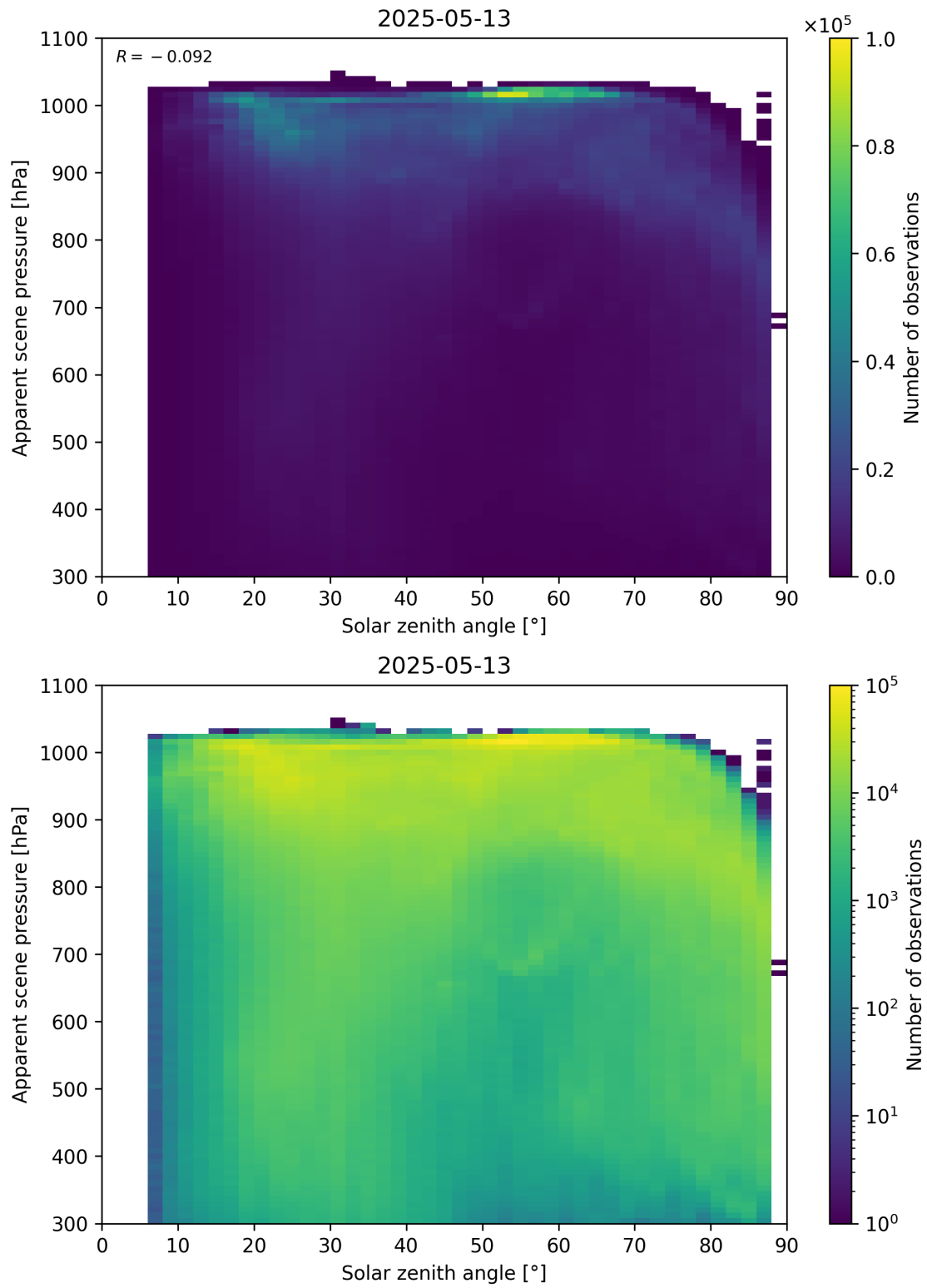
Figure 108: Scatter density plot of “Solar zenith angle” against “Apparent scene pressure” for 2025-05-12 to 2025-05-14.
