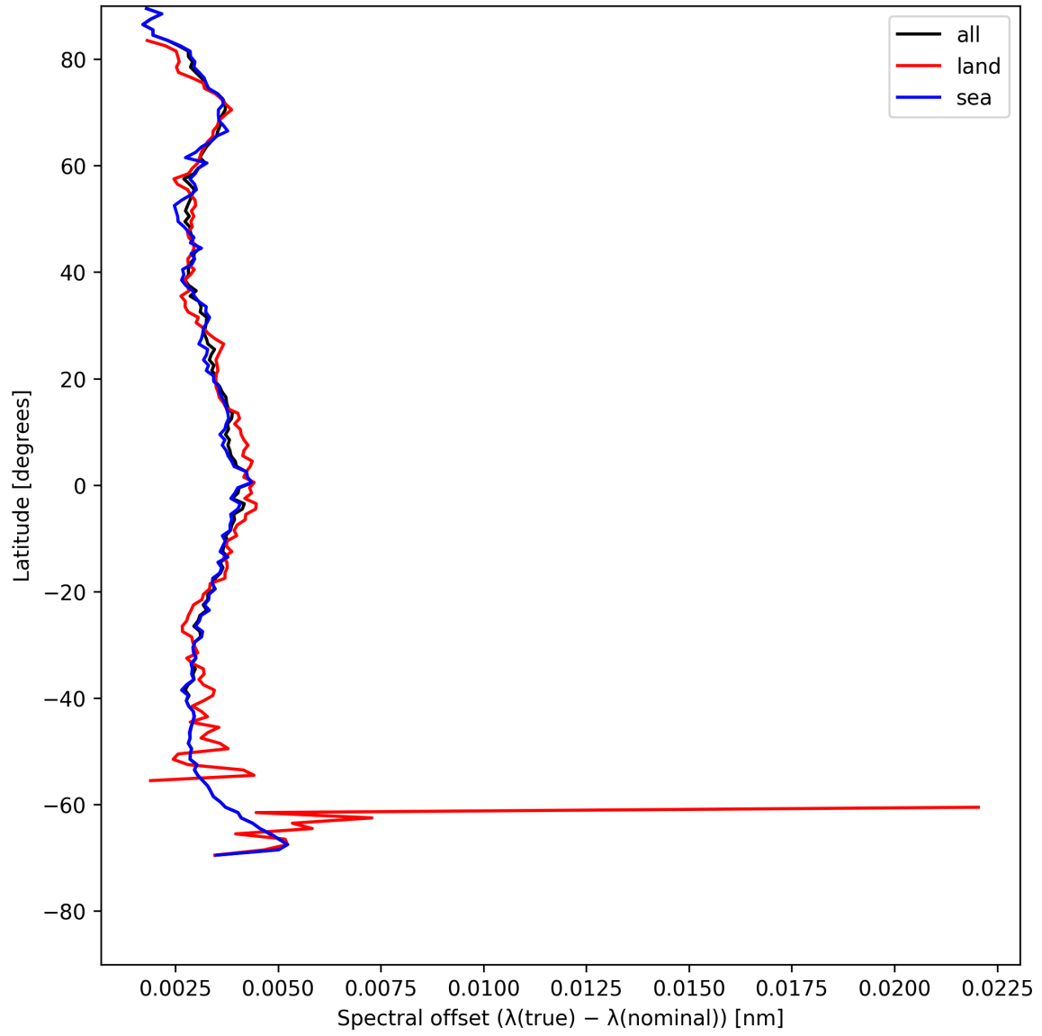
Figure 28: Zonal average of “Spectral offset ( \lambda_{\text{true}} - \lambda_{\text{nominal}} )” for 2025-05-12 to 2025-05-14.
