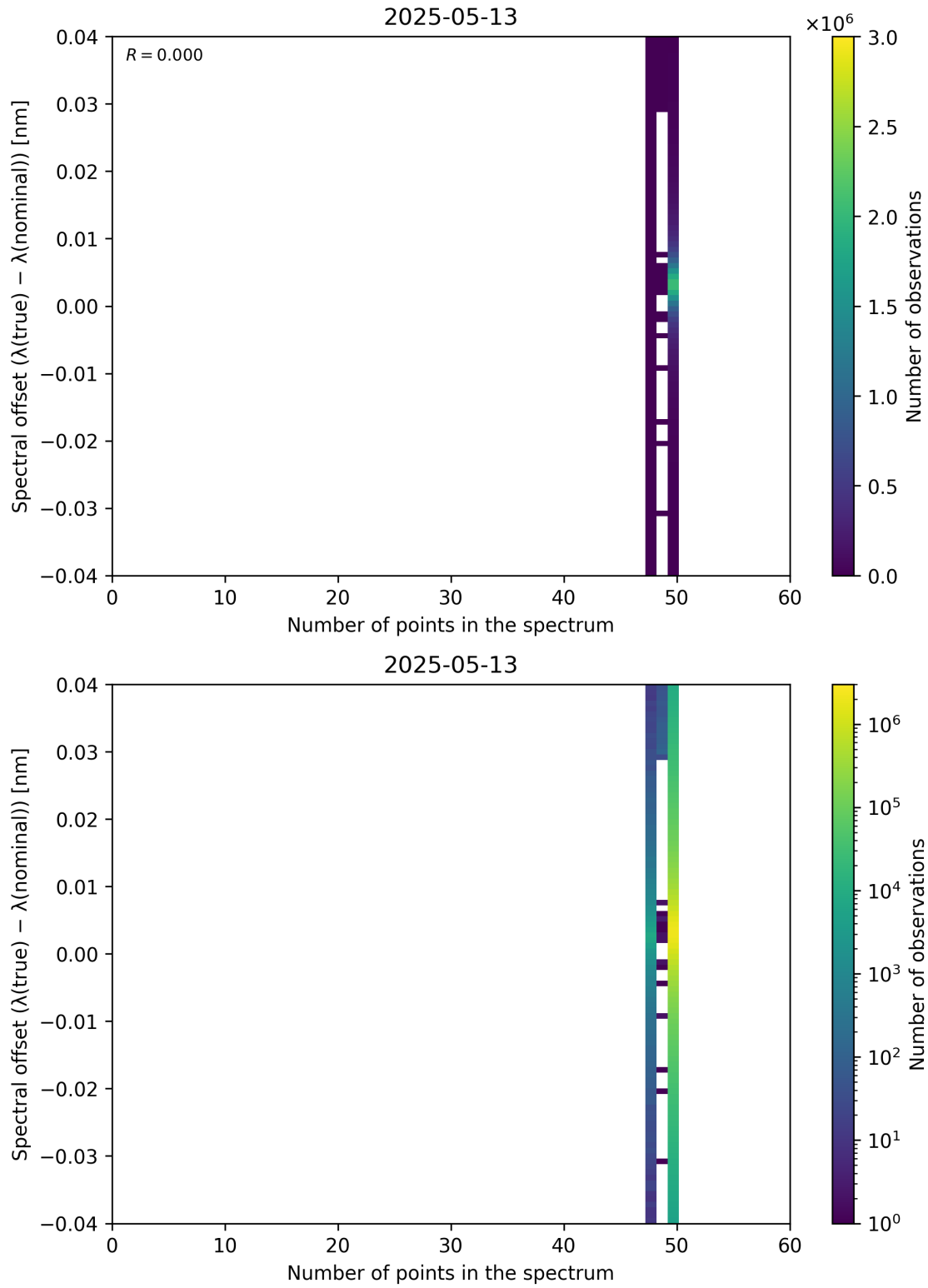
Figure 101: Scatter density plot of “Number of points in the spectrum” against “Spectral offset ( \lambda_{\text{true}} - \lambda_{\text{nominal}} )” for 2025-05-12 to 2025-05-14.
