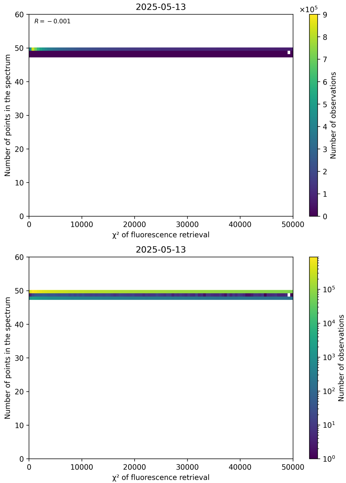
Figure 68: Scatter density plot of “ \chi^2 of fluorescence retrieval” against “Number of points in the spectrum” for 2025-05-12 to 2025-05-14.
