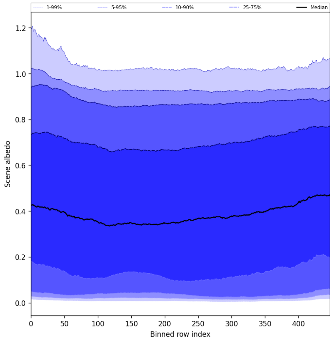
Figure 51: Along track statistics of “Scene albedo” for 2025-05-12 to 2025-05-14
