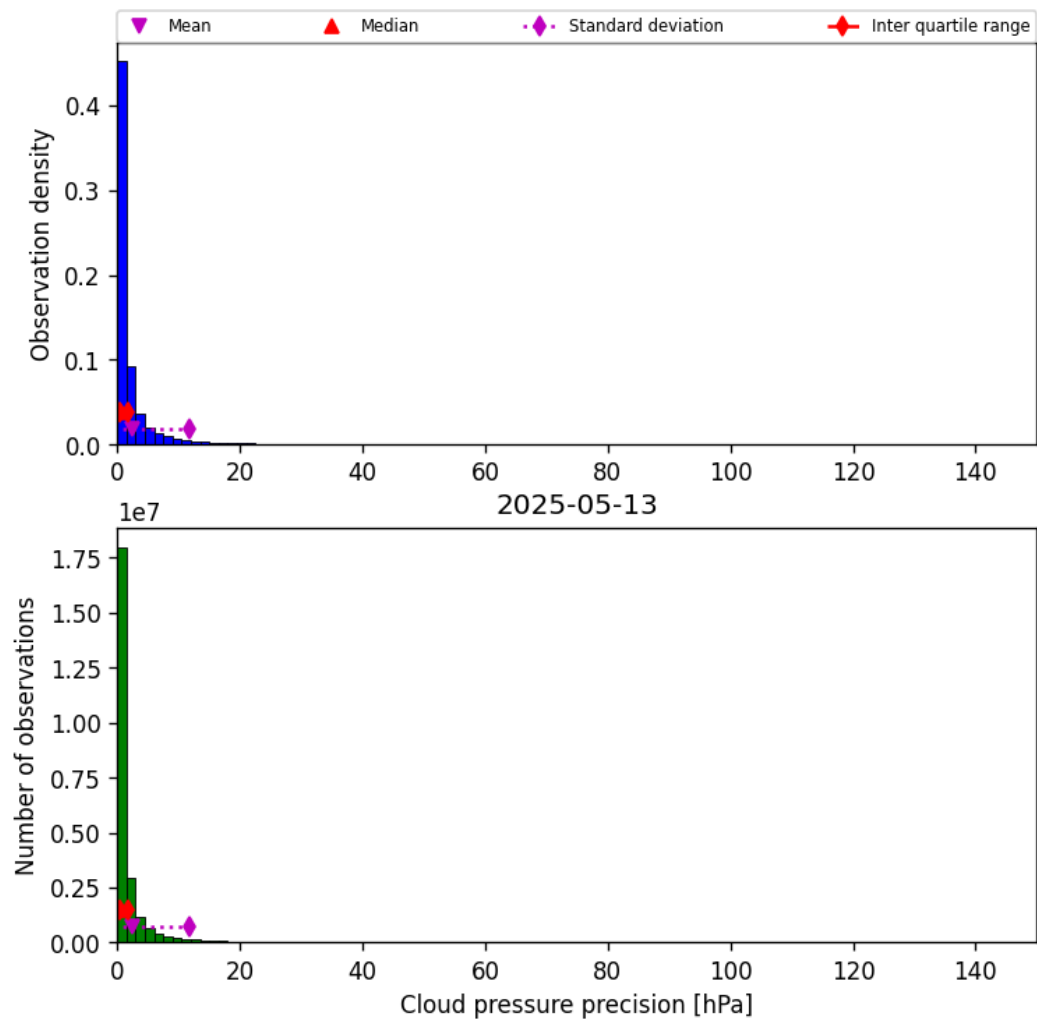
Figure 31: Histogram of “Cloud pressure precision” for 2025-05-12 to 2025-05-14
