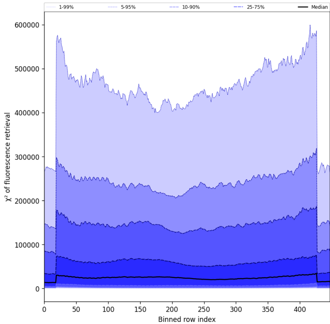
Figure 59: Along track statistics of “ \chi^2 of fluorescence retrieval” for 2025-05-12 to 2025-05-14
