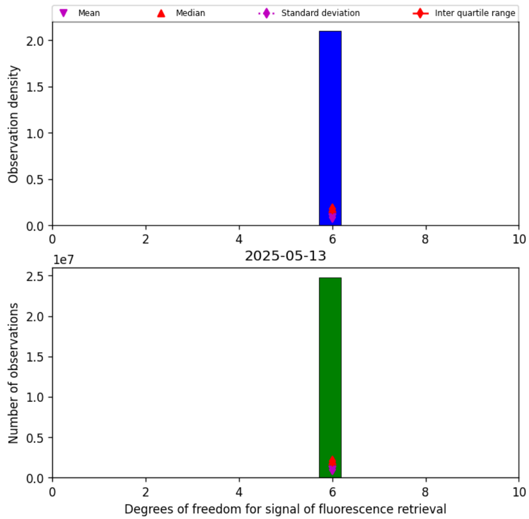
Figure 43: Histogram of "Degrees of freedom for signal of fluorescence retrieval" for 2025-05-12 to 2025-05-14
