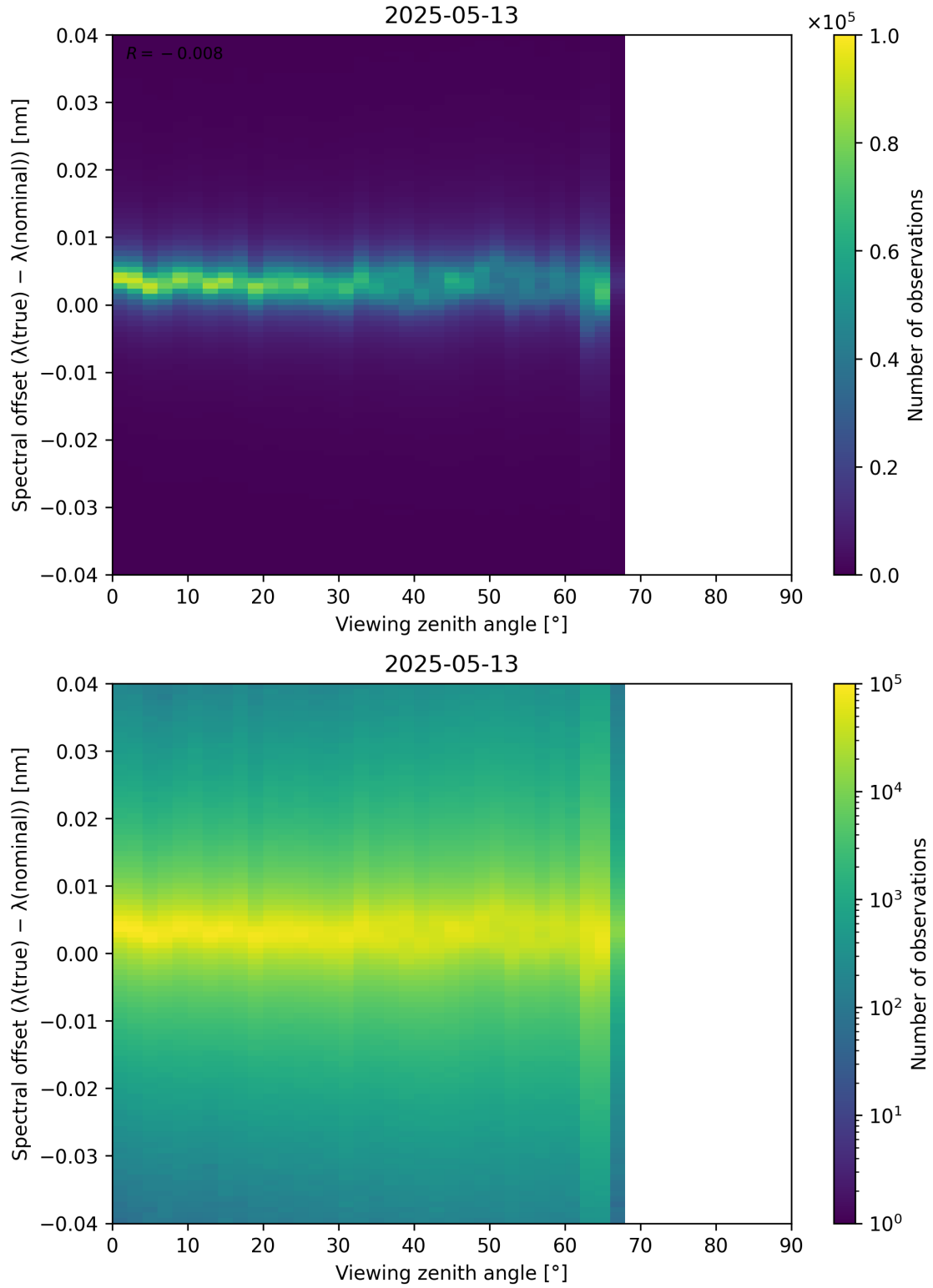
Figure 128: Scatter density plot of “Viewing zenith angle” against “Spectral offset ( \lambda_{\text{true}} - \lambda_{\text{nominal}} )” for 2025-05-12 to 2025-05-14.
