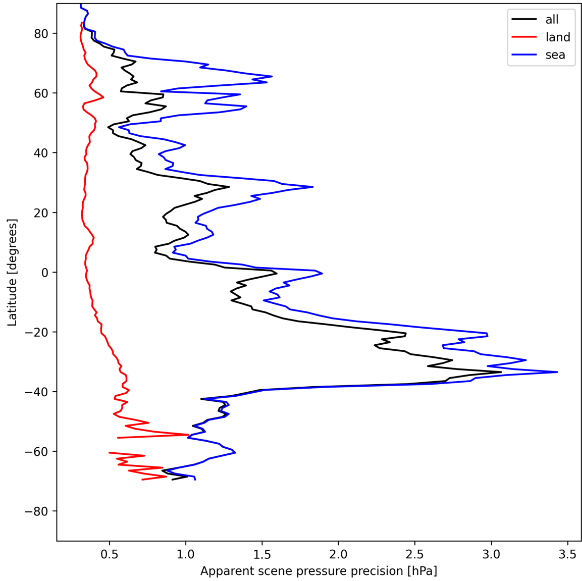
Figure 20: Zonal average of “Apparent scene pressure precision” for 2025-05-12 to 2025-05-14.
