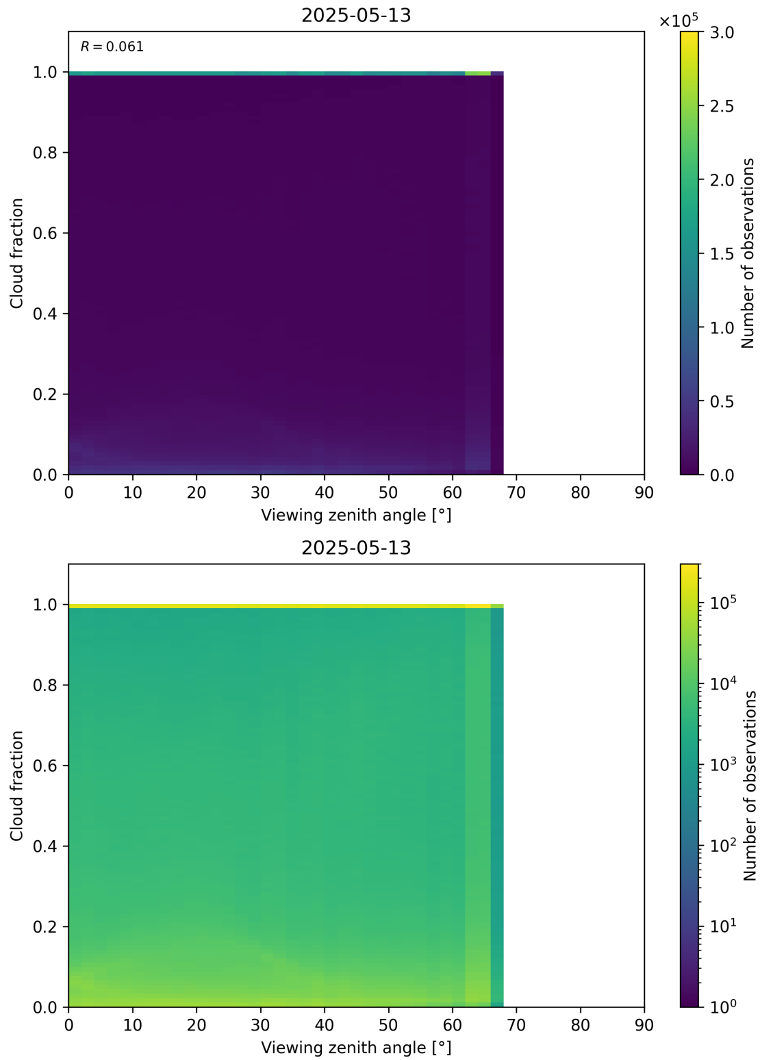
Figure 120: Scatter density plot of “Viewing zenith angle” against “Cloud fraction” for 2025-05-12 to 2025-05-14.
