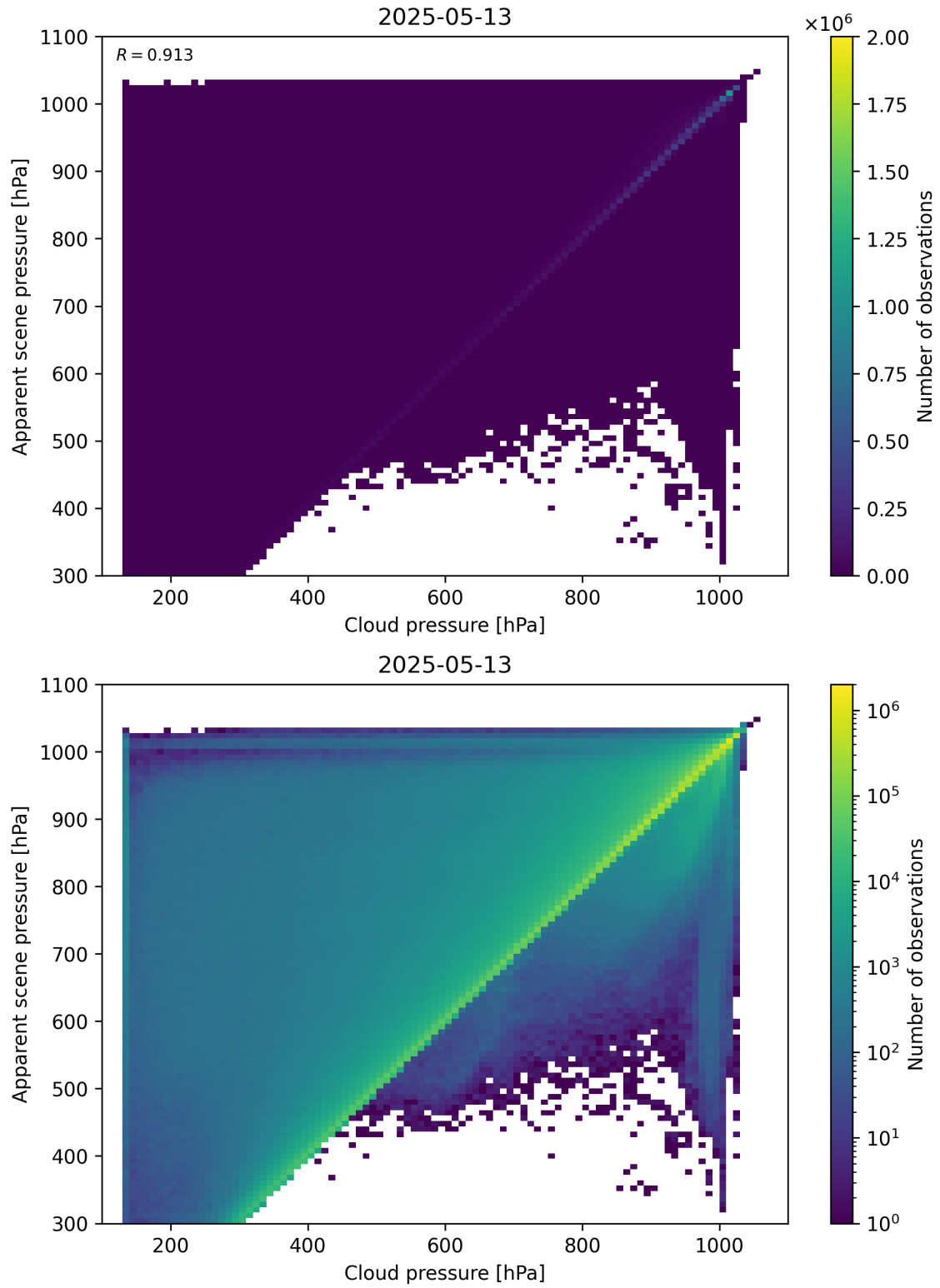
Figure 77: Scatter density plot of “Cloud pressure” against “Apparent scene pressure” for 2025-05-12 to 2025-05-14.
