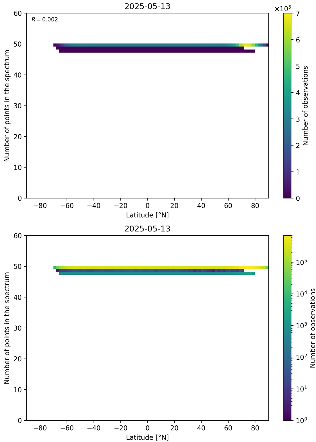
Figure 94: Scatter density plot of “Latitude” against “Number of points in the spectrum” for 2025-05-12 to 2025-05-14.
