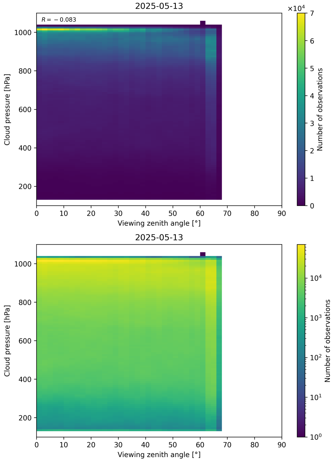
Figure 121: Scatter density plot of “Viewing zenith angle” against “Cloud pressure” for 2025-05-12 to 2025-05-14.
