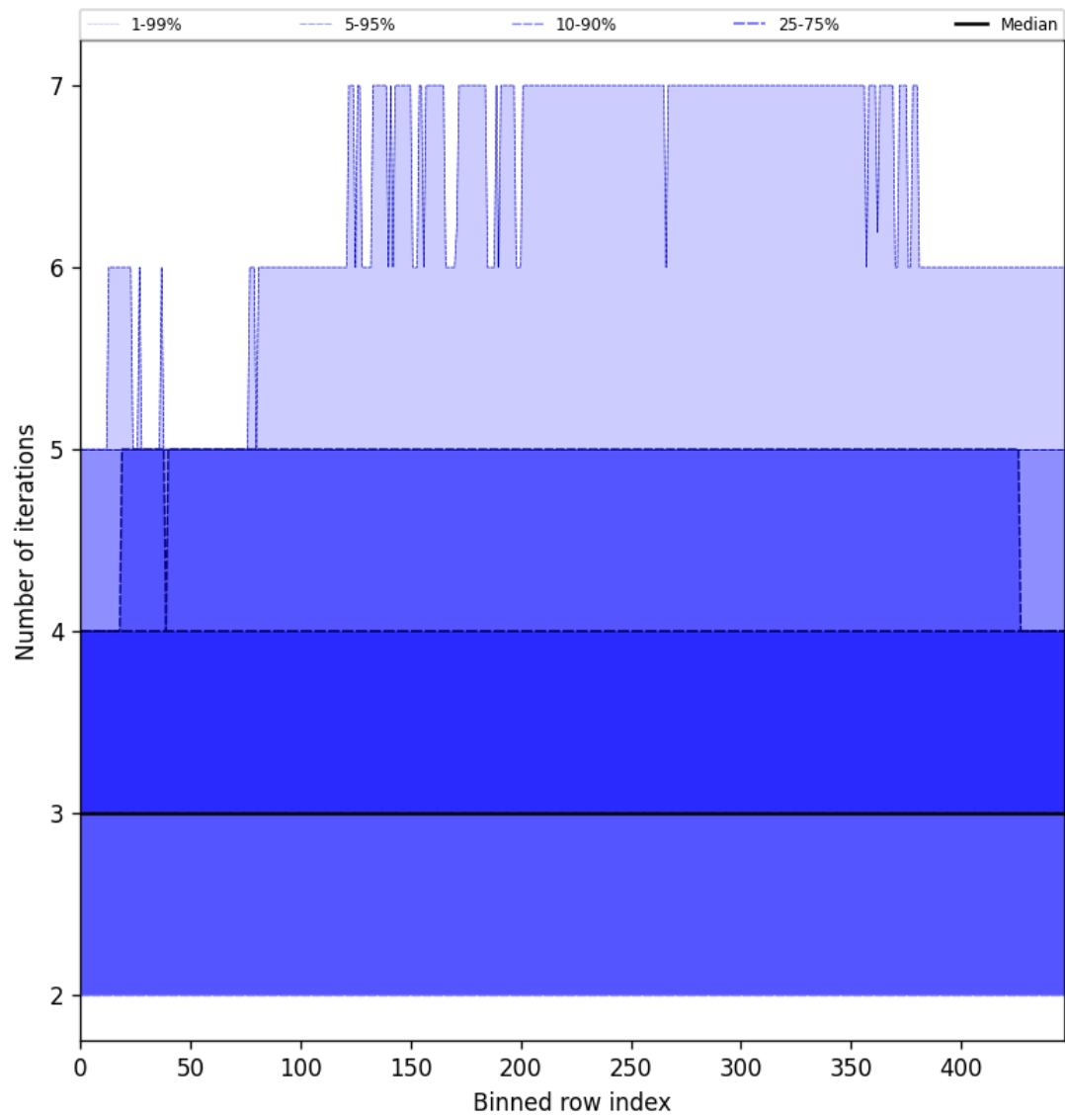
Figure 56: Along track statistics of “Number of iterations” for 2025-05-12 to 2025-05-14
