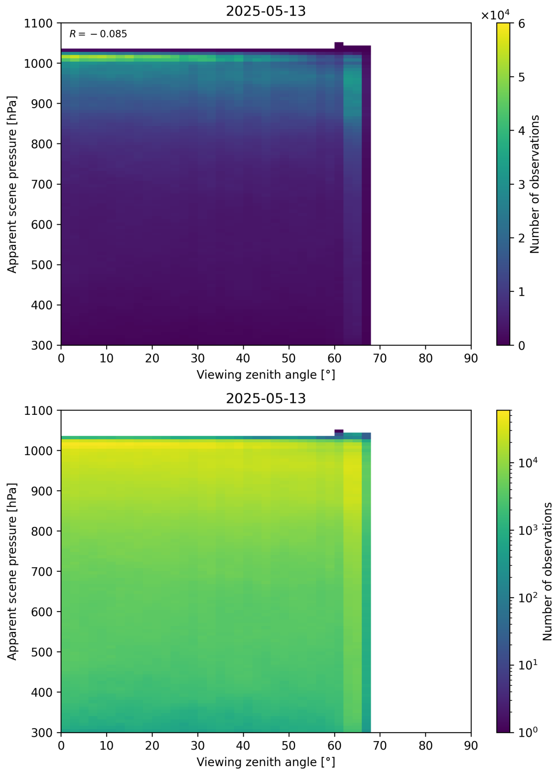
Figure 118: Scatter density plot of “Viewing zenith angle” against “Apparent scene pressure” for 2025-05-12 to 2025-05-14.
