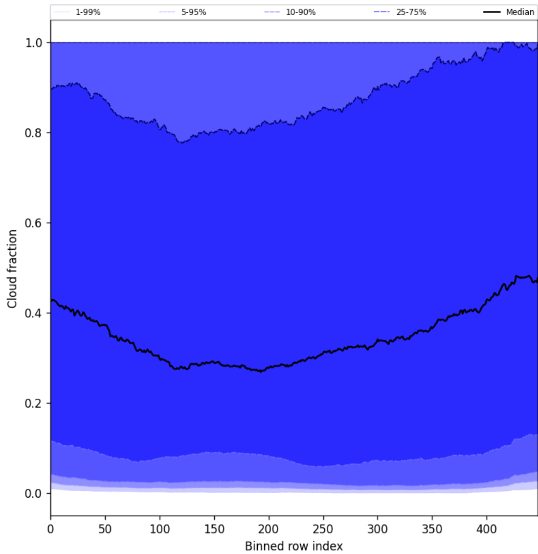
Figure 49: Along track statistics of “Cloud fraction” for 2025-05-12 to 2025-05-14
