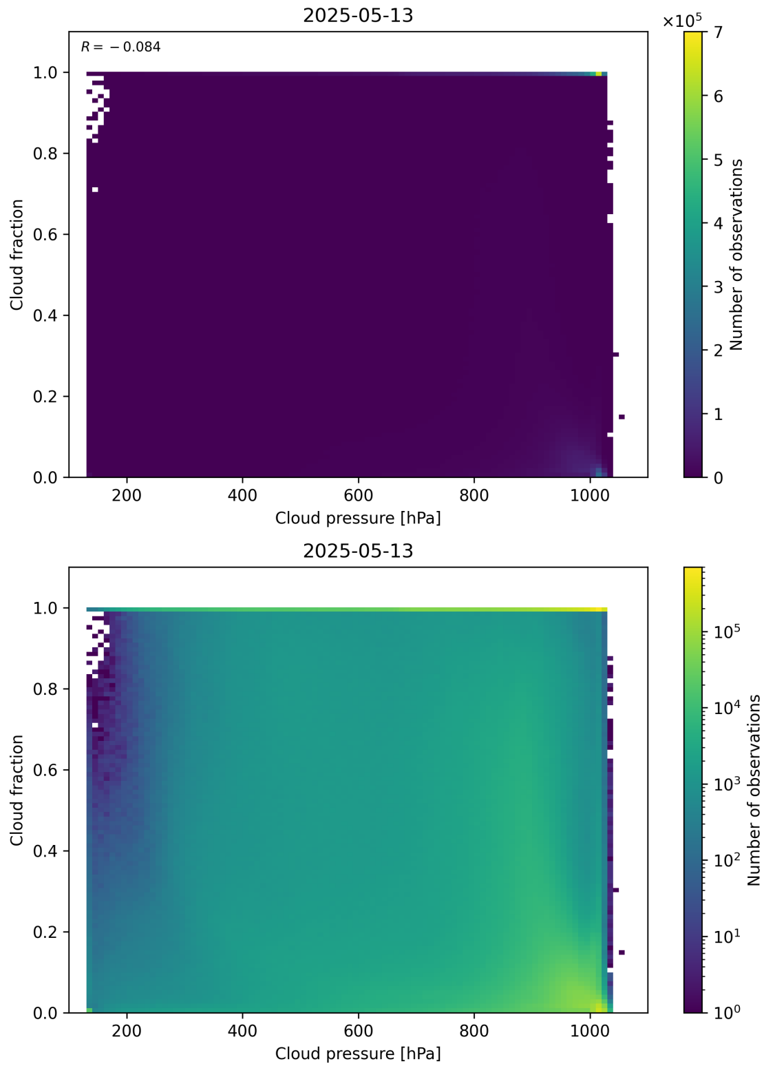
Figure 79: Scatter density plot of “Cloud pressure” against “Cloud fraction” for 2025-05-12 to 2025-05-14.
