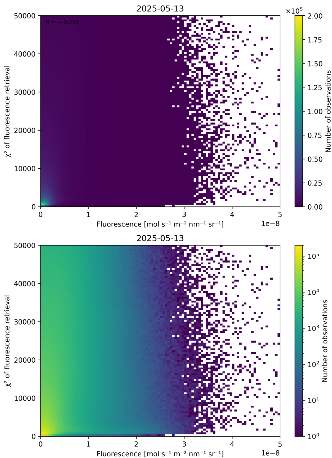
Figure 85: Scatter density plot of “Fluorescence” against “ \chi^2 of fluorescence retrieval” for 2025-05-12 to 2025-05-14.
