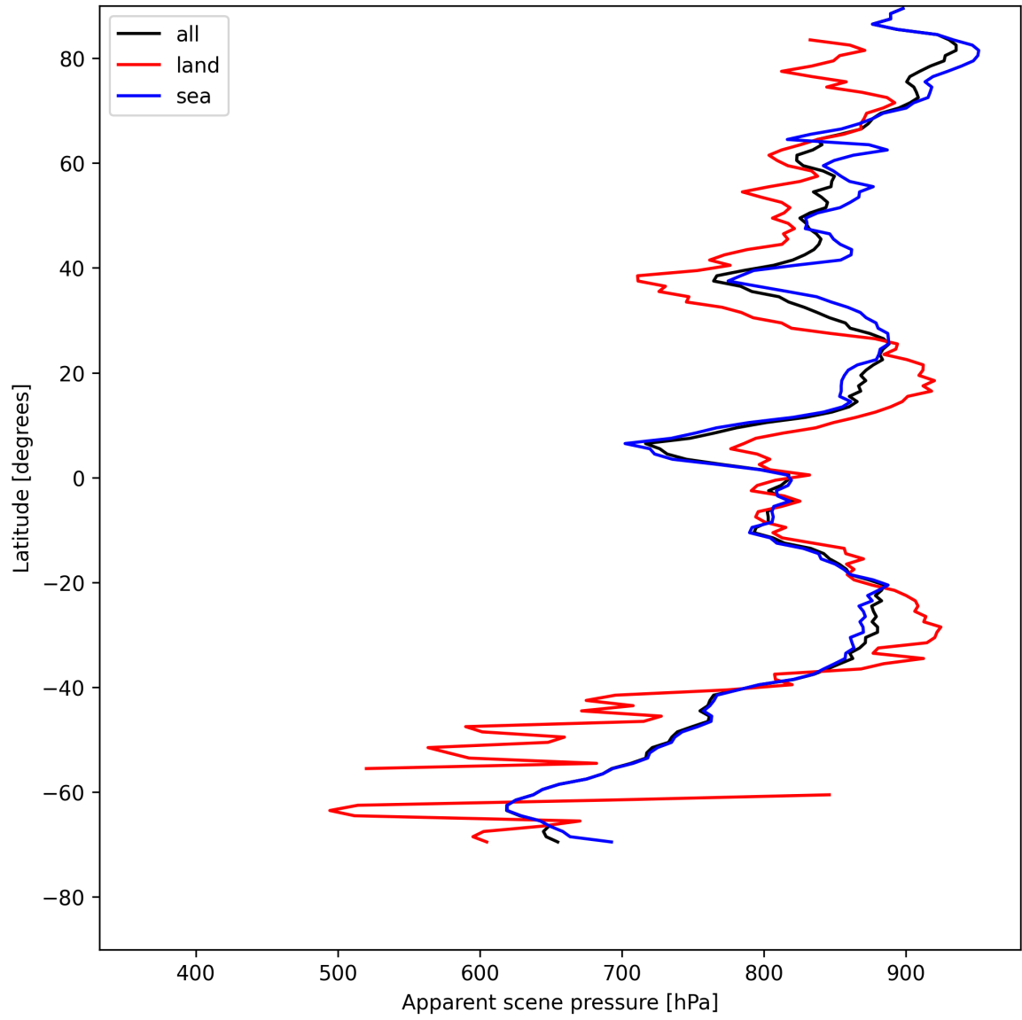
Figure 19: Zonal average of “Apparent scene pressure” for 2025-05-12 to 2025-05-14.
