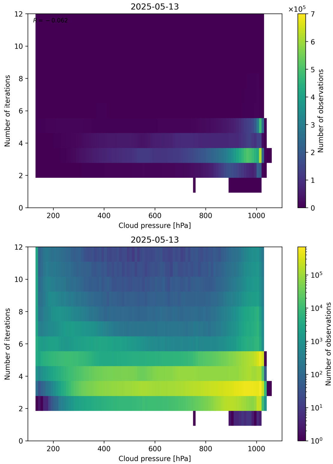
Figure 81: Scatter density plot of “Cloud pressure” against “Number of iterations” for 2025-05-12 to 2025-05-14.
