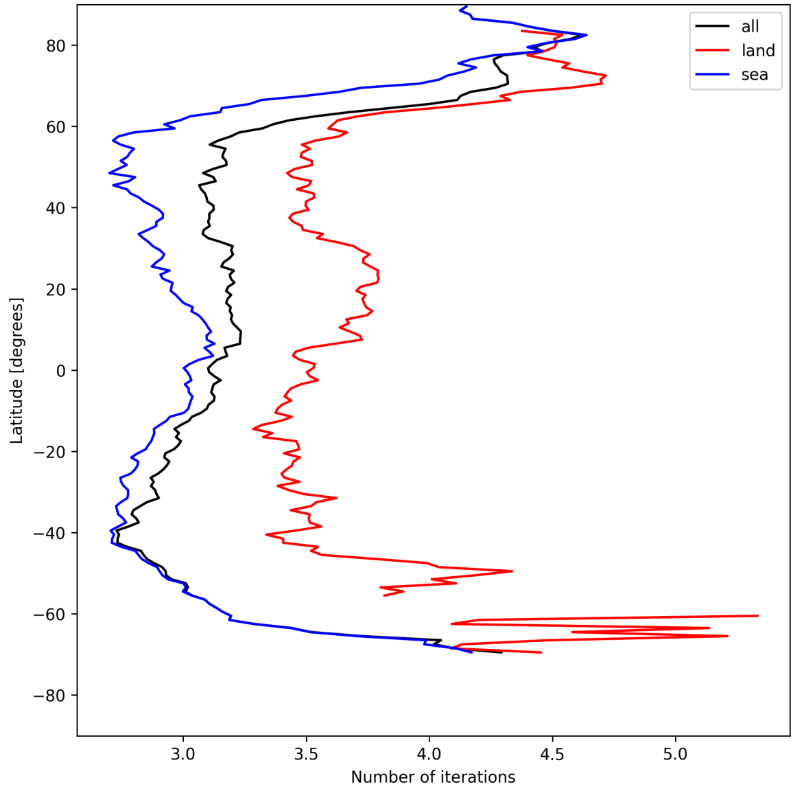
Figure 22: Zonal average of “Number of iterations” for 2025-05-12 to 2025-05-14.
