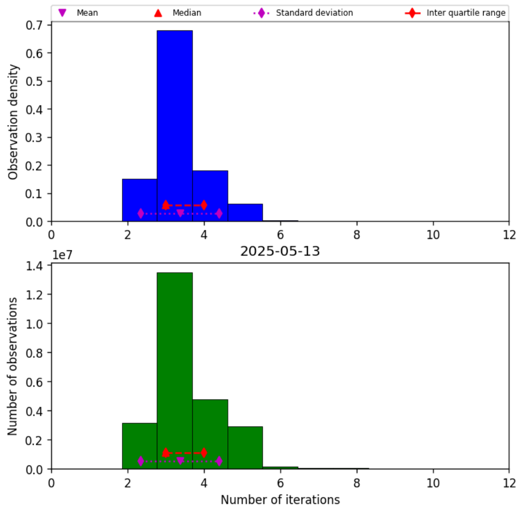
Figure 39: Histogram of “Number of iterations” for 2025-05-12 to 2025-05-14
