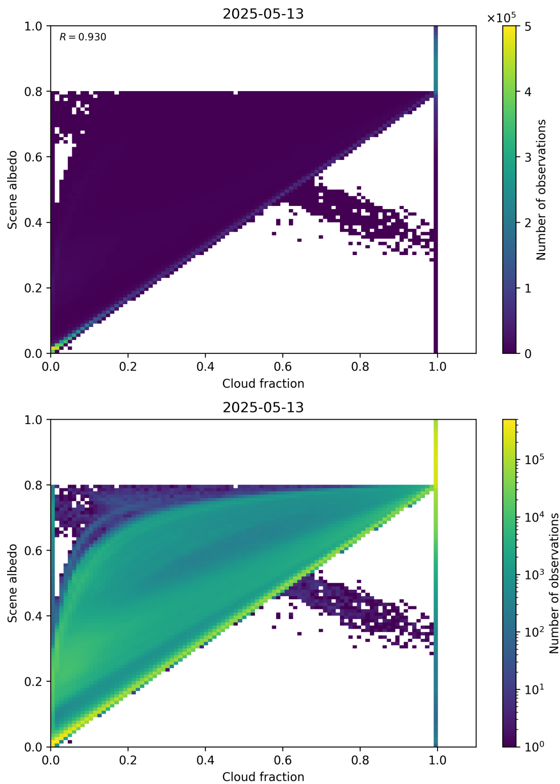
Figure 75: Scatter density plot of “Cloud fraction” against “Scene albedo” for 2025-05-12 to 2025-05-14.
