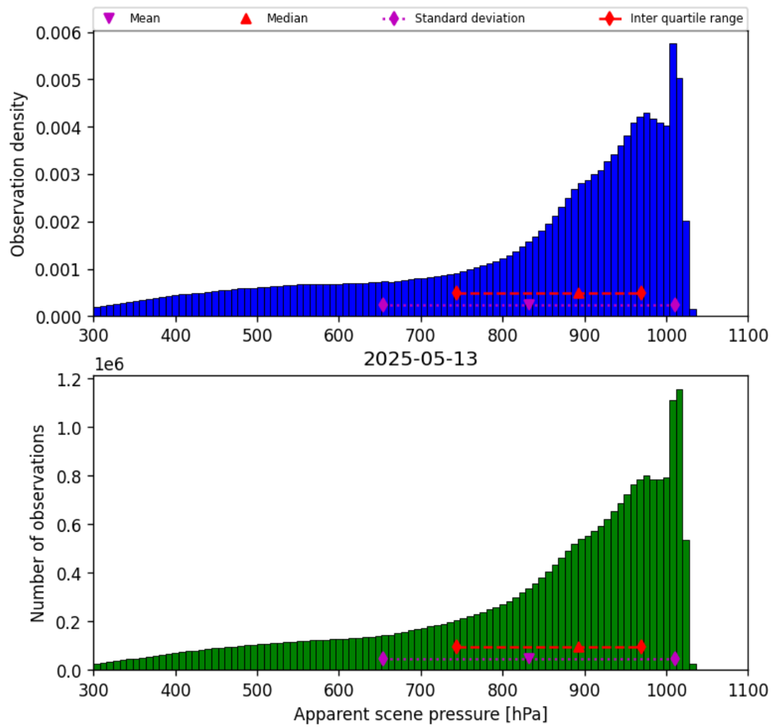
Figure 36: Histogram of “Apparent scene pressure” for 2025-05-12 to 2025-05-14
