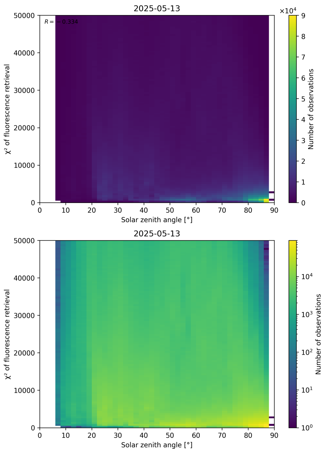
Figure 109: Scatter density plot of “Solar zenith angle” against “ \chi^2 of fluorescence retrieval” for 2025-05-12 to 2025-05-14.
