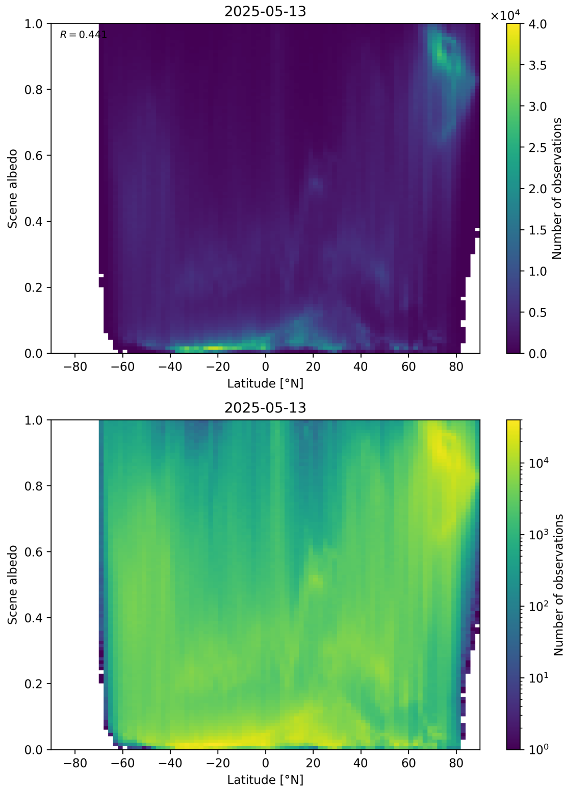
Figure 95: Scatter density plot of “Latitude” against “Scene albedo” for 2025-05-12 to 2025-05-14.
