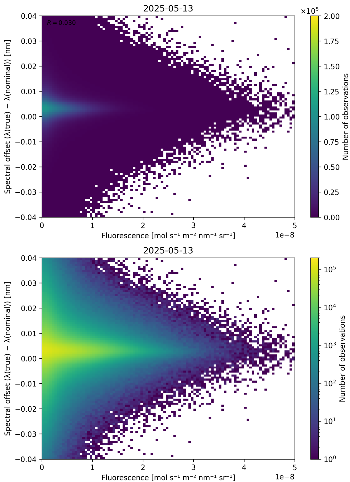
Figure 87: Scatter density plot of “Fluorescence” against “Spectral offset ( \lambda_{\text{true}} - \lambda_{\text{nominal}} )” for 2025-05-12 to 2025-05-14.
