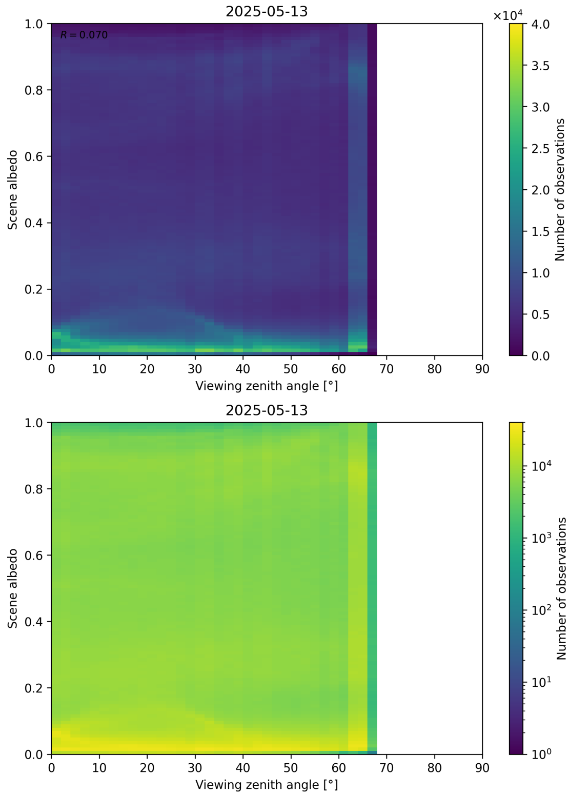
Figure 126: Scatter density plot of “Viewing zenith angle” against “Scene albedo” for 2025-05-12 to 2025-05-14.
