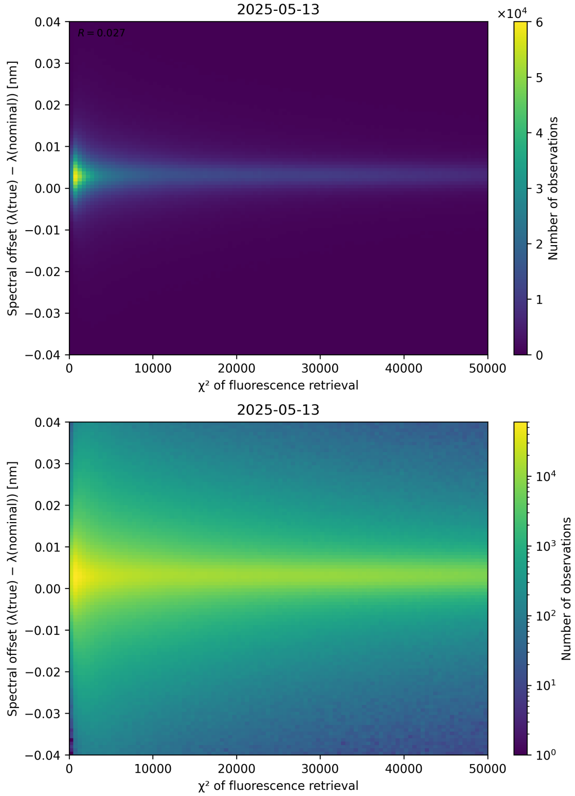
Figure 69: Scatter density plot of “ \chi^2 of fluorescence retrieval” against “Spectral offset ( \lambda_{\text{true}} - \lambda_{\text{nominal}} )” for 2025-05-12 to 2025-05-14.
