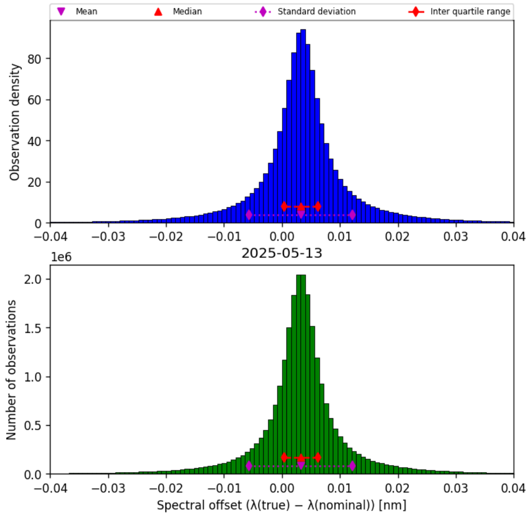
Figure 45: Histogram of “Spectral offset ( \lambda_{\text{true}} - \lambda_{\text{nominal}} )” for 2025-05-12 to 2025-05-14
