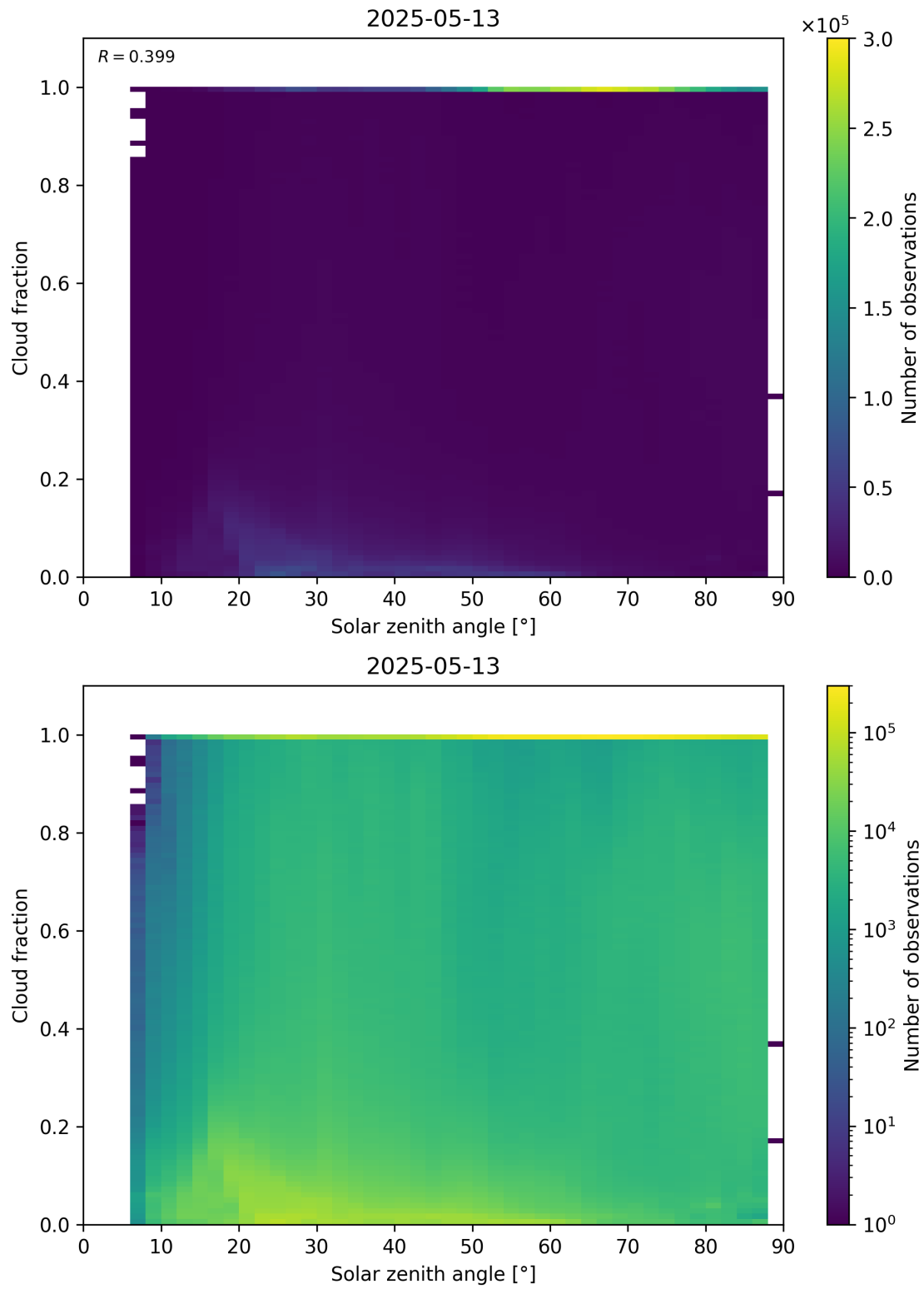
Figure 110: Scatter density plot of “Solar zenith angle” against “Cloud fraction” for 2025-05-12 to 2025-05-14.
