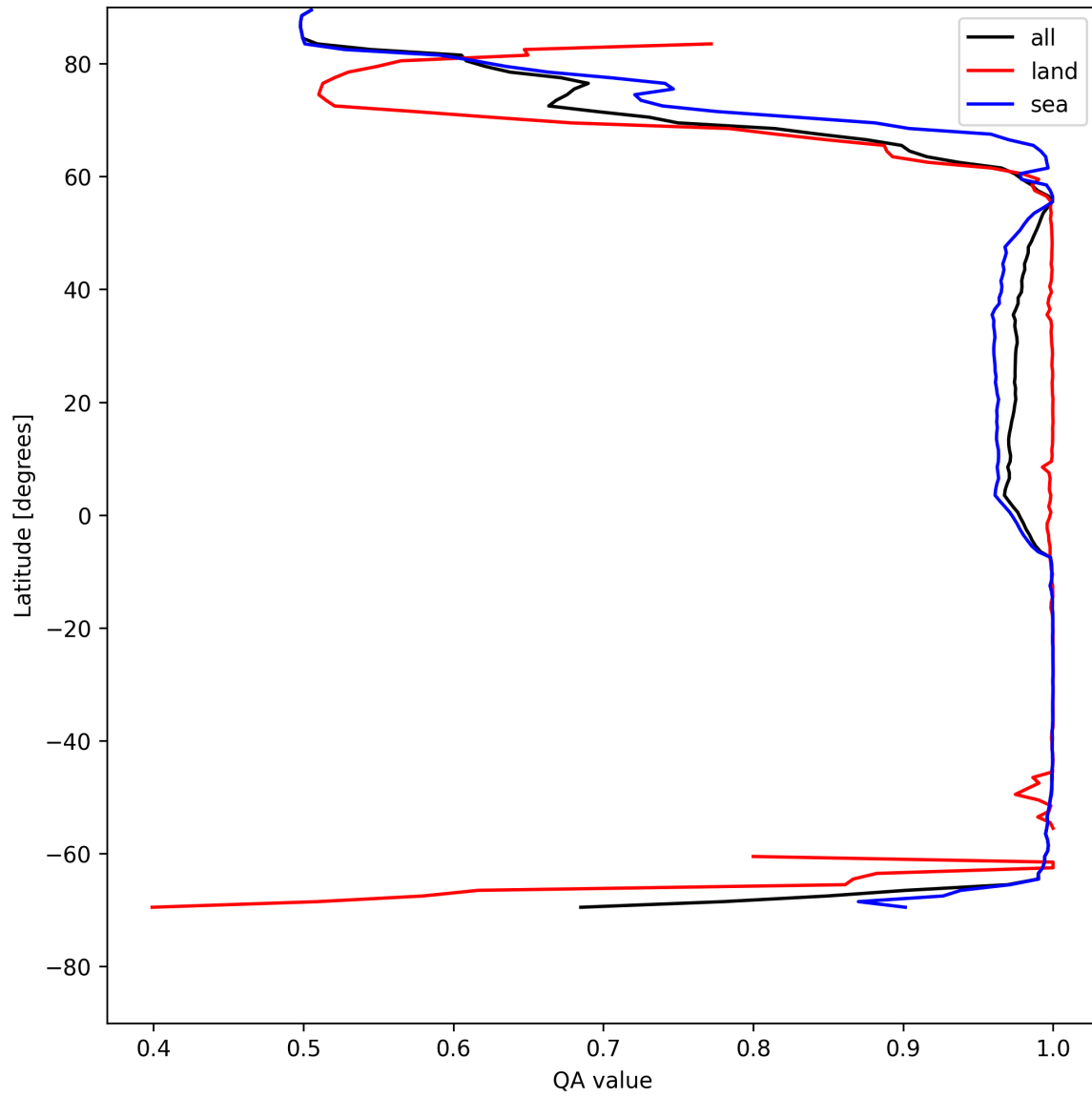
Figure 12: Zonal average of “QA value” for 2025-05-12 to 2025-05-14.
