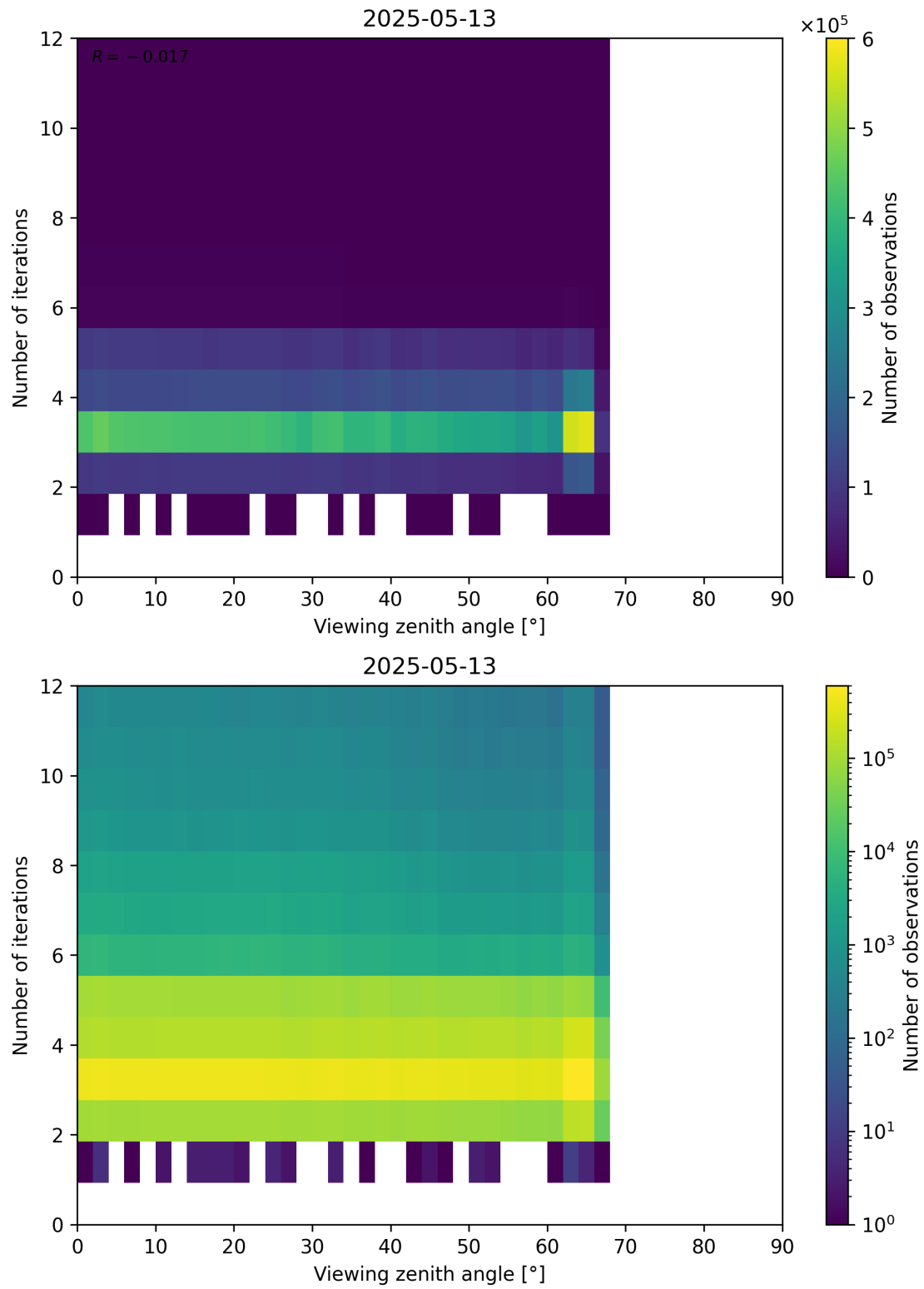
Figure 124: Scatter density plot of “Viewing zenith angle” against “Number of iterations” for 2025-05-12 to 2025-05-14.
