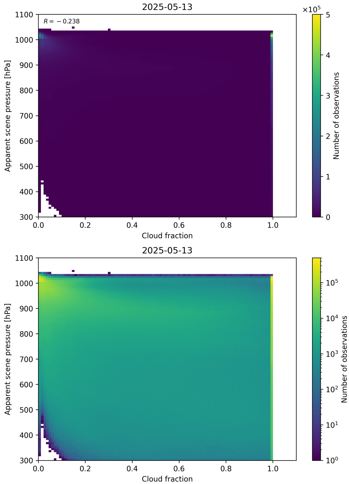
Figure 70: Scatter density plot of “Cloud fraction” against “Apparent scene pressure” for 2025-05-12 to 2025-05-14.
