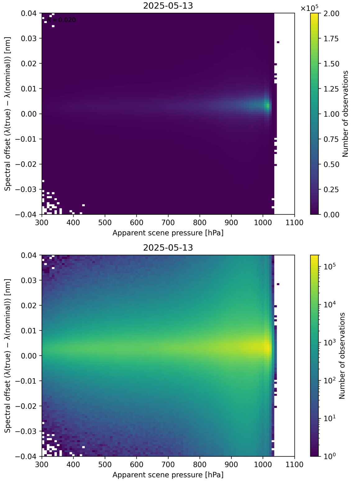
Figure 67: Scatter density plot of “Apparent scene pressure” against “Spectral offset ( \lambda_{\text{true}} - \lambda_{\text{nominal}} )” for 2025-05-12 to 2025-05-14.
