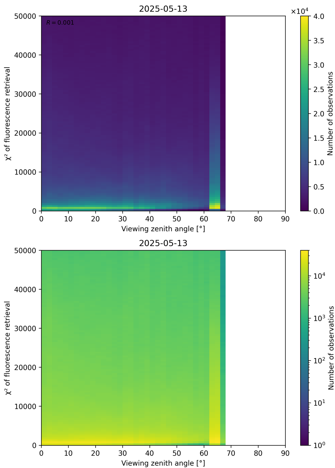
Figure 119: Scatter density plot of “Viewing zenith angle” against “ \chi^2 of fluorescence retrieval” for 2025-05-12 to 2025-05-14.
