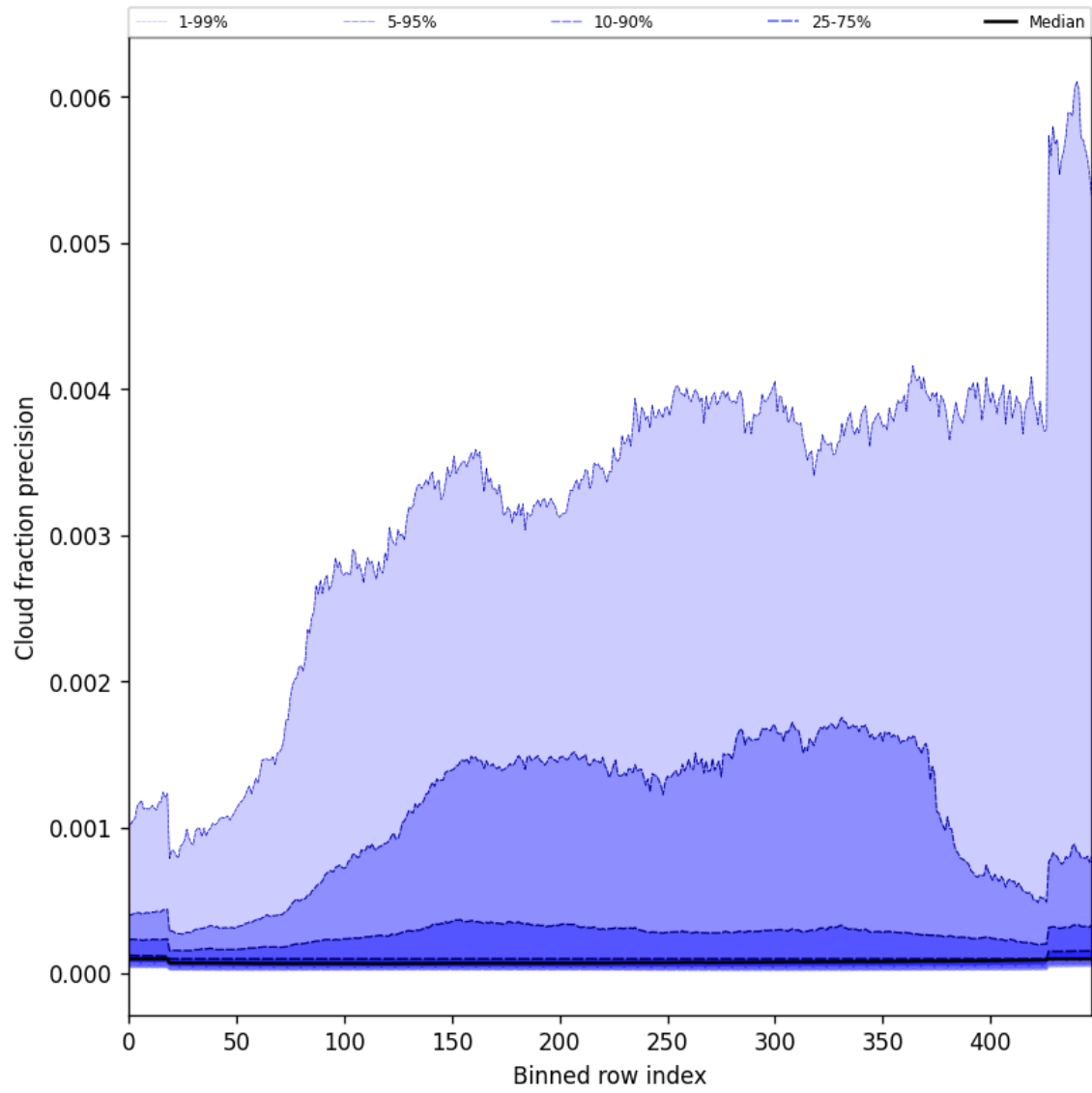
Figure 50: Along track statistics of “Cloud fraction precision” for 2025-05-12 to 2025-05-14
