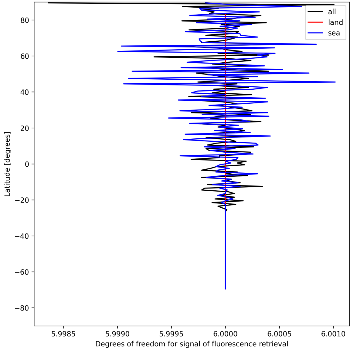
Figure 26: Zonal average of “Degrees of freedom for signal of fluorescence retrieval” for 2025-05-12 to 2025-05-14.
