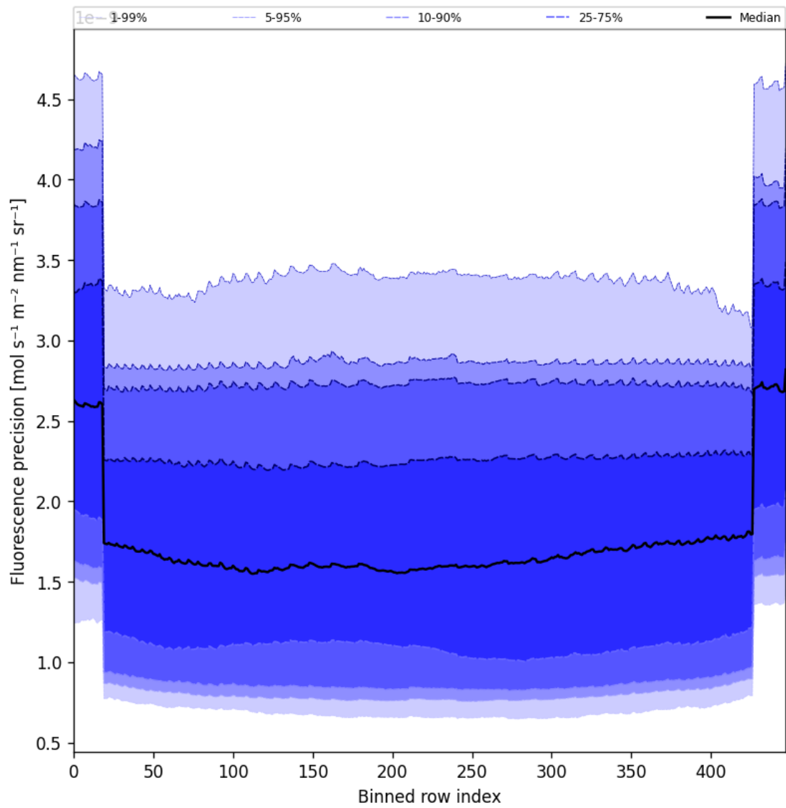
Figure 58: Along track statistics of “Fluorescence precision” for 2025-05-12 to 2025-05-14
