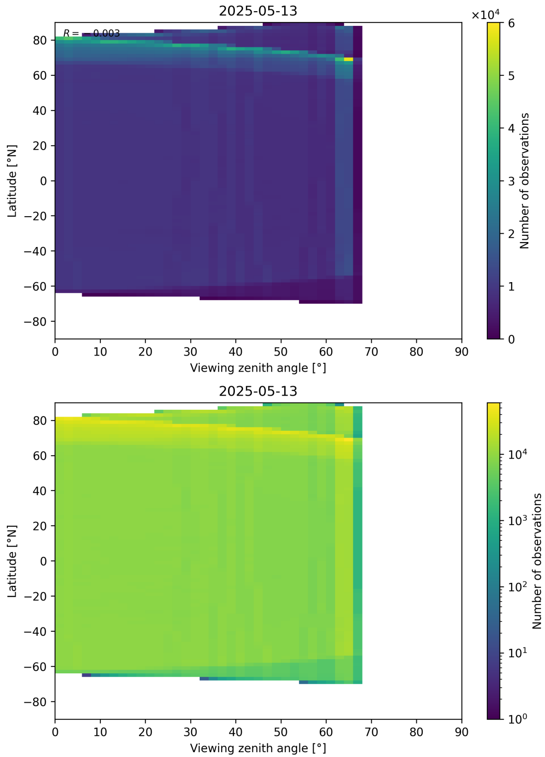
Figure 123: Scatter density plot of “Viewing zenith angle” against “Latitude” for 2025-05-12 to 2025-05-14.
