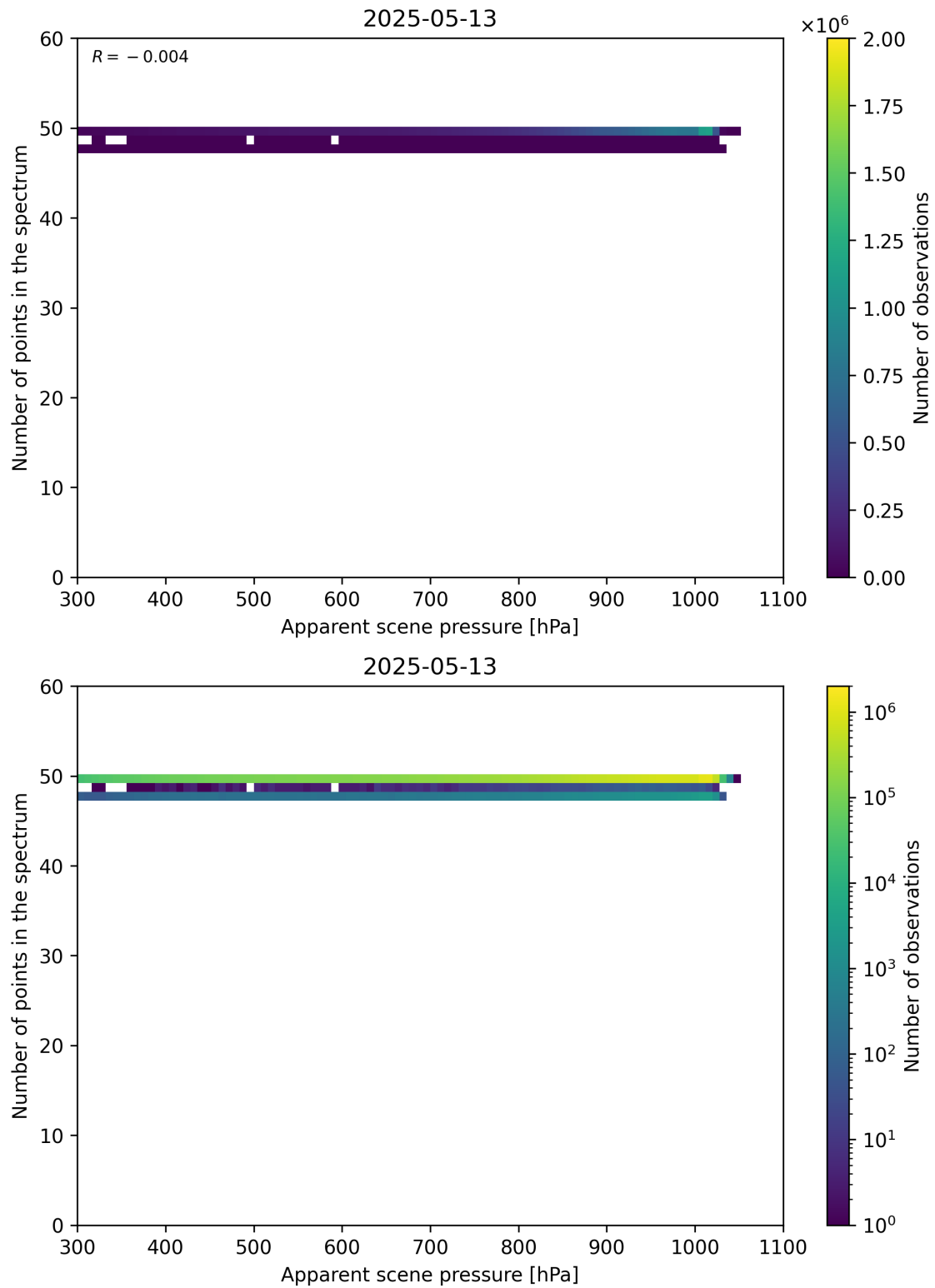
Figure 66: Scatter density plot of “Apparent scene pressure” against “Number of points in the spectrum” for 2025-05-12 to 2025-05-14.
