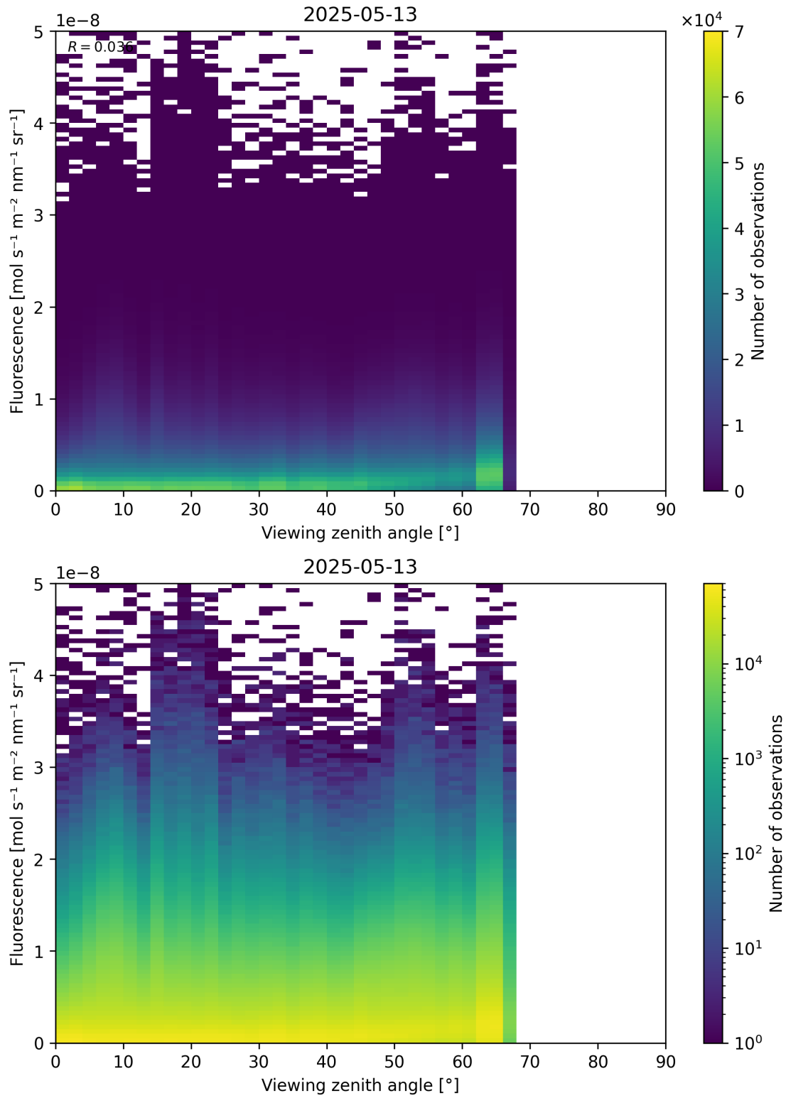
Figure 122: Scatter density plot of “Viewing zenith angle” against “Fluorescence” for 2025-05-12 to 2025-05-14.
