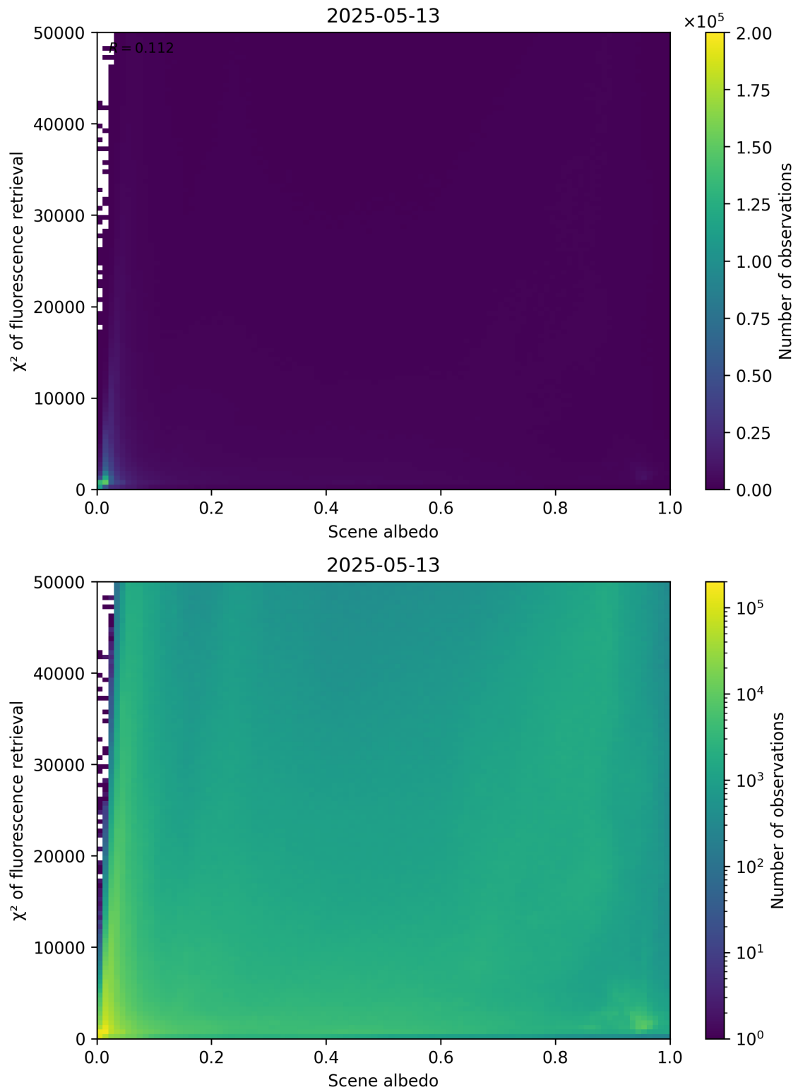
Figure 103: Scatter density plot of “Scene albedo” against “ \chi^2 of fluorescence retrieval” for 2025-05-12 to 2025-05-14.
