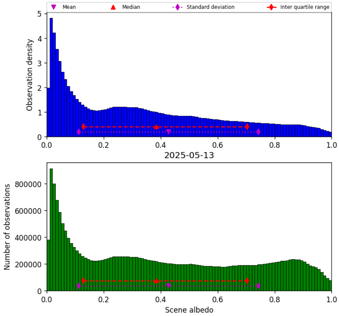
Figure 34: Histogram of “Scene albedo” for 2025-05-12 to 2025-05-14
