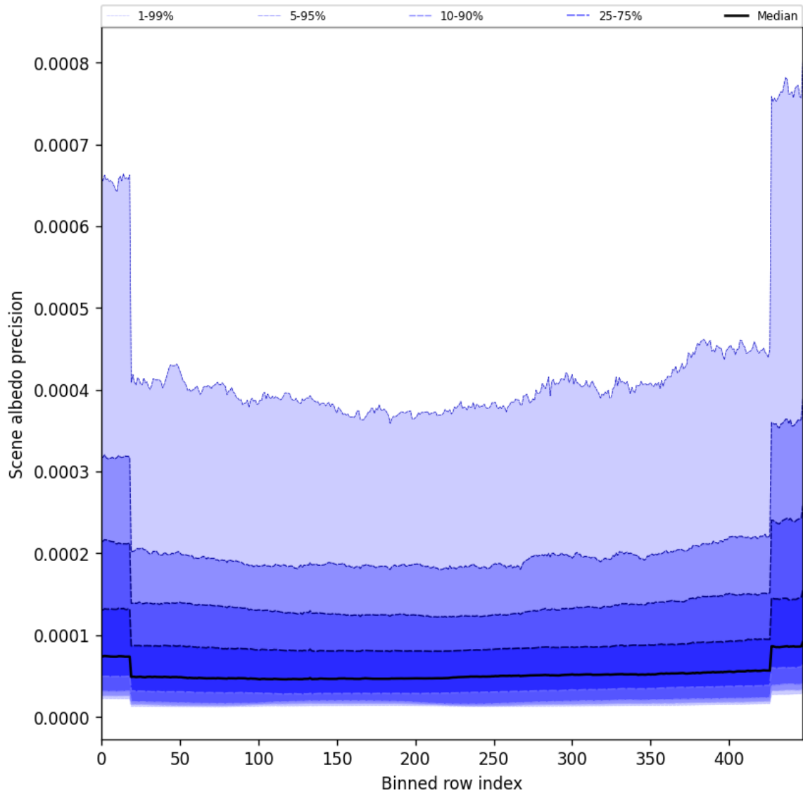
Figure 52: Along track statistics of “Scene albedo precision” for 2025-05-12 to 2025-05-14
