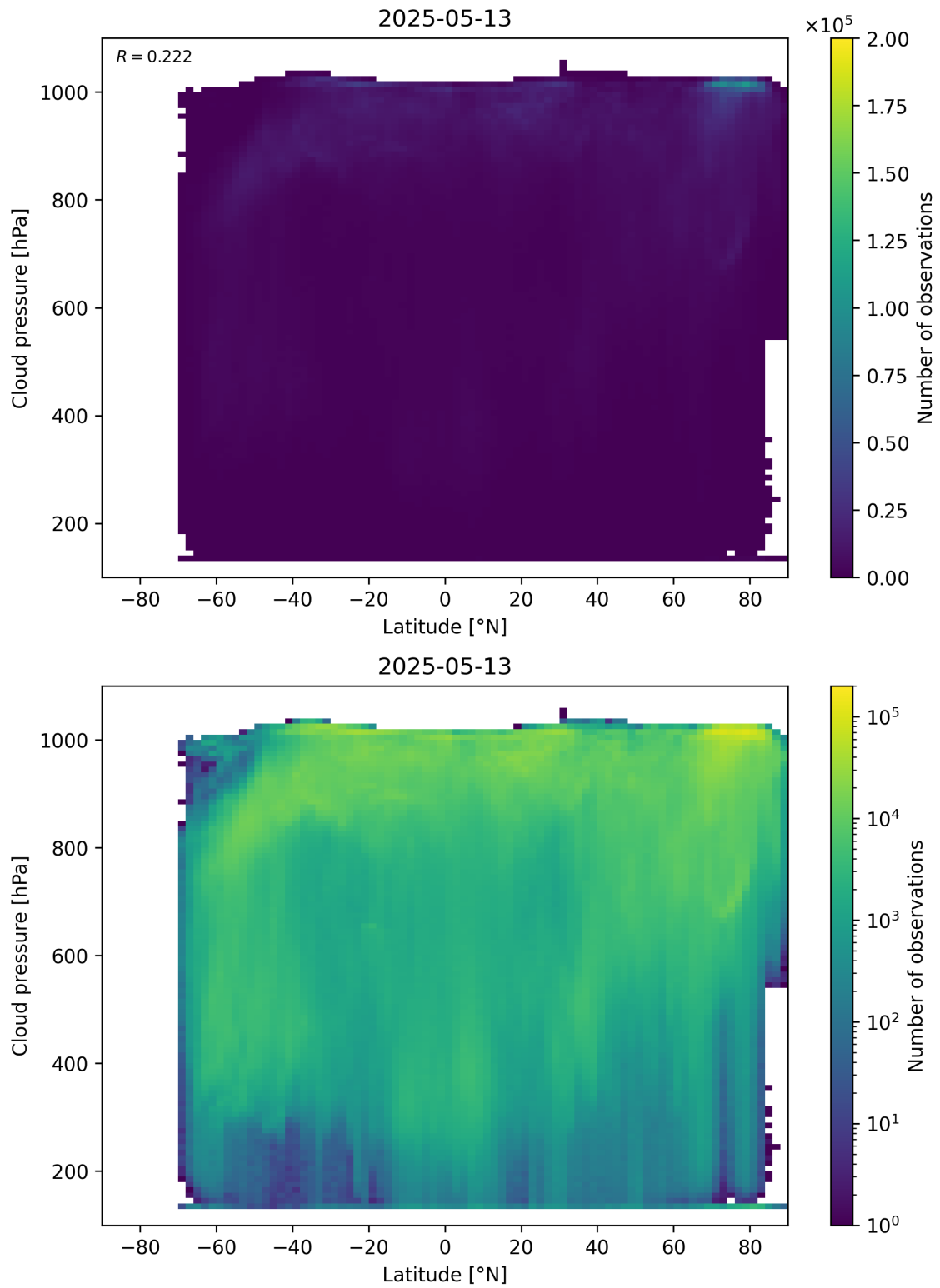
Figure 91: Scatter density plot of “Latitude” against “Cloud pressure” for 2025-05-12 to 2025-05-14.
