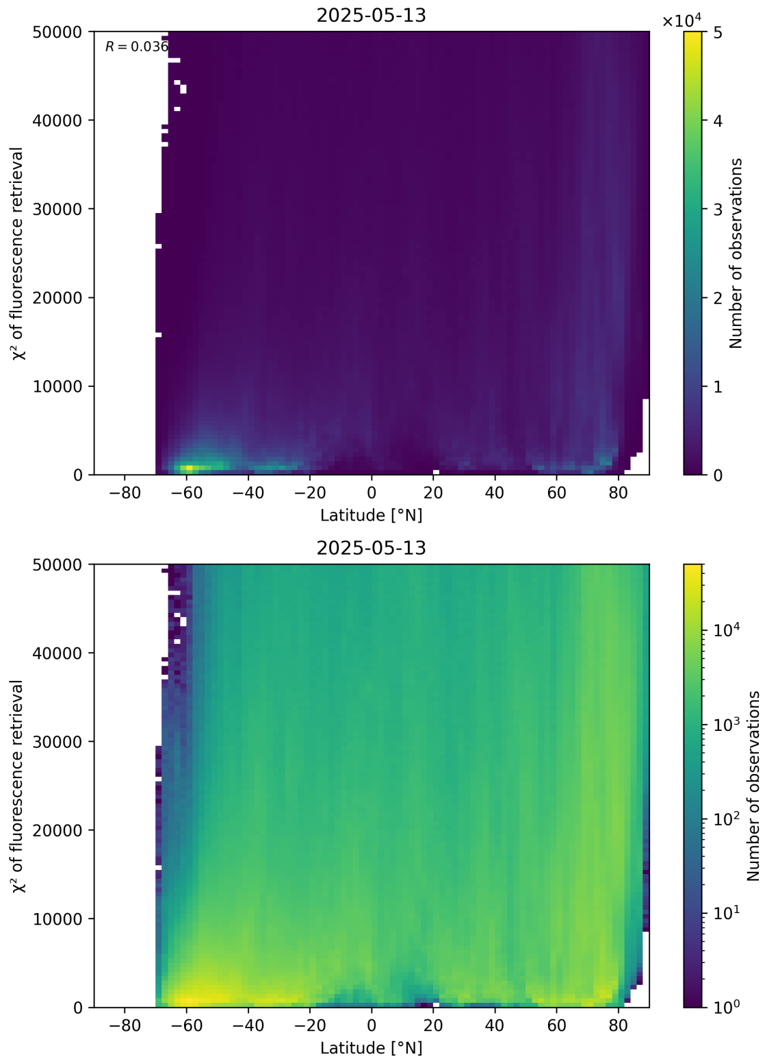
Figure 89: Scatter density plot of “Latitude” against “ \chi^2 of fluorescence retrieval” for 2025-05-12 to 2025-05-14.
