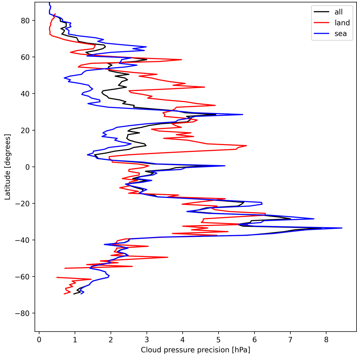
Figure 14: Zonal average of “Cloud pressure precision” for 2025-05-12 to 2025-05-14.
