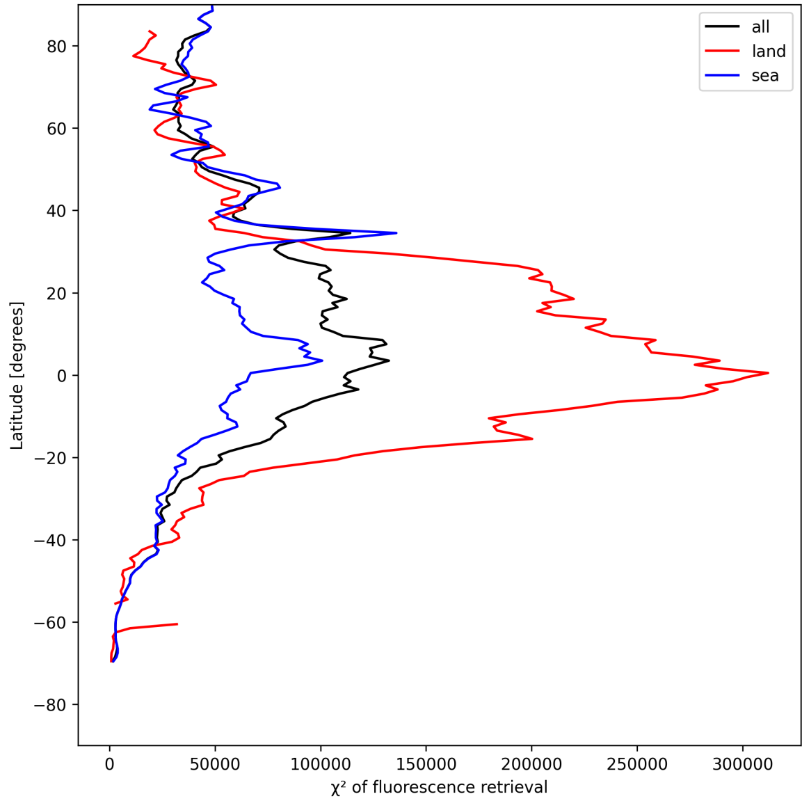
Figure 25: Zonal average of “ \chi^2 of fluorescence retrieval” for 2025-05-12 to 2025-05-14.
