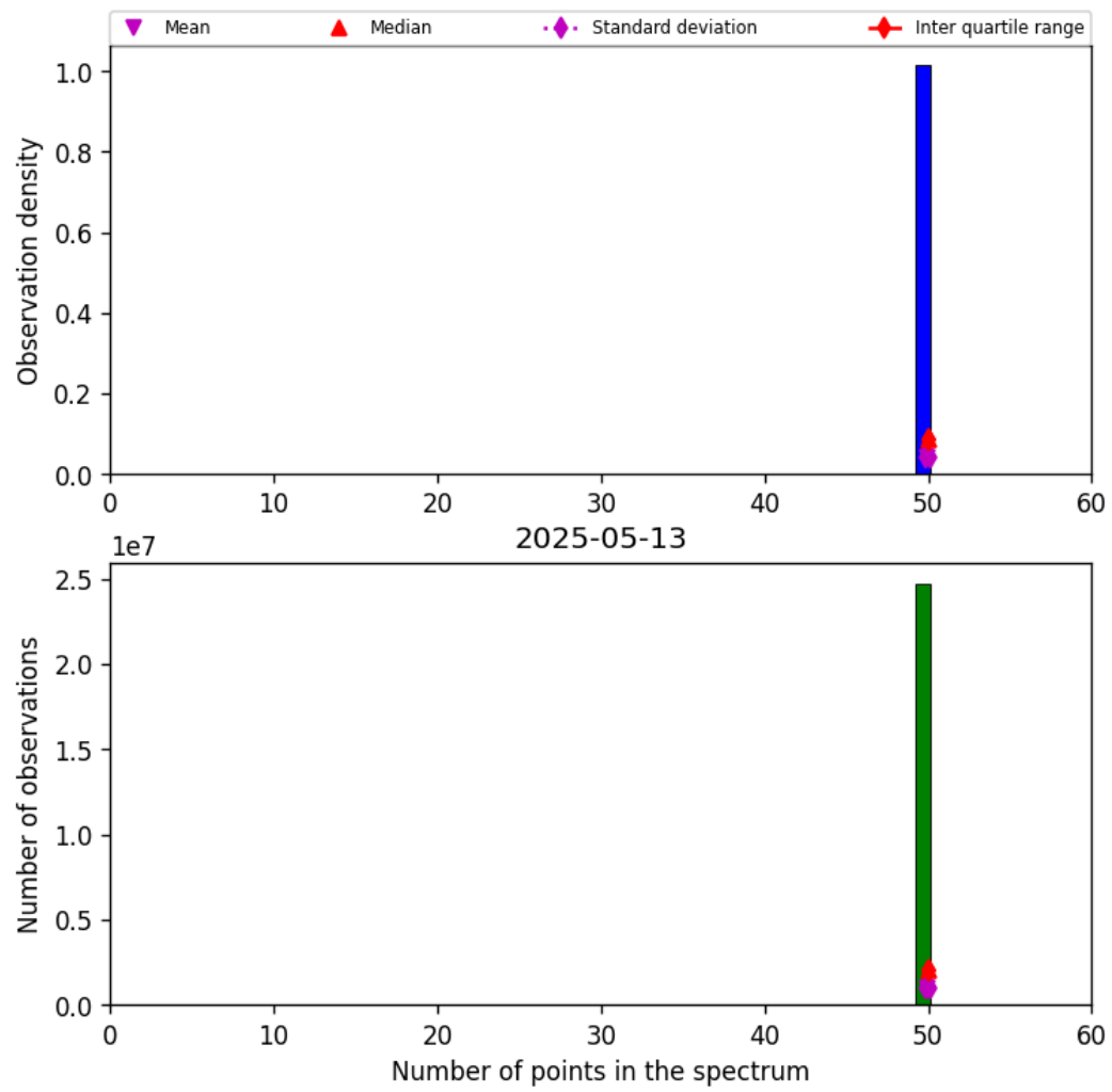
Figure 44: Histogram of "Number of points in the spectrum" for 2025-05-12 to 2025-05-14
