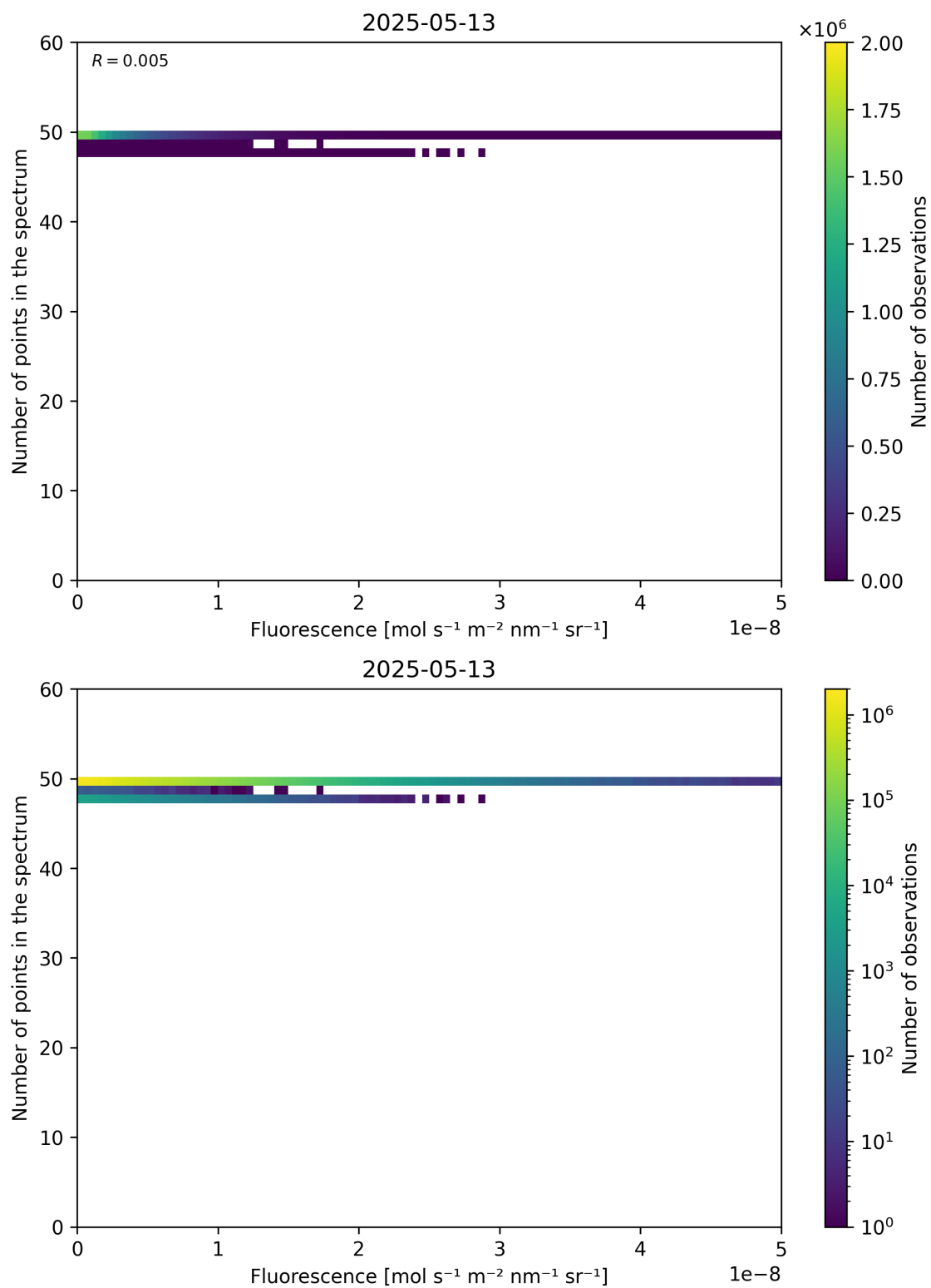
Figure 86: Scatter density plot of “Fluorescence” against “Number of points in the spectrum” for 2025-05-12 to 2025-05-14.
