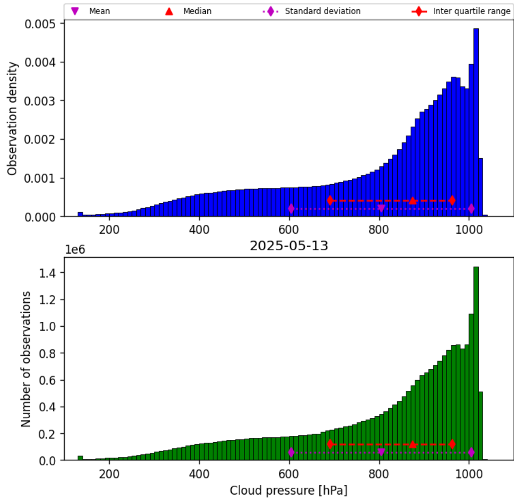
Figure 30: Histogram of “Cloud pressure” for 2025-05-12 to 2025-05-14
