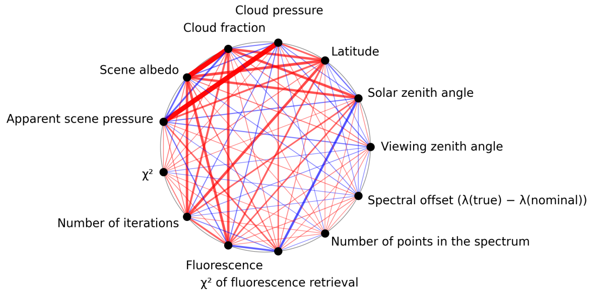
Figure 1: Map of correlation graph for 2025-05-12 to 2025-05-14.
