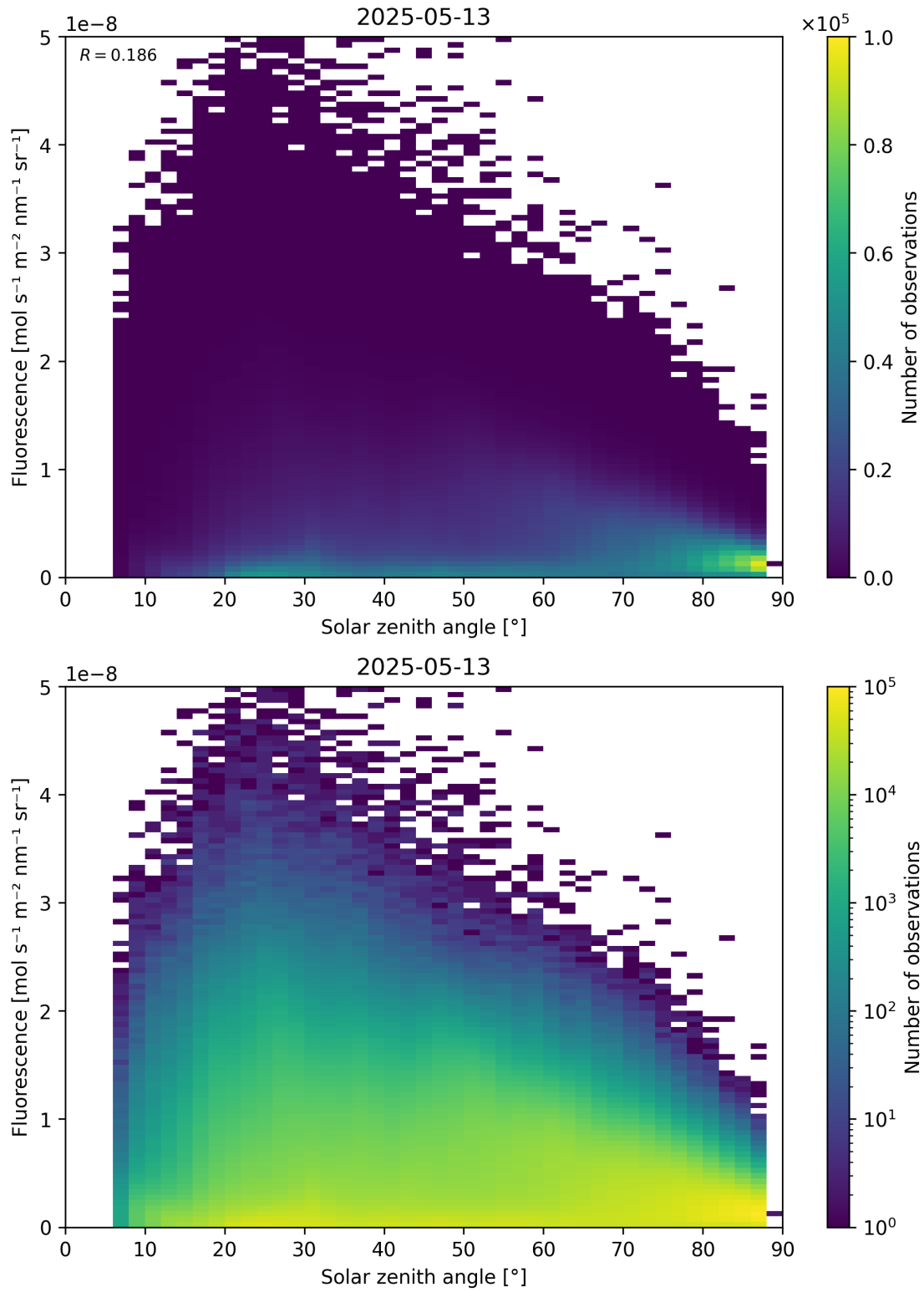
Figure 112: Scatter density plot of “Solar zenith angle” against “Fluorescence” for 2025-05-12 to 2025-05-14.
