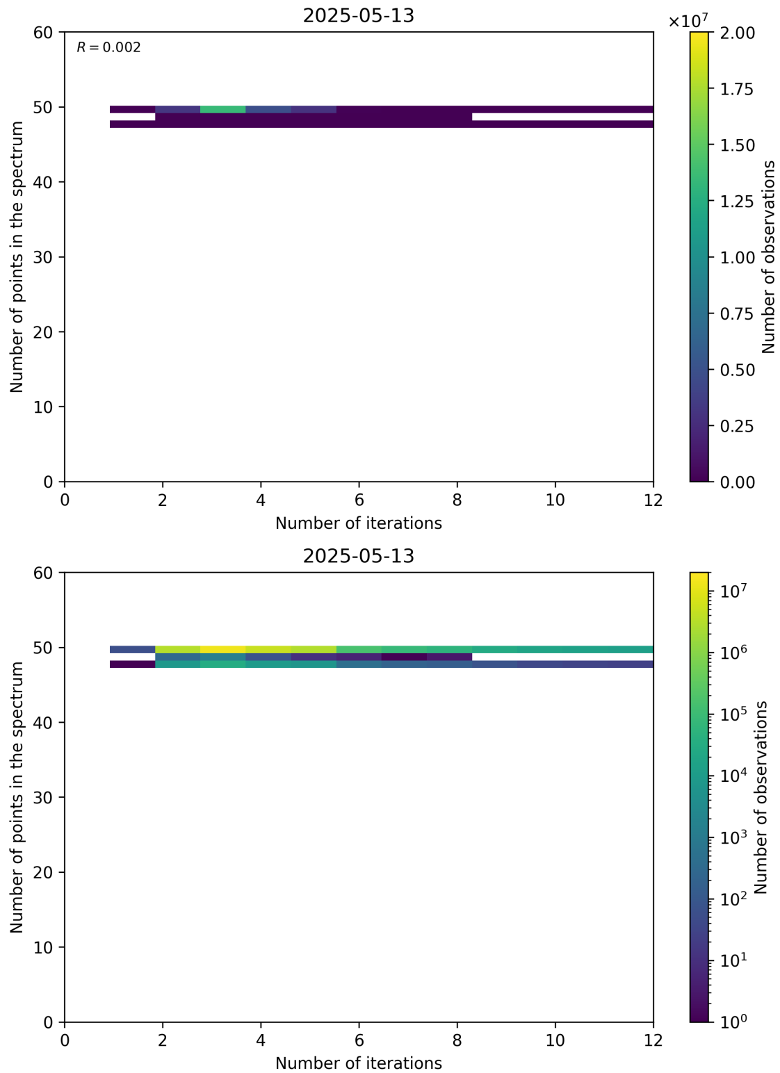
Figure 99: Scatter density plot of “Number of iterations” against “Number of points in the spectrum” for 2025-05-12 to 2025-05-14.
