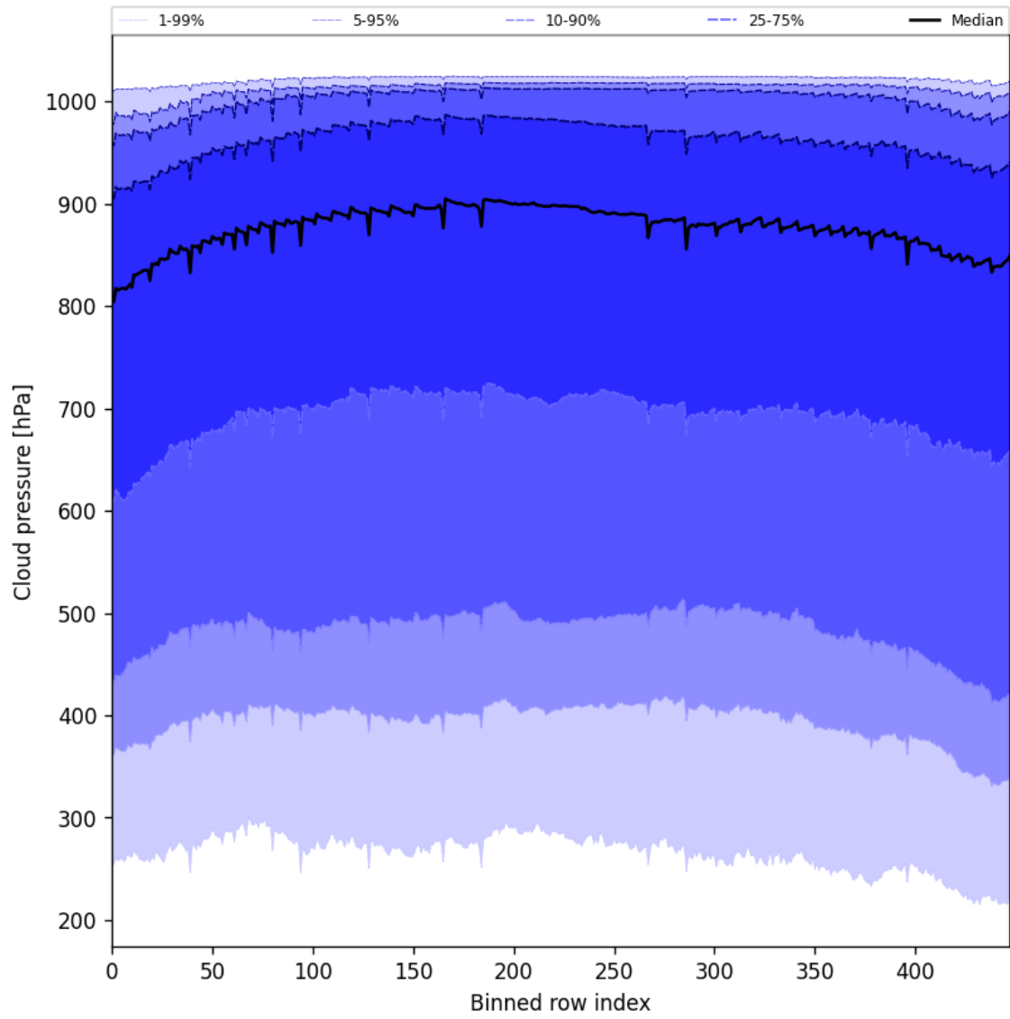
Figure 47: Along track statistics of “Cloud pressure” for 2025-05-12 to 2025-05-14
