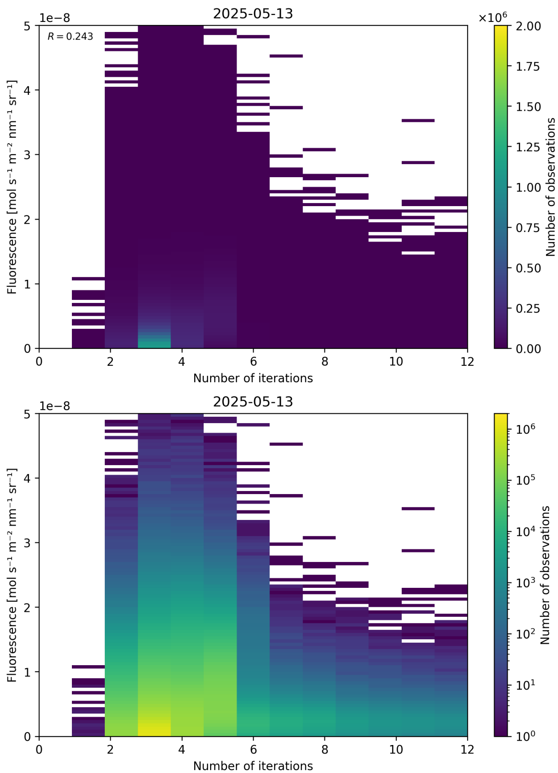
Figure 98: Scatter density plot of “Number of iterations” against “Fluorescence” for 2025-05-12 to 2025-05-14.
