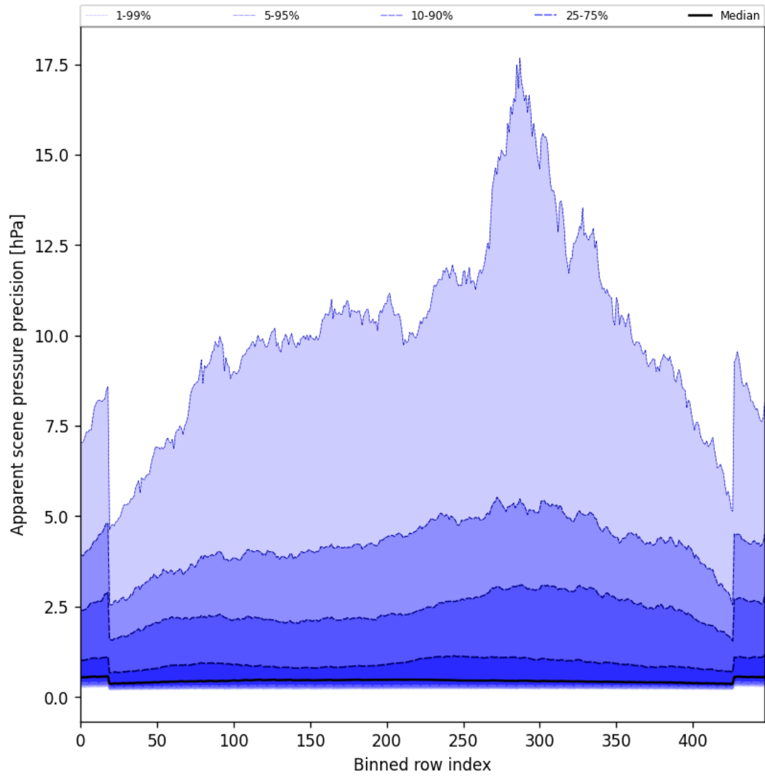
Figure 54: Along track statistics of “Apparent scene pressure precision” for 2025-05-12 to 2025-05-14
