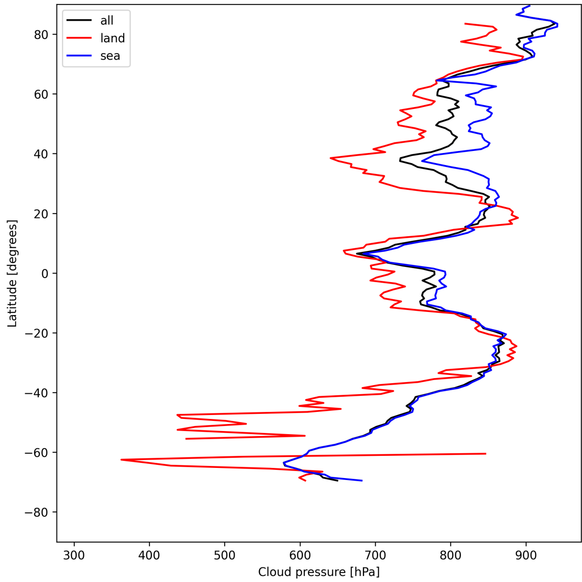
Figure 13: Zonal average of “Cloud pressure” for 2025-05-12 to 2025-05-14.
