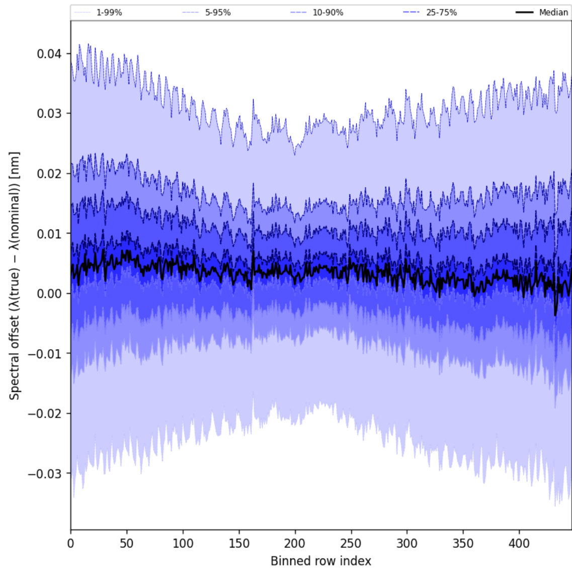
Figure 62: Along track statistics of “Spectral offset ( \lambda_{\text{true}} - \lambda_{\text{nominal}} )” for 2025-05-12 to 2025-05-14
