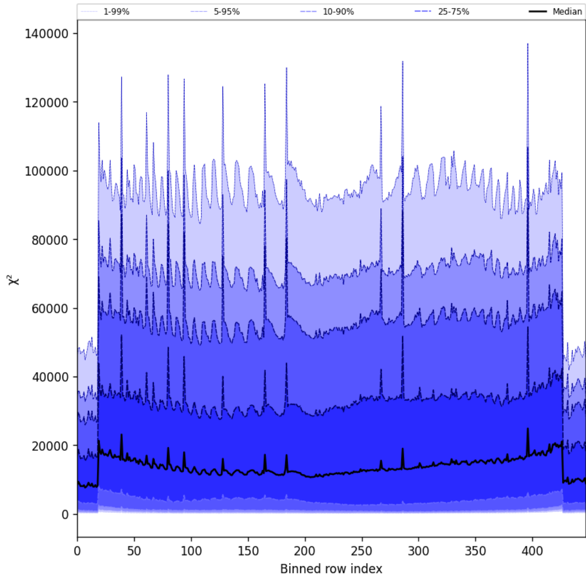
Figure 55: Along track statistics of “ \chi^2 ” for 2025-05-12 to 2025-05-14
