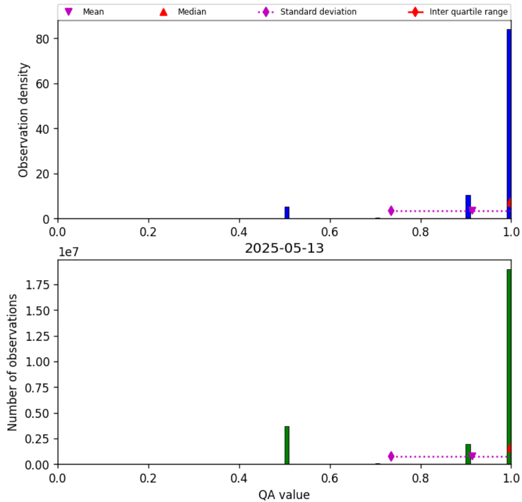
Figure 29: Histogram of “QA value” for 2025-05-12 to 2025-05-14
