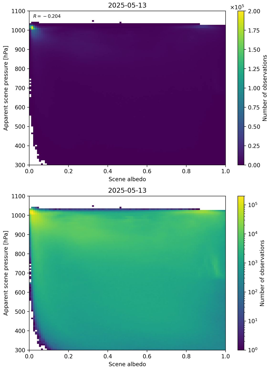
Figure 102: Scatter density plot of “Scene albedo” against “Apparent scene pressure” for 2025-05-12 to 2025-05-14.
