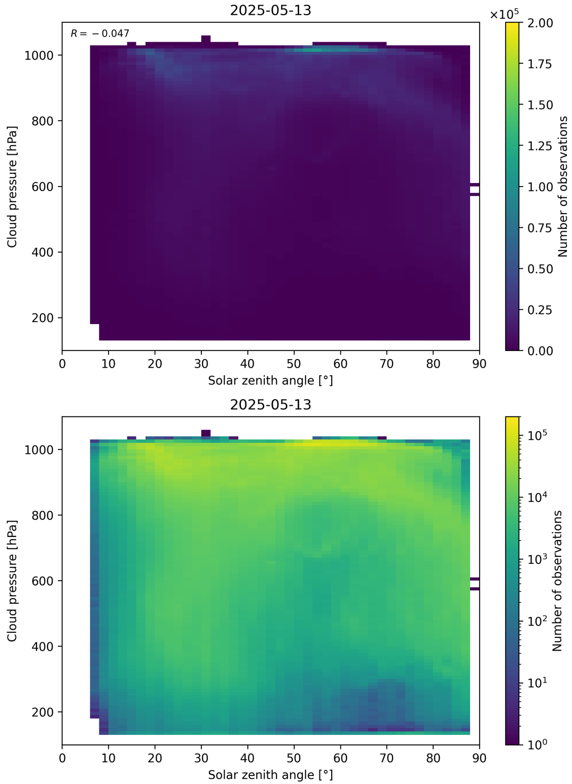
Figure 111: Scatter density plot of “Solar zenith angle” against “Cloud pressure” for 2025-05-12 to 2025-05-14.
