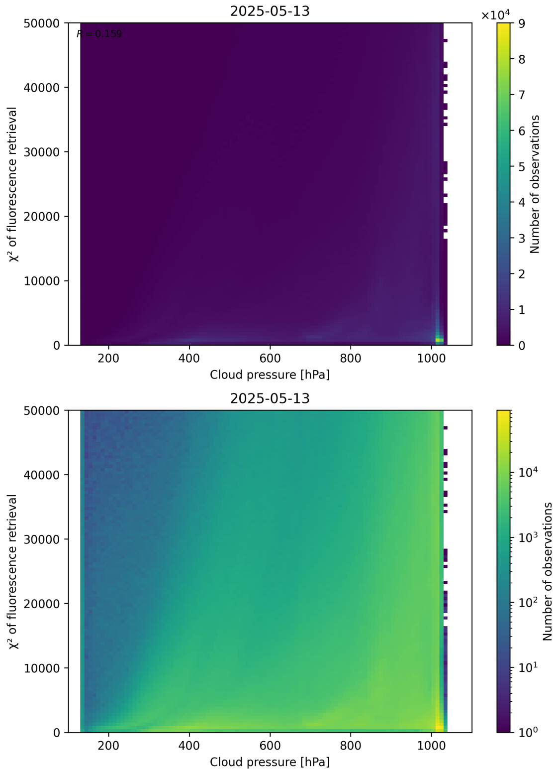
Figure 78: Scatter density plot of “Cloud pressure” against “ \chi^2 of fluorescence retrieval” for 2025-05-12 to 2025-05-14.
