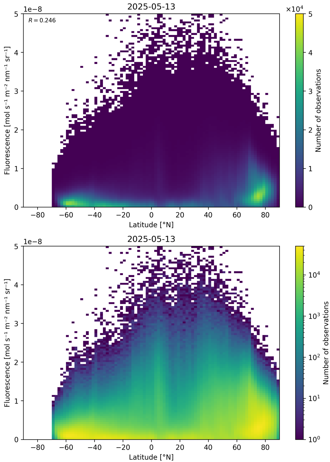
Figure 92: Scatter density plot of “Latitude” against “Fluorescence” for 2025-05-12 to 2025-05-14.
