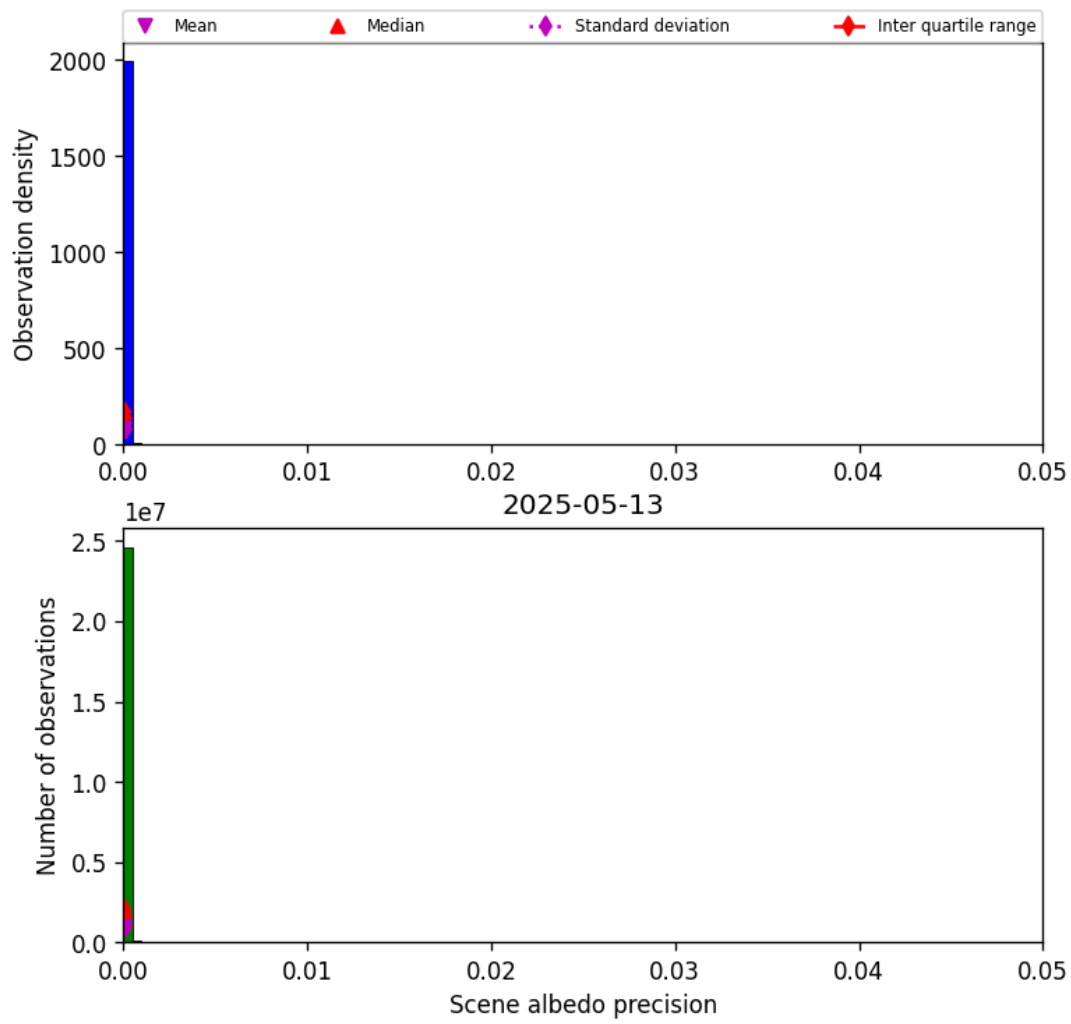
Figure 35: Histogram of “Scene albedo precision” for 2025-05-12 to 2025-05-14
