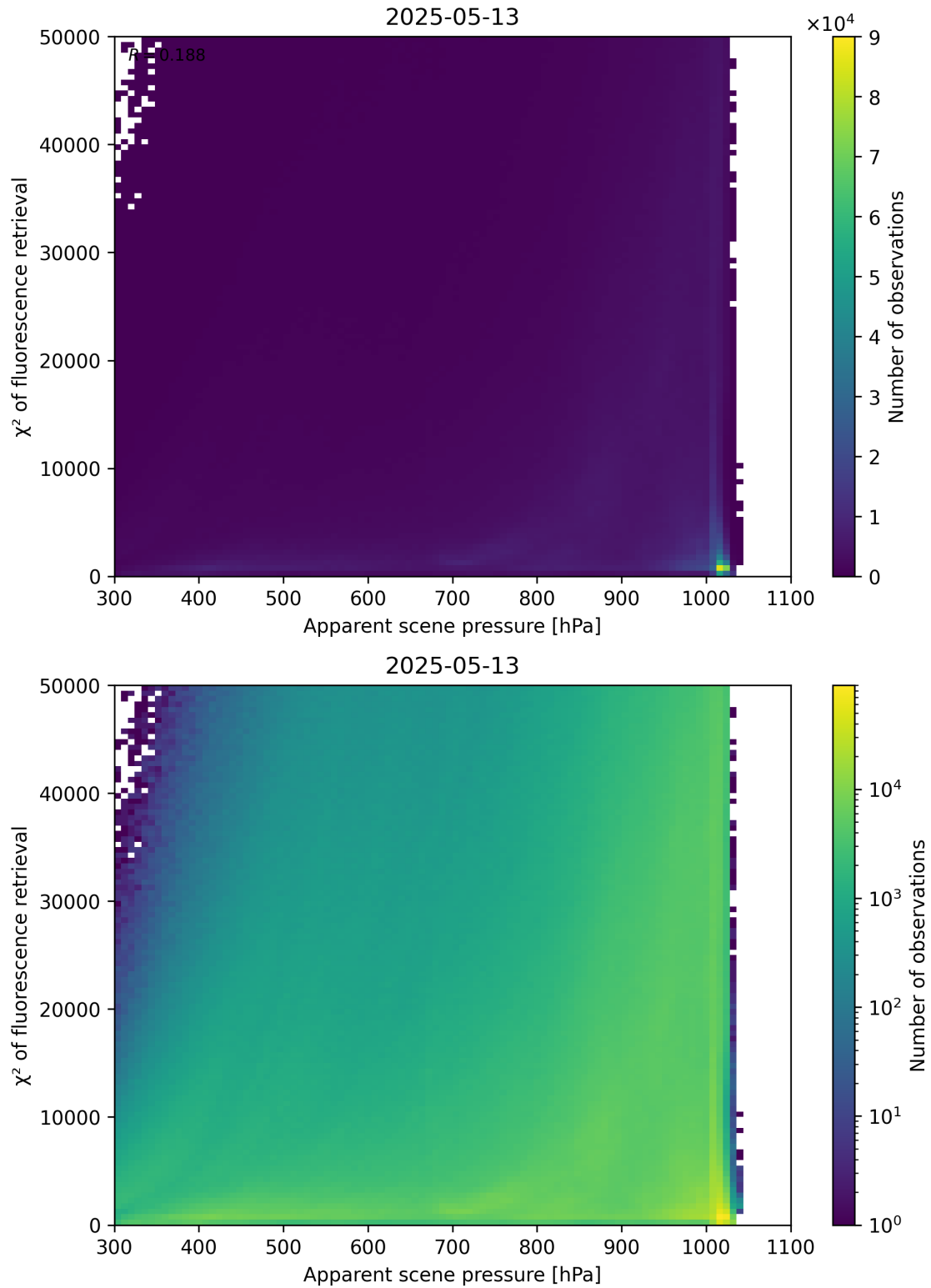
Figure 63: Scatter density plot of “Apparent scene pressure” against “ \chi^2 of fluorescence retrieval” for 2025-05-12 to 2025-05-14.
