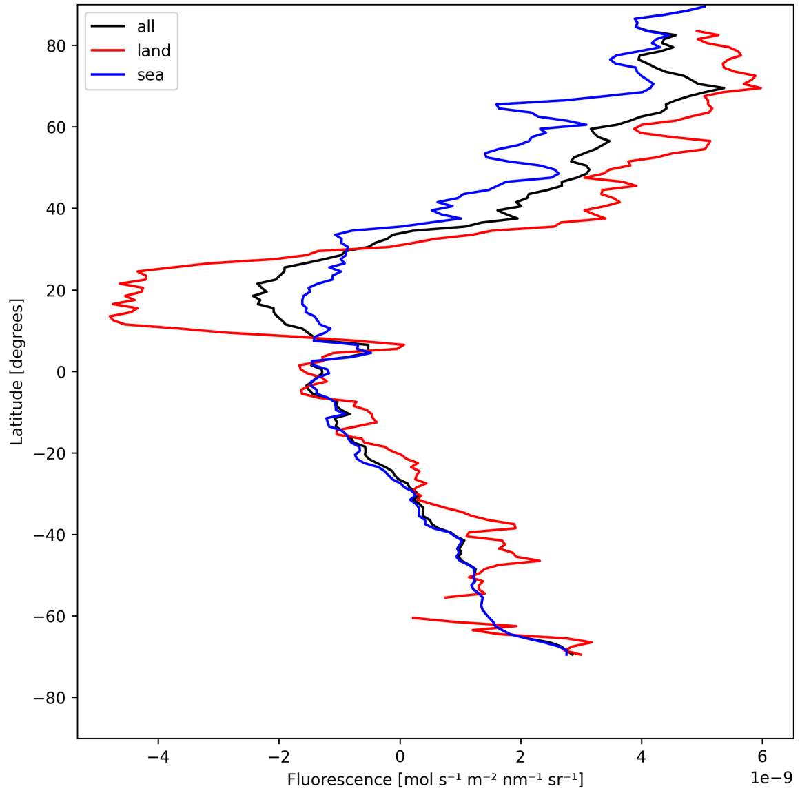
Figure 23: Zonal average of “Fluorescence” for 2025-05-12 to 2025-05-14.
