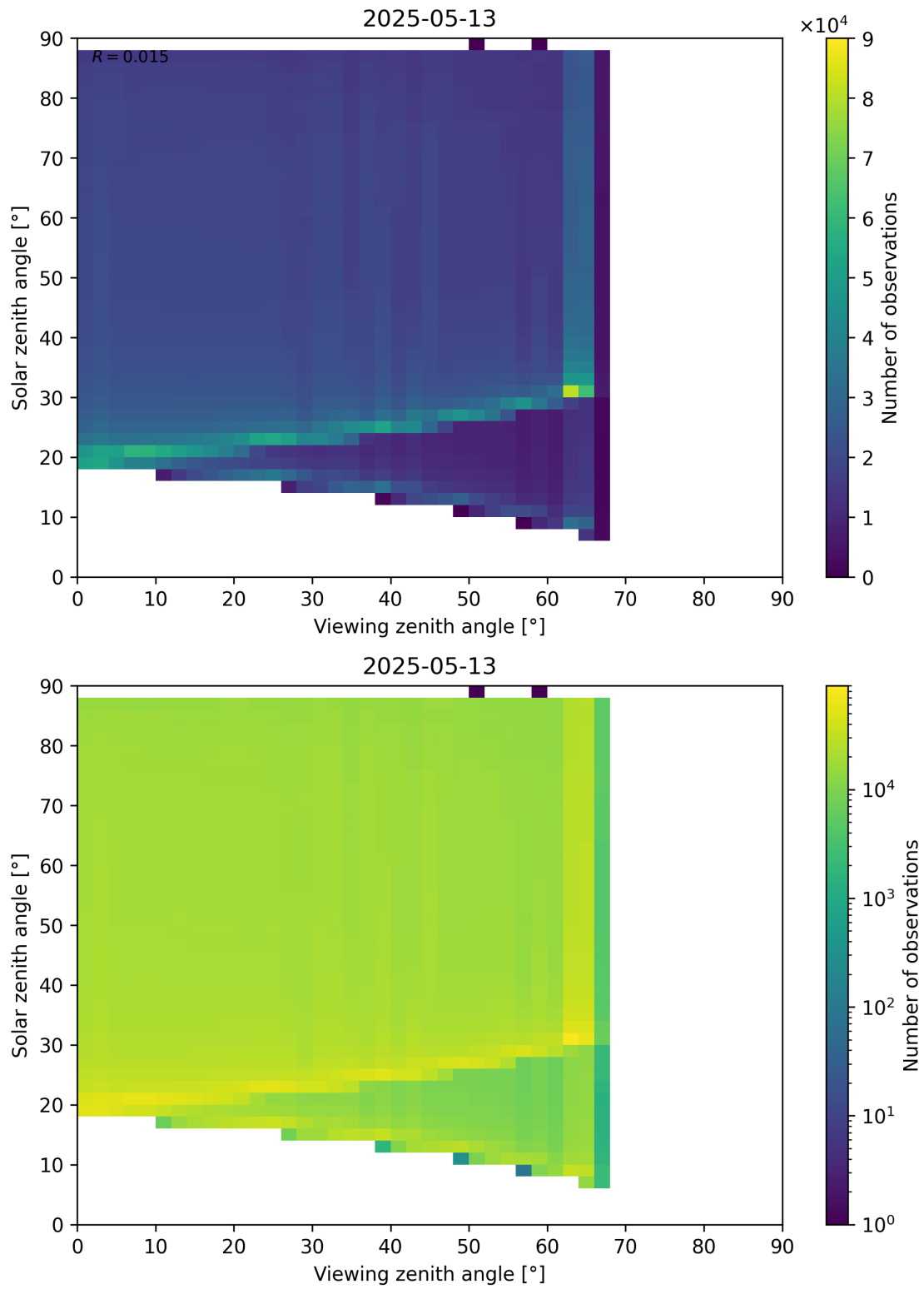
Figure 127: Scatter density plot of “Viewing zenith angle” against “Solar zenith angle” for 2025-05-12 to 2025-05-14.
