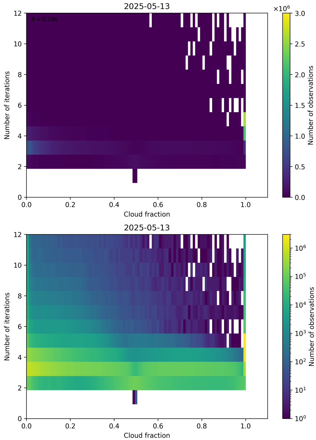
Figure 73: Scatter density plot of “Cloud fraction” against “Number of iterations” for 2025-05-12 to 2025-05-14.
