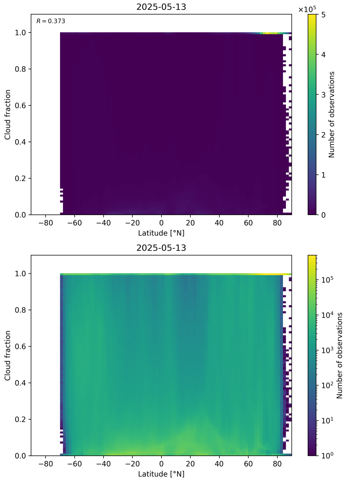
Figure 90: Scatter density plot of “Latitude” against “Cloud fraction” for 2025-05-12 to 2025-05-14.
