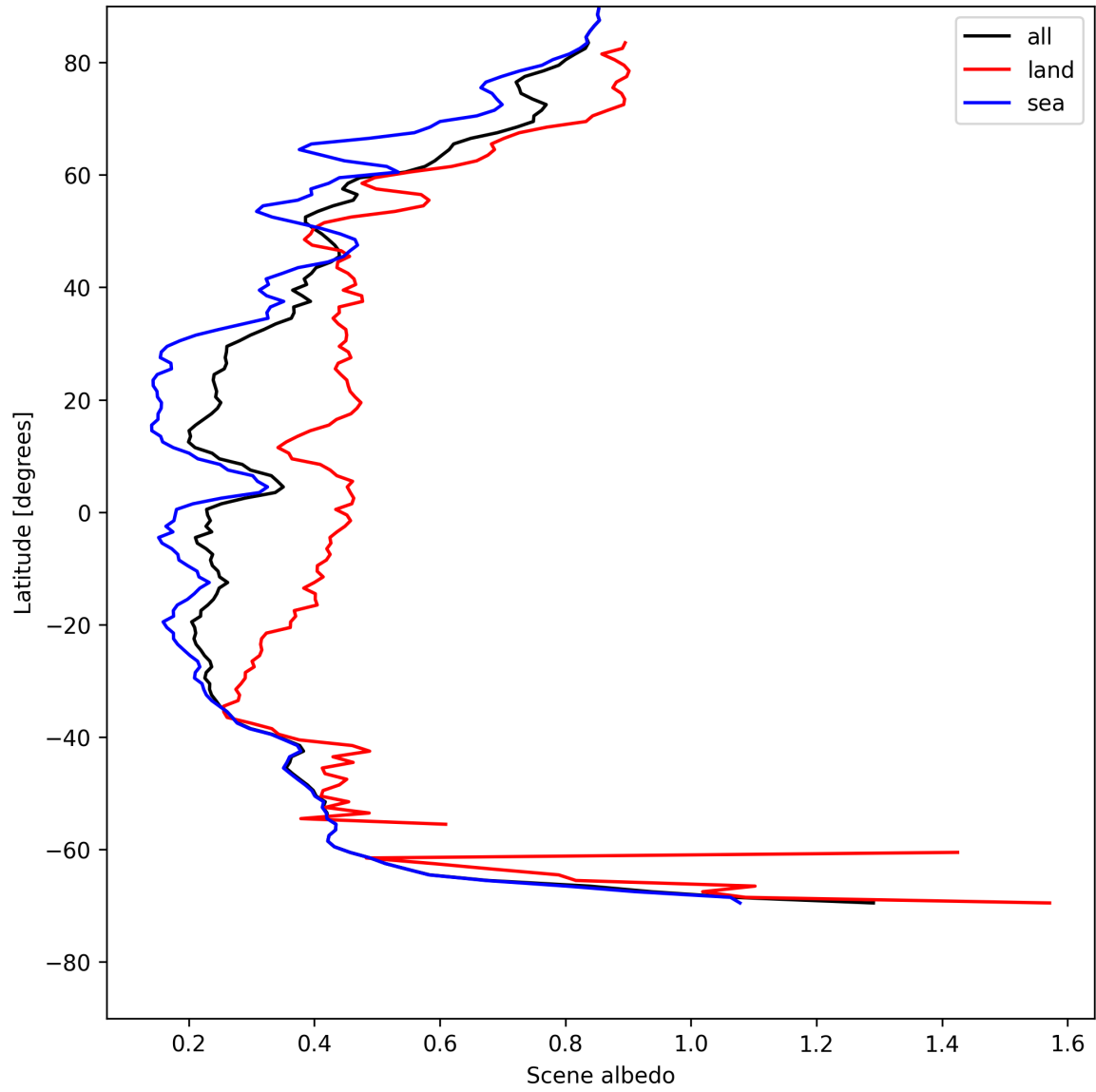
Figure 17: Zonal average of “Scene albedo” for 2025-05-12 to 2025-05-14.
