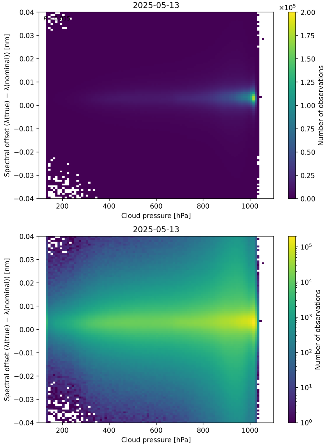
Figure 84: Scatter density plot of “Cloud pressure” against “Spectral offset ( \lambda_{\text{true}} - \lambda_{\text{nominal}} )” for 2025-05-12 to 2025-05-14.
