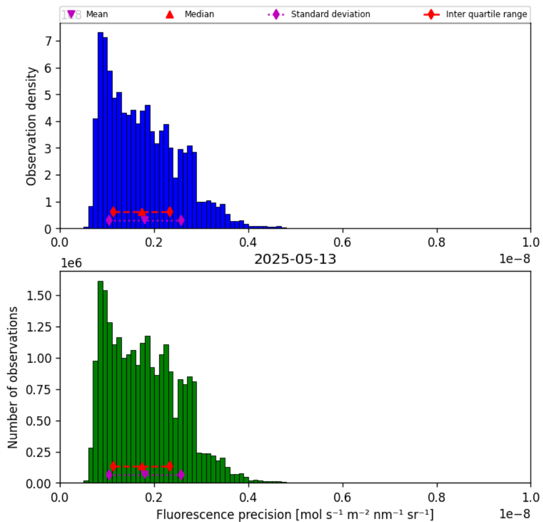
Figure 41: Histogram of “Fluorescence precision” for 2025-05-12 to 2025-05-14
