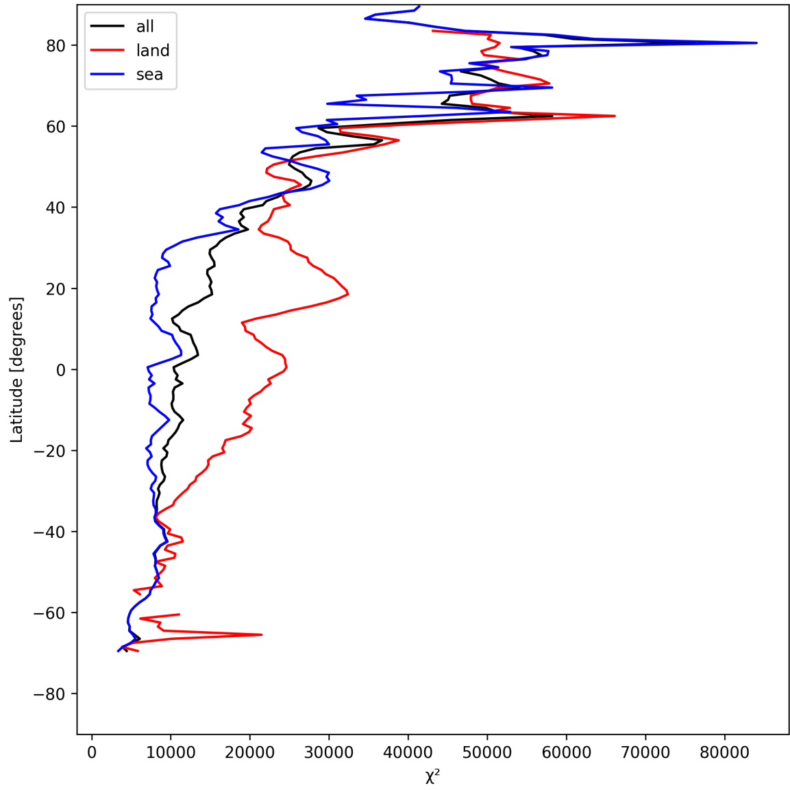
Figure 21: Zonal average of “ \chi^2 ” for 2025-05-12 to 2025-05-14.
