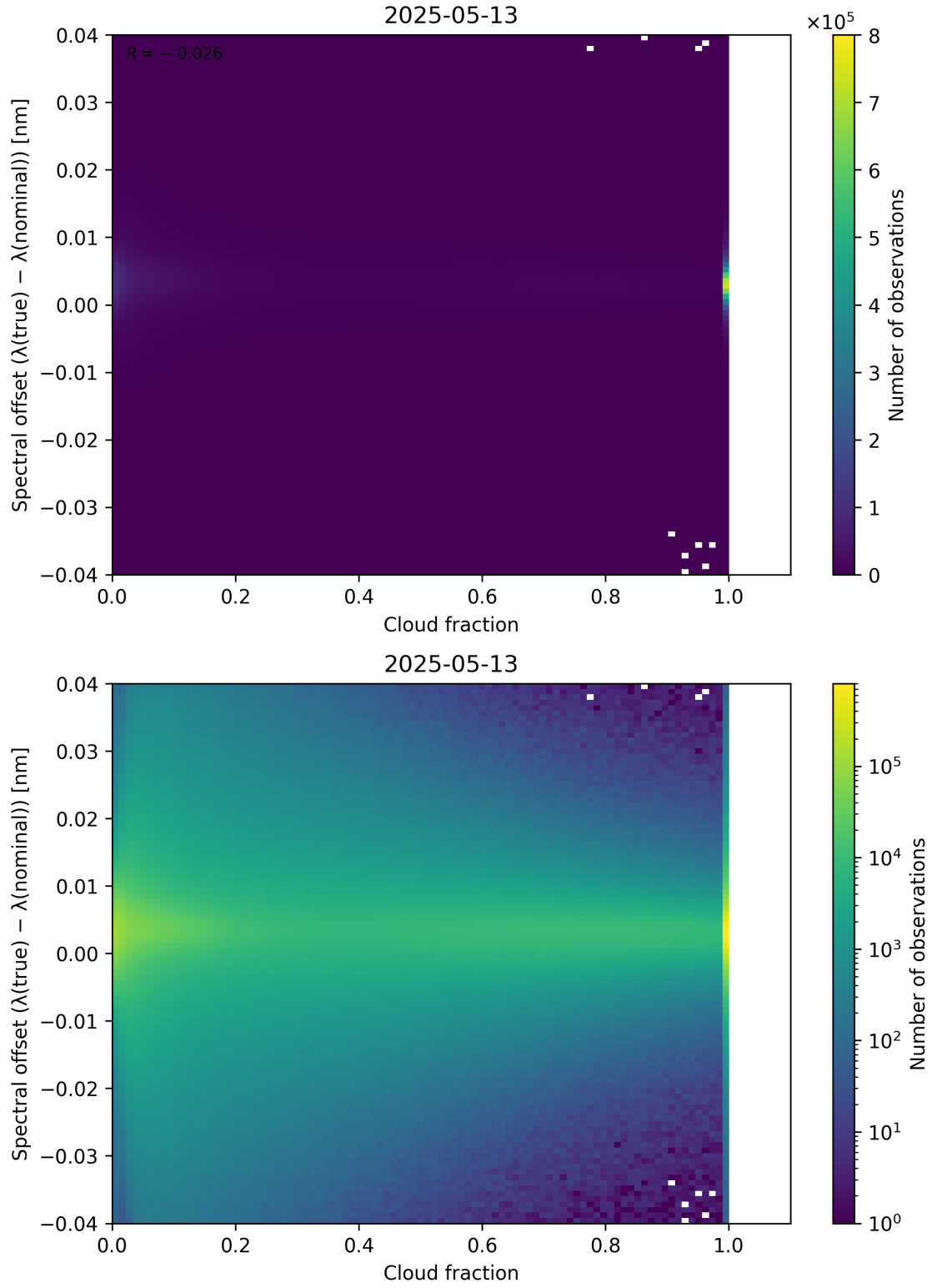
Figure 76: Scatter density plot of “Cloud fraction” against “Spectral offset ( \lambda_{\text{true}} - \lambda_{\text{nominal}} )” for 2025-05-12 to 2025-05-14.
