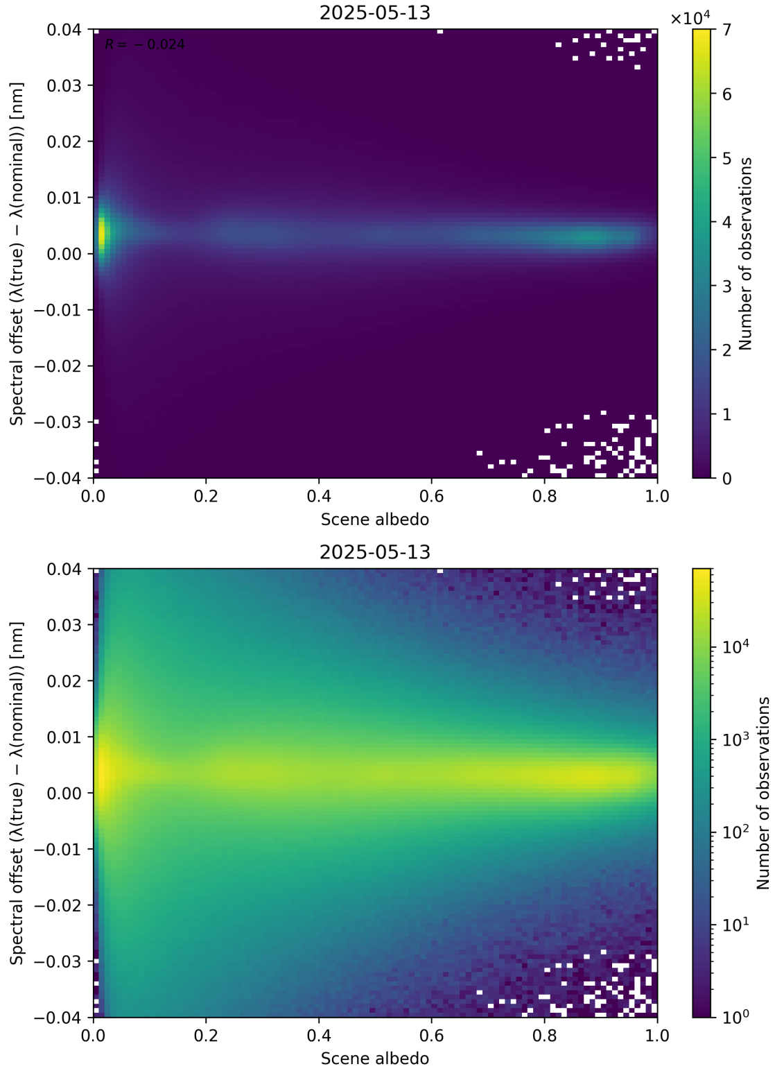
Figure 107: Scatter density plot of “Scene albedo” against “Spectral offset ( \lambda_{\text{true}} - \lambda_{\text{nominal}} )” for 2025-05-12 to 2025-05-14.
