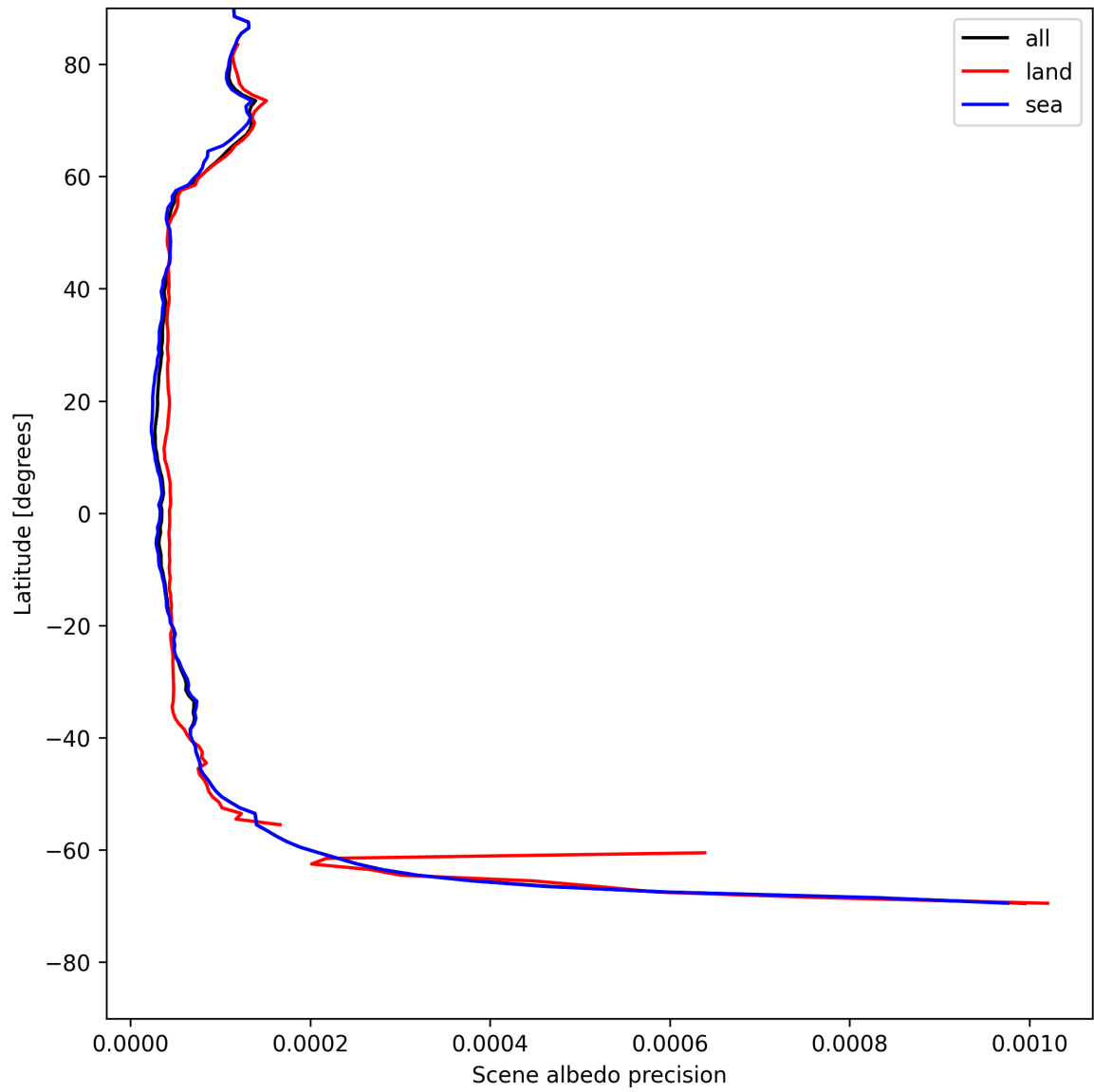
Figure 18: Zonal average of “Scene albedo precision” for 2025-05-12 to 2025-05-14.
