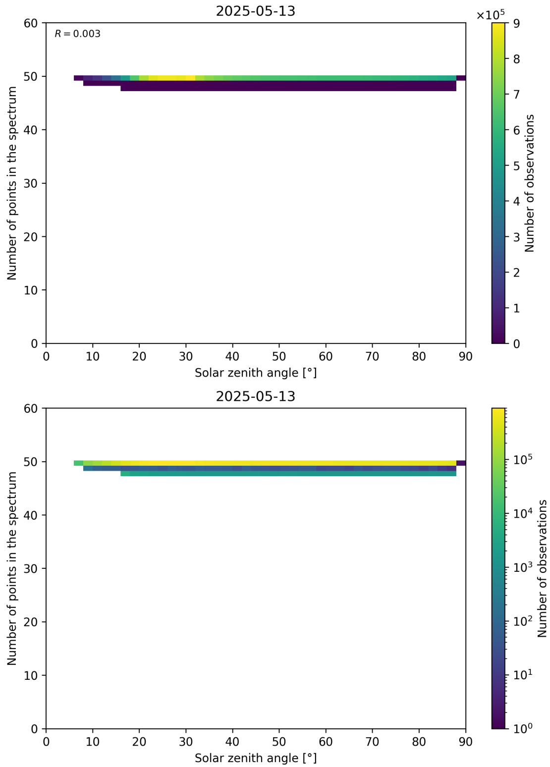
Figure 115: Scatter density plot of “Solar zenith angle” against “Number of points in the spectrum” for 2025-05-12 to 2025-05-14.
