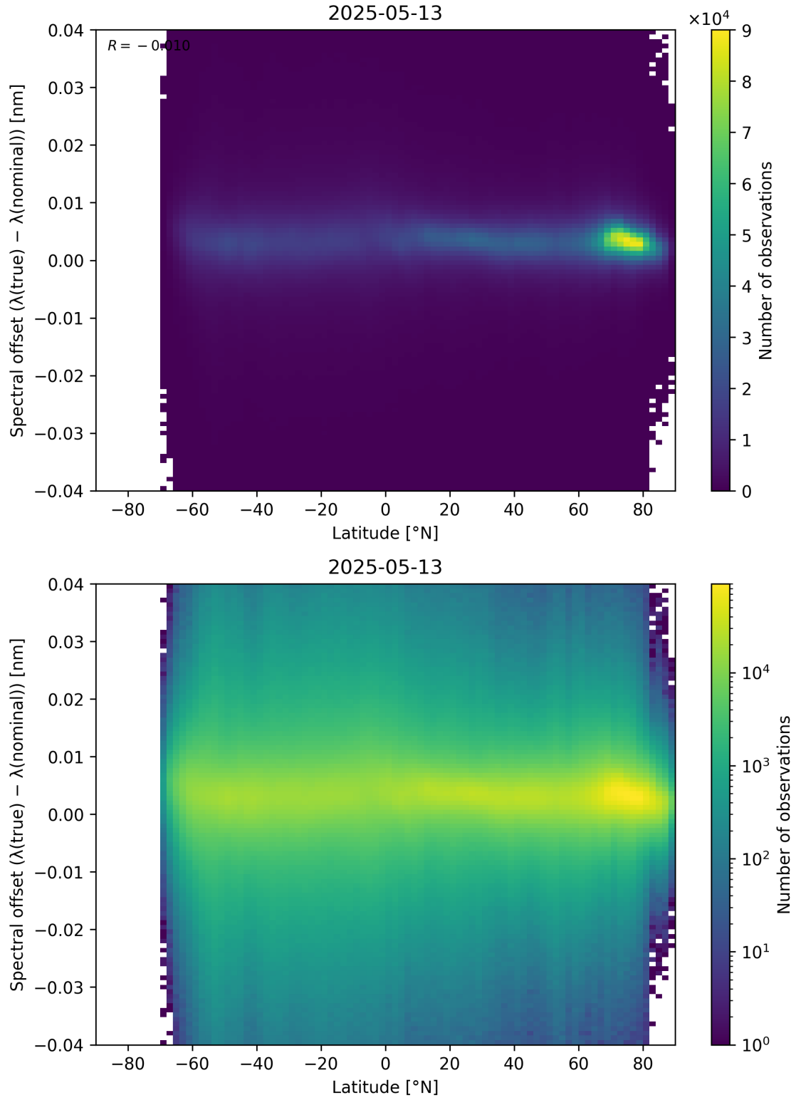
Figure 96: Scatter density plot of “Latitude” against “Spectral offset ( \lambda_{\text{true}} - \lambda_{\text{nominal}} )” for 2025-05-12 to 2025-05-14.
