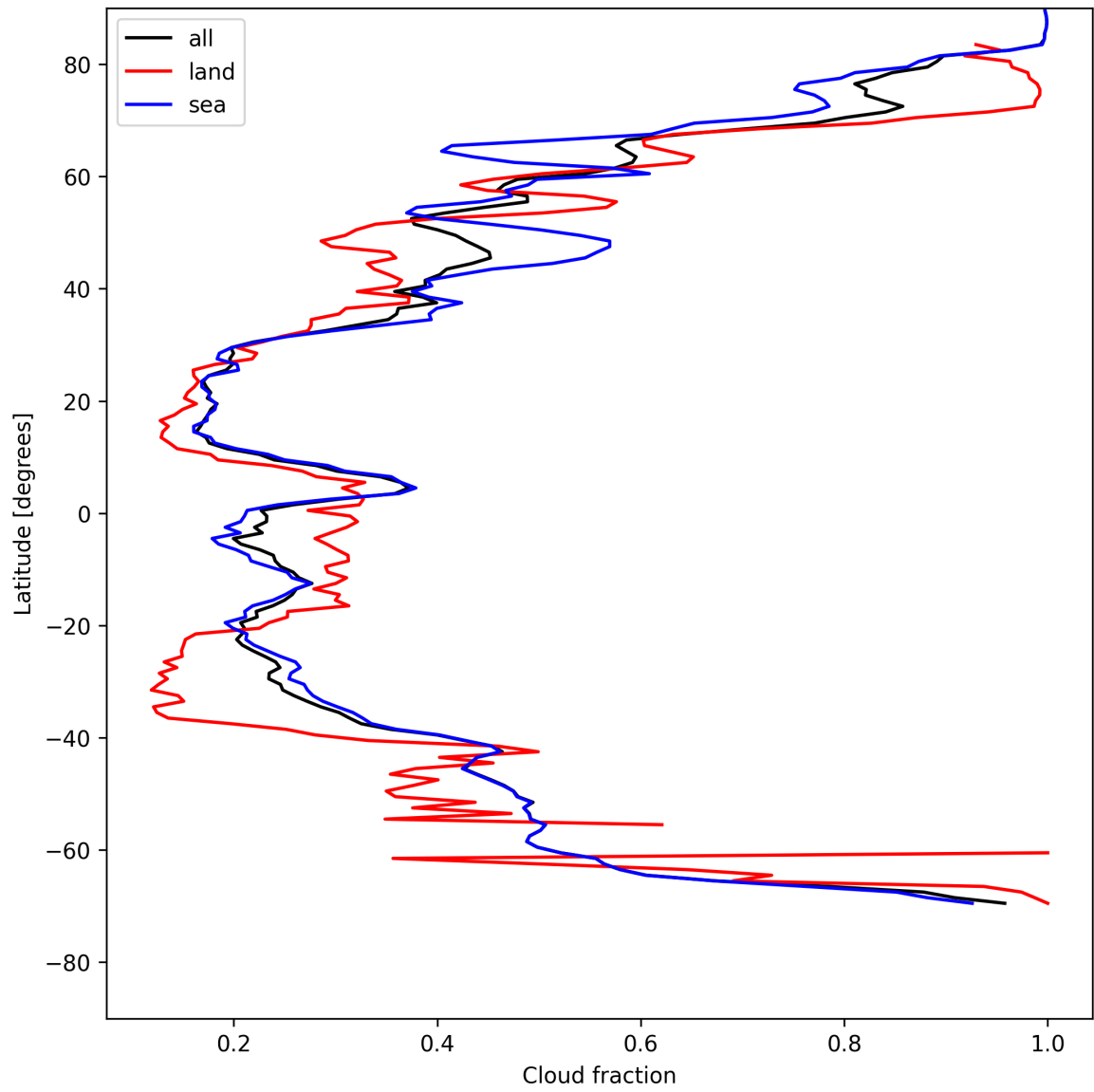
Figure 15: Zonal average of “Cloud fraction” for 2025-05-12 to 2025-05-14.
