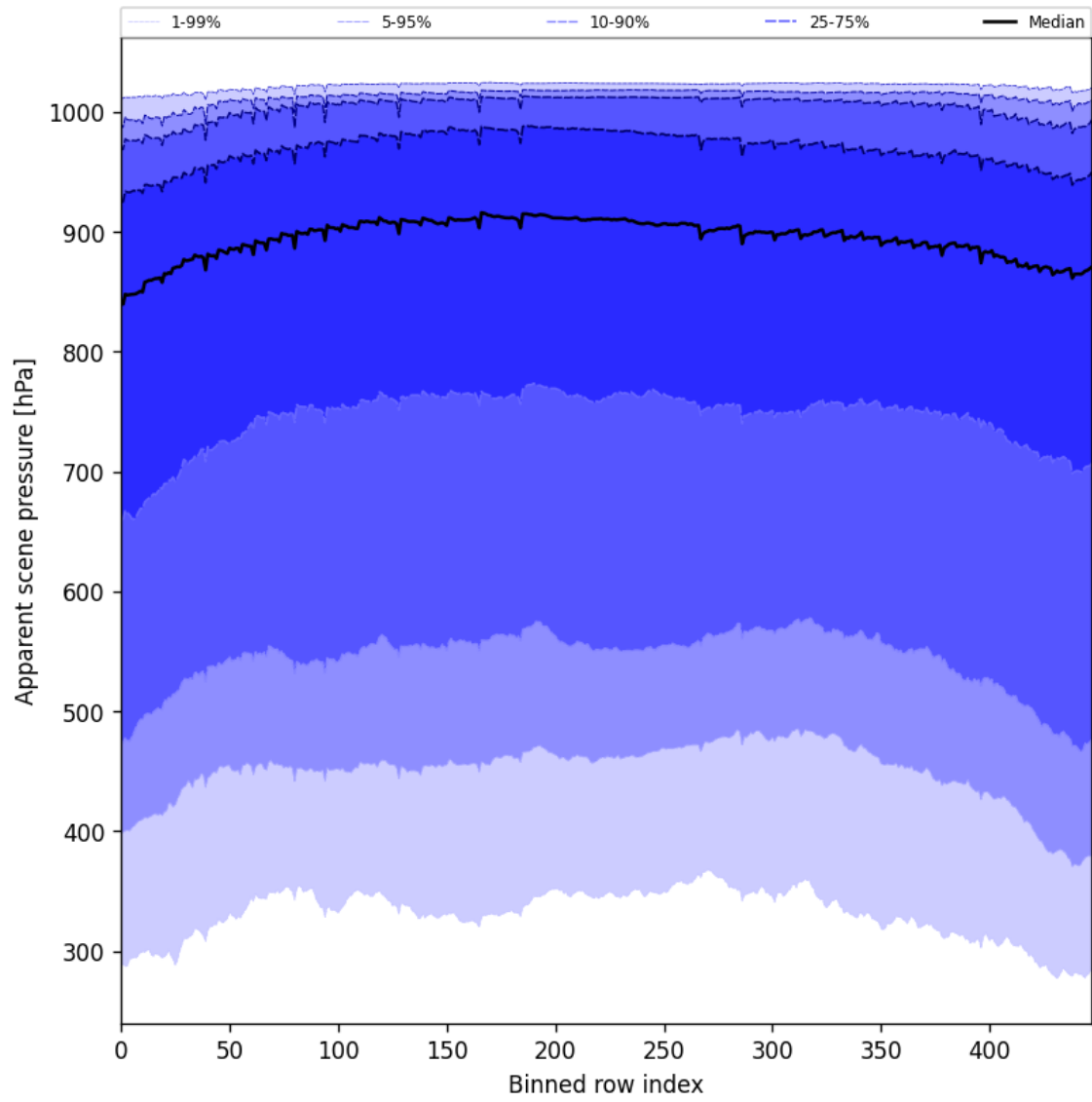
Figure 53: Along track statistics of “Apparent scene pressure” for 2025-05-12 to 2025-05-14
