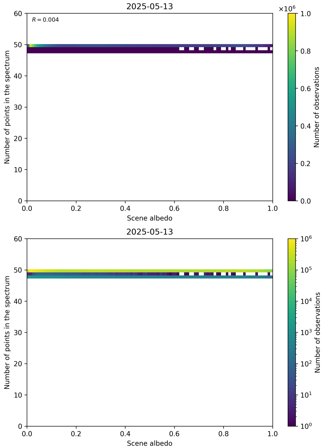
Figure 106: Scatter density plot of “Scene albedo” against “Number of points in the spectrum” for 2025-05-12 to 2025-05-14.
