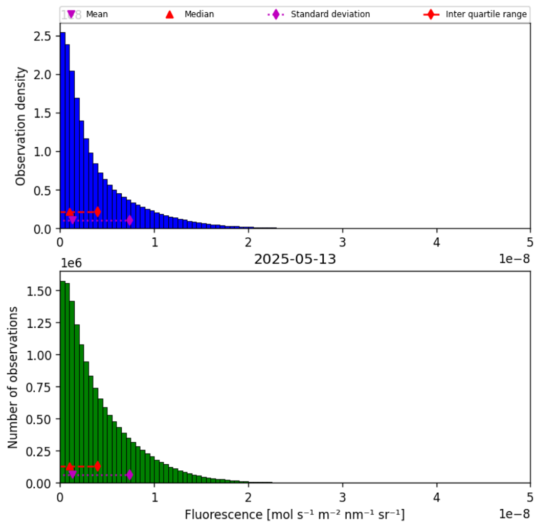
Figure 40: Histogram of “Fluorescence” for 2025-05-12 to 2025-05-14
