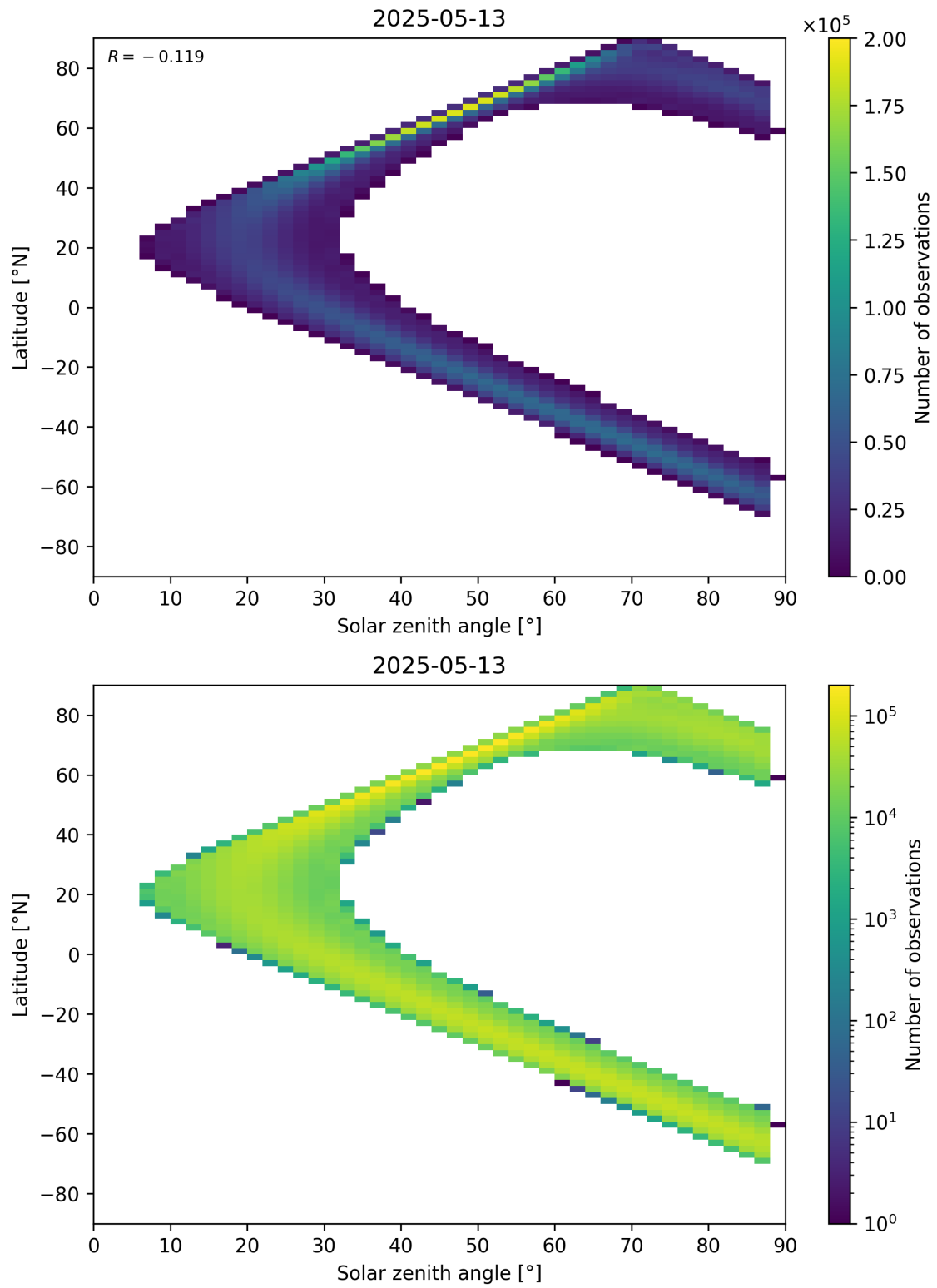
Figure 113: Scatter density plot of “Solar zenith angle” against “Latitude” for 2025-05-12 to 2025-05-14.
