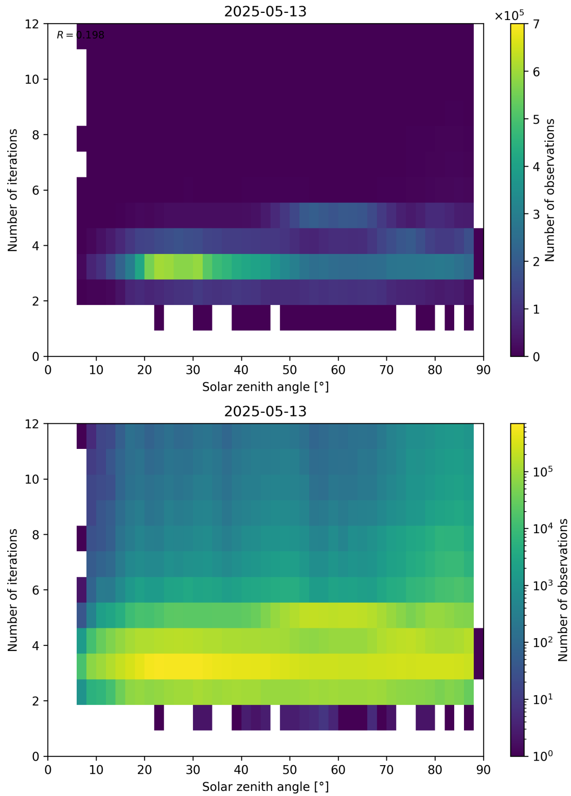
Figure 114: Scatter density plot of “Solar zenith angle” against “Number of iterations” for 2025-05-12 to 2025-05-14.
