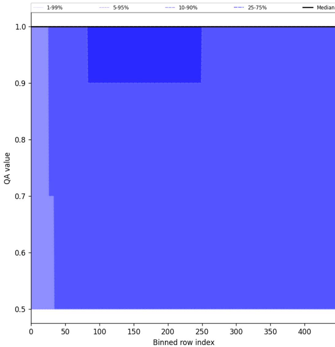
Figure 46: Along track statistics of “QA value” for 2025-05-12 to 2025-05-14
