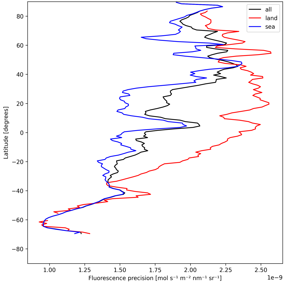
Figure 24: Zonal average of “Fluorescence precision” for 2025-05-12 to 2025-05-14.
