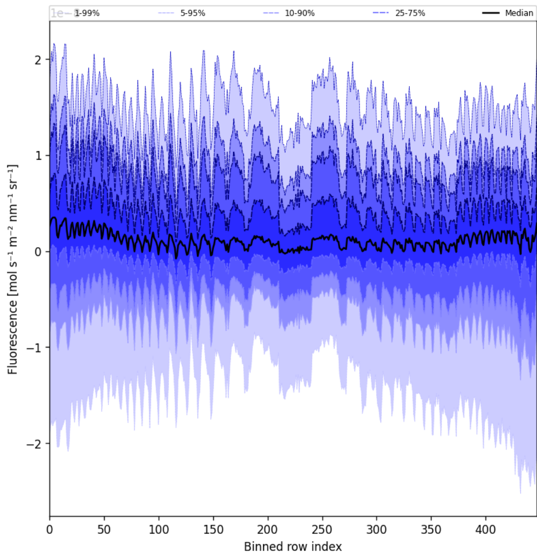
Figure 57: Along track statistics of “Fluorescence” for 2025-05-12 to 2025-05-14
