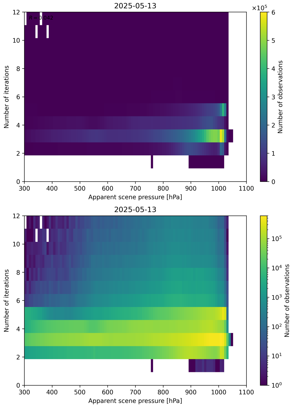
Figure 65: Scatter density plot of “Apparent scene pressure” against “Number of iterations” for 2025-05-12 to 2025-05-14.
