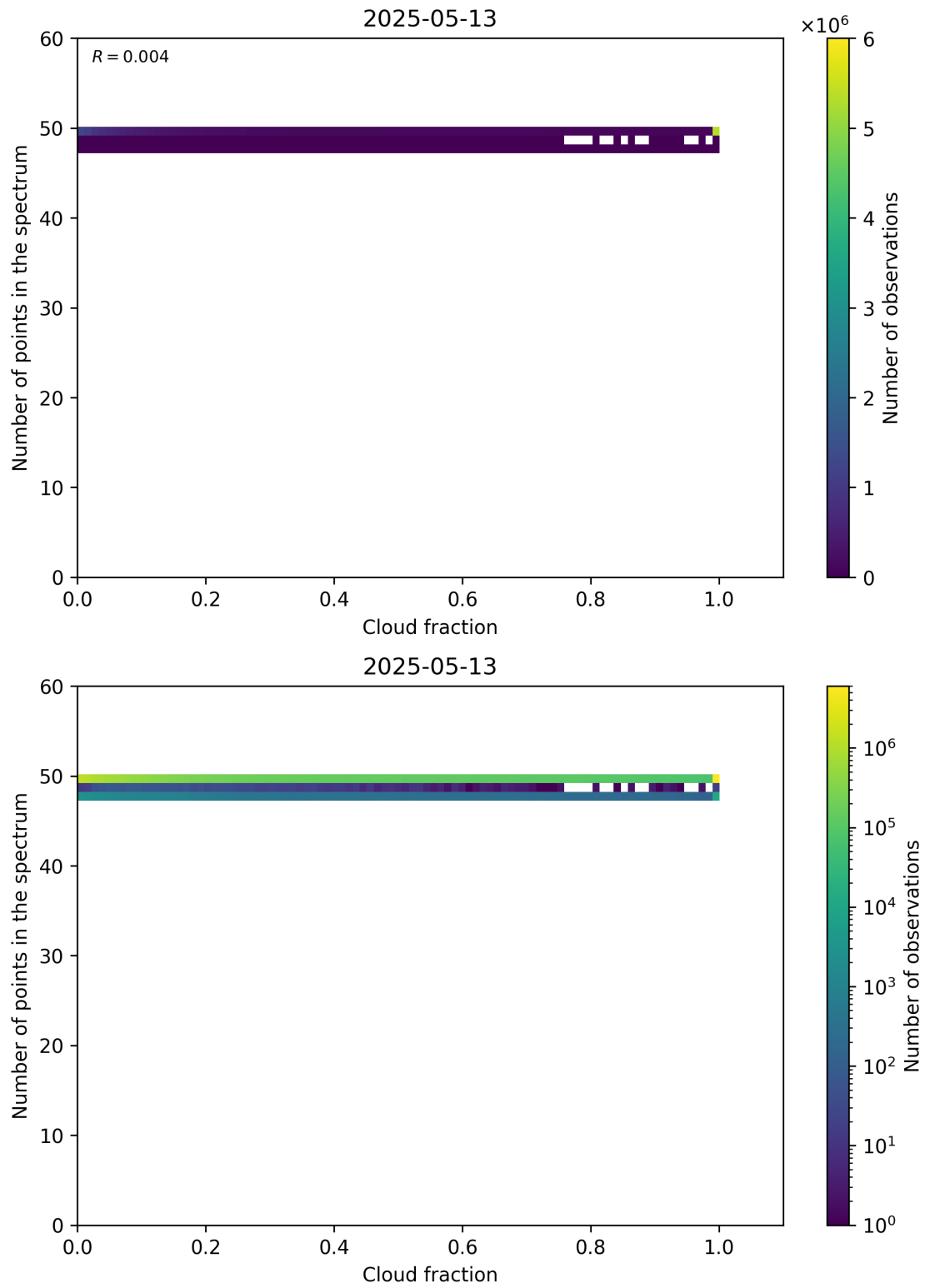
Figure 74: Scatter density plot of “Cloud fraction” against “Number of points in the spectrum” for 2025-05-12 to 2025-05-14.
