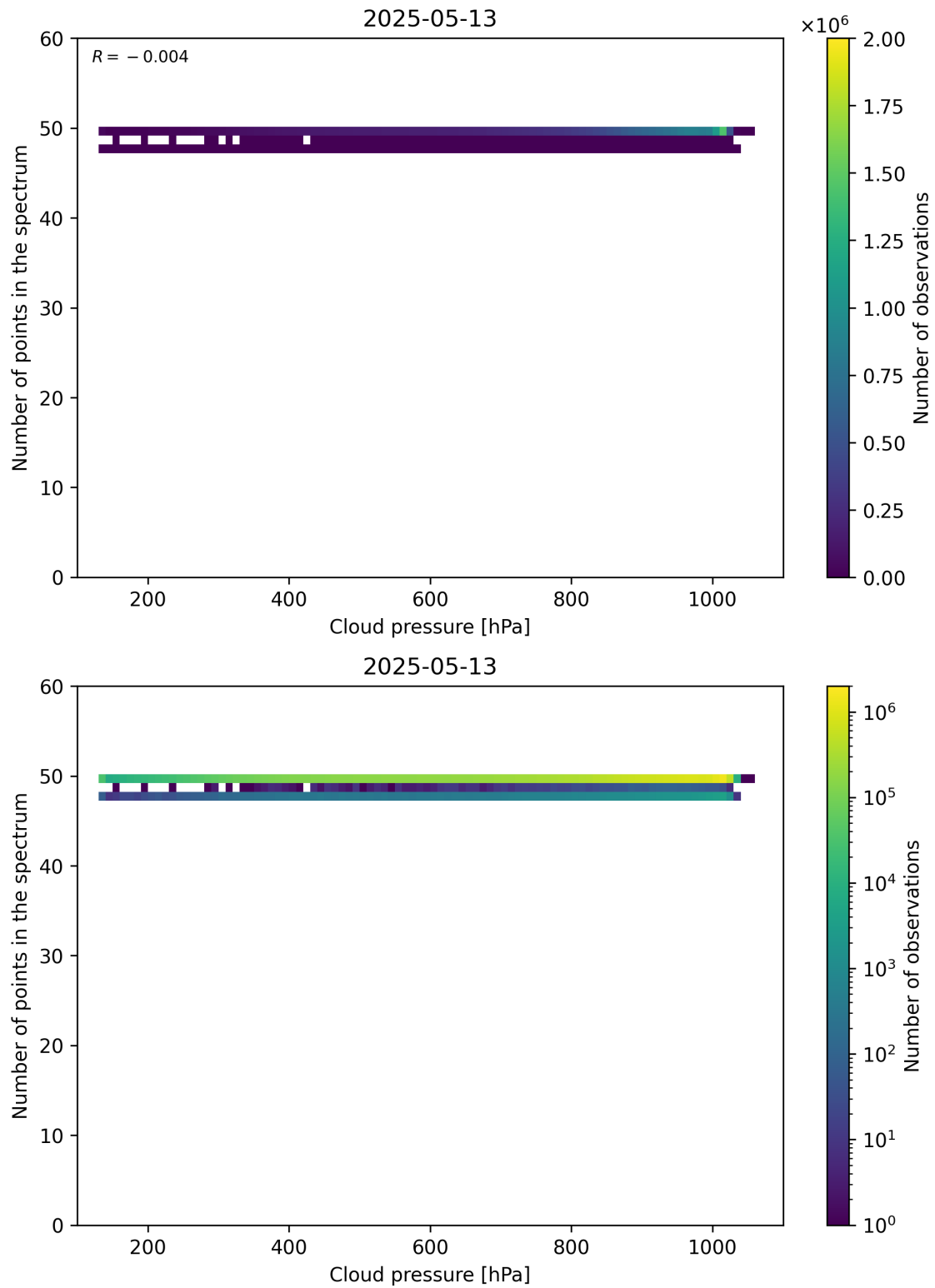
Figure 82: Scatter density plot of “Cloud pressure” against “Number of points in the spectrum” for 2025-05-12 to 2025-05-14.
