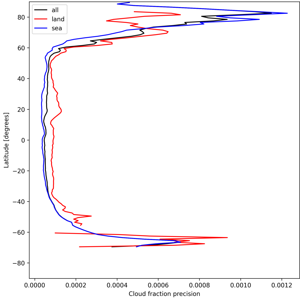
Figure 16: Zonal average of “Cloud fraction precision” for 2025-05-12 to 2025-05-14.
