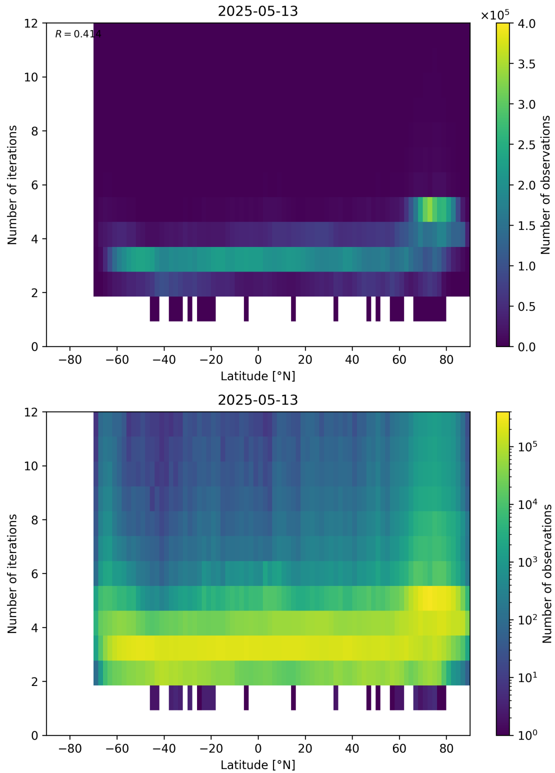
Figure 93: Scatter density plot of “Latitude” against “Number of iterations” for 2025-05-12 to 2025-05-14.
