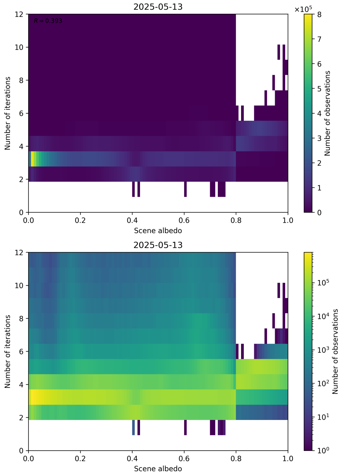
Figure 105: Scatter density plot of “Scene albedo” against “Number of iterations” for 2025-05-12 to 2025-05-14.
