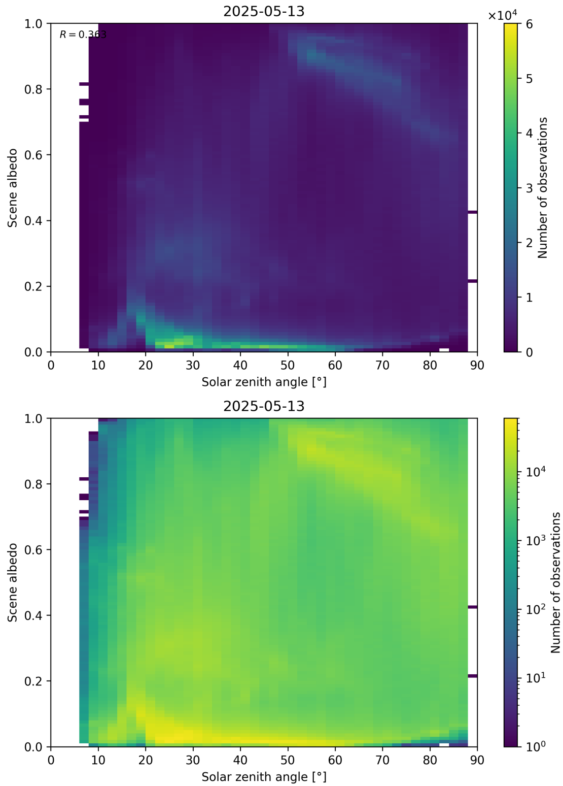
Figure 116: Scatter density plot of “Solar zenith angle” against “Scene albedo” for 2025-05-12 to 2025-05-14.
