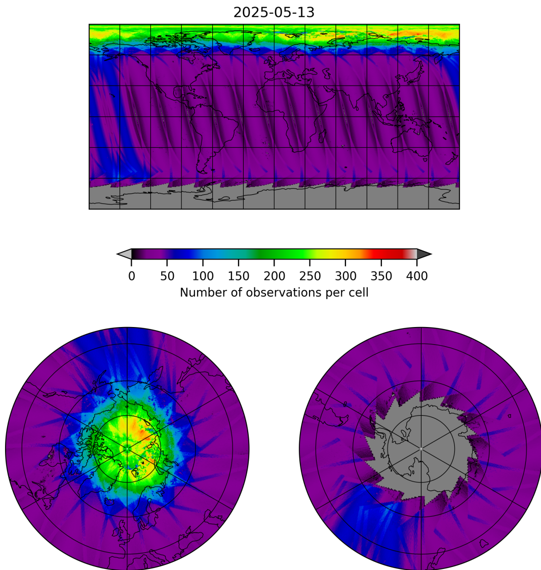
Figure 11: Map of the number of observations for 2025-05-12 to 2025-05-14
