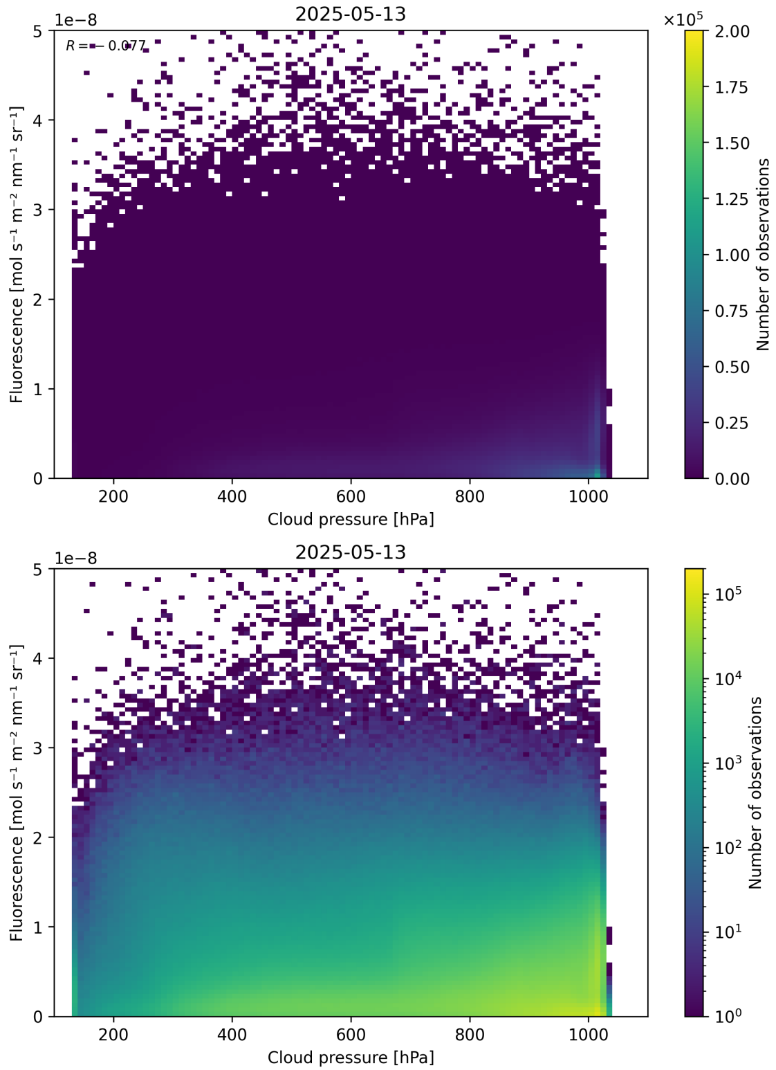
Figure 80: Scatter density plot of “Cloud pressure” against “Fluorescence” for 2025-05-12 to 2025-05-14.
