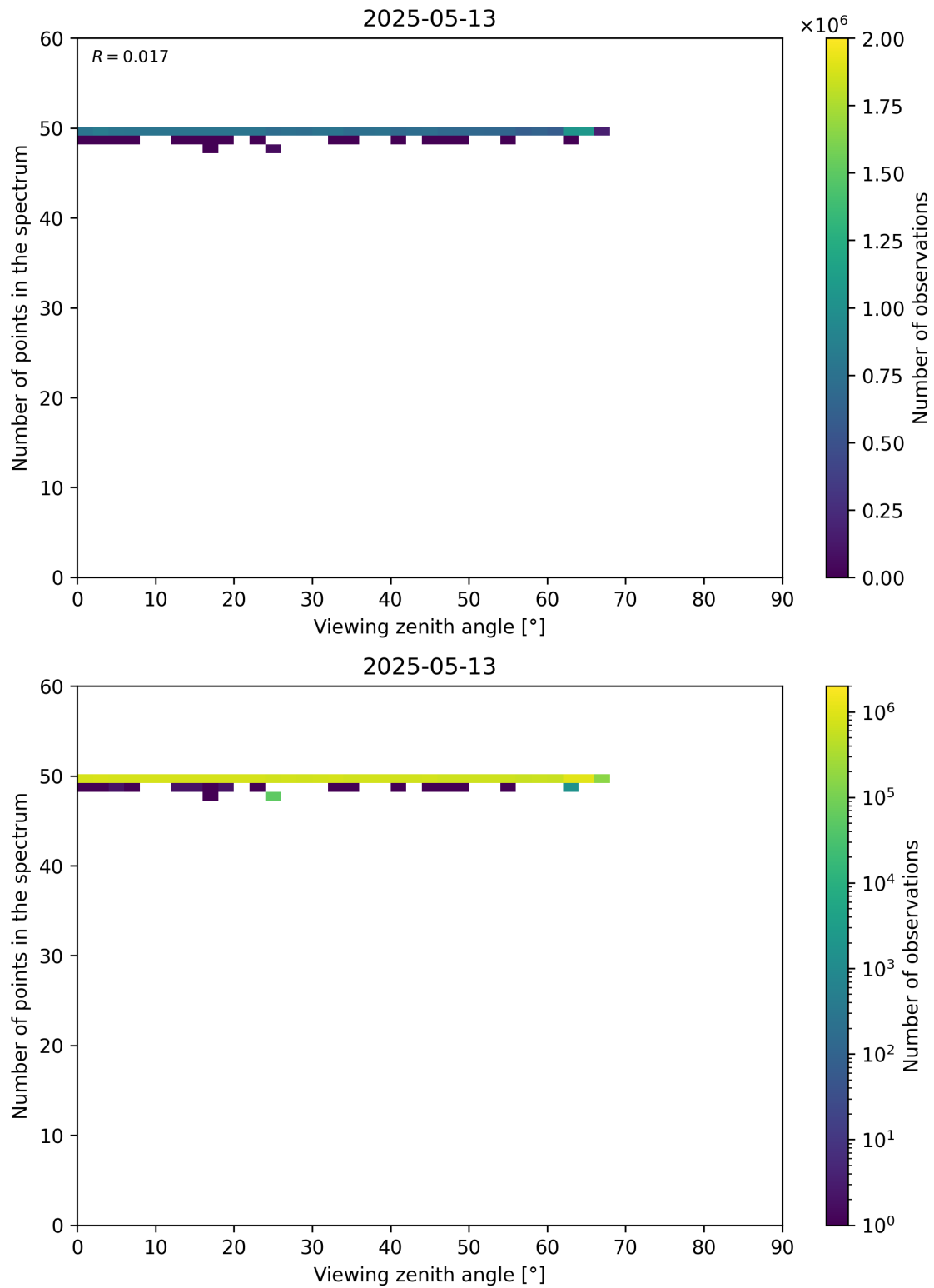
Figure 125: Scatter density plot of “Viewing zenith angle” against “Number of points in the spectrum” for 2025-05-12 to 2025-05-14.
